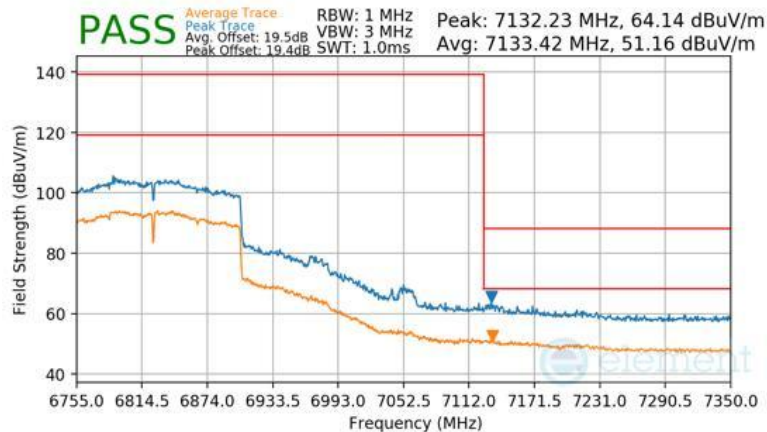
Plot 7-388 Antenna 3b Radiated Upper Band Edge (Peak & Average – UNII Band 7)
