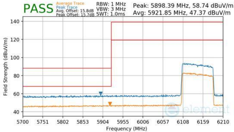
Plot 7-384 Antenna 3b Radiated Lower Band Edge (Peak & Average – UNII Band 5)
