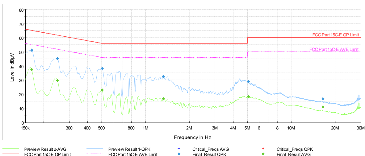
Plot 7-440. AC Line Conducted Plot with 802.11be SDM Primary – Ch.61 (L1), with AC/DC Adapter
