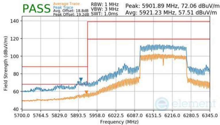
Plot 7-419 SDM Primary Radiated Lower Band Edge (Peak & Average – UNII Band 5)
