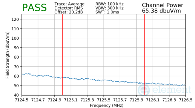
Plot 7-377 Antenna 3b Radiated Integrated Band Edge (Average – UNII Band 8)
