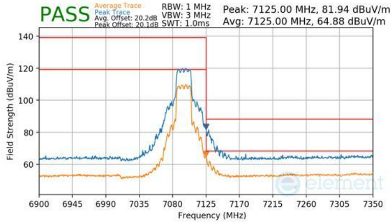
Plot 7-427 SDM Diversity Radiated Upper Band Edge (Peak & Average – UNII Band 8)
