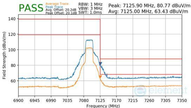
Plot 7-395 Antenna 1b Radiated Upper Band Edge (Peak & Average – UNII Band 8)
