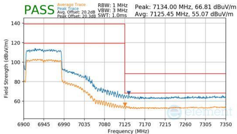
Plot 7-433 SDM Diversity Radiated Upper Band Edge (Peak & Average – UNII Band 8)
