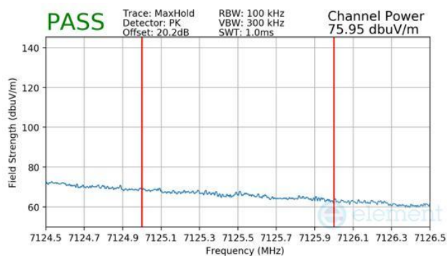
Plot 7-392 Antenna 1b Radiated Integrated Band Edge (Peak – UNII Band 8)
