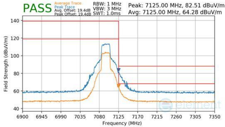
Plot 7-379 Antenna 3b Radiated Upper Band Edge (Peak & Average – UNII Band 8)
