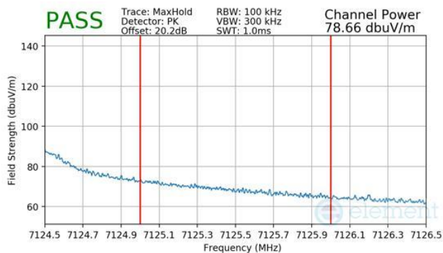
Plot 7-396 Antenna 1b Radiated Integrated Band Edge (Peak – UNII Band 8)
