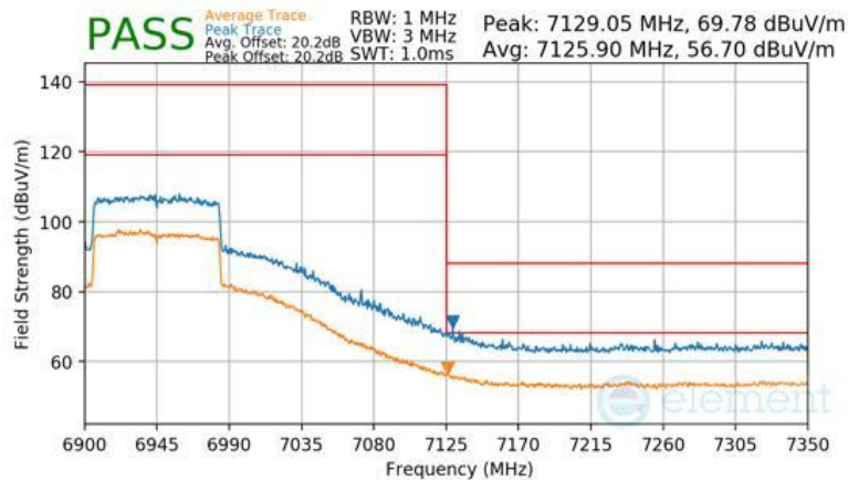
Plot 7-401 Antenna 1b Radiated Upper Band Edge (Peak & Average – UNII Band 8)
