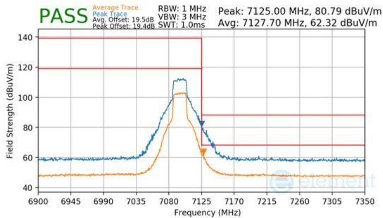
Plot 7-375 Antenna 3b Radiated Upper Band Edge (Peak & Average – UNII Band 8)
