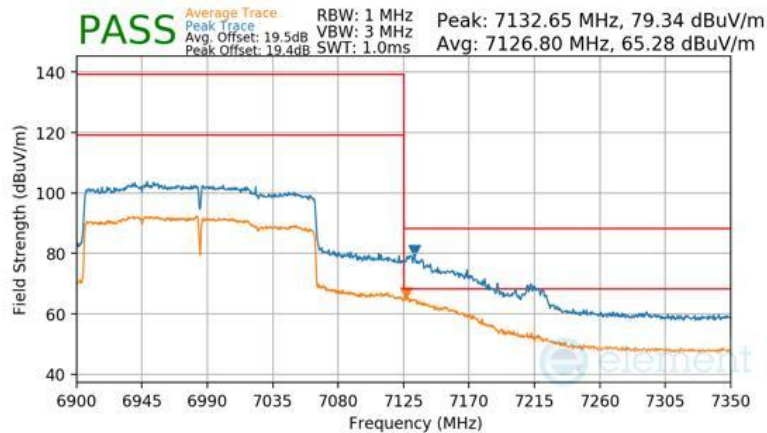
Plot 7-389 Antenna 3b Radiated Upper Band Edge (Peak & Average – UNII Band 8)
