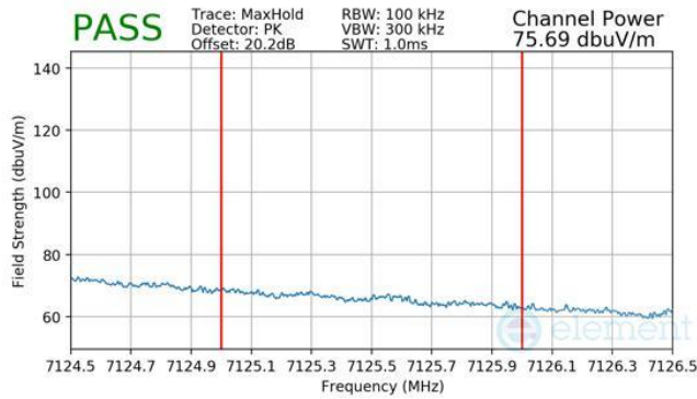
Plot 7-376 Antenna 3b Radiated Integrated Band Edge (Peak – UNII Band 8)
