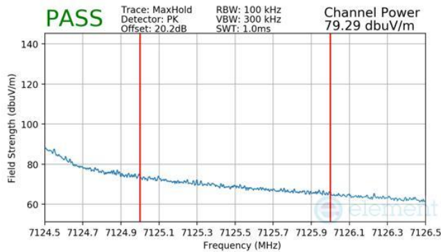
Plot 7-428 SDM Diversity Radiated Integrated Band Edge (Peak – UNII Band 8)
