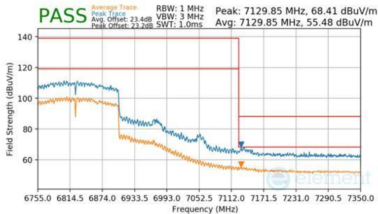
Plot 7-420 SDM Primary Radiated Upper Band Edge (Peak & Average – UNII Band 7)
