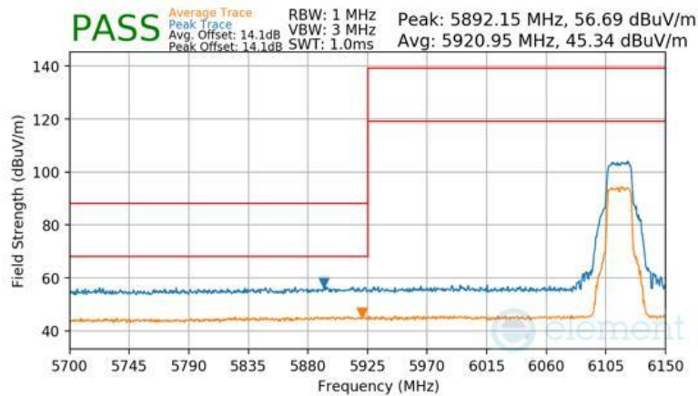
Plot 7-390 Antenna 1b Radiated Lower Band Edge (Peak & Average – UNII Band 5)
