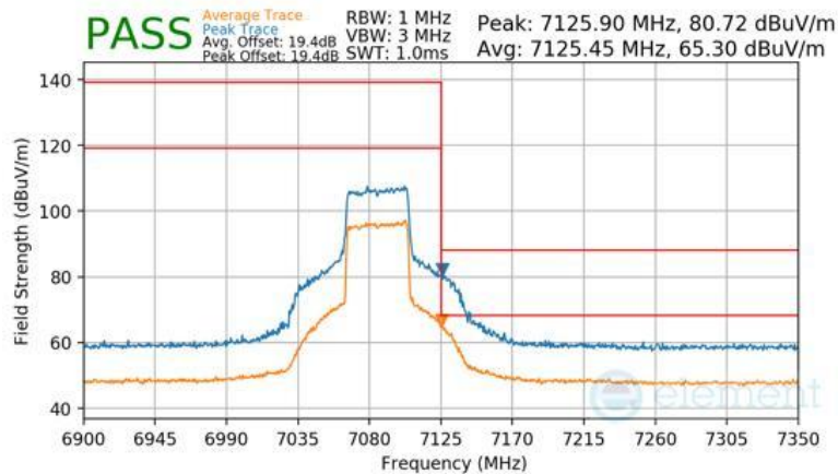
Plot 7-383 Antenna 3b Radiated Upper Band Edge (Peak & Average – UNII Band 8)
