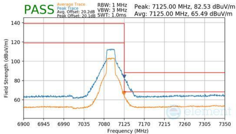
Plot 7-391 Antenna 1b Radiated Upper Band Edge (Peak & Average – UNII Band 8)
