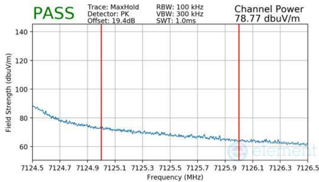
Plot 7-380 Antenna 3b Radiated Integrated Band Edge (Peak – UNII Band 8)
