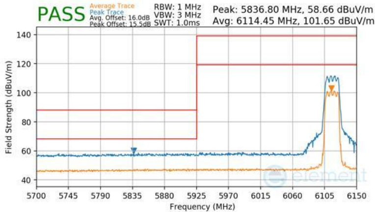
Plot 7-426 SDM Diversity Radiated Lower Band Edge (Peak & Average – UNII Band 5)
