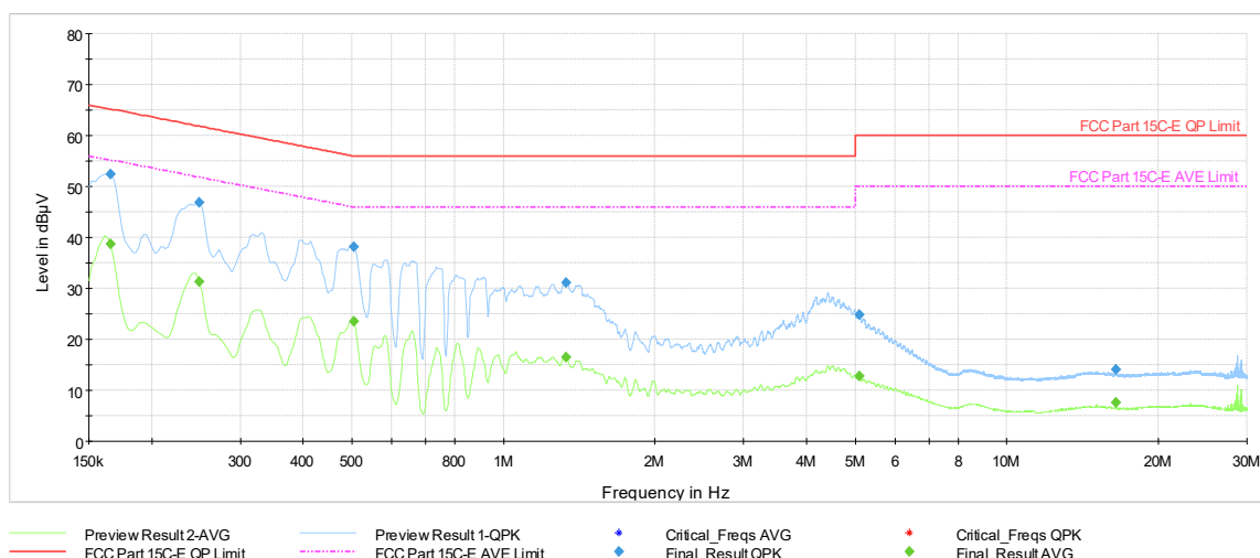
Plot 7-443. AC Line Conducted Plot with 802.11be SDM Diversity – Ch. 61 (N), with AC/DC Adapter
