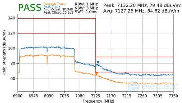
Plot 7-405 Antenna 1b Radiated Upper Band Edge (Peak & Average – UNII Band 8)
