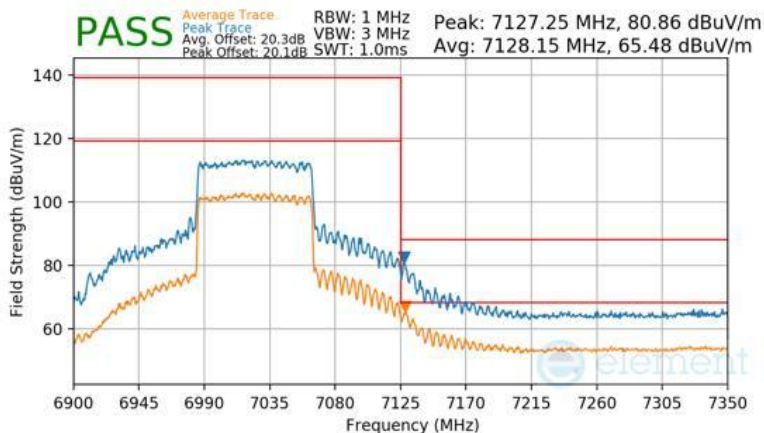
Plot 7-434 SDM Diversity Radiated Upper Band Edge (Peak & Average – UNII Band 8)
