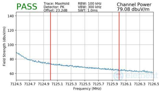
Plot 7-412 SDM Primary Radiated Integrated Band Edge (Peak – UNII Band 8)
