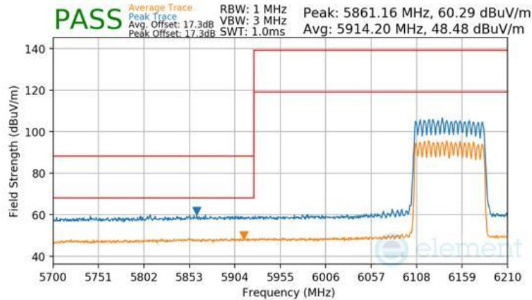
Plot 7-416 SDM Primary Radiated Lower Band Edge (Peak & Average – UNII Band 5)
