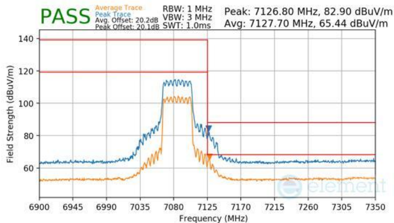
Plot 7-431 SDM Diversity Radiated Upper Band Edge (Peak & Average – UNII Band 8)
