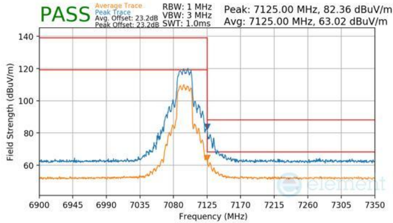
Plot 7-411 SDM Primary Radiated Upper Band Edge (Peak & Average – UNII Band 8)
