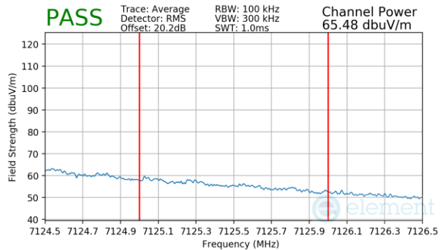
Plot 7-425 CDD Diversity Radiated Integrated Band Edge (Average – UNII Band 8)
