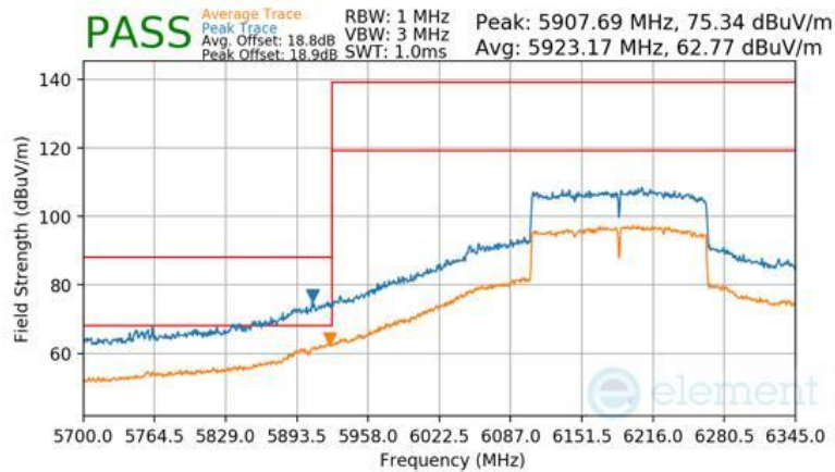
Plot 7-403 Antenna 1b Radiated Lower Band Edge (Peak & Average – UNII Band 5)
