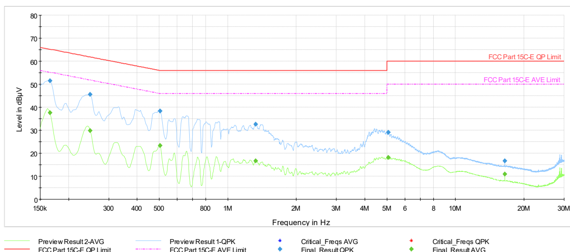
Plot 7-442. AC Line Conducted Plot with 802.11be SDM Diversity – Ch.61 (L1), with AC/DC Adapter
