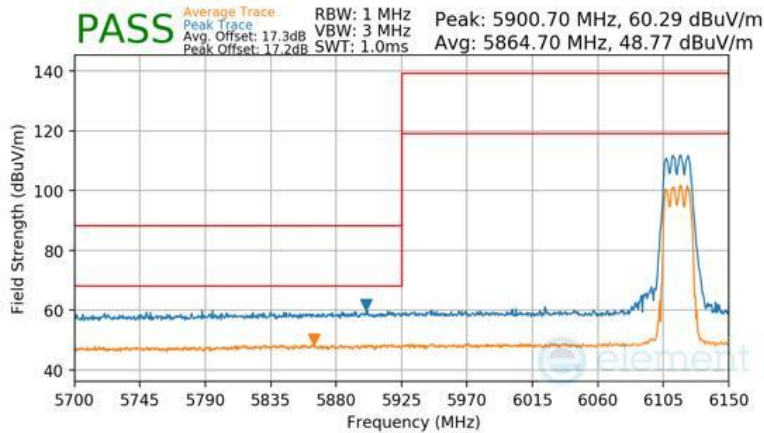
Plot 7-410 SDM Primary Radiated Lower Band Edge (Peak & Average – UNII Band 5)
