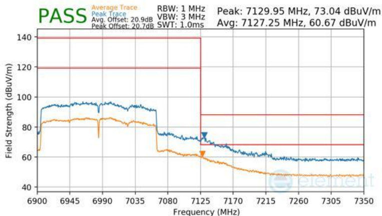
Plot 7-373 Antenna 5T Radiated Upper Band Edge (Peak & Average – UNII Band 8)
