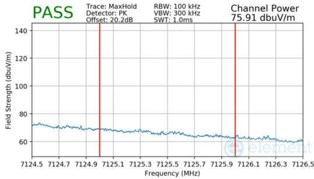
Plot 7-424 CDD Diversity Radiated Integrated Band Edge (Peak – UNII Band 8)
