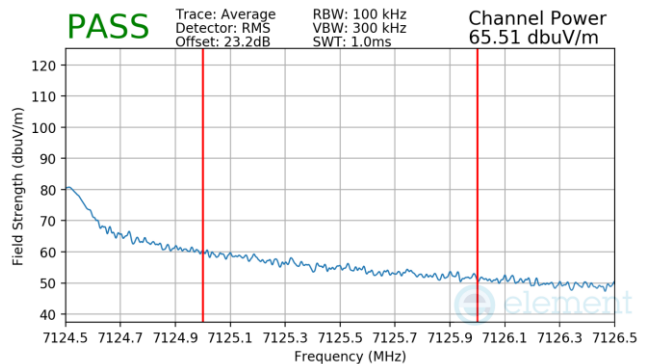
Plot 7-413 SDM Primary Radiated Integrated Band Edge (Average – UNII Band 8)
