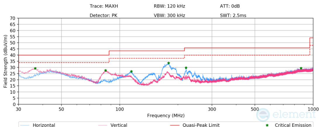
Plot 7-438. Radiated Spurious Emissions below 1GHz SDM Primary, 802.11be, Ch.61 with AC/DC Adapter
