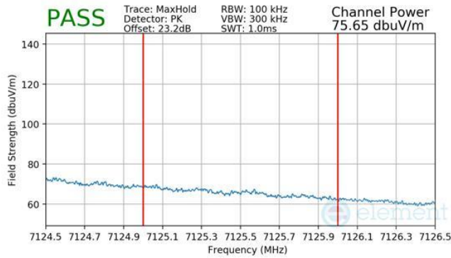
Plot 7-408 CDD Primary Radiated Integrated Band Edge (Peak – UNII Band 8)
