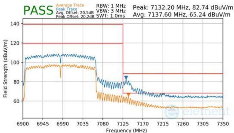
Plot 7-437 SDM Diversity Radiated Upper Band Edge (Peak & Average – UNII Band 8)
