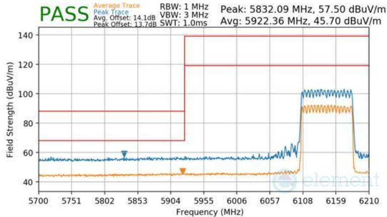
Plot 7-432 SDM Diversity Radiated Lower Band Edge (Peak & Average – UNII Band 5)
