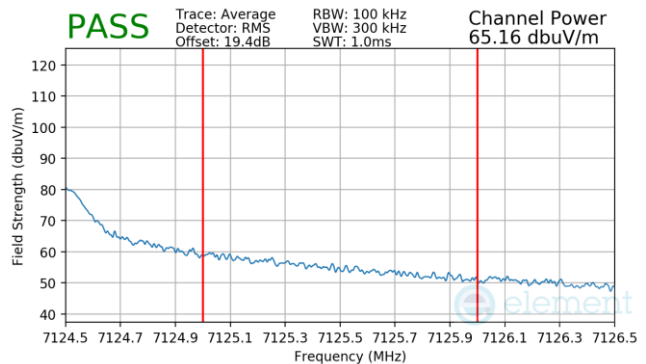
Plot 7-381 Antenna 3b Radiated Integrated Band Edge (Average – UNII Band 8)
