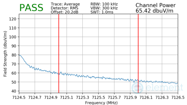
Plot 7-429 SDM Diversity Radiated Integrated Band Edge (Average – UNII Band 8)
