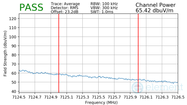
Plot 7-409 CDD Primary Radiated Integrated Band Edge (Average – UNII Band 8)
