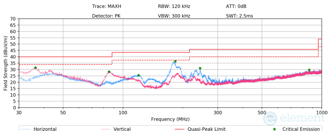
Plot 7-439. Radiated Spurious Emissions below 1GHz SDM Diversity, 802.11be, Ch.61 with AC/DC Adapter
