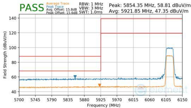
Plot 7-378 Antenna 3b Radiated Lower Band Edge (Peak & Average – UNII Band 5)
