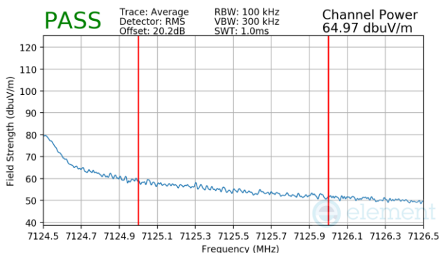
Plot 7-397 Antenna 1b Radiated Integrated Band Edge (Average – UNII Band 8)
