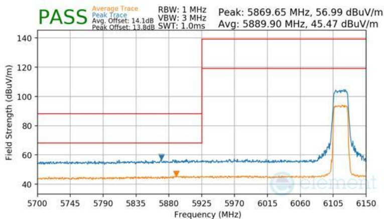
Plot 7-394 Antenna 1b Radiated Lower Band Edge (Peak & Average – UNII Band 5)
