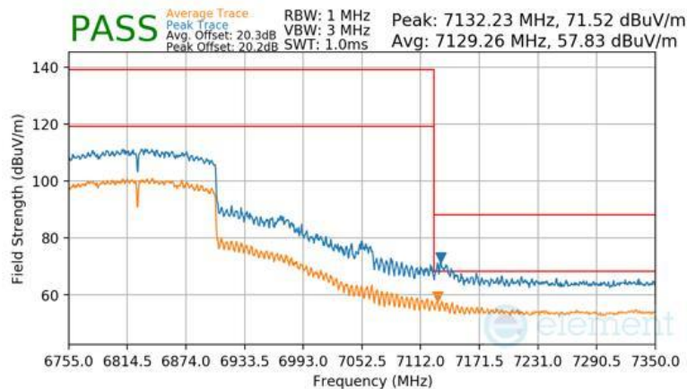
Plot 7-436 SDM Diversity Radiated Upper Band Edge (Peak & Average – UNII Band 7)
