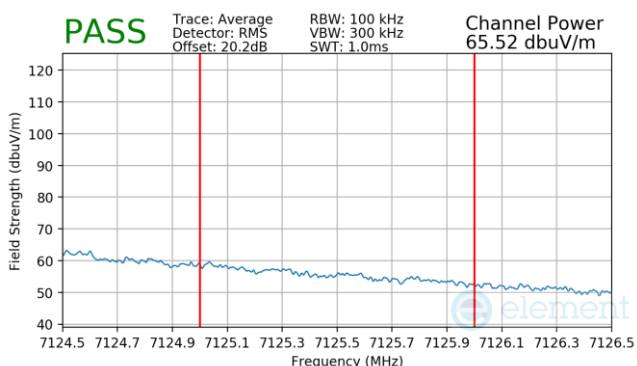
Plot 7-393 Antenna 1b Radiated Integrated Band Edge (Average – UNII Band 8)
