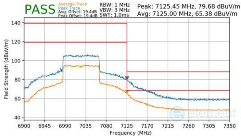
Plot 7-386 Antenna 3b Radiated Upper Band Edge (Peak & Average – UNII Band 8)
