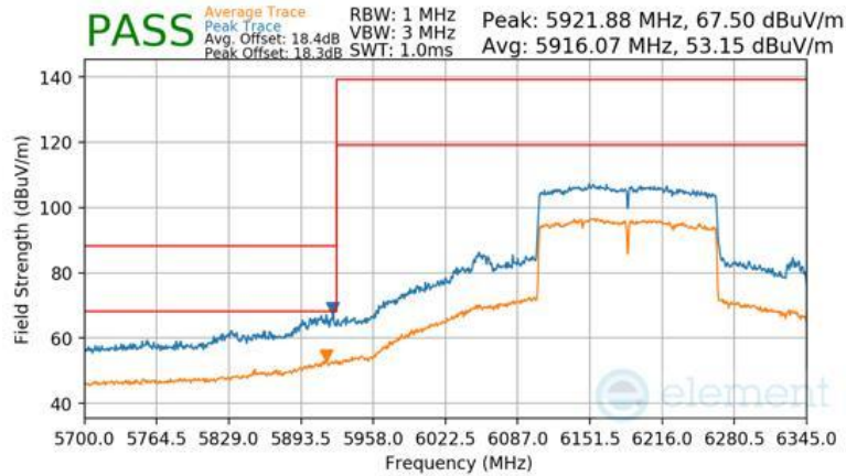
Plot 7-387 Antenna 3b Radiated Lower Band Edge (Peak & Average – UNII Band 5)
