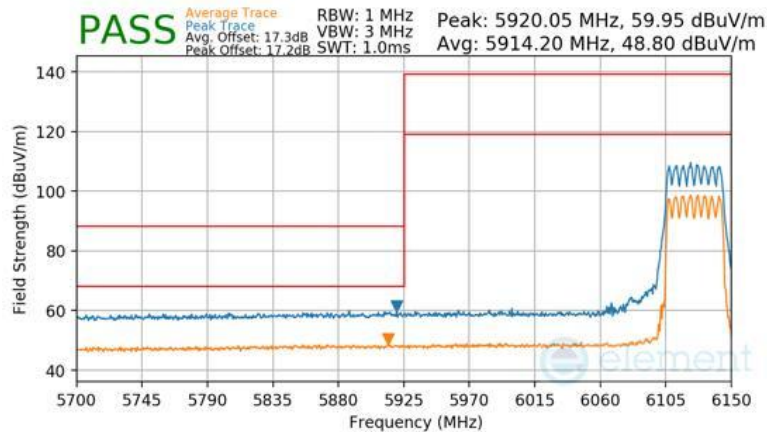
Plot 7-414 SDM Primary Radiated Lower Band Edge (Peak & Average – UNII Band 5)
