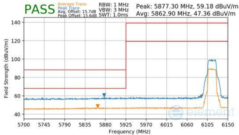
Plot 7-374 Antenna 3b Radiated Lower Band Edge (Peak & Average – UNII Band 5)
