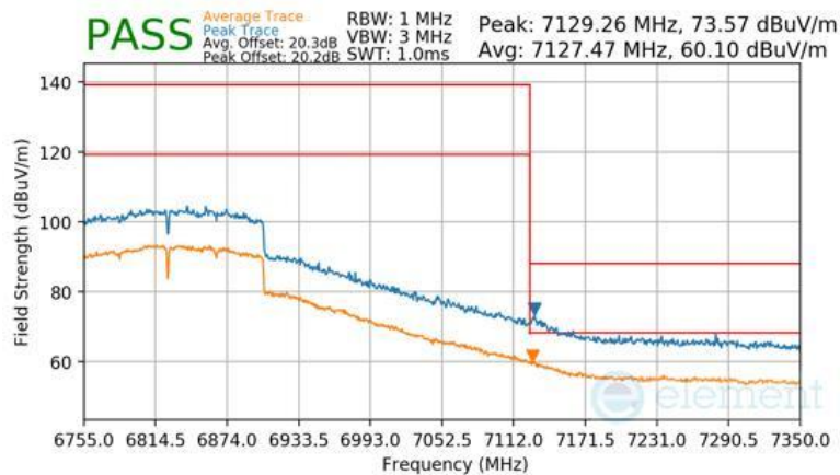
Plot 7-404 Antenna 1b Radiated Upper Band Edge (Peak & Average – UNII Band 7)
