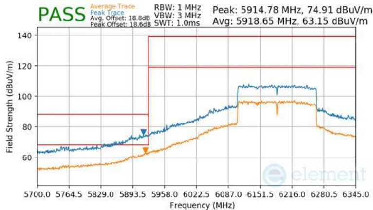
Plot 7-435 SDM Diversity Radiated Lower Band Edge (Peak & Average – UNII Band 5)
