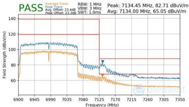
Plot 7-421 SDM Primary Radiated Upper Band Edge (Peak & Average – UNII Band 8)
