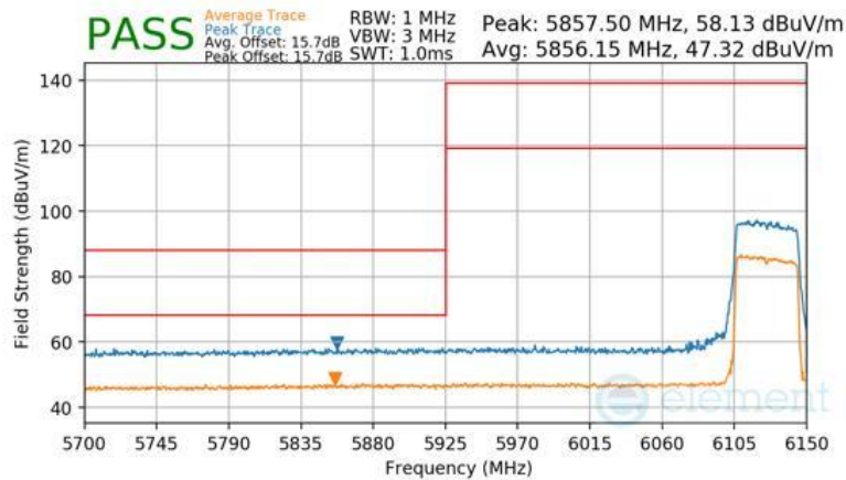
Plot 7-382 Antenna 3b Radiated Lower Band Edge (Peak & Average – UNII Band 5)
