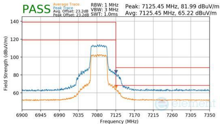
Plot 7-415 SDM Primary Radiated Upper Band Edge (Peak & Average – UNII Band 8)
