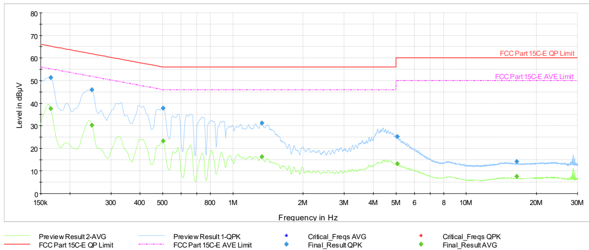
Plot 7-441. AC Line Conducted Plot with 802.11be SDM Primary – Ch. 61 (N), with AC/DC Adapter
