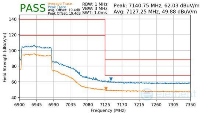
Plot 7-385 Antenna 3b Radiated Upper Band Edge (Peak & Average – UNII Band 8)
