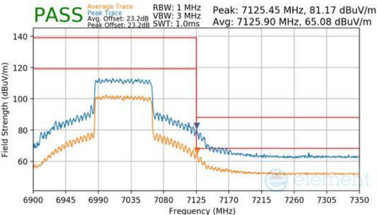
Plot 7-418 SDM Primary Radiated Upper Band Edge (Peak & Average – UNII Band 8)
