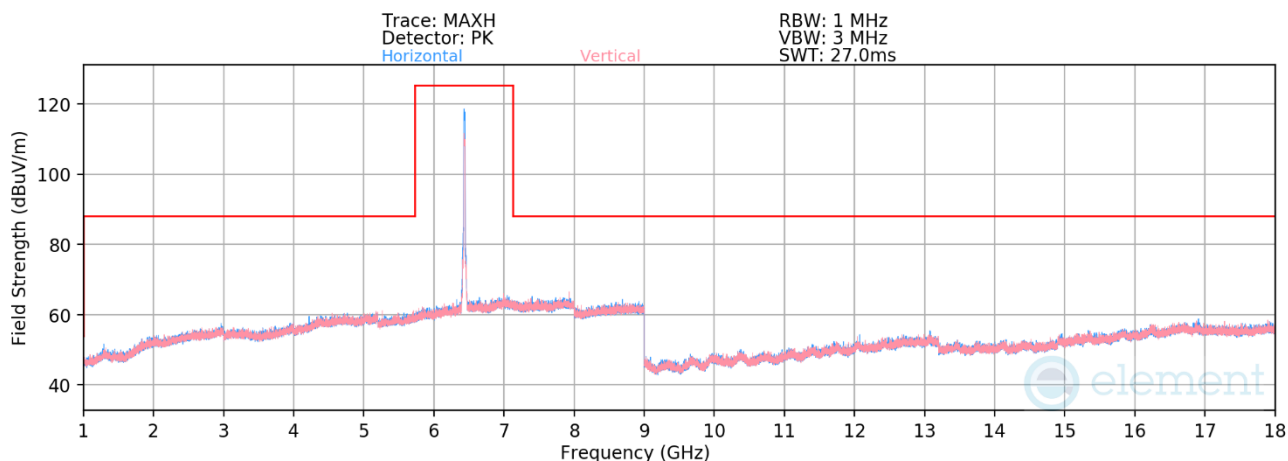
Plot 7-532. Radiated Spurious Emissions 1-18GHz CDD Primary (802.11be – Ch. 97)
