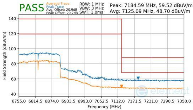
Plot 7-578 Antenna 5T Radiated Upper Band Edge (Peak & Average – UNII Band 7)
