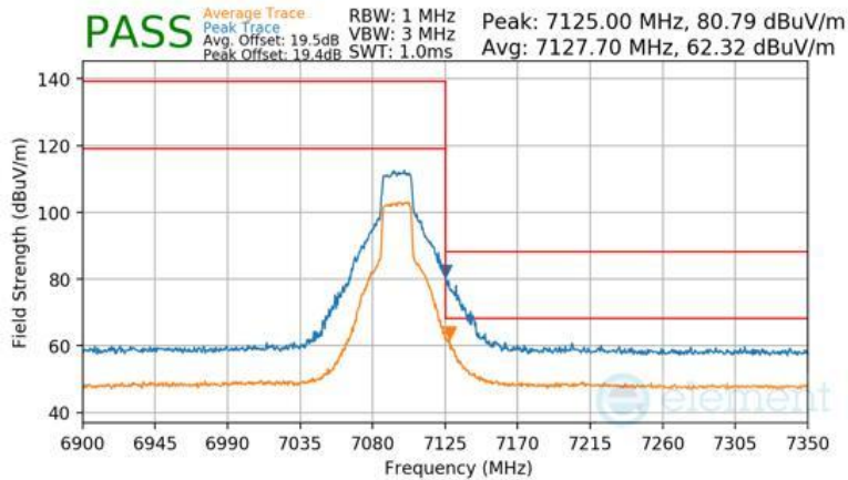
Plot 7-581 Antenna 3b Radiated Upper Band Edge (Peak & Average – UNII Band 8)
