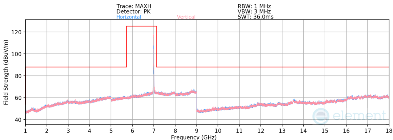
Plot 7-557. Radiated Spurious Emissions 1-18GHz CDD Diversity (802.11be – Ch. 209)
