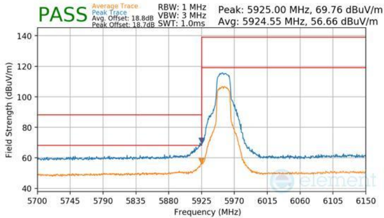
Plot 7-580 Antenna 3b Radiated Lower Band Edge (Peak & Average – UNII Band 5)
