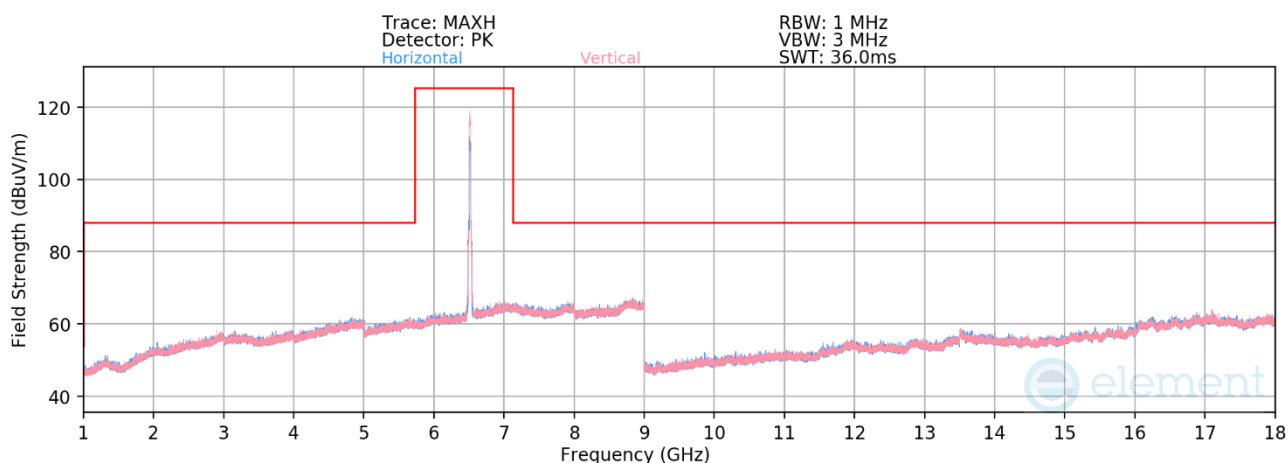
Plot 7-551. Radiated Spurious Emissions 1-18GHz CDD Diversity (802.11be – Ch. 113)
