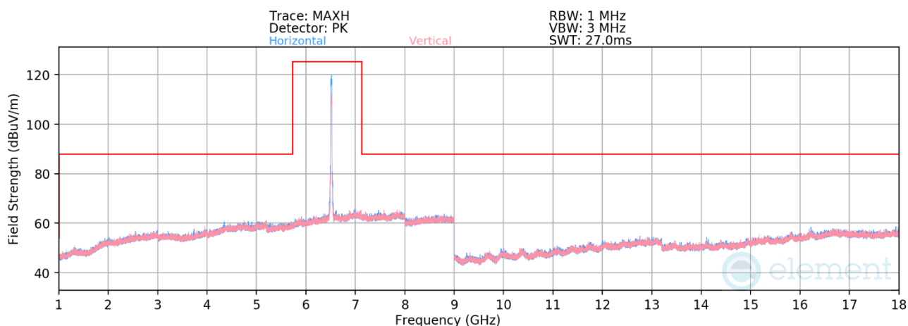
Plot 7-535. Radiated Spurious Emissions 1-18GHz CDD Primary (802.11be – Ch. 113)
