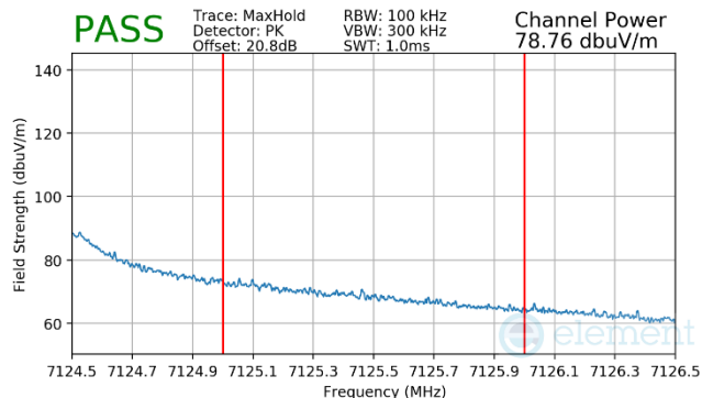
Plot 7-567 Antenna 5T Radiated Integrated Band Edge (Peak – UNII Band 8)
