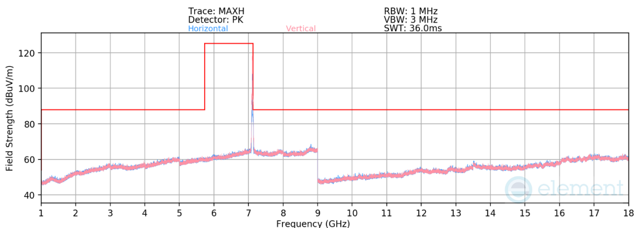
Plot 7-559. Radiated Spurious Emissions 1-18GHz CDD Diversity (802.11be – Ch. 233)
