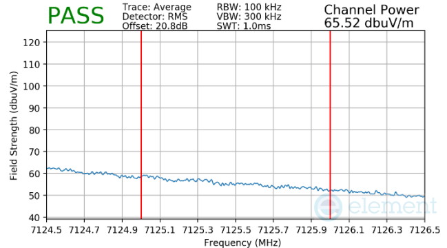
Plot 7-563 Antenna 5T Radiated Integrated Band Edge (Average – UNII Band 8)
