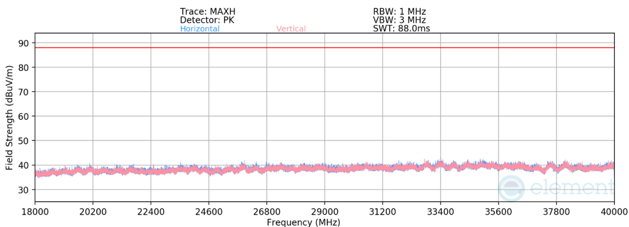
Plot 7-558. Radiated Spurious Emissions 18-40GHz CDD Diversity (802.11be – Ch. 209)
