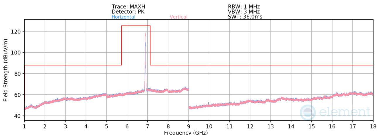
Plot 7-556. Radiated Spurious Emissions 1-18GHz CDD Diversity (802.11be – Ch. 189)
