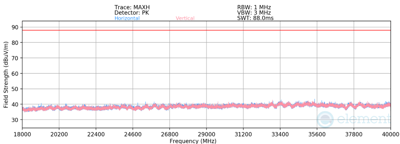
Plot 7-542. Radiated Spurious Emissions 18-40GHz CDD Primary (802.11be – Ch. 209)
