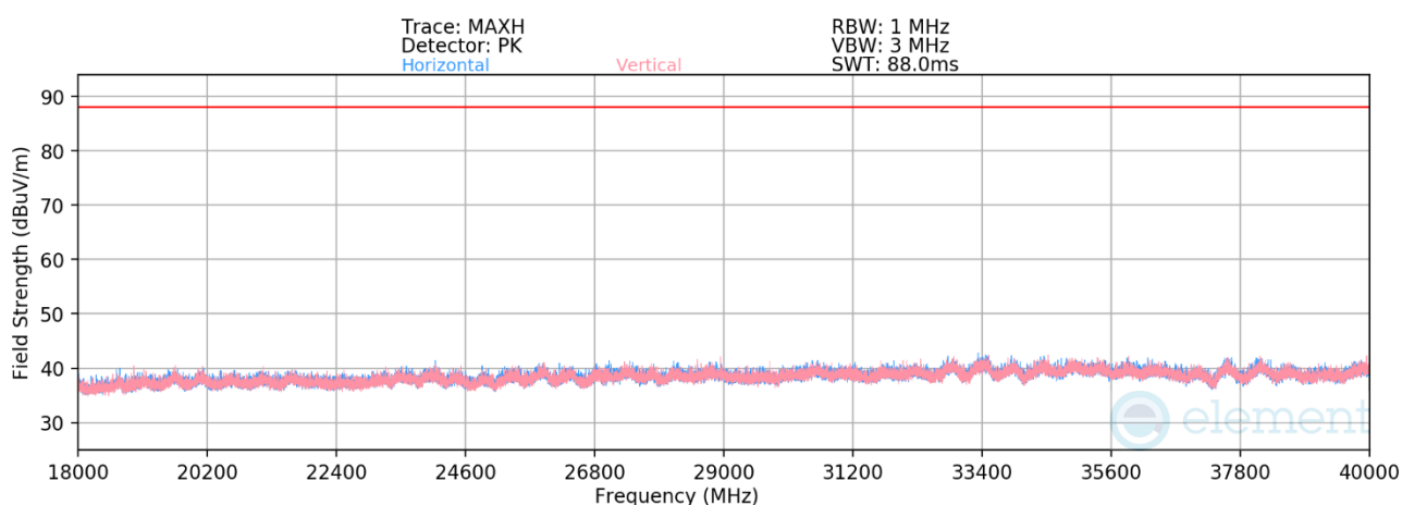
Plot 7-534. Radiated Spurious Emissions 18-40GHz CDD Primary (802.11be – Ch. 105)
