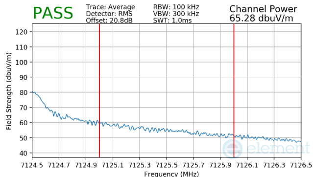
Plot 7-568 Antenna 5T Radiated Integrated Band Edge (Average – UNII Band 8)
