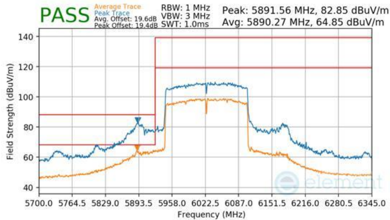
Plot 7-576 Antenna 5T Radiated Lower Band Edge (Peak & Average – UNII Band 5)
