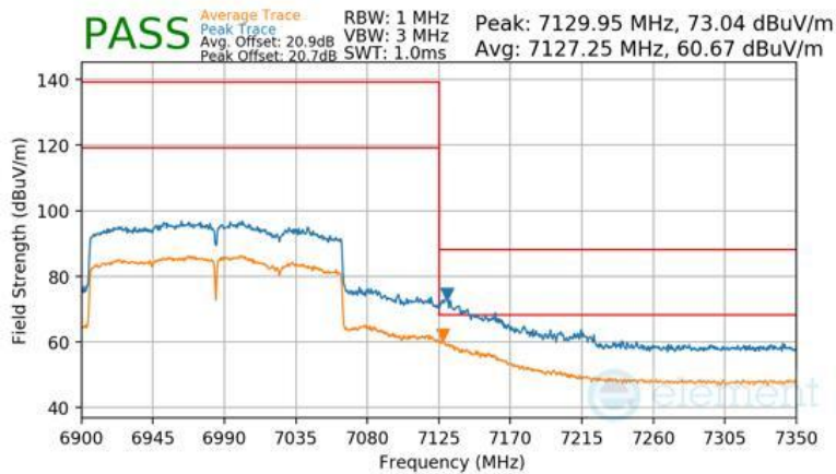
Plot 7-579 Antenna 5T Radiated Upper Band Edge (Peak & Average – UNII Band 8)
