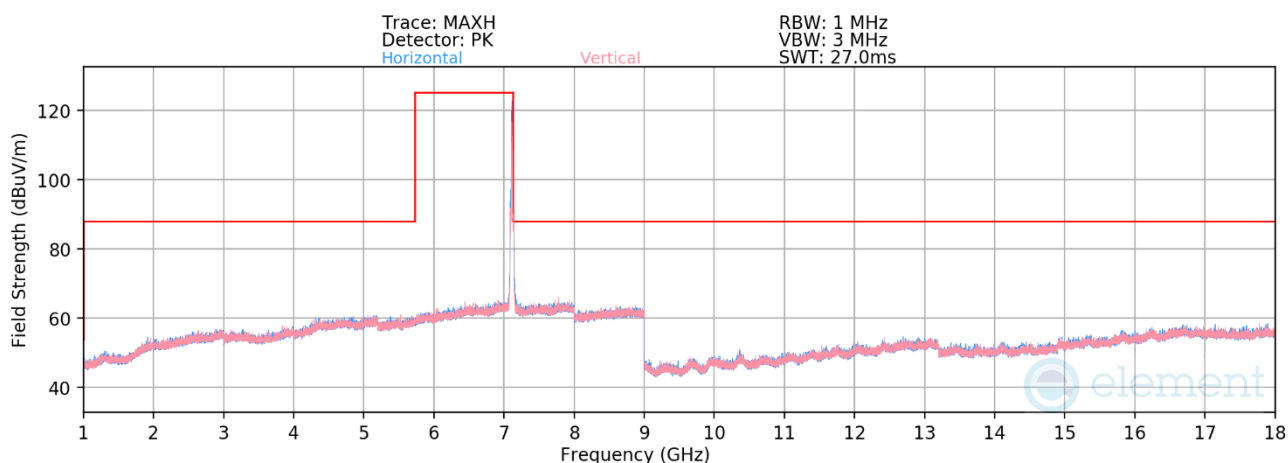
Plot 7-543. Radiated Spurious Emissions 1-18GHz CDD Primary (802.11be – Ch. 233)
