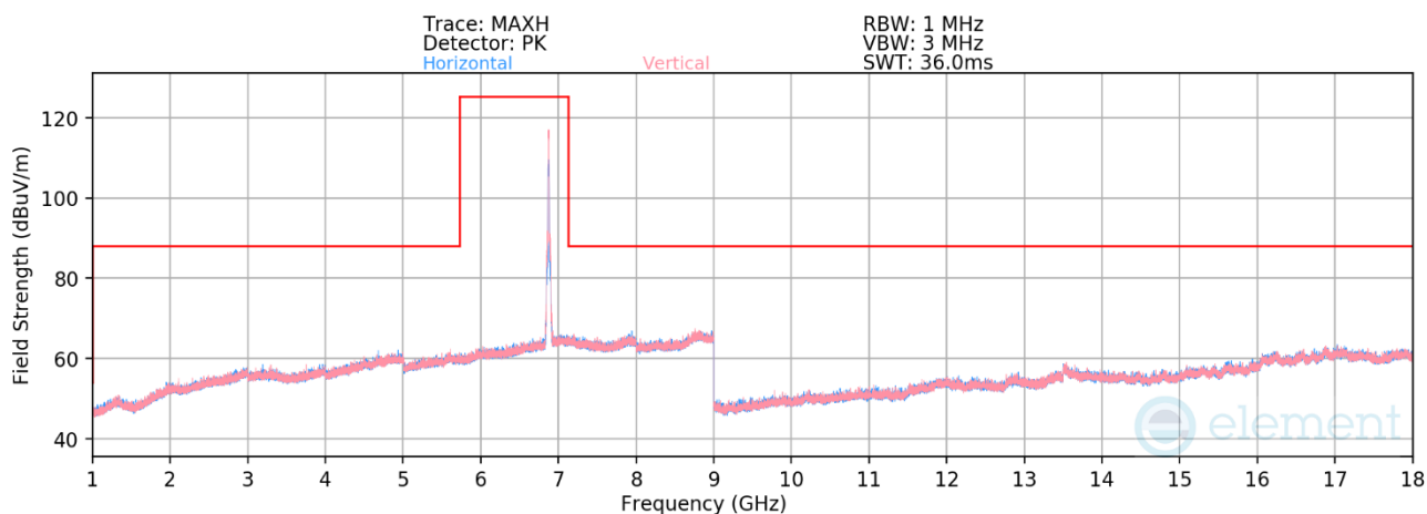
Plot 7-555. Radiated Spurious Emissions 1-18GHz CDD Diversity (802.11be – Ch. 185)
