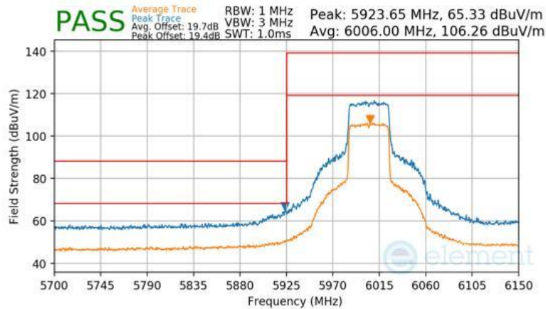
Plot 7-570 Antenna 5T Radiated Lower Band Edge (Peak & Average – UNII Band 5)
