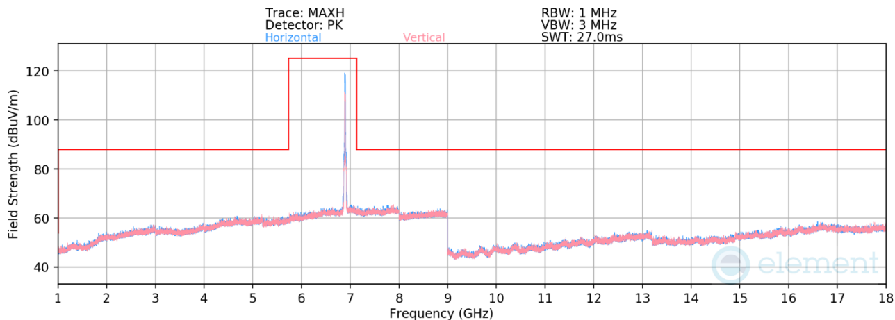
Plot 7-540. Radiated Spurious Emissions 1-18GHz CDD Primary (802.11be – Ch. 189)
