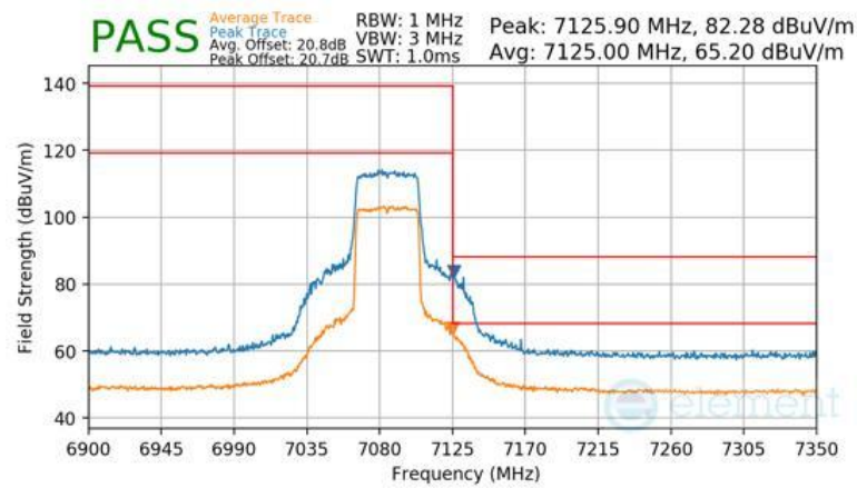
Plot 7-571 Antenna 5T Radiated Upper Band Edge (Peak & Average – UNII Band 8)
