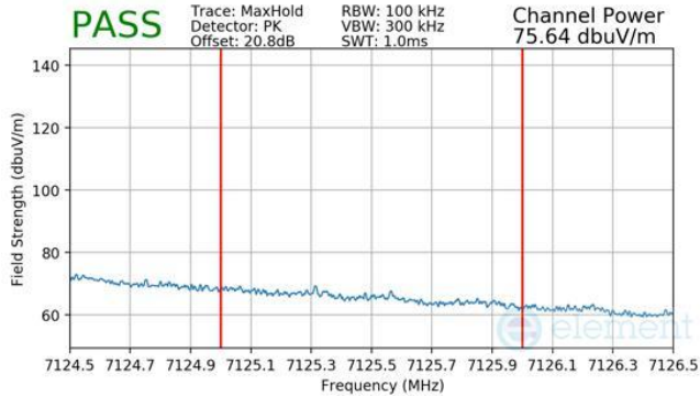
Plot 7-562 Antenna 5T Radiated Integrated Band Edge (Peak – UNII Band 8)
