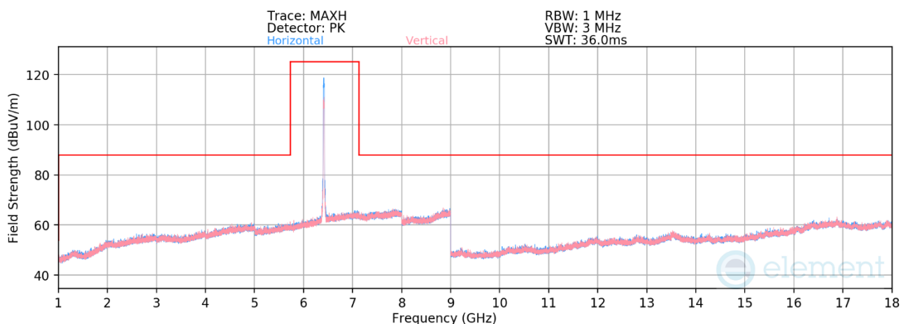
Plot 7-531. Radiated Spurious Emissions 1-18GHz CDD Primary (802.11be – Ch. 93)
