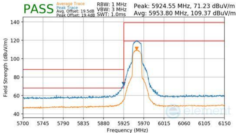
Plot 7-564 Antenna 5T Radiated Lower Band Edge (Peak & Average – UNII Band 5)
