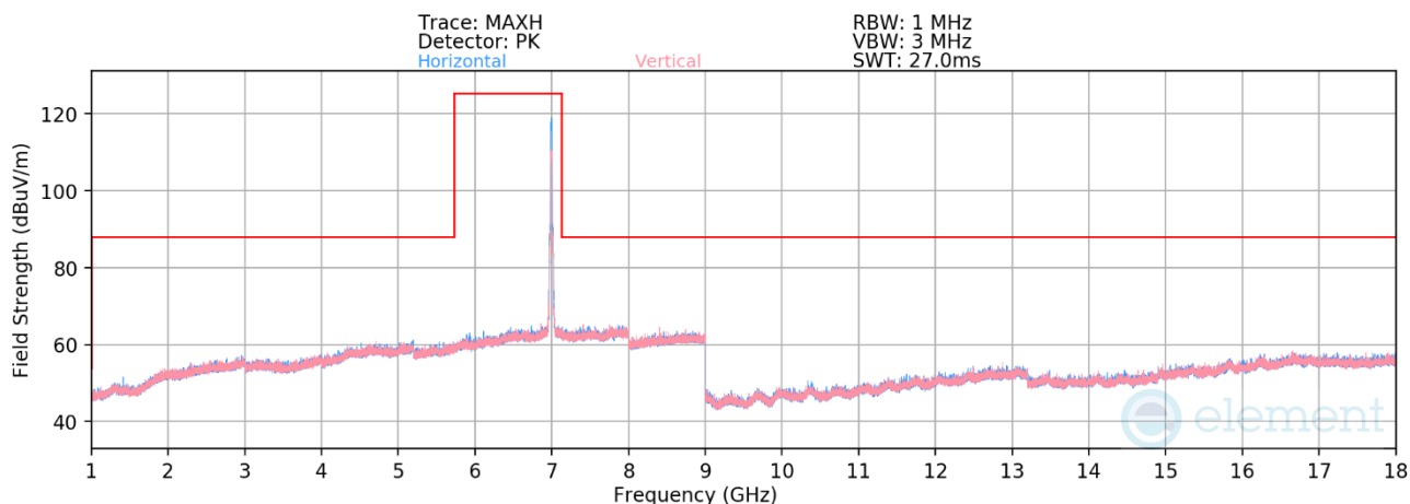
Plot 7-541. Radiated Spurious Emissions 1-18GHz CDD Primary (802.11be – Ch. 209)
