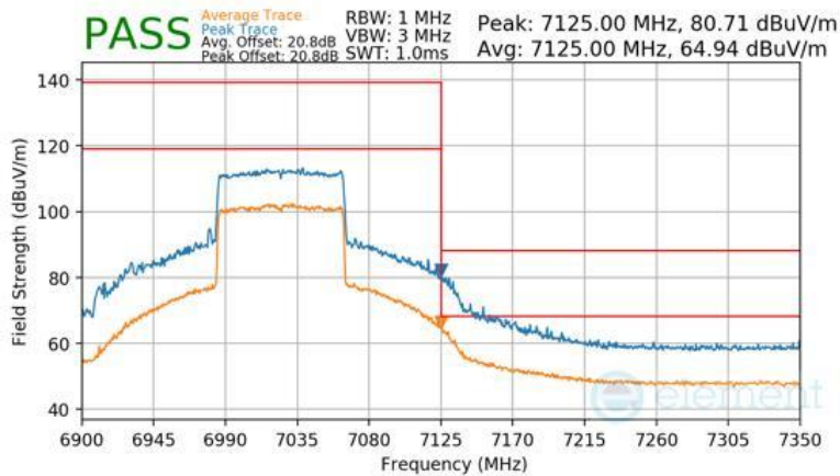
Plot 7-575 Antenna 5T Radiated Upper Band Edge (Peak & Average – UNII Band 8)
