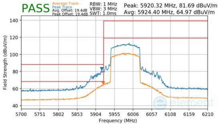
Plot 7-572 Antenna 5T Radiated Lower Band Edge (Peak & Average – UNII Band 5)
