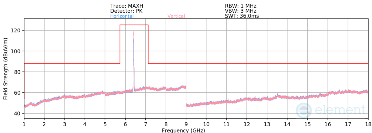
Plot 7-547. Radiated Spurious Emissions 1-18GHz CDD Diversity (802.11be – Ch. 93)
