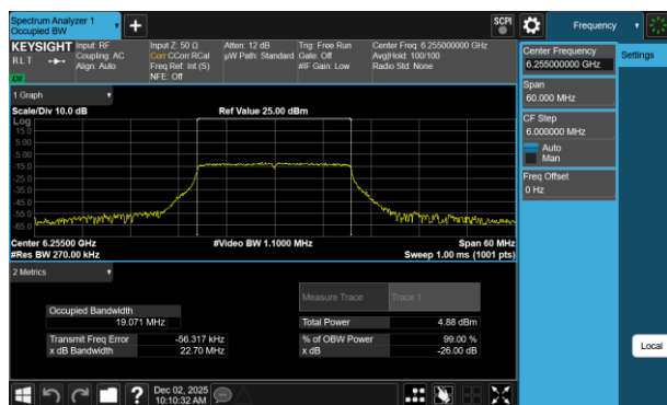
Plot 7-52 26dB BW & 99% OBW Antenna 3b (20MHz BW 802.11be(RU) RU242 Index61 - Ch.61)
