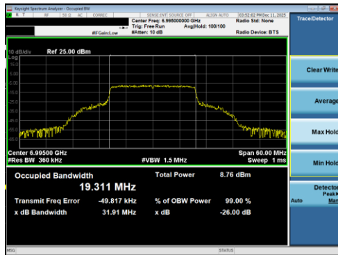
Plot 7-41 26dB BW & 99% OBW Antenna 5T (20MHz BW 802.11be(RU) RU242 Index61 - Ch.209)
