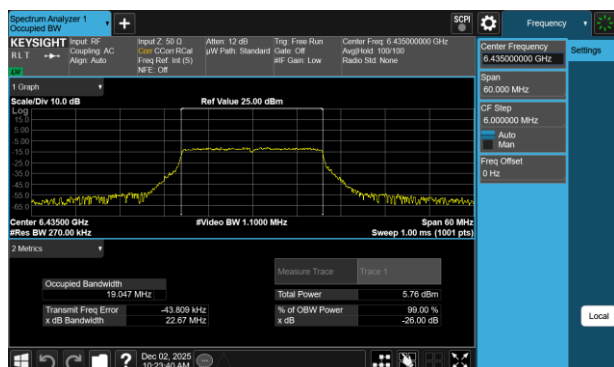
Plot 7-63 26dB BW & 99% OBW Antenna 3b (20MHz BW 802.11be(RU) RU242 Index61 - Ch.97)
