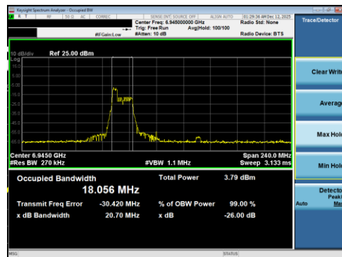
Plot 7-36 26dB BW & 99% OBW Antenna 5T (80MHz BW 802.11be(RU) RU52 Index37 - Ch.199)
