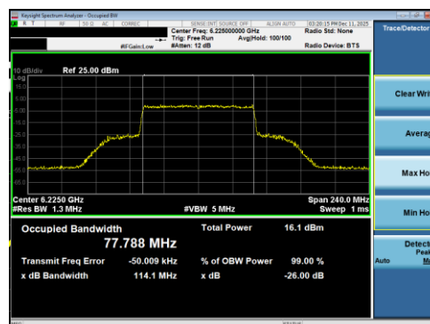
Plot 7-10 26dB BW & 99% OBW Antenna 5T (80MHz BW 802.11be(RU) RU996 Index67 - Ch.55)
