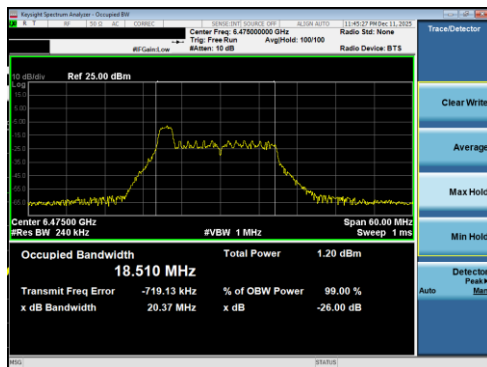
Plot 7-12 26dB BW & 99% OBW Antenna 5T (20MHz BW 802.11be(RU) RU26 Index0 - Ch.105)
