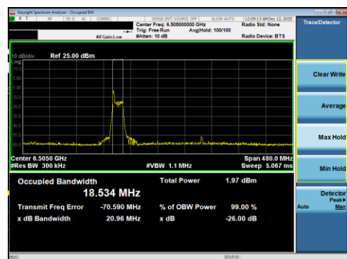
Plot 7-15 26dB BW & 99% OBW Antenna 5T (160MHz BW 802.11be(RU) RU26 Index0 - Ch.111)
