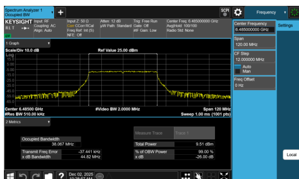
Plot 7-64 26dB BW & 99% OBW Antenna 3b (40MHz BW 802.11be(RU) RU484 Index65 - Ch.107)
