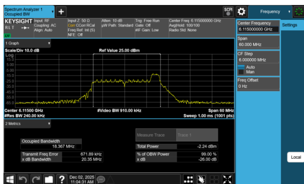
Plot 7-45 26dB BW & 99% OBW Antenna 3b (20MHz BW 802.11be(RU) RU26 Index8 - Ch.33)
