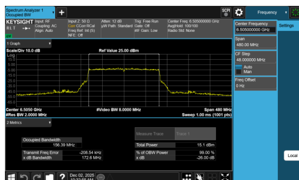
Plot 7-66 26dB BW & 99% OBW Antenna 3b (160MHz BW 802.11be(RU) RU996X2 Index68 - Ch.111)
