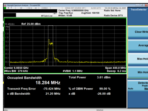
Plot 7-37 26dB BW & 99% OBW Antenna 5T (160MHz BW 802.11be(RU) RU52 Index37 - Ch.207)
