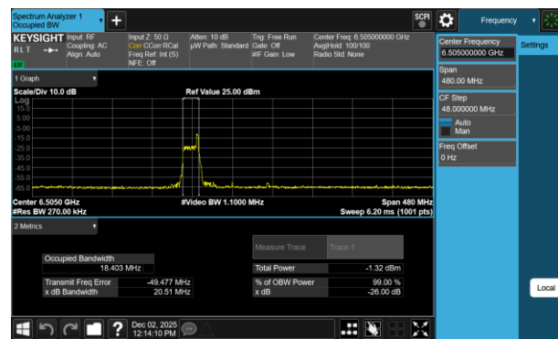
Plot 7-59 26dB BW & 99% OBW Antenna 3b (160MHz BW 802.11be(RU) RU26 Index17 - Ch.111)
