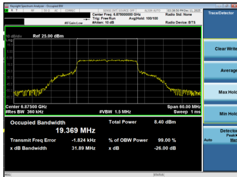
Plot 7-30 26dB BW & 99% OBW Antenna 5T (20MHz BW 802.11be(RU) RU242 Index61 - Ch.185)
