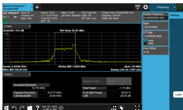
Plot 7-57 26dB BW & 99% OBW Antenna 3b (40MHz BW 802.11be(RU) RU26 Index8 - Ch.115)
