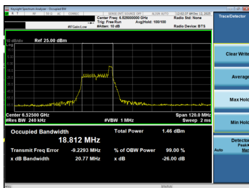
Plot 7-13 26dB BW & 99% OBW Antenna 5T (40MHz BW 802.11be(RU) RU26 Index8 - Ch.115)
