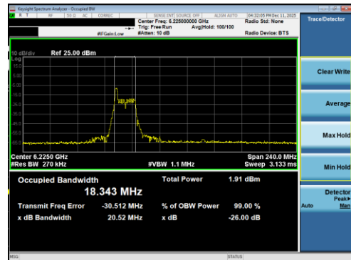
Plot 7-3 26dB BW & 99% OBW Antenna 5T (80MHz BW 802.11be(RU) RU26 Index0 - Ch.55)
