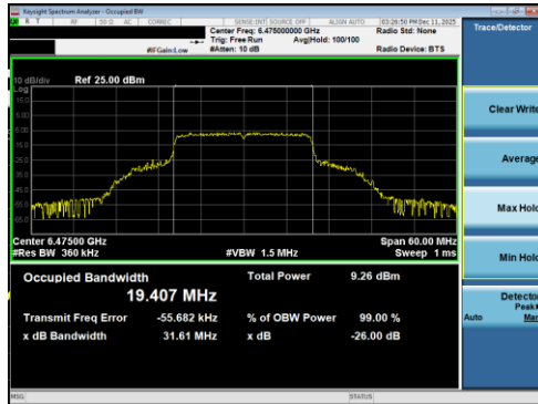
Plot 7-19 26dB BW & 99% OBW Antenna 5T (20MHz BW 802.11be(RU) RU242 Index61 - Ch.105)
