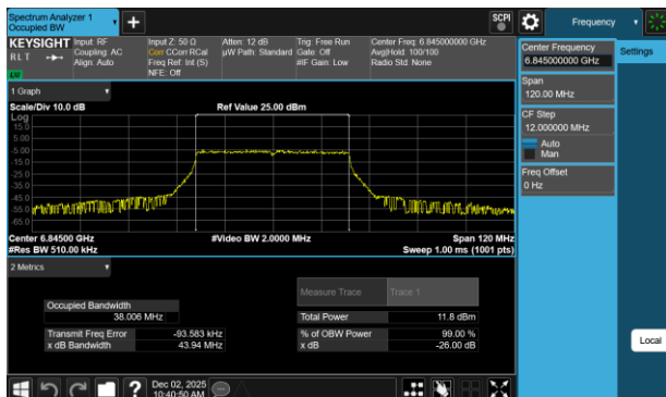
Plot 7-75 26dB BW & 99% OBW Antenna 3b (40MHz BW 802.11be(RU) RU484 Index65 - Ch.179)
