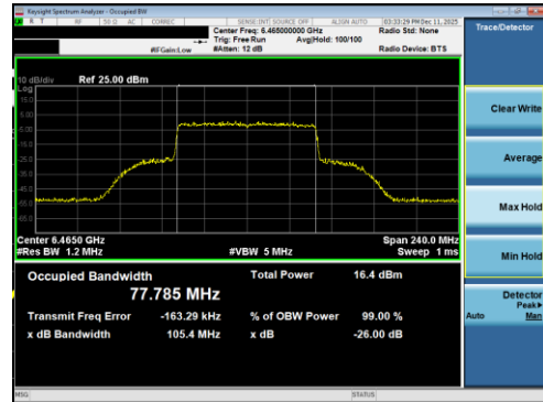
Plot 7-21 26dB BW & 99% OBW Antenna 5T (80MHz BW 802.11be(RU) RU996 Index67 - Ch.103)
