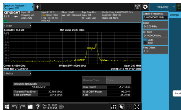
Plot 7-58 26dB BW & 99% OBW Antenna 3b (80MHz BW 802.11be(RU) RU26 Index36 - Ch.103)
