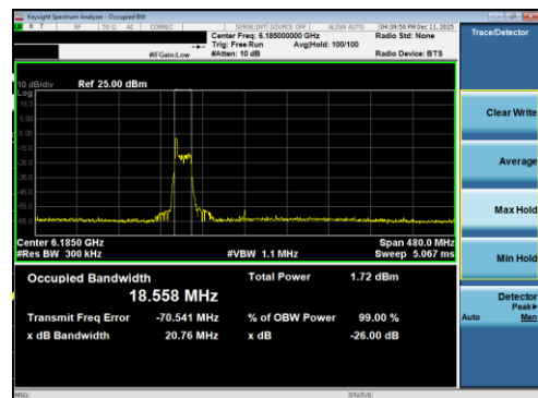
Plot 7-4 26dB BW & 99% OBW Antenna 5T (160MHz BW 802.11be(RU) RU26 Index0 - Ch.47)
