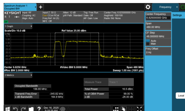
Plot 7-29 26dB BW & 99% OBW Antenna 5T (160MHz BW 802.11be(RU) RU996+484+242 Index97 - Ch.175)
