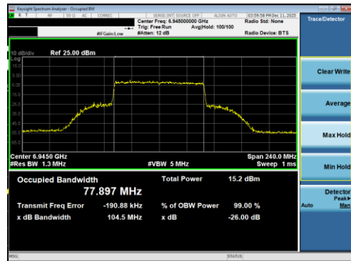
Plot 7-43 26dB BW & 99% OBW Antenna 5T (80MHz BW 802.11be(RU) RU996 Index67 - Ch.199)
