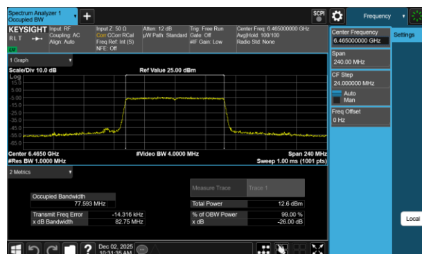
Plot 7-65 26dB BW & 99% OBW Antenna 3b (80MHz BW 802.11be(RU) RU996 Index67 - Ch.103)
