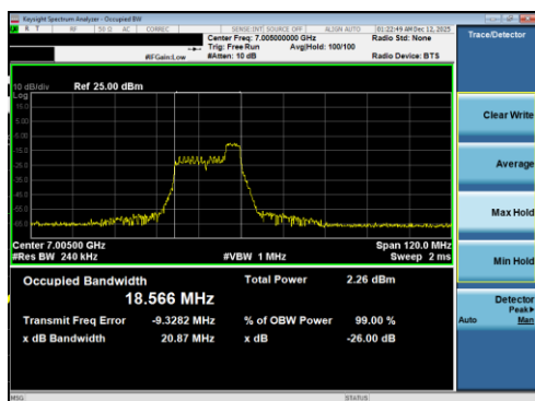
Plot 7-35 26dB BW & 99% OBW Antenna 5T (40MHz BW 802.11be(RU) RU52 Index40 - Ch.211)
