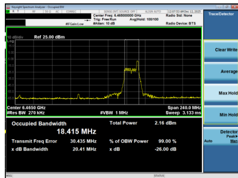
Plot 7-14 26dB BW & 99% OBW Antenna 5T (80MHz BW 802.11be(RU) RU26 Index36 - Ch.103)
