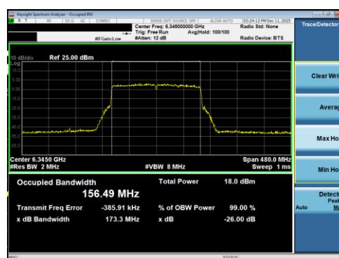
Plot 7-11 26dB BW & 99% OBW Antenna 5T (160MHz BW 802.11be(RU) RU996X2 Index68 - Ch.79)
