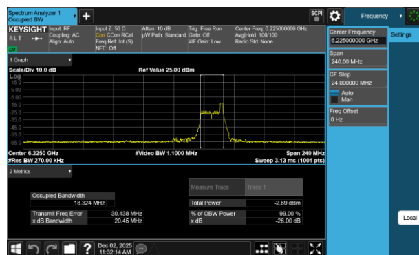
Plot 7-47 26dB BW & 99% OBW Antenna 3b (80MHz BW 802.11be(RU) RU26 Index36 - Ch.55)
