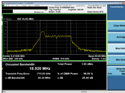
Plot 7-1 26dB BW & 99% OBW Antenna 5T (20MHz BW 802.11be(RU) RU26 Index0 - Ch.93)
