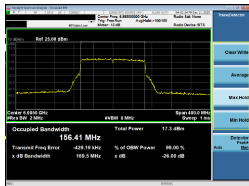
Plot 7-44 26dB BW & 99% OBW Antenna 5T (160MHz BW 802.11be(RU) RU996X2 Index68 - Ch.207)
