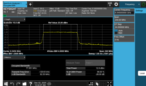
Plot 7-76 26dB BW & 99% OBW Antenna 3b (80MHz BW 802.11be(RU) RU996 Index67 - Ch.119)
