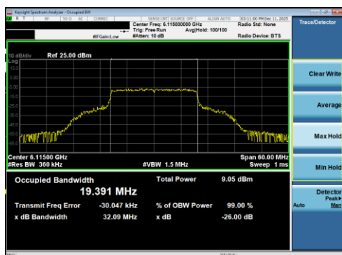
Plot 7-8 26dB BW & 99% OBW Antenna 5T (20MHz BW 802.11be(RU) RU242 Index61 - Ch.33)
