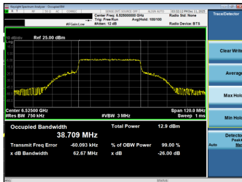
Plot 7-20 26dB BW & 99% OBW Antenna 5T (40MHz BW 802.11be(RU) RU484 Index65 - Ch.115)
