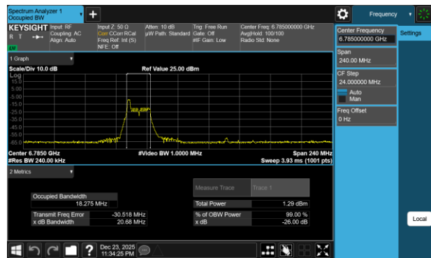
Plot 7-25 26dB BW & 99% OBW Antenna 5T (80MHz BW 802.11be(RU) RU26 Index0 - Ch.167)
