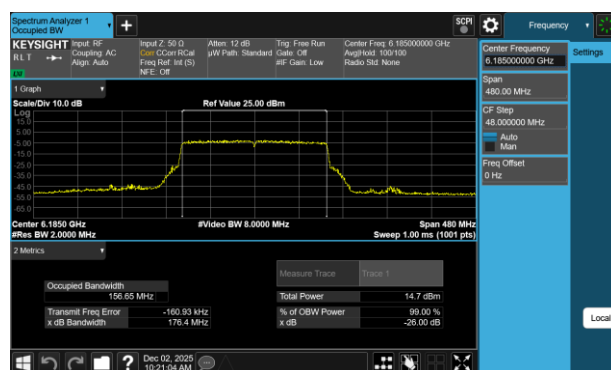
Plot 7-55 26dB BW & 99% OBW Antenna 3b (160MHz BW 802.11be(RU) RU996X2 Index68 - Ch.47)
