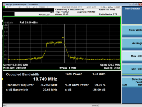
Plot 7-24 26dB BW & 99% OBW Antenna 5T (40MHz BW 802.11be(RU) RU26 Index8 - Ch.179)
