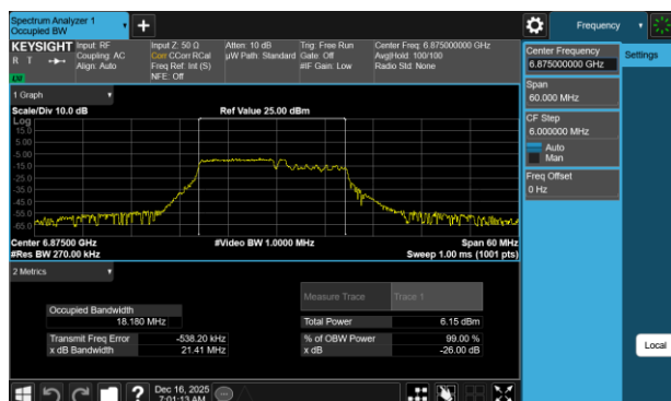
Plot 7-27 26dB BW & 99% OBW Antenna 5T (20MHz BW 802.11be(RU) RU106+26 Index82 - Ch.185)
