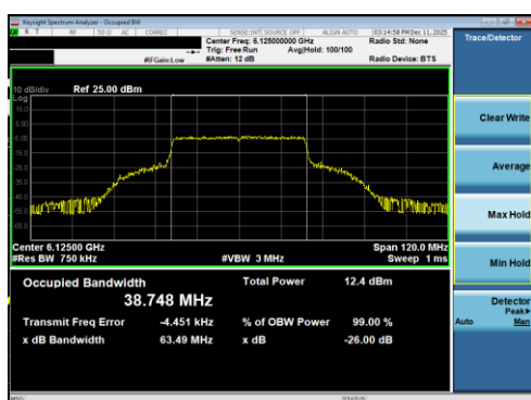
Plot 7-9 26dB BW & 99% OBW Antenna 5T (40MHz BW 802.11be(RU) RU484 Index65 - Ch.35)
