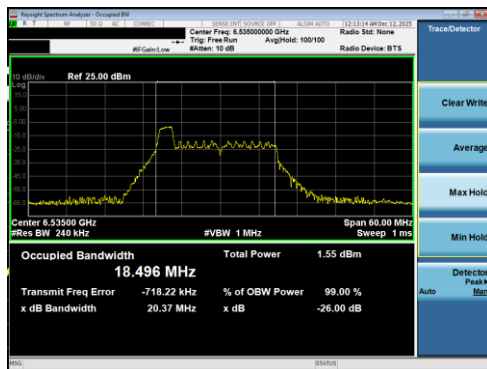
Plot 7-23 26dB BW & 99% OBW Antenna 5T (20MHz BW 802.11be(RU) RU26 Index0 - Ch.117)
