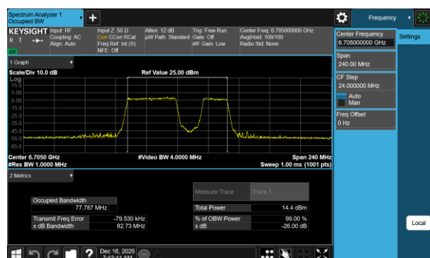
Plot 7-28 26dB BW & 99% OBW Antenna 5T (80MHz BW 802.11be(RU) RU484+242 Index92 - Ch.151)
