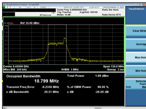
Plot 7-2 26dB BW & 99% OBW Antenna 5T (40MHz BW 802.11be(RU) RU26 Index8 - Ch.91)
