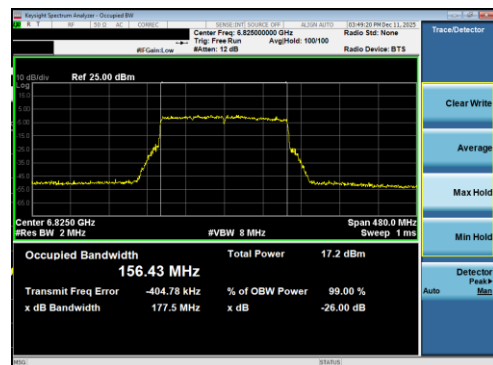
Plot 7-33 26dB BW & 99% OBW Antenna 5T (160MHz BW 802.11be(RU) RU996X2 Index68 - Ch.175)
