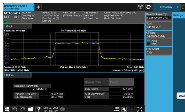
Plot 7-54 26dB BW & 99% OBW Antenna 3b (80MHz BW 802.11be(RU) RU996 Index67 - Ch.55)
