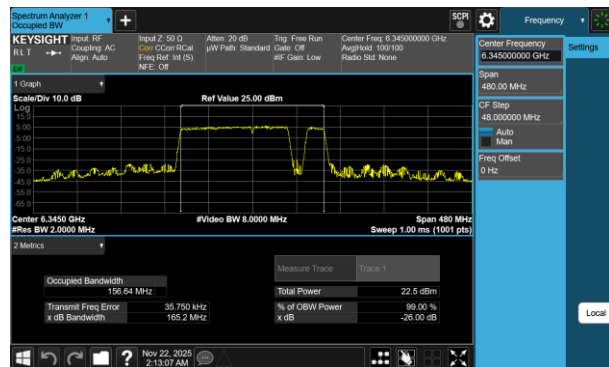
Plot 7-84 26dB BW & 99% OBW Antenna 3b (160MHz BW 802.11be(RU) RU996+484+242 Index98 - Ch.79)
