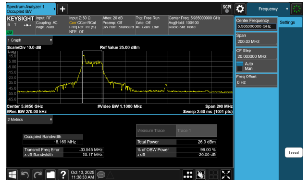
Plot 7-80 26dB BW & 99% OBW Antenna 3b (80MHz BW 802.11be(RU) RU26 Index0 - Ch.7)
