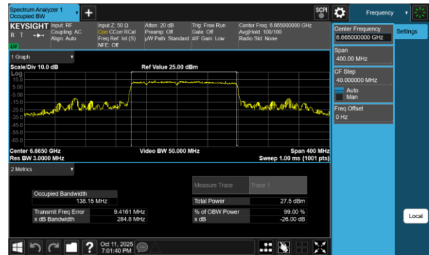
Plot 7-29 26dB BW & 99% OBW Antenna 5T (160MHz BW 802.11be(RU) RU996+484+242 Index96 - Ch.143)
