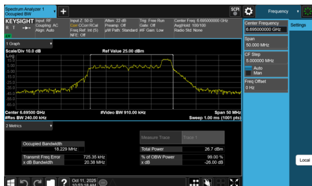
Plot 7-23 26dB BW & 99% OBW Antenna 5T (20MHz BW 802.11be(RU) RU26 Index8 - Ch.149)
