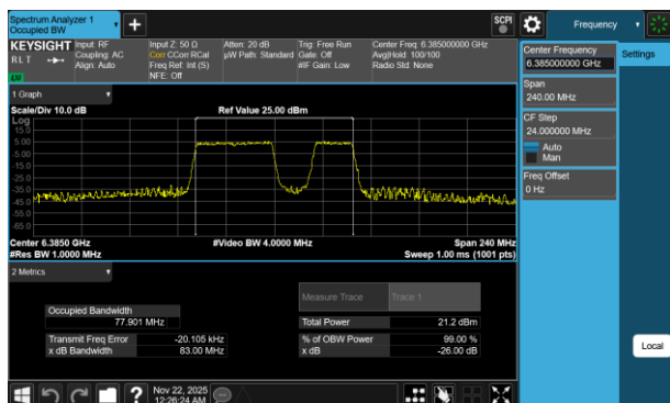
Plot 7-83 26dB BW & 99% OBW Antenna 3b (80MHz BW 802.11be(RU) RU484+242 Index92 - Ch.87)
