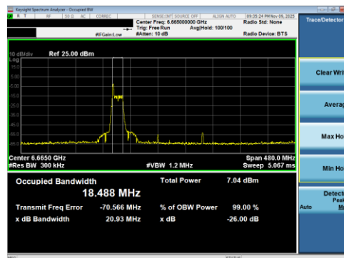
Plot 7-59 26dB BW & 99% OBW Antenna 5T (160MHz BW 802.11be(RU) RU26 Index0 - Ch.143)
