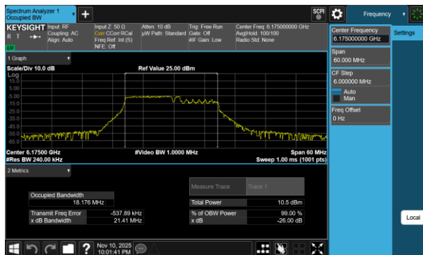
Plot 7-38 26dB BW & 99% OBW Antenna 5T (20MHz BW 802.11be(RU) RU106+26 Index82 - Ch.45)
