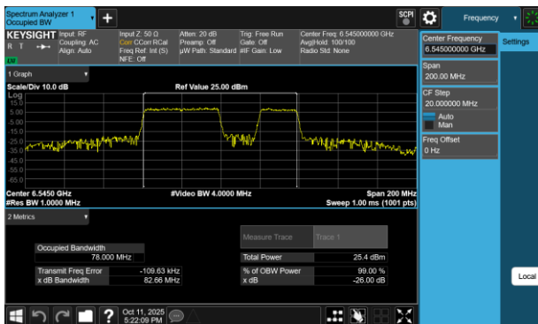
Plot 7-28 26dB BW & 99% OBW Antenna 5T (80MHz BW 802.11be(RU) RU484+242 Index92 - Ch.119)
