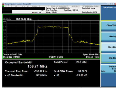
Plot 7-55 26dB BW & 99% OBW Antenna 5T (160MHz BW 802.11be(RU) RU996X2 Index68 - Ch.111)
