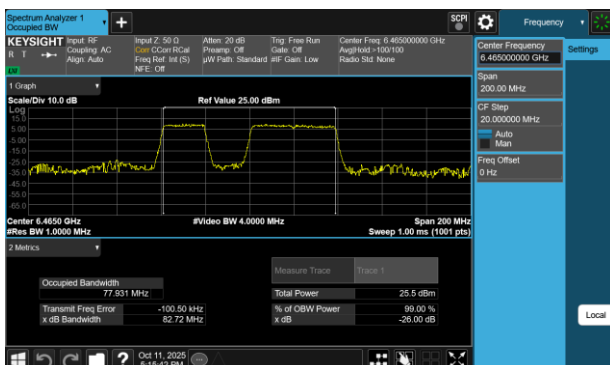
Plot 7-17 26dB BW & 99% OBW Antenna 5T (80MHz BW 802.11be(RU) RU484+242 Index91 - Ch.103)
