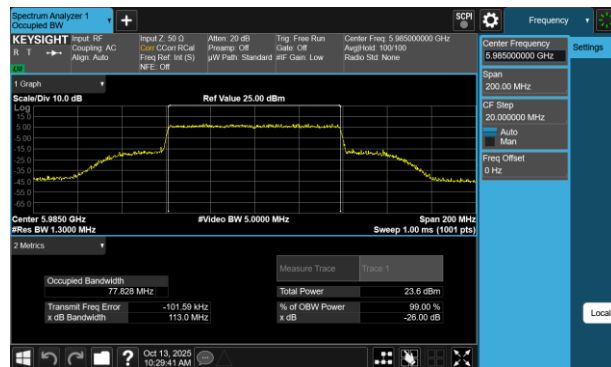
Plot 7-87 26dB BW & 99% OBW Antenna 3b (80MHz BW 802.11be(RU) RU996 Index67 - Ch.7)
