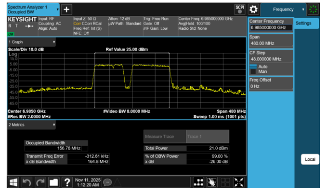
Plot 7-73 26dB BW & 99% OBW Antenna 5T (160MHz BW 802.11be(RU) RU996+484+242 Index99 - Ch.207)
