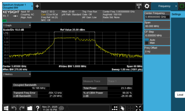
Plot 7-82 26dB BW & 99% OBW Antenna 3b (20MHz BW 802.11be(RU) RU106+26 Index82 - Ch.1)
