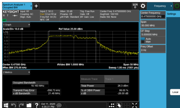
Plot 7-16 26dB BW & 99% OBW Antenna 5T (20MHz BW 802.11be(RU) RU106+26 Index82 - Ch.105)
