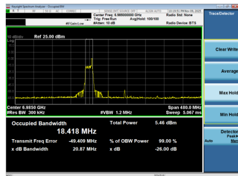
Plot 7-70 26dB BW & 99% OBW Antenna 5T (160MHz BW 802.11be(RU) RU26 Index17 - Ch.207)
