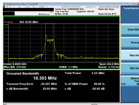
Plot 7-58 26dB BW & 99% OBW Antenna 5T (80MHz BW 802.11be(RU) RU26 Index0 - Ch.183)
