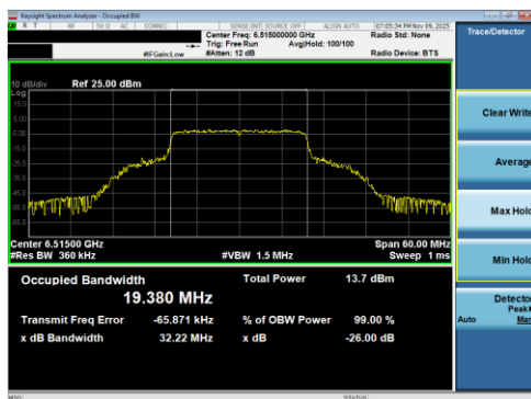
Plot 7-52 26dB BW & 99% OBW Antenna 5T (20MHz BW 802.11be(RU) RU242 Index61 - Ch.113)
