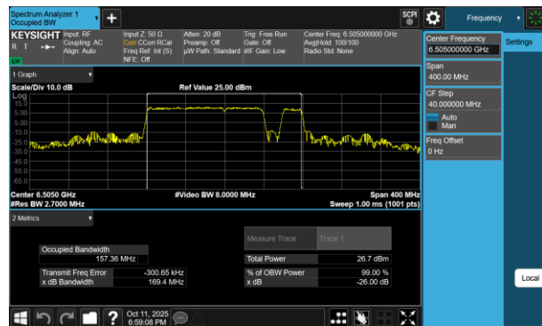
Plot 7-18 26dB BW & 99% OBW Antenna 5T (160MHz BW 802.11be(RU) RU996+484+242 Index98 - Ch.111)
