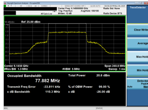
Plot 7-43 26dB BW & 99% OBW Antenna 5T (80MHz BW 802.11be(RU) RU996 Index67 - Ch.39)
