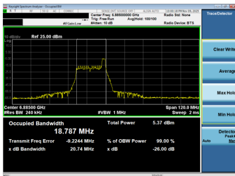
Plot 7-68 26dB BW & 99% OBW Antenna 5T (40MHz BW 802.11be(RU) RU26 Index8 - Ch.187)
