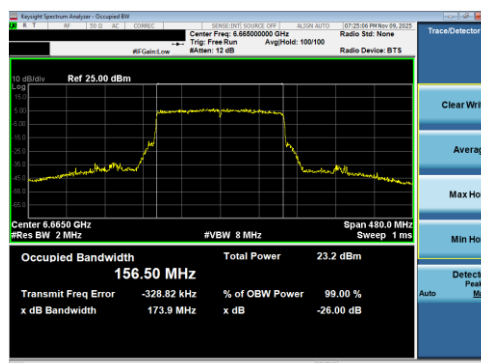
Plot 7-66 26dB BW & 99% OBW Antenna 5T (160MHz BW 802.11be(RU) RU996X2 Index68 - Ch.143)
