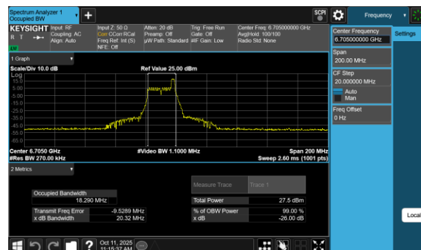
Plot 7-25 26dB BW & 99% OBW Antenna 5T (80MHz BW 802.11be(RU) RU26 Index17 - Ch.151)
