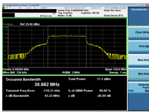
Plot 7-64 26dB BW & 99% OBW Antenna 5T (40MHz BW 802.11be(RU) RU484 Index65 - Ch.123)
