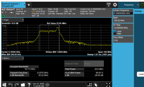
Plot 7-79 26dB BW & 99% OBW Antenna 3b (40MHz BW 802.11be(RU) RU26 Index8 - Ch.43)
