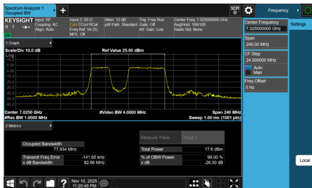
Plot 7-72 26dB BW & 99% OBW Antenna 5T (80MHz BW 802.11be(RU) RU484+242 Index91 - Ch.215)
