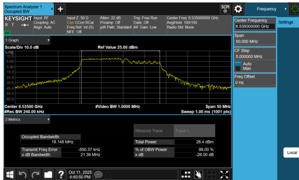
Plot 7-27 26dB BW & 99% OBW Antenna 5T (20MHz BW 802.11be(RU) RU106+26 Index82 - Ch.117)
