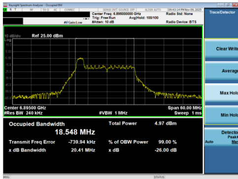
Plot 7-67 26dB BW & 99% OBW Antenna 5T (20MHz BW 802.11be(RU) RU26 Index0 - Ch.189)
