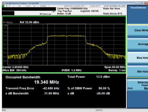
Plot 7-41 26dB BW & 99% OBW Antenna 5T (20MHz BW 802.11be(RU) RU242 Index61 - Ch.1)
