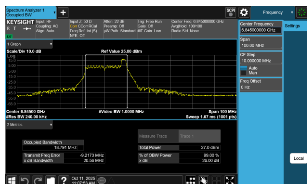
Plot 7-24 26dB BW & 99% OBW Antenna 5T (40MHz BW 802.11be(RU) RU26 Index8 - Ch.179)
