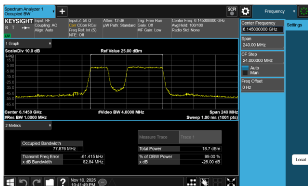
Plot 7-39 26dB BW & 99% OBW Antenna 5T (80MHz BW 802.11be(RU) RU484+242 Index91 - Ch.39)
