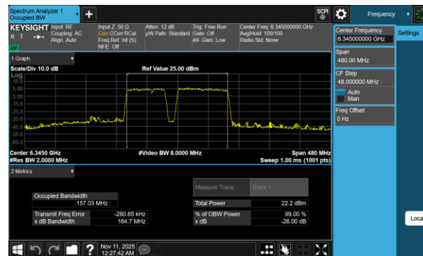
Plot 7-40 26dB BW & 99% OBW Antenna 5T (160MHz BW 802.11be(RU) RU996+484+242 Index99 - Ch.79)
