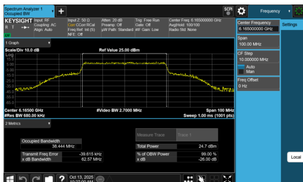
Plot 7-86 26dB BW & 99% OBW Antenna 3b (40MHz BW 802.11be(RU) RU484 Index65 - Ch.43)
