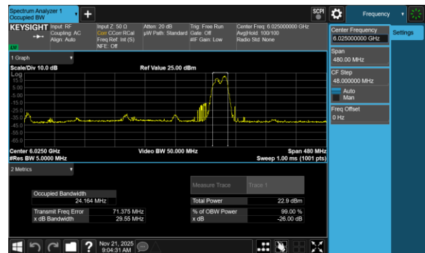
Plot 7-81 26dB BW & 99% OBW Antenna 3b (160MHz BW 802.11be(RU) RU26 Index36 - Ch.15)
