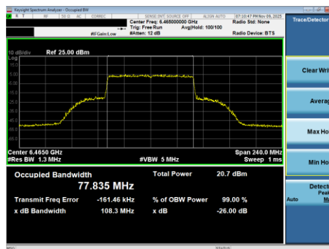
Plot 7-54 26dB BW & 99% OBW Antenna 5T (80MHz BW 802.11be(RU) RU996 Index67 - Ch.103)
