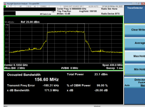
Plot 7-44 26dB BW & 99% OBW Antenna 5T (160MHz BW 802.11be(RU) RU996X2 Index68 - Ch.47)
