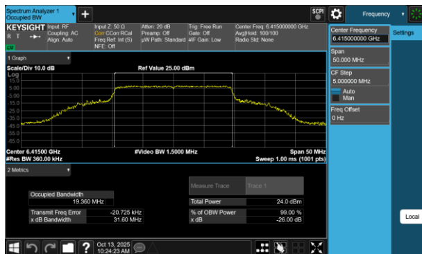
Plot 7-85 26dB BW & 99% OBW Antenna 3b (20MHz BW 802.11be(RU) RU242 Index61 - Ch.93)
