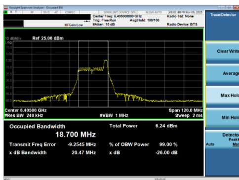
Plot 7-35 26dB BW & 99% OBW Antenna 5T (40MHz BW 802.11be(RU) RU26 Index8 - Ch.91)
