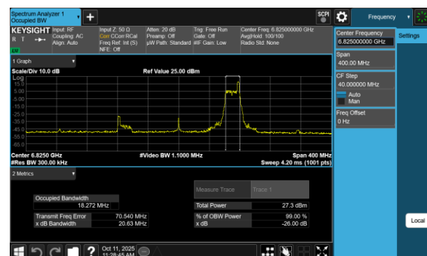
Plot 7-26 26dB BW & 99% OBW Antenna 5T (160MHz BW 802.11be(RU) RU26 Index36 - Ch.175)
