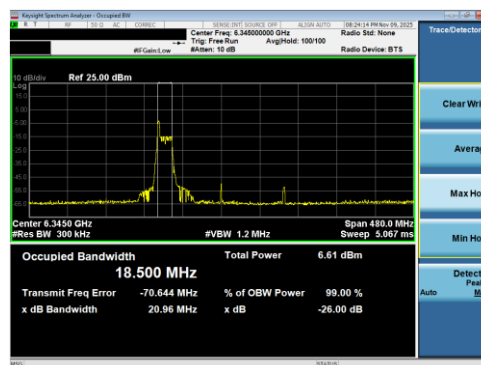
Plot 7-37 26dB BW & 99% OBW Antenna 5T (160MHz BW 802.11be(RU) RU26 Index0 - Ch.79)
