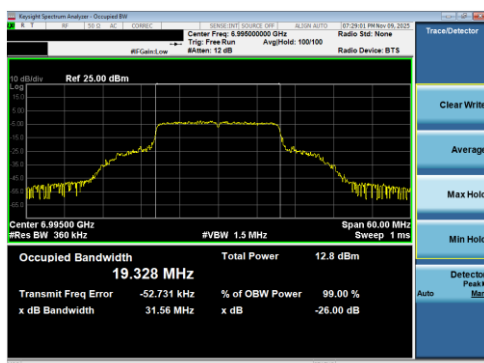
Plot 7-75 26dB BW & 99% OBW Antenna 5T (20MHz BW 802.11be(RU) RU242 Index61 - Ch.209)
