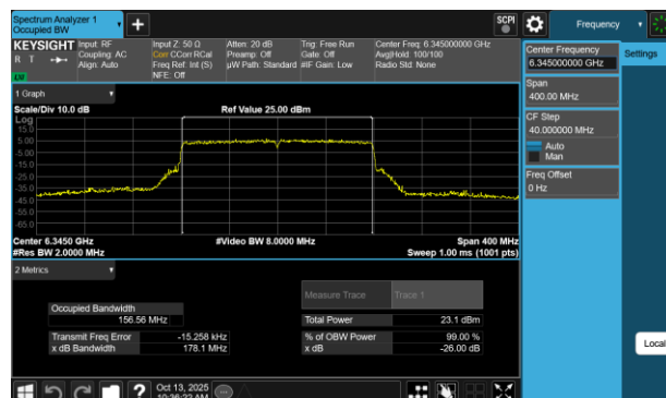
Plot 7-88 26dB BW & 99% OBW Antenna 3b (160MHz BW 802.11be(RU) RU996X2 Index68 - Ch.79)
