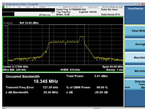
Plot 7-34 26dB BW & 99% OBW Antenna 5T (20MHz BW 802.11be(RU) RU26 Index8 - Ch.45)
