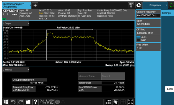
Plot 7-78 26dB BW & 99% OBW Antenna 3b (20MHz BW 802.11be(RU) RU26 Index0 - Ch.93)
