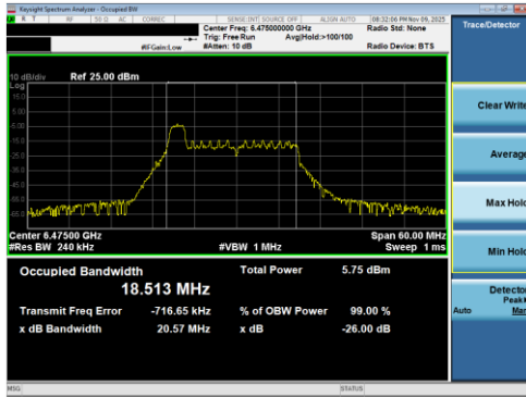
Plot 7-45 26dB BW & 99% OBW Antenna 5T (20MHz BW 802.11be(RU) RU26 Index0 - Ch.105)
