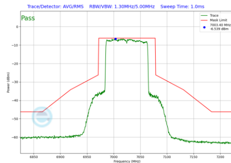
Plot 7-846 In-Band Emission Plot Antenna 5T (80MHz BW 802.11be(RU) RU996 Index67 (UNII Band 8) - Ch.215)
