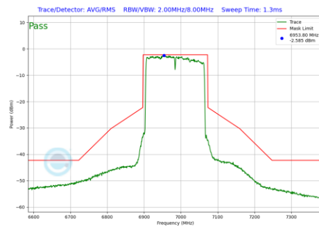
Plot 7-924 In-Band Emission Plot Antenna 3b (160MHz BW 802.11be(RU) RU996X2 Index68 (UNII Band 8) - Ch.207)
