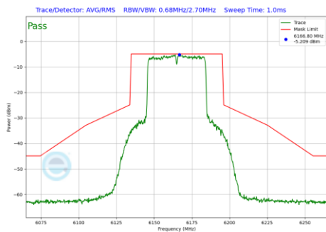
Plot 7-910 In-Band Emission Plot Antenna 3b (40MHz BW 802.11be(RU) RU484 Index65 (UNII Band 5) - Ch.43)
