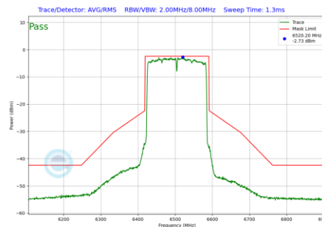
Plot 7-876 In-Band Emission Plot Antenna 3b (160MHz BW 802.11be(RU) RU996X2 Index68 (UNII Band 6) - Ch.111)
