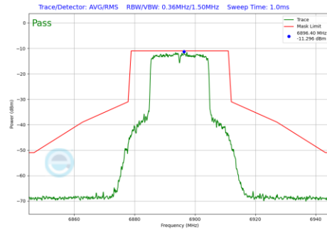
Plot 7-844 In-Band Emission Plot Antenna 5T (20MHz BW 802.11be(RU) RU242 Index61 (UNII Band 8) - Ch.189)
