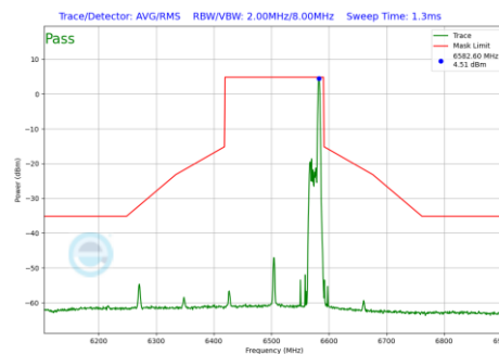
Plot 7-932 In-Band Emission Plot Antenna 1b (160MHz BW 802.11be(RU) RU26 Index36 (UNII Band 6) - Ch.111)
