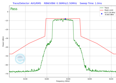
Plot 7-909 In-Band Emission Plot Antenna 3b (20MHz BW 802.11be(RU) RU242 Index61 (UNII Band 5) - Ch.45)
