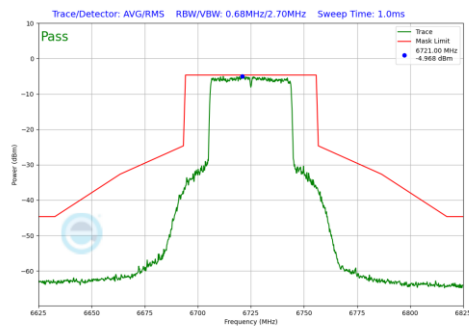
Plot 7-918 In-Band Emission Plot Antenna 3b (40MHz BW 802.11be(RU) RU484 Index65 (UNII Band 7) - Ch.155)
