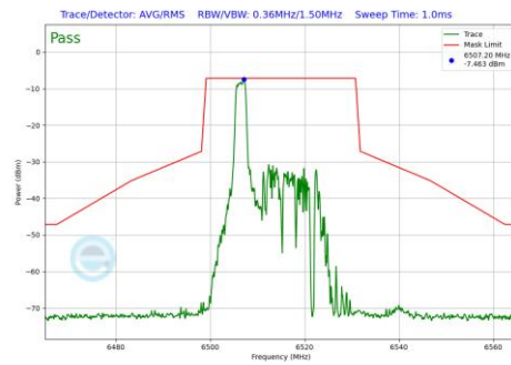
Plot 7-885 In-Band Emission Plot Antenna 3b (20MHz BW 802.11be(RU) RU26 Index0 (UNII Band 6) - Ch.113)
