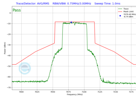
Plot 7-845 In-Band Emission Plot Antenna 5T (40MHz BW 802.11be(RU) RU484 Index65 (UNII Band 8) - Ch.227)
