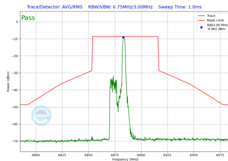
Plot 7-817 In-Band Emission Plot Antenna 5T (40MHz BW 802.11be(RU) RU26 Index8 (UNII Band 8) - Ch.187)
