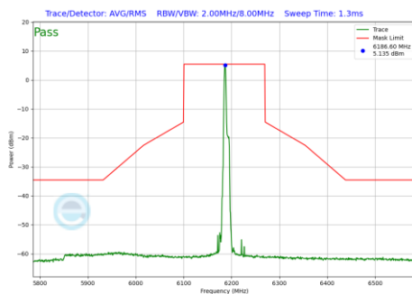
Plot 7-928 In-Band Emission Plot Antenna 1b (160MHz BW 802.11be(RU) RU26 Index0 (UNII Band 5) - Ch.47)
