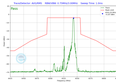
Plot 7-886 In-Band Emission Plot Antenna 3b (40MHz BW 802.11be(RU) RU26 Index17 (UNII Band 6) - Ch.115)
