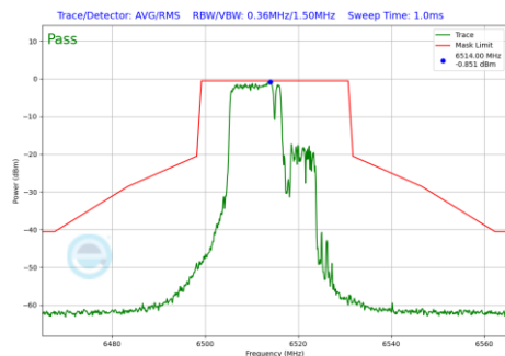
Plot 7-940 In-Band Emission Plot Antenna 1b (20MHz BW 802.11be(RU) RU106+26 Index82 (UNII Band 6) - Ch.113)
