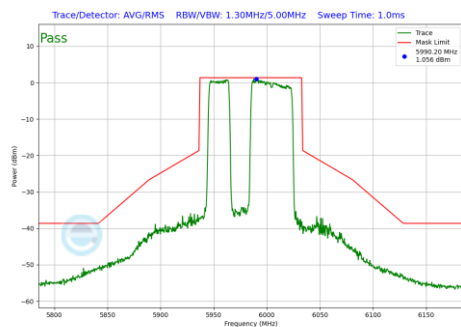
Plot 7-938 In-Band Emission Plot Antenna 1b (80MHz BW 802.11be(RU) RU484+242 Index91 (UNII Band 5) - Ch.7)
