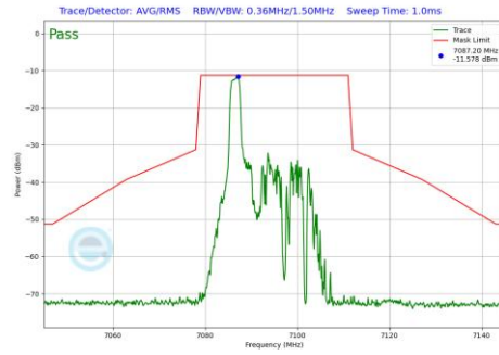
Plot 7-816 In-Band Emission Plot Antenna 5T (20MHz BW 802.11be(RU) RU26 Index0 (UNII Band 8) - Ch.229)
