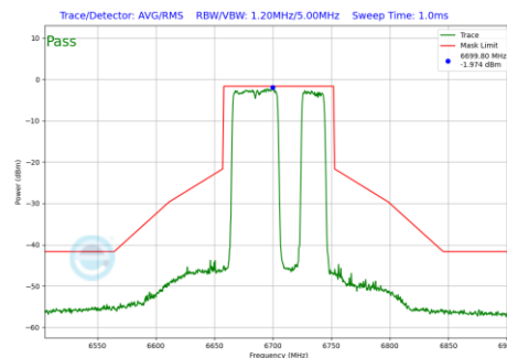
Plot 7-904 In-Band Emission Plot Antenna 3b (80MHz BW 802.11be(RU) RU484+242 Index92 (UNII Band 7) - Ch.151)
