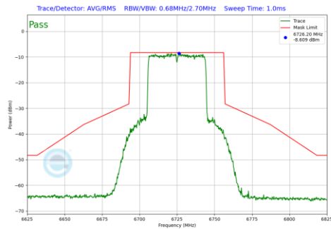
Plot 7-841 In-Band Emission Plot Antenna 5T (40MHz BW 802.11be(RU) RU484 Index65 (UNII Band 7) - Ch.155)
