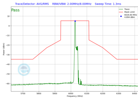
Plot 7-851 In-Band Emission Plot Antenna 3b (160MHz BW 802.11be(RU) RU26 Index0 (UNII Band 5) - Ch.15)
