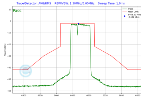
Plot 7-901 In-Band Emission Plot Antenna 3b (80MHz BW 802.11be(RU) RU484+242 Index90 (UNII Band 6) - Ch.103)
