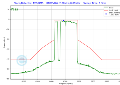
Plot 7-902 In-Band Emission Plot Antenna 3b (160MHz BW 802.11be(RU) RU996+484+242 Index97 (UNII Band 6) - Ch.111)
