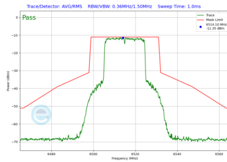
Plot 7-836 In-Band Emission Plot Antenna 5T (20MHz BW 802.11be(RU) RU242 Index61 (UNII Band 6) - Ch.113)
