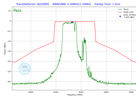
Plot 7-943 In-Band Emission Plot Antenna 1b (20MHz BW 802.11be(RU) RU106+26 Index82 (UNII Band 7) - Ch.117)
