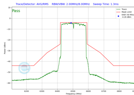
Plot 7-839 In-Band Emission Plot Antenna 5T (160MHz BW 802.11be(RU) RU996X2 Index68 (UNII Band 6) - Ch.111)
