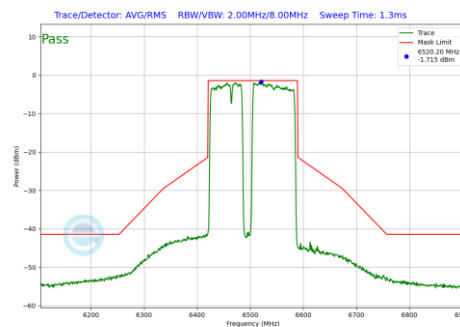
Plot 7-865 In-Band Emission Plot Antenna 3b (160MHz BW 802.11be(RU) RU996+484+242 Index99 (UNII Band 6) - Ch.111)
