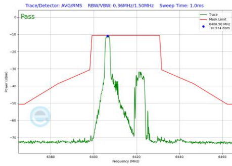
Plot 7-804 In-Band Emission Plot Antenna 5T (20MHz BW 802.11be(RU) RU26 Index0 (UNII Band 5) - Ch.93)
