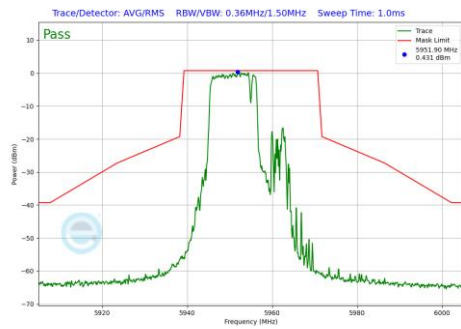
Plot 7-860 In-Band Emission Plot Antenna 3b (20MHz BW 802.11be(RU) RU106+26 Index82 (UNII Band 5) - Ch.1)
