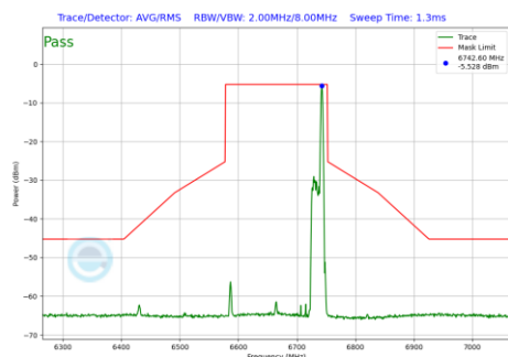
Plot 7-815 In-Band Emission Plot Antenna 5T (160MHz BW 802.11be(RU) RU26 Index36 (UNII Band 7) - Ch.143)
