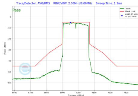
Plot 7-847 In-Band Emission Plot Antenna 5T (160MHz BW 802.11be(RU) RU996X2 Index68 (UNII Band 8) - Ch.207)
