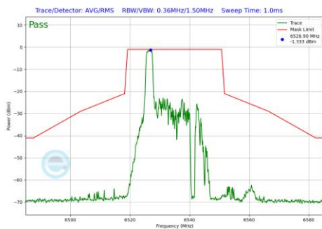
Plot 7-933 In-Band Emission Plot Antenna 1b (20MHz BW 802.11be(RU) RU26 Index0 (UNII Band 7) - Ch.117)
