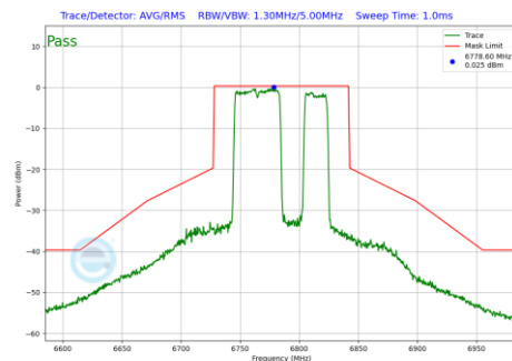
Plot 7-944 In-Band Emission Plot Antenna 1b (80MHz BW 802.11be(RU) RU484+242 Index92 (UNII Band 7) - Ch.167)
