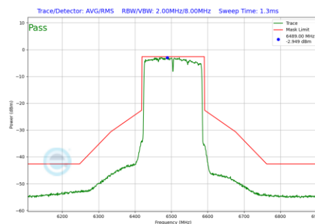
Plot 7-916 In-Band Emission Plot Antenna 3b (160MHz BW 802.11be(RU) RU996X2 Index68 (UNII Band 6) - Ch.111)
