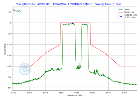
Plot 7-867 In-Band Emission Plot Antenna 3b (80MHz BW 802.11be(RU) RU484+242 Index92 (UNII Band 7) - Ch.119)
