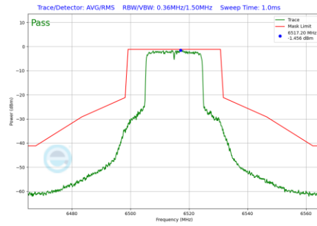
Plot 7-950 In-Band Emission Plot Antenna 1b (20MHz BW 802.11be(RU) RU242 Index61 (UNII Band 6) - Ch.113)
