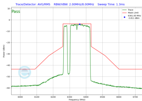
Plot 7-822 In-Band Emission Plot Antenna 5T (160MHz BW 802.11be(RU) RU996+484+242 Index97 (UNII Band 5) - Ch.79)
