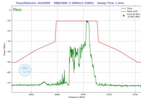
Plot 7-812 In-Band Emission Plot Antenna 5T (20MHz BW 802.11be(RU) RU26 Index8 (UNII Band 7) - Ch.149)
