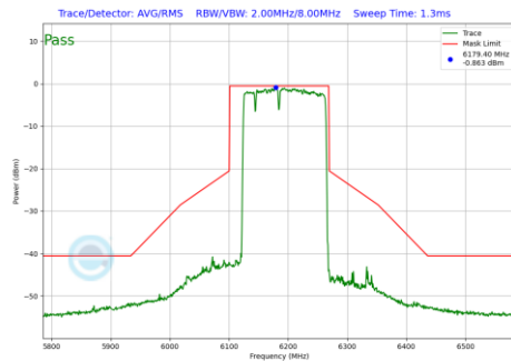
Plot 7-899 In-Band Emission Plot Antenna 3b (160MHz BW 802.11be(RU) RU996+484+242 Index96 (UNII Band 5) - Ch.47)
