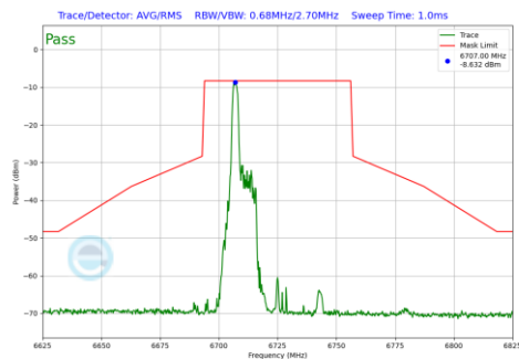
Plot 7-813 In-Band Emission Plot Antenna 5T (40MHz BW 802.11be(RU) RU26 Index0 (UNII Band 7) - Ch.155)
