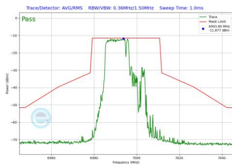
Plot 7-829 In-Band Emission Plot Antenna 5T (20MHz BW 802.11be(RU) RU106+26 Index82 (UNII Band 8) - Ch.209)
