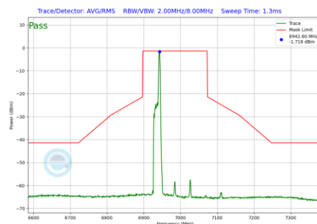
Plot 7-896 In-Band Emission Plot Antenna 3b (160MHz BW 802.11be(RU) RU26 Index17 (UNII Band 8) - Ch.207)
