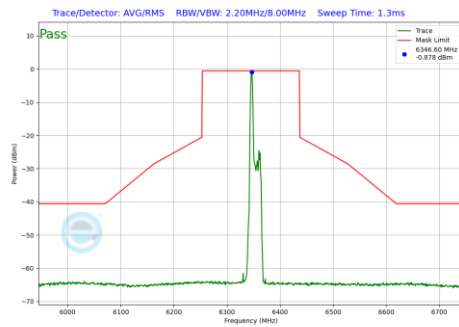
Plot 7-961 In-Band Emission Plot Antenna 1b (160MHz BW 802.11be(RU) RU26 Index0 (UNII Band 5) - Ch.79)
