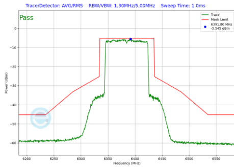
Plot 7-834 In-Band Emission Plot Antenna 5T (80MHz BW 802.11be(RU) RU996 Index67 (UNII Band 5) - Ch.87)
