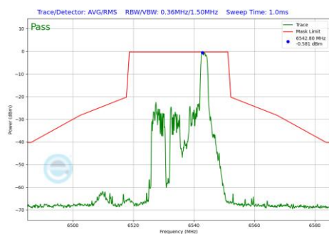
Plot 7-856 In-Band Emission Plot Antenna 3b (20MHz BW 802.11be(RU) RU26 Index8 (UNII Band 7) - Ch.117)
