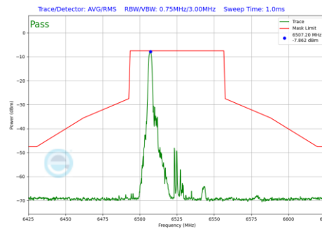
Plot 7-809 In-Band Emission Plot Antenna 5T (40MHz BW 802.11be(RU) RU26 Index0 (UNII Band 6) - Ch.115)
