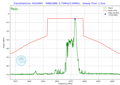
Plot 7-882 In-Band Emission Plot Antenna 3b (40MHz BW 802.11be(RU) RU26 Index17 (UNII Band 5) - Ch.3)
