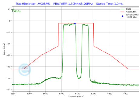
Plot 7-898 In-Band Emission Plot Antenna 3b (80MHz BW 802.11be(RU) RU484+242 Index92 (UNII Band 5) - Ch.39)
