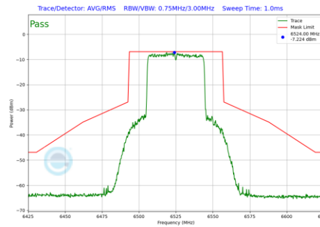
Plot 7-837 In-Band Emission Plot Antenna 5T (40MHz BW 802.11be(RU) RU484 Index65 (UNII Band 6) - Ch.115)
