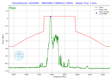
Plot 7-849 In-Band Emission Plot Antenna 3b (40MHz BW 802.11be(RU) RU26 Index0 (UNII Band 5) - Ch.3)
