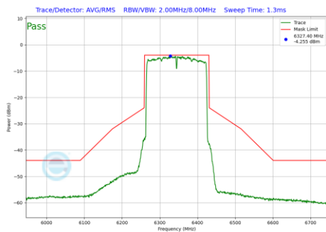
Plot 7-835 In-Band Emission Plot Antenna 5T (160MHz BW 802.11be(RU) RU996X2 Index68 (UNII Band 5) - Ch.79)
