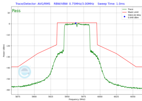
Plot 7-947 In-Band Emission Plot Antenna 1b (40MHz BW 802.11be(RU) RU484 Index65 (UNII Band 5) - Ch.3)
