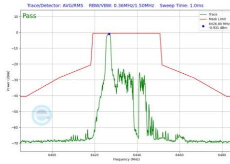
Plot 7-929 In-Band Emission Plot Antenna 1b (20MHz BW 802.11be(RU) RU26 Index0 (UNII Band 6) - Ch.97)
