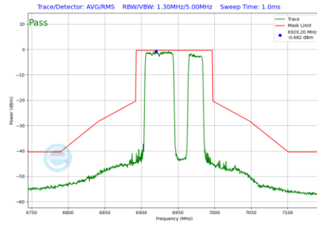
Plot 7-907 In-Band Emission Plot Antenna 3b (80MHz BW 802.11be(RU) RU484+242 Index92 (UNII Band 8) - Ch.199)
