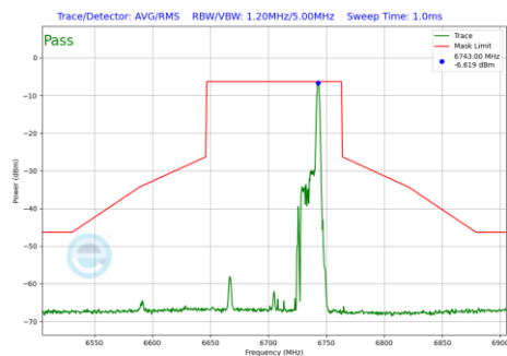
Plot 7-814 In-Band Emission Plot Antenna 5T (80MHz BW 802.11be(RU) RU26 Index36 (UNII Band 7) - Ch.151)
