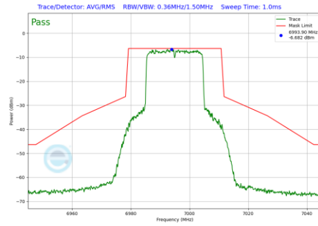
Plot 7-921 In-Band Emission Plot Antenna 3b (20MHz BW 802.11be(RU) RU242 Index61 (UNII Band 8) - Ch.209)
