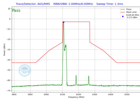
Plot 7-884 In-Band Emission Plot Antenna 3b (160MHz BW 802.11be(RU) RU26 Index0 (UNII Band 5) - Ch.47)
