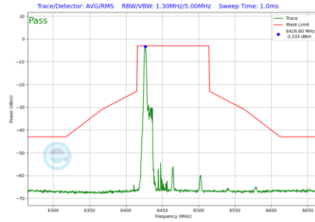
Plot 7-964 In-Band Emission Plot Antenna 1b (80MHz BW 802.11be(RU) RU26 Index0 (UNII Band 6) - Ch.103)
