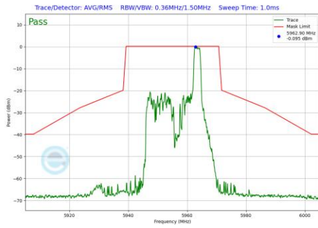
Plot 7-848 In-Band Emission Plot Antenna 3b (20MHz BW 802.11be(RU) RU26 Index8 (UNII Band 5) - Ch.1)
