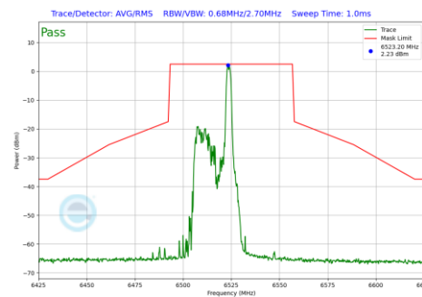
Plot 7-853 In-Band Emission Plot Antenna 3b (40MHz BW 802.11be(RU) RU26 Index8 (UNII Band 6) - Ch.115)
