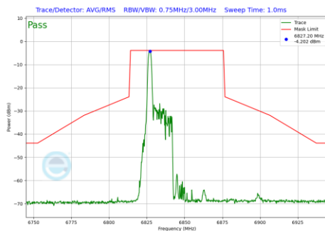
Plot 7-890 In-Band Emission Plot Antenna 3b (40MHz BW 802.11be(RU) RU26 Index0 (UNII Band 7) - Ch.179)
