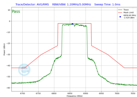
Plot 7-919 In-Band Emission Plot Antenna 3b (80MHz BW 802.11be(RU) RU996 Index67 (UNII Band 7) - Ch.183)
