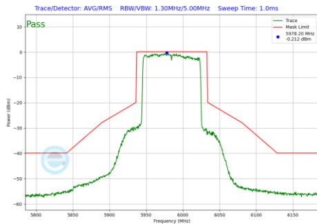
Plot 7-948 In-Band Emission Plot Antenna 1b (80MHz BW 802.11be(RU) RU996 Index67 (UNII Band 5) - Ch.7)
