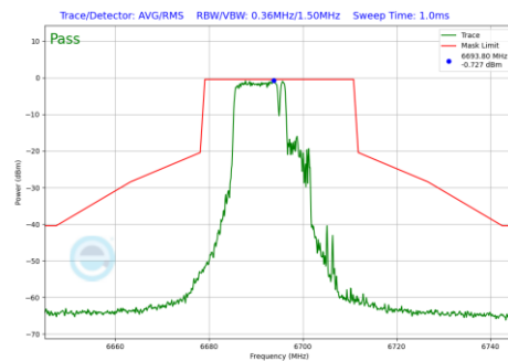
Plot 7-866 In-Band Emission Plot Antenna 3b (20MHz BW 802.11be(RU) RU106+26 Index82 (UNII Band 7) - Ch.149)
