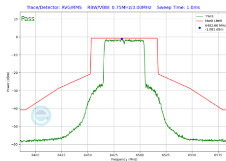
Plot 7-874 In-Band Emission Plot Antenna 3b (40MHz BW 802.11be(RU) RU484 Index65 (UNII Band 6) - Ch.107)
