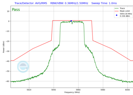
Plot 7-946 In-Band Emission Plot Antenna 1b (20MHz BW 802.11be(RU) RU242 Index61 (UNII Band 5) - Ch.1)
