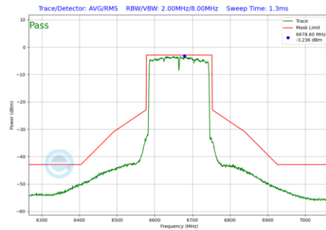
Plot 7-957 In-Band Emission Plot Antenna 1b (160MHz BW 802.11be(RU) RU996X2 Index68 (UNII Band 7) - Ch.143)
