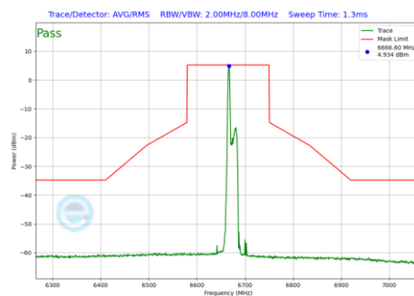
Plot 7-859 In-Band Emission Plot Antenna 3b (160MHz BW 802.11be(RU) RU26 Index0 (UNII Band 7) - Ch.143)
