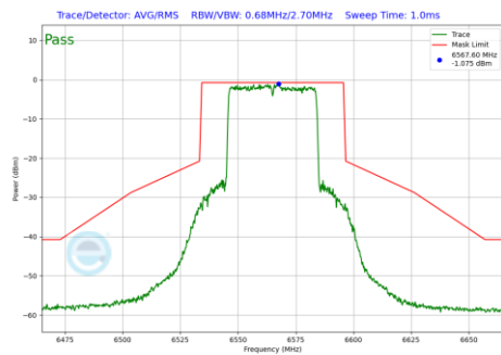
Plot 7-878 In-Band Emission Plot Antenna 3b (40MHz BW 802.11be(RU) RU484 Index65 (UNII Band 7) - Ch.123)
