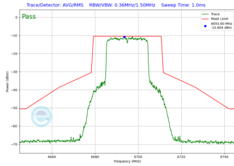
Plot 7-840 In-Band Emission Plot Antenna 5T (20MHz BW 802.11be(RU) RU242 Index61 (UNII Band 7) - Ch.149)
