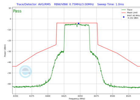
Plot 7-914 In-Band Emission Plot Antenna 3b (40MHz BW 802.11be(RU) RU484 Index65 (UNII Band 6) - Ch.99)
