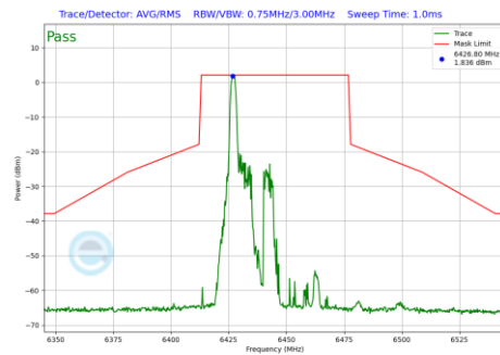
Plot 7-930 In-Band Emission Plot Antenna 1b (40MHz BW 802.11be(RU) RU26 Index0 (UNII Band 6) - Ch.99)
