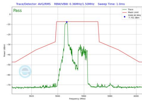
Plot 7-881 In-Band Emission Plot Antenna 3b (20MHz BW 802.11be(RU) RU26 Index0 (UNII Band 5) - Ch.1)
