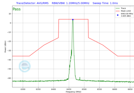
Plot 7-854 In-Band Emission Plot Antenna 3b (80MHz BW 802.11be(RU) RU26 Index17 (UNII Band 6) - Ch.103)
