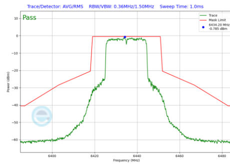
Plot 7-873 In-Band Emission Plot Antenna 3b (20MHz BW 802.11be(RU) RU242 Index61 (UNII Band 6) - Ch.97)
