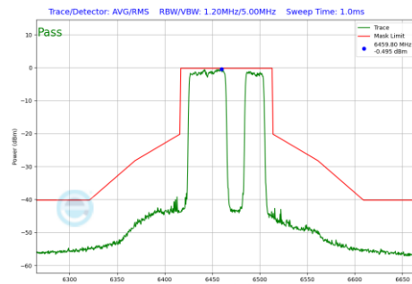
Plot 7-864 In-Band Emission Plot Antenna 3b (80MHz BW 802.11be(RU) RU484+242 Index92 (UNII Band 6) - Ch.103)
