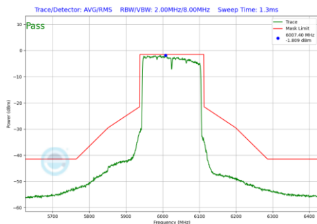
Plot 7-949 In-Band Emission Plot Antenna 1b (160MHz BW 802.11be(RU) RU996X2 Index68 (UNII Band 5) - Ch.15)
