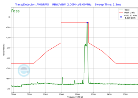
Plot 7-807 In-Band Emission Plot Antenna 5T (160MHz BW 802.11be(RU) RU26 Index36 (UNII Band 5) - Ch.47)
