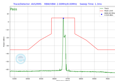
Plot 7-936 In-Band Emission Plot Antenna 1b (160MHz BW 802.11be(RU) RU26 Index0 (UNII Band 7) - Ch.143)
