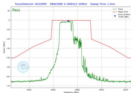
Plot 7-863 In-Band Emission Plot Antenna 3b (20MHz BW 802.11be(RU) RU106+26 Index82 (UNII Band 6) - Ch.105)
