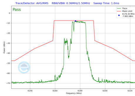
Plot 7-897 In-Band Emission Plot Antenna 3b (20MHz BW 802.11be(RU) RU106+26 Index83 (UNII Band 5) - Ch.45)
