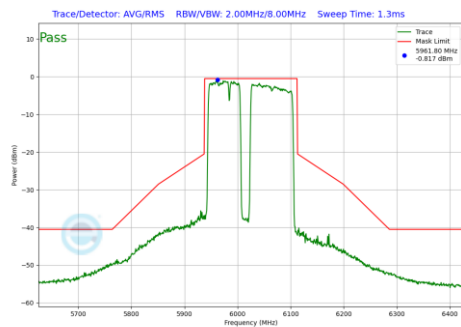
Plot 7-939 In-Band Emission Plot Antenna 1b (160MHz BW 802.11be(RU) RU996+484+242 Index99 (UNII Band 5) - Ch.15)
