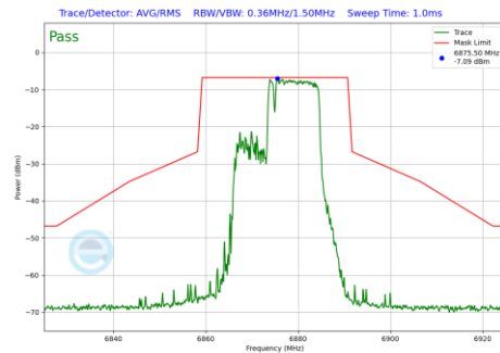
Plot 7-903 In-Band Emission Plot Antenna 3b (20MHz BW 802.11be(RU) RU106+26 Index83 (UNII Band 7) - Ch.185)
