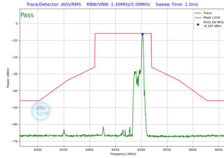
Plot 7-810 In-Band Emission Plot Antenna 5T (80MHz BW 802.11be(RU) RU26 Index36 (UNII Band 6) - Ch.103)
