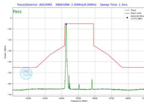
Plot 7-811 In-Band Emission Plot Antenna 5T (160MHz BW 802.11be(RU) RU26 Index0 (UNII Band 6) - Ch.111)
