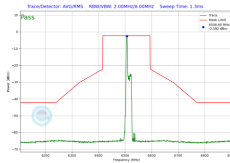
Plot 7-965 In-Band Emission Plot Antenna 1b (160MHz BW 802.11be(RU) RU26 Index0 (UNII Band 6) - Ch.111)
