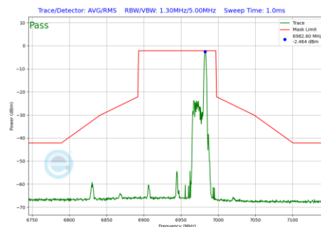
Plot 7-895 In-Band Emission Plot Antenna 3b (80MHz BW 802.11be(RU) RU26 Index36 (UNII Band 8) - Ch.199)
