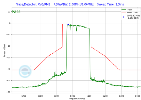
Plot 7-862 In-Band Emission Plot Antenna 3b (160MHz BW 802.11be(RU) RU996+484+242 Index96 (UNII Band 5) - Ch.15)
