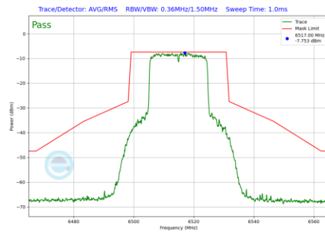
Plot 7-913 In-Band Emission Plot Antenna 3b (20MHz BW 802.11be(RU) RU242 Index61 (UNII Band 6) - Ch.113)
