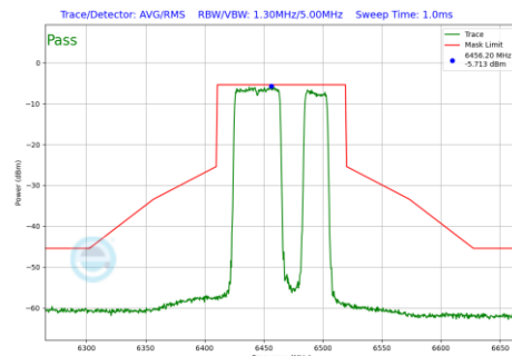
Plot 7-824 In-Band Emission Plot Antenna 5T (80MHz BW 802.11be(RU) RU484+242 Index92 (UNII Band 6) - Ch.103)
