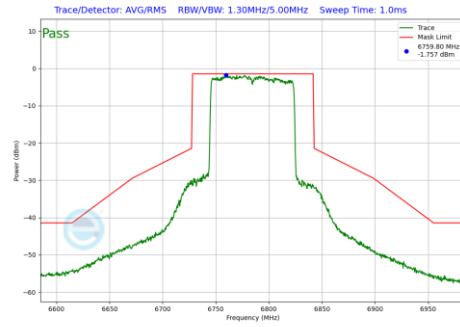
Plot 7-956 In-Band Emission Plot Antenna 1b (80MHz BW 802.11be(RU) RU996 Index67 (UNII Band 7) - Ch.167)
