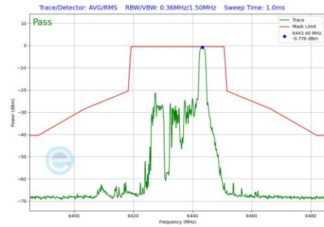
Plot 7-852 In-Band Emission Plot Antenna 3b (20MHz BW 802.11be(RU) RU26 Index8 (UNII Band 6) - Ch.97)
