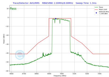
Plot 7-908 In-Band Emission Plot Antenna 3b (160MHz BW 802.11be(RU) RU996+484+242 Index96 (UNII Band 8) - Ch.207)
