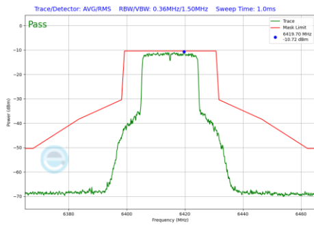
Plot 7-832 In-Band Emission Plot Antenna 5T (20MHz BW 802.11be(RU) RU242 Index61 (UNII Band 5) - Ch.93)
