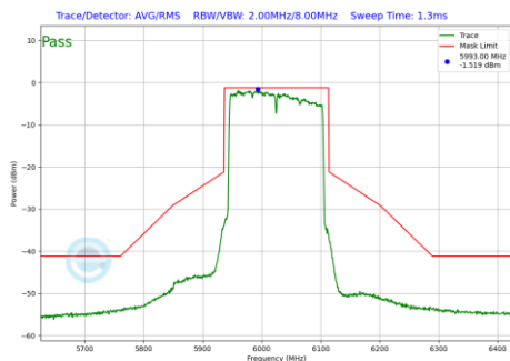
Plot 7-872 In-Band Emission Plot Antenna 3b (160MHz BW 802.11be(RU) RU996X2 Index68 (UNII Band 5) - Ch.15)
