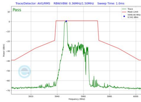
Plot 7-925 In-Band Emission Plot Antenna 1b (20MHz BW 802.11be(RU) RU26 Index0 (UNII Band 5) - Ch.1)
