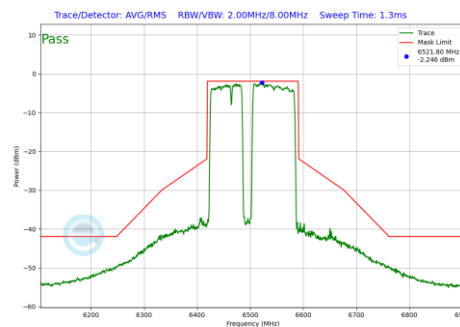
Plot 7-942 In-Band Emission Plot Antenna 1b (160MHz BW 802.11be(RU) RU996+484+242 Index99 (UNII Band 6) - Ch.111)
