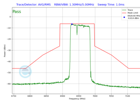
Plot 7-830 In-Band Emission Plot Antenna 5T (80MHz BW 802.11be(RU) RU484+242 Index90 (UNII Band 8) - Ch.199)
