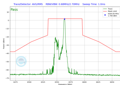
Plot 7-857 In-Band Emission Plot Antenna 3b (40MHz BW 802.11be(RU) RU26 Index8 (UNII Band 7) - Ch.123)
