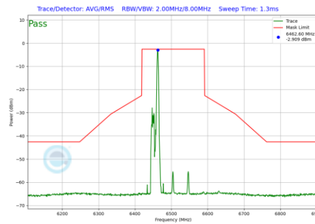
Plot 7-888 In-Band Emission Plot Antenna 3b (160MHz BW 802.11be(RU) RU26 Index17 (UNII Band 6) - Ch.111)
