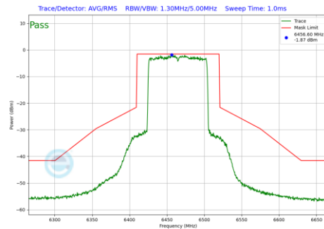
Plot 7-952 In-Band Emission Plot Antenna 1b (80MHz BW 802.11be(RU) RU996 Index67 (UNII Band 6) - Ch.103)
