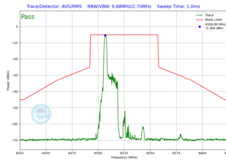
Plot 7-963 In-Band Emission Plot Antenna 1b (40MHz BW 802.11be(RU) RU26 Index0 (UNII Band 6) - Ch.115)
