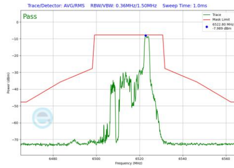
Plot 7-962 In-Band Emission Plot Antenna 1b (20MHz BW 802.11be(RU) RU26 Index8 (UNII Band 6) - Ch.113)
