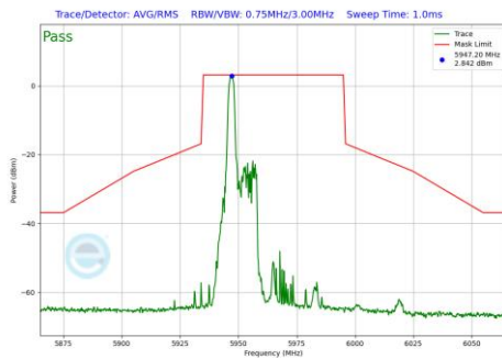
Plot 7-926 In-Band Emission Plot Antenna 1b (40MHz BW 802.11be(RU) RU26 Index0 (UNII Band 5) - Ch.3)
