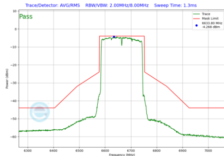
Plot 7-843 In-Band Emission Plot Antenna 5T (160MHz BW 802.11be(RU) RU996X2 Index68 (UNII Band 7) - Ch.143)
