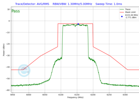
Plot 7-911 In-Band Emission Plot Antenna 3b (80MHz BW 802.11be(RU) RU996 Index67 (UNII Band 5) - Ch.39)
