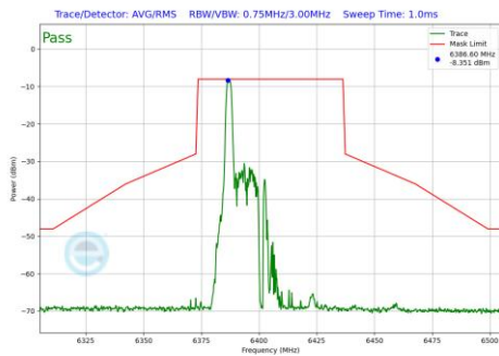
Plot 7-805 In-Band Emission Plot Antenna 5T (40MHz BW 802.11be(RU) RU26 Index0 (UNII Band 5) - Ch.91)
