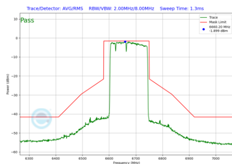
Plot 7-868 In-Band Emission Plot Antenna 3b (160MHz BW 802.11be(RU) RU996+484+242 Index96 (UNII Band 7) - Ch.143)
