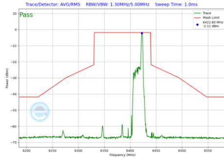
Plot 7-960 In-Band Emission Plot Antenna 1b (80MHz BW 802.11be(RU) RU26 Index36 (UNII Band 5) - Ch.87)
