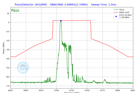
Plot 7-934 In-Band Emission Plot Antenna 1b (40MHz BW 802.11be(RU) RU26 Index0 (UNII Band 7) - Ch.155)
