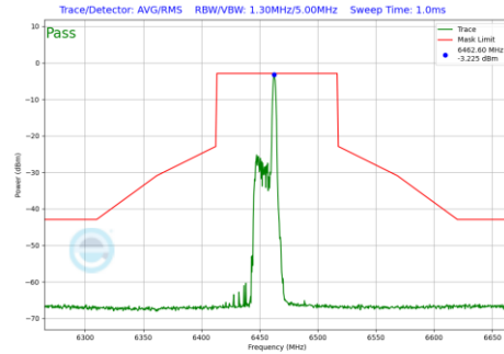
Plot 7-887 In-Band Emission Plot Antenna 3b (80MHz BW 802.11be(RU) RU26 Index17 (UNII Band 6) - Ch.103)
