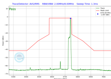
Plot 7-892 In-Band Emission Plot Antenna 3b (160MHz BW 802.11be(RU) RU26 Index36 (UNII Band 7) - Ch.143)
