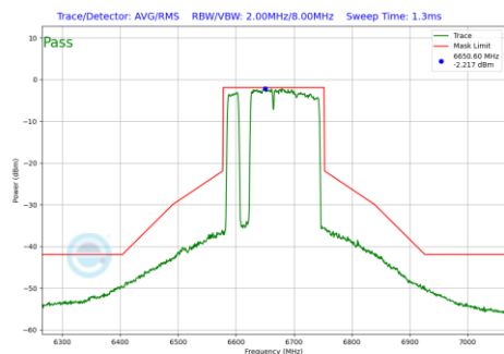
Plot 7-945 In-Band Emission Plot Antenna 1b (160MHz BW 802.11be(RU) RU996+484+242 Index97 (UNII Band 7) - Ch.143)
