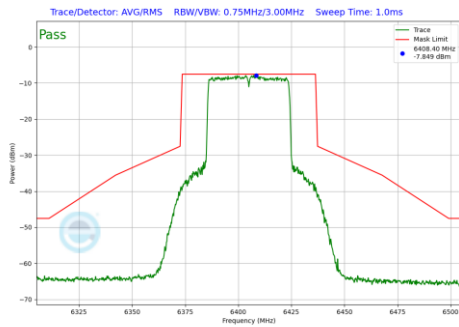
Plot 7-833 In-Band Emission Plot Antenna 5T (40MHz BW 802.11be(RU) RU484 Index65 (UNII Band 5) - Ch.91)
