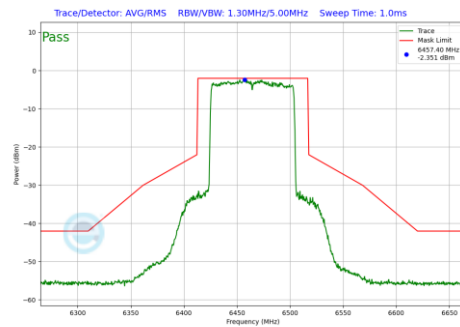
Plot 7-915 In-Band Emission Plot Antenna 3b (80MHz BW 802.11be(RU) RU996 Index67 (UNII Band 6) - Ch.103)
