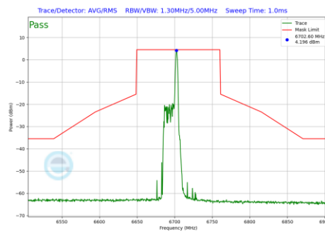
Plot 7-935 In-Band Emission Plot Antenna 1b (80MHz BW 802.11be(RU) RU26 Index17 (UNII Band 7) - Ch.151)
