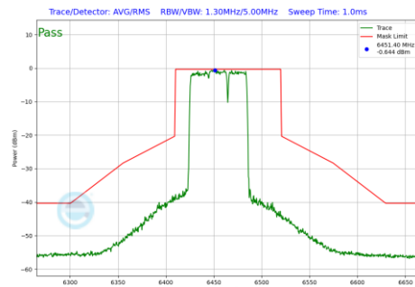
Plot 7-941 In-Band Emission Plot Antenna 1b (80MHz BW 802.11be(RU) RU484+242 Index93 (UNII Band 6) - Ch.103)
