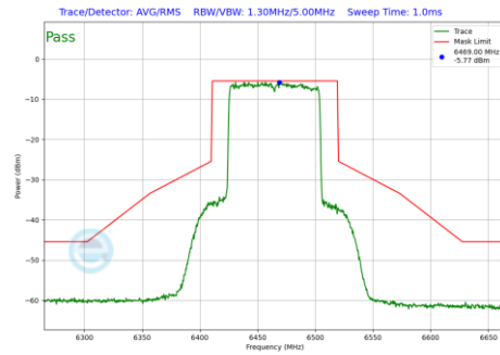
Plot 7-838 In-Band Emission Plot Antenna 5T (80MHz BW 802.11be(RU) RU996 Index67 (UNII Band 6) - Ch.103)
