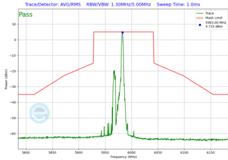
Plot 7-850 In-Band Emission Plot Antenna 3b (80MHz BW 802.11be(RU) RU26 Index17 (UNII Band 5) - Ch.7)
