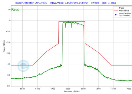
Plot 7-905 In-Band Emission Plot Antenna 3b (160MHz BW 802.11be(RU) RU996+484+242 Index96 (UNII Band 7) - Ch.175)
