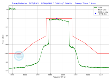
Plot 7-871 In-Band Emission Plot Antenna 3b (80MHz BW 802.11be(RU) RU996 Index67 (UNII Band 5) - Ch.7)
