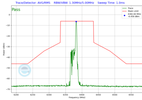
Plot 7-806 In-Band Emission Plot Antenna 5T (80MHz BW 802.11be(RU) RU26 Index17 (UNII Band 5) - Ch.87)
