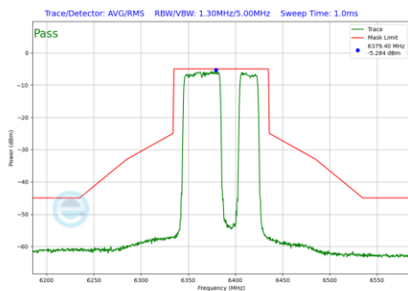
Plot 7-821 In-Band Emission Plot Antenna 5T (80MHz BW 802.11be(RU) RU484+242 Index92 (UNII Band 5) - Ch.87)
