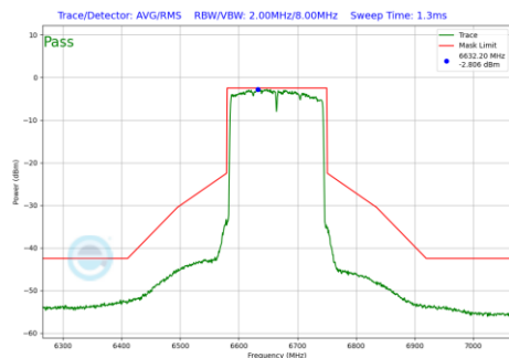
Plot 7-880 In-Band Emission Plot Antenna 3b (160MHz BW 802.11be(RU) RU996X2 Index68 (UNII Band 7) - Ch.143)
