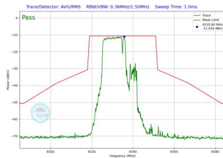
Plot 7-826 In-Band Emission Plot Antenna 5T (20MHz BW 802.11be(RU) RU106+26 Index82 (UNII Band 7) - Ch.117)
