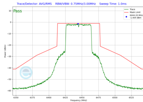
Plot 7-951 In-Band Emission Plot Antenna 1b (40MHz BW 802.11be(RU) RU484 Index65 (UNII Band 6) - Ch.99)
