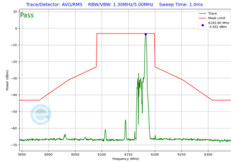
Plot 7-883 In-Band Emission Plot Antenna 3b (80MHz BW 802.11be(RU) RU26 Index36 (UNII Band 5) - Ch.39)
