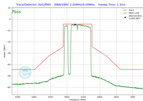
Plot 7-828 In-Band Emission Plot Antenna 5T (160MHz BW 802.11be(RU) RU996+484+242 Index97 (UNII Band 7) - Ch.143)
