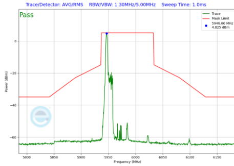
Plot 7-927 In-Band Emission Plot Antenna 1b (80MHz BW 802.11be(RU) RU26 Index0 (UNII Band 5) - Ch.7)
