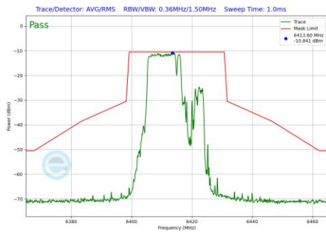
Plot 7-820 In-Band Emission Plot Antenna 5T (20MHz BW 802.11be(RU) RU106+26 Index82 (UNII Band 5) - Ch.93)
