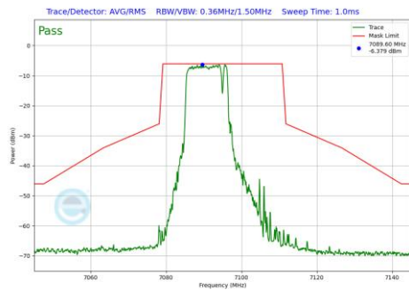
Plot 7-906 In-Band Emission Plot Antenna 3b (20MHz BW 802.11be(RU) RU106+26 Index82 (UNII Band 8) - Ch.229)
