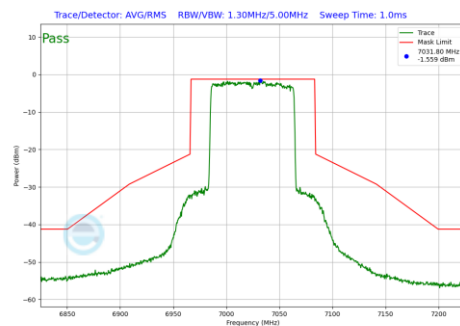
Plot 7-923 In-Band Emission Plot Antenna 3b (80MHz BW 802.11be(RU) RU996 Index67 (UNII Band 8) - Ch.215)
