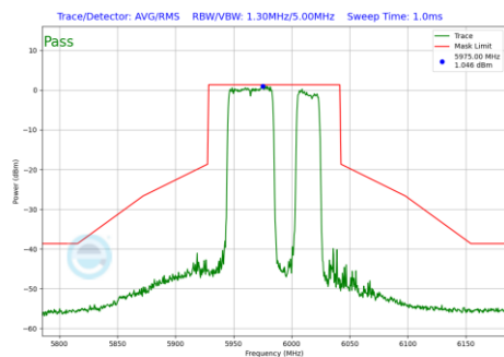
Plot 7-861 In-Band Emission Plot Antenna 3b (80MHz BW 802.11be(RU) RU484+242 Index92 (UNII Band 5) - Ch.7)
