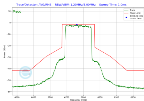
Plot 7-879 In-Band Emission Plot Antenna 3b (80MHz BW 802.11be(RU) RU996 Index67 (UNII Band 7) - Ch.167)
