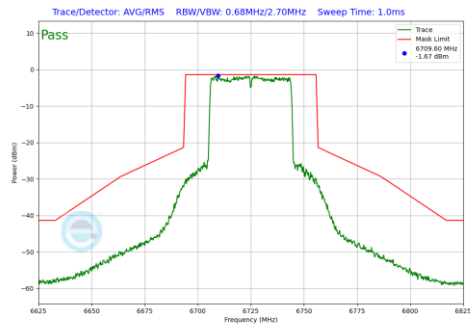
Plot 7-955 In-Band Emission Plot Antenna 1b (40MHz BW 802.11be(RU) RU484 Index65 (UNII Band 7) - Ch.155)
