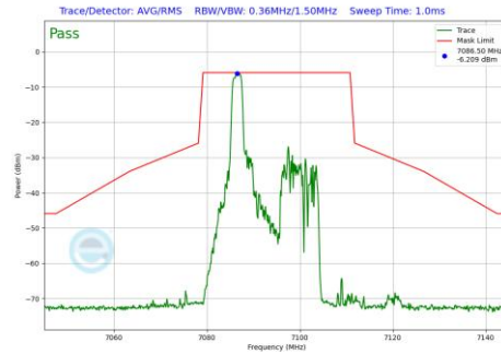
Plot 7-893 In-Band Emission Plot Antenna 3b (20MHz BW 802.11be(RU) RU26 Index0 (UNII Band 8) - Ch.229)
