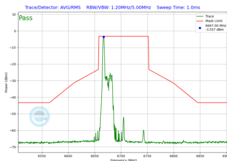
Plot 7-891 In-Band Emission Plot Antenna 3b (80MHz BW 802.11be(RU) RU26 Index0 (UNII Band 7) - Ch.151)
