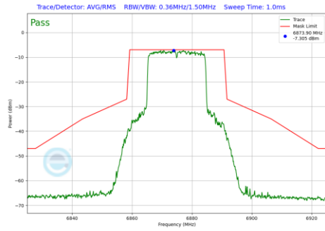
Plot 7-917 In-Band Emission Plot Antenna 3b (20MHz BW 802.11be(RU) RU242 Index61 (UNII Band 7) - Ch.185)
