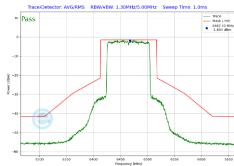
Plot 7-875 In-Band Emission Plot Antenna 3b (80MHz BW 802.11be(RU) RU996 Index67 (UNII Band 6) - Ch.103)
