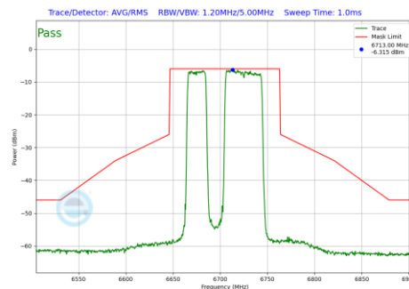
Plot 7-827 In-Band Emission Plot Antenna 5T (80MHz BW 802.11be(RU) RU484+242 Index91 (UNII Band 7) - Ch.151)
