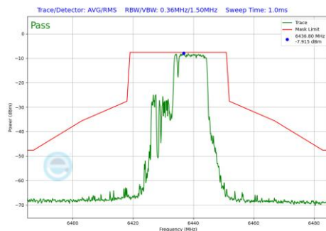
Plot 7-900 In-Band Emission Plot Antenna 3b (20MHz BW 802.11be(RU) RU106+26 Index83 (UNII Band 6) - Ch.97)
