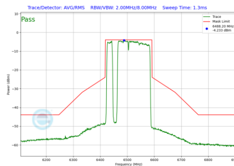
Plot 7-825 In-Band Emission Plot Antenna 5T (160MHz BW 802.11be(RU) RU996+484+242 Index97 (UNII Band 6) - Ch.111)
