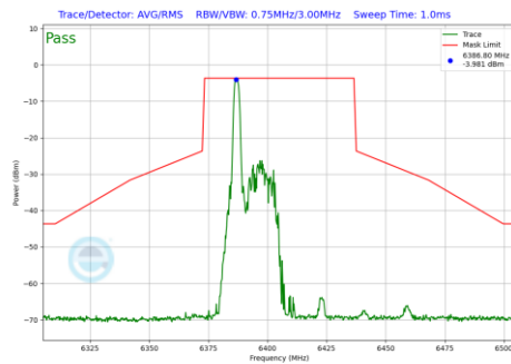
Plot 7-959 In-Band Emission Plot Antenna 1b (40MHz BW 802.11be(RU) RU26 Index0 (UNII Band 5) - Ch.91)
