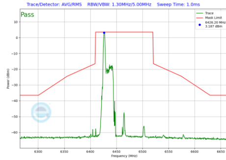
Plot 7-931 In-Band Emission Plot Antenna 1b (80MHz BW 802.11be(RU) RU26 Index0 (UNII Band 6) - Ch.103)
