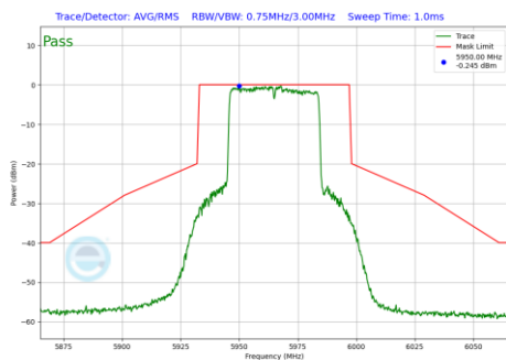
Plot 7-870 In-Band Emission Plot Antenna 3b (40MHz BW 802.11be(RU) RU484 Index65 (UNII Band 5) - Ch.3)
