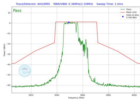
Plot 7-937 In-Band Emission Plot Antenna 1b (20MHz BW 802.11be(RU) RU106+26 Index82 (UNII Band 5) - Ch.1)
