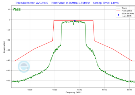
Plot 7-954 In-Band Emission Plot Antenna 1b (20MHz BW 802.11be(RU) RU242 Index61 (UNII Band 7) - Ch.117)
