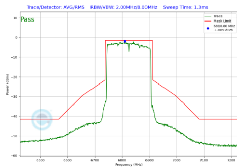
Plot 7-920 In-Band Emission Plot Antenna 3b (160MHz BW 802.11be(RU) RU996X2 Index68 (UNII Band 7) - Ch.175)
