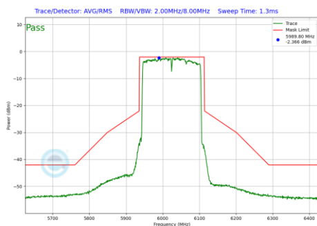
Plot 7-912 In-Band Emission Plot Antenna 3b (160MHz BW 802.11be(RU) RU996X2 Index68 (UNII Band 5) - Ch.15)
