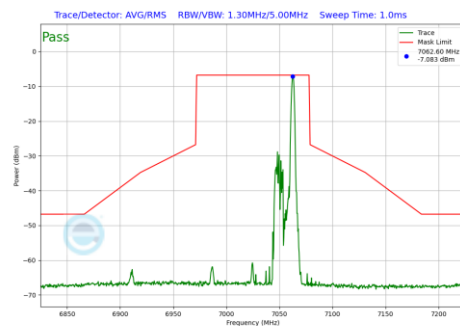
Plot 7-818 In-Band Emission Plot Antenna 5T (80MHz BW 802.11be(RU) RU26 Index36 (UNII Band 8) - Ch.215)
