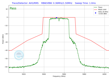
Plot 7-869 In-Band Emission Plot Antenna 3b (20MHz BW 802.11be(RU) RU242 Index61 (UNII Band 5) - Ch.1)
