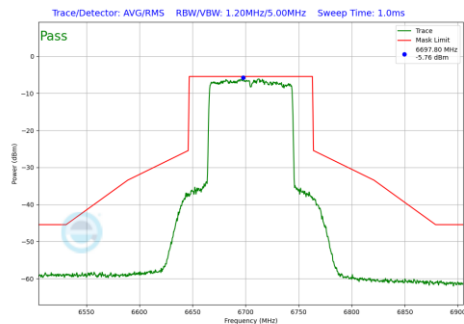
Plot 7-842 In-Band Emission Plot Antenna 5T (80MHz BW 802.11be(RU) RU996 Index67 (UNII Band 7) - Ch.151)
