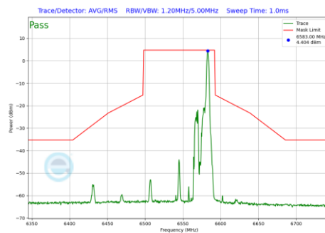
Plot 7-858 In-Band Emission Plot Antenna 3b (80MHz BW 802.11be(RU) RU26 Index36 (UNII Band 7) - Ch.119)
