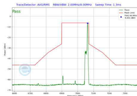
Plot 7-819 In-Band Emission Plot Antenna 5T (160MHz BW 802.11be(RU) RU26 Index36 (UNII Band 8) - Ch.207)
