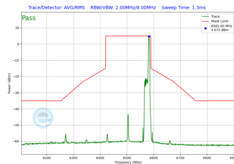
Plot 7-855 In-Band Emission Plot Antenna 3b (160MHz BW 802.11be(RU) RU26 Index36 (UNII Band 6) - Ch.111)
