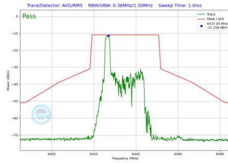
Plot 7-808 In-Band Emission Plot Antenna 5T (20MHz BW 802.11be(RU) RU26 Index0 (UNII Band 6) - Ch.97)
