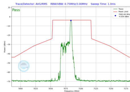
Plot 7-894 In-Band Emission Plot Antenna 3b (40MHz BW 802.11be(RU) RU26 Index8 (UNII Band 8) - Ch.227)
