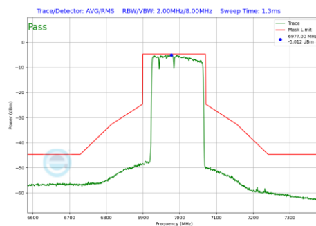
Plot 7-831 In-Band Emission Plot Antenna 5T (160MHz BW 802.11be(RU) RU996+484+242 Index96 (UNII Band 8) - Ch.207)
