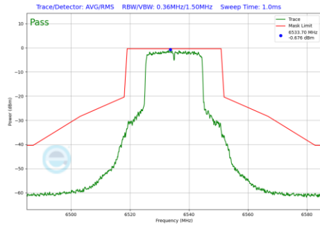
Plot 7-877 In-Band Emission Plot Antenna 3b (20MHz BW 802.11be(RU) RU242 Index61 (UNII Band 7) - Ch.117)
