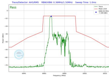
Plot 7-889 In-Band Emission Plot Antenna 3b (20MHz BW 802.11be(RU) RU26 Index0 (UNII Band 7) - Ch.185)
