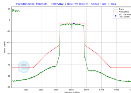
Plot 7-953 In-Band Emission Plot Antenna 1b (160MHz BW 802.11be(RU) RU996X2 Index68 (UNII Band 6) - Ch.111)
