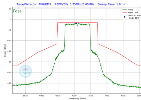
Plot 7-922 In-Band Emission Plot Antenna 3b (40MHz BW 802.11be(RU) RU484 Index65 (UNII Band 8) - Ch.211)
