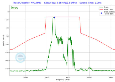
Plot 7-958 In-Band Emission Plot Antenna 1b (20MHz BW 802.11be(RU) RU26 Index0 (UNII Band 5) - Ch.93)
