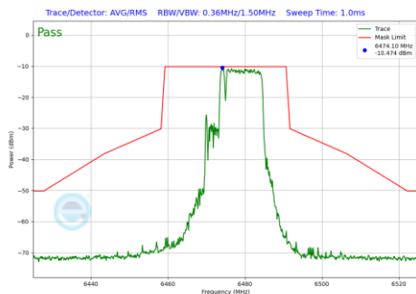
Plot 7-823 In-Band Emission Plot Antenna 5T (20MHz BW 802.11be(RU) RU106+26 Index83 (UNII Band 6) - Ch.105)
