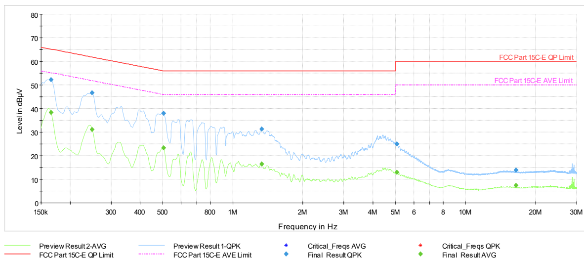
Plot 7-1171. AC Line Conducted Plot with 11be UNII Band 5 SDM Diversity – RU52 – Ch.61 (N) with AC/DC Adapter
