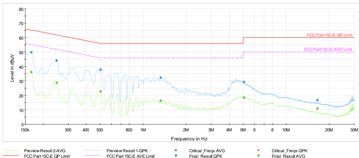
Plot 7-1168. AC Line Conducted Plot with 11be UNII Band 5 SDM Primary – RU242 – Ch.61 (L1) with AC/DC Adapter
