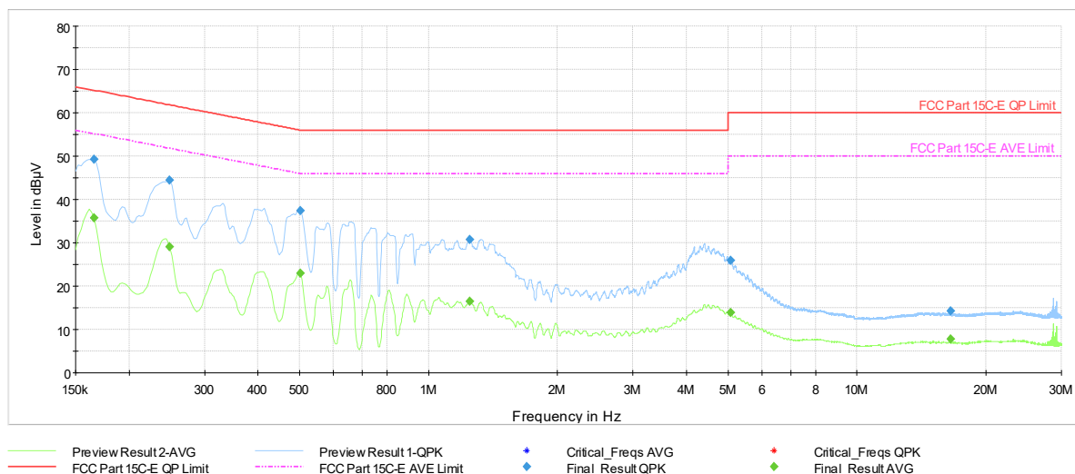
Plot 7-1169. AC Line Conducted Plot with 11be UNII Band 5 SDM Primary – RU242 – Ch.61 (N) with AC/DC Adapter
