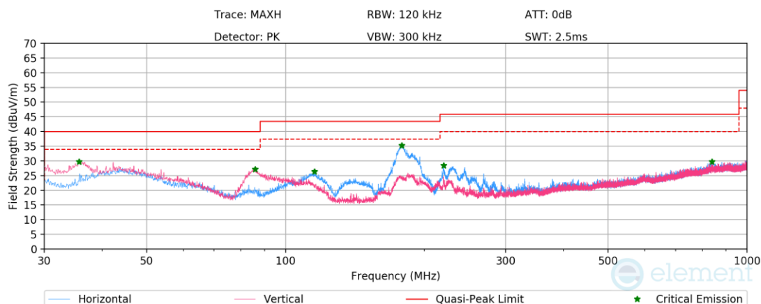
Plot 7-1162. Radiated Spurious Emissions below 1GHz SDM Primary (802.11be – Ch.61 – RU52) with AC/DC Adapter
