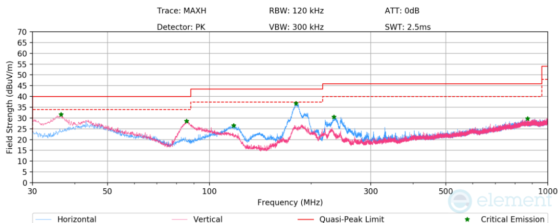
Plot 7-1164. Radiated Spurious Emissions below 1GHz SDM Diversity (802.11be – Ch.61 – RU52) with AC/DC Adapter
