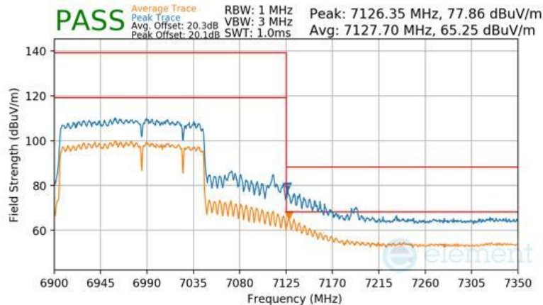
Plot 7-1159 SDM Diversity Radiated Upper Band Edge (Peak & Average – UNII Band 8) - RU996+484+242 (H)
