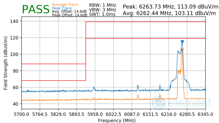
Plot 7-1133 SDM Diversity Radiated Lower Band Edge (Peak & Average – UNII Band 5) – RU52 (H)
