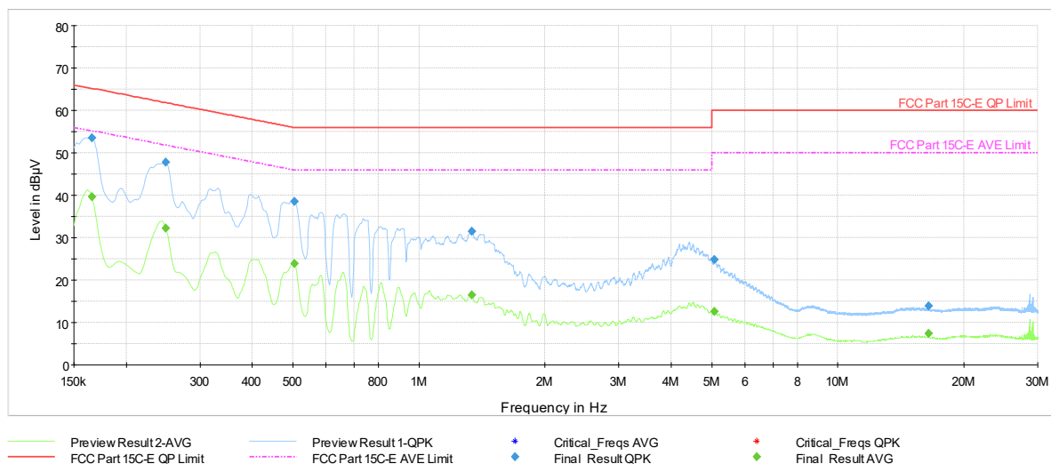
Plot 7-1173. AC Line Conducted Plot with 11be UNII Band 5 SDM Diversity – RU242 – Ch.61 (N) with AC/DC Adapter
