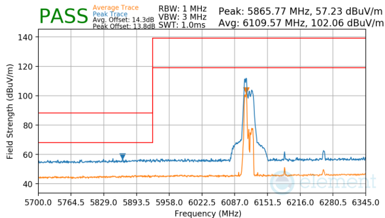
Plot 7-1132 SDM Diversity Radiated Lower Band Edge (Peak & Average – UNII Band 5) – RU52 (L)
