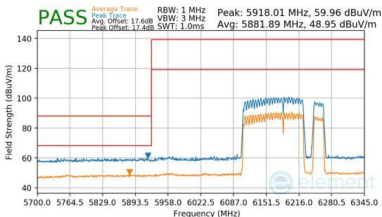
Plot 7-1149 SDM Diversity Radiated Lower Band Edge (Peak & Average – UNII Band 5) - RU996+484+242 (H)
