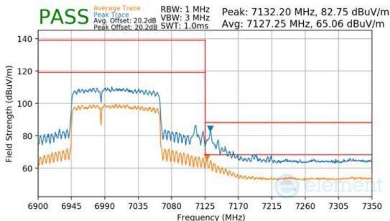
Plot 7-1140 SDM Diversity Radiated Upper Band Edge (Peak & Average – UNII Band 8) - RU996+484 (L)
