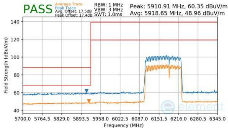
Plot 7-1139 SDM Diversity Radiated Lower Band Edge (Peak & Average – UNII Band 5) - RU996+484 (H)
