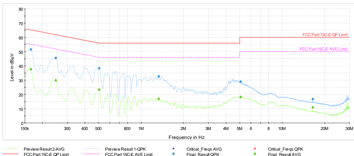
Plot 7-1170. AC Line Conducted Plot with 11be UNII Band 5 SDM Diversity – RU52 – Ch.61 (L1) with AC/DC Adapter
