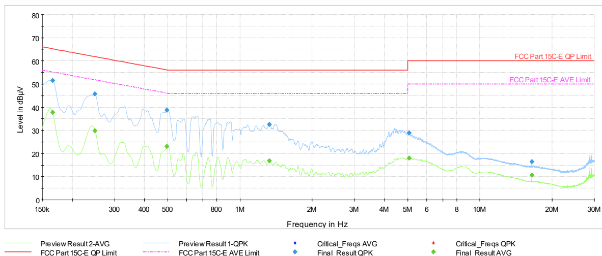
Plot 7-1166. AC Line Conducted Plot with 11be UNII Band 5 SDM Primary – RU52 – Ch.61 (L1) with AC/DC Adapter
