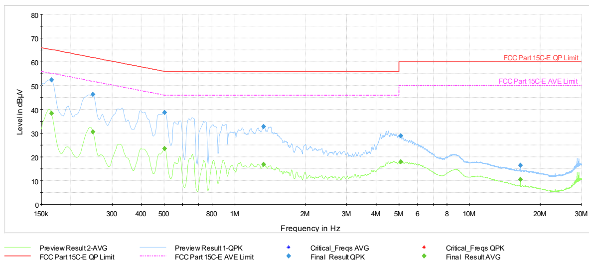
Plot 7-1172. AC Line Conducted Plot with 11be UNII Band 5 SDM Diversity – RU242 – Ch.61 (L1) with AC/DC Adapter
