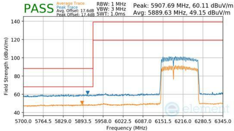
Plot 7-1136 SDM Diversity Radiated Lower Band Edge (Peak & Average – UNII Band 5) - RU996+484 (L)
