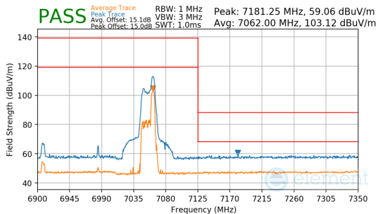
Plot 7-1135 SDM Diversity Radiated Upper Band Edge (Peak & Average – UNII Band 8) - RU26 (H)
