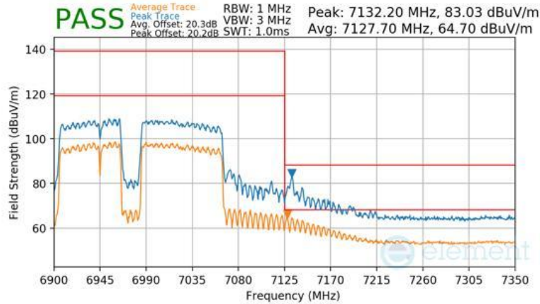
Plot 7-1158 SDM Diversity Radiated Upper Band Edge (Peak & Average – UNII Band 8) - RU996+484+242 (L)
