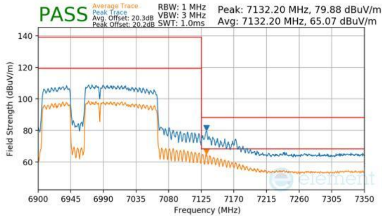
Plot 7-1156 SDM Diversity Radiated Upper Band Edge (Peak & Average – UNII Band 8) - RU996+484+242 (L)
