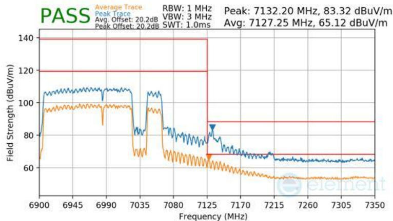
Plot 7-1157 SDM Diversity Radiated Upper Band Edge (Peak & Average – UNII Band 8) - RU996+484+242 (H)
