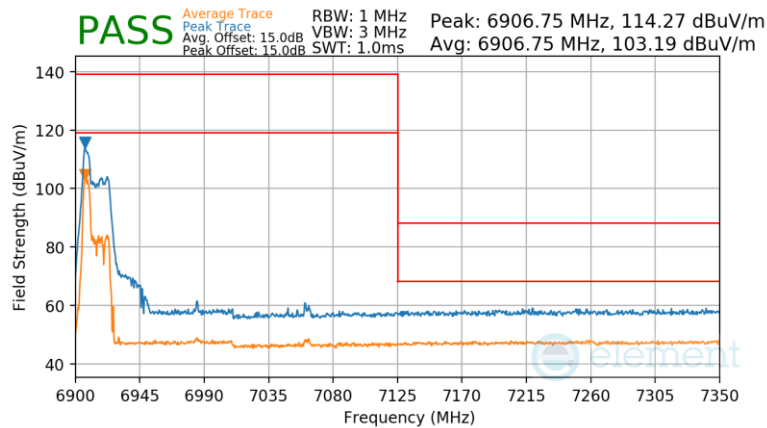
Plot 7-1134 SDM Diversity Radiated Upper Band Edge (Peak & Average – UNII Band 8) - RU26 (L)
