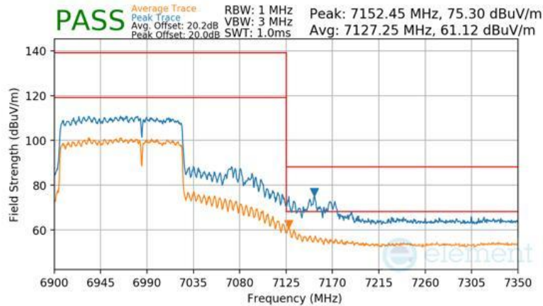
Plot 7-1143 SDM Diversity Radiated Upper Band Edge (Peak & Average – UNII Band 8) - RU996+484 (H)
