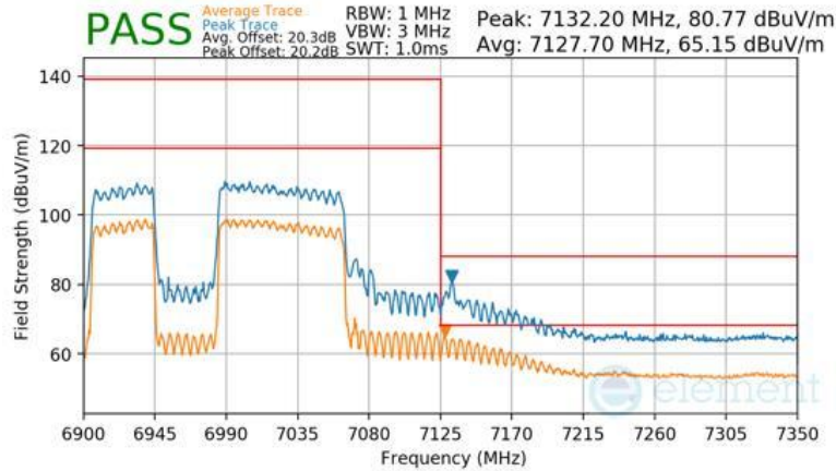
Plot 7-1142 SDM Diversity Radiated Upper Band Edge (Peak & Average – UNII Band 8) - RU996+484 (L)
