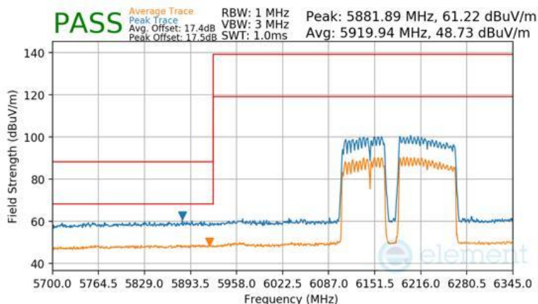
Plot 7-1150 SDM Diversity Radiated Lower Band Edge (Peak & Average – UNII Band 5) - RU996+484+242 (L)
