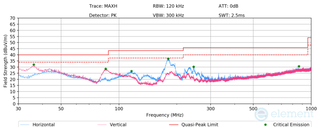
Plot 7-1165. Radiated Spurious Emissions below 1GHz SDM Diversity (802.11be – Ch.61 – RU242) with AC/DC Adapter
