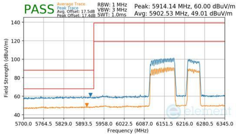
Plot 7-1137 SDM Diversity Radiated Lower Band Edge (Peak & Average – UNII Band 5) - RU996+484 (H)
