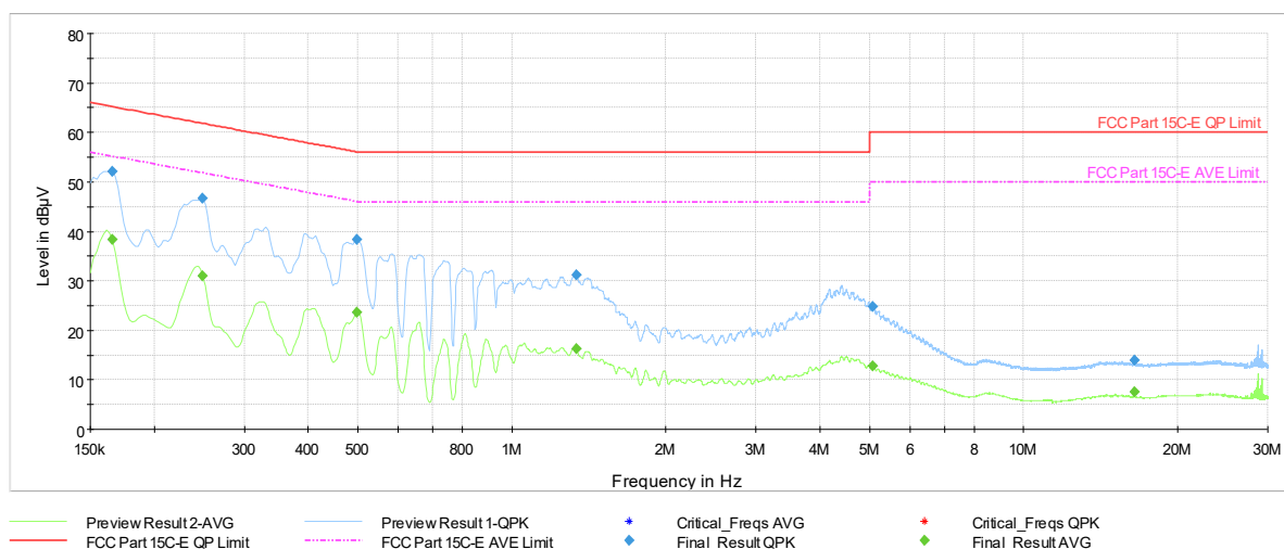
Plot 7-1167. AC Line Conducted Plot with 11be UNII Band 5 SDM Primary – RU52 – Ch.61 (N) with AC/DC Adapter
