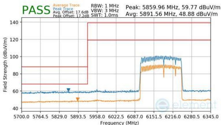
Plot 7-1151 SDM Diversity Radiated Lower Band Edge (Peak & Average – UNII Band 5) - RU996+484+242 (H)
