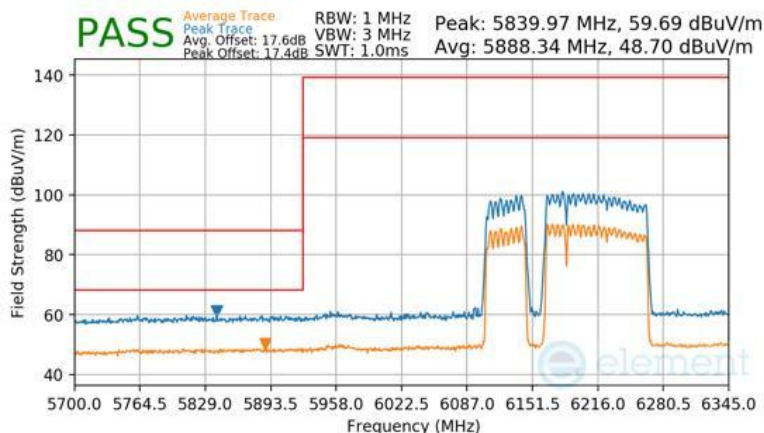
Plot 7-1148 SDM Diversity Radiated Lower Band Edge (Peak & Average – UNII Band 5) - RU996+484+242 (L)
