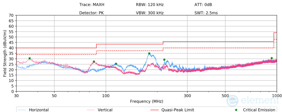
Plot 7-1163. Radiated Spurious Emissions below 1GHz SDM Primary (802.11be – Ch.61 – RU242) with AC/DC Adapter
