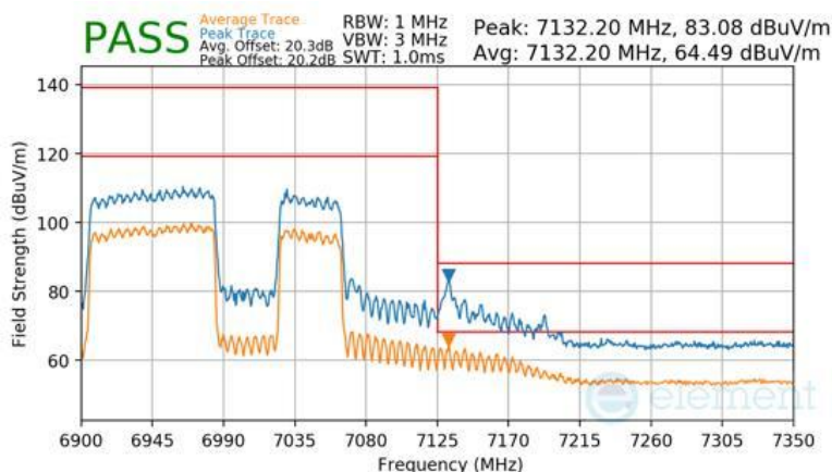
Plot 7-1141 SDM Diversity Radiated Upper Band Edge (Peak & Average – UNII Band 8) - RU996+484 (H)
