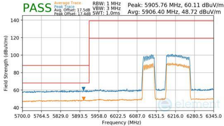
Plot 7-1138 SDM Diversity Radiated Lower Band Edge (Peak & Average – UNII Band 5) - RU996+484 (L)
