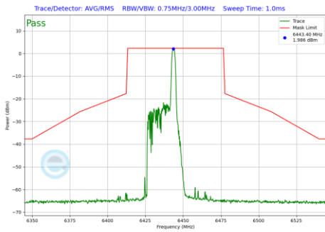
Plot 7-1018 In-Band Emission Plot CDD Primary Antenna 3b (40MHz BW 802.11be(RU) RU26 Index8 (UNII Band 6) - Ch.99)
