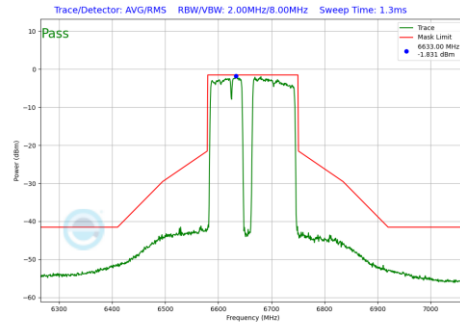
Plot 7-1042 In-Band Emission Plot CDD Primary Antenna 3b (160MHz BW 802.11be(RU) RU996+484+242 Index99 (UNII Band 7) - Ch.143)
