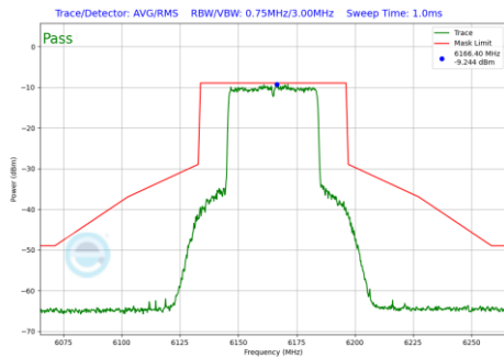
Plot 7-1124 In-Band Emission Plot SDM Primary Antenna 5T (40MHz BW 802.11be(RU) RU484 Index65 (UNII Band 5) - Ch.43)
