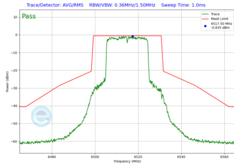
Plot 7-1059 In-Band Emission Plot CDD Primary Antenna 3b (20MHz BW 802.11be(RU) RU242 Index61 (UNII Band 6) - Ch.113)
