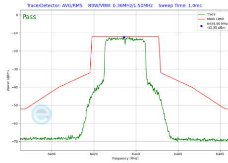
Plot 7-1127 In-Band Emission Plot SDM Primary Antenna 5T (20MHz BW 802.11be(RU) RU242 Index61 (UNII Band 6) - Ch.97)
