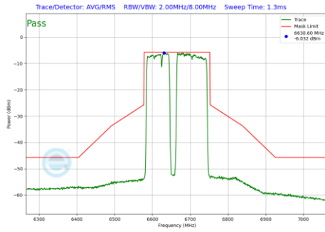
Plot 7-1107 In-Band Emission Plot SDM Primary Antenna 5T (160MHz BW 802.11be(RU) RU996+484+242 Index99 (UNII Band 7) - Ch.143)
