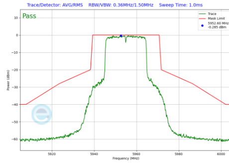
Plot 7-1055 In-Band Emission Plot CDD Primary Antenna 3b (20MHz BW 802.11be(RU) RU242 Index61 (UNII Band 5) - Ch.1)
