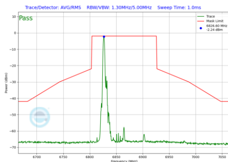
Plot 7-968 In-Band Emission Plot Antenna 1b (80MHz BW 802.11be(RU) RU26 Index0 (UNII Band 7) - Ch.183)
