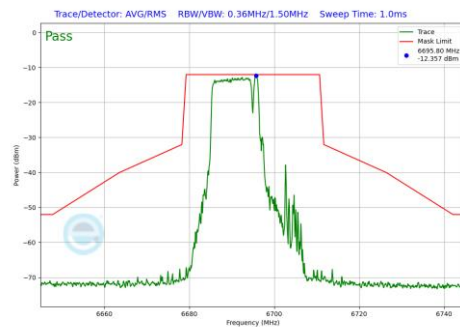
Plot 7-1105 In-Band Emission Plot SDM Primary Antenna 5T (20MHz BW 802.11be(RU) RU106+26 Index82 (UNII Band 7) - Ch.149)
