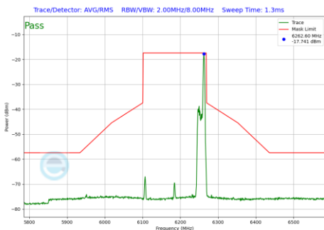
Plot 7-1086 In-Band Emission Plot SDM Primary Antenna 3b (160MHz BW 802.11be(RU) RU26 Index36 (UNII Band 5) - Ch.47)
