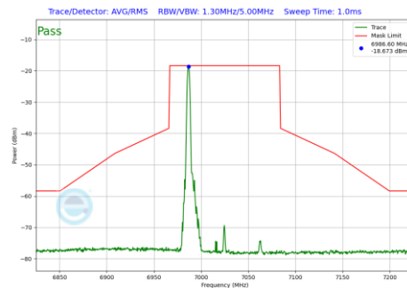
Plot 7-1097 In-Band Emission Plot SDM Primary Antenna 3b (80MHz BW 802.11be(RU) RU26 Index0 (UNII Band 8) - Ch.215)
