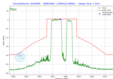
Plot 7-1035 In-Band Emission Plot CDD Primary Antenna 3b (80MHz BW 802.11be(RU) RU484+242 Index92 (UNII Band 5) - Ch.7)
