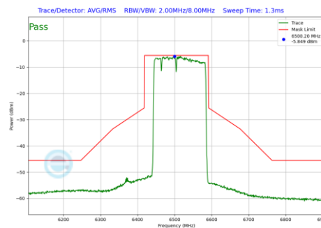
Plot 7-1104 In-Band Emission Plot SDM Primary Antenna 5T (160MHz BW 802.11be(RU) RU996+484+242 Index96 (UNII Band 6) - Ch.111)
