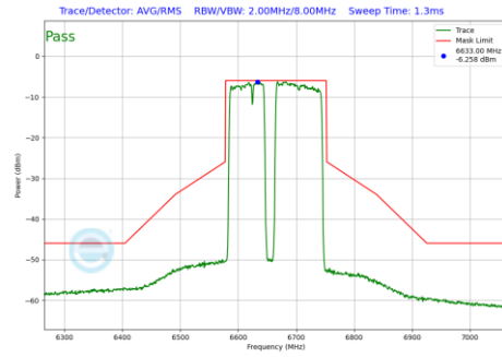
Plot 7-1119 In-Band Emission Plot SDM Primary Antenna 3b (160MHz BW 802.11be(RU) RU996+484+242 Index99 (UNII Band 7) - Ch.143)
