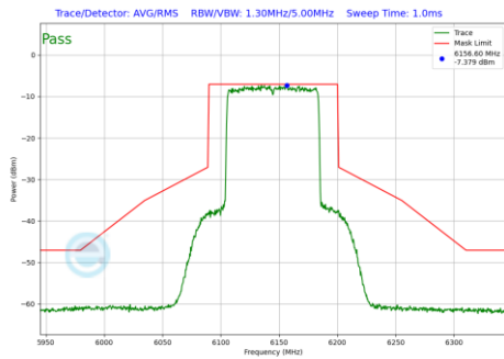
Plot 7-1125 In-Band Emission Plot SDM Primary Antenna 5T (80MHz BW 802.11be(RU) RU996 Index67 (UNII Band 5) - Ch.39)
