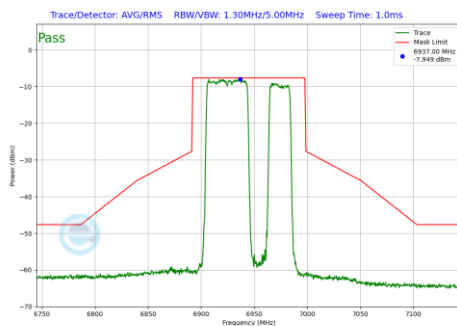
Plot 7-1109 In-Band Emission Plot SDM Primary Antenna 5T (80MHz BW 802.11be(RU) RU484+242 Index92 (UNII Band 8) - Ch.199)
