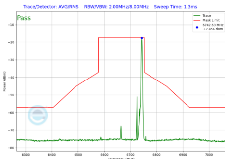
Plot 7-1094 In-Band Emission Plot SDM Primary Antenna 3b (160MHz BW 802.11be(RU) RU26 Index36 (UNII Band 7) - Ch.143)
