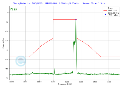
Plot 7-1070 In-Band Emission Plot SDM Primary Antenna 5T (160MHz BW 802.11be(RU) RU26 Index36 (UNII Band 5) - Ch.47)
