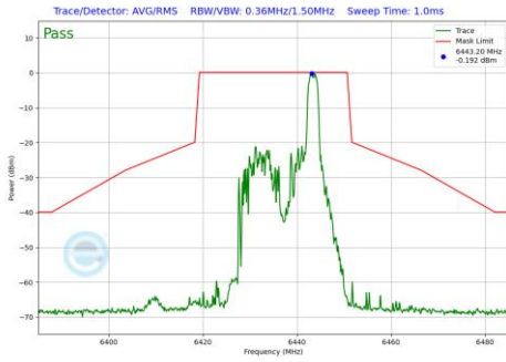
Plot 7-1017 In-Band Emission Plot CDD Primary Antenna 3b (20MHz BW 802.11be(RU) RU26 Index8 (UNII Band 6) - Ch.97)
