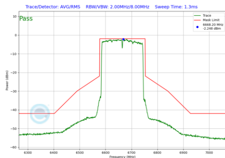
Plot 7-1054 In-Band Emission Plot CDD Primary Antenna 5T (160MHz BW 802.11be(RU) RU996X2 Index68 (UNII Band 7) - Ch.143)
