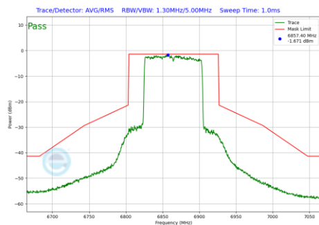
Plot 7-995 In-Band Emission Plot Antenna 1b (80MHz BW 802.11be(RU) RU996 Index67 (UNII Band 7) - Ch.183)
