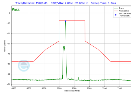
Plot 7-1082 In-Band Emission Plot SDM Primary Antenna 5T (160MHz BW 802.11be(RU) RU26 Index17 (UNII Band 8) - Ch.207)
