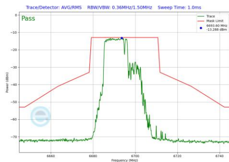
Plot 7-1117 In-Band Emission Plot SDM Primary Antenna 3b (20MHz BW 802.11be(RU) RU106+26 Index82 (UNII Band 7) - Ch.149)
