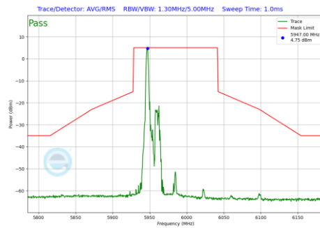
Plot 7-1015 In-Band Emission Plot CDD Primary Antenna 3b (80MHz BW 802.11be(RU) RU26 Index0 (UNII Band 5) - Ch.7)
