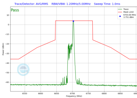
Plot 7-1011 In-Band Emission Plot CDD Primary Antenna 5T (80MHz BW 802.11be(RU) RU26 Index17 (UNII Band 7) - Ch.151)
