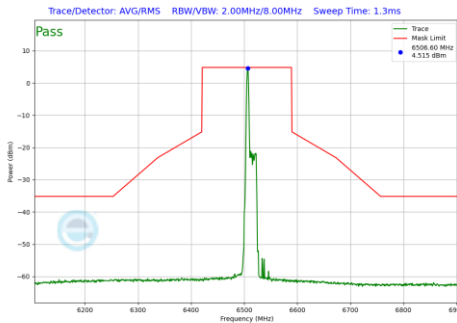
Plot 7-1020 In-Band Emission Plot CDD Primary Antenna 3b (160MHz BW 802.11be(RU) RU26 Index0 (UNII Band 6) - Ch.111)
