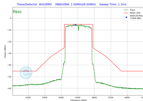
Plot 7-1130 In-Band Emission Plot SDM Primary Antenna 5T (160MHz BW 802.11be(RU) RU996X2 Index68 (UNII Band 6) - Ch.111)
