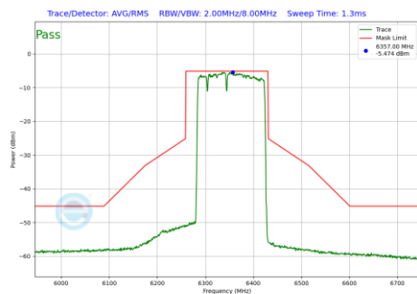
Plot 7-1101 In-Band Emission Plot SDM Primary Antenna 5T (160MHz BW 802.11be(RU) RU996+484+242 Index96 (UNII Band 5) - Ch.79)
