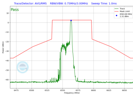
Plot 7-1010 In-Band Emission Plot CDD Primary Antenna 5T (40MHz BW 802.11be(RU) RU26 Index8 (UNII Band 7) - Ch.123)
