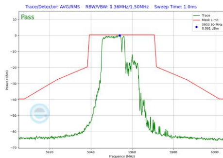
Plot 7-1034 In-Band Emission Plot CDD Primary Antenna 3b (20MHz BW 802.11be(RU) RU106+26 Index82 (UNII Band 5) - Ch.1)
