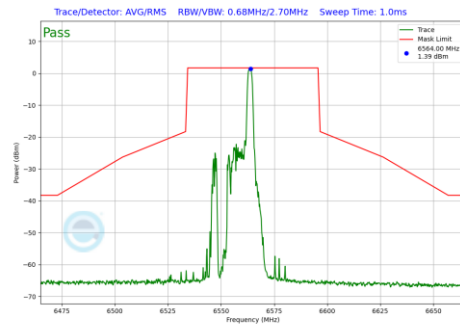
Plot 7-1022 In-Band Emission Plot CDD Primary Antenna 3b (40MHz BW 802.11be(RU) RU26 Index8 (UNII Band 7) - Ch.123)
