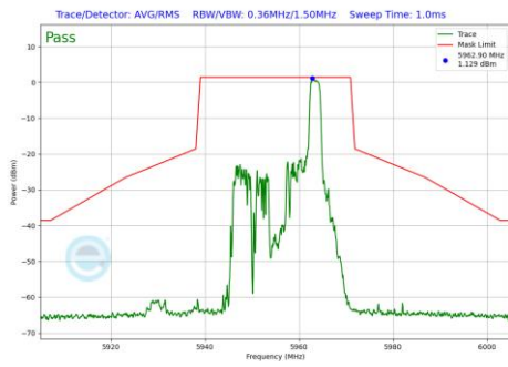
Plot 7-1001 In-Band Emission Plot CDD Primary Antenna 5T (20MHz BW 802.11be(RU) RU26 Index8 (UNII Band 5) - Ch.1)
