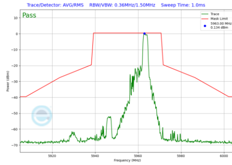
Plot 7-1013 In-Band Emission Plot CDD Primary Antenna 3b (20MHz BW 802.11be(RU) RU26 Index8 (UNII Band 5) - Ch.1)
