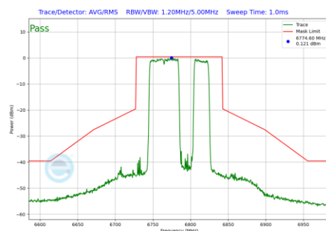
Plot 7-1032 In-Band Emission Plot CDD Primary Antenna 5T (80MHz BW 802.11be(RU) RU484+242 Index92 (UNII Band 7) - Ch.167)
