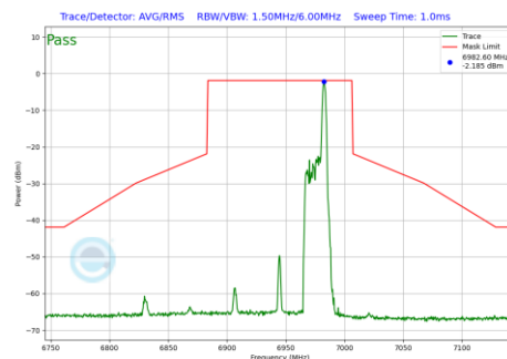
Plot 7-972 In-Band Emission Plot Antenna 1b (80MHz BW 802.11be(RU) RU26 Index36 (UNII Band 8) - Ch.199)
