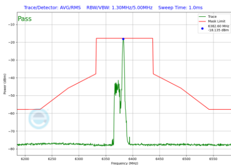
Plot 7-1085 In-Band Emission Plot SDM Primary Antenna 3b (80MHz BW 802.11be(RU) RU26 Index17 (UNII Band 5) - Ch.87)
