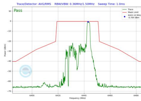
Plot 7-1005 In-Band Emission Plot CDD Primary Antenna 5T (20MHz BW 802.11be(RU) RU26 Index8 (UNII Band 6) - Ch.97)
