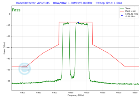
Plot 7-1115 In-Band Emission Plot SDM Primary Antenna 3b (80MHz BW 802.11be(RU) RU484+242 Index91 (UNII Band 6) - Ch.103)
