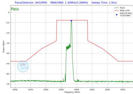
Plot 7-1069 In-Band Emission Plot SDM Primary Antenna 5T (80MHz BW 802.11be(RU) RU26 Index17 (UNII Band 5) - Ch.87)
