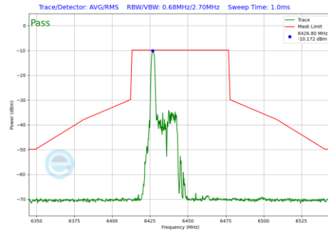
Plot 7-1072 In-Band Emission Plot SDM Primary Antenna 5T (40MHz BW 802.11be(RU) RU26 Index0 (UNII Band 6) - Ch.99)
