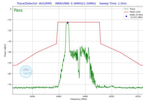
Plot 7-1071 In-Band Emission Plot SDM Primary Antenna 5T (20MHz BW 802.11be(RU) RU26 Index0 (UNII Band 6) - Ch.105)
