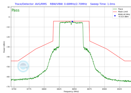
Plot 7-994 In-Band Emission Plot Antenna 1b (40MHz BW 802.11be(RU) RU484 Index65 (UNII Band 7) - Ch.179)
