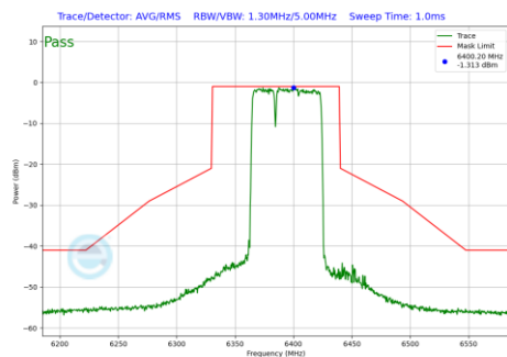
Plot 7-975 In-Band Emission Plot Antenna 1b (80MHz BW 802.11be(RU) RU484+242 Index90 (UNII Band 5) - Ch.87)
