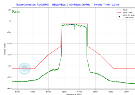
Plot 7-1066 In-Band Emission Plot CDD Primary Antenna 3b (160MHz BW 802.11be(RU) RU996X2 Index68 (UNII Band 7) - Ch.143)
