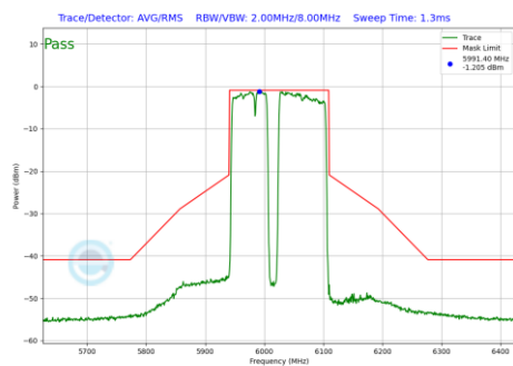
Plot 7-1027 In-Band Emission Plot CDD Primary Antenna 5T (160MHz BW 802.11be(RU) RU996+484+242 Index99 (UNII Band 5) - Ch.15)
