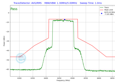
Plot 7-1129 In-Band Emission Plot SDM Primary Antenna 5T (80MHz BW 802.11be(RU) RU996 Index67 (UNII Band 6) - Ch.103)
