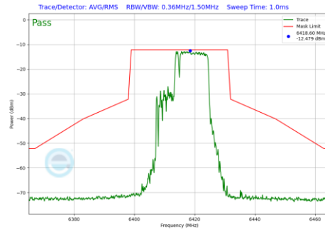
Plot 7-1111 In-Band Emission Plot SDM Primary Antenna 3b (20MHz BW 802.11be(RU) RU106+26 Index83 (UNII Band 5) - Ch.93)
