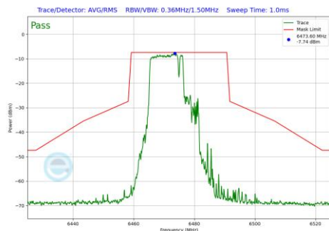
Plot 7-977 In-Band Emission Plot Antenna 1b (20MHz BW 802.11be(RU) RU106+26 Index82 (UNII Band 6) - Ch.105)
