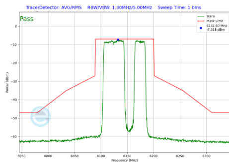
Plot 7-1100 In-Band Emission Plot SDM Primary Antenna 5T (80MHz BW 802.11be(RU) RU484+242 Index92 (UNII Band 5) - Ch.39)
