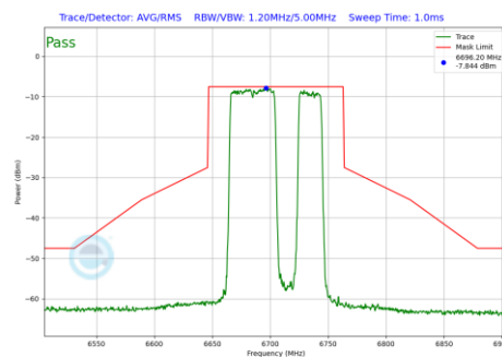
Plot 7-1106 In-Band Emission Plot SDM Primary Antenna 5T (80MHz BW 802.11be(RU) RU484+242 Index92 (UNII Band 7) - Ch.151)
