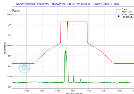
Plot 7-1090 In-Band Emission Plot SDM Primary Antenna 3b (160MHz BW 802.11be(RU) RU26 Index17 (UNII Band 6) - Ch.111)
