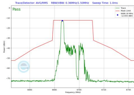
Plot 7-1075 In-Band Emission Plot SDM Primary Antenna 5T (20MHz BW 802.11be(RU) RU26 Index0 (UNII Band 7) - Ch.149)
