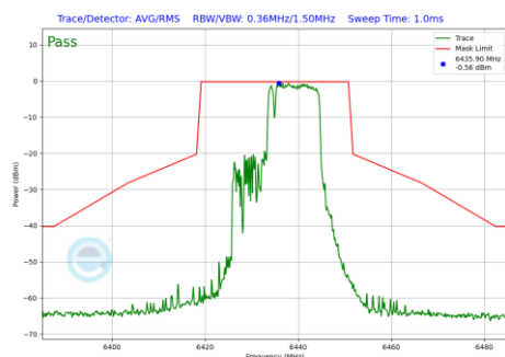
Plot 7-1028 In-Band Emission Plot CDD Primary Antenna 5T (20MHz BW 802.11be(RU) RU106+26 Index83 (UNII Band 6) - Ch.97)
