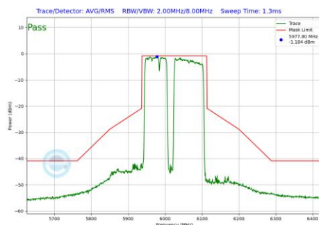
Plot 7-1036 In-Band Emission Plot CDD Primary Antenna 3b (160MHz BW 802.11be(RU) RU996+484+242 Index99 (UNII Band 5) - Ch.15)
