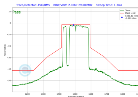
Plot 7-979 In-Band Emission Plot Antenna 1b (160MHz BW 802.11be(RU) RU996+484+242 Index97 (UNII Band 6) - Ch.111)
