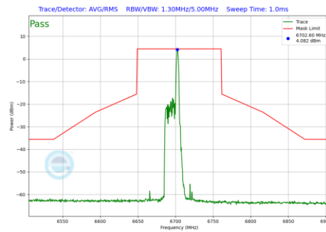
Plot 7-1023 In-Band Emission Plot CDD Primary Antenna 3b (80MHz BW 802.11be(RU) RU26 Index17 (UNII Band 7) - Ch.151)
