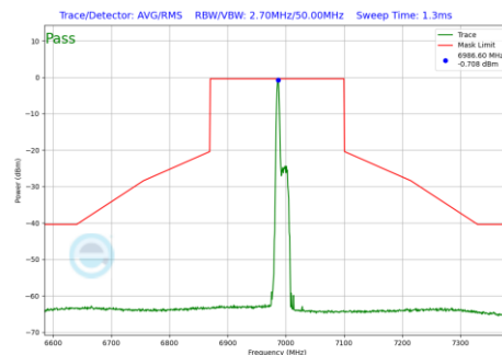
Plot 7-973 In-Band Emission Plot Antenna 1b (160MHz BW 802.11be(RU) RU26 Index0 (UNII Band 8) - Ch.207)
