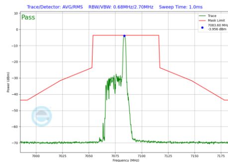
Plot 7-971 In-Band Emission Plot Antenna 1b (40MHz BW 802.11be(RU) RU26 Index8 (UNII Band 8) - Ch.227)
