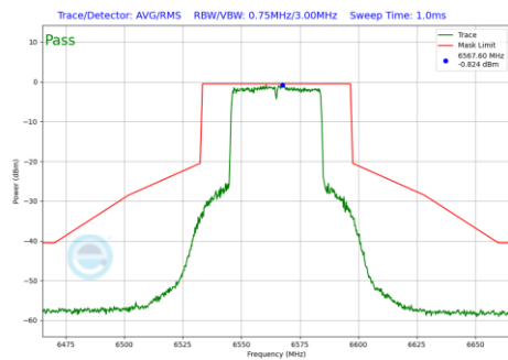
Plot 7-1052 In-Band Emission Plot CDD Primary Antenna 5T (40MHz BW 802.11be(RU) RU484 Index65 (UNII Band 7) - Ch.123)
