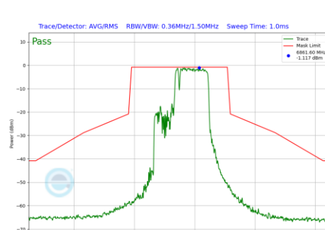
Plot 7-1040 In-Band Emission Plot CDD Primary Antenna 3b (20MHz BW 802.11be(RU) RU106+26 Index83 (UNII Band 7) - Ch.181)
