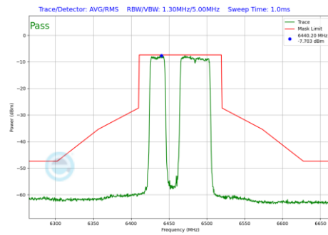
Plot 7-1103 In-Band Emission Plot SDM Primary Antenna 5T (80MHz BW 802.11be(RU) RU484+242 Index91 (UNII Band 6) - Ch.103)
