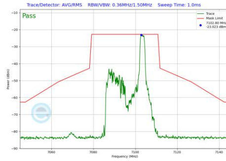
Plot 7-1095 In-Band Emission Plot SDM Primary Antenna 3b (20MHz BW 802.11be(RU) RU26 Index8 (UNII Band 8) - Ch.229)
