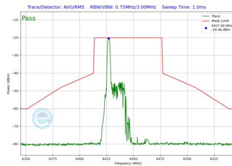
Plot 7-1088 In-Band Emission Plot SDM Primary Antenna 3b (40MHz BW 802.11be(RU) RU26 Index0 (UNII Band 6) - Ch.99)
