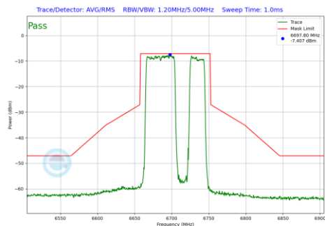
Plot 7-1118 In-Band Emission Plot SDM Primary Antenna 3b (80MHz BW 802.11be(RU) RU484+242 Index92 (UNII Band 7) - Ch.151)
