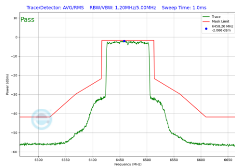
Plot 7-1061 In-Band Emission Plot CDD Primary Antenna 3b (80MHz BW 802.11be(RU) RU996 Index67 (UNII Band 6) - Ch.103)
