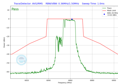
Plot 7-1031 In-Band Emission Plot CDD Primary Antenna 5T (20MHz BW 802.11be(RU) RU106+26 Index83 (UNII Band 7) - Ch.181)
