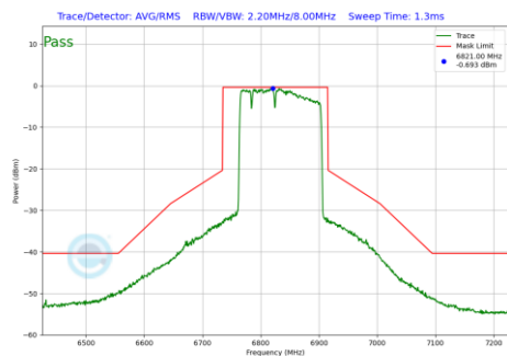
Plot 7-982 In-Band Emission Plot Antenna 1b (160MHz BW 802.11be(RU) RU996+484+242 Index96 (UNII Band 7) - Ch.175)
