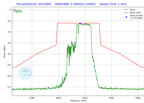
Plot 7-1099 In-Band Emission Plot SDM Primary Antenna 5T (20MHz BW 802.11be(RU) RU106+26 Index83 (UNII Band 5) - Ch.93)
