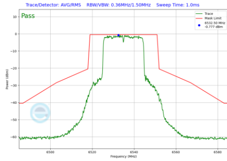
Plot 7-1051 In-Band Emission Plot CDD Primary Antenna 5T (20MHz BW 802.11be(RU) RU242 Index61 (UNII Band 7) - Ch.117)
