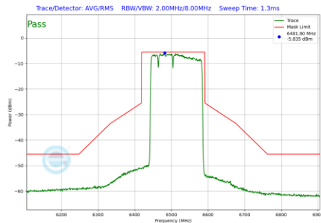
Plot 7-1116 In-Band Emission Plot SDM Primary Antenna 3b (160MHz BW 802.11be(RU) RU996+484+242 Index96 (UNII Band 6) - Ch.111)
