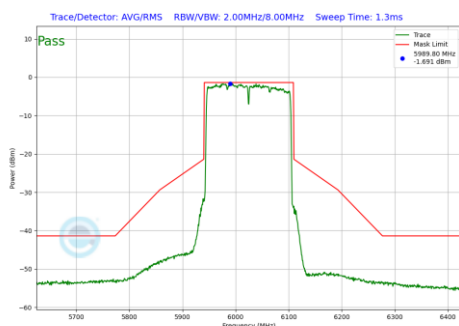
Plot 7-1046 In-Band Emission Plot CDD Primary Antenna 5T (160MHz BW 802.11be(RU) RU996X2 Index68 (UNII Band 5) - Ch.15)
