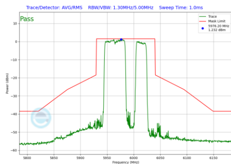
Plot 7-1026 In-Band Emission Plot CDD Primary Antenna 5T (80MHz BW 802.11be(RU) RU484+242 Index92 (UNII Band 5) - Ch.7)
