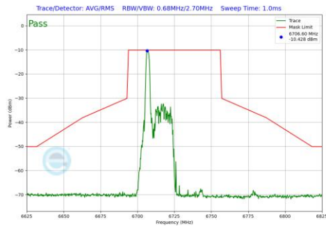
Plot 7-1076 In-Band Emission Plot SDM Primary Antenna 5T (40MHz BW 802.11be(RU) RU26 Index0 (UNII Band 7) - Ch.155)
