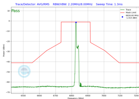
Plot 7-969 In-Band Emission Plot Antenna 1b (160MHz BW 802.11be(RU) RU26 Index0 (UNII Band 7) - Ch.175)
