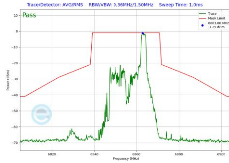
Plot 7-1021 In-Band Emission Plot CDD Primary Antenna 3b (20MHz BW 802.11be(RU) RU26 Index8 (UNII Band 7) - Ch.181)
