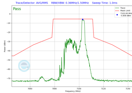
Plot 7-970 In-Band Emission Plot Antenna 1b (20MHz BW 802.11be(RU) RU26 Index8 (UNII Band 8) - Ch.229)
