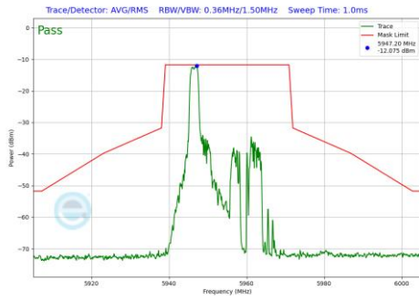
Plot 7-1067 In-Band Emission Plot SDM Primary Antenna 5T (20MHz BW 802.11be(RU) RU26 Index0 (UNII Band 5) - Ch.1)
