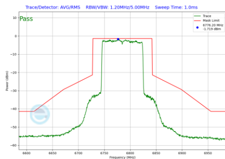
Plot 7-1053 In-Band Emission Plot CDD Primary Antenna 5T (80MHz BW 802.11be(RU) RU996 Index67 (UNII Band 7) - Ch.167)
