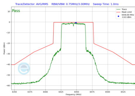
Plot 7-1060 In-Band Emission Plot CDD Primary Antenna 3b (40MHz BW 802.11be(RU) RU484 Index65 (UNII Band 6) - Ch.99)
