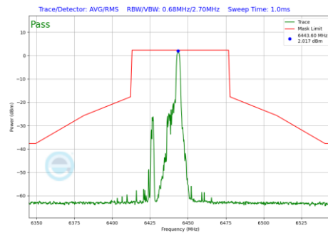
Plot 7-1006 In-Band Emission Plot CDD Primary Antenna 5T (40MHz BW 802.11be(RU) RU26 Index8 (UNII Band 6) - Ch.99)
