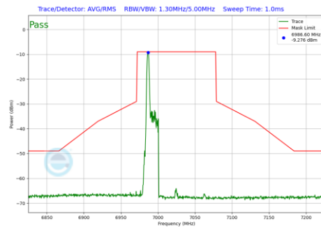
Plot 7-1081 In-Band Emission Plot SDM Primary Antenna 5T (80MHz BW 802.11be(RU) RU26 Index0 (UNII Band 8) - Ch.215)
