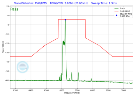
Plot 7-1012 In-Band Emission Plot CDD Primary Antenna 5T (160MHz BW 802.11be(RU) RU26 Index17 (UNII Band 7) - Ch.143)
