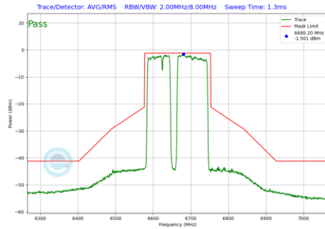
Plot 7-1033 In-Band Emission Plot CDD Primary Antenna 5T (160MHz BW 802.11be(RU) RU996+484+242 Index99 (UNII Band 7) - Ch.143)
