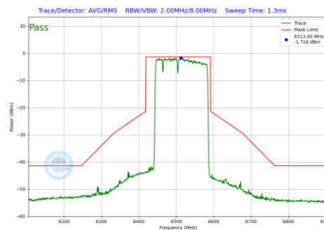
Plot 7-1030 In-Band Emission Plot CDD Primary Antenna 5T (160MHz BW 802.11be(RU) RU996+484+242 Index96 (UNII Band 6) - Ch.111)
