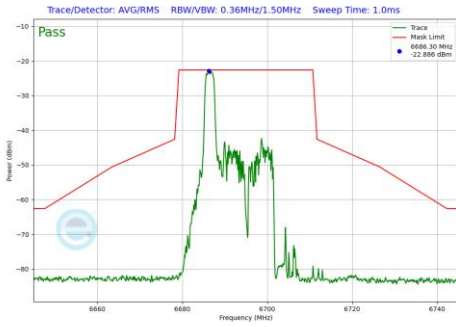
Plot 7-1091 In-Band Emission Plot SDM Primary Antenna 3b (20MHz BW 802.11be(RU) RU26 Index0 (UNII Band 7) - Ch.149)
