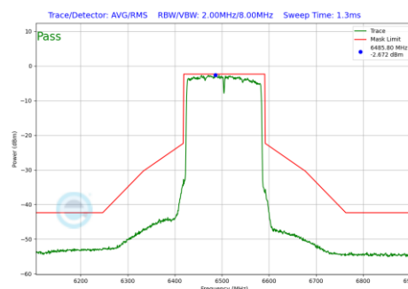
Plot 7-1050 In-Band Emission Plot CDD Primary Antenna 5T (160MHz BW 802.11be(RU) RU996X2 Index68 (UNII Band 6) - Ch.111)
