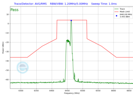
Plot 7-1019 In-Band Emission Plot CDD Primary Antenna 3b (80MHz BW 802.11be(RU) RU26 Index17 (UNII Band 6) - Ch.103)
