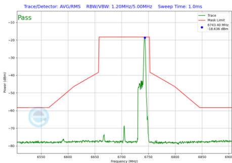
Plot 7-1093 In-Band Emission Plot SDM Primary Antenna 3b (80MHz BW 802.11be(RU) RU26 Index36 (UNII Band 7) - Ch.151)
