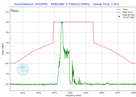
Plot 7-1084 In-Band Emission Plot SDM Primary Antenna 3b (40MHz BW 802.11be(RU) RU26 Index0 (UNII Band 5) - Ch.91)
