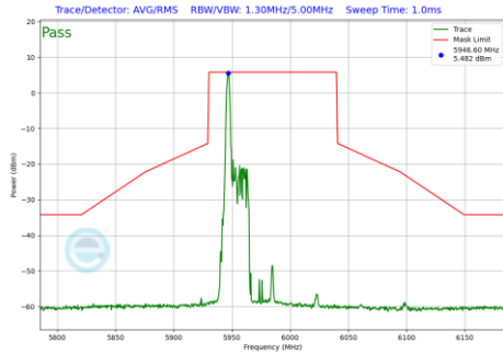
Plot 7-1003 In-Band Emission Plot CDD Primary Antenna 5T (80MHz BW 802.11be(RU) RU26 Index0 (UNII Band 5) - Ch.7)
