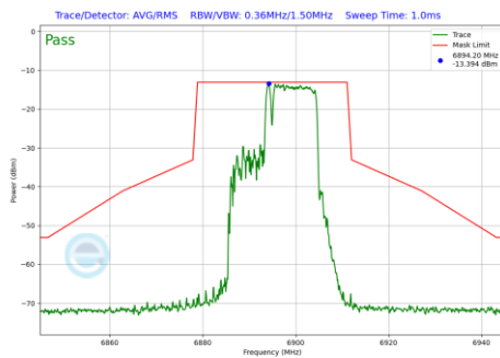
Plot 7-1108 In-Band Emission Plot SDM Primary Antenna 5T (20MHz BW 802.11be(RU) RU106+26 Index83 (UNII Band 8) - Ch.189)
