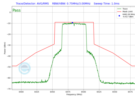
Plot 7-1128 In-Band Emission Plot SDM Primary Antenna 5T (40MHz BW 802.11be(RU) RU484 Index65 (UNII Band 6) - Ch.107)
