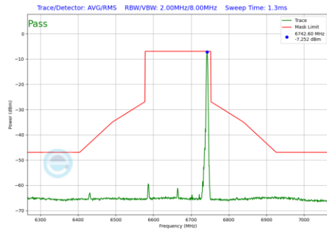
Plot 7-1078 In-Band Emission Plot SDM Primary Antenna 5T (160MHz BW 802.11be(RU) RU26 Index36 (UNII Band 7) - Ch.143)
