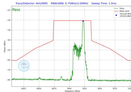
Plot 7-1096 In-Band Emission Plot SDM Primary Antenna 3b (40MHz BW 802.11be(RU) RU26 Index17 (UNII Band 8) - Ch.211)
