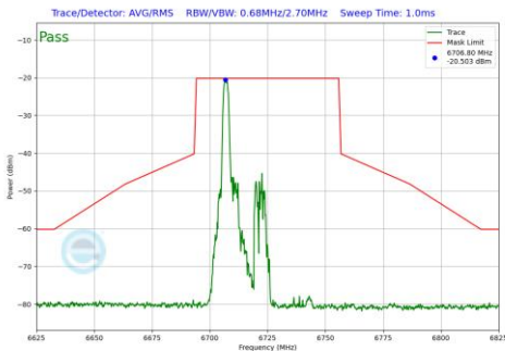
Plot 7-1092 In-Band Emission Plot SDM Primary Antenna 3b (40MHz BW 802.11be(RU) RU26 Index0 (UNII Band 7) - Ch.155)
