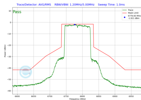
Plot 7-1065 In-Band Emission Plot CDD Primary Antenna 3b (80MHz BW 802.11be(RU) RU996 Index67 (UNII Band 7) - Ch.167)
