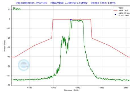
Plot 7-1037 In-Band Emission Plot CDD Primary Antenna 3b (20MHz BW 802.11be(RU) RU106+26 Index83 (UNII Band 6) - Ch.97)
