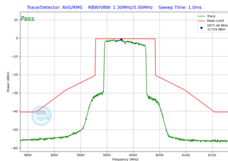
Plot 7-1057 In-Band Emission Plot CDD Primary Antenna 3b (80MHz BW 802.11be(RU) RU996 Index67 (UNII Band 5) - Ch.7)
