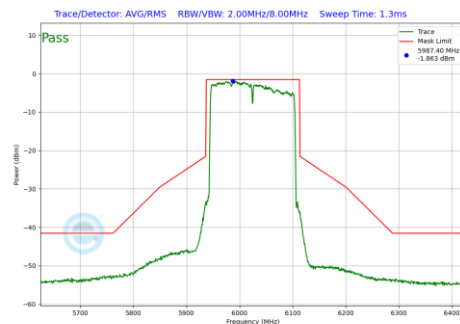
Plot 7-1058 In-Band Emission Plot CDD Primary Antenna 3b (160MHz BW 802.11be(RU) RU996X2 Index68 (UNII Band 5) - Ch.15)
