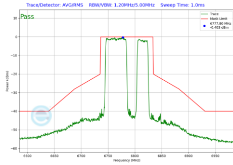
Plot 7-1041 In-Band Emission Plot CDD Primary Antenna 3b (80MHz BW 802.11be(RU) RU484+242 Index92 (UNII Band 7) - Ch.167)
