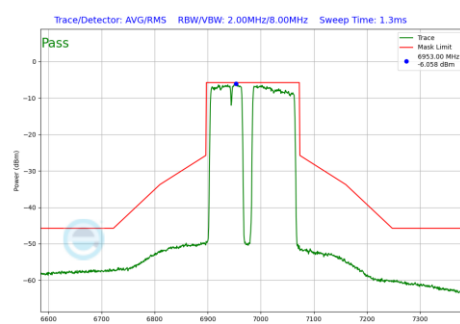
Plot 7-1122 In-Band Emission Plot SDM Primary Antenna 3b (160MHz BW 802.11be(RU) RU996+484+242 Index99 (UNII Band 8) - Ch.207)
