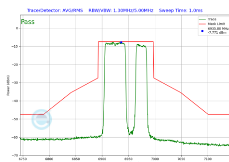
Plot 7-1121 In-Band Emission Plot SDM Primary Antenna 3b (80MHz BW 802.11be(RU) RU484+242 Index92 (UNII Band 8) - Ch.199)
