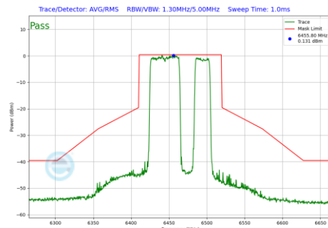
Plot 7-1029 In-Band Emission Plot CDD Primary Antenna 5T (80MHz BW 802.11be(RU) RU484+242 Index92 (UNII Band 6) - Ch.103)
