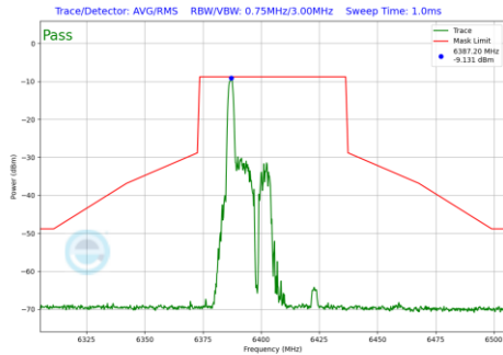
Plot 7-1068 In-Band Emission Plot SDM Primary Antenna 5T (40MHz BW 802.11be(RU) RU26 Index0 (UNII Band 5) - Ch.91)
