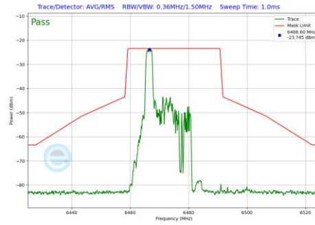
Plot 7-1087 In-Band Emission Plot SDM Primary Antenna 3b (20MHz BW 802.11be(RU) RU26 Index0 (UNII Band 6) - Ch.105)
