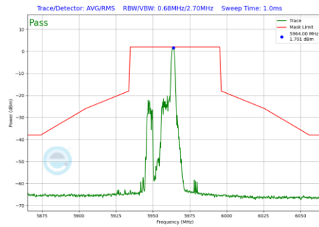
Plot 7-1014 In-Band Emission Plot CDD Primary Antenna 3b (40MHz BW 802.11be(RU) RU26 Index8 (UNII Band 5) - Ch.3)
