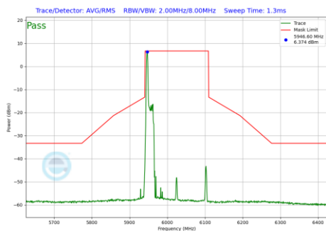
Plot 7-1004 In-Band Emission Plot CDD Primary Antenna 5T (160MHz BW 802.11be(RU) RU26 Index0 (UNII Band 5) - Ch.15)
