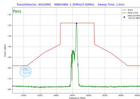
Plot 7-1089 In-Band Emission Plot SDM Primary Antenna 3b (80MHz BW 802.11be(RU) RU26 Index17 (UNII Band 6) - Ch.103)
