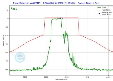
Plot 7-1025 In-Band Emission Plot CDD Primary Antenna 5T (20MHz BW 802.11be(RU) RU106+26 Index82 (UNII Band 5) - Ch.1)
