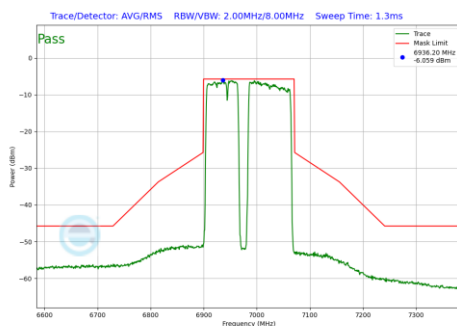
Plot 7-1110 In-Band Emission Plot SDM Primary Antenna 5T (160MHz BW 802.11be(RU) RU996+484+242 Index99 (UNII Band 8) - Ch.207)
