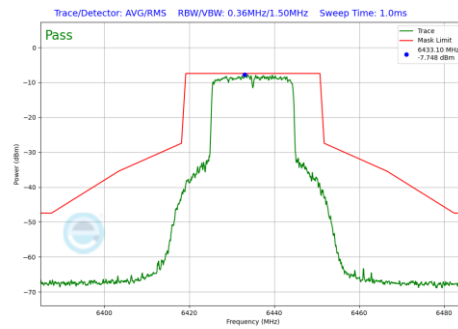
Plot 7-989 In-Band Emission Plot Antenna 1b (20MHz BW 802.11be(RU) RU242 Index61 (UNII Band 6) - Ch.97)
