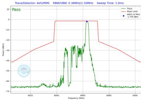
Plot 7-1009 In-Band Emission Plot CDD Primary Antenna 5T (20MHz BW 802.11be(RU) RU26 Index8 (UNII Band 7) - Ch.181)
