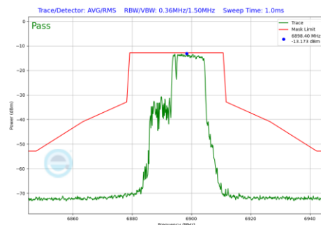
Plot 7-1120 In-Band Emission Plot SDM Primary Antenna 3b (20MHz BW 802.11be(RU) RU106+26 Index83 (UNII Band 8) - Ch.189)
