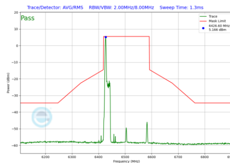
Plot 7-1008 In-Band Emission Plot CDD Primary Antenna 5T (160MHz BW 802.11be(RU) RU26 Index0 (UNII Band 6) - Ch.111)
