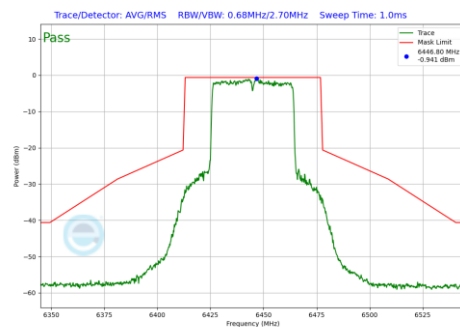
Plot 7-1048 In-Band Emission Plot CDD Primary Antenna 5T (40MHz BW 802.11be(RU) RU484 Index65 (UNII Band 6) - Ch.99)
