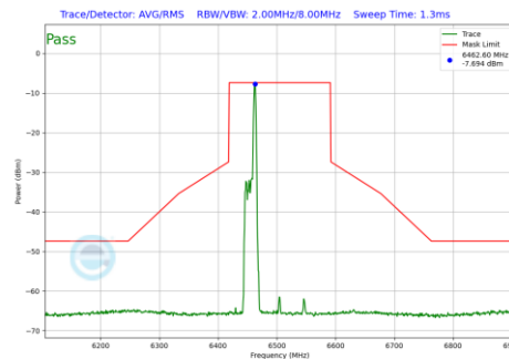
Plot 7-1074 In-Band Emission Plot SDM Primary Antenna 5T (160MHz BW 802.11be(RU) RU26 Index17 (UNII Band 6) - Ch.111)
