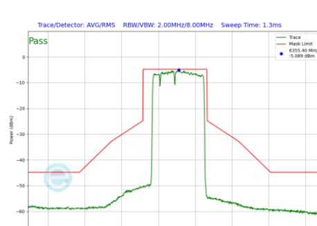
Plot 7-1113 In-Band Emission Plot SDM Primary Antenna 3b (160MHz BW 802.11be(RU) RU996+484+242 Index96 (UNII Band 5) - Ch.79)
