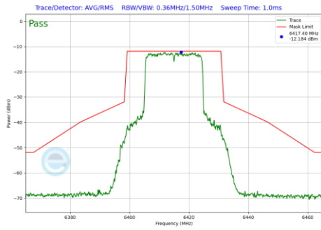
Plot 7-1123 In-Band Emission Plot SDM Primary Antenna 5T (20MHz BW 802.11be(RU) RU242 Index61 (UNII Band 5) - Ch.93)
