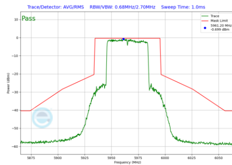
Plot 7-1056 In-Band Emission Plot CDD Primary Antenna 3b (40MHz BW 802.11be(RU) RU484 Index65 (UNII Band 5) - Ch.3)
