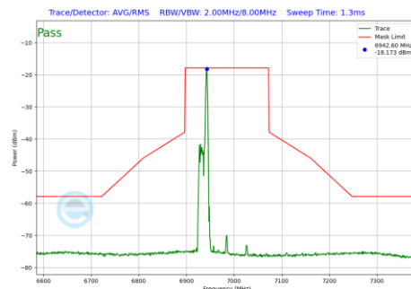
Plot 7-1098 In-Band Emission Plot SDM Primary Antenna 3b (160MHz BW 802.11be(RU) RU26 Index17 (UNII Band 8) - Ch.207)
