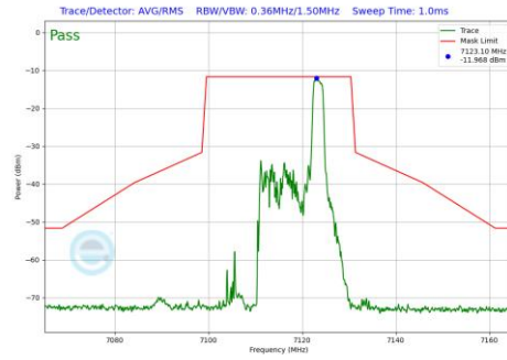
Plot 7-1079 In-Band Emission Plot SDM Primary Antenna 5T (20MHz BW 802.11be(RU) RU26 Index8 (UNII Band 8) - Ch.233)
