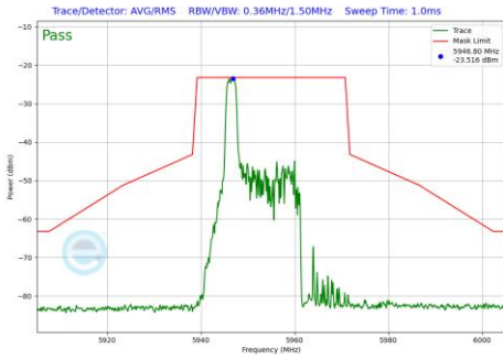
Plot 7-1083 In-Band Emission Plot SDM Primary Antenna 3b (20MHz BW 802.11be(RU) RU26 Index0 (UNII Band 5) - Ch.1)
