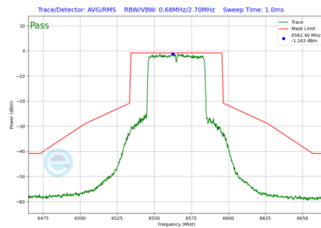
Plot 7-1064 In-Band Emission Plot CDD Primary Antenna 3b (40MHz BW 802.11be(RU) RU484 Index65 (UNII Band 7) - Ch.123)
