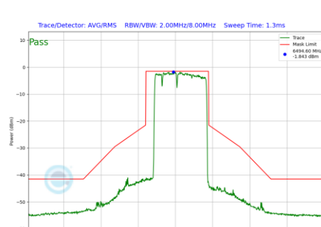
Plot 7-1039 In-Band Emission Plot CDD Primary Antenna 3b (160MHz BW 802.11be(RU) RU996+484+242 Index96 (UNII Band 6) - Ch.111)
