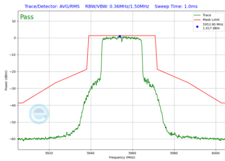
Plot 7-1043 In-Band Emission Plot CDD Primary Antenna 5T (20MHz BW 802.11be(RU) RU242 Index61 (UNII Band 5) - Ch.1)
