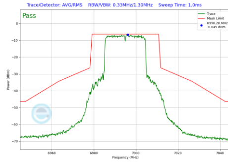
Plot 7-997 In-Band Emission Plot Antenna 1b (20MHz BW 802.11be(RU) RU242 Index61 (UNII Band 8) - Ch.209)
