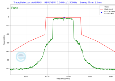
Plot 7-1063 In-Band Emission Plot CDD Primary Antenna 3b (20MHz BW 802.11be(RU) RU242 Index61 (UNII Band 7) - Ch.117)
