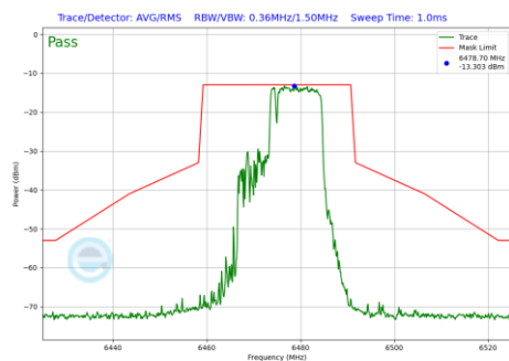
Plot 7-1102 In-Band Emission Plot SDM Primary Antenna 5T (20MHz BW 802.11be(RU) RU106+26 Index83 (UNII Band 6) - Ch.105)
