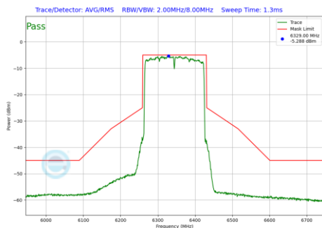
Plot 7-1126 In-Band Emission Plot SDM Primary Antenna 5T (160MHz BW 802.11be(RU) RU996X2 Index68 (UNII Band 5) - Ch.79)
