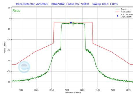
Plot 7-998 In-Band Emission Plot Antenna 1b (40MHz BW 802.11be(RU) RU484 Index65 (UNII Band 8) - Ch.227)
