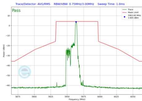
Plot 7-1002 In-Band Emission Plot CDD Primary Antenna 5T (40MHz BW 802.11be(RU) RU26 Index8 (UNII Band 5) - Ch.3)
