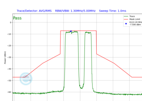
Plot 7-1112 In-Band Emission Plot SDM Primary Antenna 3b (80MHz BW 802.11be(RU) RU484+242 Index92 (UNII Band 5) - Ch.39)
