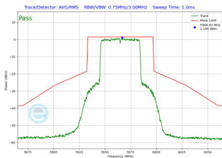
Plot 7-1044 In-Band Emission Plot CDD Primary Antenna 5T (40MHz BW 802.11be(RU) RU484 Index65 (UNII Band 5) - Ch.3)
