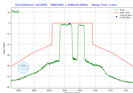
Plot 7-983 In-Band Emission Plot Antenna 1b (80MHz BW 802.11be(RU) RU484+242 Index92 (UNII Band 8) - Ch.215)
