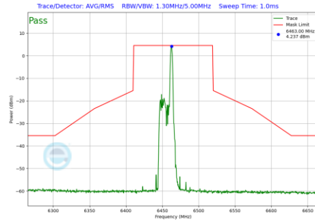
Plot 7-1007 In-Band Emission Plot CDD Primary Antenna 5T (80MHz BW 802.11be(RU) RU26 Index17 (UNII Band 6) - Ch.103)
