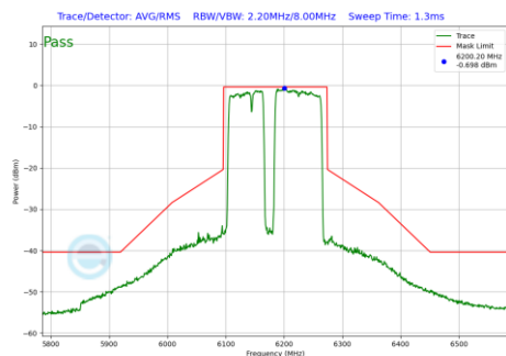
Plot 7-976 In-Band Emission Plot Antenna 1b (160MHz BW 802.11be(RU) RU996+484+242 Index99 (UNII Band 5) - Ch.47)
