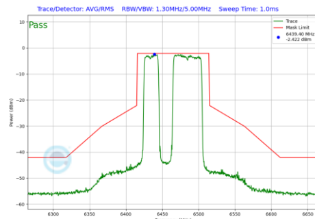
Plot 7-978 In-Band Emission Plot Antenna 1b (80MHz BW 802.11be(RU) RU484+242 Index91 (UNII Band 6) - Ch.103)
