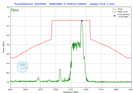
Plot 7-967 In-Band Emission Plot Antenna 1b (40MHz BW 802.11be(RU) RU26 Index17 (UNII Band 7) - Ch.155)
