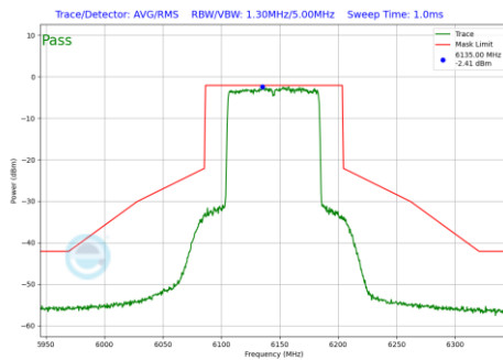
Plot 7-987 In-Band Emission Plot Antenna 1b (80MHz BW 802.11be(RU) RU996 Index67 (UNII Band 5) - Ch.39)
