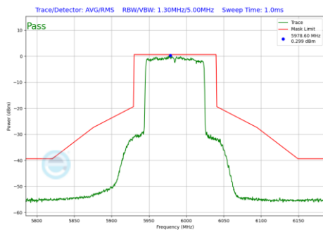
Plot 7-1045 In-Band Emission Plot CDD Primary Antenna 5T (80MHz BW 802.11be(RU) RU996 Index67 (UNII Band 5) - Ch.7)
