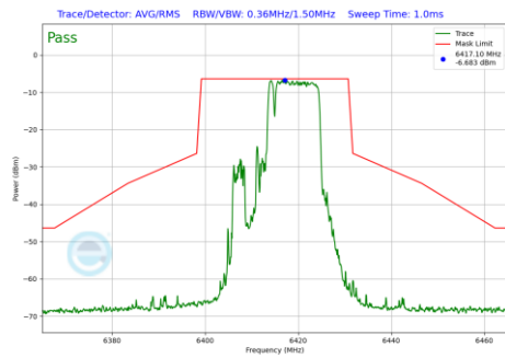
Plot 7-974 In-Band Emission Plot Antenna 1b (20MHz BW 802.11be(RU) RU106+26 Index83 (UNII Band 5) - Ch.93)
