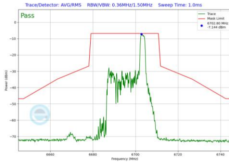
Plot 7-966 In-Band Emission Plot Antenna 1b (20MHz BW 802.11be(RU) RU26 Index8 (UNII Band 7) - Ch.149)
