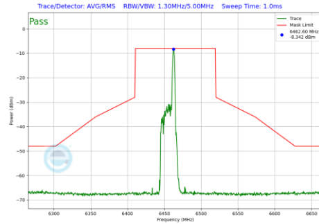
Plot 7-1073 In-Band Emission Plot SDM Primary Antenna 5T (80MHz BW 802.11be(RU) RU26 Index17 (UNII Band 6) - Ch.103)
