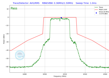
Plot 7-1047 In-Band Emission Plot CDD Primary Antenna 5T (20MHz BW 802.11be(RU) RU242 Index61 (UNII Band 6) - Ch.113)
