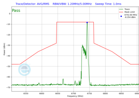
Plot 7-1077 In-Band Emission Plot SDM Primary Antenna 5T (80MHz BW 802.11be(RU) RU26 Index36 (UNII Band 7) - Ch.151)
