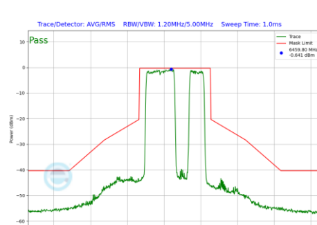
Plot 7-1038 In-Band Emission Plot CDD Primary Antenna 3b (80MHz BW 802.11be(RU) RU484+242 Index92 (UNII Band 6) - Ch.103)
