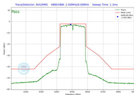
Plot 7-1062 In-Band Emission Plot CDD Primary Antenna 3b (160MHz BW 802.11be(RU) RU996X2 Index68 (UNII Band 6) - Ch.111)
