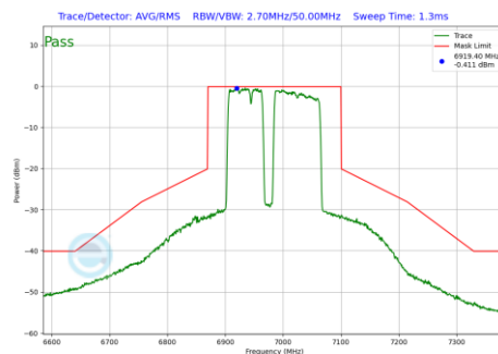
Plot 7-984 In-Band Emission Plot Antenna 1b (160MHz BW 802.11be(RU) RU996+484+242 Index99 (UNII Band 8) - Ch.207)
