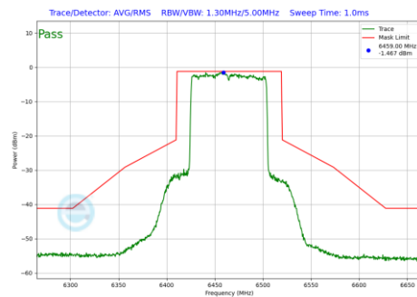
Plot 7-1049 In-Band Emission Plot CDD Primary Antenna 5T (80MHz BW 802.11be(RU) RU996 Index67 (UNII Band 6) - Ch.103)
