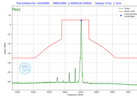
Plot 7-1024 In-Band Emission Plot CDD Primary Antenna 3b (160MHz BW 802.11be(RU) RU26 Index17 (UNII Band 7) - Ch.143)
