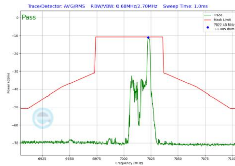
Plot 7-1080 In-Band Emission Plot SDM Primary Antenna 5T (40MHz BW 802.11be(RU) RU26 Index17 (UNII Band 8) - Ch.211)
