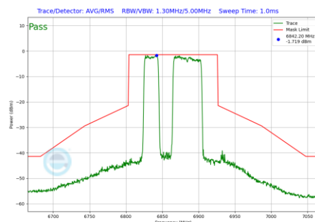
Plot 7-981 In-Band Emission Plot Antenna 1b (80MHz BW 802.11be(RU) RU484+242 Index91 (UNII Band 7) - Ch.183)
