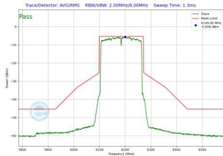
Plot 7-1294 In-Band Emission Plot SDM Diversity Antenna 5T (160MHz BW 802.11be(RU) RU996X2 Index68 (UNII Band 5) - Ch.47)
