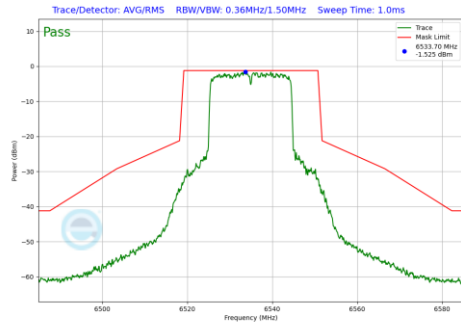
Plot 7-1205 In-Band Emission Plot CDD Diversity Antenna 1b (20MHz BW 802.11be(RU) RU242 Index61 (UNII Band 7) - Ch.117)
