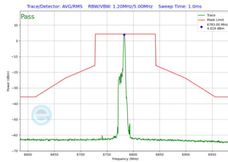
Plot 7-1177 In-Band Emission Plot CDD Diversity Antenna 5T (80MHz BW 802.11be(RU) RU26 Index17 (UNII Band 7) - Ch.167)
