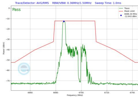
Plot 7-1245 In-Band Emission Plot SDM Diversity Antenna 5T (20MHz BW 802.11be(RU) RU26 Index0 (UNII Band 7) - Ch.149)
