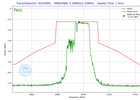
Plot 7-1259 In-Band Emission Plot CDD Diversity Antenna 1b (20MHz BW 802.11be(RU) RU106+26 Index83 (UNII Band 7) - Ch.149)
