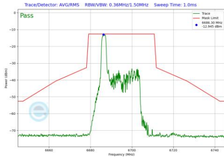
Plot 7-1229 In-Band Emission Plot SDM Diversity Antenna 1b (20MHz BW 802.11be(RU) RU26 Index0 (UNII Band 7) - Ch.149)
