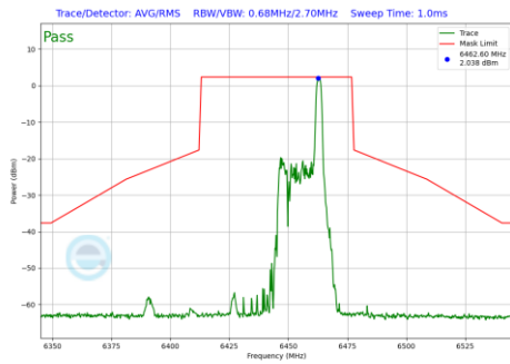
Plot 7-1172 In-Band Emission Plot CDD Diversity Antenna 5T (40MHz BW 802.11be(RU) RU26 Index17 (UNII Band 6) - Ch.99)
