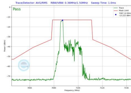
Plot 7-1233 In-Band Emission Plot SDM Diversity Antenna 1b (20MHz BW 802.11be(RU) RU26 Index0 (UNII Band 8) - Ch.229)
