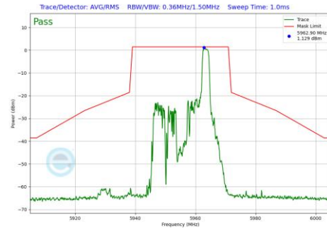
Plot 7-1167 In-Band Emission Plot CDD Diversity Antenna 5T (20MHz BW 802.11be(RU) RU26 Index8 (UNII Band 5) - Ch.1)
