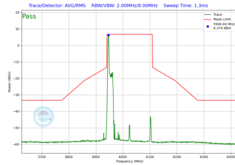
Plot 7-1170 In-Band Emission Plot CDD Diversity Antenna 5T (160MHz BW 802.11be(RU) RU26 Index0 (UNII Band 5) - Ch.15)
