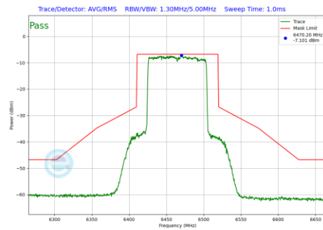
Plot 7-1297 In-Band Emission Plot SDM Diversity Antenna 5T (80MHz BW 802.11be(RU) RU996 Index67 (UNII Band 6) - Ch.103)
