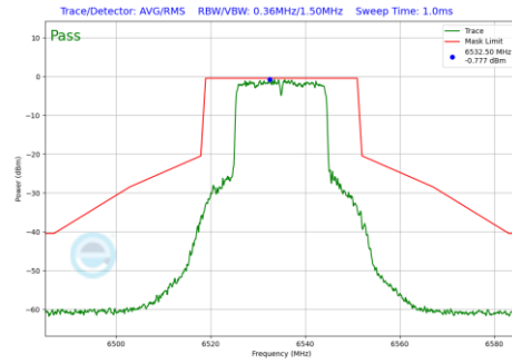
Plot 7-1217 In-Band Emission Plot CDD Diversity Antenna 5T (20MHz BW 802.11be(RU) RU242 Index61 (UNII Band 7) - Ch.117)
