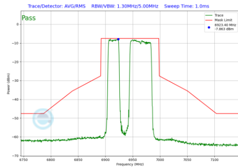
Plot 7-1273 In-Band Emission Plot CDD Diversity Antenna 5T (80MHz BW 802.11be(RU) RU484+242 Index91 (UNII Band 8) - Ch.199)
