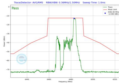
Plot 7-1241 In-Band Emission Plot SDM Diversity Antenna 5T (20MHz BW 802.11be(RU) RU26 Index8 (UNII Band 6) - Ch.105)
