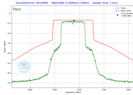
Plot 7-1287 In-Band Emission Plot SDM Diversity Antenna 1b (20MHz BW 802.11be(RU) RU242 Index61 (UNII Band 8) - Ch.233)
