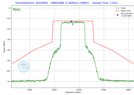
Plot 7-1139 In-Band Emission Plot SDM Primary Antenna 3b (20MHz BW 802.11be(RU) RU242 Index61 (UNII Band 5) - Ch.93)
