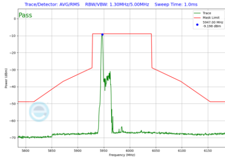
Plot 7-1223 In-Band Emission Plot SDM Diversity Antenna 1b (80MHz BW 802.11be(RU) RU26 Index0 (UNII Band 5) - Ch.7)
