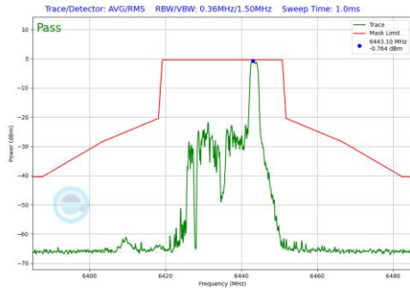
Plot 7-1171 In-Band Emission Plot CDD Diversity Antenna 5T (20MHz BW 802.11be(RU) RU26 Index8 (UNII Band 6) - Ch.97)
