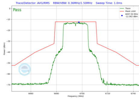
Plot 7-1283 In-Band Emission Plot SDM Diversity Antenna 1b (20MHz BW 802.11be(RU) RU242 Index61 (UNII Band 7) - Ch.149)
