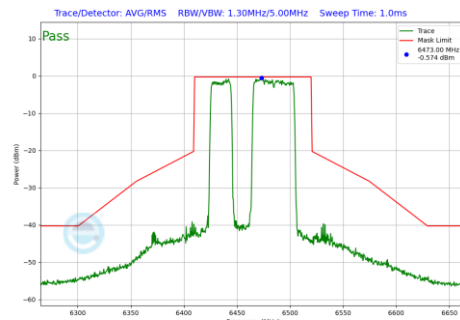
Plot 7-1183 In-Band Emission Plot CDD Diversity Antenna 1b (80MHz BW 802.11be(RU) RU484+242 Index91 (UNII Band 6) - Ch.103)
