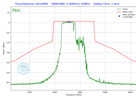
Plot 7-1179 In-Band Emission Plot CDD Diversity Antenna 1b (20MHz BW 802.11be(RU) RU106+26 Index82 (UNII Band 5) - Ch.1)
