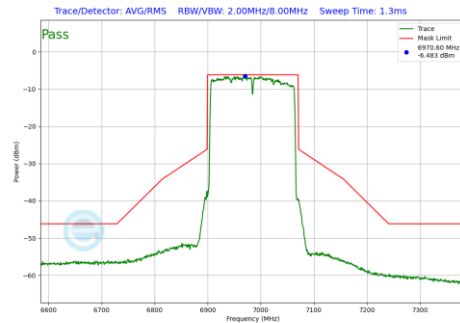
Plot 7-1138 In-Band Emission Plot SDM Primary Antenna 5T (160MHz BW 802.11be(RU) RU996X2 Index68 (UNII Band 8) - Ch.207)
