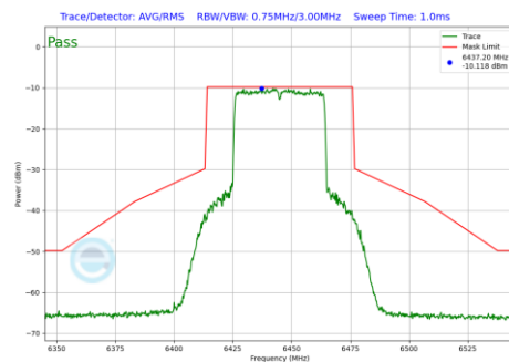
Plot 7-1280 In-Band Emission Plot SDM Diversity Antenna 1b (40MHz BW 802.11be(RU) RU484 Index65 (UNII Band 6) - Ch.99)
