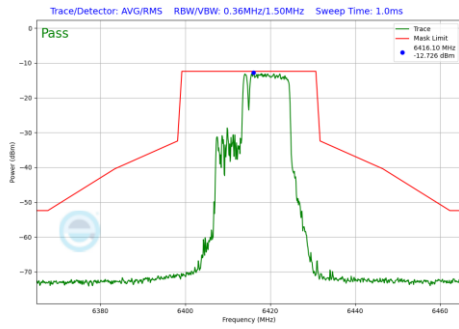
Plot 7-1253 In-Band Emission Plot CDD Diversity Antenna 1b (20MHz BW 802.11be(RU) RU106+26 Index83 (UNII Band 5) - Ch.93)
