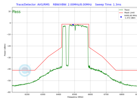
Plot 7-1184 In-Band Emission Plot CDD Diversity Antenna 1b (160MHz BW 802.11be(RU) RU996+484+242 Index97 (UNII Band 6) - Ch.111)
