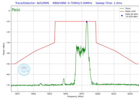
Plot 7-1222 In-Band Emission Plot SDM Diversity Antenna 1b (40MHz BW 802.11be(RU) RU26 Index17 (UNII Band 5) - Ch.3)
