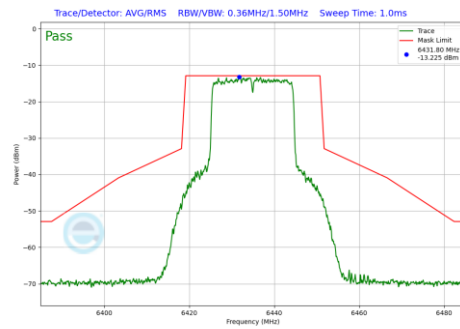
Plot 7-1279 In-Band Emission Plot SDM Diversity Antenna 1b (20MHz BW 802.11be(RU) RU242 Index61 (UNII Band 6) - Ch.97)
