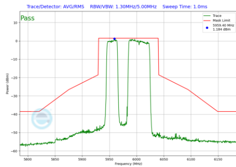
Plot 7-1189 In-Band Emission Plot CDD Diversity Antenna 5T (80MHz BW 802.11be(RU) RU484+242 Index91 (UNII Band 5) - Ch.7)
