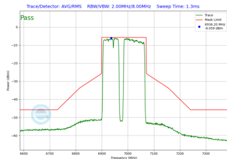
Plot 7-1274 In-Band Emission Plot CDD Diversity Antenna 5T (160MHz BW 802.11be(RU) RU996+484+242 Index99 (UNII Band 8) - Ch.207)
