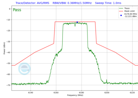
Plot 7-1291 In-Band Emission Plot SDM Diversity Antenna 5T (20MHz BW 802.11be(RU) RU242 Index61 (UNII Band 5) - Ch.45)
