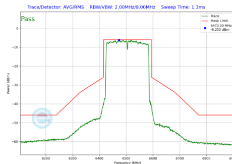
Plot 7-1282 In-Band Emission Plot SDM Diversity Antenna 1b (160MHz BW 802.11be(RU) RU996X2 Index68 (UNII Band 6) - Ch.111)
