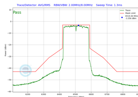
Plot 7-1204 In-Band Emission Plot CDD Diversity Antenna 1b (160MHz BW 802.11be(RU) RU996X2 Index68 (UNII Band 6) - Ch.111)
