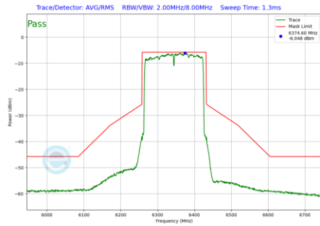
Plot 7-1142 In-Band Emission Plot SDM Primary Antenna 3b (160MHz BW 802.11be(RU) RU996X2 Index68 (UNII Band 5) - Ch.79)
