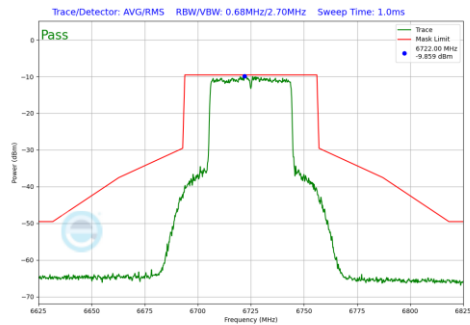
Plot 7-1132 In-Band Emission Plot SDM Primary Antenna 5T (40MHz BW 802.11be(RU) RU484 Index65 (UNII Band 7) - Ch.155)
