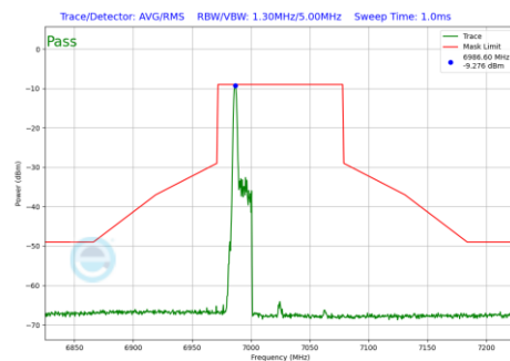
Plot 7-1251 In-Band Emission Plot SDM Diversity Antenna 5T (80MHz BW 802.11be(RU) RU26 Index0 (UNII Band 8) - Ch.215)
