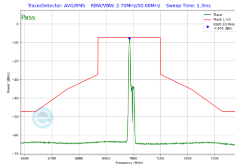
Plot 7-1236 In-Band Emission Plot SDM Diversity Antenna 1b (160MHz BW 802.11be(RU) RU26 Index0 (UNII Band 8) - Ch.207)
