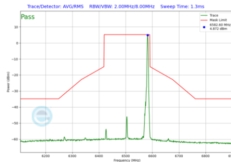
Plot 7-1162 In-Band Emission Plot CDD Diversity Antenna 1b (160MHz BW 802.11be(RU) RU26 Index36 (UNII Band 6) - Ch.111)
