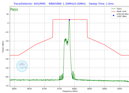
Plot 7-1165 In-Band Emission Plot CDD Diversity Antenna 1b (80MHz BW 802.11be(RU) RU26 Index17 (UNII Band 7) - Ch.167)
