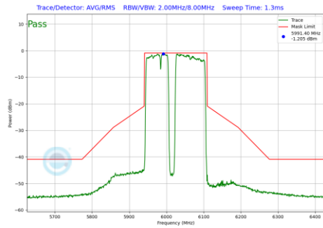
Plot 7-1190 In-Band Emission Plot CDD Diversity Antenna 5T (160MHz BW 802.11be(RU) RU996+484+242 Index99 (UNII Band 5) - Ch.15)
