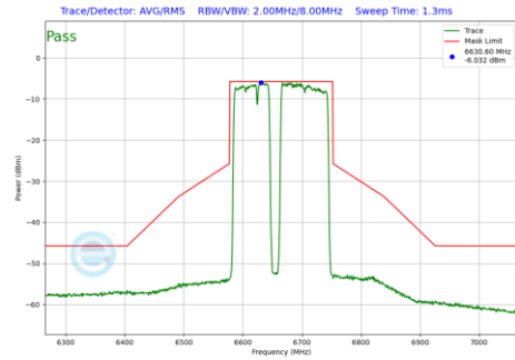
Plot 7-1272 In-Band Emission Plot CDD Diversity Antenna 5T (160MHz BW 802.11be(RU) RU996+484+242 Index99 (UNII Band 7) - Ch.143)
