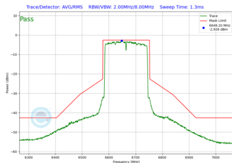
Plot 7-1208 In-Band Emission Plot CDD Diversity Antenna 1b (160MHz BW 802.11be(RU) RU996X2 Index68 (UNII Band 7) - Ch.143)
