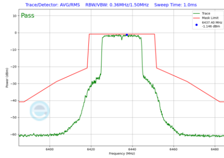
Plot 7-1213 In-Band Emission Plot CDD Diversity Antenna 5T (20MHz BW 802.11be(RU) RU242 Index61 (UNII Band 6) - Ch.97)
