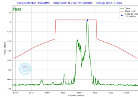
Plot 7-1160 In-Band Emission Plot CDD Diversity Antenna 1b (40MHz BW 802.11be(RU) RU26 Index17 (UNII Band 6) - Ch.99)
