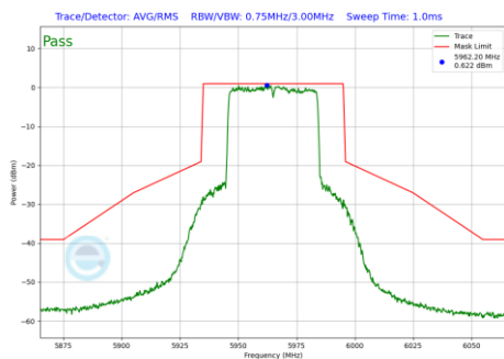
Plot 7-1198 In-Band Emission Plot CDD Diversity Antenna 1b (40MHz BW 802.11be(RU) RU484 Index65 (UNII Band 5) - Ch.3)
