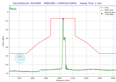
Plot 7-1224 In-Band Emission Plot SDM Diversity Antenna 1b (160MHz BW 802.11be(RU) RU26 Index0 (UNII Band 5) - Ch.15)
