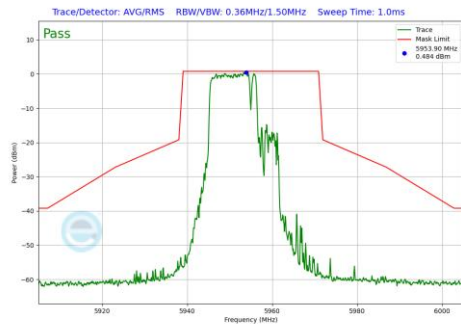
Plot 7-1188 In-Band Emission Plot CDD Diversity Antenna 5T (20MHz BW 802.11be(RU) RU106+26 Index82 (UNII Band 5) - Ch.1)
