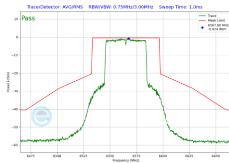
Plot 7-1218 In-Band Emission Plot CDD Diversity Antenna 5T (40MHz BW 802.11be(RU) RU484 Index65 (UNII Band 7) - Ch.123)
