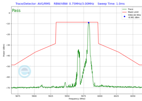
Plot 7-1238 In-Band Emission Plot SDM Diversity Antenna 5T (40MHz BW 802.11be(RU) RU26 Index17 (UNII Band 5) - Ch.3)
