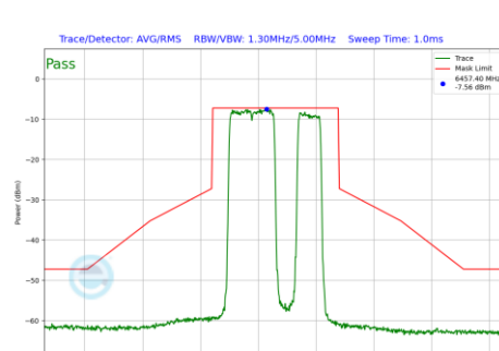
Plot 7-1268 In-Band Emission Plot CDD Diversity Antenna 5T (80MHz BW 802.11be(RU) RU484+242 Index92 (UNII Band 6) - Ch.103)
