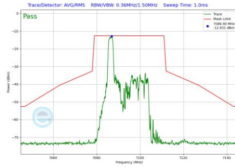
Plot 7-1249 In-Band Emission Plot SDM Diversity Antenna 5T (20MHz BW 802.11be(RU) RU26 Index0 (UNII Band 8) - Ch.229)
