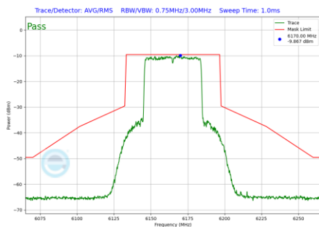
Plot 7-1276 In-Band Emission Plot SDM Diversity Antenna 1b (40MHz BW 802.11be(RU) RU484 Index65 (UNII Band 5) - Ch.43)
