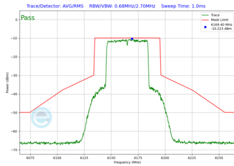
Plot 7-1140 In-Band Emission Plot SDM Primary Antenna 3b (40MHz BW 802.11be(RU) RU484 Index65 (UNII Band 5) - Ch.43)
