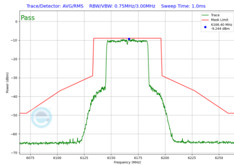
Plot 7-1292 In-Band Emission Plot SDM Diversity Antenna 5T (40MHz BW 802.11be(RU) RU484 Index65 (UNII Band 5) - Ch.43)
