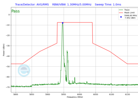
Plot 7-1239 In-Band Emission Plot SDM Diversity Antenna 5T (80MHz BW 802.11be(RU) RU26 Index0 (UNII Band 5) - Ch.7)
