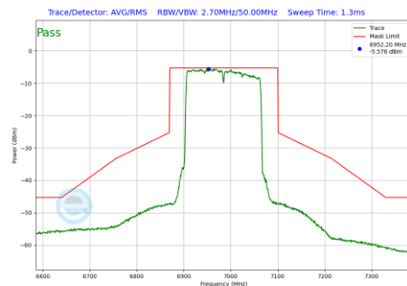
Plot 7-1290 In-Band Emission Plot SDM Diversity Antenna 1b (160MHz BW 802.11be(RU) RU996X2 Index68 (UNII Band 8) - Ch.207)
