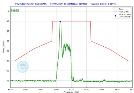
Plot 7-1246 In-Band Emission Plot SDM Diversity Antenna 5T (40MHz BW 802.11be(RU) RU26 Index0 (UNII Band 7) - Ch.155)
