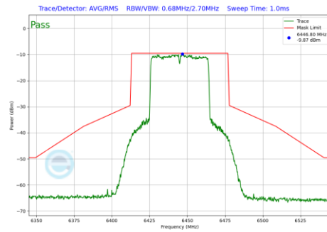
Plot 7-1296 In-Band Emission Plot SDM Diversity Antenna 5T (40MHz BW 802.11be(RU) RU484 Index65 (UNII Band 6) - Ch.99)
