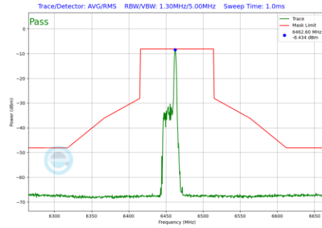
Plot 7-1227 In-Band Emission Plot SDM Diversity Antenna 1b (80MHz BW 802.11be(RU) RU26 Index17 (UNII Band 6) - Ch.103)
