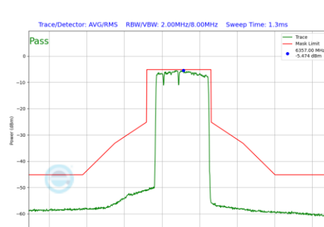
Plot 7-1266 In-Band Emission Plot CDD Diversity Antenna 5T (160MHz BW 802.11be(RU) RU996+484+242 Index96 (UNII Band 5) - Ch.79)
