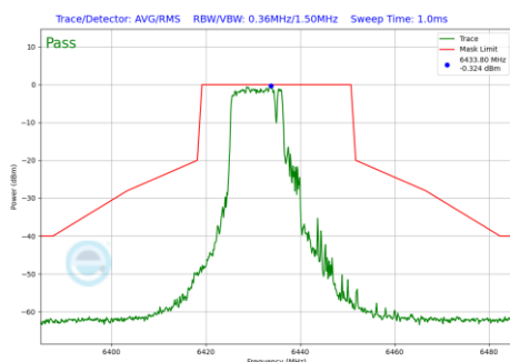
Plot 7-1182 In-Band Emission Plot CDD Diversity Antenna 1b (20MHz BW 802.11be(RU) RU106+26 Index82 (UNII Band 6) - Ch.97)
