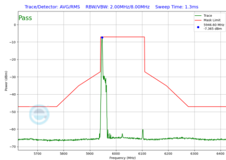
Plot 7-1240 In-Band Emission Plot SDM Diversity Antenna 5T (160MHz BW 802.11be(RU) RU26 Index0 (UNII Band 5) - Ch.15)
