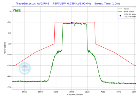
Plot 7-1288 In-Band Emission Plot SDM Diversity Antenna 1b (40MHz BW 802.11be(RU) RU484 Index65 (UNII Band 8) - Ch.211)
