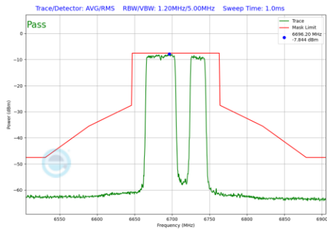
Plot 7-1271 In-Band Emission Plot CDD Diversity Antenna 5T (80MHz BW 802.11be(RU) RU484+242 Index92 (UNII Band 7) - Ch.151)
