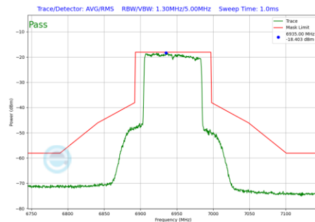
Plot 7-1153 In-Band Emission Plot SDM Primary Antenna 3b (80MHz BW 802.11be(RU) RU996 Index67 (UNII Band 8) - Ch.199)
