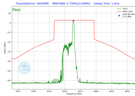
Plot 7-1176 In-Band Emission Plot CDD Diversity Antenna 5T (40MHz BW 802.11be(RU) RU26 Index8 (UNII Band 7) - Ch.123)
