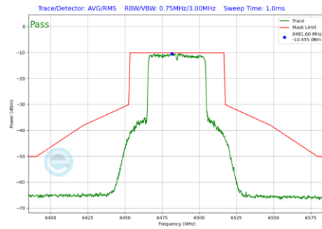
Plot 7-1144 In-Band Emission Plot SDM Primary Antenna 3b (40MHz BW 802.11be(RU) RU484 Index65 (UNII Band 6) - Ch.107)
