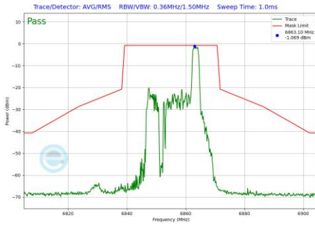
Plot 7-1163 In-Band Emission Plot CDD Diversity Antenna 1b (20MHz BW 802.11be(RU) RU26 Index8 (UNII Band 7) - Ch.181)
