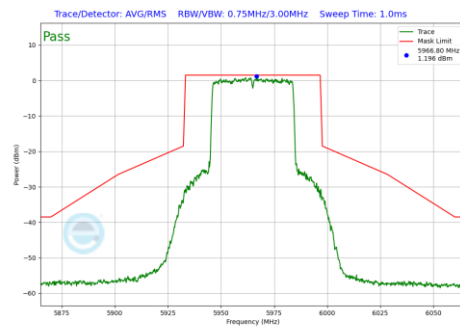
Plot 7-1210 In-Band Emission Plot CDD Diversity Antenna 5T (40MHz BW 802.11be(RU) RU484 Index65 (UNII Band 5) - Ch.3)
