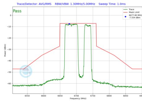
Plot 7-1260 In-Band Emission Plot CDD Diversity Antenna 1b (80MHz BW 802.11be(RU) RU484+242 Index92 (UNII Band 7) - Ch.151)
