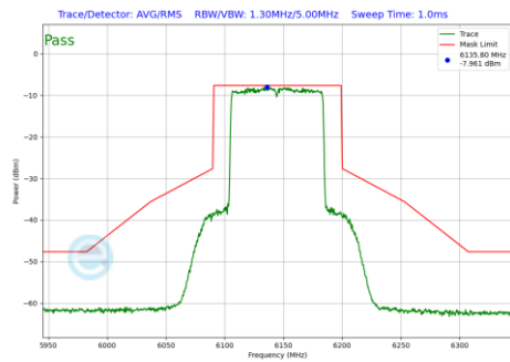
Plot 7-1141 In-Band Emission Plot SDM Primary Antenna 3b (80MHz BW 802.11be(RU) RU996 Index67 (UNII Band 5) - Ch.39)
