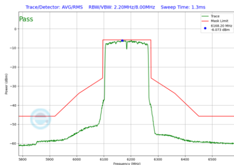
Plot 7-1278 In-Band Emission Plot SDM Diversity Antenna 1b (160MHz BW 802.11be(RU) RU996X2 Index68 (UNII Band 5) - Ch.47)
