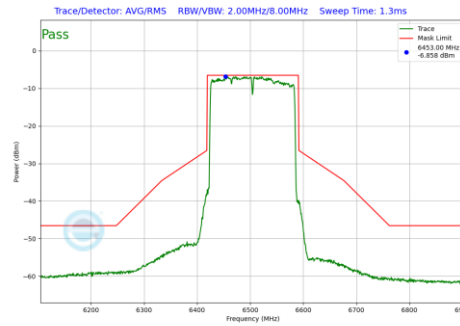
Plot 7-1146 In-Band Emission Plot SDM Primary Antenna 3b (160MHz BW 802.11be(RU) RU996X2 Index68 (UNII Band 6) - Ch.111)
