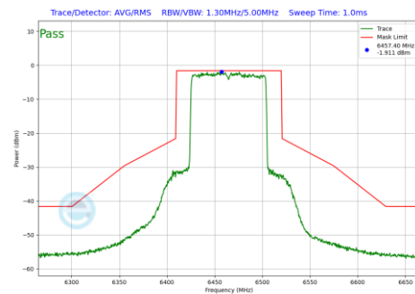
Plot 7-1203 In-Band Emission Plot CDD Diversity Antenna 1b (80MHz BW 802.11be(RU) RU996 Index67 (UNII Band 6) - Ch.103)
