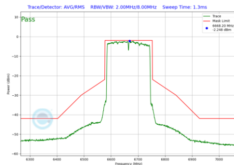
Plot 7-1220 In-Band Emission Plot CDD Diversity Antenna 5T (160MHz BW 802.11be(RU) RU996X2 Index68 (UNII Band 7) - Ch.143)
