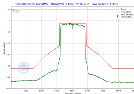
Plot 7-1216 In-Band Emission Plot CDD Diversity Antenna 5T (160MHz BW 802.11be(RU) RU996X2 Index68 (UNII Band 6) - Ch.111)
