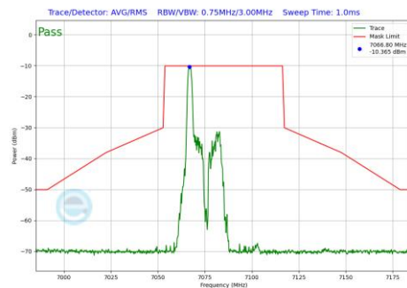
Plot 7-1250 In-Band Emission Plot SDM Diversity Antenna 5T (40MHz BW 802.11be(RU) RU26 Index0 (UNII Band 8) - Ch.227)
