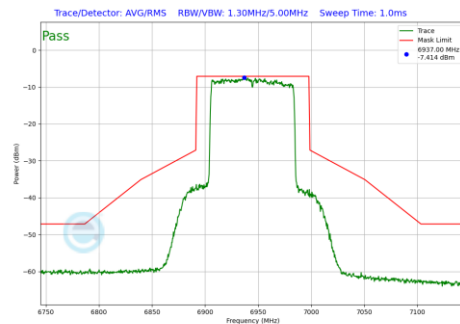
Plot 7-1137 In-Band Emission Plot SDM Primary Antenna 5T (80MHz BW 802.11be(RU) RU996 Index67 (UNII Band 8) - Ch.199)
