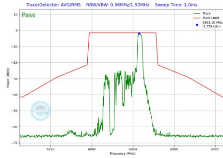
Plot 7-1175 In-Band Emission Plot CDD Diversity Antenna 5T (20MHz BW 802.11be(RU) RU26 Index8 (UNII Band 7) - Ch.181)
