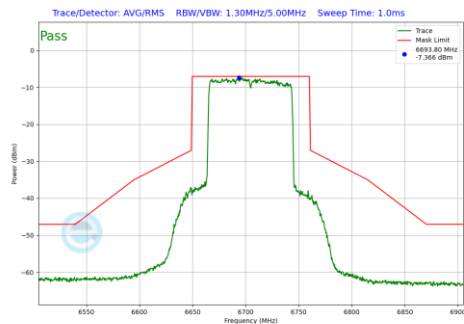
Plot 7-1285 In-Band Emission Plot SDM Diversity Antenna 1b (80MHz BW 802.11be(RU) RU996 Index67 (UNII Band 7) - Ch.151)
