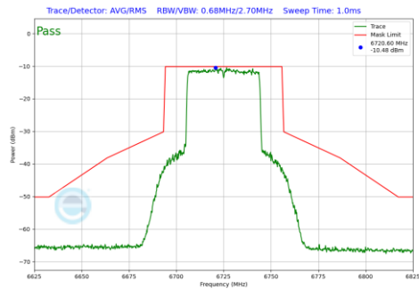
Plot 7-1148 In-Band Emission Plot SDM Primary Antenna 3b (40MHz BW 802.11be(RU) RU484 Index65 (UNII Band 7) - Ch.155)
