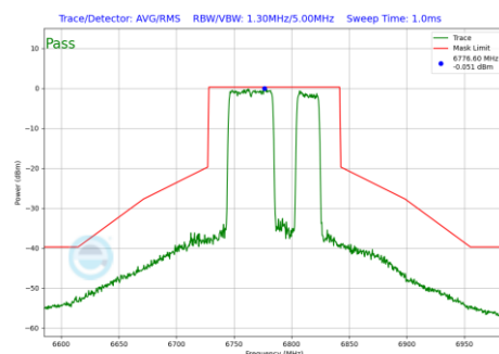
Plot 7-1186 In-Band Emission Plot CDD Diversity Antenna 1b (80MHz BW 802.11be(RU) RU484+242 Index92 (UNII Band 7) - Ch.167)
