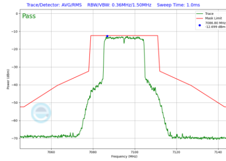
Plot 7-1135 In-Band Emission Plot SDM Primary Antenna 5T (20MHz BW 802.11be(RU) RU242 Index61 (UNII Band 8) - Ch.229)
