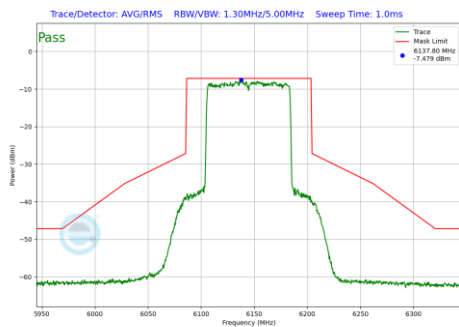
Plot 7-1277 In-Band Emission Plot SDM Diversity Antenna 1b (80MHz BW 802.11be(RU) RU996 Index67 (UNII Band 5) - Ch.39)
