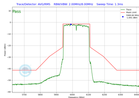
Plot 7-1212 In-Band Emission Plot CDD Diversity Antenna 5T (160MHz BW 802.11be(RU) RU996X2 Index68 (UNII Band 5) - Ch.15)
