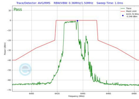
Plot 7-1191 In-Band Emission Plot CDD Diversity Antenna 5T (20MHz BW 802.11be(RU) RU106+26 Index82 (UNII Band 6) - Ch.97)
