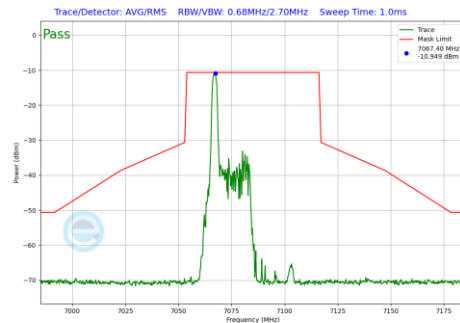
Plot 7-1234 In-Band Emission Plot SDM Diversity Antenna 1b (40MHz BW 802.11be(RU) RU26 Index0 (UNII Band 8) - Ch.227)
