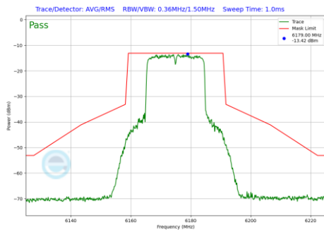
Plot 7-1275 In-Band Emission Plot SDM Diversity Antenna 1b (20MHz BW 802.11be(RU) RU242 Index61 (UNII Band 5) - Ch.45)
