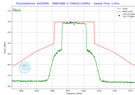
Plot 7-1152 In-Band Emission Plot SDM Primary Antenna 3b (40MHz BW 802.11be(RU) RU484 Index65 (UNII Band 8) - Ch.227)
