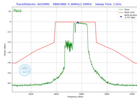
Plot 7-1185 In-Band Emission Plot CDD Diversity Antenna 1b (20MHz BW 802.11be(RU) RU106+26 Index83 (UNII Band 7) - Ch.181)
