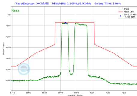
Plot 7-1262 In-Band Emission Plot CDD Diversity Antenna 1b (80MHz BW 802.11be(RU) RU484+242 Index91 (UNII Band 8) - Ch.199)
