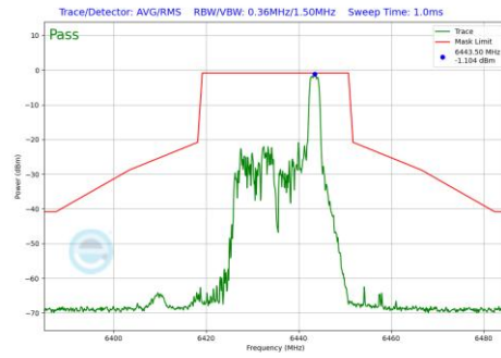
Plot 7-1159 In-Band Emission Plot CDD Diversity Antenna 1b (20MHz BW 802.11be(RU) RU26 Index8 (UNII Band 6) - Ch.97)
