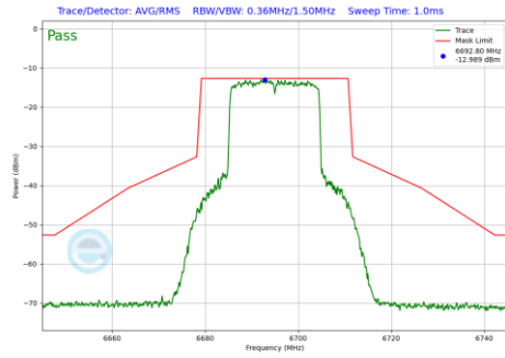
Plot 7-1147 In-Band Emission Plot SDM Primary Antenna 3b (20MHz BW 802.11be(RU) RU242 Index61 (UNII Band 7) - Ch.149)
