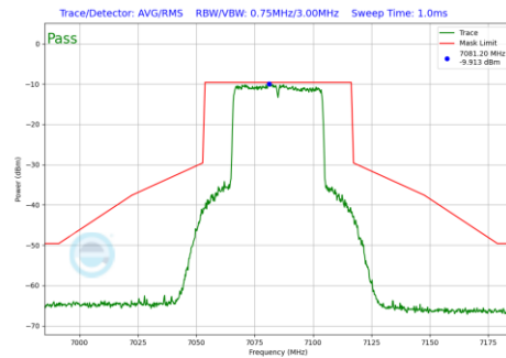
Plot 7-1136 In-Band Emission Plot SDM Primary Antenna 5T (40MHz BW 802.11be(RU) RU484 Index65 (UNII Band 8) - Ch.227)
