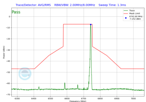
Plot 7-1248 In-Band Emission Plot SDM Diversity Antenna 5T (160MHz BW 802.11be(RU) RU26 Index36 (UNII Band 7) - Ch.143)
