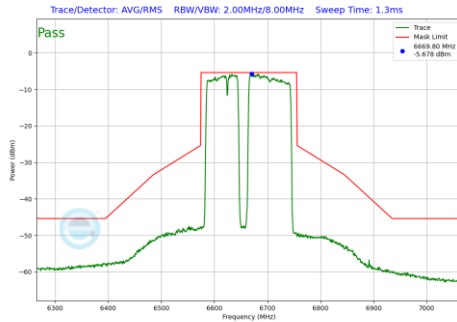
Plot 7-1261 In-Band Emission Plot CDD Diversity Antenna 1b (160MHz BW 802.11be(RU) RU996+484+242 Index99 (UNII Band 7) - Ch.143)
