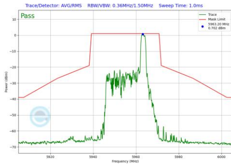
Plot 7-1155 In-Band Emission Plot CDD Diversity Antenna 1b (20MHz BW 802.11be(RU) RU26 Index8 (UNII Band 5) - Ch.1)
