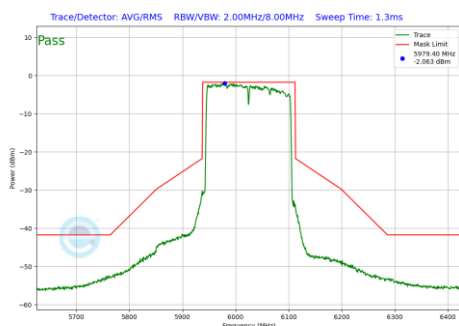
Plot 7-1200 In-Band Emission Plot CDD Diversity Antenna 1b (160MHz BW 802.11be(RU) RU996X2 Index68 (UNII Band 5) - Ch.15)
