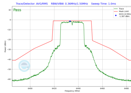
Plot 7-1201 In-Band Emission Plot CDD Diversity Antenna 1b (20MHz BW 802.11be(RU) RU242 Index61 (UNII Band 6) - Ch.97)
