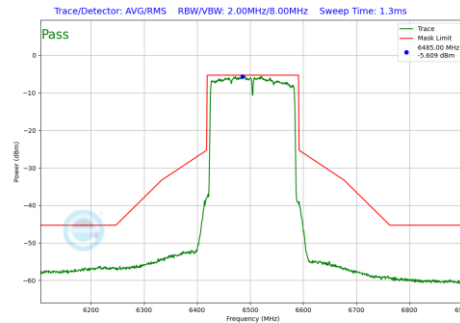
Plot 7-1298 In-Band Emission Plot SDM Diversity Antenna 5T (160MHz BW 802.11be(RU) RU996X2 Index68 (UNII Band 6) - Ch.111)
