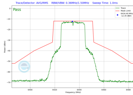
Plot 7-1295 In-Band Emission Plot SDM Diversity Antenna 5T (20MHz BW 802.11be(RU) RU242 Index61 (UNII Band 6) - Ch.97)
