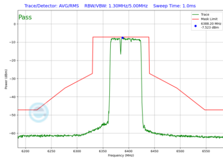
Plot 7-1254 In-Band Emission Plot CDD Diversity Antenna 1b (80MHz BW 802.11be(RU) RU484+242 Index90 (UNII Band 5) - Ch.87)
