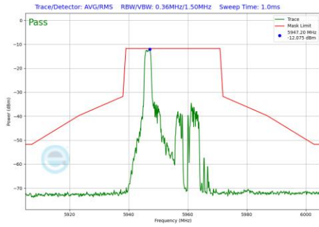
Plot 7-1237 In-Band Emission Plot SDM Diversity Antenna 5T (20MHz BW 802.11be(RU) RU26 Index0 (UNII Band 5) - Ch.1)
