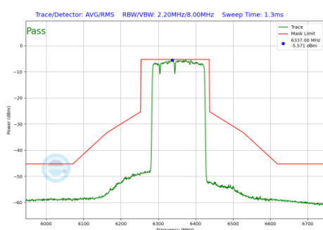
Plot 7-1255 In-Band Emission Plot CDD Diversity Antenna 1b (160MHz BW 802.11be(RU) RU996+484+242 Index96 (UNII Band 5) - Ch.79)
