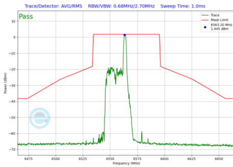
Plot 7-1164 In-Band Emission Plot CDD Diversity Antenna 1b (40MHz BW 802.11be(RU) RU26 Index8 (UNII Band 7) - Ch.123)
