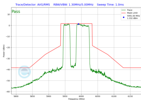
Plot 7-1180 In-Band Emission Plot CDD Diversity Antenna 1b (80MHz BW 802.11be(RU) RU484+242 Index91 (UNII Band 5) - Ch.7)
