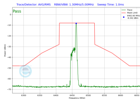
Plot 7-1243 In-Band Emission Plot SDM Diversity Antenna 5T (80MHz BW 802.11be(RU) RU26 Index17 (UNII Band 6) - Ch.103)
