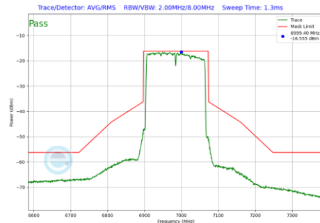
Plot 7-1154 In-Band Emission Plot SDM Primary Antenna 3b (160MHz BW 802.11be(RU) RU996X2 Index68 (UNII Band 8) - Ch.207)
