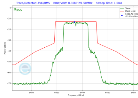
Plot 7-1143 In-Band Emission Plot SDM Primary Antenna 3b (20MHz BW 802.11be(RU) RU242 Index61 (UNII Band 6) - Ch.97)
