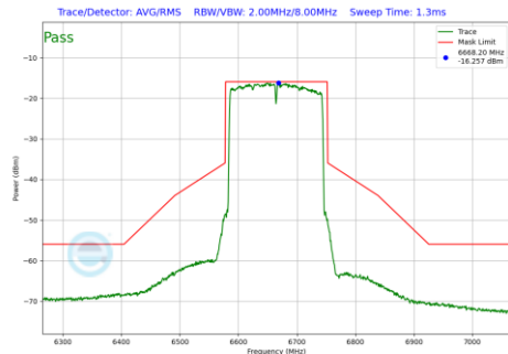
Plot 7-1150 In-Band Emission Plot SDM Primary Antenna 3b (160MHz BW 802.11be(RU) RU996X2 Index68 (UNII Band 7) - Ch.143)
