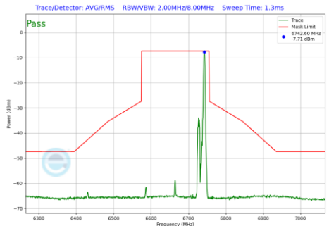
Plot 7-1232 In-Band Emission Plot SDM Diversity Antenna 1b (160MHz BW 802.11be(RU) RU26 Index36 (UNII Band 7) - Ch.143)
