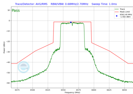
Plot 7-1206 In-Band Emission Plot CDD Diversity Antenna 1b (40MHz BW 802.11be(RU) RU484 Index65 (UNII Band 7) - Ch.123)
