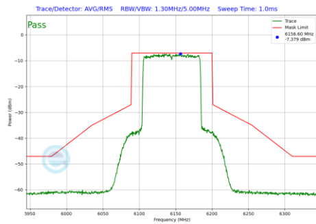
Plot 7-1293 In-Band Emission Plot SDM Diversity Antenna 5T (80MHz BW 802.11be(RU) RU996 Index67 (UNII Band 5) - Ch.39)
