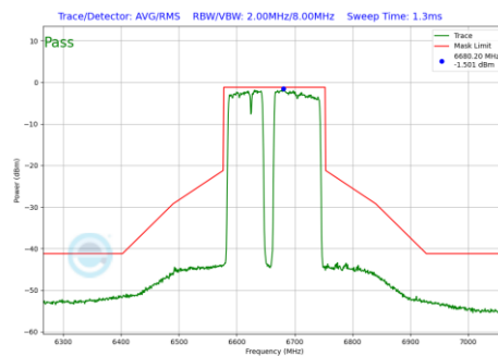
Plot 7-1196 In-Band Emission Plot CDD Diversity Antenna 5T (160MHz BW 802.11be(RU) RU996+484+242 Index99 (UNII Band 7) - Ch.143)
