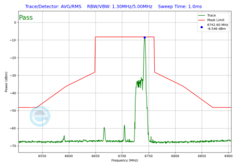
Plot 7-1231 In-Band Emission Plot SDM Diversity Antenna 1b (80MHz BW 802.11be(RU) RU26 Index36 (UNII Band 7) - Ch.151)
