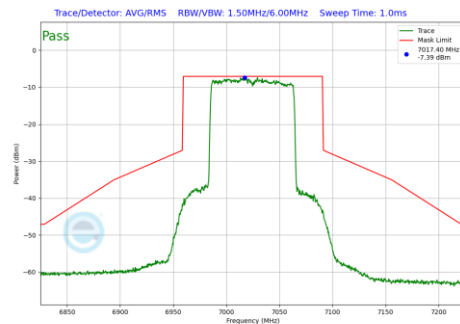
Plot 7-1289 In-Band Emission Plot SDM Diversity Antenna 1b (80MHz BW 802.11be(RU) RU996 Index67 (UNII Band 8) - Ch.215)
