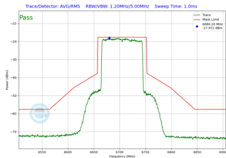
Plot 7-1149 In-Band Emission Plot SDM Primary Antenna 3b (80MHz BW 802.11be(RU) RU996 Index67 (UNII Band 7) - Ch.151)
