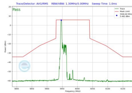
Plot 7-1169 In-Band Emission Plot CDD Diversity Antenna 5T (80MHz BW 802.11be(RU) RU26 Index0 (UNII Band 5) - Ch.7)
