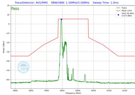
Plot 7-1157 In-Band Emission Plot CDD Diversity Antenna 1b (80MHz BW 802.11be(RU) RU26 Index0 (UNII Band 5) - Ch.7)
