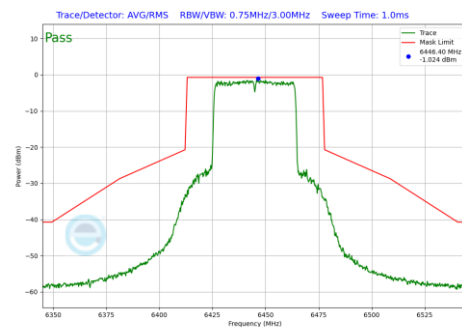
Plot 7-1202 In-Band Emission Plot CDD Diversity Antenna 1b (40MHz BW 802.11be(RU) RU484 Index65 (UNII Band 6) - Ch.99)
