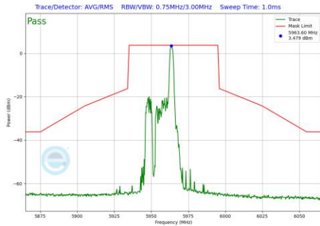
Plot 7-1156 In-Band Emission Plot CDD Diversity Antenna 1b (40MHz BW 802.11be(RU) RU26 Index8 (UNII Band 5) - Ch.3)
