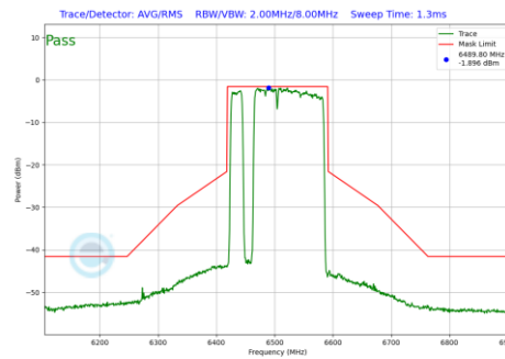
Plot 7-1193 In-Band Emission Plot CDD Diversity Antenna 5T (160MHz BW 802.11be(RU) RU996+484+242 Index97 (UNII Band 6) - Ch.111)
