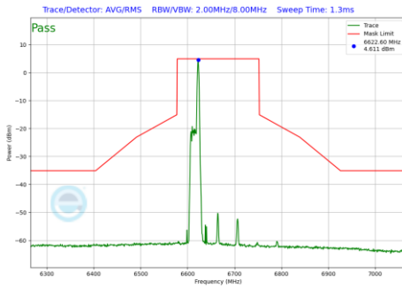
Plot 7-1166 In-Band Emission Plot CDD Diversity Antenna 1b (160MHz BW 802.11be(RU) RU26 Index17 (UNII Band 7) - Ch.143)
