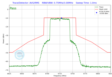
Plot 7-1284 In-Band Emission Plot SDM Diversity Antenna 1b (40MHz BW 802.11be(RU) RU484 Index65 (UNII Band 7) - Ch.155)
