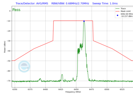
Plot 7-1242 In-Band Emission Plot SDM Diversity Antenna 5T (40MHz BW 802.11be(RU) RU26 Index17 (UNII Band 6) - Ch.99)
