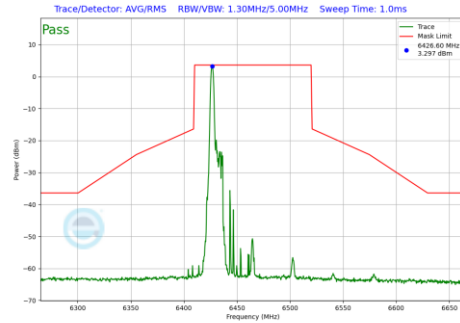
Plot 7-1161 In-Band Emission Plot CDD Diversity Antenna 1b (80MHz BW 802.11be(RU) RU26 Index0 (UNII Band 6) - Ch.103)
