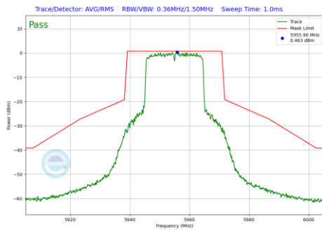
Plot 7-1197 In-Band Emission Plot CDD Diversity Antenna 1b (20MHz BW 802.11be(RU) RU242 Index61 (UNII Band 5) - Ch.1)
