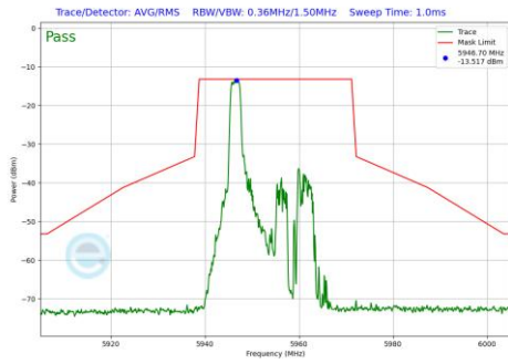
Plot 7-1221 In-Band Emission Plot SDM Diversity Antenna 1b (20MHz BW 802.11be(RU) RU26 Index0 (UNII Band 5) - Ch.1)
