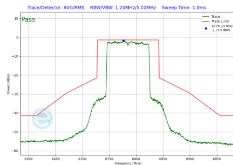
Plot 7-1219 In-Band Emission Plot CDD Diversity Antenna 5T (80MHz BW 802.11be(RU) RU996 Index67 (UNII Band 7) - Ch.167)
