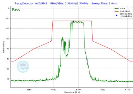
Plot 7-1270 In-Band Emission Plot CDD Diversity Antenna 5T (20MHz BW 802.11be(RU) RU106+26 Index83 (UNII Band 7) - Ch.149)
