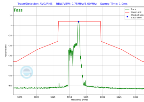
Plot 7-1168 In-Band Emission Plot CDD Diversity Antenna 5T (40MHz BW 802.11be(RU) RU26 Index8 (UNII Band 5) - Ch.3)
