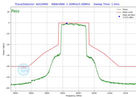
Plot 7-1199 In-Band Emission Plot CDD Diversity Antenna 1b (80MHz BW 802.11be(RU) RU996 Index67 (UNII Band 5) - Ch.7)
