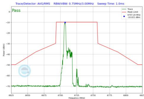
Plot 7-1230 In-Band Emission Plot SDM Diversity Antenna 1b (40MHz BW 802.11be(RU) RU26 Index0 (UNII Band 7) - Ch.155)
