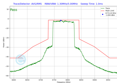
Plot 7-1207 In-Band Emission Plot CDD Diversity Antenna 1b (80MHz BW 802.11be(RU) RU996 Index67 (UNII Band 7) - Ch.167)
