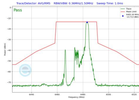
Plot 7-1225 In-Band Emission Plot SDM Diversity Antenna 1b (20MHz BW 802.11be(RU) RU26 Index8 (UNII Band 6) - Ch.105)
