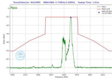
Plot 7-1226 In-Band Emission Plot SDM Diversity Antenna 1b (40MHz BW 802.11be(RU) RU26 Index17 (UNII Band 6) - Ch.99)
