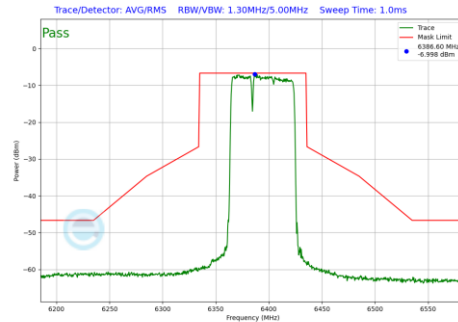
Plot 7-1265 In-Band Emission Plot CDD Diversity Antenna 5T (80MHz BW 802.11be(RU) RU484+242 Index90 (UNII Band 5) - Ch.87)
