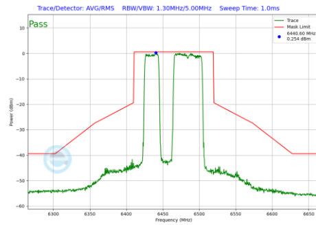
Plot 7-1192 In-Band Emission Plot CDD Diversity Antenna 5T (80MHz BW 802.11be(RU) RU484+242 Index91 (UNII Band 6) - Ch.103)
