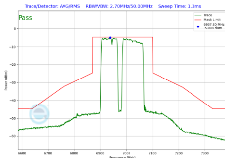
Plot 7-1263 In-Band Emission Plot CDD Diversity Antenna 1b (160MHz BW 802.11be(RU) RU996+484+242 Index99 (UNII Band 8) - Ch.207)
