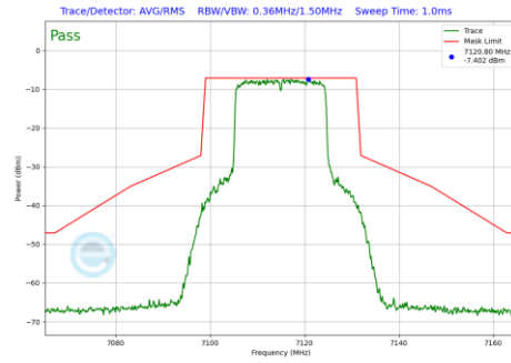
Plot 7-1151 In-Band Emission Plot SDM Primary Antenna 3b (20MHz BW 802.11be(RU) RU242 Index61 (UNII Band 8) - Ch.233)
