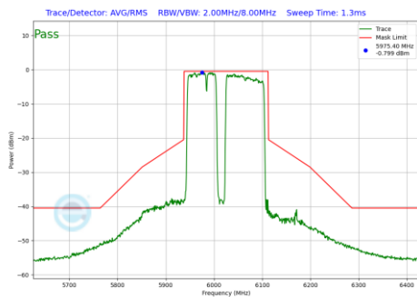
Plot 7-1181 In-Band Emission Plot CDD Diversity Antenna 1b (160MHz BW 802.11be(RU) RU996+484+242 Index99 (UNII Band 5) - Ch.15)
