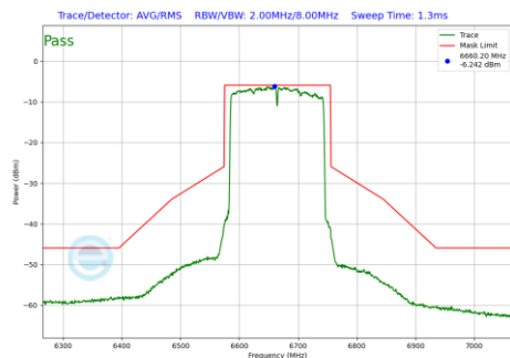
Plot 7-1286 In-Band Emission Plot SDM Diversity Antenna 1b (160MHz BW 802.11be(RU) RU996X2 Index68 (UNII Band 7) - Ch.143)
