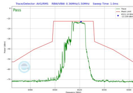
Plot 7-1267 In-Band Emission Plot CDD Diversity Antenna 5T (20MHz BW 802.11be(RU) RU106+26 Index83 (UNII Band 6) - Ch.113)
