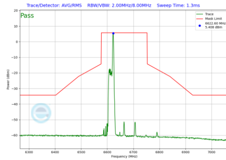
Plot 7-1178 In-Band Emission Plot CDD Diversity Antenna 5T (160MHz BW 802.11be(RU) RU26 Index17 (UNII Band 7) - Ch.143)
