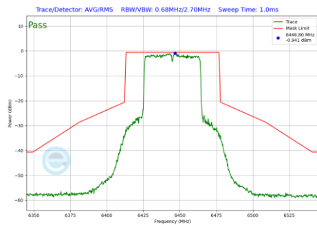
Plot 7-1214 In-Band Emission Plot CDD Diversity Antenna 5T (40MHz BW 802.11be(RU) RU484 Index65 (UNII Band 6) - Ch.99)
