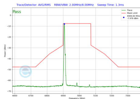
Plot 7-1252 In-Band Emission Plot SDM Diversity Antenna 5T (160MHz BW 802.11be(RU) RU26 Index0 (UNII Band 8) - Ch.207)
