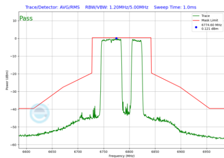
Plot 7-1195 In-Band Emission Plot CDD Diversity Antenna 5T (80MHz BW 802.11be(RU) RU484+242 Index92 (UNII Band 7) - Ch.167)
