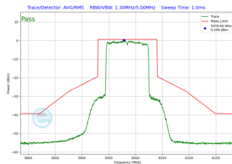
Plot 7-1211 In-Band Emission Plot CDD Diversity Antenna 5T (80MHz BW 802.11be(RU) RU996 Index67 (UNII Band 5) - Ch.7)
