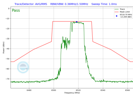
Plot 7-1256 In-Band Emission Plot CDD Diversity Antenna 1b (20MHz BW 802.11be(RU) RU106+26 Index83 (UNII Band 6) - Ch.113)
