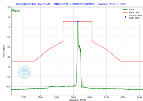
Plot 7-1158 In-Band Emission Plot CDD Diversity Antenna 1b (160MHz BW 802.11be(RU) RU26 Index0 (UNII Band 5) - Ch.15)
