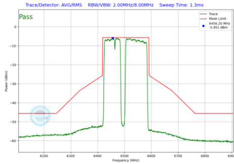
Plot 7-1269 In-Band Emission Plot CDD Diversity Antenna 5T (160MHz BW 802.11be(RU) RU996+484+242 Index99 (UNII Band 6) - Ch.111)
