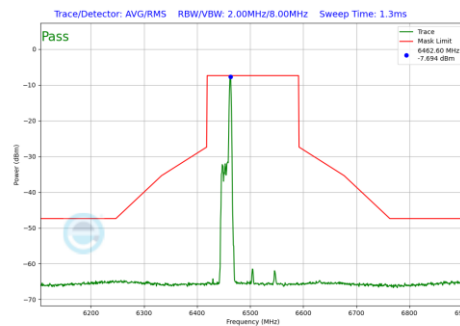
Plot 7-1244 In-Band Emission Plot SDM Diversity Antenna 5T (160MHz BW 802.11be(RU) RU26 Index17 (UNII Band 6) - Ch.111)
