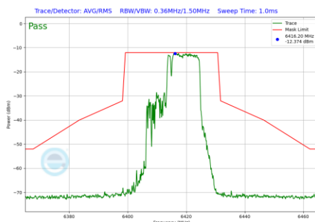
Plot 7-1264 In-Band Emission Plot CDD Diversity Antenna 5T (20MHz BW 802.11be(RU) RU106+26 Index83 (UNII Band 5) - Ch.93)
