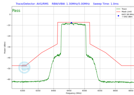
Plot 7-1145 In-Band Emission Plot SDM Primary Antenna 3b (80MHz BW 802.11be(RU) RU996 Index67 (UNII Band 6) - Ch.103)
