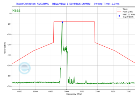
Plot 7-1235 In-Band Emission Plot SDM Diversity Antenna 1b (80MHz BW 802.11be(RU) RU26 Index0 (UNII Band 8) - Ch.215)
