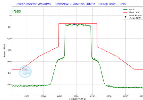
Plot 7-1133 In-Band Emission Plot SDM Primary Antenna 5T (80MHz BW 802.11be(RU) RU996 Index67 (UNII Band 7) - Ch.151)
