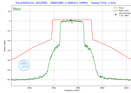
Plot 7-1209 In-Band Emission Plot CDD Diversity Antenna 5T (20MHz BW 802.11be(RU) RU242 Index61 (UNII Band 5) - Ch.1)
