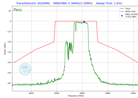
Plot 7-1194 In-Band Emission Plot CDD Diversity Antenna 5T (20MHz BW 802.11be(RU) RU106+26 Index83 (UNII Band 7) - Ch.181)
