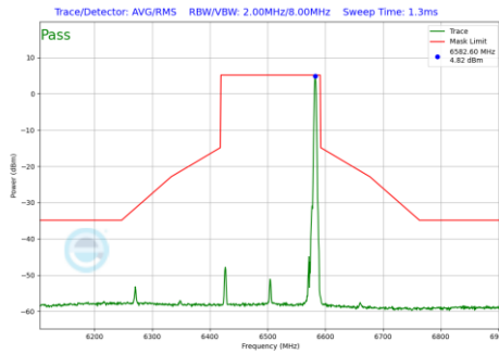
Plot 7-1174 In-Band Emission Plot CDD Diversity Antenna 5T (160MHz BW 802.11be(RU) RU26 Index36 (UNII Band 6) - Ch.111)
