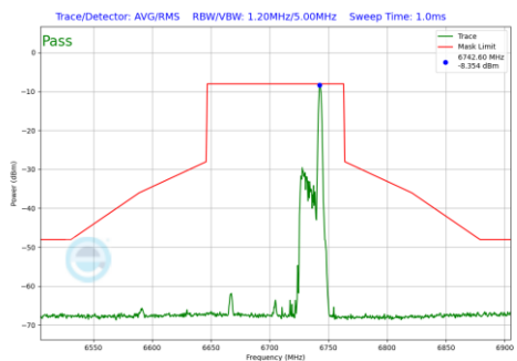
Plot 7-1247 In-Band Emission Plot SDM Diversity Antenna 5T (80MHz BW 802.11be(RU) RU26 Index36 (UNII Band 7) - Ch.151)
