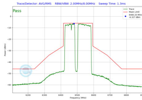
Plot 7-1258 In-Band Emission Plot CDD Diversity Antenna 1b (160MHz BW 802.11be(RU) RU996+484+242 Index99 (UNII Band 6) - Ch.111)
