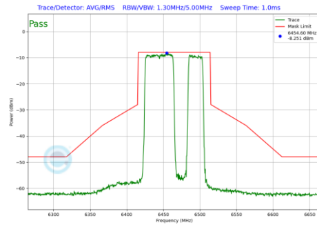
Plot 7-1257 In-Band Emission Plot CDD Diversity Antenna 1b (80MHz BW 802.11be(RU) RU484+242 Index92 (UNII Band 6) - Ch.103)
