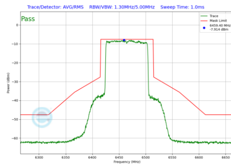
Plot 7-1281 In-Band Emission Plot SDM Diversity Antenna 1b (80MHz BW 802.11be(RU) RU996 Index67 (UNII Band 6) - Ch.103)
