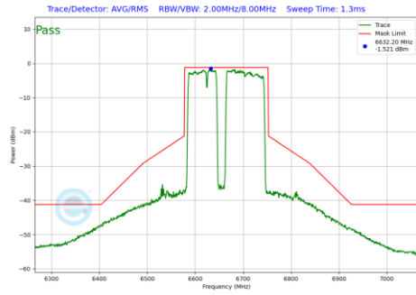
Plot 7-1187 In-Band Emission Plot CDD Diversity Antenna 1b (160MHz BW 802.11be(RU) RU996+484+242 Index99 (UNII Band 7) - Ch.143)
