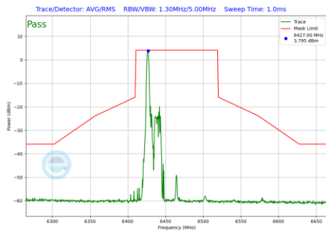
Plot 7-1173 In-Band Emission Plot CDD Diversity Antenna 5T (80MHz BW 802.11be(RU) RU26 Index0 (UNII Band 6) - Ch.103)
