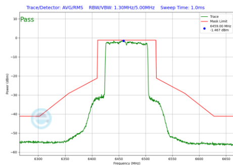
Plot 7-1215 In-Band Emission Plot CDD Diversity Antenna 5T (80MHz BW 802.11be(RU) RU996 Index67 (UNII Band 6) - Ch.103)
