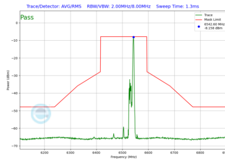
Plot 7-1228 In-Band Emission Plot SDM Diversity Antenna 1b (160MHz BW 802.11be(RU) RU26 Index17 (UNII Band 6) - Ch.111)
