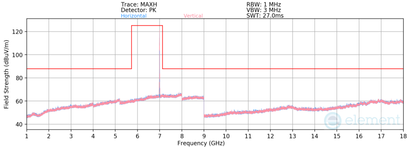
Plot 7-1371. Radiated Spurious Emissions above 1GHz SDM Primary (802.11be – Ch. 209 – RU26)
