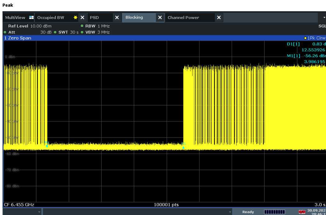
Plot 7-1343. Contention Based Protocol Timing Plot – UNII 6 – 20MHz Channel 101
