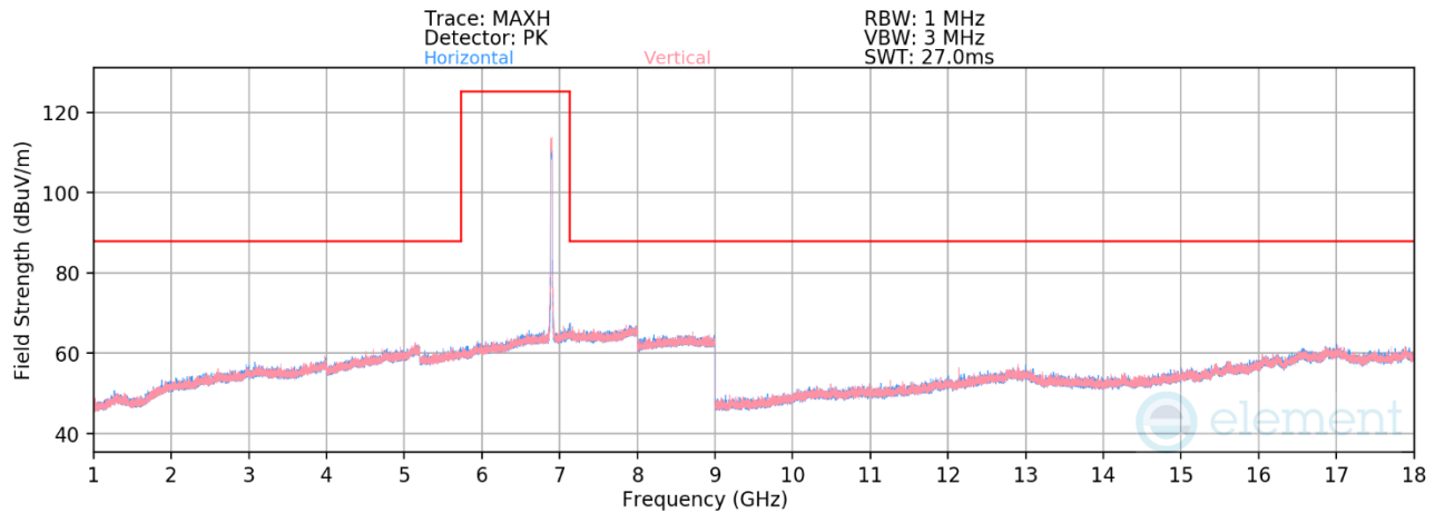
Plot 7-1386. Radiated Spurious Emissions above 1GHz SDM Primary (802.11be – Ch. 189 – RU242)
