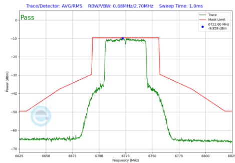
Plot 7-1300 In-Band Emission Plot SDM Diversity Antenna 5T (40MHz BW 802.11be(RU) RU484 Index65 (UNII Band 7) - Ch.155)
