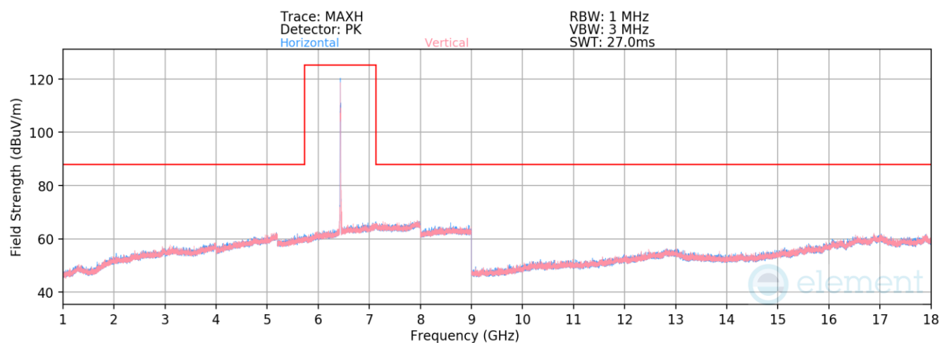
Plot 7-1362. Radiated Spurious Emissions above 1GHz CDD Primary (802.11be – Ch. 97 – RU26)
