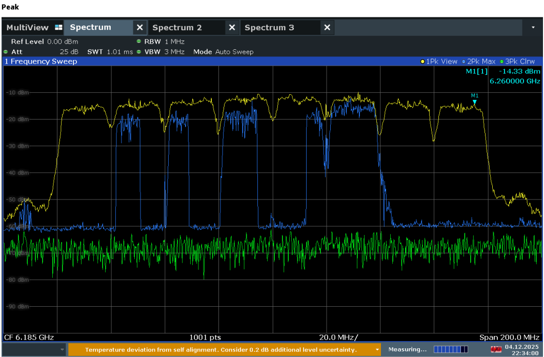
Plot 7-1357. 160MHz Bandwidth, AWGN Signal Injected – 6260MHz
