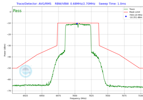
Plot 7-1304 In-Band Emission Plot SDM Diversity Antenna 5T (40MHz BW 802.11be(RU) RU484 Index65 (UNII Band 8) - Ch.211)
