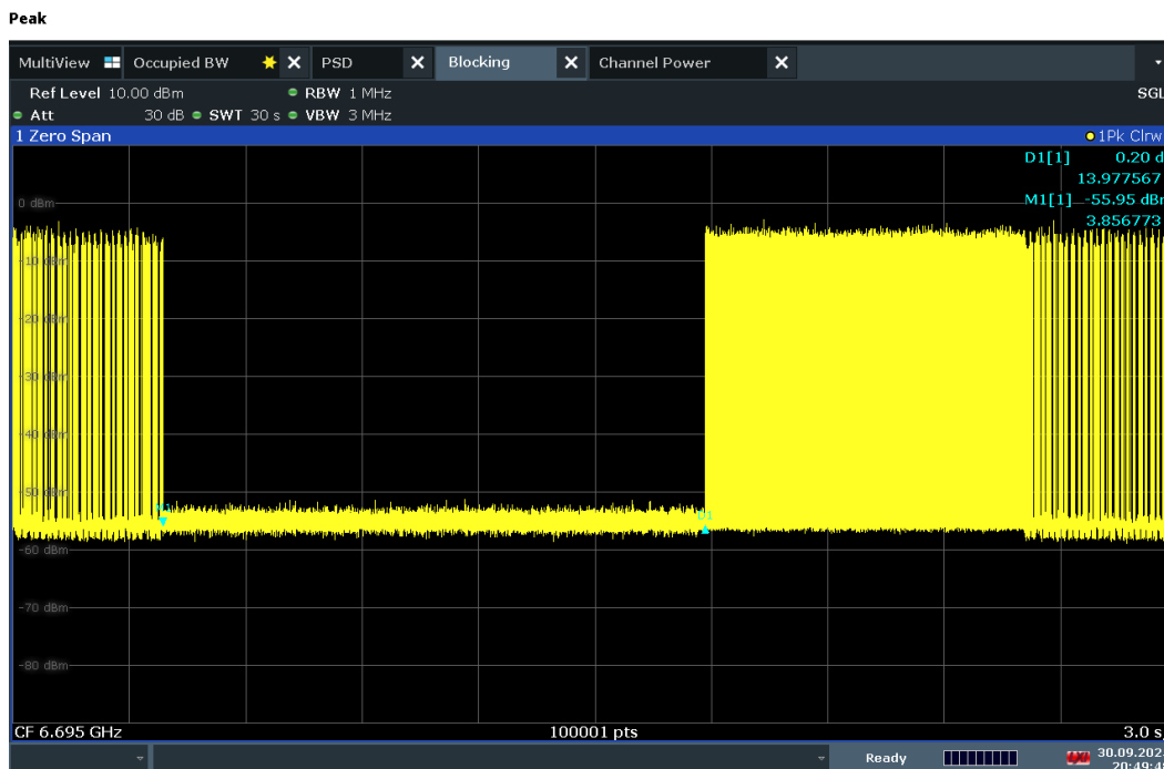
Plot 7-1347. Contention Based Protocol Timing Plot – UNII 7 – 20MHz Channel 149
