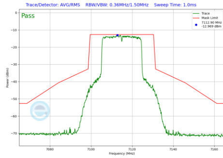
Plot 7-1303 In-Band Emission Plot SDM Diversity Antenna 5T (20MHz BW 802.11be(RU) RU242 Index61 (UNII Band 8) - Ch.233)
