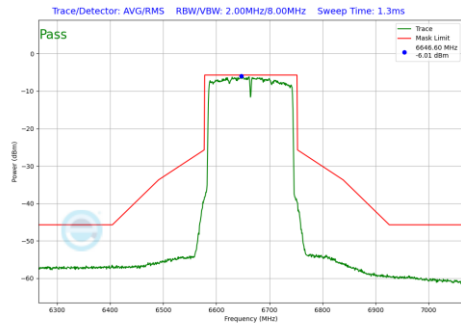
Plot 7-1302 In-Band Emission Plot SDM Diversity Antenna 5T (160MHz BW 802.11be(RU) RU996X2 Index68 (UNII Band 7) - Ch.143)
