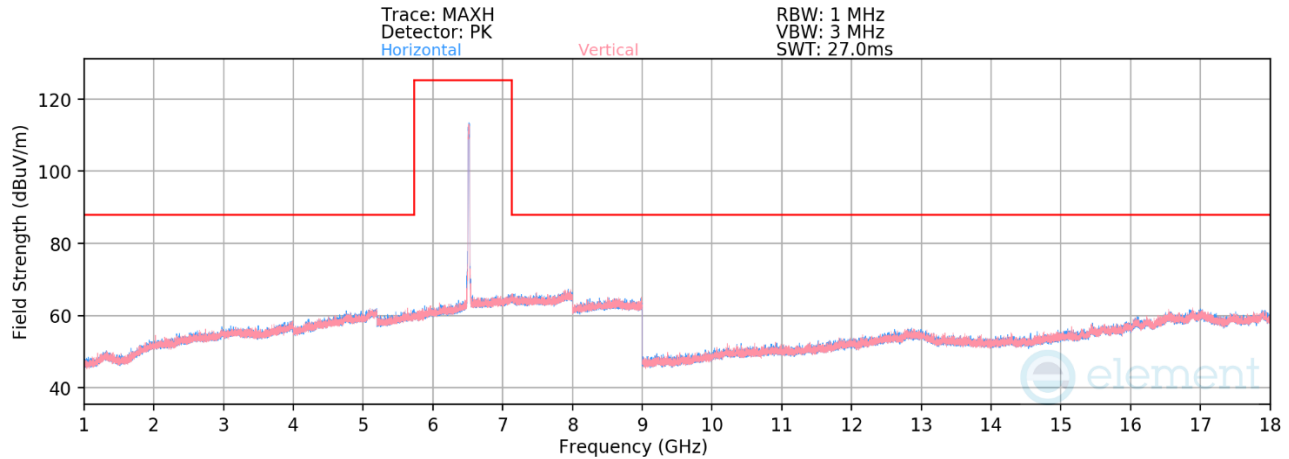
Plot 7-1381. Radiated Spurious Emissions above 1GHz CDD Primary (802.11be – Ch. 113 – RU242)
