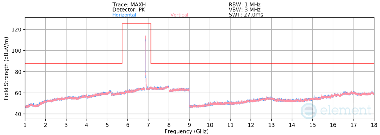
Plot 7-1385. Radiated Spurious Emissions above 1GHz SDM Primary (802.11be – Ch. 185 – RU242)
