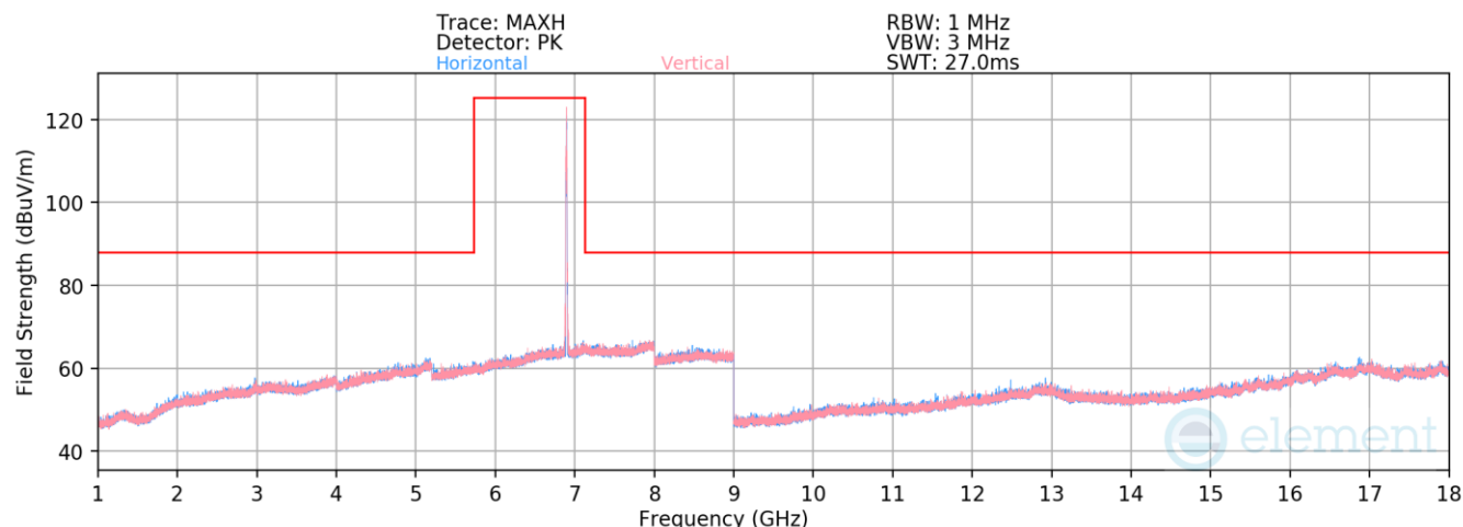
Plot 7-1370. Radiated Spurious Emissions above 1GHz SDM Primary (802.11be – Ch. 189 – RU26)
