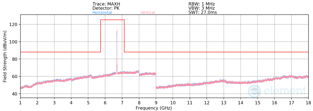
Plot 7-1383. Radiated Spurious Emissions above 1GHz CDD Primary (802.11be – Ch. 149 – RU242)
