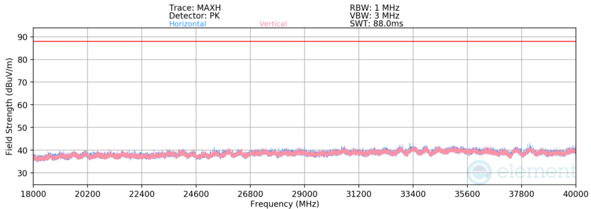
Plot 7-1372. Radiated Spurious Emissions 18-40GHz SDM Primary (802.11be – Ch. 209 – RU26)
