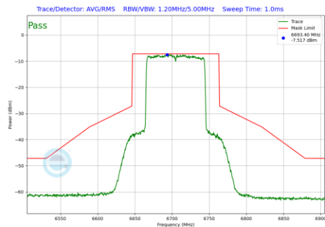
Plot 7-1301 In-Band Emission Plot SDM Diversity Antenna 5T (80MHz BW 802.11be(RU) RU996 Index67 (UNII Band 7) - Ch.151)
