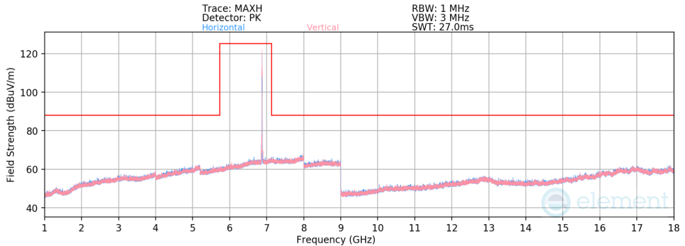
Plot 7-1369. Radiated Spurious Emissions above 1GHz SDM Primary (802.11be – Ch. 185 – RU26)
