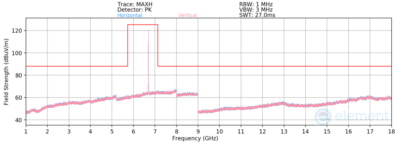
Plot 7-1367. Radiated Spurious Emissions above 1GHz CDD Primary (802.11be – Ch. 149 – RU26)
