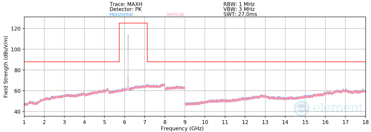
Plot 7-1375. Radiated Spurious Emissions above 1GHz CDD Primary (802.11be – Ch. 45 – RU242)
