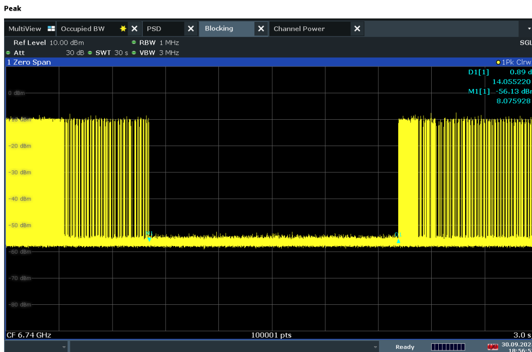
Plot 7-1349. Contention Based Protocol Timing Plot – UNII 7 – 160MHz Channel 143 – Mid
