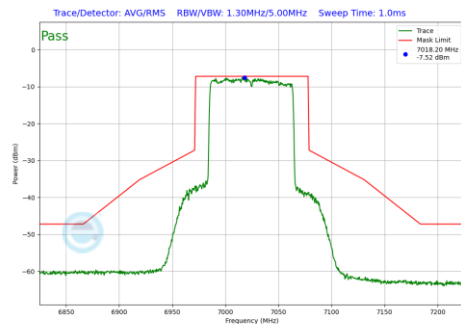
Plot 7-1305 In-Band Emission Plot SDM Diversity Antenna 5T (80MHz BW 802.11be(RU) RU996 Index67 (UNII Band 8) - Ch.215)
