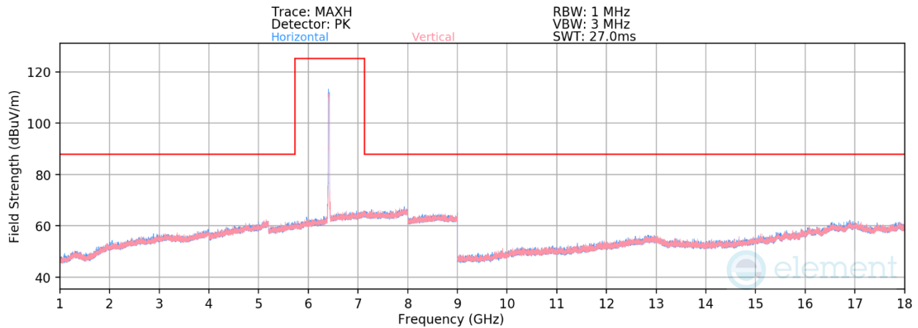
Plot 7-1377. Radiated Spurious Emissions above 1GHz CDD Primary (802.11be – Ch. 93 – RU242)
