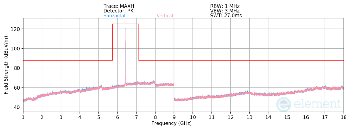
Plot 7-1361. Radiated Spurious Emissions above 1GHz CDD Primary (802.11be – Ch. 93 – RU26)
