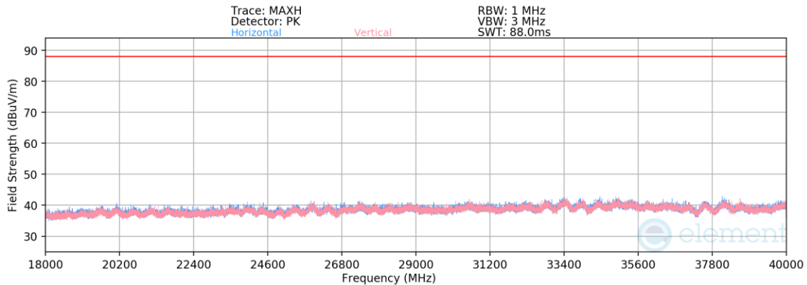
Plot 7-1368. Radiated Spurious Emissions 18-40GHz CDD Primary (802.11be – Ch. 149 – RU26)
