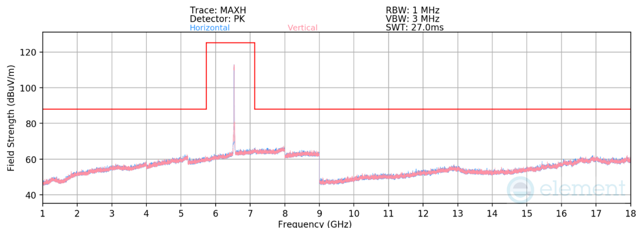
Plot 7-1382. Radiated Spurious Emissions above 1GHz CDD Primary (802.11be – Ch. 117 – RU242)
