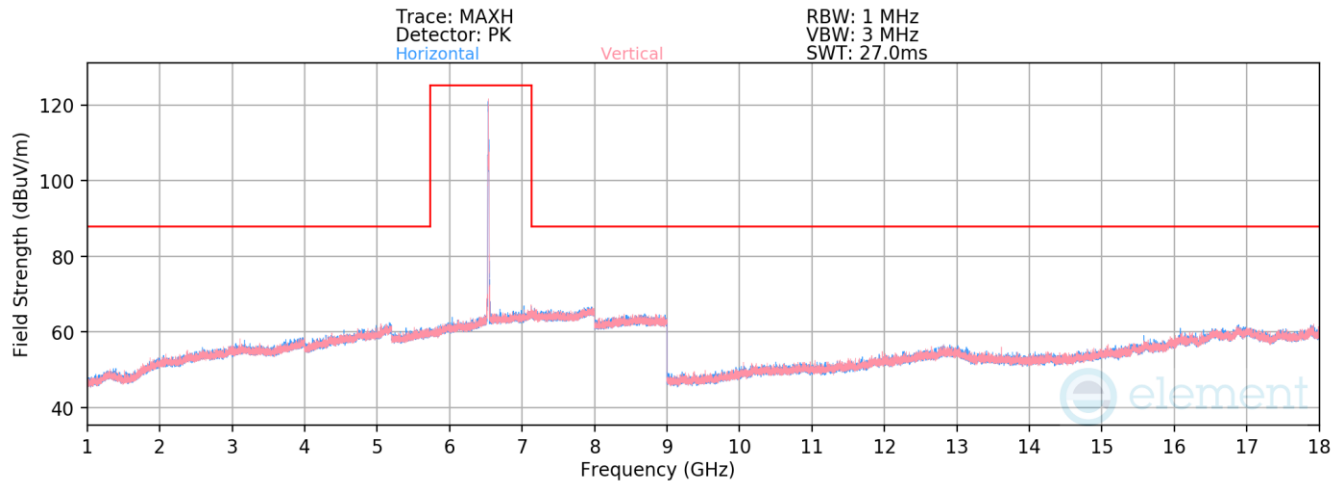
Plot 7-1366. Radiated Spurious Emissions above 1GHz CDD Primary (802.11be – Ch. 117 – RU26)
