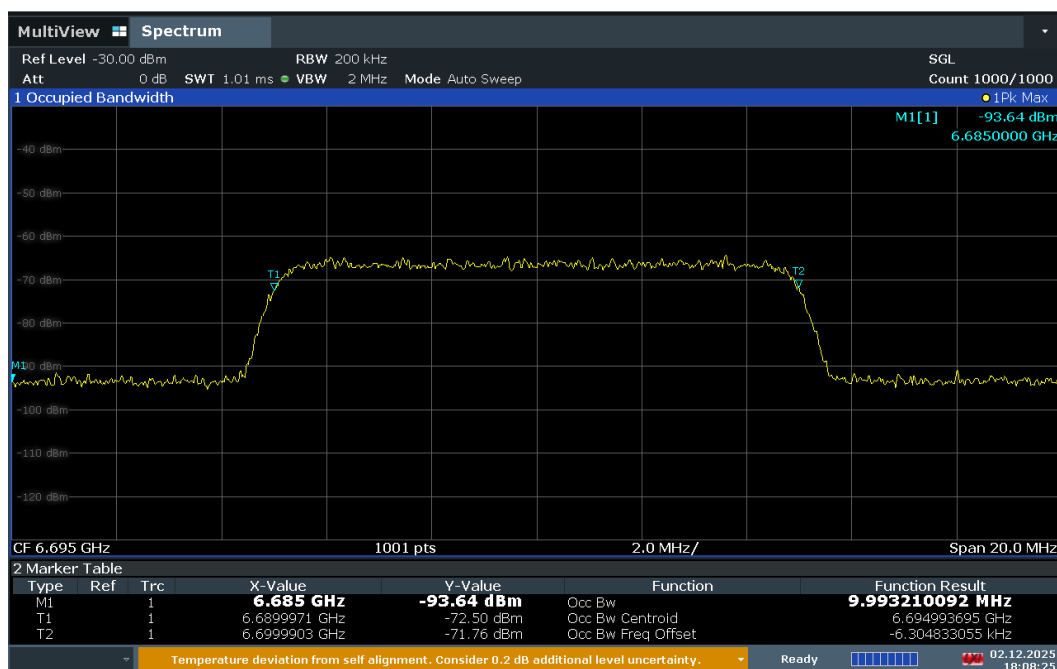
Plot 7-1315. AWGN Signal – UNII 7 – 20MHz
