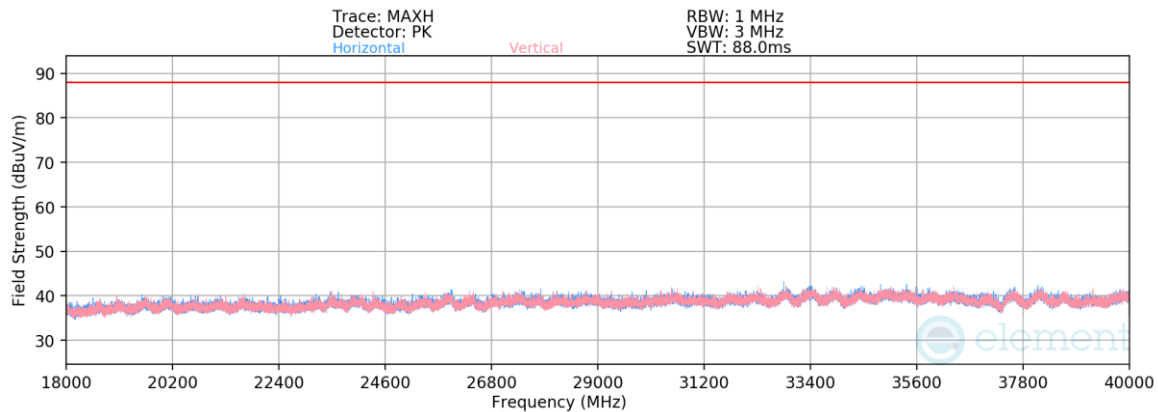
Plot 7-1384. Radiated Spurious Emissions 18-40GHz CDD Primary (802.11be – Ch. 149 – RU242)
