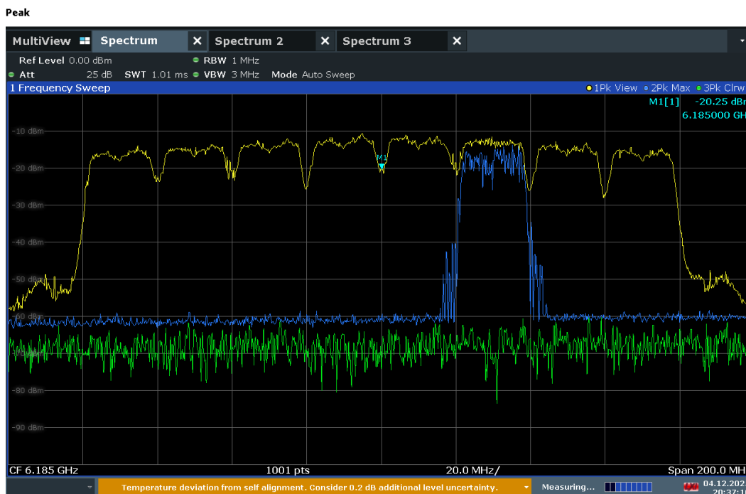
Plot 7-1356. 160MHz Bandwidth, AWGN Signal Injected – 6185MHz
