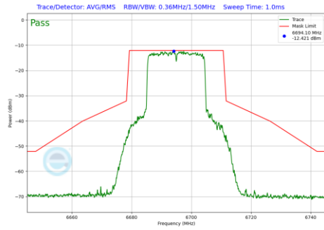
Plot 7-1299 In-Band Emission Plot SDM Diversity Antenna 5T (20MHz BW 802.11be(RU) RU242 Index61 (UNII Band 7) - Ch.149)
