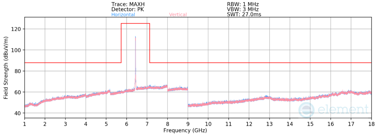
Plot 7-1378. Radiated Spurious Emissions above 1GHz CDD Primary (802.11be – Ch. 97 – RU242)
