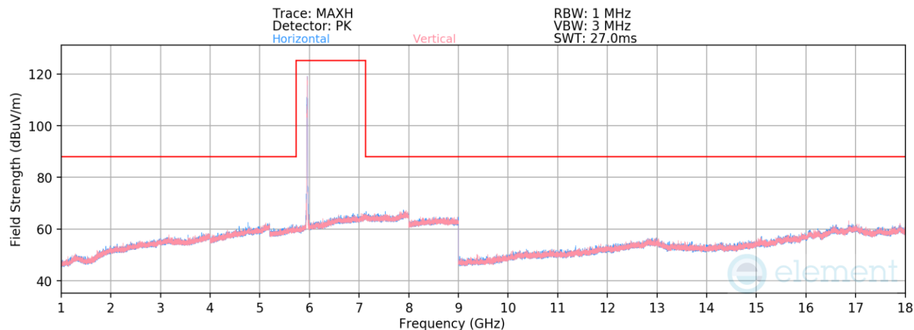
Plot 7-1358. Radiated Spurious Emissions above 1GHz CDD Primary (802.11be – Ch. 1 – RU26)
