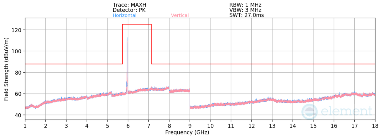
Plot 7-1374. Radiated Spurious Emissions above 1GHz CDD Primary (802.11be – Ch. 1 – RU242)
