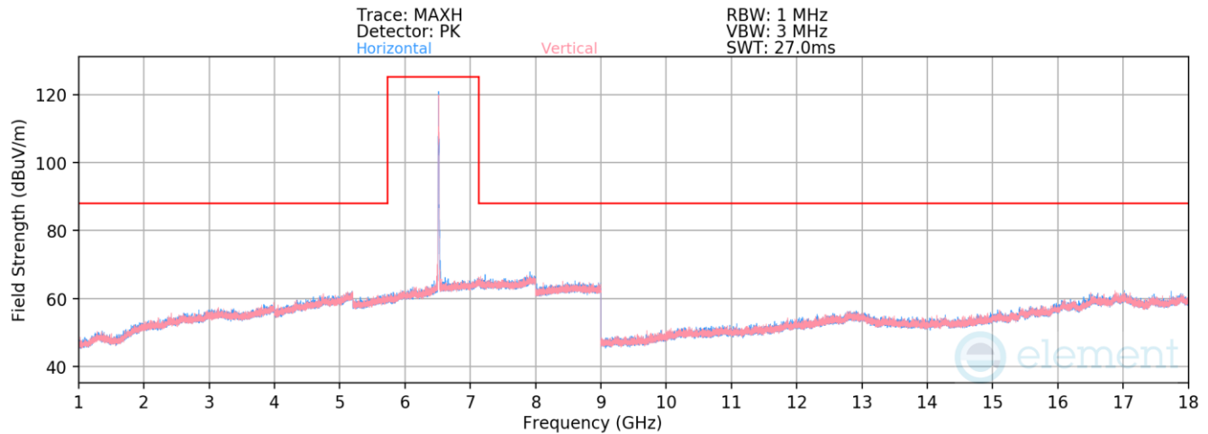
Plot 7-1365. Radiated Spurious Emissions above 1GHz CDD Primary (802.11be – Ch. 113 – RU26)
