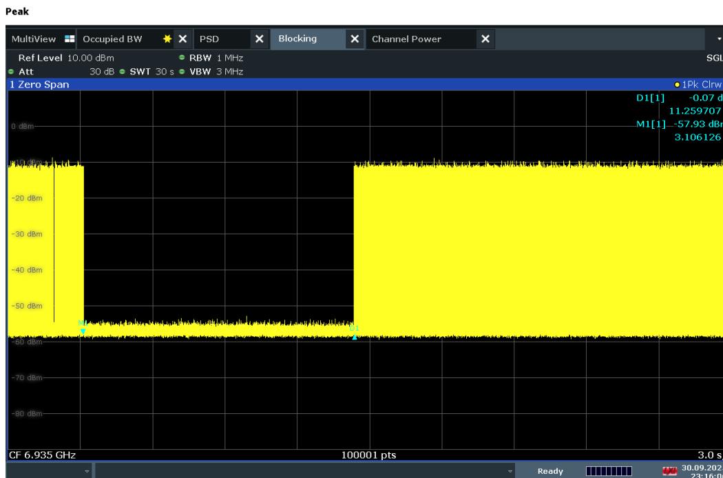
Plot 7-1351. Contention Based Protocol Timing Plot – UNII 8 – 20MHz Channel 197
