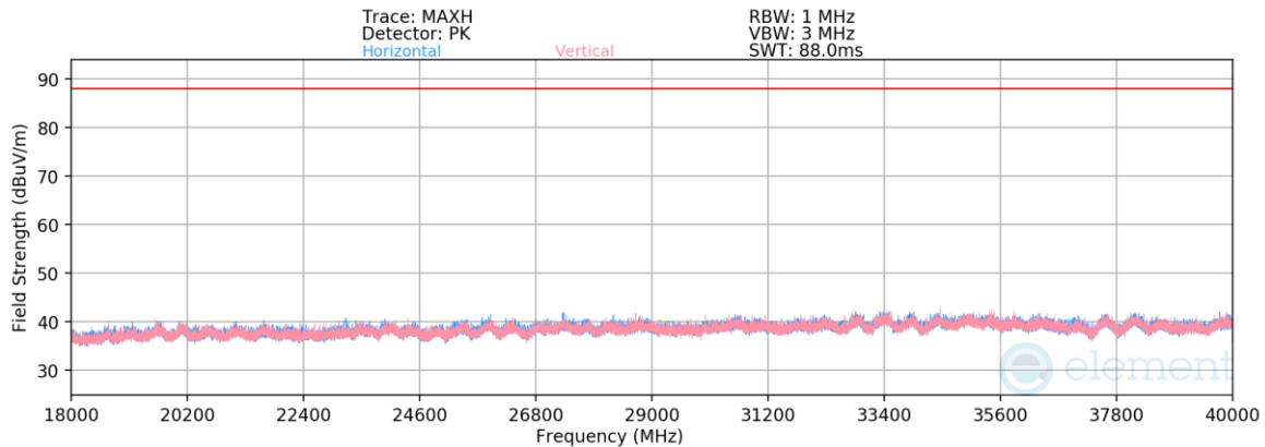
Plot 7-1360. Radiated Spurious Emissions 18-40GHz CDD Primary (802.11be – Ch. 45 – RU26)
