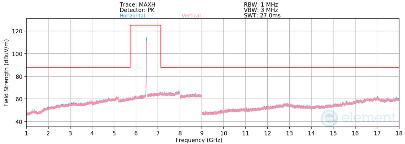
Plot 7-1379. Radiated Spurious Emissions above 1GHz CDD Primary (802.11be – Ch. 105 – RU242)
