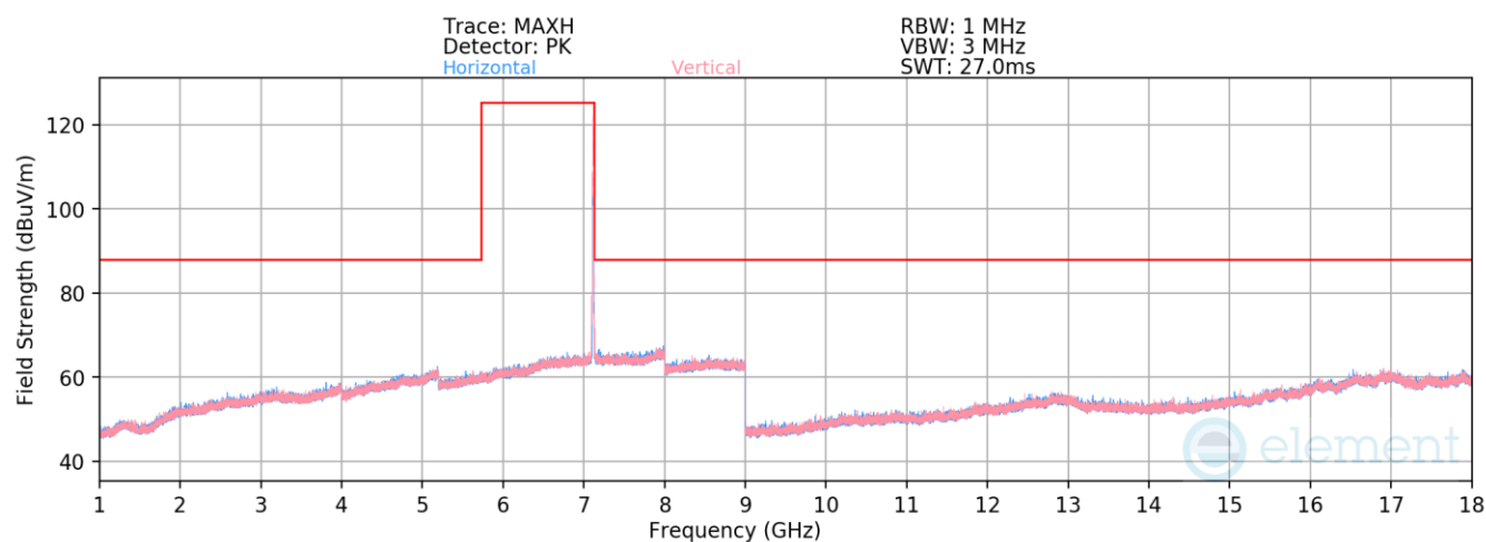
Plot 7-1373. Radiated Spurious Emissions above 1GHz SDM Primary (802.11be – Ch. 229 – RU26)
