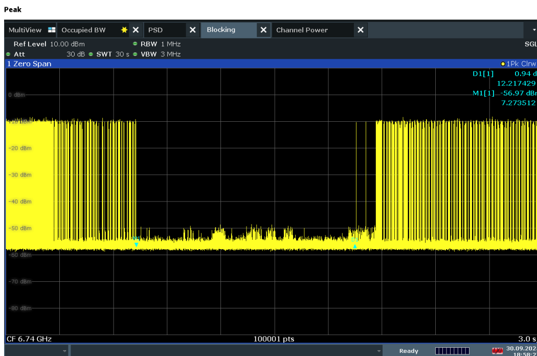
Plot 7-1350. Contention Based Protocol Timing Plot – UNII 7 – 160MHz Channel 143 – High
