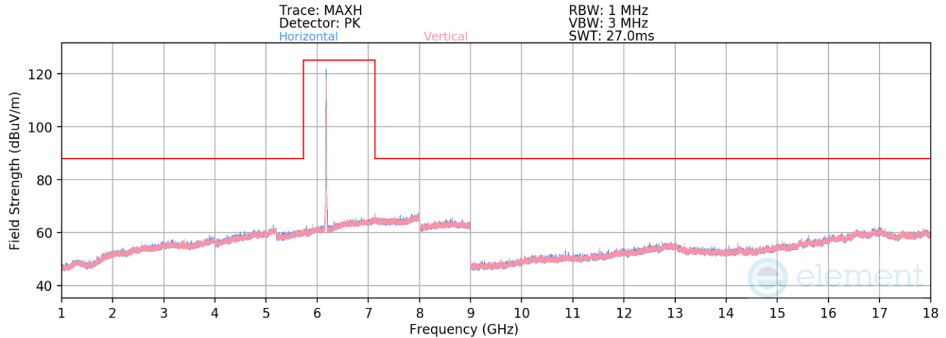
Plot 7-1359. Radiated Spurious Emissions above 1GHz CDD Primary (802.11be – Ch. 45 – RU26)
