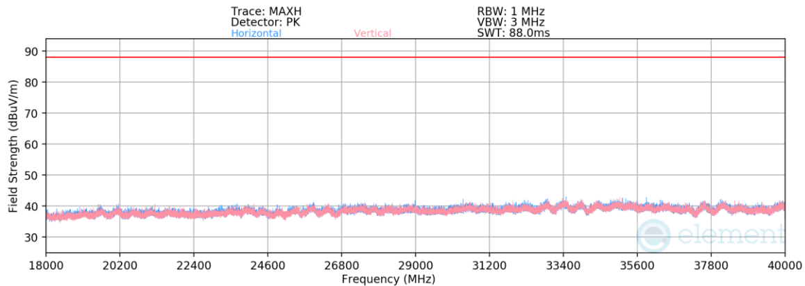
Plot 7-1376. Radiated Spurious Emissions 18-40GHz CDD Primary (802.11be – Ch. 45 – RU242)
