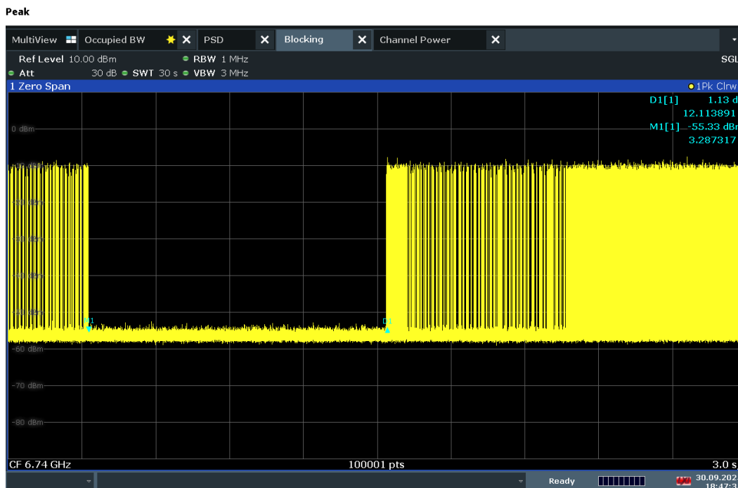
Plot 7-1348. Contention Based Protocol Timing Plot – UNII 7 – 160MHz Channel 143 – Low
