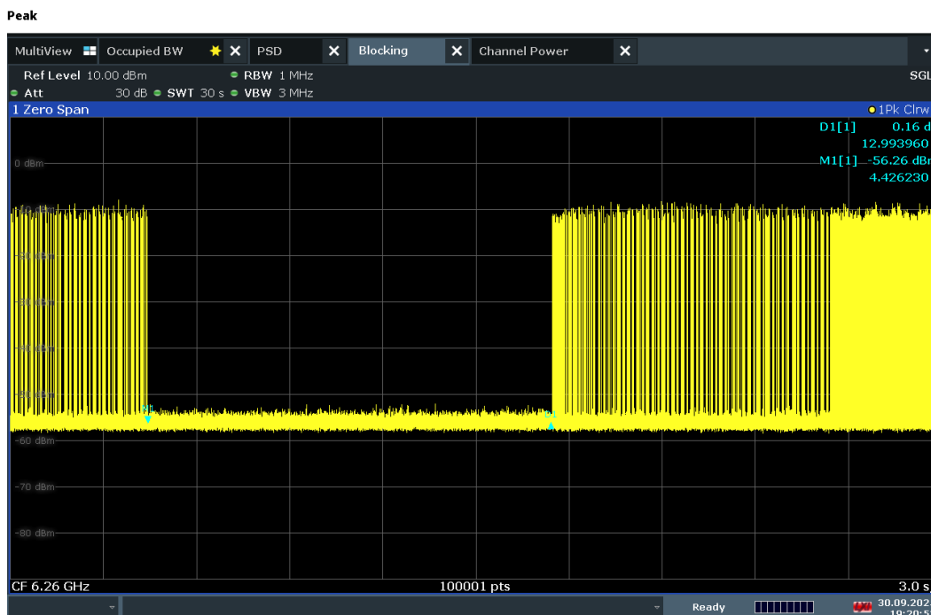
Plot 7-1342. Contention Based Protocol Timing Plot – UNII 5 – 160MHz Channel 47 – High
