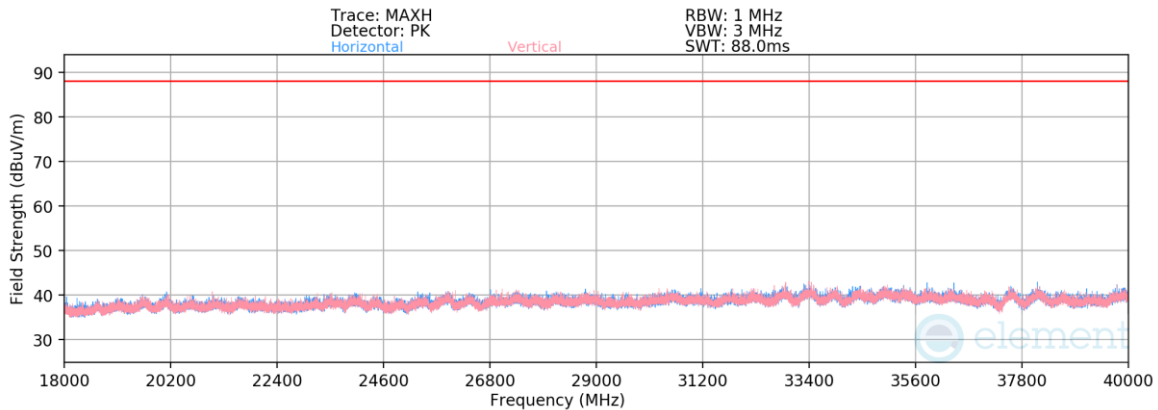
Plot 7-1364. Radiated Spurious Emissions 18-40GHz CDD Primary (802.11be – Ch. 105 – RU26)
