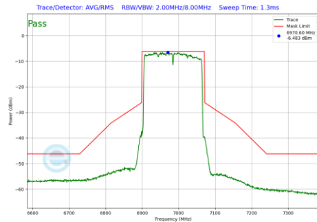
Plot 7-1306 In-Band Emission Plot SDM Diversity Antenna 5T (160MHz BW 802.11be(RU) RU996X2 Index68 (UNII Band 8) - Ch.207)
