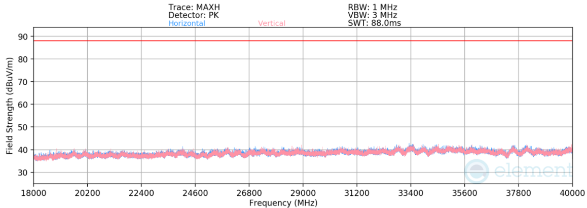
Plot 7-1380. Radiated Spurious Emissions 18-40GHz CDD Primary (802.11be – Ch. 105 – RU242)
