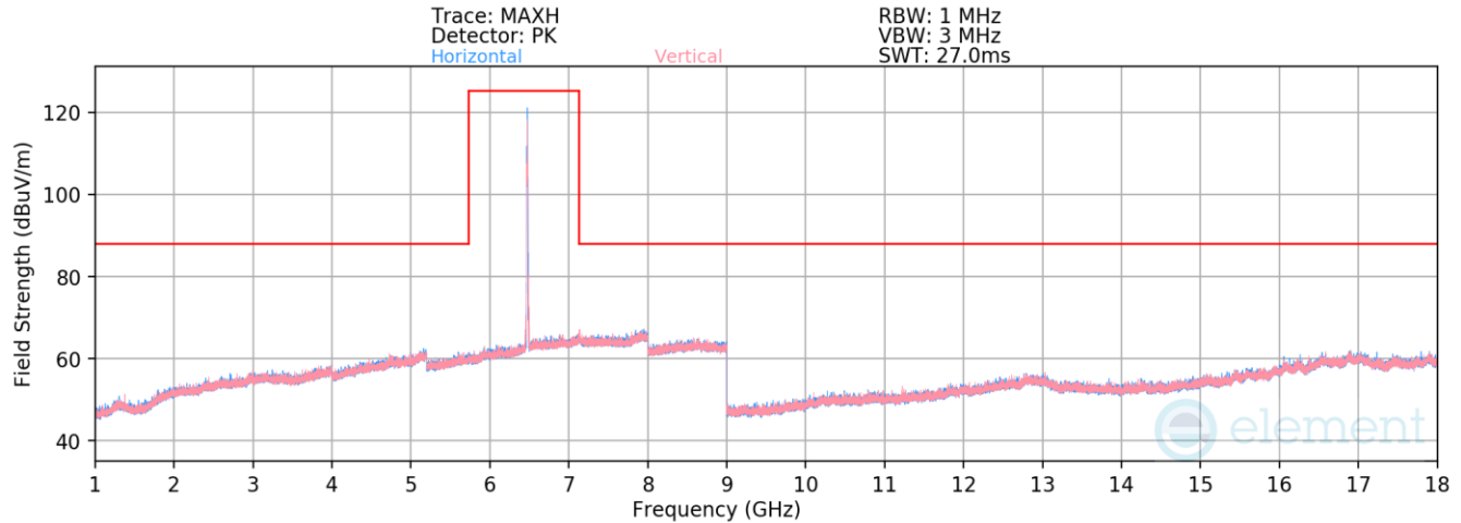
Plot 7-1363. Radiated Spurious Emissions above 1GHz CDD Primary (802.11be – Ch. 105 – RU26)
