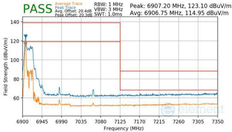
Plot 7-1704 SDM Diversity Radiated Upper Band Edge (Peak & Average – UNII Band 8) - RU26 (L)
