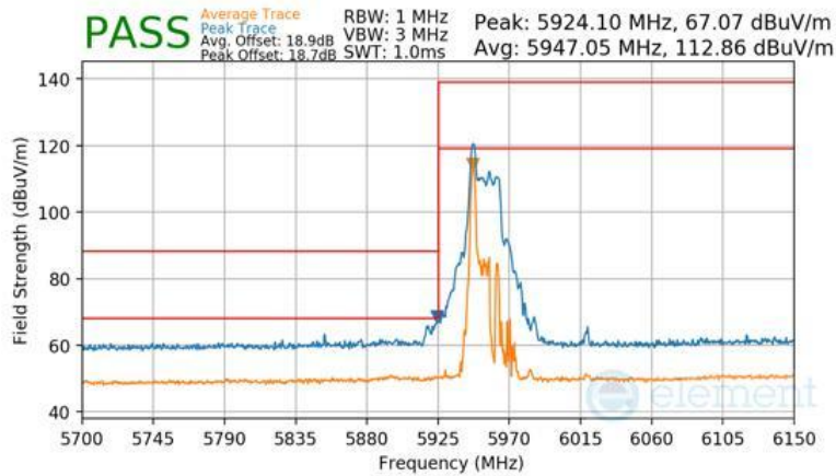
Plot 7-1682 CDD Diversity Radiated Lower Band Edge (Peak & Average – UNII Band 5) - RU26
