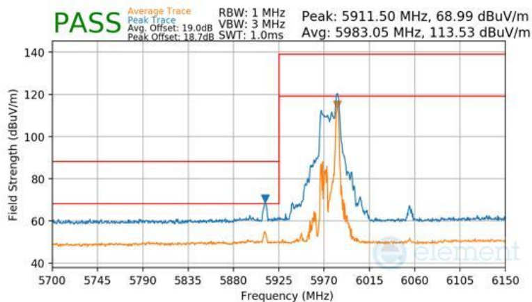
Plot 7-1683 CDD Diversity Radiated Lower Band Edge (Peak & Average – UNII Band 5) - RU26
