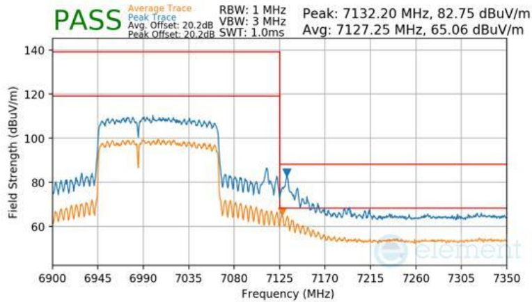
Plot 7-1710 SDM Diversity Radiated Upper Band Edge (Peak & Average – UNII Band 8) - RU996+484 (L)
