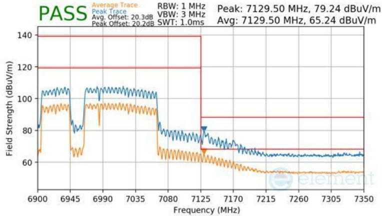
Plot 7-1664 SDM Primary Radiated Upper Band Edge (Peak & Average – UNII Band 8) - RU996+484+242 (L)
