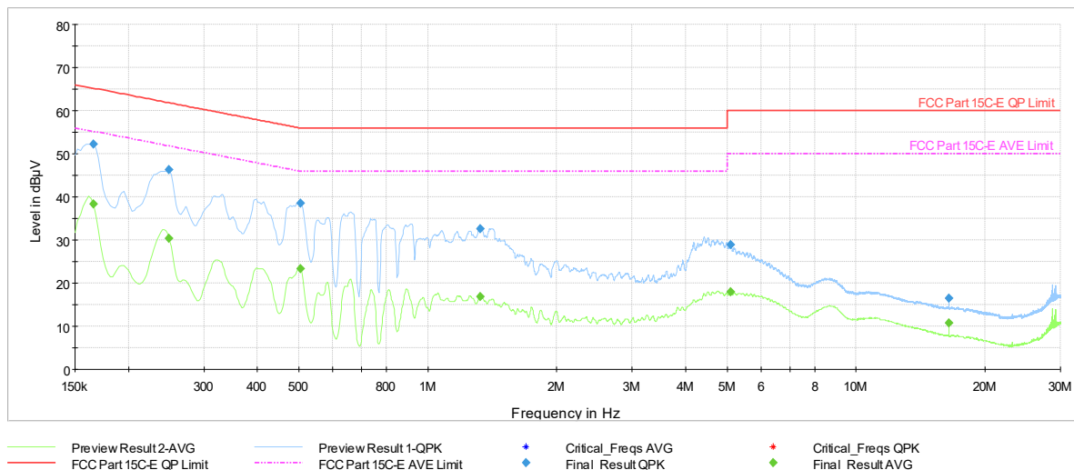
Plot 7-1742. AC Line Conducted Plot with 11be CDD Diversity UNII Band 5 – RU242 – Ch.45 (L1) with AC/DC Adapter
