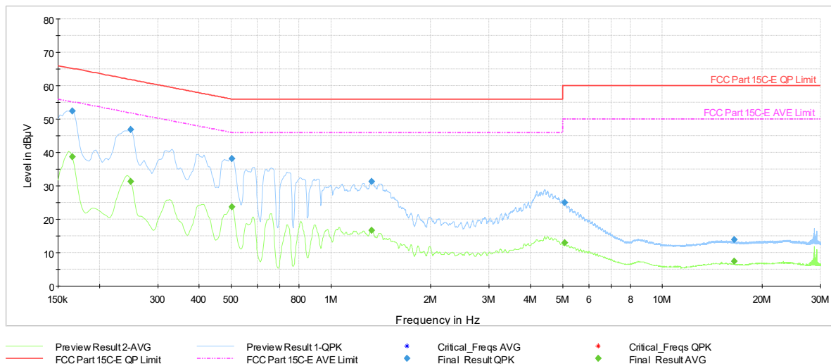
Plot 7-1741. AC Line Conducted Plot with 11be CDD Diversity UNII Band 5 – RU26 – Ch.45 (N) with AC/DC Adapter
