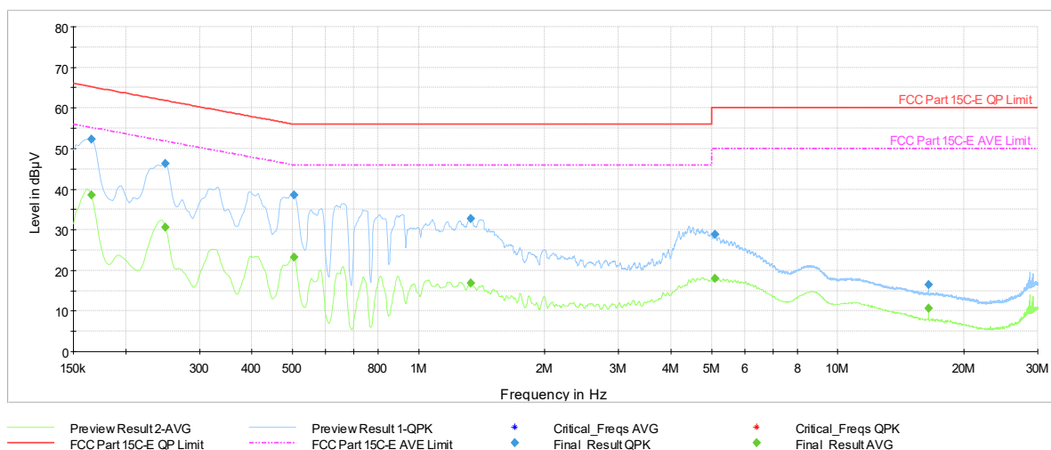
Plot 7-1736. AC Line Conducted Plot with 11be CDD Primary UNII Band 5 – RU26 – Ch.45 (L1) with AC/DC Adapter
