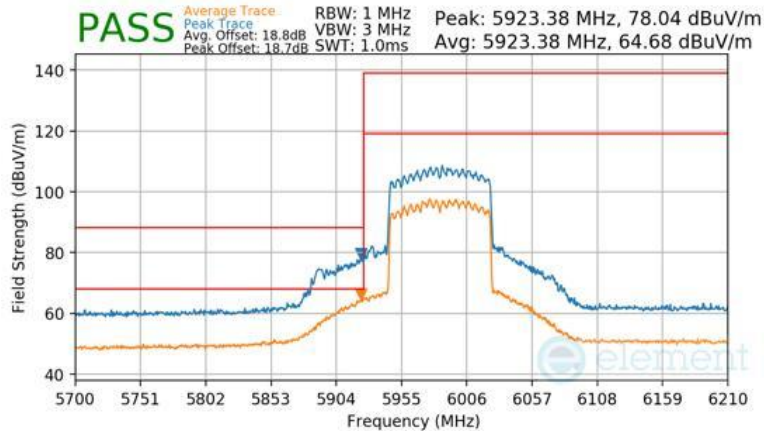
Plot 7-1700 CDD Diversity Radiated Lower Band Edge (Peak & Average – UNII Band 5) - RU996
