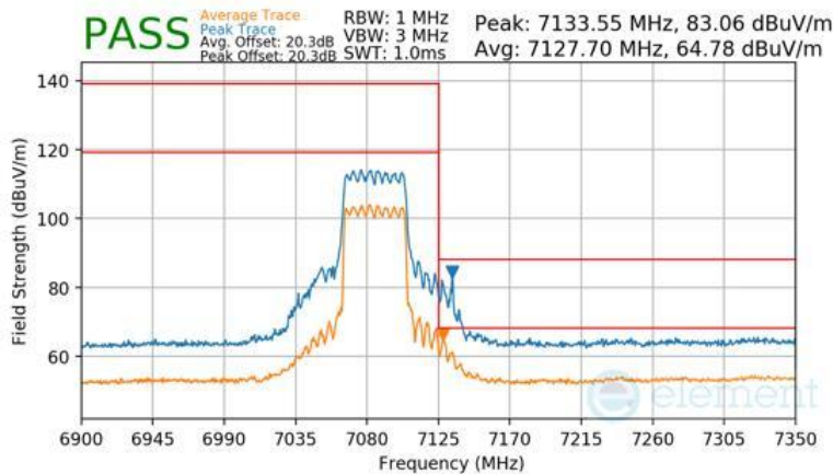
Plot 7-1687 SDM Diversity Radiated Upper Band Edge (Peak & Average – UNII Band 8) - RU484
