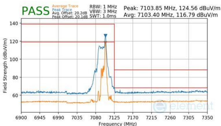
Plot 7-1673 SDM Diversity Radiated Upper Band Edge (Peak & Average – UNII Band 8) - RU26
