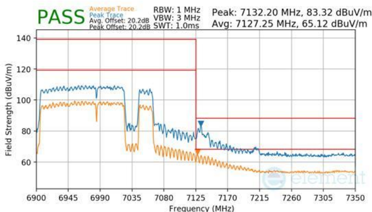
Plot 7-1727 SDM Diversity Radiated Upper Band Edge (Peak & Average – UNII Band 8) - RU996+484+242 (H)
