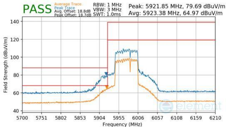
Plot 7-1695 CDD Diversity Radiated Lower Band Edge (Peak & Average – UNII Band 5) - RU484+242
