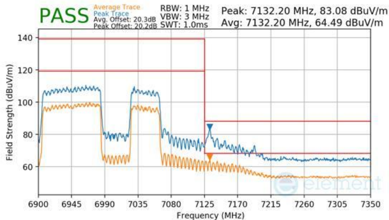
Plot 7-1711 SDM Diversity Radiated Upper Band Edge (Peak & Average – UNII Band 8) - RU996+484 (H)
