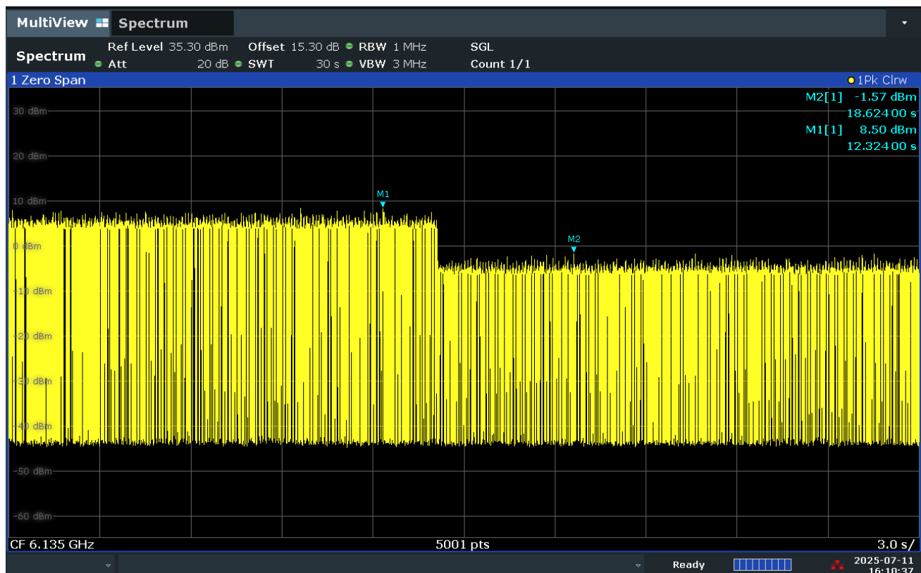
Plot 7-1747. Client device observation from Standard Power AP to Low Power Indoor AP
