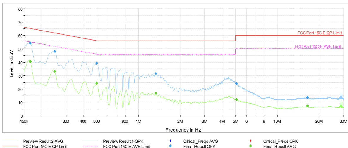
Plot 7-1737. AC Line Conducted Plot with 11be CDD Primary UNII Band 5 – RU26 – Ch.45 (N) with AC/DC Adapter
