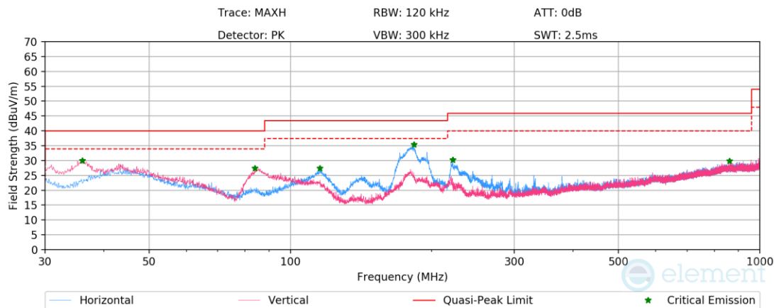
Plot 7-1733. Radiated Spurious Emissions below 1GHz CDD Primary (802.11be – Ch.45 – RU242) with AC/DC Adapter
