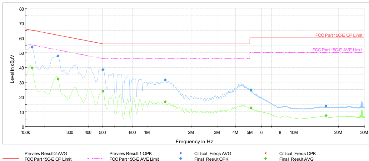
Plot 7-1743. AC Line Conducted Plot with 11be CDD Diversity UNII Band 5 – RU242 – Ch.45 (N) with AC/DC Adapter
