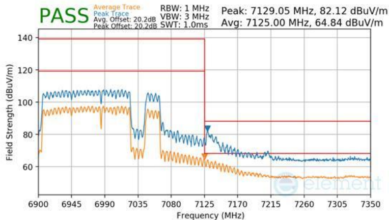
Plot 7-1665 SDM Primary Radiated Upper Band Edge (Peak & Average – UNII Band 8) - RU996+484+242 (H)
