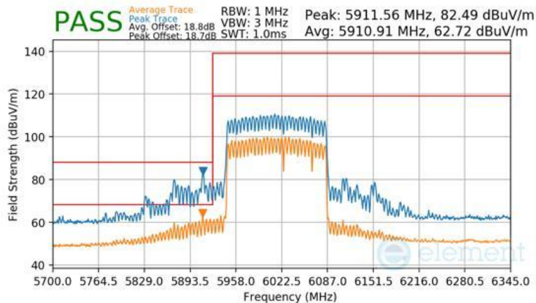
Plot 7-1659 CDD Primary Radiated Lower Band Edge (Peak & Average – UNII Band 5) - RU996+484+242 (H)
