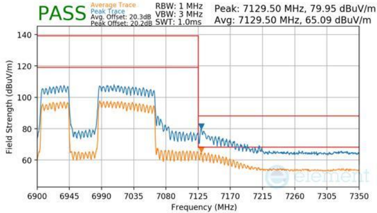
Plot 7-1650 SDM Primary Radiated Upper Band Edge (Peak & Average – UNII Band 8) - RU996+484 (L)
