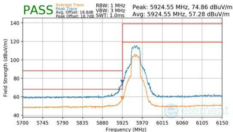
Plot 7-1678 CDD Diversity Radiated Lower Band Edge (Peak & Average – UNII Band 5) - RU242
