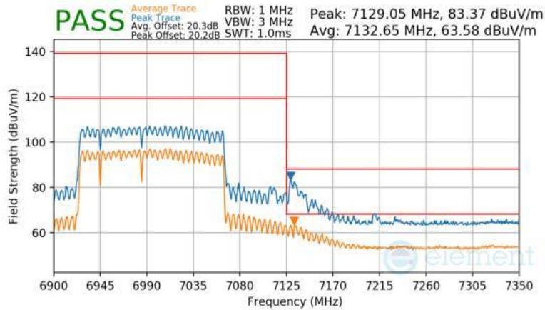
Plot 7-1660 SDM Primary Radiated Upper Band Edge (Peak & Average – UNII Band 8) - RU996+484+242 (L)
