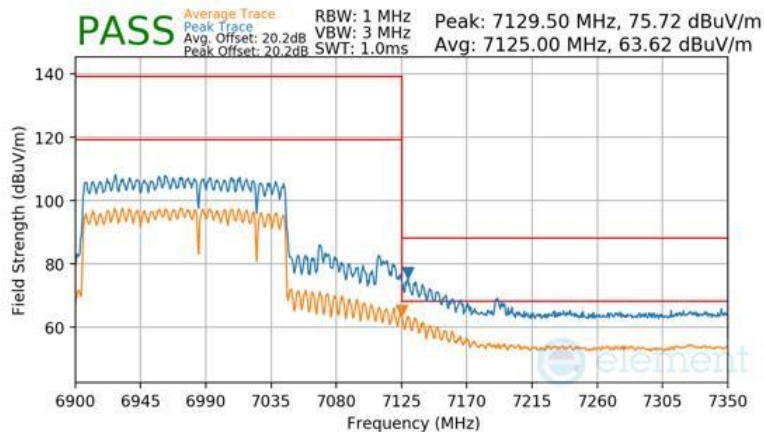
Plot 7-1667 SDM Primary Radiated Upper Band Edge (Peak & Average – UNII Band 8) - RU996+484+242 (H)
