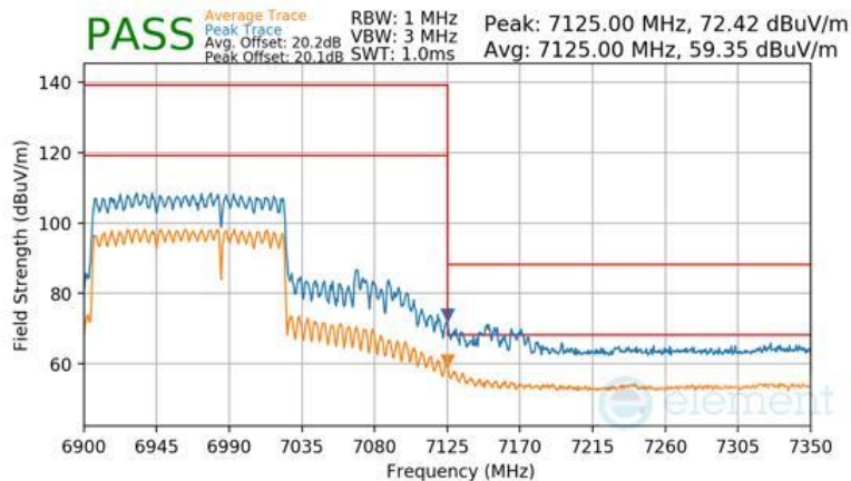
Plot 7-1651 SDM Primary Radiated Upper Band Edge (Peak & Average – UNII Band 8) - RU996+484 (H)
