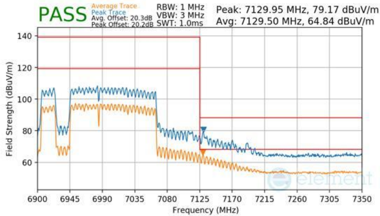
Plot 7-1662 SDM Primary Radiated Upper Band Edge (Peak & Average – UNII Band 8) - RU996+484+242 (L)
