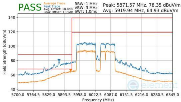
Plot 7-1715 CDD Diversity Radiated Lower Band Edge (Peak & Average – UNII Band 5) - RU996+484+242 (H)
