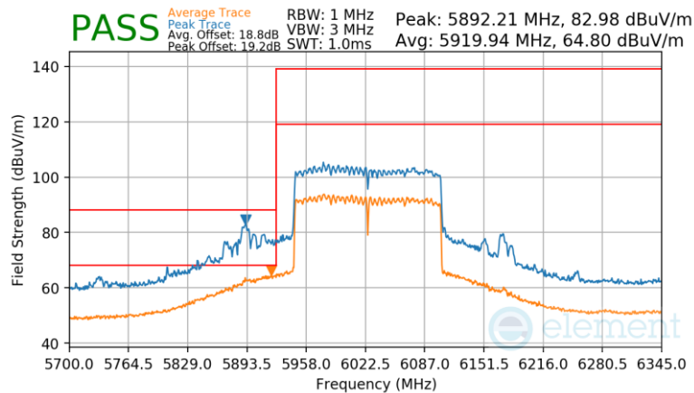
Plot 7-1730 CDD Diversity Radiated Lower Band Edge (Peak & Average – UNII Band 5) – RU996X2
