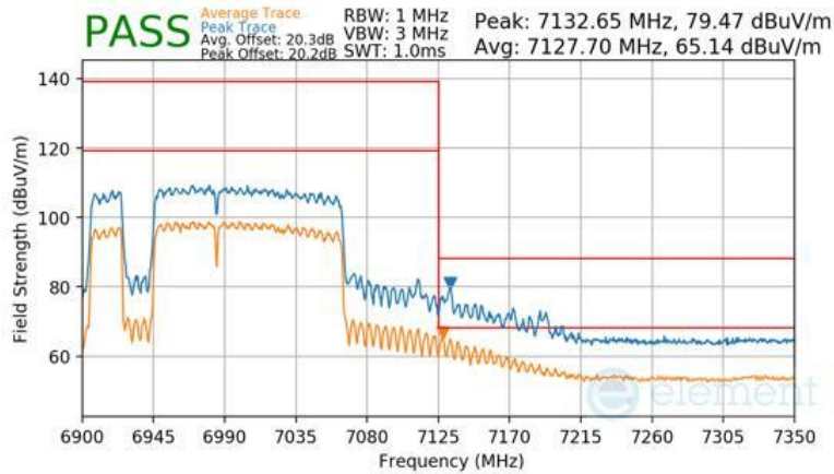
Plot 7-1724 SDM Diversity Radiated Upper Band Edge (Peak & Average – UNII Band 8) - RU996+484+242 (L)
