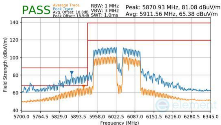
Plot 7-1653 CDD Primary Radiated Lower Band Edge (Peak & Average – UNII Band 5) - RU996+484+242 (H)
