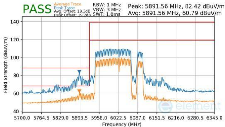
Plot 7-1657 CDD Primary Radiated Lower Band Edge (Peak & Average – UNII Band 5) - RU996+484+242 (H)
