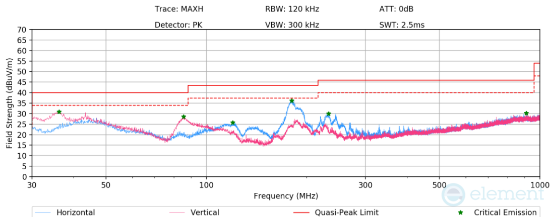
Plot 7-1735. Radiated Spurious Emissions below 1GHz CDD Diversity (802.11be – Ch.45 – RU242) with AC/DC Adapter
