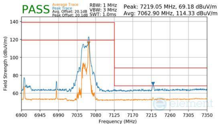
Plot 7-1705 SDM Diversity Radiated Upper Band Edge (Peak & Average – UNII Band 8) - RU26 (H)
