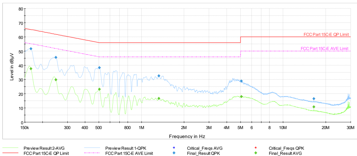
Plot 7-1740. AC Line Conducted Plot with 11be CDD Diversity UNII Band 5 – RU26 – Ch.45 (L1) with AC/DC Adapter
