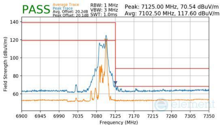
Plot 7-1685 SDM Diversity Radiated Upper Band Edge (Peak & Average – UNII Band 8) - RU26
