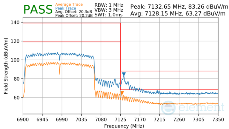
Plot 7-1731 SDM Diversity Radiated Upper Band Edge (Peak & Average – UNII Band 8) – RU996X2
