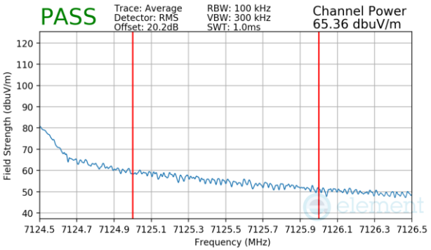
Plot 7-1681 SDM Diversity Radiated Upper Band Edge (Average – UNII Band 8) – RU242
