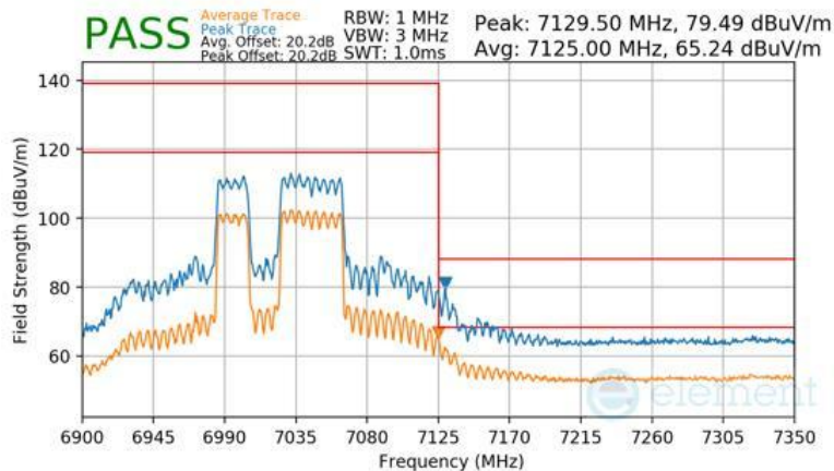
Plot 7-1697 SDM Diversity Radiated Upper Band Edge (Peak & Average – UNII Band 8) - RU484+242
