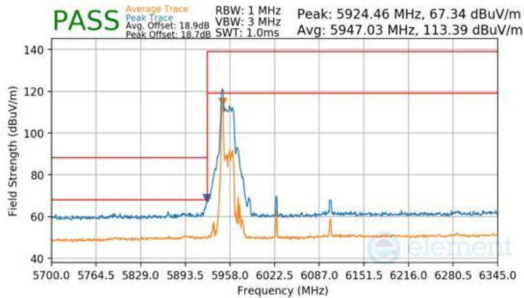
Plot 7-1702 CDD Diversity Radiated Lower Band Edge (Peak & Average – UNII Band 5) - RU26 (L)
