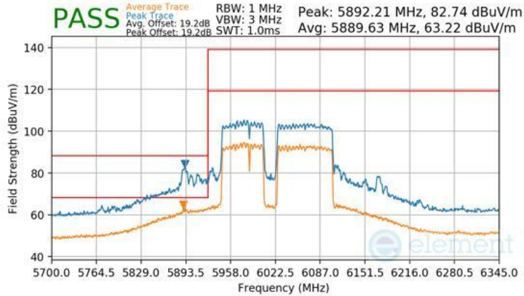
Plot 7-1720 CDD Diversity Radiated Lower Band Edge (Peak & Average – UNII Band 5) - RU996+484+242 (L)
