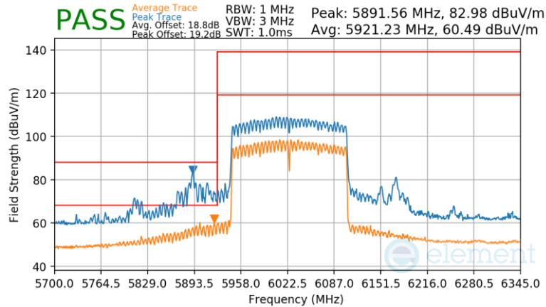
Plot 7-1668 CDD Primary Radiated Lower Band Edge (Peak & Average – UNII Band 5) – RU996X2
