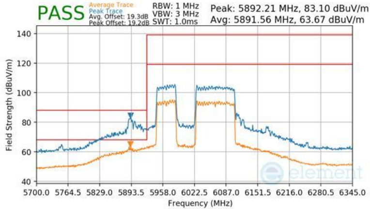
Plot 7-1708 CDD Diversity Radiated Lower Band Edge (Peak & Average – UNII Band 5) - RU996+484 (L)
