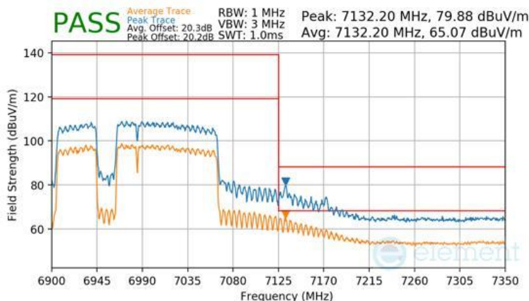
Plot 7-1726 SDM Diversity Radiated Upper Band Edge (Peak & Average – UNII Band 8) - RU996+484+242 (L)
