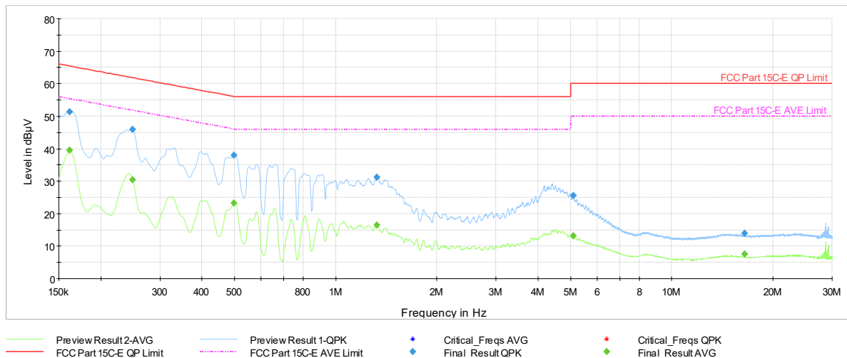
Plot 7-1739. AC Line Conducted Plot with 11be CDD Primary UNII Band 5 – RU242 – Ch.45 (N) with AC/DC Adapter
