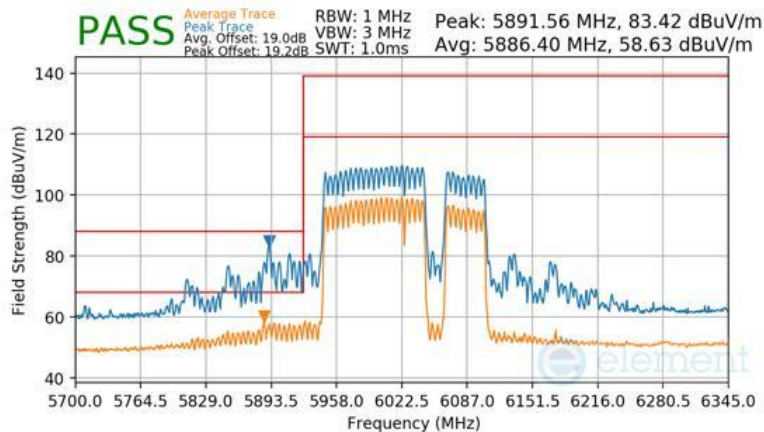
Plot 7-1655 CDD Primary Radiated Lower Band Edge (Peak & Average – UNII Band 5) - RU996+484+242 (H)
