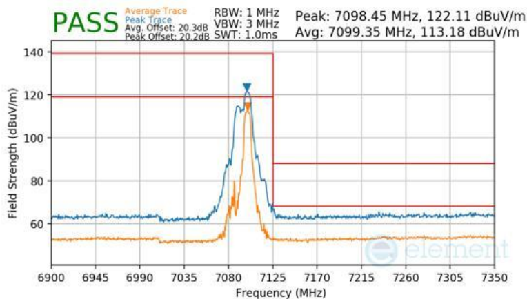
Plot 7-1677 SDM Diversity Radiated Upper Band Edge (Peak & Average – UNII Band 8) - RU52+26
