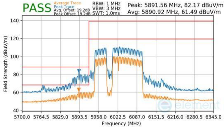
Plot 7-1656 CDD Primary Radiated Lower Band Edge (Peak & Average – UNII Band 5) - RU996+484+242 (L)
