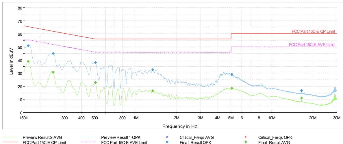
Plot 7-1738. AC Line Conducted Plot with 11be CDD Primary UNII Band 5 – RU242 – Ch.45 (L1) with AC/DC Adapter
