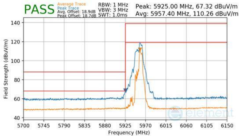
Plot 7-1675 CDD Diversity Radiated Lower Band Edge (Peak & Average – UNII Band 5) - RU52+26
