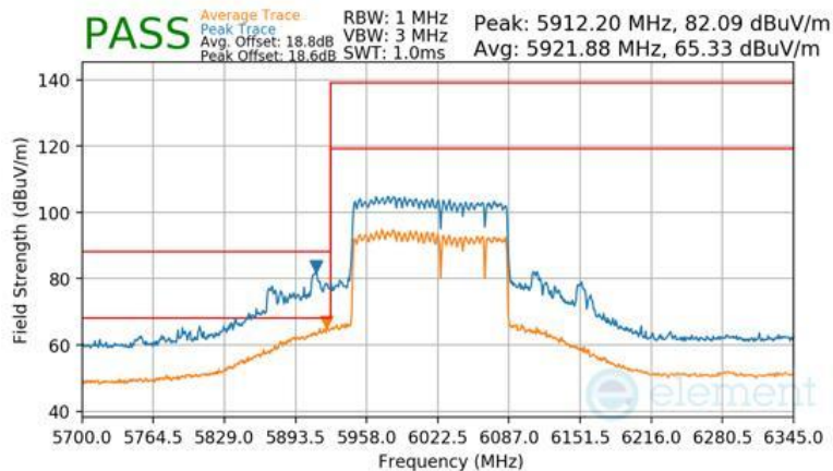
Plot 7-1721 CDD Diversity Radiated Lower Band Edge (Peak & Average – UNII Band 5) - RU996+484+242 (H)
