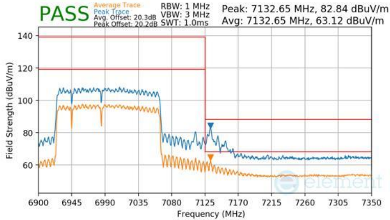
Plot 7-1722 SDM Diversity Radiated Upper Band Edge (Peak & Average – UNII Band 8) - RU996+484+242 (L)
