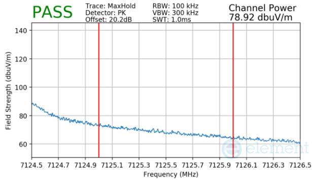
Plot 7-1680 SDM Diversity Radiated Upper Band Edge (Peak – UNII Band 8) – RU242
