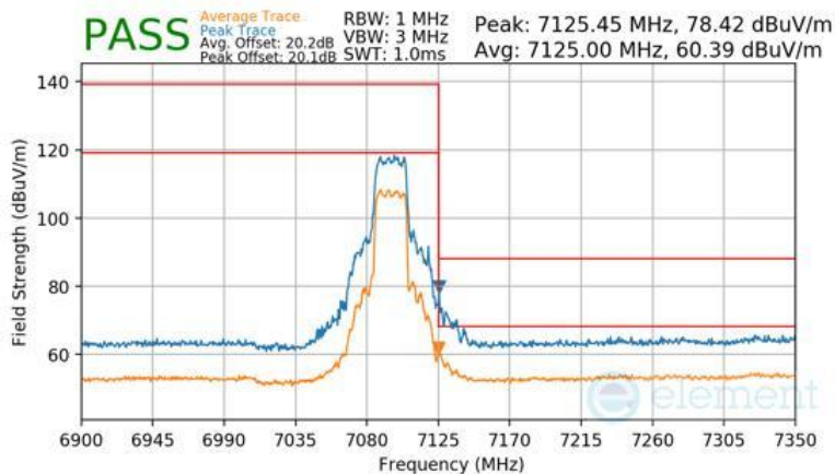
Plot 7-1679 SDM Diversity Radiated Upper Band Edge (Peak & Average – UNII Band 8) - RU242
