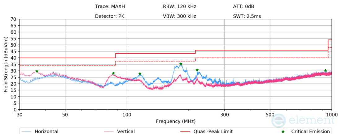
Plot 7-1732. Radiated Spurious Emissions below 1GHz CDD Primary (802.11be – Ch.45 – RU26) with AC/DC Adapter
