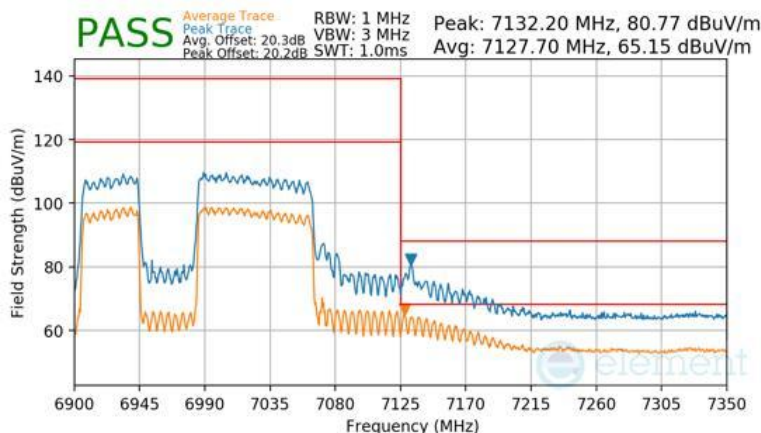
Plot 7-1712 SDM Diversity Radiated Upper Band Edge (Peak & Average – UNII Band 8) - RU996+484 (L)
