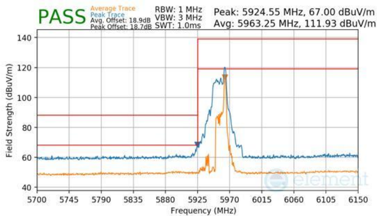
Plot 7-1671 CDD Diversity Radiated Lower Band Edge (Peak & Average – UNII Band 5) - RU26
