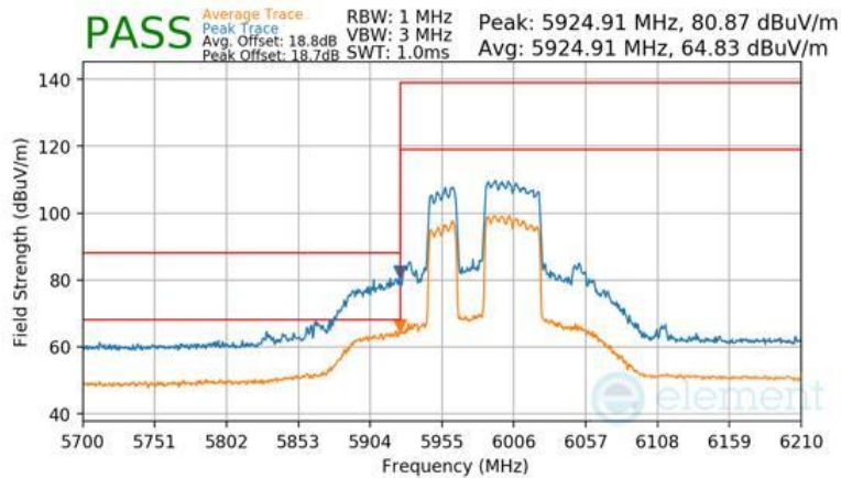
Plot 7-1693 CDD Diversity Radiated Lower Band Edge (Peak & Average – UNII Band 5) - RU484+242
