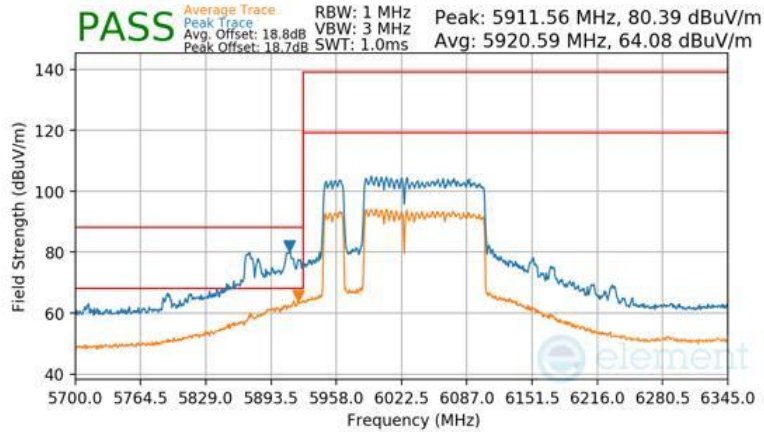
Plot 7-1716 CDD Diversity Radiated Lower Band Edge (Peak & Average – UNII Band 5) - RU996+484+242 (L)
