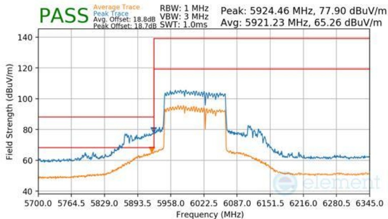
Plot 7-1709 CDD Diversity Radiated Lower Band Edge (Peak & Average – UNII Band 5) - RU996+484 (H)
