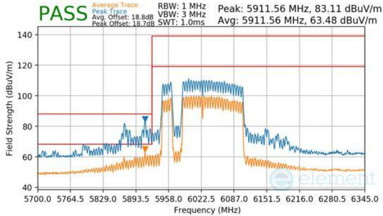
Plot 7-1654 CDD Primary Radiated Lower Band Edge (Peak & Average – UNII Band 5) - RU996+484+242 (L)
