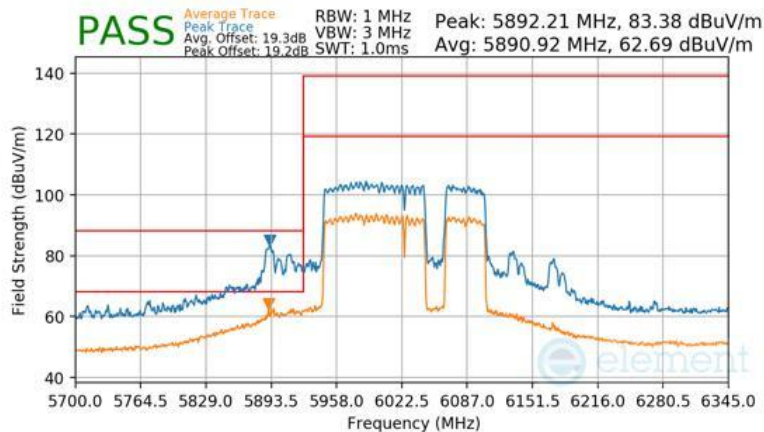
Plot 7-1717 CDD Diversity Radiated Lower Band Edge (Peak & Average – UNII Band 5) - RU996+484+242 (H)
