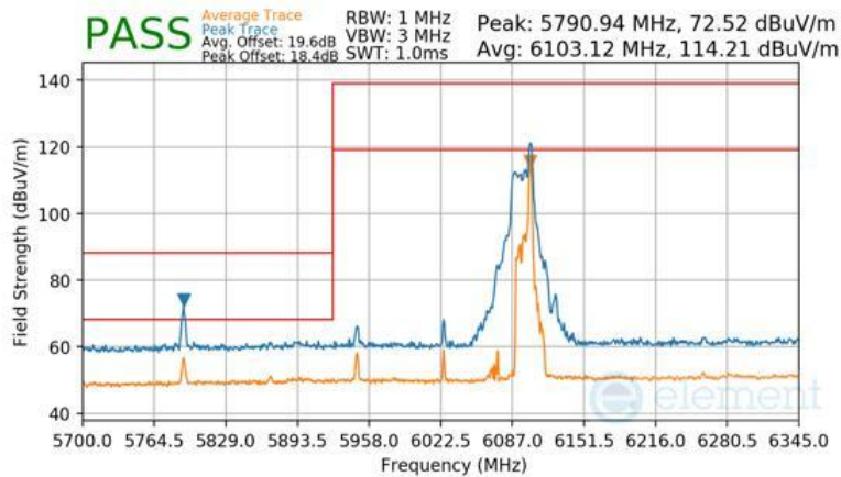
Plot 7-1703 CDD Diversity Radiated Lower Band Edge (Peak & Average – UNII Band 5) - RU26 (H)
