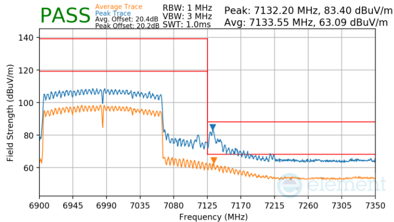
Plot 7-1669 SDM Primary Radiated Upper Band Edge (Peak & Average – UNII Band 8) – RU996X2
