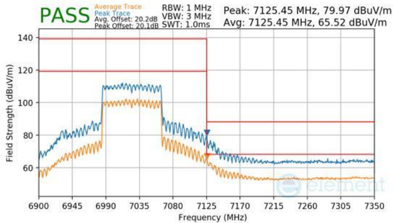
Plot 7-1701 SDM Diversity Radiated Upper Band Edge (Peak & Average – UNII Band 8) - RU996
