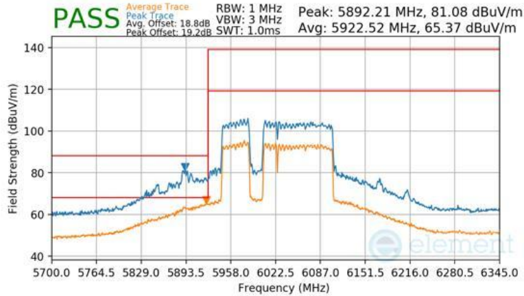
Plot 7-1718 CDD Diversity Radiated Lower Band Edge (Peak & Average – UNII Band 5) - RU996+484+242 (L)
