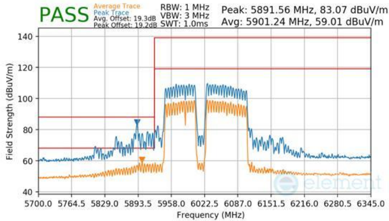
Plot 7-1658 CDD Primary Radiated Lower Band Edge (Peak & Average – UNII Band 5) - RU996+484+242 (L)
