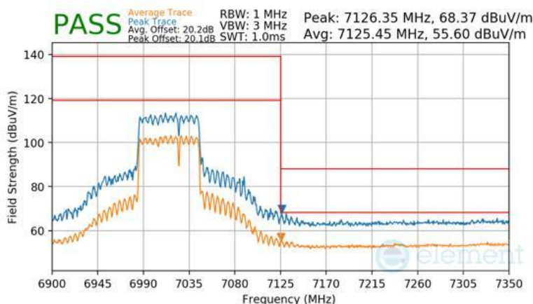
Plot 7-1699 SDM Diversity Radiated Upper Band Edge (Peak & Average – UNII Band 8) - RU484+242
