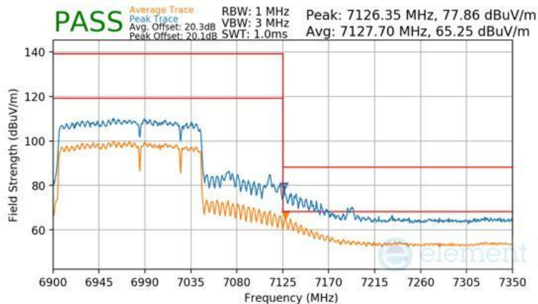
Plot 7-1729 SDM Diversity Radiated Upper Band Edge (Peak & Average – UNII Band 8) - RU996+484+242 (H)
