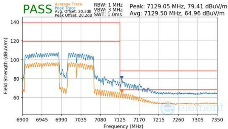
Plot 7-1661 SDM Primary Radiated Upper Band Edge (Peak & Average – UNII Band 8) - RU996+484+242 (H)
