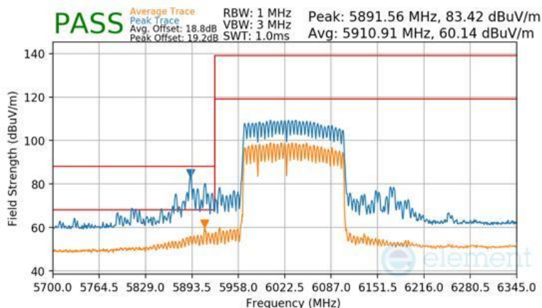
Plot 7-1652 CDD Primary Radiated Lower Band Edge (Peak & Average – UNII Band 5) - RU996+484+242 (L)
