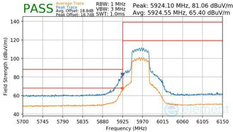
Plot 7-1686 CDD Diversity Radiated Lower Band Edge (Peak & Average – UNII Band 5) - RU484
