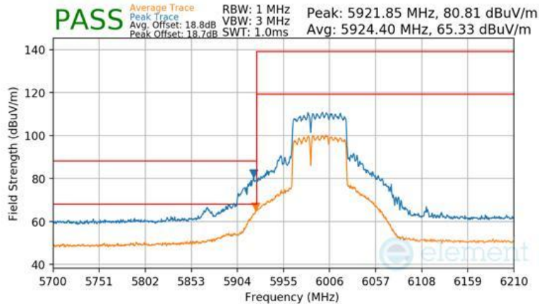
Plot 7-1692 CDD Diversity Radiated Lower Band Edge (Peak & Average – UNII Band 5) - RU484+242
