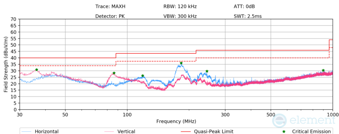
Plot 7-1734. Radiated Spurious Emissions below 1GHz CDD Diversity (802.11be – Ch.45 – RU26) with AC/DC Adapter
