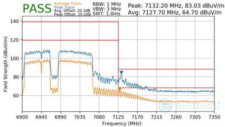
Plot 7-1728 SDM Diversity Radiated Upper Band Edge (Peak & Average – UNII Band 8) - RU996+484+242 (L)
