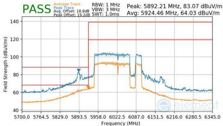
Plot 7-1719 CDD Diversity Radiated Lower Band Edge (Peak & Average – UNII Band 5) - RU996+484+242 (H)
