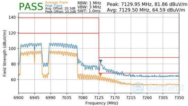
Plot 7-1666 SDM Primary Radiated Upper Band Edge (Peak & Average – UNII Band 8) - RU996+484+242 (L)
