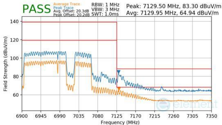
Plot 7-1663 SDM Primary Radiated Upper Band Edge (Peak & Average – UNII Band 8) - RU996+484+242 (H)
