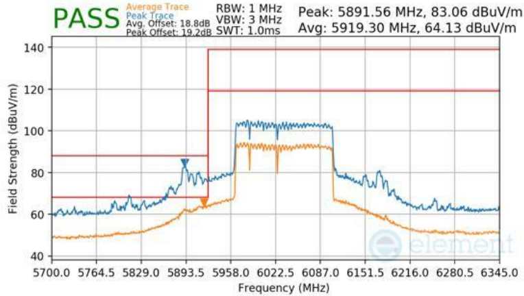
Plot 7-1714 CDD Diversity Radiated Lower Band Edge (Peak & Average – UNII Band 5) - RU996+484+242 (L)
