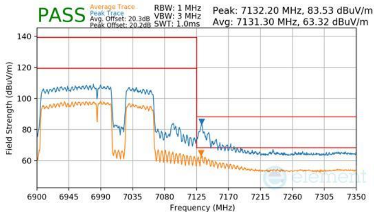
Plot 7-1725 SDM Diversity Radiated Upper Band Edge (Peak & Average – UNII Band 8) - RU996+484+242 (H)
