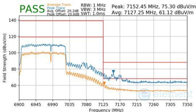
Plot 7-1713 SDM Diversity Radiated Upper Band Edge (Peak & Average – UNII Band 8) - RU996+484 (H)
