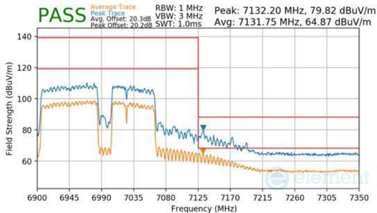
Plot 7-1723 SDM Diversity Radiated Upper Band Edge (Peak & Average – UNII Band 8) - RU996+484+242 (H)
