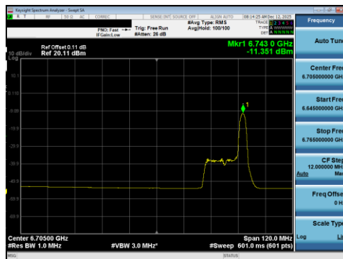
Plot 7-157 PSD Antenna 5T (80MHz BW 802.11be(RU) RU26 Index36 - Ch.151)
