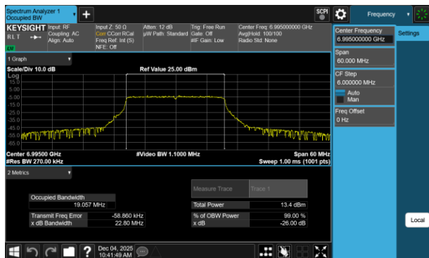
Plot 7-130 26dB BW & 99% OBW Antenna 1b (20MHz BW 802.11be(RU) RU242 Index61 - Ch.209)
