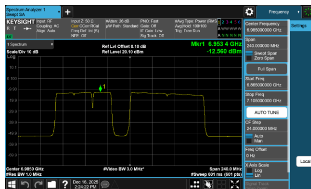
Plot 7-172 PSD Antenna 5T (160MHz BW 802.11be(RU) RU996+484+242 Index99 - Ch.207)
