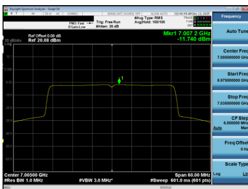
Plot 7-174 PSD Antenna 5T (40MHz BW 802.11be(RU) RU484 Index65 - Ch.211)
