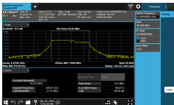
Plot 7-104 26dB BW & 99% OBW Antenna 1b (20MHz BW 802.11be(RU) RU106+26 Index82 - Ch.97)
