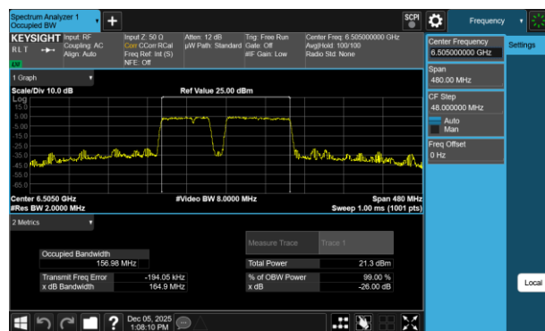
Plot 7-106 26dB BW & 99% OBW Antenna 1b (160MHz BW 802.11be(RU) RU996+484+242 Index99 - Ch.111)
