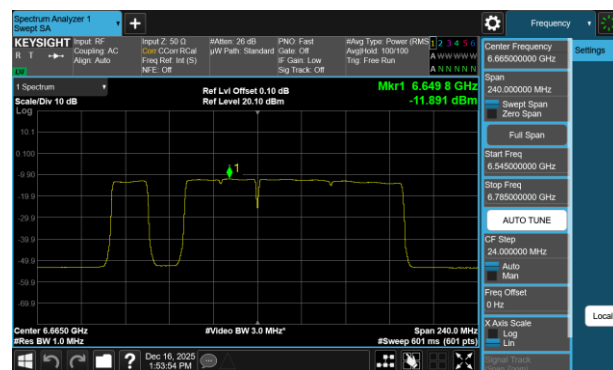
Plot 7-161 PSD Antenna 5T (160MHz BW 802.11be(RU) RU996+484+242 Index97 - Ch.143)
