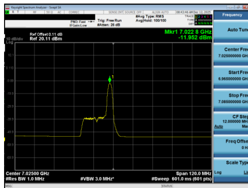
Plot 7-168 PSD Antenna 5T (80MHz BW 802.11be(RU) RU26 Index17 - Ch.215)
