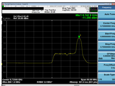
Plot 7-156 PSD Antenna 5T (40MHz BW 802.11be(RU) RU26 Index17 - Ch.155)
