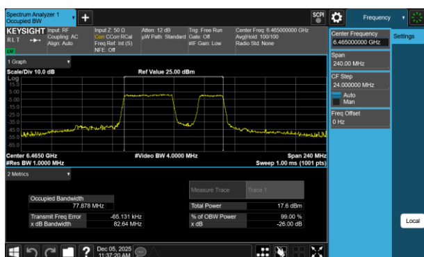
Plot 7-105 26dB BW & 99% OBW Antenna 1b (80MHz BW 802.11be(RU) RU484+242 Index92 - Ch.103)
