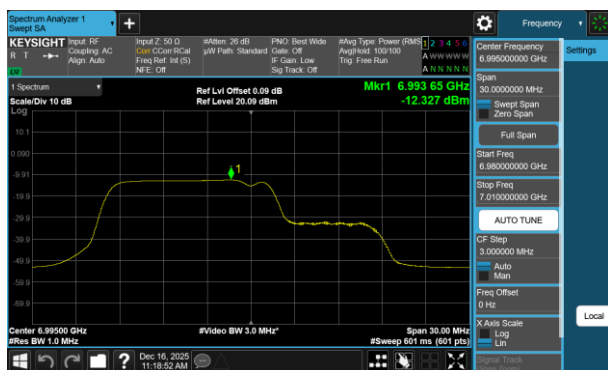
Plot 7-170 PSD Antenna 5T (20MHz BW 802.11be(RU) RU106+26 Index82 - Ch.209)
