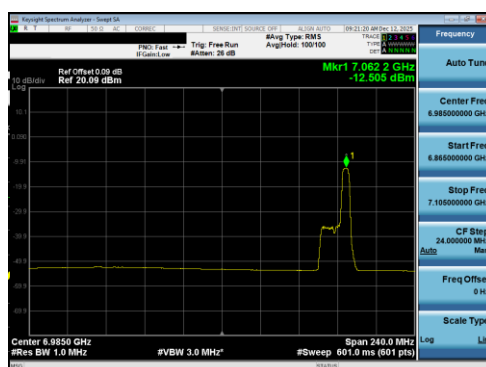
Plot 7-169 PSD Antenna 5T (160MHz BW 802.11be(RU) RU52 Index52 - Ch.207)
