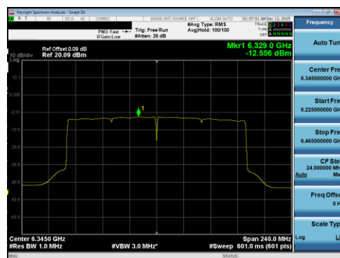
Plot 7-143 PSD Antenna 5T (160MHz BW 802.11be(RU) RU996X2 Index68 - Ch.79)
