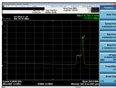
Plot 7-158 PSD Antenna 5T (160MHz BW 802.11be(RU) RU26 Index36 - Ch.143)
