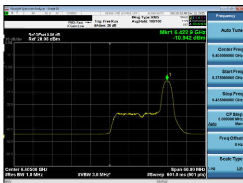
Plot 7-134 PSD Antenna 5T (40MHz BW 802.11be(RU) RU26 Index17 - Ch.91)
