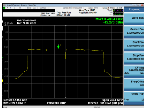
Plot 7-154 PSD Antenna 5T (160MHz BW 802.11be(RU) RU996X2 Index68 - Ch.111)
