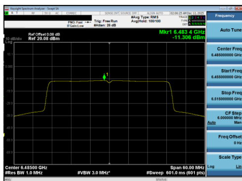
Plot 7-152 PSD Antenna 5T (40MHz BW 802.11be(RU) RU484 Index65 - Ch.107)
