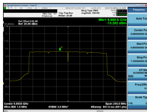
Plot 7-176 PSD Antenna 5T (160MHz BW 802.11be(RU) RU996X2 Index68 - Ch.207)
