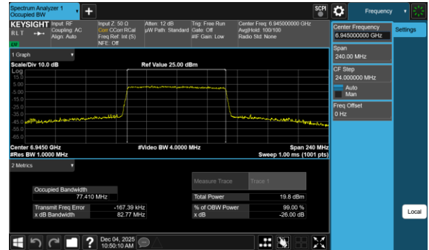
Plot 7-131 26dB BW & 99% OBW Antenna 1b (80MHz BW 802.11be(RU) RU996 Index67 - Ch.199)
