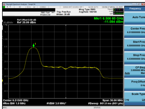
Plot 7-144 PSD Antenna 5T (20MHz BW 802.11be(RU) RU26 Index0 - Ch.113)
