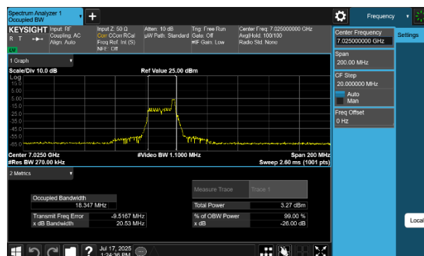
Plot 7-124 26dB BW & 99% OBW Antenna 1b (80MHz BW 802.11be(RU) RU26 Index17 - Ch.215)
