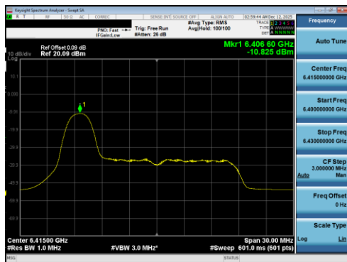
Plot 7-133 PSD Antenna 5T (20MHz BW 802.11be(RU) RU26 Index0 - Ch.93)
