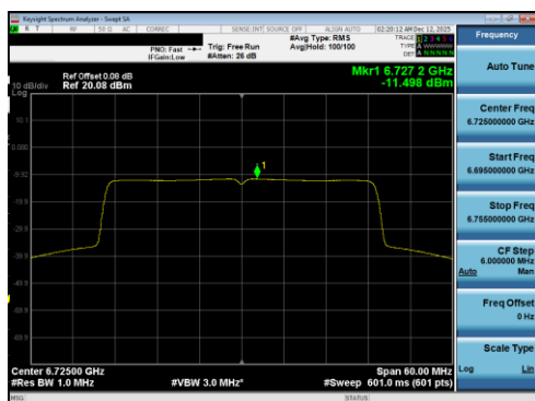
Plot 7-163 PSD Antenna 5T (40MHz BW 802.11be(RU) RU484 Index65 - Ch.155)
