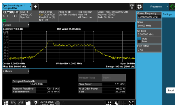
Plot 7-122 26dB BW & 99% OBW Antenna 1b (20MHz BW 802.11be(RU) RU26 Index0 - Ch.229)
