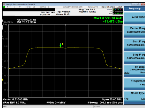
Plot 7-162 PSD Antenna 5T (20MHz BW 802.11be(RU) RU242 Index61 - Ch.117)
