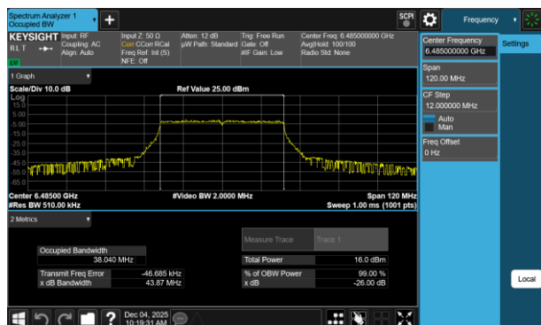
Plot 7-108 26dB BW & 99% OBW Antenna 1b (40MHz BW 802.11be(RU) RU484 Index65 - Ch.107)
