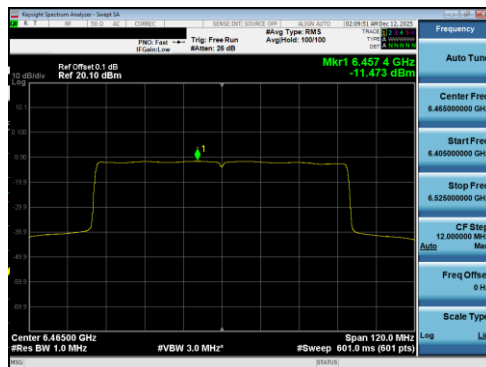
Plot 7-153 PSD Antenna 5T (80MHz BW 802.11be(RU) RU996 Index67 - Ch.103)
