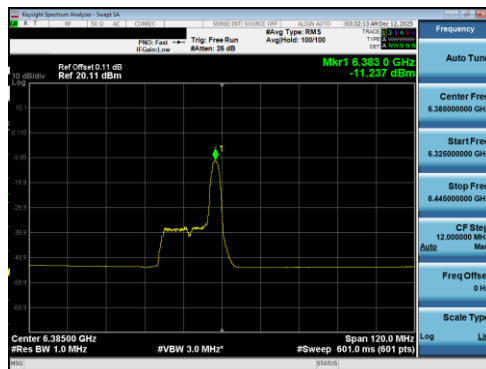
Plot 7-135 PSD Antenna 5T (80MHz BW 802.11be(RU) RU26 Index17 - Ch.87)
