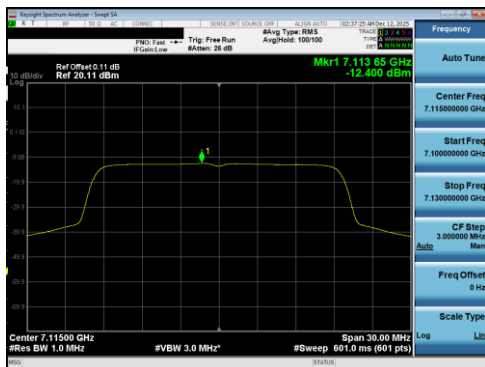
Plot 7-173 PSD Antenna 5T (20MHz BW 802.11be(RU) RU242 Index61 - Ch.233)
