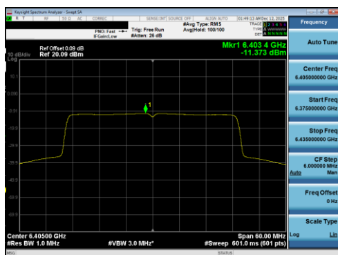
Plot 7-141 PSD Antenna 5T (40MHz BW 802.11be(RU) RU484 Index65 - Ch.91)
