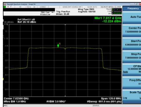
Plot 7-175 PSD Antenna 5T (80MHz BW 802.11be(RU) RU996 Index67 - Ch.215)
