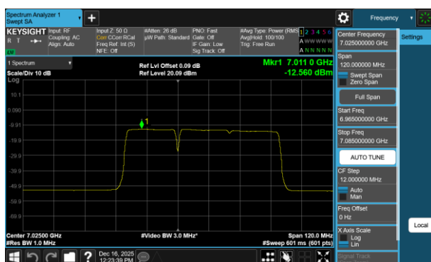
Plot 7-171 PSD Antenna 5T (80MHz BW 802.11be(RU) RU484+242 Index90 - Ch.215)
