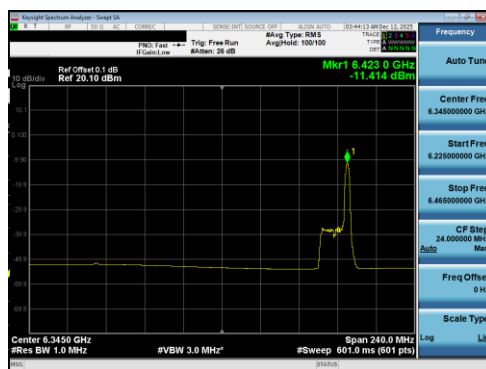
Plot 7-136 PSD Antenna 5T (160MHz BW 802.11be(RU) RU26 Index36 - Ch.79)
