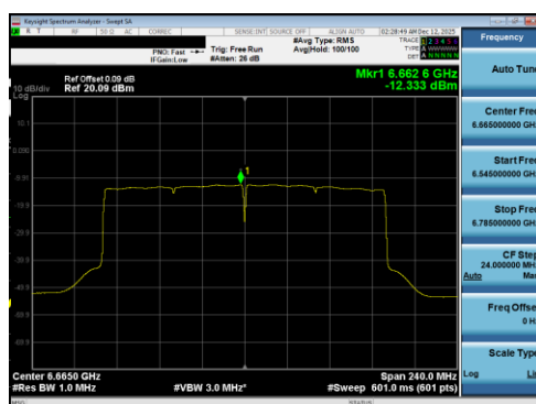
Plot 7-165 PSD Antenna 5T (160MHz BW 802.11be(RU) RU996X2 Index68 - Ch.143)
