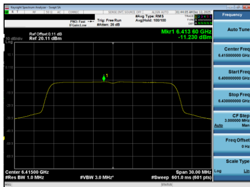
Plot 7-140 PSD Antenna 5T (20MHz BW 802.11be(RU) RU242 Index61 - Ch.93)
