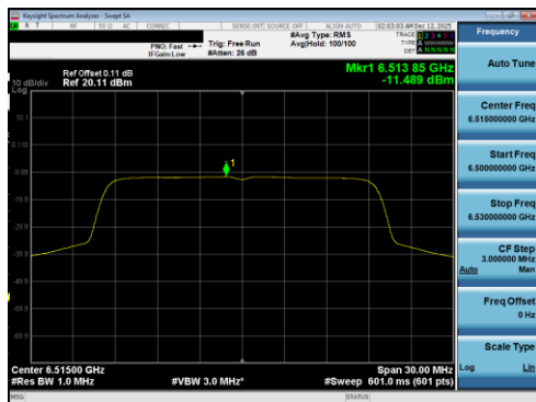
Plot 7-151 PSD Antenna 5T (20MHz BW 802.11be(RU) RU242 Index61 - Ch.113)
