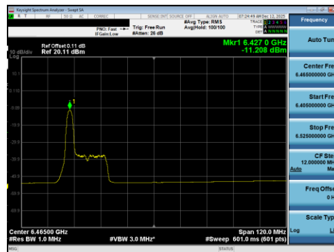
Plot 7-146 PSD Antenna 5T (80MHz BW 802.11be(RU) RU26 Index0 - Ch.103)
