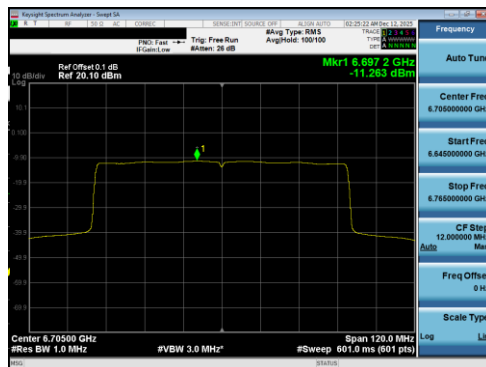
Plot 7-164 PSD Antenna 5T (80MHz BW 802.11be(RU) RU996 Index67 - Ch.151)
