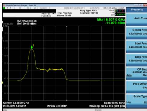
Plot 7-145 PSD Antenna 5T (40MHz BW 802.11be(RU) RU26 Index0 - Ch.115)
