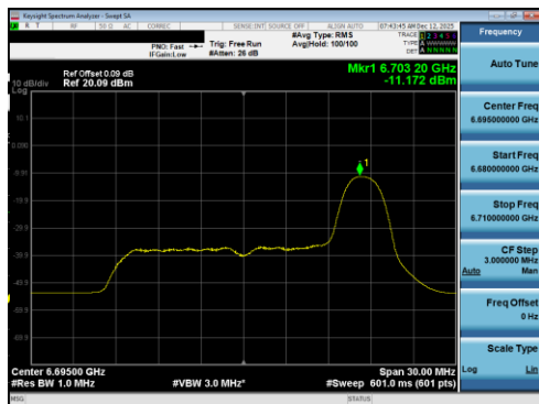
Plot 7-155 PSD Antenna 5T (20MHz BW 802.11be(RU) RU26 Index8 - Ch.149)
