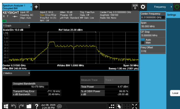
Plot 7-100 26dB BW & 99% OBW Antenna 1b (20MHz BW 802.11be(RU) RU26 Index0 - Ch.113)
