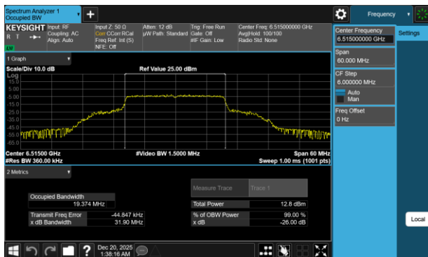
Plot 7-107 26dB BW & 99% OBW Antenna 1b (20MHz BW 802.11be(RU) RU242 Index61 - Ch.113)
