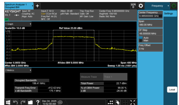
Plot 7-132 26dB BW & 99% OBW Antenna 1b (160MHz BW 802.11be(RU) RU996X2 Index68 - Ch.207)
