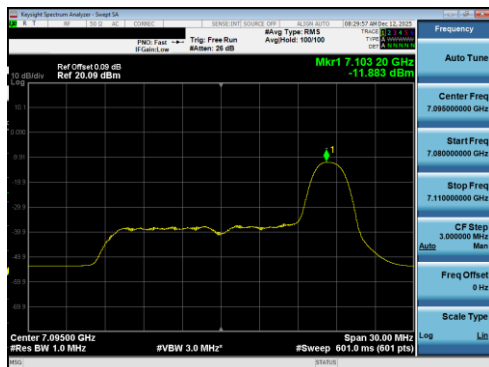
Plot 7-166 PSD Antenna 5T (20MHz BW 802.11be(RU) RU26 Index8 - Ch.229)
