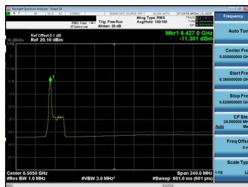
Plot 7-147 PSD Antenna 5T (160MHz BW 802.11be(RU) RU26 Index0 - Ch.111)
