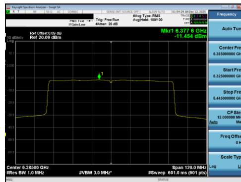
Plot 7-142 PSD Antenna 5T (80MHz BW 802.11be(RU) RU996 Index67 - Ch.87)
