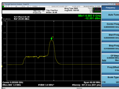
Plot 7-167 PSD Antenna 5T (40MHz BW 802.11be(RU) RU26 Index8 - Ch.187)
