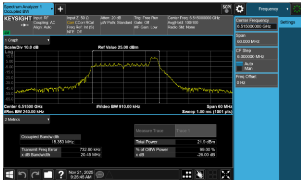
Plot 7-89 26dB BW & 99% OBW Antenna 3b (20MHz BW 802.11be(RU) RU26 Index8 - Ch.113)
