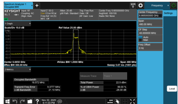
Plot 7-180 26dB BW & 99% OBW Antenna 1b (160MHz BW 802.11be(RU) RU26 Index0 - Ch.143)
