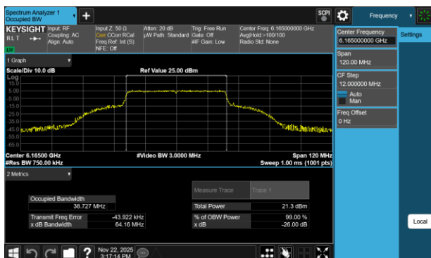
Plot 7-163 26dB BW & 99% OBW Antenna 1b (40MHz BW 802.11be(RU) RU484 Index65 - Ch.43)
