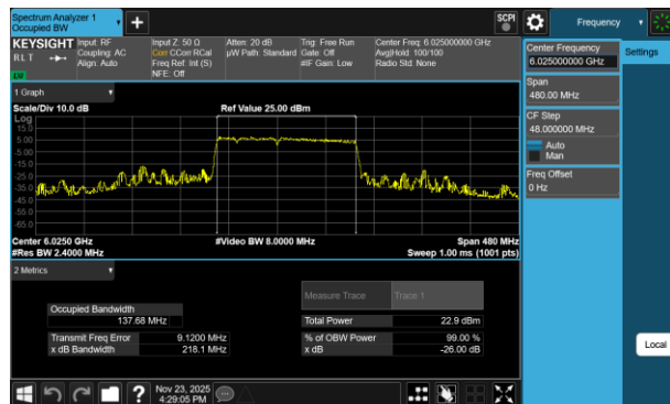
Plot 7-161 26dB BW & 99% OBW Antenna 1b (160MHz BW 802.11be(RU) RU996+484+242 Index96 - Ch.15)
