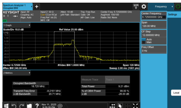
Plot 7-134 26dB BW & 99% OBW Antenna 3b (40MHz BW 802.11be(RU) RU26 Index8 - Ch.155)
