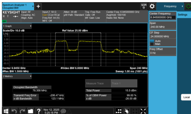
Plot 7-149 26dB BW & 99% OBW Antenna 3b (80MHz BW 802.11be(RU) RU484+242 Index91 - Ch.199)
