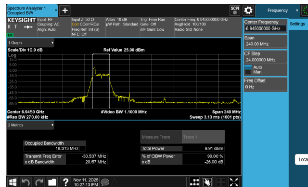
Plot 7-146 26dB BW & 99% OBW Antenna 3b (80MHz BW 802.11be(RU) RU26 Index0 - Ch.199)
