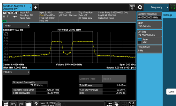
Plot 7-127 26dB BW & 99% OBW Antenna 3b (80MHz BW 802.11be(RU) RU484+242 Index91 - Ch.103)
