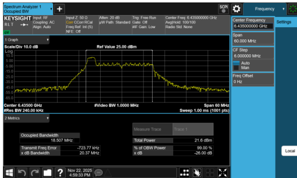
Plot 7-166 26dB BW & 99% OBW Antenna 1b (20MHz BW 802.11be(RU) RU26 Index0 - Ch.97)
