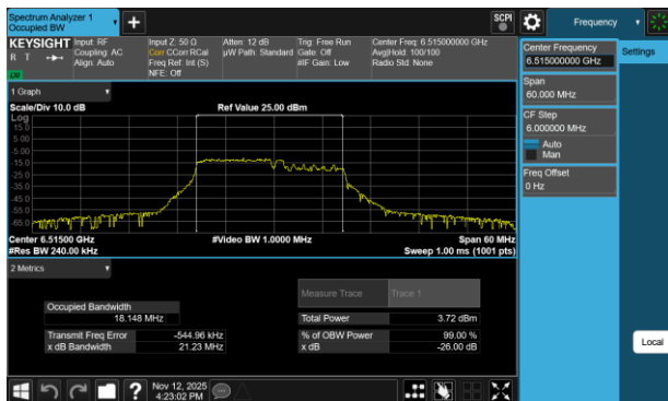
Plot 7-126 26dB BW & 99% OBW Antenna 3b (20MHz BW 802.11be(RU) RU106+26 Index82 - Ch.113)
