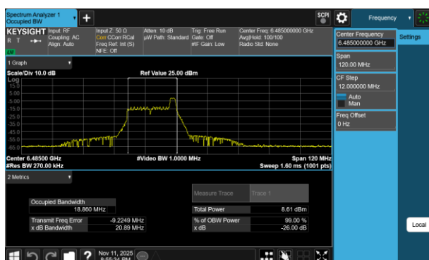
Plot 7-123 26dB BW & 99% OBW Antenna 3b (40MHz BW 802.11be(RU) RU26 Index8 - Ch.107)
