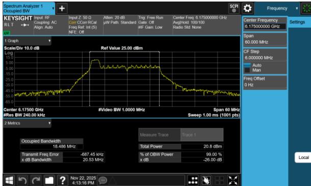
Plot 7-155 26dB BW & 99% OBW Antenna 1b (20MHz BW 802.11be(RU) RU26 Index0 - Ch.45)
