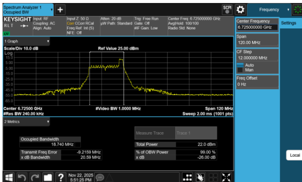
Plot 7-178 26dB BW & 99% OBW Antenna 1b (40MHz BW 802.11be(RU) RU26 Index8 - Ch.155)
