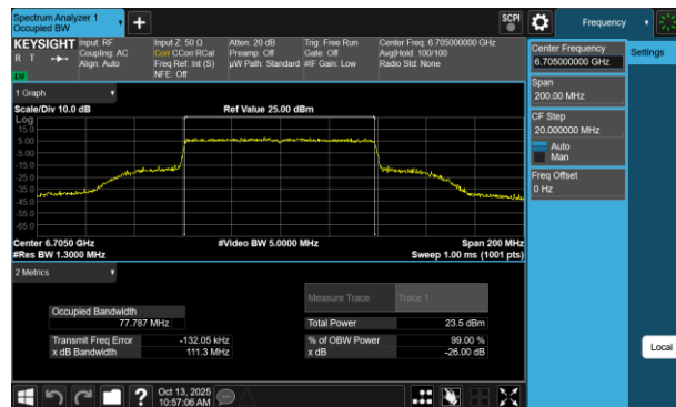
Plot 7-109 26dB BW & 99% OBW Antenna 3b (80MHz BW 802.11be(RU) RU996 Index67 - Ch.151)
