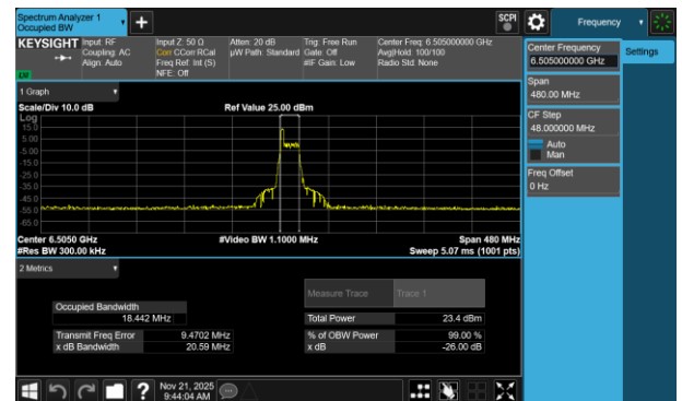
Plot 7-92 26dB BW & 99% OBW Antenna 3b (160MHz BW 802.11be(RU) RU26 Index0 - Ch.111)
