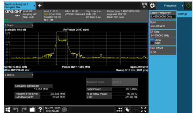
Plot 7-91 26dB BW & 99% OBW Antenna 3b (80MHz BW 802.11be(RU) RU26 Index0 - Ch.103)
