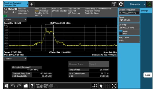
Plot 7-179 26dB BW & 99% OBW Antenna 1b (80MHz BW 802.11be(RU) RU26 Index0 - Ch.151)
