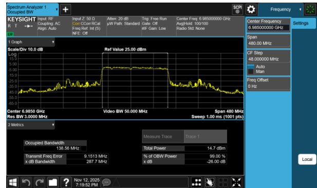
Plot 7-150 26dB BW & 99% OBW Antenna 3b (160MHz BW 802.11be(RU) RU996+484+242 Index96 - Ch.207)
