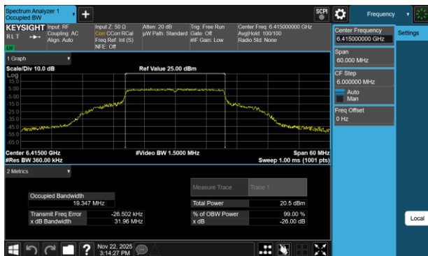
Plot 7-162 26dB BW & 99% OBW Antenna 1b (20MHz BW 802.11be(RU) RU242 Index61 - Ch.93)
