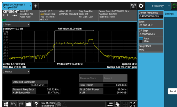
Plot 7-122 26dB BW & 99% OBW Antenna 3b (20MHz BW 802.11be(RU) RU26 Index8 - Ch.105)
