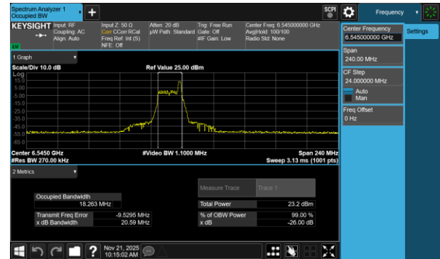
Plot 7-102 26dB BW & 99% OBW Antenna 3b (80MHz BW 802.11be(RU) RU26 Index17 - Ch.119)
