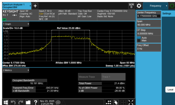
Plot 7-159 26dB BW & 99% OBW Antenna 1b (20MHz BW 802.11be(RU) RU106+26 Index82 - Ch.45)
