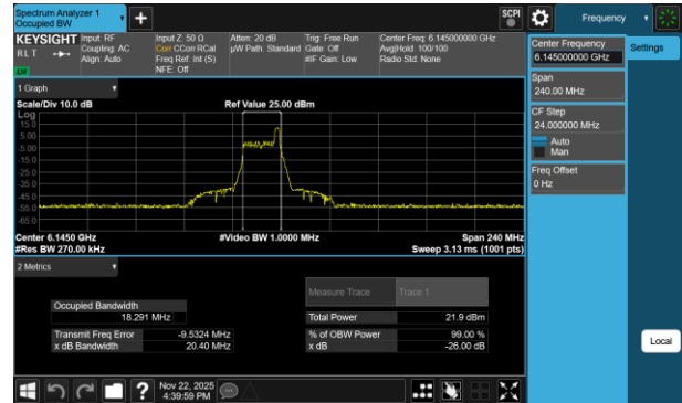
Plot 7-157 26dB BW & 99% OBW Antenna 1b (80MHz BW 802.11be(RU) RU26 Index17 - Ch.39)
