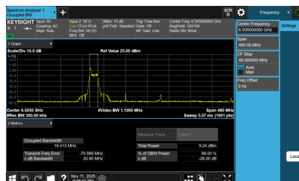
Plot 7-125 26dB BW & 99% OBW Antenna 3b (160MHz BW 802.11be(RU) RU26 Index0 - Ch.111)
