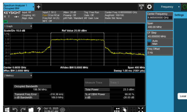
Plot 7-110 26dB BW & 99% OBW Antenna 3b (160MHz BW 802.11be(RU) RU996X2 Index68 - Ch.143)
