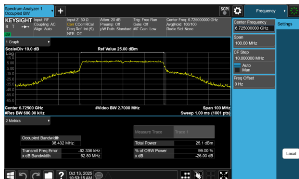
Plot 7-108 26dB BW & 99% OBW Antenna 3b (40MHz BW 802.11be(RU) RU484 Index65 - Ch.155)
