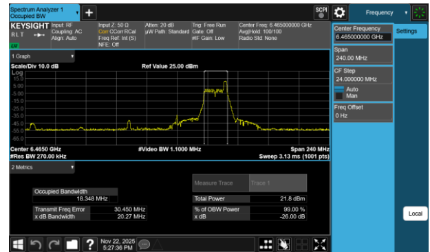
Plot 7-168 26dB BW & 99% OBW Antenna 1b (80MHz BW 802.11be(RU) RU26 Index36 - Ch.103)
