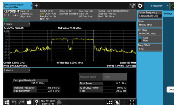
Plot 7-128 26dB BW & 99% OBW Antenna 3b (160MHz BW 802.11be(RU) RU996+484+242 Index99 - Ch.111)
