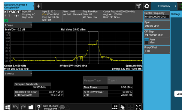
Plot 7-124 26dB BW & 99% OBW Antenna 3b (80MHz BW 802.11be(RU) RU26 Index36 - Ch.103)
