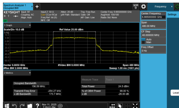
Plot 7-143 26dB BW & 99% OBW Antenna 3b (160MHz BW 802.11be(RU) RU996X2 Index68 - Ch.143)
