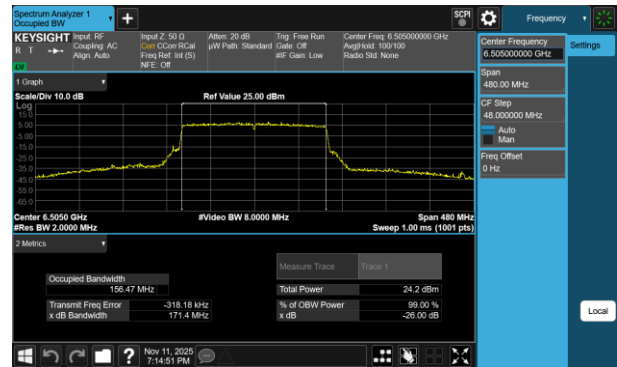
Plot 7-132 26dB BW & 99% OBW Antenna 3b (160MHz BW 802.11be(RU) RU996X2 Index68 - Ch.111)
