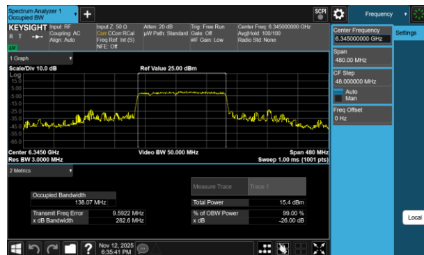
Plot 7-117 26dB BW & 99% OBW Antenna 3b (160MHz BW 802.11be(RU) RU996+484+242 Index96 - Ch.79)
