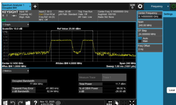
Plot 7-116 26dB BW & 99% OBW Antenna 3b (80MHz BW 802.11be(RU) RU484+242 Index92 - Ch.39)
