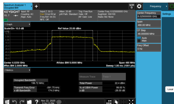
Plot 7-165 26dB BW & 99% OBW Antenna 1b (160MHz BW 802.11be(RU) RU996X2 Index68 - Ch.15)
