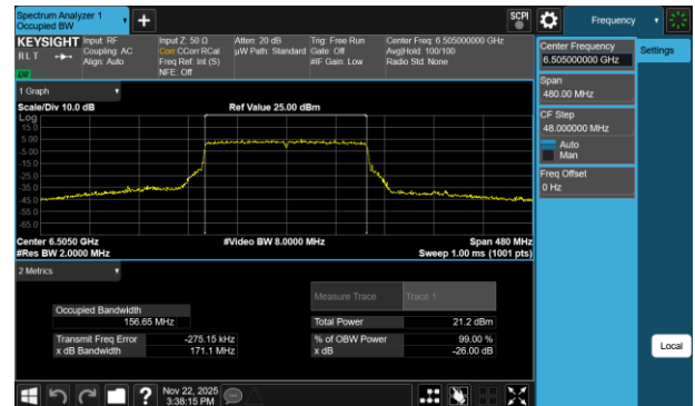
Plot 7-176 26dB BW & 99% OBW Antenna 1b (160MHz BW 802.11be(RU) RU996X2 Index68 - Ch.111)
