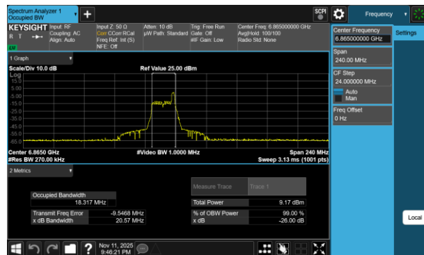
Plot 7-135 26dB BW & 99% OBW Antenna 3b (80MHz BW 802.11be(RU) RU26 Index17 - Ch.183)
