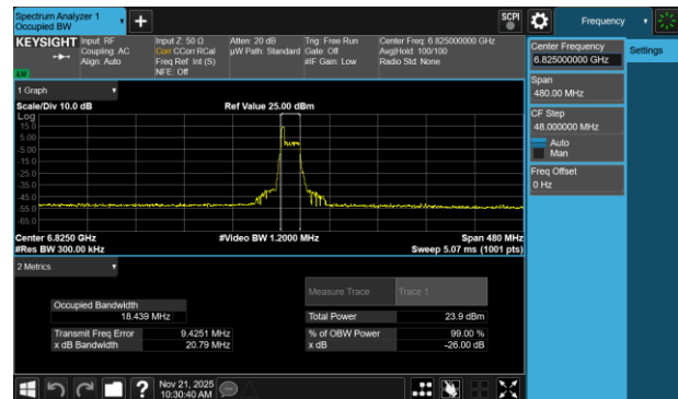
Plot 7-103 26dB BW & 99% OBW Antenna 3b (160MHz BW 802.11be(RU) RU26 Index0 - Ch.175)
