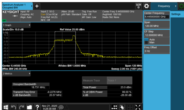
Plot 7-90 26dB BW & 99% OBW Antenna 3b (40MHz BW 802.11be(RU) RU26 Index8 - Ch.99)
