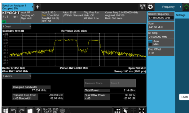
Plot 7-160 26dB BW & 99% OBW Antenna 1b (80MHz BW 802.11be(RU) RU484+242 Index92 - Ch.39)
