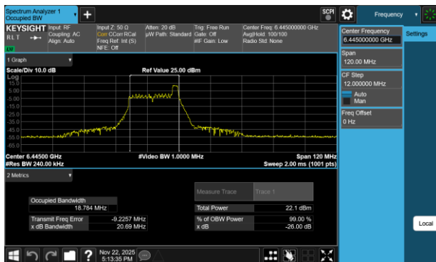
Plot 7-167 26dB BW & 99% OBW Antenna 1b (40MHz BW 802.11be(RU) RU26 Index8 - Ch.99)
