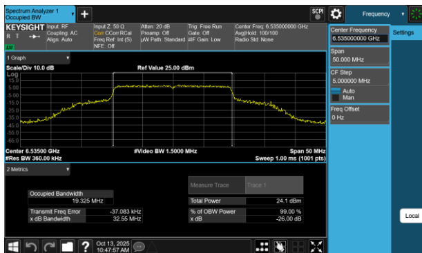
Plot 7-107 26dB BW & 99% OBW Antenna 3b (20MHz BW 802.11be(RU) RU242 Index61 - Ch.117)
