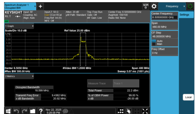
Plot 7-169 26dB BW & 99% OBW Antenna 1b (160MHz BW 802.11be(RU) RU26 Index0 - Ch.111)
