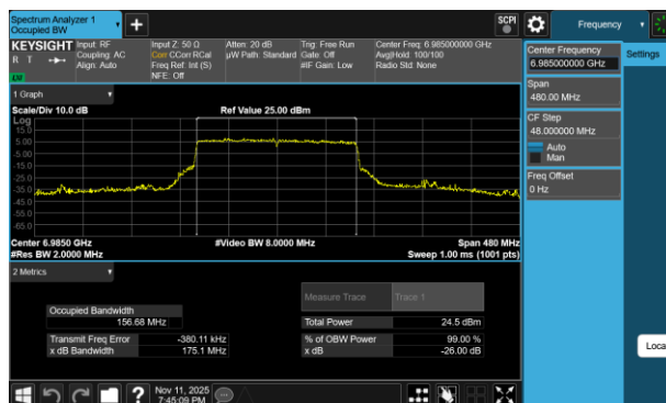
Plot 7-154 26dB BW & 99% OBW Antenna 3b (160MHz BW 802.11be(RU) RU996X2 Index68 - Ch.207)
