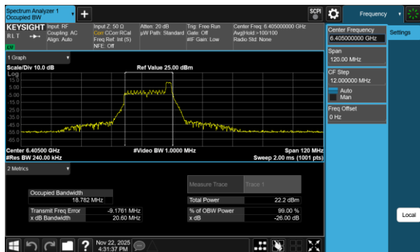
Plot 7-156 26dB BW & 99% OBW Antenna 1b (40MHz BW 802.11be(RU) RU26 Index8 - Ch.91)
