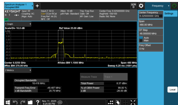
Plot 7-114 26dB BW & 99% OBW Antenna 3b (160MHz BW 802.11be(RU) RU26 Index17 - Ch.15)
