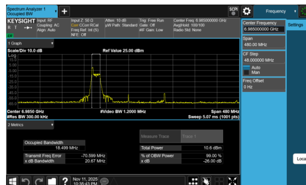
Plot 7-147 26dB BW & 99% OBW Antenna 3b (160MHz BW 802.11be(RU) RU26 Index0 - Ch.207)
