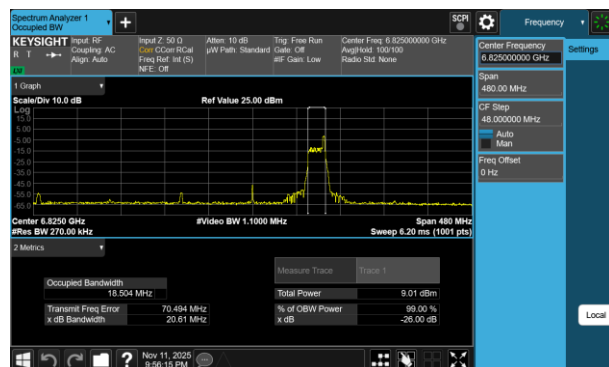
Plot 7-136 26dB BW & 99% OBW Antenna 3b (160MHz BW 802.11be(RU) RU26 Index36 - Ch.175)
