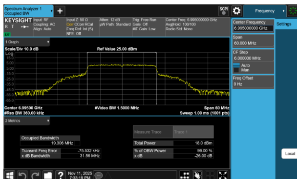
Plot 7-152 26dB BW & 99% OBW Antenna 3b (20MHz BW 802.11be(RU) RU242 Index61 - Ch.209)
