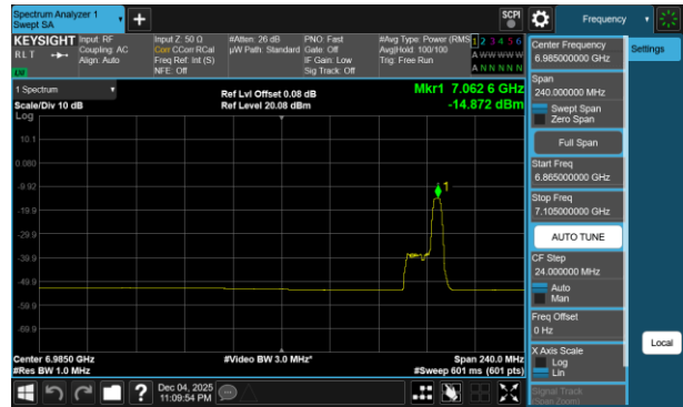
Plot 7-426 PSD SDM Diversity Antenna 1b (160MHz BW 802.11be(RU) RU52 Index52 - Ch.207)
