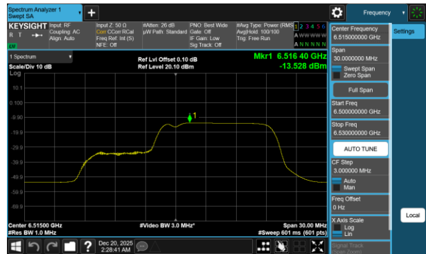
Plot 7-386 PSD SDM Diversity Antenna 1b (20MHz BW 802.11be(RU) RU106+26 Index83 - Ch.113)
