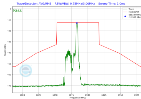
Plot 7-454 In-Band Emission Plot Antenna 5T (40MHz BW 802.11be(RU) RU26 Index8 (UNII Band 8) - Ch.187)
