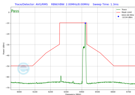
Plot 7-444 In-Band Emission Plot Antenna 5T (160MHz BW 802.11be(RU) RU26 Index36 (UNII Band 5) - Ch.79)
