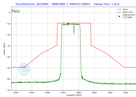
Plot 7-458 In-Band Emission Plot Antenna 5T (80MHz BW 802.11be(RU) RU484+242 Index93 (UNII Band 5) - Ch.87)
