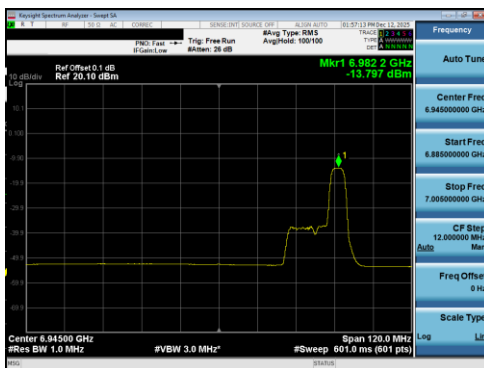
Plot 7-421 PSD SDM Diversity Antenna 5T (80MHz BW 802.11be(RU) RU52 Index52 - Ch.199)
