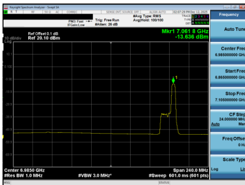
Plot 7-422 PSD SDM Diversity Antenna 5T (160MHz BW 802.11be(RU) RU52 Index52 - Ch.207)
