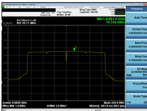
Plot 7-414 PSD SDM Diversity Antenna 5T (160MHz BW 802.11be(RU) RU996X2 Index68 - Ch.143)
