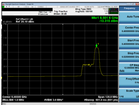
Plot 7-377 PSD SDM Diversity Antenna 5T (80MHz BW 802.11be(RU) RU52 Index52 - Ch.103)
