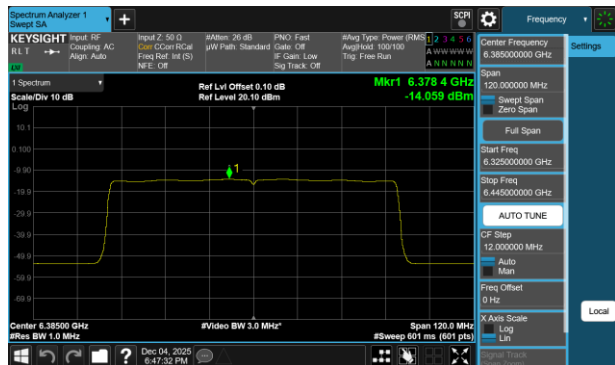
Plot 7-373 PSD SDM Diversity Antenna 1b (80MHz BW 802.11be(RU) RU996 Index67 - Ch.87)
