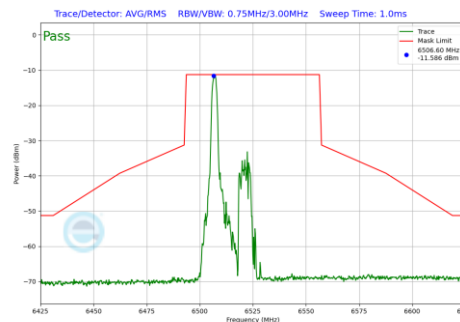
Plot 7-446 In-Band Emission Plot Antenna 5T (40MHz BW 802.11be(RU) RU26 Index0 (UNII Band 6) - Ch.115)
