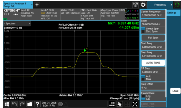
Plot 7-401 PSD SDM Diversity Antenna 1b (20MHz BW 802.11be(RU) RU52 Index39 - Ch.149)
