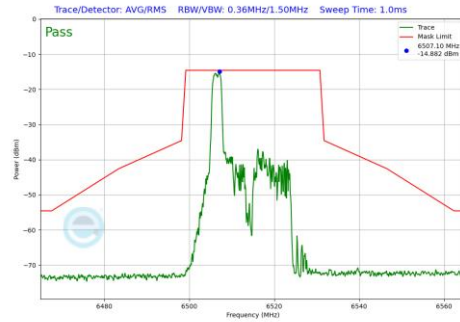
Plot 7-445 In-Band Emission Plot Antenna 5T (20MHz BW 802.11be(RU) RU26 Index0 (UNII Band 6) - Ch.113)
