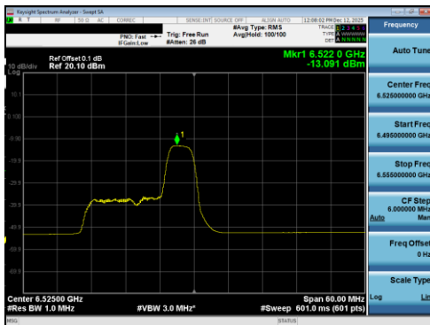
Plot 7-376 PSD SDM Diversity Antenna 5T (40MHz BW 802.11be(RU) RU52 Index40 - Ch.115)
