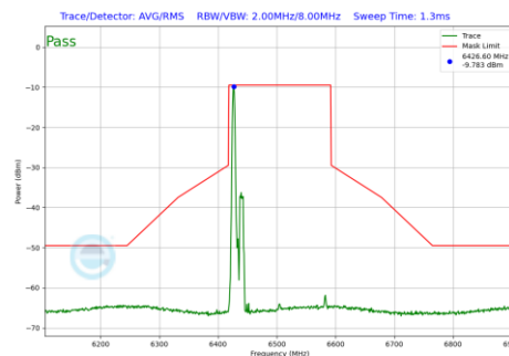
Plot 7-448 In-Band Emission Plot Antenna 5T (160MHz BW 802.11be(RU) RU26 Index0 (UNII Band 6) - Ch.111)
