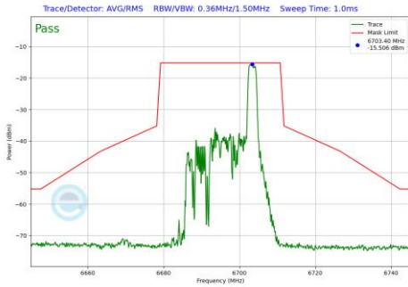
Plot 7-449 In-Band Emission Plot Antenna 5T (20MHz BW 802.11be(RU) RU26 Index8 (UNII Band 7) - Ch.149)
