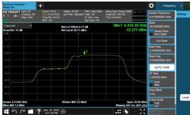
Plot 7-361 PSD SDM Diversity Antenna 5T (20MHz BW 802.11be(RU) RU106+26 Index83 - Ch.93)
