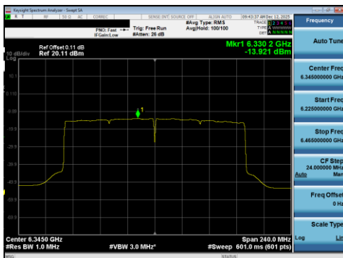
Plot 7-370 PSD SDM Diversity Antenna 5T (160MHz BW 802.11be(RU) RU996X2 Index68 - Ch.79)
