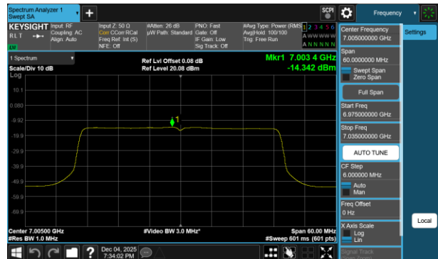
Plot 7-438 PSD SDM Diversity Antenna 1b (40MHz BW 802.11be(RU) RU484 Index65 - Ch.211)
