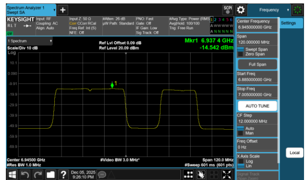
Plot 7-431 PSD SDM Diversity Antenna 1b (80MHz BW 802.11be(RU) RU484+242 Index92 - Ch.199)
