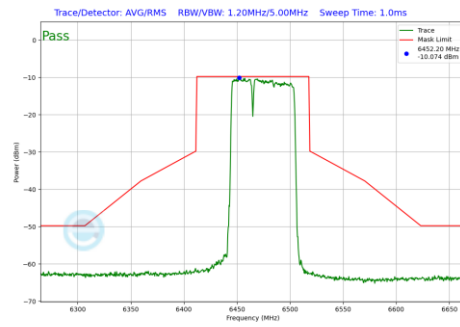
Plot 7-461 In-Band Emission Plot Antenna 5T (80MHz BW 802.11be(RU) RU484+242 Index90 (UNII Band 6) - Ch.103)
