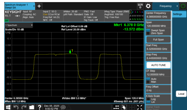
Plot 7-365 PSD SDM Diversity Antenna 1b (80MHz BW 802.11be(RU) RU484+242 Index92 - Ch.87)
