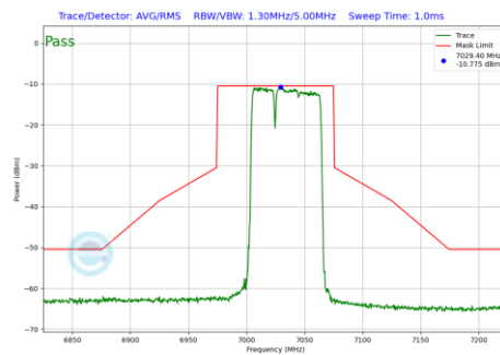
Plot 7-467 In-Band Emission Plot Antenna 5T (80MHz BW 802.11be(RU) RU484+242 Index90 (UNII Band 8) - Ch.215)
