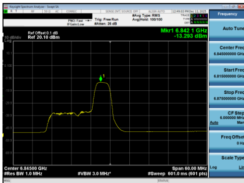
Plot 7-398 PSD SDM Diversity Antenna 5T (40MHz BW 802.11be(RU) RU52 Index40 - Ch.179)
