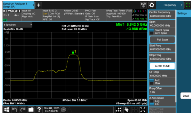
Plot 7-402 PSD SDM Diversity Antenna 1b (40MHz BW 802.11be(RU) RU52 Index40 - Ch.179)
