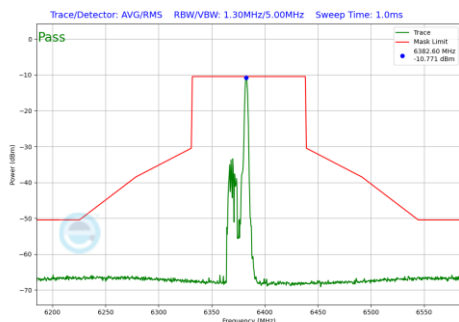
Plot 7-443 In-Band Emission Plot Antenna 5T (80MHz BW 802.11be(RU) RU26 Index17 (UNII Band 5) - Ch.87)
