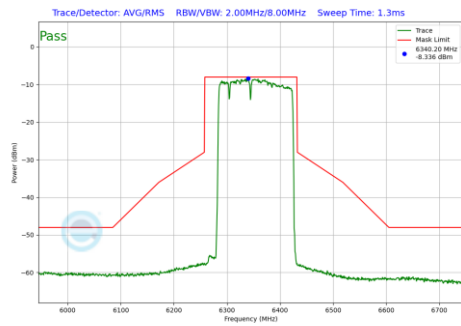
Plot 7-459 In-Band Emission Plot Antenna 5T (160MHz BW 802.11be(RU) RU996+484+242 Index96 (UNII Band 5) - Ch.79)
