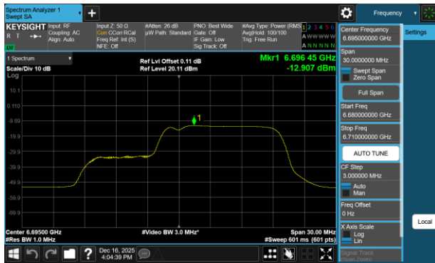
Plot 7-405 PSD SDM Diversity Antenna 5T (20MHz BW 802.11be(RU) RU106+26 Index83 - Ch.149)
