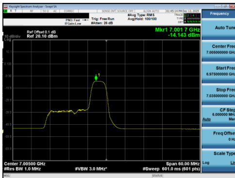
Plot 7-420 PSD SDM Diversity Antenna 5T (40MHz BW 802.11be(RU) RU52 Index40 - Ch.211)
