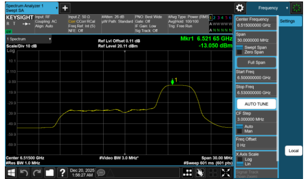
Plot 7-379 PSD SDM Diversity Antenna 1b (20MHz BW 802.11be(RU) RU52 Index40 - Ch.113)
