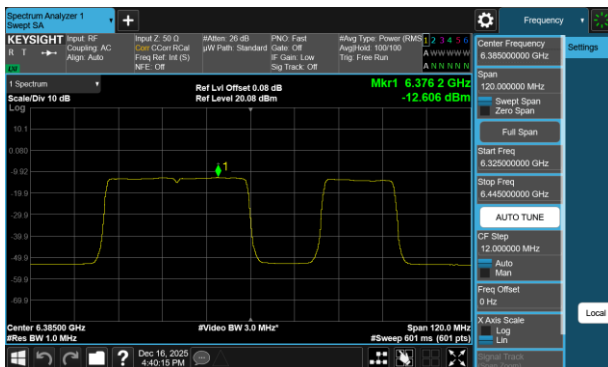
Plot 7-362 PSD SDM Diversity Antenna 5T (80MHz BW 802.11be(RU) RU484+242 Index92 - Ch.87)
