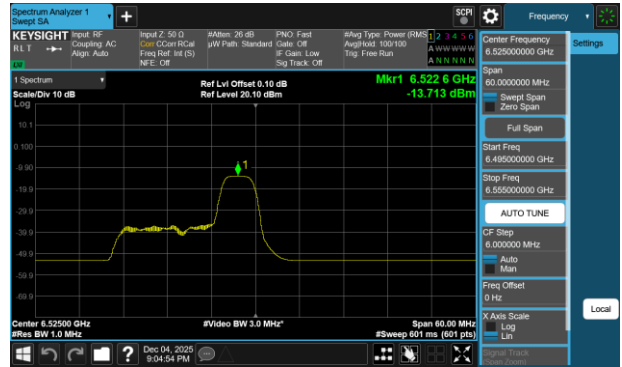
Plot 7-380 PSD SDM Diversity Antenna 1b (40MHz BW 802.11be(RU) RU52 Index40 - Ch.115)
