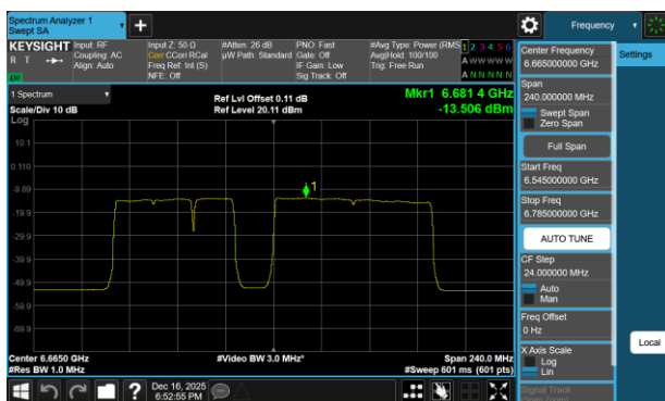
Plot 7-407 PSD SDM Diversity Antenna 5T (160MHz BW 802.11be(RU) RU996+484+242 Index99 - Ch.143)
