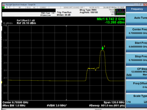
Plot 7-399 PSD SDM Diversity Antenna 5T (80MHz BW 802.11be(RU) RU52 Index52 - Ch.151)
