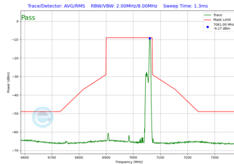
Plot 7-456 In-Band Emission Plot Antenna 5T (160MHz BW 802.11be(RU) RU52 Index52 (UNII Band 8) - Ch.207)
