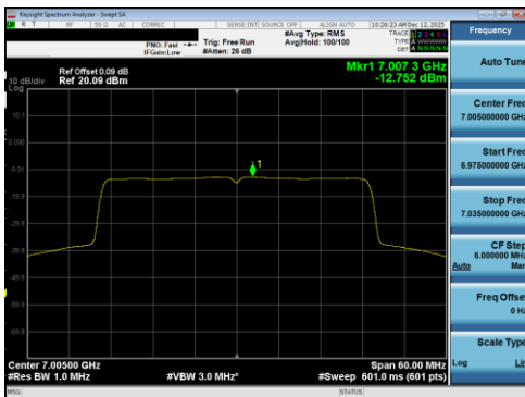
Plot 7-434 PSD SDM Diversity Antenna 5T (40MHz BW 802.11be(RU) RU484 Index65 - Ch.211)
