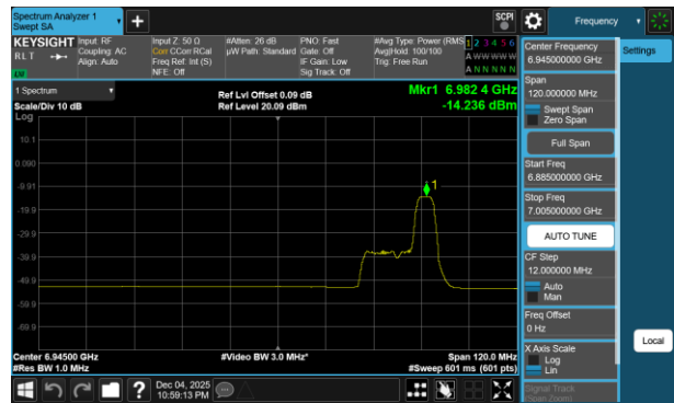
Plot 7-425 PSD SDM Diversity Antenna 1b (80MHz BW 802.11be(RU) RU52 Index52 - Ch.199)
