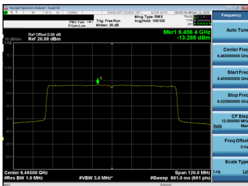
Plot 7-391 PSD SDM Diversity Antenna 5T (80MHz BW 802.11be(RU) RU996 Index67 - Ch.103)
