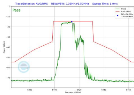
Plot 7-457 In-Band Emission Plot Antenna 5T (20MHz BW 802.11be(RU) RU106+26 Index82 (UNII Band 5) - Ch.93)
