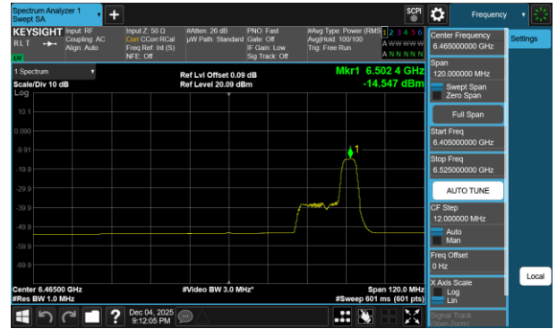
Plot 7-381 PSD SDM Diversity Antenna 1b (80MHz BW 802.11be(RU) RU52 Index52 - Ch.103)
