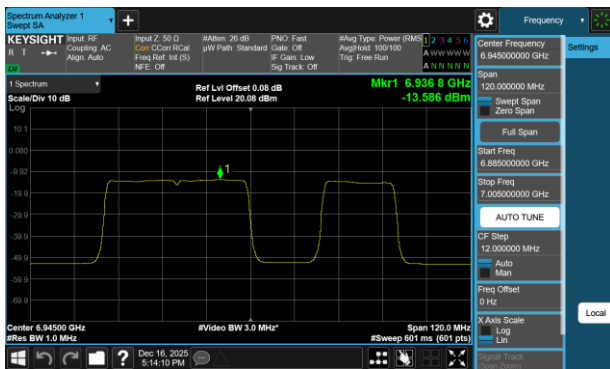
Plot 7-428 PSD SDM Diversity Antenna 5T (80MHz BW 802.11be(RU) RU484+242 Index92 - Ch.199)
