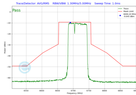
Plot 7-464 In-Band Emission Plot Antenna 5T (80MHz BW 802.11be(RU) RU484+242 Index90 (UNII Band 7) - Ch.151)
