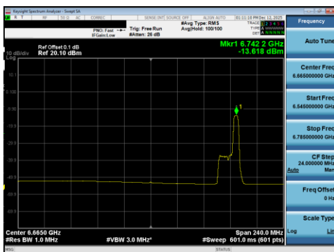
Plot 7-400 PSD SDM Diversity Antenna 5T (160MHz BW 802.11be(RU) RU52 Index52 - Ch.143)
