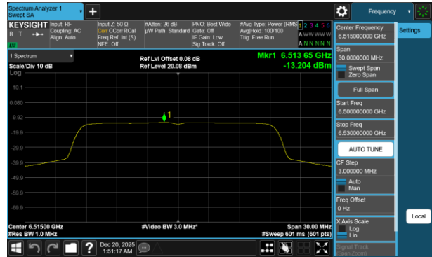
Plot 7-393 PSD SDM Diversity Antenna 1b (20MHz BW 802.11be(RU) RU242 Index61 - Ch.113)
