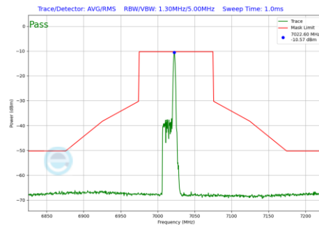
Plot 7-455 In-Band Emission Plot Antenna 5T (80MHz BW 802.11be(RU) RU26 Index17 (UNII Band 8) - Ch.215)
