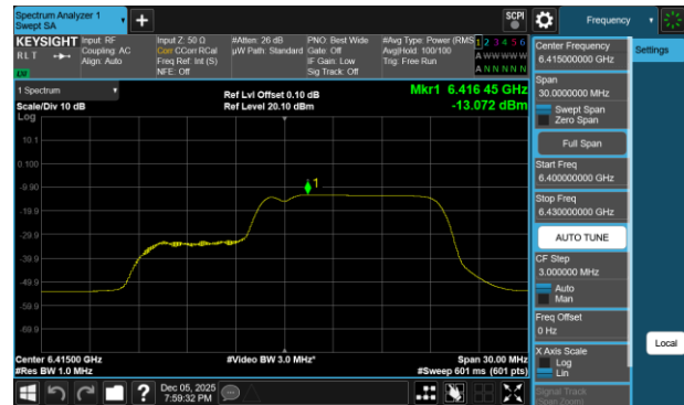
Plot 7-364 PSD SDM Diversity Antenna 1b (20MHz BW 802.11be(RU) RU106+26 Index83 - Ch.93)
