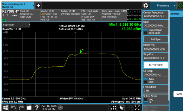
Plot 7-383 PSD SDM Diversity Antenna 5T (20MHz BW 802.11be(RU) RU106+26 Index83 - Ch.113)
