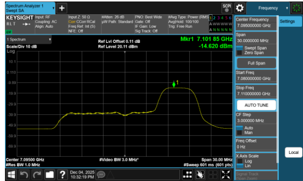
Plot 7-423 PSD SDM Diversity Antenna 1b (20MHz BW 802.11be(RU) RU52 Index40 - Ch.229)
