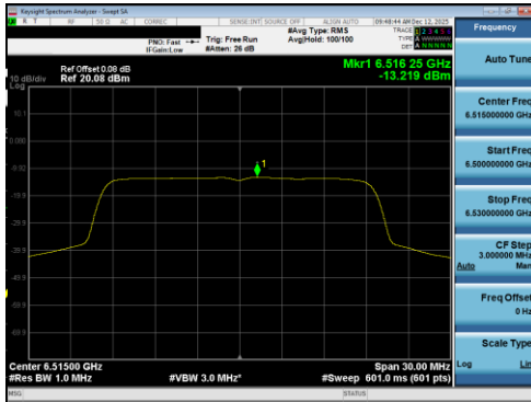
Plot 7-389 PSD SDM Diversity Antenna 5T (20MHz BW 802.11be(RU) RU242 Index61 - Ch.113)
