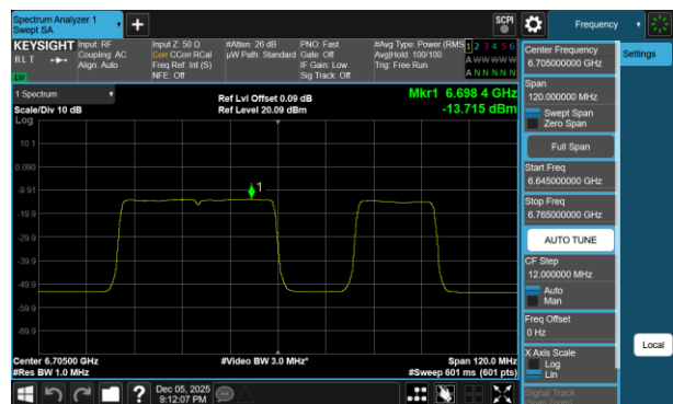
Plot 7-409 PSD SDM Diversity Antenna 1b (80MHz BW 802.11be(RU) RU484+242 Index92 - Ch.151)
