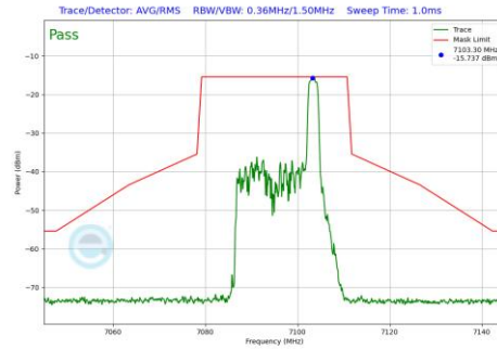
Plot 7-453 In-Band Emission Plot Antenna 5T (20MHz BW 802.11be(RU) RU26 Index8 (UNII Band 8) - Ch.229)
