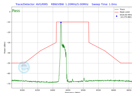
Plot 7-447 In-Band Emission Plot Antenna 5T (80MHz BW 802.11be(RU) RU26 Index0 (UNII Band 6) - Ch.103)
