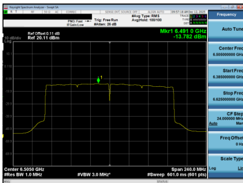
Plot 7-392 PSD SDM Diversity Antenna 5T (160MHz BW 802.11be(RU) RU996X2 Index68 - Ch.111)
