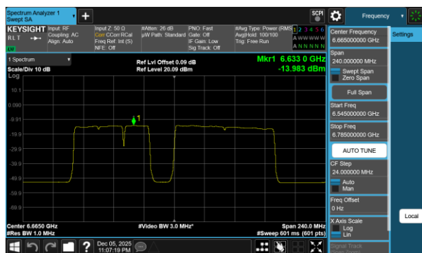
Plot 7-410 PSD SDM Diversity Antenna 1b (160MHz BW 802.11be(RU) RU996+484+242 Index99 - Ch.143)
