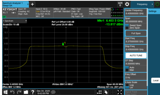
Plot 7-372 PSD SDM Diversity Antenna 1b (40MHz BW 802.11be(RU) RU484 Index65 - Ch.91)
