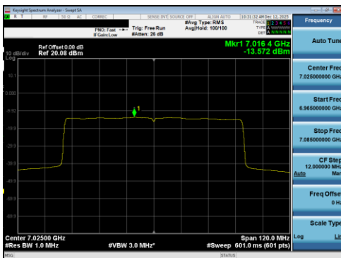
Plot 7-435 PSD SDM Diversity Antenna 5T (80MHz BW 802.11be(RU) RU996 Index67 - Ch.215)
