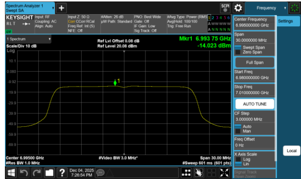
Plot 7-437 PSD SDM Diversity Antenna 1b (20MHz BW 802.11be(RU) RU242 Index61 - Ch.209)
