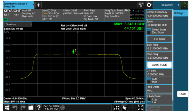
Plot 7-416 PSD SDM Diversity Antenna 1b (40MHz BW 802.11be(RU) RU484 Index65 - Ch.179)
