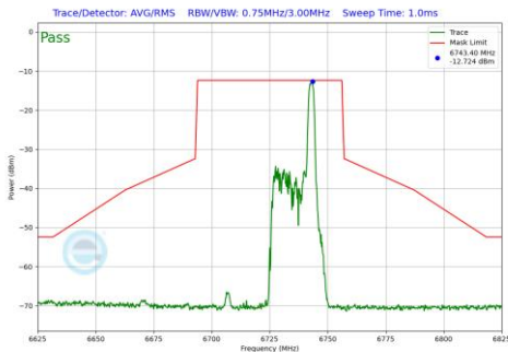
Plot 7-450 In-Band Emission Plot Antenna 5T (40MHz BW 802.11be(RU) RU26 Index17 (UNII Band 7) - Ch.155)
