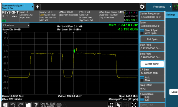
Plot 7-363 PSD SDM Diversity Antenna 5T (160MHz BW 802.11be(RU) RU996+484+242 Index99 - Ch.79)
