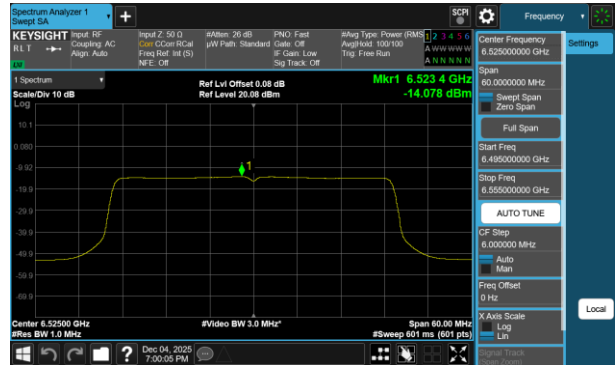
Plot 7-394 PSD SDM Diversity Antenna 1b (40MHz BW 802.11be(RU) RU484 Index65 - Ch.115)
