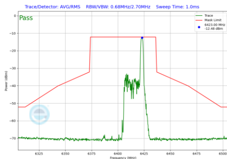
Plot 7-442 In-Band Emission Plot Antenna 5T (40MHz BW 802.11be(RU) RU26 Index17 (UNII Band 5) - Ch.91)
