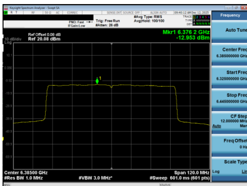
Plot 7-369 PSD SDM Diversity Antenna 5T (80MHz BW 802.11be(RU) RU996 Index67 - Ch.87)
