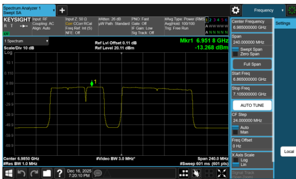
Plot 7-429 PSD SDM Diversity Antenna 5T (160MHz BW 802.11be(RU) RU996+484+242 Index99 - Ch.207)
