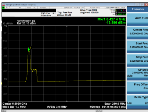
Plot 7-378 PSD SDM Diversity Antenna 5T (160MHz BW 802.11be(RU) RU52 Index37 - Ch.111)
