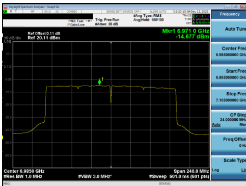
Plot 7-436 PSD SDM Diversity Antenna 5T (160MHz BW 802.11be(RU) RU996X2 Index68 - Ch.207)
