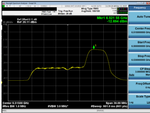
Plot 7-375 PSD SDM Diversity Antenna 5T (20MHz BW 802.11be(RU) RU52 Index40 - Ch.113)
