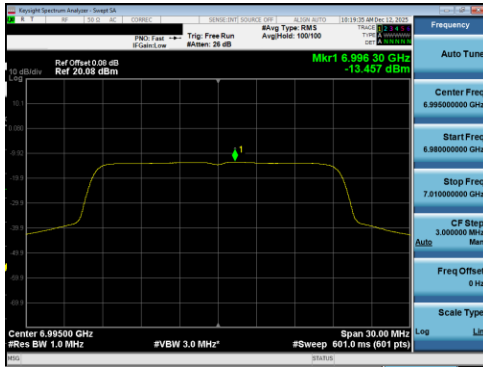
Plot 7-433 PSD SDM Diversity Antenna 5T (20MHz BW 802.11be(RU) RU242 Index61 - Ch.209)
