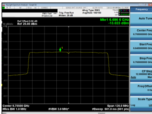
Plot 7-413 PSD SDM Diversity Antenna 5T (80MHz BW 802.11be(RU) RU996 Index67 - Ch.151)
