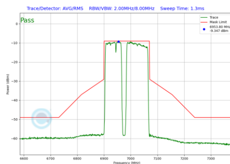
Plot 7-468 In-Band Emission Plot Antenna 5T (160MHz BW 802.11be(RU) RU996+484+242 Index99 (UNII Band 8) - Ch.207)
