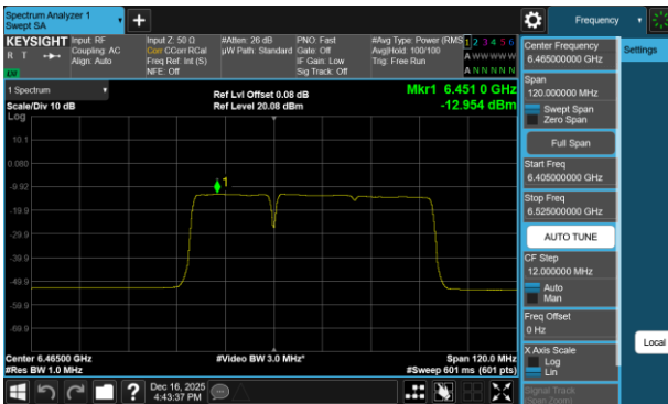
Plot 7-384 PSD SDM Diversity Antenna 5T (80MHz BW 802.11be(RU) RU484+242 Index90 - Ch.103)
