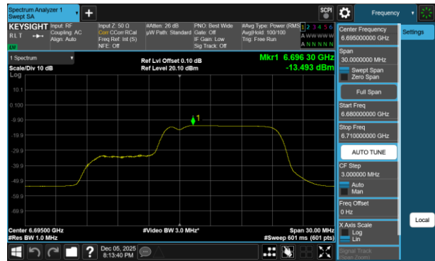
Plot 7-408 PSD SDM Diversity Antenna 1b (20MHz BW 802.11be(RU) RU106+26 Index83 - Ch.149)
