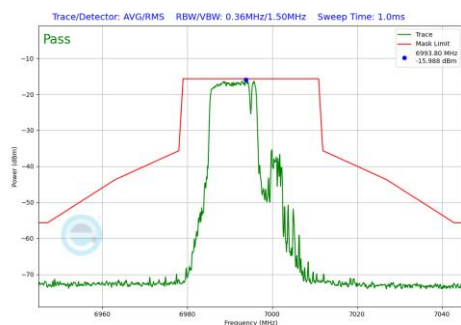
Plot 7-466 In-Band Emission Plot Antenna 5T (20MHz BW 802.11be(RU) RU106+26 Index82 (UNII Band 8) - Ch.209)
