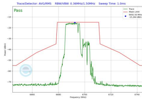
Plot 7-463 In-Band Emission Plot Antenna 5T (20MHz BW 802.11be(RU) RU106+26 Index82 (UNII Band 7) - Ch.149)
