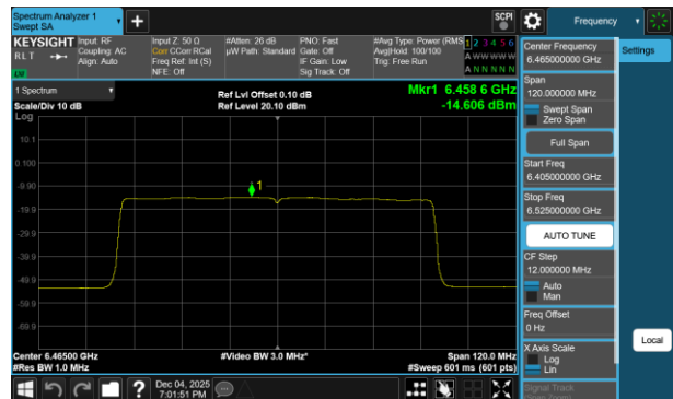
Plot 7-395 PSD SDM Diversity Antenna 1b (80MHz BW 802.11be(RU) RU996 Index67 - Ch.103)
