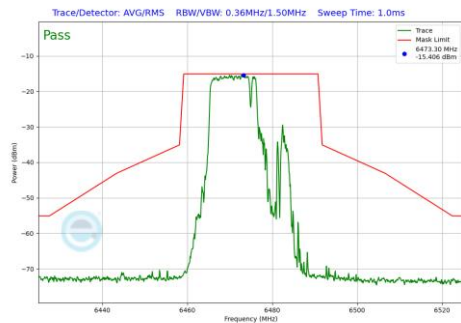
Plot 7-460 In-Band Emission Plot Antenna 5T (20MHz BW 802.11be(RU) RU106+26 Index82 (UNII Band 6) - Ch.105)
