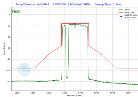
Plot 7-465 In-Band Emission Plot Antenna 5T (160MHz BW 802.11be(RU) RU996+484+242 Index97 (UNII Band 7) - Ch.143)
