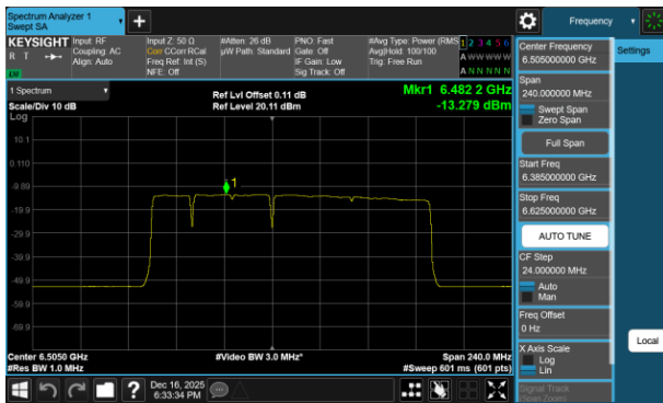
Plot 7-385 PSD SDM Diversity Antenna 5T (160MHz BW 802.11be(RU) RU996+484+242 Index96 - Ch.111)
