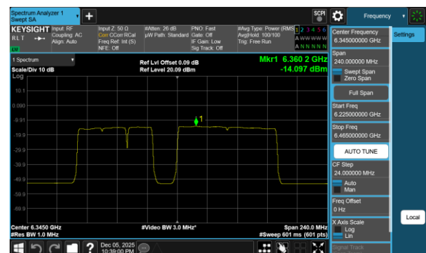
Plot 7-366 PSD SDM Diversity Antenna 1b (160MHz BW 802.11be(RU) RU996+484+242 Index99 - Ch.79)
