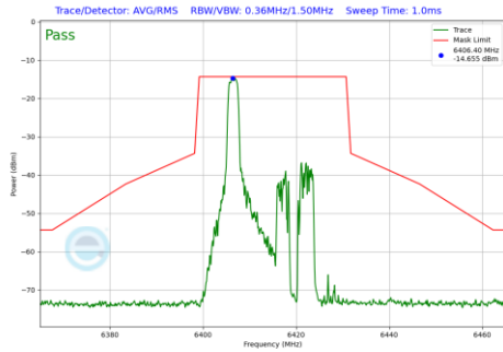
Plot 7-441 In-Band Emission Plot Antenna 5T (20MHz BW 802.11be(RU) RU26 Index0 (UNII Band 5) - Ch.93)
