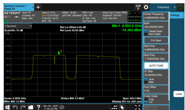
Plot 7-432 PSD SDM Diversity Antenna 1b (160MHz BW 802.11be(RU) RU996+484+242 Index99 - Ch.207)
