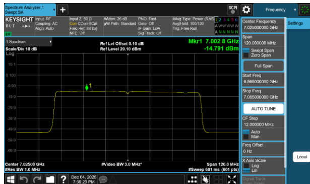
Plot 7-439 PSD SDM Diversity Antenna 1b (80MHz BW 802.11be(RU) RU996 Index67 - Ch.215)
