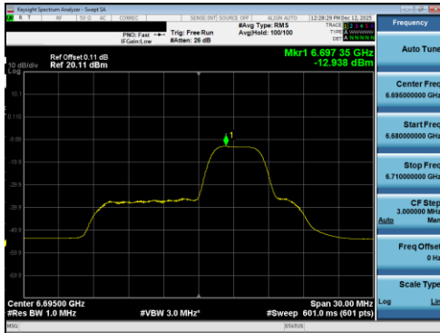
Plot 7-397 PSD SDM Diversity Antenna 5T (20MHz BW 802.11be(RU) RU52 Index39 - Ch.149)
