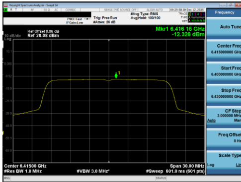
Plot 7-367 PSD SDM Diversity Antenna 5T (20MHz BW 802.11be(RU) RU242 Index61 - Ch.93)
