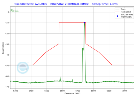
Plot 7-452 In-Band Emission Plot Antenna 5T (160MHz BW 802.11be(RU) RU26 Index36 (UNII Band 7) - Ch.143)
