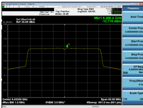
Plot 7-368 PSD SDM Diversity Antenna 5T (40MHz BW 802.11be(RU) RU484 Index65 - Ch.91)
