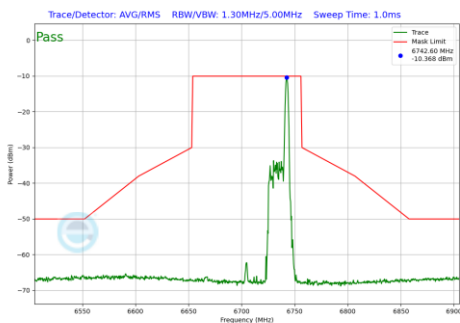
Plot 7-451 In-Band Emission Plot Antenna 5T (80MHz BW 802.11be(RU) RU26 Index36 (UNII Band 7) - Ch.151)
