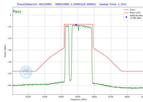
Plot 7-462 In-Band Emission Plot Antenna 5T (160MHz BW 802.11be(RU) RU996+484+242 Index97 (UNII Band 6) - Ch.111)
