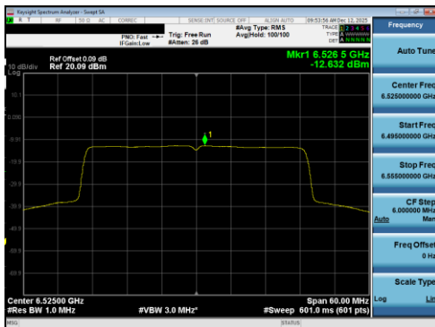
Plot 7-390 PSD SDM Diversity Antenna 5T (40MHz BW 802.11be(RU) RU484 Index65 - Ch.115)
