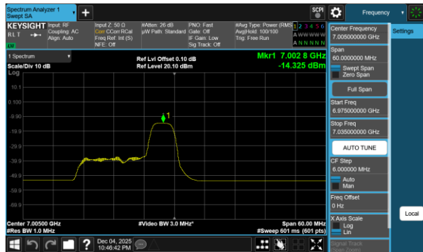
Plot 7-424 PSD SDM Diversity Antenna 1b (40MHz BW 802.11be(RU) RU52 Index40 - Ch.211)
