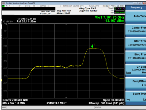
Plot 7-419 PSD SDM Diversity Antenna 5T (20MHz BW 802.11be(RU) RU52 Index40 - Ch.229)
