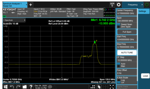
Plot 7-403 PSD SDM Diversity Antenna 1b (80MHz BW 802.11be(RU) RU52 Index52 - Ch.151)
