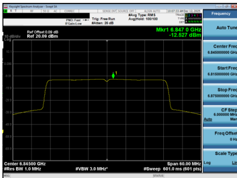
Plot 7-412 PSD SDM Diversity Antenna 5T (40MHz BW 802.11be(RU) RU484 Index65 - Ch.179)
