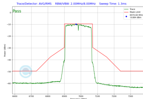
Plot 7-484 In-Band Emission Plot Antenna 5T (160MHz BW 802.11be(RU) RU996X2 Index68 (UNII Band 8) - Ch.207)
