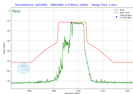
Plot 7-554 In-Band Emission Plot Antenna 1b (20MHz BW 802.11be(RU) RU106+26 Index83 (UNII Band 8) - Ch.229)
