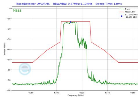
Plot 7-501 In-Band Emission Plot Antenna 3b (20MHz BW 802.11be(RU) RU106+26 Index82 (UNII Band 5) - Ch.33)
