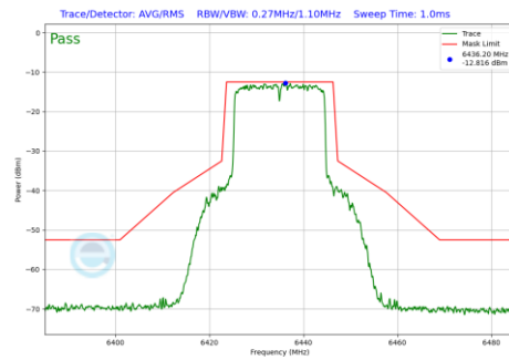
Plot 7-517 In-Band Emission Plot Antenna 3b (20MHz BW 802.11be(RU) RU242 Index61 (UNII Band 6) - Ch.97)
