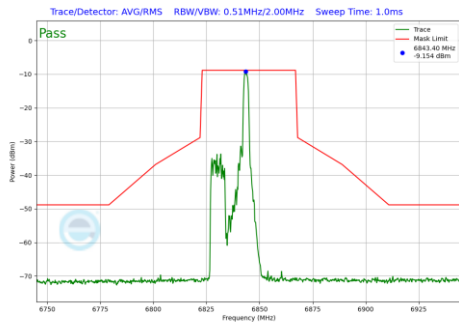
Plot 7-494 In-Band Emission Plot Antenna 3b (40MHz BW 802.11be(RU) RU26 Index8 (UNII Band 7) - Ch.179)
