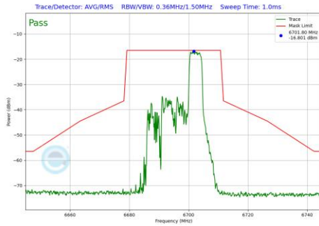
Plot 7-581 In-Band Emission Plot SDM Primary Antenna 5T (20MHz BW 802.11be(RU) RU52 Index40 (UNII Band 7) - Ch.149)
