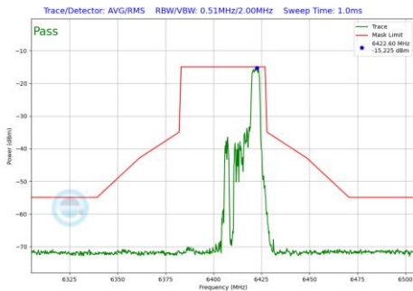
Plot 7-590 In-Band Emission Plot SDM Primary Antenna 3b (40MHz BW 802.11be(RU) RU52 Index44 (UNII Band 5) - Ch.91)
