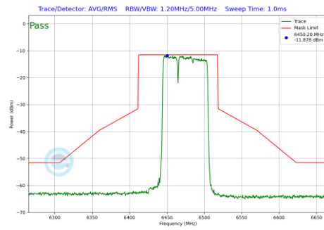
Plot 7-609 In-Band Emission Plot SDM Primary Antenna 5T (80MHz BW 802.11be(RU) RU484+242 Index90 (UNII Band 6) - Ch.103)
