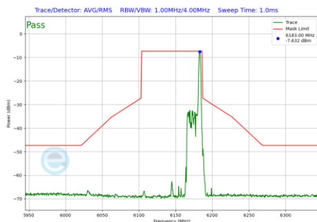
Plot 7-487 In-Band Emission Plot Antenna 3b (80MHz BW 802.11be(RU) RU26 Index36 (UNII Band 5) - Ch.39)
