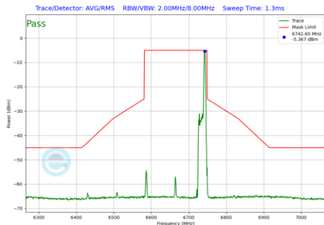
Plot 7-496 In-Band Emission Plot Antenna 3b (160MHz BW 802.11be(RU) RU26 Index36 (UNII Band 7) - Ch.143)
