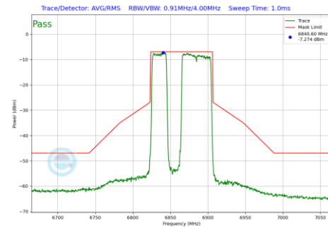
Plot 7-508 In-Band Emission Plot Antenna 3b (80MHz BW 802.11be(RU) RU484+242 Index91 (UNII Band 7) - Ch.183)
