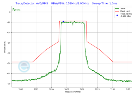
Plot 7-570 In-Band Emission Plot Antenna 1b (40MHz BW 802.11be(RU) RU484 Index65 (UNII Band 8) - Ch.227)
