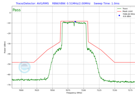
Plot 7-526 In-Band Emission Plot Antenna 3b (40MHz BW 802.11be(RU) RU484 Index65 (UNII Band 8) - Ch.227)
