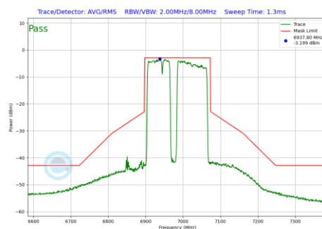
Plot 7-556 In-Band Emission Plot Antenna 1b (160MHz BW 802.11be(RU) RU996+484+242 Index99 (UNII Band 8) - Ch.207)
