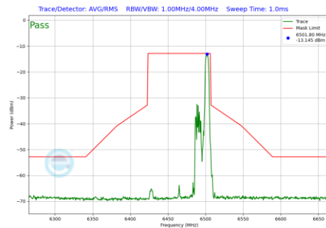
Plot 7-595 In-Band Emission Plot SDM Primary Antenna 3b (80MHz BW 802.11be(RU) RU52 Index52 (UNII Band 6) - Ch.103)
