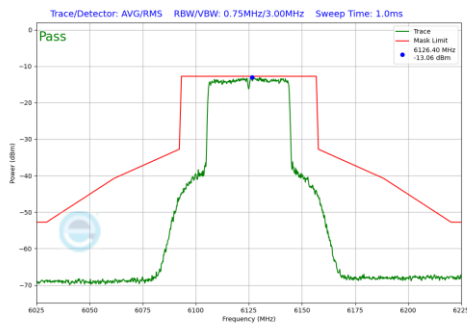
Plot 7-630 In-Band Emission Plot SDM Primary Antenna 5T (40MHz BW 802.11be(RU) RU484 Index65 (UNII Band 5) - Ch.35)
