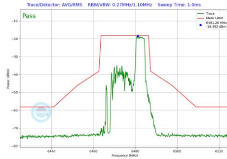
Plot 7-593 In-Band Emission Plot SDM Primary Antenna 3b (20MHz BW 802.11be(RU) RU52 Index40 (UNII Band 6) - Ch.105)
