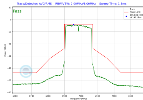
Plot 7-528 In-Band Emission Plot Antenna 3b (160MHz BW 802.11be(RU) RU996X2 Index68 (UNII Band 8) - Ch.207)
