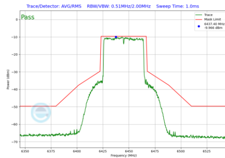
Plot 7-518 In-Band Emission Plot Antenna 3b (40MHz BW 802.11be(RU) RU484 Index65 (UNII Band 6) - Ch.99)
