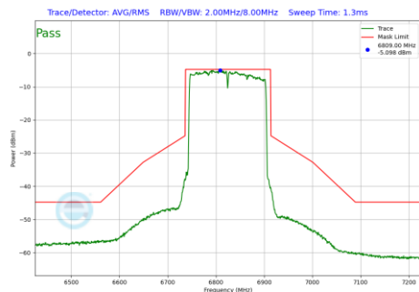
Plot 7-524 In-Band Emission Plot Antenna 3b (160MHz BW 802.11be(RU) RU996X2 Index68 (UNII Band 7) - Ch.175)
