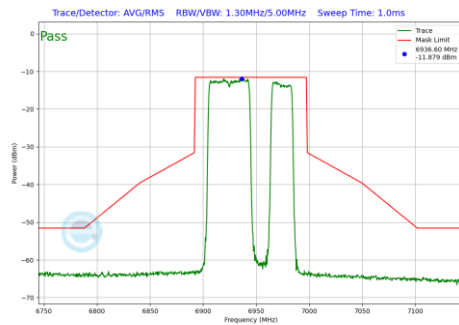
Plot 7-615 In-Band Emission Plot SDM Primary Antenna 5T (80MHz BW 802.11be(RU) RU484+242 Index92 (UNII Band 8) - Ch.199)
