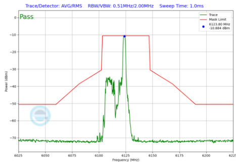
Plot 7-486 In-Band Emission Plot Antenna 3b (40MHz BW 802.11be(RU) RU26 Index8 (UNII Band 5) - Ch.35)
