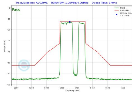
Plot 7-618 In-Band Emission Plot SDM Primary Antenna 3b (80MHz BW 802.11be(RU) RU484+242 Index92 (UNII Band 5) - Ch.87)
