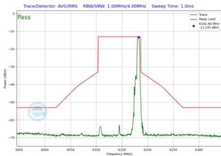
Plot 7-591 In-Band Emission Plot SDM Primary Antenna 3b (80MHz BW 802.11be(RU) RU52 Index52 (UNII Band 5) - Ch.39)
