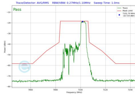
Plot 7-601 In-Band Emission Plot SDM Primary Antenna 3b (20MHz BW 802.11be(RU) RU52 Index40 (UNII Band 8) - Ch.229)
