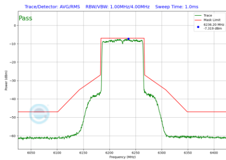
Plot 7-515 In-Band Emission Plot Antenna 3b (80MHz BW 802.11be(RU) RU996 Index67 (UNII Band 5) - Ch.55)
