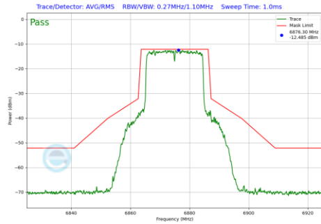
Plot 7-521 In-Band Emission Plot Antenna 3b (20MHz BW 802.11be(RU) RU242 Index61 (UNII Band 7) - Ch.185)
