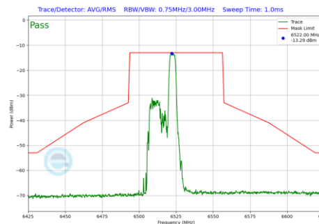
Plot 7-578 In-Band Emission Plot SDM Primary Antenna 5T (40MHz BW 802.11be(RU) RU52 Index40 (UNII Band 6) - Ch.115)
