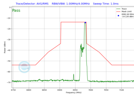
Plot 7-603 In-Band Emission Plot SDM Primary Antenna 3b (80MHz BW 802.11be(RU) RU52 Index52 (UNII Band 8) - Ch.199)
