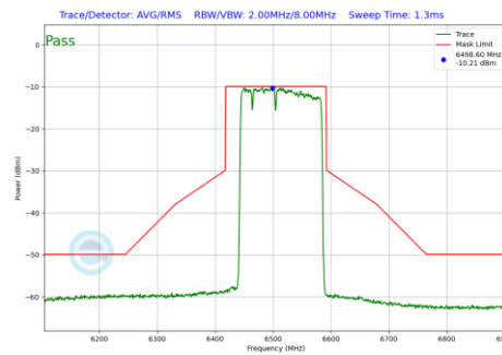
Plot 7-610 In-Band Emission Plot SDM Primary Antenna 5T (160MHz BW 802.11be(RU) RU996+484+242 Index96 (UNII Band 6) - Ch.111)
