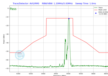
Plot 7-579 In-Band Emission Plot SDM Primary Antenna 5T (80MHz BW 802.11be(RU) RU52 Index52 (UNII Band 6) - Ch.103)
