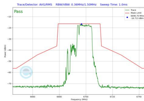
Plot 7-611 In-Band Emission Plot SDM Primary Antenna 5T (20MHz BW 802.11be(RU) RU106+26 Index83 (UNII Band 7) - Ch.149)
