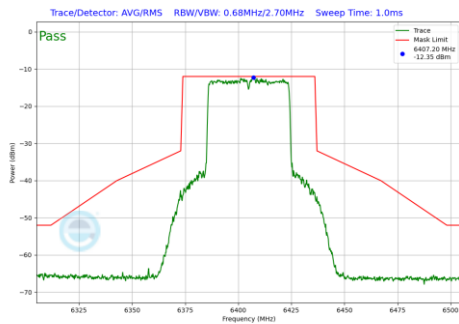
Plot 7-470 In-Band Emission Plot Antenna 5T (40MHz BW 802.11be(RU) RU484 Index65 (UNII Band 5) - Ch.91)
