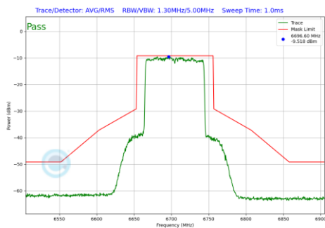
Plot 7-479 In-Band Emission Plot Antenna 5T (80MHz BW 802.11be(RU) RU996 Index67 (UNII Band 7) - Ch.151)
