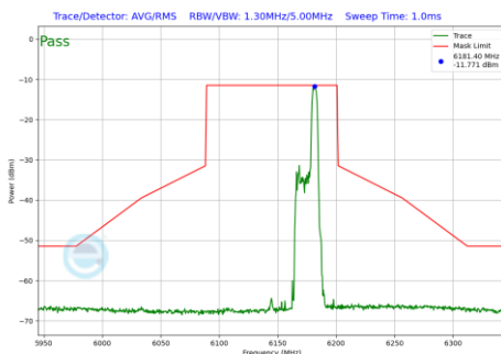
Plot 7-575 In-Band Emission Plot SDM Primary Antenna 5T (80MHz BW 802.11be(RU) RU52 Index52 (UNII Band 5) - Ch.39)
