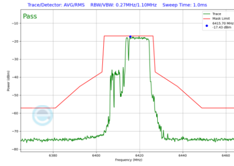
Plot 7-617 In-Band Emission Plot SDM Primary Antenna 3b (20MHz BW 802.11be(RU) RU106+26 Index83 (UNII Band 5) - Ch.93)
