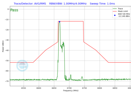
Plot 7-599 In-Band Emission Plot SDM Primary Antenna 3b (80MHz BW 802.11be(RU) RU52 Index37 (UNII Band 7) - Ch.151)
