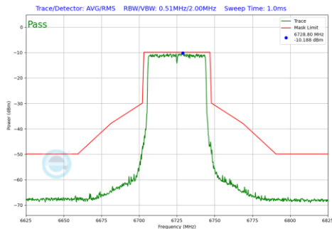
Plot 7-566 In-Band Emission Plot Antenna 1b (40MHz BW 802.11be(RU) RU484 Index65 (UNII Band 7) - Ch.155)
