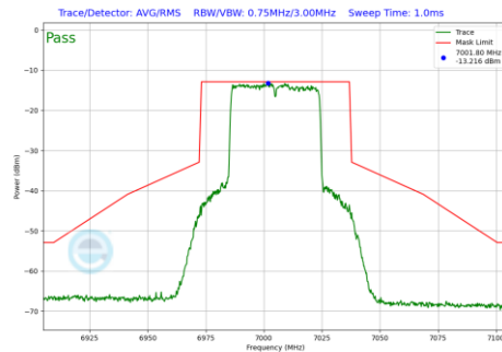
Plot 7-482 In-Band Emission Plot Antenna 5T (40MHz BW 802.11be(RU) RU484 Index65 (UNII Band 8) - Ch.211)
