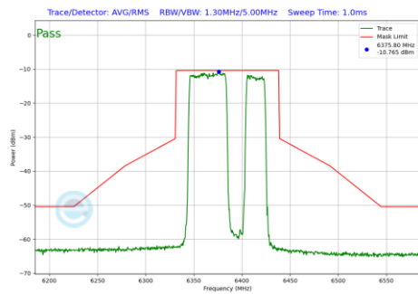
Plot 7-606 In-Band Emission Plot SDM Primary Antenna 5T (80MHz BW 802.11be(RU) RU484+242 Index92 (UNII Band 5) - Ch.87)
