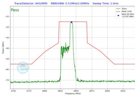
Plot 7-598 In-Band Emission Plot SDM Primary Antenna 3b (40MHz BW 802.11be(RU) RU52 Index40 (UNII Band 7) - Ch.179)
