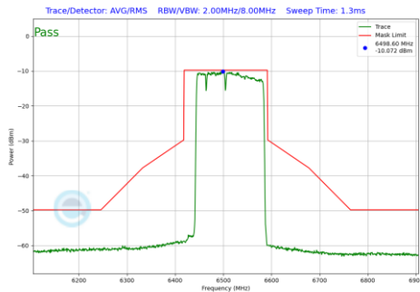
Plot 7-622 In-Band Emission Plot SDM Primary Antenna 3b (160MHz BW 802.11be(RU) RU996+484+242 Index96 (UNII Band 6) - Ch.111)
