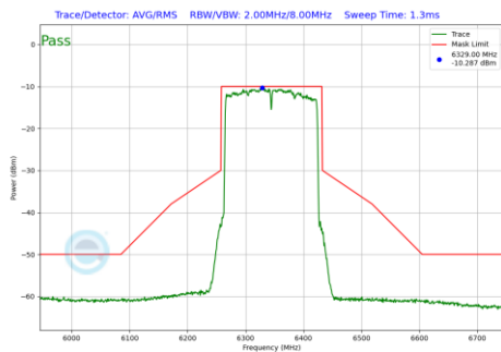
Plot 7-632 In-Band Emission Plot SDM Primary Antenna 5T (160MHz BW 802.11be(RU) RU996X2 Index68 (UNII Band 5) - Ch.79)
