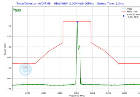
Plot 7-536 In-Band Emission Plot Antenna 1b (160MHz BW 802.11be(RU) RU26 Index0 (UNII Band 6) - Ch.111)
