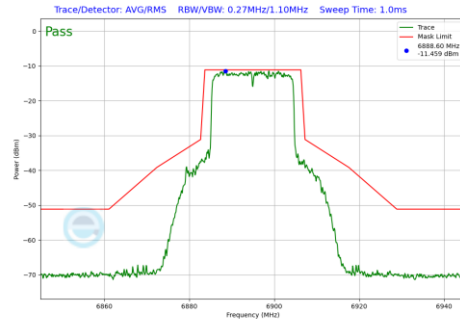
Plot 7-525 In-Band Emission Plot Antenna 3b (20MHz BW 802.11be(RU) RU242 Index61 (UNII Band 8) - Ch.189)
