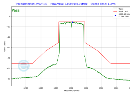
Plot 7-564 In-Band Emission Plot Antenna 1b (160MHz BW 802.11be(RU) RU996X2 Index68 (UNII Band 6) - Ch.111)
