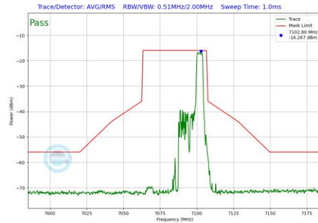
Plot 7-602 In-Band Emission Plot SDM Primary Antenna 3b (40MHz BW 802.11be(RU) RU52 Index44 (UNII Band 8) - Ch.227)
