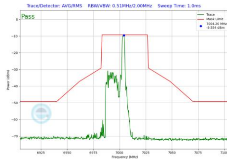
Plot 7-498 In-Band Emission Plot Antenna 3b (40MHz BW 802.11be(RU) RU26 Index8 (UNII Band 8) - Ch.211)
