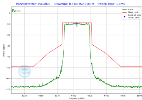
Plot 7-558 In-Band Emission Plot Antenna 1b (40MHz BW 802.11be(RU) RU484 Index65 (UNII Band 5) - Ch.91)
