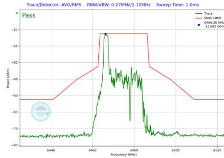
Plot 7-489 In-Band Emission Plot Antenna 3b (20MHz BW 802.11be(RU) RU26 Index0 (UNII Band 6) - Ch.105)
