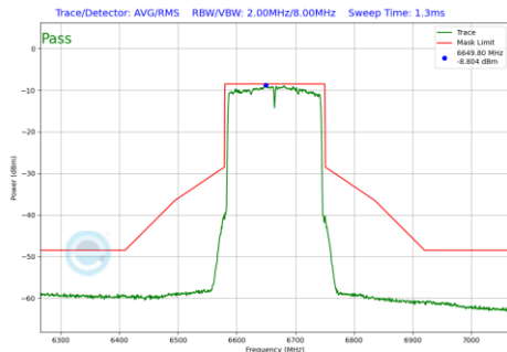
Plot 7-480 In-Band Emission Plot Antenna 5T (160MHz BW 802.11be(RU) RU996X2 Index68 (UNII Band 7) - Ch.143)
