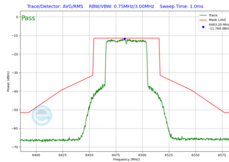
Plot 7-474 In-Band Emission Plot Antenna 5T (40MHz BW 802.11be(RU) RU484 Index65 (UNII Band 6) - Ch.107)
