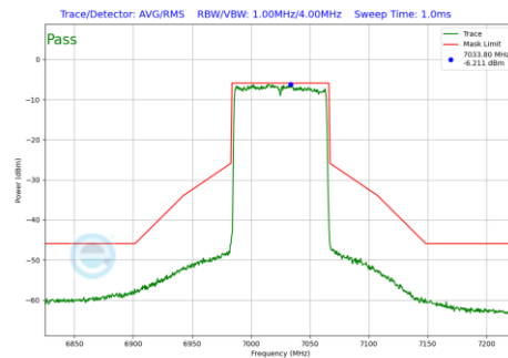
Plot 7-571 In-Band Emission Plot Antenna 1b (80MHz BW 802.11be(RU) RU996 Index67 (UNII Band 8) - Ch.215)
