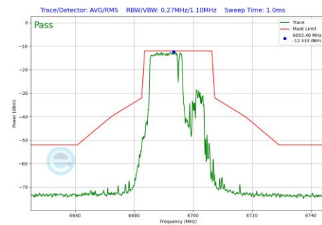
Plot 7-507 In-Band Emission Plot Antenna 3b (20MHz BW 802.11be(RU) RU106+26 Index82 (UNII Band 7) - Ch.149)
