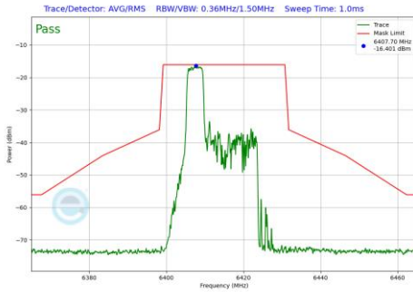
Plot 7-573 In-Band Emission Plot SDM Primary Antenna 5T (20MHz BW 802.11be(RU) RU52 Index37 (UNII Band 5) - Ch.93)
