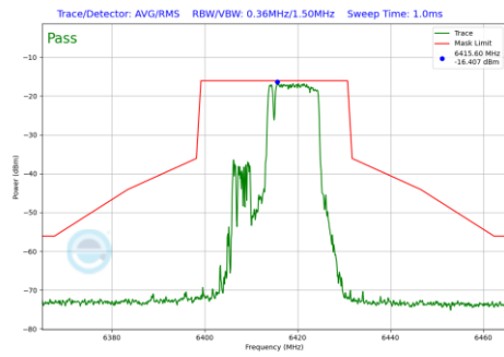
Plot 7-605 In-Band Emission Plot SDM Primary Antenna 5T (20MHz BW 802.11be(RU) RU106+26 Index83 (UNII Band 5) - Ch.93)
