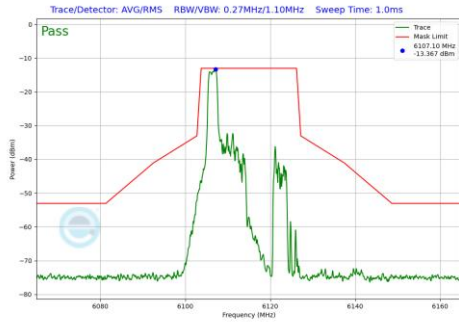
Plot 7-485 In-Band Emission Plot Antenna 3b (20MHz BW 802.11be(RU) RU26 Index0 (UNII Band 5) - Ch.33)
