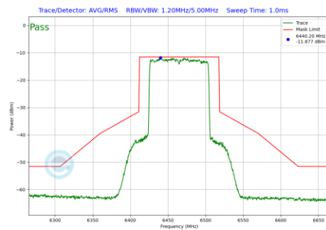
Plot 7-635 In-Band Emission Plot SDM Primary Antenna 5T (80MHz BW 802.11be(RU) RU996 Index67 (UNII Band 6) - Ch.103)
