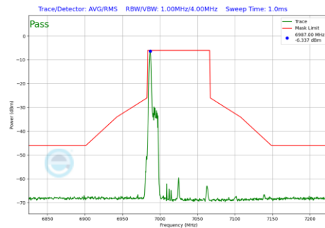
Plot 7-499 In-Band Emission Plot Antenna 3b (80MHz BW 802.11be(RU) RU26 Index0 (UNII Band 8) - Ch.215)
