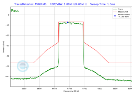
Plot 7-567 In-Band Emission Plot Antenna 1b (80MHz BW 802.11be(RU) RU996 Index67 (UNII Band 7) - Ch.151)
