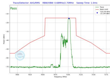
Plot 7-586 In-Band Emission Plot SDM Primary Antenna 5T (40MHz BW 802.11be(RU) RU52 Index44 (UNII Band 8) - Ch.227)
