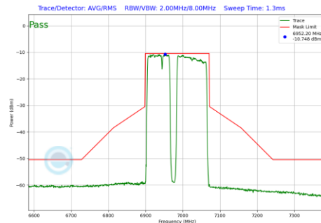
Plot 7-628 In-Band Emission Plot SDM Primary Antenna 3b (160MHz BW 802.11be(RU) RU996+484+242 Index99 (UNII Band 8) - Ch.207)
