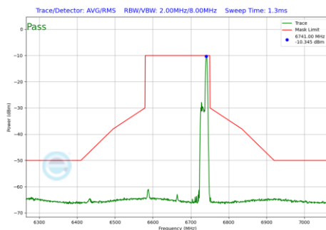
Plot 7-584 In-Band Emission Plot SDM Primary Antenna 5T (160MHz BW 802.11be(RU) RU52 Index52 (UNII Band 7) - Ch.143)
