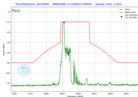
Plot 7-538 In-Band Emission Plot Antenna 1b (40MHz BW 802.11be(RU) RU26 Index0 (UNII Band 7) - Ch.179)
