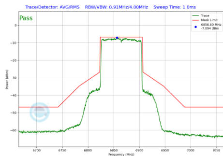
Plot 7-523 In-Band Emission Plot Antenna 3b (80MHz BW 802.11be(RU) RU996 Index67 (UNII Band 7) - Ch.183)
