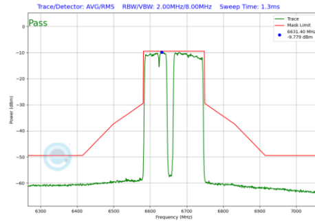
Plot 7-625 In-Band Emission Plot SDM Primary Antenna 3b (160MHz BW 802.11be(RU) RU996+484+242 Index99 (UNII Band 7) - Ch.143)
