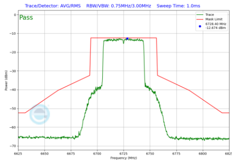
Plot 7-478 In-Band Emission Plot Antenna 5T (40MHz BW 802.11be(RU) RU484 Index65 (UNII Band 7) - Ch.155)
