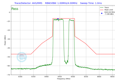
Plot 7-505 In-Band Emission Plot Antenna 3b (80MHz BW 802.11be(RU) RU484+242 Index92 (UNII Band 6) - Ch.103)
