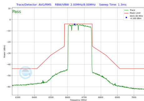
Plot 7-509 In-Band Emission Plot Antenna 3b (160MHz BW 802.11be(RU) RU996+484+242 Index96 (UNII Band 7) - Ch.143)
