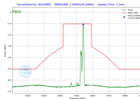
Plot 7-580 In-Band Emission Plot SDM Primary Antenna 5T (160MHz BW 802.11be(RU) RU52 Index44 (UNII Band 6) - Ch.111)
