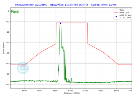
Plot 7-583 In-Band Emission Plot SDM Primary Antenna 5T (80MHz BW 802.11be(RU) RU52 Index37 (UNII Band 7) - Ch.151)
