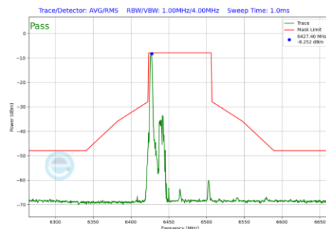
Plot 7-491 In-Band Emission Plot Antenna 3b (80MHz BW 802.11be(RU) RU26 Index0 (UNII Band 6) - Ch.103)
