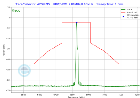
Plot 7-540 In-Band Emission Plot Antenna 1b (160MHz BW 802.11be(RU) RU26 Index0 (UNII Band 7) - Ch.175)
