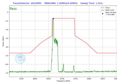
Plot 7-495 In-Band Emission Plot Antenna 3b (80MHz BW 802.11be(RU) RU26 Index0 (UNII Band 7) - Ch.151)
