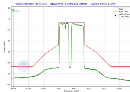
Plot 7-512 In-Band Emission Plot Antenna 3b (160MHz BW 802.11be(RU) RU996+484+242 Index99 (UNII Band 8) - Ch.207)
