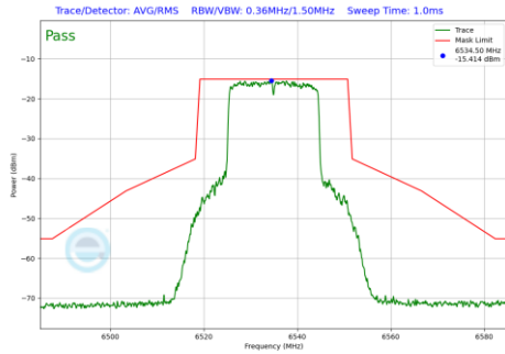
Plot 7-477 In-Band Emission Plot Antenna 5T (20MHz BW 802.11be(RU) RU242 Index61 (UNII Band 7) - Ch.117)
