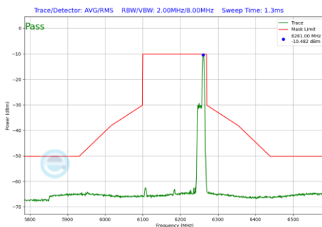
Plot 7-576 In-Band Emission Plot SDM Primary Antenna 5T (160MHz BW 802.11be(RU) RU52 Index52 (UNII Band 5) - Ch.47)
