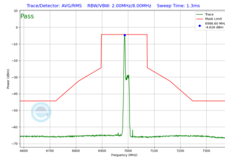
Plot 7-544 In-Band Emission Plot Antenna 1b (160MHz BW 802.11be(RU) RU26 Index0 (UNII Band 8) - Ch.207)
