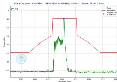
Plot 7-542 In-Band Emission Plot Antenna 1b (40MHz BW 802.11be(RU) RU26 Index8 (UNII Band 8) - Ch.211)
