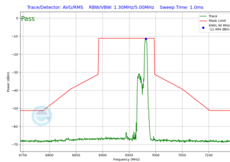
Plot 7-587 In-Band Emission Plot SDM Primary Antenna 5T (80MHz BW 802.11be(RU) RU52 Index52 (UNII Band 8) - Ch.199)
