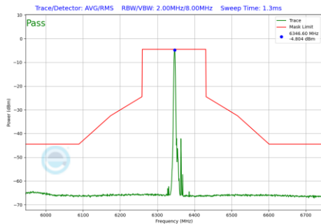
Plot 7-532 In-Band Emission Plot Antenna 1b (160MHz BW 802.11be(RU) RU26 Index0 (UNII Band 5) - Ch.79)
