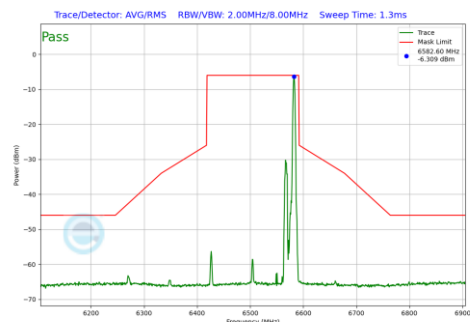
Plot 7-492 In-Band Emission Plot Antenna 3b (160MHz BW 802.11be(RU) RU26 Index36 (UNII Band 6) - Ch.111)
