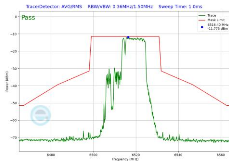
Plot 7-548 In-Band Emission Plot Antenna 1b (20MHz BW 802.11be(RU) RU106+26 Index83 (UNII Band 6) - Ch.113)
