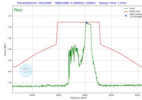
Plot 7-577 In-Band Emission Plot SDM Primary Antenna 5T (20MHz BW 802.11be(RU) RU52 Index40 (UNII Band 6) - Ch.105)
