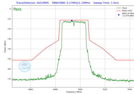
Plot 7-569 In-Band Emission Plot Antenna 1b (20MHz BW 802.11be(RU) RU242 Index61 (UNII Band 8) - Ch.209)
