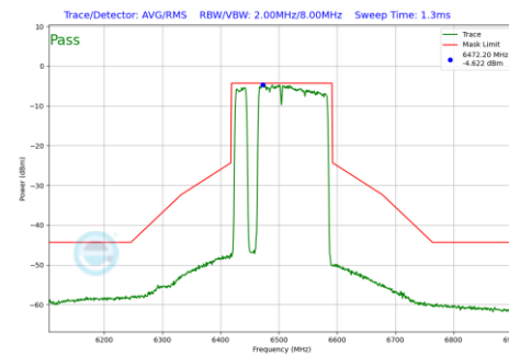
Plot 7-506 In-Band Emission Plot Antenna 3b (160MHz BW 802.11be(RU) RU996+484+242 Index97 (UNII Band 6) - Ch.111)
