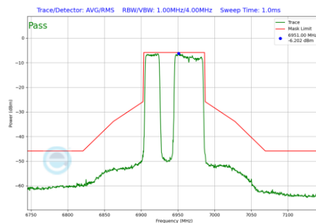
Plot 7-555 In-Band Emission Plot Antenna 1b (80MHz BW 802.11be(RU) RU484+242 Index91 (UNII Band 8) - Ch.199)
