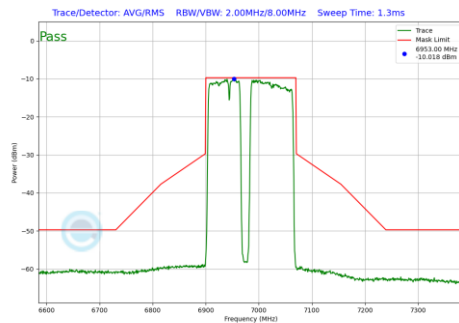
Plot 7-616 In-Band Emission Plot SDM Primary Antenna 5T (160MHz BW 802.11be(RU) RU996+484+242 Index99 (UNII Band 8) - Ch.207)
