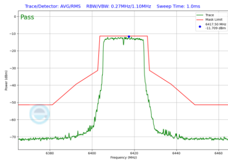
Plot 7-557 In-Band Emission Plot Antenna 1b (20MHz BW 802.11be(RU) RU242 Index61 (UNII Band 5) - Ch.93)
