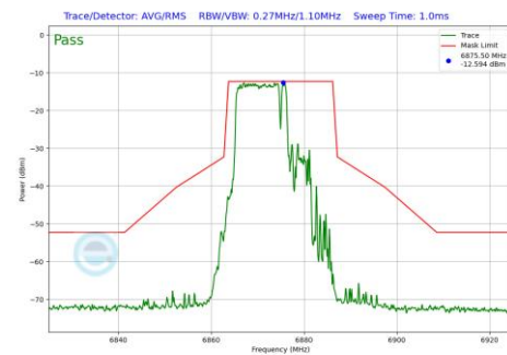
Plot 7-551 In-Band Emission Plot Antenna 1b (20MHz BW 802.11be(RU) RU106+26 Index82 (UNII Band 7) - Ch.185)
