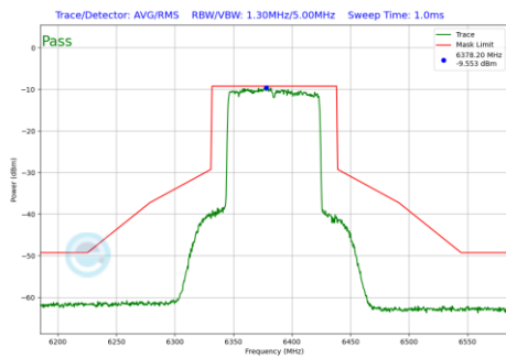
Plot 7-471 In-Band Emission Plot Antenna 5T (80MHz BW 802.11be(RU) RU996 Index67 (UNII Band 5) - Ch.87)
