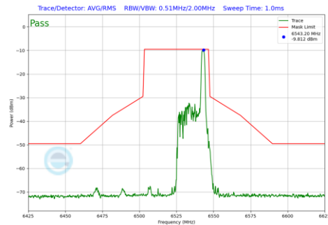
Plot 7-490 In-Band Emission Plot Antenna 3b (40MHz BW 802.11be(RU) RU26 Index17 (UNII Band 6) - Ch.115)
