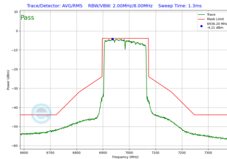
Plot 7-572 In-Band Emission Plot Antenna 1b (160MHz BW 802.11be(RU) RU996X2 Index68 (UNII Band 8) - Ch.207)
