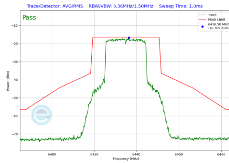
Plot 7-633 In-Band Emission Plot SDM Primary Antenna 5T (20MHz BW 802.11be(RU) RU242 Index61 (UNII Band 6) - Ch.97)
