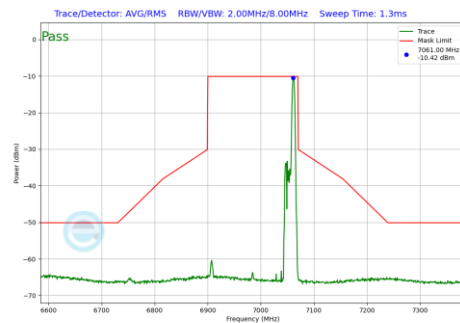
Plot 7-588 In-Band Emission Plot SDM Primary Antenna 5T (160MHz BW 802.11be(RU) RU52 Index52 (UNII Band 8) - Ch.207)
