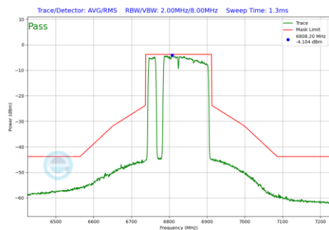
Plot 7-553 In-Band Emission Plot Antenna 1b (160MHz BW 802.11be(RU) RU996+484+242 Index97 (UNII Band 7) - Ch.175)
