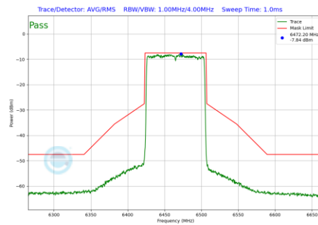
Plot 7-563 In-Band Emission Plot Antenna 1b (80MHz BW 802.11be(RU) RU996 Index67 (UNII Band 6) - Ch.103)
