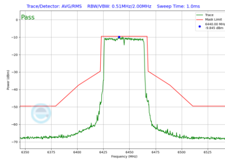
Plot 7-562 In-Band Emission Plot Antenna 1b (40MHz BW 802.11be(RU) RU484 Index65 (UNII Band 6) - Ch.99)
