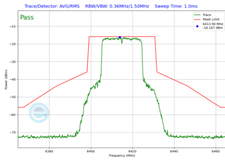
Plot 7-629 In-Band Emission Plot SDM Primary Antenna 5T (20MHz BW 802.11be(RU) RU242 Index61 (UNII Band 5) - Ch.93)
