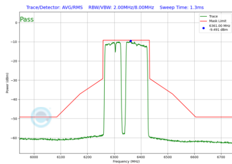
Plot 7-607 In-Band Emission Plot SDM Primary Antenna 5T (160MHz BW 802.11be(RU) RU996+484+242 Index99 (UNII Band 5) - Ch.79)
