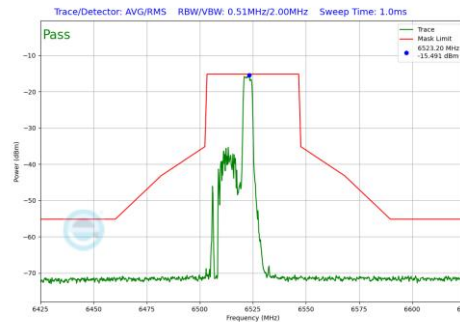
Plot 7-594 In-Band Emission Plot SDM Primary Antenna 3b (40MHz BW 802.11be(RU) RU52 Index40 (UNII Band 6) - Ch.115)
