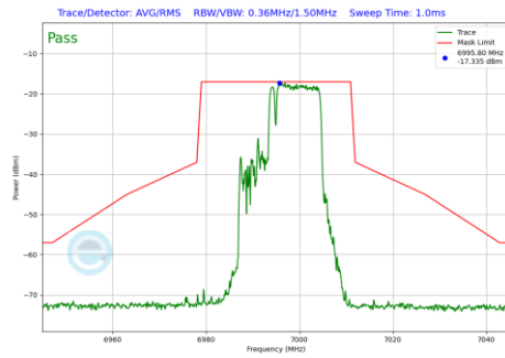
Plot 7-614 In-Band Emission Plot SDM Primary Antenna 5T (20MHz BW 802.11be(RU) RU106+26 Index83 (UNII Band 8) - Ch.209)
