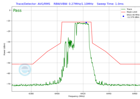
Plot 7-545 In-Band Emission Plot Antenna 1b (20MHz BW 802.11be(RU) RU106+26 Index83 (UNII Band 5) - Ch.93)
