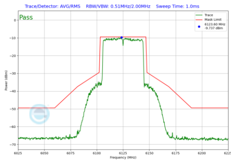
Plot 7-514 In-Band Emission Plot Antenna 3b (40MHz BW 802.11be(RU) RU484 Index65 (UNII Band 5) - Ch.35)
