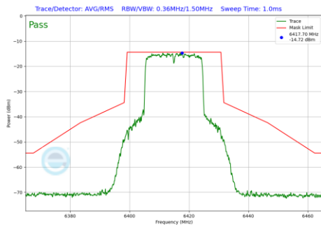
Plot 7-469 In-Band Emission Plot Antenna 5T (20MHz BW 802.11be(RU) RU242 Index61 (UNII Band 5) - Ch.93)
