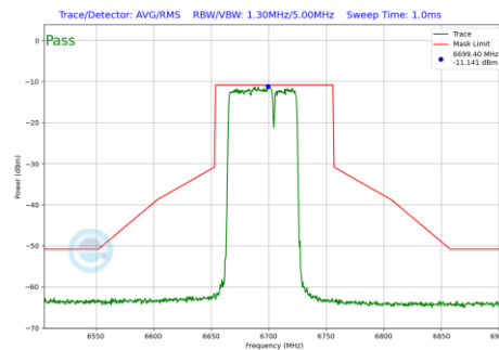
Plot 7-612 In-Band Emission Plot SDM Primary Antenna 5T (80MHz BW 802.11be(RU) RU484+242 Index93 (UNII Band 7) - Ch.151)
