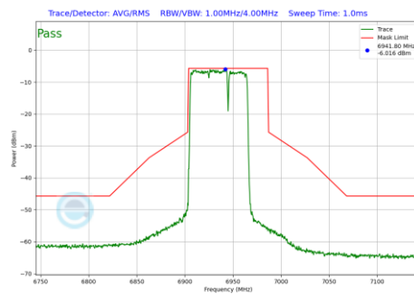
Plot 7-511 In-Band Emission Plot Antenna 3b (80MHz BW 802.11be(RU) RU484+242 Index93 (UNII Band 8) - Ch.199)
