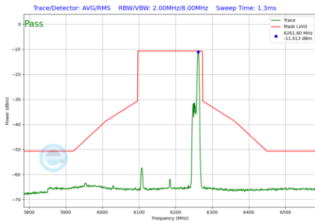
Plot 7-592 In-Band Emission Plot SDM Primary Antenna 3b (160MHz BW 802.11be(RU) RU52 Index52 (UNII Band 5) - Ch.47)
