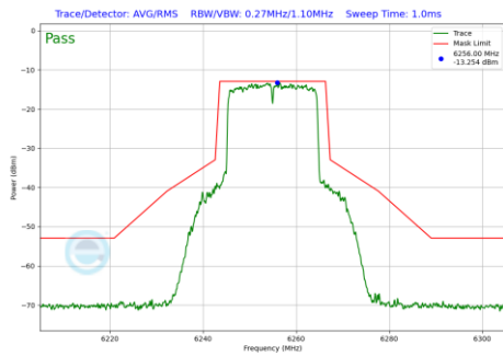
Plot 7-513 In-Band Emission Plot Antenna 3b (20MHz BW 802.11be(RU) RU242 Index61 (UNII Band 5) - Ch.61)
