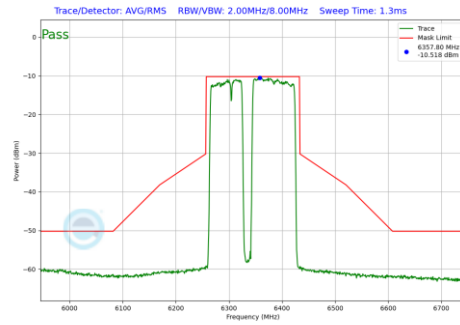
Plot 7-619 In-Band Emission Plot SDM Primary Antenna 3b (160MHz BW 802.11be(RU) RU996+484+242 Index99 (UNII Band 5) - Ch.79)
