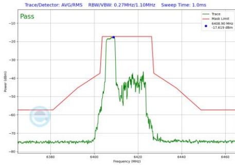
Plot 7-589 In-Band Emission Plot SDM Primary Antenna 3b (20MHz BW 802.11be(RU) RU52 Index37 (UNII Band 5) - Ch.93)
