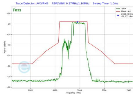
Plot 7-626 In-Band Emission Plot SDM Primary Antenna 3b (20MHz BW 802.11be(RU) RU106+26 Index83 (UNII Band 8) - Ch.209)
