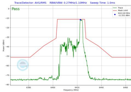
Plot 7-529 In-Band Emission Plot Antenna 1b (20MHz BW 802.11be(RU) RU26 Index8 (UNII Band 5) - Ch.93)
