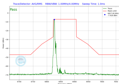
Plot 7-539 In-Band Emission Plot Antenna 1b (80MHz BW 802.11be(RU) RU26 Index0 (UNII Band 7) - Ch.183)
