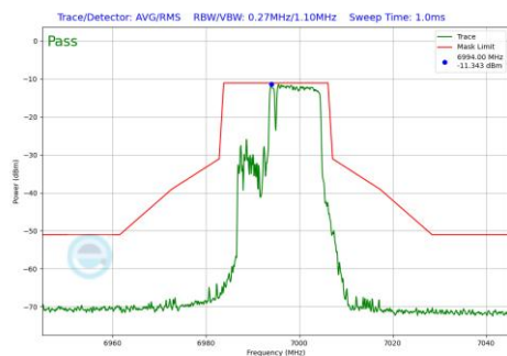
Plot 7-510 In-Band Emission Plot Antenna 3b (20MHz BW 802.11be(RU) RU106+26 Index83 (UNII Band 8) - Ch.209)
