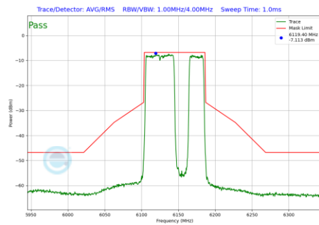
Plot 7-502 In-Band Emission Plot Antenna 3b (80MHz BW 802.11be(RU) RU484+242 Index92 (UNII Band 5) - Ch.39)
