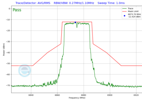
Plot 7-565 In-Band Emission Plot Antenna 1b (20MHz BW 802.11be(RU) RU242 Index61 (UNII Band 7) - Ch.185)
