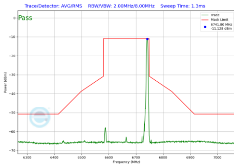
Plot 7-600 In-Band Emission Plot SDM Primary Antenna 3b (160MHz BW 802.11be(RU) RU52 Index52 (UNII Band 7) - Ch.143)
