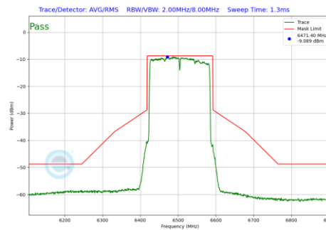
Plot 7-476 In-Band Emission Plot Antenna 5T (160MHz BW 802.11be(RU) RU996X2 Index68 (UNII Band 6) - Ch.111)
