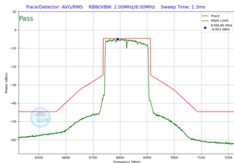
Plot 7-568 In-Band Emission Plot Antenna 1b (160MHz BW 802.11be(RU) RU996X2 Index68 (UNII Band 7) - Ch.175)
