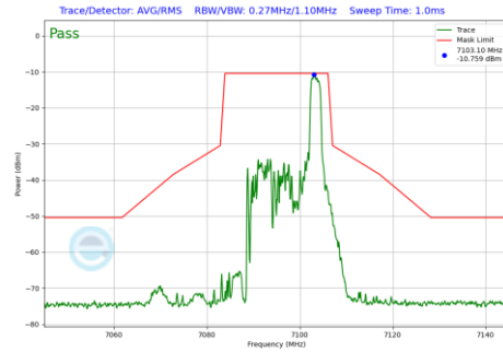
Plot 7-497 In-Band Emission Plot Antenna 3b (20MHz BW 802.11be(RU) RU26 Index8 (UNII Band 8) - Ch.229)
