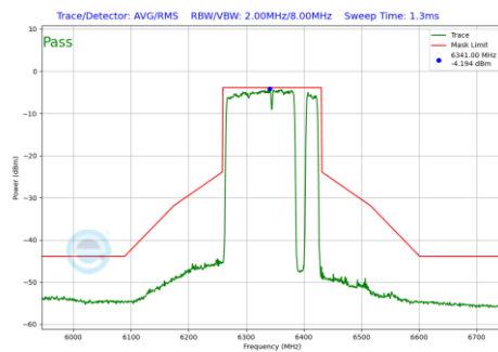
Plot 7-547 In-Band Emission Plot Antenna 1b (160MHz BW 802.11be(RU) RU996+484+242 Index98 (UNII Band 5) - Ch.79)
