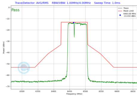
Plot 7-621 In-Band Emission Plot SDM Primary Antenna 3b (80MHz BW 802.11be(RU) RU484+242 Index90 (UNII Band 6) - Ch.103)
