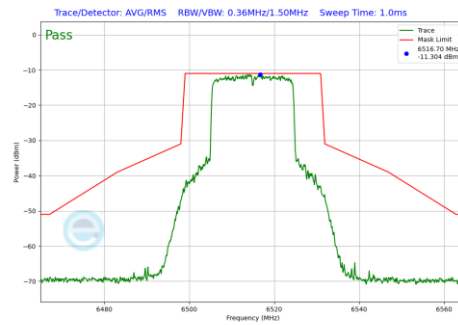
Plot 7-561 In-Band Emission Plot Antenna 1b (20MHz BW 802.11be(RU) RU242 Index61 (UNII Band 6) - Ch.113)
