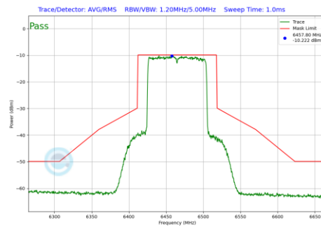
Plot 7-475 In-Band Emission Plot Antenna 5T (80MHz BW 802.11be(RU) RU996 Index67 (UNII Band 6) - Ch.103)
