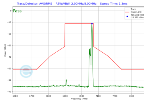
Plot 7-604 In-Band Emission Plot SDM Primary Antenna 3b (160MHz BW 802.11be(RU) RU52 Index52 (UNII Band 8) - Ch.207)
