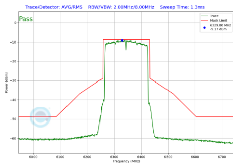
Plot 7-472 In-Band Emission Plot Antenna 5T (160MHz BW 802.11be(RU) RU996X2 Index68 (UNII Band 5) - Ch.79)
