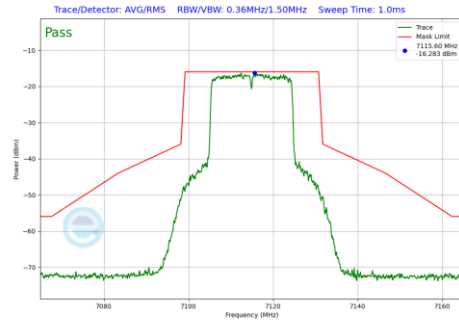
Plot 7-481 In-Band Emission Plot Antenna 5T (20MHz BW 802.11be(RU) RU242 Index61 (UNII Band 8) - Ch.233)
