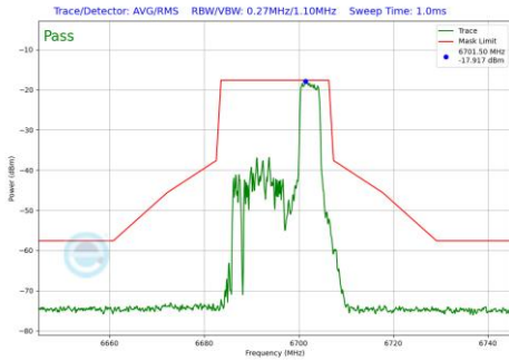
Plot 7-597 In-Band Emission Plot SDM Primary Antenna 3b (20MHz BW 802.11be(RU) RU52 Index40 (UNII Band 7) - Ch.149)
