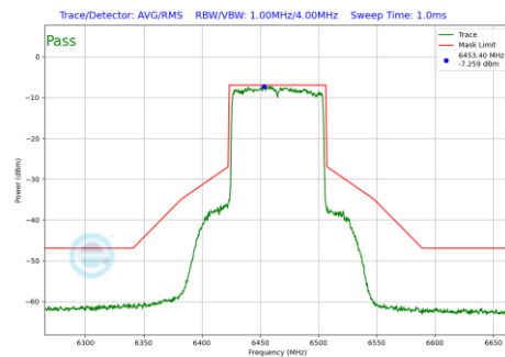
Plot 7-519 In-Band Emission Plot Antenna 3b (80MHz BW 802.11be(RU) RU996 Index67 (UNII Band 6) - Ch.103)
