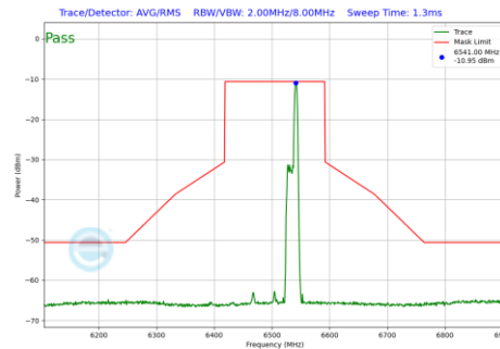
Plot 7-596 In-Band Emission Plot SDM Primary Antenna 3b (160MHz BW 802.11be(RU) RU52 Index44 (UNII Band 6) - Ch.111)
