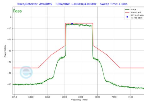
Plot 7-527 In-Band Emission Plot Antenna 3b (80MHz BW 802.11be(RU) RU996 Index67 (UNII Band 8) - Ch.199)
