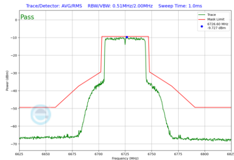
Plot 7-522 In-Band Emission Plot Antenna 3b (40MHz BW 802.11be(RU) RU484 Index65 (UNII Band 7) - Ch.155)
