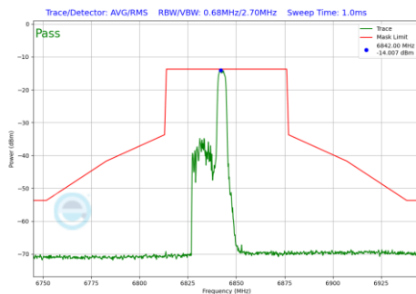
Plot 7-582 In-Band Emission Plot SDM Primary Antenna 5T (40MHz BW 802.11be(RU) RU52 Index40 (UNII Band 7) - Ch.179)
