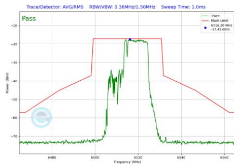
Plot 7-608 In-Band Emission Plot SDM Primary Antenna 5T (20MHz BW 802.11be(RU) RU106+26 Index83 (UNII Band 6) - Ch.113)
