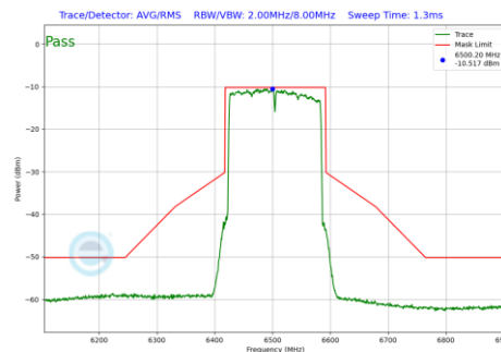
Plot 7-636 In-Band Emission Plot SDM Primary Antenna 5T (160MHz BW 802.11be(RU) RU996X2 Index68 (UNII Band 6) - Ch.111)
