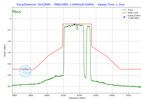
Plot 7-503 In-Band Emission Plot Antenna 3b (160MHz BW 802.11be(RU) RU996+484+242 Index98 (UNII Band 5) - Ch.47)
