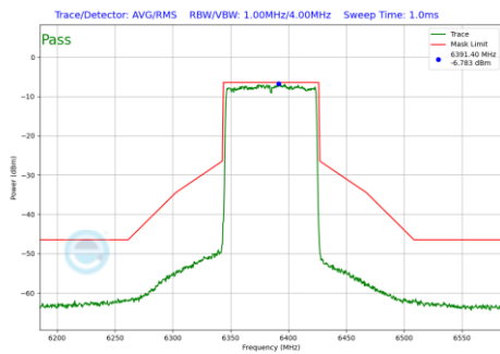
Plot 7-559 In-Band Emission Plot Antenna 1b (80MHz BW 802.11be(RU) RU996 Index67 (UNII Band 5) - Ch.87)
