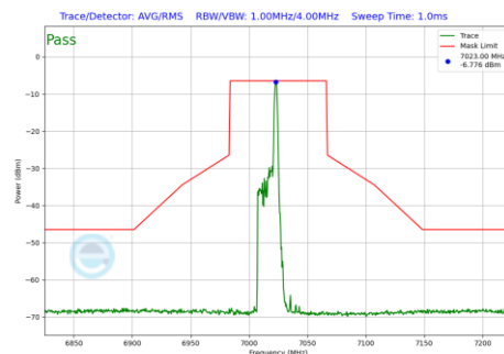
Plot 7-543 In-Band Emission Plot Antenna 1b (80MHz BW 802.11be(RU) RU26 Index17 (UNII Band 8) - Ch.215)
