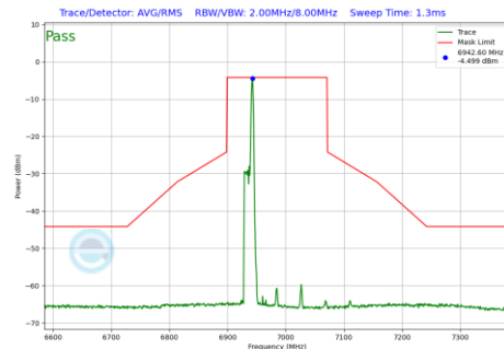
Plot 7-500 In-Band Emission Plot Antenna 3b (160MHz BW 802.11be(RU) RU26 Index17 (UNII Band 8) - Ch.207)
