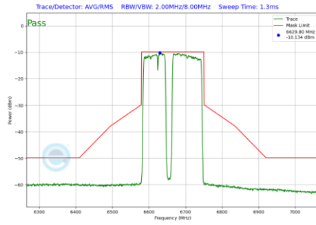
Plot 7-613 In-Band Emission Plot SDM Primary Antenna 5T (160MHz BW 802.11be(RU) RU996+484+242 Index99 (UNII Band 7) - Ch.143)
