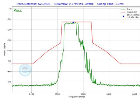
Plot 7-504 In-Band Emission Plot Antenna 3b (20MHz BW 802.11be(RU) RU106+26 Index82 (UNII Band 6) - Ch.113)
