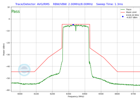
Plot 7-560 In-Band Emission Plot Antenna 1b (160MHz BW 802.11be(RU) RU996X2 Index68 (UNII Band 5) - Ch.79)
