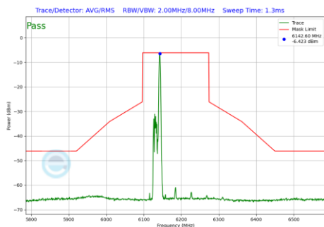
Plot 7-488 In-Band Emission Plot Antenna 3b (160MHz BW 802.11be(RU) RU26 Index17 (UNII Band 5) - Ch.47)
