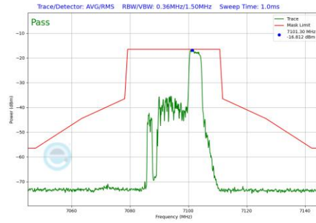
Plot 7-585 In-Band Emission Plot SDM Primary Antenna 5T (20MHz BW 802.11be(RU) RU52 Index40 (UNII Band 8) - Ch.229)
