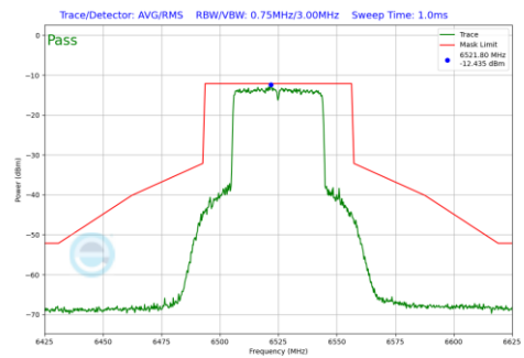
Plot 7-634 In-Band Emission Plot SDM Primary Antenna 5T (40MHz BW 802.11be(RU) RU484 Index65 (UNII Band 6) - Ch.115)
