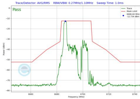
Plot 7-537 In-Band Emission Plot Antenna 1b (20MHz BW 802.11be(RU) RU26 Index0 (UNII Band 7) - Ch.149)
