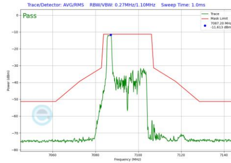
Plot 7-541 In-Band Emission Plot Antenna 1b (20MHz BW 802.11be(RU) RU26 Index0 (UNII Band 8) - Ch.229)
