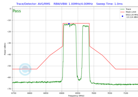
Plot 7-627 In-Band Emission Plot SDM Primary Antenna 3b (80MHz BW 802.11be(RU) RU484+242 Index92 (UNII Band 8) - Ch.199)
