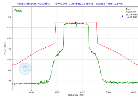
Plot 7-473 In-Band Emission Plot Antenna 5T (20MHz BW 802.11be(RU) RU242 Index61 (UNII Band 6) - Ch.113)
