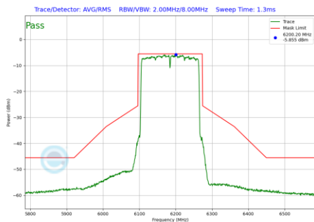
Plot 7-516 In-Band Emission Plot Antenna 3b (160MHz BW 802.11be(RU) RU996X2 Index68 (UNII Band 5) - Ch.47)
