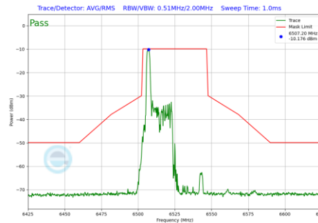
Plot 7-534 In-Band Emission Plot Antenna 1b (40MHz BW 802.11be(RU) RU26 Index0 (UNII Band 6) - Ch.115)
