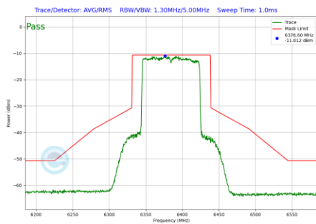
Plot 7-631 In-Band Emission Plot SDM Primary Antenna 5T (80MHz BW 802.11be(RU) RU996 Index67 (UNII Band 5) - Ch.87)
