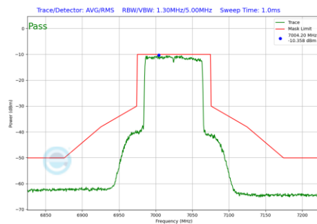
Plot 7-483 In-Band Emission Plot Antenna 5T (80MHz BW 802.11be(RU) RU996 Index67 (UNII Band 8) - Ch.215)
