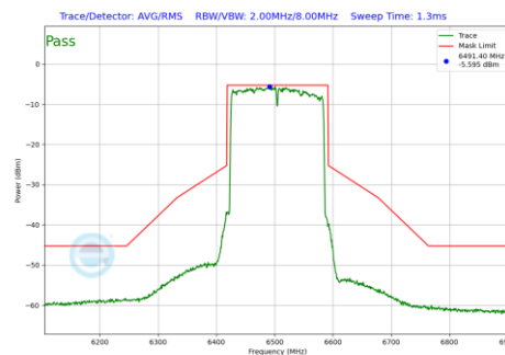
Plot 7-520 In-Band Emission Plot Antenna 3b (160MHz BW 802.11be(RU) RU996X2 Index68 (UNII Band 6) - Ch.111)
