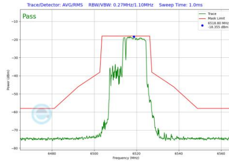
Plot 7-620 In-Band Emission Plot SDM Primary Antenna 3b (20MHz BW 802.11be(RU) RU106+26 Index83 (UNII Band 6) - Ch.113)
