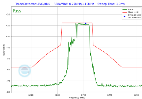
Plot 7-623 In-Band Emission Plot SDM Primary Antenna 3b (20MHz BW 802.11be(RU) RU106+26 Index83 (UNII Band 7) - Ch.149)
