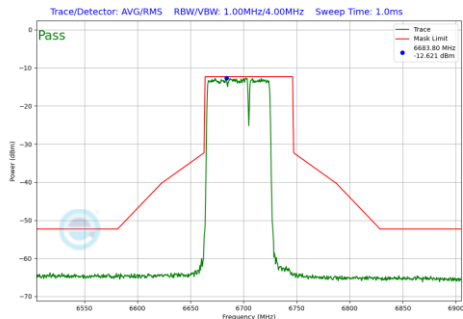
Plot 7-624 In-Band Emission Plot SDM Primary Antenna 3b (80MHz BW 802.11be(RU) RU484+242 Index93 (UNII Band 7) - Ch.151)
