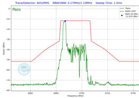
Plot 7-493 In-Band Emission Plot Antenna 3b (20MHz BW 802.11be(RU) RU26 Index0 (UNII Band 7) - Ch.149)
