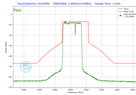
Plot 7-549 In-Band Emission Plot Antenna 1b (80MHz BW 802.11be(RU) RU484+242 Index93 (UNII Band 6) - Ch.103)
