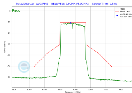
Plot 7-644 In-Band Emission Plot SDM Primary Antenna 5T (160MHz BW 802.11be(RU) RU996X2 Index68 (UNII Band 8) - Ch.207)
