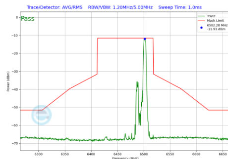
Plot 7-683 In-Band Emission Plot SDM Diversity Antenna 5T (80MHz BW 802.11be(RU) RU52 Index52 (UNII Band 6) - Ch.103)
