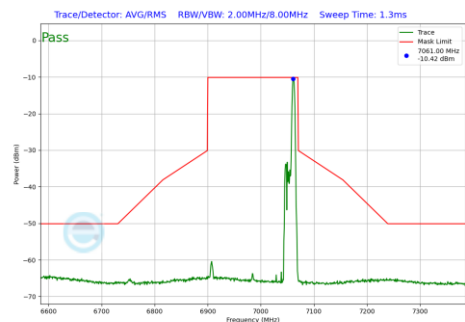
Plot 7-692 In-Band Emission Plot SDM Diversity Antenna 5T (160MHz BW 802.11be(RU) RU52 Index52 (UNII Band 8) - Ch.207)
