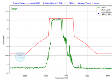
Plot 7-702 In-Band Emission Plot SDM Diversity Antenna 1b (20MHz BW 802.11be(RU) RU106+26 Index82 (UNII Band 8) - Ch.209)
