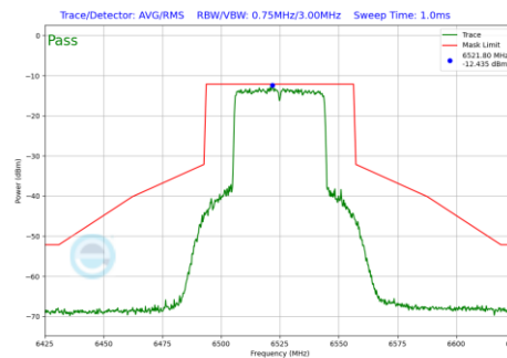
Plot 7-738 In-Band Emission Plot SDM Diversity Antenna 5T (40MHz BW 802.11be(RU) RU484 Index65 (UNII Band 6) - Ch.115)
