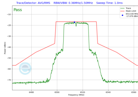
Plot 7-737 In-Band Emission Plot SDM Diversity Antenna 5T (20MHz BW 802.11be(RU) RU242 Index61 (UNII Band 6) - Ch.113)
