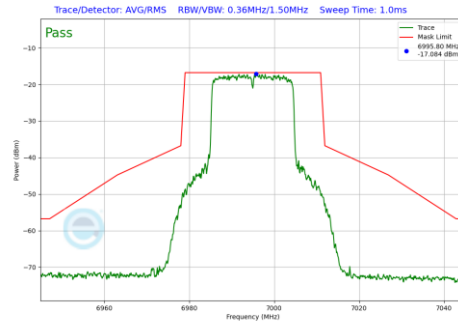
Plot 7-745 In-Band Emission Plot SDM Diversity Antenna 5T (20MHz BW 802.11be(RU) RU242 Index61 (UNII Band 8) - Ch.209)
