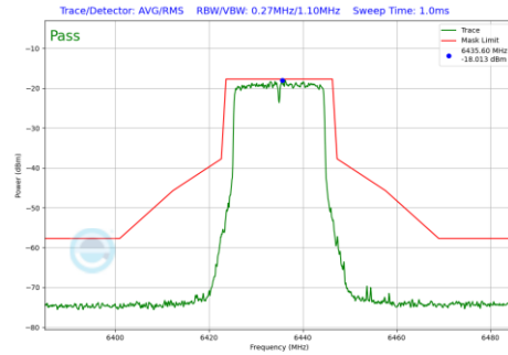
Plot 7-649 In-Band Emission Plot SDM Primary Antenna 3b (20MHz BW 802.11be(RU) RU242 Index61 (UNII Band 6) - Ch.97)
