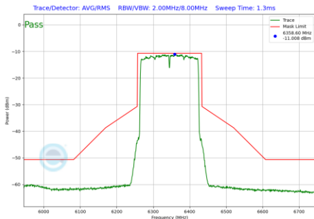
Plot 7-648 In-Band Emission Plot SDM Primary Antenna 3b (160MHz BW 802.11be(RU) RU996X2 Index68 (UNII Band 5) - Ch.79)
