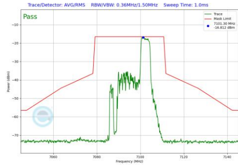
Plot 7-689 In-Band Emission Plot SDM Diversity Antenna 5T (20MHz BW 802.11be(RU) RU52 Index40 (UNII Band 8) - Ch.229)
