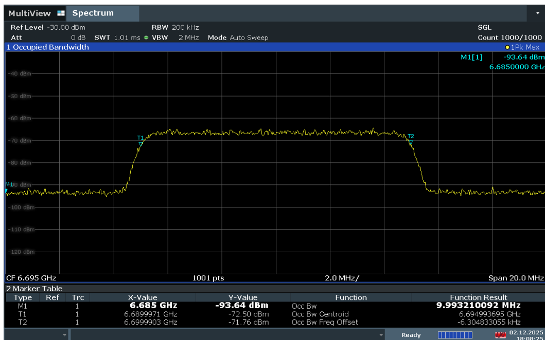
Plot 7-757. AWGN Signal – UNII 7 – 20MHz
