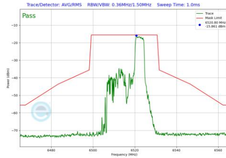
Plot 7-681 In-Band Emission Plot SDM Diversity Antenna 5T (20MHz BW 802.11be(RU) RU52 Index40 (UNII Band 6) - Ch.113)
