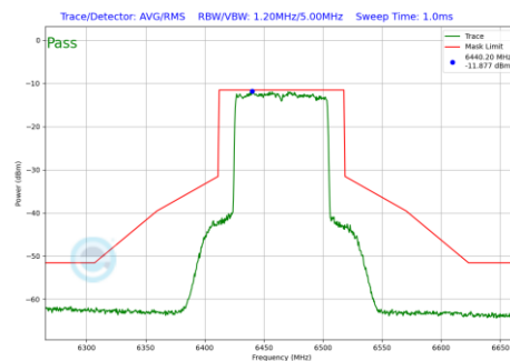
Plot 7-739 In-Band Emission Plot SDM Diversity Antenna 5T (80MHz BW 802.11be(RU) RU996 Index67 (UNII Band 6) - Ch.103)
