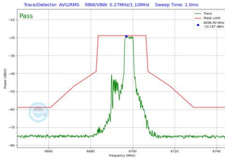
Plot 7-669 In-Band Emission Plot SDM Diversity Antenna 1b (20MHz BW 802.11be(RU) RU52 Index39 (UNII Band 7) - Ch.149)
