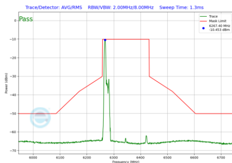
Plot 7-680 In-Band Emission Plot SDM Diversity Antenna 5T (160MHz BW 802.11be(RU) RU52 Index37 (UNII Band 5) - Ch.79)
