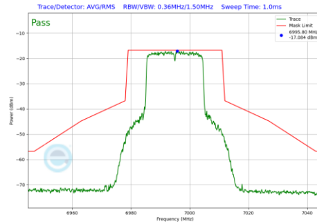
Plot 7-641 In-Band Emission Plot SDM Primary Antenna 5T (20MHz BW 802.11be(RU) RU242 Index61 (UNII Band 8) - Ch.209)
