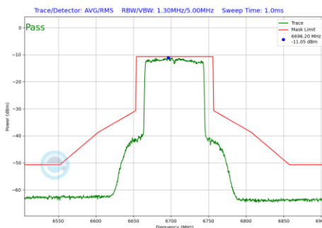
Plot 7-743 In-Band Emission Plot SDM Diversity Antenna 5T (80MHz BW 802.11be(RU) RU996 Index67 (UNII Band 7) - Ch.151)
