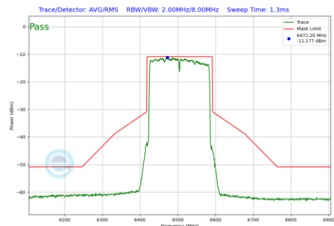
Plot 7-652 In-Band Emission Plot SDM Primary Antenna 3b (160MHz BW 802.11be(RU) RU996X2 Index68 (UNII Band 6) - Ch.111)
