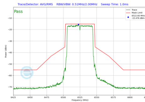
Plot 7-722 In-Band Emission Plot SDM Diversity Antenna 1b (40MHz BW 802.11be(RU) RU484 Index65 (UNII Band 6) - Ch.115)
