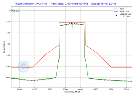
Plot 7-720 In-Band Emission Plot SDM Diversity Antenna 1b (160MHz BW 802.11be(RU) RU996X2 Index68 (UNII Band 5) - Ch.79)
