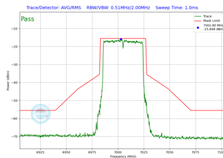
Plot 7-730 In-Band Emission Plot SDM Diversity Antenna 1b (40MHz BW 802.11be(RU) RU484 Index65 (UNII Band 8) - Ch.211)
