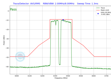
Plot 7-707 In-Band Emission Plot SDM Diversity Antenna 5T (160MHz BW 802.11be(RU) RU996+484+242 Index99 (UNII Band 5) - Ch.79)
