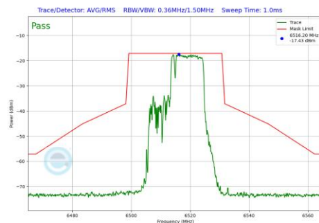
Plot 7-708 In-Band Emission Plot SDM Diversity Antenna 5T (20MHz BW 802.11be(RU) RU106+26 Index83 (UNII Band 6) - Ch.113)
