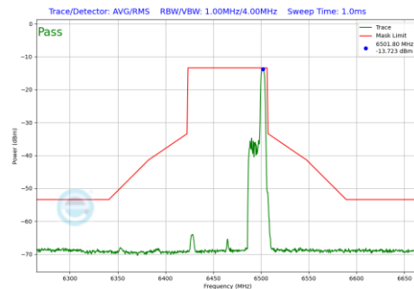
Plot 7-667 In-Band Emission Plot SDM Diversity Antenna 1b (80MHz BW 802.11be(RU) RU52 Index52 (UNII Band 6) - Ch.103)
