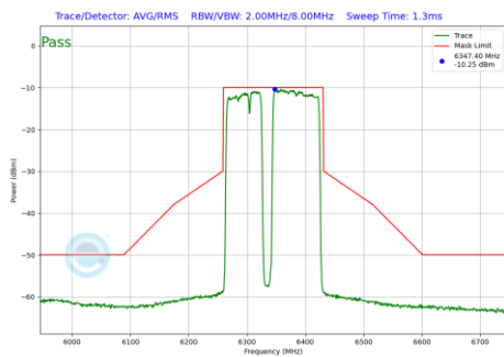
Plot 7-695 In-Band Emission Plot SDM Diversity Antenna 1b (160MHz BW 802.11be(RU) RU996+484+242 Index99 (UNII Band 5) - Ch.79)
