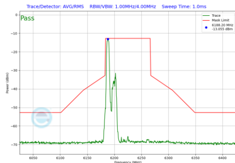
Plot 7-663 In-Band Emission Plot SDM Diversity Antenna 1b (80MHz BW 802.11be(RU) RU52 Index37 (UNII Band 5) - Ch.55)
