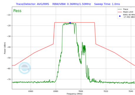
Plot 7-714 In-Band Emission Plot SDM Diversity Antenna 5T (20MHz BW 802.11be(RU) RU106+26 Index82 (UNII Band 8) - Ch.209)
