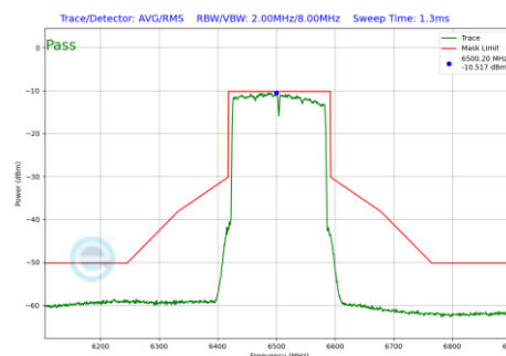
Plot 7-740 In-Band Emission Plot SDM Diversity Antenna 5T (160MHz BW 802.11be(RU) RU996X2 Index68 (UNII Band 6) - Ch.111)
