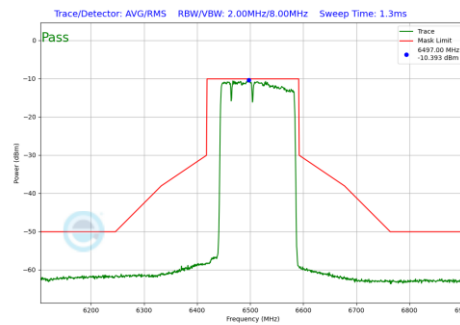
Plot 7-698 In-Band Emission Plot SDM Diversity Antenna 1b (160MHz BW 802.11be(RU) RU996+484+242 Index96 (UNII Band 6) - Ch.111)
