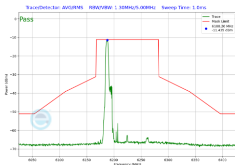
Plot 7-679 In-Band Emission Plot SDM Diversity Antenna 5T (80MHz BW 802.11be(RU) RU52 Index37 (UNII Band 5) - Ch.55)
