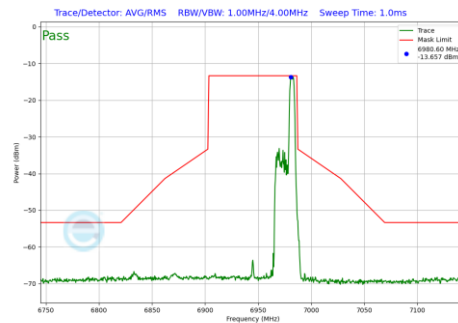
Plot 7-675 In-Band Emission Plot SDM Diversity Antenna 1b (80MHz BW 802.11be(RU) RU52 Index52 (UNII Band 8) - Ch.199)
