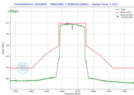
Plot 7-728 In-Band Emission Plot SDM Diversity Antenna 1b (160MHz BW 802.11be(RU) RU996X2 Index68 (UNII Band 7) - Ch.143)
