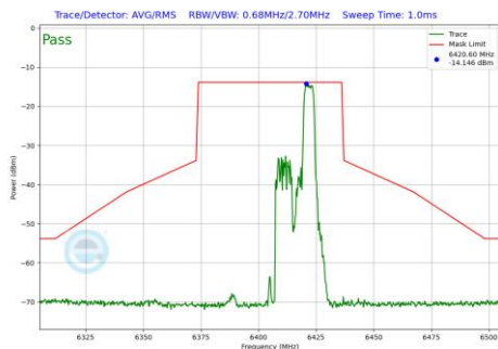
Plot 7-678 In-Band Emission Plot SDM Diversity Antenna 5T (40MHz BW 802.11be(RU) RU52 Index44 (UNII Band 5) - Ch.91)
