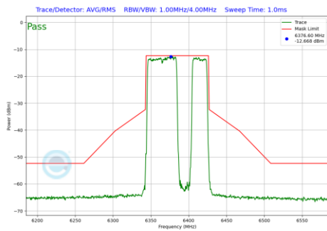
Plot 7-694 In-Band Emission Plot SDM Diversity Antenna 1b (80MHz BW 802.11be(RU) RU484+242 Index92 (UNII Band 5) - Ch.87)
