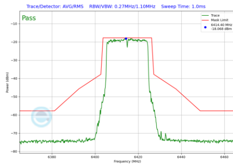
Plot 7-717 In-Band Emission Plot SDM Diversity Antenna 1b (20MHz BW 802.11be(RU) RU242 Index61 (UNII Band 5) - Ch.93)
