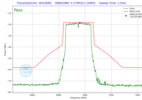
Plot 7-657 In-Band Emission Plot SDM Primary Antenna 3b (20MHz BW 802.11be(RU) RU242 Index61 (UNII Band 8) - Ch.209)
