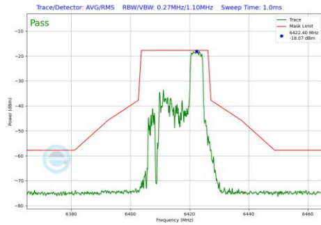
Plot 7-661 In-Band Emission Plot SDM Diversity Antenna 1b (20MHz BW 802.11be(RU) RU52 Index40 (UNII Band 5) - Ch.93)
