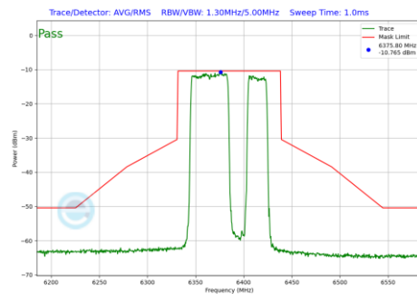
Plot 7-706 In-Band Emission Plot SDM Diversity Antenna 5T (80MHz BW 802.11be(RU) RU484+242 Index92 (UNII Band 5) - Ch.87)
