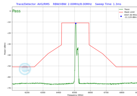
Plot 7-668 In-Band Emission Plot SDM Diversity Antenna 1b (160MHz BW 802.11be(RU) RU52 Index37 (UNII Band 6) - Ch.111)
