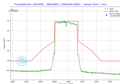
Plot 7-748 In-Band Emission Plot SDM Diversity Antenna 5T (160MHz BW 802.11be(RU) RU996X2 Index68 (UNII Band 8) - Ch.207)
