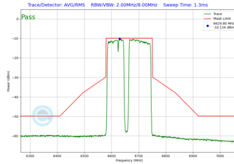
Plot 7-713 In-Band Emission Plot SDM Diversity Antenna 5T (160MHz BW 802.11be(RU) RU996+484+242 Index99 (UNII Band 7) - Ch.143)
