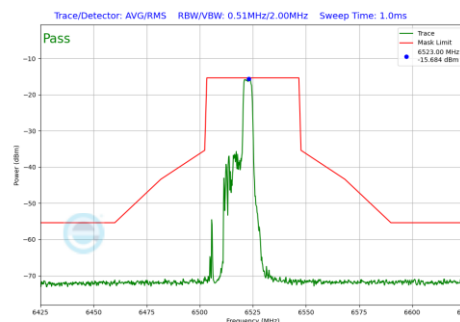
Plot 7-666 In-Band Emission Plot SDM Diversity Antenna 1b (40MHz BW 802.11be(RU) RU52 Index40 (UNII Band 6) - Ch.115)
