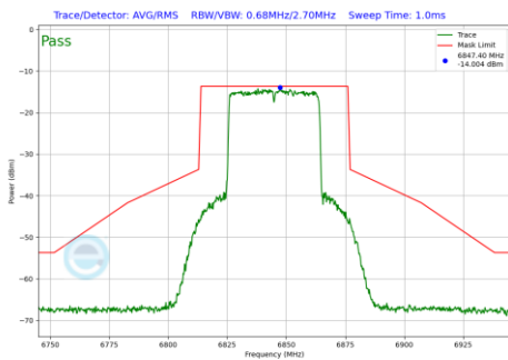
Plot 7-638 In-Band Emission Plot SDM Primary Antenna 5T (40MHz BW 802.11be(RU) RU484 Index65 (UNII Band 7) - Ch.179)
