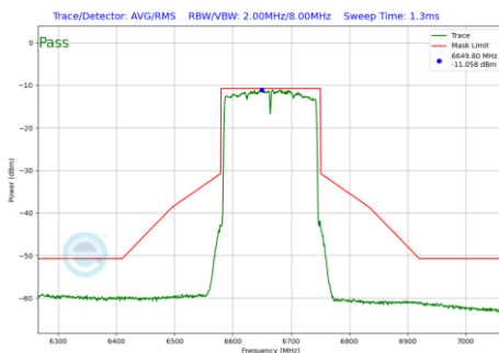
Plot 7-744 In-Band Emission Plot SDM Diversity Antenna 5T (160MHz BW 802.11be(RU) RU996X2 Index68 (UNII Band 7) - Ch.143)
