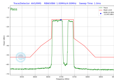
Plot 7-700 In-Band Emission Plot SDM Diversity Antenna 1b (80MHz BW 802.11be(RU) RU484+242 Index92 (UNII Band 7) - Ch.151)
