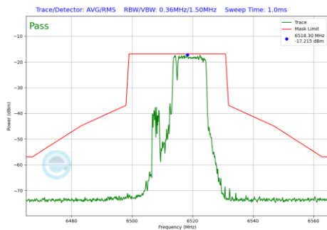
Plot 7-696 In-Band Emission Plot SDM Diversity Antenna 1b (20MHz BW 802.11be(RU) RU106+26 Index83 (UNII Band 6) - Ch.113)
