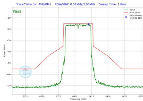
Plot 7-718 In-Band Emission Plot SDM Diversity Antenna 1b (40MHz BW 802.11be(RU) RU484 Index65 (UNII Band 5) - Ch.91)
