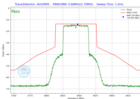
Plot 7-742 In-Band Emission Plot SDM Diversity Antenna 5T (40MHz BW 802.11be(RU) RU484 Index65 (UNII Band 7) - Ch.179)
