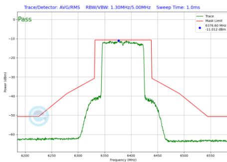
Plot 7-735 In-Band Emission Plot SDM Diversity Antenna 5T (80MHz BW 802.11be(RU) RU996 Index67 (UNII Band 5) - Ch.87)
