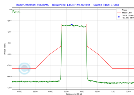
Plot 7-731 In-Band Emission Plot SDM Diversity Antenna 1b (80MHz BW 802.11be(RU) RU996 Index67 (UNII Band 8) - Ch.215)
