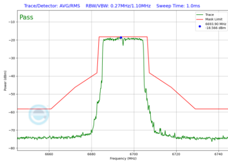
Plot 7-725 In-Band Emission Plot SDM Diversity Antenna 1b (20MHz BW 802.11be(RU) RU242 Index61 (UNII Band 7) - Ch.149)
