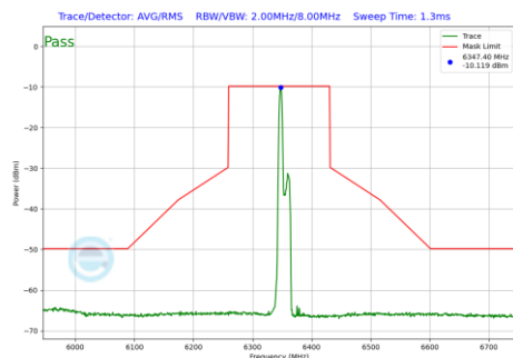
Plot 7-664 In-Band Emission Plot SDM Diversity Antenna 1b (160MHz BW 802.11be(RU) RU52 Index37 (UNII Band 5) - Ch.79)
