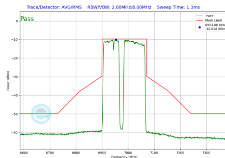
Plot 7-716 In-Band Emission Plot SDM Diversity Antenna 5T (160MHz BW 802.11be(RU) RU996+484+242 Index99 (UNII Band 8) - Ch.207)
