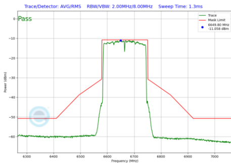
Plot 7-640 In-Band Emission Plot SDM Primary Antenna 5T (160MHz BW 802.11be(RU) RU996X2 Index68 (UNII Band 7) - Ch.143)
