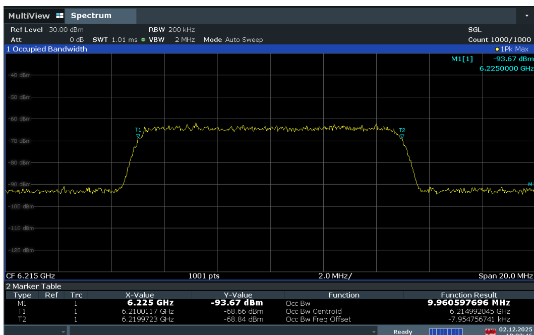
Plot 7-749. AWGN Signal – UNII 5 – 20MHz
