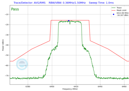
Plot 7-733 In-Band Emission Plot SDM Diversity Antenna 5T (20MHz BW 802.11be(RU) RU242 Index61 (UNII Band 5) - Ch.93)
