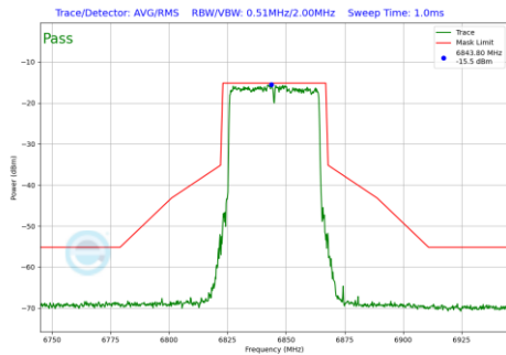
Plot 7-654 In-Band Emission Plot SDM Primary Antenna 3b (40MHz BW 802.11be(RU) RU484 Index65 (UNII Band 7) - Ch.179)
