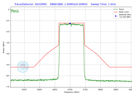
Plot 7-655 In-Band Emission Plot SDM Primary Antenna 3b (80MHz BW 802.11be(RU) RU996 Index67 (UNII Band 7) - Ch.151)
