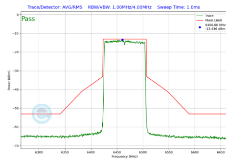
Plot 7-723 In-Band Emission Plot SDM Diversity Antenna 1b (80MHz BW 802.11be(RU) RU996 Index67 (UNII Band 6) - Ch.103)
