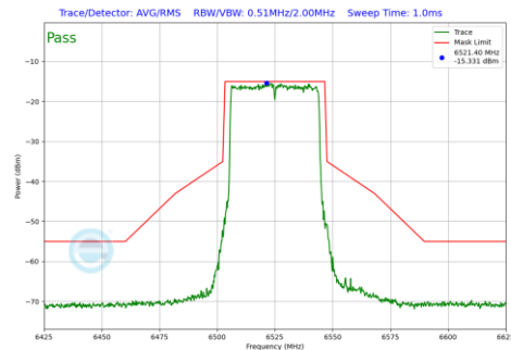
Plot 7-650 In-Band Emission Plot SDM Primary Antenna 3b (40MHz BW 802.11be(RU) RU484 Index65 (UNII Band 6) - Ch.115)
