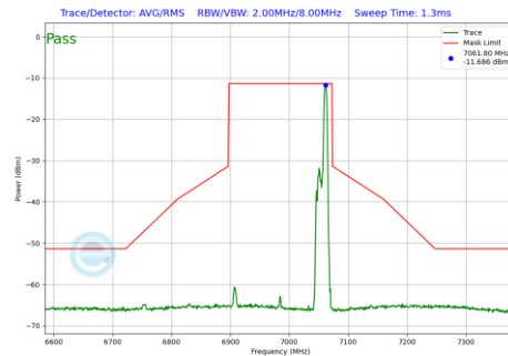
Plot 7-676 In-Band Emission Plot SDM Diversity Antenna 1b (160MHz BW 802.11be(RU) RU52 Index52 (UNII Band 8) - Ch.207)
