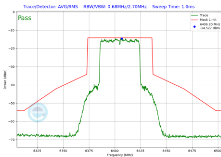
Plot 7-734 In-Band Emission Plot SDM Diversity Antenna 5T (40MHz BW 802.11be(RU) RU484 Index65 (UNII Band 5) - Ch.91)
