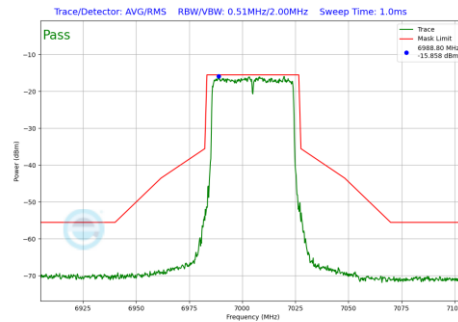
Plot 7-658 In-Band Emission Plot SDM Primary Antenna 3b (40MHz BW 802.11be(RU) RU484 Index65 (UNII Band 8) - Ch.211)
