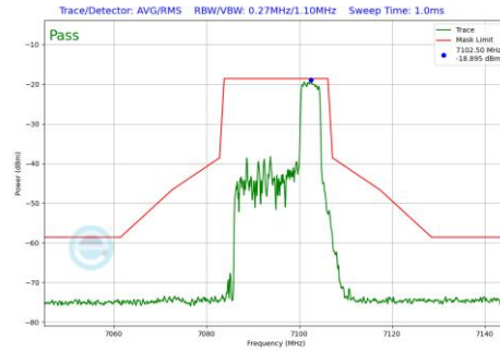
Plot 7-673 In-Band Emission Plot SDM Diversity Antenna 1b (20MHz BW 802.11be(RU) RU52 Index40 (UNII Band 8) - Ch.229)
