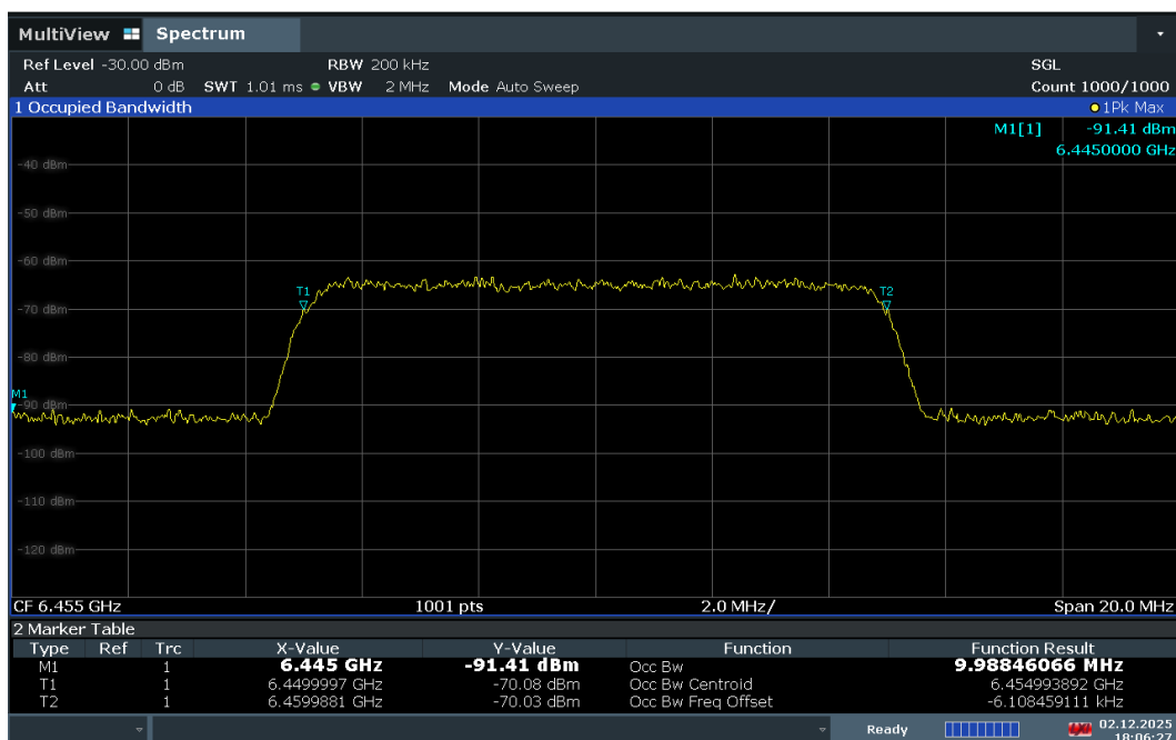
Plot 7-753. AWGN Signal – UNII 6 – 20MHz
