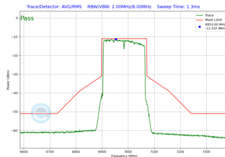
Plot 7-660 In-Band Emission Plot SDM Primary Antenna 3b (160MHz BW 802.11be(RU) RU996X2 Index68 (UNII Band 8) - Ch.207)
