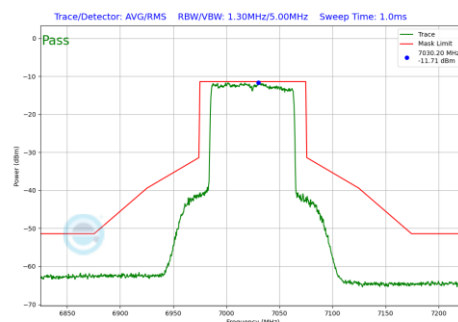
Plot 7-747 In-Band Emission Plot SDM Diversity Antenna 5T (80MHz BW 802.11be(RU) RU996 Index67 (UNII Band 8) - Ch.215)
