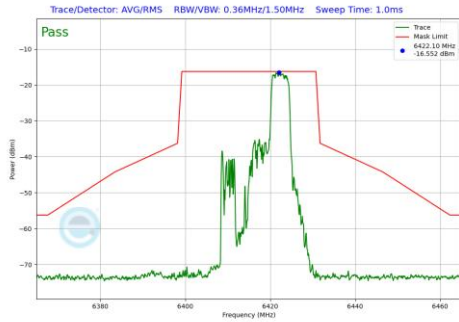
Plot 7-677 In-Band Emission Plot SDM Diversity Antenna 5T (20MHz BW 802.11be(RU) RU52 Index40 (UNII Band 5) - Ch.93)
