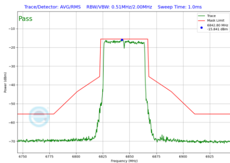
Plot 7-726 In-Band Emission Plot SDM Diversity Antenna 1b (40MHz BW 802.11be(RU) RU484 Index65 (UNII Band 7) - Ch.179)
