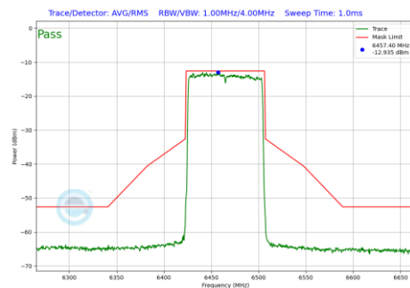
Plot 7-651 In-Band Emission Plot SDM Primary Antenna 3b (80MHz BW 802.11be(RU) RU996 Index67 (UNII Band 6) - Ch.103)
