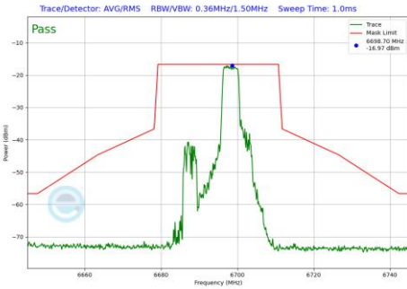
Plot 7-685 In-Band Emission Plot SDM Diversity Antenna 5T (20MHz BW 802.11be(RU) RU52 Index39 (UNII Band 7) - Ch.149)
