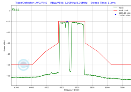
Plot 7-701 In-Band Emission Plot SDM Diversity Antenna 1b (160MHz BW 802.11be(RU) RU996+484+242 Index99 (UNII Band 7) - Ch.143)
