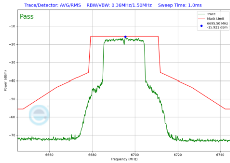
Plot 7-637 In-Band Emission Plot SDM Primary Antenna 5T (20MHz BW 802.11be(RU) RU242 Index61 (UNII Band 7) - Ch.149)
