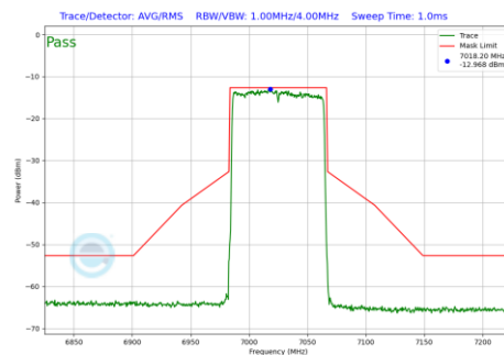
Plot 7-659 In-Band Emission Plot SDM Primary Antenna 3b (80MHz BW 802.11be(RU) RU996 Index67 (UNII Band 8) - Ch.215)
