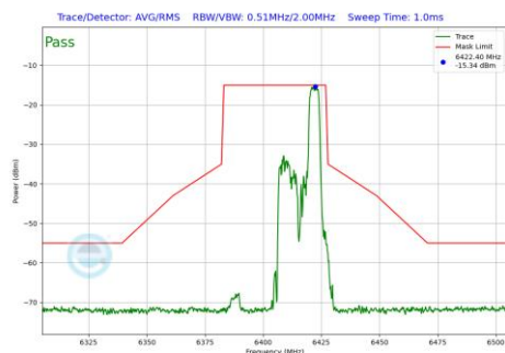
Plot 7-662 In-Band Emission Plot SDM Diversity Antenna 1b (40MHz BW 802.11be(RU) RU52 Index44 (UNII Band 5) - Ch.91)
