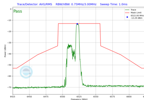
Plot 7-682 In-Band Emission Plot SDM Diversity Antenna 5T (40MHz BW 802.11be(RU) RU52 Index40 (UNII Band 6) - Ch.115)
