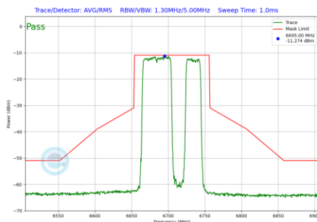
Plot 7-712 In-Band Emission Plot SDM Diversity Antenna 5T (80MHz BW 802.11be(RU) RU484+242 Index92 (UNII Band 7) - Ch.151)
