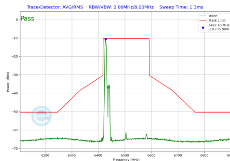
Plot 7-684 In-Band Emission Plot SDM Diversity Antenna 5T (160MHz BW 802.11be(RU) RU52 Index37 (UNII Band 6) - Ch.111)
