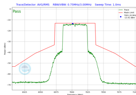
Plot 7-746 In-Band Emission Plot SDM Diversity Antenna 5T (40MHz BW 802.11be(RU) RU484 Index65 (UNII Band 8) - Ch.211)
