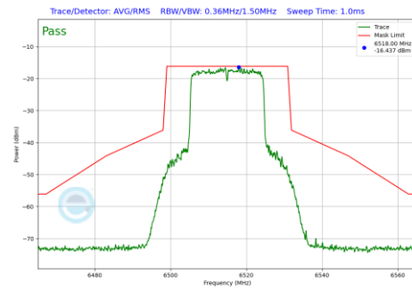
Plot 7-721 In-Band Emission Plot SDM Diversity Antenna 1b (20MHz BW 802.11be(RU) RU242 Index61 (UNII Band 6) - Ch.113)
