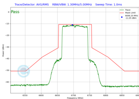
Plot 7-639 In-Band Emission Plot SDM Primary Antenna 5T (80MHz BW 802.11be(RU) RU996 Index67 (UNII Band 7) - Ch.151)
