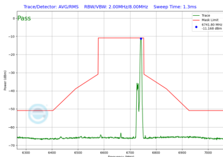
Plot 7-672 In-Band Emission Plot SDM Diversity Antenna 1b (160MHz BW 802.11be(RU) RU52 Index52 (UNII Band 7) - Ch.143)
