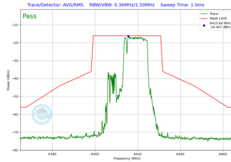
Plot 7-705 In-Band Emission Plot SDM Diversity Antenna 5T (20MHz BW 802.11be(RU) RU106+26 Index83 (UNII Band 5) - Ch.93)
