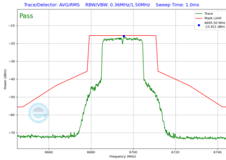
Plot 7-741 In-Band Emission Plot SDM Diversity Antenna 5T (20MHz BW 802.11be(RU) RU242 Index61 (UNII Band 7) - Ch.149)
