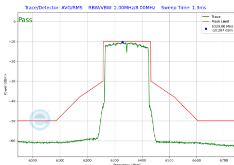
Plot 7-736 In-Band Emission Plot SDM Diversity Antenna 5T (160MHz BW 802.11be(RU) RU996X2 Index68 (UNII Band 5) - Ch.79)
