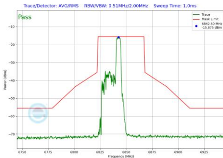
Plot 7-670 In-Band Emission Plot SDM Diversity Antenna 1b (40MHz BW 802.11be(RU) RU52 Index40 (UNII Band 7) - Ch.179)
