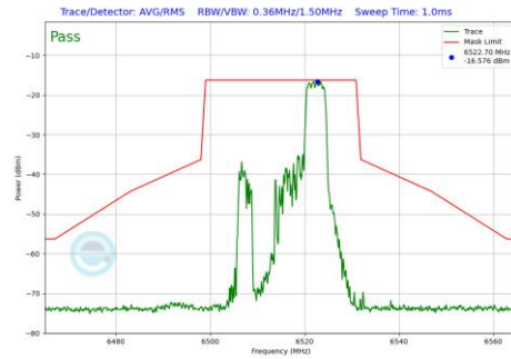
Plot 7-665 In-Band Emission Plot SDM Diversity Antenna 1b (20MHz BW 802.11be(RU) RU52 Index40 (UNII Band 6) - Ch.113)
