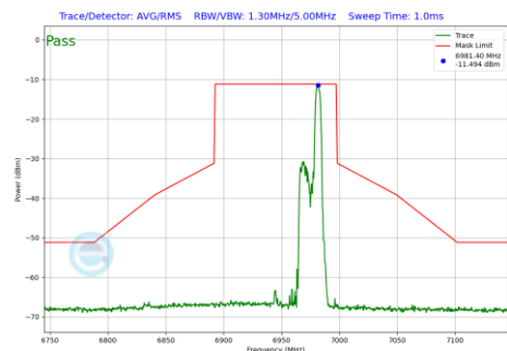
Plot 7-691 In-Band Emission Plot SDM Diversity Antenna 5T (80MHz BW 802.11be(RU) RU52 Index52 (UNII Band 8) - Ch.199)
