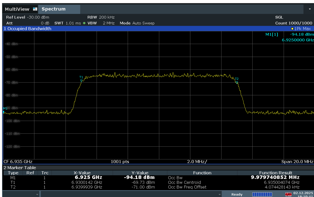
Plot 7-761. AWGN Signal – UNII 8 – 20MHz
