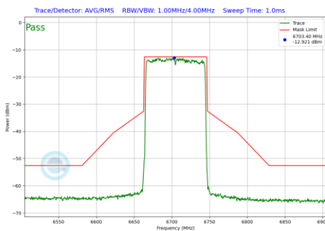
Plot 7-727 In-Band Emission Plot SDM Diversity Antenna 1b (80MHz BW 802.11be(RU) RU996 Index67 (UNII Band 7) - Ch.151)
