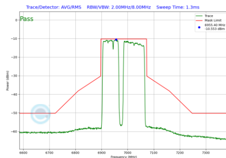
Plot 7-704 In-Band Emission Plot SDM Diversity Antenna 1b (160MHz BW 802.11be(RU) RU996+484+242 Index99 (UNII Band 8) - Ch.207)
