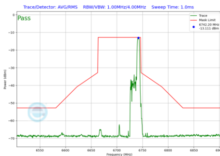
Plot 7-671 In-Band Emission Plot SDM Diversity Antenna 1b (80MHz BW 802.11be(RU) RU52 Index52 (UNII Band 7) - Ch.151)
