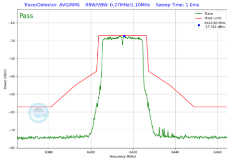
Plot 7-645 In-Band Emission Plot SDM Primary Antenna 3b (20MHz BW 802.11be(RU) RU242 Index61 (UNII Band 5) - Ch.93)
