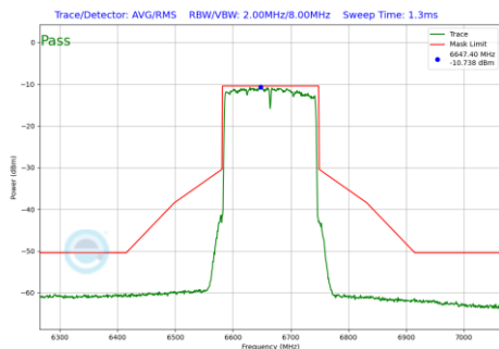
Plot 7-656 In-Band Emission Plot SDM Primary Antenna 3b (160MHz BW 802.11be(RU) RU996X2 Index68 (UNII Band 7) - Ch.143)
