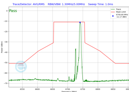
Plot 7-687 In-Band Emission Plot SDM Diversity Antenna 5T (80MHz BW 802.11be(RU) RU52 Index52 (UNII Band 7) - Ch.151)
