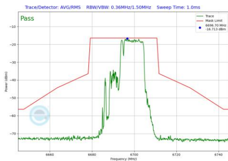
Plot 7-711 In-Band Emission Plot SDM Diversity Antenna 5T (20MHz BW 802.11be(RU) RU106+26 Index83 (UNII Band 7) - Ch.149)
