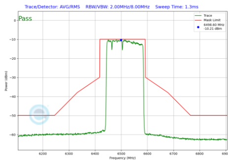
Plot 7-710 In-Band Emission Plot SDM Diversity Antenna 5T (160MHz BW 802.11be(RU) RU996+484+242 Index96 (UNII Band 6) - Ch.111)
