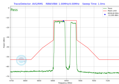
Plot 7-703 In-Band Emission Plot SDM Diversity Antenna 1b (80MHz BW 802.11be(RU) RU484+242 Index92 (UNII Band 8) - Ch.199)
