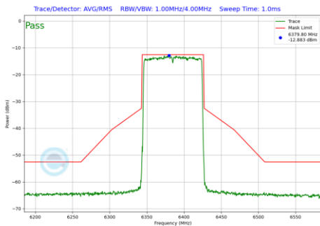
Plot 7-647 In-Band Emission Plot SDM Primary Antenna 3b (80MHz BW 802.11be(RU) RU996 Index67 (UNII Band 5) - Ch.87)
