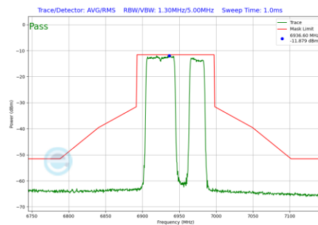
Plot 7-715 In-Band Emission Plot SDM Diversity Antenna 5T (80MHz BW 802.11be(RU) RU484+242 Index92 (UNII Band 8) - Ch.199)
