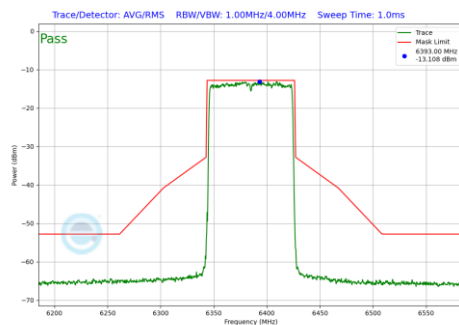
Plot 7-719 In-Band Emission Plot SDM Diversity Antenna 1b (80MHz BW 802.11be(RU) RU996 Index67 (UNII Band 5) - Ch.87)
