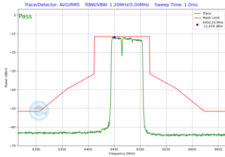
Plot 7-709 In-Band Emission Plot SDM Diversity Antenna 5T (80MHz BW 802.11be(RU) RU484+242 Index90 (UNII Band 6) - Ch.103)
