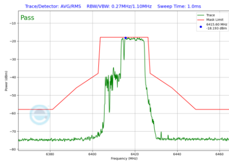
Plot 7-693 In-Band Emission Plot SDM Diversity Antenna 1b (20MHz BW 802.11be(RU) RU106+26 Index83 (UNII Band 5) - Ch.93)
