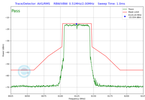
Plot 7-646 In-Band Emission Plot SDM Primary Antenna 3b (40MHz BW 802.11be(RU) RU484 Index65 (UNII Band 5) - Ch.35)
