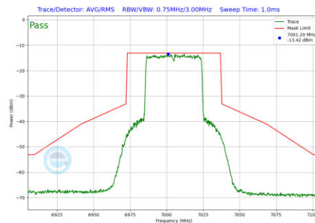
Plot 7-642 In-Band Emission Plot SDM Primary Antenna 5T (40MHz BW 802.11be(RU) RU484 Index65 (UNII Band 8) - Ch.211)
