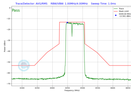
Plot 7-697 In-Band Emission Plot SDM Diversity Antenna 1b (80MHz BW 802.11be(RU) RU484+242 Index90 (UNII Band 6) - Ch.103)
