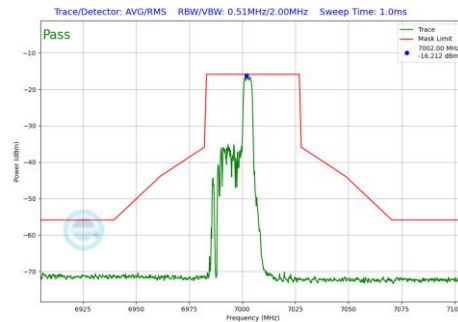
Plot 7-674 In-Band Emission Plot SDM Diversity Antenna 1b (40MHz BW 802.11be(RU) RU52 Index40 (UNII Band 8) - Ch.211)
