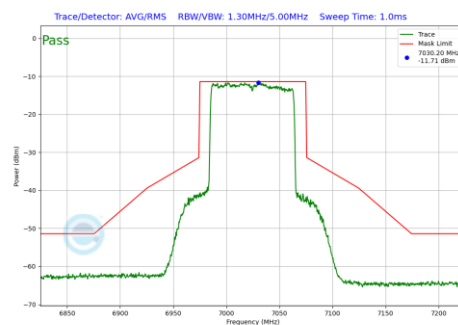
Plot 7-643 In-Band Emission Plot SDM Primary Antenna 5T (80MHz BW 802.11be(RU) RU996 Index67 (UNII Band 8) - Ch.215)
