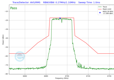
Plot 7-653 In-Band Emission Plot SDM Primary Antenna 3b (20MHz BW 802.11be(RU) RU242 Index61 (UNII Band 7) - Ch.149)
