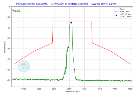
Plot 7-690 In-Band Emission Plot SDM Diversity Antenna 5T (40MHz BW 802.11be(RU) RU52 Index40 (UNII Band 8) - Ch.211)
