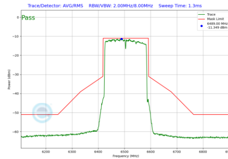
Plot 7-724 In-Band Emission Plot SDM Diversity Antenna 1b (160MHz BW 802.11be(RU) RU996X2 Index68 (UNII Band 6) - Ch.111)
