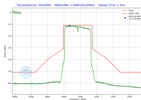
Plot 7-732 In-Band Emission Plot SDM Diversity Antenna 1b (160MHz BW 802.11be(RU) RU996X2 Index68 (UNII Band 8) - Ch.207)
