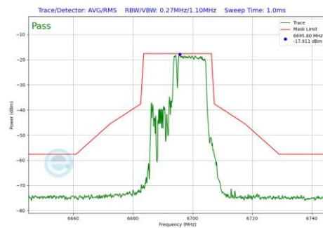
Plot 7-699 In-Band Emission Plot SDM Diversity Antenna 1b (20MHz BW 802.11be(RU) RU106+26 Index83 (UNII Band 7) - Ch.149)
