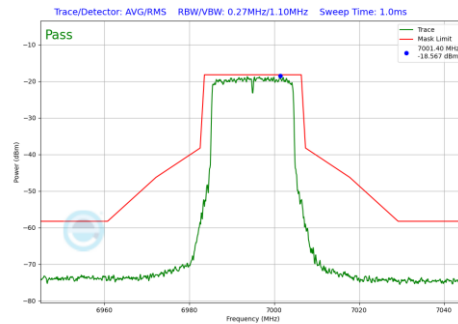
Plot 7-729 In-Band Emission Plot SDM Diversity Antenna 1b (20MHz BW 802.11be(RU) RU242 Index61 (UNII Band 8) - Ch.209)
