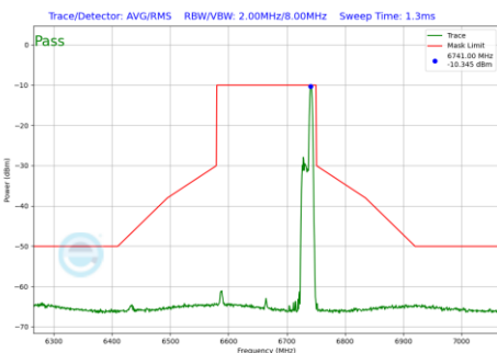
Plot 7-688 In-Band Emission Plot SDM Diversity Antenna 5T (160MHz BW 802.11be(RU) RU52 Index52 (UNII Band 7) - Ch.143)
