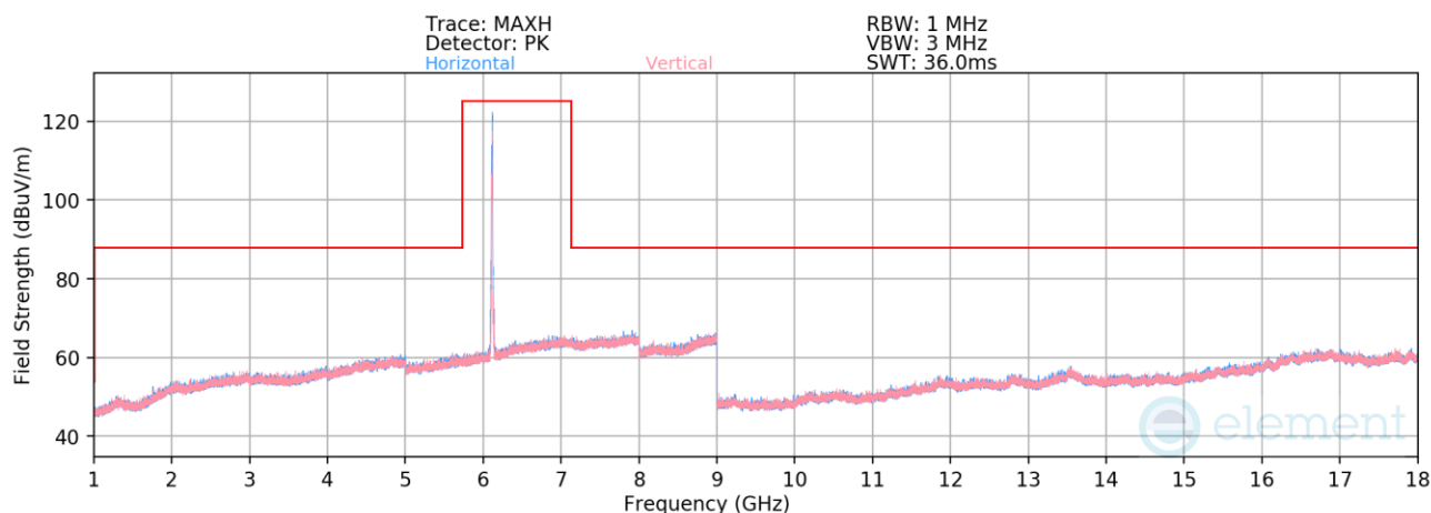
Plot 7-800. Radiated Spurious Emissions above 1GHz SDM Primary (802.11be – Ch. 33 – RU52)
