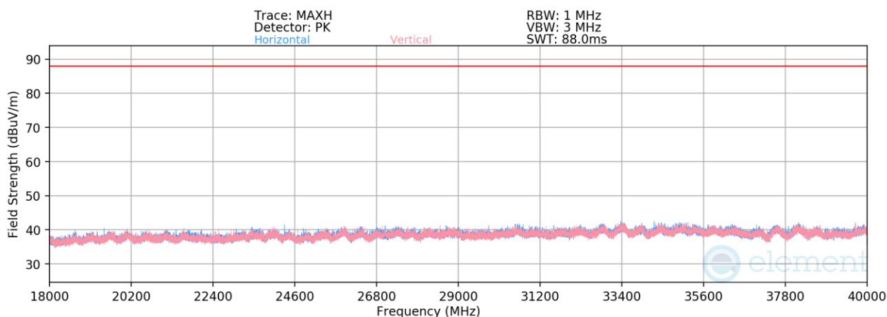
Plot 7-838. Radiated Spurious Emissions 18-40GHz SDM Diversity (802.11be – Ch. 105 – RU52)
