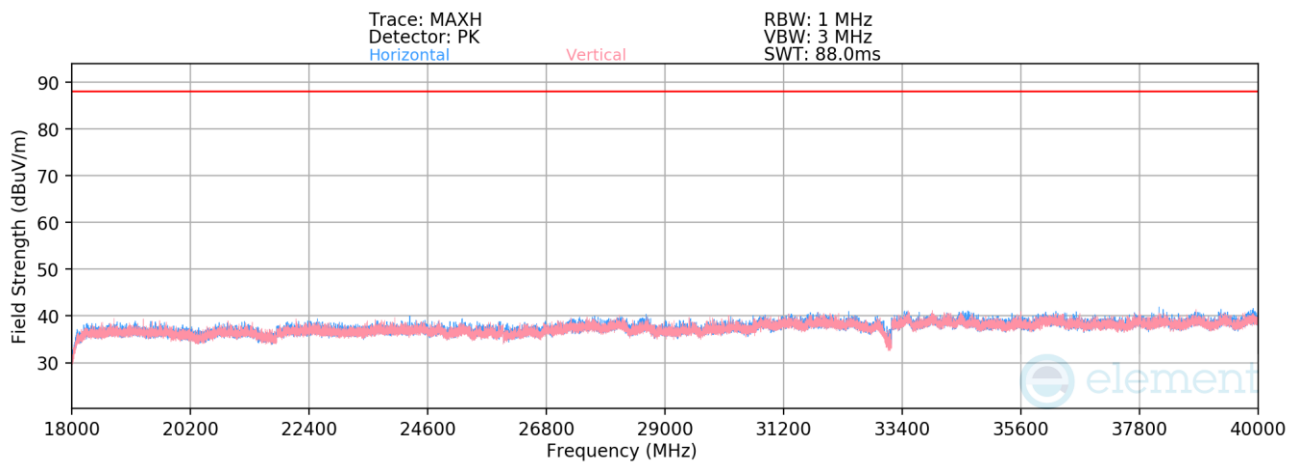
Plot 7-818. Radiated Spurious Emissions 18-40GHz SDM Primary (802.11be – Ch. 61 – RU242)
