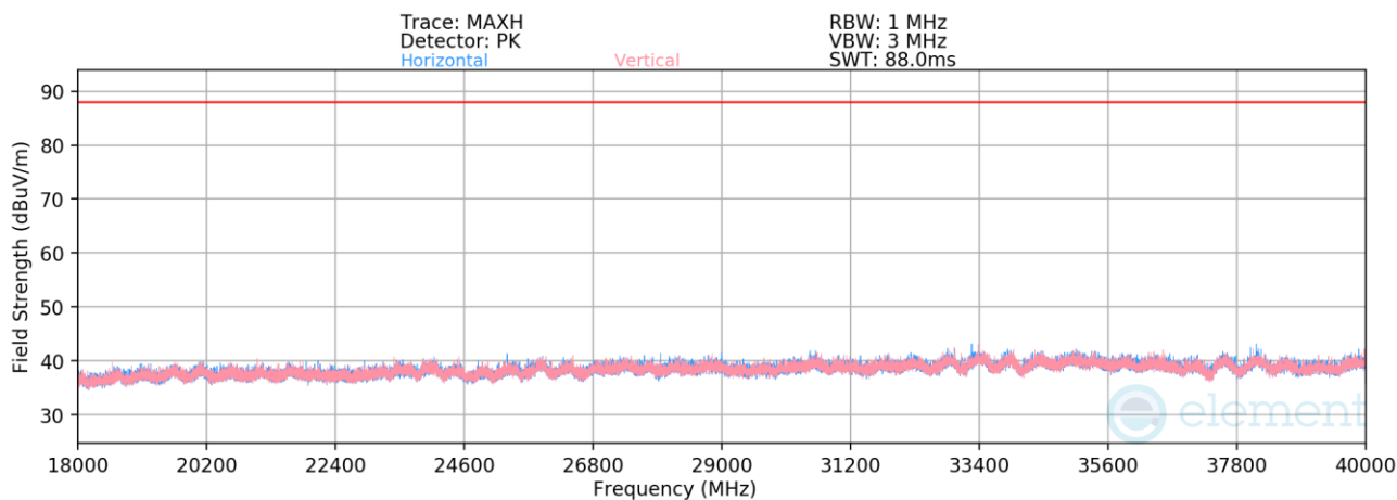
Plot 7-814. Radiated Spurious Emissions 18-40GHz SDM Primary (802.11be – Ch. 209 – RU52)
