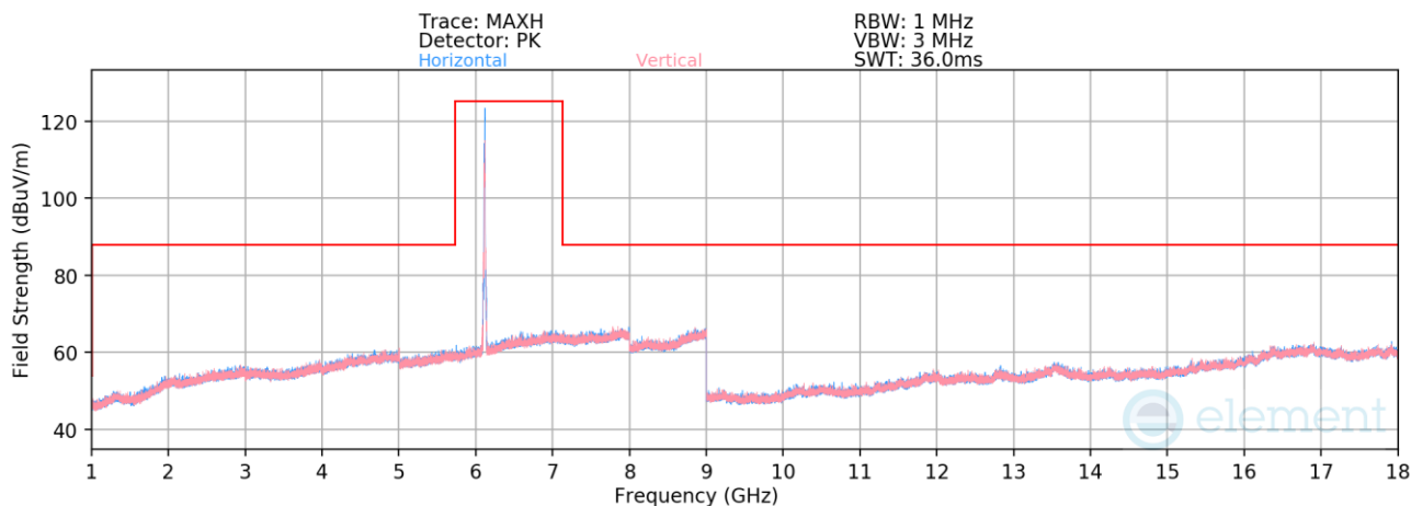
Plot 7-832. Radiated Spurious Emissions above 1GHz SDM Diversity (802.11be – Ch. 33 – RU52)
