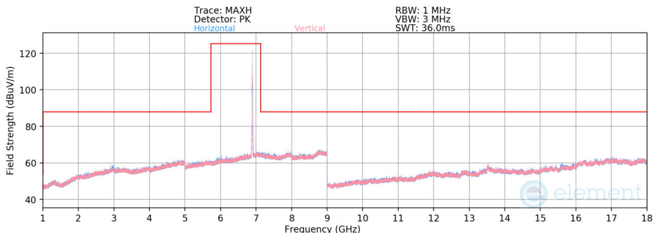
Plot 7-844. Radiated Spurious Emissions above 1GHz SDM Diversity (802.11be – Ch. 189 – RU52)
