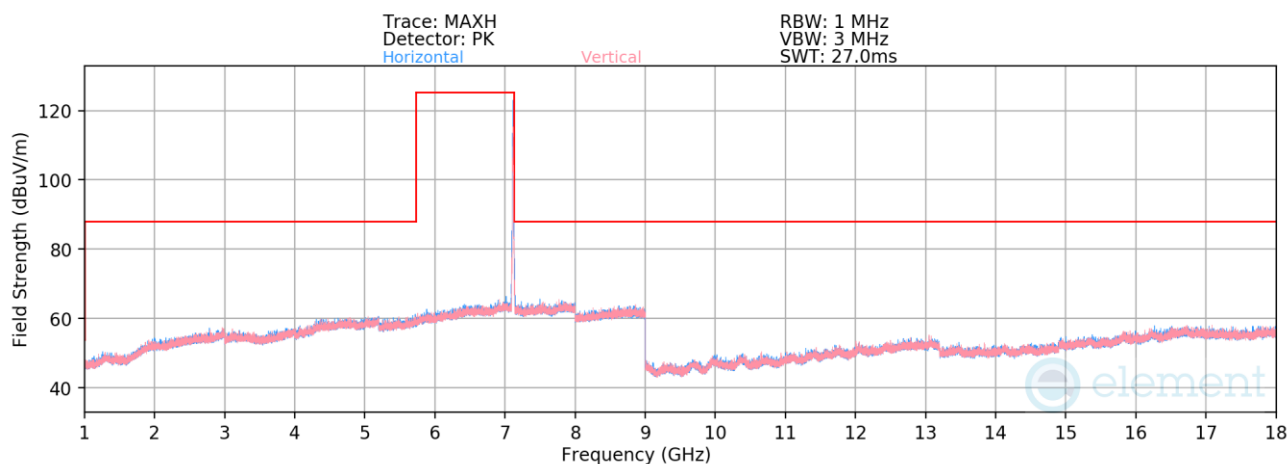
Plot 7-815. Radiated Spurious Emissions above 1GHz SDM Primary (802.11be – Ch. 229 – RU52)
