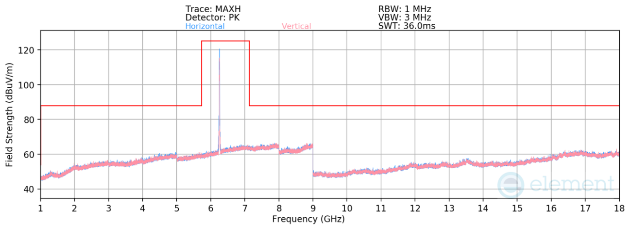
Plot 7-801. Radiated Spurious Emissions above 1GHz SDM Primary (802.11be – Ch. 61 – RU52)
