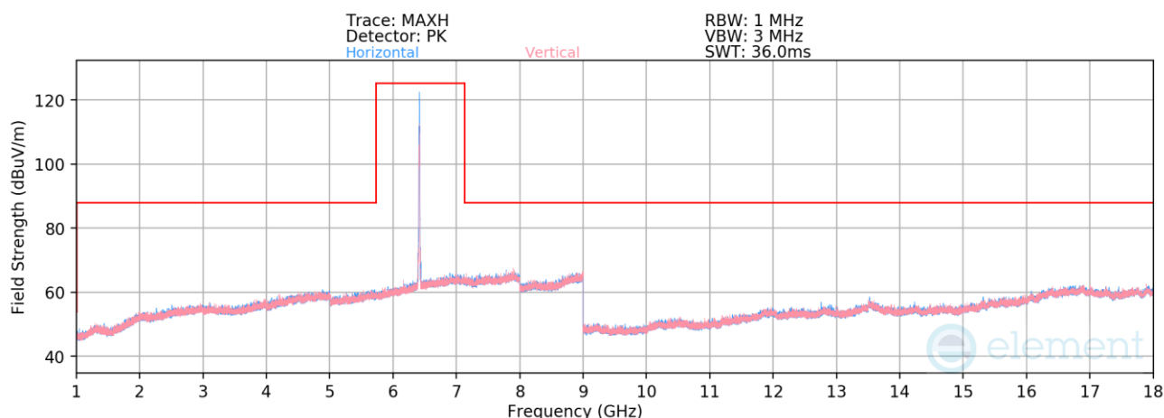
Plot 7-803. Radiated Spurious Emissions above 1GHz SDM Primary (802.11be – Ch. 93 – RU52)
