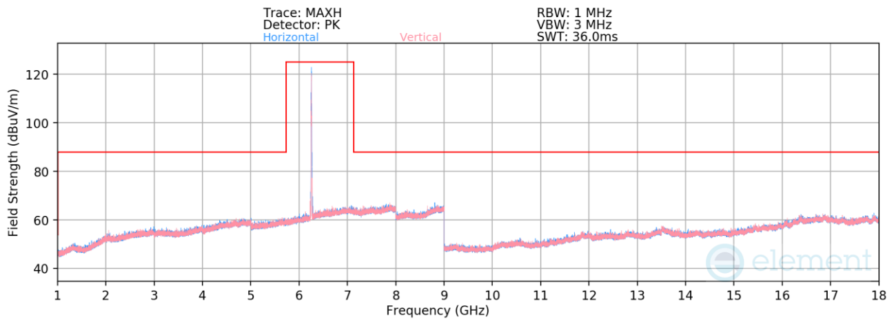
Plot 7-833. Radiated Spurious Emissions above 1GHz SDM Diversity (802.11be – Ch. 61 – RU52)
