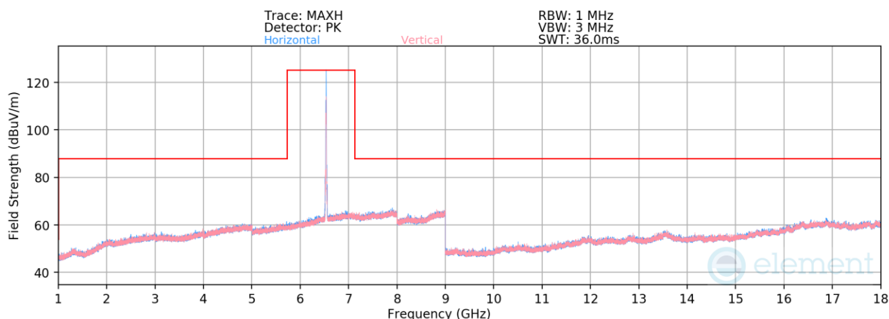
Plot 7-840. Radiated Spurious Emissions above 1GHz SDM Diversity (802.11be – Ch. 117 – RU52)
