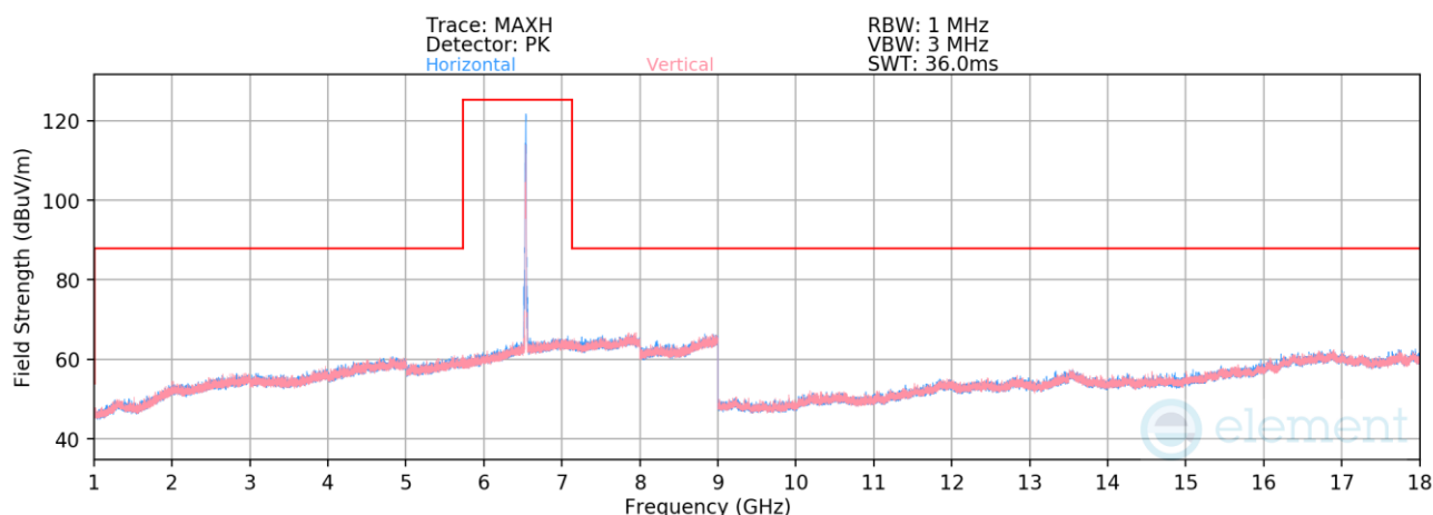
Plot 7-808. Radiated Spurious Emissions above 1GHz SDM Primary (802.11be – Ch. 117 – RU52)
