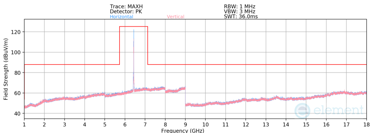
Plot 7-804. Radiated Spurious Emissions above 1GHz SDM Primary (802.11be – Ch. 97 – RU52)
