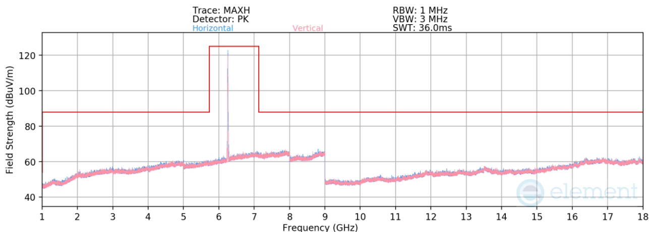
Plot 7-849. Radiated Spurious Emissions above 1GHz SDM Diversity (802.11be – Ch. 45 – RU242)
