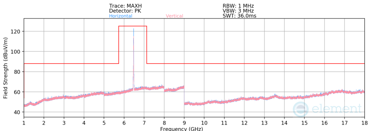
Plot 7-837. Radiated Spurious Emissions above 1GHz SDM Diversity (802.11be – Ch. 105 – RU52)
