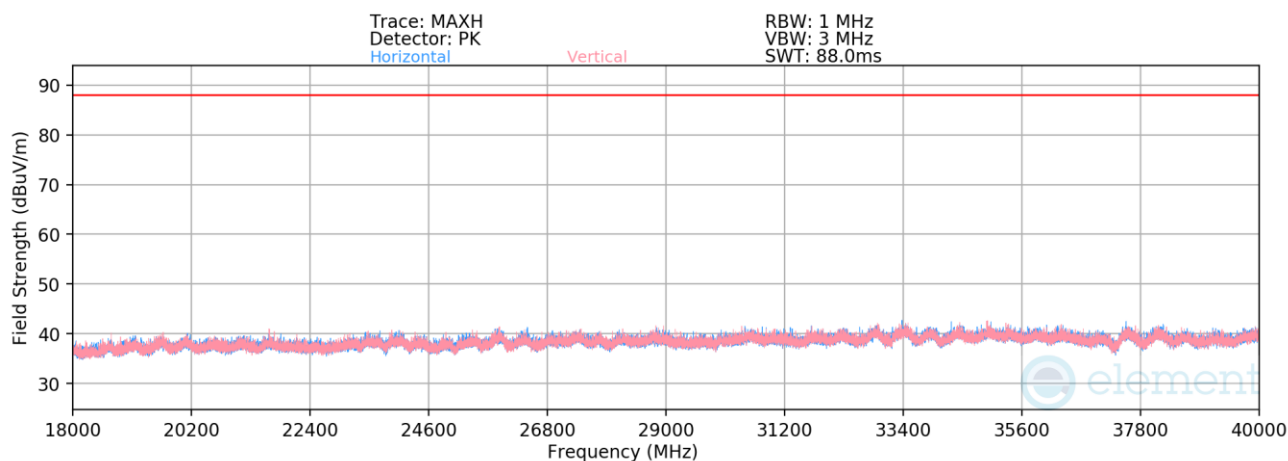
Plot 7-846. Radiated Spurious Emissions 18-40GHz SDM Diversity (802.11be – Ch. 209 – RU52)
