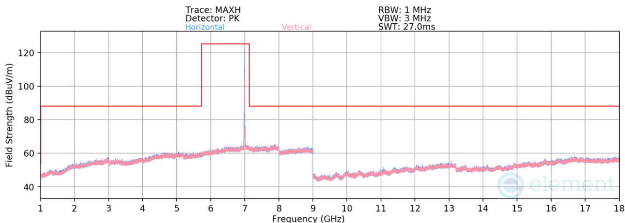
Plot 7-813. Radiated Spurious Emissions above 1GHz SDM Primary (802.11be – Ch. 209 – RU52)
