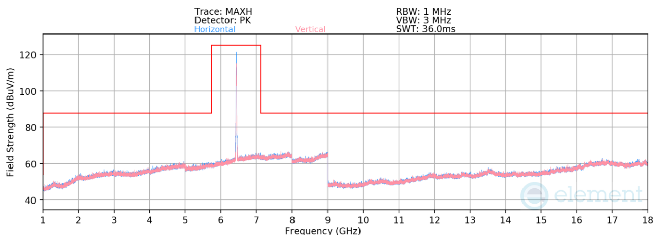
Plot 7-836. Radiated Spurious Emissions above 1GHz SDM Diversity (802.11be – Ch. 97 – RU52)
