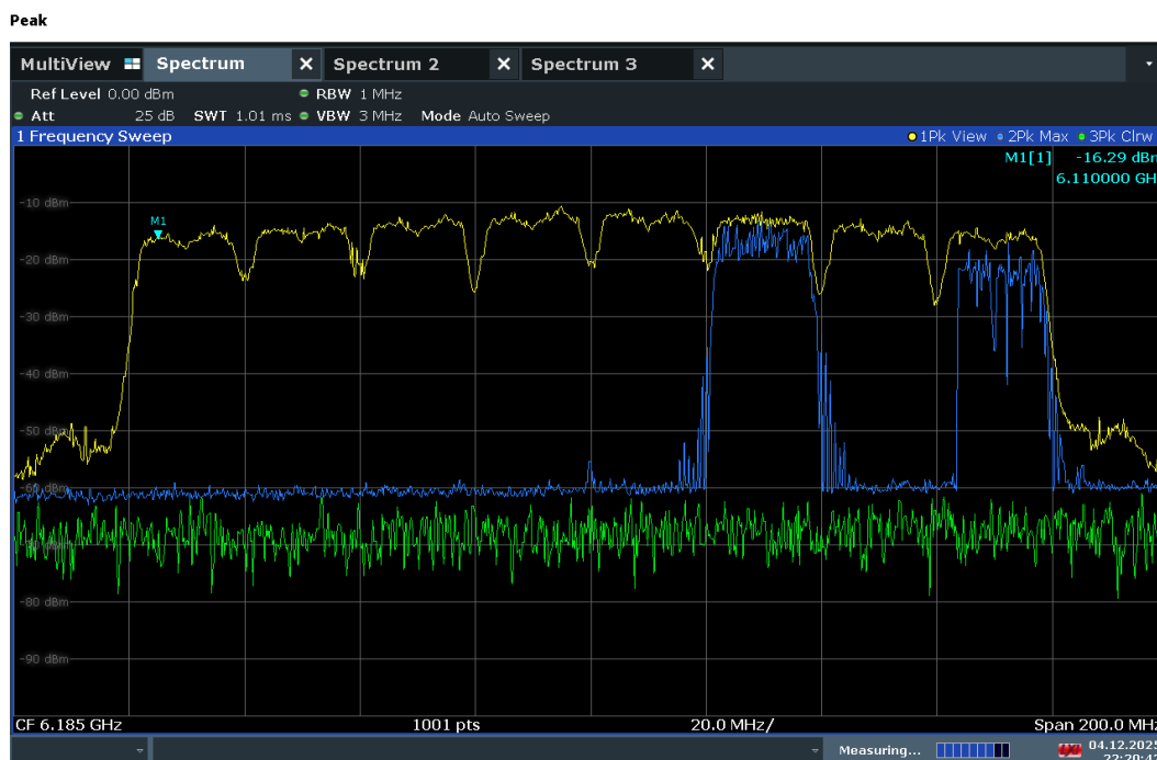
Plot 7-797. 160MHz Bandwidth, AWGN Signal Injected – 6110Mhz
