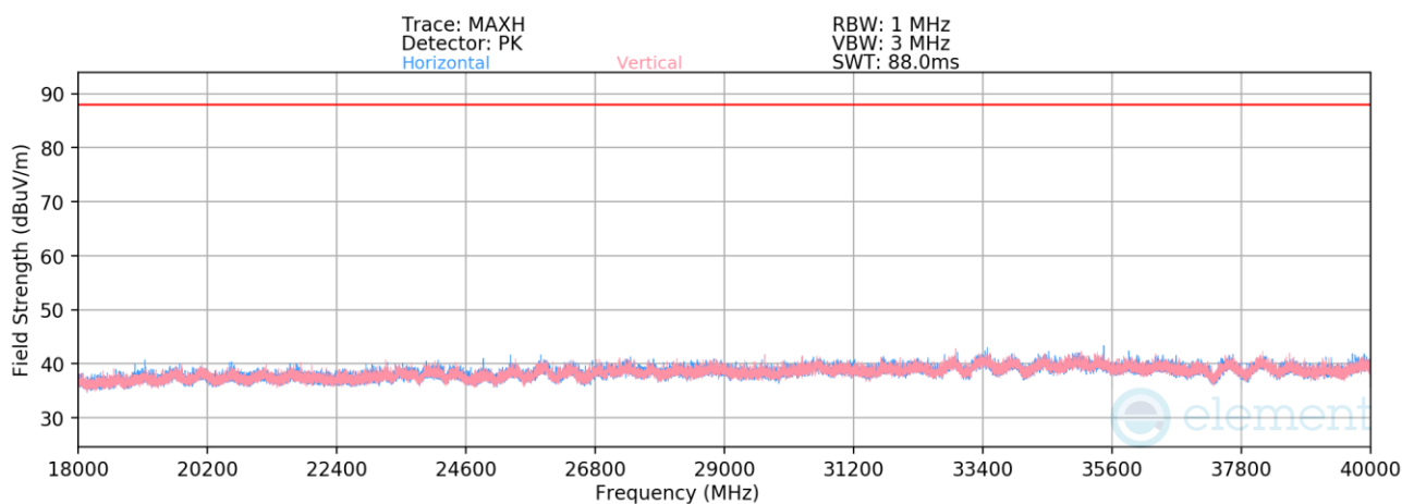
Plot 7-830. Radiated Spurious Emissions 18-40GHz SDM Primary (802.11be – Ch. 209 – RU242)
