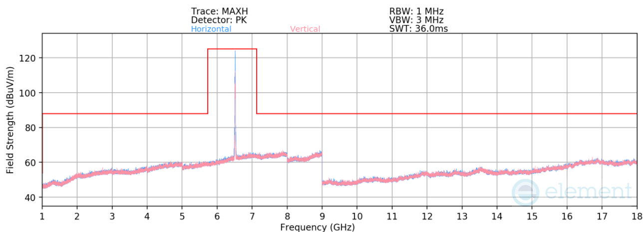
Plot 7-807. Radiated Spurious Emissions above 1GHz SDM Primary (802.11be – Ch. 113 – RU52)
