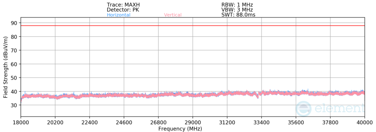
Plot 7-834. Radiated Spurious Emissions 18-40GHz SDM Diversity (802.11be – Ch. 61 – RU52)
