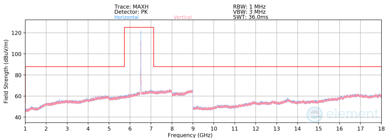
Plot 7-839. Radiated Spurious Emissions above 1GHz SDM Diversity (802.11be – Ch. 113 – RU52)
