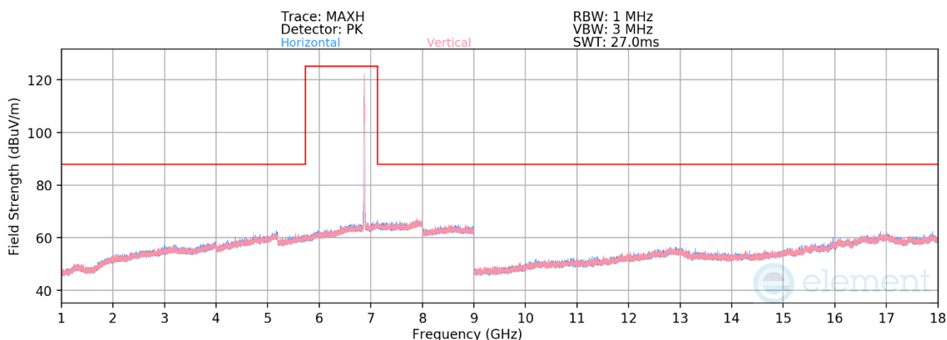
Plot 7-843. Radiated Spurious Emissions above 1GHz SDM Diversity (802.11be – Ch. 185 – RU52)
