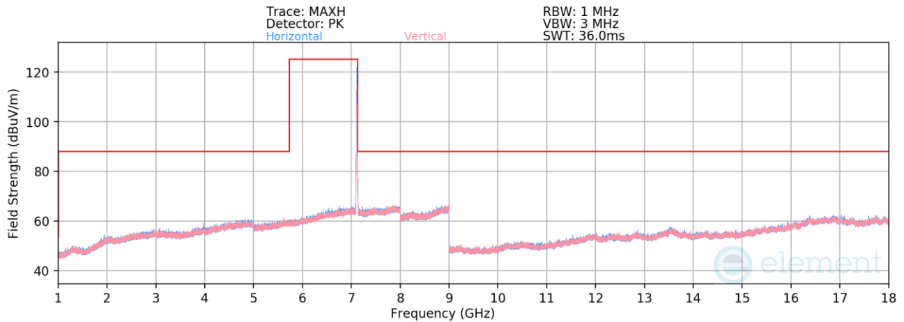
Plot 7-847. Radiated Spurious Emissions above 1GHz SDM Diversity (802.11be – Ch. 229 – RU52)
