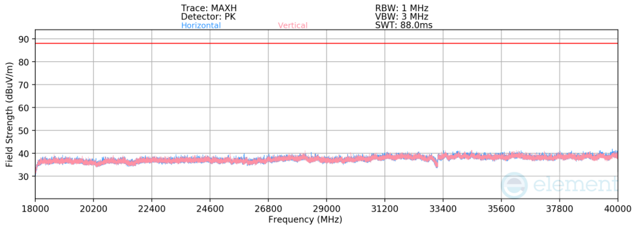
Plot 7-802. Radiated Spurious Emissions 18-40GHz SDM Primary (802.11be – Ch. 61 – RU52)
