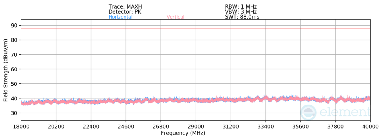
Plot 7-842. Radiated Spurious Emissions 18-40GHz SDM Diversity (802.11be – Ch. 149 – RU52)
