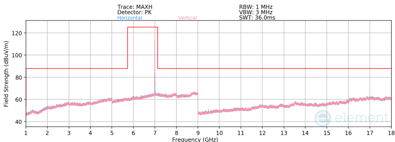
Plot 7-845. Radiated Spurious Emissions above 1GHz SDM Diversity (802.11be – Ch. 209 – RU52)
