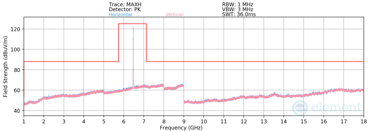
Plot 7-805. Radiated Spurious Emissions above 1GHz SDM Primary (802.11be – Ch. 105 – RU52)
