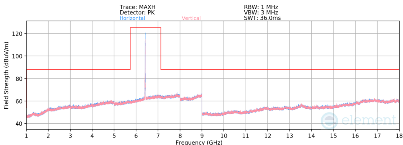
Plot 7-835. Radiated Spurious Emissions above 1GHz SDM Diversity (802.11be – Ch. 93 – RU52)
