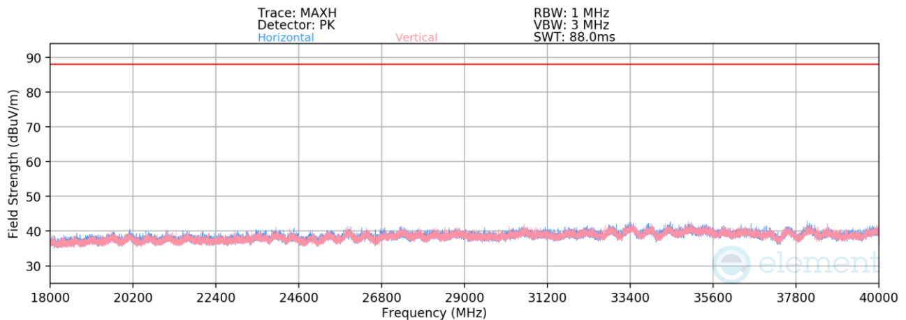
Plot 7-810. Radiated Spurious Emissions 18-40GHz SDM Primary (802.11be – Ch. 149 – RU52)
