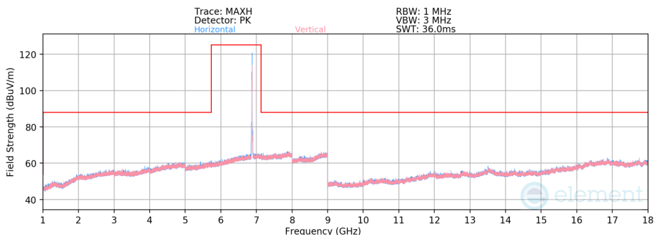
Plot 7-811. Radiated Spurious Emissions above 1GHz SDM Primary (802.11be – Ch. 185 – RU52)
