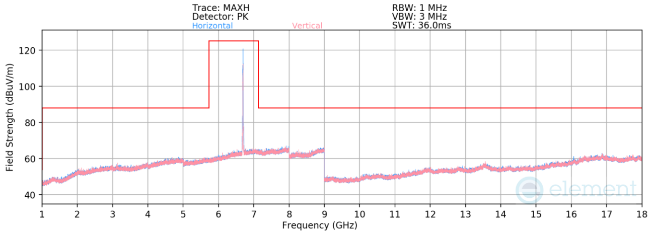
Plot 7-809. Radiated Spurious Emissions above 1GHz SDM Primary (802.11be – Ch. 149 – RU52)
