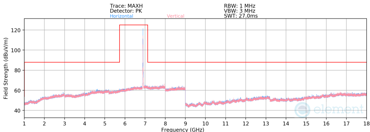
Plot 7-812. Radiated Spurious Emissions above 1GHz SDM Primary (802.11be – Ch. 189 – RU52)
