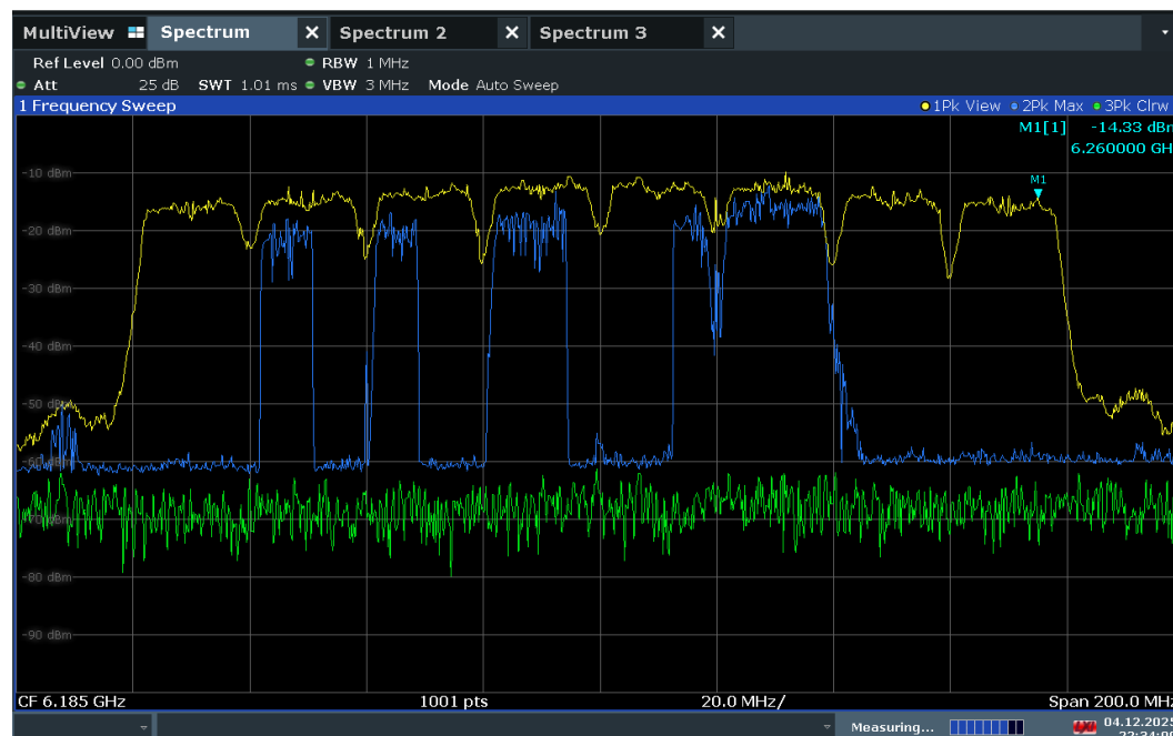
Plot 7-799. 160MHz Bandwidth, AWGN Signal Injected – 6260MHz
