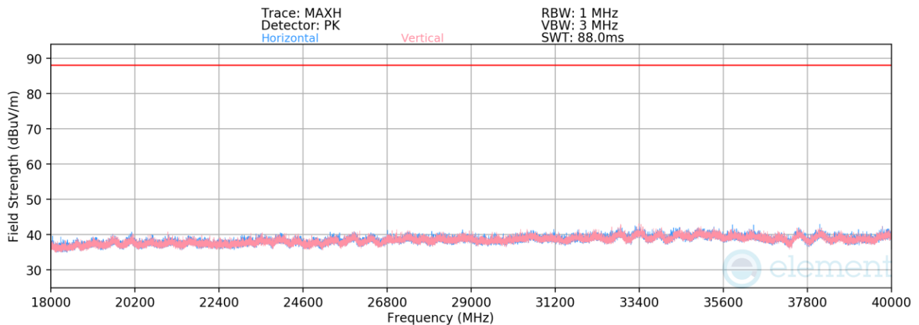
Plot 7-806. Radiated Spurious Emissions 18-40GHz SDM Primary (802.11be – Ch. 105 – RU52)
