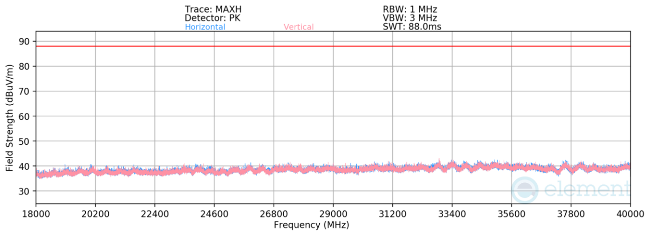
Plot 7-854. Radiated Spurious Emissions 18-40GHz SDM Diversity (802.11be – Ch. 105 – RU242)
