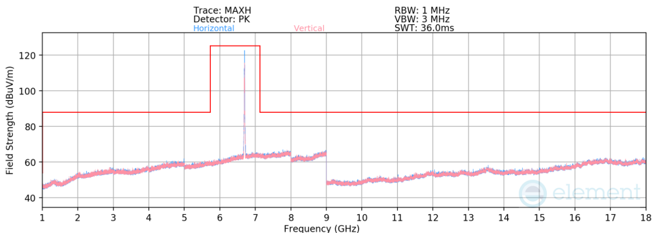
Plot 7-841. Radiated Spurious Emissions above 1GHz SDM Diversity (802.11be – Ch. 149 – RU52)
