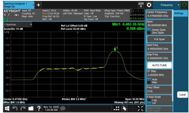
Plot 7-709 PSD CDD Diversity Antenna 1b (20MHz BW 802.11be(RU) RU26 Index8 - Ch.105)
