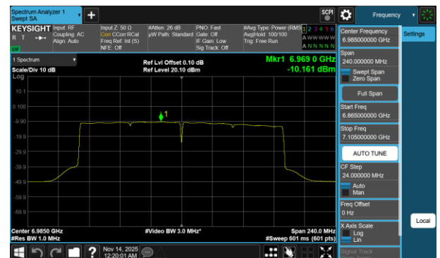
Plot 7-770 PSD CDD Diversity Antenna 1b (160MHz BW 802.11be(RU) RU996X2 Index68 - Ch.207)
