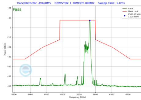
Plot 7-781 In-Band Emission Plot Antenna 5T (80MHz BW 802.11be(RU) RU26 Index36 (UNII Band 7) - Ch.119)
