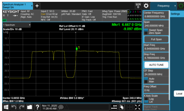
Plot 7-737 PSD CDD Diversity Antenna 5T (160MHz BW 802.11be(RU) RU996+484+242 Index99 - Ch.143)
