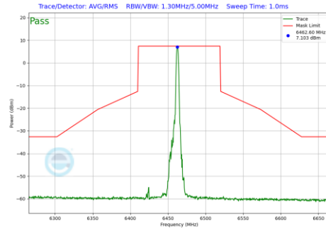
Plot 7-777 In-Band Emission Plot Antenna 5T (80MHz BW 802.11be(RU) RU26 Index17 (UNII Band 6) - Ch.103)
