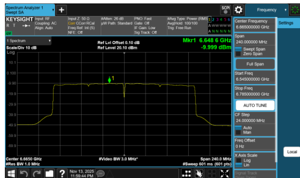
Plot 7-748 PSD CDD Diversity Antenna 1b (160MHz BW 802.11be(RU) RU996X2 Index68 - Ch.143)
