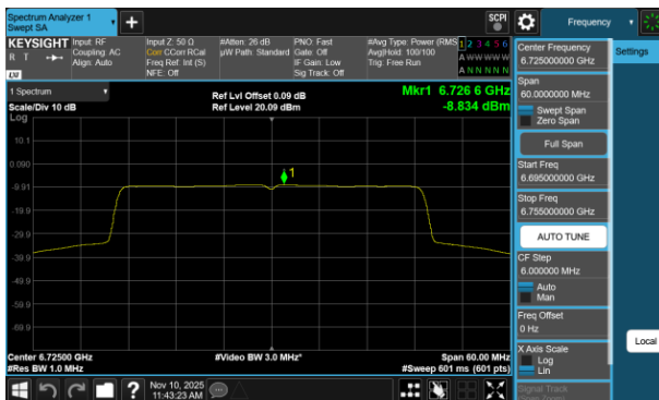
Plot 7-742 PSD CDD Diversity Antenna 5T (40MHz BW 802.11be(RU) RU484 Index65 - Ch.155)
