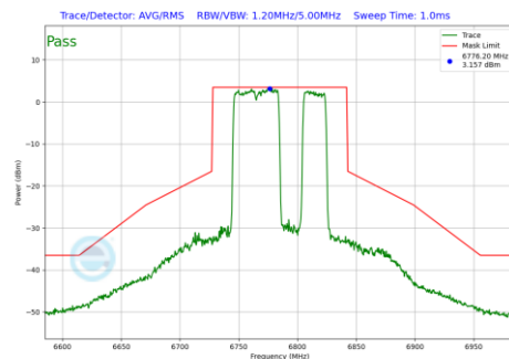
Plot 7-790 In-Band Emission Plot Antenna 5T (80MHz BW 802.11be(RU) RU484+242 Index92 (UNII Band 7) - Ch.167)
