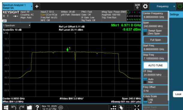
Plot 7-766 PSD CDD Diversity Antenna 5T (160MHz BW 802.11be(RU) RU996X2 Index68 - Ch.207)
