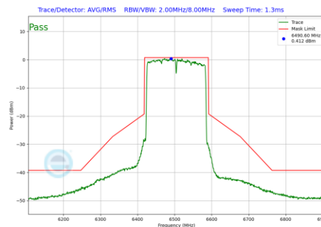
Plot 7-799 In-Band Emission Plot Antenna 5T (160MHz BW 802.11be(RU) RU996X2 Index68 (UNII Band 6) - Ch.111)
