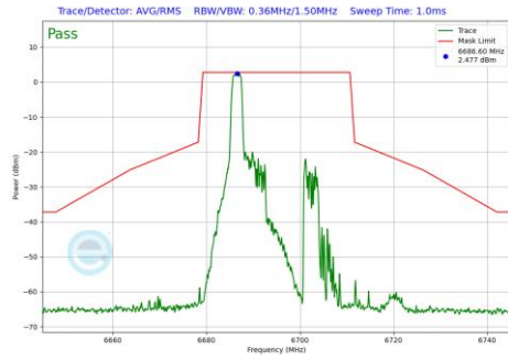
Plot 7-779 In-Band Emission Plot Antenna 5T (20MHz BW 802.11be(RU) RU26 Index0 (UNII Band 7) - Ch.149)
