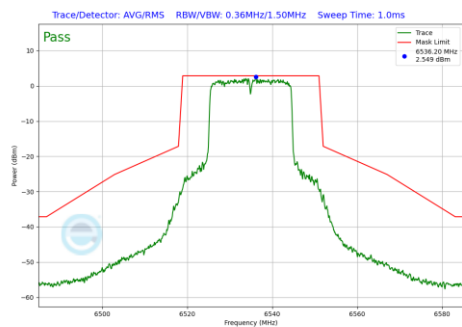
Plot 7-800 In-Band Emission Plot Antenna 5T (20MHz BW 802.11be(RU) RU242 Index61 (UNII Band 7) - Ch.117)
