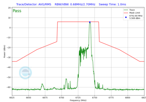
Plot 7-780 In-Band Emission Plot Antenna 5T (40MHz BW 802.11be(RU) RU26 Index17 (UNII Band 7) - Ch.155)
