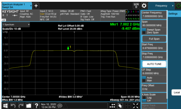
Plot 7-764 PSD CDD Diversity Antenna 5T (40MHz BW 802.11be(RU) RU484 Index65 - Ch.211)
