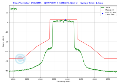
Plot 7-794 In-Band Emission Plot Antenna 5T (80MHz BW 802.11be(RU) RU996 Index67 (UNII Band 5) - Ch.87)
