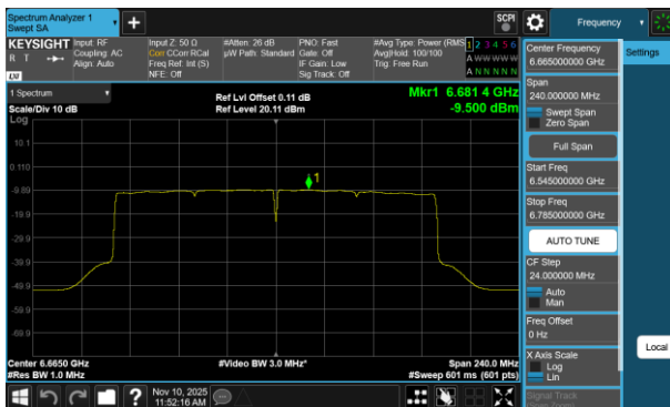
Plot 7-744 PSD CDD Diversity Antenna 5T (160MHz BW 802.11be(RU) RU996X2 Index68 - Ch.143)
