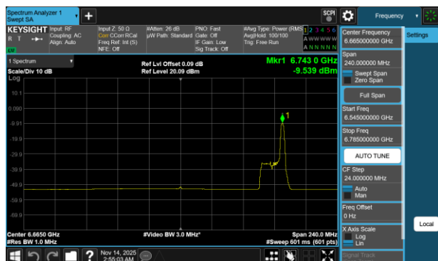
Plot 7-734 PSD CDD Diversity Antenna 1b (160MHz BW 802.11be(RU) RU26 Index36 - Ch.143)
