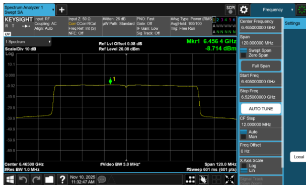
Plot 7-721 PSD CDD Diversity Antenna 5T (80MHz BW 802.11be(RU) RU996 Index67 - Ch.103)
