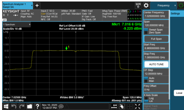
Plot 7-765 PSD CDD Diversity Antenna 5T (80MHz BW 802.11be(RU) RU996 Index67 - Ch.215)
