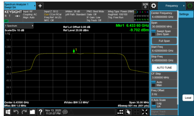
Plot 7-723 PSD CDD Diversity Antenna 1b (20MHz BW 802.11be(RU) RU242 Index61 - Ch.97)
