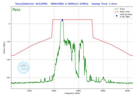
Plot 7-771 In-Band Emission Plot Antenna 5T (20MHz BW 802.11be(RU) RU26 Index0 (UNII Band 5) - Ch.1)
