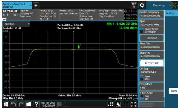
Plot 7-119 PSD CDD Diversity Antenna 5T (20MHz BW 802.11be(RU) RU242 Index61 - Ch.97)
