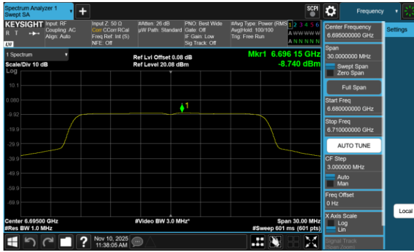
Plot 7-741 PSD CDD Diversity Antenna 5T (20MHz BW 802.11be(RU) RU242 Index61 - Ch.149)
