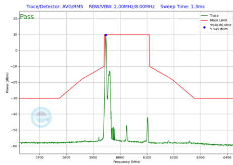
Plot 7-774 In-Band Emission Plot Antenna 5T (160MHz BW 802.11be(RU) RU26 Index0 (UNII Band 5) - Ch.15)
