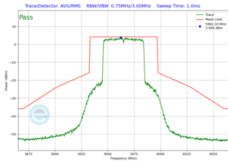
Plot 7-793 In-Band Emission Plot Antenna 5T (40MHz BW 802.11be(RU) RU484 Index65 (UNII Band 5) - Ch.3)
