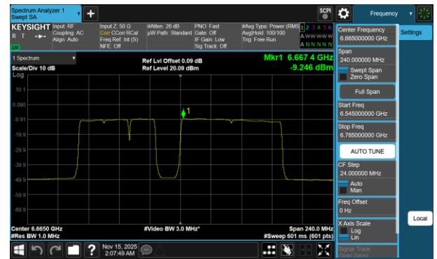
Plot 7-740 PSD CDD Diversity Antenna 1b (160MHz BW 802.11be(RU) RU996+484+242 Index99 - Ch.143)
