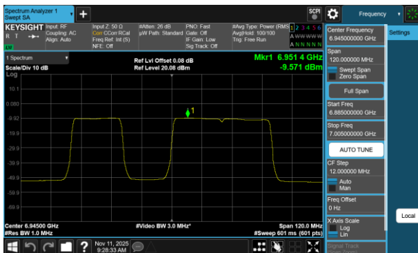
Plot 7-758 PSD CDD Diversity Antenna 5T (80MHz BW 802.11be(RU) RU484+242 Index91 - Ch.199)
