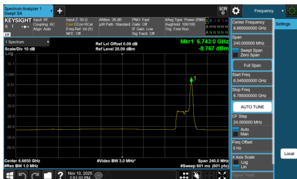
Plot 7-730 PSD CDD Diversity Antenna 5T (160MHz BW 802.11be(RU) RU26 Index36 - Ch.143)
