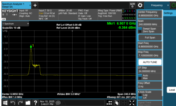
Plot 7-752 PSD CDD Diversity Antenna 5T (160MHz BW 802.11be(RU) RU26 Index0 - Ch.207)
