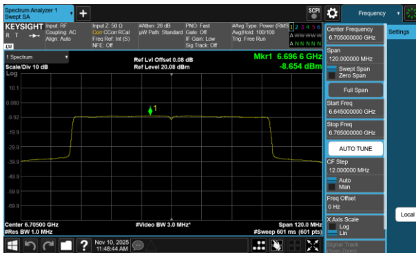
Plot 7-743 PSD CDD Diversity Antenna 5T (80MHz BW 802.11be(RU) RU996 Index67 - Ch.151)
