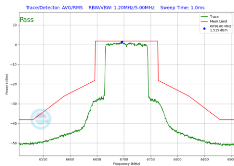
Plot 7-802 In-Band Emission Plot Antenna 5T (80MHz BW 802.11be(RU) RU996 Index67 (UNII Band 7) - Ch.151)
