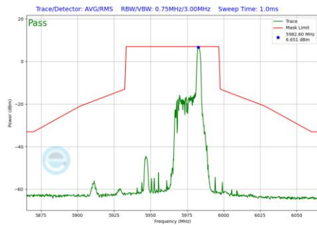
Plot 7-772 In-Band Emission Plot Antenna 5T (40MHz BW 802.11be(RU) RU26 Index17 (UNII Band 5) - Ch.3)
