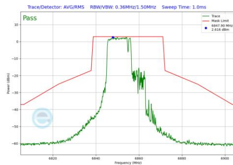
Plot 7-789 In-Band Emission Plot Antenna 5T (20MHz BW 802.11be(RU) RU106+26 Index82 (UNII Band 7) - Ch.181)
