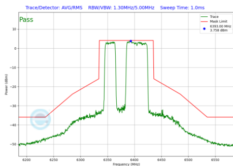
Plot 7-784 In-Band Emission Plot Antenna 5T (80MHz BW 802.11be(RU) RU484+242 Index91 (UNII Band 5) - Ch.87)
