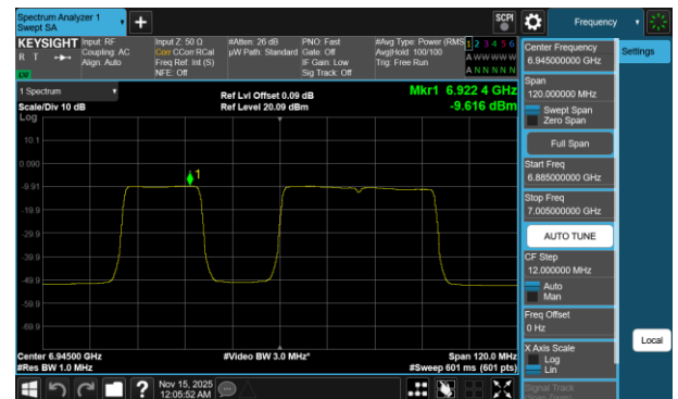
Plot 7-761 PSD CDD Diversity Antenna 1b (80MHz BW 802.11be(RU) RU484+242 Index91 - Ch.199)
