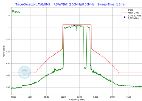
Plot 7-785 In-Band Emission Plot Antenna 5T (160MHz BW 802.11be(RU) RU996+484+242 Index98 (UNII Band 5) - Ch.47)
