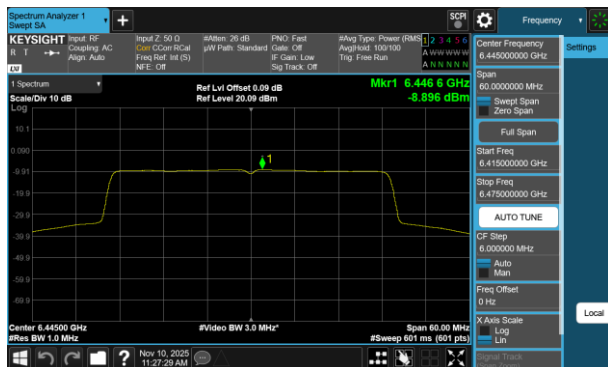
Plot 7-720 PSD CDD Diversity Antenna 5T (40MHz BW 802.11be(RU) RU484 Index65 - Ch.99)
