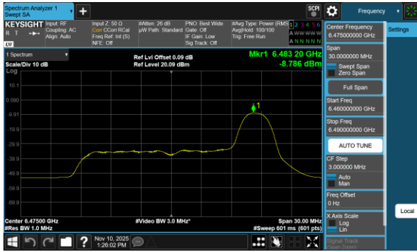
Plot 7-705 PSD CDD Diversity Antenna 5T (20MHz BW 802.11be(RU) RU26 Index8 - Ch.105)
