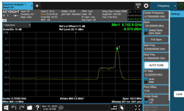
Plot 7-729 PSD CDD Diversity Antenna 5T (80MHz BW 802.11be(RU) RU26 Index36 - Ch.151)
