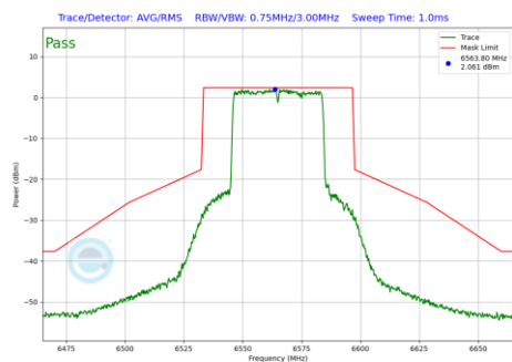
Plot 7-801 In-Band Emission Plot Antenna 5T (40MHz BW 802.11be(RU) RU484 Index65 (UNII Band 7) - Ch.123)
