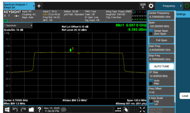
Plot 7-747 PSD CDD Diversity Antenna 1b (80MHz BW 802.11be(RU) RU996 Index67 - Ch.151)
