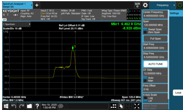
Plot 7-707 PSD CDD Diversity Antenna 5T (80MHz BW 802.11be(RU) RU26 Index17 - Ch.103)
