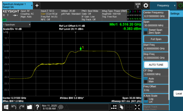
Plot 7-713 PSD CDD Diversity Antenna 5T (20MHz BW 802.11be(RU) RU106+26 Index83 - Ch.113)
