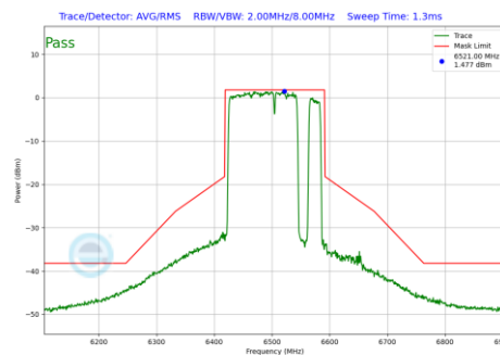
Plot 7-788 In-Band Emission Plot Antenna 5T (160MHz BW 802.11be(RU) RU996+484+242 Index98 (UNII Band 6) - Ch.111)
