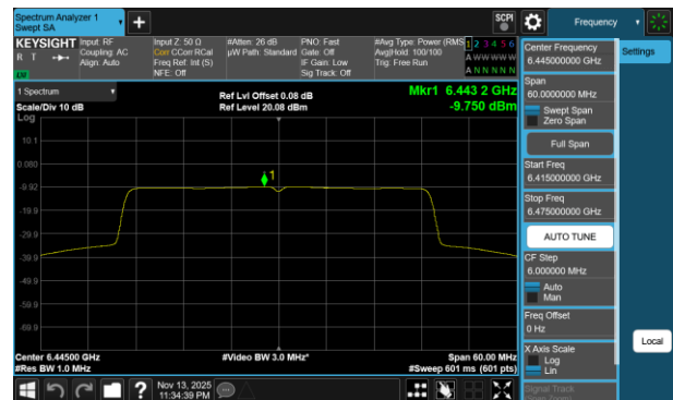
Plot 7-724 PSD CDD Diversity Antenna 1b (40MHz BW 802.11be(RU) RU484 Index65 - Ch.99)
