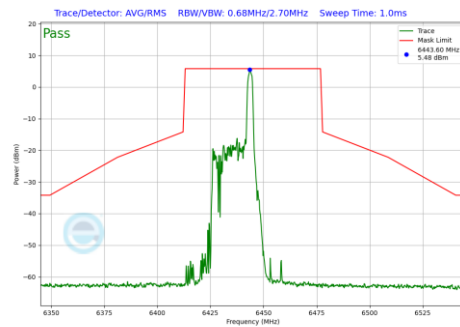
Plot 7-776 In-Band Emission Plot Antenna 5T (40MHz BW 802.11be(RU) RU26 Index8 (UNII Band 6) - Ch.99)
