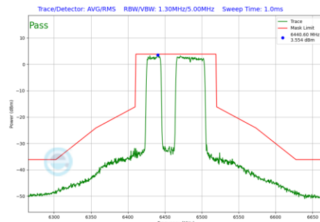
Plot 7-787 In-Band Emission Plot Antenna 5T (80MHz BW 802.11be(RU) RU484+242 Index91 (UNII Band 6) - Ch.103)
