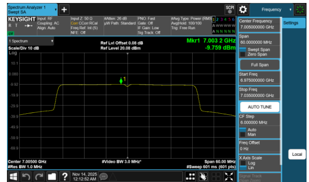
Plot 7-768 PSD CDD Diversity Antenna 1b (40MHz BW 802.11be(RU) RU484 Index65 - Ch.211)
