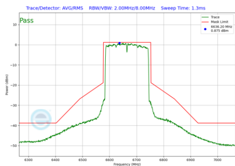
Plot 7-803 In-Band Emission Plot Antenna 5T (160MHz BW 802.11be(RU) RU996X2 Index68 (UNII Band 7) - Ch.143)
