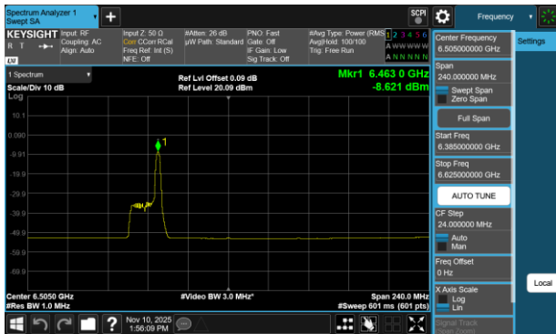
Plot 7-708 PSD CDD Diversity Antenna 5T (160MHz BW 802.11be(RU) RU26 Index17 - Ch.111)
