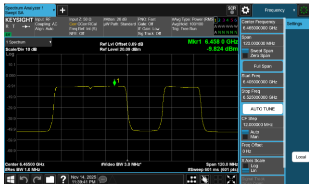
Plot 7-717 PSD CDD Diversity Antenna 1b (80MHz BW 802.11be(RU) RU484+242 Index92 - Ch.103)
