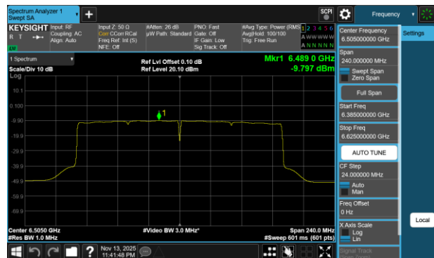
Plot 7-726 PSD CDD Diversity Antenna 1b (160MHz BW 802.11be(RU) RU996X2 Index68 - Ch.111)
