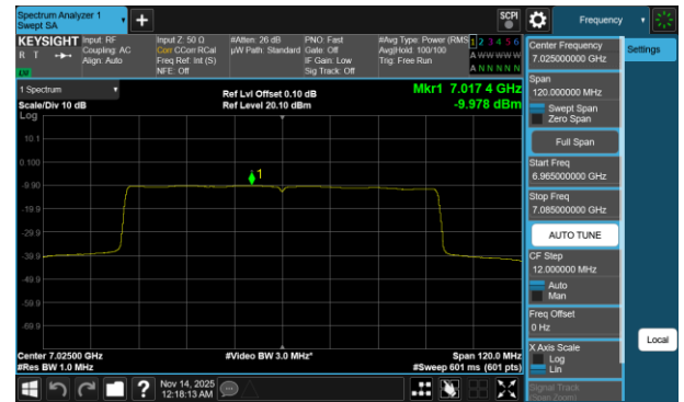
Plot 7-769 PSD CDD Diversity Antenna 1b (80MHz BW 802.11be(RU) RU996 Index67 - Ch.215)
