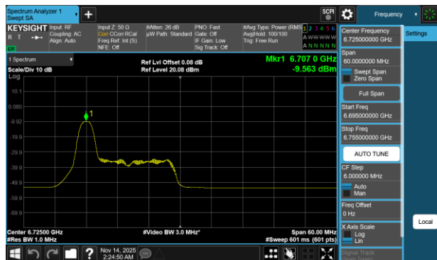
Plot 7-732 PSD CDD Diversity Antenna 1b (40MHz BW 802.11be(RU) RU26 Index0 - Ch.155)
