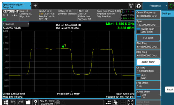
Plot 7-714 PSD CDD Diversity Antenna 5T (80MHz BW 802.11be(RU) RU484+242 Index92 - Ch.103)
