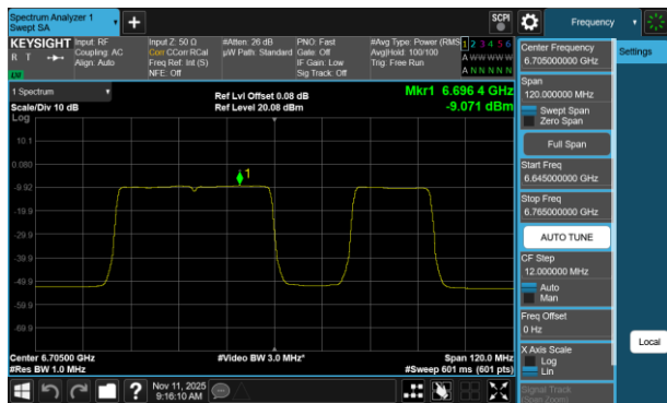
Plot 7-736 PSD CDD Diversity Antenna 5T (80MHz BW 802.11be(RU) RU484+242 Index92 - Ch.151)
