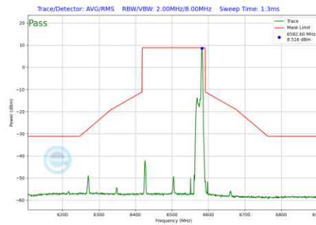
Plot 7-778 In-Band Emission Plot Antenna 5T (160MHz BW 802.11be(RU) RU26 Index36 (UNII Band 6) - Ch.111)
