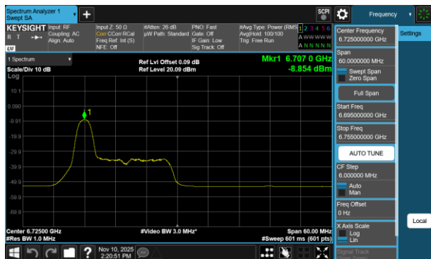
Plot 7-728 PSD CDD Diversity Antenna 5T (40MHz BW 802.11be(RU) RU26 Index0 - Ch.155)
