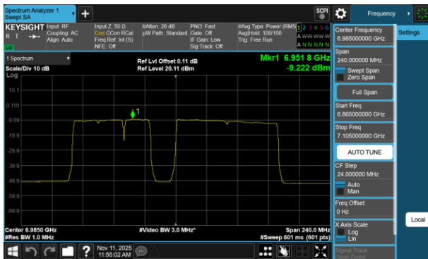
Plot 7-759 PSD CDD Diversity Antenna 5T (160MHz BW 802.11be(RU) RU996+484+242 Index99 - Ch.207)
