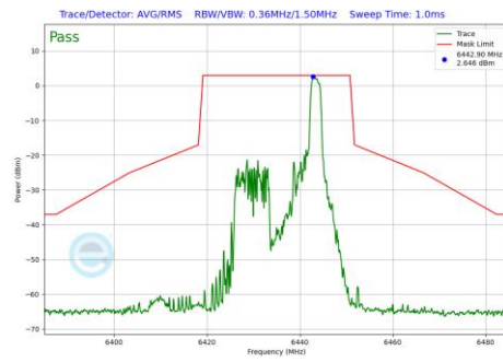
Plot 7-775 In-Band Emission Plot Antenna 5T (20MHz BW 802.11be(RU) RU26 Index8 (UNII Band 6) - Ch.97)
