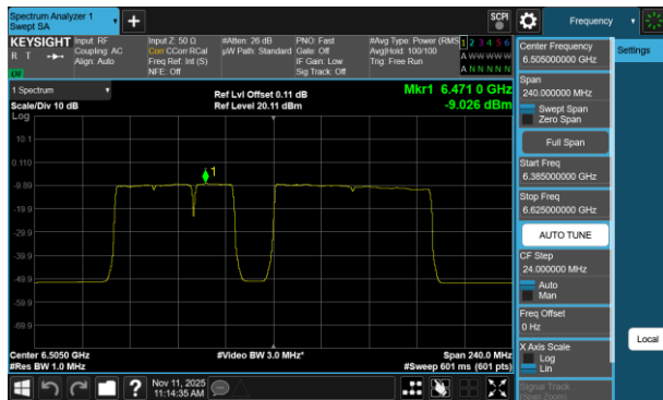
Plot 7-715 PSD CDD Diversity Antenna 5T (160MHz BW 802.11be(RU) RU996+484+242 Index99 - Ch.111)
