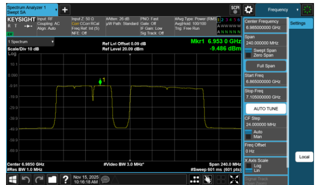
Plot 7-762 PSD CDD Diversity Antenna 1b (160MHz BW 802.11be(RU) RU996+484+242 Index99 - Ch.207)
