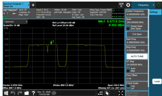
Plot 7-718 PSD CDD Diversity Antenna 1b (160MHz BW 802.11be(RU) RU996+484+242 Index99 - Ch.111)
