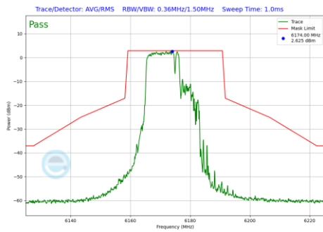
Plot 7-783 In-Band Emission Plot Antenna 5T (20MHz BW 802.11be(RU) RU106+26 Index82 (UNII Band 5) - Ch.45)
