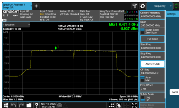
Plot 7-722 PSD CDD Diversity Antenna 5T (160MHz BW 802.11be(RU) RU996X2 Index68 - Ch.111)
