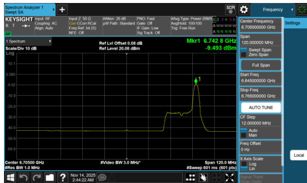
Plot 7-733 PSD CDD Diversity Antenna 1b (80MHz BW 802.11be(RU) RU26 Index36 - Ch.151)
