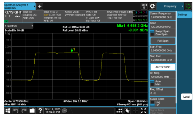
Plot 7-739 PSD CDD Diversity Antenna 1b (80MHz BW 802.11be(RU) RU484+242 Index92 - Ch.151)
