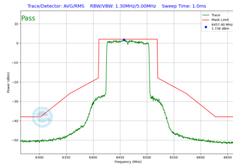
Plot 7-798 In-Band Emission Plot Antenna 5T (80MHz BW 802.11be(RU) RU996 Index67 (UNII Band 6) - Ch.103)
