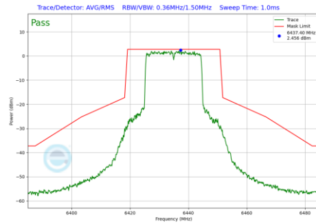
Plot 7-796 In-Band Emission Plot Antenna 5T (20MHz BW 802.11be(RU) RU242 Index61 (UNII Band 6) - Ch.97)
