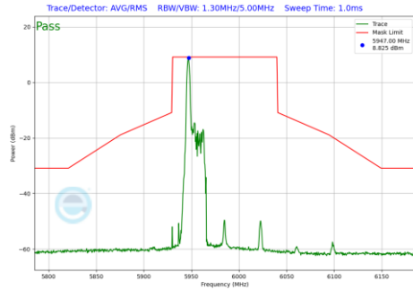
Plot 7-773 In-Band Emission Plot Antenna 5T (80MHz BW 802.11be(RU) RU26 Index0 (UNII Band 5) - Ch.7)
