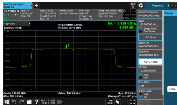
Plot 7-725 PSD CDD Diversity Antenna 1b (80MHz BW 802.11be(RU) RU996 Index67 - Ch.103)
