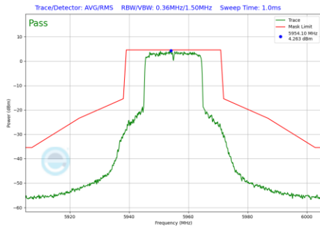
Plot 7-792 In-Band Emission Plot Antenna 5T (20MHz BW 802.11be(RU) RU242 Index61 (UNII Band 5) - Ch.1)
