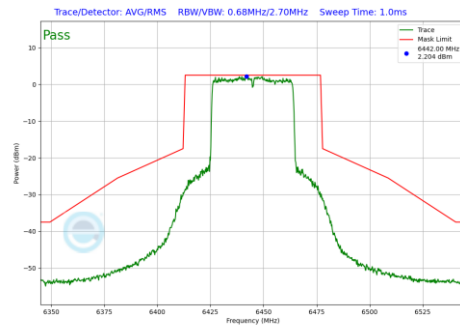
Plot 7-797 In-Band Emission Plot Antenna 5T (40MHz BW 802.11be(RU) RU484 Index65 (UNII Band 6) - Ch.99)
