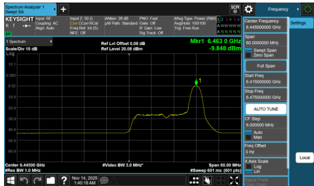
Plot 7-710 PSD CDD Diversity Antenna 1b (40MHz BW 802.11be(RU) RU26 Index17 - Ch.99)
