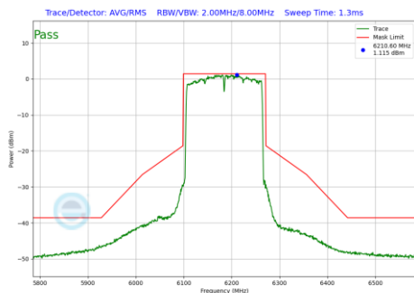
Plot 7-795 In-Band Emission Plot Antenna 5T (160MHz BW 802.11be(RU) RU996X2 Index68 (UNII Band 5) - Ch.47)
