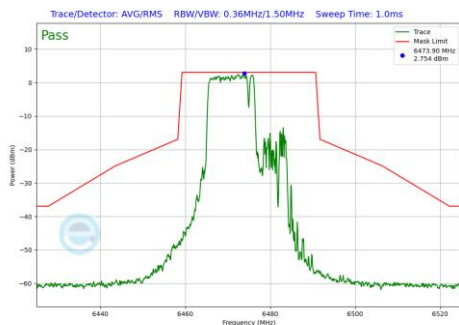
Plot 7-786 In-Band Emission Plot Antenna 5T (20MHz BW 802.11be(RU) RU106+26 Index82 (UNII Band 6) - Ch.105)
