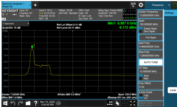
Plot 7-751 PSD CDD Diversity Antenna 5T (80MHz BW 802.11be(RU) RU26 Index0 - Ch.215)
