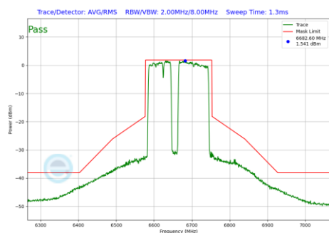
Plot 7-791 In-Band Emission Plot Antenna 5T (160MHz BW 802.11be(RU) RU996+484+242 Index99 (UNII Band 7) - Ch.143)
