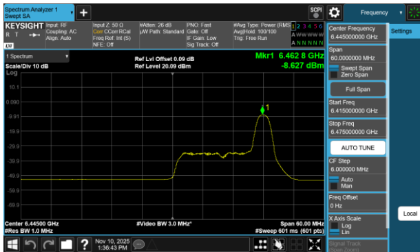
Plot 7-706 PSD CDD Diversity Antenna 5T (40MHz BW 802.11be(RU) RU26 Index17 - Ch.99)
