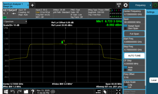
Plot 7-746 PSD CDD Diversity Antenna 1b (40MHz BW 802.11be(RU) RU484 Index65 - Ch.155)
