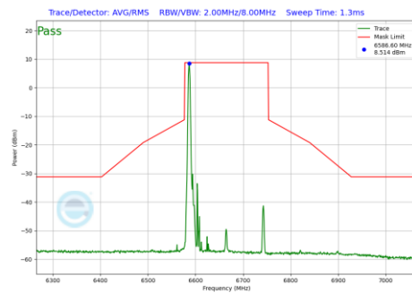
Plot 7-782 In-Band Emission Plot Antenna 5T (160MHz BW 802.11be(RU) RU26 Index0 (UNII Band 7) - Ch.143)
