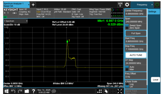
Plot 7-756 PSD CDD Diversity Antenna 1b (160MHz BW 802.11be(RU) RU26 Index0 - Ch.207)
