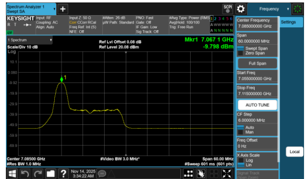
Plot 7-754 PSD CDD Diversity Antenna 1b (40MHz BW 802.11be(RU) RU26 Index0 - Ch.227)
