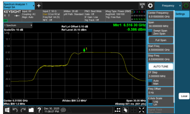
Plot 7-716 PSD CDD Diversity Antenna 1b (20MHz BW 802.11be(RU) RU106+26 Index83 - Ch.113)
