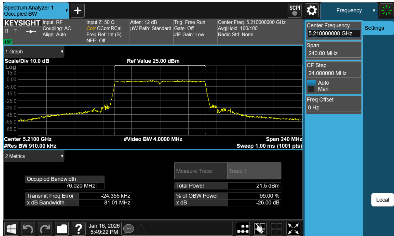
Plot 7-3 26dB BW & 99% OBW Antenna 5T (80MHz BW 802.11ac - Ch.42)
