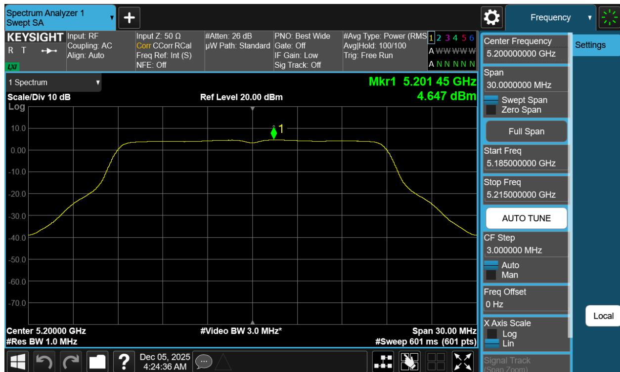
Plot 7-40 PSD Antenna 3b (20MHz BW 802.11n - Ch.40)
