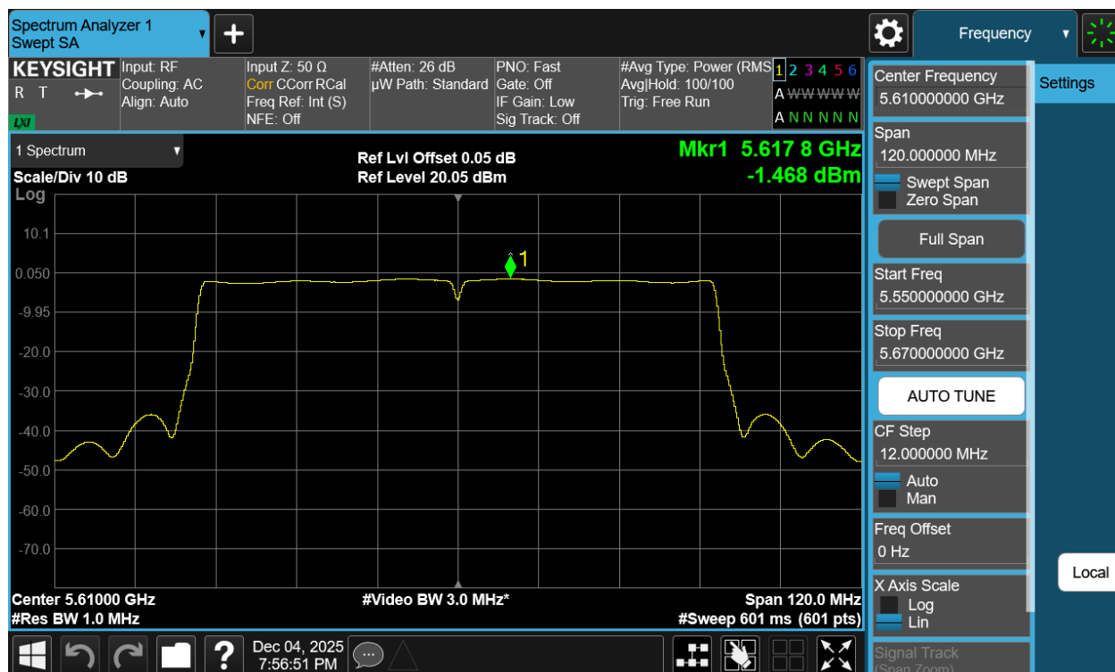
Plot 7-35 PSD Antenna 3b (80MHz BW 802.11ac - Ch.122)
