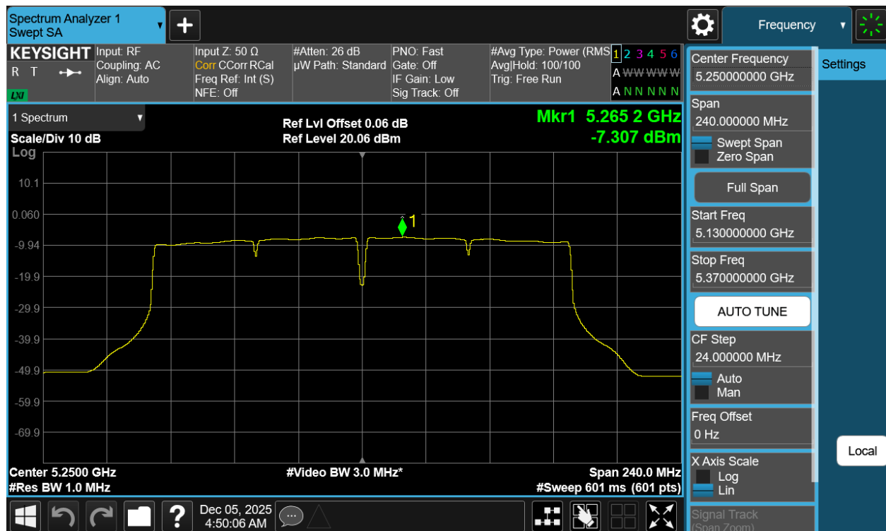
Plot 7-43 PSD Antenna 3b (160MHz BW 802.11ac - Ch.50)
