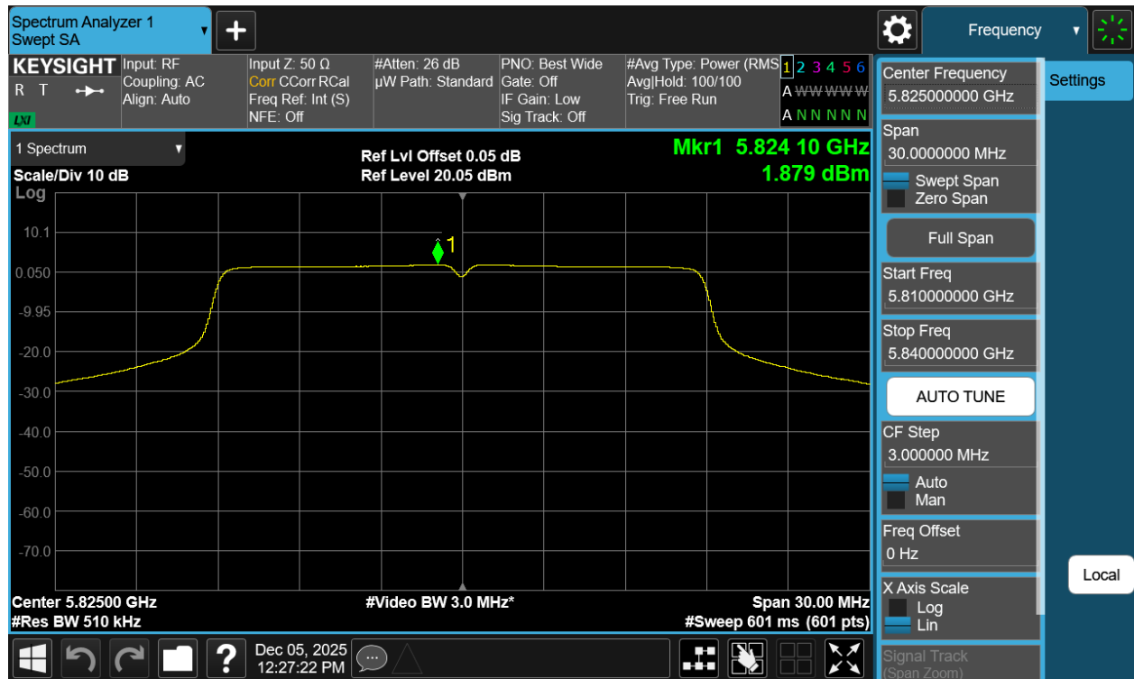
Plot 7-48 PSD Antenna 1b (20MHz BW 802.11a - Ch.165)
