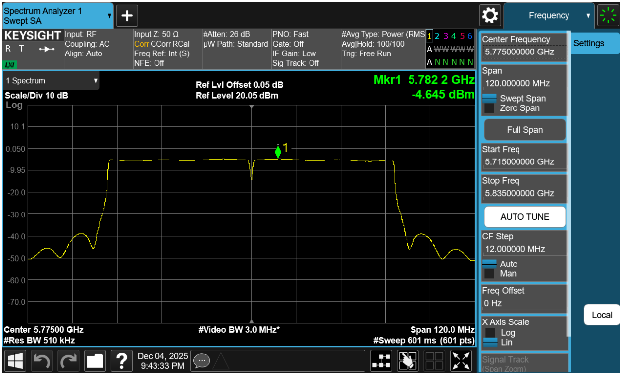
Plot 7-39 PSD Antenna 3b (80MHz BW 802.11ac - Ch.155)
