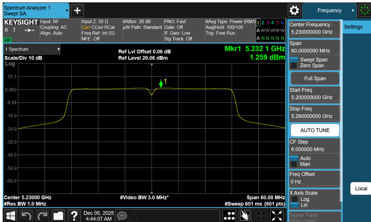
Plot 7-41 PSD Antenna 3b (40MHz BW 802.11n - Ch.46)
