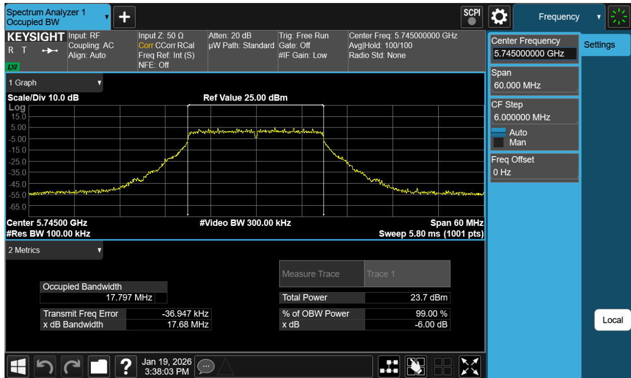
Plot 7-19 6dB OBW Antenna 1b (20MHz BW 802.11a - Ch.149)
