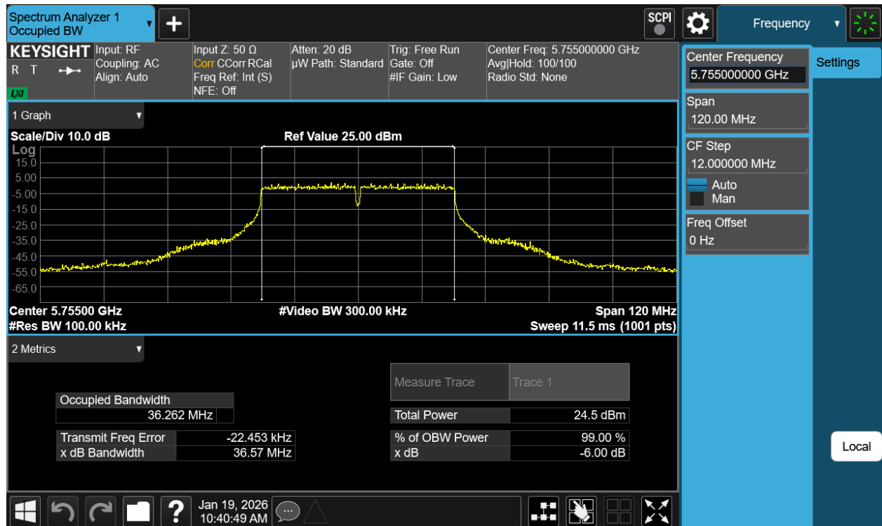
Plot 7-17 6dB OBW Antenna 3b (40MHz BW 802.11n - Ch.151)
