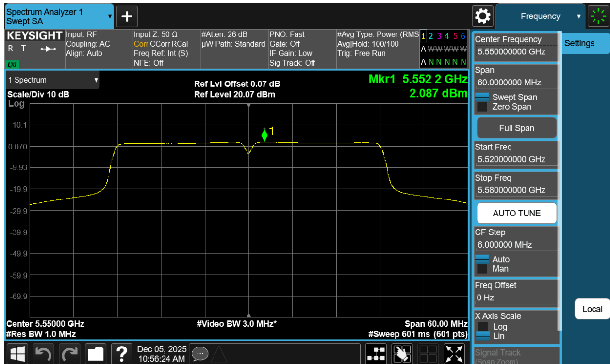
Plot 7-45 PSD Antenna 1b (40MHz BW 802.11n - Ch.110)
