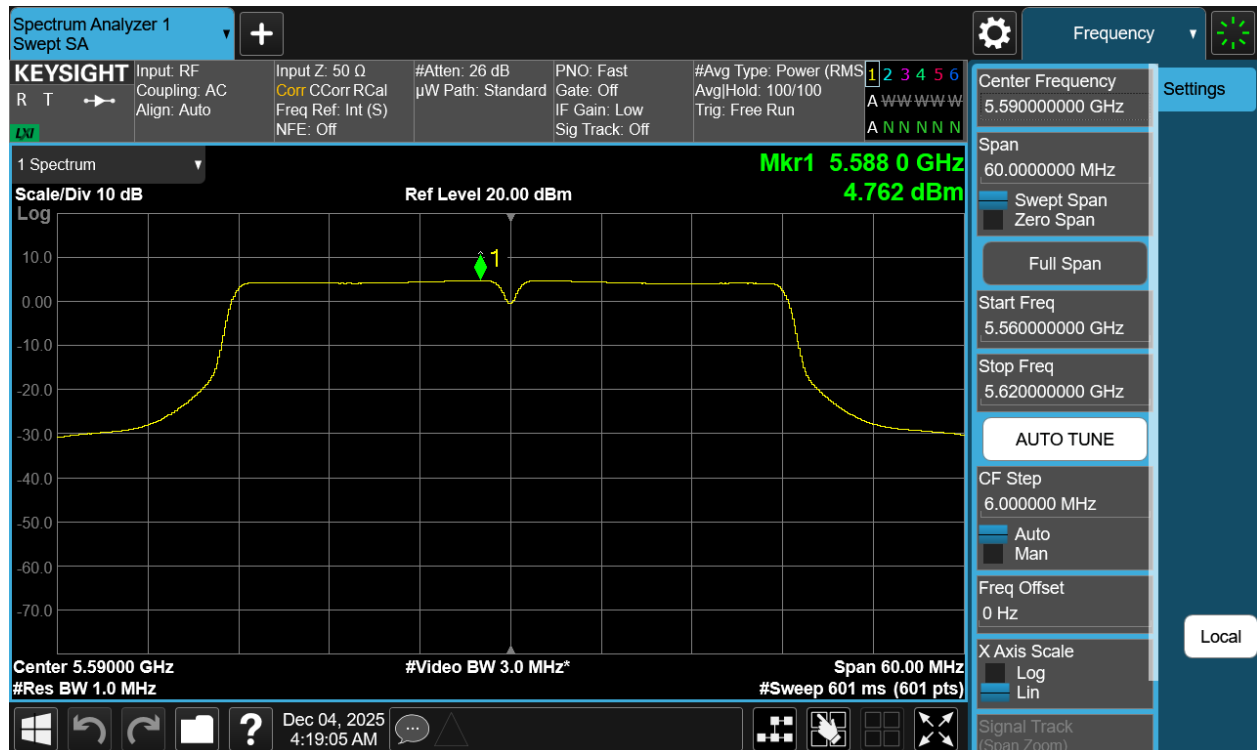
Plot 7-23 PSD Antenna 5T (40MHz BW 802.11n - Ch.118)
