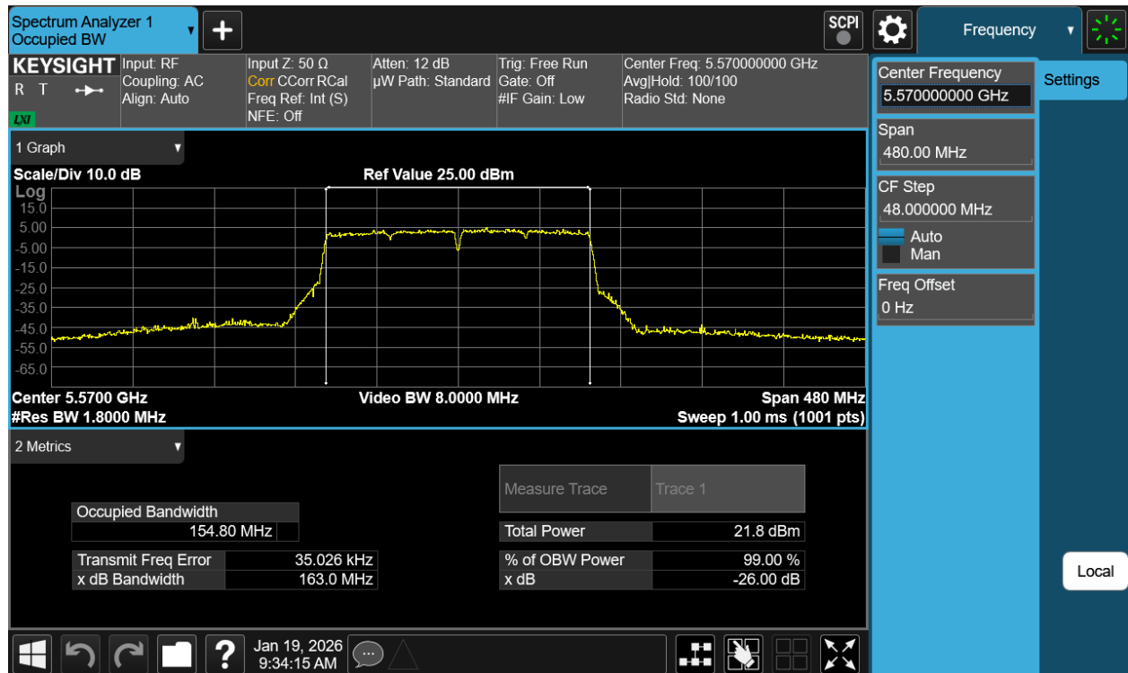
Plot 7-8 26dB BW & 99% OBW Antenna 3b (160MHz BW 802.11ac - Ch.114)
