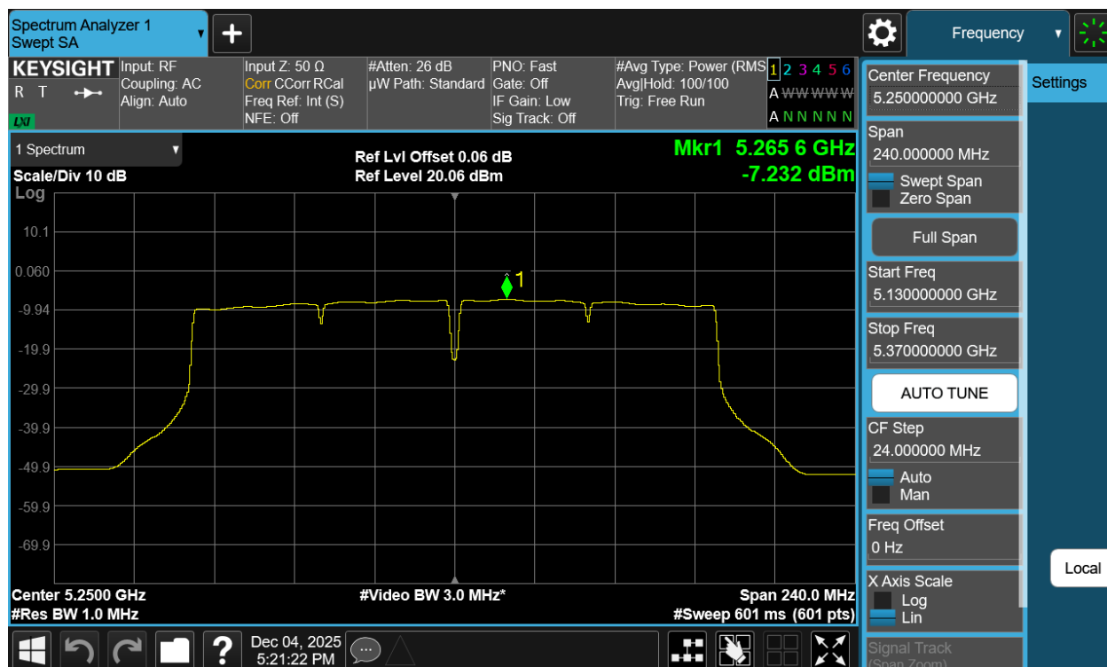
Plot 7-36 PSD Antenna 3b (160MHz BW 802.11ac - Ch.50)
