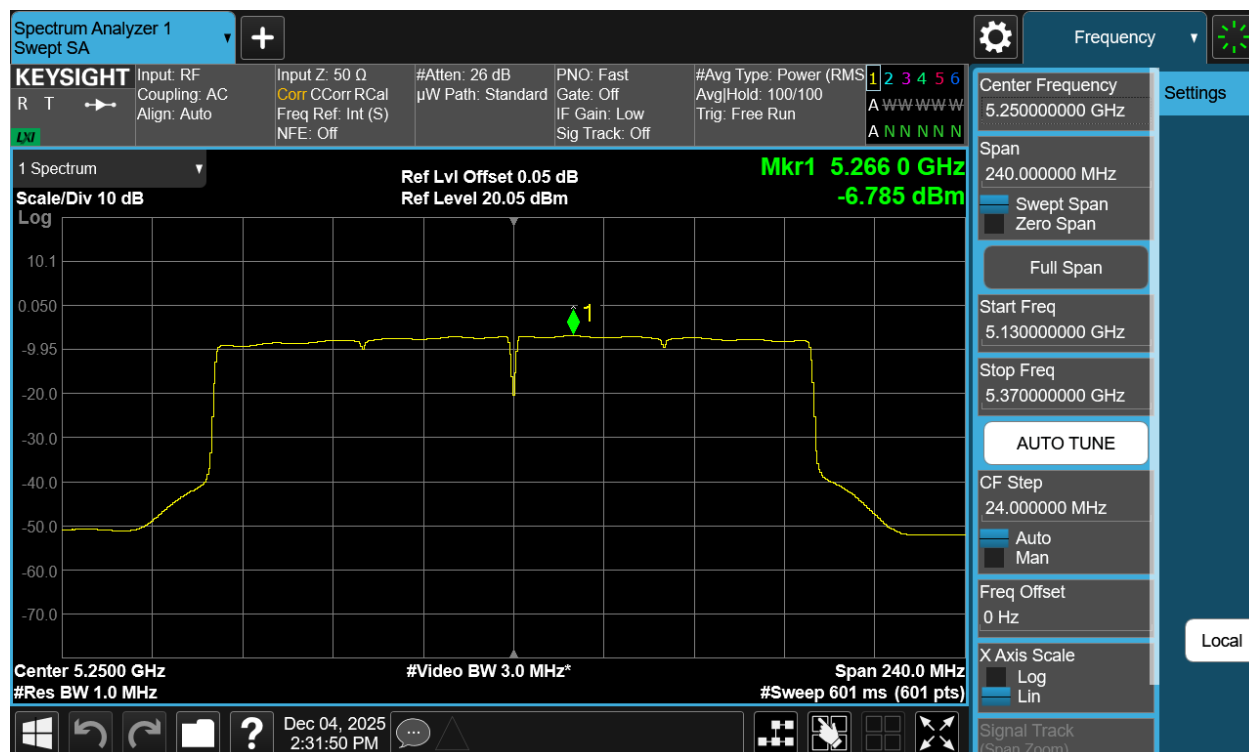
Plot 7-32 PSD Antenna 5T (160MHz BW 802.11be(SU) - Ch.50)
