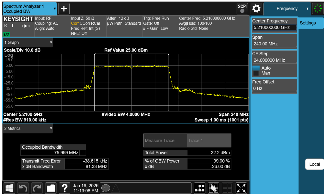
Plot 7-7 26dB BW & 99% OBW Antenna 3b (80MHz BW 802.11ac - Ch.42)
