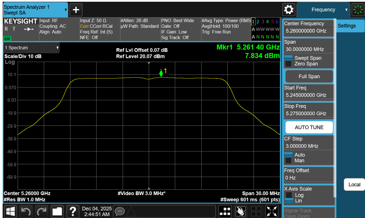
Plot 7-22 PSD Antenna 5T (20MHz BW 802.11n - Ch.52)
