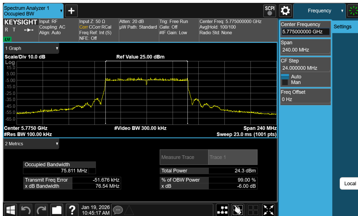
Plot 7-18 6dB OBW Antenna 3b (80MHz BW 802.11ac - Ch.155)
