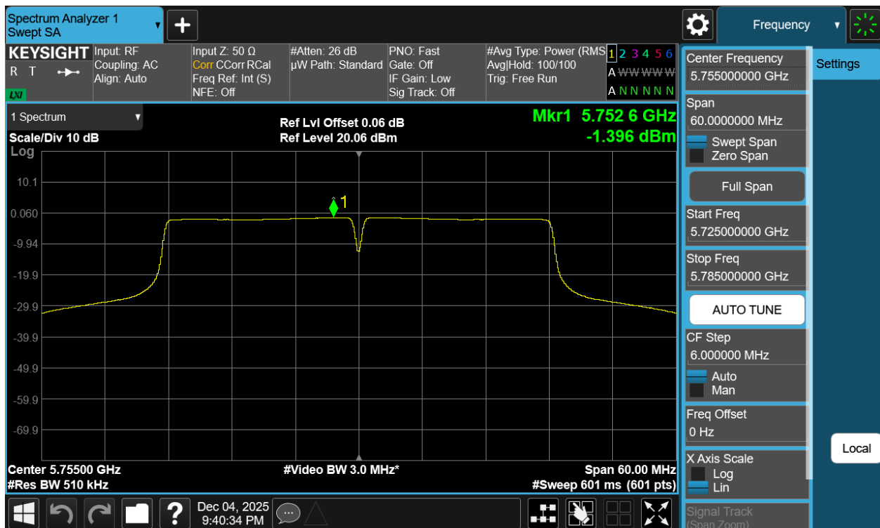
Plot 7-38 PSD Antenna 3b (40MHz BW 802.11n - Ch.151)
