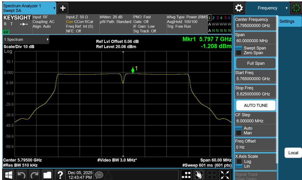
Plot 7-49 PSD Antenna 1b (40MHz BW 802.11n - Ch.159)
