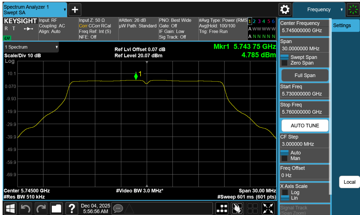
Plot 7-26 PSD Antenna 5T (20MHz BW 802.11n - Ch.149)
