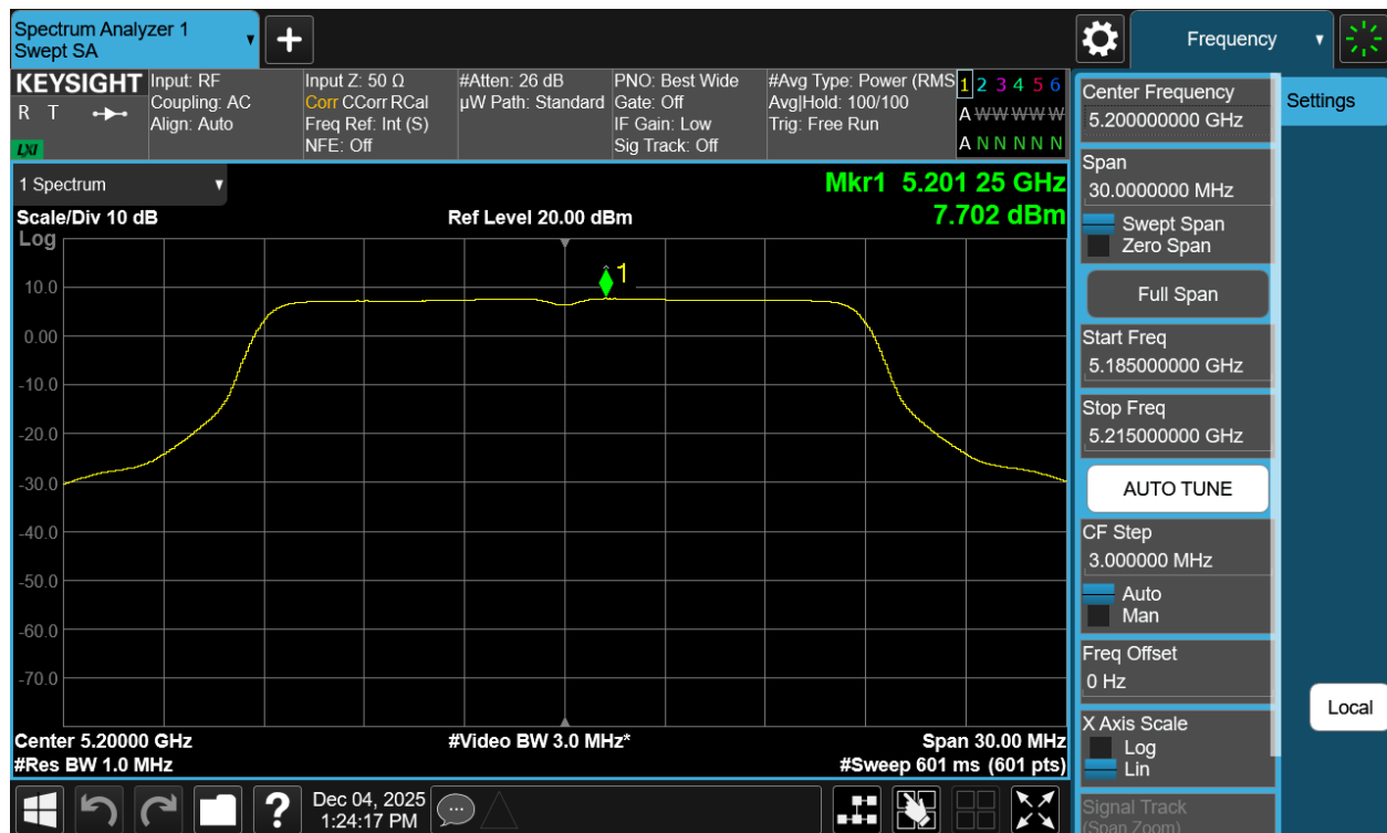
Plot 7-29 PSD Antenna 5T (20MHz BW 802.11a - Ch.40)
