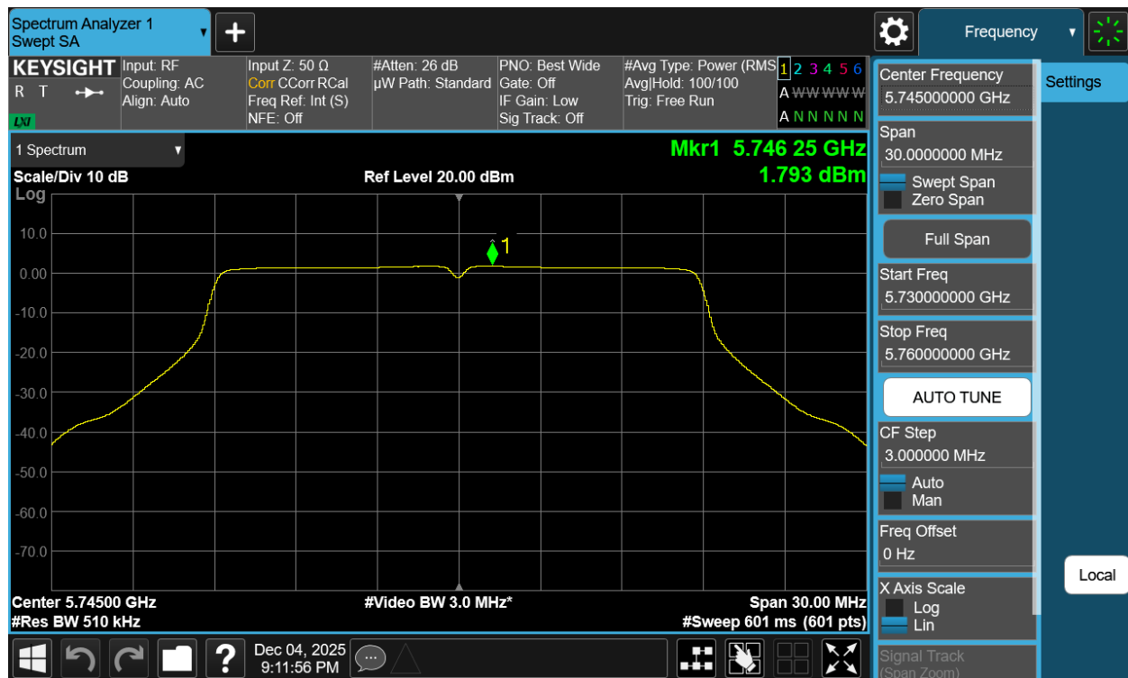
Plot 7-37 PSD Antenna 3b (20MHz BW 802.11a - Ch.149)
