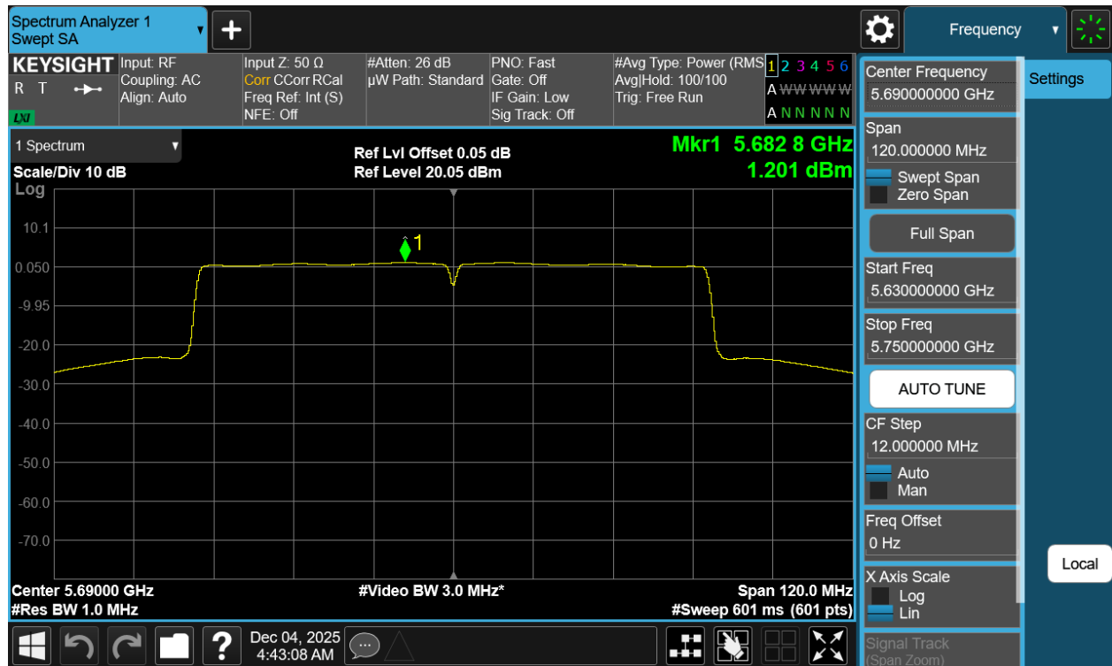
Plot 7-24 PSD Antenna 5T (80MHz BW 802.11ac - Ch.138)
