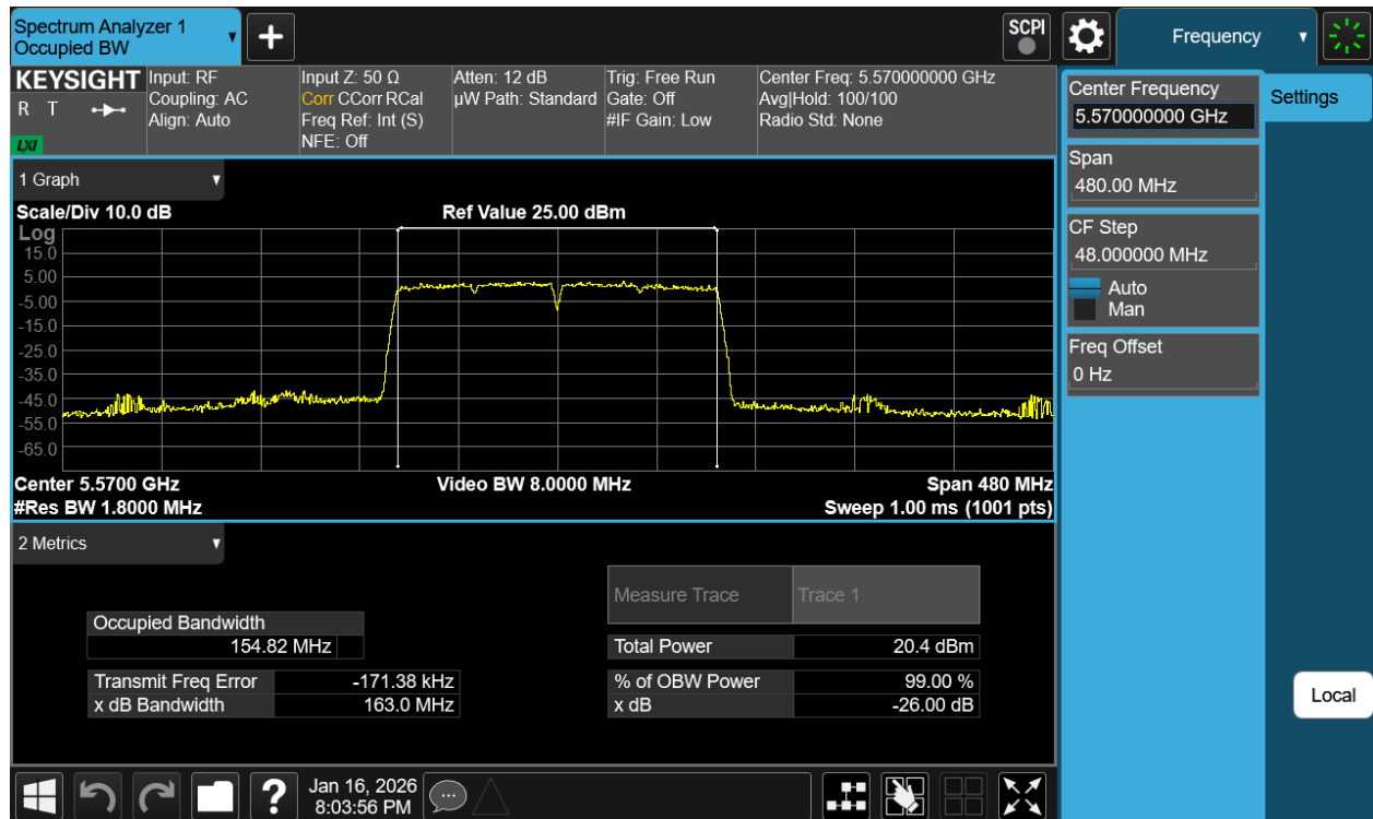
Plot 7-4 26dB BW & 99% OBW Antenna 5T (160MHz BW 802.11ac - Ch.114)
