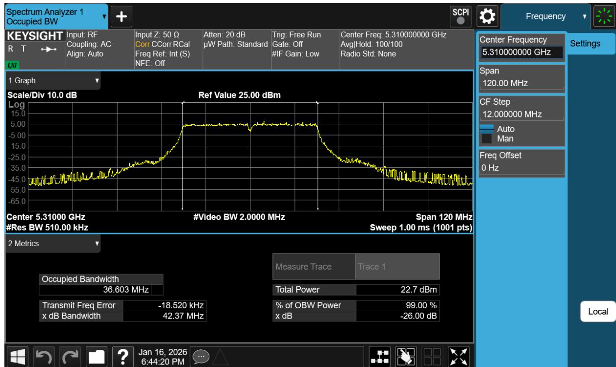
Plot 7-2 26dB BW & 99% OBW Antenna 5T (40MHz BW 802.11n - Ch.62)
