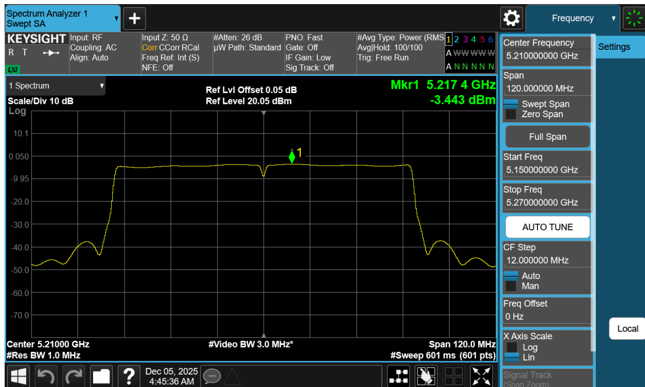
Plot 7-42 PSD Antenna 3b (80MHz BW 802.11ac - Ch.42)
