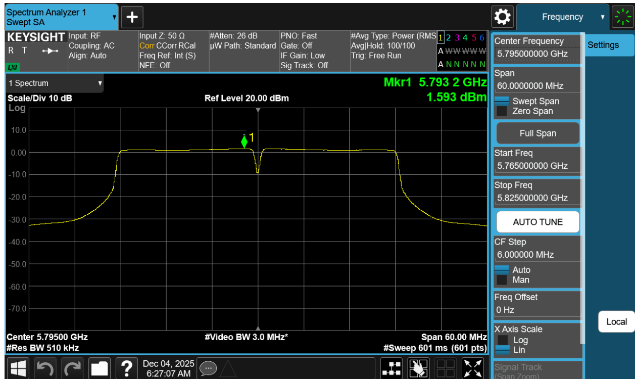
Plot 7-27 PSD Antenna 5T (40MHz BW 802.11n - Ch.159)
