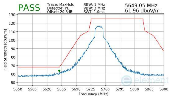
Plot 7-427. CDD Diversity (Peak, Ch.149, 802.11be(SU), MCS11)
