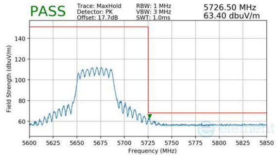
Plot 7-384. CDD Primary (Peak, Ch.134, 802.11be(SU), MCS11)
