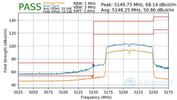
Plot 7-449. CDD Diversity (Peak & Average, Ch.42, 802.11ac, MCS9)
