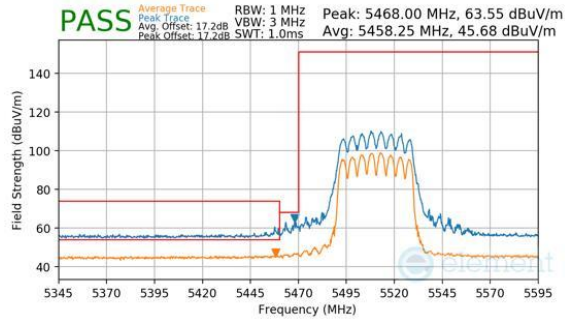
Plot 7-381. CDD Primary (Peak & Average, Ch.102, 802.11be(SU), MCS11)
