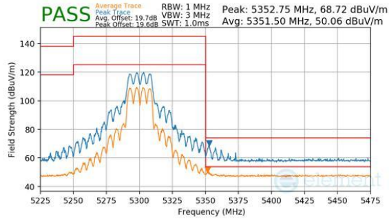
Plot 7-359. CDD Primary (Peak & Average, Ch.60, 802.11be(SU), MCS11)
