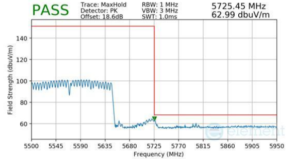
Plot 7-404. CDD Primary (Peak, Ch.114, 802.11ac, MCS9)
