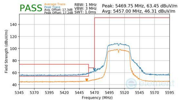
Plot 7-433. CDD Diversity (Peak & Average, Ch.102, 802.11n, MCS7)
