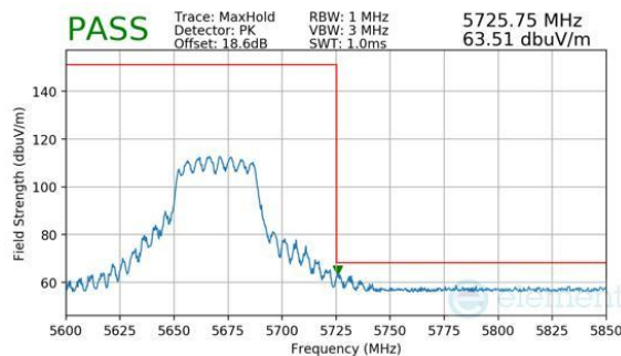
Plot 7-374. CDD Primary (Peak, Ch.134, 802.11n, MCS7)
