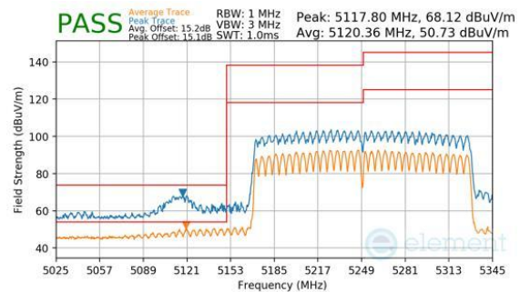
Plot 7-405. CDD Primary (Peak & Average, Ch.50, 802.11be(SU), MCS11)
