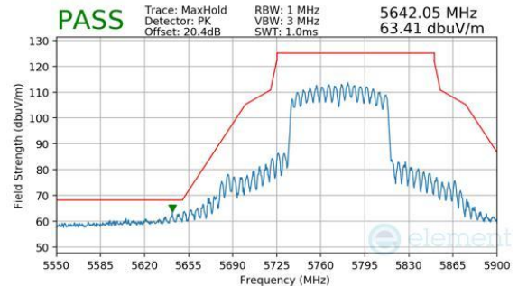
Plot 7-392. CDD Primary (Peak, Ch.155, 802.11ac, MCS9)
