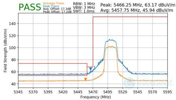
Plot 7-423. CDD Diversity (Peak & Average, Ch.100, 802.11be(SU), MCS11)
