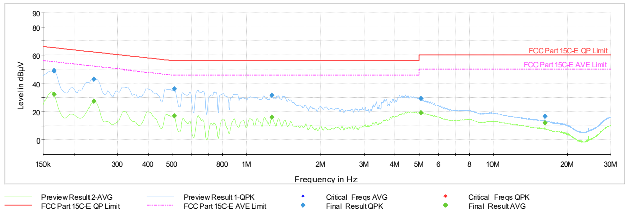
Plot 7-475. AC Line Conducted Plot with 802.11n CDD Primary – Ch.40 (L1), with AC/DC adapter
