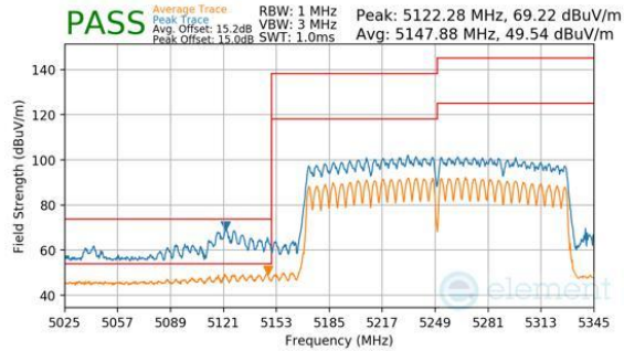
Plot 7-401. CDD Primary (Peak & Average, Ch.50, 802.11ac, MCS9)
