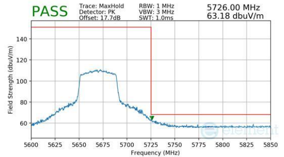
Plot 7-446. CDD Diversity (Peak, Ch.134, 802.11be(SU), MCS11)
