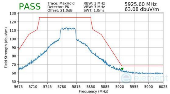
Plot 7-438. CDD Diversity (Peak, Ch.159, 802.11n, MCS7)
