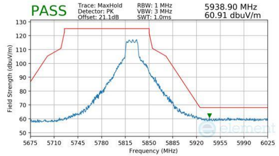
Plot 7-418. CDD Diversity (Peak, Ch.165, 802.11n, MCS7)
