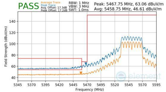
Plot 7-372. CDD Primary (Peak & Average, Ch.110, 802.11n, MCS7)
