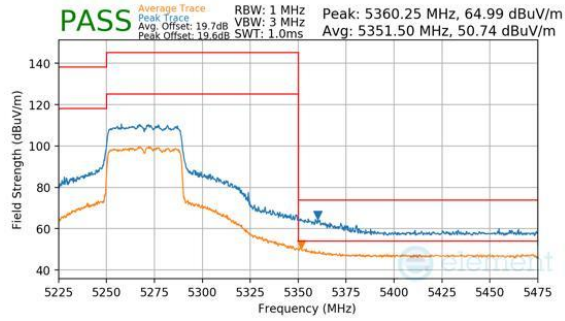
Plot 7-441. CDD Diversity (Peak & Average, Ch.54, 802.11be(SU), MCS11)
