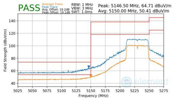
Plot 7-430. CDD Diversity (Peak & Average, Ch.46, 802.11n, MCS7)
