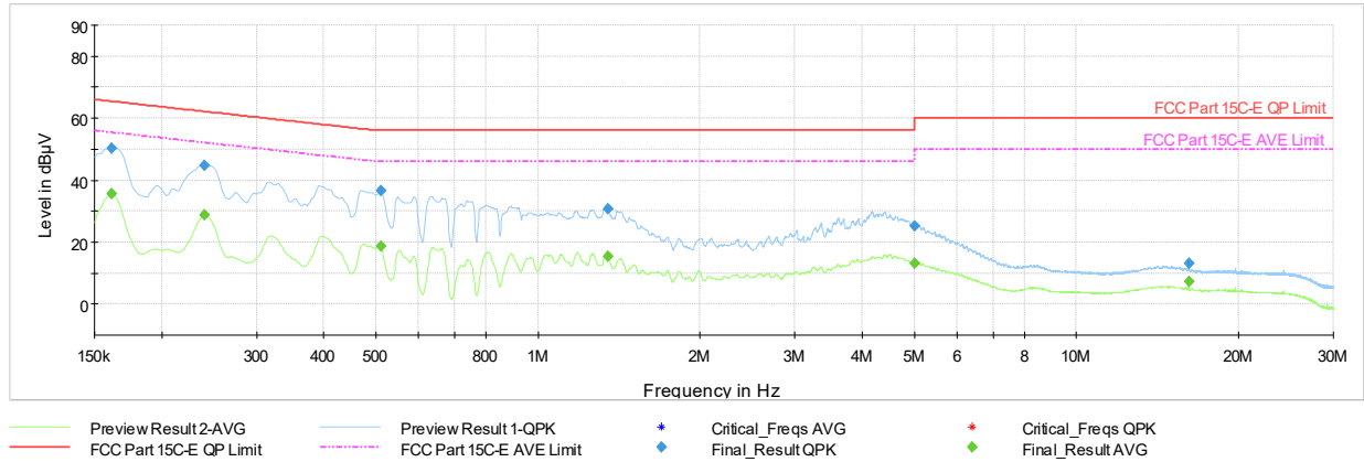
Plot 7-480. AC Line Conducted Plot with 802.11n CDD Diversity – Ch.40 (N), with AC/DC adapter
