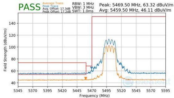
Plot 7-361. CDD Primary (Peak & Average, Ch.100, 802.11be(SU), MCS11)
