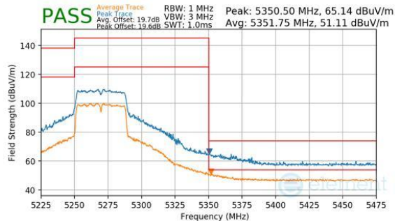
Plot 7-431. CDD Diversity (Peak & Average, Ch.54, 802.11n, MCS7)
