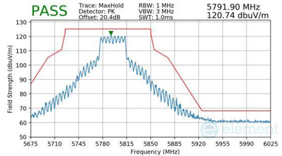
Plot 7-376. CDD Primary (Peak, Ch.159, 802.11n, MCS7)
