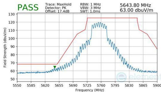
Plot 7-375. CDD Primary (Peak, Ch.151, 802.11n, MCS7)
