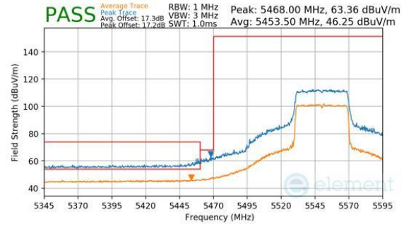
Plot 7-444. CDD Diversity (Peak & Average, Ch.110, 802.11be(SU), MCS11)
