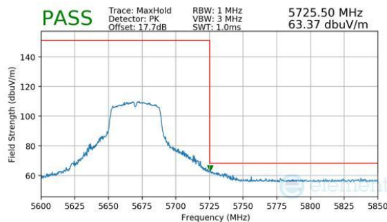
Plot 7-436. CDD Diversity (Peak, Ch.134, 802.11n, MCS7)
