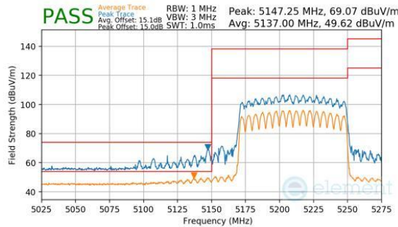
Plot 7-394. CDD Primary (Peak & Average, Ch.42, 802.11be(SU), MCS11)
