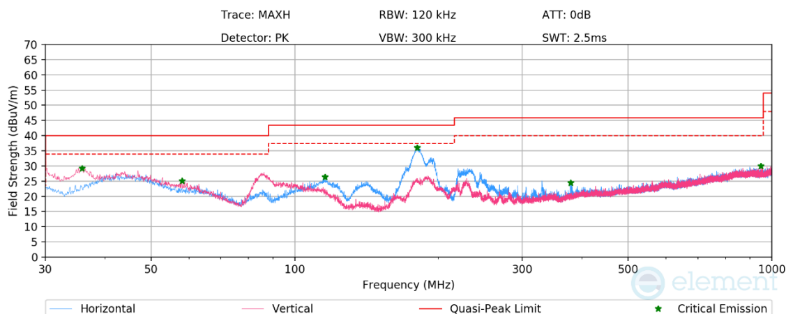
Plot 7-471. Radiated Spurious Emissions below 1GHz CDD Primary, 802.11n, Ch.40 with AC/DC Adapter
