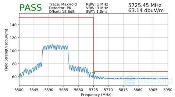
Plot 7-391. CDD Primary (Peak, Ch.122, 802.11ac, MCS9)
