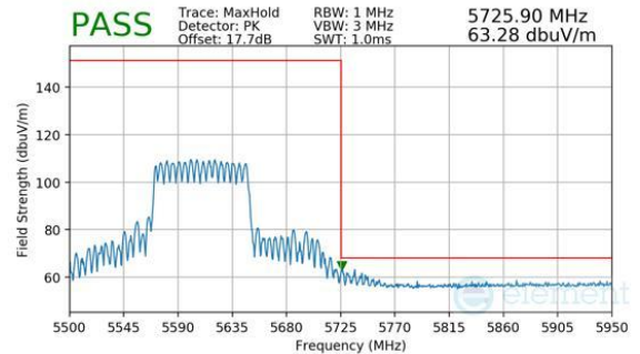
Plot 7-398. CDD Primary (Peak, Ch.122, 802.11be(SU), MCS11)
