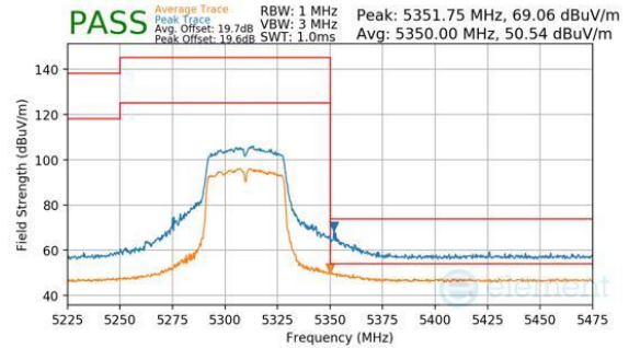
Plot 7-432. CDD Diversity (Peak & Average, Ch.62, 802.11n, MCS7)
