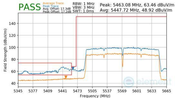
Plot 7-465. CDD Diversity (Peak & Average, Ch.114, 802.11ac, MCS9)
