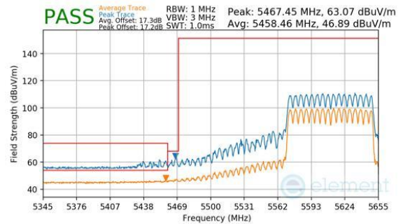
Plot 7-397. CDD Primary (Peak & Average, Ch.122, 802.11be(SU), MCS11)
