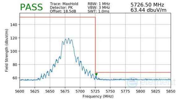
Plot 7-363. CDD Primary (Peak, Ch.136, 802.11be(SU), MCS11)
