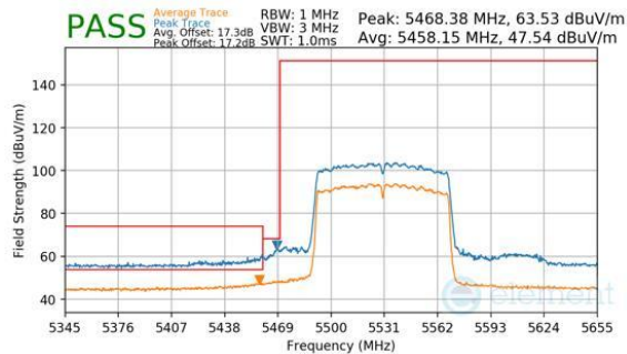
Plot 7-451. CDD Diversity (Peak & Average, Ch.106, 802.11ac, MCS9)
