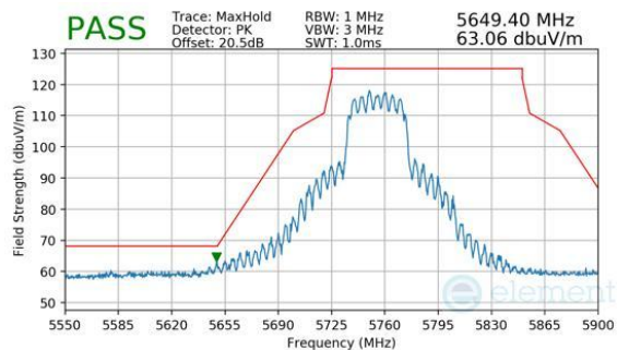
Plot 7-385. CDD Primary (Peak, Ch.151, 802.11be(SU), MCS11)
