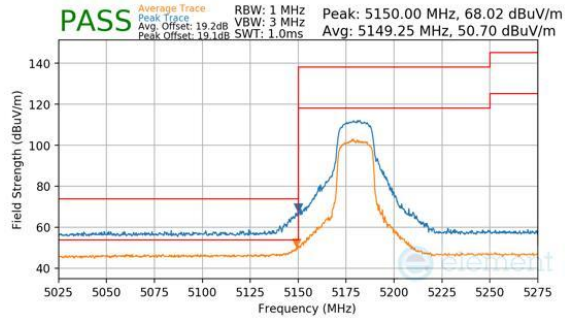
Plot 7-409. CDD Diversity (Peak & Average, Ch.36, 802.11n, MCS7)
