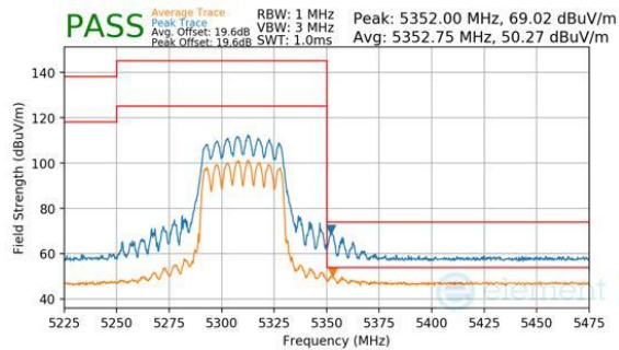
Plot 7-380. CDD Primary (Peak & Average, Ch.62, 802.11be(SU), MCS11)
