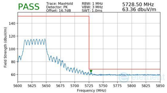
Plot 7-383. CDD Primary (Peak, Ch.126, 802.11be(SU), MCS11)
