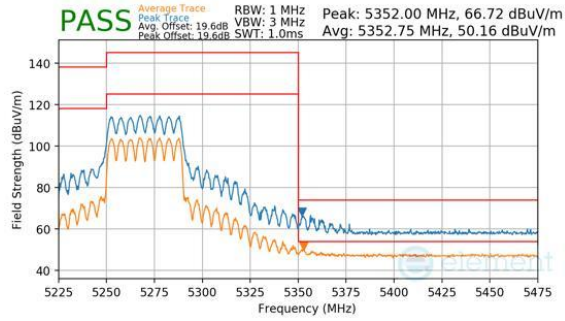
Plot 7-379. CDD Primary (Peak & Average, Ch.54, 802.11be(SU), MCS11)
