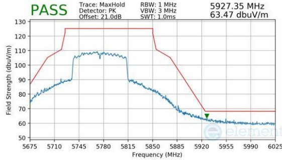
Plot 7-455. CDD Diversity (Peak, Ch.155, 802.11ac, MCS9)
