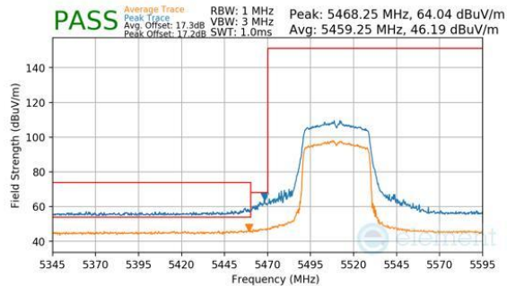
Plot 7-443. CDD Diversity (Peak & Average, Ch.102, 802.11be(SU), MCS11)
