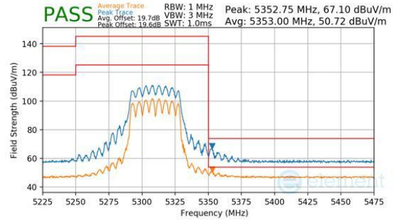
Plot 7-370. CDD Primary (Peak & Average, Ch.62, 802.11n, MCS7)
