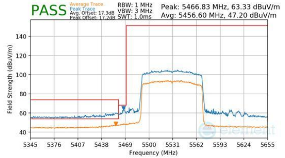
Plot 7-458. CDD Diversity (Peak & Average, Ch.106, 802.11be(SU), MCS11)
