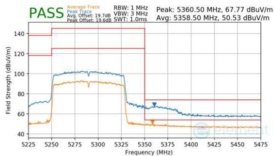
Plot 7-450. CDD Diversity (Peak & Average, Ch.58, 802.11ac, MCS9)
