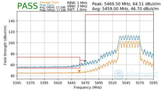
Plot 7-382. CDD Primary (Peak & Average, Ch.110, 802.11be(SU), MCS11)
