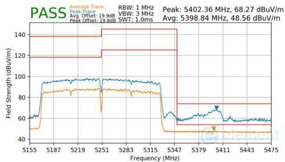
Plot 7-464. CDD Diversity (Peak & Average, Ch.50, 802.11ac, MCS9)
