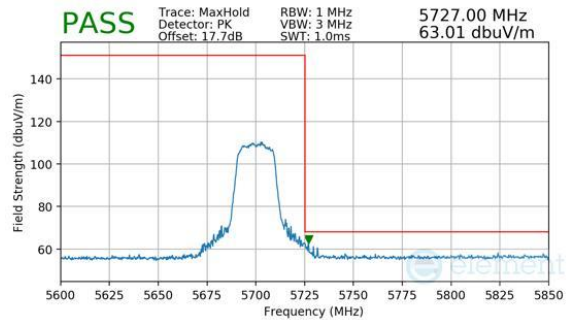
Plot 7-426. CDD Diversity (Peak, Ch.140, 802.11be(SU), MCS11)
