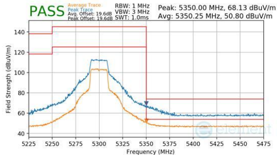
Plot 7-411. CDD Diversity (Peak & Average, Ch.60, 802.11n, MCS7)
