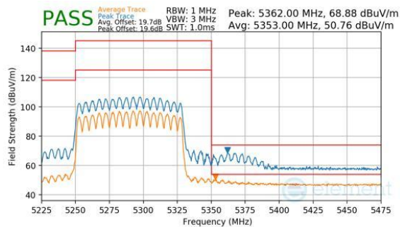
Plot 7-388. CDD Primary (Peak & Average, Ch.58, 802.11ac, MCS9)
