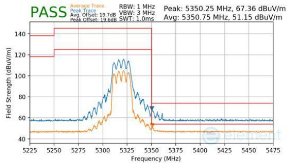
Plot 7-360. CDD Primary (Peak & Average, Ch.64, 802.11be(SU), MCS11)
