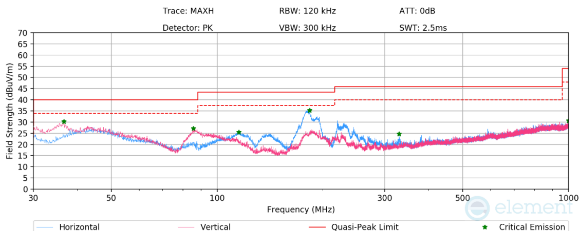
Plot 7-473. Radiated Spurious Emissions below 1GHz CDD Diversity, 802.11n, Ch.40 with AC/DC Adapter
