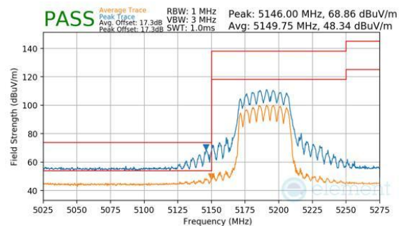
Plot 7-377. CDD Primary (Peak & Average, Ch.38, 802.11be(SU), MCS11)
