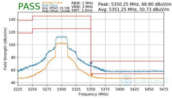
Plot 7-421. CDD Diversity (Peak & Average, Ch.60, 802.11be(SU), MCS11)
