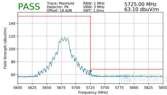
Plot 7-353. CDD Primary (Peak, Ch.136, 802.11n, MCS7)
