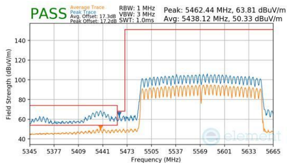
Plot 7-407. CDD Primary (Peak & Average, Ch.114, 802.11be(SU), MCS11)
