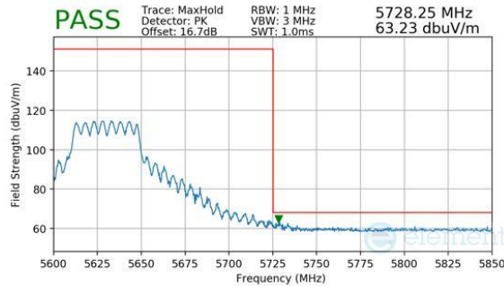
Plot 7-373. CDD Primary (Peak, Ch.126, 802.11n, MCS7)
