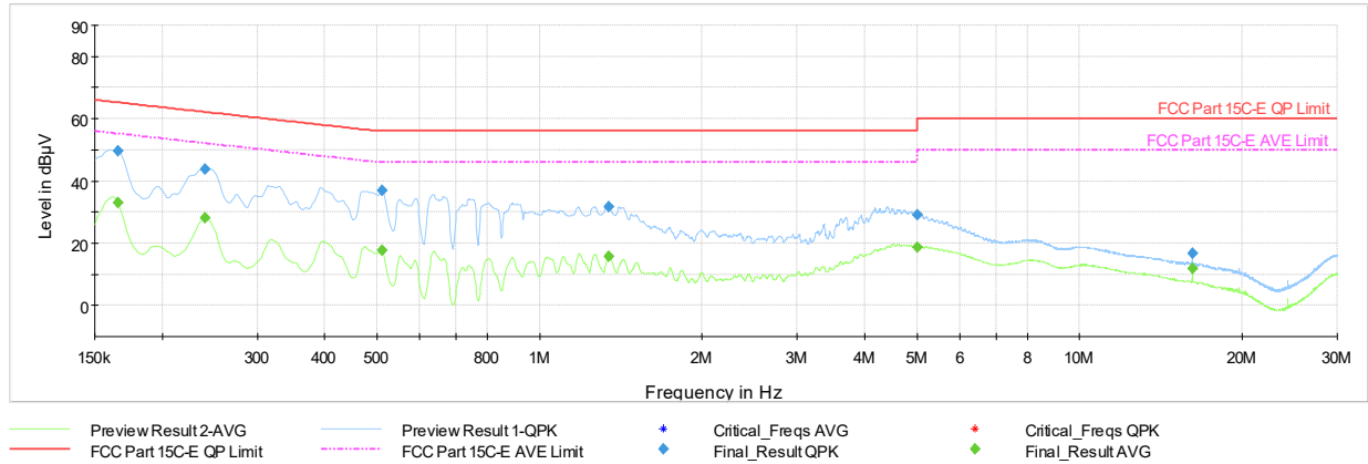
Plot 7-481. AC Line Conducted Plot with 802.11be(SU) CDD Diversity – Ch.40 (L1), with AC/DC adapter
