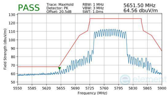
Plot 7-399. CDD Primary (Peak, Ch.155, 802.11be(SU), MCS11)
