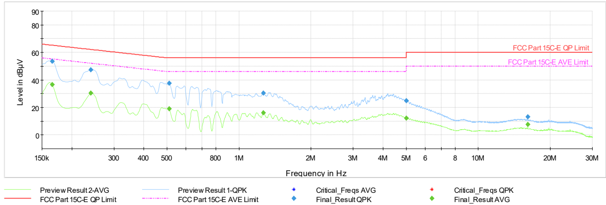
Plot 7-478. AC Line Conducted Plot with 802.11be(SU) CDD Primary – Ch.40 (N), with AC/DC adapter
