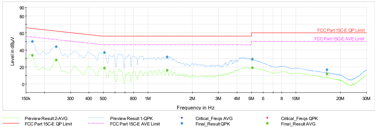
Plot 7-479. AC Line Conducted Plot with 802.11n CDD Diversity – Ch.40 (L1), with AC/DC adapter
