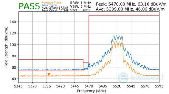
Plot 7-362. CDD Primary (Peak & Average, Ch.104, 802.11be(SU), MCS11)
