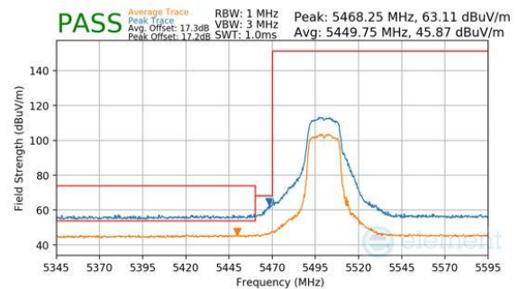
Plot 7-413. CDD Diversity (Peak & Average, Ch.100, 802.11n, MCS7)
