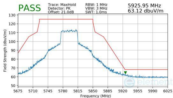
Plot 7-448. CDD Diversity (Peak, Ch.159, 802.11be(SU), MCS11)
