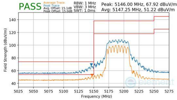
Plot 7-367. CDD Primary (Peak & Average, Ch.38, 802.11n, MCS7)
