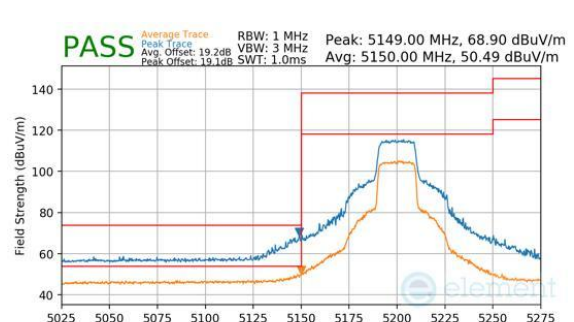
Plot 7-420. CDD Diversity (Peak & Average, Ch.40, 802.11be(SU), MCS11)
