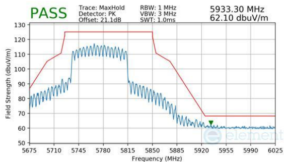
Plot 7-400. CDD Primary (Peak, Ch.155, 802.11be(SU), MCS11)
