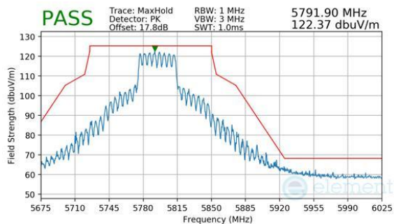
Plot 7-386. CDD Primary (Peak, Ch.159, 802.11be(SU), MCS11)
