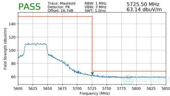
Plot 7-435. CDD Diversity (Peak, Ch.126, 802.11n, MCS7)
