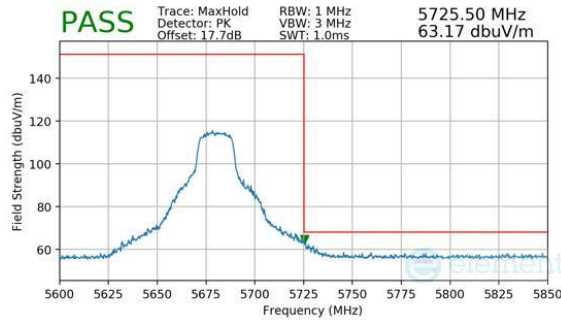
Plot 7-415. CDD Diversity (Peak, Ch.136, 802.11n, MCS7)
