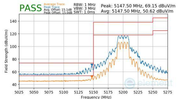
Plot 7-358. CDD Primary (Peak & Average, Ch.40, 802.11be(SU), MCS11)
