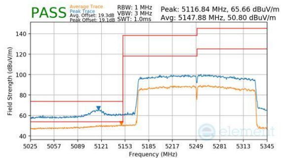
Plot 7-467. CDD Diversity (Peak & Average, Ch.50, 802.11be(SU), MCS11)
