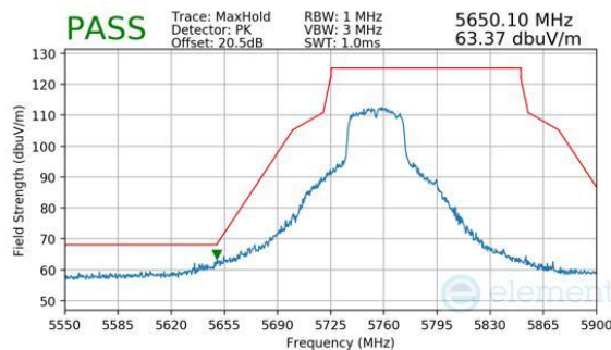
Plot 7-437. CDD Diversity (Peak, Ch.151, 802.11n, MCS7)
