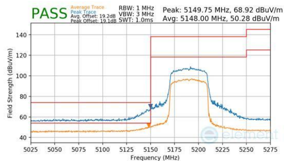
Plot 7-439. CDD Diversity (Peak & Average, Ch.38, 802.11be(SU), MCS11)
