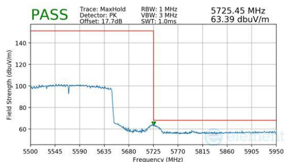
Plot 7-470. CDD Diversity (Peak, Ch.114, 802.11be(SU), MCS11)
