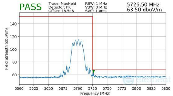
Plot 7-364. CDD Primary (Peak, Ch.140, 802.11be(SU), MCS11)
