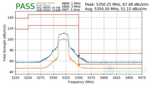
Plot 7-422. CDD Diversity (Peak & Average, Ch.64, 802.11be(SU), MCS11)
