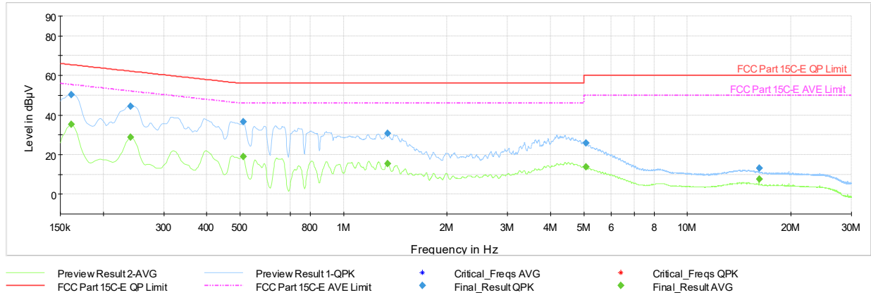
Plot 7-482. AC Line Conducted Plot with 802.11be(SU) CDD Diversity – Ch.40 (N), with AC/DC adapter
