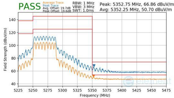
Plot 7-369. CDD Primary (Peak & Average, Ch.54, 802.11n, MCS7)
