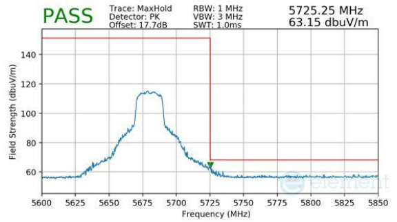
Plot 7-425. CDD Diversity (Peak, Ch.136, 802.11be(SU), MCS11)
