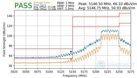
Plot 7-368. CDD Primary (Peak & Average, Ch.46, 802.11n, MCS7)
