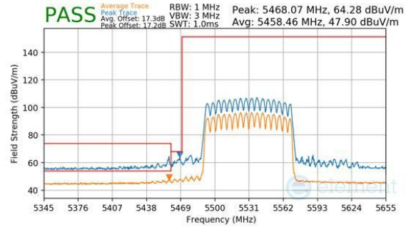
Plot 7-396. CDD Primary (Peak & Average, Ch.106, 802.11be(SU), MCS11)
