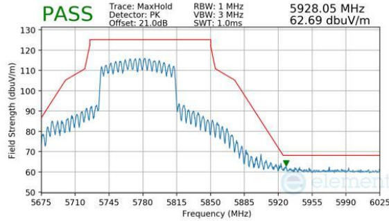
Plot 7-393. CDD Primary (Peak, Ch.155, 802.11ac, MCS9)
