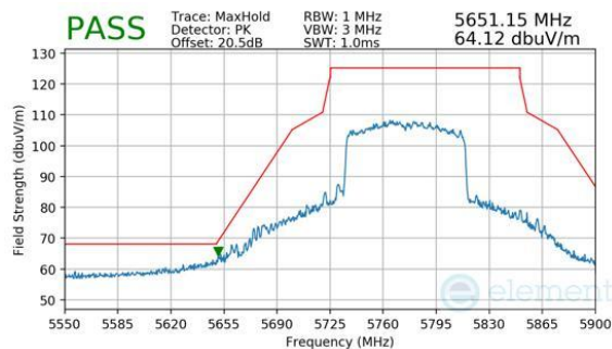
Plot 7-461. CDD Diversity (Peak, Ch.155, 802.11be(SU), MCS11)
