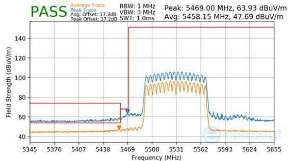
Plot 7-389. CDD Primary (Peak & Average, Ch.106, 802.11ac, MCS9)
