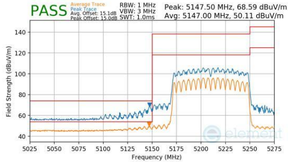
Plot 7-387. CDD Primary (Peak & Average, Ch.42, 802.11ac, MCS9)
