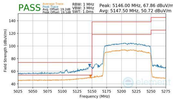
Plot 7-456. CDD Diversity (Peak & Average, Ch.42, 802.11be(SU), MCS11)
