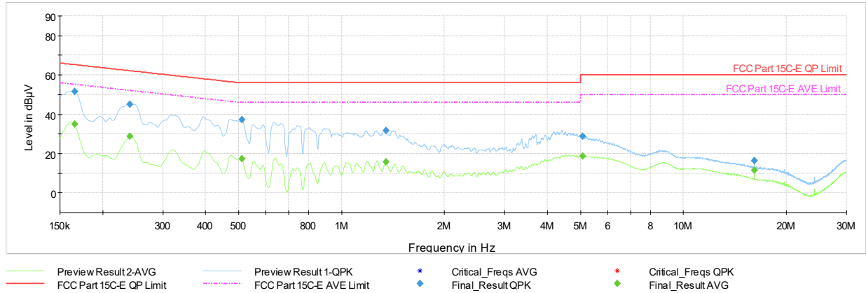
Plot 7-477. AC Line Conducted Plot with 802.11be(SU) CDD Primary – Ch.40 (L1), with AC/DC adapter
