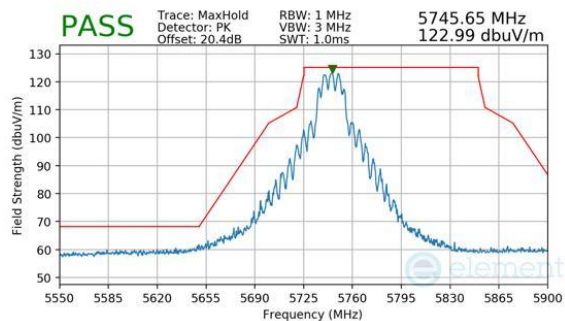
Plot 7-365. CDD Primary (Peak, Ch.149, 802.11be(SU), MCS11)
