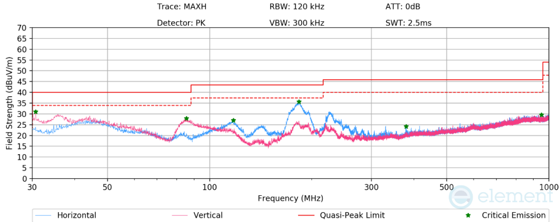
Plot 7-472. Radiated Spurious Emissions below 1GHz CDD Primary, 802.11be (SU), Ch.40 with AC/DC Adapter
