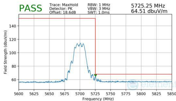
Plot 7-354. CDD Primary (Peak, Ch.140, 802.11n, MCS7)
