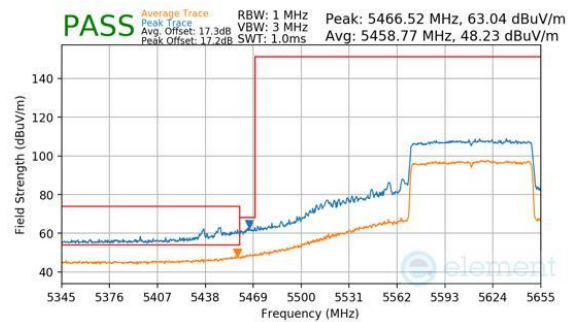
Plot 7-459. CDD Diversity (Peak & Average, Ch.122, 802.11be(SU), MCS11)
