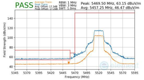
Plot 7-424. CDD Diversity (Peak & Average, Ch.104, 802.11be(SU), MCS11)
