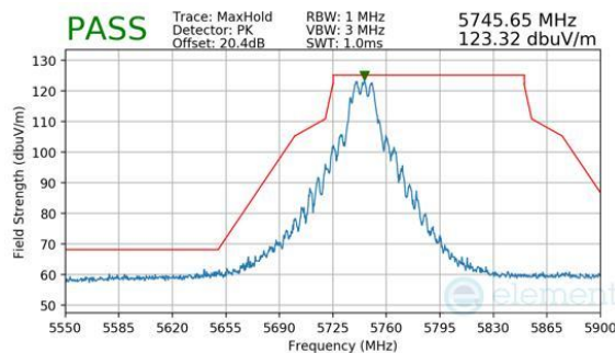
Plot 7-355. CDD Primary (Peak, Ch.149, 802.11n, MCS7)
