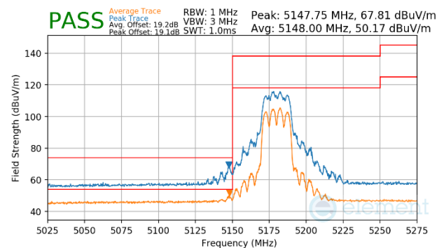
Plot 7-357. CDD Primary (Peak & Average, Ch.36, 802.11be(SU), MCS11)
