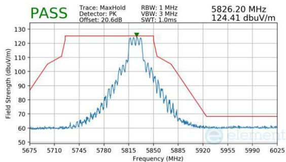
Plot 7-366. CDD Primary (Peak, Ch.165, 802.11be(SU), MCS11)
