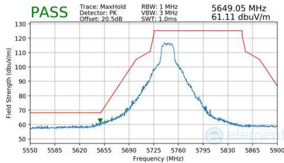
Plot 7-417. CDD Diversity (Peak, Ch.149, 802.11n, MCS7)
