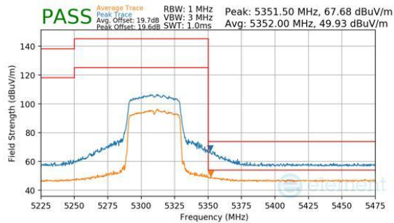
Plot 7-442. CDD Diversity (Peak & Average, Ch.62, 802.11be(SU), MCS11)
