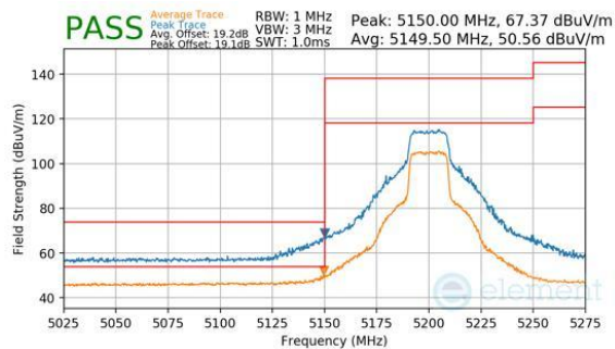
Plot 7-410. CDD Diversity (Peak & Average, Ch.40, 802.11n, MCS7)
