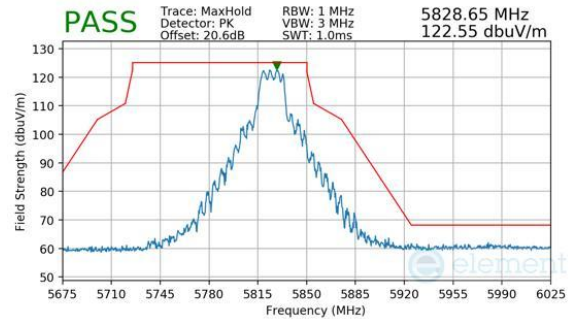
Plot 7-356. CDD Primary (Peak, Ch.165, 802.11n, MCS7)
