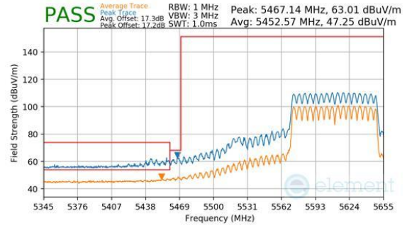
Plot 7-390. CDD Primary (Peak & Average, Ch.122, 802.11ac, MCS9)
