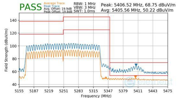
Plot 7-406. CDD Primary (Peak & Average, Ch.50, 802.11be(SU), MCS11)
