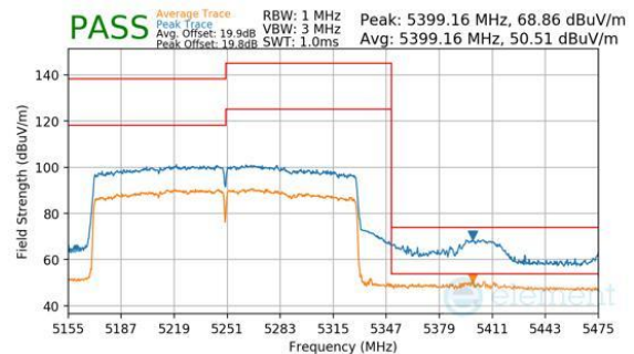
Plot 7-468. CDD Diversity (Peak & Average, Ch.50, 802.11be(SU), MCS11)
