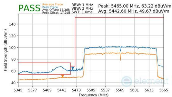
Plot 7-469. CDD Diversity (Peak & Average, Ch.114, 802.11be(SU), MCS11)
