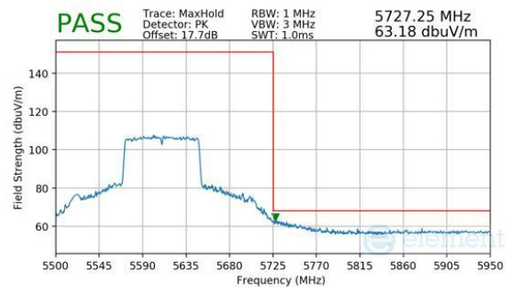
Plot 7-453. CDD Diversity (Peak, Ch.122, 802.11ac, MCS9)
