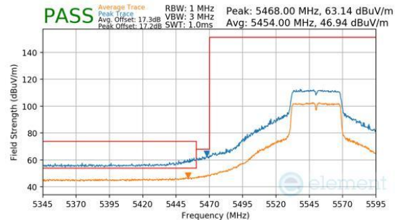
Plot 7-434. CDD Diversity (Peak & Average, Ch.110, 802.11n, MCS7)
