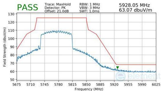
Plot 7-462. CDD Diversity (Peak, Ch.155, 802.11be(SU), MCS11)
