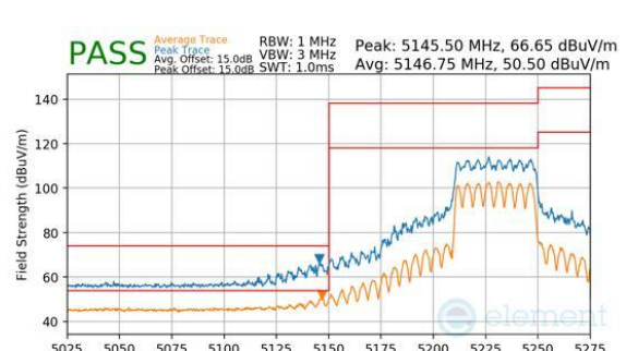
Plot 7-378. CDD Primary (Peak & Average, Ch.46, 802.11be(SU), MCS11)
