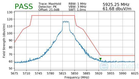
Plot 7-428. CDD Diversity (Peak, Ch.165, 802.11be(SU), MCS11)
