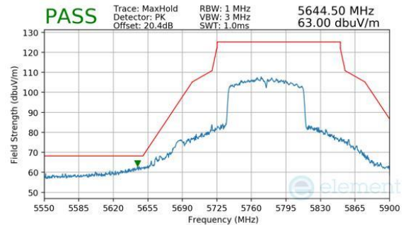
Plot 7-454. CDD Diversity (Peak, Ch.155, 802.11ac, MCS9)
