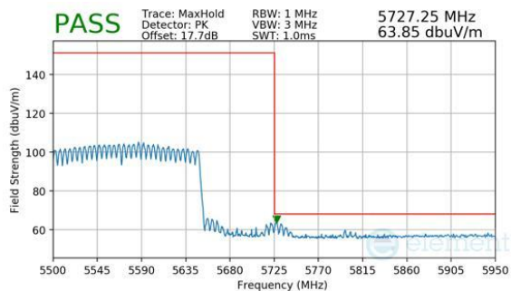
Plot 7-408. CDD Primary (Peak, Ch.114, 802.11be(SU), MCS11)
