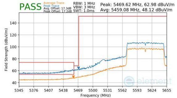
Plot 7-452. CDD Diversity (Peak & Average, Ch.122, 802.11ac, MCS9)
