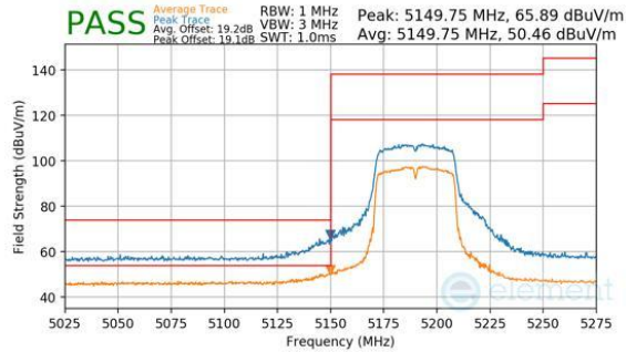
Plot 7-429. CDD Diversity (Peak & Average, Ch.38, 802.11n, MCS7)
