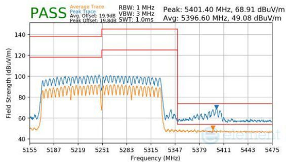
Plot 7-402. CDD Primary (Peak & Average, Ch.50, 802.11ac, MCS9)
