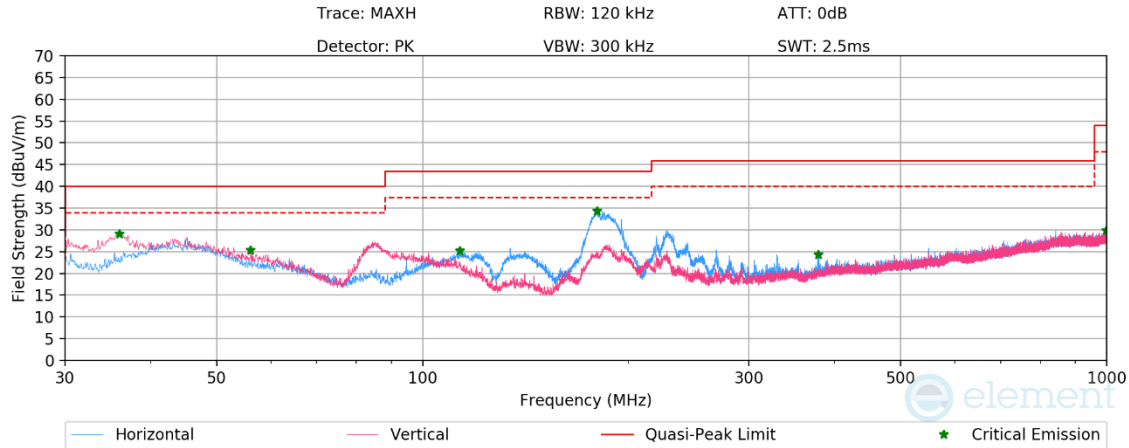
Plot 7-474. Radiated Spurious Emissions below 1GHz CDD Diversity, 802.11be (SU), Ch.40 with AC/DC Adapter
