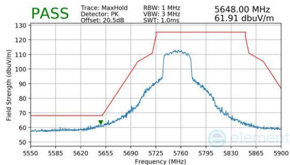
Plot 7-447. CDD Diversity (Peak, Ch.151, 802.11be(SU), MCS11)
