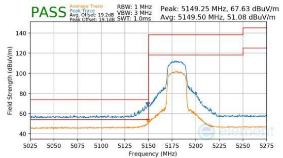
Plot 7-419. CDD Diversity (Peak & Average, Ch.36, 802.11be(SU), MCS11)
