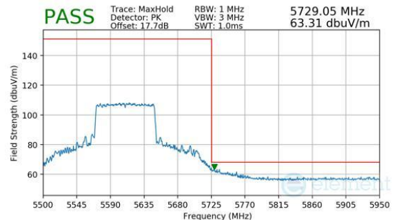
Plot 7-460. CDD Diversity (Peak, Ch.122, 802.11be(SU), MCS11)
