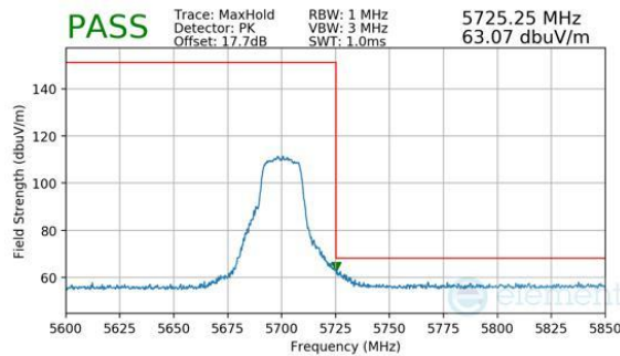
Plot 7-416. CDD Diversity (Peak, Ch.140, 802.11n, MCS7)
