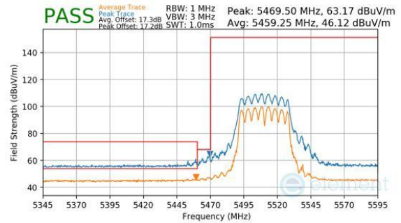
Plot 7-371. CDD Primary (Peak & Average, Ch.102, 802.11n, MCS7)
