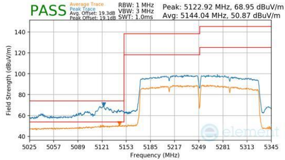
Plot 7-463. CDD Diversity (Peak & Average, Ch.50, 802.11ac, MCS9)
