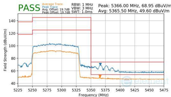
Plot 7-457. CDD Diversity (Peak & Average, Ch.58, 802.11be(SU), MCS11)
