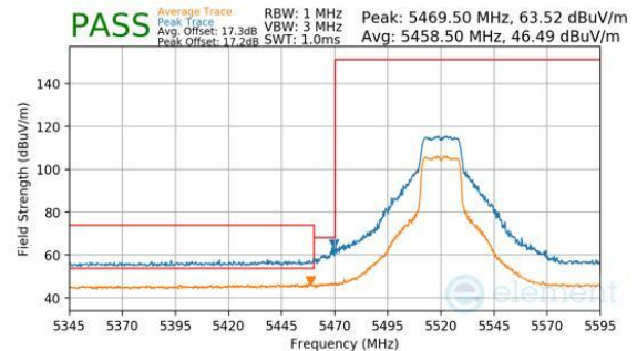
Plot 7-414. CDD Diversity (Peak & Average, Ch.104, 802.11n, MCS7)
