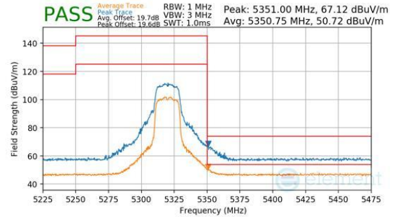
Plot 7-412. CDD Diversity (Peak & Average, Ch.64, 802.11n, MCS7)
