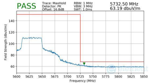
Plot 7-445. CDD Diversity (Peak, Ch.126, 802.11be(SU), MCS11)
