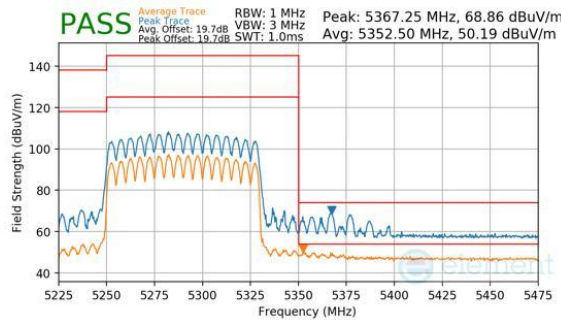
Plot 7-395. CDD Primary (Peak & Average, Ch.58, 802.11be(SU), MCS11)
