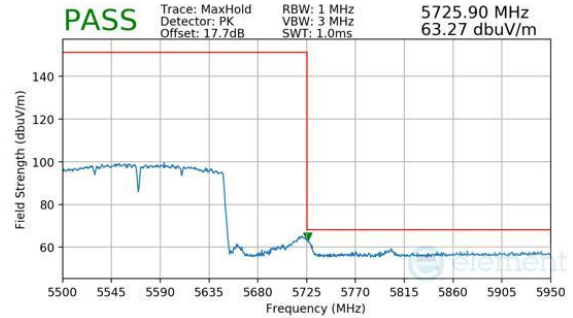
Plot 7-466. CDD Diversity (Peak, Ch.114, 802.11ac, MCS9)
