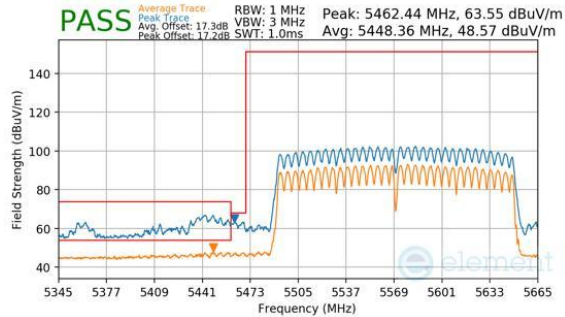
Plot 7-403. CDD Primary (Peak & Average, Ch.114, 802.11ac, MCS9)
