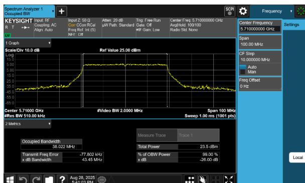
Plot 7-20 26dB BW & 99% OBW Antenna 3b (40MHz BW 802.11be(RU) RU484 Index65 - Ch.142)
