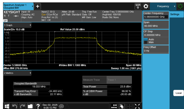
Plot 7-8 26dB BW & 99% OBW Antenna 5T (20MHz BW 802.11be(RU) RU242 Index61 - Ch.116)
