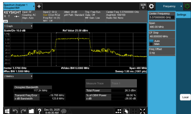
Plot 7-7 26dB BW & 99% OBW Antenna 5T (160MHz BW 802.11be(RU) RU996+484 Index95 - Ch.114)
