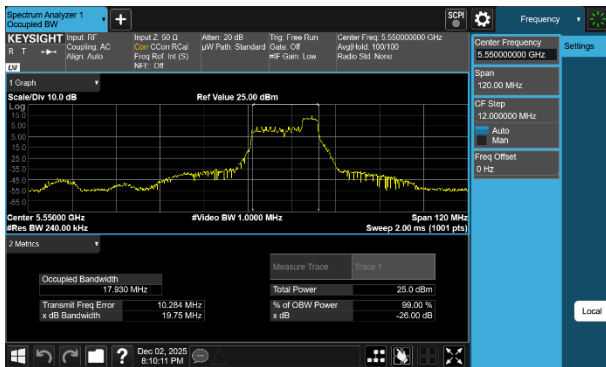
Plot 7-2 26dB BW & 99% OBW Antenna 5T (40MHz BW 802.11be(RU) RU52 Index44 - Ch.110)
