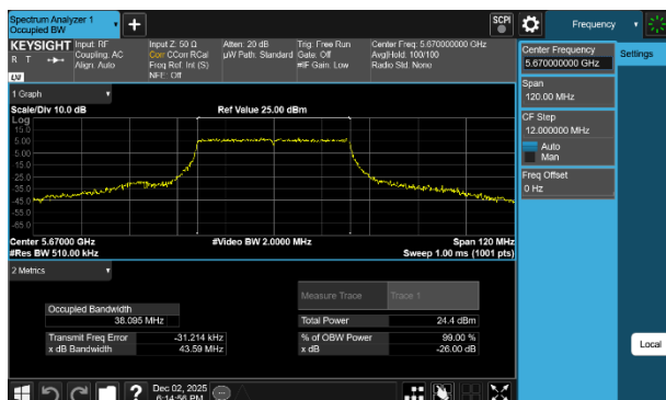
Plot 7-9 26dB BW & 99% OBW Antenna 5T (40MHz BW 802.11be(RU) RU484 Index65 - Ch.134)
