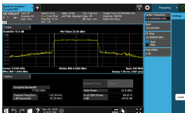
Plot 7-10 26dB BW & 99% OBW Antenna 5T (80MHz BW 802.11be(RU) RU996 Index67 - Ch.122)
