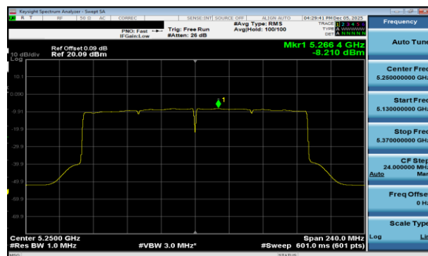
Plot 7-68 PSD Antenna 5T (160MHz BW 802.11be(RU) RU996X2 Index68 - Ch.50)
