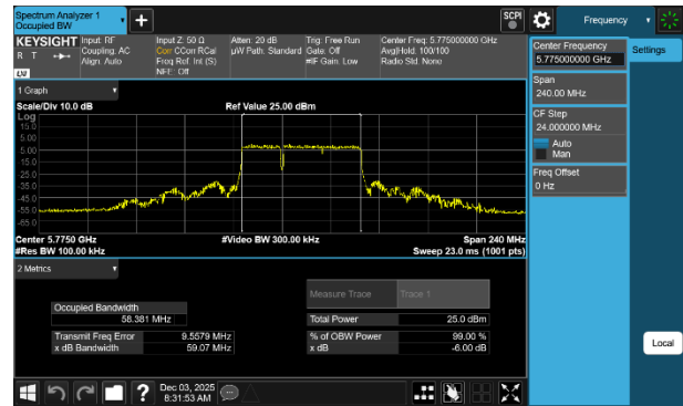
Plot 7-38 6dB OBW Antenna 5T (80MHz BW 802.11be(RU) RU484+242 Index90 - Ch.155)
