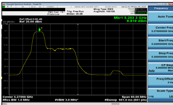
Plot 7-59 PSD Antenna 5T (40MHz BW 802.11be(RU) RU52 Index37 - Ch.54)
