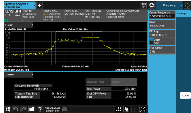
Plot 7-27 26dB BW & 99% OBW Antenna 1b (20MHz BW 802.11be(RU) RU52+26 Index72 - Ch.116)
