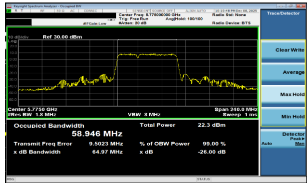
Plot 7-46 26dB BW & 99% OBW Antenna 3b (80MHz BW 802.11be(RU) RU484+242 Index90 - Ch.155)
