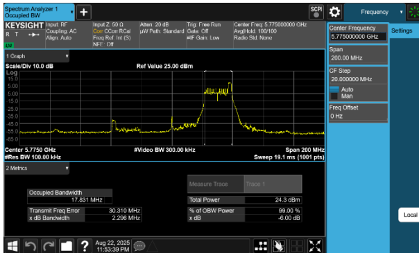
Plot 7-52 6dB OBW Antenna 1b (80MHz BW 802.11be(RU) RU26 Index36 - Ch.155)
