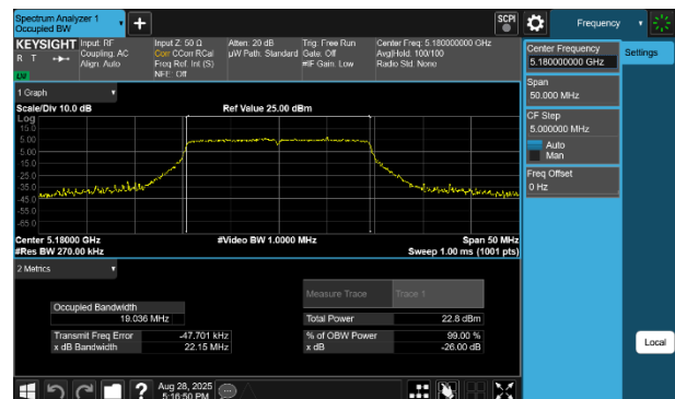
Plot 7-19 26dB BW & 99% OBW Antenna 3b (20MHz BW 802.11be(RU) RU242 Index61 - Ch.36)
