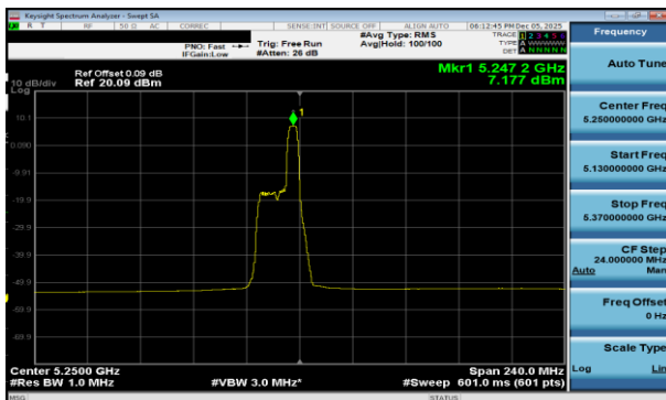
Plot 7-61 PSD Antenna 5T (160MHz BW 802.11be(RU) RU52 Index52 - Ch.50)
