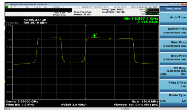
Plot 7-63 PSD Antenna 5T (80MHz BW 802.11be(RU) RU484+242 Index91 - Ch.138)
