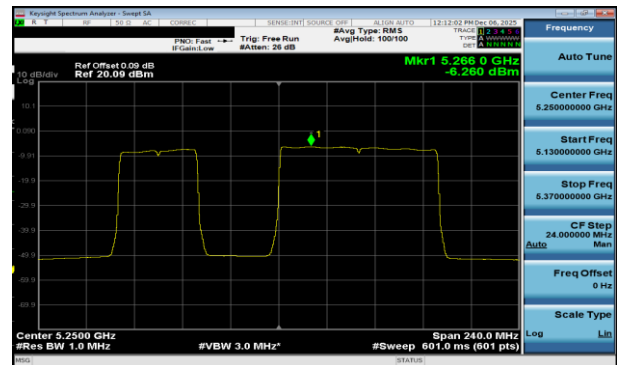
Plot 7-64 PSD Antenna 5T (160MHz BW 802.11be(RU) RU996+484 Index95 - Ch.50)
