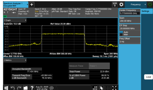
Plot 7-57 6dB OBW Antenna 1b (80MHz BW 802.11be(RU) RU996 Index67 - Ch.155)
