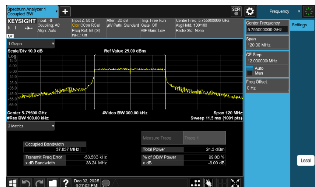
Plot 7-40 6dB OBW Antenna 5T (40MHz BW 802.11be(RU) RU484 Index65 - Ch.151)
