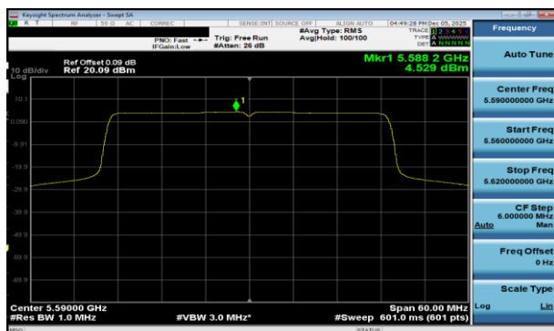
Plot 7-66 PSD Antenna 5T (40MHz BW 802.11be(RU) RU484 Index65 - Ch.118)
