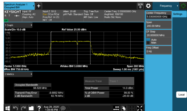
Plot 7-17 26dB BW & 99% OBW Antenna 3b (80MHz BW 802.11be(RU) RU484+242 Index93 - Ch.106)
