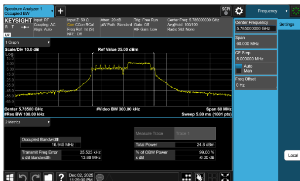
Plot 7-37 6dB OBW Antenna 5T (20MHz BW 802.11be(RU) RU52+26 Index72 - Ch.157)
