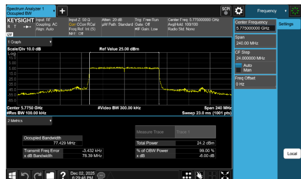
Plot 7-41 6dB OBW Antenna 5T (80MHz BW 802.11be(RU) RU996 Index67 - Ch.155)
