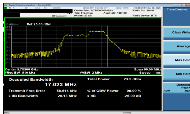
Plot 7-45 26dB BW & 99% OBW Antenna 3b (20MHz BW 802.11be(RU) RU52+26 Index72 - Ch.157)
