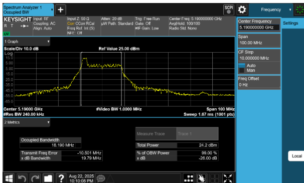
Plot 7-24 26dB BW & 99% OBW Antenna 1b (40MHz BW 802.11be(RU) RU26 Index0 - Ch.38)
