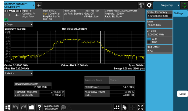
Plot 7-16 26dB BW & 99% OBW Antenna 3b (20MHz BW 802.11be(RU) RU52+26 Index71 - Ch.64)
