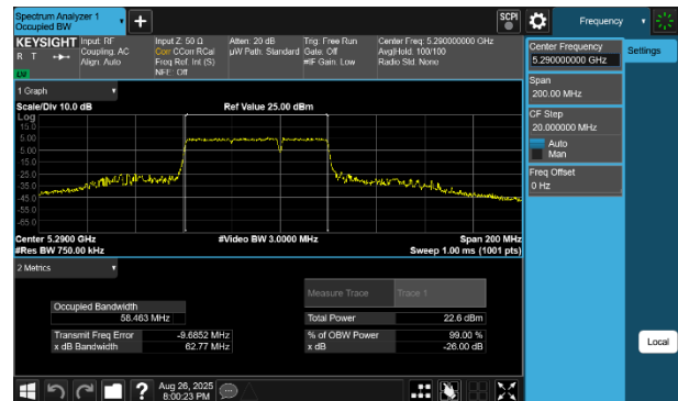
Plot 7-28 26dB BW & 99% OBW Antenna 1b (80MHz BW 802.11be(RU) RU484+242 Index93 - Ch.58)
