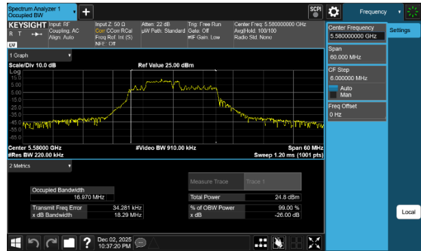
Plot 7-5 26dB BW & 99% OBW Antenna 5T (20MHz BW 802.11be(RU) RU52+26 Index71 - Ch.116)
