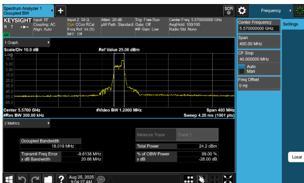
Plot 7-26 26dB BW & 99% OBW Antenna 1b (160MHz BW 802.11be(RU) RU52 Index52 - Ch.114)
