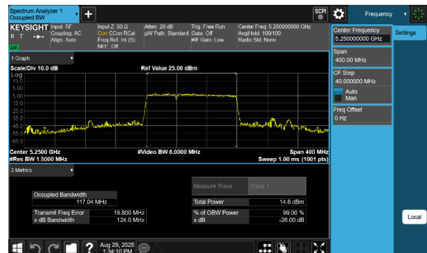
Plot 7-18 26dB BW & 99% OBW Antenna 3b (160MHz BW 802.11be(RU) RU996+484 Index94 - Ch.50)
