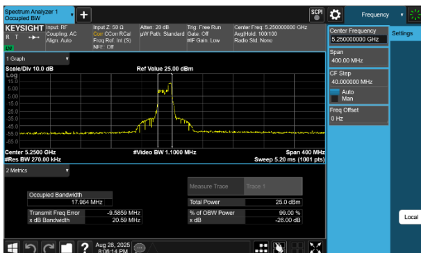
Plot 7-15 26dB BW & 99% OBW Antenna 3b (160MHz BW 802.11be(RU) RU52 Index52 - Ch.50)
