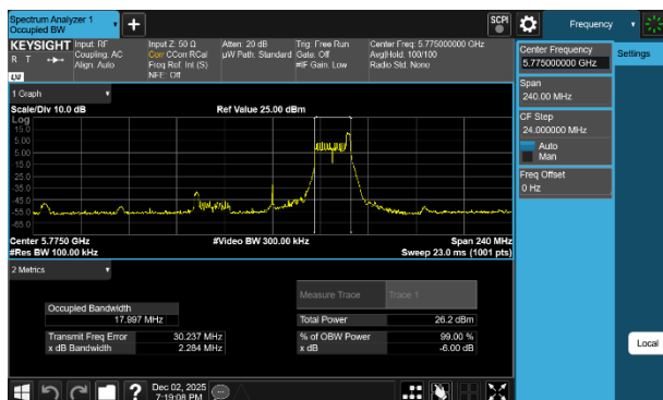
Plot 7-36 6dB OBW Antenna 5T (80MHz BW 802.11be(RU) RU26 Index36 - Ch.155)
