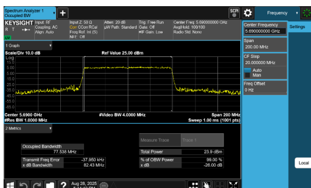
Plot 7-21 26dB BW & 99% OBW Antenna 3b (80MHz BW 802.11be(RU) RU996 Index67 - Ch.138)
