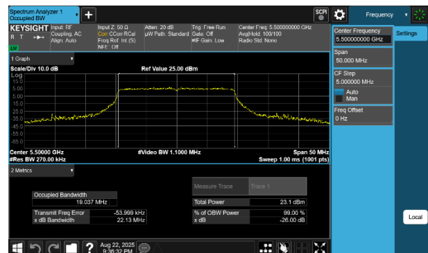
Plot 7-30 26dB BW & 99% OBW Antenna 1b (20MHz BW 802.11be(RU) RU242 Index61 - Ch.100)
