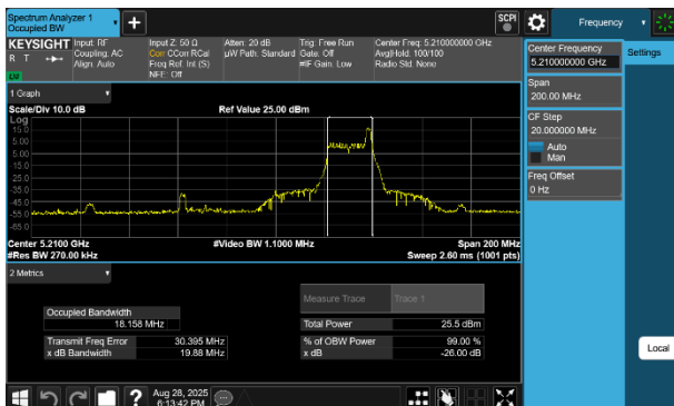
Plot 7-14 26dB BW & 99% OBW Antenna 3b (80MHz BW 802.11be(RU) RU26 Index36 - Ch.42)
