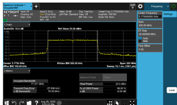
Plot 7-49 6dB OBW Antenna 3b (80MHz BW 802.11be(RU) RU996 Index67 - Ch.155)
