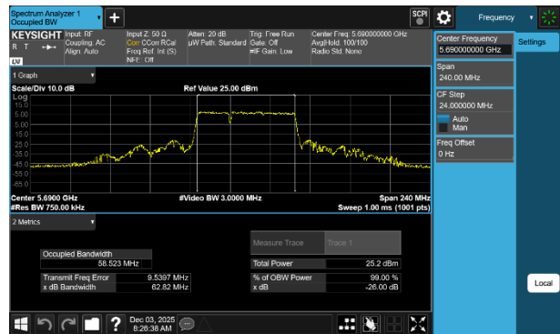
Plot 7-6 26dB BW & 99% OBW Antenna 5T (80MHz BW 802.11be(RU) RU484+242 Index90 - Ch.138)
