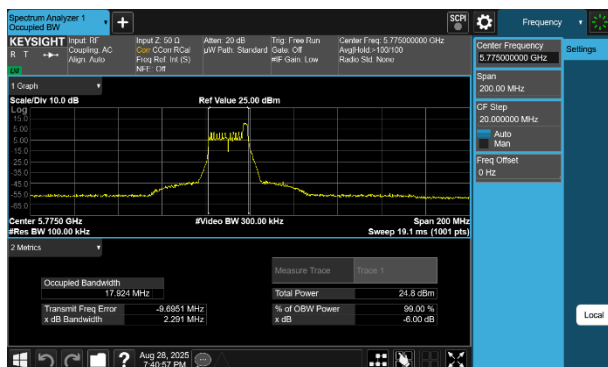
Plot 7-44 6dB OBW Antenna 3b (80MHz BW 802.11be(RU) RU26 Index17 - Ch.155)
