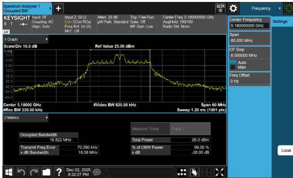
Plot 7-1 26dB BW & 99% OBW Antenna 5T (20MHz BW 802.11be(RU) RU26 Index4 - Ch.36)
