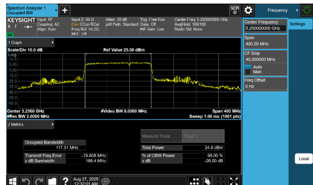
Plot 7-29 26dB BW & 99% OBW Antenna 1b (160MHz BW 802.11be(RU) RU996+484 Index95 - Ch.50)
