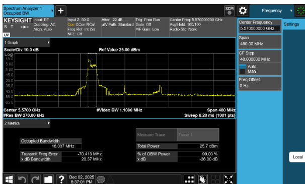
Plot 7-4 26dB BW & 99% OBW Antenna 5T (160MHz BW 802.11be(RU) RU52 Index37 - Ch.114)
