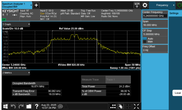
Plot 7-23 26dB BW & 99% OBW Antenna 1b (20MHz BW 802.11be(RU) RU26 Index4 - Ch.48)
