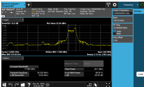
Plot 7-3 26dB BW & 99% OBW Antenna 5T (80MHz BW 802.11be(RU) RU52 Index52 - Ch.138)
