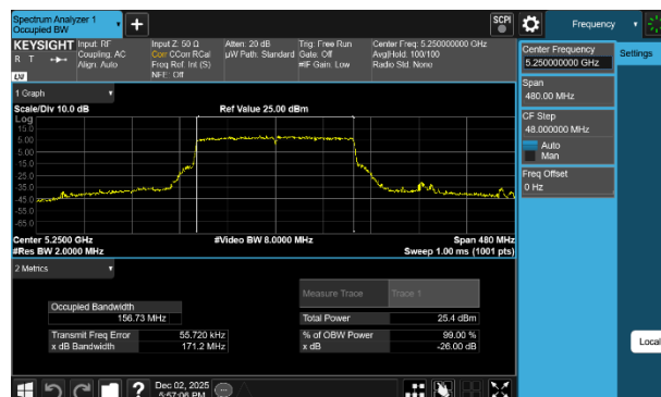
Plot 7-11 26dB BW & 99% OBW Antenna 5T (160MHz BW 802.11be(RU) RU996X2 Index68 - Ch.50)
