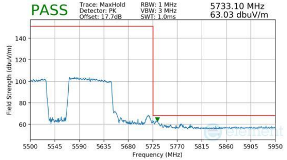
Plot 7-1139. CDD Diversity (Peak, RU996+484, Index 95 (L), Ch.114, MCS11)
