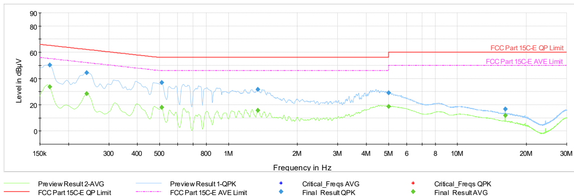
Plot 7-1186. AC Line Conducted Plot with 11be CDD Primary – RU242 – Ch.40 (L1) with AC/DC Adapter
