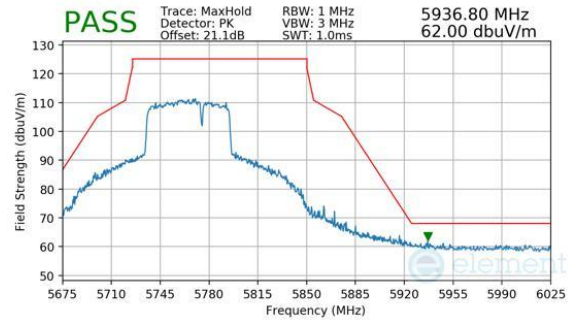
Plot 7-1108. CDD Diversity (Peak, RU484+242, Index 93, Ch.155, MCS11)
