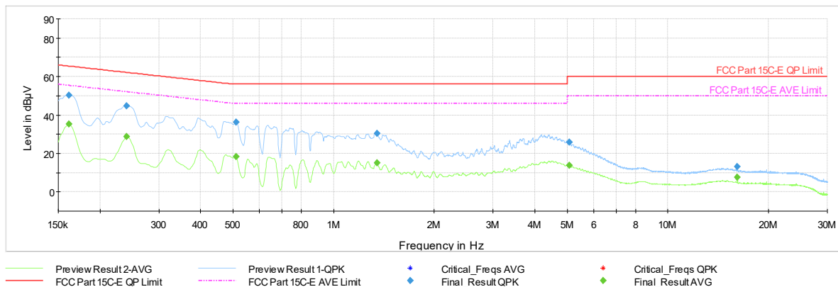
Plot 7-1185. AC Line Conducted Plot with 11be CDD Primary – RU78 – Ch.40 (N) with AC/DC Adapter
