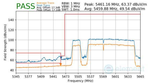
Plot 7-1158. CDD Diversity (Peak & Average, RU996+484+242, Index 97 (L), Ch.114, MCS11)
