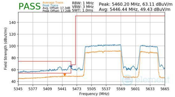
Plot 7-1133. CDD Diversity (Peak & Average, RU996+484, Index 94 (H), Ch.114, MCS11)
