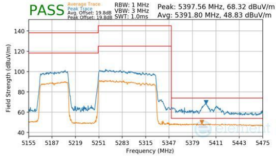
Plot 7-1130. CDD Diversity (Peak & Average, RU996+484, Index 95 (L), Ch.50, MCS11)
