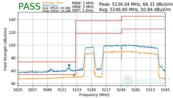
Plot 7-1142. CDD Diversity (Peak & Average, RU996+484+242, Index 97 (L), Ch.50, MCS11)
