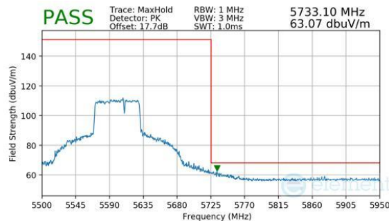
Plot 7-1100. CDD Diversity (Peak, RU484+242, Index 93, Ch.122, MCS11)
