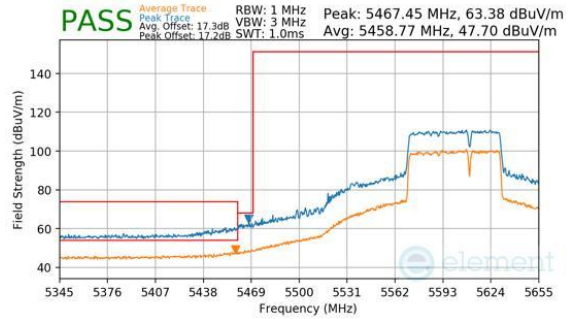
Plot 7-1096. CDD Diversity (Peak & Average, RU484+242, Index 93, Ch.122, MCS11)
