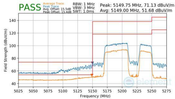
Plot 7-1083. CDD Diversity (Peak & Average, RU484+242, Index 92, Ch.42, MCS11)
