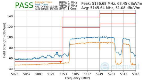
Plot 7-1144. CDD Diversity (Peak & Average, RU996+484+242, Index 98 (H), Ch.50, MCS11)
