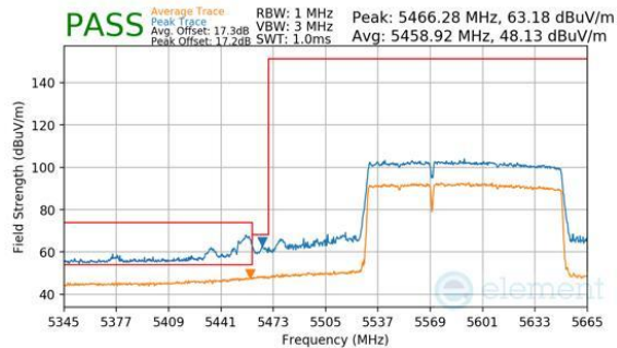
Plot 7-1132. CDD Diversity (Peak & Average, RU996+484, Index 94 (L), Ch.114, MCS11)
