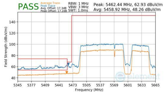
Plot 7-1159. CDD Diversity (Peak & Average, RU996+484+242, Index 97 (H), Ch.114, MCS11)
