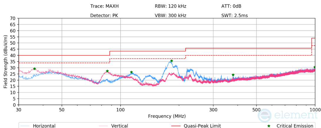
Plot 7-1176. RSE below 1GHz CDD Primary (RU26 – Ch.40), with AC/DC Adapter
