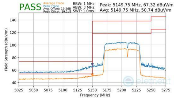
Plot 7-1084. CDD Diversity (Peak & Average, RU484+242, Index 93, Ch.42, MCS11)
