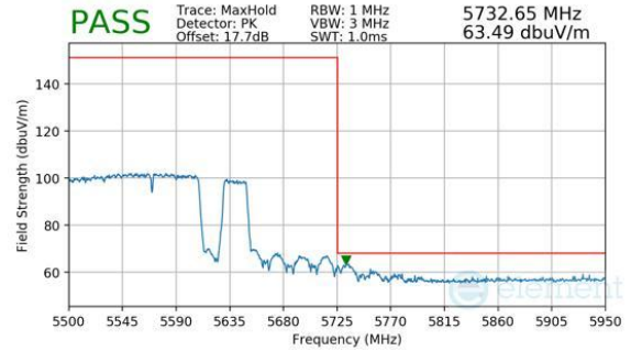
Plot 7-1169. CDD Diversity (Peak, RU996+484+242, Index 98 (H), Ch.114, MCS11)
