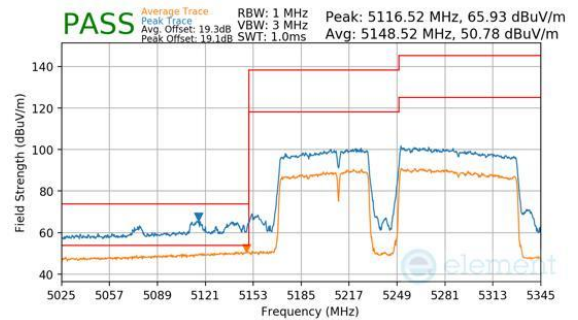
Plot 7-1146. CDD Diversity (Peak & Average, RU996+484+242, Index 99 (L), Ch.50, MCS11)
