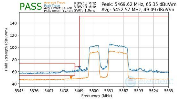
Plot 7-1090. CDD Diversity (Peak & Average, RU484+242, Index 91, Ch.106, MCS11)
