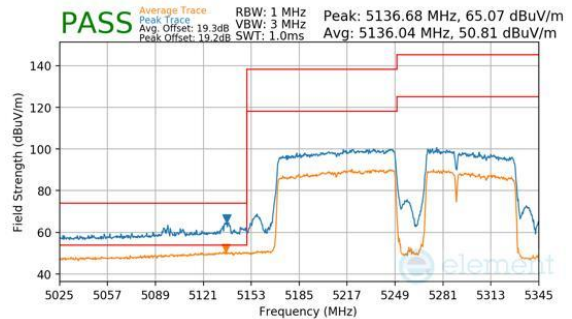
Plot 7-1141. CDD Diversity (Peak & Average, RU996+484+242, Index 96 (H), Ch.50, MCS11)
