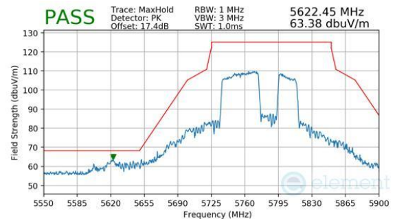
Plot 7-1103. CDD Diversity (Peak, RU484+242, Index 92, Ch.155, MCS11)
