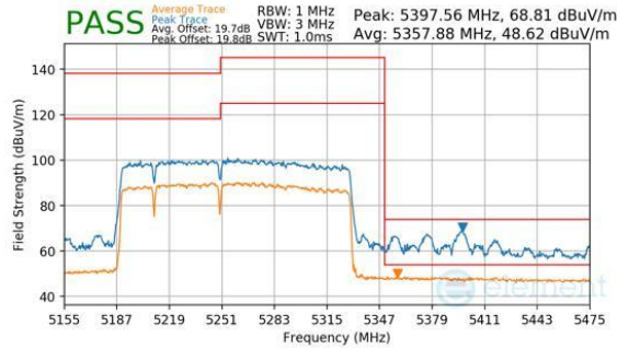
Plot 7-1148. CDD Diversity (Peak & Average, RU996+484+242, Index 96 (L), Ch.50, MCS11)
