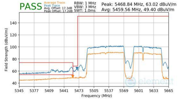
Plot 7-1157. CDD Diversity (Peak & Average, RU996+484+242, Index 96 (H), Ch.114, MCS11)
