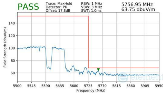
Plot 7-1167. CDD Diversity (Peak, RU996+484+242, Index 97 (H), Ch.114, MCS11)
