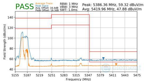
Plot 7-1118. CDD Diversity (Peak & Average, RU52, Index 37 (L), Ch.50, MCS11)
