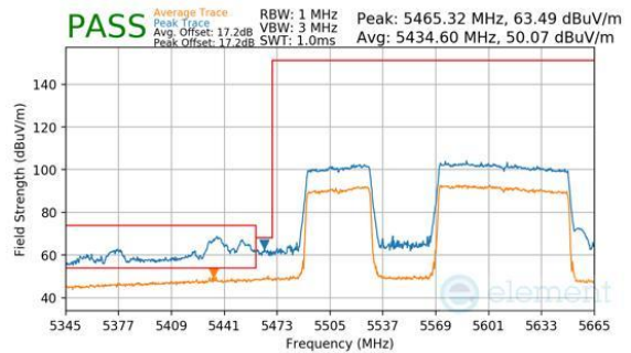
Plot 7-1134. CDD Diversity (Peak & Average, RU996+484, Index 95 (L), Ch.114, MCS11)
