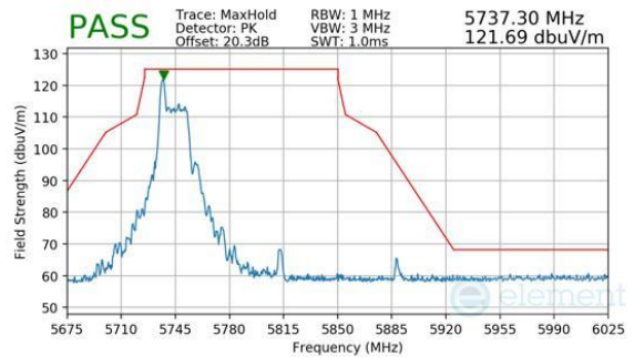
Plot 7-1073. CDD Diversity (Peak, RU26, Index 0, Ch.155, MCS11)
