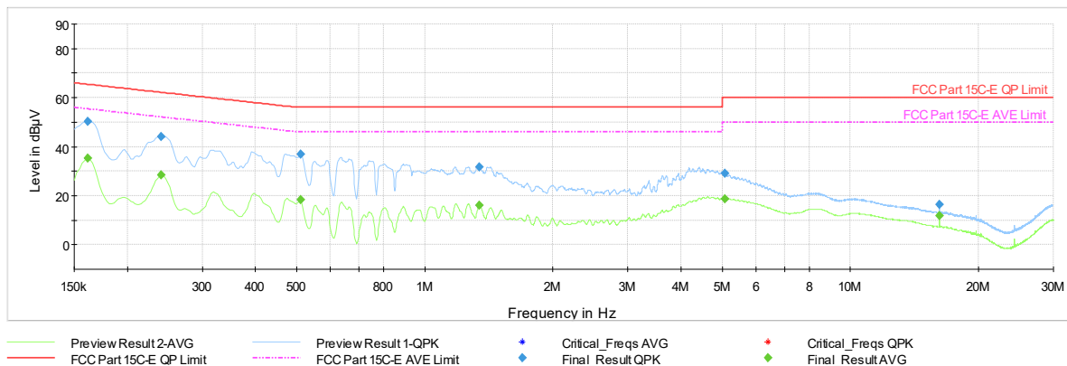
Plot 7-1190. AC Line Conducted Plot with 11be CDD Diversity – RU78 – Ch.40 (L1) with AC/DC Adapter
