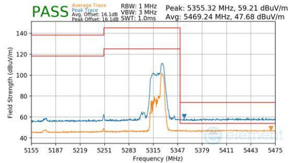
Plot 7-1119. CDD Diversity (Peak & Average, RU52, Index 52 (H), Ch.50, MCS11)
