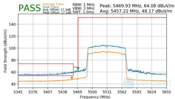
Plot 7-1111. CDD Diversity (Peak & Average, RU996, Index 67, Ch.106, MCS11)
