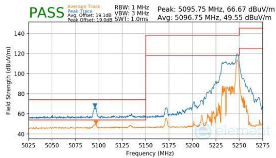
Plot 7-1070. CDD Diversity (Peak & Average, RU26, Index 36, Ch.42, MCS11)
