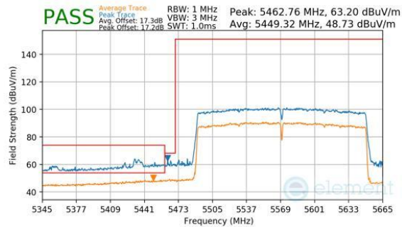
Plot 7-1174. CDD Diversity (Peak & Average, RU996X2, Index 68, Ch.114, MCS11)
