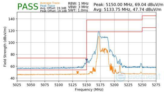
Plot 7-1069. CDD Diversity (Peak & Average, RU26, Index 0, Ch.42, MCS11)
