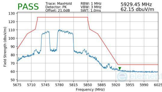
Plot 7-1106. CDD Diversity (Peak, RU484+242, Index 91, Ch.155, MCS11)
