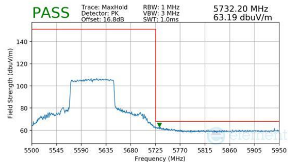
Plot 7-1113. CDD Diversity (Peak, RU996, Index 67, Ch.122, MCS11)
