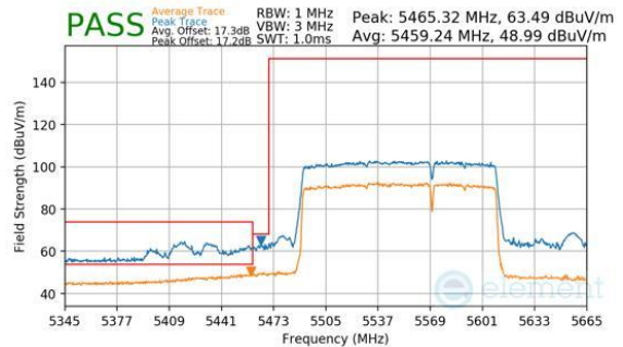
Plot 7-1135. CDD Diversity (Peak & Average, RU996+484, Index 95 (H), Ch.114, MCS11)
