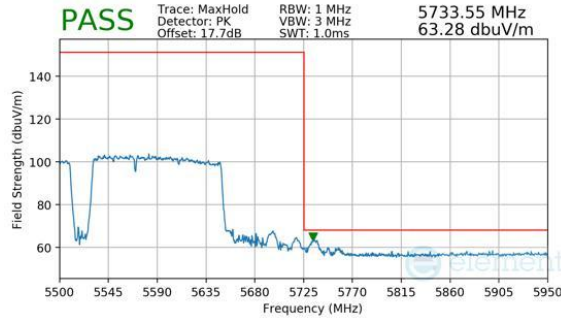
Plot 7-1166. CDD Diversity (Peak, RU996+484+242, Index 97 (L), Ch.114, MCS11)
