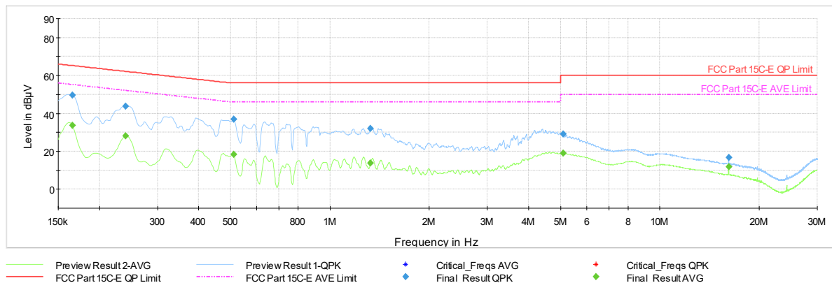
Plot 7-1184. AC Line Conducted Plot with 11be CDD Primary – RU78 – Ch.40 (L1) with AC/DC Adapter
