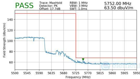
Plot 7-1138. CDD Diversity (Peak, RU996+484, Index 95 (H), Ch.114, MCS11)
