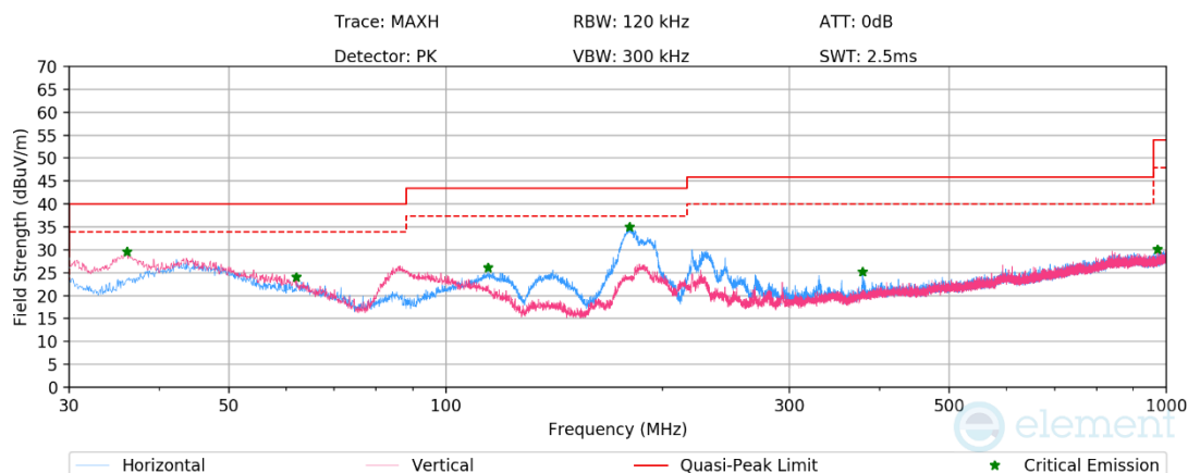
Plot 7-1181. RSE below 1GHz CDD Diversity (RU242 – Ch.40), with AC/DC Adapter
