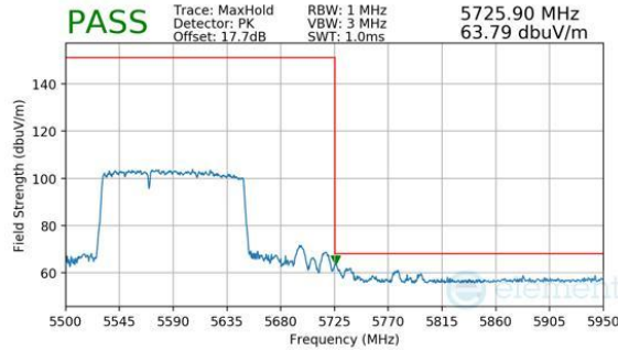
Plot 7-1136. CDD Diversity (Peak, RU996+484, Index 94 (L), Ch.114, MCS11)
