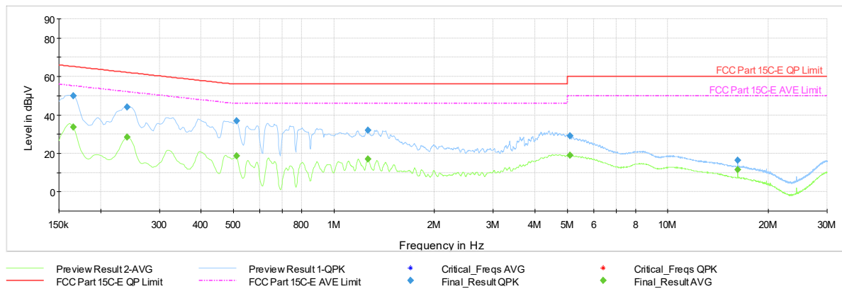
Plot 7-1192. AC Line Conducted Plot with 11be CDD Diversity – RU242 – Ch.40 (L1) with AC/DC Adapter
