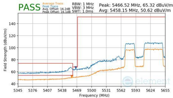
Plot 7-1094. CDD Diversity (Peak & Average, RU484+242, Index 91, Ch.122, MCS11)
