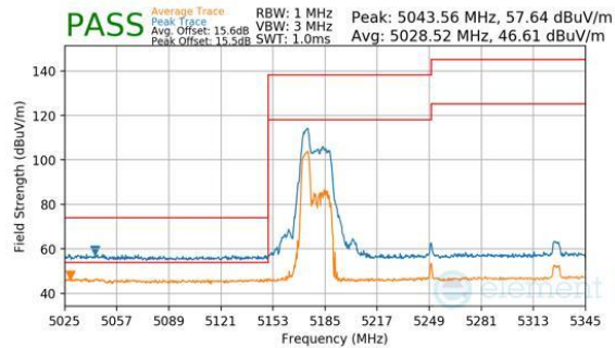
Plot 7-1116. CDD Diversity (Peak & Average, RU52, Index 37 (L), Ch.50, MCS11)
