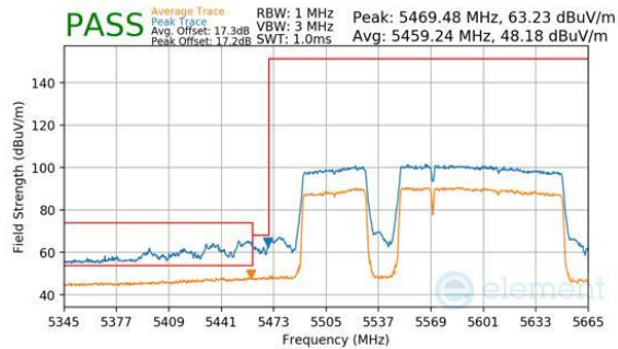
Plot 7-1160. CDD Diversity (Peak & Average, RU996+484+242, Index 98 (L), Ch.114, MCS11)
