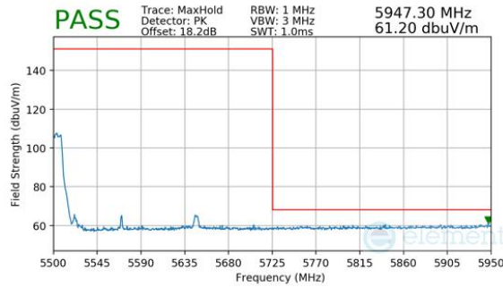
Plot 7-1122. CDD Diversity (Peak, RU52, Index 37 (L), Ch.114, MCS11)
