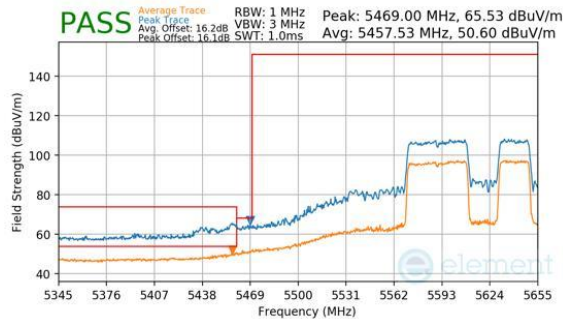
Plot 7-1095. CDD Diversity (Peak & Average, RU484+242, Index 92, Ch.122, MCS11)
