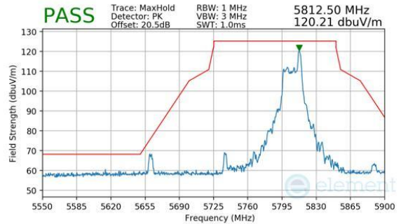
Plot 7-1072. CDD Diversity (Peak, RU26, Index 36, Ch.155, MCS11)
