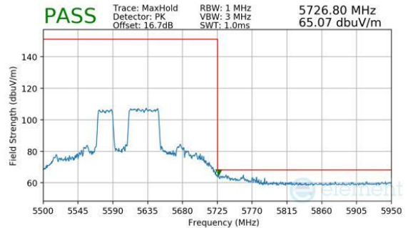
Plot 7-1098. CDD Diversity (Peak, RU484+242, Index 91, Ch.122, MCS11)
