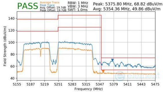
Plot 7-1154. CDD Diversity (Peak & Average, RU996+484+242, Index 99 (L), Ch.50, MCS11)
