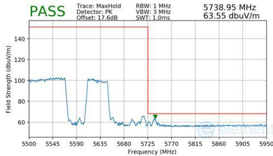
Plot 7-1137. CDD Diversity (Peak, RU996+484, Index 94 (H), Ch.114, MCS11)
