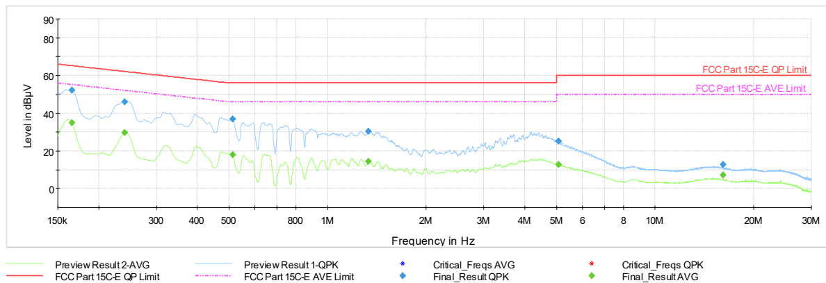
Plot 7-1183. AC Line Conducted Plot with 11be CDD Primary – RU26 – Ch.40 (N) with AC/DC Adapter
