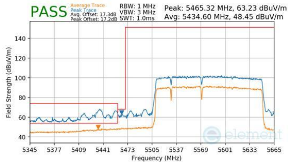
Plot 7-1156. CDD Diversity (Peak & Average, RU996+484+242, Index 96 (L), Ch.114, MCS11)
