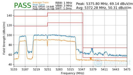
Plot 7-1150. CDD Diversity (Peak & Average, RU996+484+242, Index 97 (L), Ch.50, MCS11)
