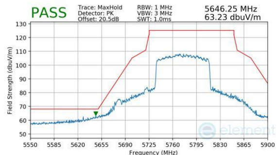
Plot 7-1114. CDD Diversity (Peak, RU996, Index 67, Ch.155, MCS11)
