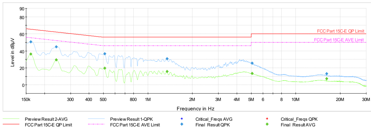
Plot 7-1191. AC Line Conducted Plot with 11be CDD Diversity – RU78 – Ch.40 (N) with AC/DC Adapter
