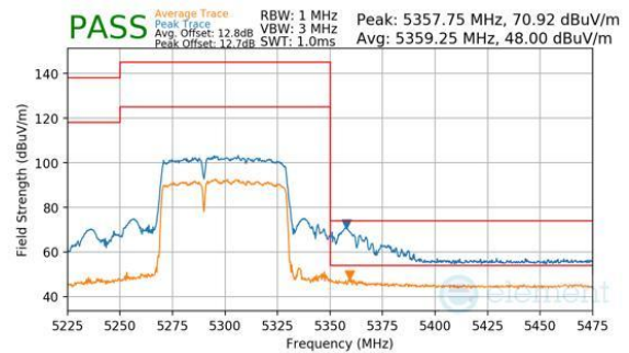
Plot 7-1085. CDD Diversity (Peak & Average, RU484+242, Index 90, Ch.58, MCS11)
