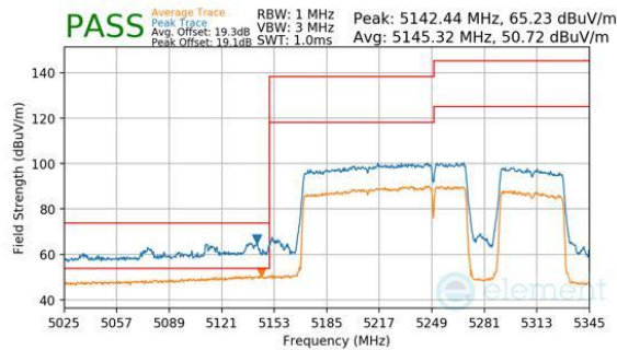
Plot 7-1143. CDD Diversity (Peak & Average, RU996+484+242, Index 97 (H), Ch.50, MCS11)
