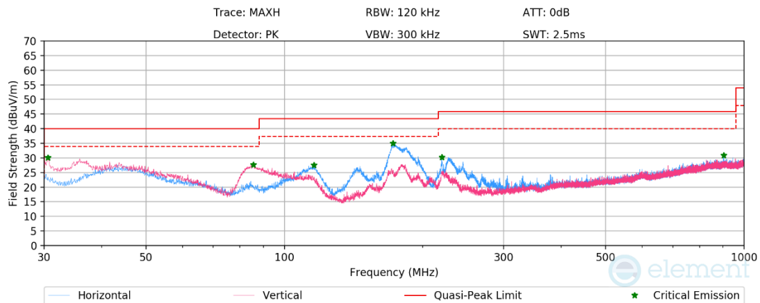
Plot 7-1180. RSE below 1GHz CDD Diversity (RU78 – Ch.40), with AC/DC Adapter
