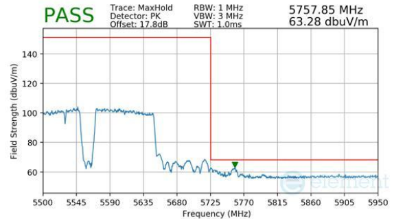
Plot 7-1171. CDD Diversity (Peak, RU996+484+242, Index 99 (L), Ch.114, MCS11)
