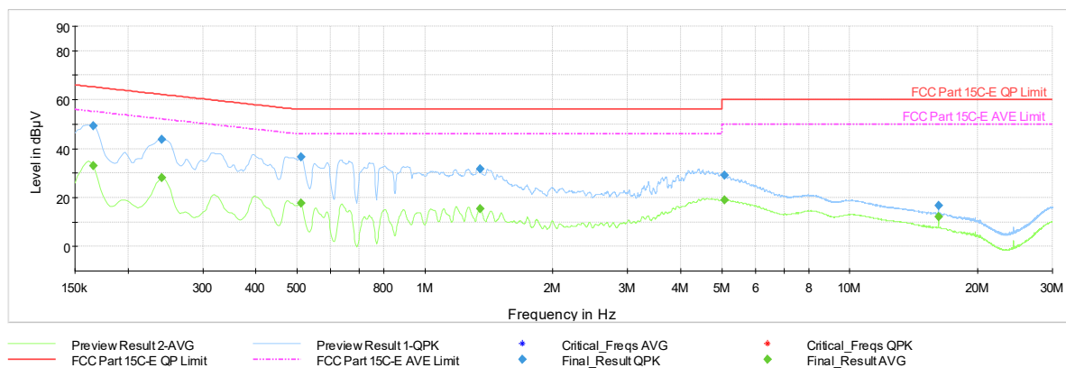
Plot 7-1188. AC Line Conducted Plot with 11be CDD Diversity – RU26 – Ch.40 (L1) with AC/DC Adapter
