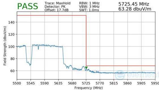
Plot 7-1168. CDD Diversity (Peak, RU996+484+242, Index 98 (L), Ch.114, MCS11)
