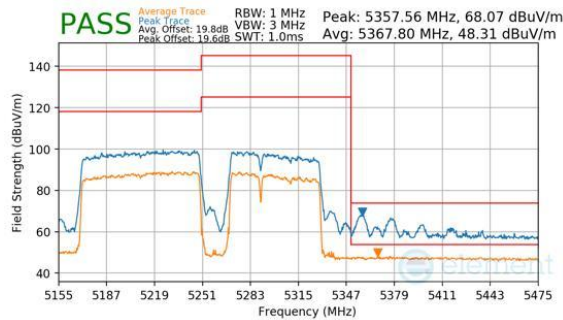
Plot 7-1149. CDD Diversity (Peak & Average, RU996+484+242, Index 96 (H), Ch.50, MCS11)
