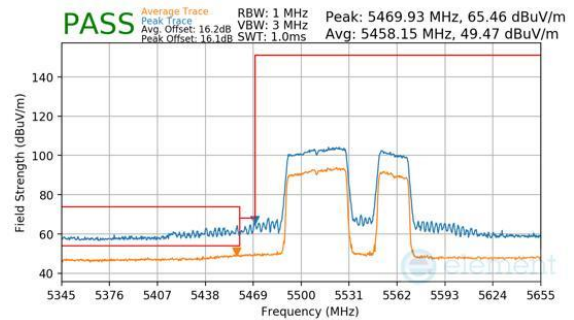
Plot 7-1091. CDD Diversity (Peak & Average, RU484+242, Index 92, Ch.106, MCS11)
