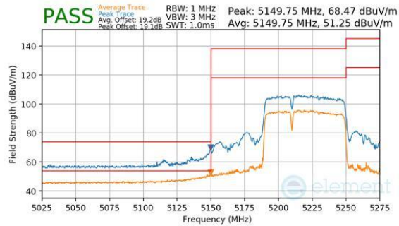
Plot 7-1081. CDD Diversity (Peak & Average, RU484+242, Index 90, Ch.42, MCS11)
