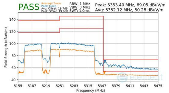
Plot 7-1152. CDD Diversity (Peak & Average, RU996+484+242, Index 98 (L), Ch.50, MCS11)
