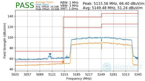
Plot 7-1172. CDD Diversity (Peak & Average, RU996X2, Index 68, Ch.50, MCS11)
