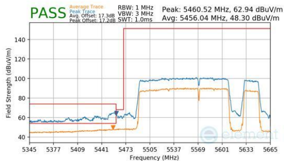
Plot 7-1161. CDD Diversity (Peak & Average, RU996+484+242, Index 98 (H), Ch.114, MCS11)
