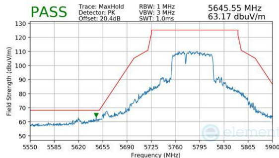
Plot 7-1101. CDD Diversity (Peak, RU484+242, Index 90, Ch.155, MCS11)
