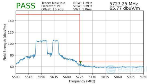
Plot 7-1099. CDD Diversity (Peak, RU484+242, Index 92, Ch.122, MCS11)
