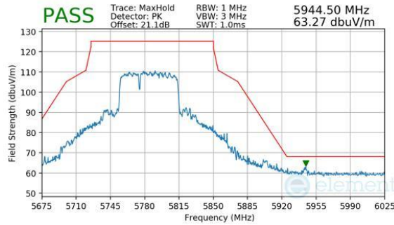
Plot 7-1105. CDD Diversity (Peak, RU484+242, Index 90, Ch.155, MCS11)
