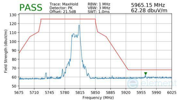
Plot 7-1074. CDD Diversity (Peak, RU26, Index 36, Ch.155, MCS11)
