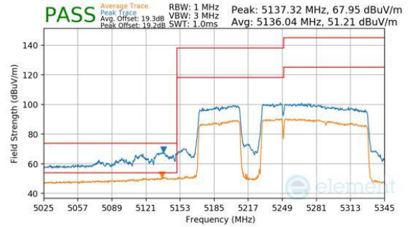
Plot 7-1145. CDD Diversity (Peak & Average, RU996+484+242, Index 98 (L), Ch.50, MCS11)
