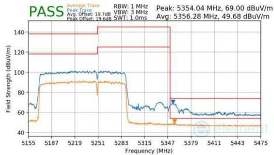
Plot 7-1131. CDD Diversity (Peak & Average, RU996+484, Index 95 (H), Ch.50, MCS11)
