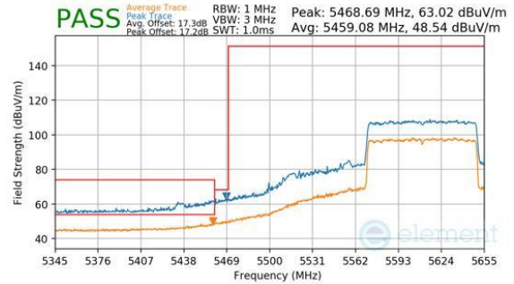
Plot 7-1112. CDD Diversity (Peak & Average, RU996, Index 67, Ch.122, MCS11)
