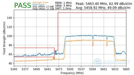
Plot 7-1163. CDD Diversity (Peak & Average, RU996+484+242, Index 99 (H), Ch.114, MCS11)
