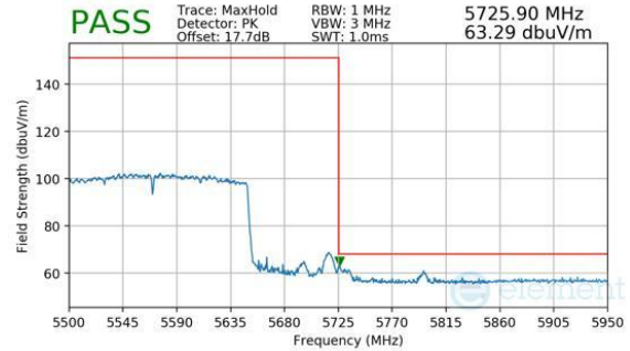
Plot 7-1175. CDD Diversity (Peak, RU996X2, Index 68, Ch.114, MCS11)
