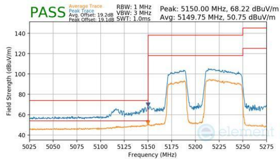
Plot 7-1082. CDD Diversity (Peak & Average, RU484+242, Index 91, Ch.42, MCS11)
