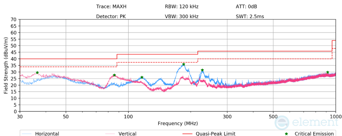
Plot 7-1179. RSE below 1GHz CDD Diversity (RU26 – Ch.40), with AC/DC Adapter
