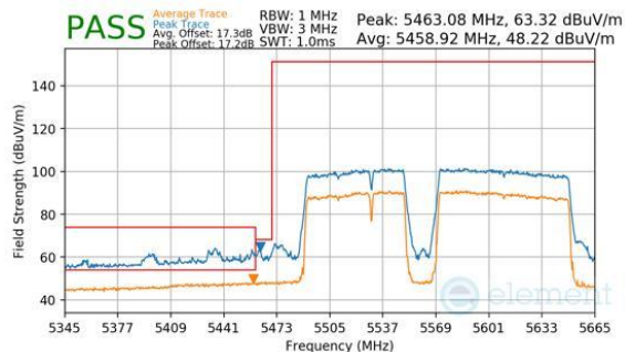
Plot 7-1162. CDD Diversity (Peak & Average, RU996+484+242, Index 99 (L), Ch.114, MCS11)
