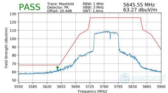
Plot 7-1104. CDD Diversity (Peak, RU484+242, Index 93, Ch.155, MCS11)
