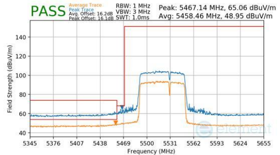
Plot 7-1092. CDD Diversity (Peak & Average, RU484+242, Index 93, Ch.106, MCS11)
