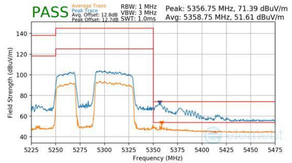
Plot 7-1086. CDD Diversity (Peak & Average, RU484+242, Index 91, Ch.58, MCS11)
