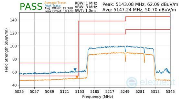
Plot 7-1147. CDD Diversity (Peak & Average, RU996+484+242, Index 99 (H), Ch.50, MCS11)
