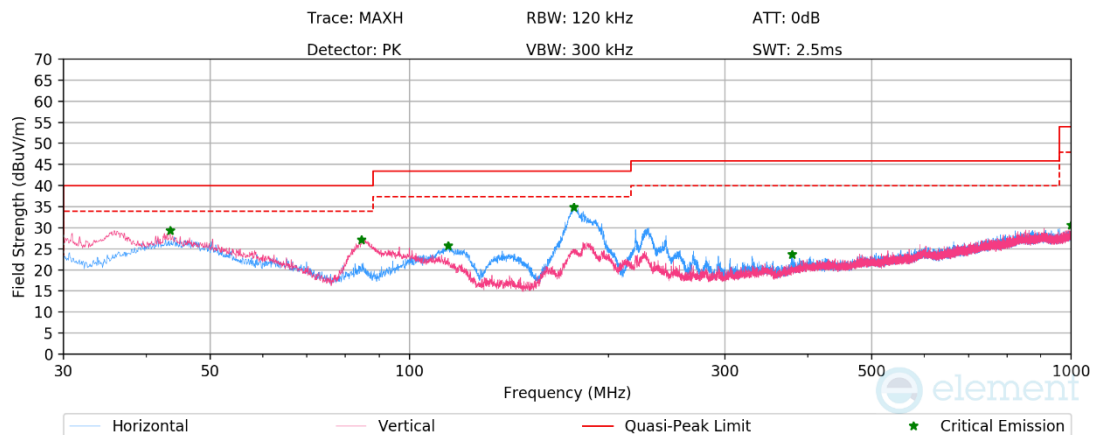
Plot 7-1178. RSE below 1GHz CDD Primary (RU242 – Ch.40), with AC/DC Adapter
