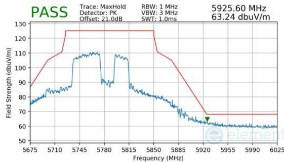
Plot 7-1107. CDD Diversity (Peak, RU484+242, Index 92, Ch.155, MCS11)
