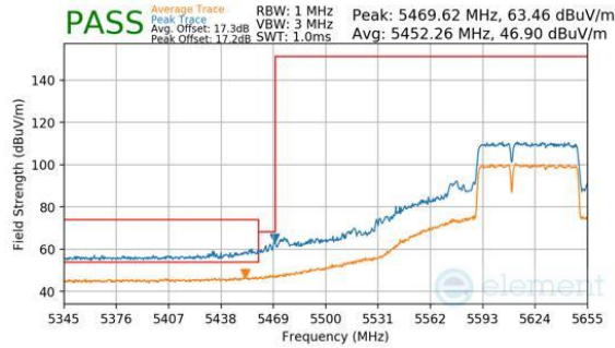
Plot 7-1093. CDD Diversity (Peak & Average, RU484+242, Index 90, Ch.122, MCS11)
