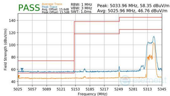
Plot 7-1117. CDD Diversity (Peak & Average, RU52, Index 52 (H), Ch.50, MCS11)
