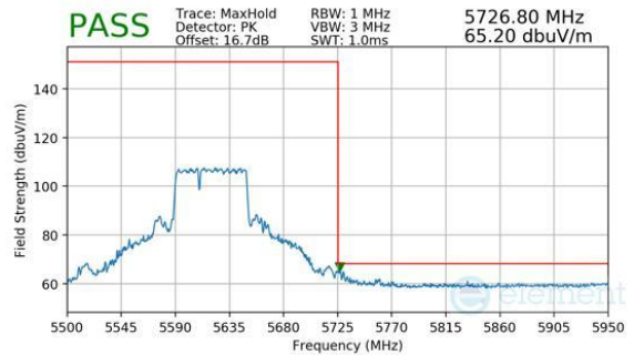
Plot 7-1097. CDD Diversity (Peak, RU484+242, Index 90, Ch.122, MCS11)
