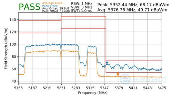
Plot 7-1153. CDD Diversity (Peak & Average, RU996+484+242, Index 98 (H), Ch.50, MCS11)
