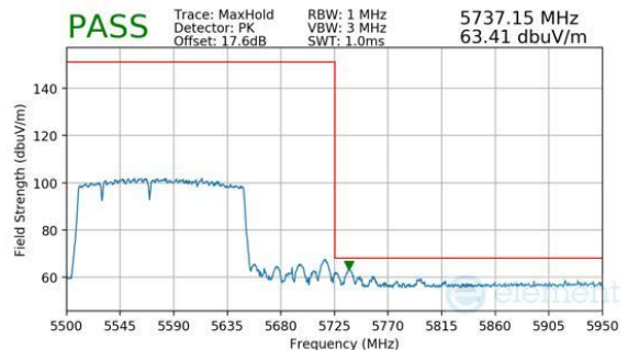
Plot 7-1165. CDD Diversity (Peak, RU996+484+242, Index 96 (L), Ch.114, MCS11)
