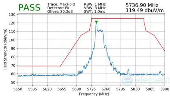
Plot 7-1071. CDD Diversity (Peak, RU26, Index 0, Ch.155, MCS11)
