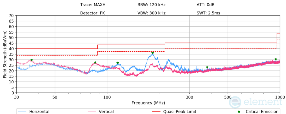
Plot 7-1177. RSE below 1GHz CDD Primary (RU78 – Ch.40), with AC/DC Adapter
