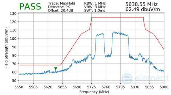
Plot 7-1102. CDD Diversity (Peak, RU484+242, Index 91, Ch.155, MCS11)
