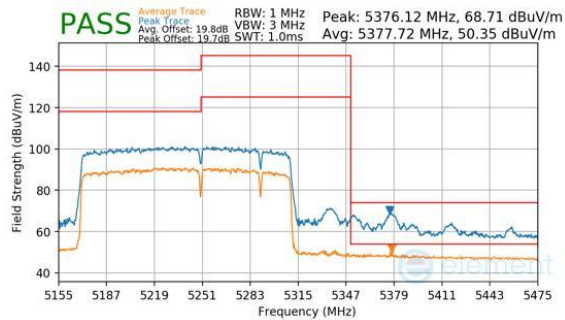
Plot 7-1155. CDD Diversity (Peak & Average, RU996+484+242, Index 99 (H), Ch.50, MCS11)
