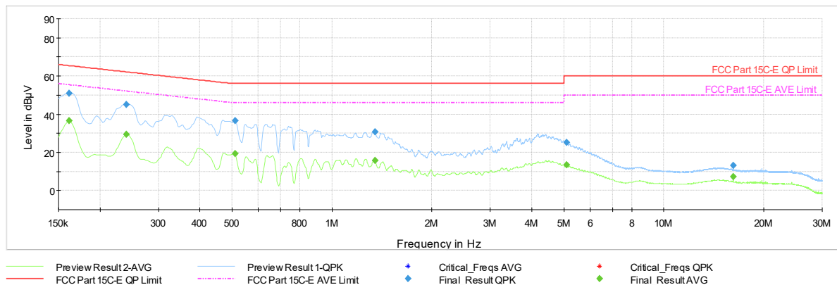
Plot 7-1193. AC Line Conducted Plot with 11be CDD Diversity – RU242 – Ch.40 (N) with AC/DC Adapter
