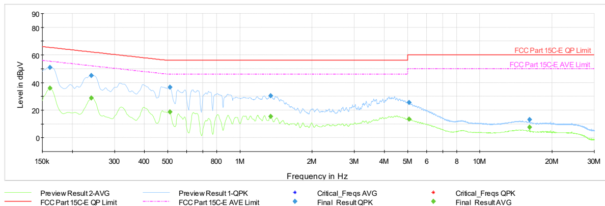
Plot 7-1187. AC Line Conducted Plot with 11be CDD Primary – RU242 – Ch.40 (N) with AC/DC Adapter
