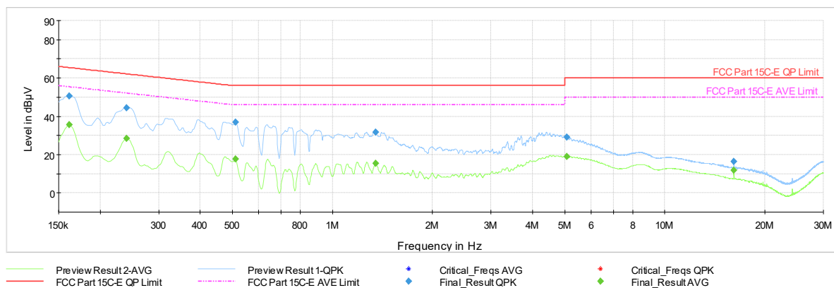
Plot 7-1182. AC Line Conducted Plot with 11be CDD Primary – RU26 – Ch.40 (L1) with AC/DC Adapter
