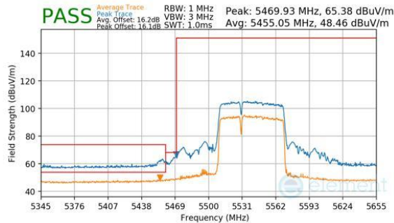
Plot 7-1089. CDD Diversity (Peak & Average, RU484+242, Index 90, Ch.106, MCS11)
