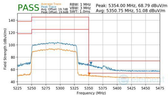
Plot 7-1110. CDD Diversity (Peak & Average, RU996, Index 67, Ch.58, MCS11)
