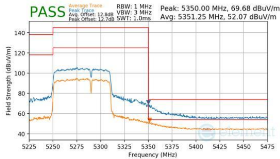
Plot 7-1088. CDD Diversity (Peak & Average, RU484+242, Index 93, Ch.58, MCS11)
