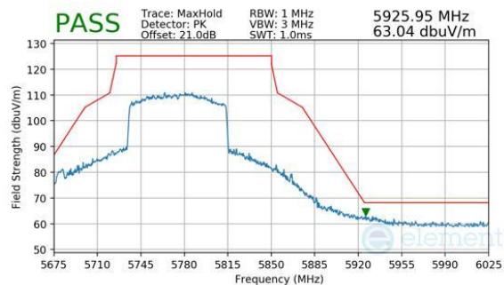
Plot 7-1115. CDD Diversity (Peak, RU996, Index 67, Ch.155, MCS11)
