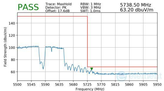
Plot 7-1164. CDD Diversity (Peak, RU996+484+242, Index 96 (H), Ch.114, MCS11)
