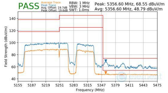
Plot 7-1151. CDD Diversity (Peak & Average, RU996+484+242, Index 97 (H), Ch.50, MCS11)
