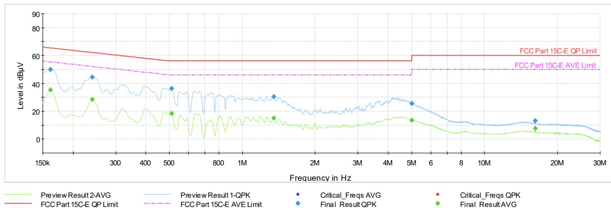
Plot 7-1189. AC Line Conducted Plot with 11be CDD Diversity – RU26 – Ch.40 (N) with AC/DC Adapter
