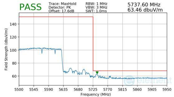
Plot 7-1170. CDD Diversity (Peak, RU996+484+242, Index 99 (H), Ch.114, MCS11)
