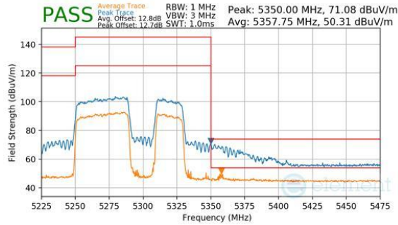
Plot 7-1087. CDD Diversity (Peak & Average, RU484+242, Index 92, Ch.58, MCS11)
