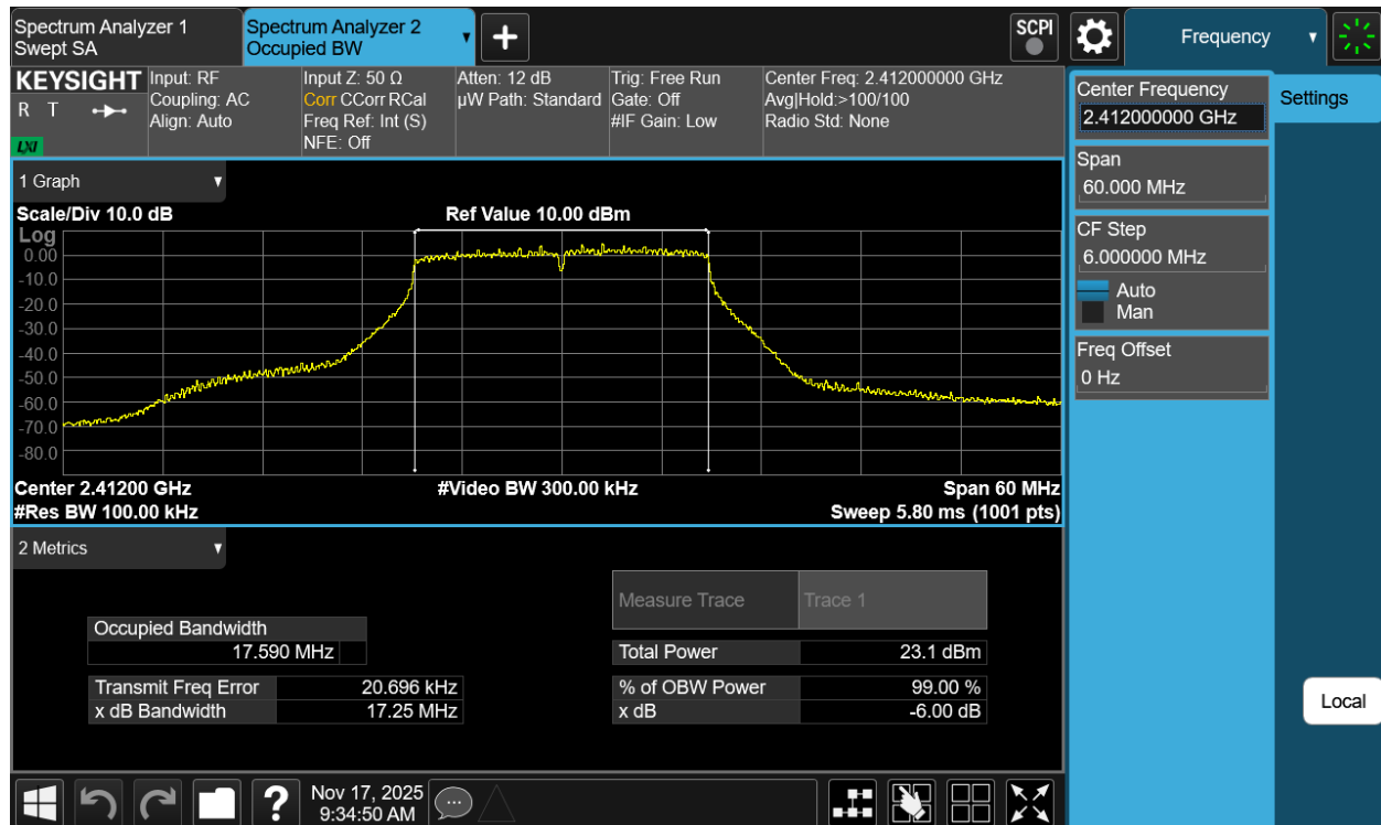
Plot 7-14 6dB OBW Antenna 1a (20MHz BW 802.11g - Ch.1)
