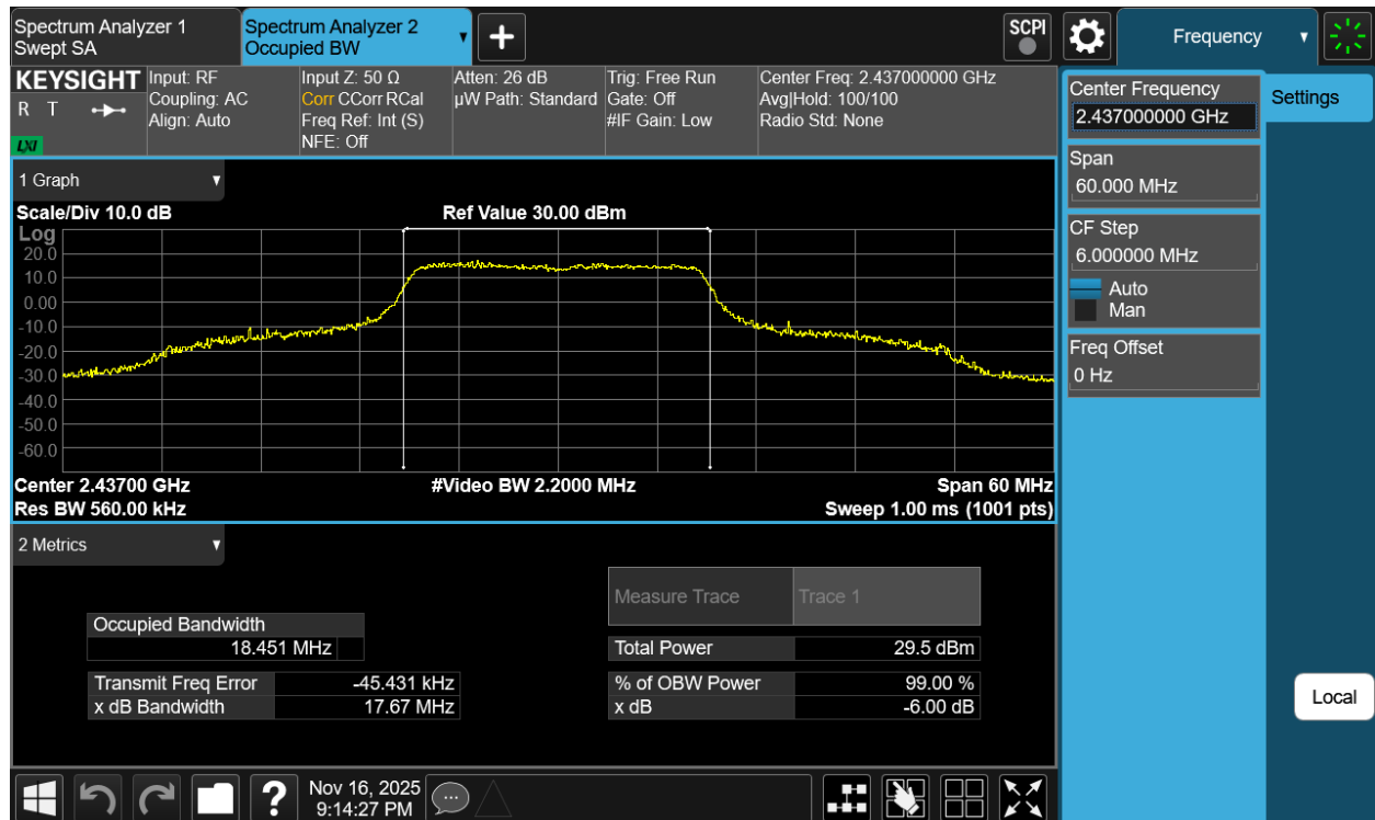
Plot 7-2 99% OBW Antenna 3a (20MHz BW 802.11g - Ch.6)
