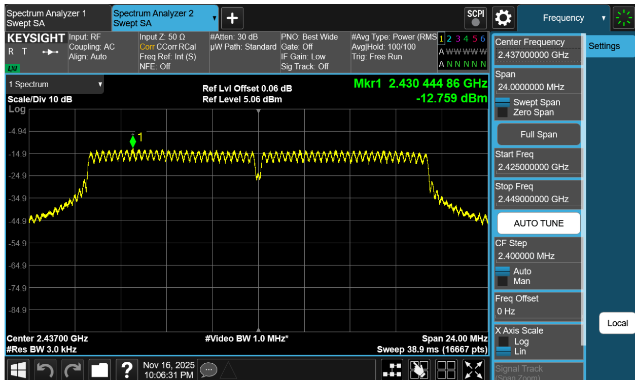
Plot 7-18 PSD Antenna 3a (20MHz BW 802.11g - Ch.6)
