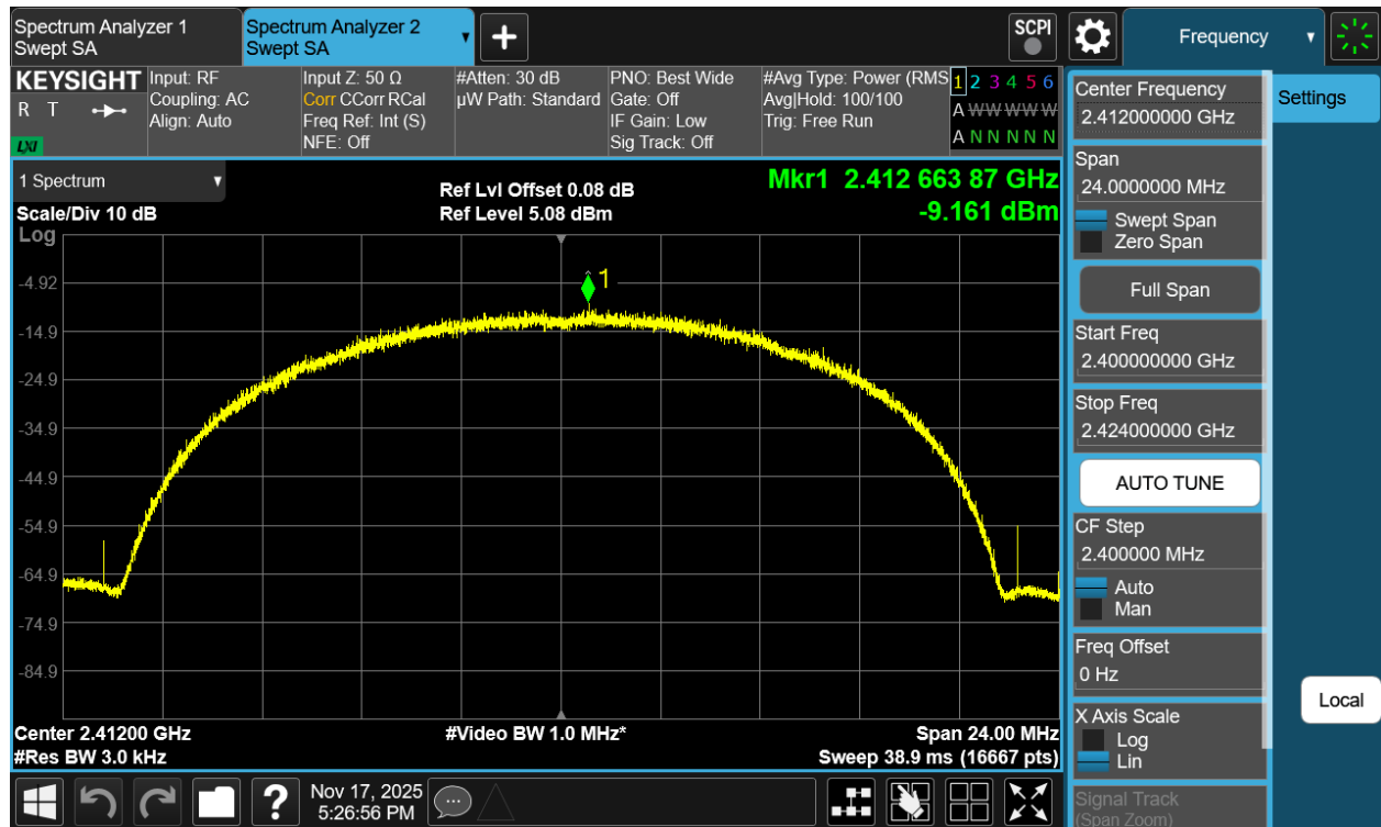
Plot 7-29 PSD CDD Antenna 1a (20MHz BW 802.11b - Ch.1)
