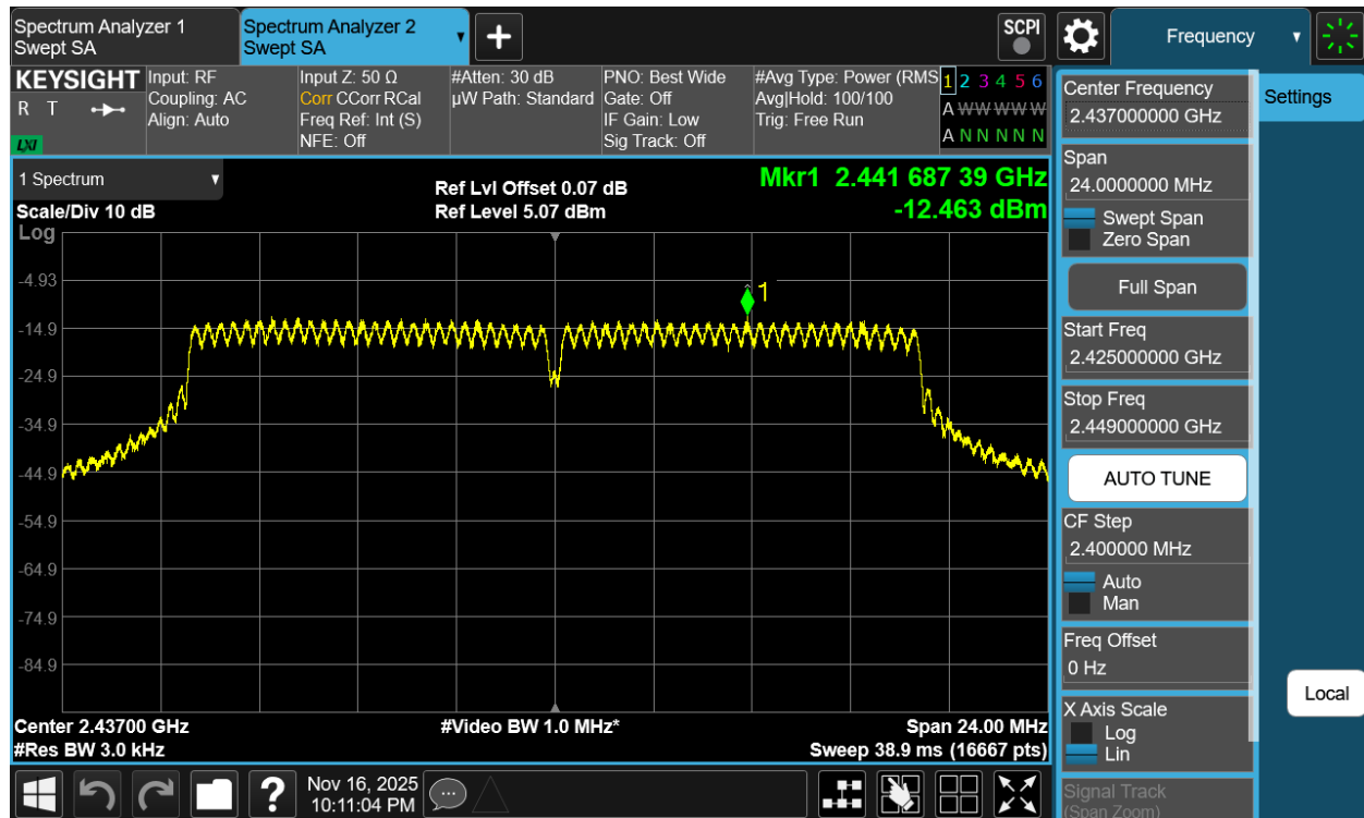
Plot 7-19 PSD Antenna 3a (20MHz BW 802.11n - Ch.6)
