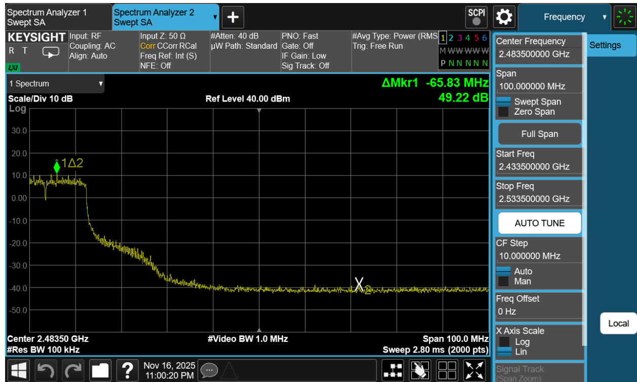
Plot 7-43. Band Edge Plot Antenna 3a (802.11g – Ch. 6)
