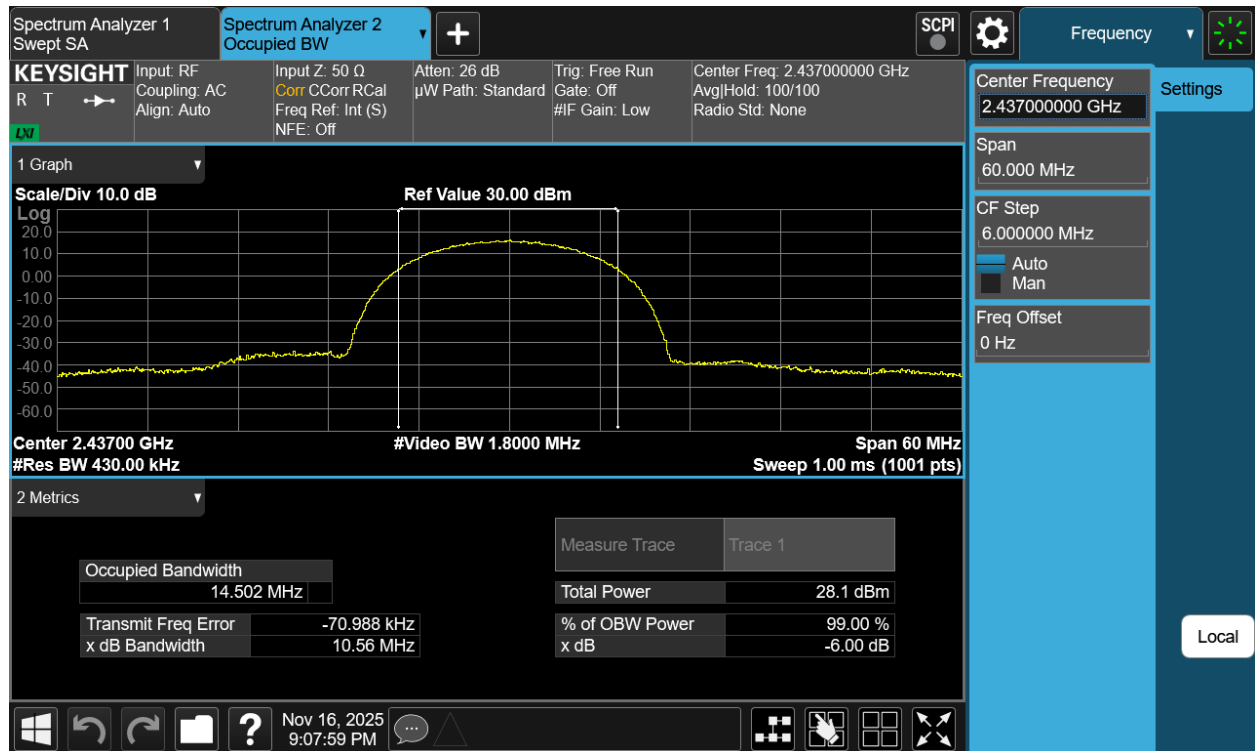
Plot 7-1 99% OBW Antenna 3a (20MHz BW 802.11b - Ch.6)
