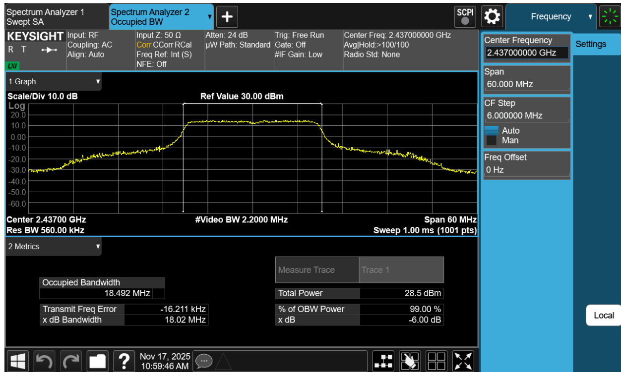
Plot 7-7 99% OBW Antenna 1a (20MHz BW 802.11n - Ch.6)
