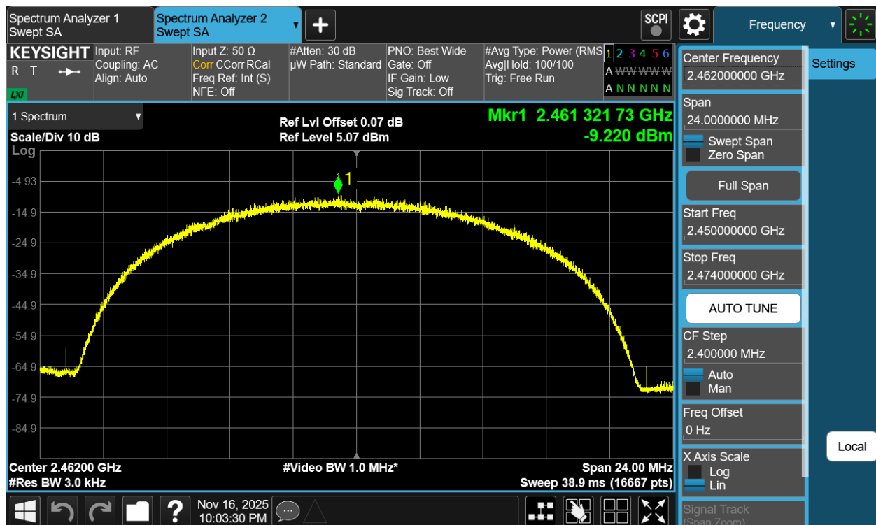
Plot 7-17 PSD Antenna 3a (20MHz BW 802.11b - Ch.11)
