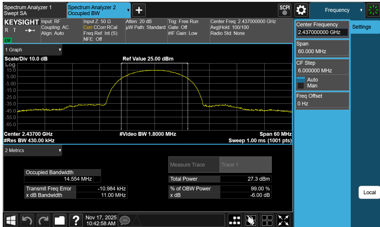
Plot 7-5 99% OBW Antenna 1a (20MHz BW 802.11b - Ch.6)
