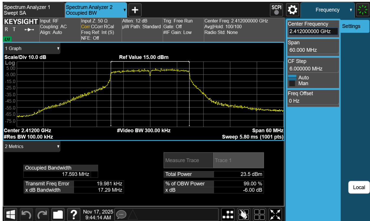
Plot 7-15 6dB OBW Antenna 1a (20MHz BW 802.11n - Ch.1)
