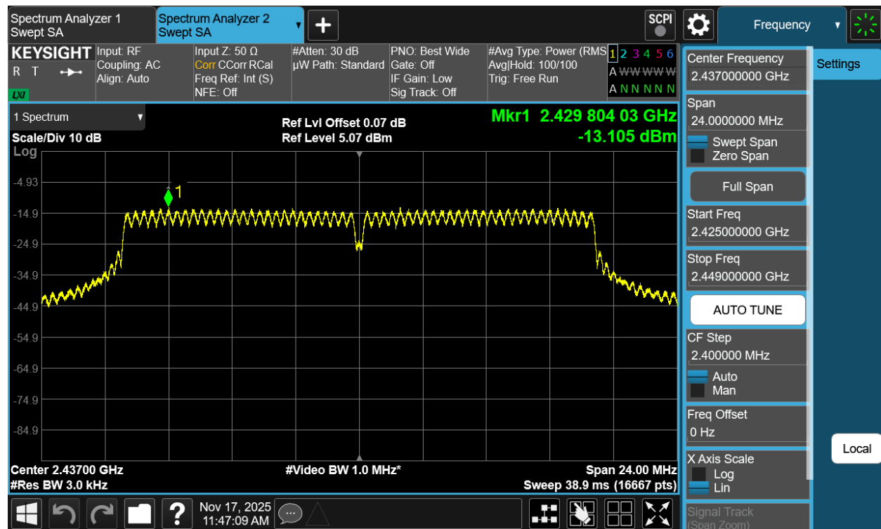
Plot 7-22 PSD Antenna 1a (20MHz BW 802.11g - Ch.6)
