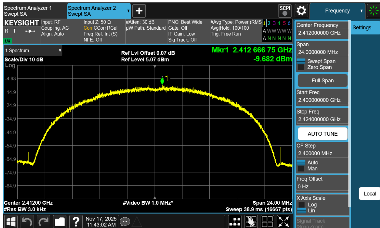
Plot 7-21 PSD Antenna 1a (20MHz BW 802.11b - Ch.1)
