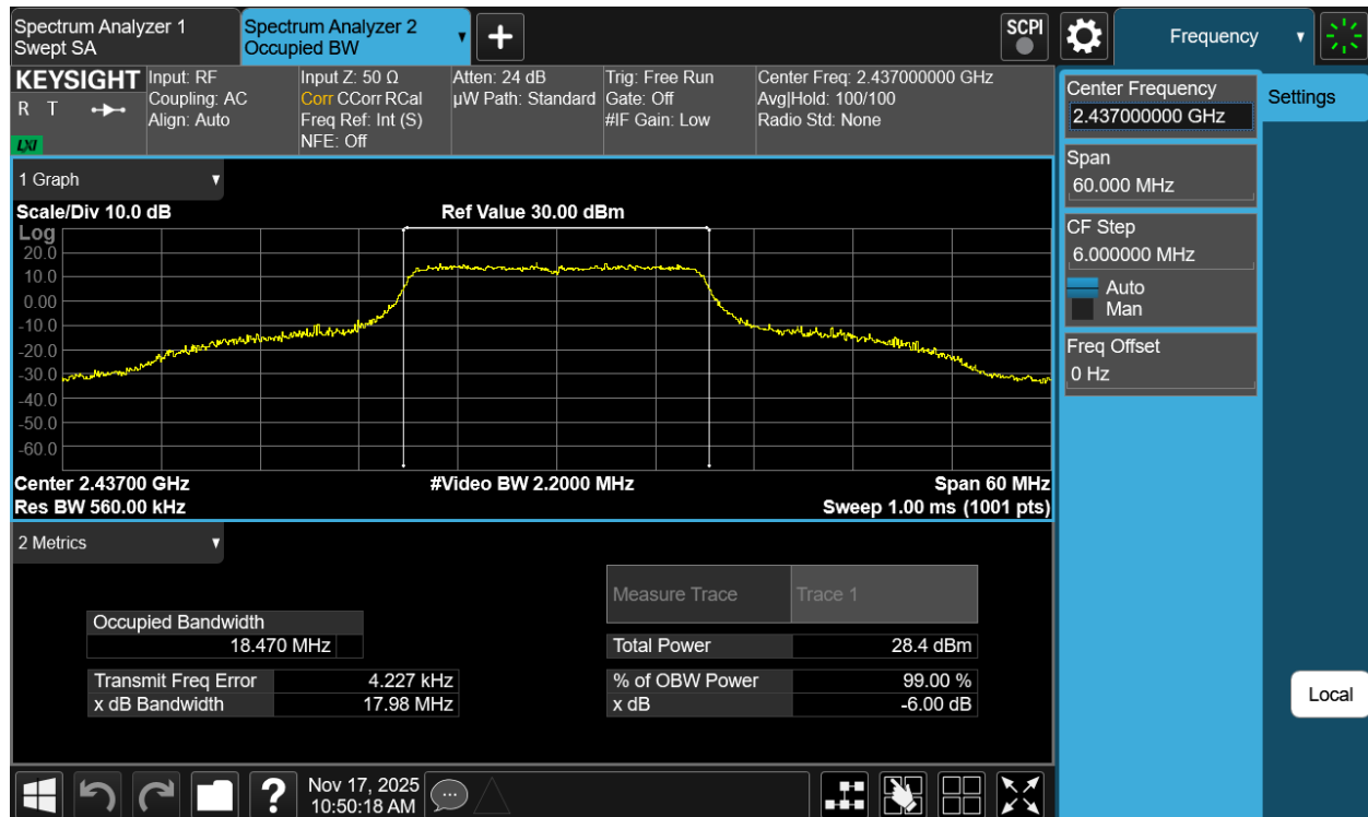
Plot 7-6 99% OBW Antenna 1a (20MHz BW 802.11g - Ch.6)
