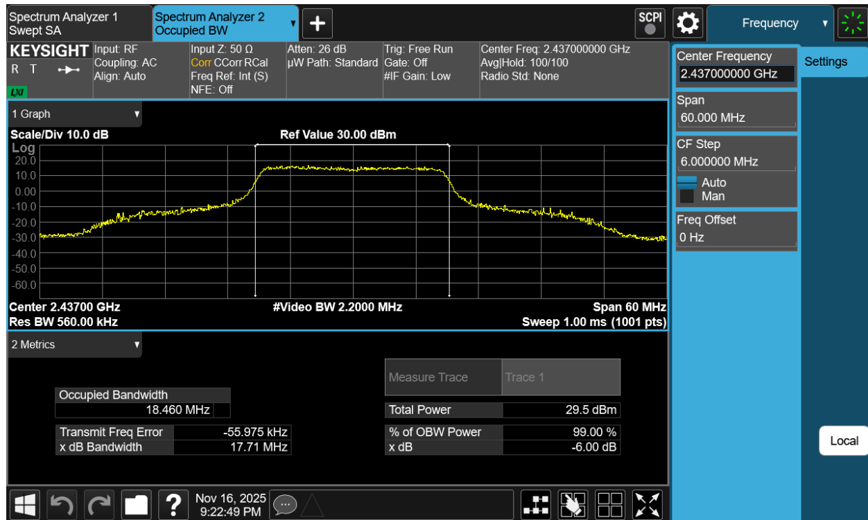
Plot 7-3 99% OBW Antenna 3a (20MHz BW 802.11n - Ch.6)
