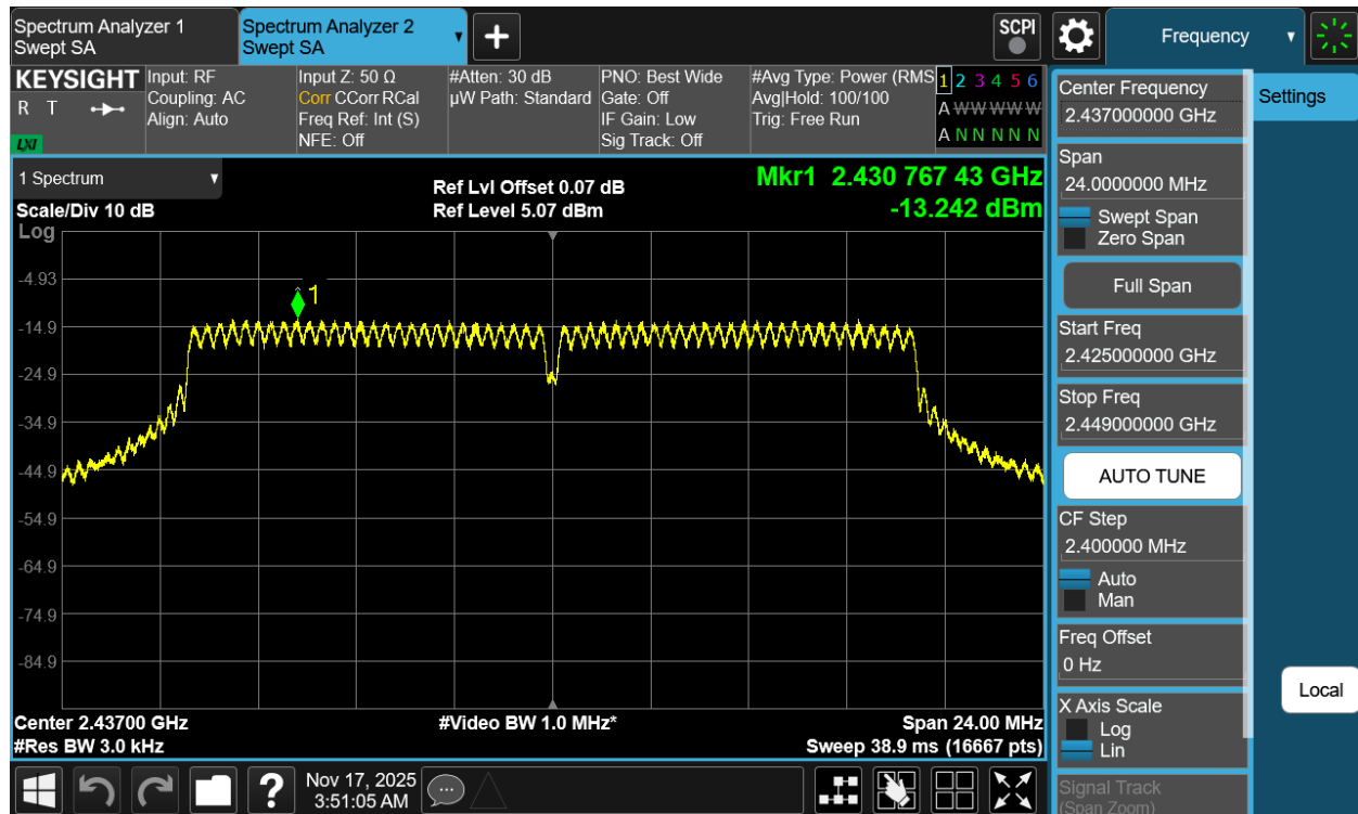
Plot 7-27 PSD CDD Antenna 3a (20MHz BW 802.11n - Ch.6)
