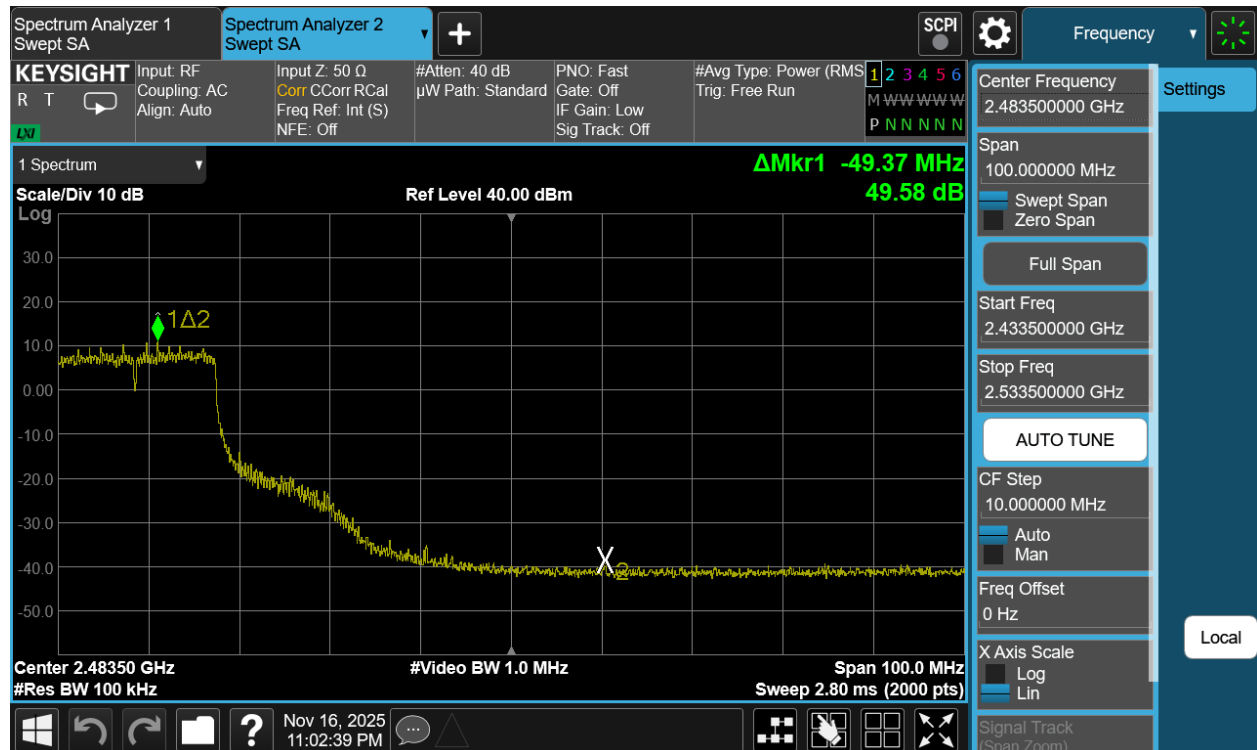
Plot 7-44. Band Edge Plot Antenna 3a (802.11g – Ch. 7)
