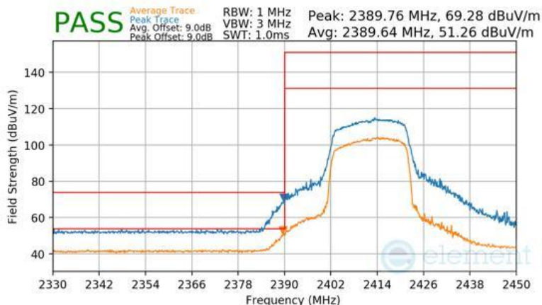
Plot 7-167 Radiated Restricted Lower Band Edge Measurement Antenna 3a
