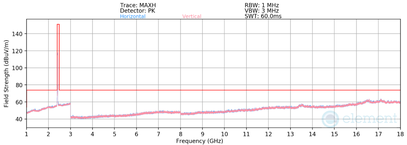
Plot 7-137. Radiated Spurious Emissions Above 1GHz CDD (802.11b – Ch. 1)
