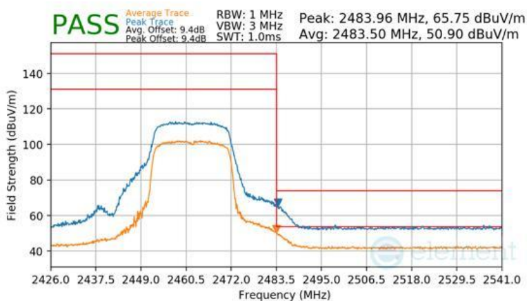
Plot 7-178 Radiated Restricted Upper Band Edge Measurement Antenna 3a
