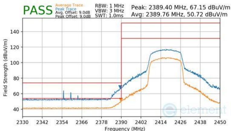
Plot 7-168 Radiated Restricted Lower Band Edge Measurement Antenna 3a
