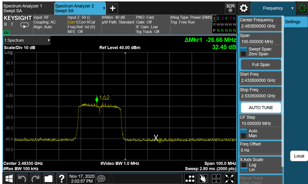
Plot 7-124. Band Edge Plot Antenna 1a (802.11be (SU - 2.4GHz) – Ch. 13)
