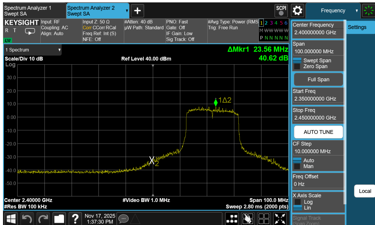
Plot 7-113. Band Edge Plot Antenna 1a (802.11be (SU - 2.4GHz) – Ch. 3)
