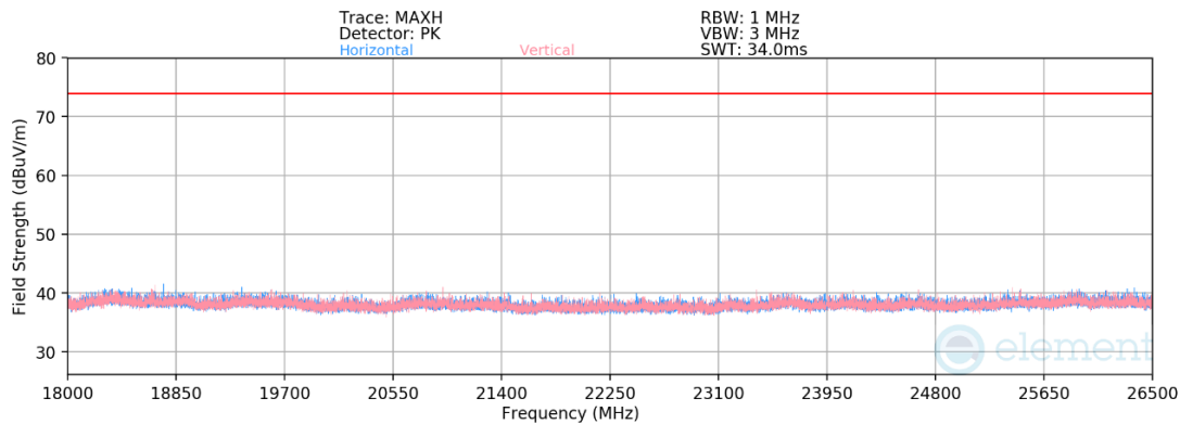
Plot 7-143. Radiated Spurious Emissions Above 18GHz CDD (802.11n – Ch.6)
