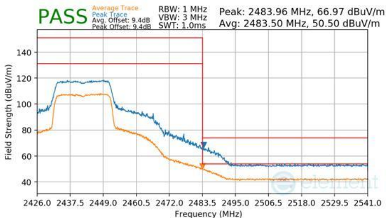
Plot 7-174 Radiated Restricted Upper Band Edge Measurement Antenna 3a
