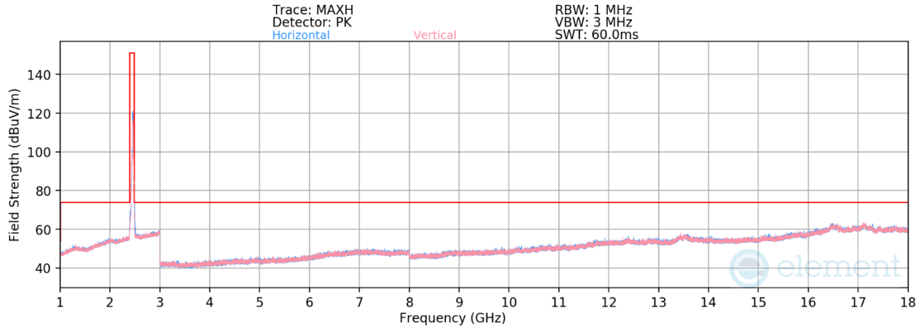
Plot 7-148. Radiated Spurious Emissions above 1GHz CDD (802.11be (SU) – Ch. 11)
