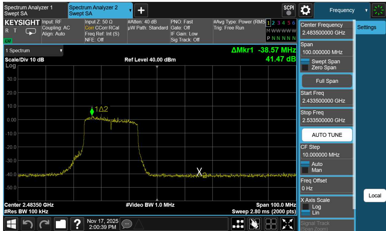
Plot 7-123. Band Edge Plot Antenna 1a (802.11be (SU - 2.4GHz) – Ch. 12)
