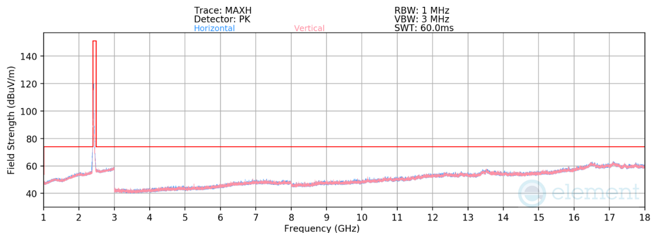
Plot 7-141. Radiated Spurious Emissions Above 1GHz CDD (802.11n – Ch. 1)
