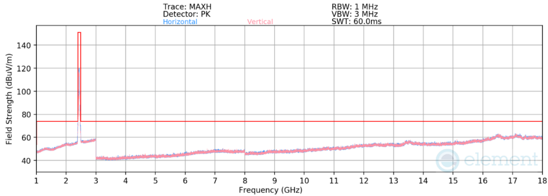
Plot 7-142. Radiated Spurious Emissions Above 1GHz CDD (802.11n – Ch. 6)
