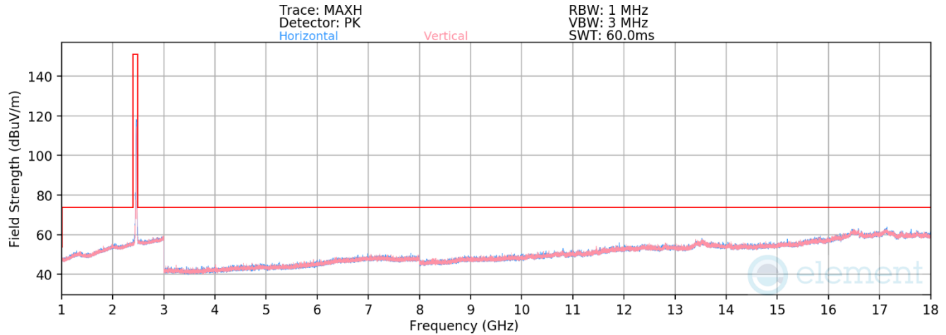
Plot 7-140. Radiated Spurious Emissions Above 1GHz CDD (802.11b – Ch. 11)
