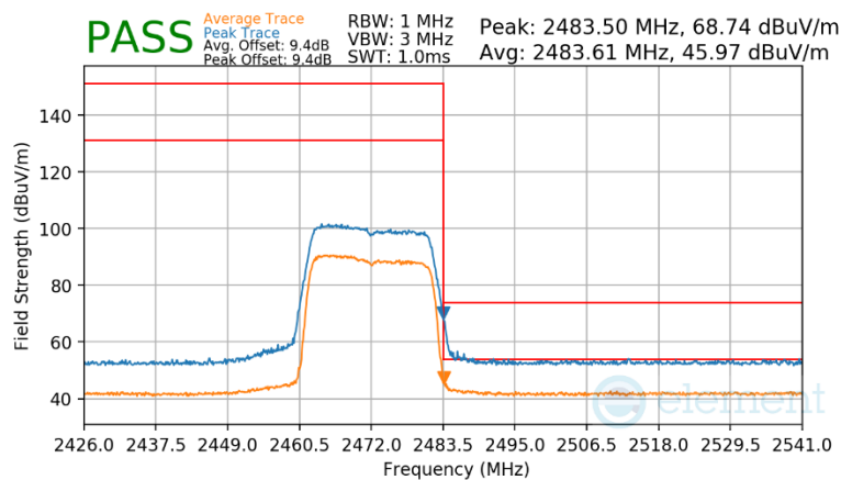
Plot 7-180 Radiated Restricted Upper Band Edge Measurement Antenna 3a
