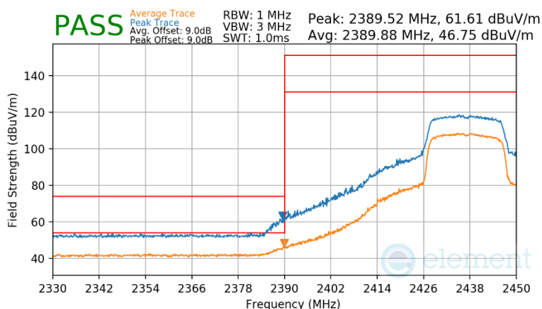
Plot 7-172 Radiated Restricted Lower Band Edge Measurement Antenna 3a
