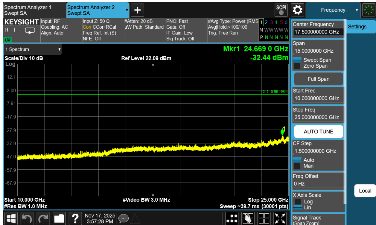
Plot 7-134. Conducted Spurious Plot Antenna 1a (802.11b – Ch. 6)
