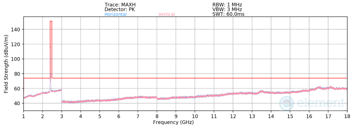
Plot 7-138. Radiated Spurious Emissions Above 1GHz CDD (802.11b – Ch. 6)
