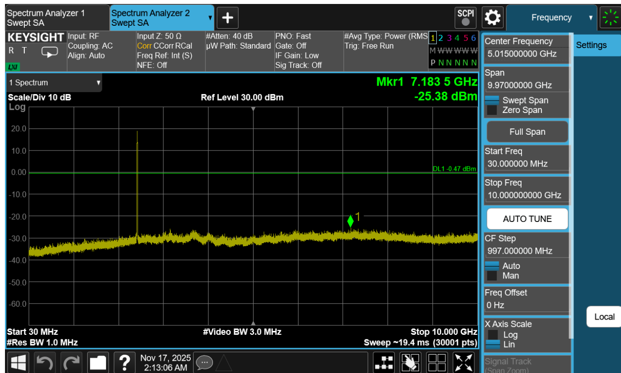
Plot 7-127. Conducted Spurious Plot Antenna 3a (802.11b – Ch. 6)
