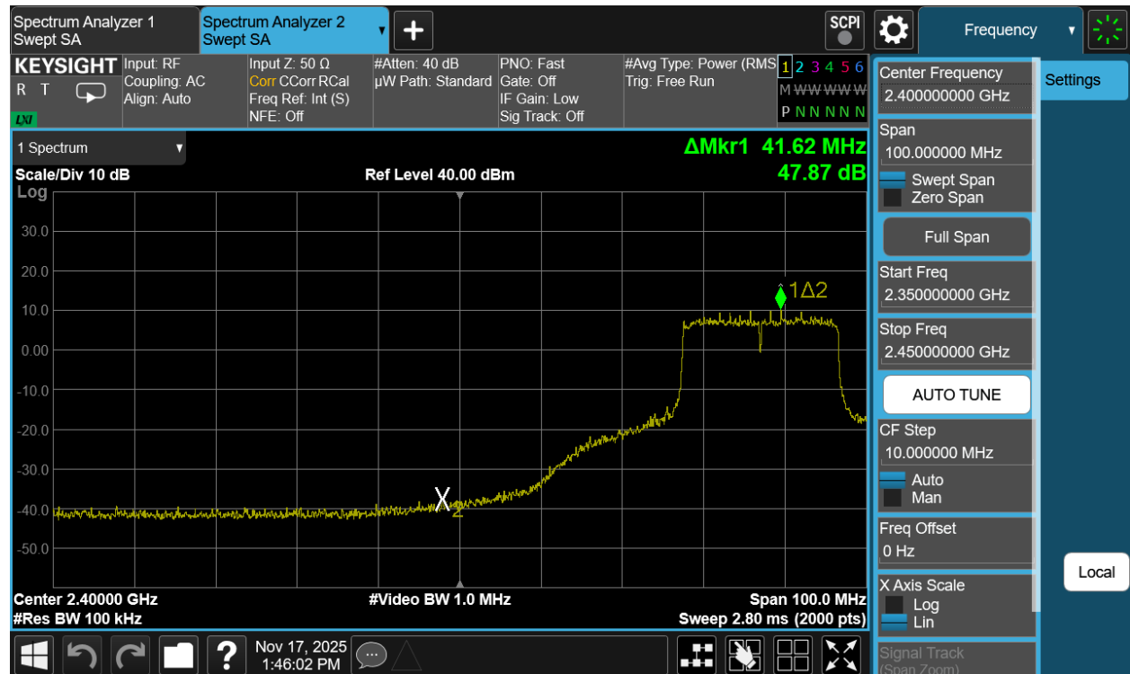
Plot 7-116. Band Edge Plot Antenna 1a (802.11be (SU - 2.4GHz) – Ch. 6(Low))
