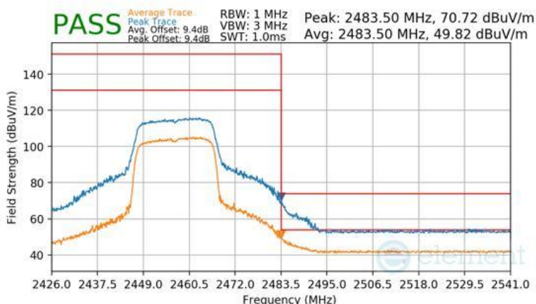
Plot 7-177 Radiated Restricted Upper Band Edge Measurement Antenna 3a
