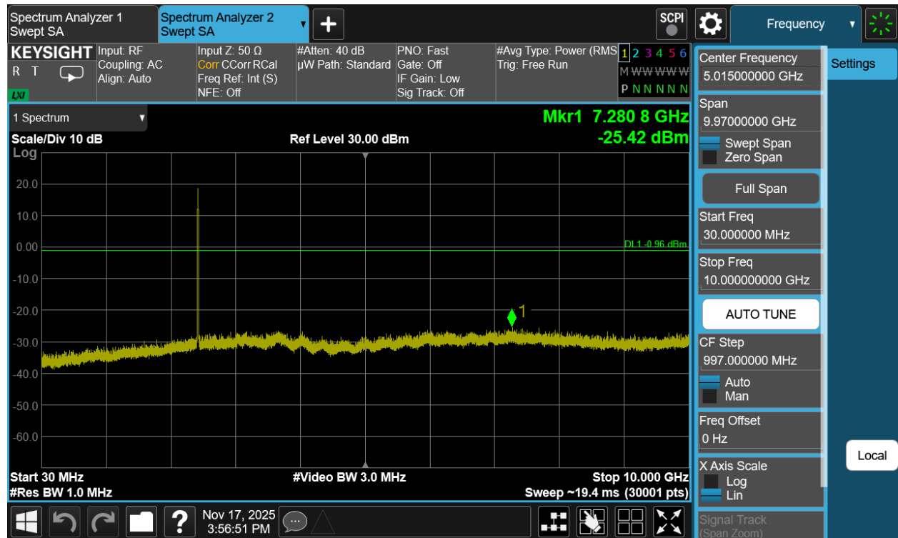
Plot 7-133. Conducted Spurious Plot Antenna 1a (802.11b – Ch. 6)
