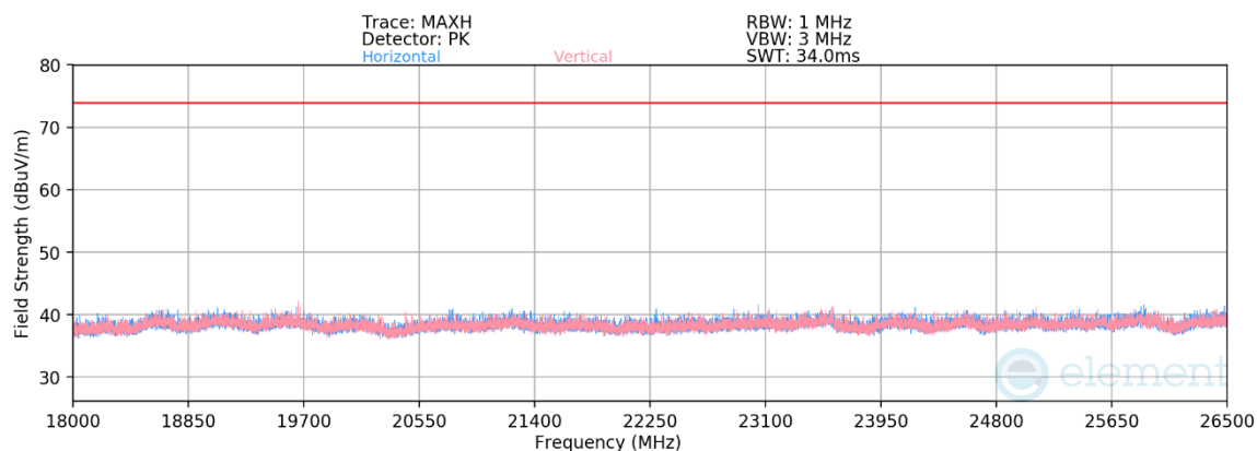
Plot 7-139. Radiated Spurious Emissions Above 18GHz CDD (802.11b – Ch.6)
