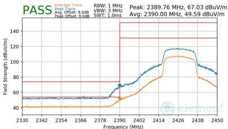
Plot 7-170 Radiated Restricted Lower Band Edge Measurement Antenna 3a
