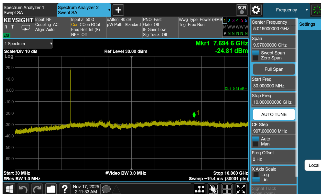
Plot 7-125. Conducted Spurious Plot Antenna 3a (802.11b – Ch. 1)
