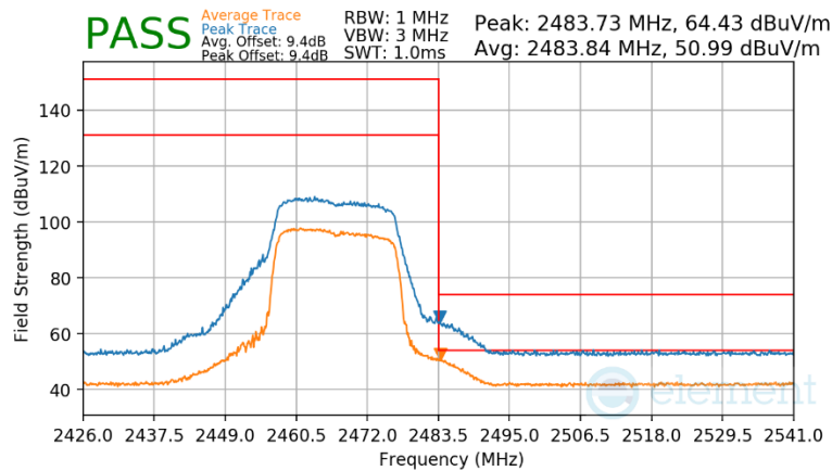
Plot 7-179 Radiated Restricted Upper Band Edge Measurement Antenna 3a
