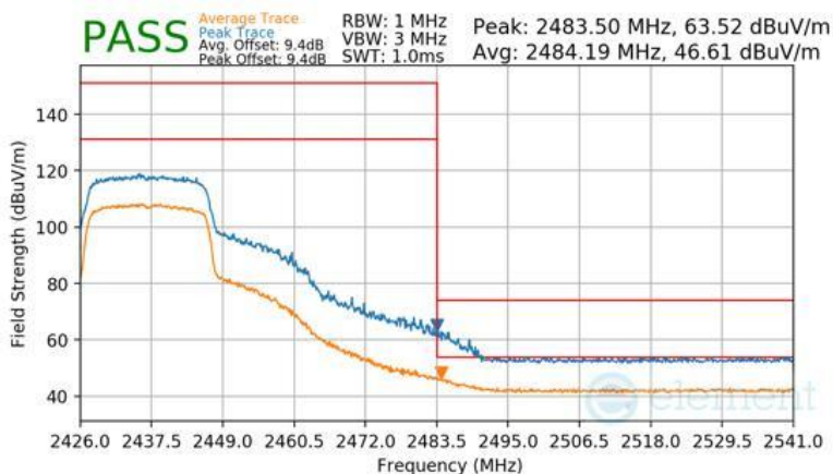
Plot 7-173 Radiated Restricted Upper Band Edge Measurement Antenna 3a
