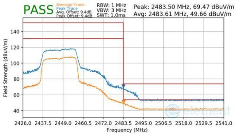
Plot 7-175 Radiated Restricted Upper Band Edge Measurement Antenna 3a
