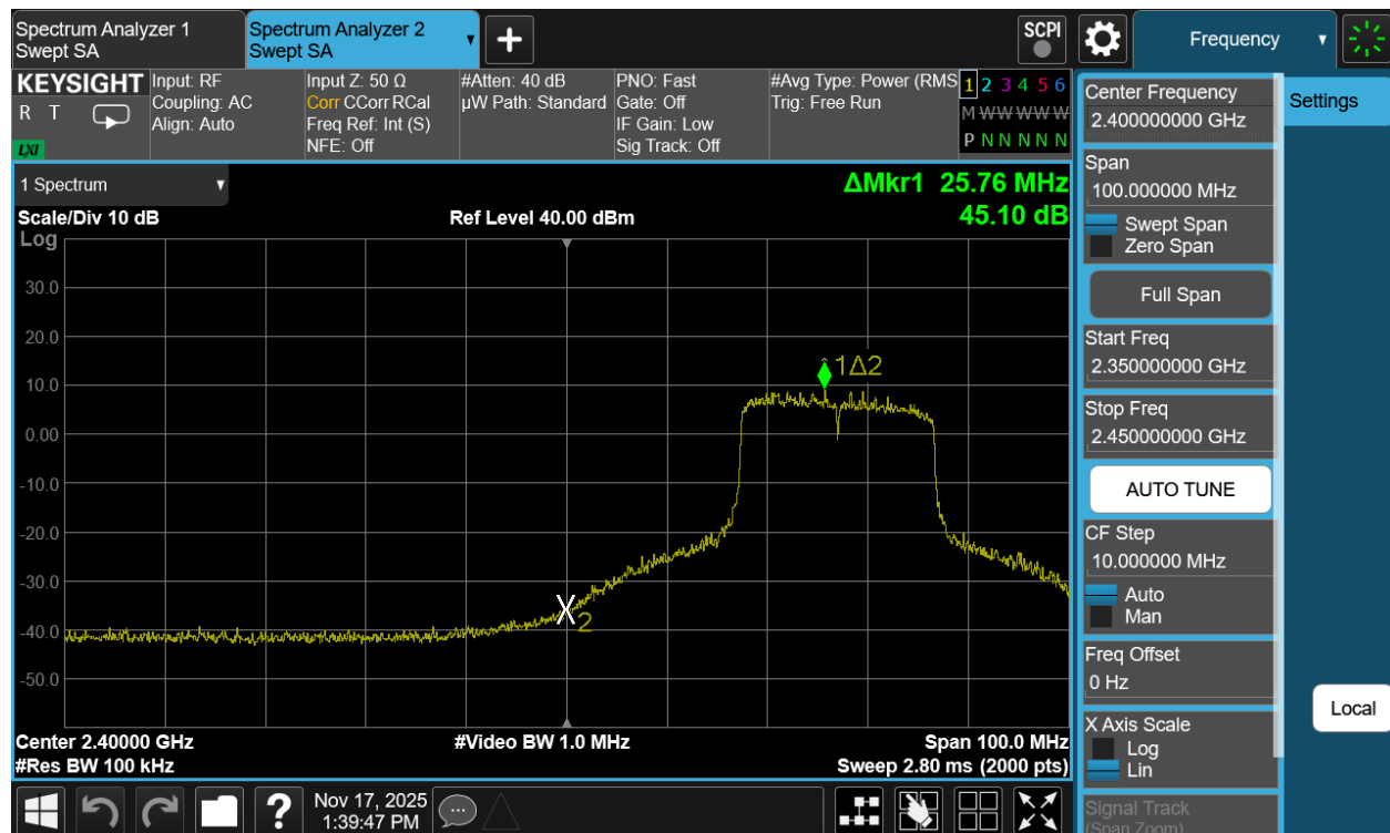
Plot 7-114. Band Edge Plot Antenna 1a (802.11be (SU - 2.4GHz) – Ch. 4)
