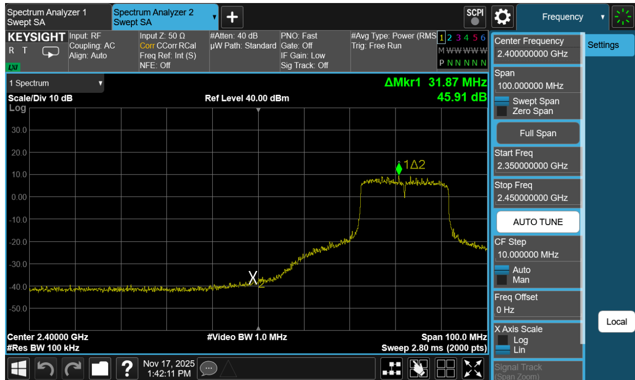
Plot 7-115. Band Edge Plot Antenna 1a (802.11be (SU - 2.4GHz) – Ch. 5)
