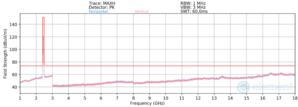
Plot 7-146. Radiated Spurious Emissions above 1GHz CDD (802.11be (SU) – Ch. 6)
