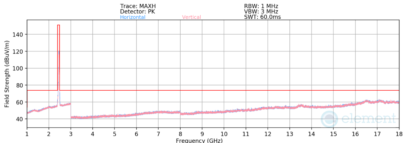
Plot 7-144. Radiated Spurious Emissions above 1GHz CDD (802.11n – Ch. 11)
