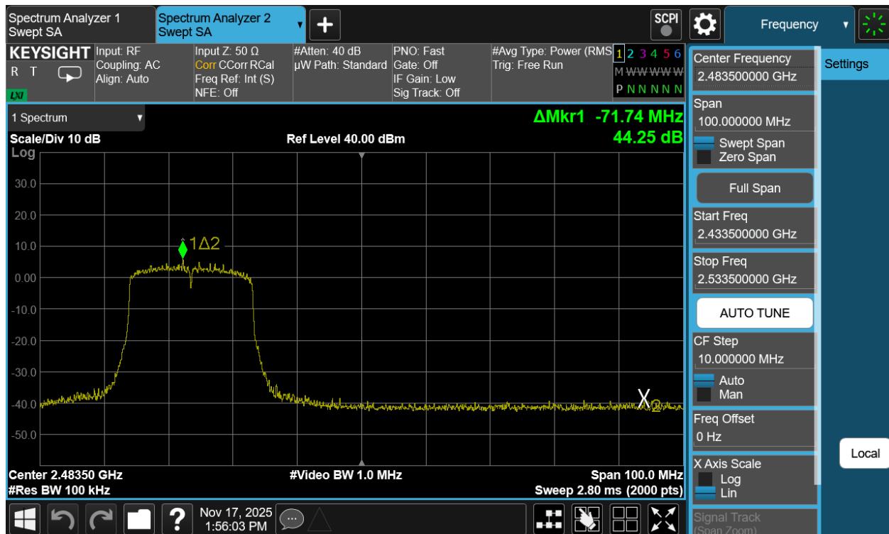
Plot 7-121. Band Edge Plot Antenna 1a (802.11be (SU - 2.4GHz) – Ch. 10)
