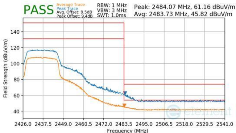
Plot 7-159 Radiated Restricted Upper Band Edge Measurement Antenna 3a
