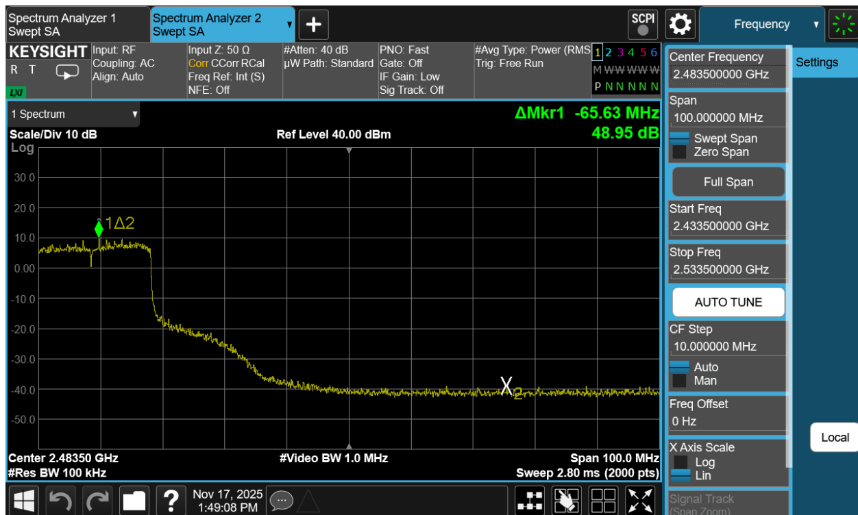
Plot 7-118. Band Edge Plot Antenna 1a (802.11be (SU - 2.4GHz) – Ch. 7)
