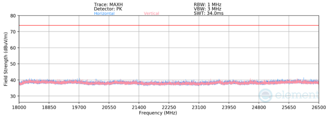
Plot 7-147. Radiated Spurious Emissions above 18GHz CDD (802.11be (SU) – Ch.6)
