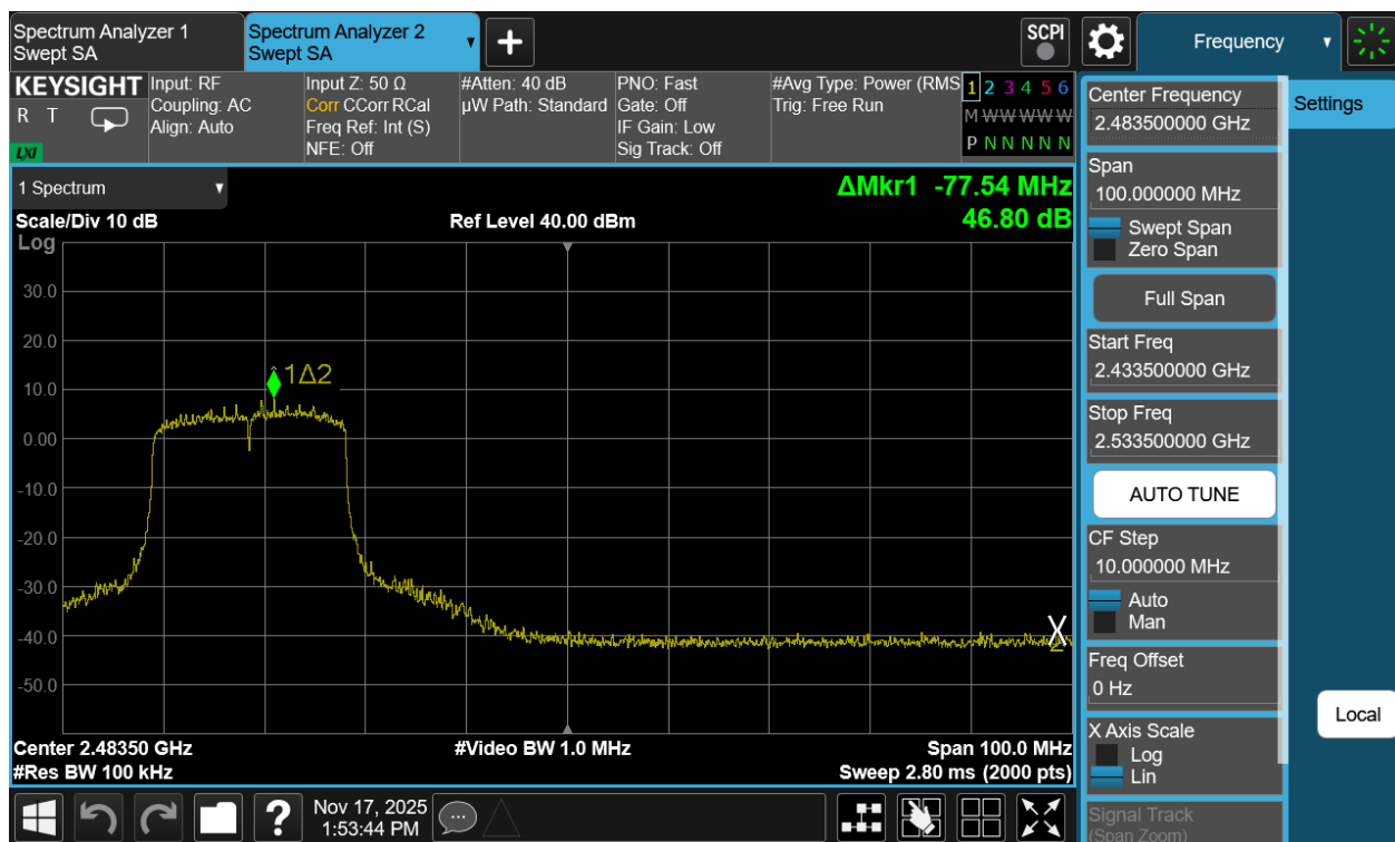
Plot 7-120. Band Edge Plot Antenna 1a (802.11be (SU - 2.4GHz) – Ch. 9)
