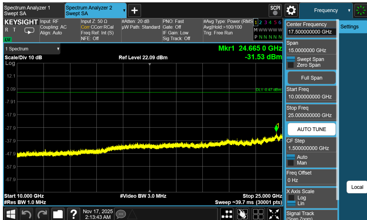
Plot 7-128. Conducted Spurious Plot Antenna 3a (802.11b – Ch. 6)
