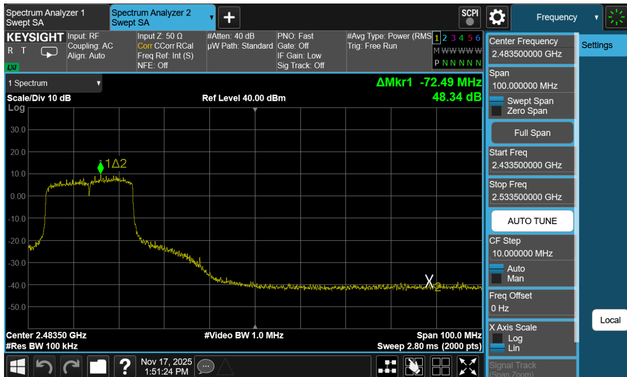
Plot 7-119. Band Edge Plot Antenna 1a (802.11be (SU - 2.4GHz) – Ch. 8)
