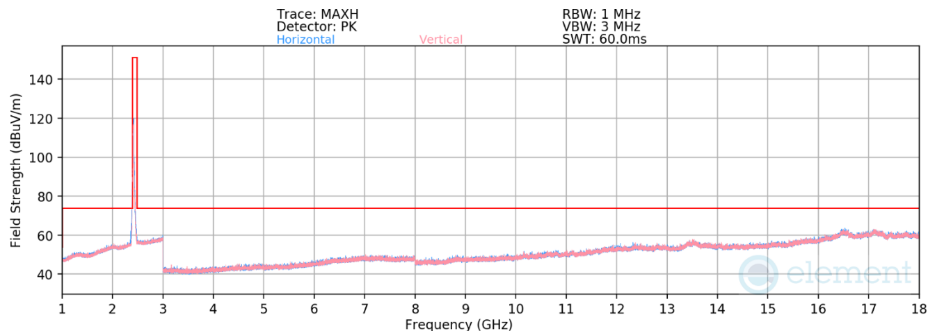
Plot 7-145. Radiated Spurious Emissions above 1GHz CDD (802.11be (SU) – Ch. 1)
