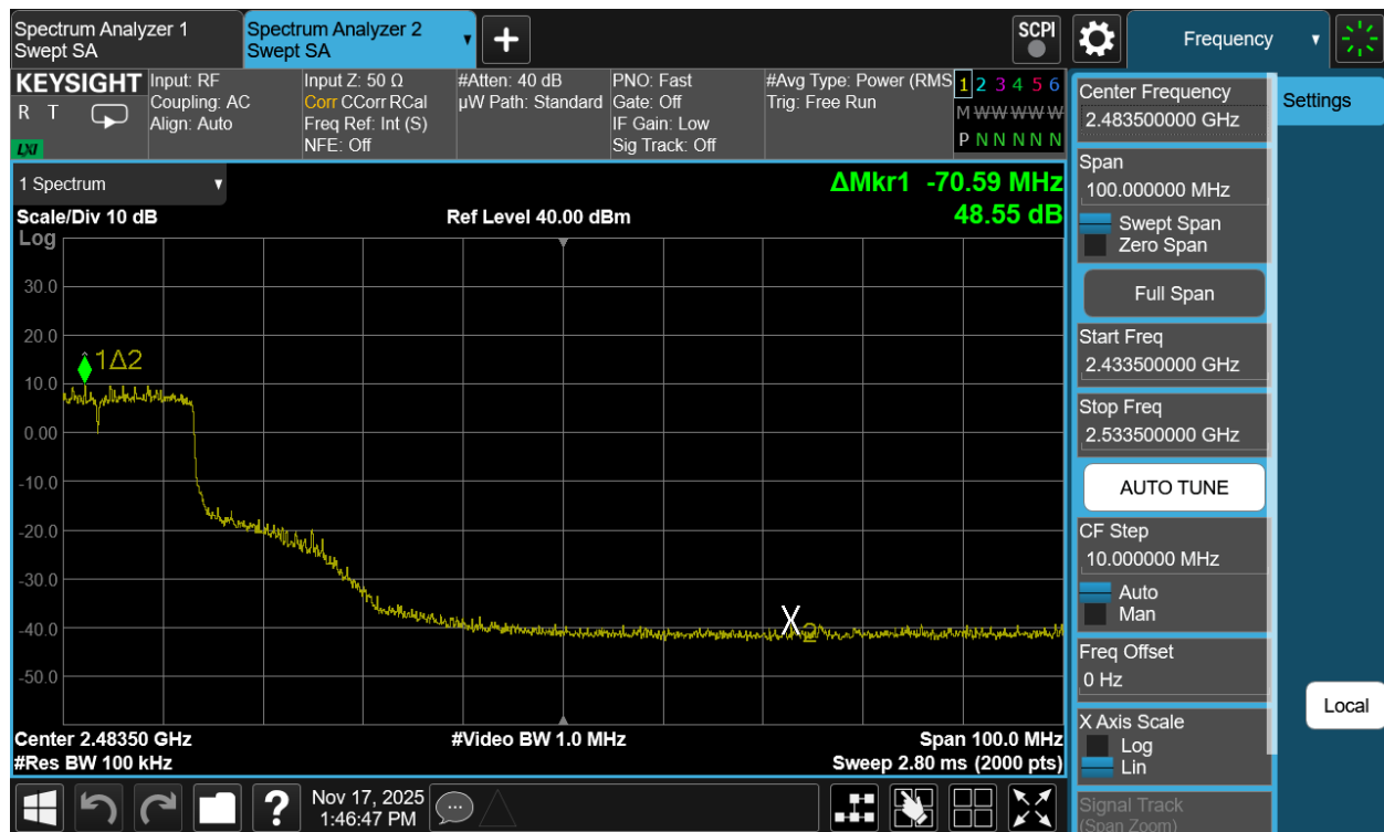
Plot 7-117. Band Edge Plot Antenna 1a (802.11be (SU - 2.4GHz) – Ch. 6(High))
