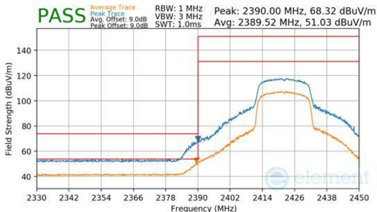
Plot 7-169 Radiated Restricted Lower Band Edge Measurement Antenna 3a
