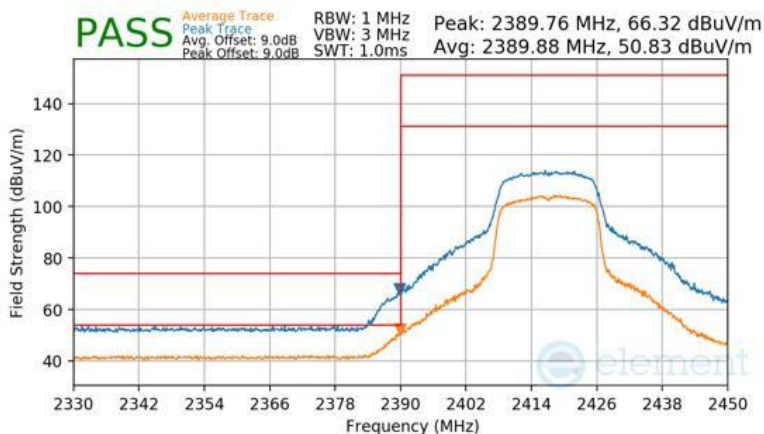
Plot 7-186 Radiated Restricted Lower Band Edge Measurement Antenna 1a
