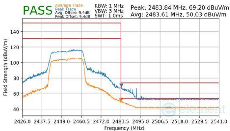
Plot 7-176 Radiated Restricted Upper Band Edge Measurement Antenna 3a
