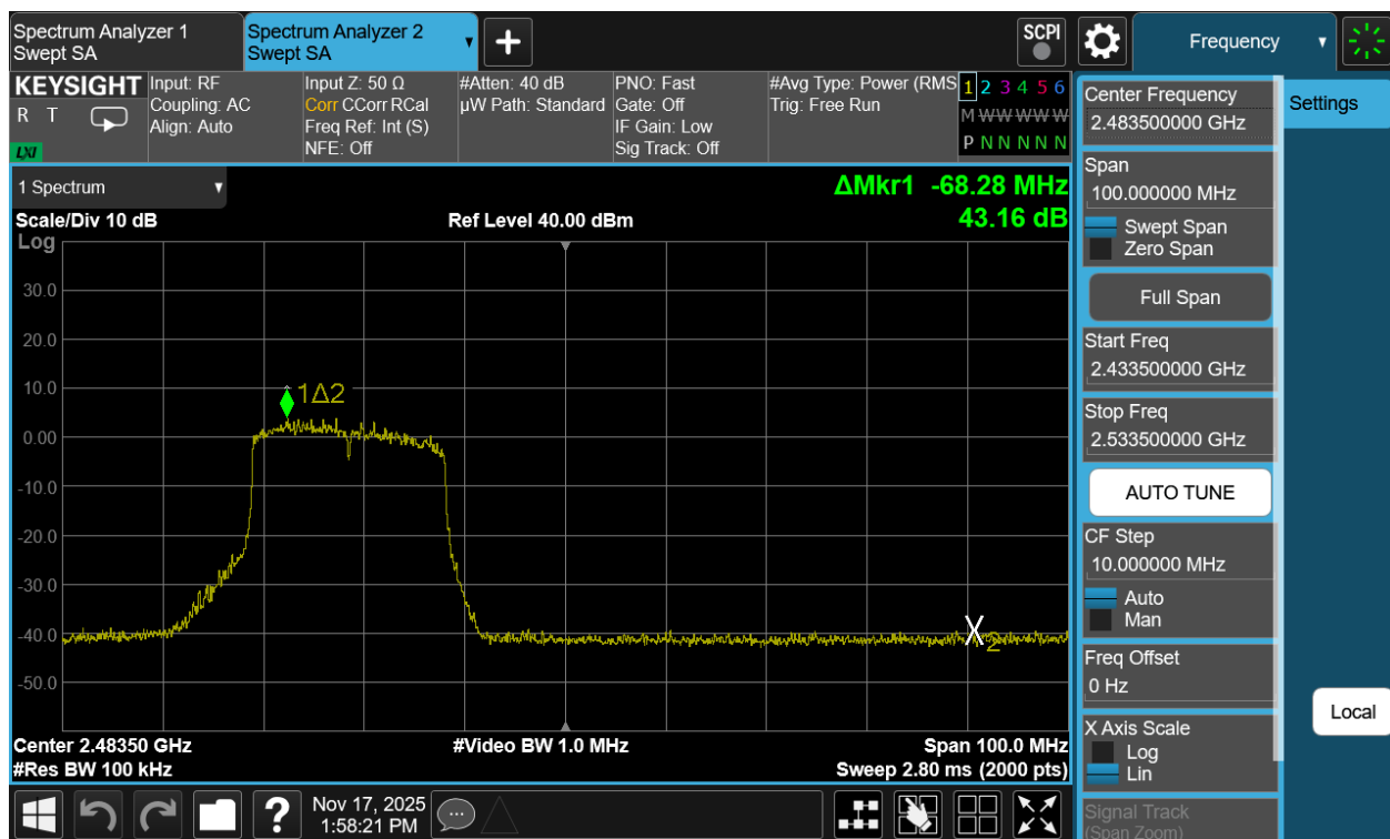
Plot 7-122. Band Edge Plot Antenna 1a (802.11be (SU - 2.4GHz) – Ch. 11)
