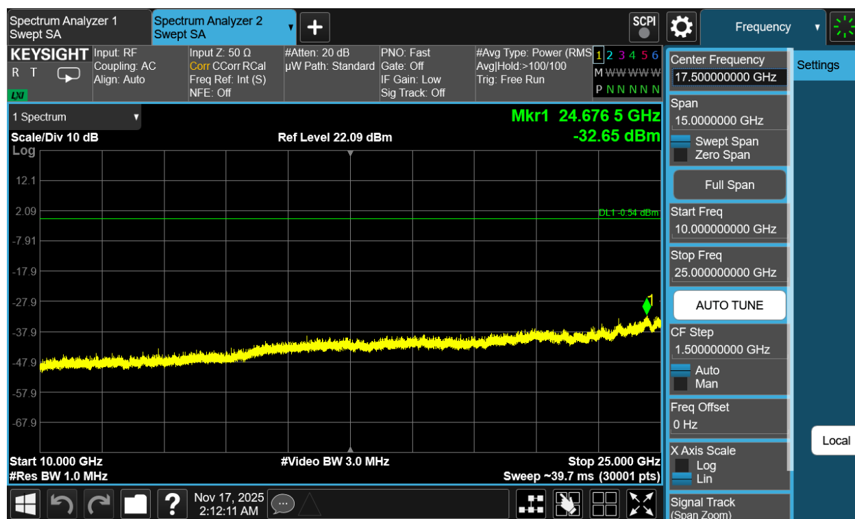
Plot 7-126. Conducted Spurious Plot Antenna 3a (802.11b – Ch. 1)
