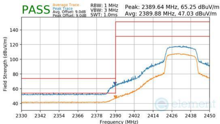
Plot 7-171 Radiated Restricted Lower Band Edge Measurement Antenna 3a
