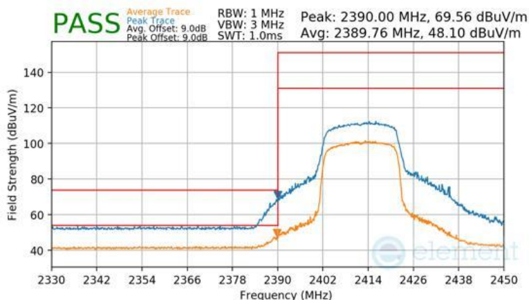
Plot 7-198 Radiated Restricted Lower Band Edge Measurement Antenna 1a
