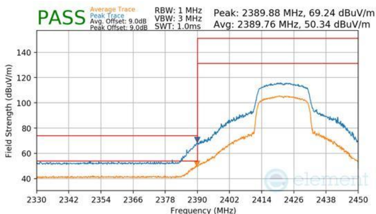
Plot 7-200 Radiated Restricted Lower Band Edge Measurement Antenna 1a
