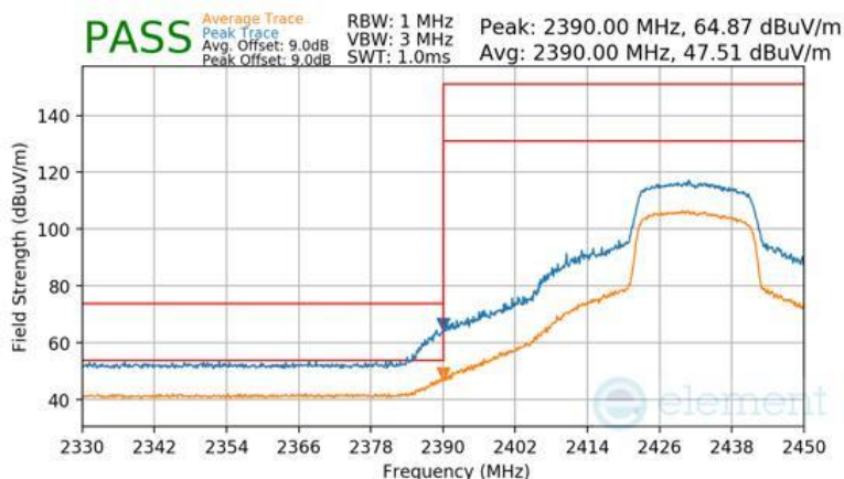
Plot 7-202 Radiated Restricted Lower Band Edge Measurement Antenna 1a
