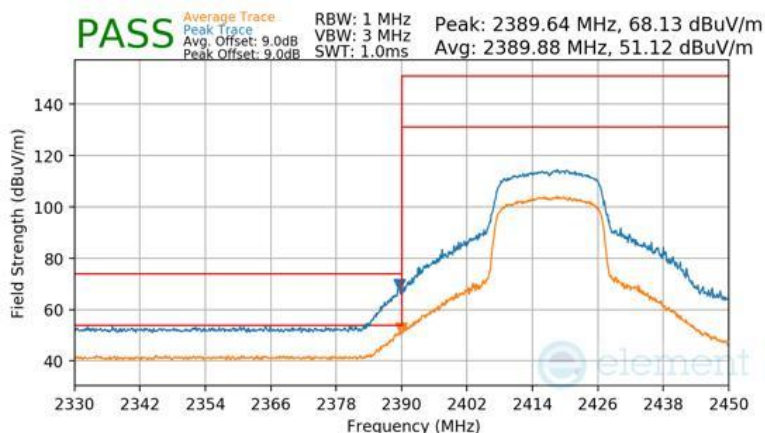
Plot 7-199 Radiated Restricted Lower Band Edge Measurement Antenna 1a
