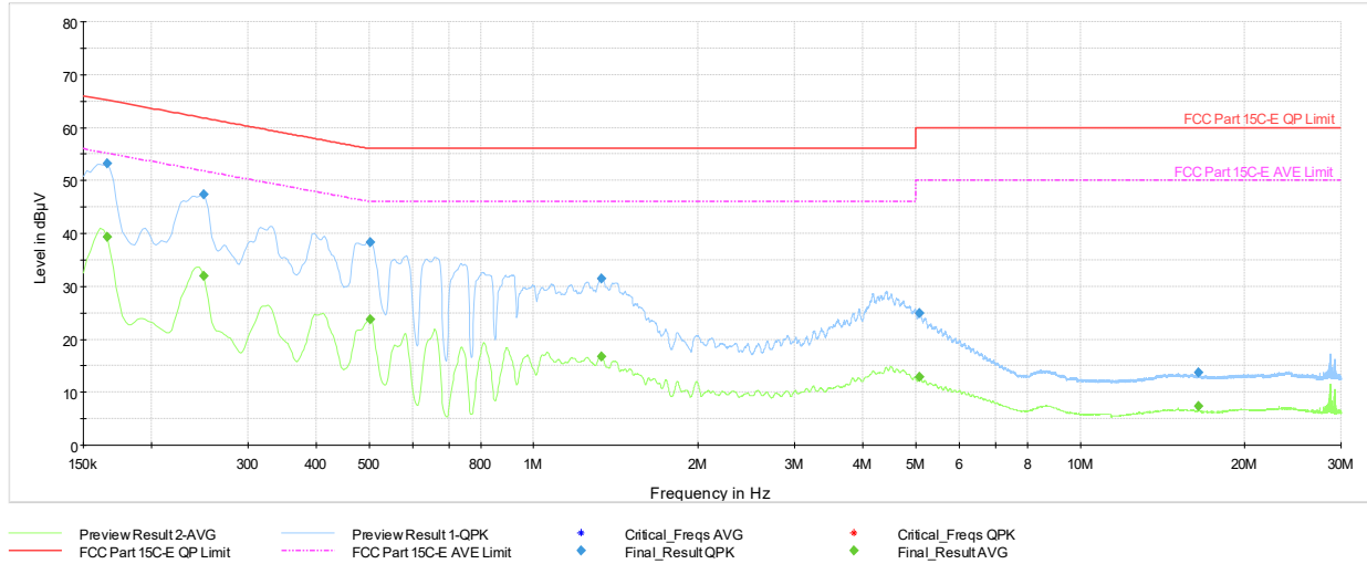
Plot 7-247. AC Line Conducted Plot with CDD 11n Ch.6 (N, with AC/DC Adaptor)
