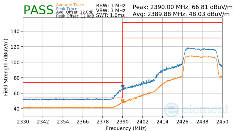
Plot 7-203 Radiated Restricted Lower Band Edge Measurement Antenna 1a
