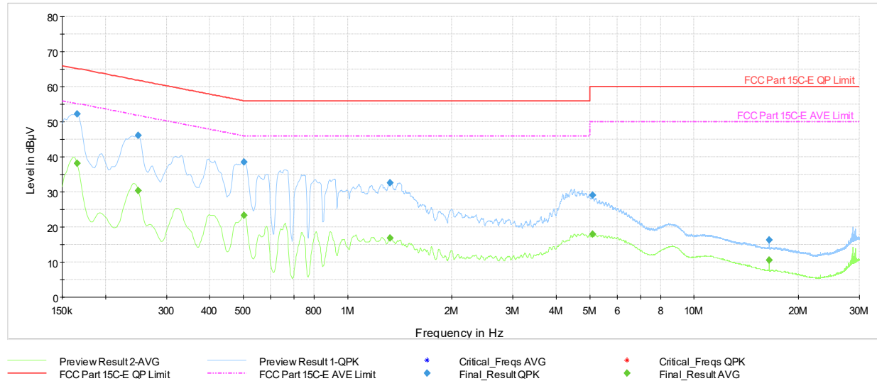
Plot 7-246. AC Line Conducted Plot with CDD 11n Ch.6 (L1, with AC/DC Adaptor)
