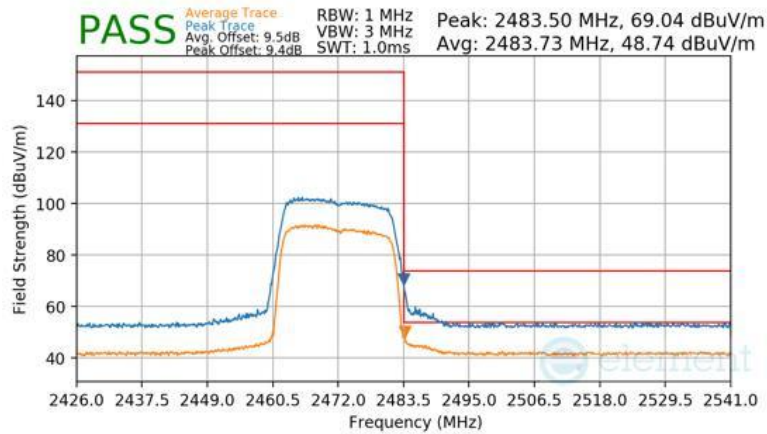
Plot 7-211 Radiated Restricted Upper Band Edge Measurement Antenna 1a
