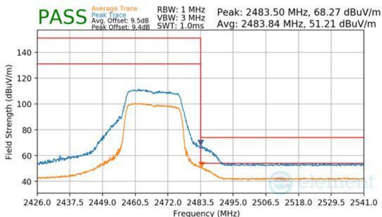
Plot 7-210 Radiated Restricted Upper Band Edge Measurement Antenna 1a
