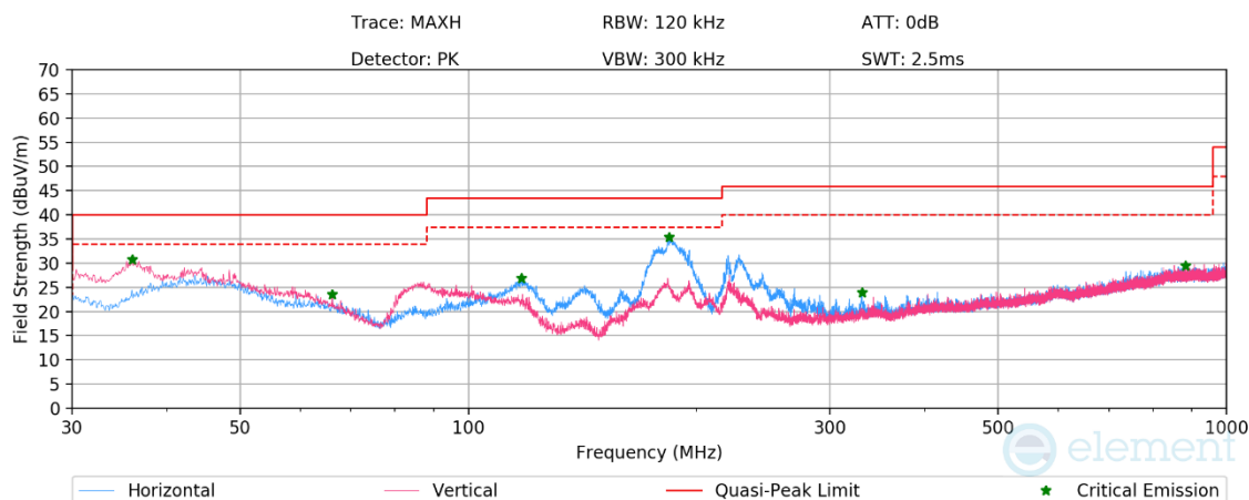
Plot 7-244. Radiated Spurious Emissions Below 1GHz CDD 11n Ch.6, with AC/DC Adaptor
