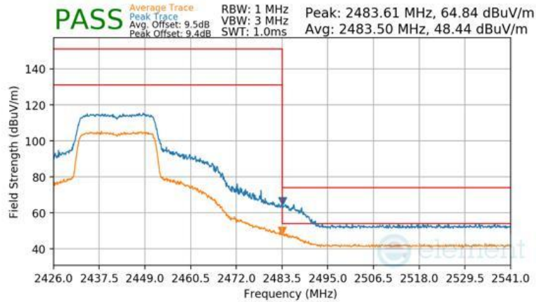
Plot 7-205 Radiated Restricted Upper Band Edge Measurement Antenna 1a
