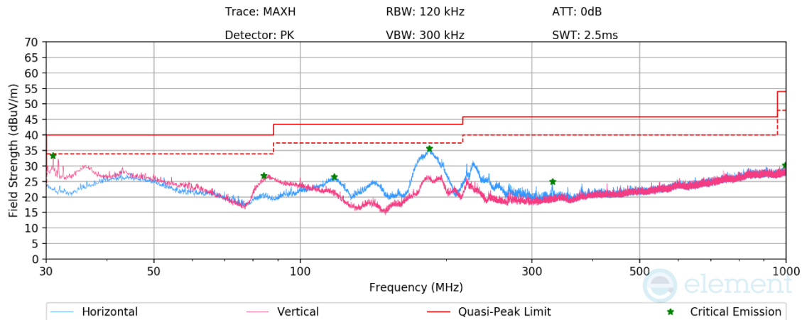
Plot 7-245. Radiated Spurious Emissions Below 1GHz CDD 11be - SU Ch.6, with AC/DC Adaptor
