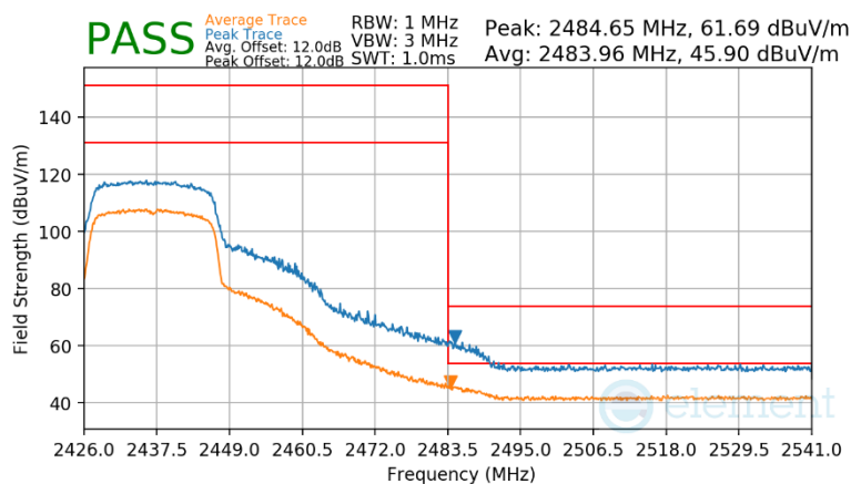
Plot 7-204 Radiated Restricted Upper Band Edge Measurement Antenna 1a
