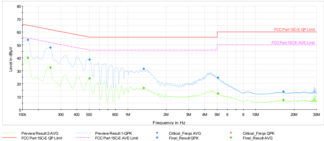
Plot 7-249. AC Line Conducted Plot with CDD 11be - SU Ch.6 (N, with AC/DC Adaptor)
