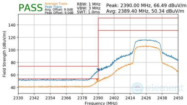
Plot 7-201 Radiated Restricted Lower Band Edge Measurement Antenna 1a
