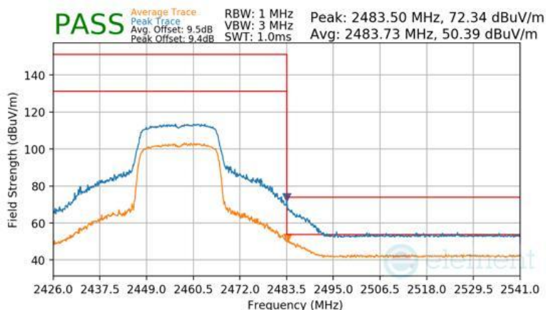
Plot 7-208 Radiated Restricted Upper Band Edge Measurement Antenna 1a
