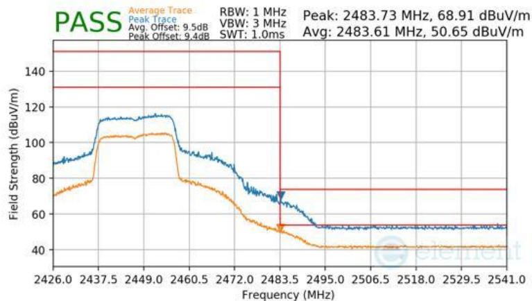
Plot 7-206 Radiated Restricted Upper Band Edge Measurement Antenna 1a
