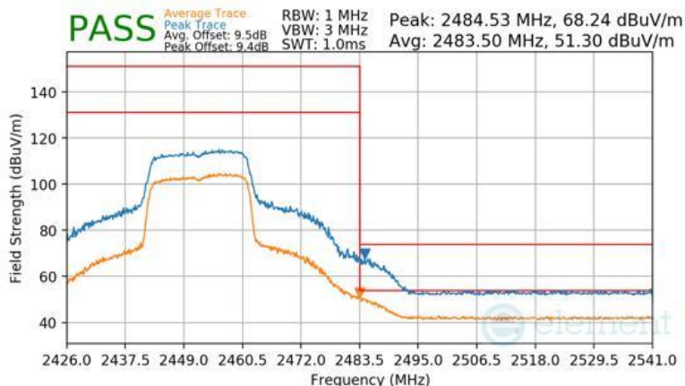
Plot 7-207 Radiated Restricted Upper Band Edge Measurement Antenna 1a
