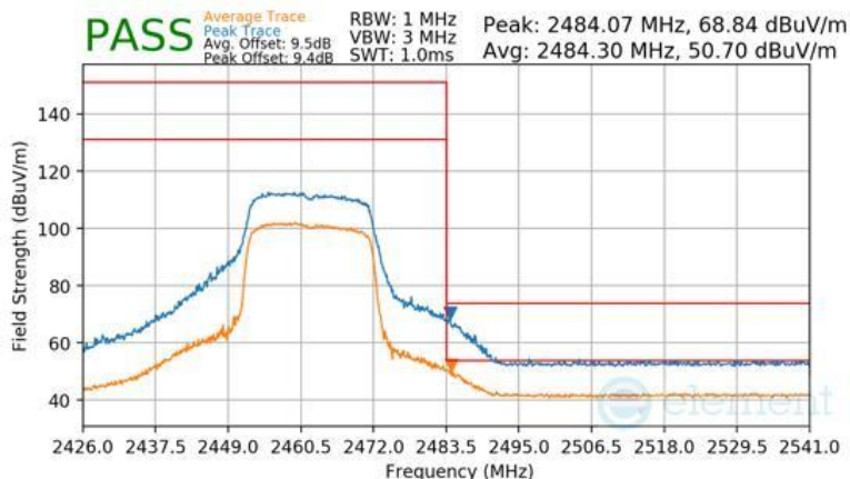
Plot 7-209 Radiated Restricted Upper Band Edge Measurement Antenna 1a
