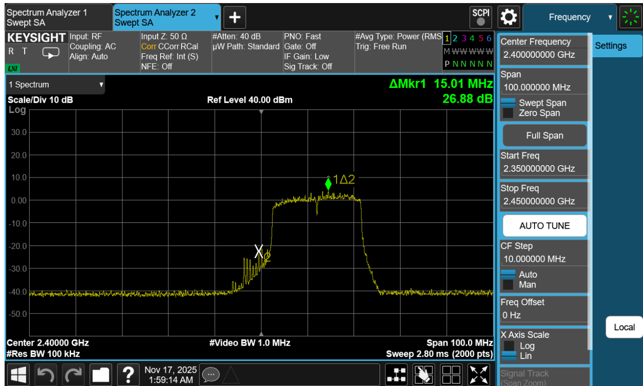
Plot 7-37. Band Edge Antenna 3a (802.11be OFDMA – RU242 – Ch. 1)
