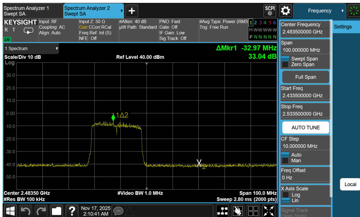
Plot 7-50. Band Edge Antenna 3a (802.11be OFDMA – RU242 – Ch. 13)
