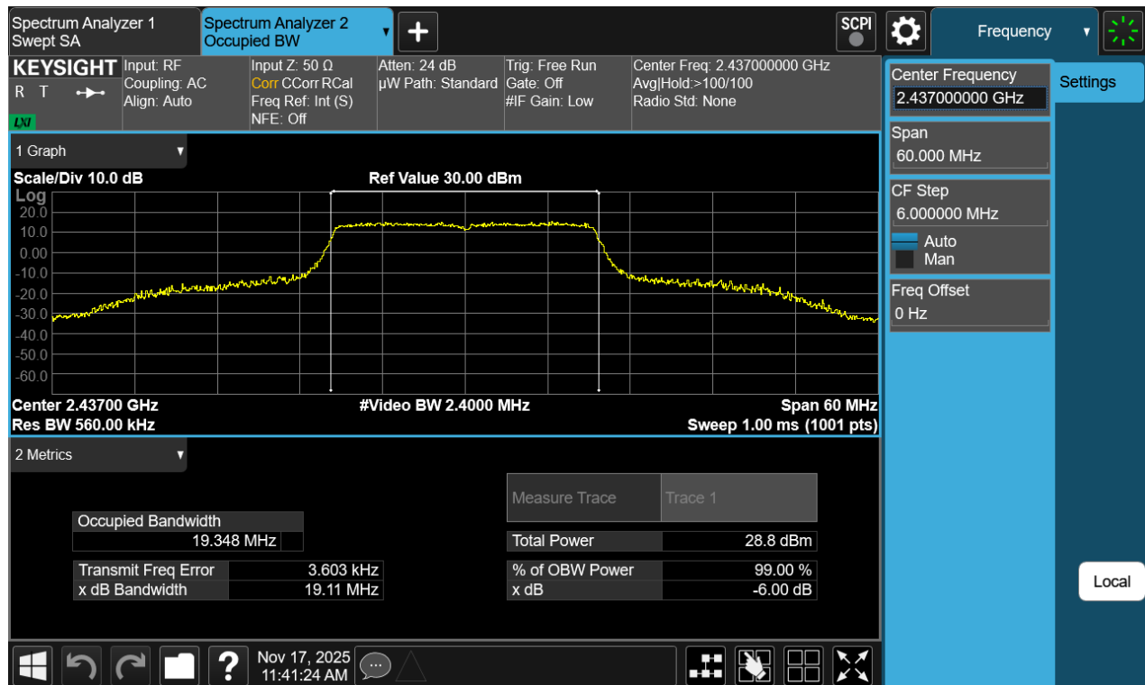
Plot 7-6 99% OBW Antenna 1a (20MHz BW 802.11be(RU) RU242 Index61 - Ch.6)
