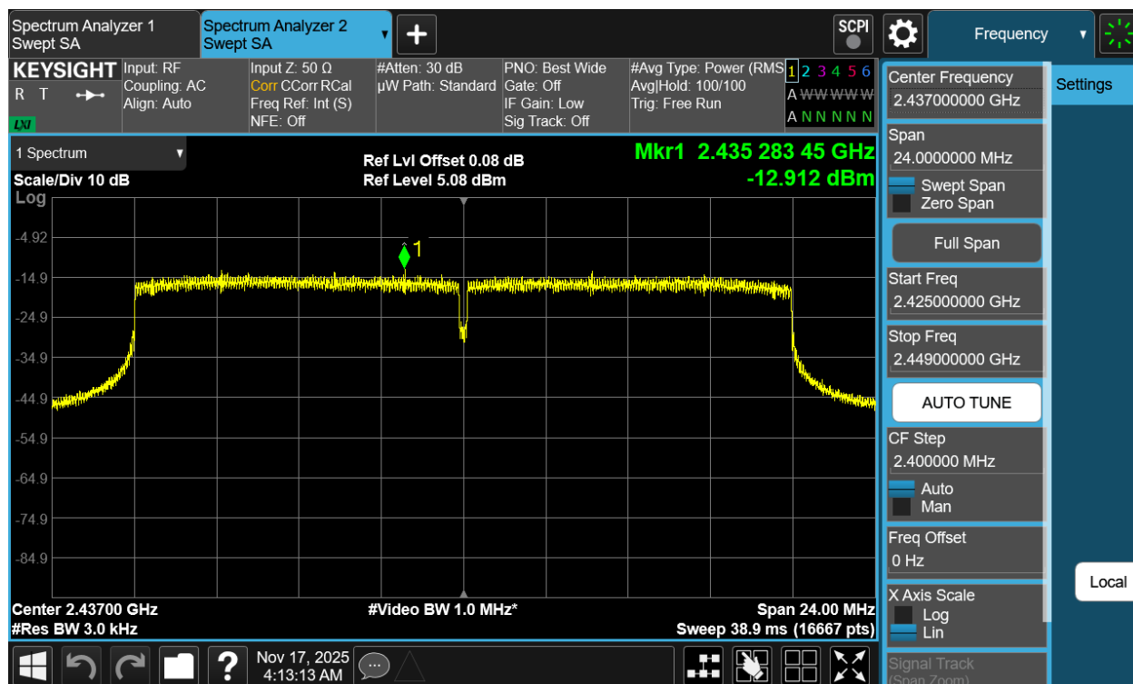
Plot 7-26 PSD CDD Antenna 3a (20MHz BW 802.11be(RU) RU242 Index61 - Ch.6)
