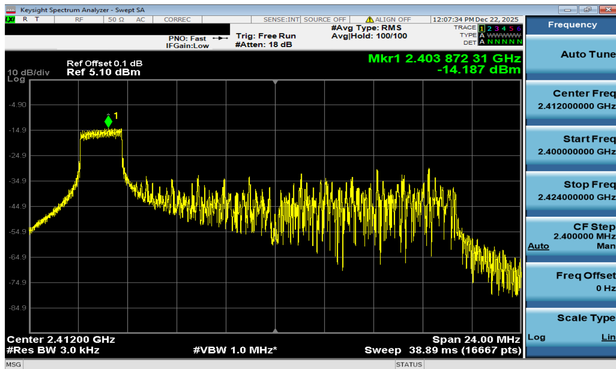
Plot 7-25 PSD CDD Antenna 3a (20MHz BW 802.11be(RU) RU26 Index0 - Ch.1)
