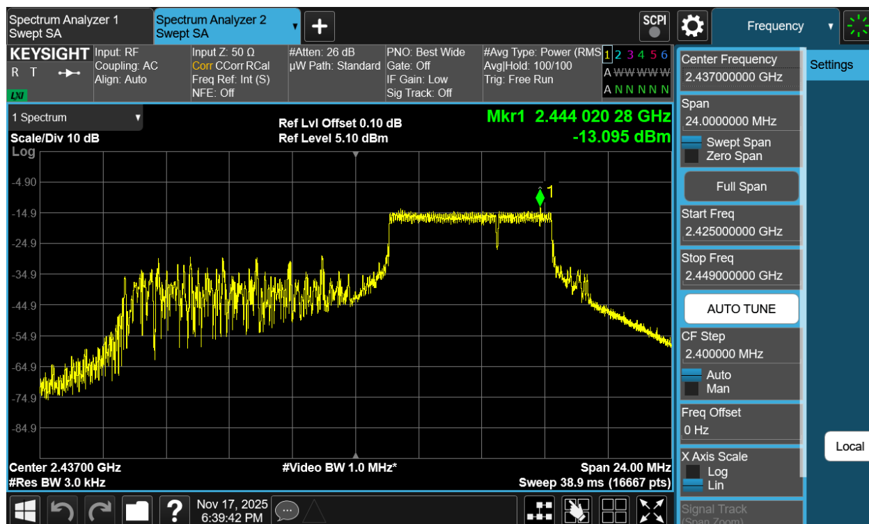
Plot 7-19 PSD Antenna 3a (20MHz BW 802.11be(RU) RU52+26 Index72 - Ch.6)
