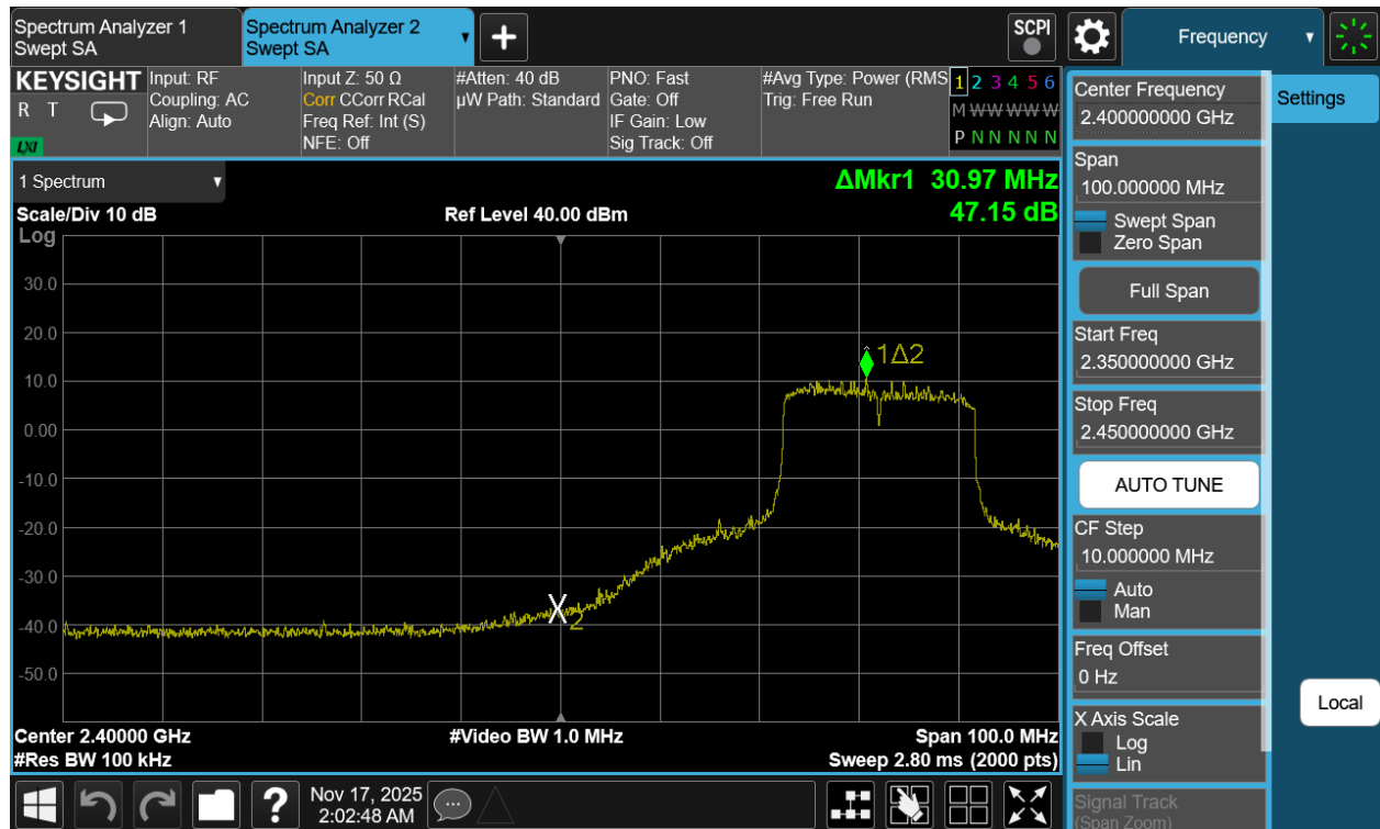
Plot 7-41. Band Edge Antenna 3a (802.11be OFDMA – RU242 – Ch. 5)
