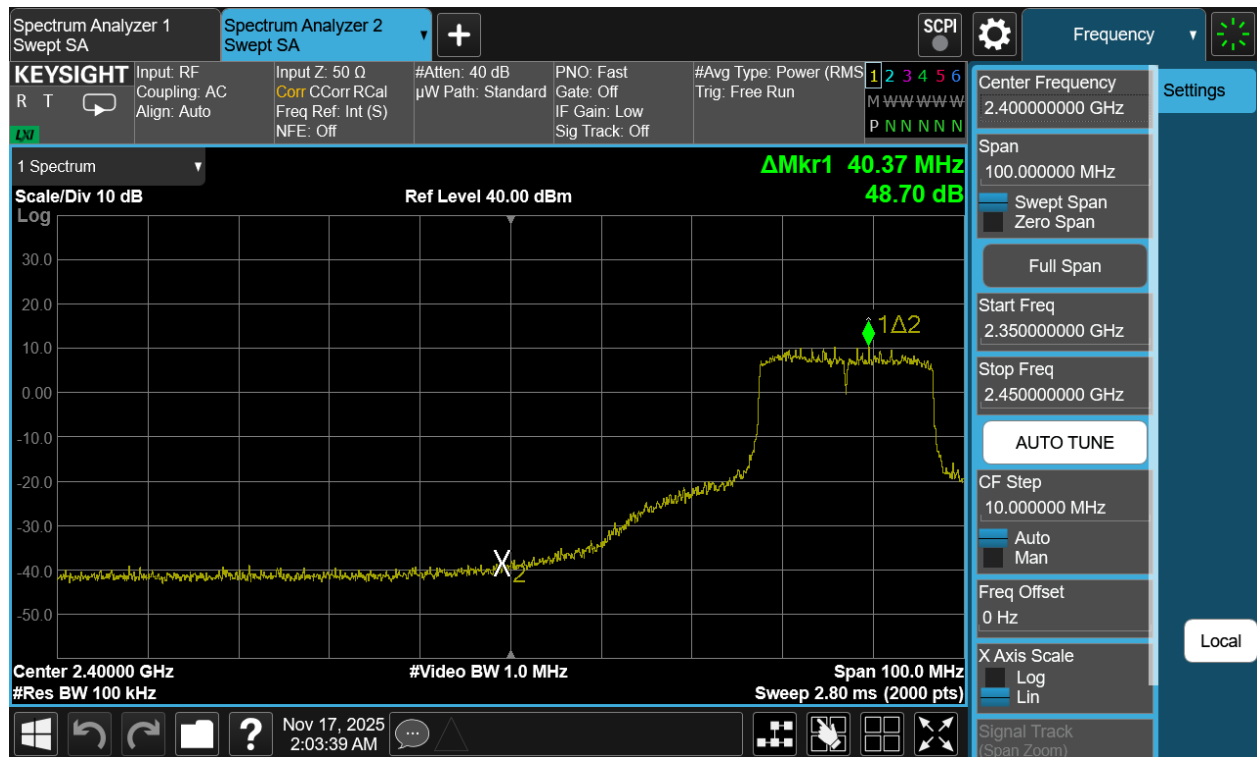
Plot 7-42. Band Edge Antenna 3a (802.11be OFDMA – RU242 – Ch. 6(Low Channel))
