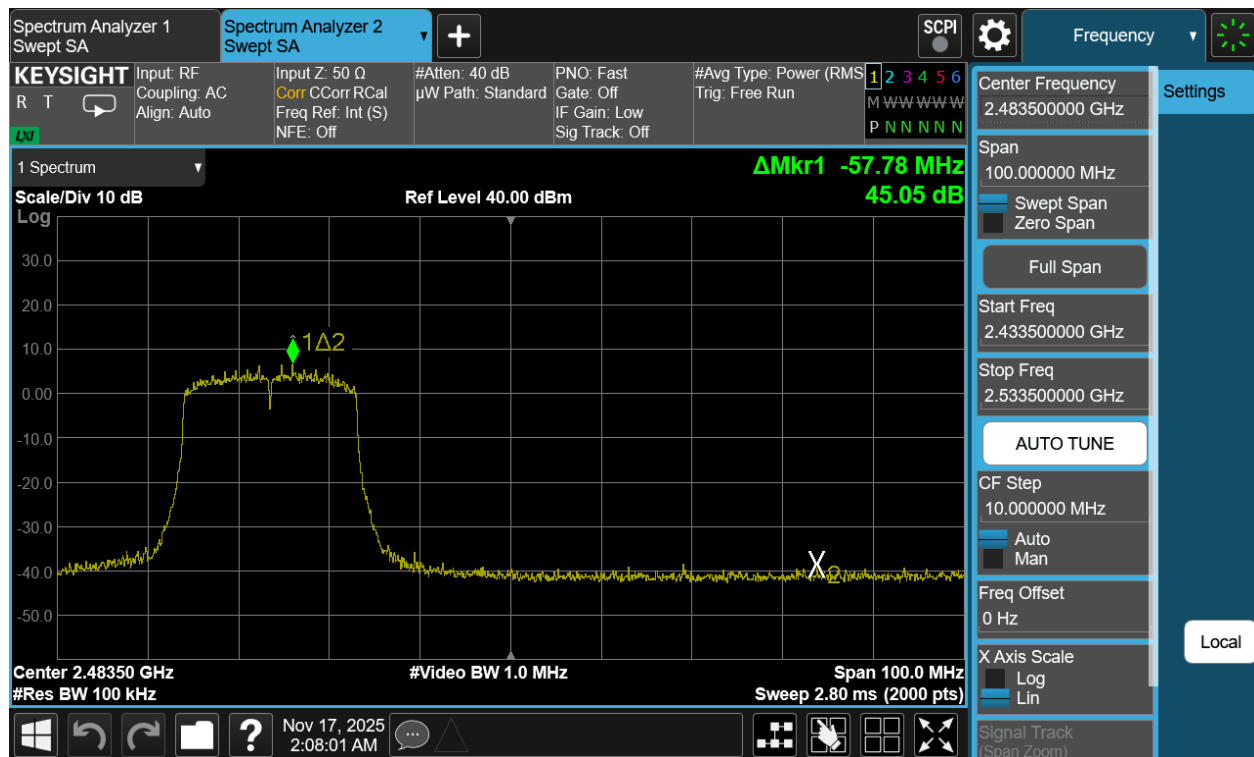
Plot 7-47. Band Edge Antenna 3a (802.11be OFDMA – RU242 – Ch. 10)
