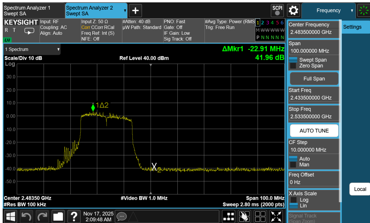
Plot 7-49. Band Edge Antenna 3a (802.11be OFDMA – RU242 – Ch. 12)
