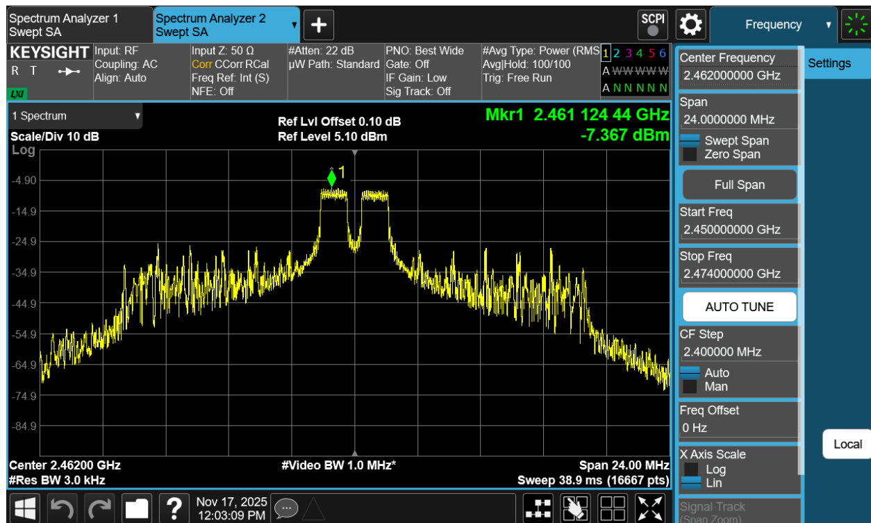
Plot 7-21 PSD Antenna 1a (20MHz BW 802.11be(RU) RU26 Index4 - Ch.11)
