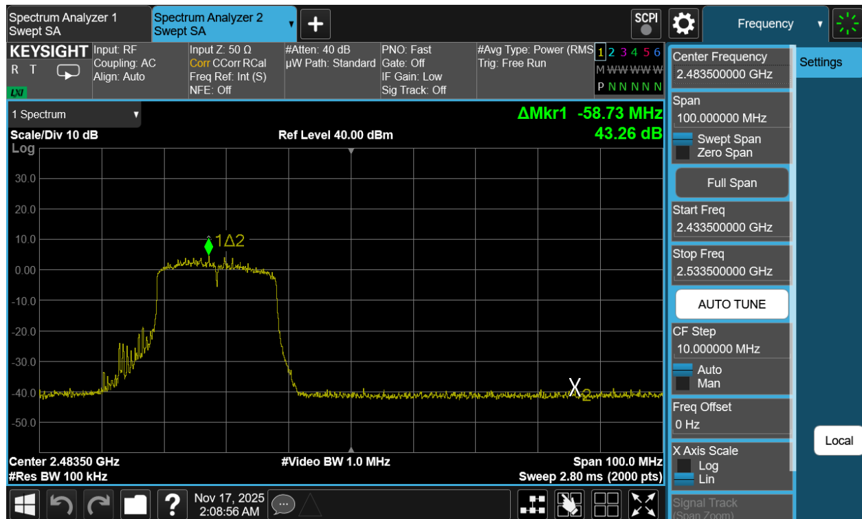
Plot 7-48. Band Edge Antenna 3a (802.11be OFDMA – RU242 – Ch. 11)
