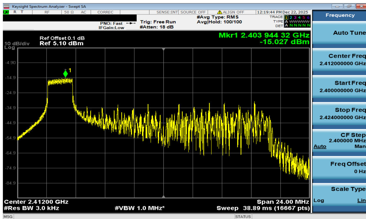
Plot 7-29 PSD CDD Antenna 1a (20MHz BW 802.11be(RU) RU26 Index0 - Ch.1)
