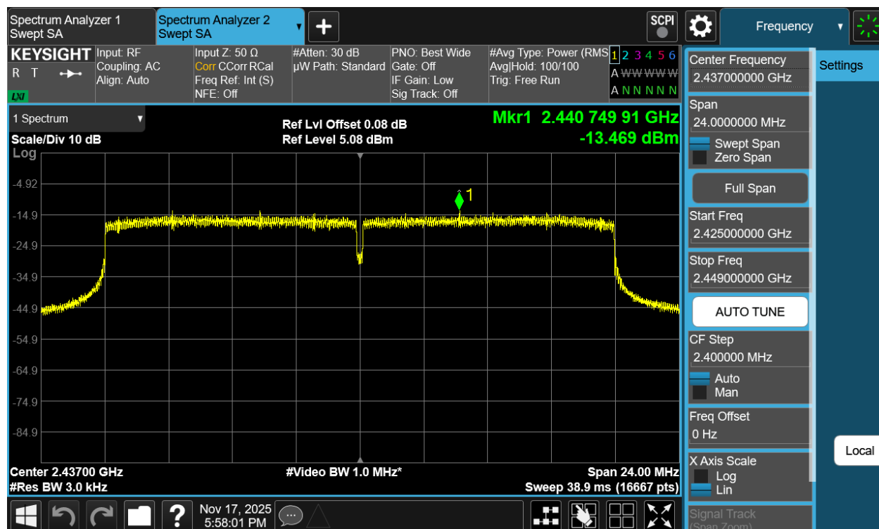
Plot 7-30 PSD CDD Antenna 1a (20MHz BW 802.11be(RU) RU242 Index61 - Ch.6)
