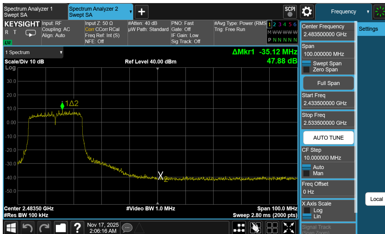
Plot 7-45. Band Edge Antenna 3a (802.11be OFDMA – RU242 – Ch. 8)
