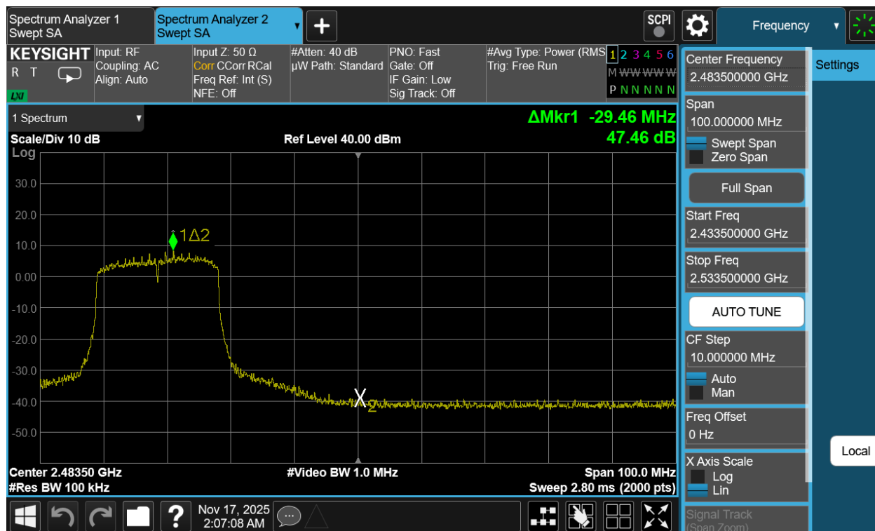
Plot 7-46. Band Edge Antenna 3a (802.11be OFDMA – RU242 – Ch. 9)
