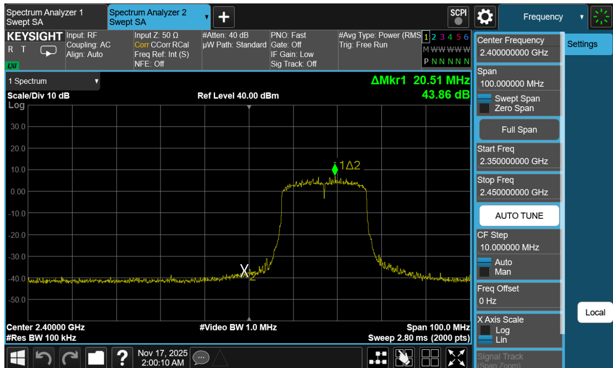
Plot 7-38. Band Edge Antenna 3a (802.11be OFDMA – RU242 – Ch. 2)
