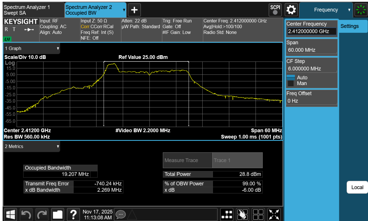
Plot 7-5 99% OBW Antenna 1a (20MHz BW 802.11be(RU) RU26 Index0 - Ch.1)
