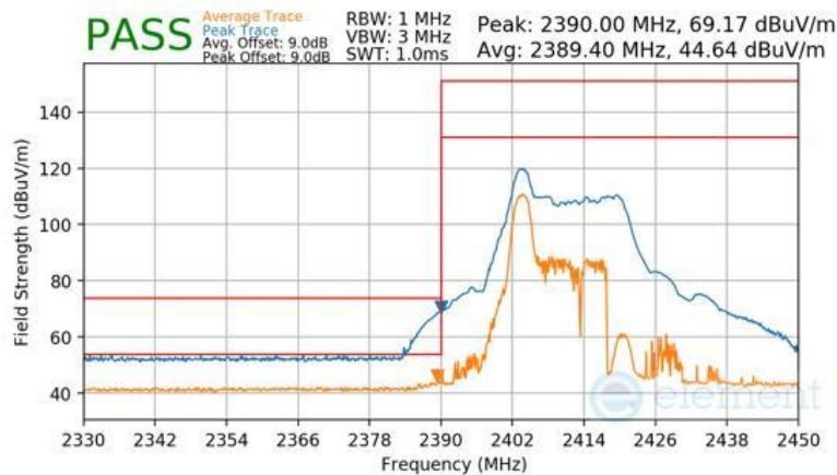
Plot 7-133 Radiated Restricted Lower Band Edge Measurement Antenna 1a (Peak & Average – RU26)
