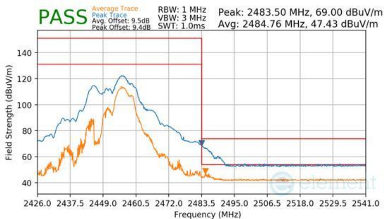
Plot 7-175 Radiated Restricted Upper Band Edge Measurement CDD (Peak & Average – RU52+26)
