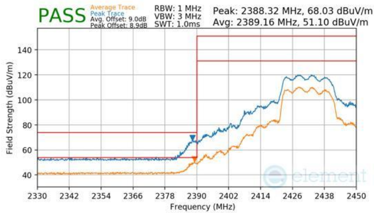
Plot 7-188 Radiated Restricted Lower Band Edge Measurement CDD (Peak & Average – RU242)
