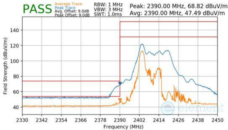
Plot 7-164 Radiated Restricted Lower Band Edge Measurement CDD (Peak & Average – RU26)
