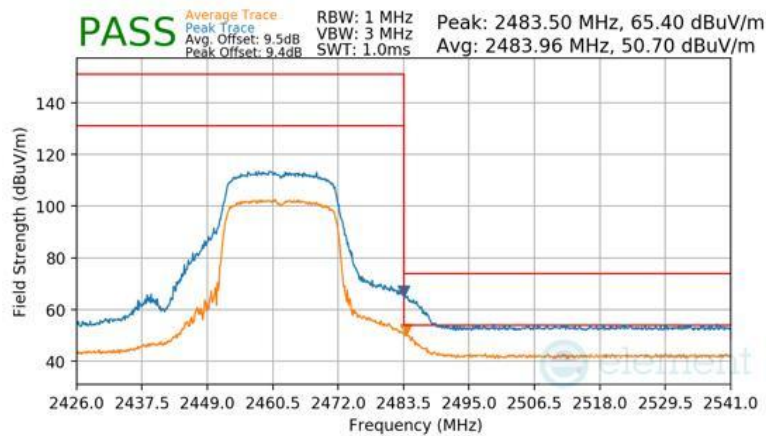
Plot 7-130 Radiated Restricted Upper Band Edge Measurement Antenna 3a (Peak & Average – RU242)
