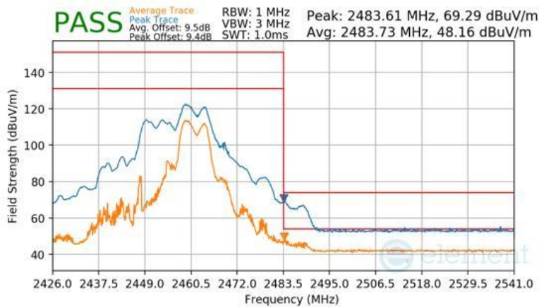
Plot 7-177 Radiated Restricted Upper Band Edge Measurement CDD (Peak & Average – RU52+26)
