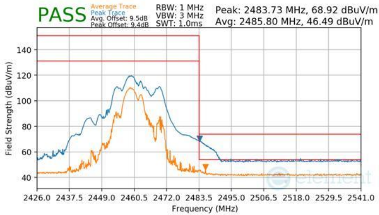
Plot 7-178 Radiated Restricted Upper Band Edge Measurement CDD (Peak & Average – RU52+26)
