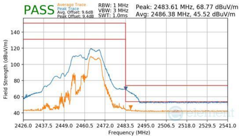
Plot 7-179 Radiated Restricted Upper Band Edge Measurement CDD (Peak & Average – RU52+26)
