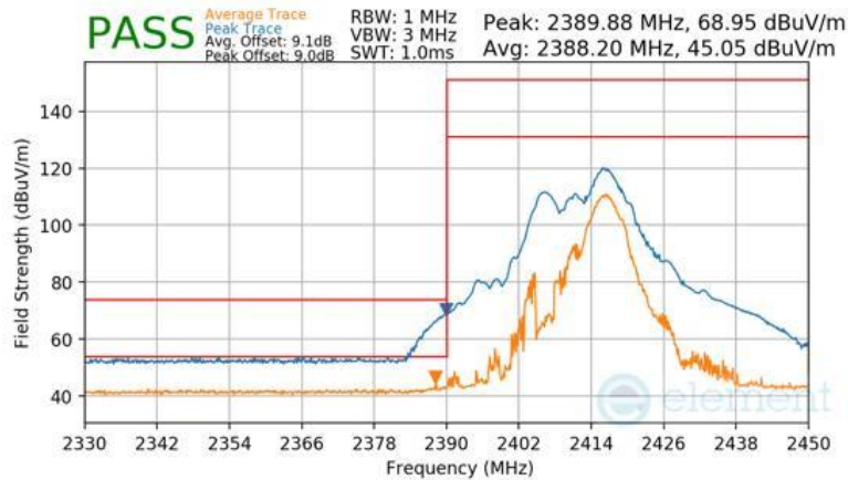
Plot 7-169 Radiated Restricted Lower Band Edge Measurement CDD (Peak & Average – RU52+26)
