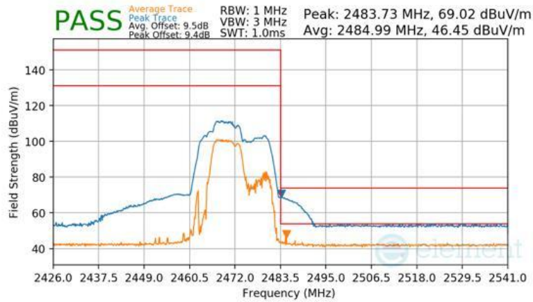
Plot 7-148 Radiated Restricted Upper Band Edge Measurement Antenna 1a (Peak & Average – RU52+26)
