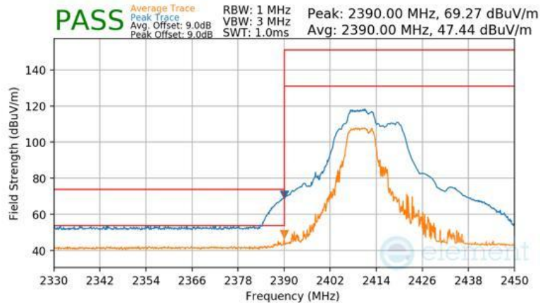
Plot 7-136 Radiated Restricted Lower Band Edge Measurement Antenna 1a (Peak & Average – RU52+26)
