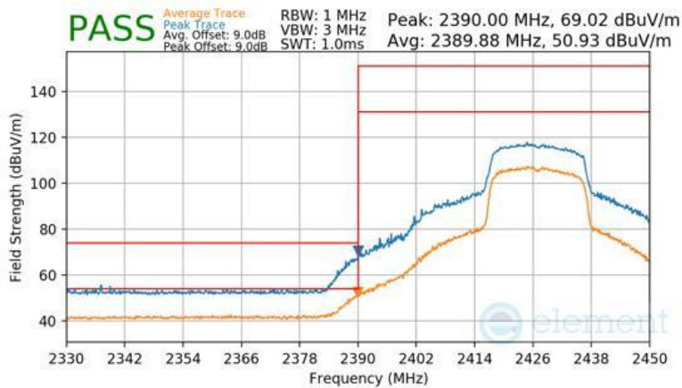
Plot 7-153 Radiated Restricted Lower Band Edge Measurement Antenna 1a (Peak & Average – RU242)
