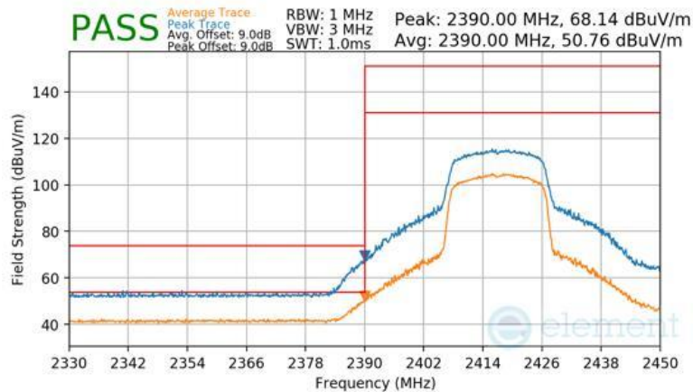
Plot 7-151 Radiated Restricted Lower Band Edge Measurement Antenna 1a (Peak & Average – RU242)
