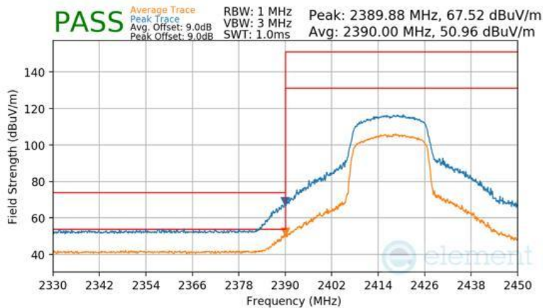
Plot 7-120 Radiated Restricted Lower Band Edge Measurement Antenna 3a (Peak & Average – RU242)
