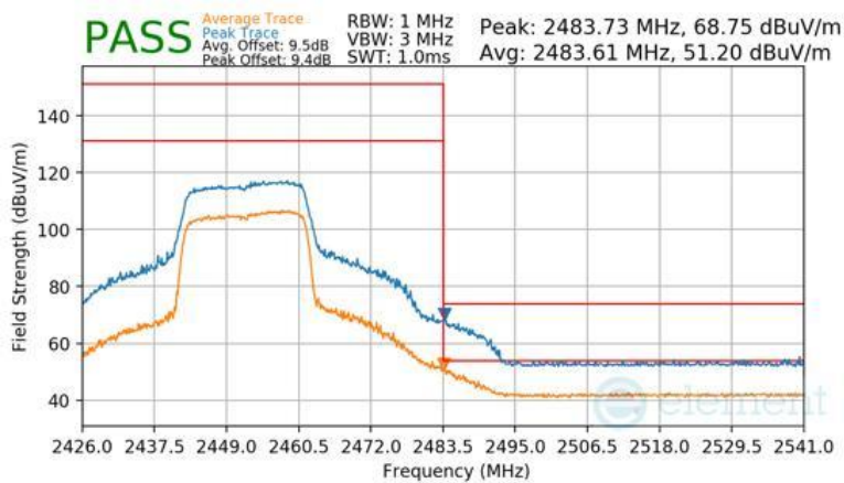
Plot 7-128 Radiated Restricted Upper Band Edge Measurement Antenna 3a (Peak & Average – RU242)
