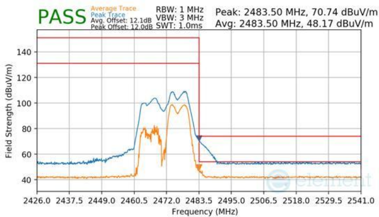
Plot 7-183 Radiated Restricted Upper Band Edge Measurement CDD (Peak & Average – RU52+26)
