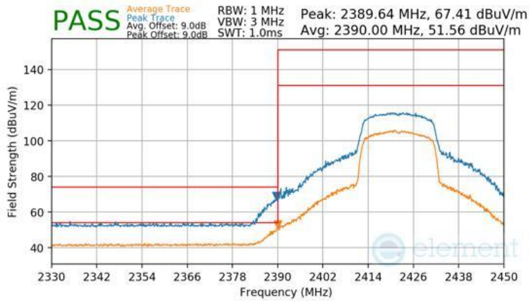
Plot 7-152 Radiated Restricted Lower Band Edge Measurement Antenna 1a (Peak & Average – RU242)
