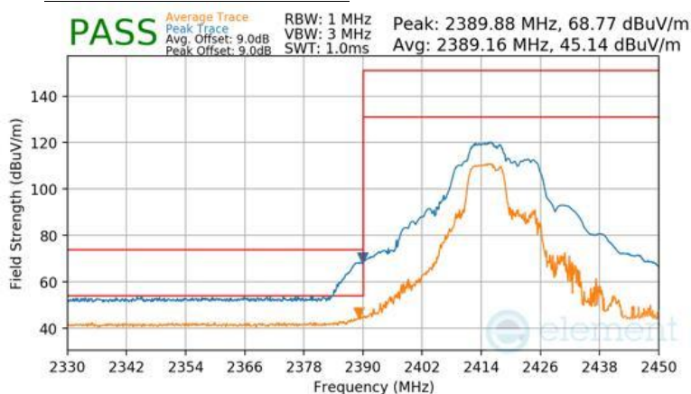
Plot 7-138 Radiated Restricted Lower Band Edge Measurement Antenna 1a (Peak & Average – RU52+26)
