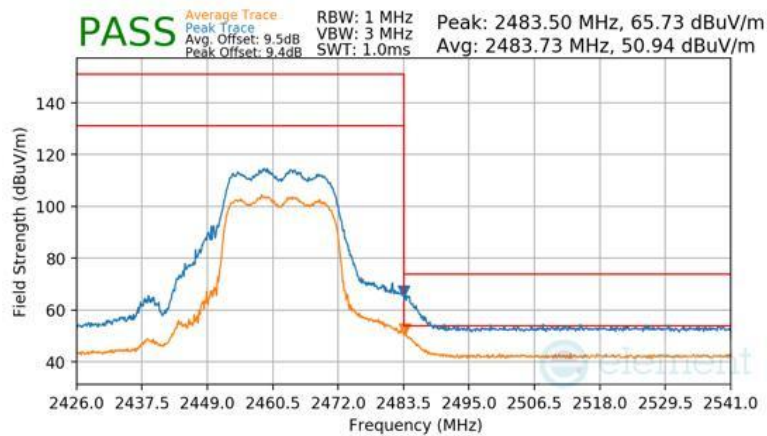
Plot 7-195 Radiated Restricted Upper Band Edge Measurement CDD (Peak & Average – RU242)
