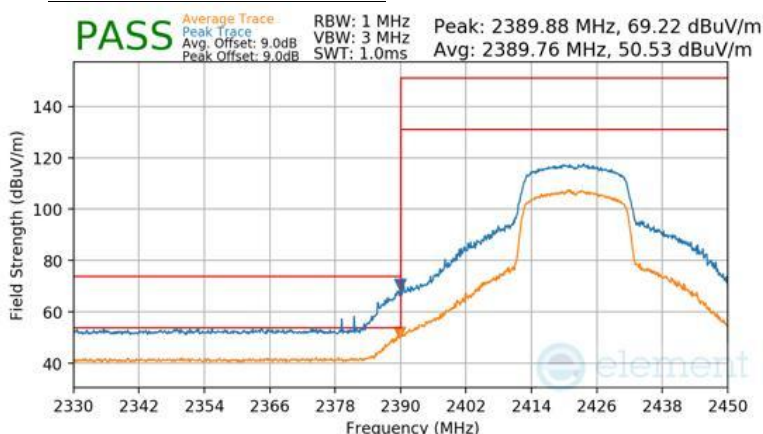
Plot 7-121 Radiated Restricted Lower Band Edge Measurement Antenna 3a (Peak & Average – RU242)
