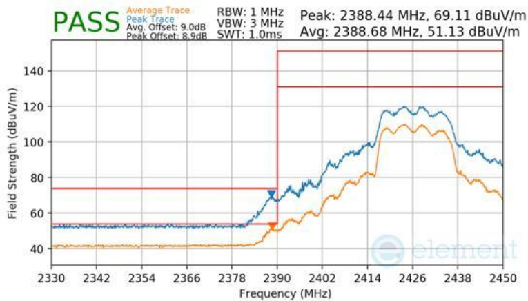
Plot 7-187 Radiated Restricted Lower Band Edge Measurement CDD (Peak & Average – RU242)
