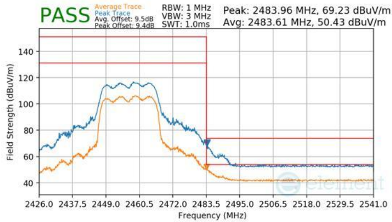
Plot 7-194 Radiated Restricted Upper Band Edge Measurement CDD (Peak & Average – RU242)
