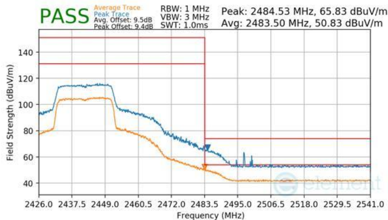
Plot 7-157 Radiated Restricted Upper Band Edge Measurement Antenna 1a (Peak & Average – RU242)
