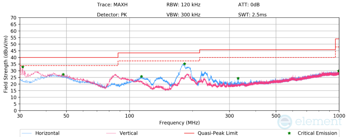
Plot 7-198. Radiated Spurious Emissions below 1GHz CDD Ch.6 (RU26), with AC/DC Adapter
