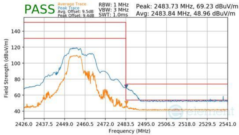
Plot 7-142 Radiated Restricted Upper Band Edge Measurement Antenna 1a (Peak & Average – RU52+26)
