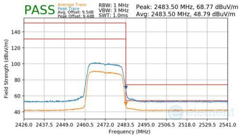
Plot 7-163 Radiated Restricted Upper Band Edge Measurement Antenna 1a (Peak & Average – RU242)
