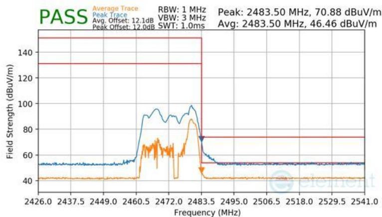
Plot 7-167 Radiated Restricted Upper Band Edge Measurement CDD (Peak & Average – RU26)
