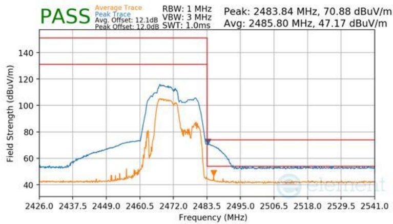
Plot 7-117 Radiated Restricted Upper Band Edge Measurement Antenna 3a (Peak & Average – RU52+26)
