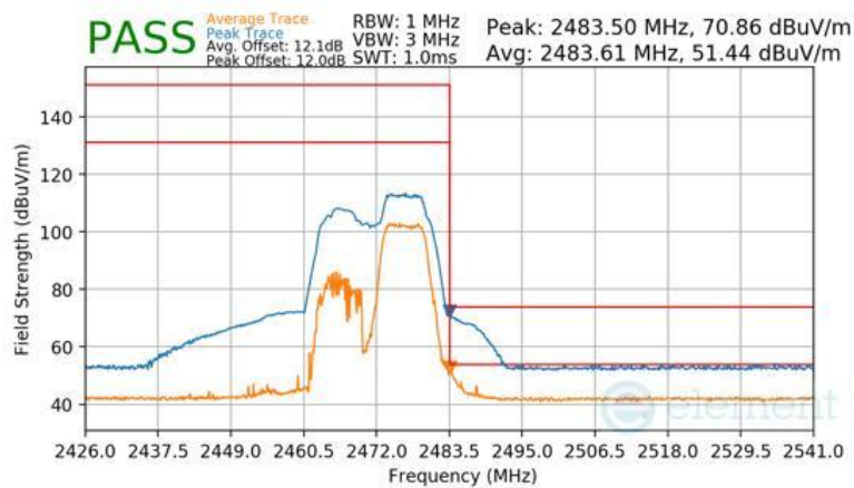
Plot 7-118 Radiated Restricted Upper Band Edge Measurement Antenna 3a (Peak & Average – RU52+26)
