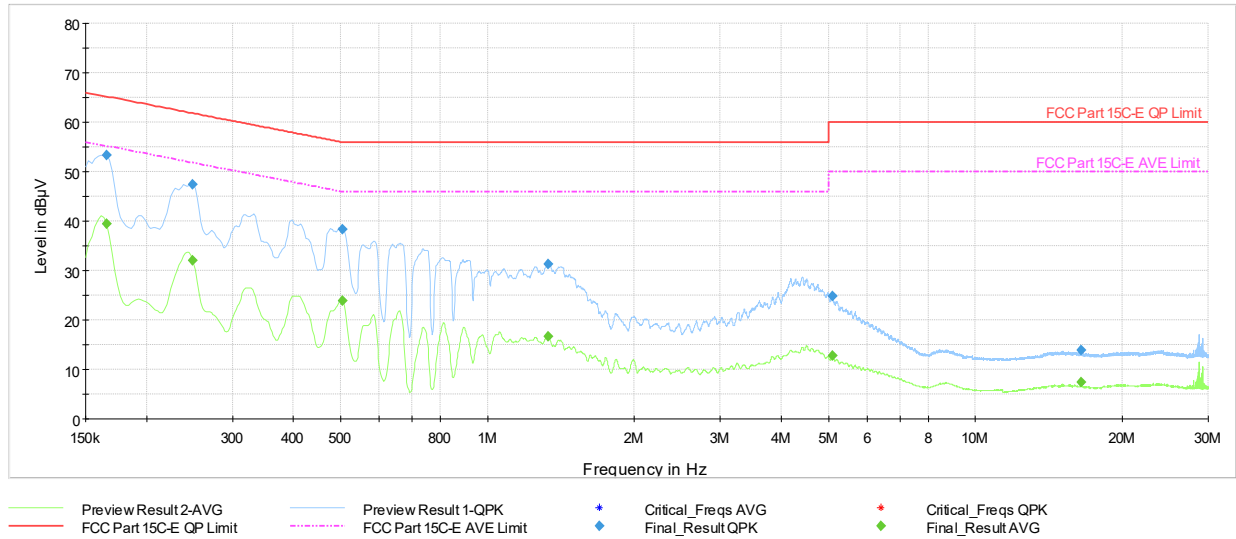
Plot 7-201. AC Line Conducted Emissions with 802.11be CDD (RU26) Ch.6 (N, with AC/DC Adapter)
