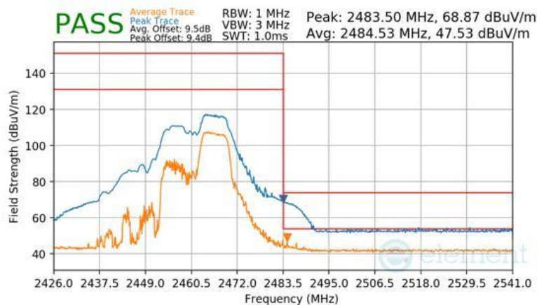
Plot 7-145 Radiated Restricted Upper Band Edge Measurement Antenna 1a (Peak & Average – RU52+26)
