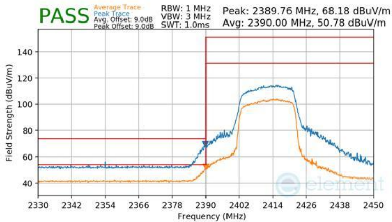
Plot 7-119 Radiated Restricted Lower Band Edge Measurement Antenna 3a (Peak & Average – RU242)
