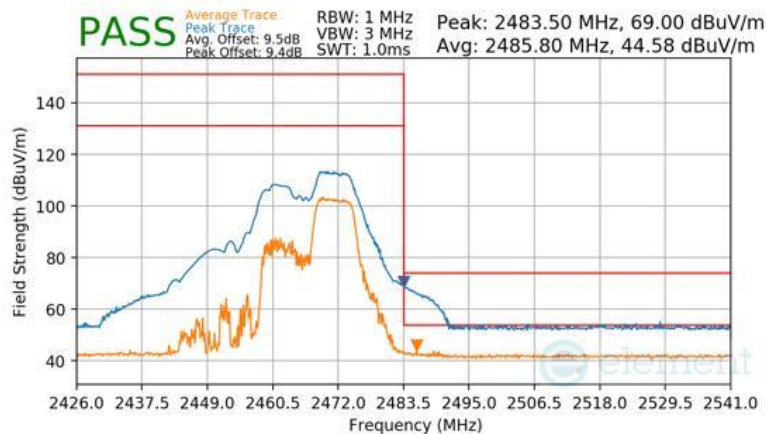
Plot 7-147 Radiated Restricted Upper Band Edge Measurement Antenna 1a (Peak & Average – RU52+26)
