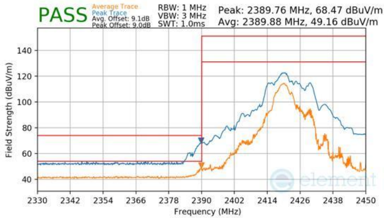
Plot 7-172 Radiated Restricted Lower Band Edge Measurement CDD (Peak & Average – RU52+26)
