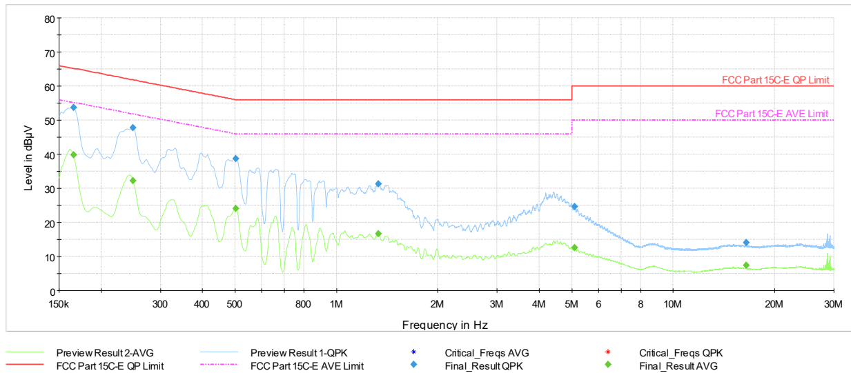
Plot 7-203. AC Line Conducted Emissions with 802.11be CDD (RU242) Ch.6 (N, with AC/DC Adapter)
