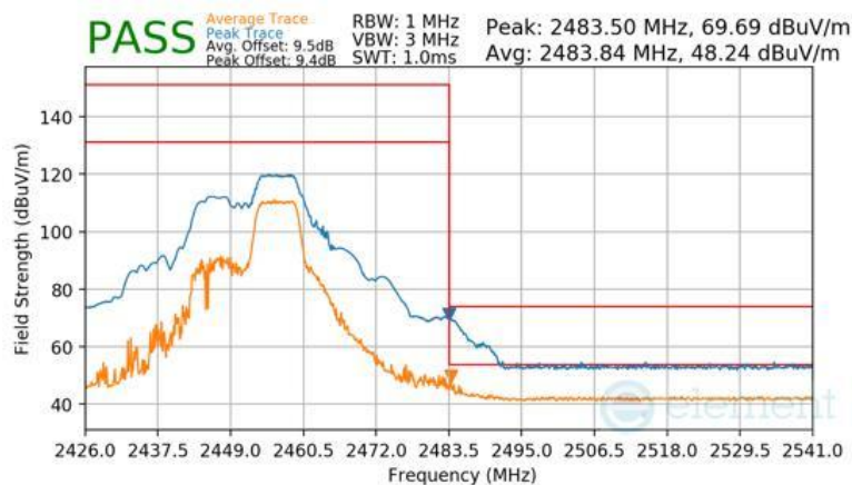
Plot 7-141 Radiated Restricted Upper Band Edge Measurement Antenna 1a (Peak & Average – RU52+26)
