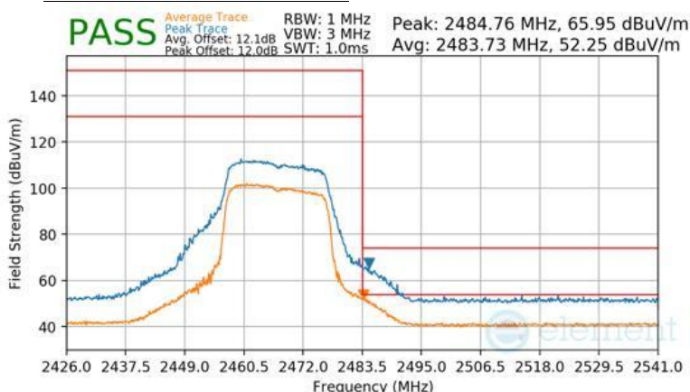
Plot 7-131 Radiated Restricted Upper Band Edge Measurement Antenna 3a (Peak & Average – RU242)
