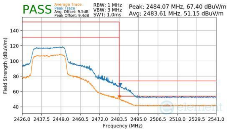
Plot 7-126 Radiated Restricted Upper Band Edge Measurement Antenna 3a (Peak & Average – RU242)
