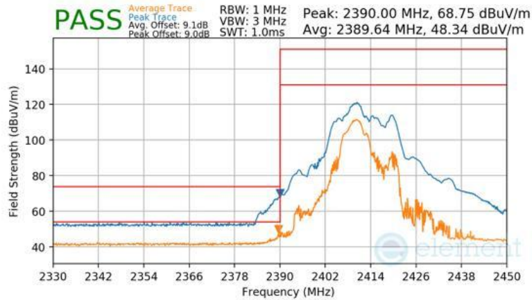
Plot 7-168 Radiated Restricted Lower Band Edge Measurement CDD (Peak & Average – RU52+26)
