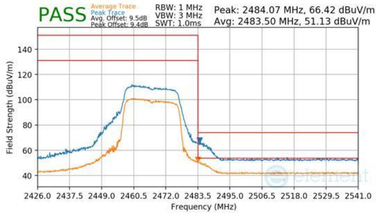
Plot 7-162 Radiated Restricted Upper Band Edge Measurement Antenna 1a (Peak & Average – RU242)
