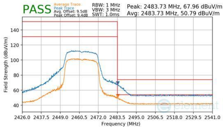
Plot 7-161 Radiated Restricted Upper Band Edge Measurement Antenna 1a (Peak & Average – RU242)
