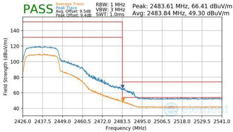
Plot 7-125 Radiated Restricted Upper Band Edge Measurement Antenna 3a (Peak & Average – RU242)
