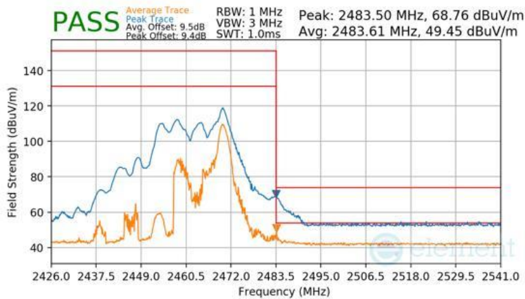
Plot 7-165 Radiated Restricted Upper Band Edge Measurement CDD (Peak & Average – RU26)
