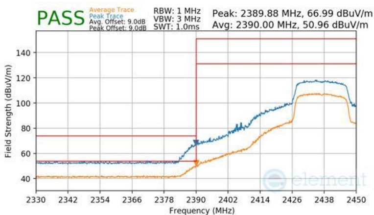
Plot 7-155 Radiated Restricted Lower Band Edge Measurement Antenna 1a (Peak & Average – RU242)
