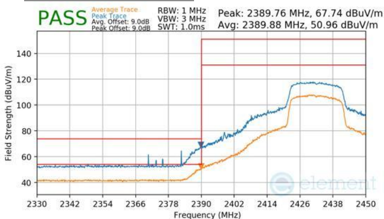
Plot 7-154 Radiated Restricted Lower Band Edge Measurement Antenna 1a (Peak & Average – RU242)
