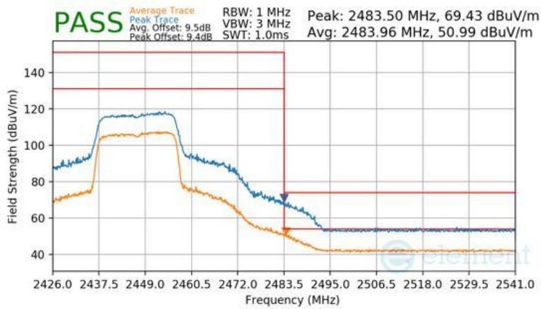
Plot 7-127 Radiated Restricted Upper Band Edge Measurement Antenna 3a (Peak & Average – RU242)
