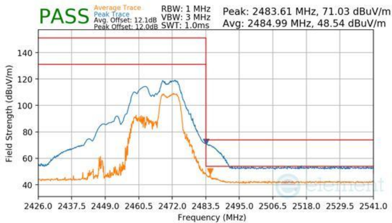
Plot 7-181 Radiated Restricted Upper Band Edge Measurement CDD (Peak & Average – RU52+26)
