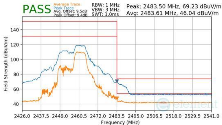
Plot 7-143 Radiated Restricted Upper Band Edge Measurement Antenna 1a (Peak & Average – RU52+26)
