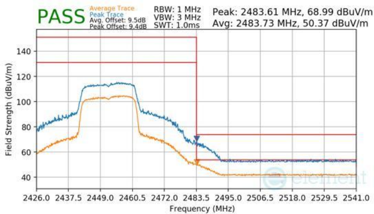
Plot 7-159 Radiated Restricted Upper Band Edge Measurement Antenna 1a (Peak & Average – RU242)
