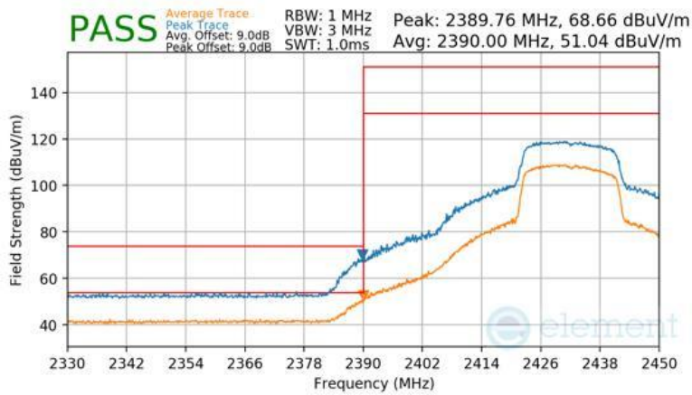
Plot 7-123 Radiated Restricted Lower Band Edge Measurement Antenna 3a (Peak & Average – RU242)
