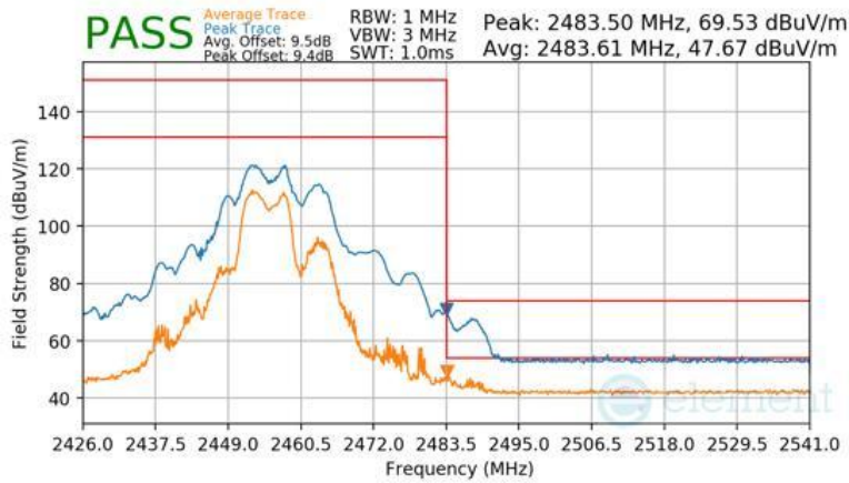
Plot 7-176 Radiated Restricted Upper Band Edge Measurement CDD (Peak & Average – RU52+26)
