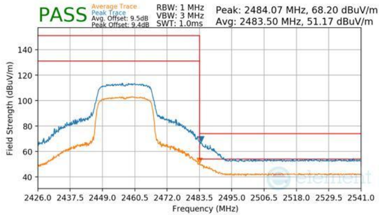
Plot 7-160 Radiated Restricted Upper Band Edge Measurement Antenna 1a (Peak & Average – RU242)
