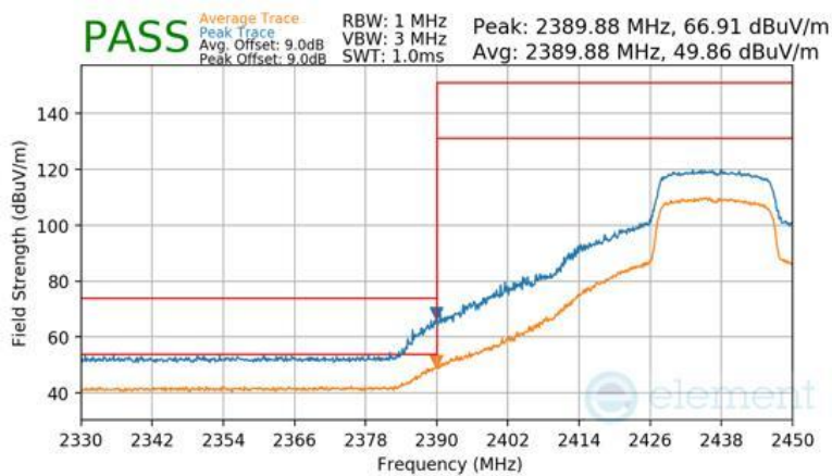
Plot 7-124 Radiated Restricted Lower Band Edge Measurement Antenna 3a (Peak & Average – RU242)
