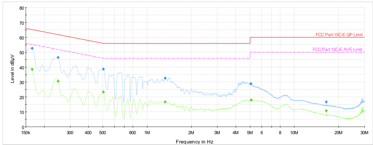
Plot 7-202. AC Line Conducted Emissions with 802.11be CDD (RU242) Ch.6 (L1, with AC/DC Adapter)
