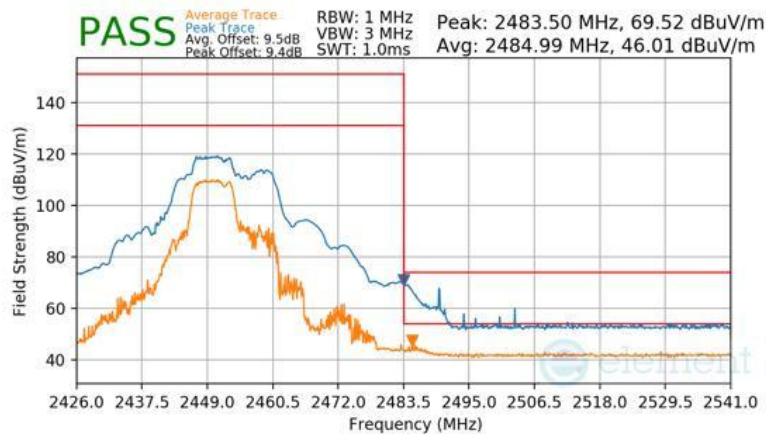
Plot 7-140 Radiated Restricted Upper Band Edge Measurement Antenna 1a (Peak & Average – RU52+26)
