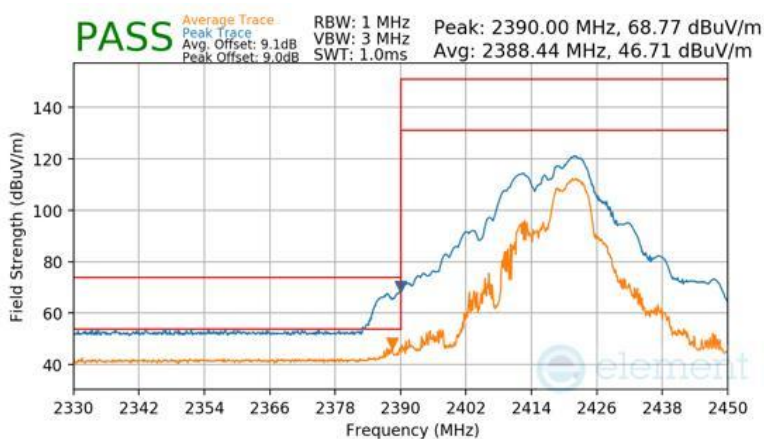
Plot 7-171 Radiated Restricted Lower Band Edge Measurement CDD (Peak & Average – RU52+26)
