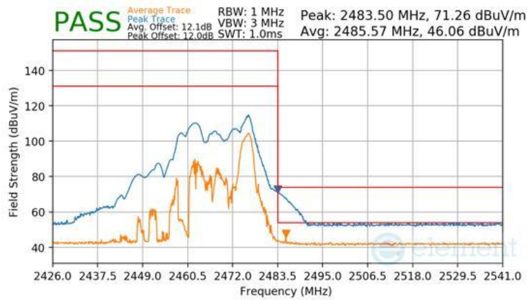
Plot 7-166 Radiated Restricted Upper Band Edge Measurement CDD (Peak & Average – RU26)
