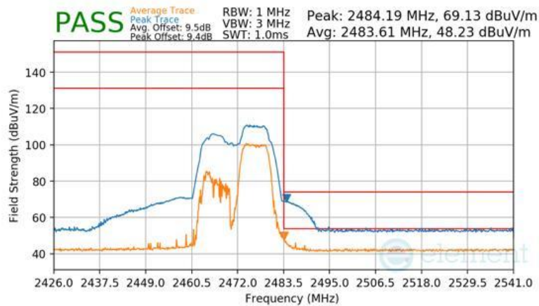
Plot 7-149 Radiated Restricted Upper Band Edge Measurement Antenna 1a (Peak & Average – RU52+26)
