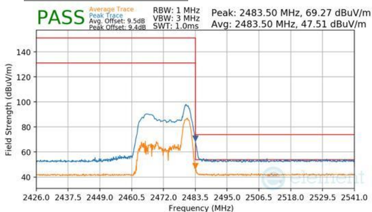
Plot 7-135 Radiated Restricted Upper Band Edge Measurement Antenna 1a (Peak & Average – RU26)
