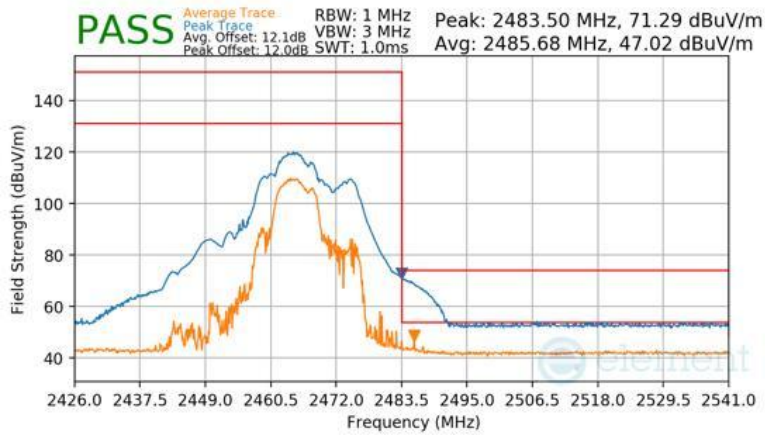
Plot 7-180 Radiated Restricted Upper Band Edge Measurement CDD (Peak & Average – RU52+26)
