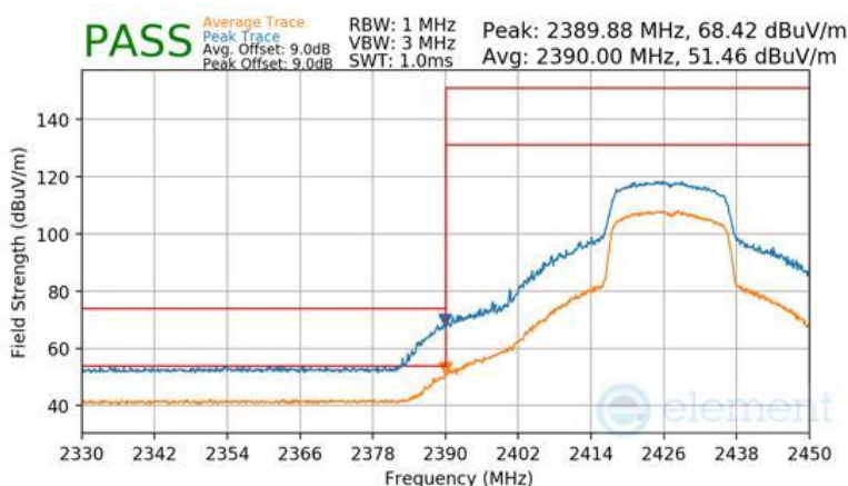
Plot 7-122 Radiated Restricted Lower Band Edge Measurement Antenna 3a (Peak & Average – RU242)
