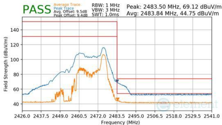
Plot 7-134 Radiated Restricted Upper Band Edge Measurement Antenna 1a (Peak & Average – RU26)
