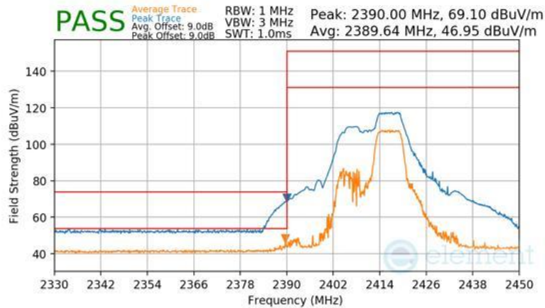
Plot 7-137 Radiated Restricted Lower Band Edge Measurement Antenna 1a (Peak & Average – RU52+26)
