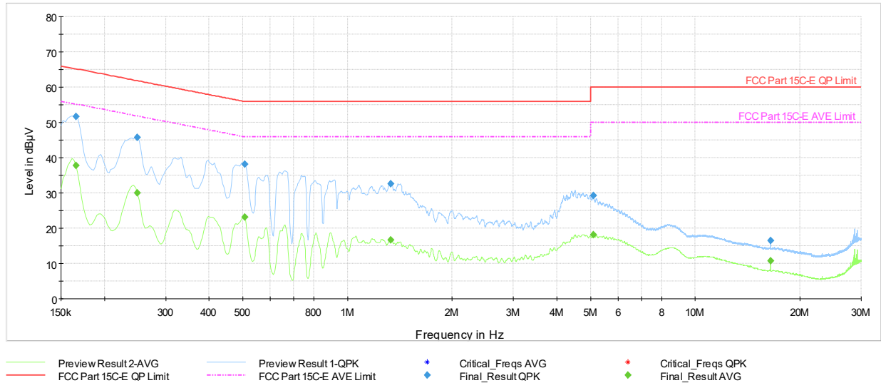
Plot 7-200. AC Line Conducted Emissions with 802.11be CDD (RU26) Ch.6 (L1, with AC/DC Adapter)
