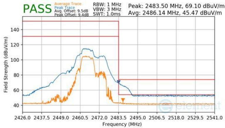
Plot 7-146 Radiated Restricted Upper Band Edge Measurement Antenna 1a (Peak & Average – RU52+26)
