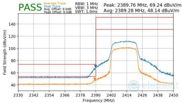
Plot 7-150 Radiated Restricted Lower Band Edge Measurement Antenna 1a (Peak & Average – RU242)
