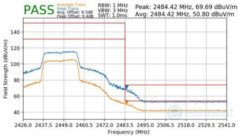
Plot 7-158 Radiated Restricted Upper Band Edge Measurement Antenna 1a (Peak & Average – RU242)
