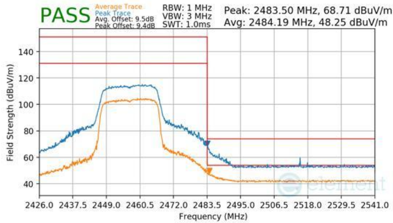
Plot 7-129 Radiated Restricted Upper Band Edge Measurement Antenna 3a (Peak & Average – RU242)
