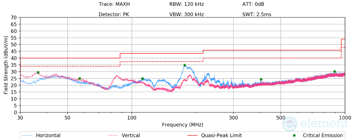
Plot 7-199. Radiated Spurious Emissions below 1GHz CDD Ch.6 (RU242), with AC/DC Adapter
