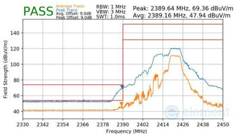
Plot 7-139 Radiated Restricted Lower Band Edge Measurement Antenna 1a (Peak & Average – RU52+26)
