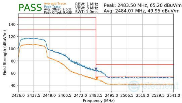
Plot 7-156 Radiated Restricted Upper Band Edge Measurement Antenna 1a (Peak & Average – RU242)
