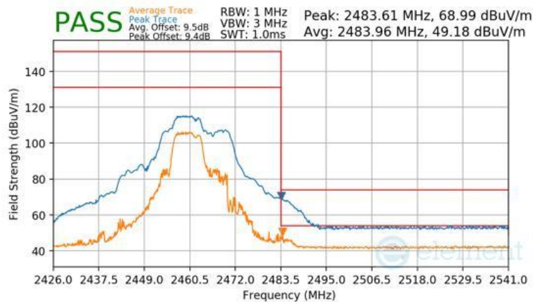
Plot 7-144 Radiated Restricted Upper Band Edge Measurement Antenna 1a (Peak & Average – RU52+26)
