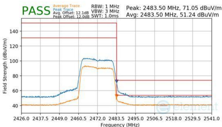
Plot 7-132 Radiated Restricted Upper Band Edge Measurement Antenna 3a (Peak & Average – RU242)
