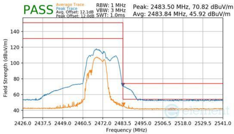
Plot 7-182 Radiated Restricted Upper Band Edge Measurement CDD (Peak & Average – RU52+26)
