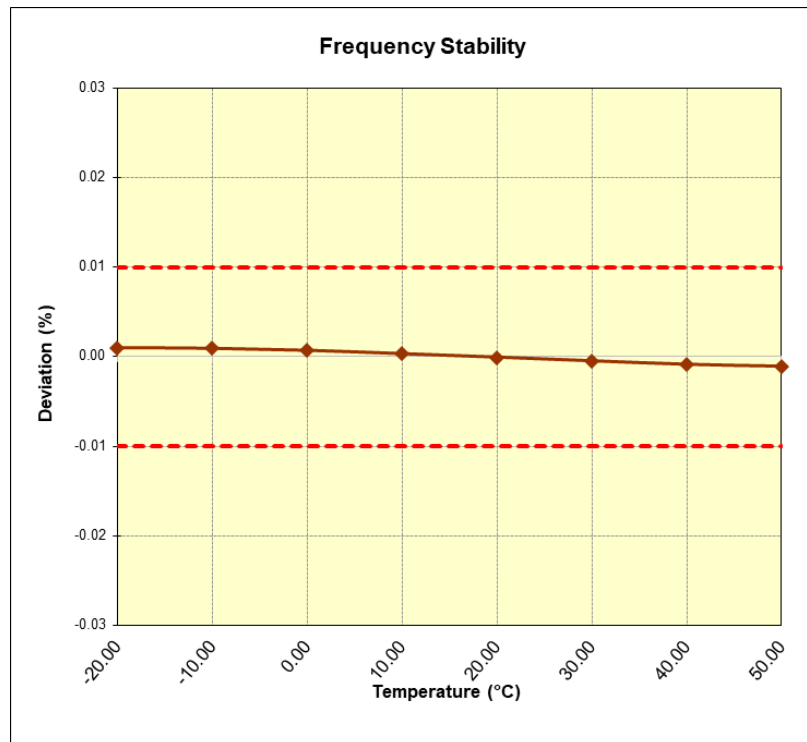
Figure 7-5. Frequency Stability Plot (Charging Rate 2.6C)
