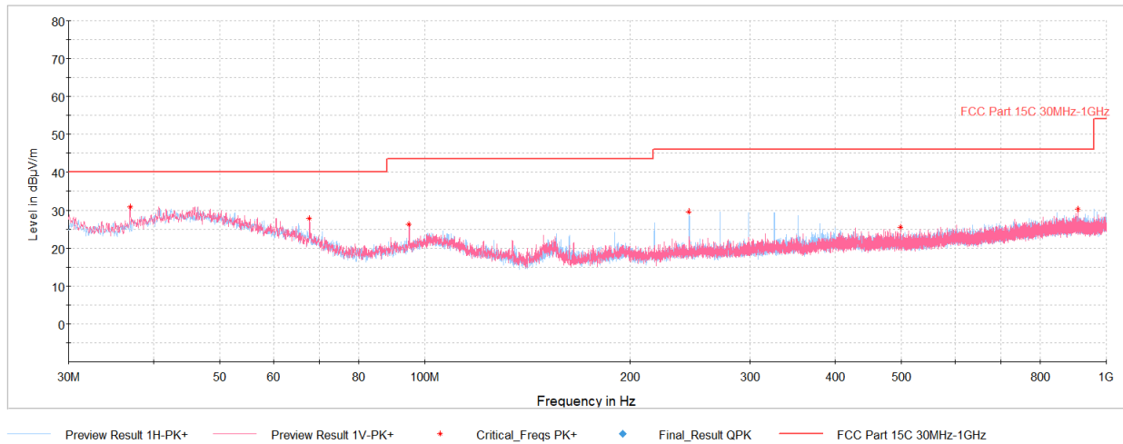
Plot 7-3. Radiated Spurious Emissions 30MHz – 1GHz (Charging Rate 2.6C, with Laptop)
