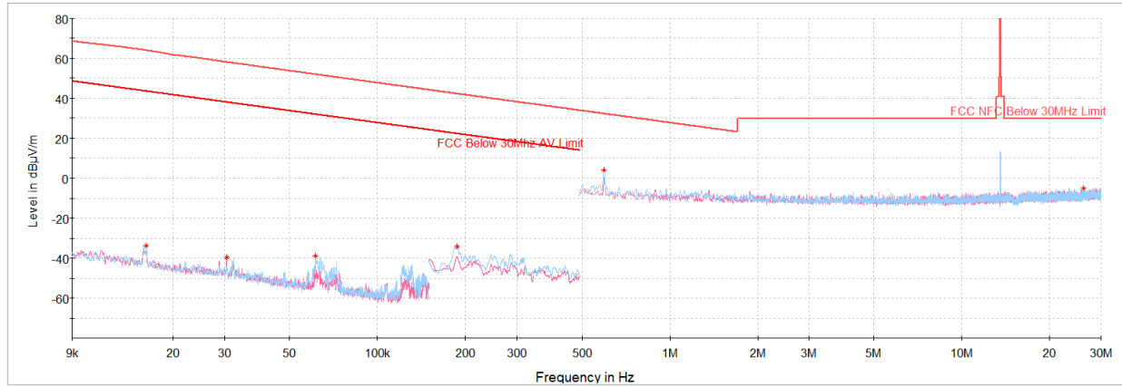
Plot 7-2. Radiated Spurious Plot 9kHz – 30MHz (Charging Rate 2.6C, with Laptop)
