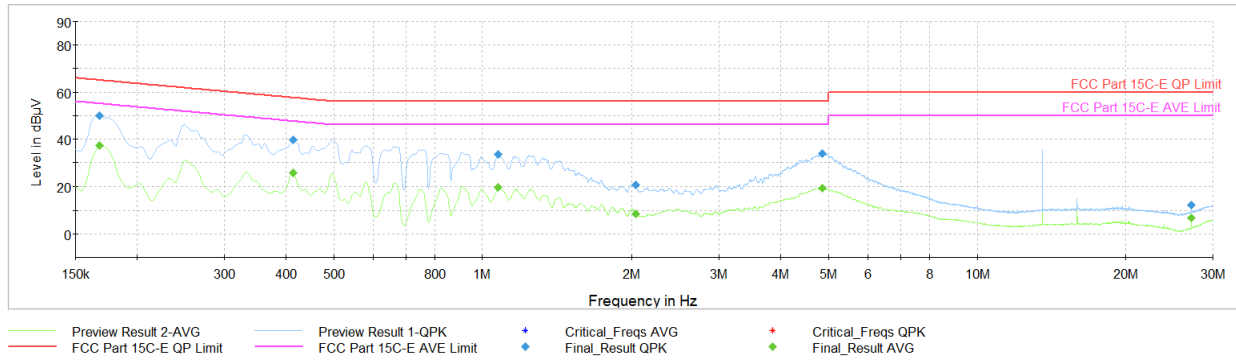
Plot 7-4. AC Line-Conducted Plot (L1, Charging Rate 2.6C, with AC/DC Adapter)
