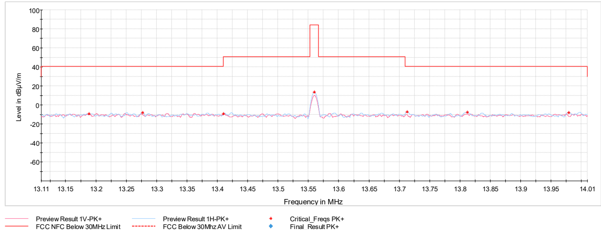
Plot 7-1. In Band Radiated Spurious Emissions (Charging Rate 2.6C, with Laptop)
