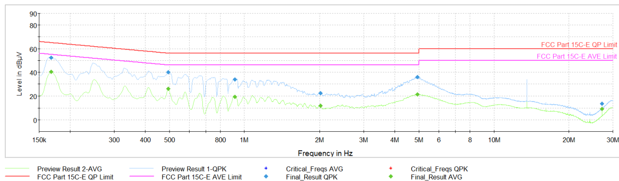
Plot 7-5. AC Line-Conducted Plot (N, Charging Rate 2.6C, with AC/DC Adapter)
