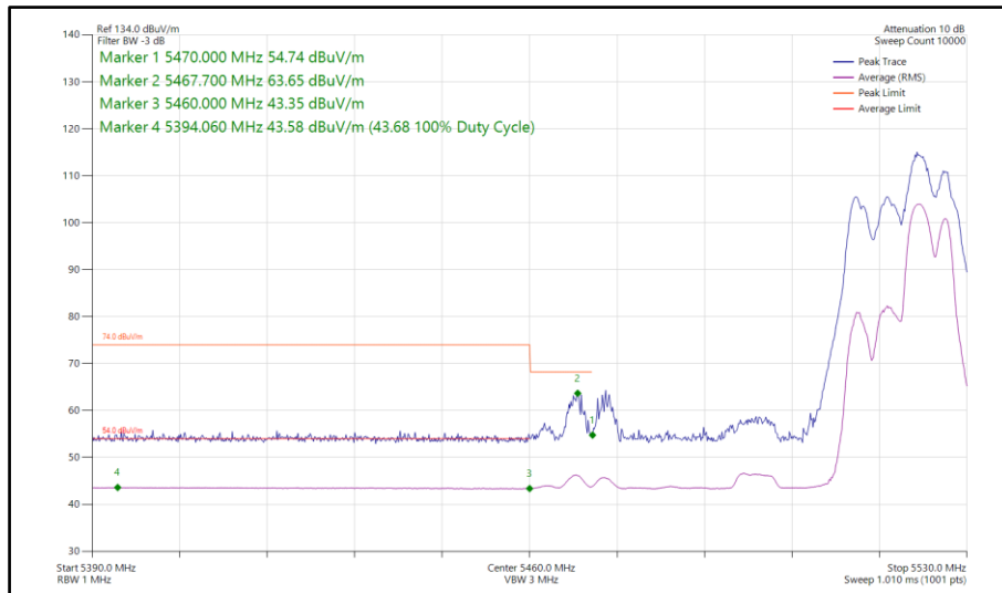
Figure 656 - 802.11be EHT40, RU52+26-75, SDM, Core 0-1 - 5510 MHz Band Edge Frequency 5470 MHz
