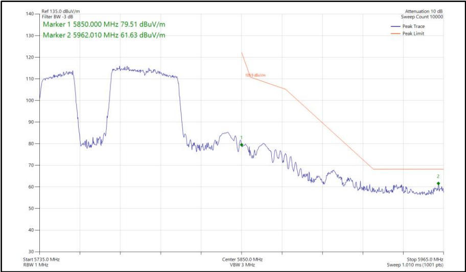
Figure 707 - 802.11be EHT80, RU484+242-91, SISO, Core 0 - 5775 MHz Band Edge Frequency 5850 MHz
