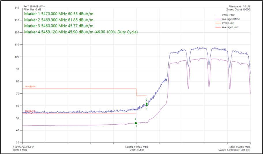
Figure 683 - 802.11a a80, SISO, Core 0 - 5530 MHz Band Edge Frequency 5470 MHz
