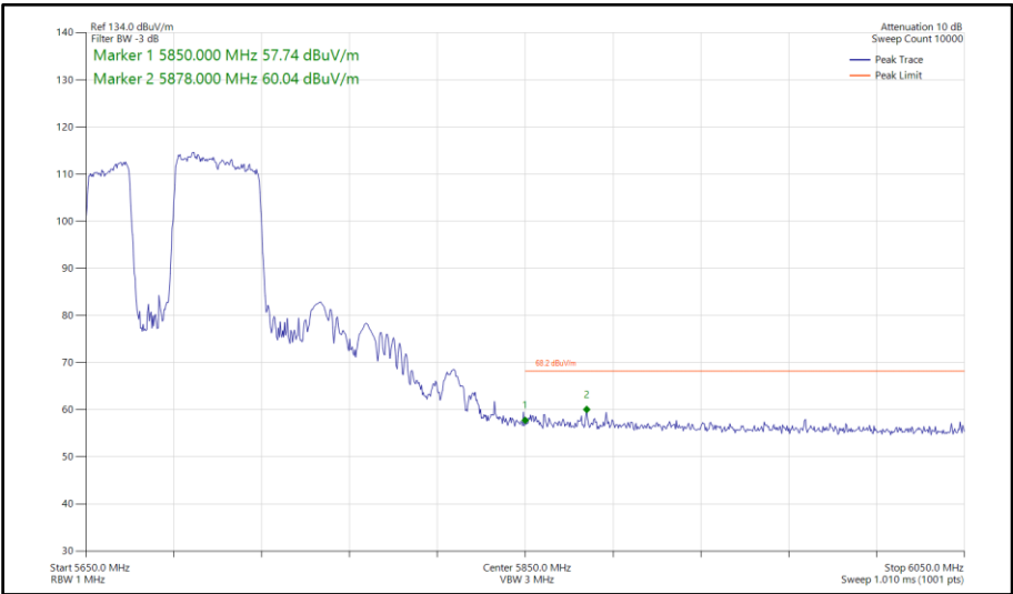
Figure 706 - 802.11be EHT80, RU484+242-91, SISO, Core 0 - 5690 MHz Band Edge Frequency 5850 MHz
