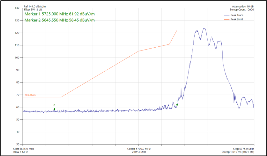
Figure 636 - 802.11ax HE40, RU106-53, CDD, Core 0-1 - 5755 MHz Band Edge Frequency 5725 MHz
