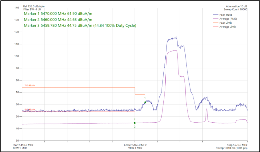
Figure 687 - 802.11be EHT80, RU106+26-82, SISO, Core 0 - 5530 MHz Band Edge Frequency 5470 MHz
