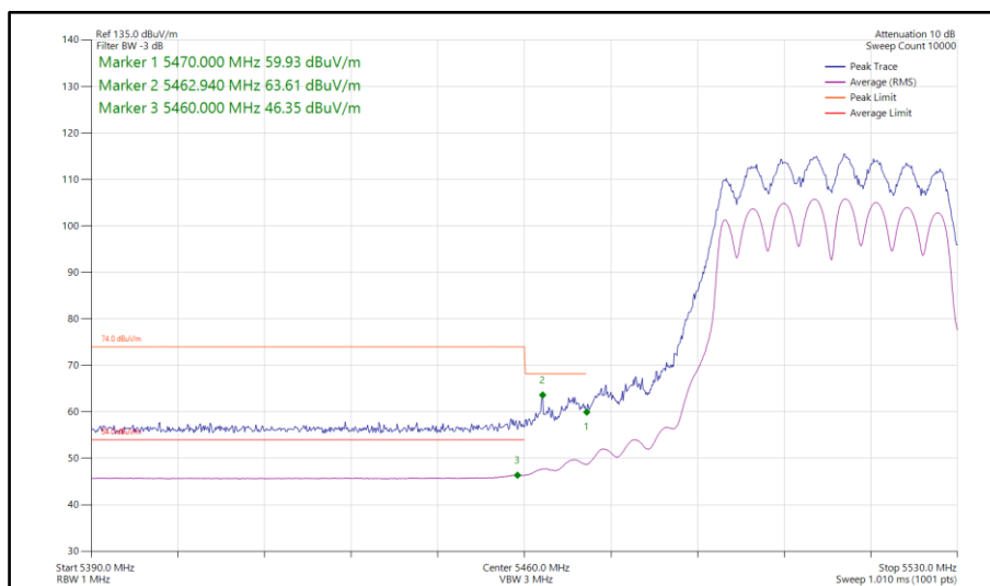
Figure 629 - 802.11n HT40, CDD, Core 0-1 - 5510 MHz Band Edge Frequency 5470 MHz
