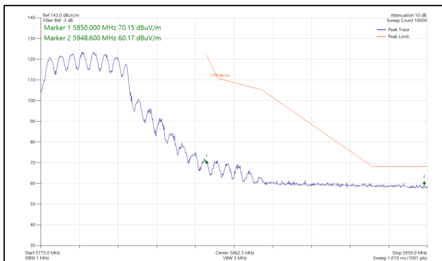
Figure 649 - 802.11ax HE40, SU, CDD, Core 0-1 - 5795 MHz Band Edge Frequency 5850 MHz
