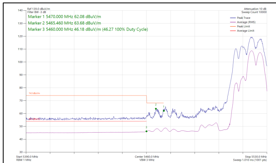
Figure 632 - 802.11be EHT40, RU106+26-85, CDD, Core 0-1 - 5510 MHz Band Edge Frequency 5470 MHz
