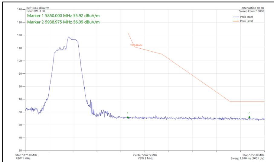
Figure 625 - 802.11ax HE40, RU106-56, SISO, Core 1 - 5795 MHz Band Edge Frequency 5850 MHz
