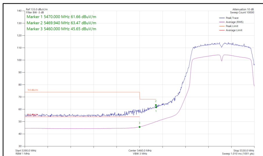
Figure 673 - 802.11ac VHT40, TxBF, Core 0-1 - 5510 MHz Band Edge Frequency 5470 MHz
