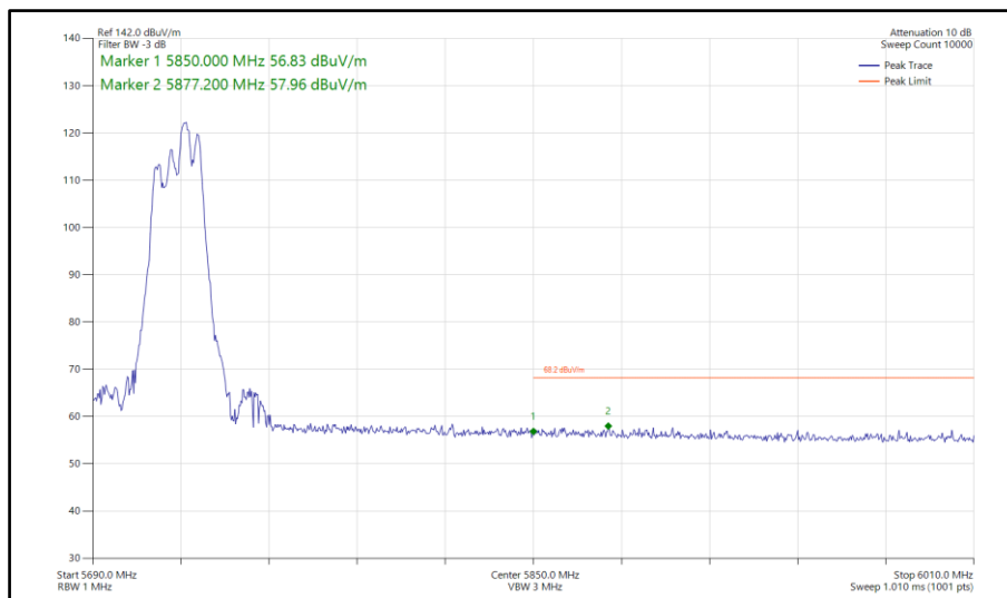
Figure 648 - 802.11ax HE40, RU106-56, CDD, Core 0-1 - 5710 MHz Band Edge Frequency 5850 MHz
