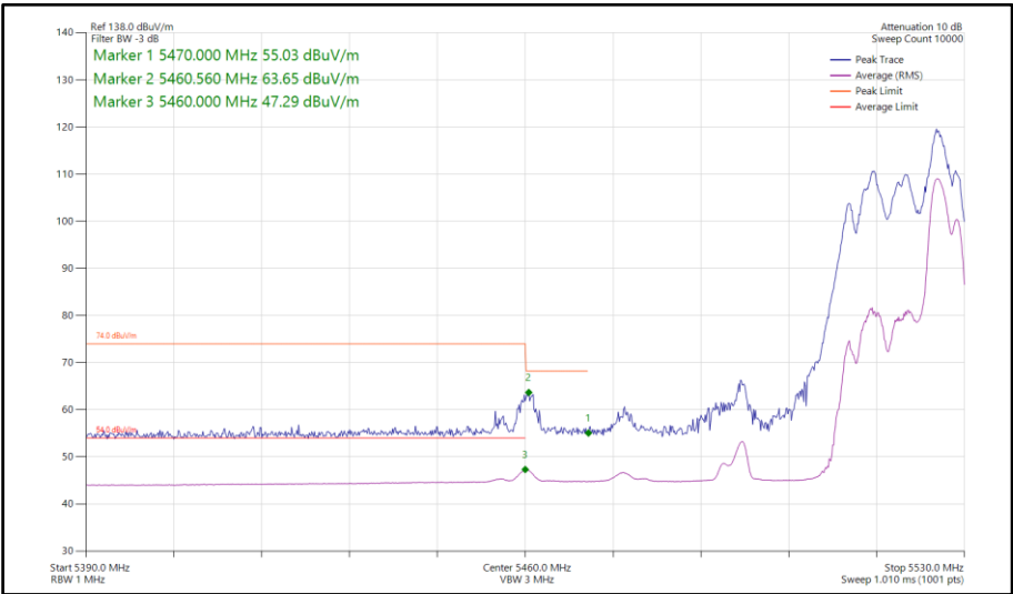
Figure 631 - 802.11ax HE40, RU52-44, CDD, Core 0-1 - 5510 MHz Band Edge Frequency 5470 MHz
