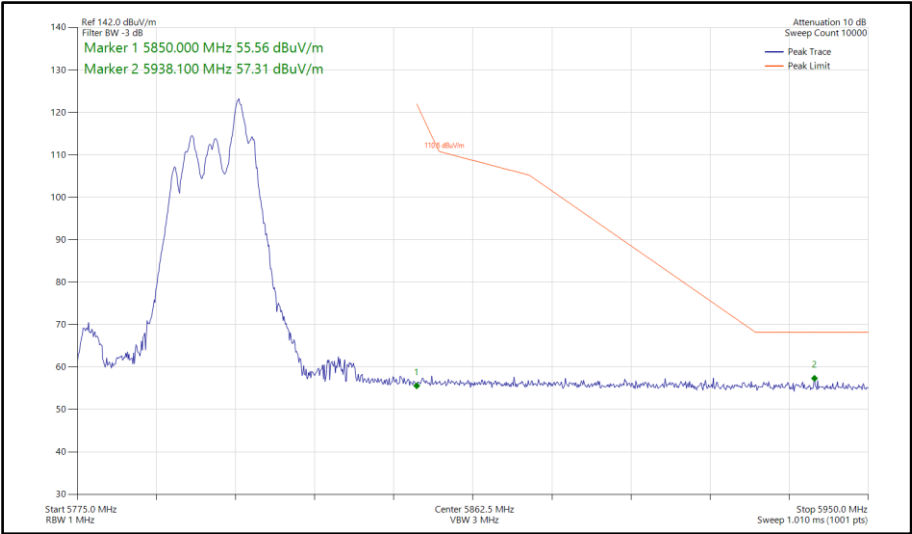
Figure 670 - 802.11ax HE40, RU52-44, SDM, Core 0-1 - 5795 MHz Band Edge Frequency 5850 MHz
