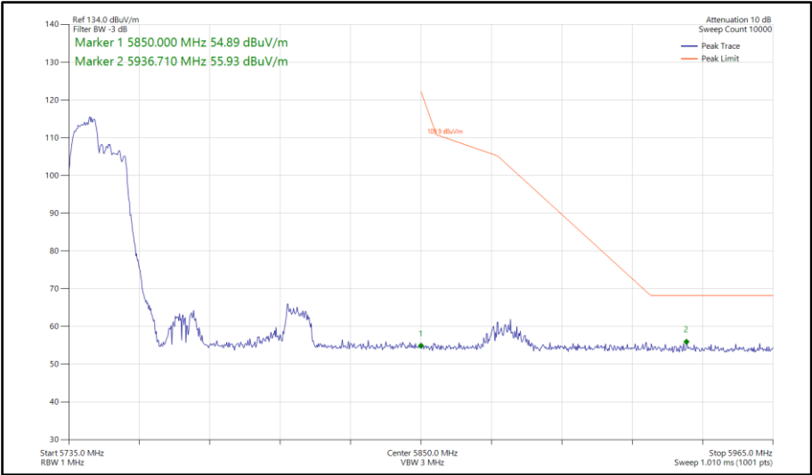
Figure 705 - 802.11ax HE80, RU106-53, SISO, Core 0 - 5775 MHz Band Edge Frequency 5850 MHz
