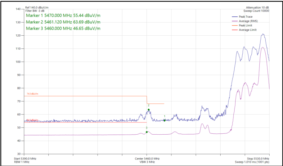
Figure 655 - 802.11ax HE40, RU52-44, SDM, Core 0-1 - 5510 MHz Band Edge Frequency 5470 MHz
