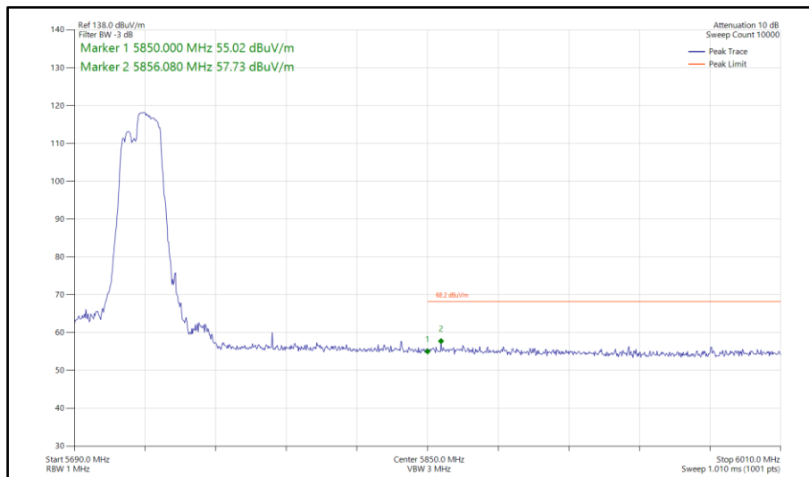
Figure 626 - 802.11be EHT40, RU106+26-85, SISO, Core 1 - 5710 MHz Band Edge Frequency 5850 MHz
