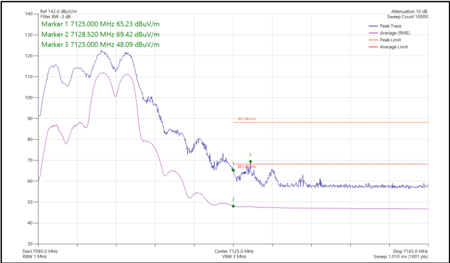
Figure 324 - 802.11ax HE20, RU106-54, CDD, Core 0-1 - 7095 MHz Band Edge Frequency 7125 MHz
