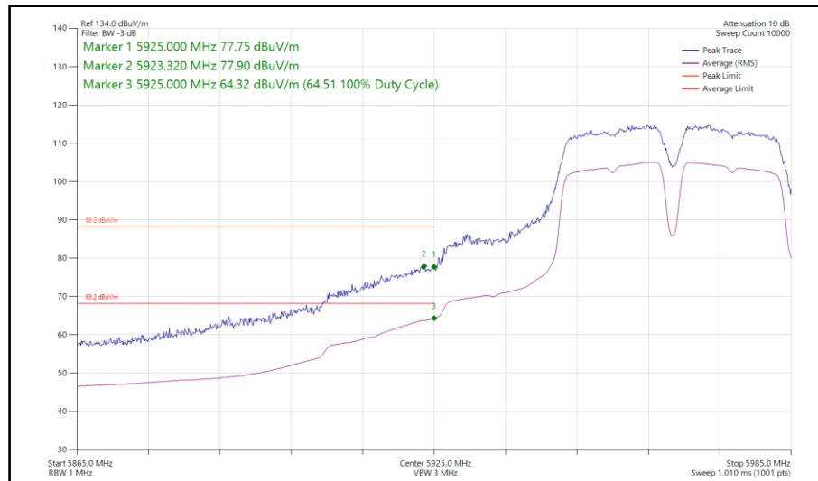
Figure 348 - 802.11a a40, SISO, Core 1 - 5965 MHz Band Edge Frequency 5925 MHz
