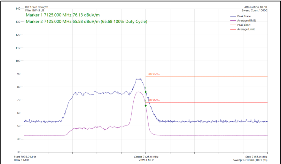
Figure 302 - 802.11ax HE20, RU26-8, SISO, Core 0 - 7115 MHz Band Edge Frequency 7125 MHz
