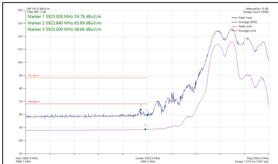
Figure 330 - 802.11ax HE20, RU106-53, SDM, Core 0-1 - 5955 MHz Band Edge Frequency 5925 MHz
