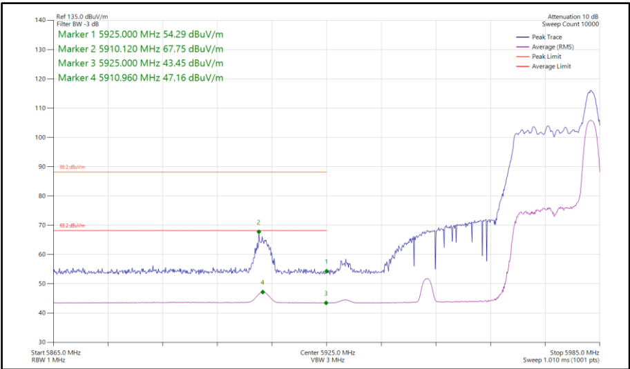
Figure 350 - 802.11ax HE40, RU26-17, SISO, Core 1 - 5965 MHz Band Edge Frequency 5925 MHz
