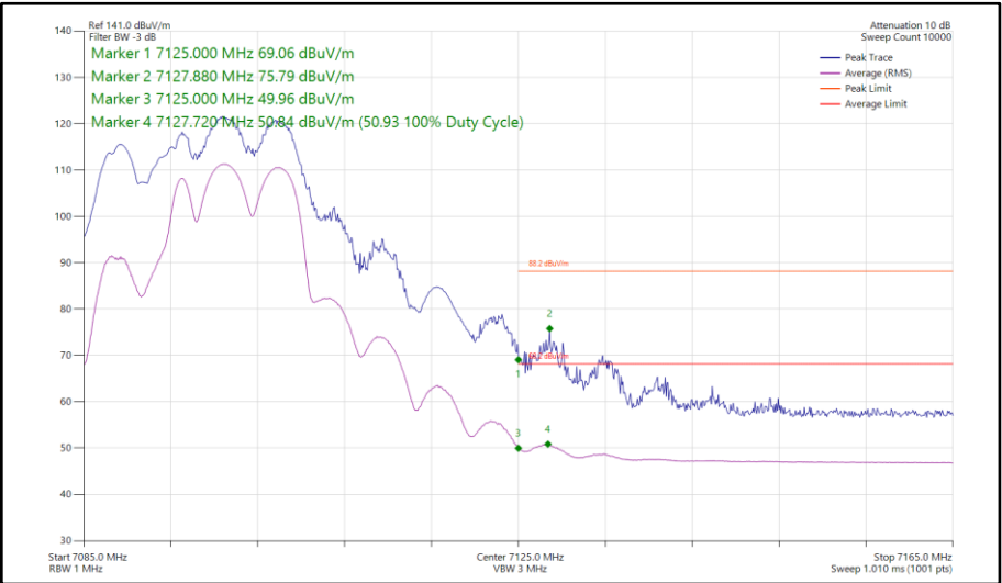
Figure 336 - 802.11be EHT20, RU106+26-83, SDM, Core 0-1 - 7095 MHz Band Edge Frequency 7125 MHz
