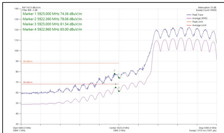
Figure 357 - 802.11ax HE40, SU, CDD, Core 0-1 - 5965 MHz Band Edge Frequency 5925 MHz
