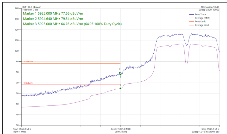
Figure 340 - 802.11a a40, SISO, Core 0 - 5965 MHz Band Edge Frequency 5925 MHz
