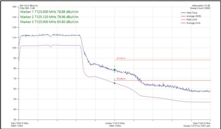
Figure 345 - 802.11ax HE40, SU, SISO, Core 0 - 7085 MHz Band Edge Frequency 7125 MHz
