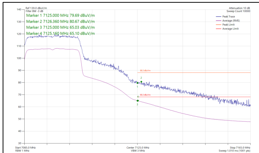
Figure 332 - 802.11ax HE20, SU, SDM, Core 0-1 - 7095 MHz Band Edge Frequency 7125 MHz
