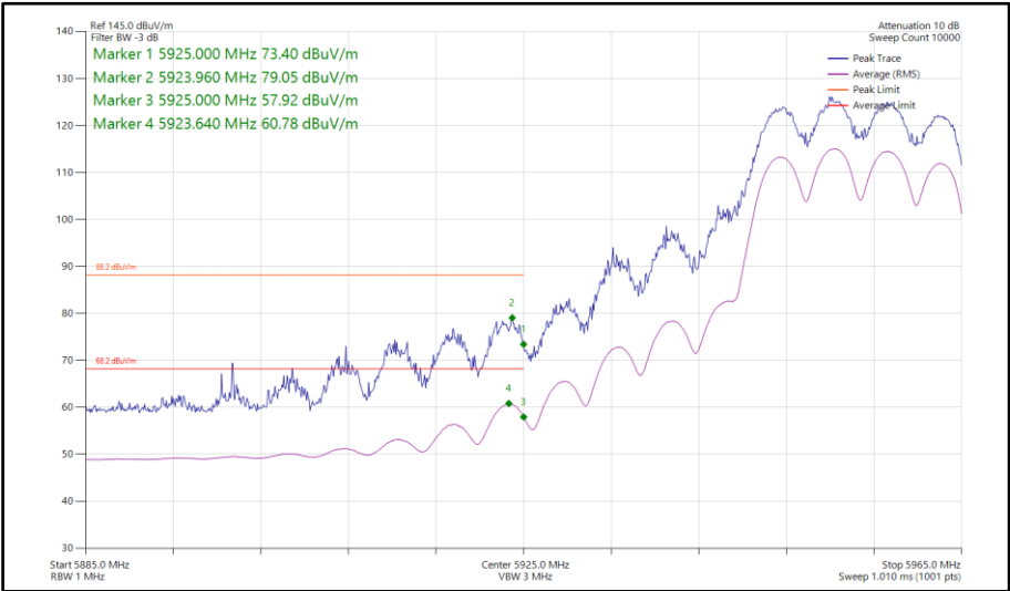
Figure 318 - 802.11ax HE20, SU, CDD, Core 0-1 - 5955 MHz Band Edge Frequency 5925 MHz
