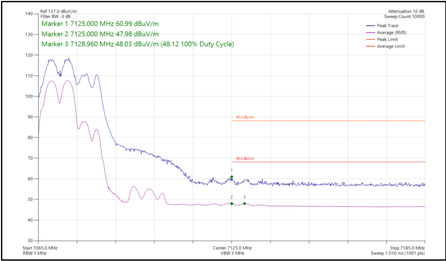
Figure 363 - 802.11be EHT40, RU106+26-82, CDD, Core 0-1 - 7085 MHz Band Edge Frequency 7125 MHz
