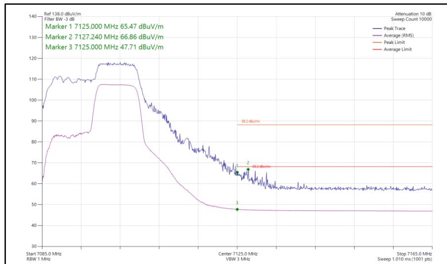
Figure 300 - 802.11ax HE20, RU106-54, SISO, Core 0 - 7095 MHz Band Edge Frequency 7125 MHz
