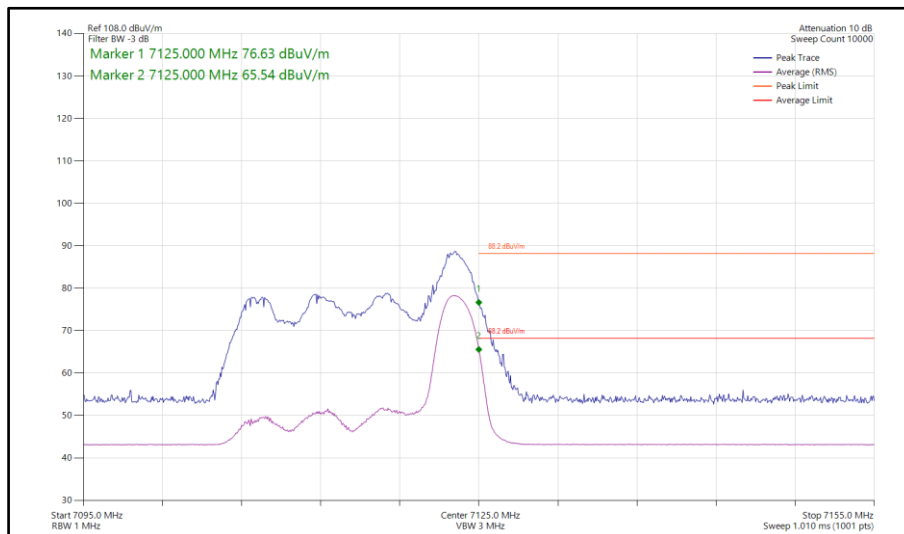
Figure 326 - 802.11ax HE20, RU26-8, CDD, Core 0-1 - 7115 MHz Band Edge Frequency 7125 MHz
