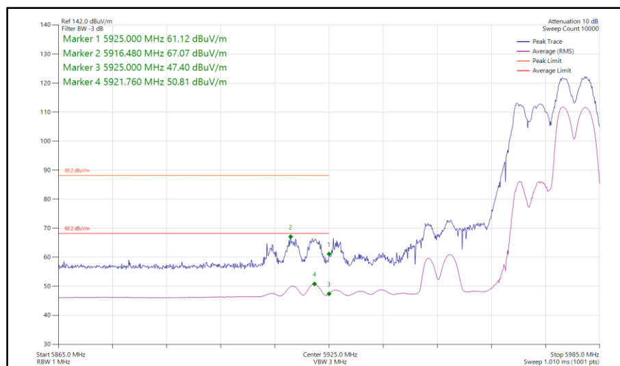
Figure 358 - 802.11ax HE40, RU106-56, CDD, Core 0-1 - 5965 MHz Band Edge Frequency 5925 MHz
