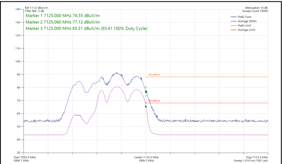
Figure 337 - 802.11be EHT20, RU106+26-83, SDM, Core 0-1 - 7115 MHz Band Edge Frequency 7125 MHz
