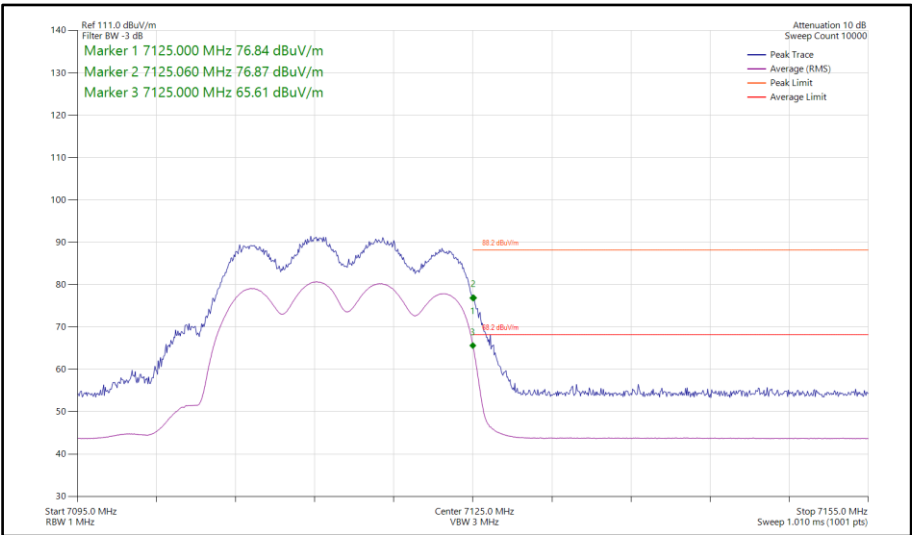
Figure 325 - 802.11ax HE20, SU, CDD, Core 0-1 - 7115 MHz Band Edge Frequency 7125 MHz
