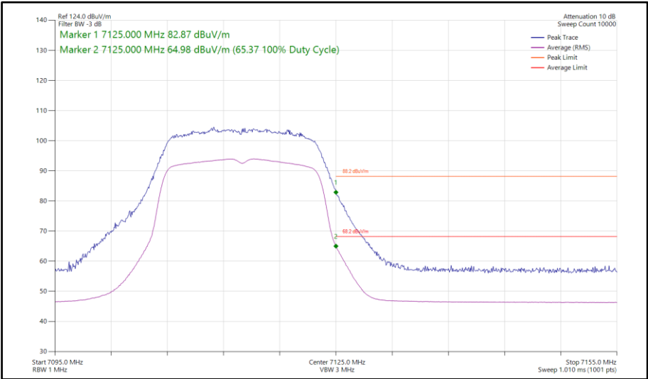
Figure 310 - 802.11a, SISO, Core 1 - 7115 MHz Band Edge Frequency 7125 MHz
