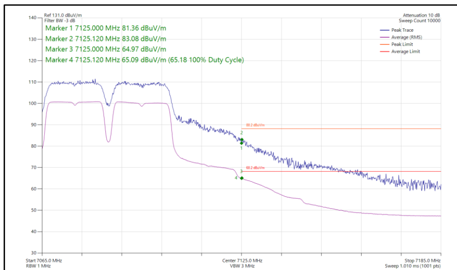
Figure 344 - 802.11a a40, SISO, Core 0 - 7085 MHz Band Edge Frequency 7125 MHz
