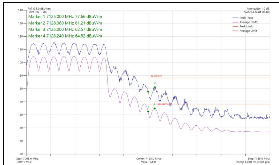
Figure 361 - 802.11ax HE40, SU, CDD, Core 0-1 - 7085 MHz Band Edge Frequency 7125 MHz
