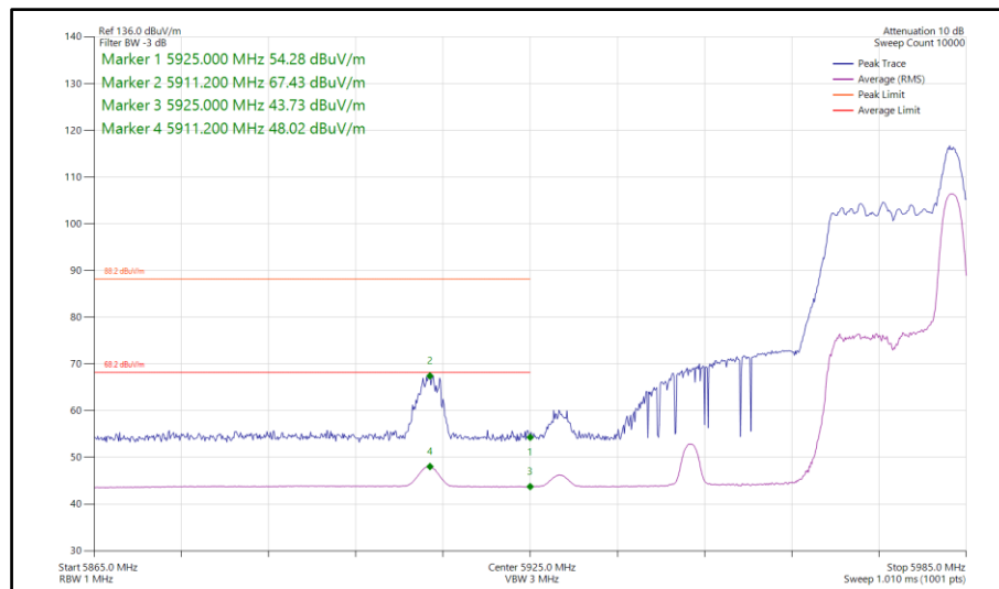
Figure 342 - 802.11ax HE40, RU26-17, SISO, Core 0 - 5965 MHz Band Edge Frequency 5925 MHz
