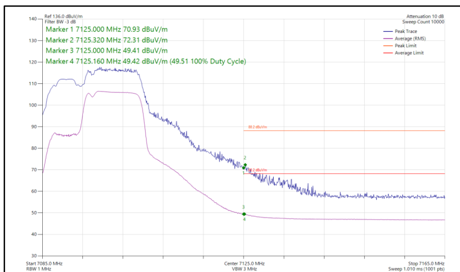
Figure 315 - 802.11be EHT20, RU106+26-83, SISO, Core 1 - 7095 MHz Band Edge Frequency 7125 MHz
