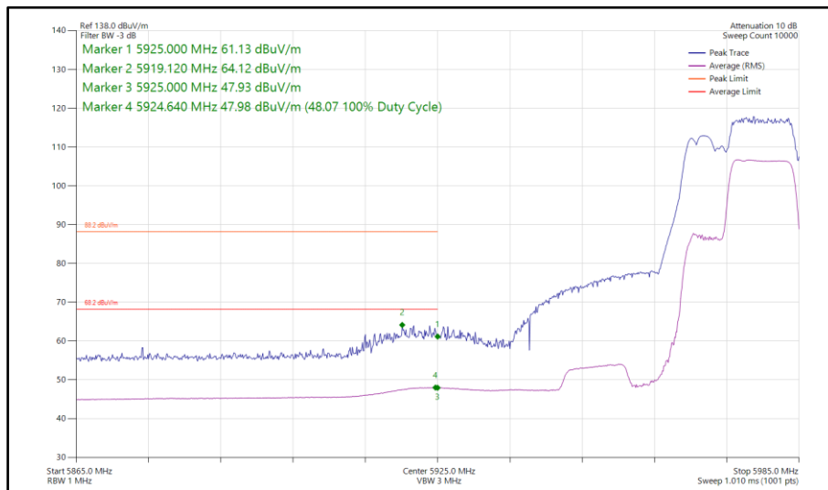
Figure 343 - 802.11be EHT40, RU106+26-85, SISO, Core 0 - 5965 MHz Band Edge Frequency 5925 MHz
