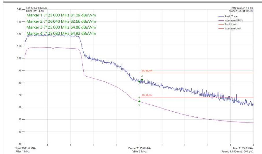
Figure 339 - 802.11ax HE20, SU, TxBF, Core 0-1 - 7095 MHz Band Edge Frequency 7125 MHz
