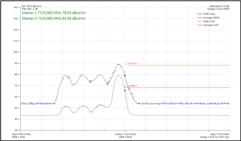
Figure 335 - 802.11ax HE20, RU26-8, SDM, Core 0-1 - 7115 MHz Band Edge Frequency 7125 MHz
