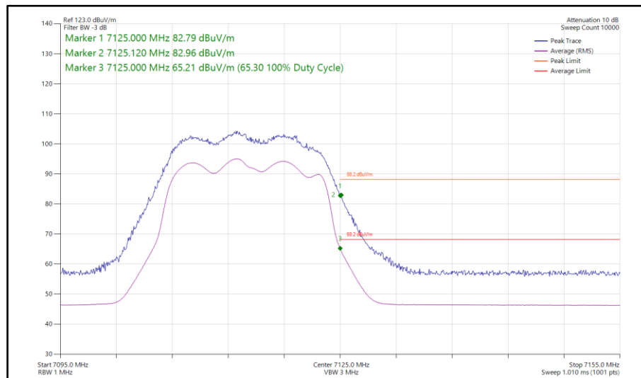
Figure 322 - 802.11a, CDD, Core 0-1 - 7115 MHz Band Edge Frequency 7125 MHz
