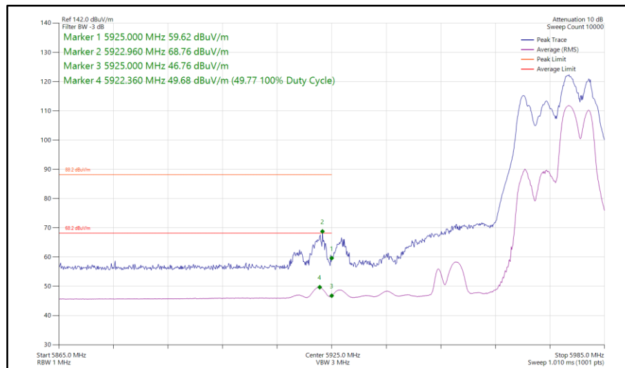
Figure 359 - 802.11be EHT40, RU52+26-75, CDD, Core 0-1 - 5965 MHz Band Edge Frequency 5925 MHz
