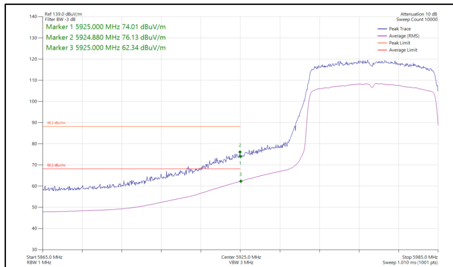
Figure 364 - 802.11ax HE40, SU, SDM, Core 0-1 - 5965 MHz Band Edge Frequency 5925 MHz
