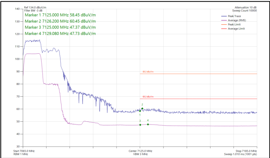
Figure 346 - 802.11ax HE40, RU106-53, SISO, Core 0 - 7085 MHz Band Edge Frequency 7125 MHz
