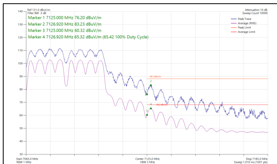
Figure 360 - 802.11a a40, CDD, Core 0-1 - 7085 MHz Band Edge Frequency 7125 MHz
