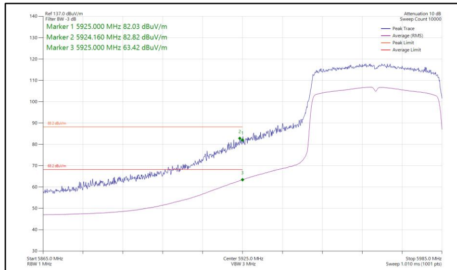
Figure 341 - 802.11ax HE40, SU, SISO, Core 0 - 5965 MHz Band Edge Frequency 5925 MHz
