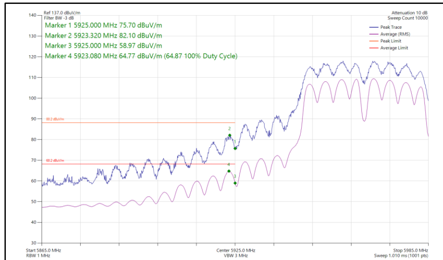
Figure 356 - 802.11a a40, CDD, Core 0-1 - 5965 MHz Band Edge Frequency 5925 MHz
