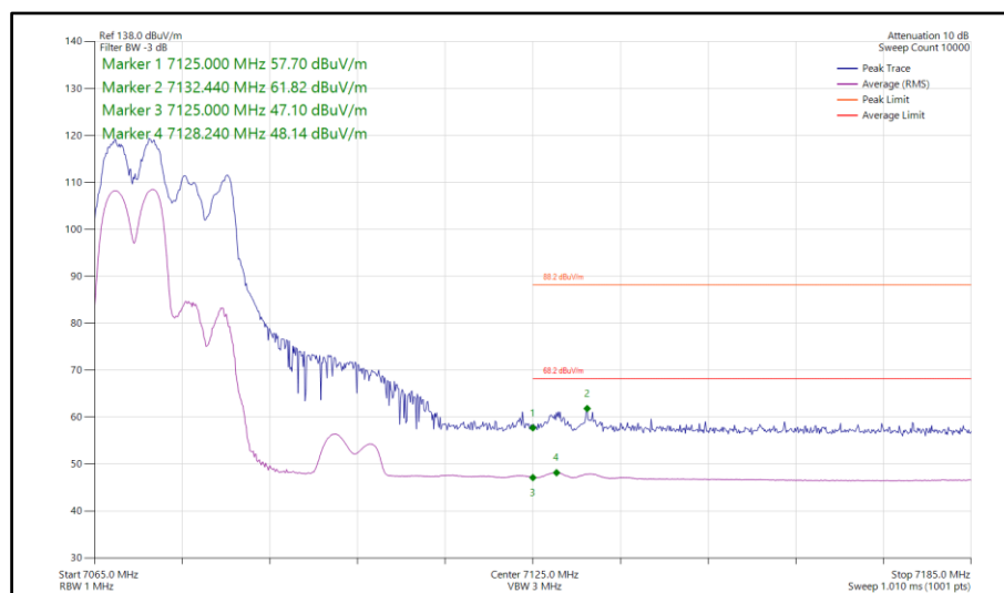
Figure 362 - 802.11ax HE40, RU106-53, CDD, Core 0-1 - 7085 MHz Band Edge Frequency 7125 MHz
