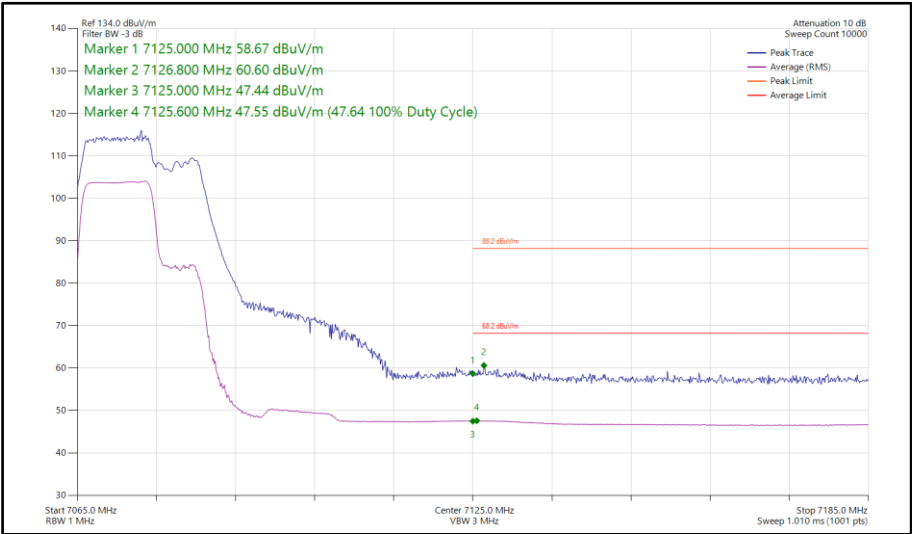
Figure 347 - 802.11be EHT40, RU106+26-82, SISO, Core 0 - 7085 MHz Band Edge Frequency 7125 MHz
