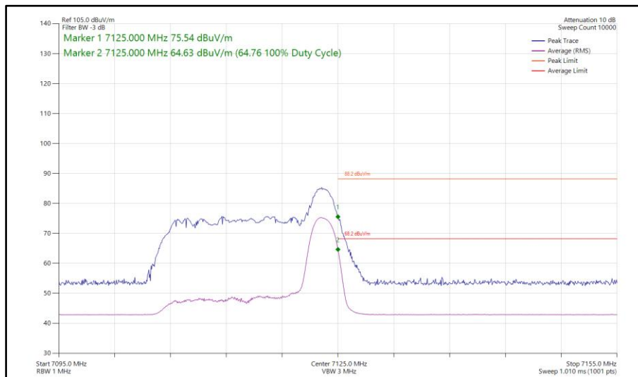
Figure 314 - 802.11ax HE20, RU26-8, SISO, Core 1 - 7115 MHz Band Edge Frequency 7125 MHz
