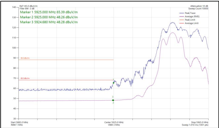
Figure 319 - 802.11ax HE20, RU106-53, CDD, Core 0-1 - 5955 MHz Band Edge Frequency 5925 MHz
