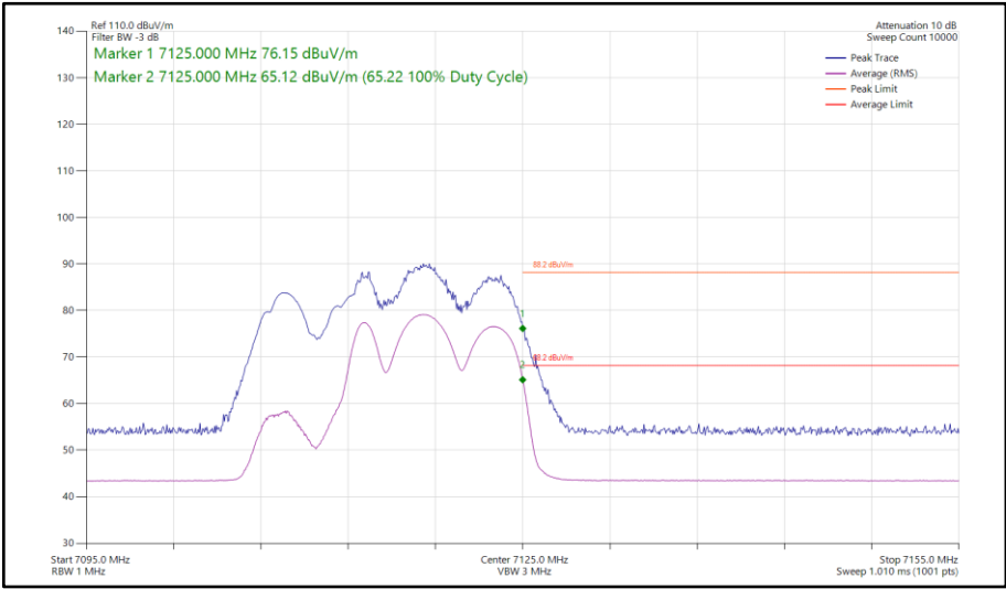
Figure 328 - 802.11be EHT20, RU106+26-83, CDD, Core 0-1 - 7115 MHz Band Edge Frequency 7125 MHz
