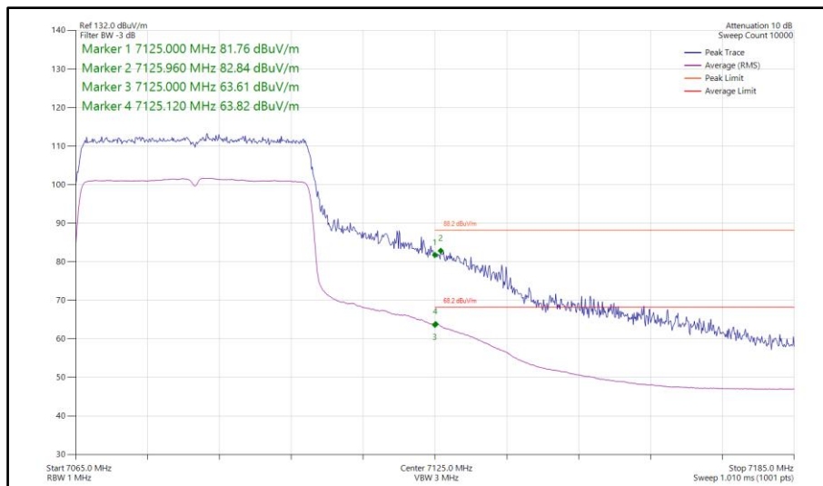
Figure 367 - 802.11ax HE40, SU, SDM, Core 0-1 - 7085 MHz Band Edge Frequency 7125 MHz
