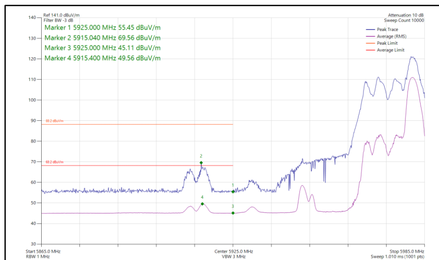
Figure 365 - 802.11ax HE40, RU52-44, SDM, Core 0-1 - 5965 MHz Band Edge Frequency 5925 MHz
