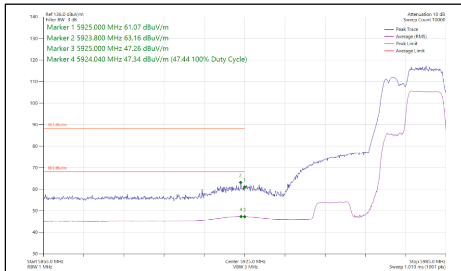
Figure 351 - 802.11be EHT40, RU106+26-85, SISO, Core 1 - 5965 MHz Band Edge Frequency 5925 MHz
