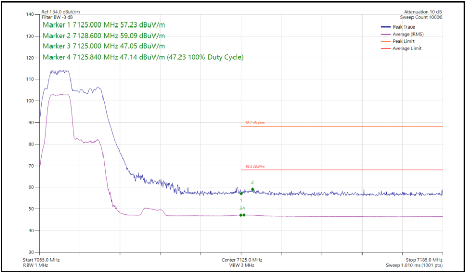
Figure 355 - 802.11be EHT40, RU52+26-70, SISO, Core 1 - 7085 MHz Band Edge Frequency 7125 MHz
