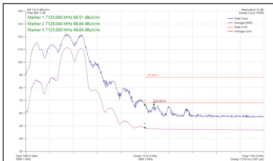
Figure 333 - 802.11ax HE20, RU106-54, SDM, Core 0-1 - 7095 MHz Band Edge Frequency 7125 MHz
