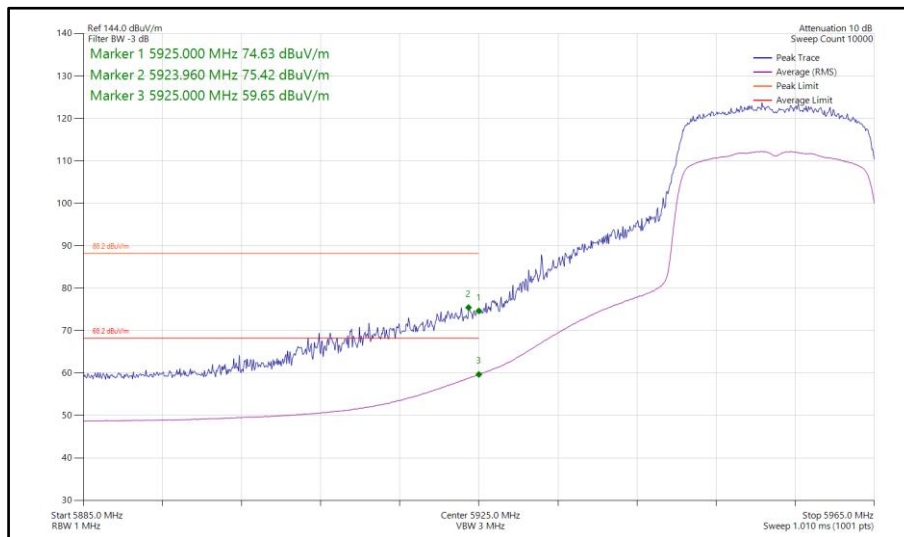
Figure 329 - 802.11ax HE20, SU, SDM, Core 0-1 - 5955 MHz Band Edge Frequency 5925 MHz
