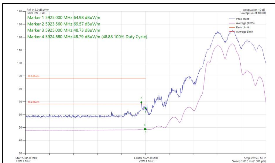
Figure 331 - 802.11be EHT20, RU106+26-82, SDM, Core 0-1 - 5955 MHz Band Edge Frequency 5925 MHz
