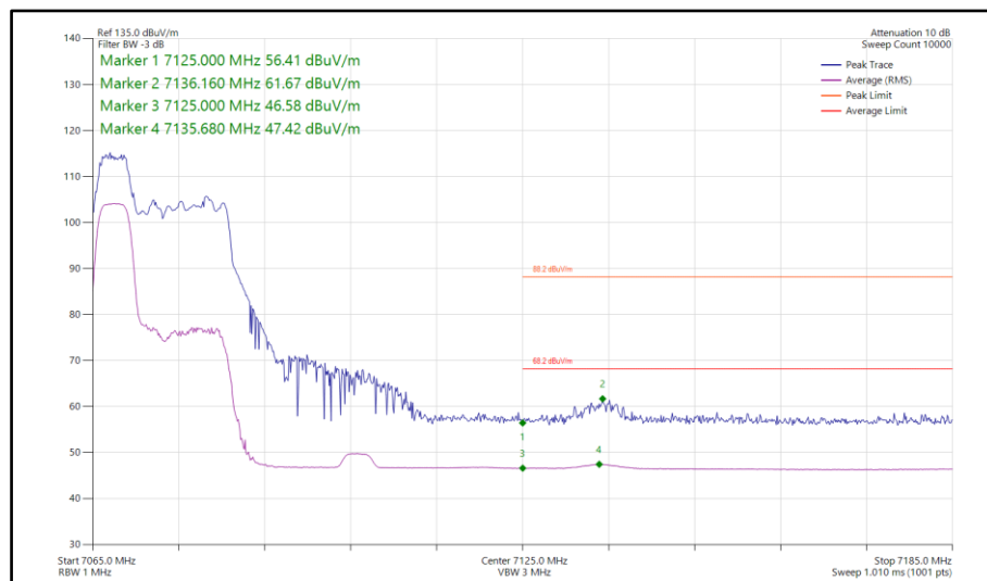
Figure 354 - 802.11ax HE40, RU52-37, SISO, Core 1 - 7085 MHz Band Edge Frequency 7125 MHz
