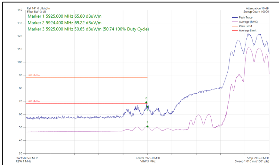
Figure 366 - 802.11be EHT40, RU106+26-85, SDM, Core 0-1 - 5965 MHz Band Edge Frequency 5925 MHz
