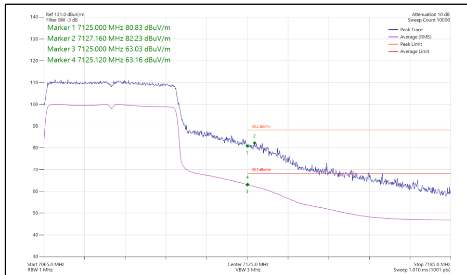
Figure 353 - 802.11ax HE40, SU, SISO, Core 1 - 7085 MHz Band Edge Frequency 7125 MHz
