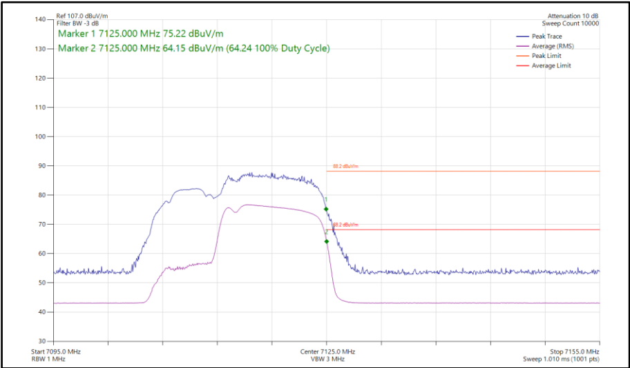
Figure 316 - 802.11be EHT20, RU106+26-83, SISO, Core 1 - 7115 MHz Band Edge Frequency 7125 MHz
