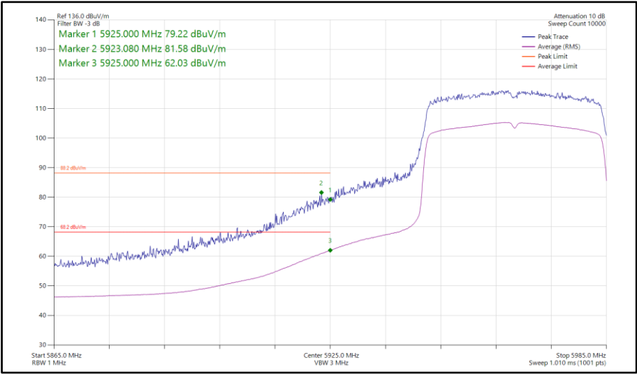
Figure 349 - 802.11ax HE40, SU, SISO, Core 1 - 5965 MHz Band Edge Frequency 5925 MHz
