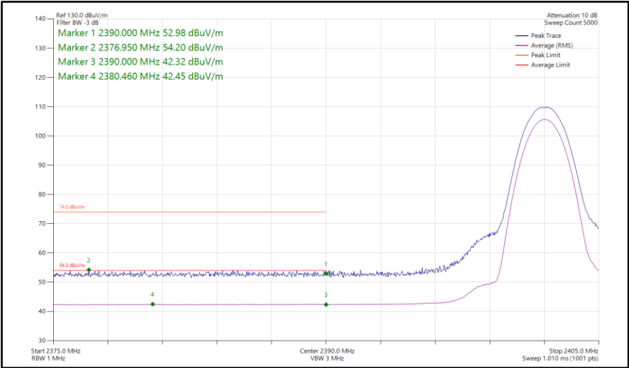
Figure 57 - Bluetooth 2DH5, SISO, Core 2 - 2402 MHz Band Edge Frequency 2390 MHz
