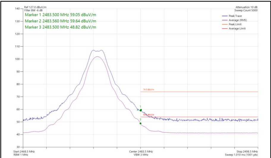
Figure 28 - Bluetooth CS1LE2M, SISO, Core 0 - 2478 MHz Band Edge Frequency 2483.5 MHz
