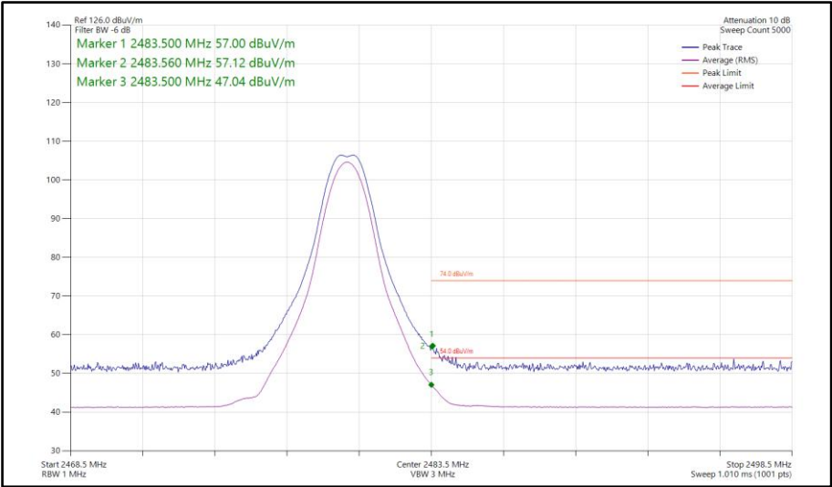
Figure 27 - Bluetooth CS1LE1M, SISO, Core 0 - 2480 MHz Band Edge Frequency 2483.5 MHz
