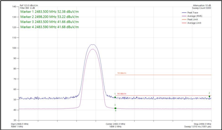
Figure 43 - Bluetooth 2DH5, SISO, Core 1 - 2480 MHz Band Edge Frequency 2483.5 MHz
