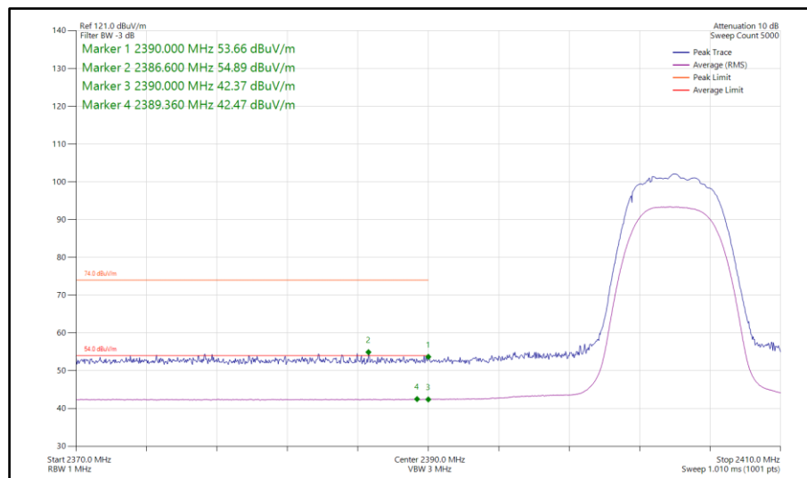
Figure 39 - Bluetooth HDRPM12, SISO, Core 1 - 2404 MHz Band Edge Frequency 2390 MHz
