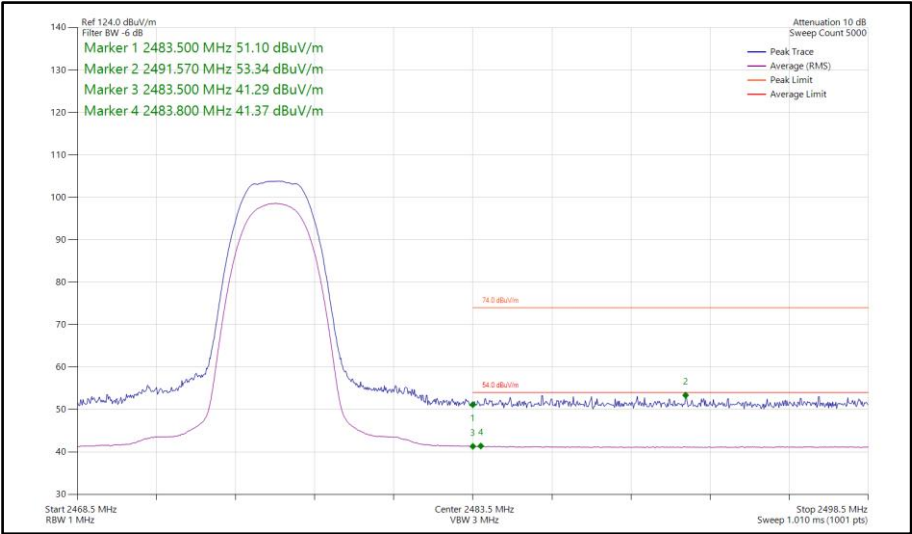
Figure 17 - Bluetooth HDR4, SISO, Core 0 - 2476 MHz Band Edge Frequency 2483.5 MHz
