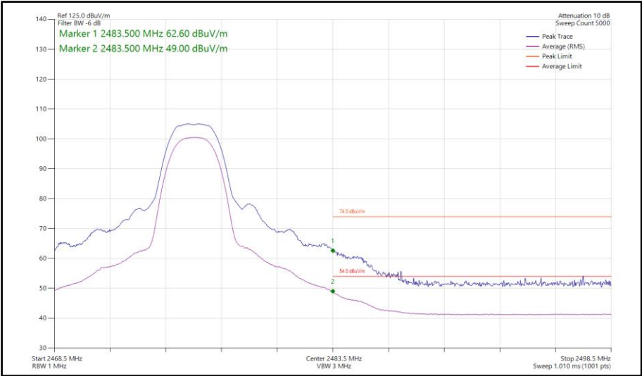
Figure 21 - Bluetooth HDT3, SISO, Core 0 - 2476 MHz Band Edge Frequency 2483.5 MHz
