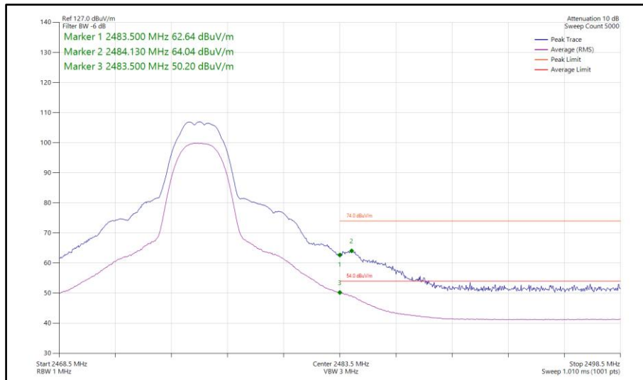
Figure 23 - Bluetooth HDT6, SISO, Core 0 - 2476 MHz Band Edge Frequency 2483.5 MHz
