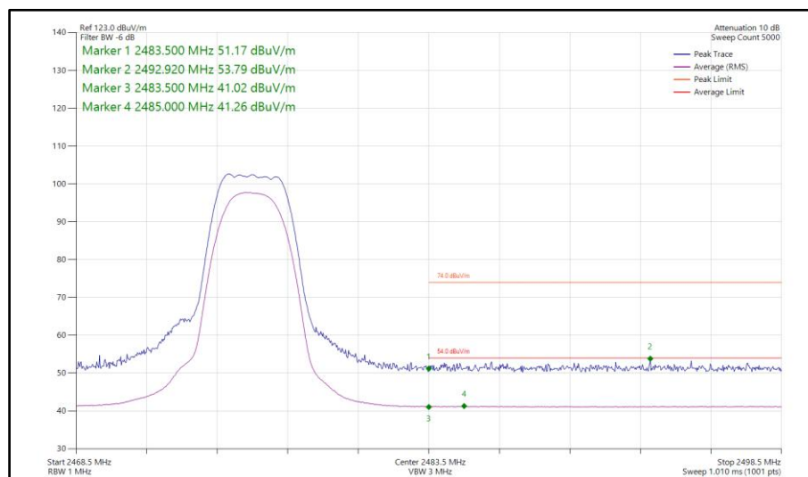
Figure 52 - Bluetooth HDRPS2, SISO, Core 1 - 2476 MHz Band Edge Frequency 2483.5 MHz
