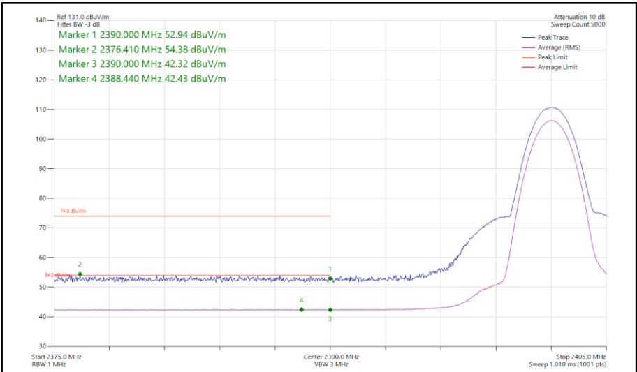
Figure 58 - Bluetooth 3DH5, SISO, Core 2 - 2402 MHz Band Edge Frequency 2390 MHz
