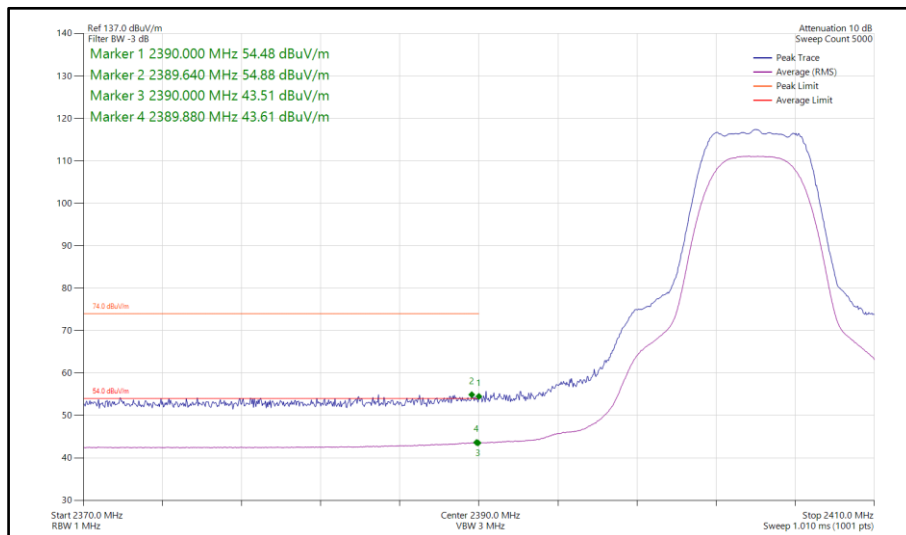
Figure 152 - Bluetooth XHDRPM8, SISO, Core 1 - 2404 MHz Band Edge Frequency 2390 MHz
