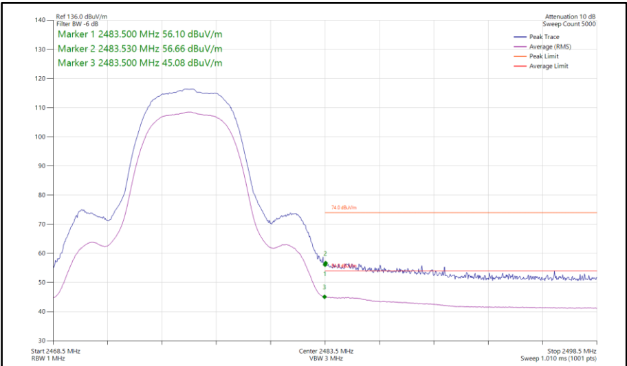
Figure 130 - Bluetooth HDR8, SISO, Core 0 - 2476 MHz Band Edge Frequency 2483.5 MHz
