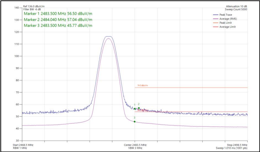
Figure 131 - Bluetooth LE1M, SISO, Core 0 - 2480 MHz Band Edge Frequency 2483.5 MHz
