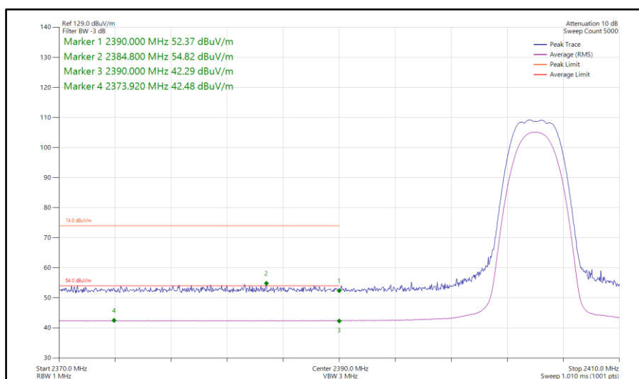
Figure 94 - Bluetooth HDRPS2, MIMO, Core 0-1 - 2404 MHz Band Edge Frequency 2390 MHz
