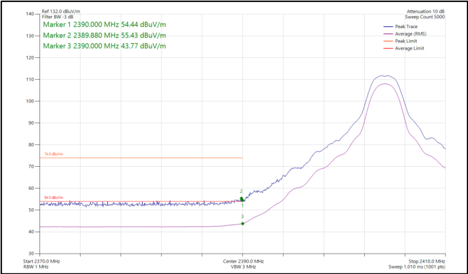
Figure 91 - Bluetooth HDT3, MIMO, Core 0-1 - 2404 MHz Band Edge Frequency 2390 MHz
