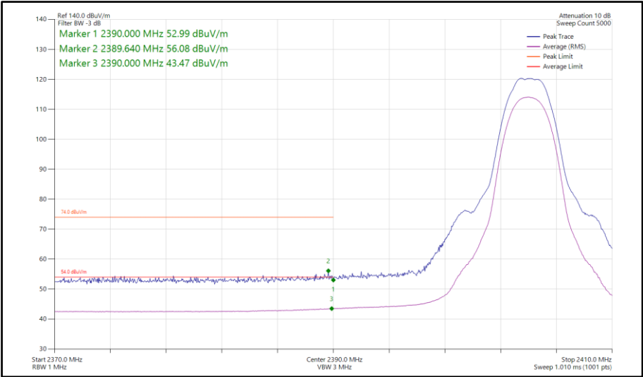
Figure 121 - Bluetooth HDT6, SISO, Core 0 - 2404 MHz Band Edge Frequency 2390 MHz
