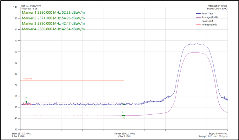
Figure 95 - Bluetooth HDRPM12, MIMO, Core 0-1 - 2404 MHz Band Edge Frequency 2390 MHz
