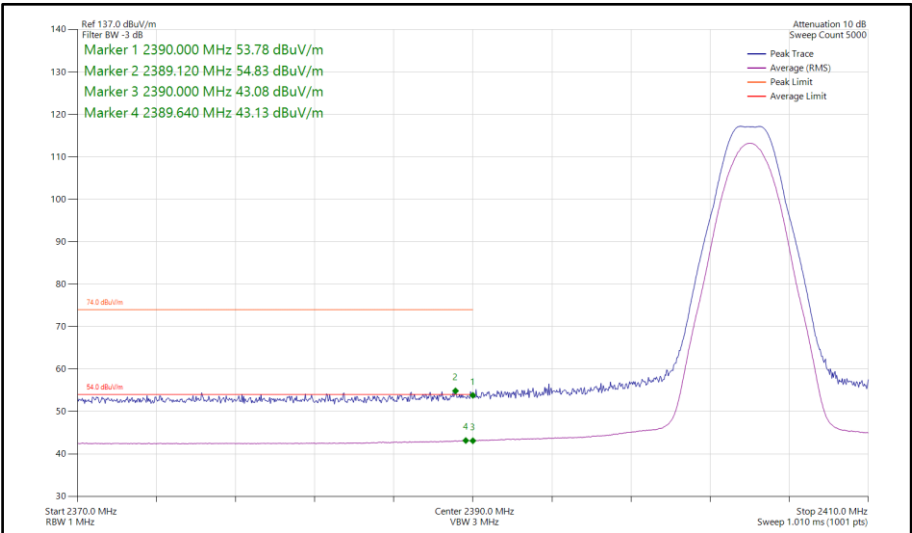
Figure 146 - Bluetooth LE2M, SISO, Core 1 - 2404 MHz Band Edge Frequency 2390 MHz
