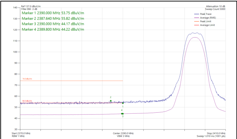
Figure 122 - Bluetooth HDRPS2, SISO, Core 0 - 2404 MHz Band Edge Frequency 2390 MHz
