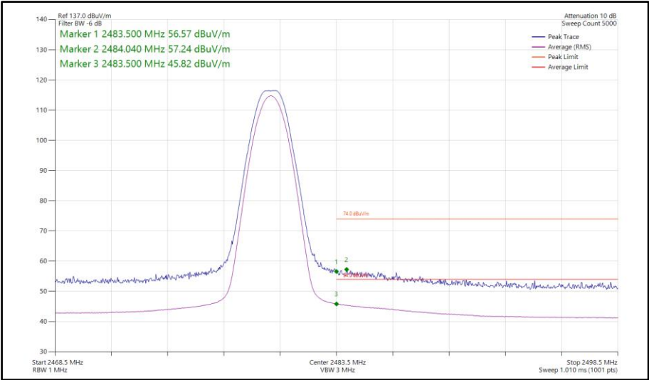
Figure 159 - Bluetooth LE1M, SISO, Core 1 - 2480 MHz Band Edge Frequency 2483.5 MHz
