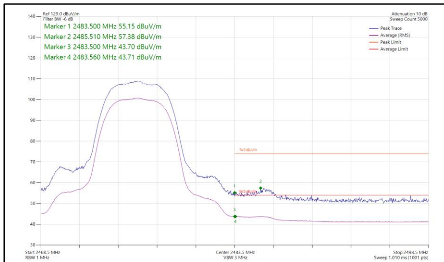
Figure 102 - Bluetooth HDR8, MIMO, Core 0-1 - 2476 MHz Band Edge Frequency 2483.5 MHz
