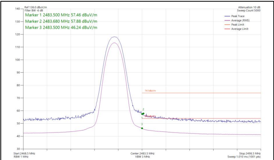
Figure 128 - Bluetooth 3DH5, SISO, Core 0 - 2480 MHz Band Edge Frequency 2483.5 MHz
