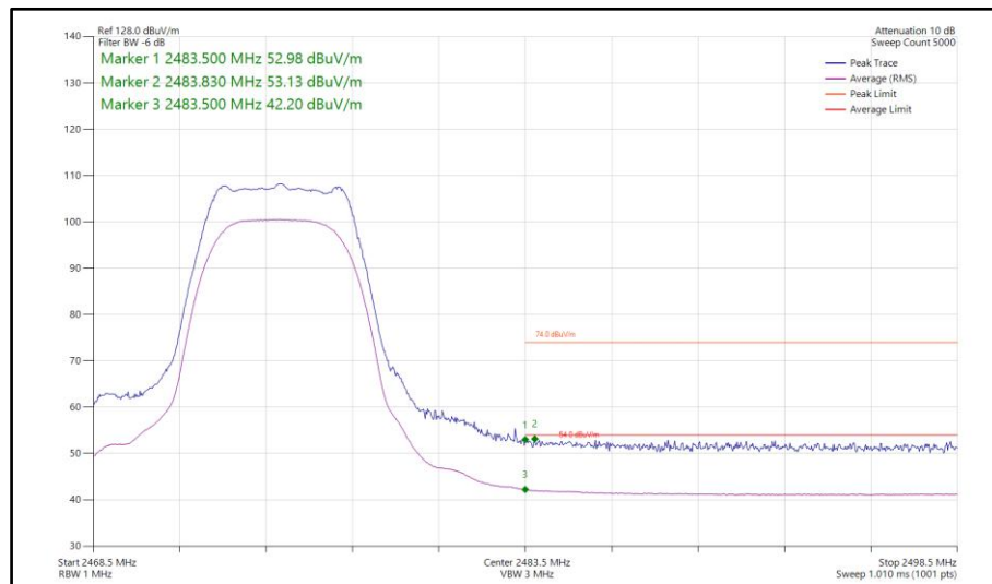
Figure 110 - Bluetooth XHDRPM8, MIMO, Core 0-1 - 2475 MHz Band Edge Frequency 2483.5 MHz
