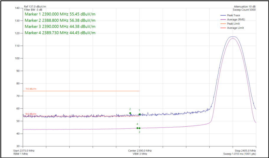
Figure 117 - Bluetooth LE1M, SISO, Core 0 - 2402 MHz Band Edge Frequency 2390 MHz
