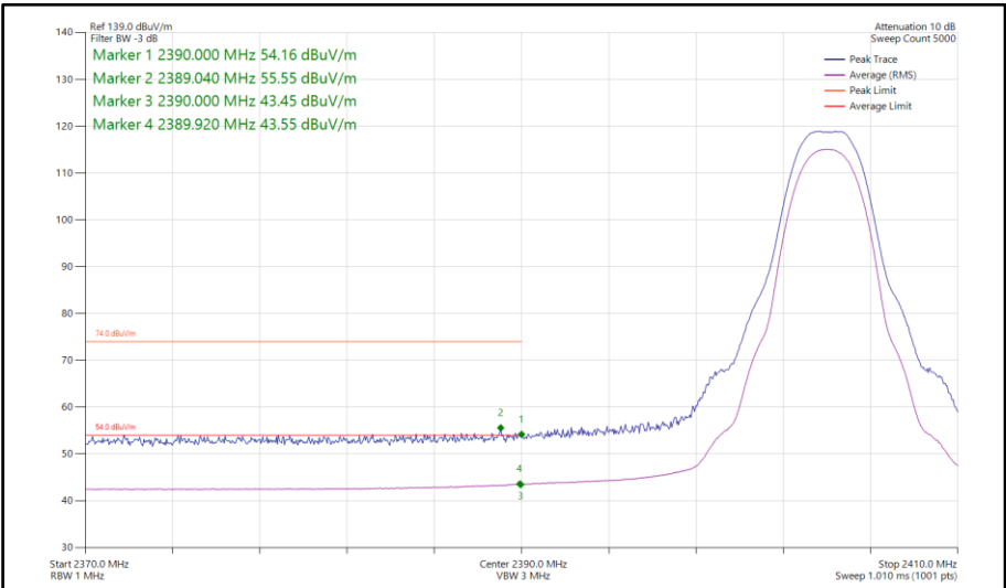
Figure 148 - Bluetooth HDT4, SISO, Core 1 - 2404 MHz Band Edge Frequency 2390 MHz
