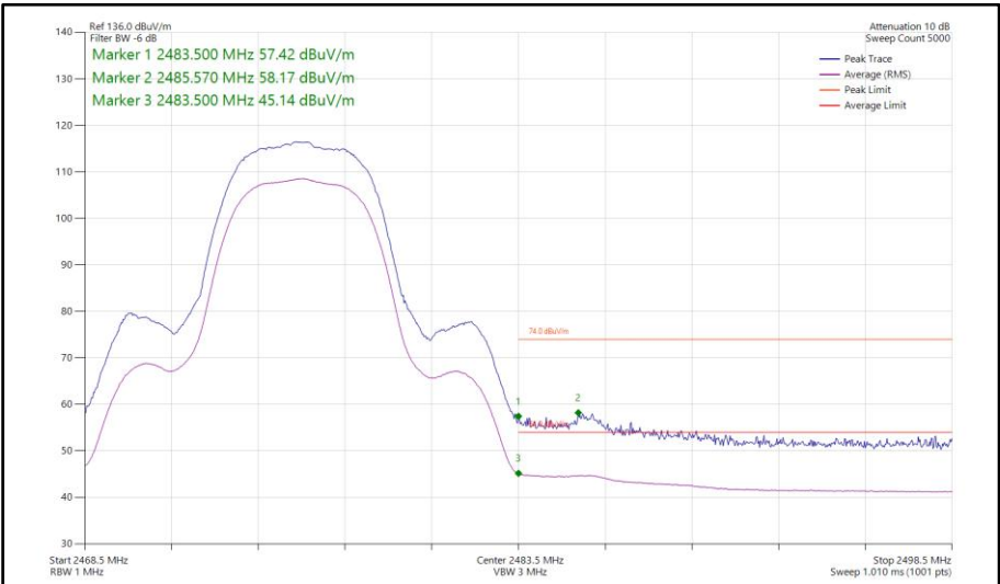
Figure 158 - Bluetooth HDR8, SISO, Core 1 - 2476 MHz Band Edge Frequency 2483.5 MHz
