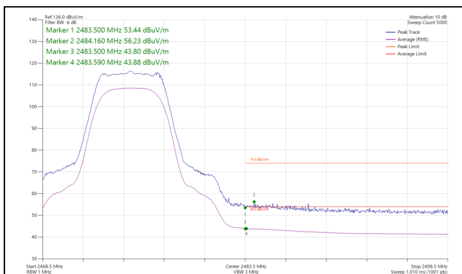
Figure 138 - Bluetooth XHDRPM8, SISO, Core 0 - 2475 MHz Band Edge Frequency 2483.5 MHz
