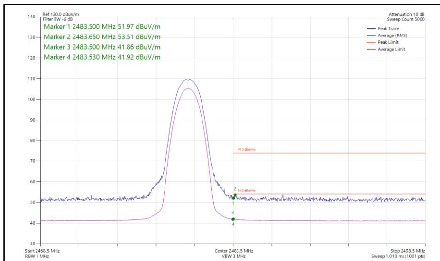
Figure 99 - Bluetooth 2DH5, MIMO, Core 0-1 - 2480 MHz Band Edge Frequency 2483.5 MHz
