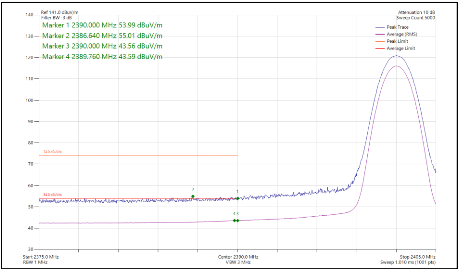
Figure 142 - Bluetooth 3DH5, SISO, Core 1 - 2402 MHz Band Edge Frequency 2390 MHz
