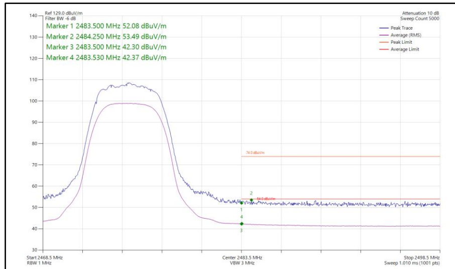
Figure 81 - Bluetooth HDRPM12, SISO, Core 2 - 2475 MHz Band Edge Frequency 2483.5 MHz
