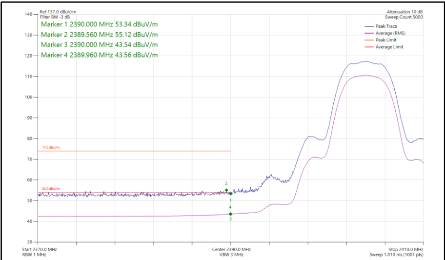
Figure 144 - Bluetooth HDR8, SISO, Core 1 - 2404 MHz Band Edge Frequency 2390 MHz
