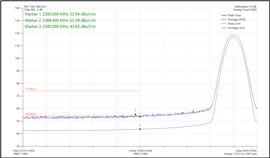
Figure 145 - Bluetooth LE1M, SISO, Core 1 - 2402 MHz Band Edge Frequency 2390 MHz
