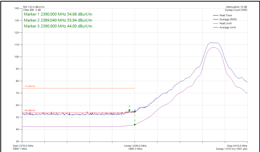
Figure 92 - Bluetooth HDT4, MIMO, Core 0-1 - 2404 MHz Band Edge Frequency 2390 MHz
