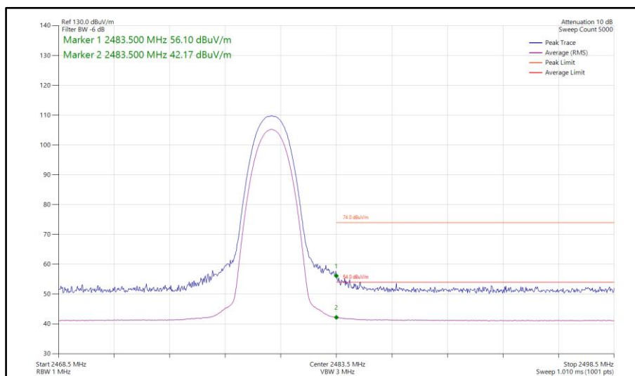
Figure 100 - Bluetooth 3DH5, MIMO, Core 0-1 - 2480 MHz Band Edge Frequency 2483.5 MHz
