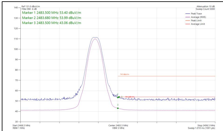
Figure 103 - Bluetooth LE1M, MIMO, Core 0-1 - 2480 MHz Band Edge Frequency 2483.5 MHz
