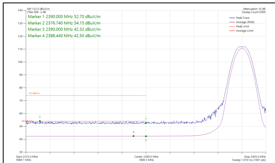
Figure 89 - Bluetooth LE1M, MIMO, Core 0-1 - 2402 MHz Band Edge Frequency 2390 MHz
