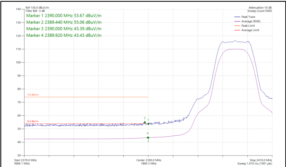
Figure 124 - Bluetooth XHDRPM8, SISO, Core 0 - 2404 MHz Band Edge Frequency 2390 MHz
