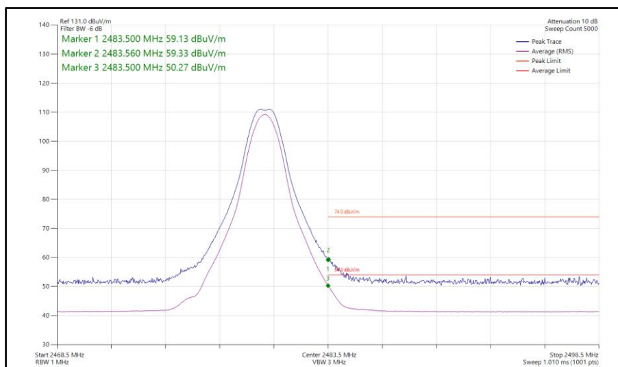
Figure 111 - Bluetooth CS1LE1M, MIMO, Core 0-1 - 2480 MHz Band Edge Frequency 2483.5 MHz
