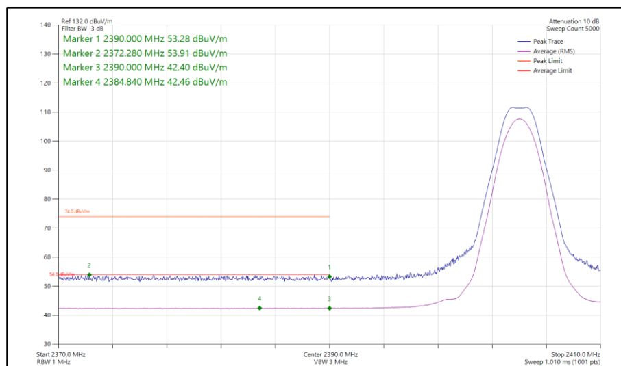
Figure 90 - Bluetooth LE2M, MIMO, Core 0-1 - 2404 MHz Band Edge Frequency 2390 MHz
