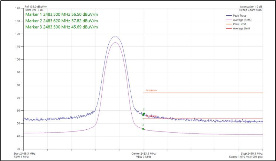
Figure 127 - Bluetooth 2DH5, SISO, Core 0 - 2480 MHz Band Edge Frequency 2483.5 MHz
