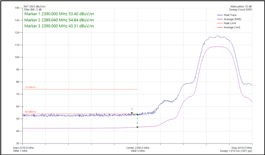
Figure 123 - Bluetooth HDRPM12, SISO, Core 0 - 2404 MHz Band Edge Frequency 2390 MHz
