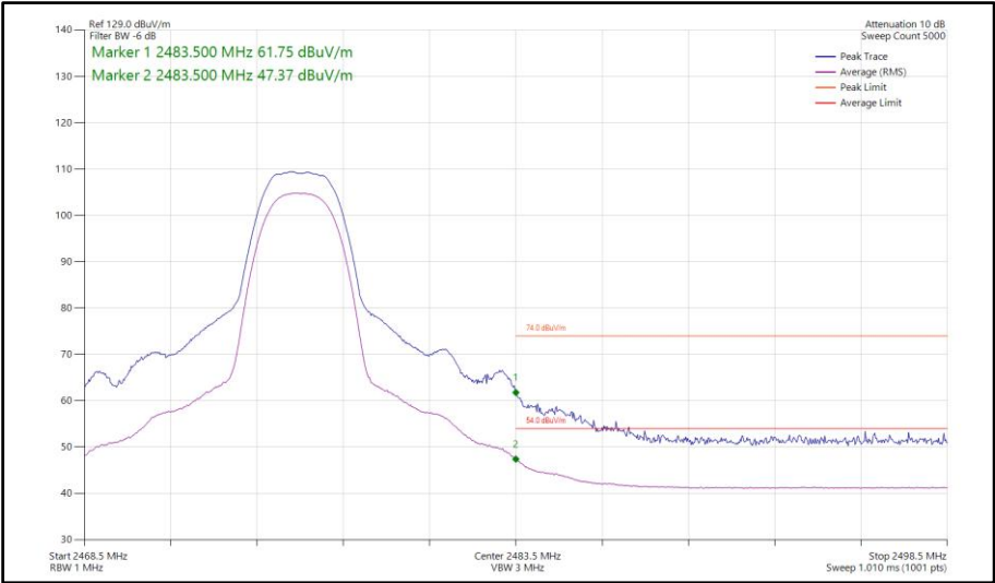
Figure 105 - Bluetooth HDT3, MIMO, Core 0-1 - 2476 MHz Band Edge Frequency 2483.5 MHz
