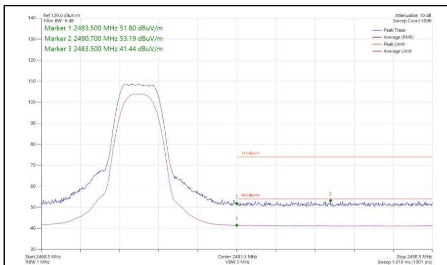
Figure 108 - Bluetooth HDRPS2, MIMO, Core 0-1 - 2476 MHz Band Edge Frequency 2483.5 MHz
