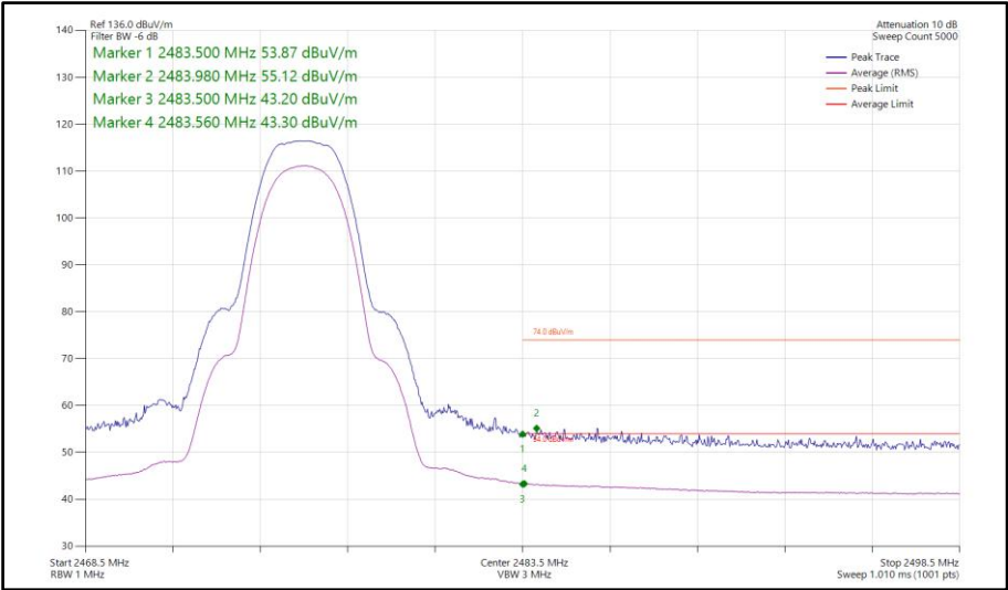
Figure 157 - Bluetooth HDR4, SISO, Core 1 - 2476 MHz Band Edge Frequency 2483.5 MHz
