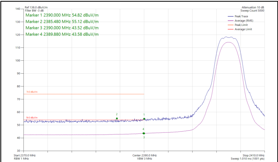
Figure 150 - Bluetooth HDRPS2, SISO, Core 1 - 2404 MHz Band Edge Frequency 2390 MHz
