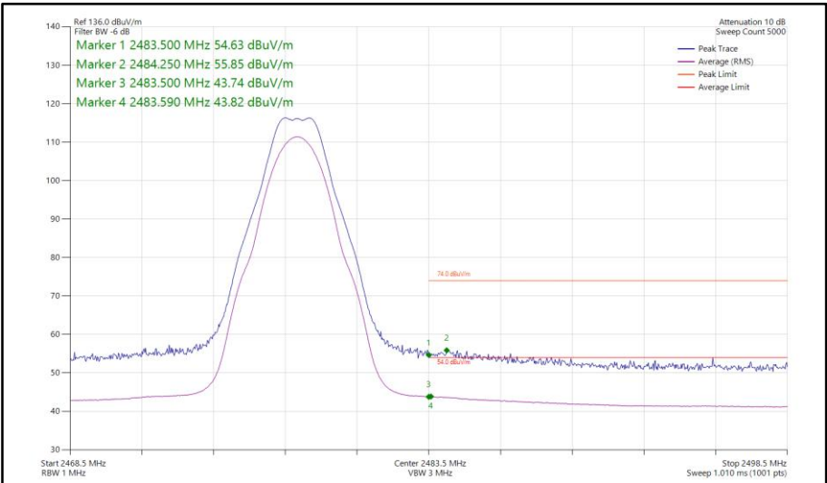
Figure 160 - Bluetooth LE2M, SISO, Core 1 - 2478 MHz Band Edge Frequency 2483.5 MHz
