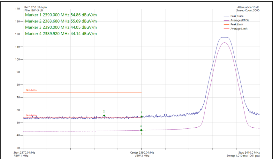
Figure 118 - Bluetooth LE2M, SISO, Core 0 - 2404 MHz Band Edge Frequency 2390 MHz
