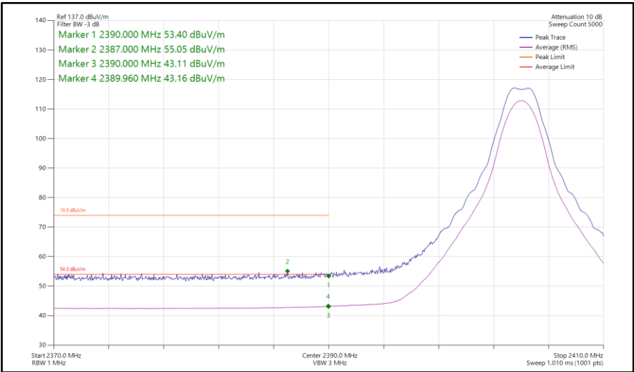
Figure 154 - Bluetooth CS1LE2M, SISO, Core 1 - 2404 MHz Band Edge Frequency 2390 MHz
