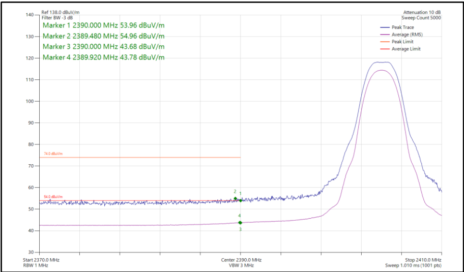
Figure 120 - Bluetooth HDT4, SISO, Core 0 - 2404 MHz Band Edge Frequency 2390 MHz
