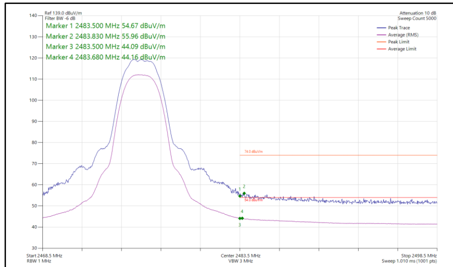
Figure 135 - Bluetooth HDT6, SISO, Core 0 - 2476 MHz Band Edge Frequency 2483.5 MHz
