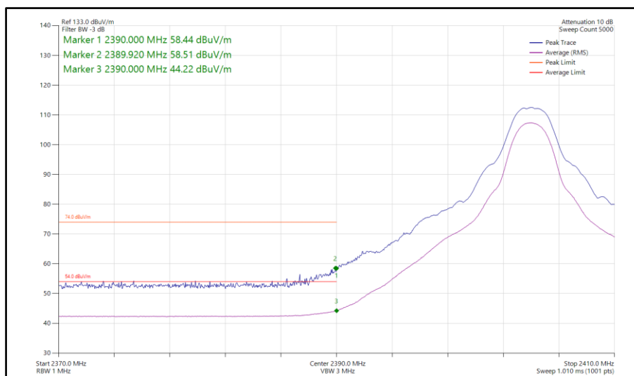
Figure 93 - Bluetooth HDT6, MIMO, Core 0-1 - 2404 MHz Band Edge Frequency 2390 MHz
