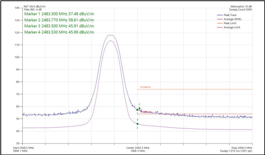
Figure 155 - Bluetooth 2DH5, SISO, Core 1 - 2480 MHz Band Edge Frequency 2483.5 MHz
