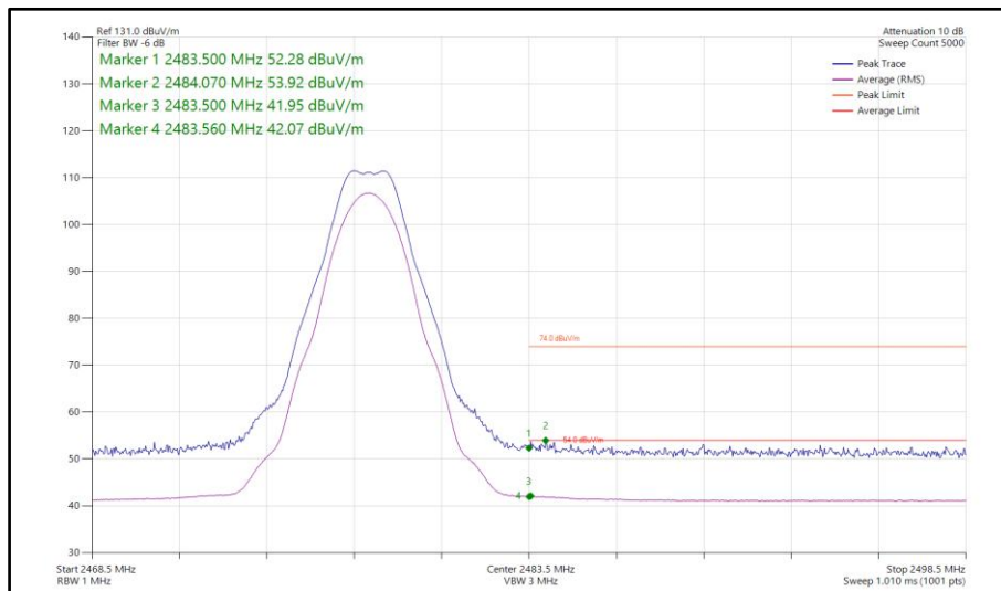
Figure 104 - Bluetooth LE2M, MIMO, Core 0-1 - 2478 MHz Band Edge Frequency 2483.5 MHz
