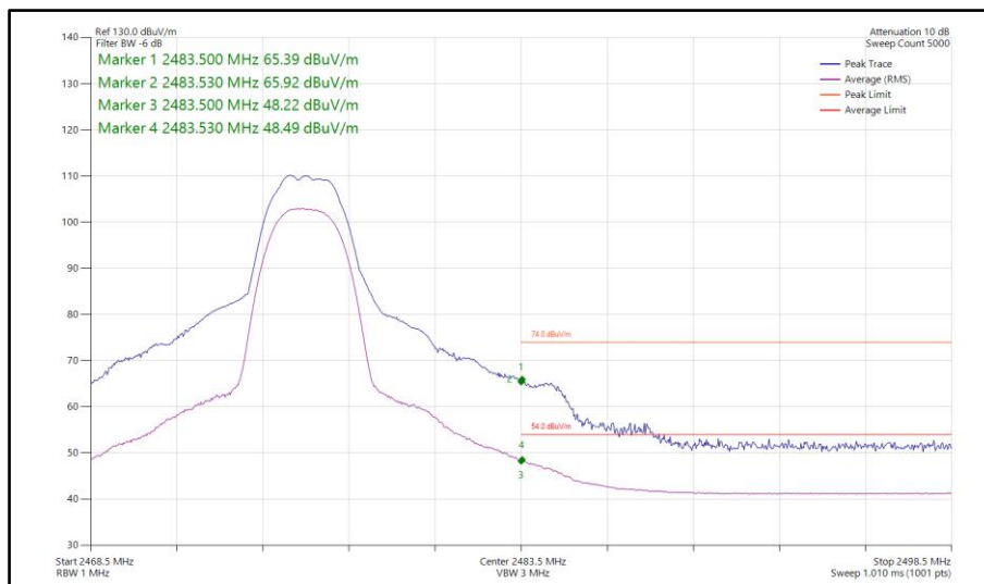
Figure 107 - Bluetooth HDT6, MIMO, Core 0-1 - 2476 MHz Band Edge Frequency 2483.5 MHz
