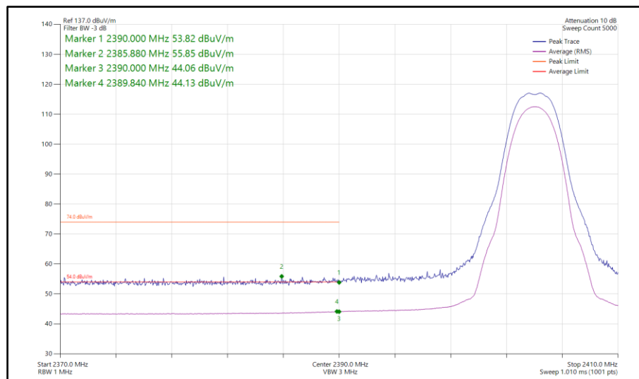
Figure 115 - Bluetooth HDR4, SISO, Core 0 - 2404 MHz Band Edge Frequency 2390 MHz
