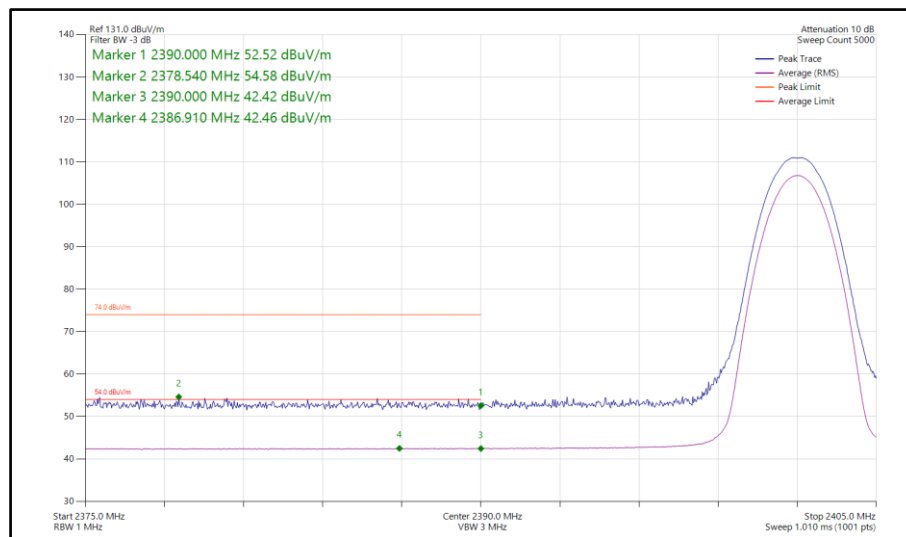
Figure 85 - Bluetooth 2DH5, MIMO, Core 0-1 - 2402 MHz Band Edge Frequency 2390 MHz
