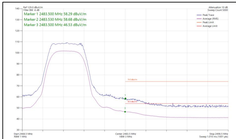
Figure 82 - Bluetooth XHDRPM8, SISO, Core 2 - 2475 MHz Band Edge Frequency 2483.5 MHz
