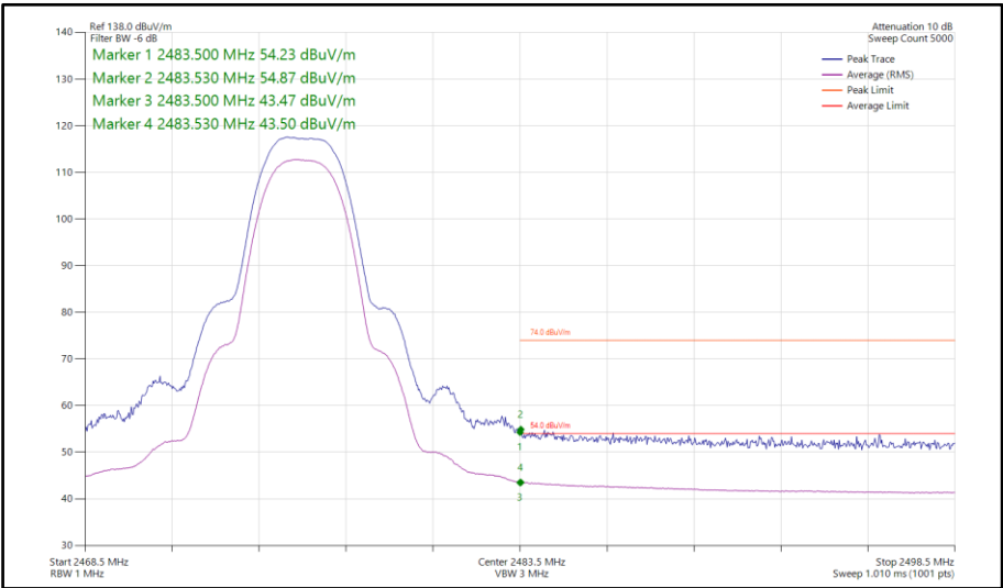
Figure 162 - Bluetooth HDT4, SISO, Core 1 - 2476 MHz Band Edge Frequency 2483.5 MHz
