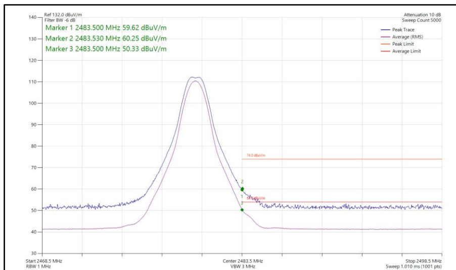
Figure 83 - Bluetooth CS1LE1M, SISO, Core 2 - 2480 MHz Band Edge Frequency 2483.5 MHz
