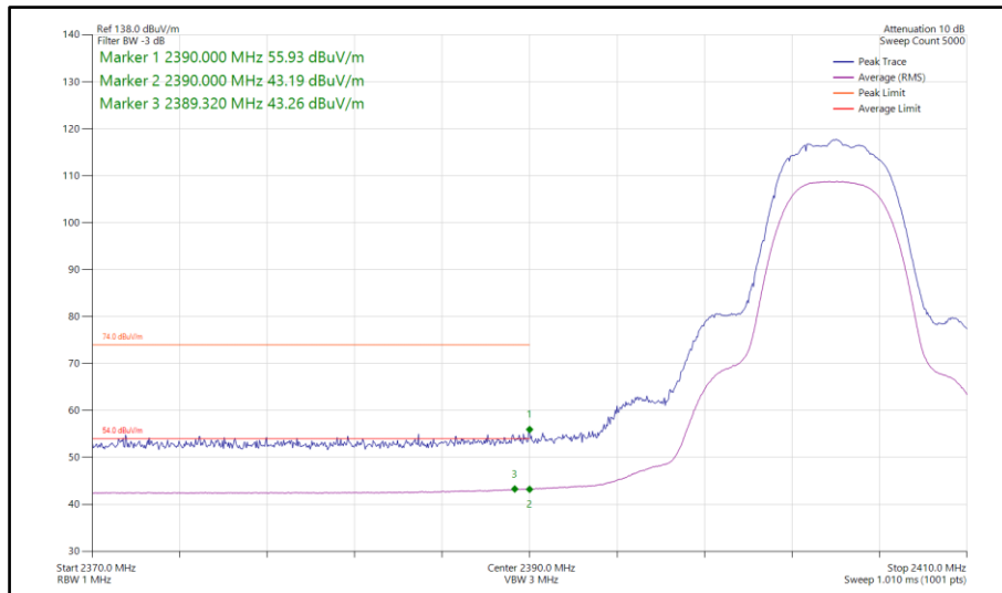
Figure 151 - Bluetooth HDRPM12, SISO, Core 1 - 2404 MHz Band Edge Frequency 2390 MHz
