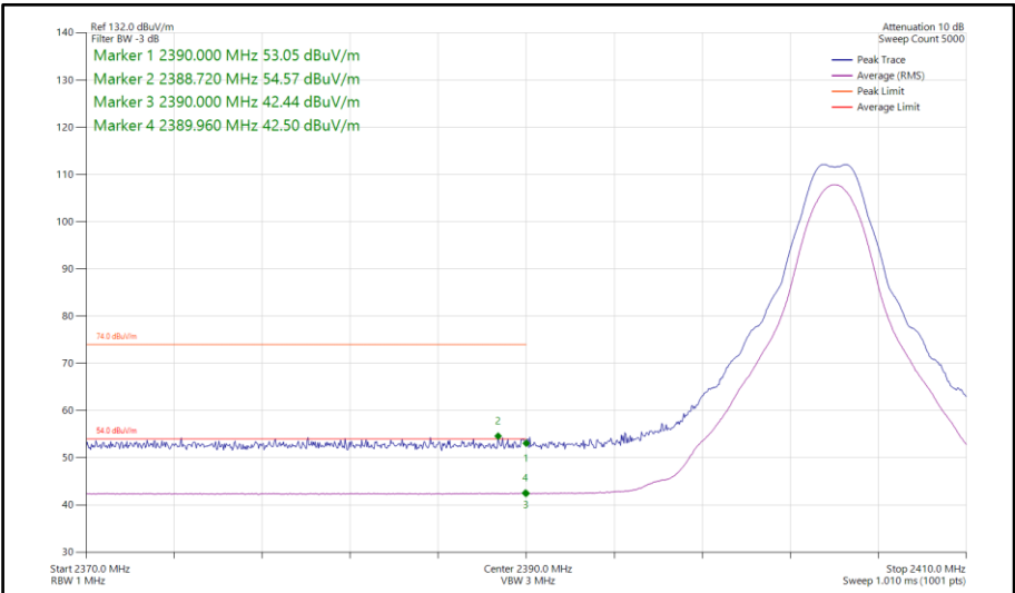
Figure 98 - Bluetooth CS1LE2M, MIMO, Core 0-1 - 2404 MHz Band Edge Frequency 2390 MHz
