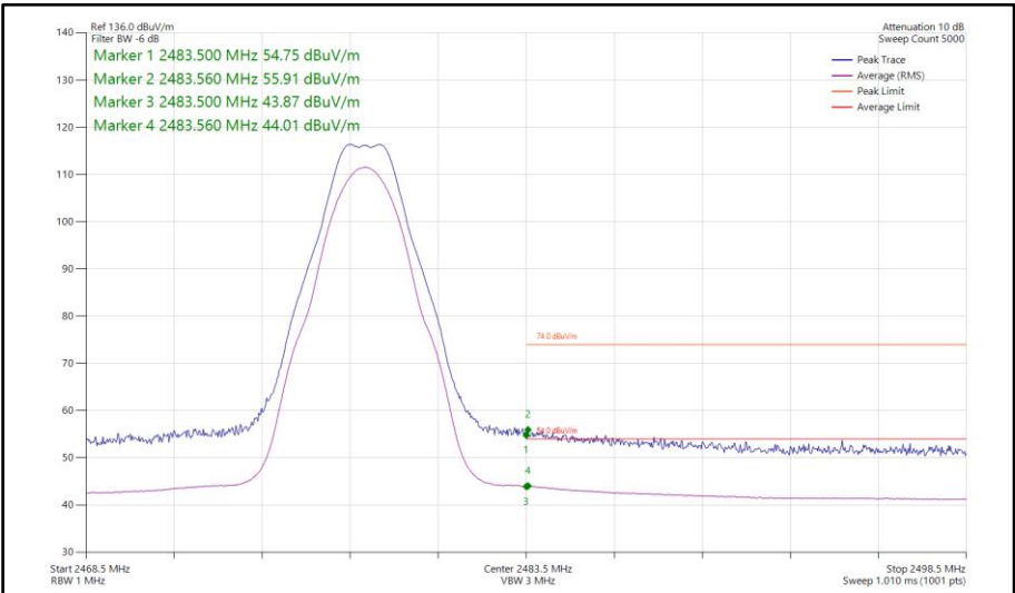
Figure 132 - Bluetooth LE2M, SISO, Core 0 - 2478 MHz Band Edge Frequency 2483.5 MHz
