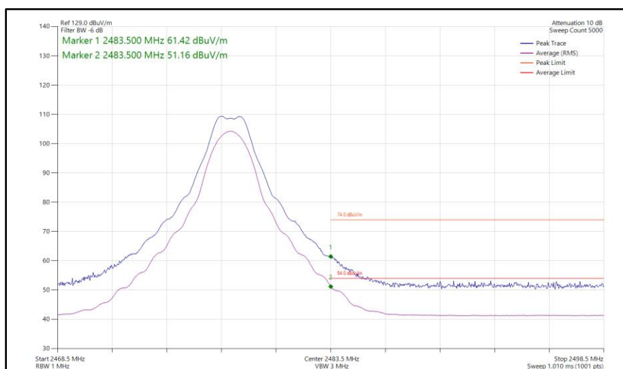
Figure 112 - Bluetooth CS1LE2M, MIMO, Core 0-1 - 2478 MHz Band Edge Frequency 2483.5 MHz
