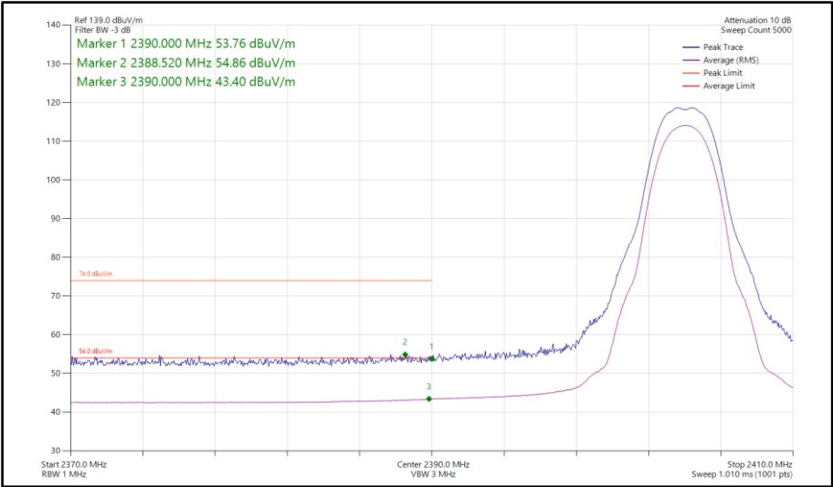
Figure 143 - Bluetooth HDR4, SISO, Core 1 - 2404 MHz Band Edge Frequency 2390 MHz
