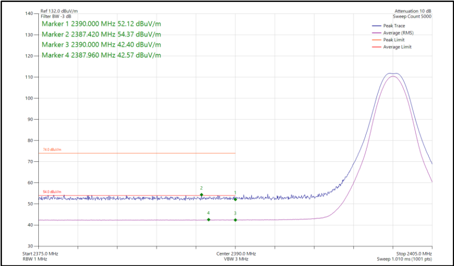
Figure 97 - Bluetooth CS1LE1M, MIMO, Core 0-1 - 2402 MHz Band Edge Frequency 2390 MHz
