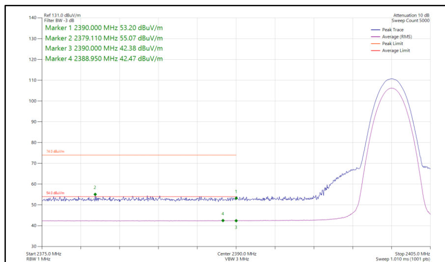
Figure 86 - Bluetooth 3DH5, MIMO, Core 0-1 - 2402 MHz Band Edge Frequency 2390 MHz
