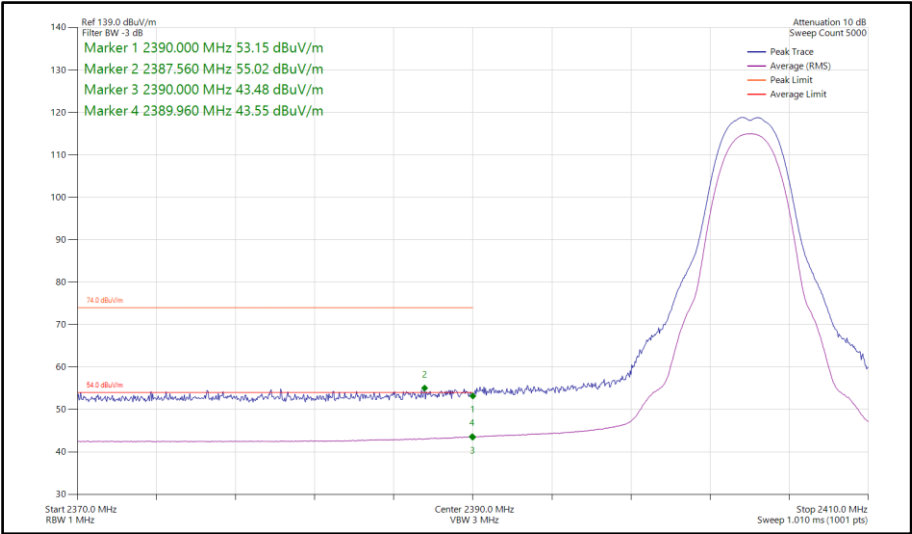
Figure 147 - Bluetooth HDT3, SISO, Core 1 - 2404 MHz Band Edge Frequency 2390 MHz
