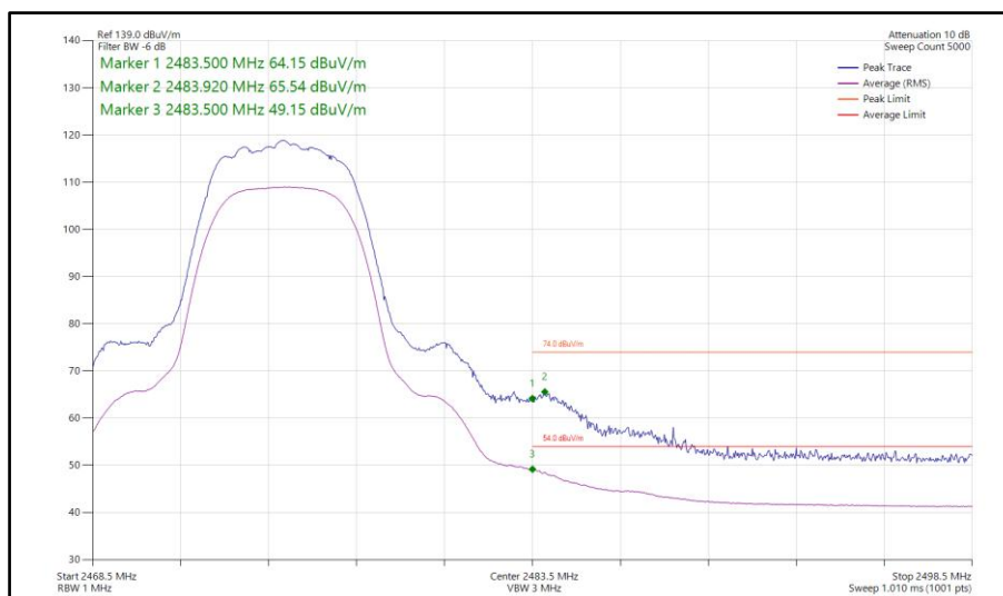
Figure 137 - Bluetooth HDRPM12, SISO, Core 0 - 2475 MHz Band Edge Frequency 2483.5 MHz
