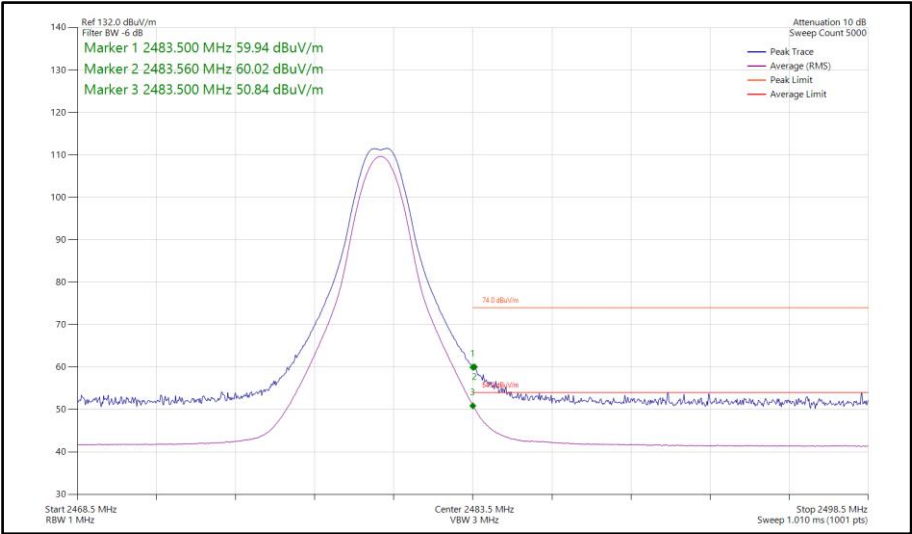
Figure 139 - Bluetooth CS1LE1M, SISO, Core 0 - 2480 MHz Band Edge Frequency 2483.5 MHz
