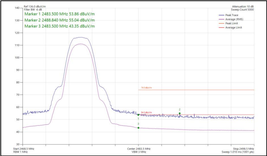
Figure 129 - Bluetooth HDR4, SISO, Core 0 - 2476 MHz Band Edge Frequency 2483.5 MHz
