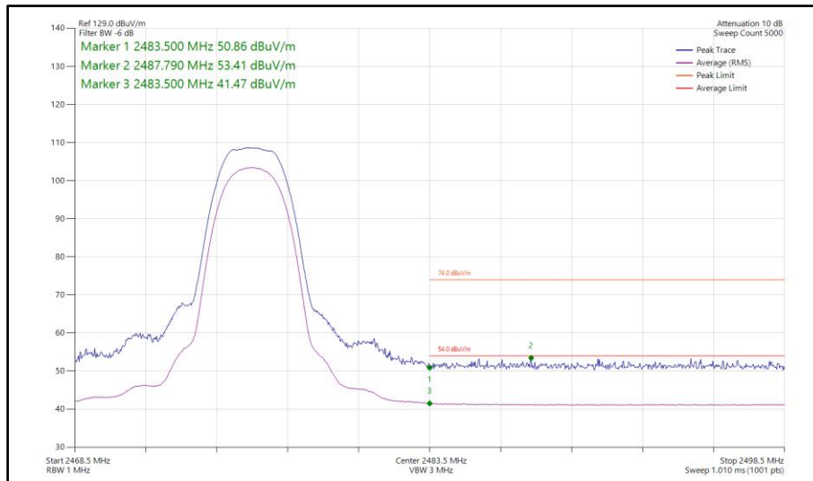
Figure 101 - Bluetooth HDR4, MIMO, Core 0-1 - 2476 MHz Band Edge Frequency 2483.5 MHz
