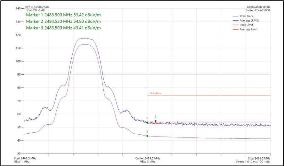
Figure 161 - Bluetooth HDT3, SISO, Core 1 - 2476 MHz Band Edge Frequency 2483.5 MHz
