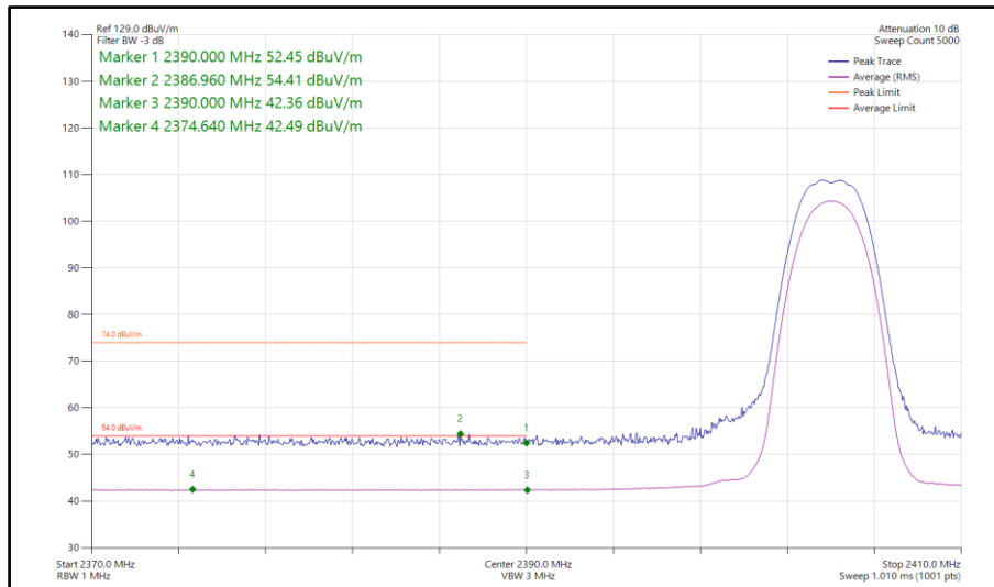
Figure 87 - Bluetooth HDR4, MIMO, Core 0-1 - 2404 MHz Band Edge Frequency 2390 MHz
