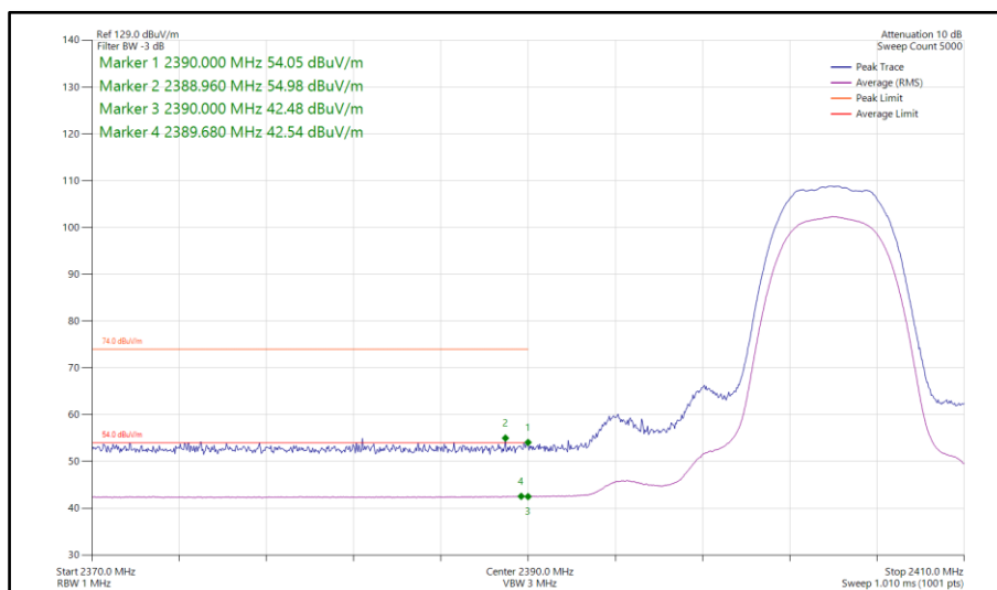
Figure 88 - Bluetooth HDR8, MIMO, Core 0-1 - 2404 MHz Band Edge Frequency 2390 MHz
