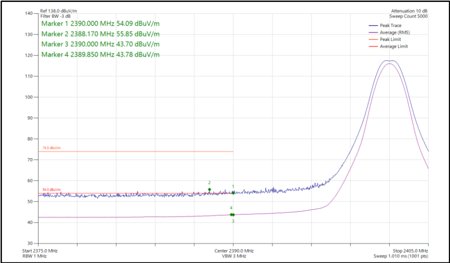
Figure 125 - Bluetooth CS1LE1M, SISO, Core 0 - 2402 MHz Band Edge Frequency 2390 MHz
