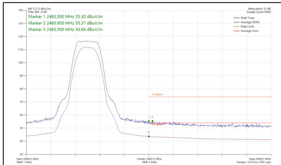
Figure 136 - Bluetooth HDRPS2, SISO, Core 0 - 2476 MHz Band Edge Frequency 2483.5 MHz
