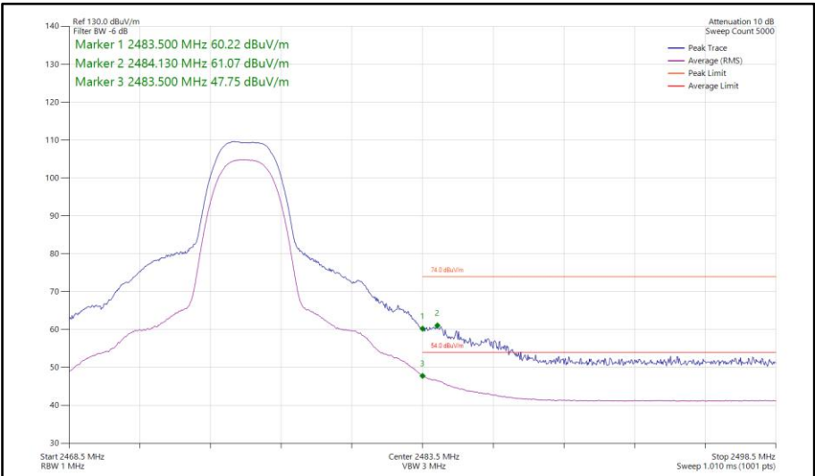
Figure 106 - Bluetooth HDT4, MIMO, Core 0-1 - 2476 MHz Band Edge Frequency 2483.5 MHz
