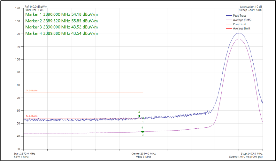
Figure 141 - Bluetooth 2DH5, SISO, Core 1 - 2402 MHz Band Edge Frequency 2390 MHz
