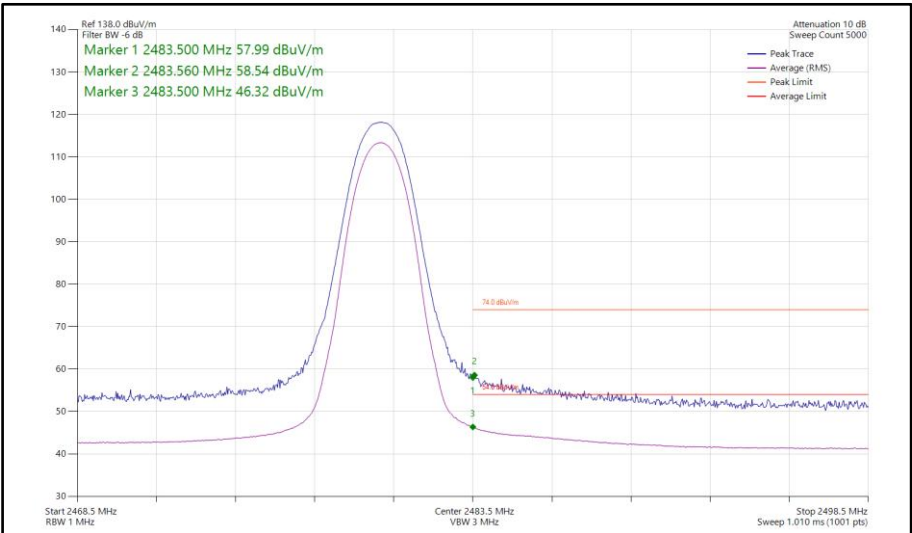
Figure 156 - Bluetooth 3DH5, SISO, Core 1 - 2480 MHz Band Edge Frequency 2483.5 MHz
