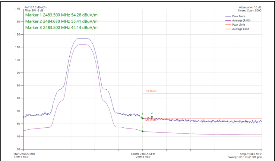
Figure 134 - Bluetooth HDT4, SISO, Core 0 - 2476 MHz Band Edge Frequency 2483.5 MHz
