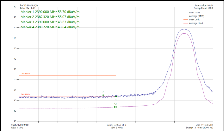
Figure 119 - Bluetooth HDT3, SISO, Core 0 - 2404 MHz Band Edge Frequency 2390 MHz
