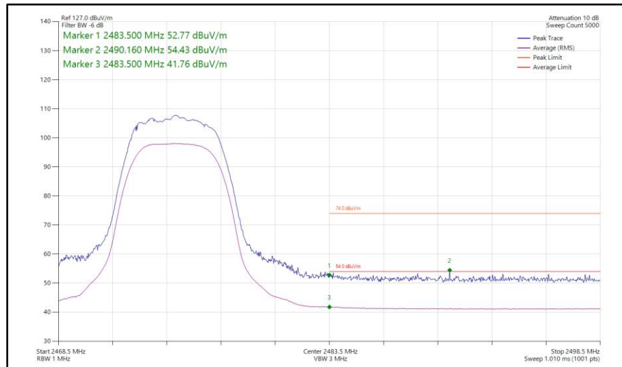
Figure 109 - Bluetooth HDRPM12, MIMO, Core 0-1 - 2475 MHz Band Edge Frequency 2483.5 MHz
