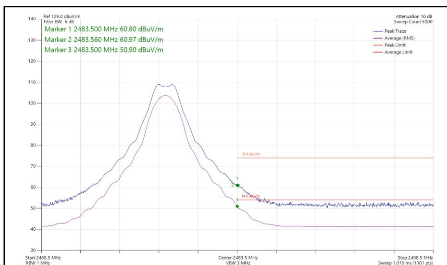
Figure 84 - Bluetooth CS1LE2M, SISO, Core 2 - 2478 MHz Band Edge Frequency 2483.5 MHz
