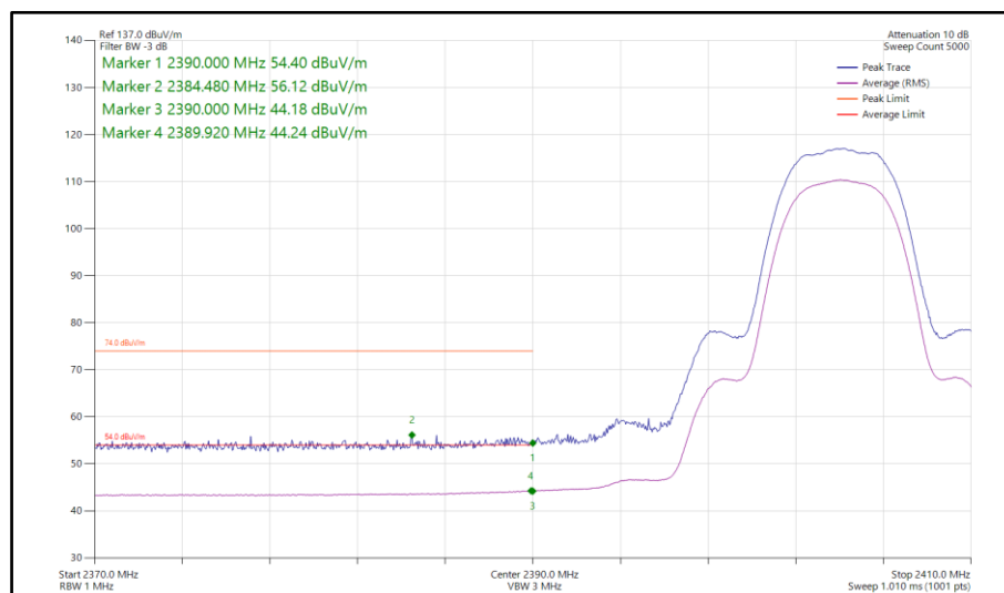
Figure 116 - Bluetooth HDR8, SISO, Core 0 - 2404 MHz Band Edge Frequency 2390 MHz
