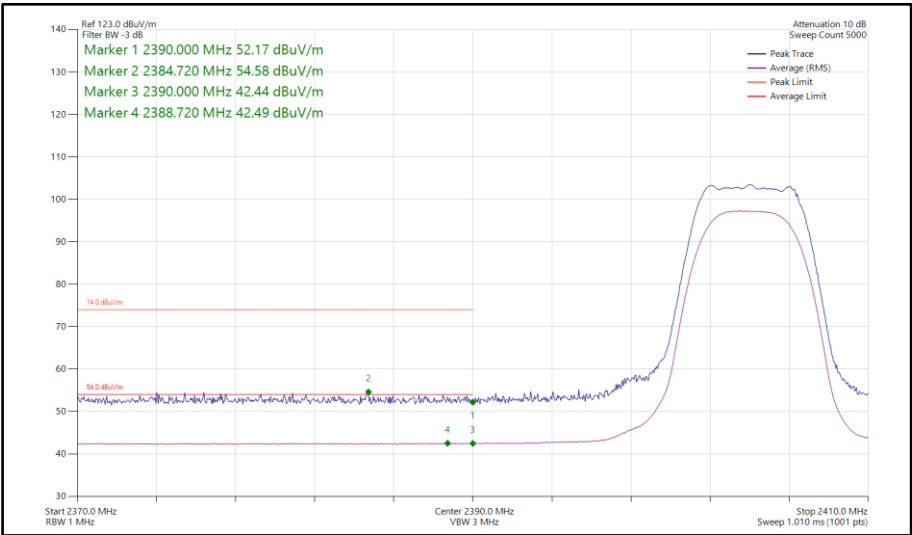
Figure 96 - Bluetooth XHDRPM8, MIMO, Core 0-1 - 2404 MHz Band Edge Frequency 2390 MHz
