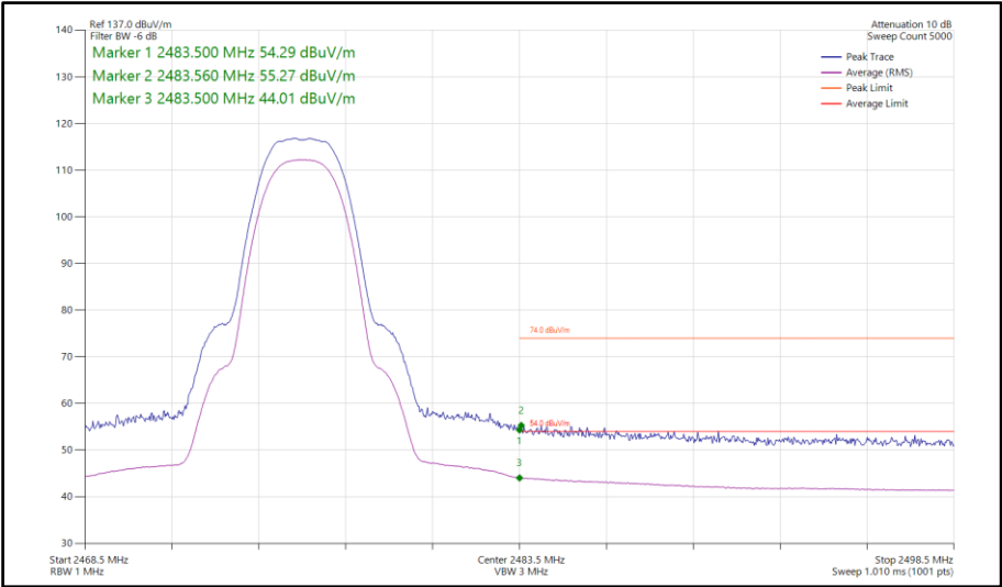
Figure 133 - Bluetooth HDT3, SISO, Core 0 - 2476 MHz Band Edge Frequency 2483.5 MHz
