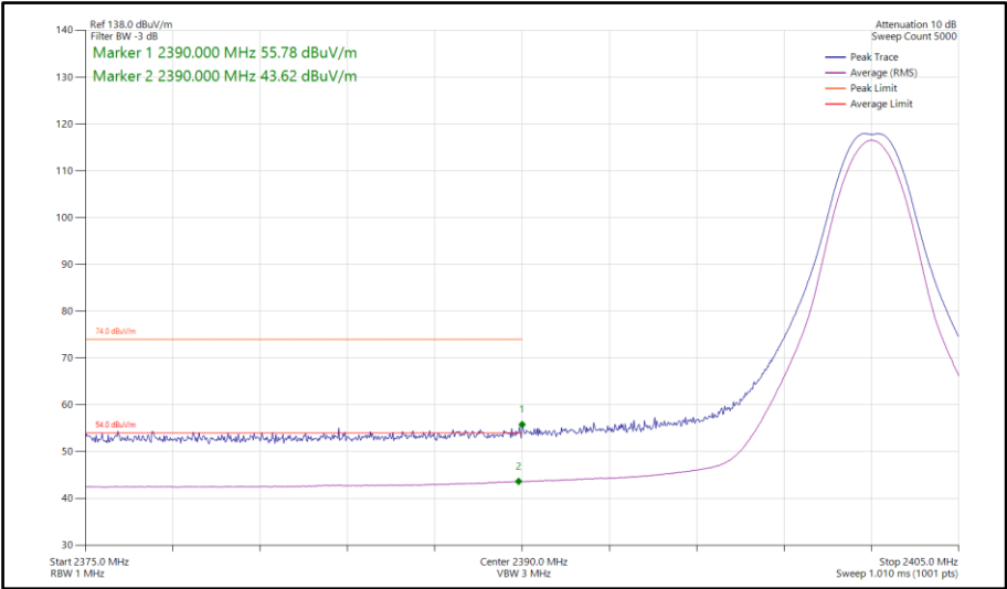
Figure 153 - Bluetooth CS1LE1M, SISO, Core 1 - 2402 MHz Band Edge Frequency 2390 MHz
