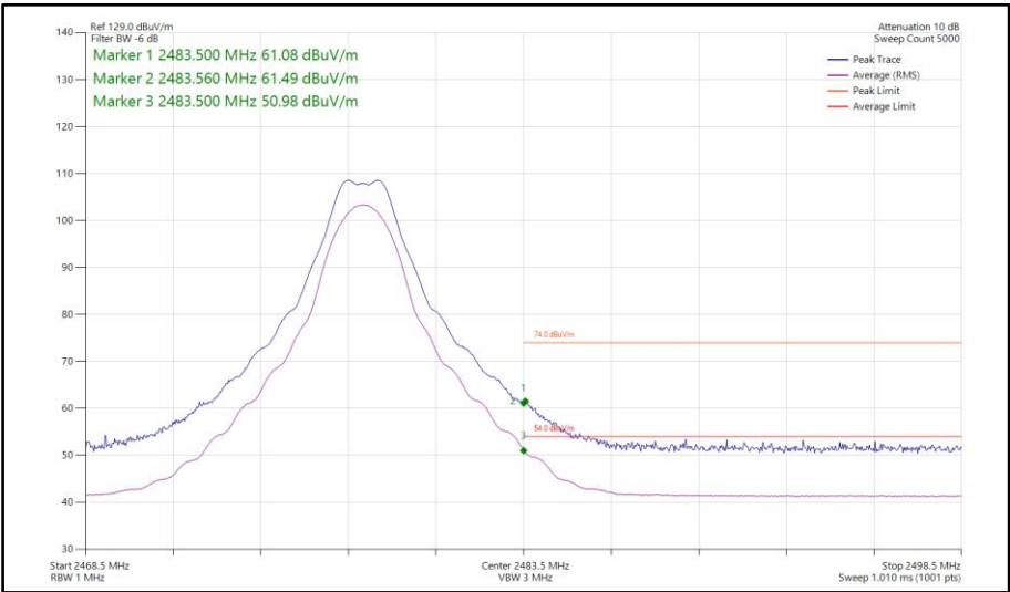
Figure 140 - Bluetooth CS1LE2M, SISO, Core 0 - 2478 MHz Band Edge Frequency 2483.5 MHz
