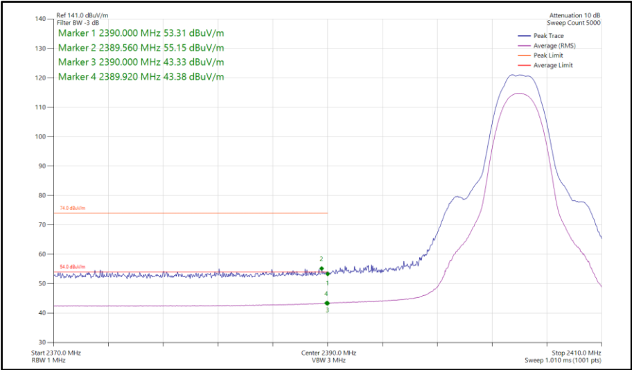
Figure 149 - Bluetooth HDT6, SISO, Core 1 - 2404 MHz Band Edge Frequency 2390 MHz
