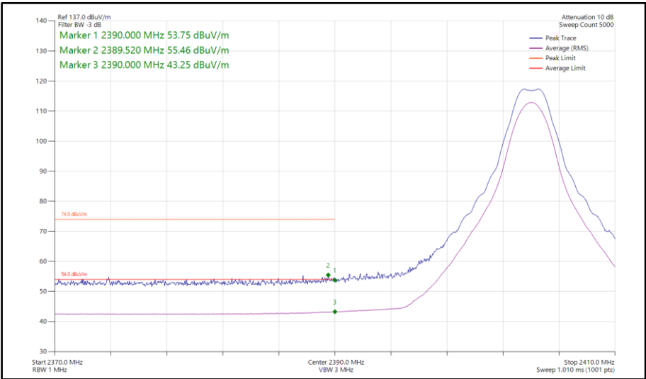
Figure 126 - Bluetooth CS1LE2M, SISO, Core 0 - 2404 MHz Band Edge Frequency 2390 MHz
