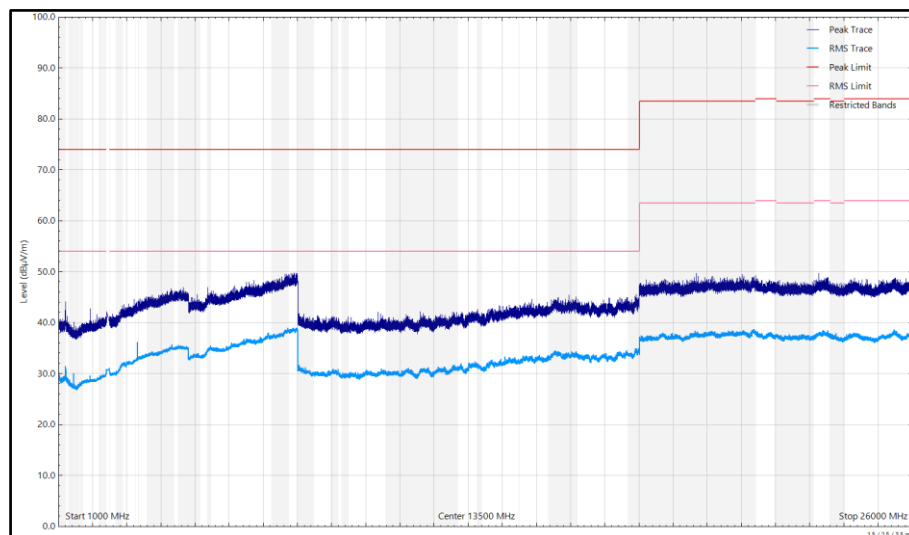
Figure 611 - 2440 MHz (CH2440), HDR8, ePA, Core 0 + Core 1, 1 GHz to 26 GHz, Horizontal
