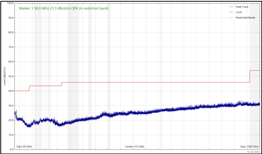
Figure 600 - 2440 MHz (CH2440), HDT4, ePA, Core 0 + Core 1, 30 MHz to 1 GHz, Vertical (Peak)
