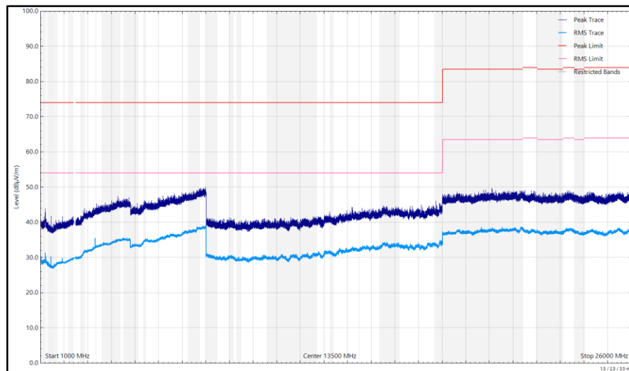
Figure 591 - 2440 MHz (CH2440), HDT4, iPA, Core 0 + Core 1, 1 GHz to 26 GHz, Horizontal
