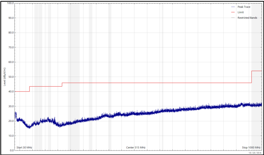
Figure 604 - 2440 MHz (CH2440), HDR8, iPA, Core 0 + Core 1, 30 MHz to 1 GHz, Vertical (Peak)
