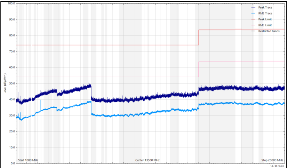
Figure 609 - 2440 MHz (CH2440), HDR8, iPA, Core 2, 1 GHz to 26 GHz, Vertical
