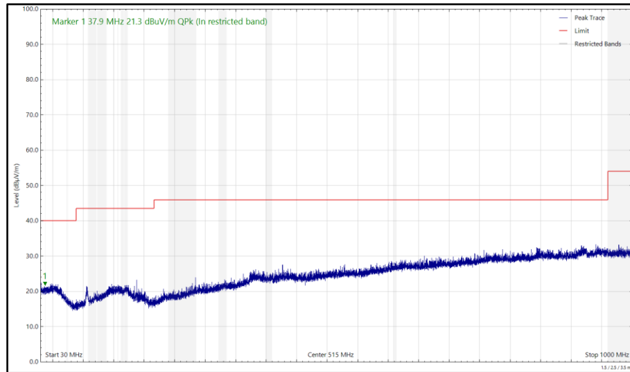
Figure 590 - 2440 MHz (CH2440), HDT4, iPA, Core 0 + Core 1, 30 MHz to 1 GHz, Horizontal (Peak)
