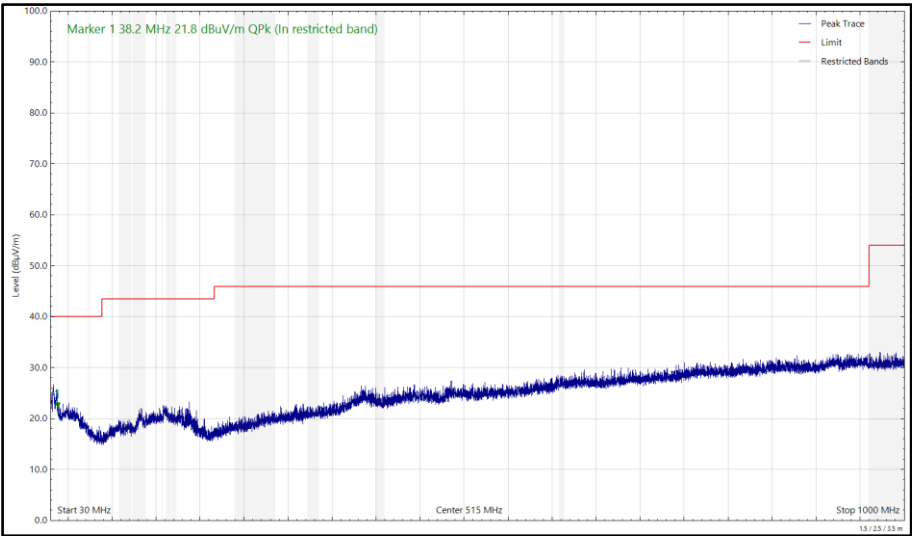
Figure 596 - 2440 MHz (CH2440), HDT4, iPA, Core 2, 30 MHz to 1 GHz, Vertical (Peak)
