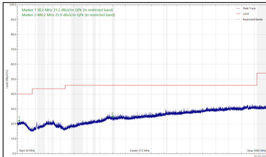
Figure 594 - 2440 MHz (CH2440), HDT4, iPA, Core 2, 30 MHz to 1 GHz, Horizontal (Peak)
