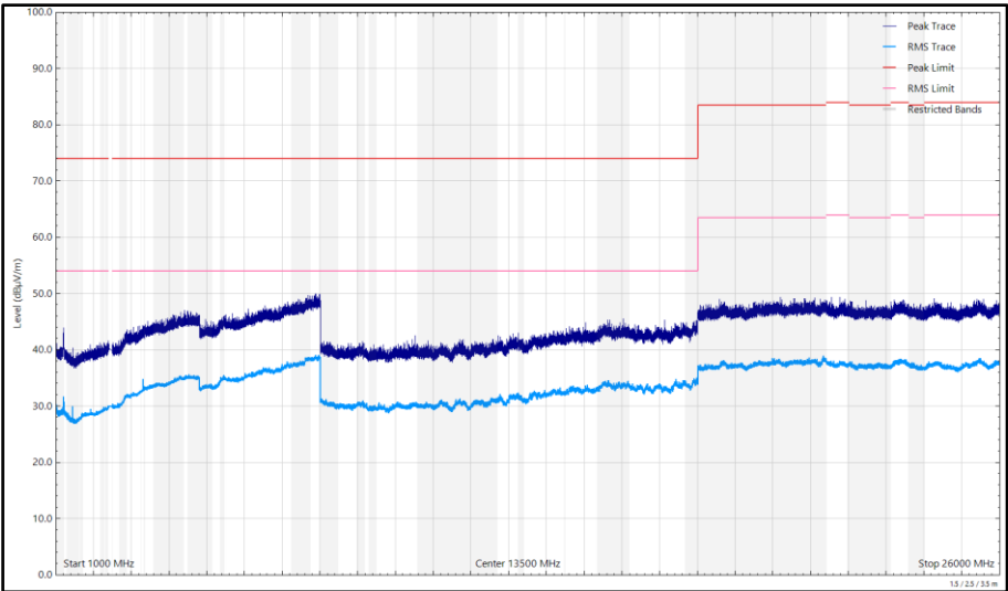
Figure 607 - 2440 MHz (CH2440), HDR8, iPA, Core 2, 1 GHz to 26 GHz, Horizontal
