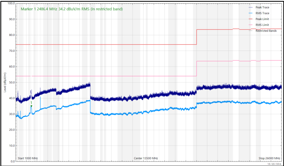
Figure 613 - 2440 MHz (CH2440), HDR8, ePA, Core 0 + Core 1, 1 GHz to 26 GHz, Vertical
