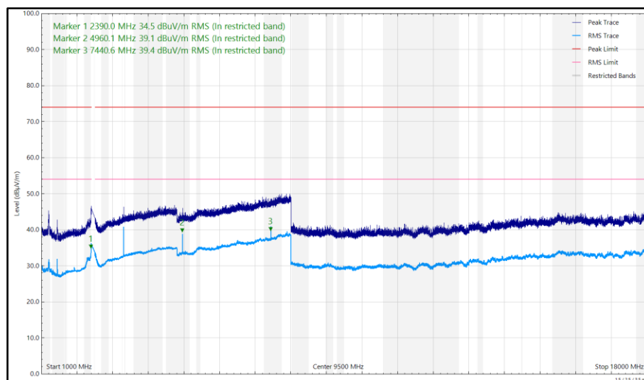
Figure 589 - 2480 MHz (CH2480), LE1M, ePA, Core 0 + Core 1, 1 GHz to 18 GHz, Vertical
