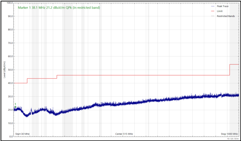
Figure 598 - 2440 MHz (CH2440), HDT4, ePA, Core 0 + Core 1, 30 MHz to 1 GHz, Horizontal (Peak)
