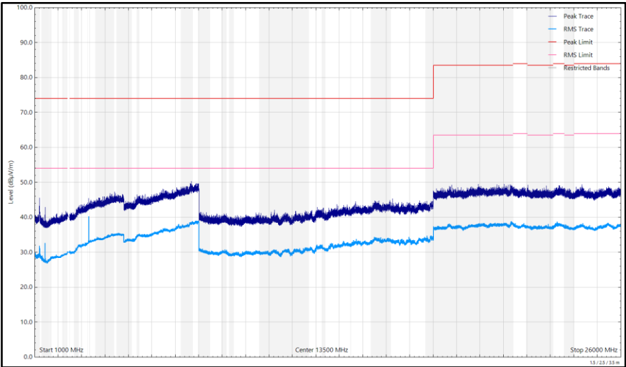
Figure 593 - 2440 MHz (CH2440), HDT4, iPA, Core 0 + Core 1, 1 GHz to 26 GHz, Vertical
