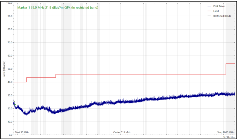
Figure 592 - 2440 MHz (CH2440), HDT4, iPA, Core 0 + Core 1, 30 MHz to 1 GHz, Vertical (Peak)
