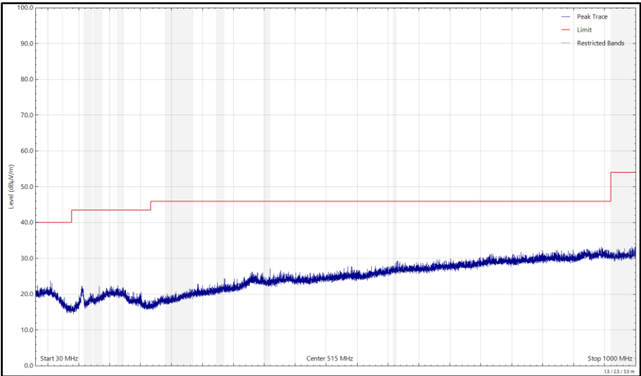
Figure 602 - 2440 MHz (CH2440), HDR8, iPA, Core 0 + Core 1, 30 MHz to 1 GHz, Horizontal (Peak)
