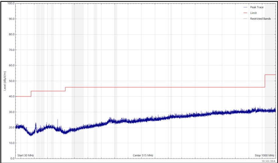
Figure 606 - 2440 MHz (CH2440), HDR8, iPA, Core 2, 30 MHz to 1 GHz, Horizontal (Peak)
