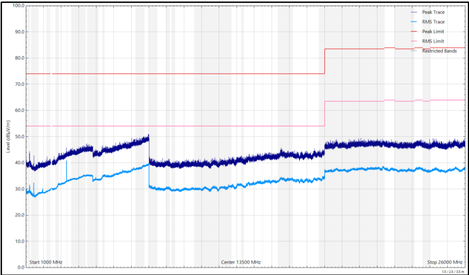
Figure 605 - 2440 MHz (CH2440), HDR8, iPA, Core 0 + Core 1, 1 GHz to 26 GHz, Vertical
