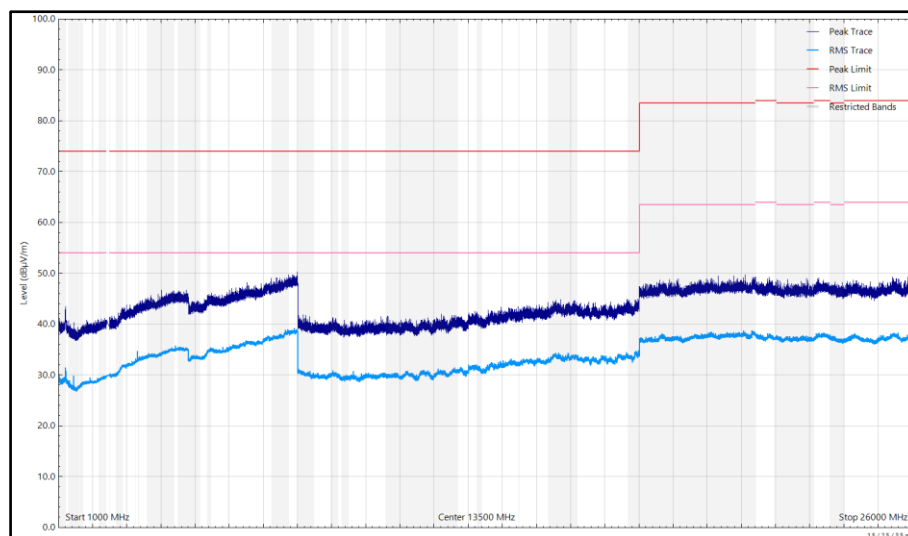
Figure 595 - 2440 MHz (CH2440), HDT4, iPA, Core 2, 1 GHz to 26 GHz, Horizontal
