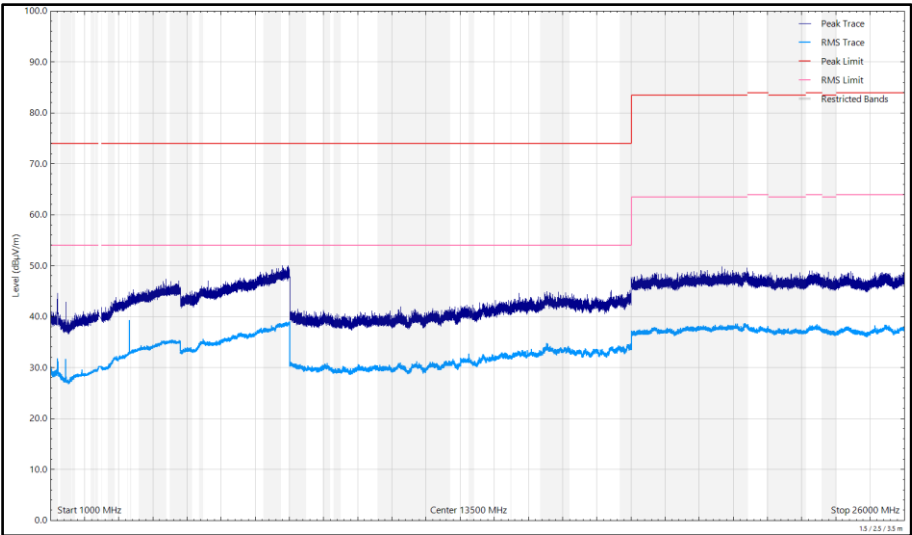
Figure 597 - 2440 MHz (CH2440), HDT4, iPA, Core 2, 1 GHz to 26 GHz, Vertical
