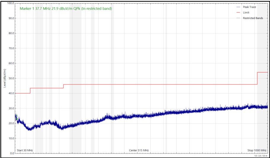
Figure 608 - 2440 MHz (CH2440), HDR8, iPA, Core 2, 30 MHz to 1 GHz, Vertical (Peak)
