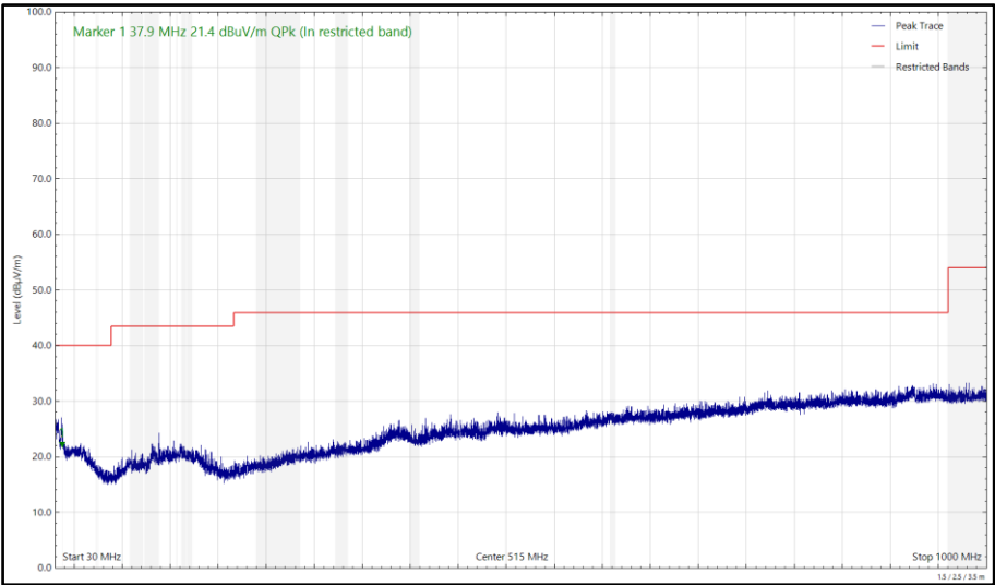
Figure 612 - 2440 MHz (CH2440), HDR8, ePA, Core 0 + Core 1, 30 MHz to 1 GHz, Vertical (Peak)
