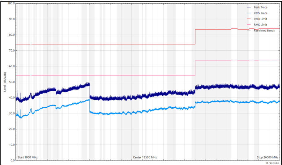
Figure 601 - 2440 MHz (CH2440), HDT4, ePA, Core 0 + Core 1, 1 GHz to 26 GHz, Vertical
