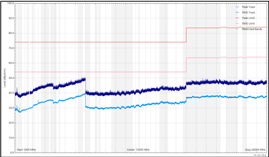
Figure 603 - 2440 MHz (CH2440), HDR8, iPA, Core 0 + Core 1, 1 GHz to 26 GHz, Horizontal
