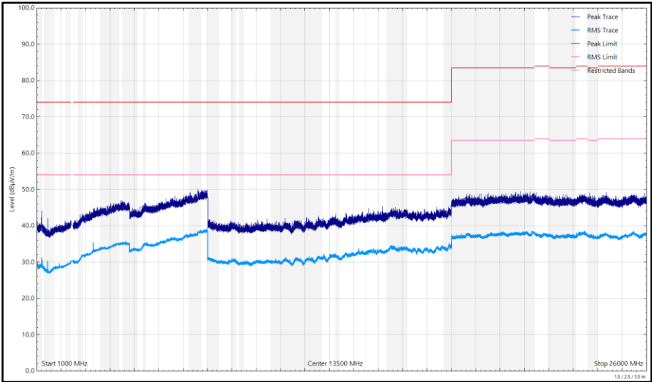
Figure 599 - 2440 MHz (CH2440), HDT4, ePA, Core 0 + Core 1, 1 GHz to 26 GHz, Horizontal
