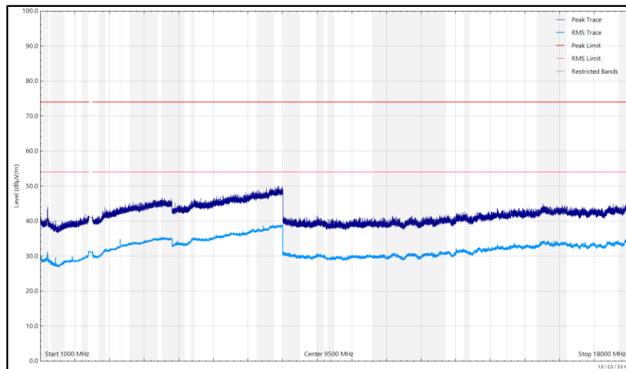
Figure 588 - 2480 MHz (CH2480), LE1M, ePA, Core 0 + Core 1, 1 GHz to 18 GHz, Horizontal
