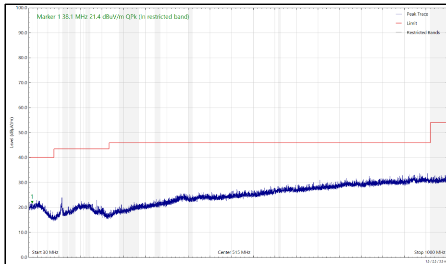
Figure 610 - 2440 MHz (CH2440), HDR8, ePA, Core 0 + Core 1, 30 MHz to 1 GHz, Horizontal (Peak)
