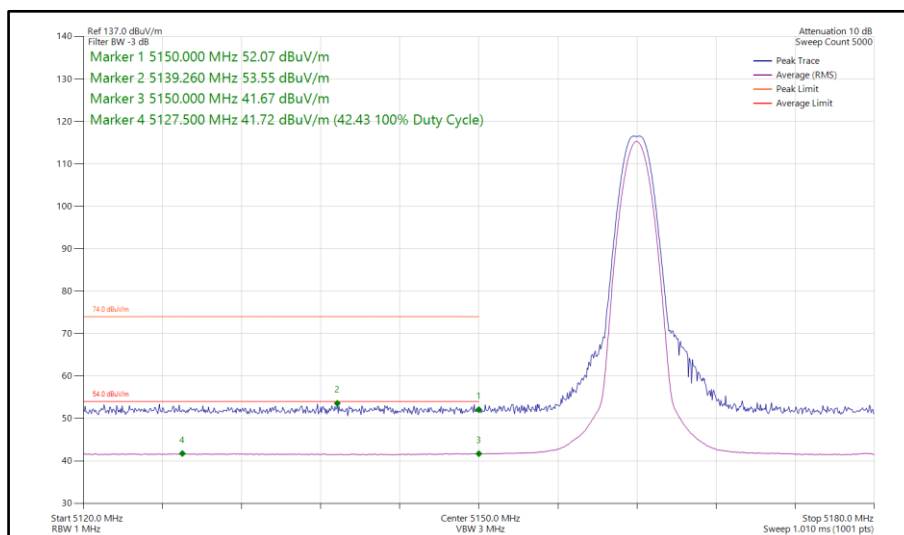
Figure 68 - Narrowband LE1M, MIMO, Core 0-1 - 5162 MHz Band Edge Frequency 5150 MHz
