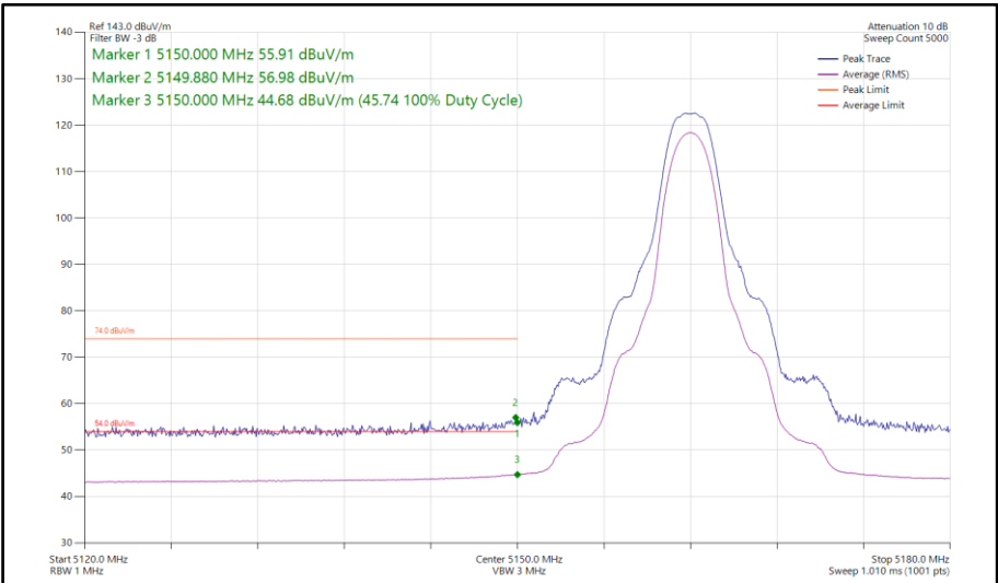
Figure 98 - Narrowband HDR4, SISO, Core 0 - 5162 MHz Band Edge Frequency 5150 MHz
