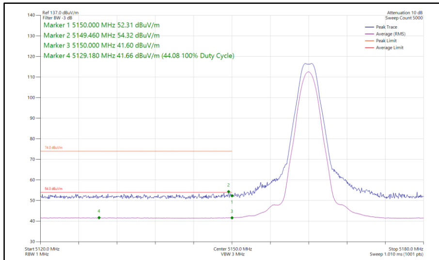
Figure 69 - Narrowband LE2M, MIMO, Core 0-1 - 5162 MHz Band Edge Frequency 5150 MHz
