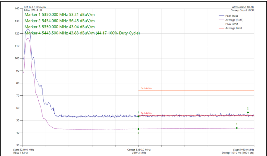
Figure 122 - Narrowband HDRPM12, SISO, Core 0 - 5245 MHz Band Edge Frequency 5350 MHz
