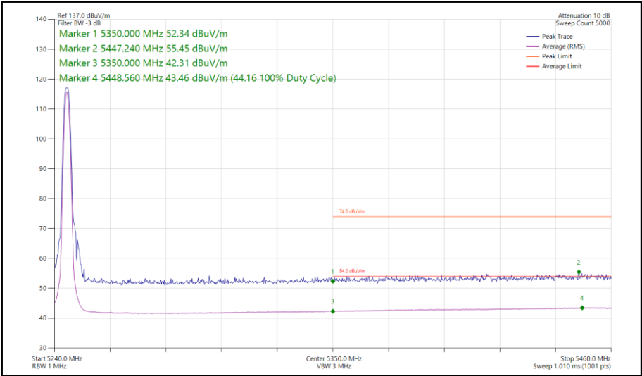
Figure 95 - Narrowband CS1LE1M, MIMO, Core 0-1 - 5245 MHz Band Edge Frequency 5350 MHz
