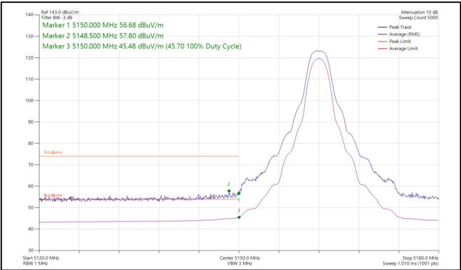
Figure 102 - Narrowband HDT3, SISO, Core 0 - 5162 MHz Band Edge Frequency 5150 MHz
