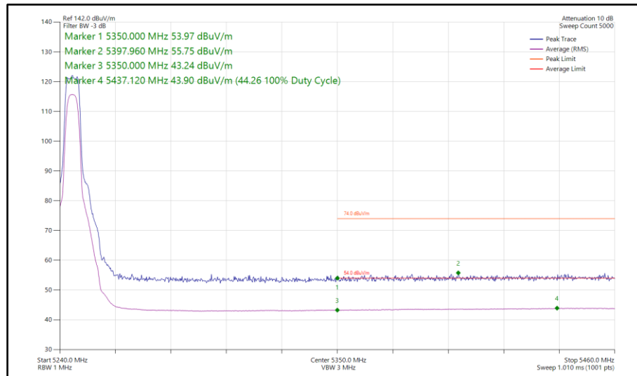
Figure 125 - Narrowband XHDRPM8, SISO, Core 0 - 5245 MHz Band Edge Frequency 5350 MHz
