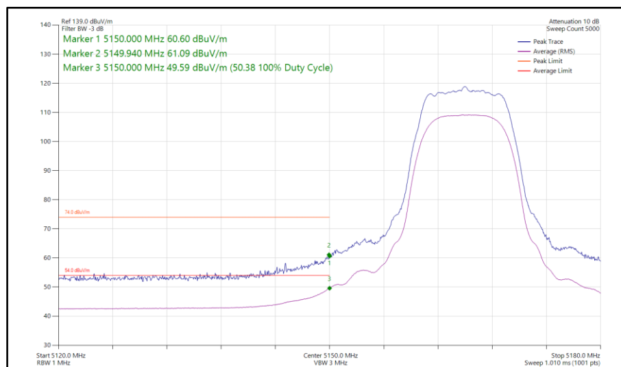
Figure 110 - Narrowband XHDRPL24, SISO, Core 0 - 5165 MHz Band Edge Frequency 5150 MHz
