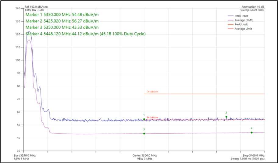
Figure 115 - Narrowband HDR8, SISO, Core 0 - 5245 MHz Band Edge Frequency 5350 MHz
