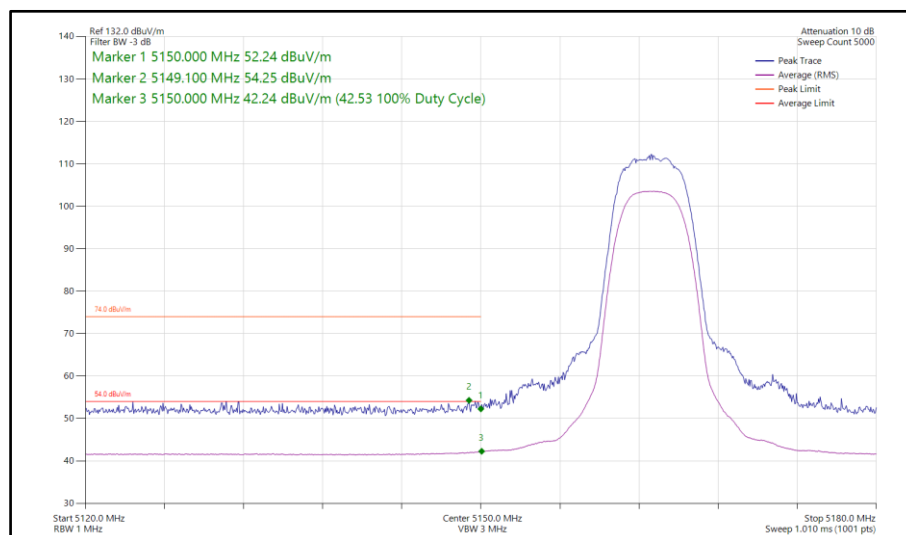
Figure 74 - Narrowband HDRPM12, MIMO, Core 0-1 - 5163 MHz Band Edge Frequency 5150 MHz
