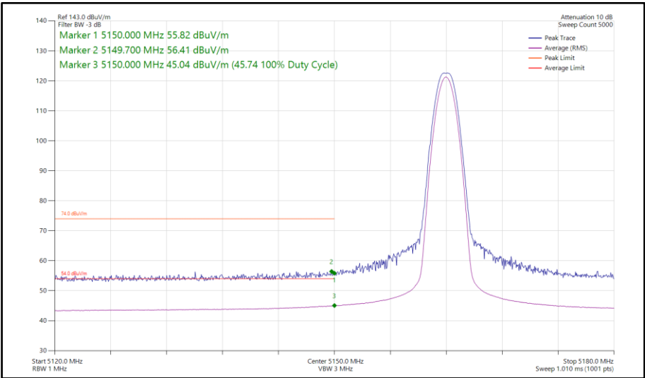
Figure 100 - Narrowband LE1M, SISO, Core 0 - 5162 MHz Band Edge Frequency 5150 MHz
