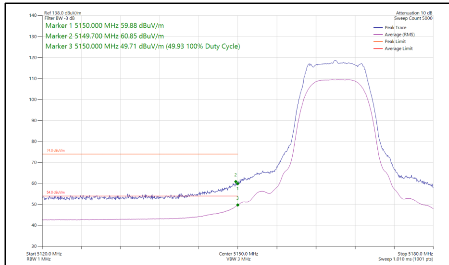
Figure 107 - Narrowband HDRPL8, SISO, Core 0 - 5165 MHz Band Edge Frequency 5150 MHz
