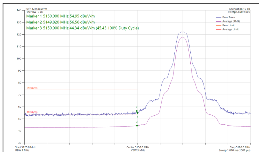
Figure 130 - Narrowband HDR4, SISO, Core 1 - 5162 MHz Band Edge Frequency 5150 MHz
