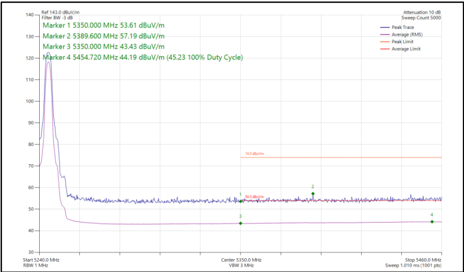
Figure 114 - Narrowband HDR4, SISO, Core 0 - 5245 MHz Band Edge Frequency 5350 MHz
