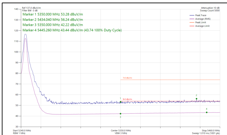
Figure 87 - Narrowband HDT4, MIMO, Core 0-1 - 5245 MHz Band Edge Frequency 5350 MHz
