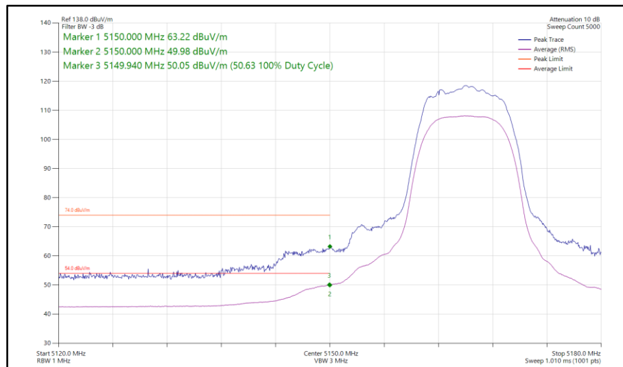
Figure 108 - Narrowband HDRPL24, SISO, Core 0 - 5165 MHz Band Edge Frequency 5150 MHz
