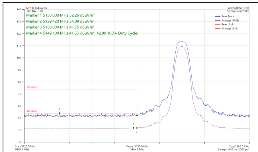
Figure 66 - Narrowband HDR4, MIMO, Core 0-1 - 5162 MHz Band Edge Frequency 5150 MHz
