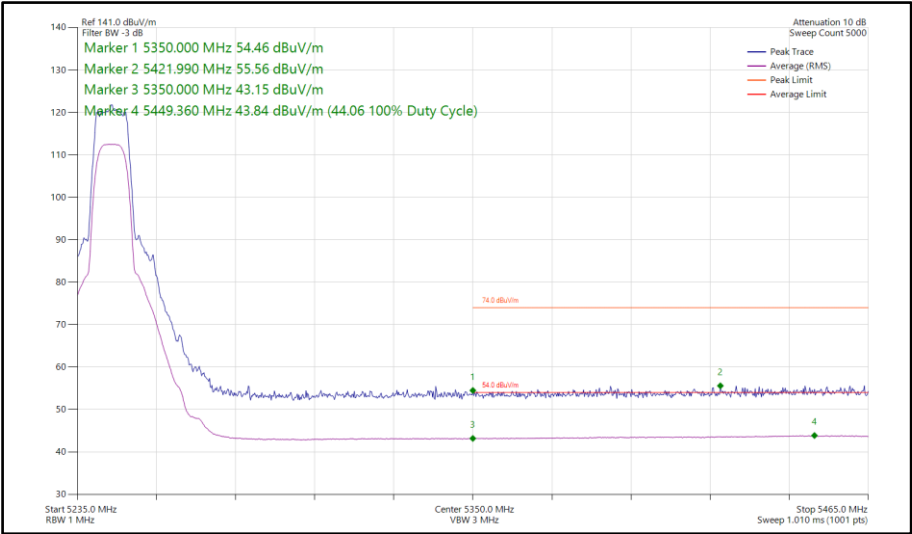
Figure 123 - Narrowband HDRPL8, SISO, Core 0 - 5245 MHz Band Edge Frequency 5350 MHz
