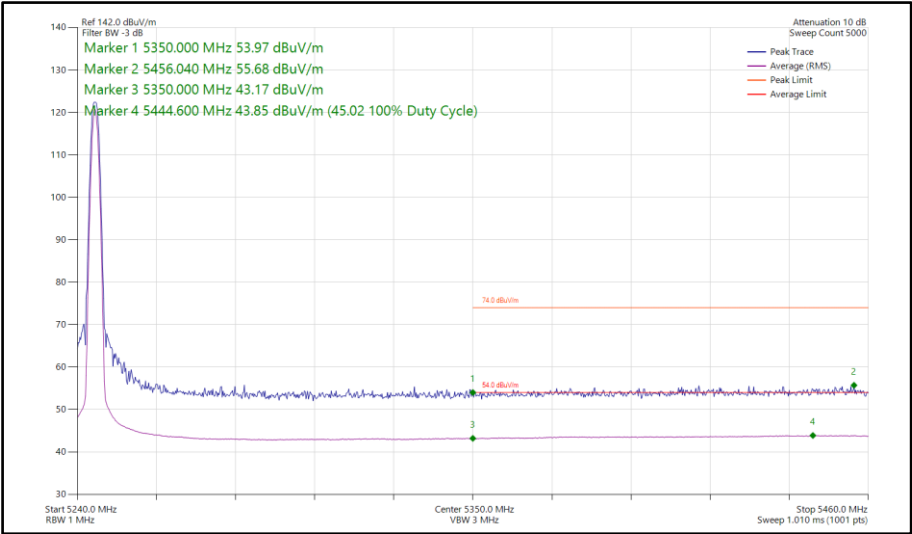
Figure 113 - Narrowband DH5, SISO, Core 0 - 5245 MHz Band Edge Frequency 5350 MHz
