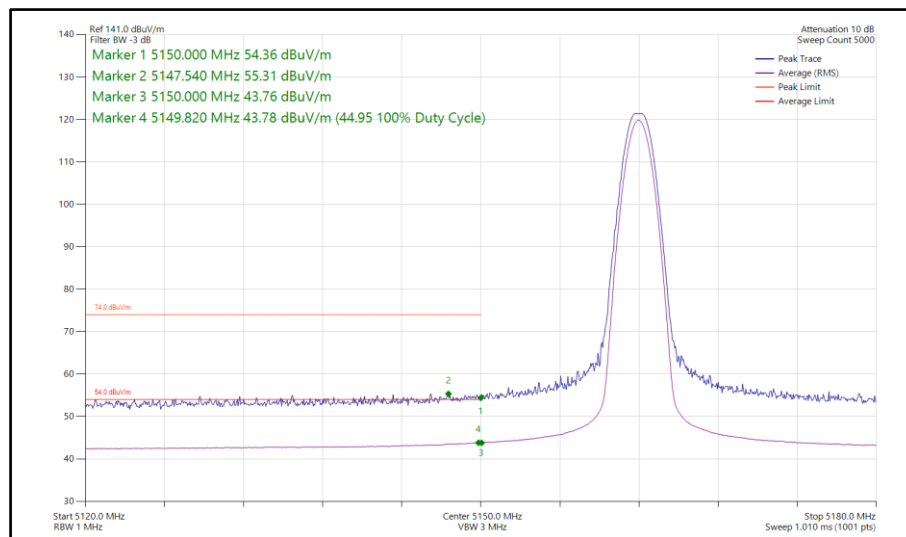
Figure 129 - Narrowband DH5, SISO, Core 1 - 5162 MHz Band Edge Frequency 5150 MHz
