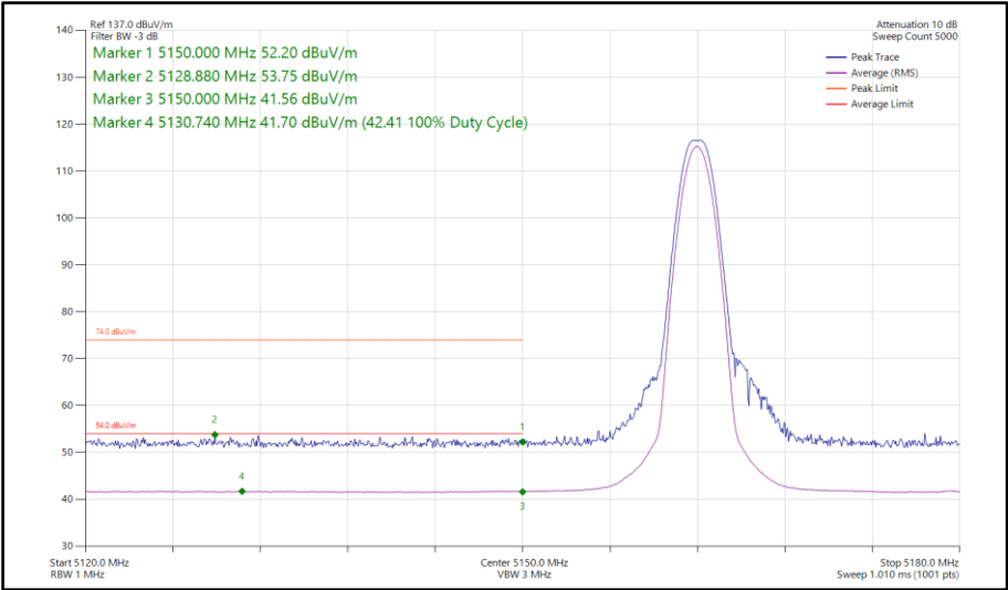
Figure 79 - Narrowband CS1LE1M, MIMO, Core 0-1 - 5162 MHz Band Edge Frequency 5150 MHz
