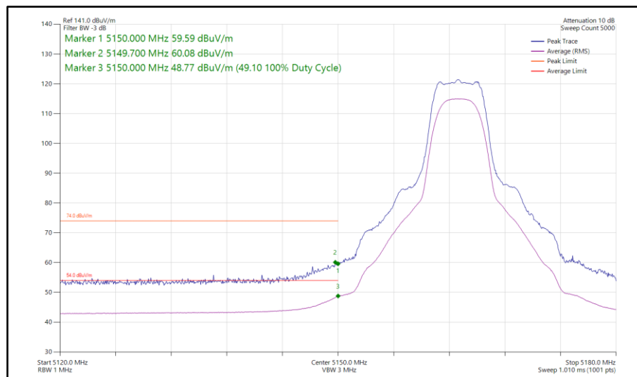
Figure 109 - Narrowband XHDRPM8, SISO, Core 0 - 5163 MHz Band Edge Frequency 5150 MHz
