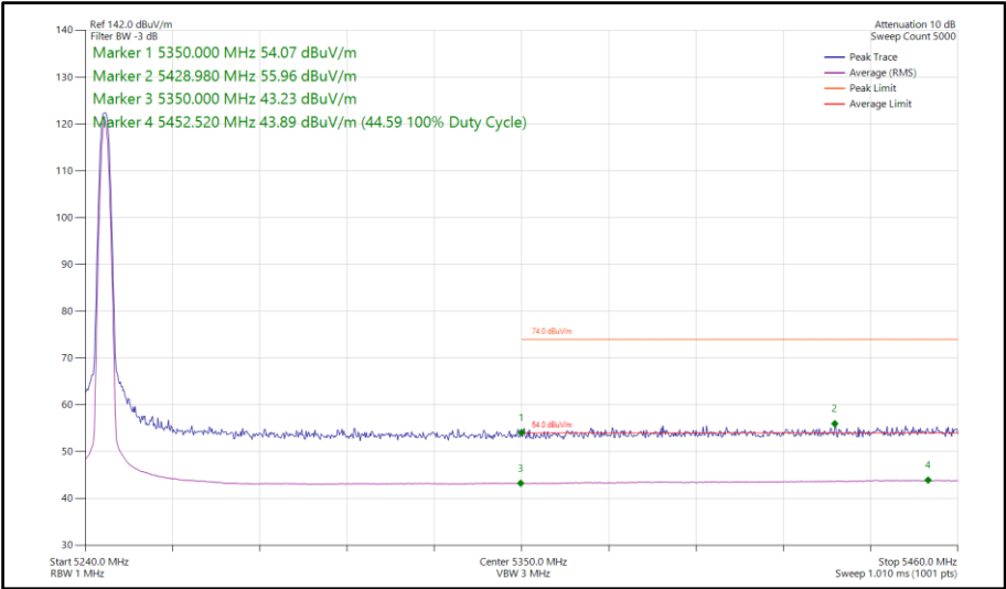
Figure 127 - Narrowband CS1LE1M, SISO, Core 0 - 5245 MHz Band Edge Frequency 5350 MHz
