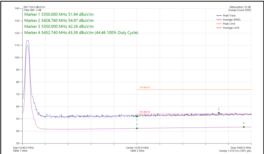
Figure 82 - Narrowband HDR4, MIMO, Core 0-1 - 5245 MHz Band Edge Frequency 5350 MHz
