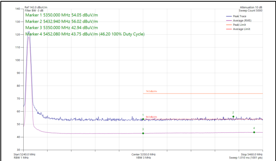
Figure 128 - Narrowband CS1LE2M, SISO, Core 0 - 5245 MHz Band Edge Frequency 5350 MHz
