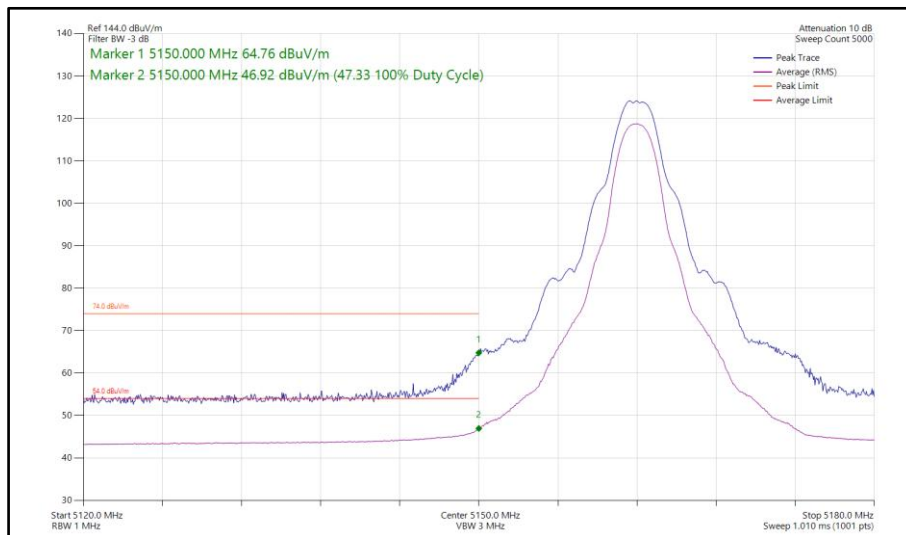
Figure 104 - Narrowband HDT6, SISO, Core 0 - 5162 MHz Band Edge Frequency 5150 MHz
