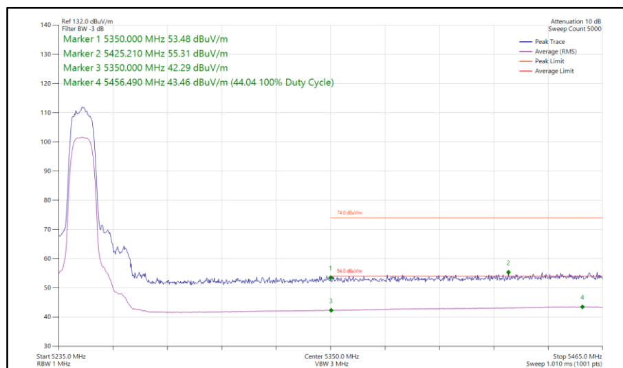
Figure 92 - Narrowband HDRPL24, MIMO, Core 0-1 - 5245 MHz Band Edge Frequency 5350 MHz
