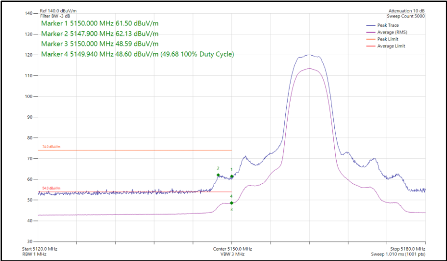
Figure 131 - Narrowband HDR8, SISO, Core 1 - 5162 MHz Band Edge Frequency 5150 MHz
