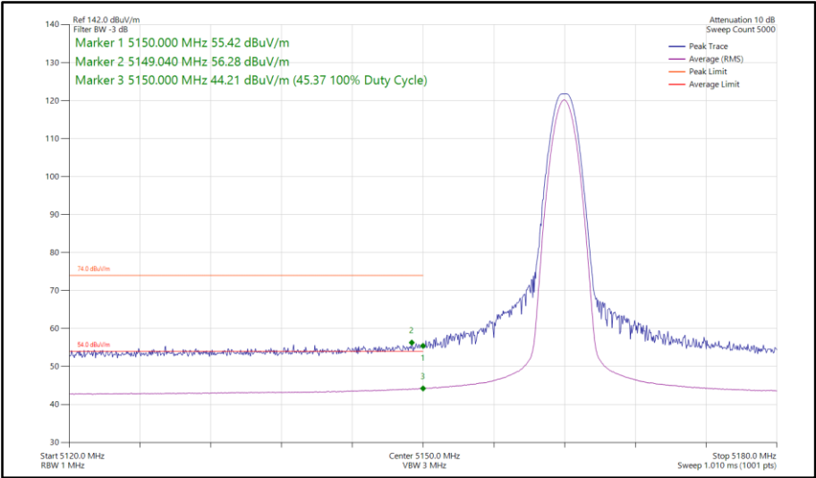
Figure 97 - Narrowband DH5, SISO, Core 0 - 5162 MHz Band Edge Frequency 5150 MHz
