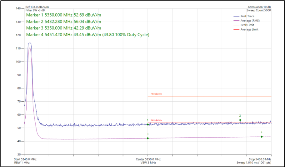
Figure 89 - Narrowband HDRPS2, MIMO, Core 0-1 - 5245 MHz Band Edge Frequency 5350 MHz
