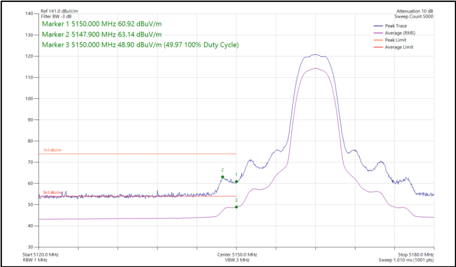
Figure 99 - Narrowband HDR8, SISO, Core 0 - 5162 MHz Band Edge Frequency 5150 MHz
