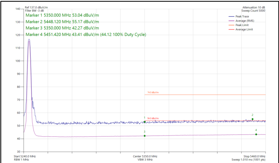
Figure 84 - Narrowband LE1M, MIMO, Core 0-1 - 5245 MHz Band Edge Frequency 5350 MHz
