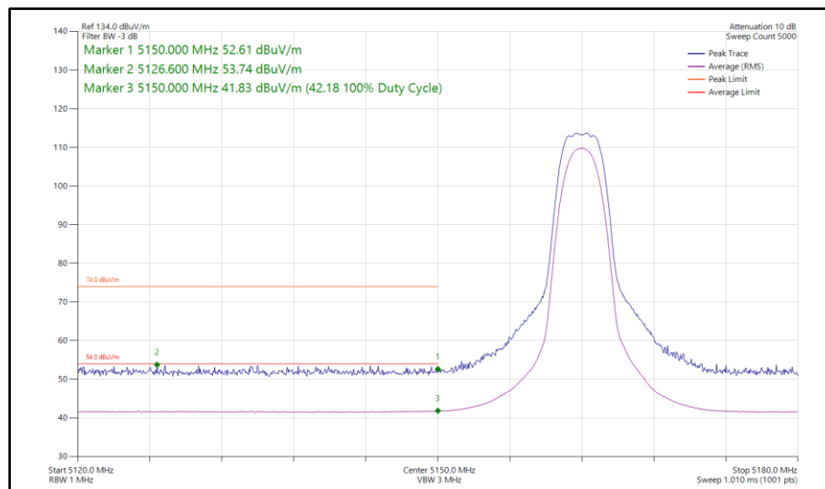
Figure 73 - Narrowband HDRPS2, MIMO, Core 0-1 - 5162 MHz Band Edge Frequency 5150 MHz
