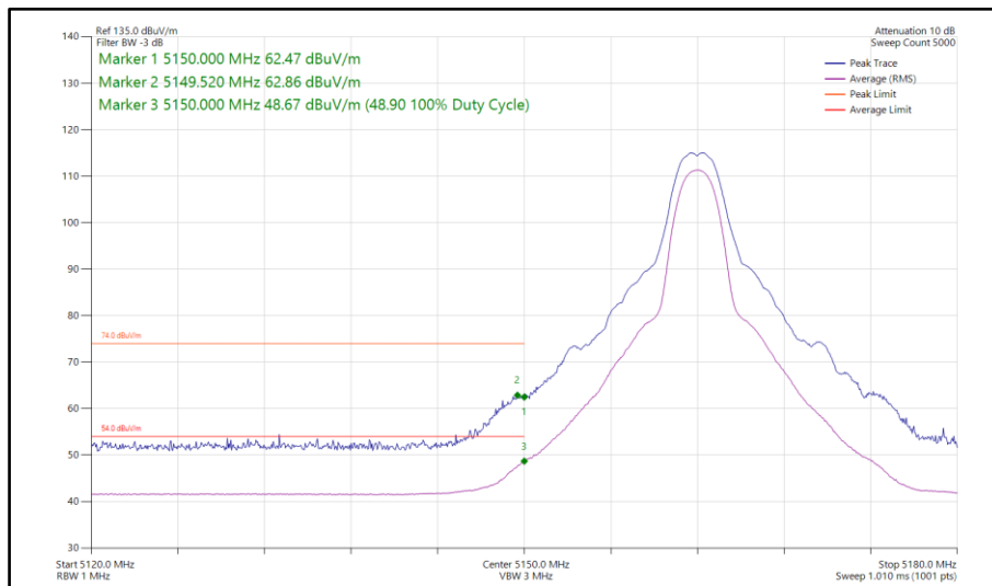
Figure 70 - Narrowband HDT3, MIMO, Core 0-1 - 5162 MHz Band Edge Frequency 5150 MHz
