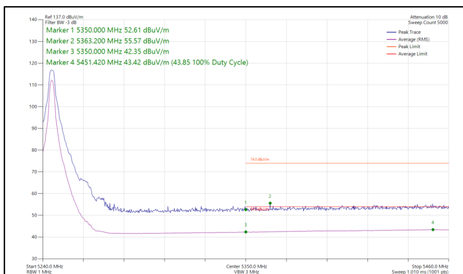
Figure 88 - Narrowband HDT6, MIMO, Core 0-1 - 5245 MHz Band Edge Frequency 5350 MHz
