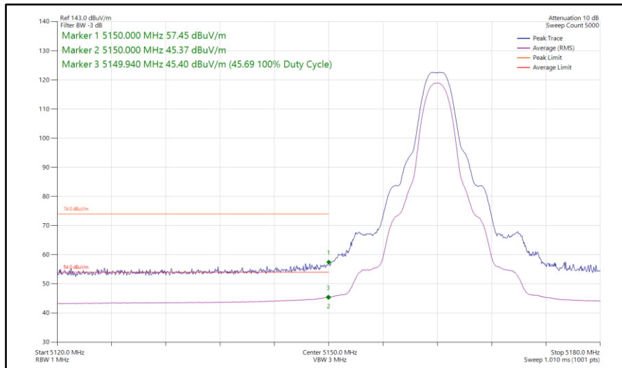
Figure 103 - Narrowband HDT4, SISO, Core 0 - 5162 MHz Band Edge Frequency 5150 MHz
