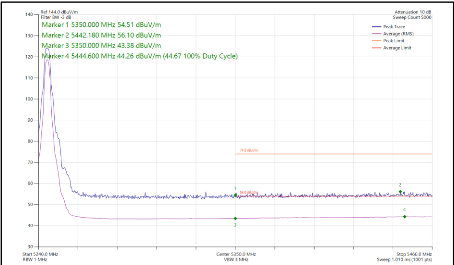
Figure 120 - Narrowband HDT6, SISO, Core 0 - 5245 MHz Band Edge Frequency 5350 MHz
