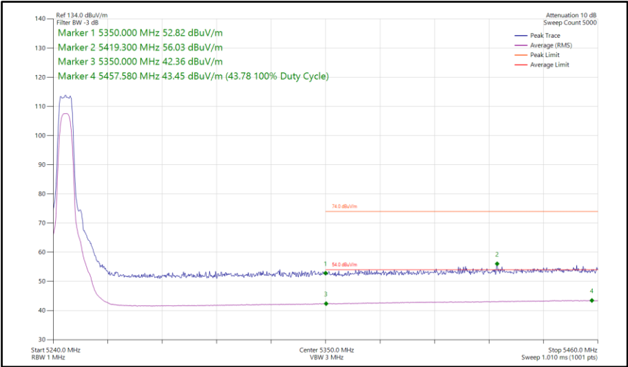
Figure 93 - Narrowband XHDRPM8, MIMO, Core 0-1 - 5245 MHz Band Edge Frequency 5350 MHz
