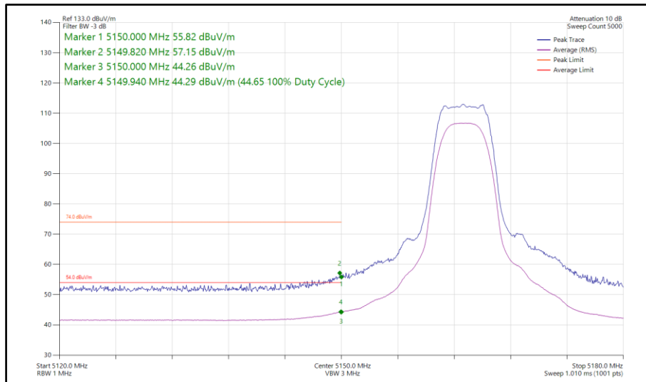
Figure 77 - Narrowband XHDRPM8, MIMO, Core 0-1 - 5163 MHz Band Edge Frequency 5150 MHz
