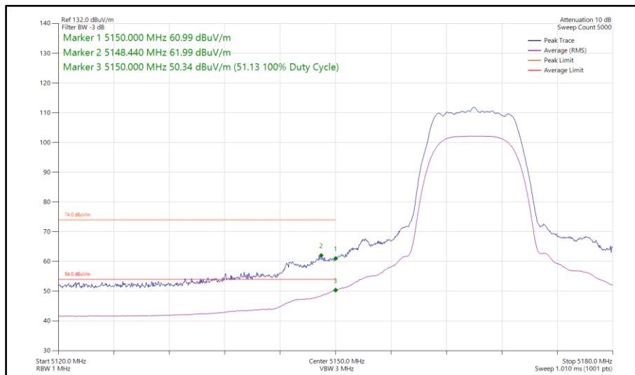
Figure 78 - Narrowband XHDRPL24, MIMO, Core 0-1 - 5165 MHz Band Edge Frequency 5150 MHz
