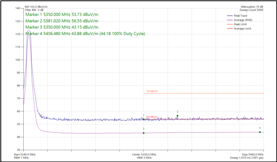
Figure 121 - Narrowband HDRPS2, SISO, Core 0 - 5245 MHz Band Edge Frequency 5350 MHz
