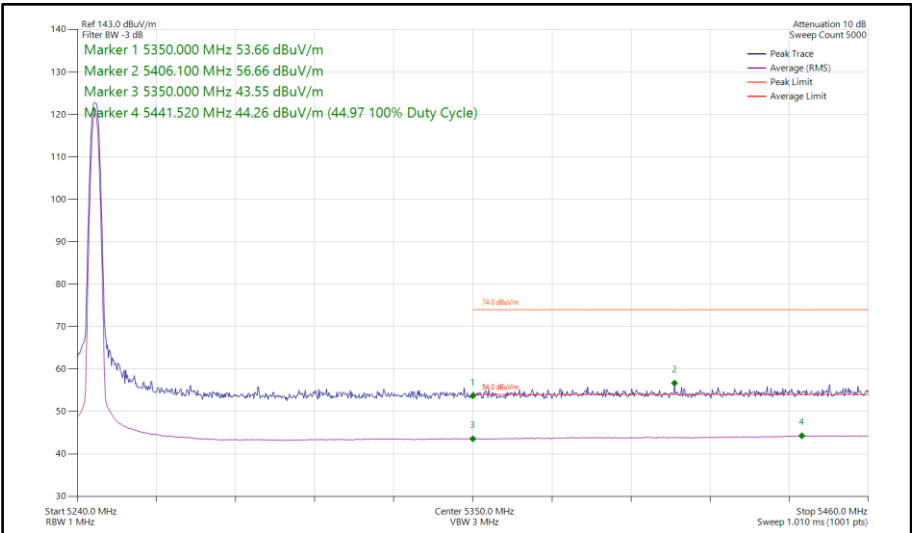
Figure 116 - Narrowband LE1M, SISO, Core 0 - 5245 MHz Band Edge Frequency 5350 MHz
