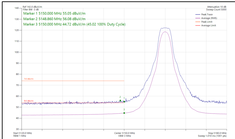
Figure 105 - Narrowband HDRPS2, SISO, Core 0 - 5162 MHz Band Edge Frequency 5150 MHz
