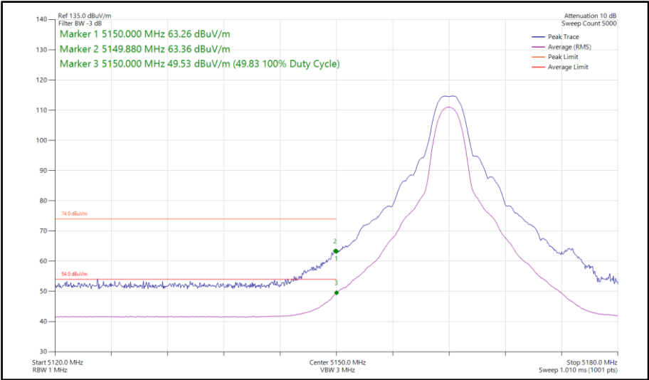
Figure 71 - Narrowband HDT4, MIMO, Core 0-1 - 5162 MHz Band Edge Frequency 5150 MHz
