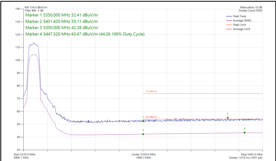
Figure 94 - Narrowband XHDRPL24, MIMO, Core 0-1 - 5245 MHz Band Edge Frequency 5350 MHz
