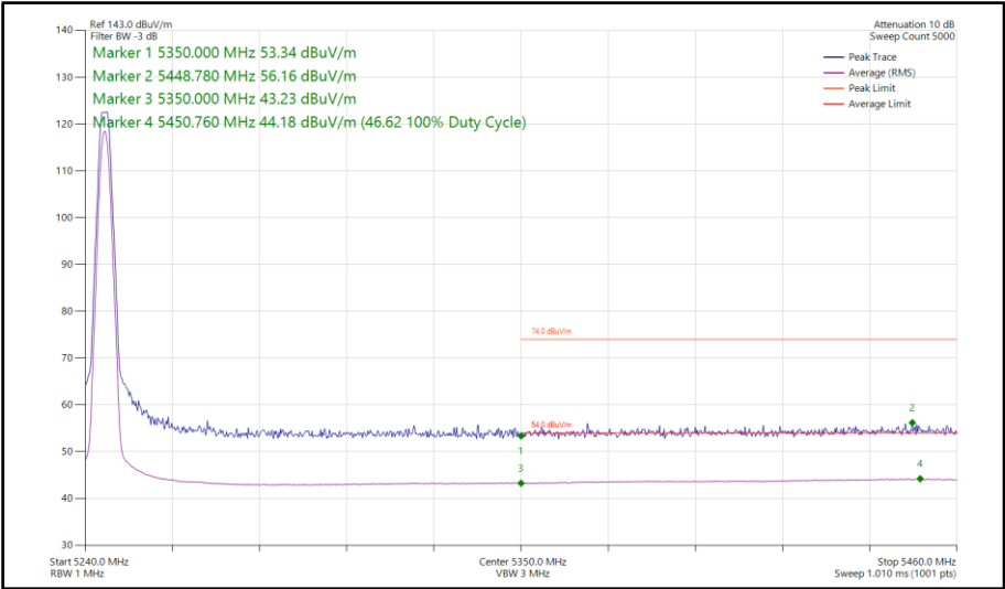
Figure 117 - Narrowband LE2M, SISO, Core 0 - 5245 MHz Band Edge Frequency 5350 MHz
