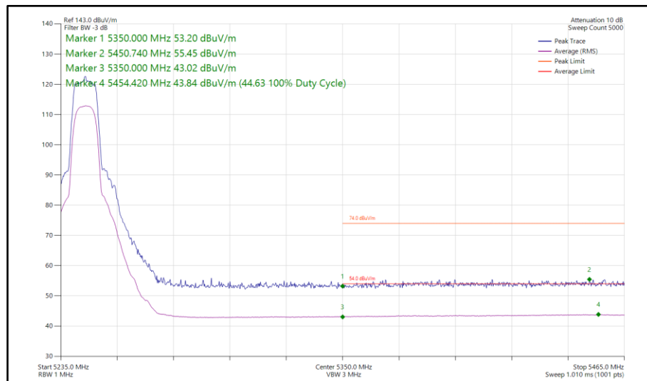
Figure 126 - Narrowband XHDRPL24, SISO, Core 0 - 5245 MHz Band Edge Frequency 5350 MHz
