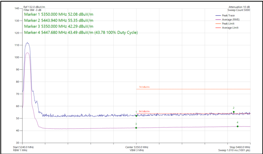
Figure 90 - Narrowband HDRPM12, MIMO, Core 0-1 - 5245 MHz Band Edge Frequency 5350 MHz
