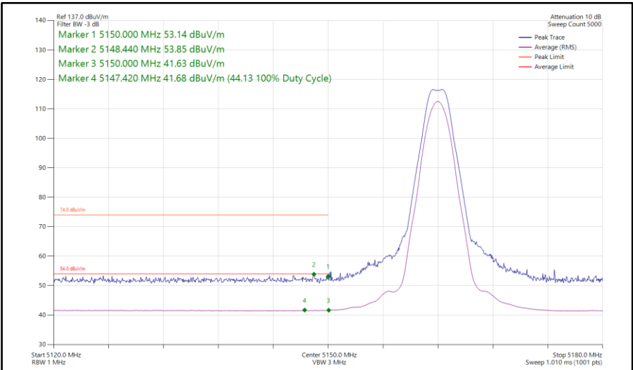
Figure 80 - Narrowband CS1LE2M, MIMO, Core 0-1 - 5162 MHz Band Edge Frequency 5150 MHz
