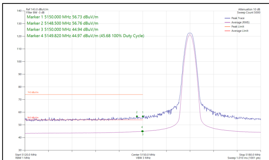
Figure 111 - Narrowband CS1LE1M, SISO, Core 0 - 5162 MHz Band Edge Frequency 5150 MHz
