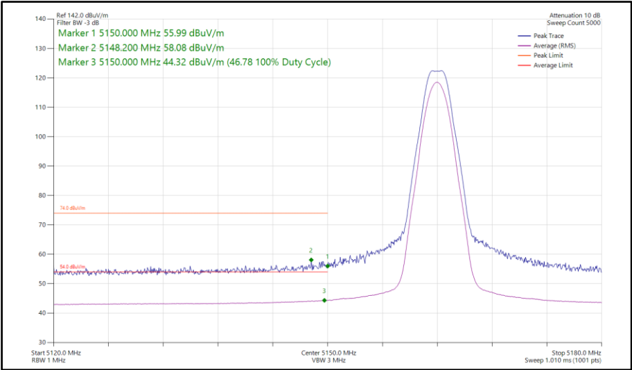
Figure 101 - Narrowband LE2M, SISO, Core 0 - 5162 MHz Band Edge Frequency 5150 MHz
