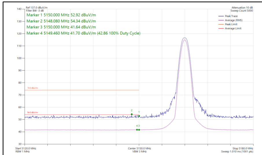
Figure 65 - Narrowband DH5, MIMO, Core 0-1 - 5162 MHz Band Edge Frequency 5150 MHz
