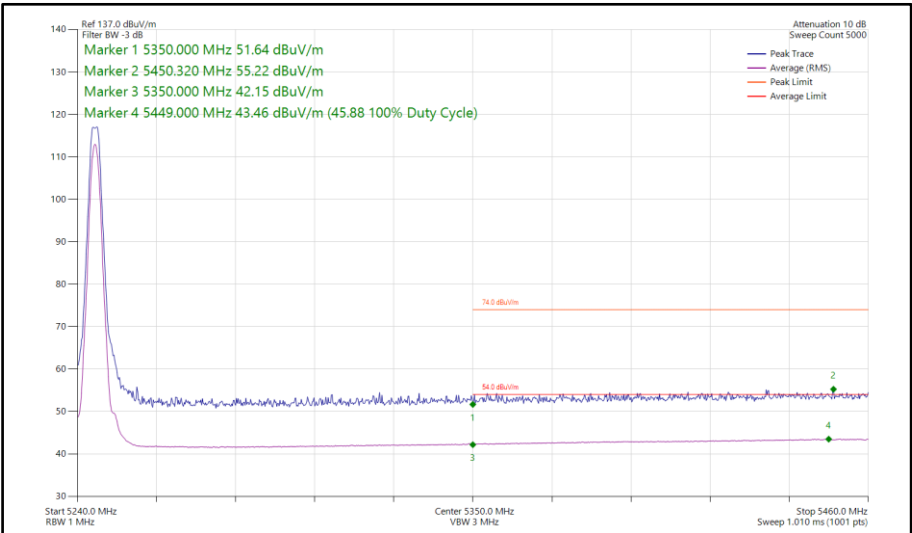
Figure 96 - Narrowband CS1LE2M, MIMO, Core 0-1 - 5245 MHz Band Edge Frequency 5350 MHz
