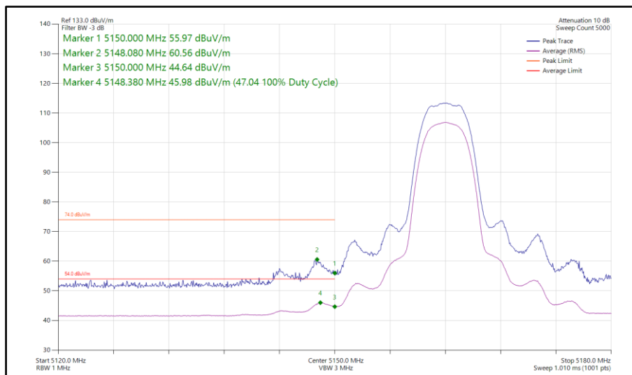
Figure 67 - Narrowband HDR8, MIMO, Core 0-1 - 5162 MHz Band Edge Frequency 5150 MHz
