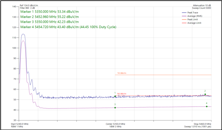
Figure 83 - Narrowband HDR8, MIMO, Core 0-1 - 5245 MHz Band Edge Frequency 5350 MHz
