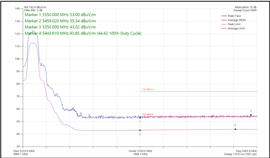
Figure 124 - Narrowband HDRPL24, SISO, Core 0 - 5245 MHz Band Edge Frequency 5350 MHz
