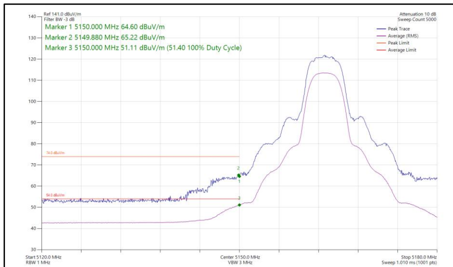
Figure 106 - Narrowband HDRPM12, SISO, Core 0 - 5163 MHz Band Edge Frequency 5150 MHz
