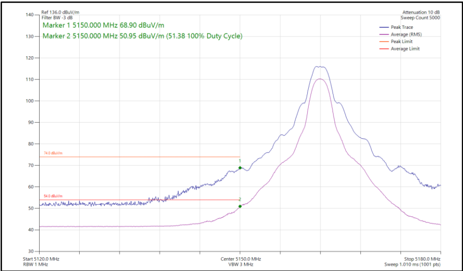
Figure 72 - Narrowband HDT6, MIMO, Core 0-1 - 5162 MHz Band Edge Frequency 5150 MHz
