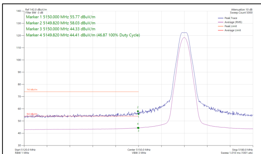
Figure 112 - Narrowband CS1LE2M, SISO, Core 0 - 5162 MHz Band Edge Frequency 5150 MHz
