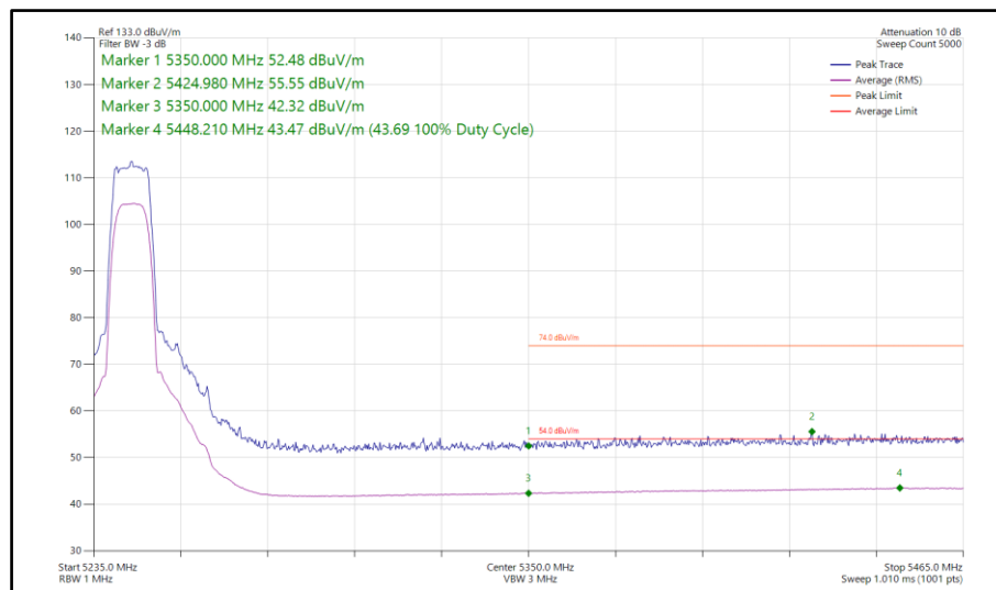
Figure 91 - Narrowband HDRPL8, MIMO, Core 0-1 - 5245 MHz Band Edge Frequency 5350 MHz
