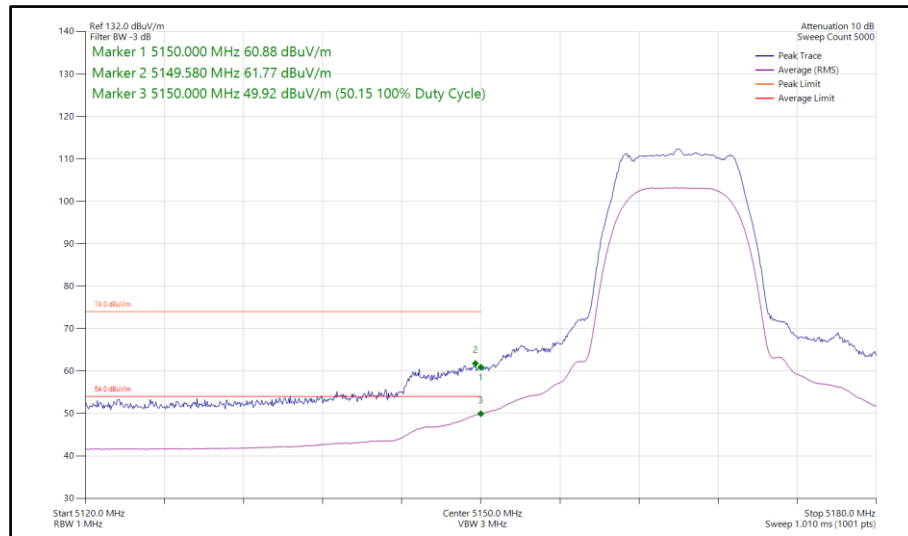
Figure 75 - Narrowband HDRPL8, MIMO, Core 0-1 - 5165 MHz Band Edge Frequency 5150 MHz
