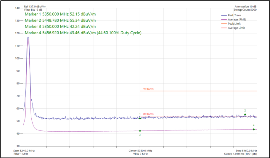
Figure 81 - Narrowband DH5, MIMO, Core 0-1 - 5245 MHz Band Edge Frequency 5350 MHz
