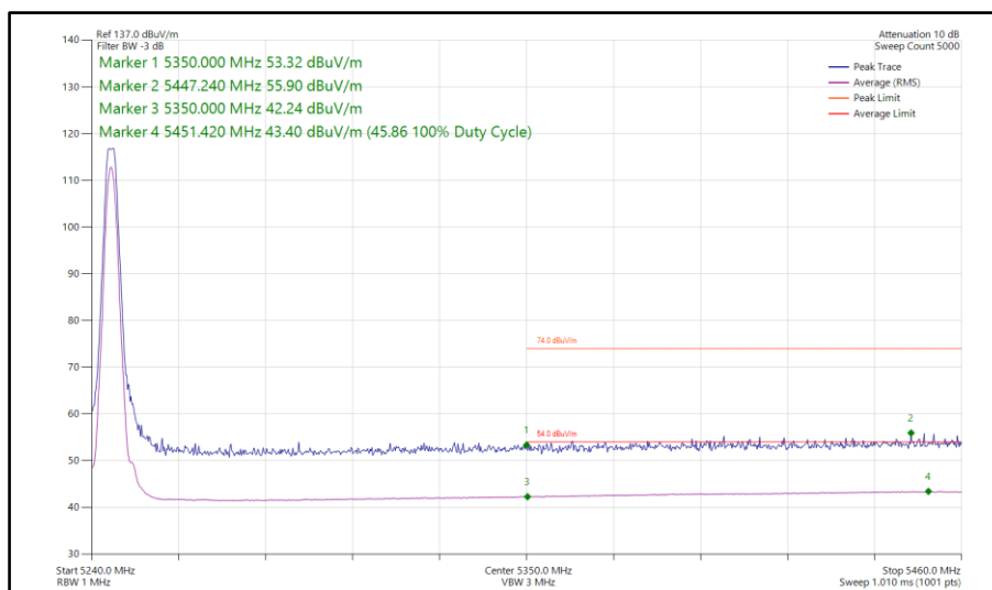
Figure 85 - Narrowband LE2M, MIMO, Core 0-1 - 5245 MHz Band Edge Frequency 5350 MHz
