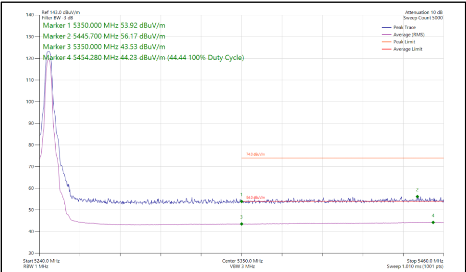
Figure 118 - Narrowband HDT3, SISO, Core 0 - 5245 MHz Band Edge Frequency 5350 MHz
