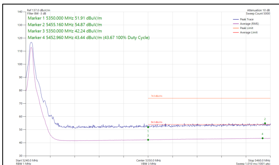
Figure 86 - Narrowband HDT3, MIMO, Core 0-1 - 5245 MHz Band Edge Frequency 5350 MHz
