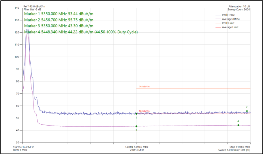
Figure 119 - Narrowband HDT4, SISO, Core 0 - 5245 MHz Band Edge Frequency 5350 MHz
