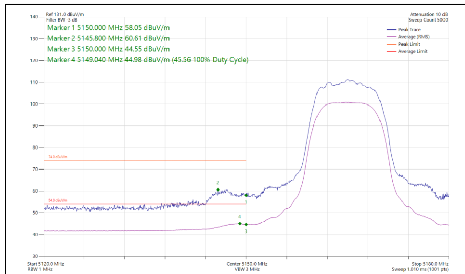
Figure 76 - Narrowband HDRPL24, MIMO, Core 0-1 - 5165 MHz Band Edge Frequency 5150 MHz
