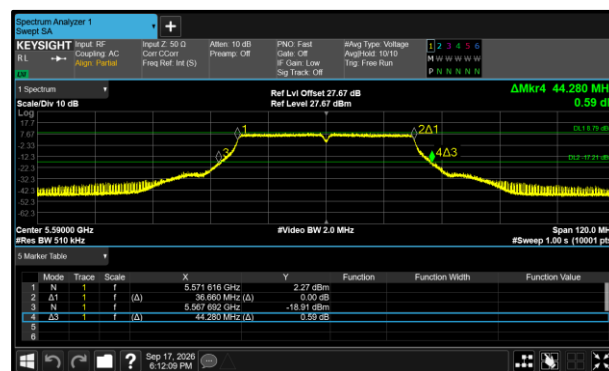
Figure 392 - 802.11n HT40 Maximum 99% OBW
