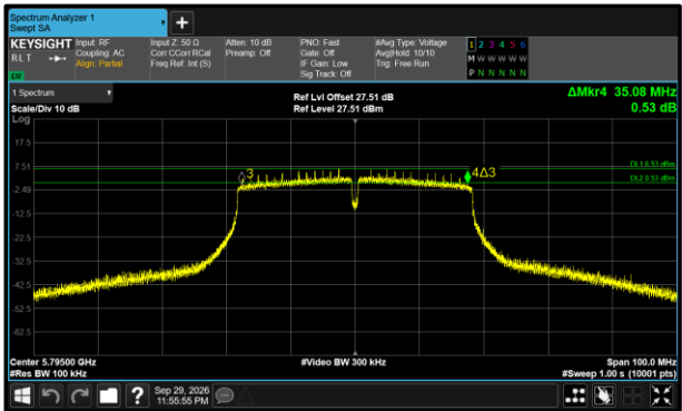
Figure 416 - 802.11n HT40 Maximum 6 dB EBW
