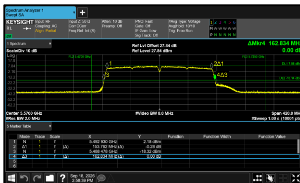
Figure 355 - 802.11ac VHT160 Minimum 99% OBW
