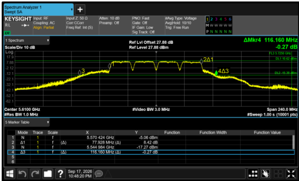
Figure 370 - 802.11a80 Maximum 99% OBW
