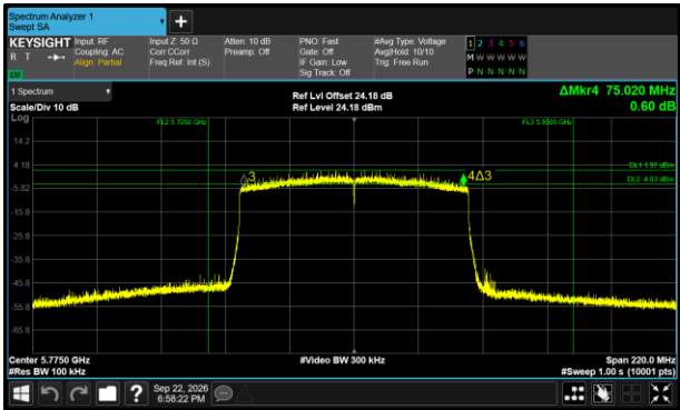
Figure 424 - 802.11ax HE80 SU Maximum 6 dB EBW
