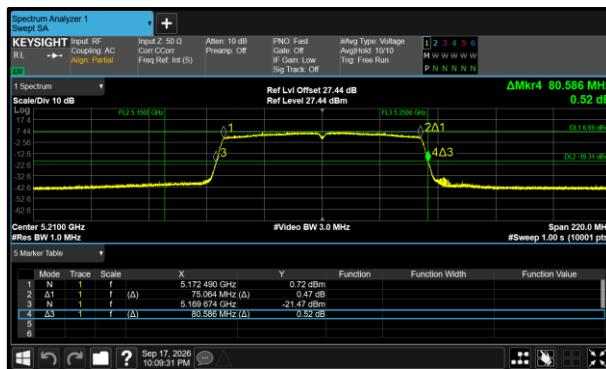
Figure 353 - 802.11ac VHT80 Minimum 99% OBW
