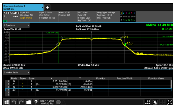
Figure 391 - 802.11n HT40 Minimum 99% OBW
