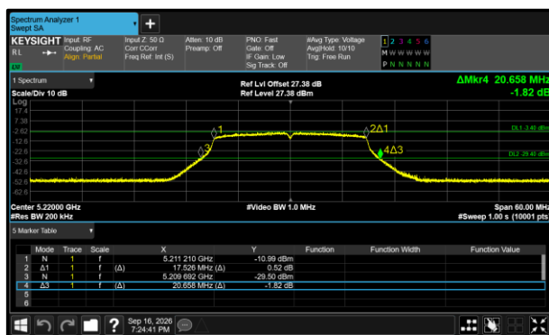
Figure 389 - 802.11n HT20 Minimum 99% OBW
