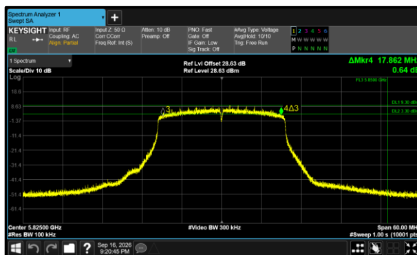
Figure 431 - 802.11ax HE20 SU Minimum 6 dB EBW
