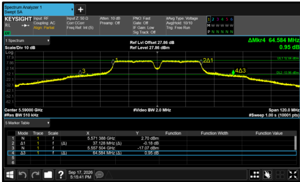
Figure 368 - 802.11a40 Maximum 99% OBW
