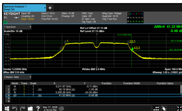
Figure 407 - 802.11a40 Minimum 99% OBW
