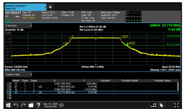
Figure 350 - 802.11n HT20 Maximum 99% OBW
