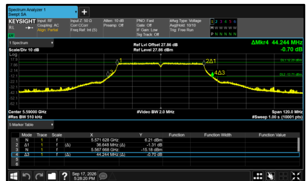
Figure 352 - 802.11n HT40 Maximum 99% OBW
