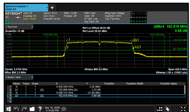
Figure 396 - 802.11ac VHT160 Maximum 99% OBW
