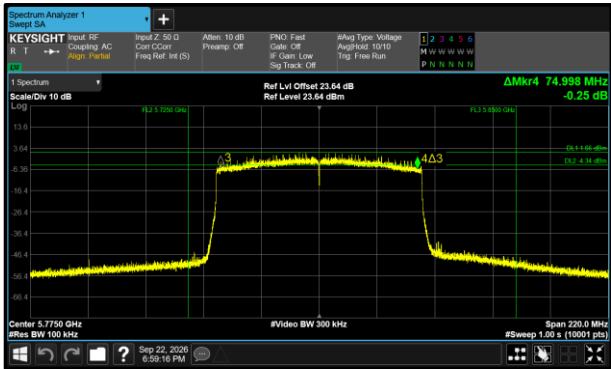
Figure 423 - 802.11ax HE80 SU Minimum 6 dB EBW
