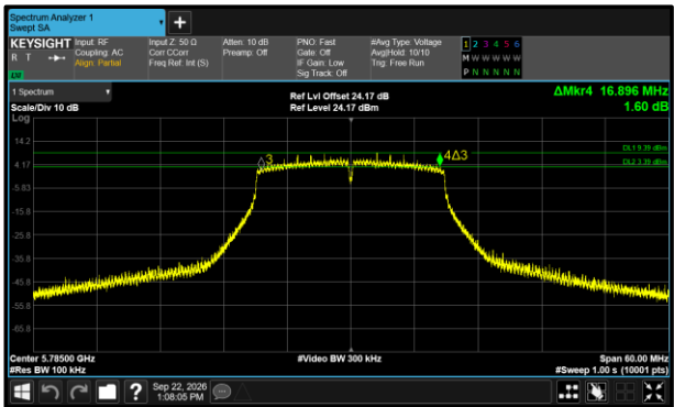
Figure 414 - 802.11n HT20 Maximum 6 dB EBW
