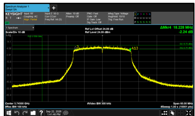
Figure 420 - 802.11ax HE20 SU Maximum 6 dB EBW
