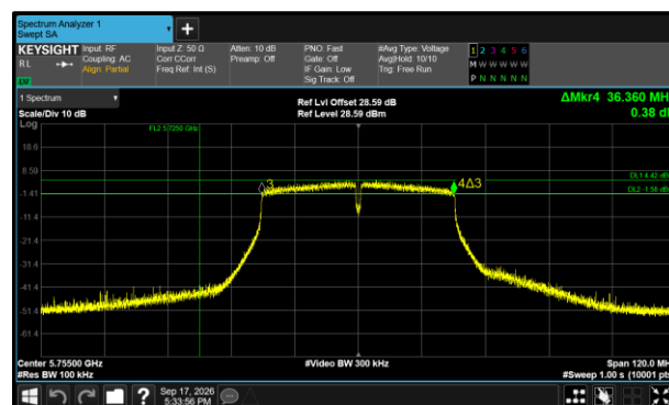
Figure 428 - 802.11n HT40 Maximum 6 dB EBW
