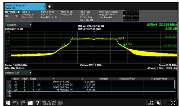
Figure 406 - 802.11a20 Maximum 99% OBW
