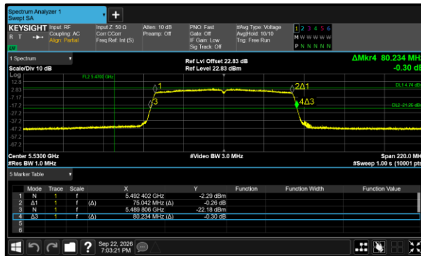
Figure 377 - 802.11ac VHT80 Minimum 99% OBW
