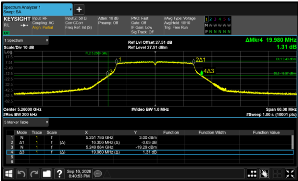
Figure 365 - 802.11a20 Minimum 99% OBW
