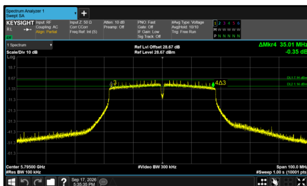
Figure 427 - 802.11n HT40 Minimum 6 dB EBW
