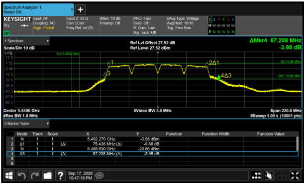
Figure 369 - 802.11a80 Minimum 99% OBW
