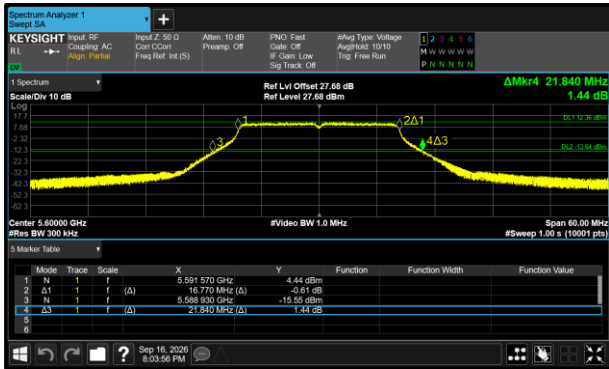
Figure 366 - 802.11a20 Maximum 99% OBW
