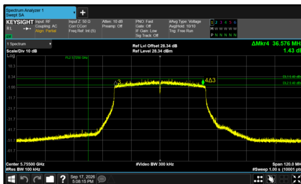
Figure 433 - 802.11ax HE40 SU Minimum 6 dB EBW
