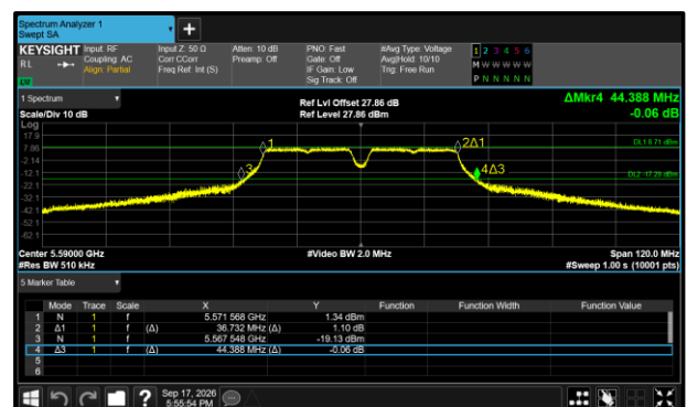
Figure 408 - 802.11a40 Maximum 99% OBW
