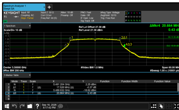
Figure 349 - 802.11n HT20 Minimum 99% OBW
