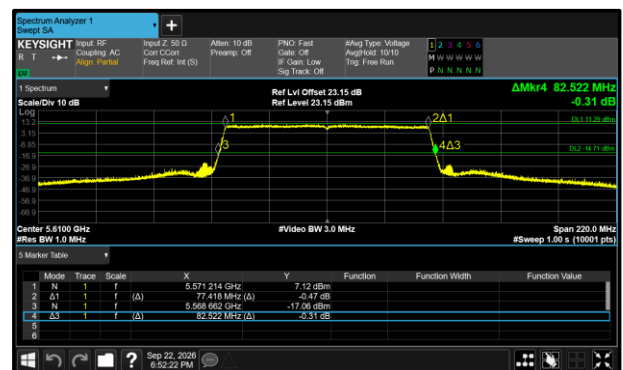
Figure 386 - 802.11ax HE80 SU Maximum 99% OBW
