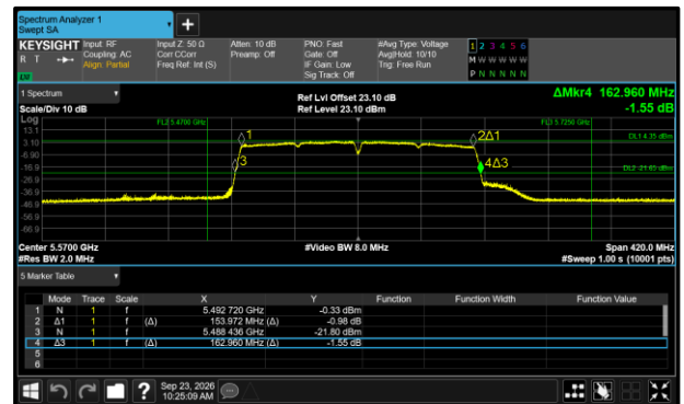
Figure 380 - 802.11ac VHT160 Maximum 99% OBW
