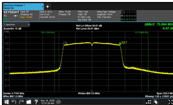
Figure 393 - 802.11ac VHT80 Minimum 99% OBW
