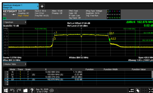
Figure 395 - 802.11ac VHT160 Minimum 99% OBW
