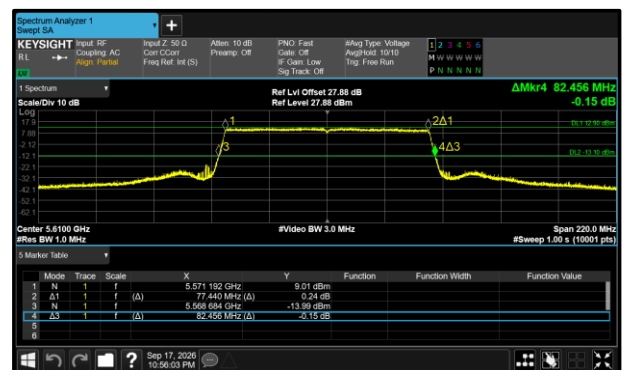
Figure 362 - 802.11ax HE80 SU Maximum 99% OBW
