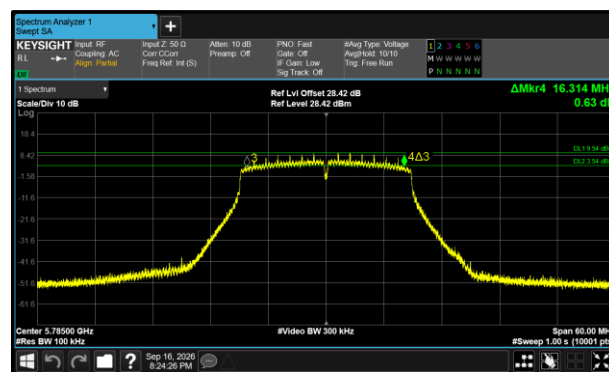
Figure 426 - 802.11n HT20 Maximum 6 dB EBW
