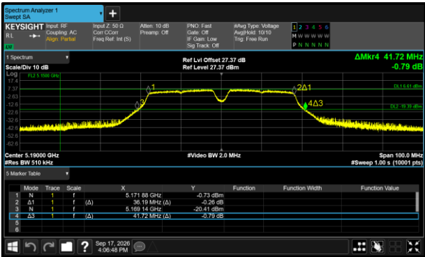
Figure 367 - 802.11a40 Minimum 99% OBW
