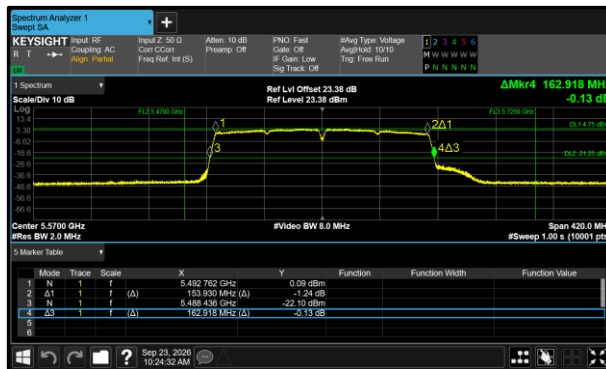
Figure 379 - 802.11ac VHT160 Minimum 99% OBW
