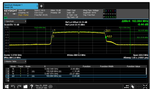
Figure 388 - 802.11ax HE160 SU Maximum 99% OBW
