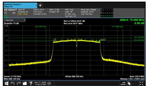
Figure 430 - 802.11ac VHT80 Maximum 6 dB EBW
