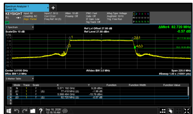
Figure 402 - 802.11ax HE80 SU Maximum 99% OBW
