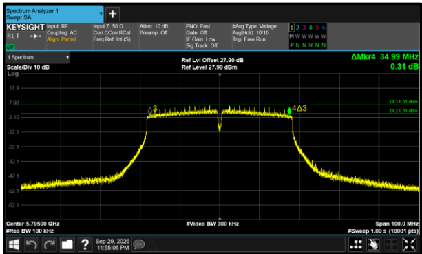
Figure 415 - 802.11n HT40 Minimum 6 dB EBW
