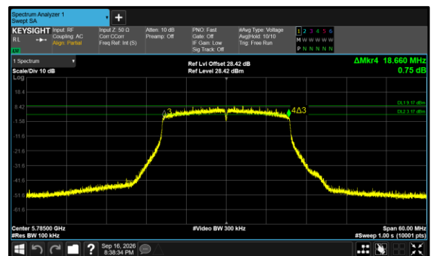
Figure 432 - 802.11ax HE20 SU Maximum 6 dB EBW
