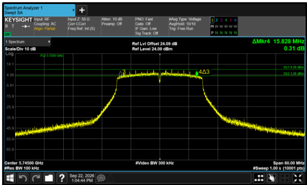
Figure 413 - 802.11n HT20 Minimum 6 dB EBW
