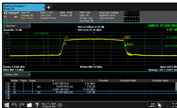
Figure 361 - 802.11ax HE80 SU Minimum 99% OBW
