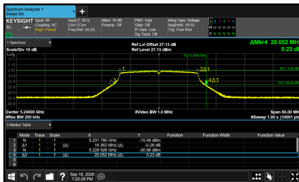
Figure 405 - 802.11a20 Minimum 99% OBW
