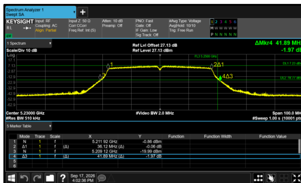
Figure 351 - 802.11n HT40 Minimum 99% OBW
