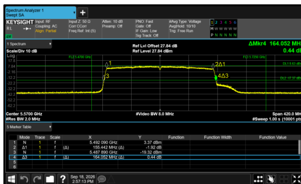
Figure 363 - 802.11ax HE160 SU Minimum 99% OBW
