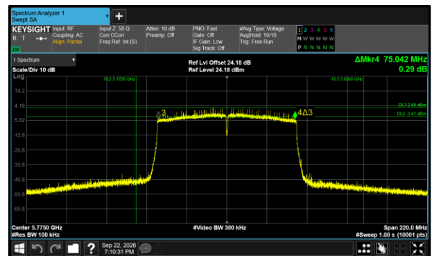
Figure 418 - 802.11ac VHT80 Maximum 6 dB EBW
