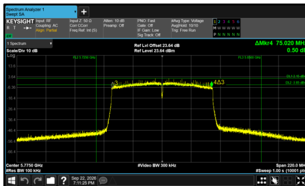
Figure 417 - 802.11ac VHT80 Minimum 6 dB EBW
