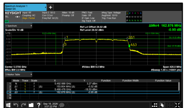
Figure 356 - 802.11ac VHT160 Maximum 99% OBW
