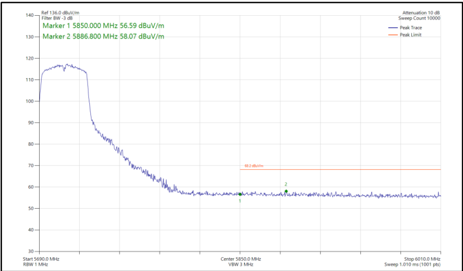
Figure 595 - 802.11n HT40, SISO, Core 0 - 5710 MHz Band Edge Frequency 5850 MHz
