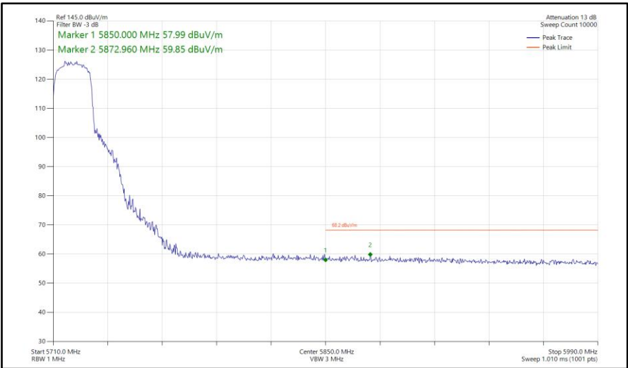
Figure 576 - 802.11ax HE20, SU, TxBF, Core 0-1 - 5720 MHz Band Edge Frequency 5850 MHz
