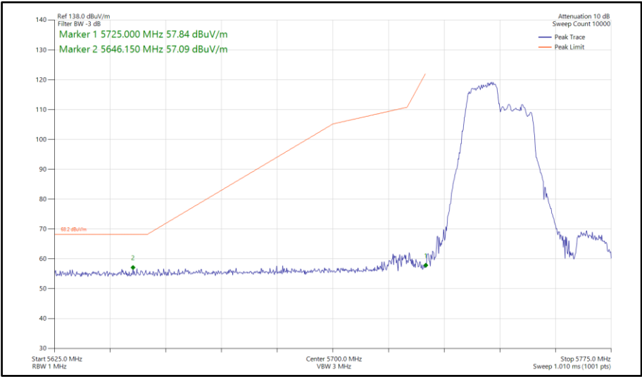
Figure 611 - 802.11ax HE40, RU106-53, SISO, Core 1 - 5755 MHz Band Edge Frequency 5725 MHz
