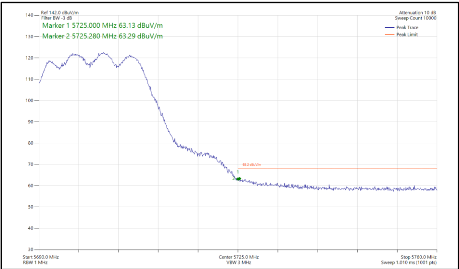
Figure 534 - 802.11n HT20, CDD, Core 0-1 - 5700 MHz Band Edge Frequency 5725 MHz
