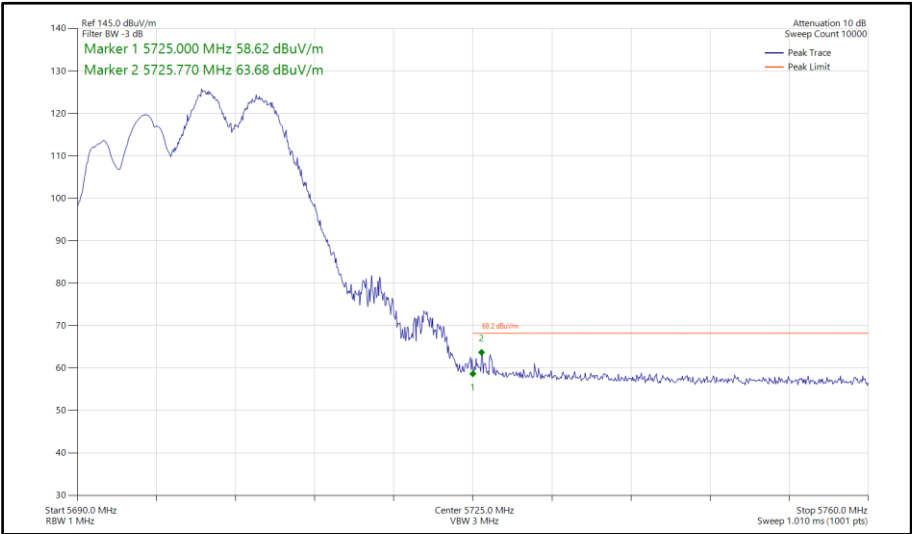
Figure 537 - 802.11be EHT20, RU106+26-83, CDD, Core 0-1 - 5700 MHz Band Edge Frequency 5725 MHz
