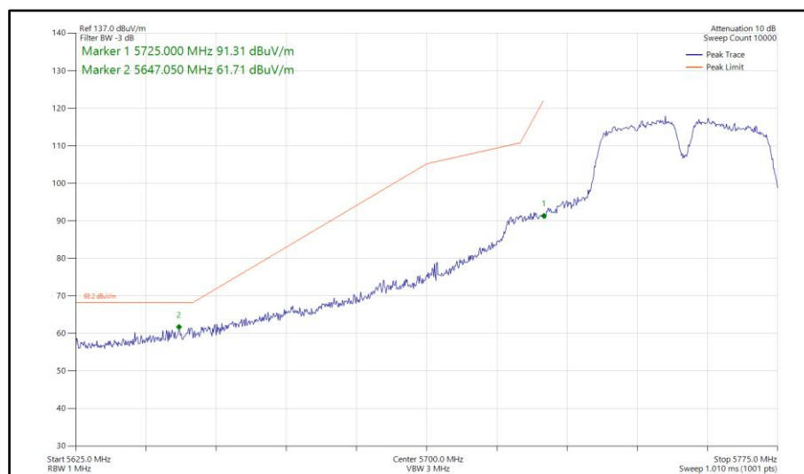
Figure 608 - 802.11a a40, SISO, Core 1 - 5755 MHz Band Edge Frequency 5725 MHz
