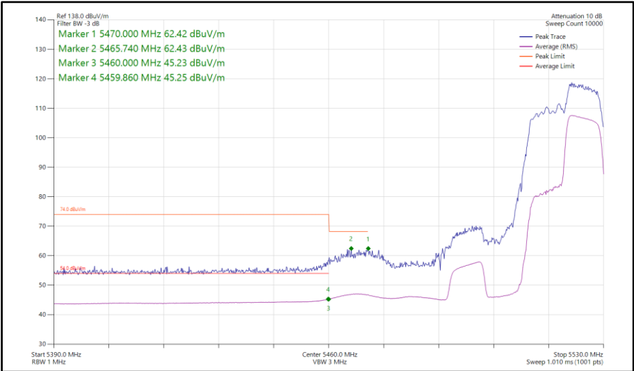
Figure 606 - 802.11ax HE40, RU106-56, SISO, Core 1 - 5510 MHz Band Edge Frequency 5470 MHz
