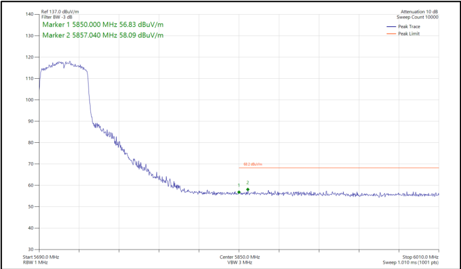
Figure 597 - 802.11ax HE40, SU, SISO, Core 0 - 5710 MHz Band Edge Frequency 5850 MHz
