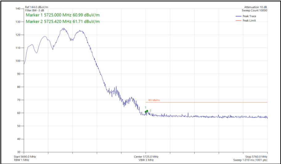
Figure 559 - 802.11be EHT20, RU106+26-83, SDM, Core 0-1 - 5700 MHz Band Edge Frequency 5725 MHz
