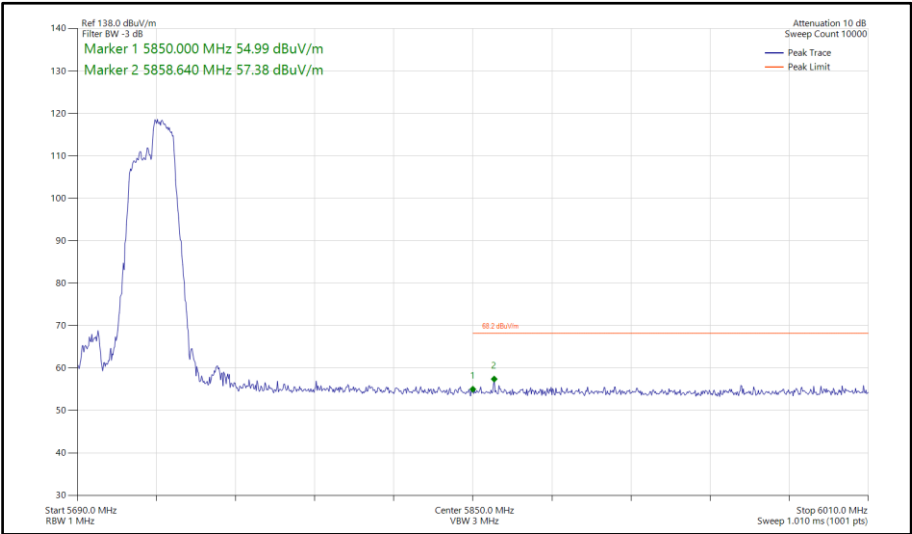
Figure 598 - 802.11ax HE40, RU106-56, SISO, Core 0 - 5710 MHz Band Edge Frequency 5850 MHz
