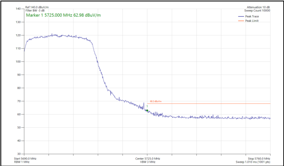
Figure 557 - 802.11ax HE20, SU, SDM, Core 0-1 - 5700 MHz Band Edge Frequency 5725 MHz
