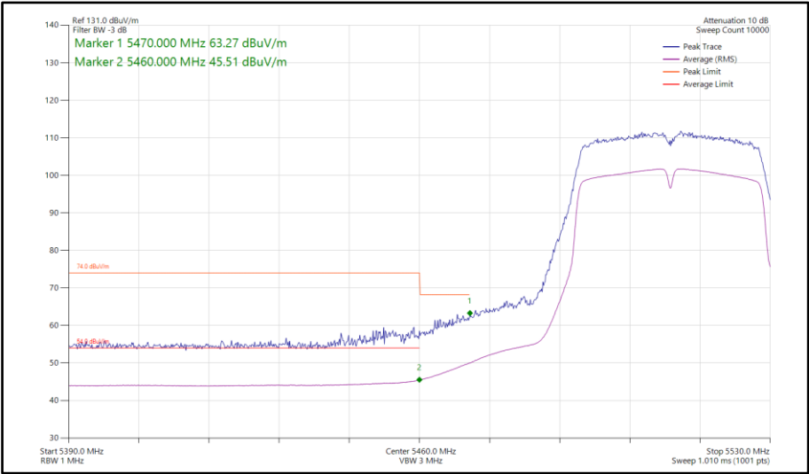
Figure 604 - 802.11n HT40, SISO, Core 1 - 5510 MHz Band Edge Frequency 5470 MHz
