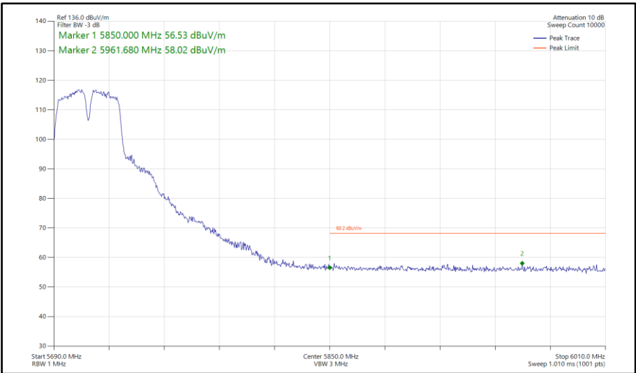
Figure 593 - 802.11a a40, SISO, Core 0 - 5710 MHz Band Edge Frequency 5850 MHz
