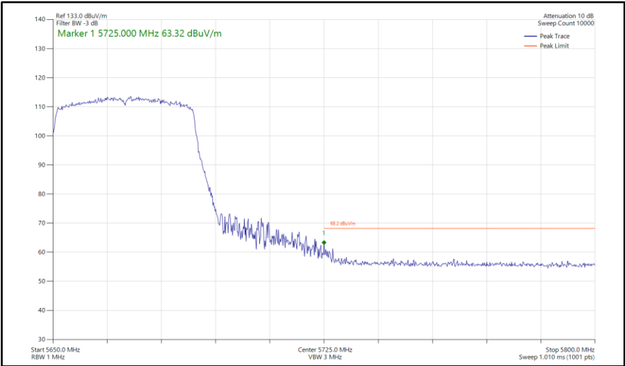
Figure 590 - 802.11ax HE40, SU, SISO, Core 0 - 5670 MHz Band Edge Frequency 5725 MHz
