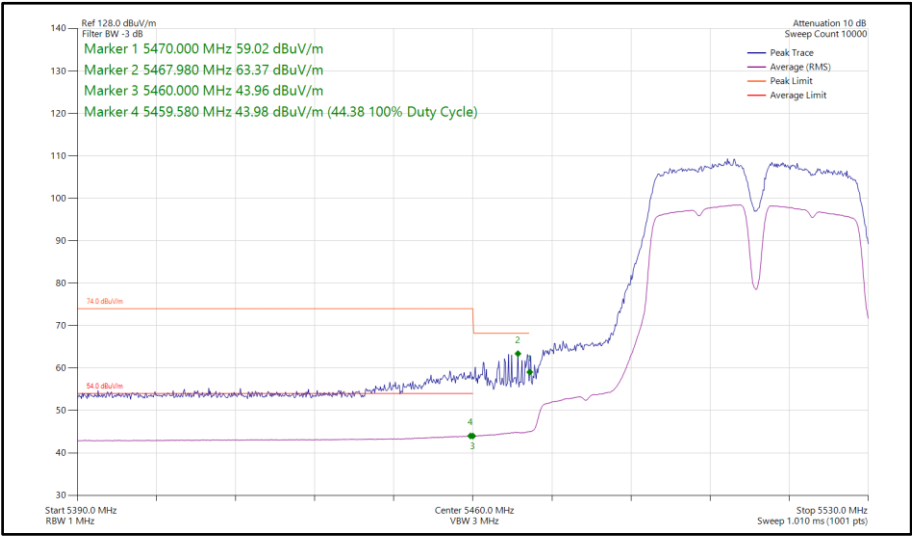
Figure 603 - 802.11a a40, SISO, Core 1 - 5510 MHz Band Edge Frequency 5470 MHz
