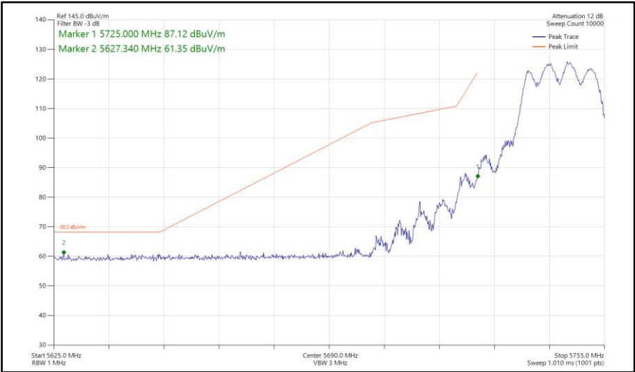
Figure 529 - 802.11n HT20, CDD, Core 0-1 - 5745 MHz Band Edge Frequency 5725 MHz
