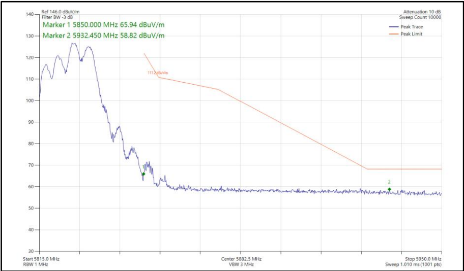
Figure 547 - 802.11be EHT20, RU106+26-83, CDD, Core 0-1 - 5825 MHz Band Edge Frequency 5850 MHz
