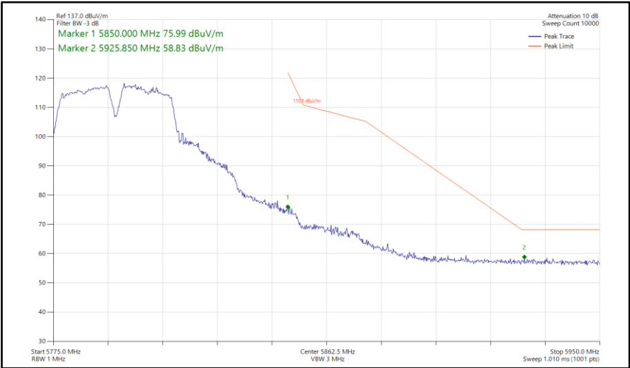
Figure 594 - 802.11a a40, SISO, Core 0 - 5795 MHz Band Edge Frequency 5850 MHz
