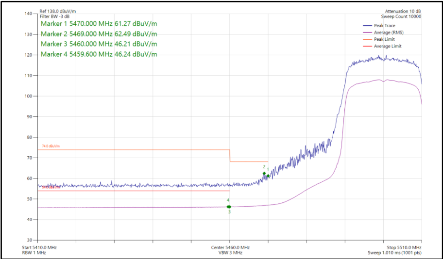
Figure 549 - 802.11ax HE20, SU, SDM, Core 0-1 - 5500 MHz Band Edge Frequency 5470 MHz
