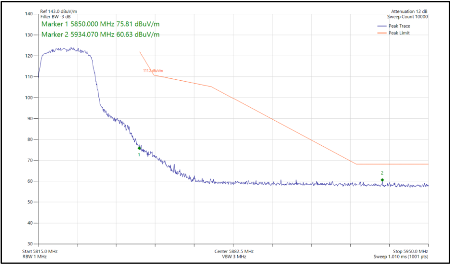
Figure 561 - 802.11n HT20, SDM, Core 0-1 - 5825 MHz Band Edge Frequency 5850 MHz
