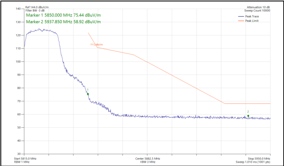
Figure 575 - 802.11ac VHT20, TxBF, Core 0-1 - 5825 MHz Band Edge Frequency 5850 MHz
