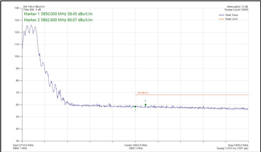
Figure 538 - 802.11a, CDD, Core 0-1 - 5720 MHz Band Edge Frequency 5850 MHz
