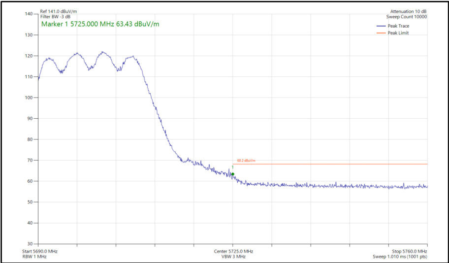
Figure 535 - 802.11ax HE20, SU, CDD, Core 0-1 - 5700 MHz Band Edge Frequency 5725 MHz
