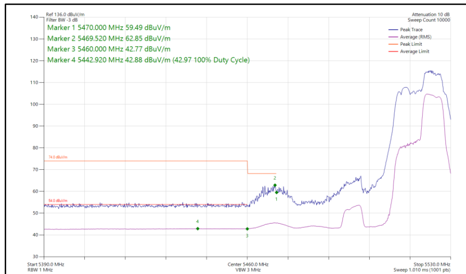
Figure 607 - 802.11be EHT40, RU52+26-75, SISO, Core 1 - 5510 MHz Band Edge Frequency 5470 MHz
