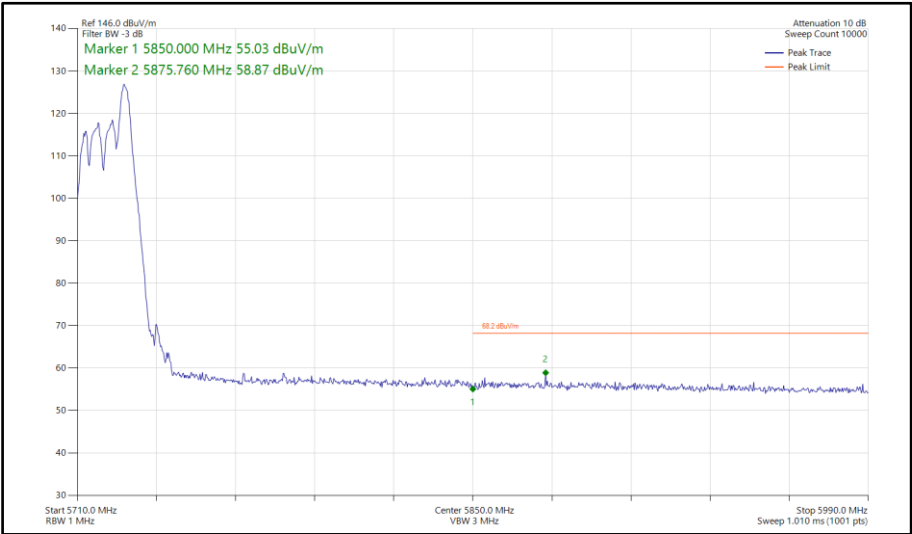
Figure 563 - 802.11ax HE20, RU52-40, SDM, Core 0-1 - 5720 MHz Band Edge Frequency 5850 MHz
