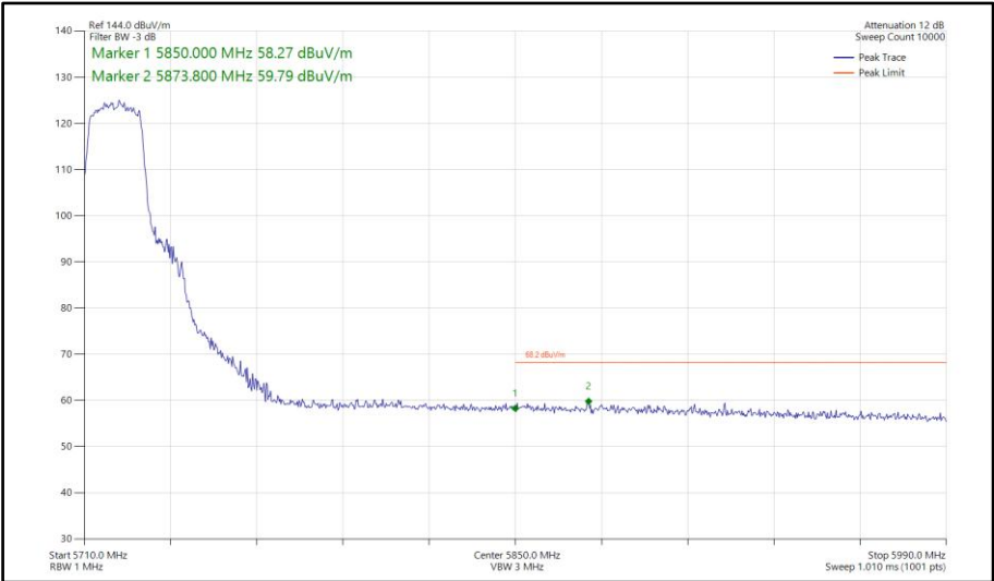
Figure 560 - 802.11n HT20, SDM, Core 0-1 - 5720 MHz Band Edge Frequency 5850 MHz
