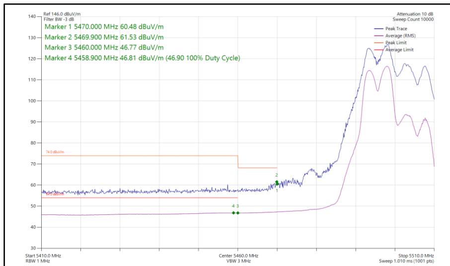
Figure 551 - 802.11be EHT20, RU52+26-70, SDM, Core 0-1 - 5500 MHz Band Edge Frequency 5470 MHz
