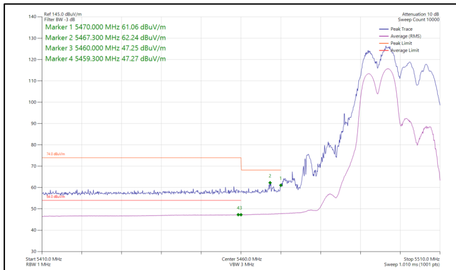
Figure 526 - 802.11ax HE20, RU106-53, CDD, Core 0-1 - 5500 MHz Band Edge Frequency 5470 MHz
