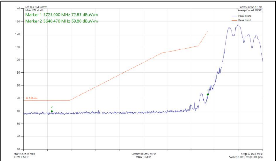
Figure 531 - 802.11ax HE20, RU106-53, CDD, Core 0-1 - 5745 MHz Band Edge Frequency 5725 MHz
