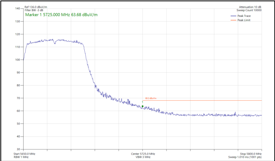
Figure 589 - 802.11n HT40, SISO, Core 0 - 5670 MHz Band Edge Frequency 5725 MHz
