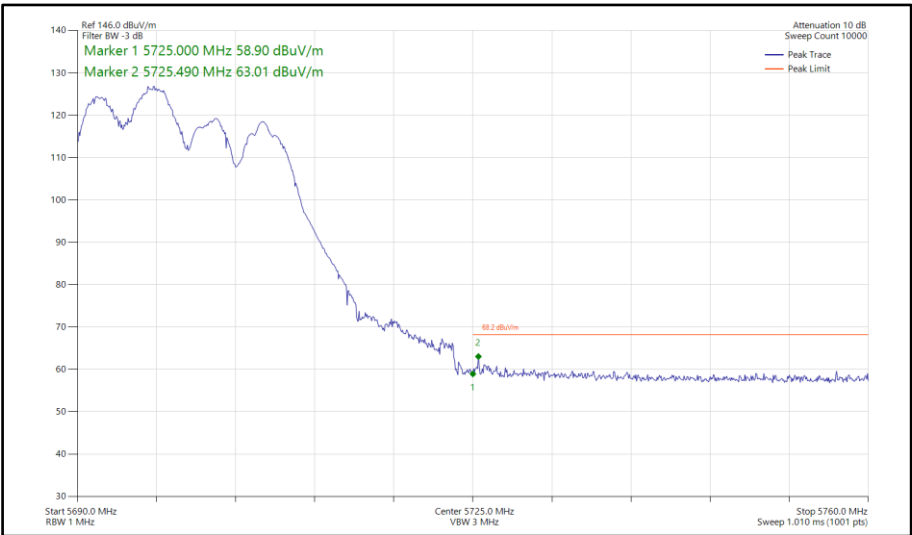
Figure 536 - 802.11ax HE20, RU106-53, CDD, Core 0-1 - 5700 MHz Band Edge Frequency 5725 MHz
