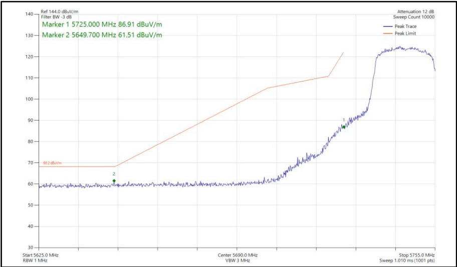
Figure 553 - 802.11ax HE20, SU, SDM, Core 0-1 - 5745 MHz Band Edge Frequency 5725 MHz
