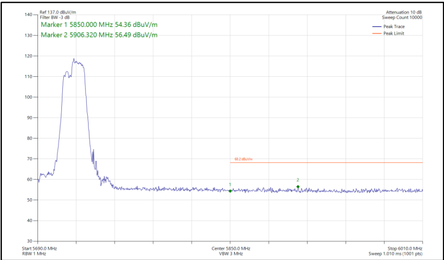
Figure 601 - 802.11be EHT40, RU106+26-85, SISO, Core 0 - 5710 MHz Band Edge Frequency 5850 MHz
