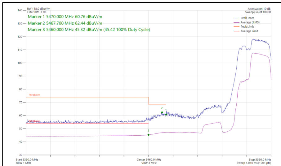
Figure 582 - 802.11be EHT40, RU106+26-85, SISO, Core 0 - 5510 MHz Band Edge Frequency 5470 MHz
