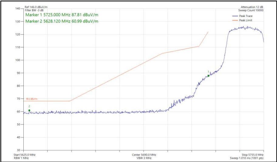
Figure 571 - 802.11ax HE20, SU, TxBF, Core 0-1 - 5745 MHz Band Edge Frequency 5725 MHz
