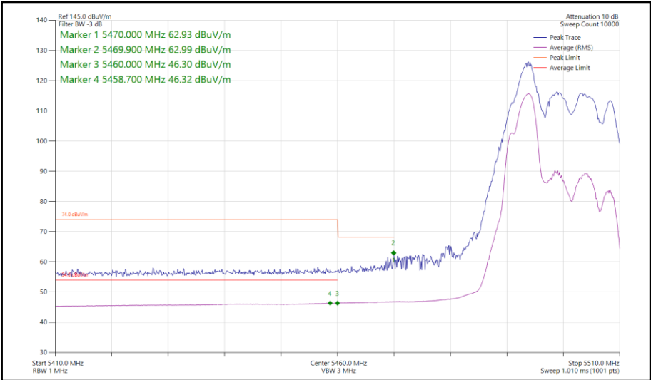
Figure 550 - 802.11ax HE20, RU52-37, SDM, Core 0-1 - 5500 MHz Band Edge Frequency 5470 MHz
