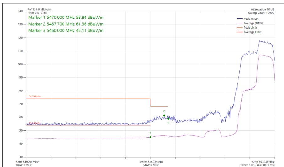
Figure 581 - 802.11ax HE40, RU106-56, SISO, Core 0 - 5510 MHz Band Edge Frequency 5470 MHz
