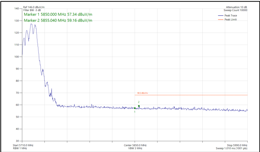
Figure 546 - 802.11be EHT20, RU106+26-83, CDD, Core 0-1 - 5720 MHz Band Edge Frequency 5850 MHz
