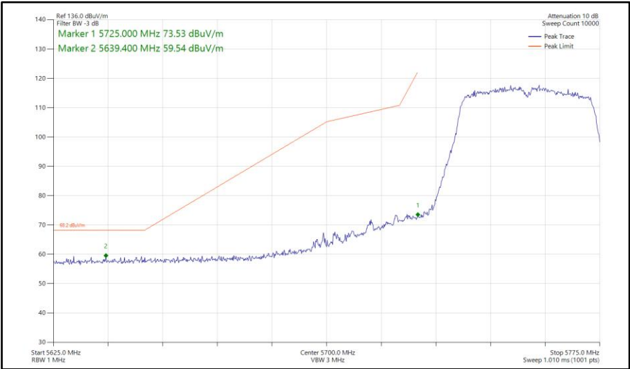
Figure 609 - 802.11n HT40, SISO, Core 1 - 5755 MHz Band Edge Frequency 5725 MHz
