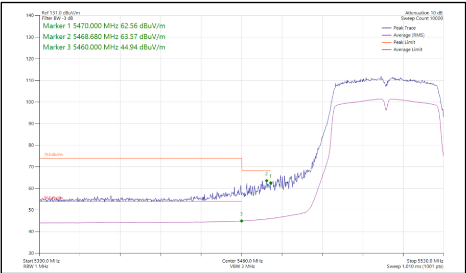
Figure 579 - 802.11n HT40, SISO, Core 0 - 5510 MHz Band Edge Frequency 5470 MHz
