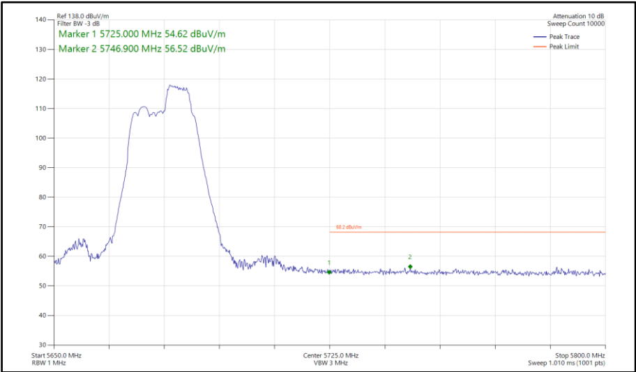
Figure 592 - 802.11be EHT40, RU52+26-75, SISO, Core 0 - 5670 MHz Band Edge Frequency 5725 MHz
