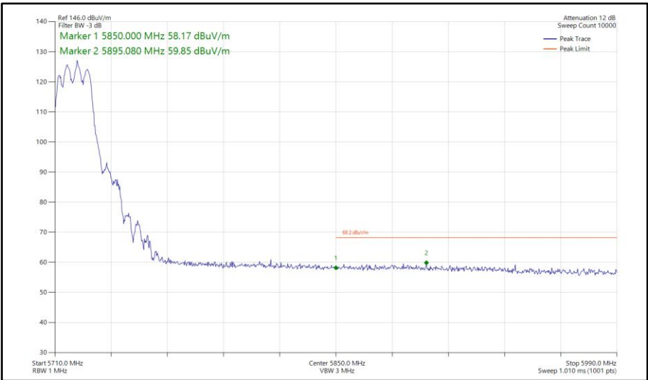
Figure 540 - 802.11n HT20, CDD, Core 0-1 - 5720 MHz Band Edge Frequency 5850 MHz
