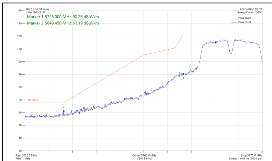
Figure 583 - 802.11a a40, SISO, Core 0 - 5755 MHz Band Edge Frequency 5725 MHz
