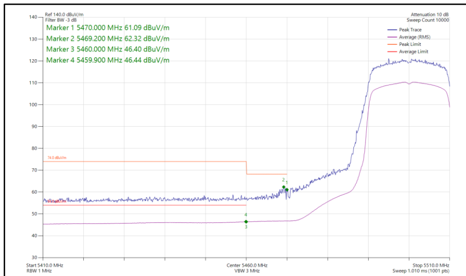
Figure 569 - 802.11ax HE20, SU, TxBF, Core 0-1 - 5500 MHz Band Edge Frequency 5470 MHz
