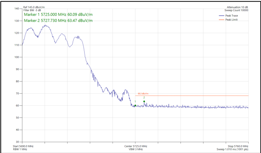
Figure 558 - 802.11ax HE20, RU106-53, SDM, Core 0-1 - 5700 MHz Band Edge Frequency 5725 MHz
