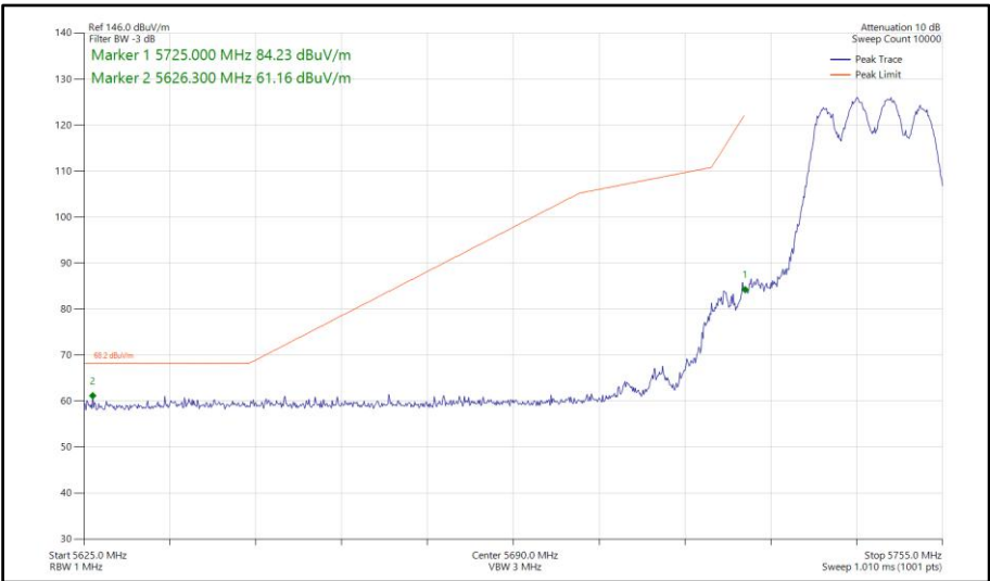
Figure 530 - 802.11ax HE20, SU, CDD, Core 0-1 - 5745 MHz Band Edge Frequency 5725 MHz
