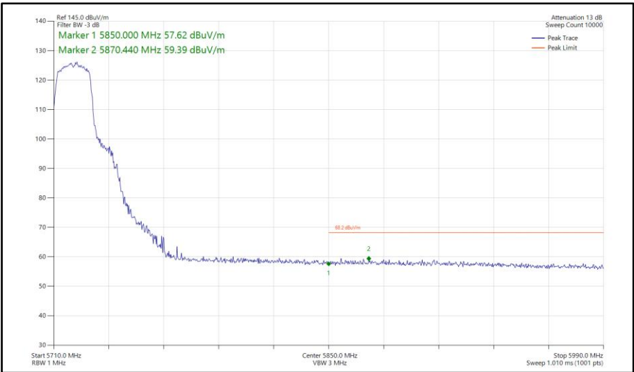
Figure 574 - 802.11ac VHT20, TxBF, Core 0-1 - 5720 MHz Band Edge Frequency 5850 MHz
