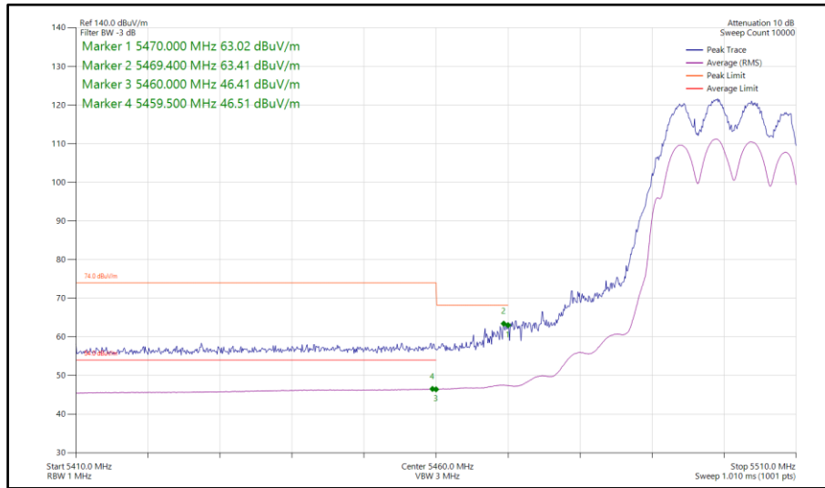
Figure 525 - 802.11ax HE20, SU, CDD, Core 0-1 - 5500 MHz Band Edge Frequency 5470 MHz
