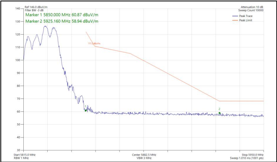
Figure 565 - 802.11ax HE20, RU106-54, SDM, Core 0-1 - 5825 MHz Band Edge Frequency 5850 MHz
