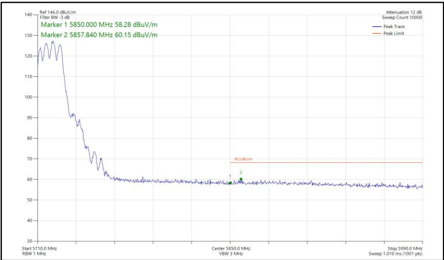
Figure 542 - 802.11ax HE20, SU, CDD, Core 0-1 - 5720 MHz Band Edge Frequency 5850 MHz
