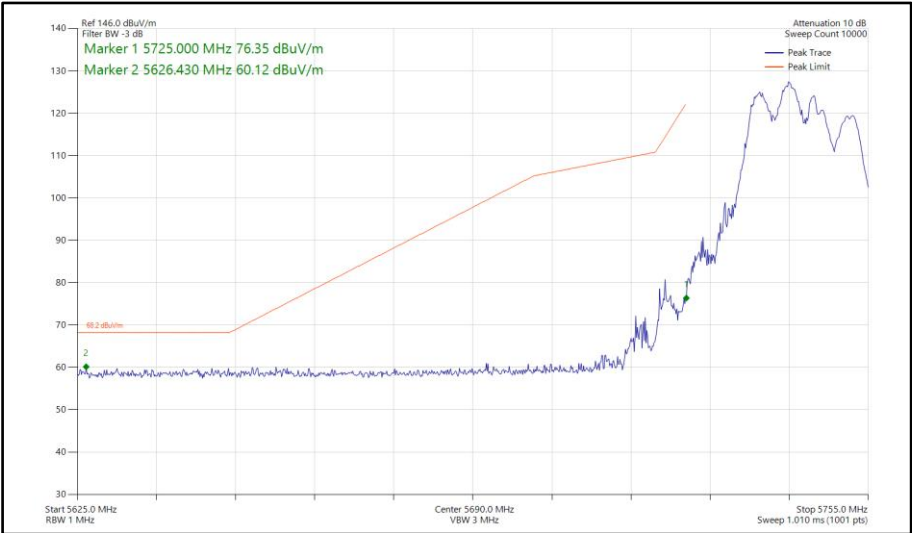
Figure 532 - 802.11be EHT20, RU106+26-82, CDD, Core 0-1 - 5745 MHz Band Edge Frequency 5725 MHz
