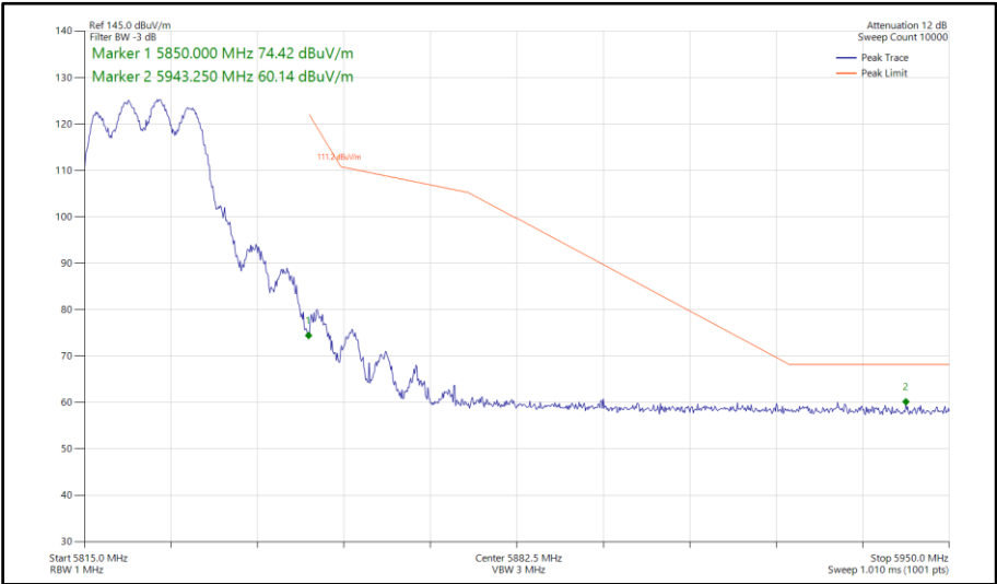
Figure 541 - 802.11n HT20, CDD, Core 0-1 - 5825 MHz Band Edge Frequency 5850 MHz
