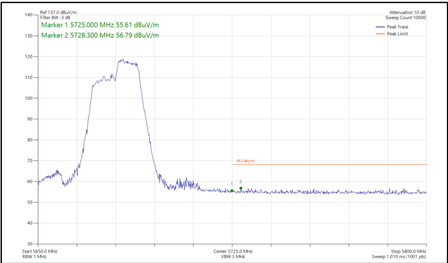
Figure 591 - 802.11ax HE40, RU106-56, SISO, Core 0 - 5670 MHz Band Edge Frequency 5725 MHz
