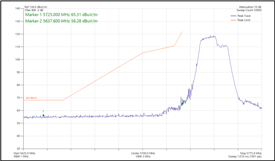
Figure 612 - 802.11be EHT40, RU106+26-82, SISO, Core 1 - 5755 MHz Band Edge Frequency 5725 MHz
