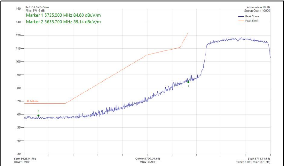
Figure 585 - 802.11ax HE40, SU, SISO, Core 0 - 5755 MHz Band Edge Frequency 5725 MHz
