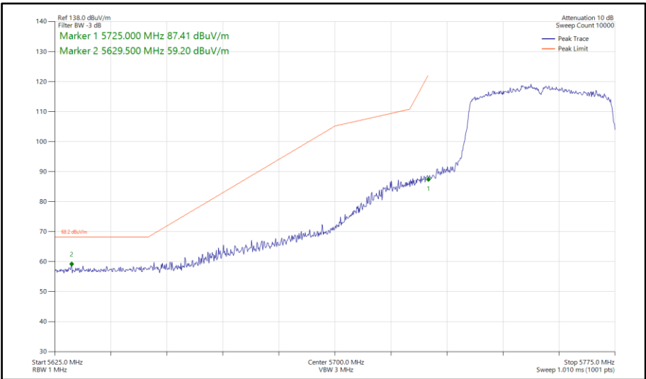
Figure 610 - 802.11ax HE40, SU, SISO, Core 1 - 5755 MHz Band Edge Frequency 5725 MHz
