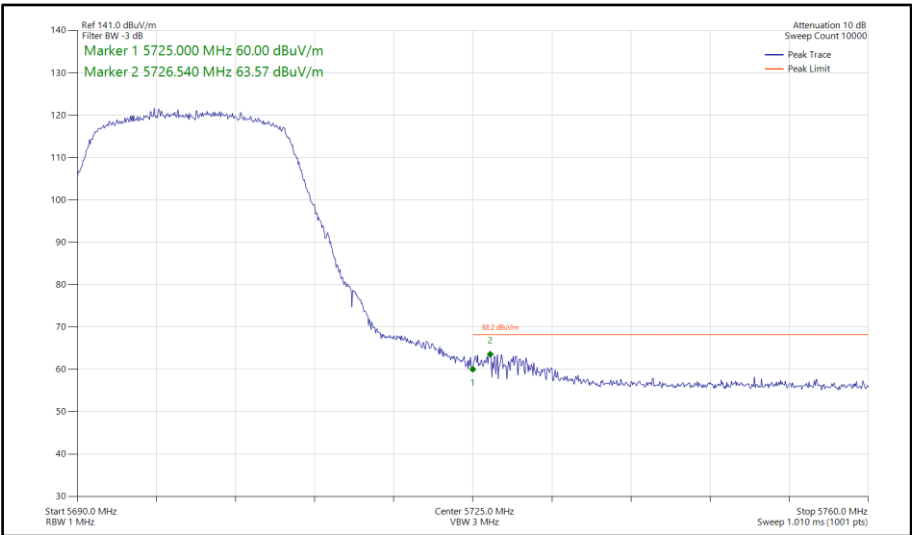
Figure 572 - 802.11ac VHT20, TxBF, Core 0-1 - 5700 MHz Band Edge Frequency 5725 MHz
