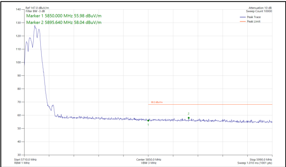
Figure 566 - 802.11be EHT20, RU52+26-72, SDM, Core 0-1 - 5720 MHz Band Edge Frequency 5850 MHz
