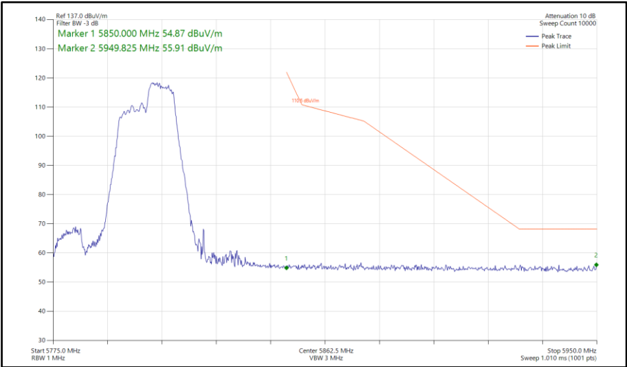
Figure 600 - 802.11ax HE40, RU106-56, SISO, Core 0 - 5795 MHz Band Edge Frequency 5850 MHz
