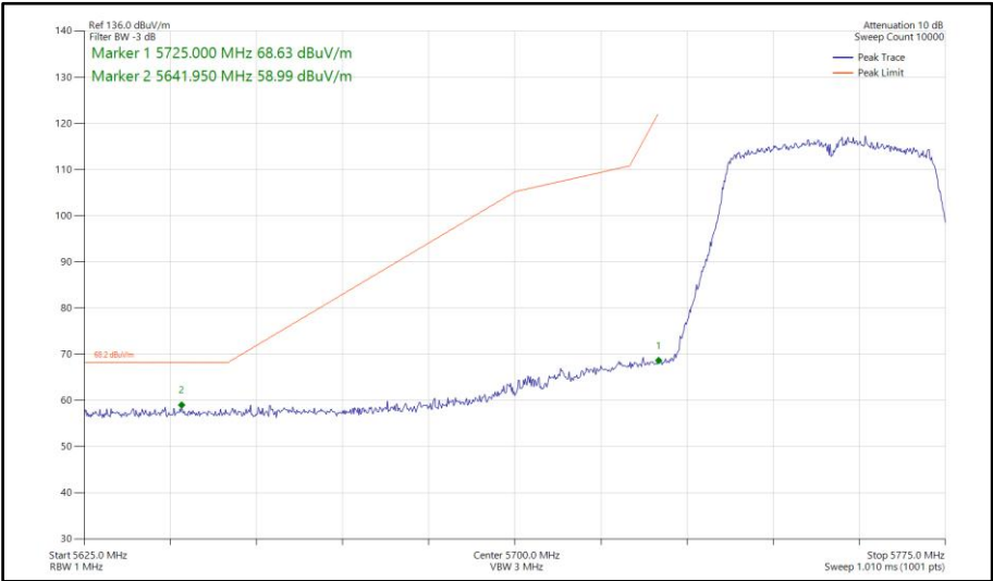
Figure 584 - 802.11n HT40, SISO, Core 0 - 5755 MHz Band Edge Frequency 5725 MHz
