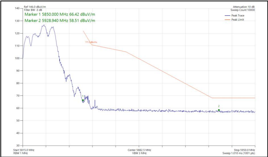
Figure 567 - 802.11be EHT20, RU106+26-83, SDM, Core 0-1 - 5825 MHz Band Edge Frequency 5850 MHz
