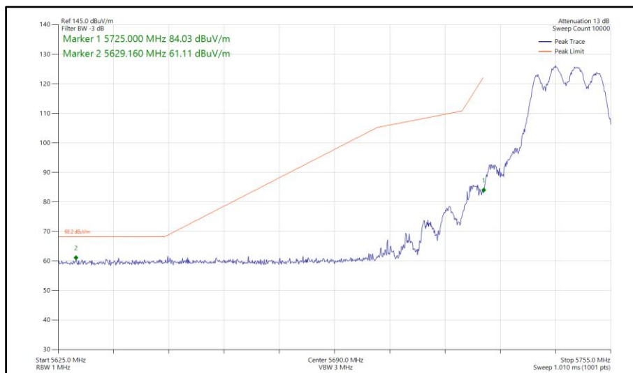
Figure 528 - 802.11a, CDD, Core 0-1 - 5745 MHz Band Edge Frequency 5725 MHz
