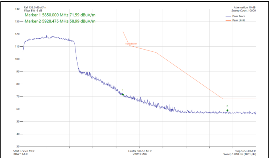
Figure 599 - 802.11ax HE40, SU, SISO, Core 0 - 5795 MHz Band Edge Frequency 5850 MHz
