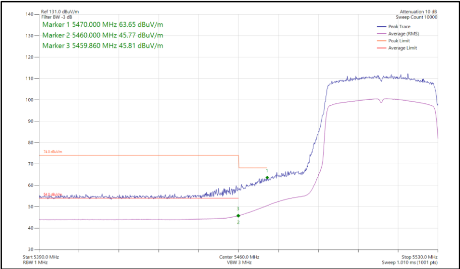
Figure 605 - 802.11ax HE40, SU, SISO, Core 1 - 5510 MHz Band Edge Frequency 5470 MHz
