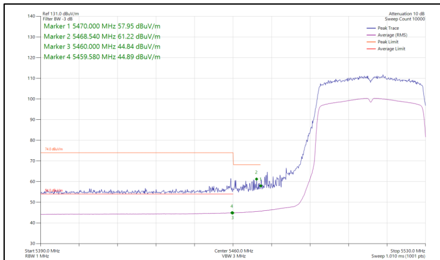
Figure 580 - 802.11ax HE40, SU, SISO, Core 0 - 5510 MHz Band Edge Frequency 5470 MHz
