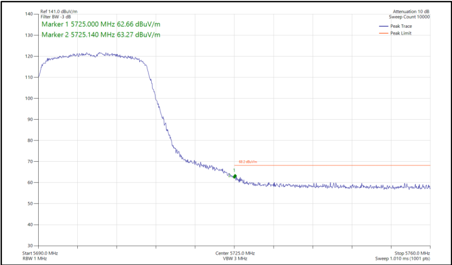
Figure 573 - 802.11ax HE20, SU, TxBF, Core 0-1 - 5700 MHz Band Edge Frequency 5725 MHz
