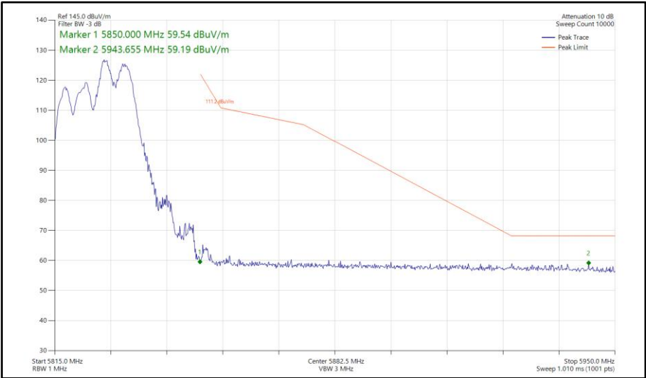
Figure 545 - 802.11ax HE20, RU106-54, CDD, Core 0-1 - 5825 MHz Band Edge Frequency 5850 MHz
