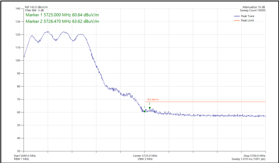
Figure 533 - 802.11a, CDD, Core 0-1 - 5700 MHz Band Edge Frequency 5725 MHz
