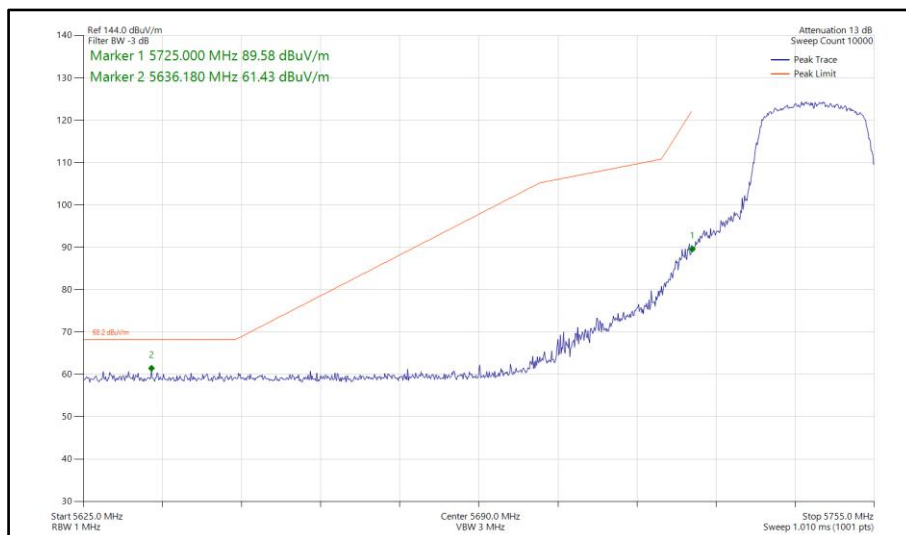
Figure 570 - 802.11ac VHT20, TxBF, Core 0-1 - 5745 MHz Band Edge Frequency 5725 MHz
