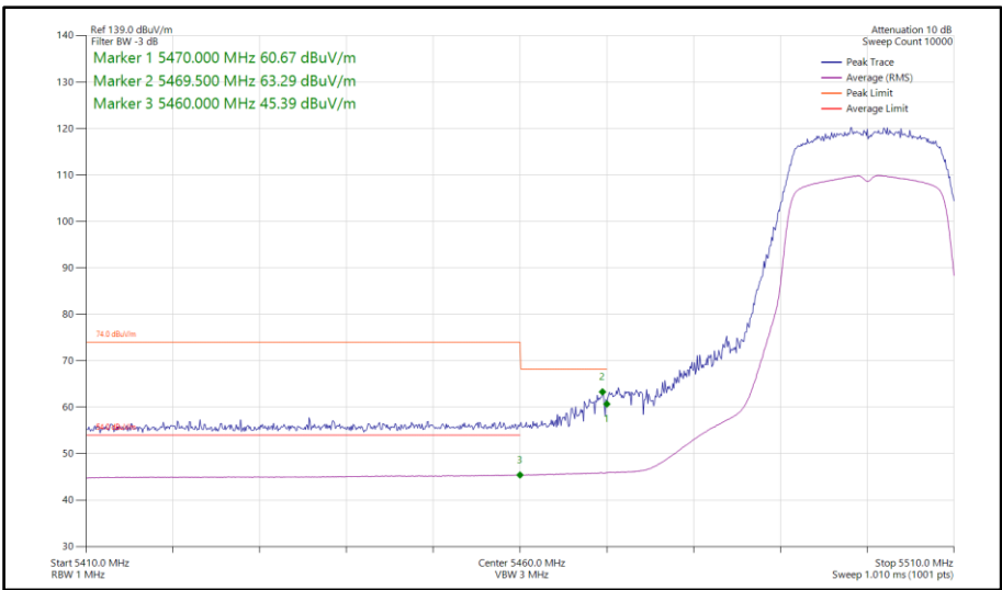
Figure 568 - 802.11ac VHT20, TxBF, Core 0-1 - 5500 MHz Band Edge Frequency 5470 MHz
