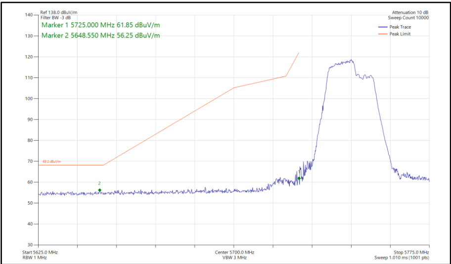
Figure 587 - 802.11be EHT40, RU106+26-82, SISO, Core 0 - 5755 MHz Band Edge Frequency 5725 MHz
