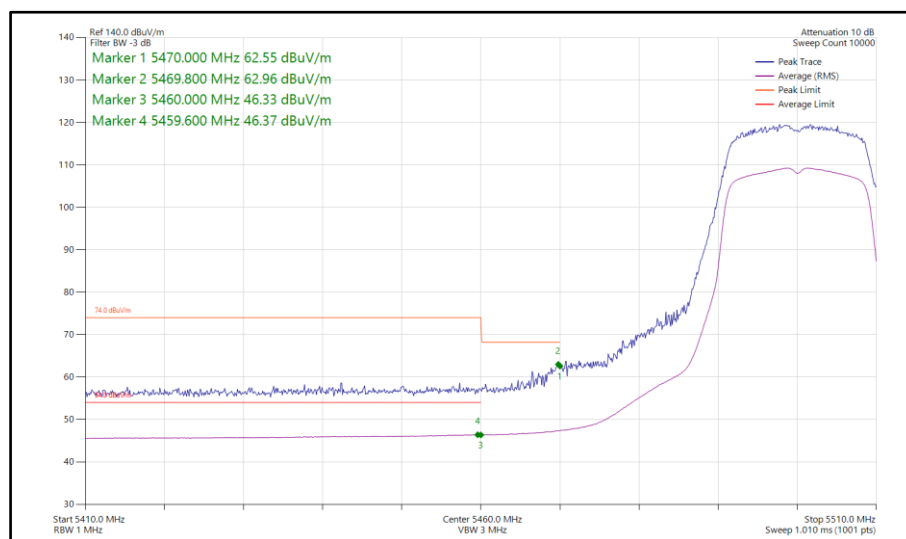
Figure 548 - 802.11n HT20, SDM, Core 0-1 - 5500 MHz Band Edge Frequency 5470 MHz
