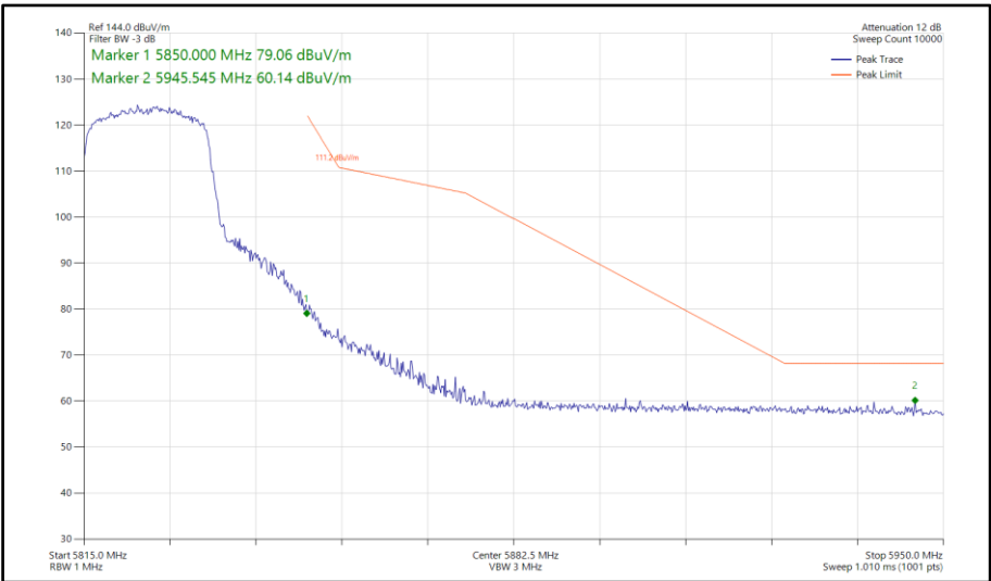
Figure 564 - 802.11ax HE20, SU, SDM, Core 0-1 - 5825 MHz Band Edge Frequency 5850 MHz
