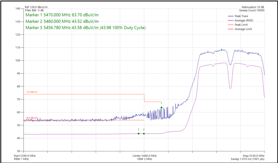
Figure 578 - 802.11a a40, SISO, Core 0 - 5510 MHz Band Edge Frequency 5470 MHz
