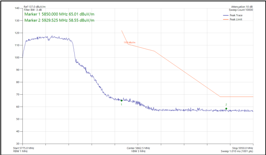
Figure 596 - 802.11n HT40, SISO, Core 0 - 5795 MHz Band Edge Frequency 5850 MHz
