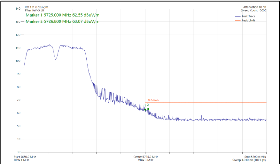
Figure 588 - 802.11a a40, SISO, Core 0 - 5670 MHz Band Edge Frequency 5725 MHz
