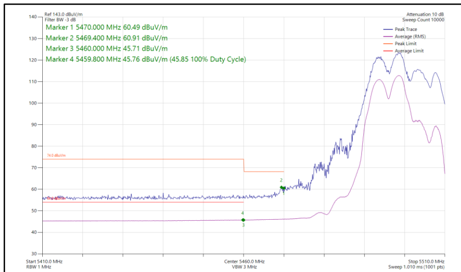
Figure 527 - 802.11be EHT20, RU106+26-82, CDD, Core 0-1 - 5500 MHz Band Edge Frequency 5470 MHz
