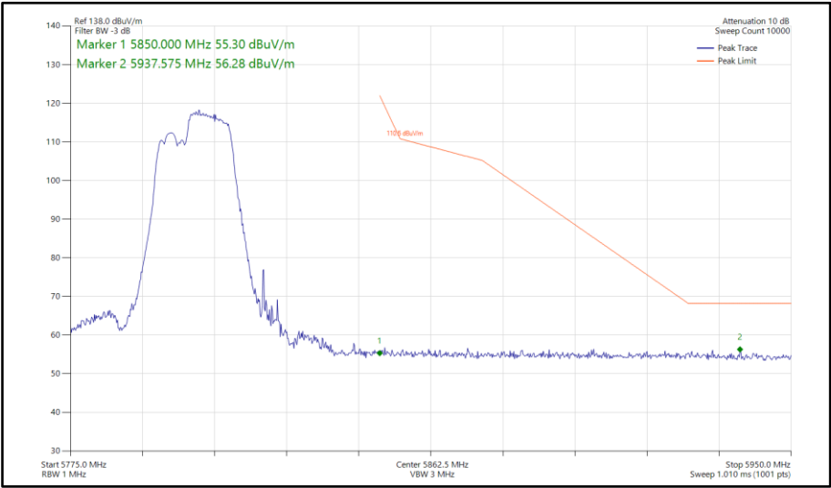
Figure 602 - 802.11be EHT40, RU106+26-85, SISO, Core 0 - 5795 MHz Band Edge Frequency 5850 MHz
