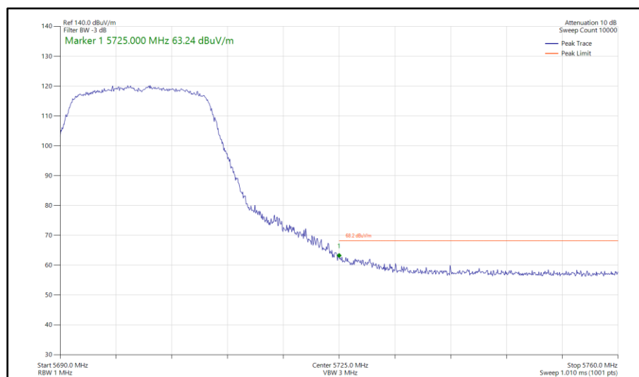
Figure 556 - 802.11n HT20, SDM, Core 0-1 - 5700 MHz Band Edge Frequency 5725 MHz
