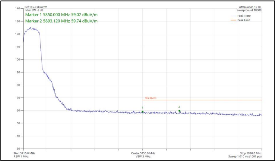
Figure 562 - 802.11ax HE20, SU, SDM, Core 0-1 - 5720 MHz Band Edge Frequency 5850 MHz
