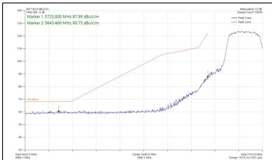
Figure 552 - 802.11n HT20, SDM, Core 0-1 - 5745 MHz Band Edge Frequency 5725 MHz
