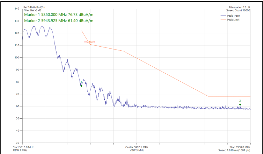
Figure 544 - 802.11ax HE20, SU, CDD, Core 0-1 - 5825 MHz Band Edge Frequency 5850 MHz
