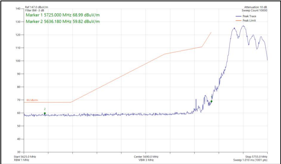
Figure 554 - 802.11ax HE20, RU106-53, SDM, Core 0-1 - 5745 MHz Band Edge Frequency 5725 MHz
