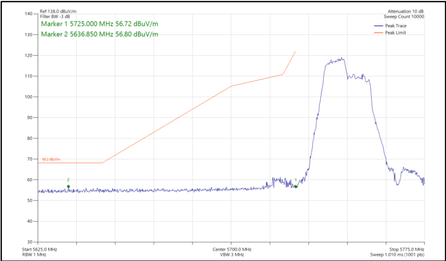
Figure 586 - 802.11ax HE40, RU106-53, SISO, Core 0 - 5755 MHz Band Edge Frequency 5725 MHz
