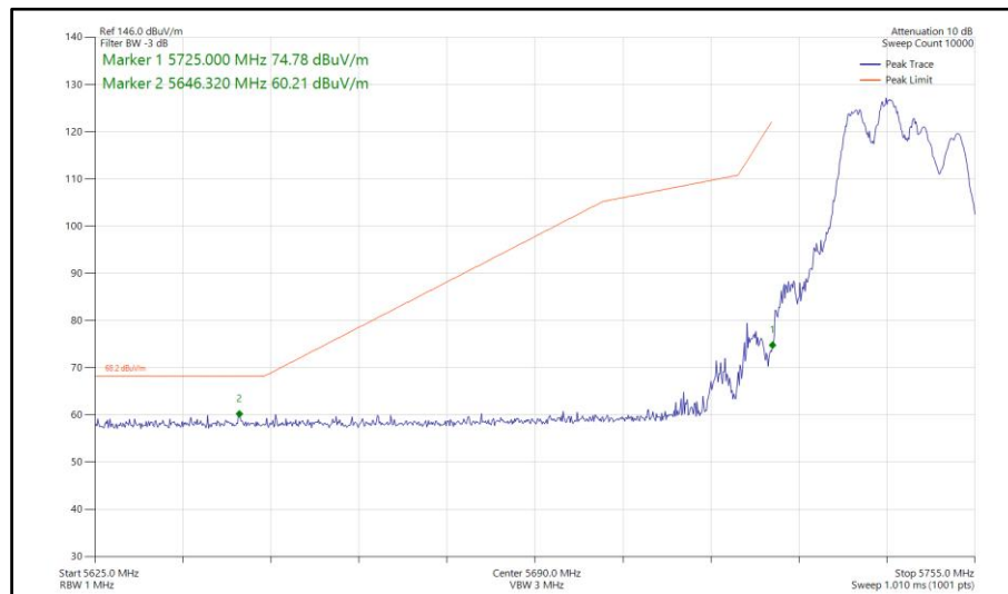
Figure 555 - 802.11be EHT20, RU106+26-82, SDM, Core 0-1 - 5745 MHz Band Edge Frequency 5725 MHz
