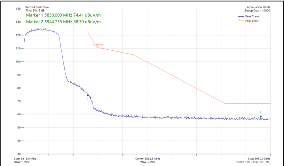
Figure 577 - 802.11ax HE20, SU, TxBF, Core 0-1 - 5825 MHz Band Edge Frequency 5850 MHz
