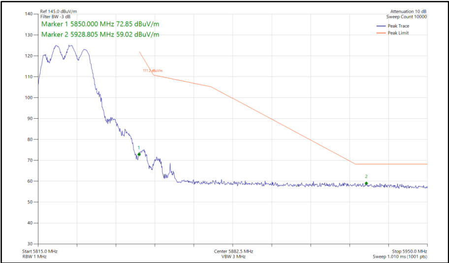
Figure 539 - 802.11a, CDD, Core 0-1 - 5825 MHz Band Edge Frequency 5850 MHz
