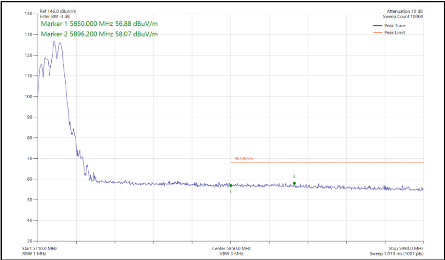
Figure 543 - 802.11ax HE20, RU106-54, CDD, Core 0-1 - 5720 MHz Band Edge Frequency 5850 MHz
