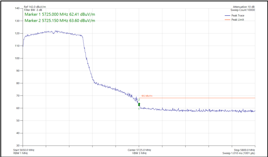
Figure 678 - 802.11ax HE40, SU, TxBF, Core 0-1 - 5670 MHz Band Edge Frequency 5725 MHz
