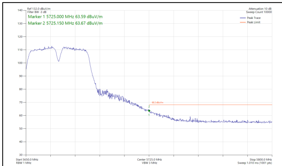
Figure 613 - 802.11a a40, SISO, Core 1 - 5670 MHz Band Edge Frequency 5725 MHz
