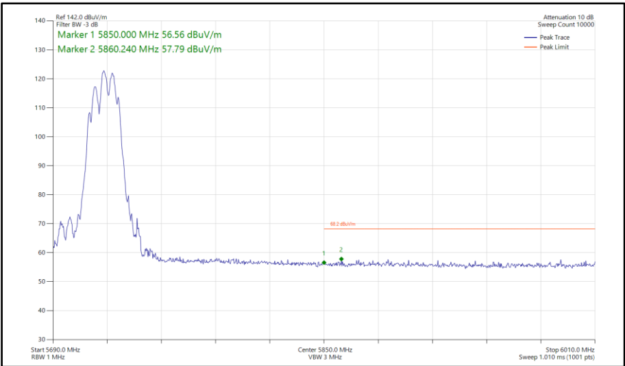
Figure 651 - 802.11be EHT40, RU106+26-85, CDD, Core 0-1 - 5710 MHz Band Edge Frequency 5850 MHz
