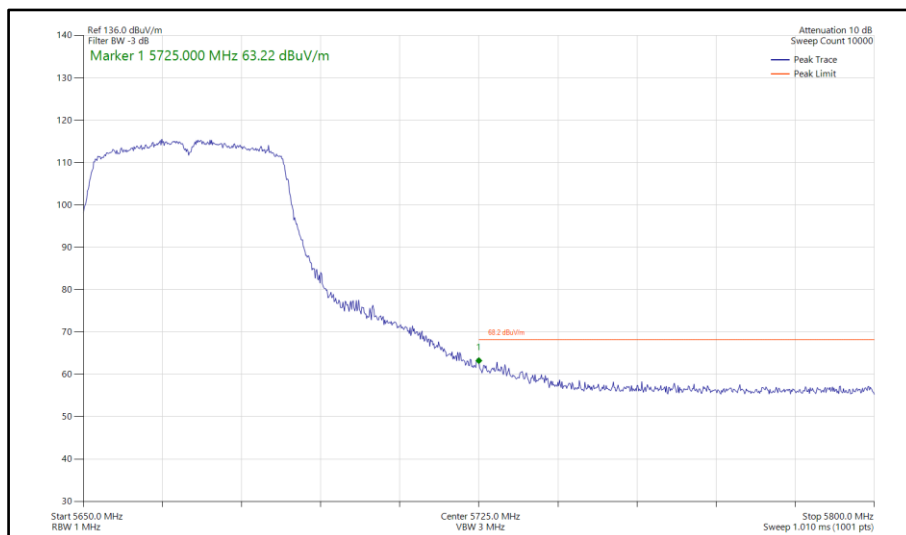
Figure 614 - 802.11n HT40, SISO, Core 1 - 5670 MHz Band Edge Frequency 5725 MHz
