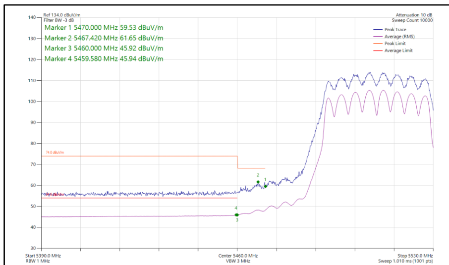
Figure 629 - 802.11n HT40, CDD, Core 0-1 - 5510 MHz Band Edge Frequency 5470 MHz
