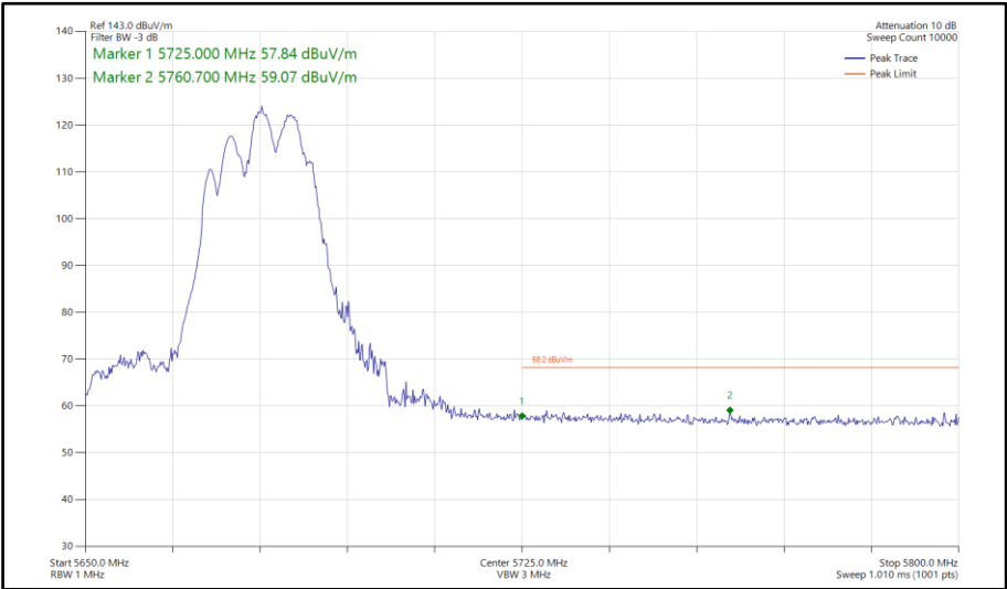
Figure 664 - 802.11be EHT40, RU106+26-85, SDM, Core 0-1 - 5670 MHz Band Edge Frequency 5725 MHz
