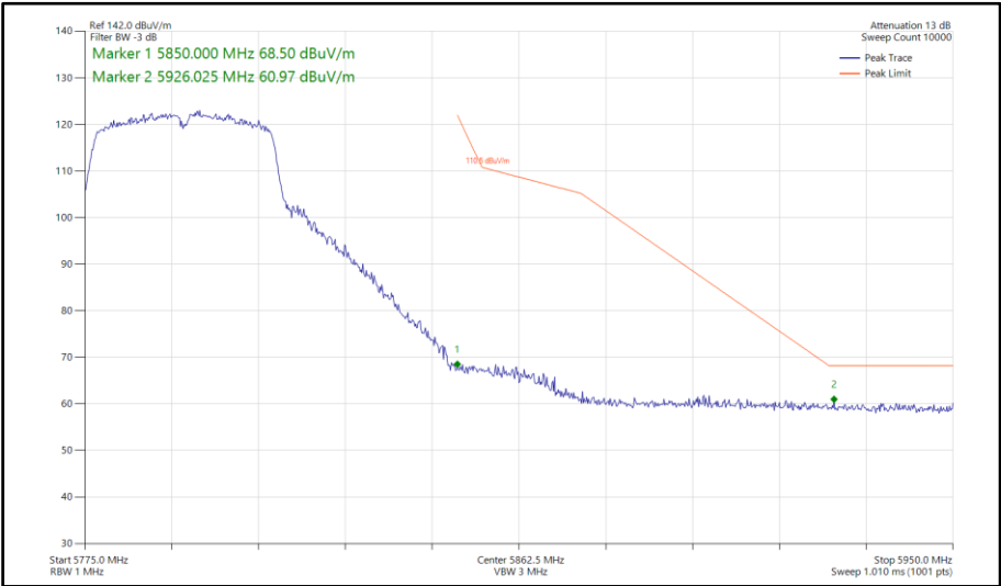
Figure 680 - 802.11ac VHT40, TxBF, Core 0-1 - 5795 MHz Band Edge Frequency 5850 MHz
