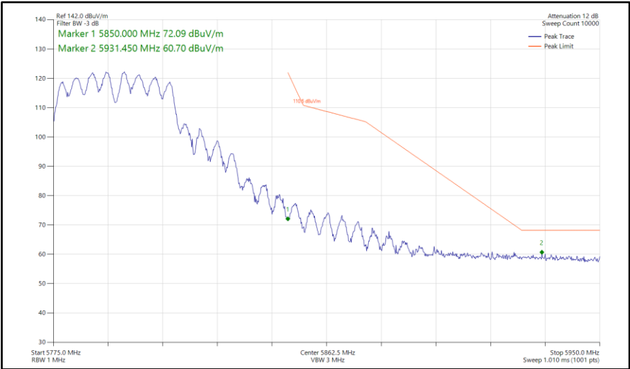
Figure 644 - 802.11a a40, CDD, Core 0-1 - 5795 MHz Band Edge Frequency 5850 MHz
