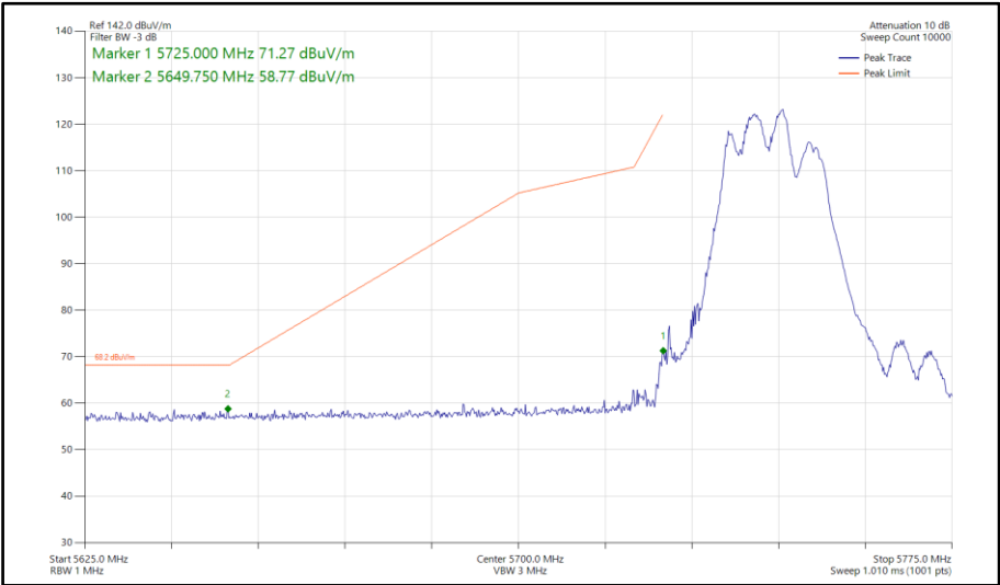
Figure 660 - 802.11be EHT40, RU106+26-82, SDM, Core 0-1 - 5755 MHz Band Edge Frequency 5725 MHz
