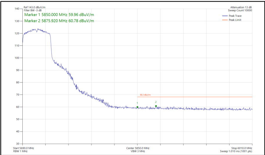
Figure 681 - 802.11ax HE40, SU, TxBF, Core 0-1 - 5710 MHz Band Edge Frequency 5850 MHz
