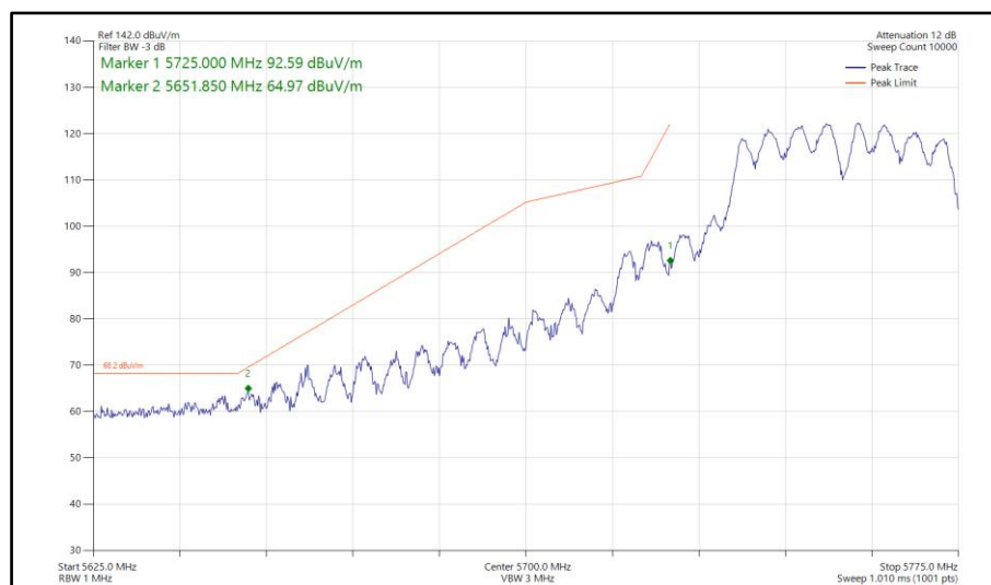
Figure 633 - 802.11a a40, CDD, Core 0-1 - 5755 MHz Band Edge Frequency 5725 MHz
