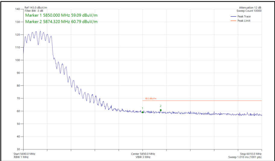
Figure 643 - 802.11a a40, CDD, Core 0-1 - 5710 MHz Band Edge Frequency 5850 MHz
