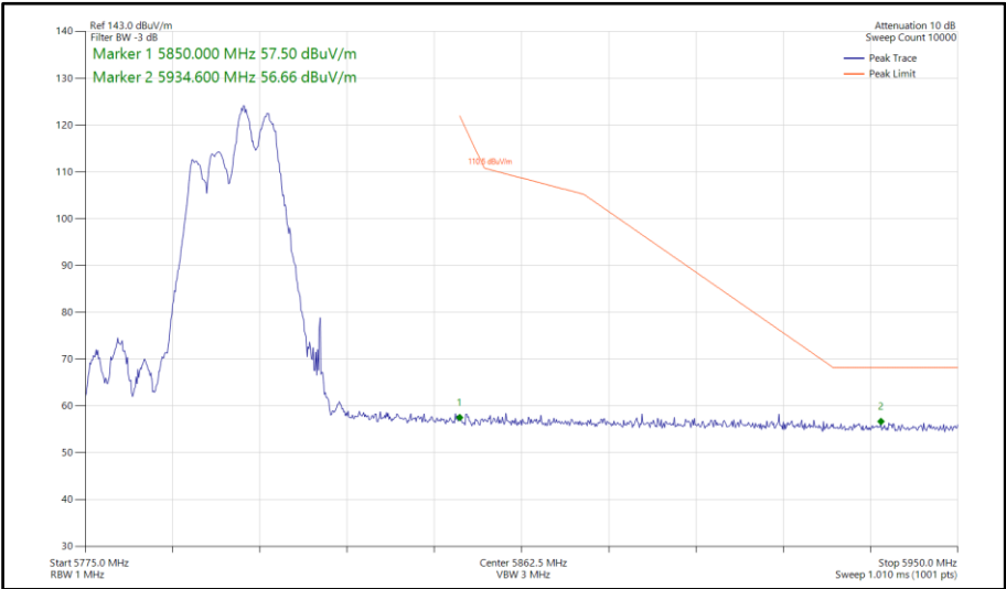
Figure 650 - 802.11ax HE40, RU106-56, CDD, Core 0-1 - 5795 MHz Band Edge Frequency 5850 MHz
