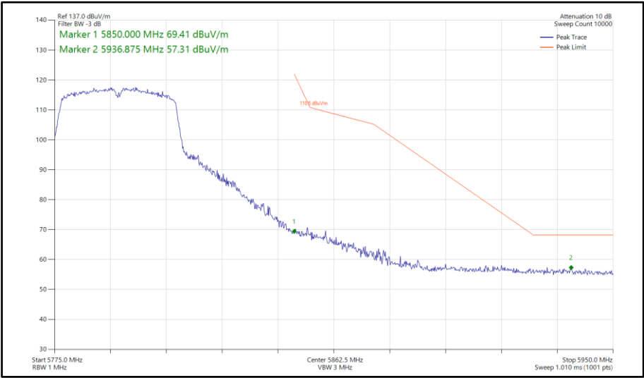
Figure 621 - 802.11n HT40, SISO, Core 1 - 5795 MHz Band Edge Frequency 5850 MHz
