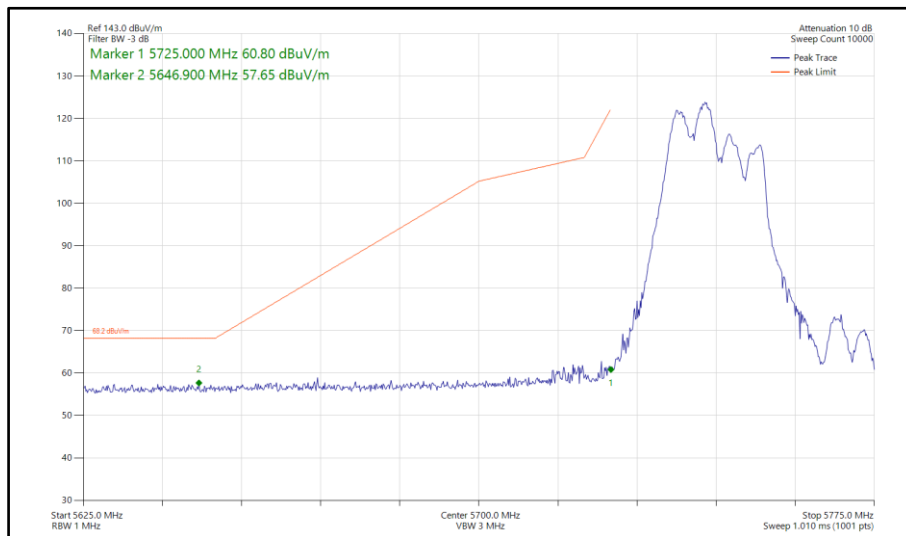
Figure 636 - 802.11ax HE40, RU106-53, CDD, Core 0-1 - 5755 MHz Band Edge Frequency 5725 MHz
