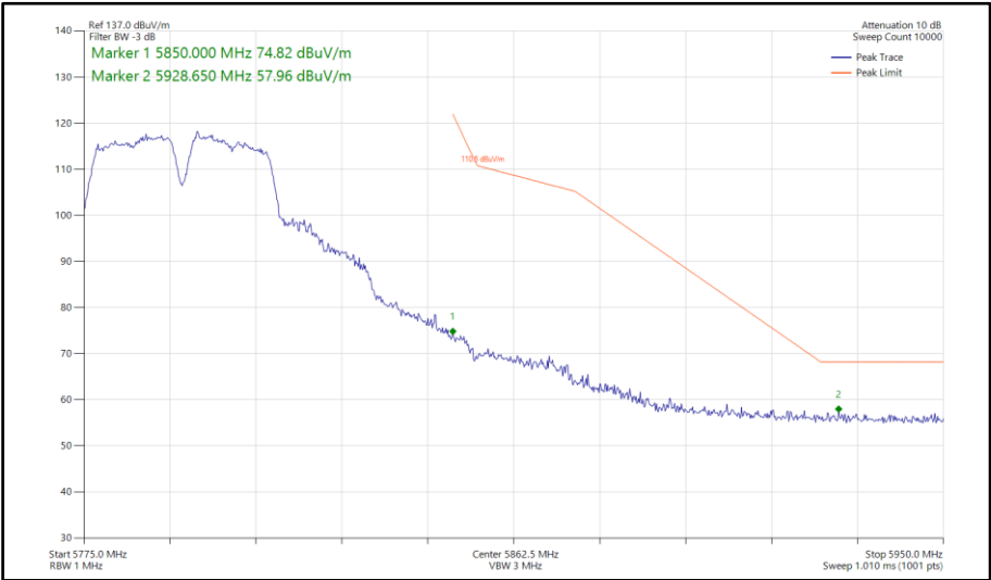
Figure 619 - 802.11a a40, SISO, Core 1 - 5795 MHz Band Edge Frequency 5850 MHz
