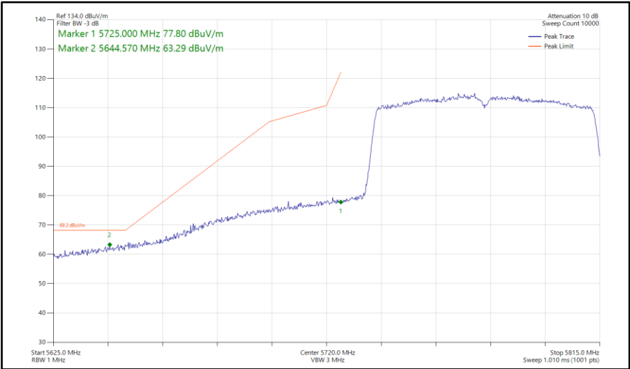
Figure 689 - 802.11ac VHT80, SISO, Core 0 - 5775 MHz Band Edge Frequency 5725 MHz
