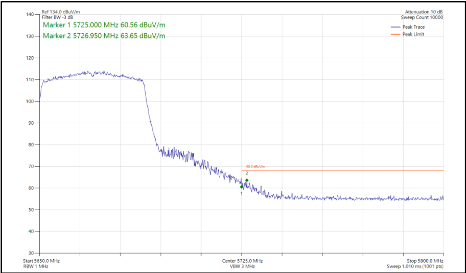
Figure 615 - 802.11ax HE40, SU, SISO, Core 1 - 5670 MHz Band Edge Frequency 5725 MHz
