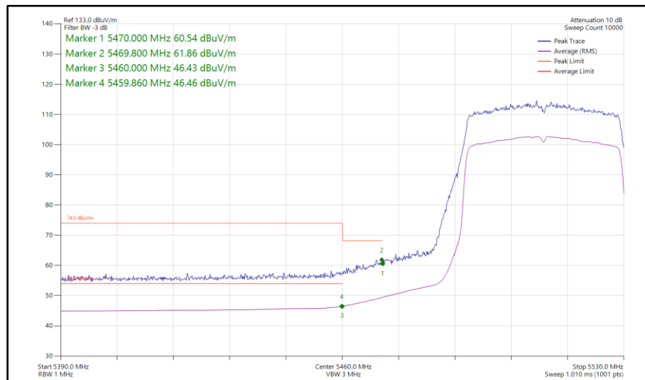
Figure 654 - 802.11ax HE40, SU, SDM, Core 0-1 - 5510 MHz Band Edge Frequency 5470 MHz
