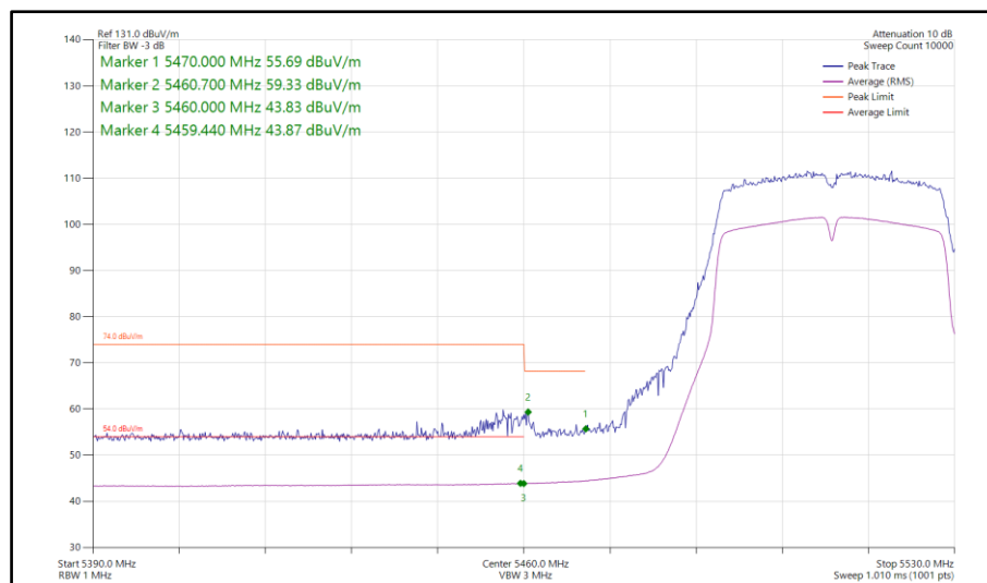
Figure 673 - 802.11ac VHT40, TxBF, Core 0-1 - 5510 MHz Band Edge Frequency 5470 MHz
