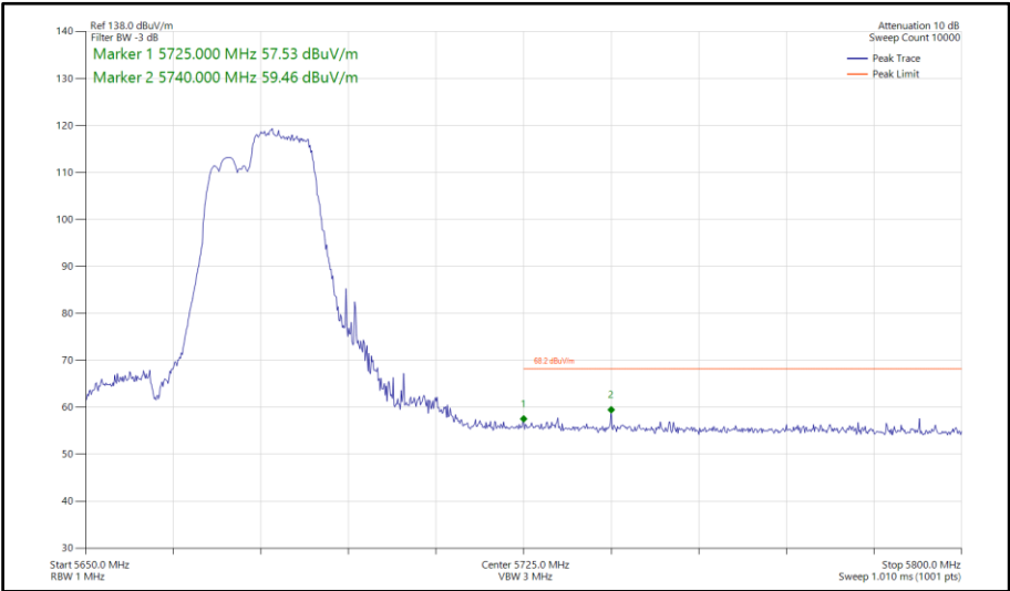
Figure 617 - 802.11be EHT40, RU106+26-85, SISO, Core 1 - 5670 MHz Band Edge Frequency 5725 MHz
