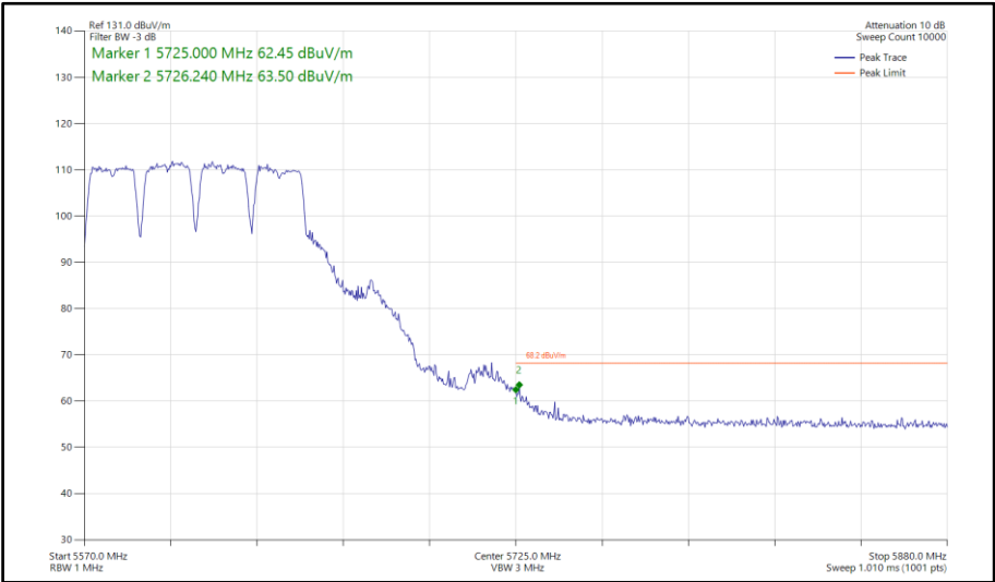
Figure 693 - 802.11a a80, SISO, Core 0 - 5610 MHz Band Edge Frequency 5725 MHz
