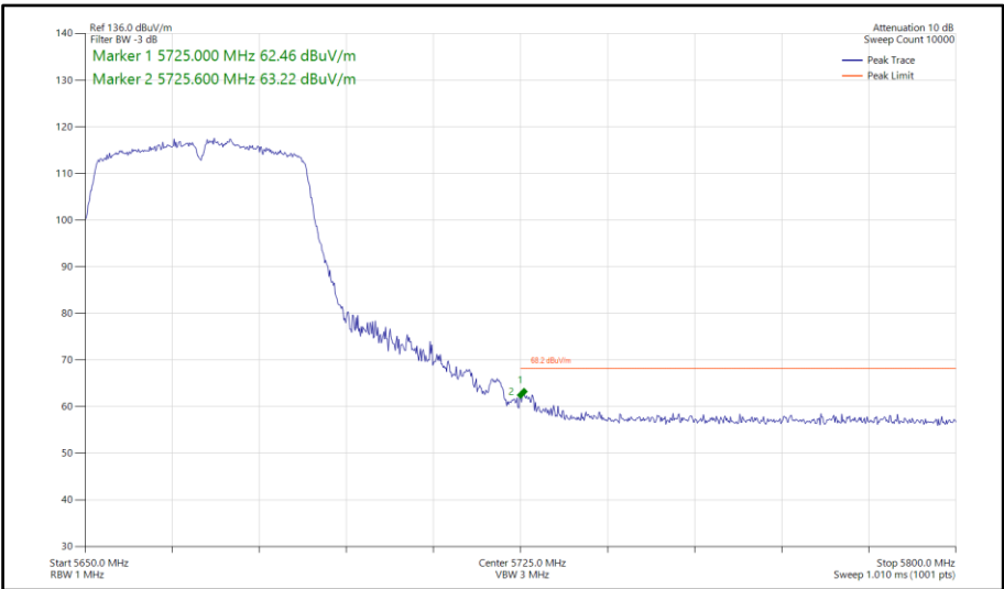
Figure 661 - 802.11n HT40, SDM, Core 0-1 - 5670 MHz Band Edge Frequency 5725 MHz
