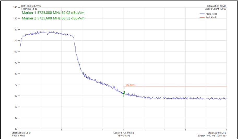
Figure 662 - 802.11ax HE40, SU, SDM, Core 0-1 - 5670 MHz Band Edge Frequency 5725 MHz
