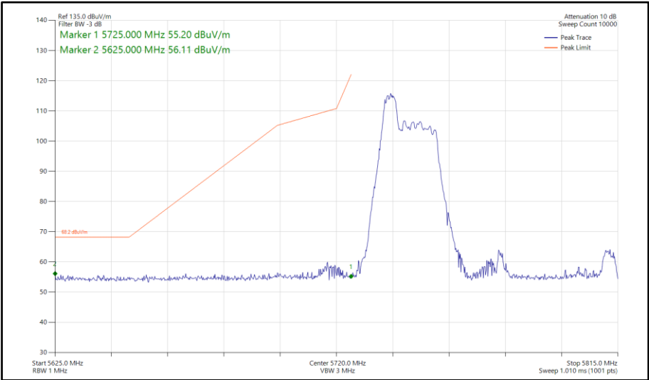
Figure 691 - 802.11ax HE80, RU52-37, SISO, Core 0 - 5775 MHz Band Edge Frequency 5725 MHz
