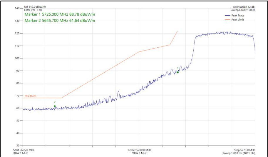
Figure 658 - 802.11ax HE40, SU, SDM, Core 0-1 - 5755 MHz Band Edge Frequency 5725 MHz
