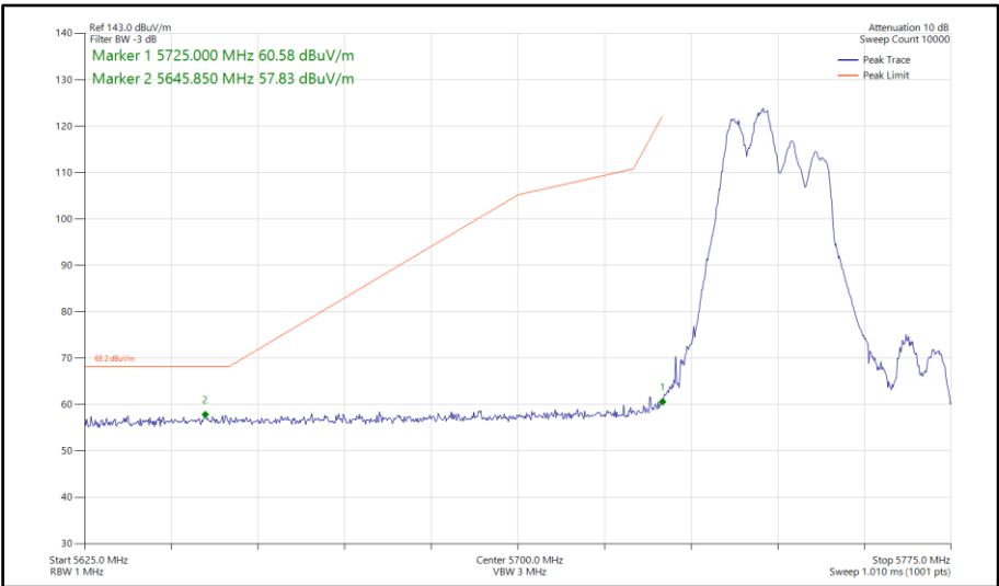
Figure 659 - 802.11ax HE40, RU106-53, SDM, Core 0-1 - 5755 MHz Band Edge Frequency 5725 MHz
