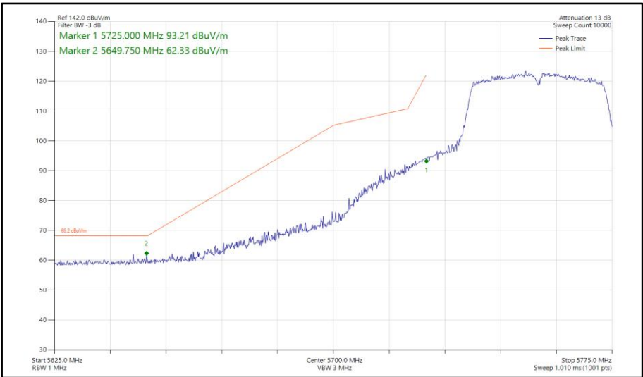
Figure 675 - 802.11ac VHT40, TxBF, Core 0-1 - 5755 MHz Band Edge Frequency 5725 MHz
