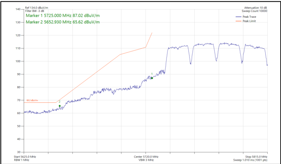
Figure 688 - 802.11a a80, SISO, Core 0 - 5775 MHz Band Edge Frequency 5725 MHz
