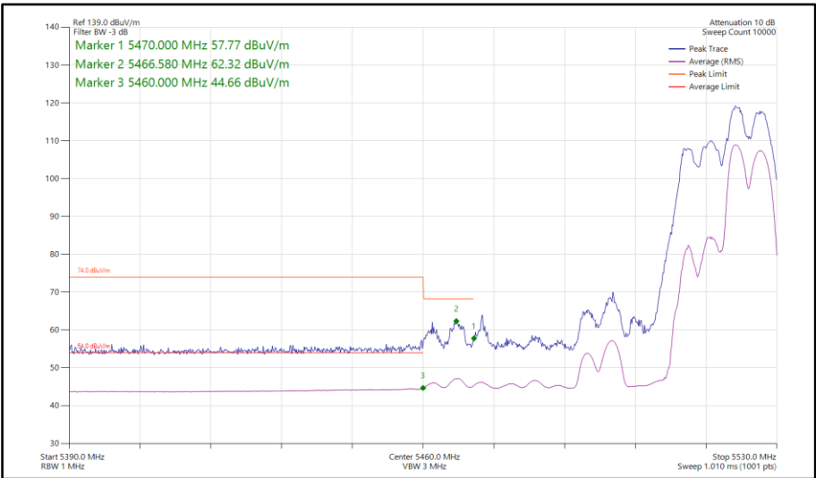
Figure 631 - 802.11ax HE40, RU106-56, CDD, Core 0-1 - 5510 MHz Band Edge Frequency 5470 MHz
