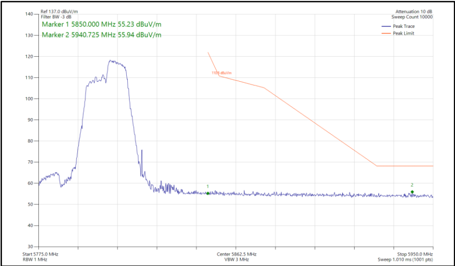
Figure 625 - 802.11ax HE40, RU106-56, SISO, Core 1 - 5795 MHz Band Edge Frequency 5850 MHz
