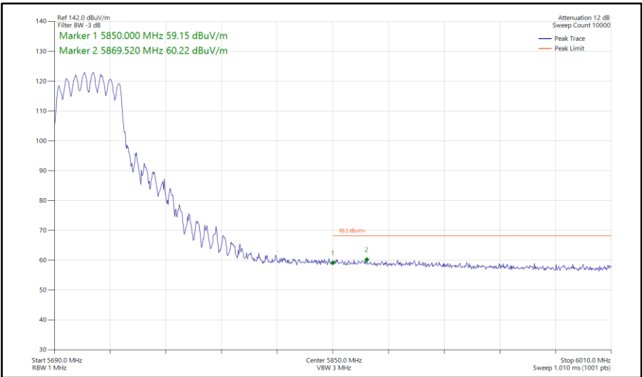
Figure 645 - 802.11n HT40, CDD, Core 0-1 - 5710 MHz Band Edge Frequency 5850 MHz
