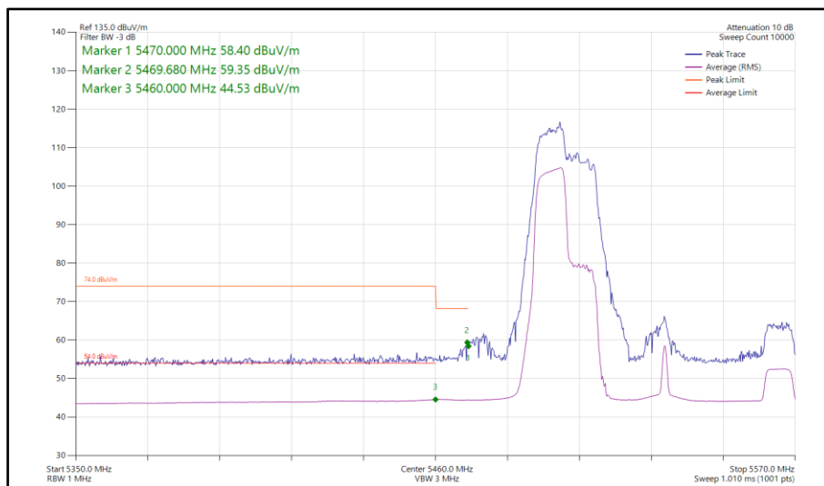
Figure 686 - 802.11ax HE80, RU106-53, SISO, Core 0 - 5530 MHz Band Edge Frequency 5470 MHz
