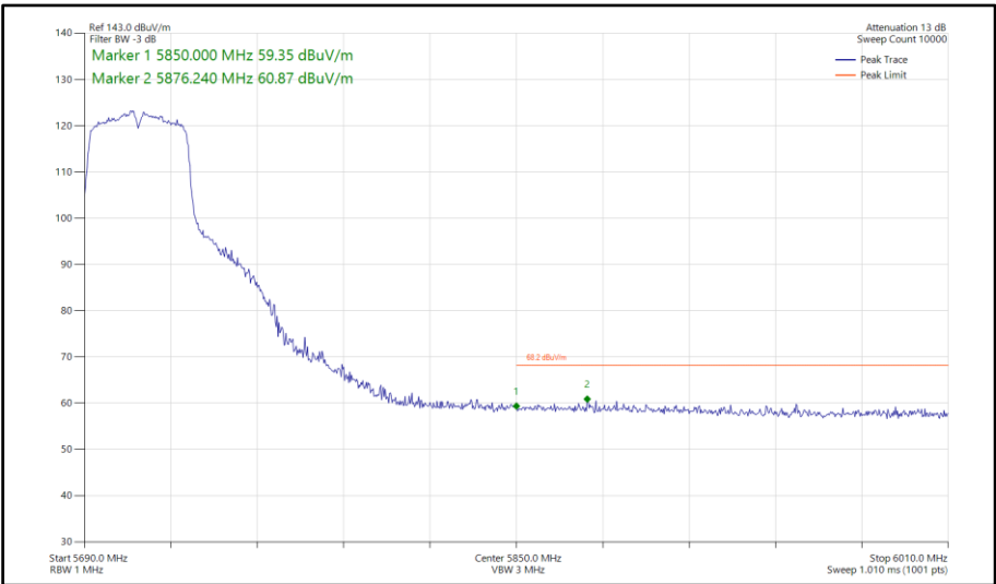
Figure 679 - 802.11ac VHT40, TxBF, Core 0-1 - 5710 MHz Band Edge Frequency 5850 MHz
