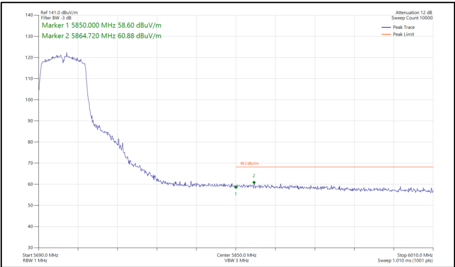
Figure 665 - 802.11n HT40, SDM, Core 0-1 - 5710 MHz Band Edge Frequency 5850 MHz
