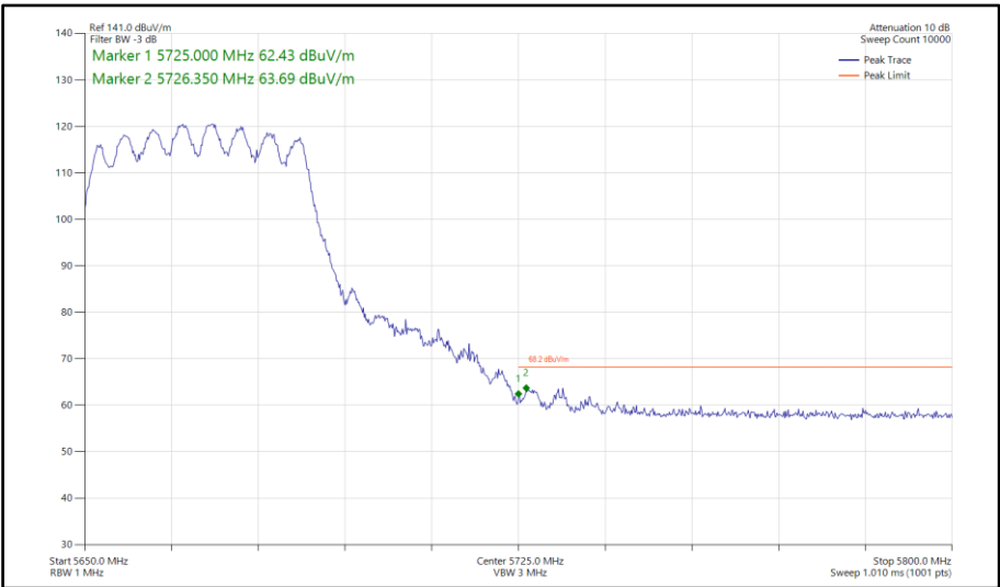
Figure 639 - 802.11n HT40, CDD, Core 0-1 - 5670 MHz Band Edge Frequency 5725 MHz
