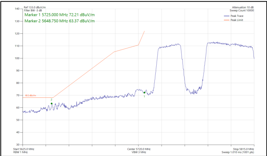
Figure 692 - 802.11be EHT80, RU484+242-91, SISO, Core 0 - 5775 MHz Band Edge Frequency 5725 MHz
