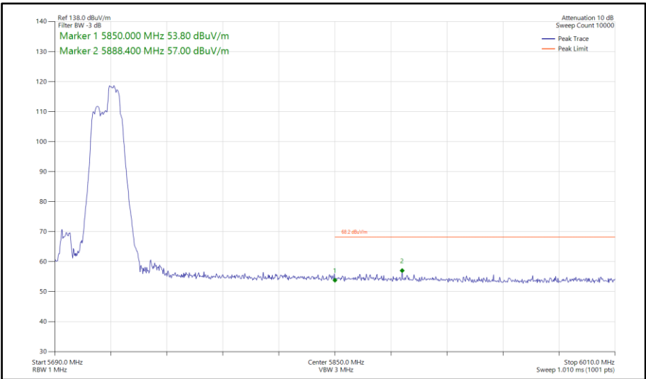
Figure 626 - 802.11be EHT40, RU52+26-75, SISO, Core 1 - 5710 MHz Band Edge Frequency 5850 MHz
