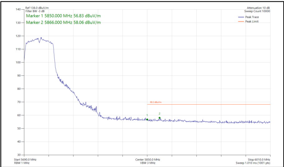
Figure 620 - 802.11n HT40, SISO, Core 1 - 5710 MHz Band Edge Frequency 5850 MHz
