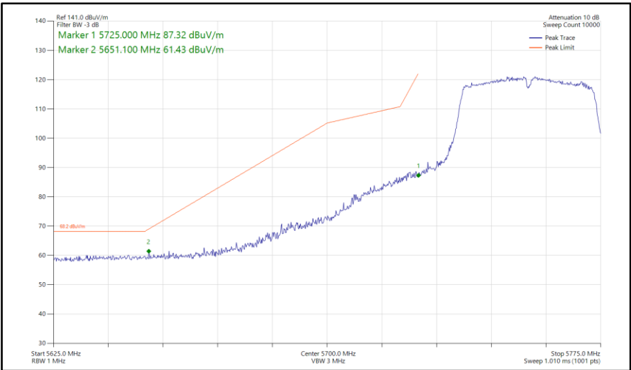
Figure 657 - 802.11n HT40, SDM, Core 0-1 - 5755 MHz Band Edge Frequency 5725 MHz
