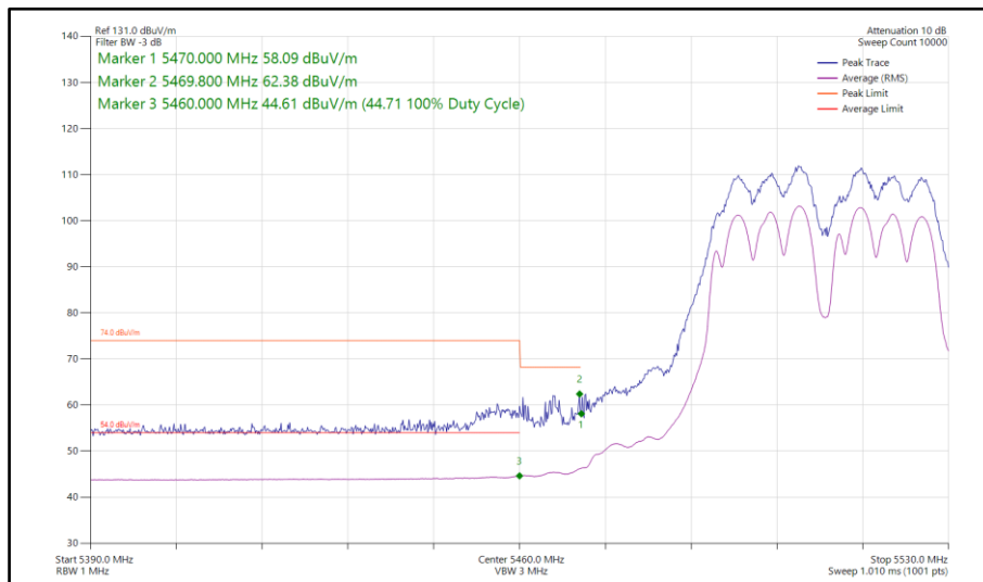
Figure 628 - 802.11a a40, CDD, Core 0-1 - 5510 MHz Band Edge Frequency 5470 MHz
