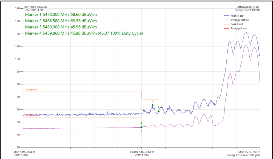
Figure 656 - 802.11be EHT40, RU106+26-85, SDM, Core 0-1 - 5510 MHz Band Edge Frequency 5470 MHz
