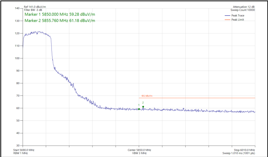
Figure 667 - 802.11ax HE40, SU, SDM, Core 0-1 - 5710 MHz Band Edge Frequency 5850 MHz
