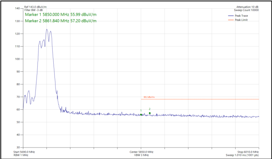
Figure 648 - 802.11ax HE40, RU106-56, CDD, Core 0-1 - 5710 MHz Band Edge Frequency 5850 MHz
