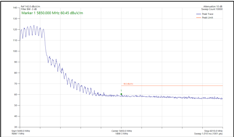
Figure 647 - 802.11ax HE40, SU, CDD, Core 0-1 - 5710 MHz Band Edge Frequency 5850 MHz
