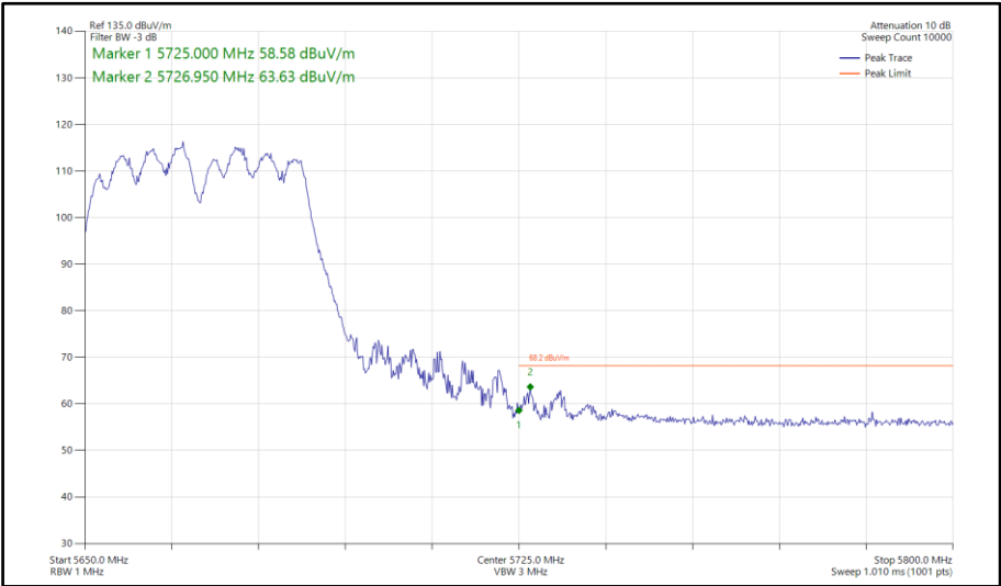
Figure 638 - 802.11a a40, CDD, Core 0-1 - 5670 MHz Band Edge Frequency 5725 MHz
