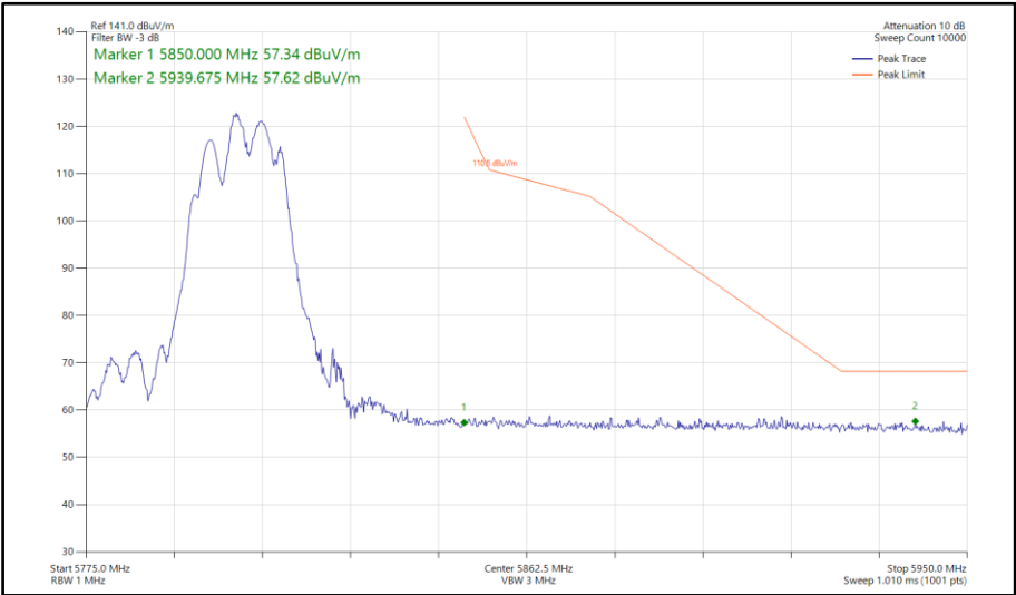
Figure 652 - 802.11be EHT40, RU106+26-85, CDD, Core 0-1 - 5795 MHz Band Edge Frequency 5850 MHz
