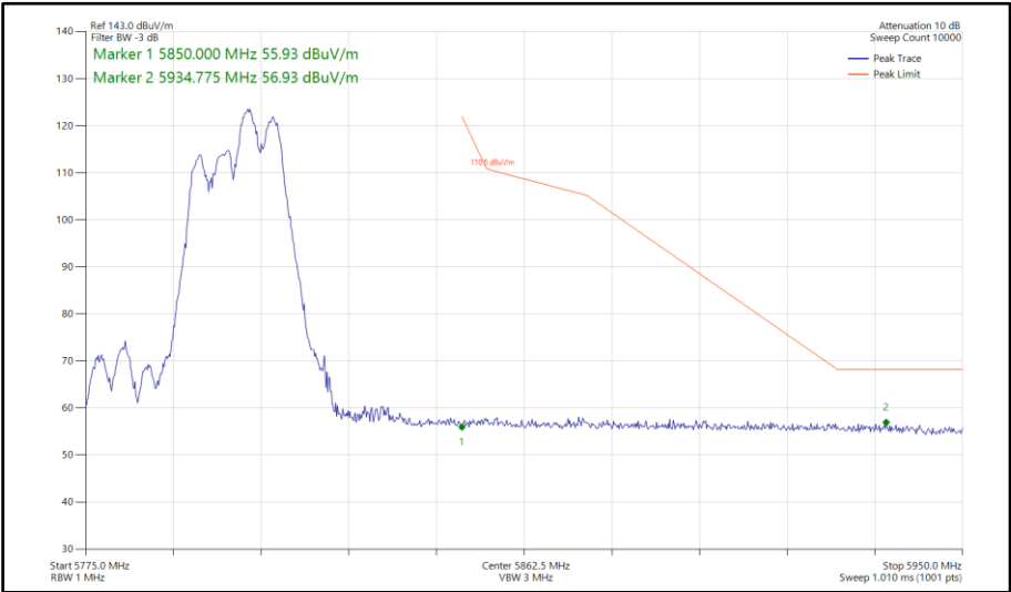
Figure 670 - 802.11ax HE40, RU106-56, SDM, Core 0-1 - 5795 MHz Band Edge Frequency 5850 MHz
