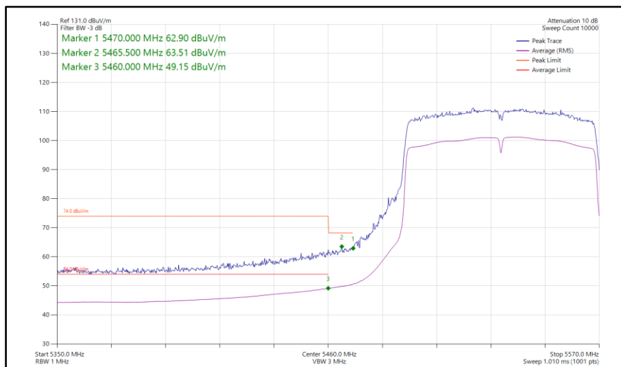
Figure 684 - 802.11ac VHT80, SISO, Core 0 - 5530 MHz Band Edge Frequency 5470 MHz
