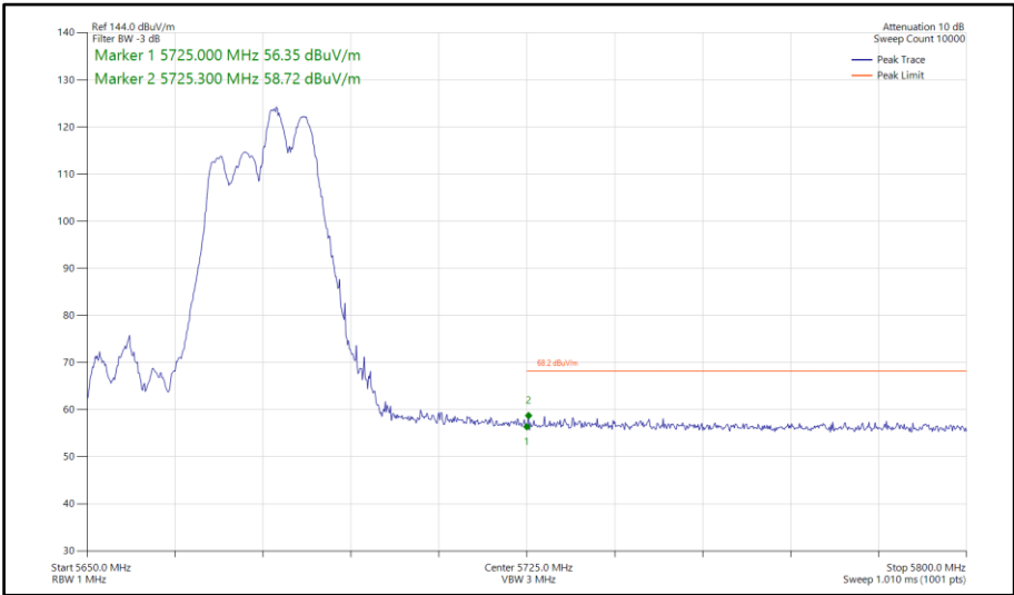
Figure 641 - 802.11ax HE40, RU106-56, CDD, Core 0-1 - 5670 MHz Band Edge Frequency 5725 MHz
