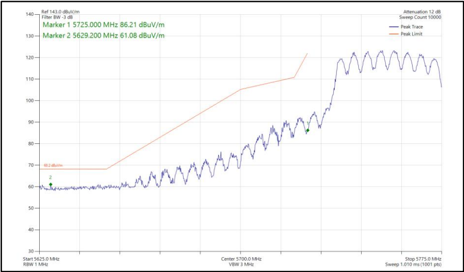
Figure 635 - 802.11ax HE40, SU, CDD, Core 0-1 - 5755 MHz Band Edge Frequency 5725 MHz
