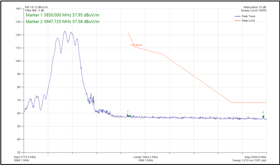
Figure 672 - 802.11be EHT40, RU106+26-85, SDM, Core 0-1 - 5795 MHz Band Edge Frequency 5850 MHz
