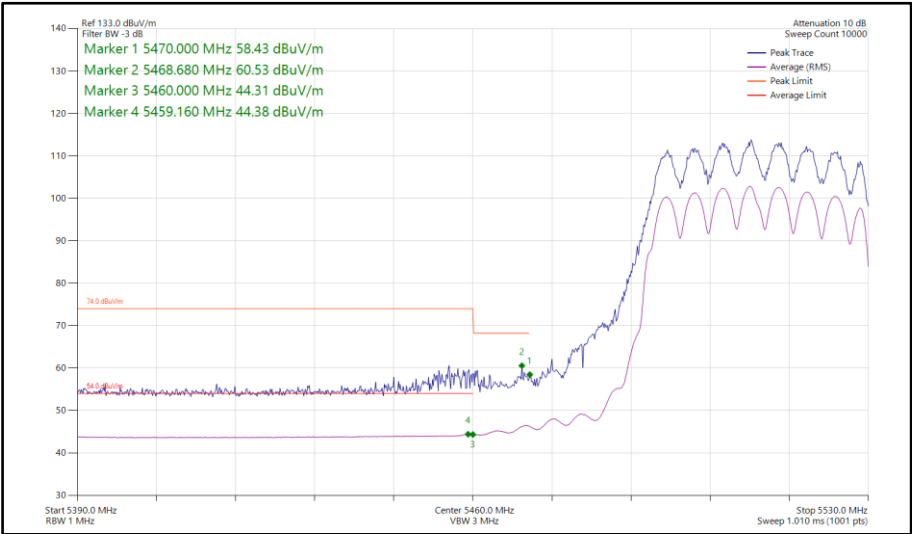
Figure 630 - 802.11ax HE40, SU, CDD, Core 0-1 - 5510 MHz Band Edge Frequency 5470 MHz
