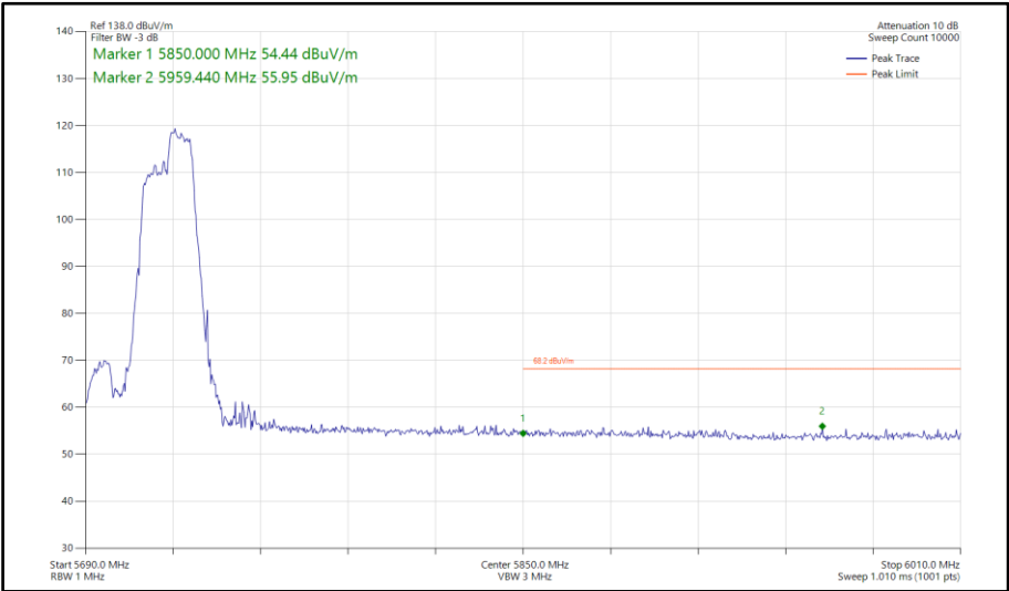
Figure 623 - 802.11ax HE40, RU106-56, SISO, Core 1 - 5710 MHz Band Edge Frequency 5850 MHz
