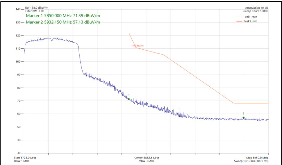
Figure 624 - 802.11ax HE40, SU, SISO, Core 1 - 5795 MHz Band Edge Frequency 5850 MHz
