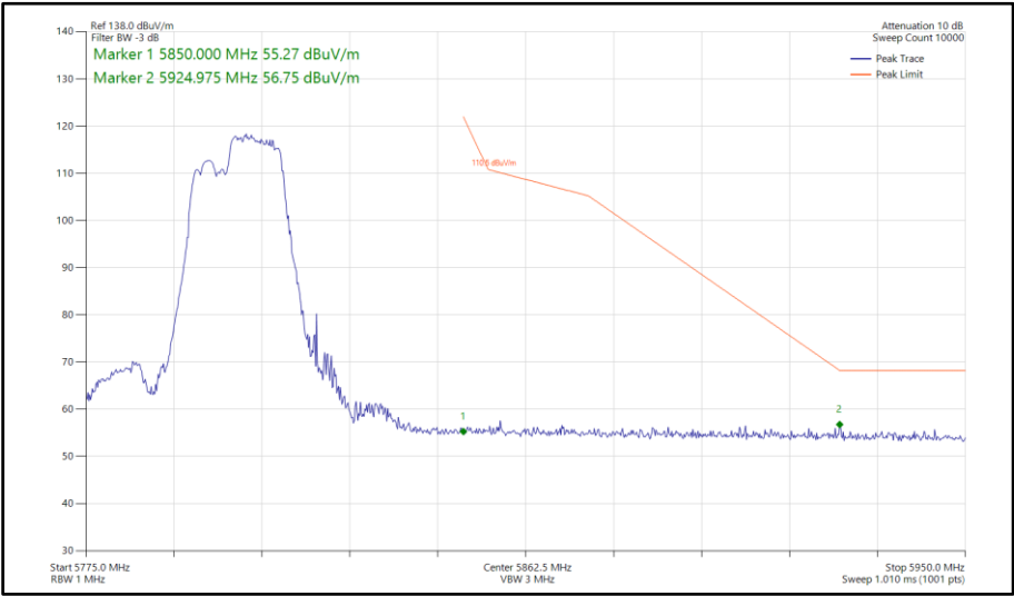
Figure 627 - 802.11be EHT40, RU106+26-85, SISO, Core 1 - 5795 MHz Band Edge Frequency 5850 MHz
