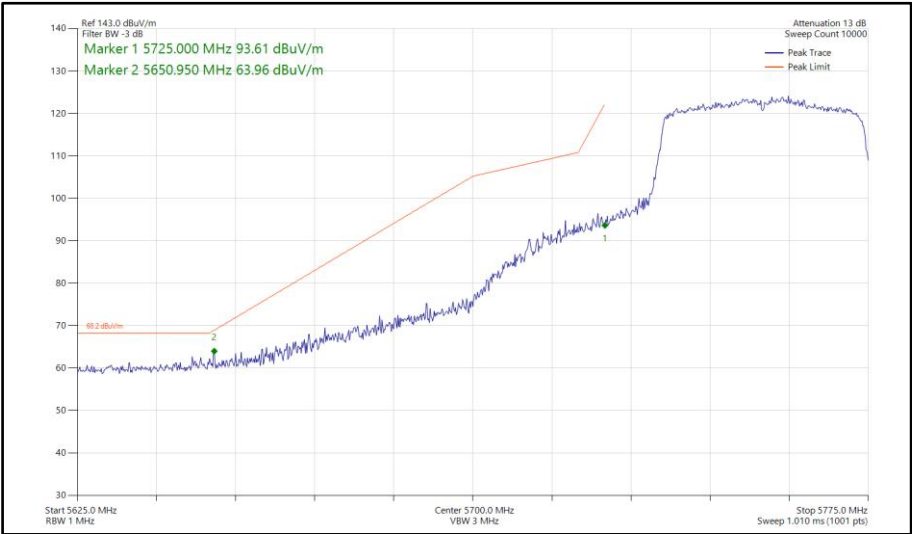
Figure 676 - 802.11ax HE40, SU, TxBF, Core 0-1 - 5755 MHz Band Edge Frequency 5725 MHz
