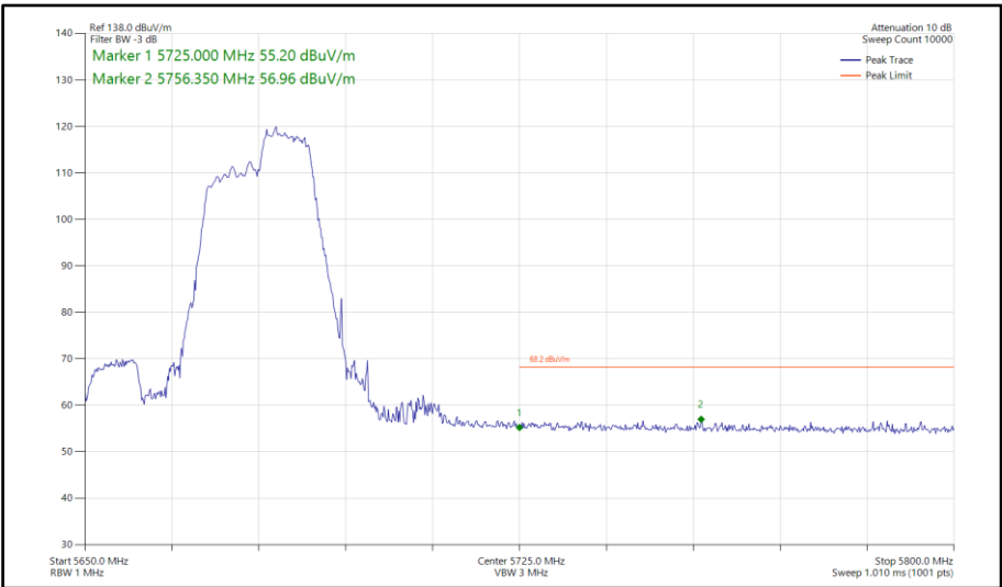
Figure 616 - 802.11ax HE40, RU106-56, SISO, Core 1 - 5670 MHz Band Edge Frequency 5725 MHz
