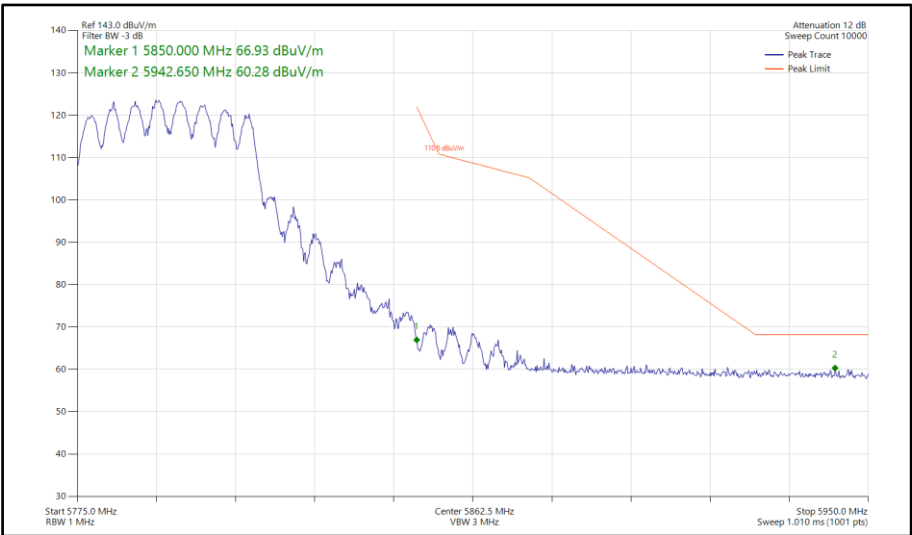
Figure 649 - 802.11ax HE40, SU, CDD, Core 0-1 - 5795 MHz Band Edge Frequency 5850 MHz
