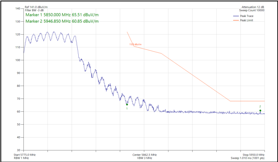
Figure 646 - 802.11n HT40, CDD, Core 0-1 - 5795 MHz Band Edge Frequency 5850 MHz
