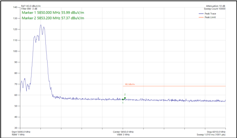
Figure 668 - 802.11ax HE40, RU106-56, SDM, Core 0-1 - 5710 MHz Band Edge Frequency 5850 MHz
