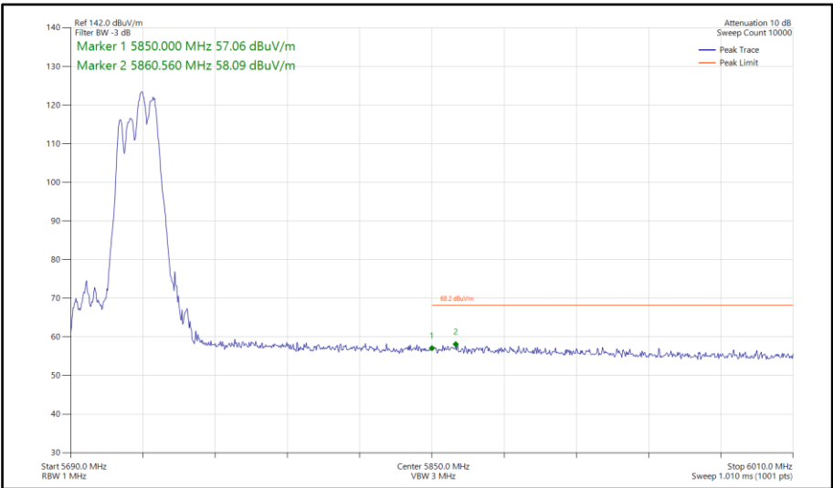
Figure 671 - 802.11be EHT40, RU106+26-85, SDM, Core 0-1 - 5710 MHz Band Edge Frequency 5850 MHz
