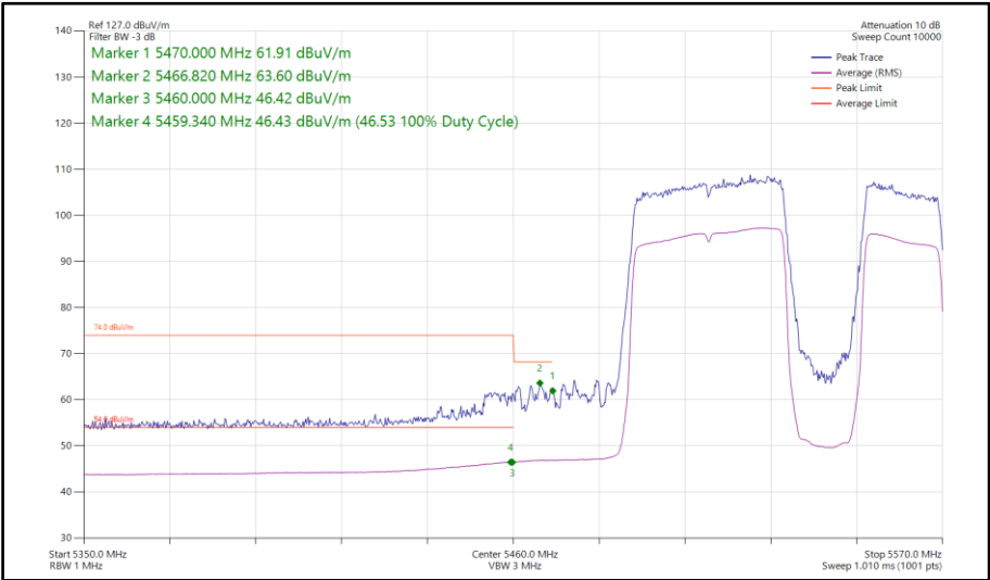
Figure 687 - 802.11be EHT80, RU484+242-92, SISO, Core 0 - 5530 MHz Band Edge Frequency 5470 MHz
