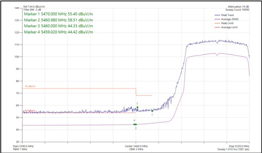
Figure 674 - 802.11ax HE40, SU, TxBF, Core 0-1 - 5510 MHz Band Edge Frequency 5470 MHz
