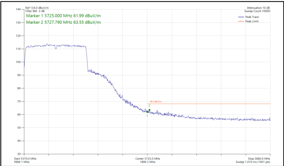
Figure 694 - 802.11ac VHT80, SISO, Core 0 - 5610 MHz Band Edge Frequency 5725 MHz
