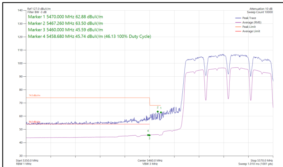
Figure 683 - 802.11a a80, SISO, Core 0 - 5530 MHz Band Edge Frequency 5470 MHz
