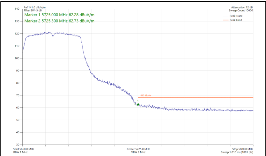
Figure 677 - 802.11ac VHT40, TxBF, Core 0-1 - 5670 MHz Band Edge Frequency 5725 MHz
