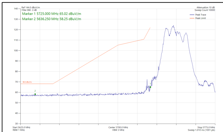
Figure 637 - 802.11be EHT40, RU106+26-82, CDD, Core 0-1 - 5755 MHz Band Edge Frequency 5725 MHz
