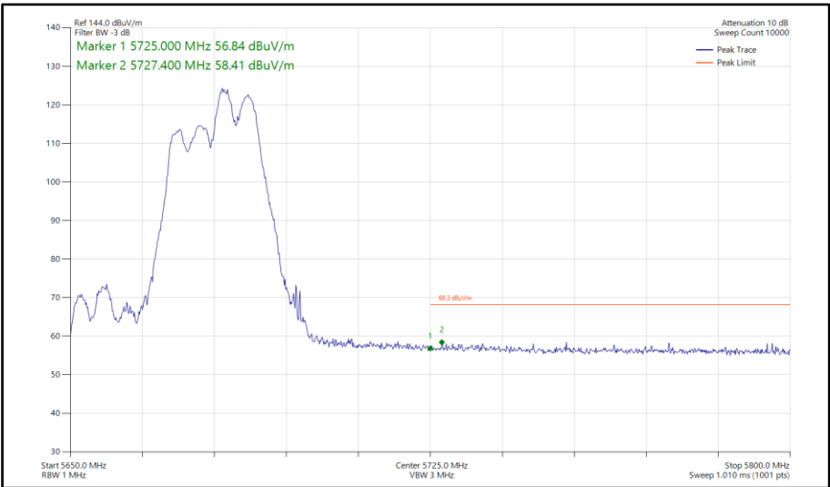
Figure 663 - 802.11ax HE40, RU106-56, SDM, Core 0-1 - 5670 MHz Band Edge Frequency 5725 MHz
