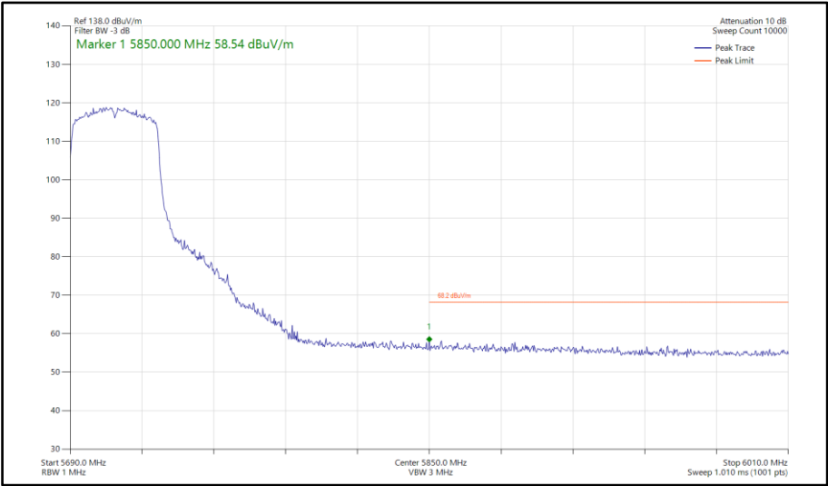
Figure 622 - 802.11ax HE40, SU, SISO, Core 1 - 5710 MHz Band Edge Frequency 5850 MHz
