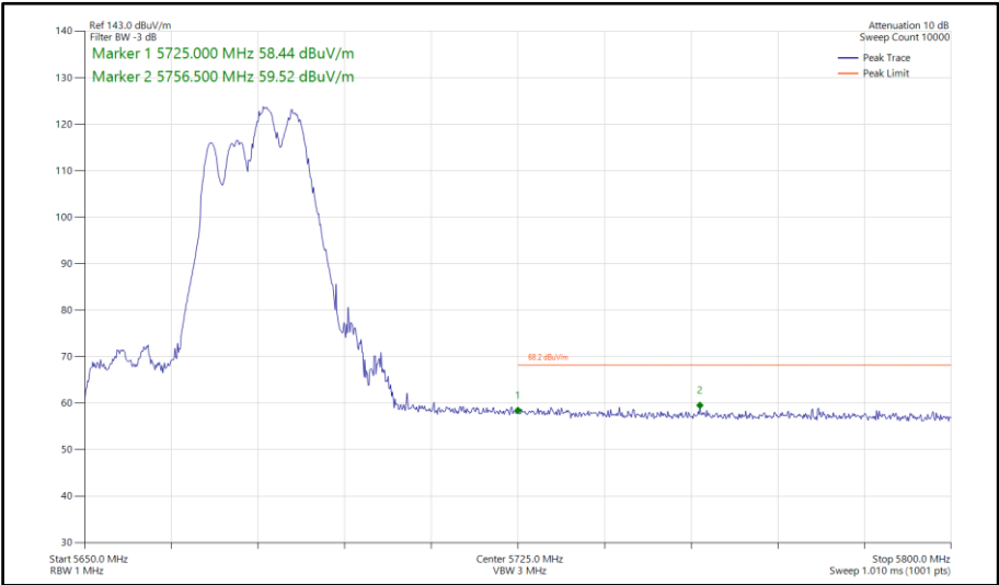
Figure 642 - 802.11be EHT40, RU106+26-85, CDD, Core 0-1 - 5670 MHz Band Edge Frequency 5725 MHz
