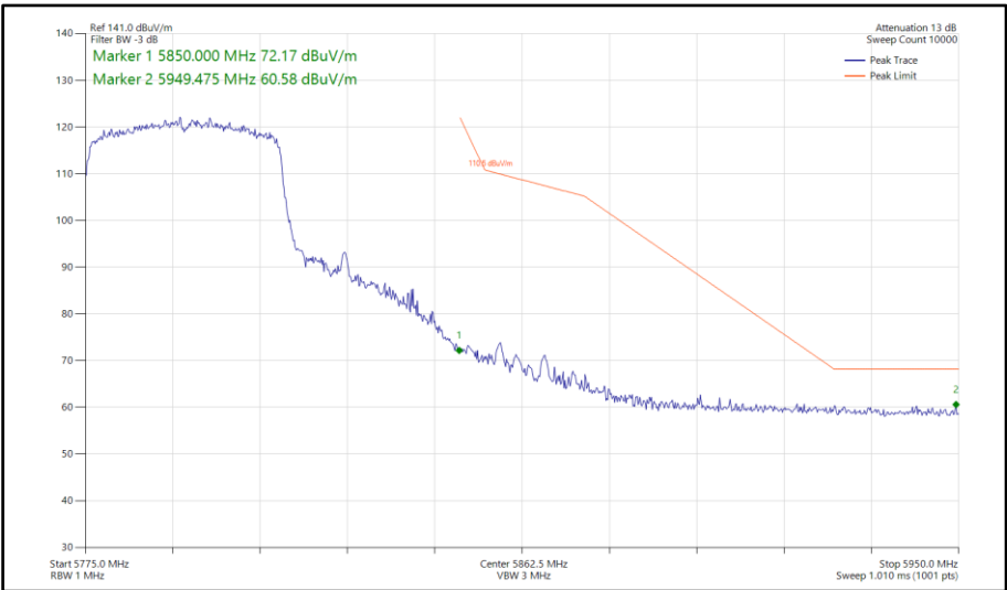
Figure 669 - 802.11ax HE40, SU, SDM, Core 0-1 - 5795 MHz Band Edge Frequency 5850 MHz
