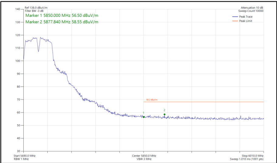
Figure 618 - 802.11a a40, SISO, Core 1 - 5710 MHz Band Edge Frequency 5850 MHz
