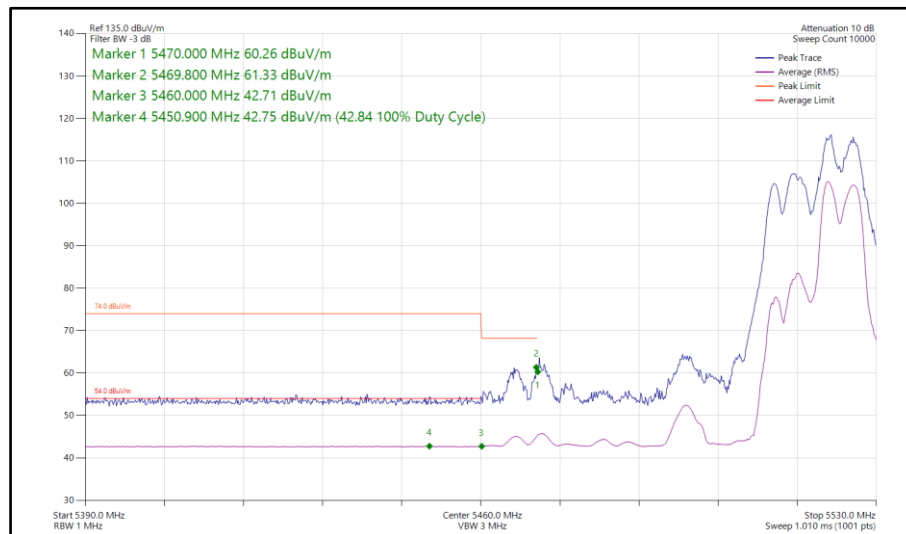
Figure 632 - 802.11be EHT40, RU52+26-75, CDD, Core 0-1 - 5510 MHz Band Edge Frequency 5470 MHz
