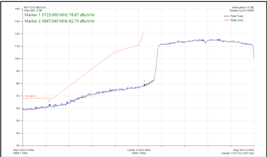
Figure 690 - 802.11ax HE80, SU, SISO, Core 0 - 5775 MHz Band Edge Frequency 5725 MHz
