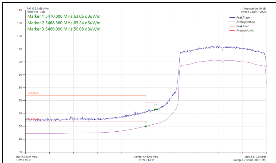
Figure 685 - 802.11ax HE80, SU, SISO, Core 0 - 5530 MHz Band Edge Frequency 5470 MHz
