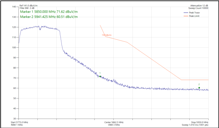
Figure 666 - 802.11n HT40, SDM, Core 0-1 - 5795 MHz Band Edge Frequency 5850 MHz
