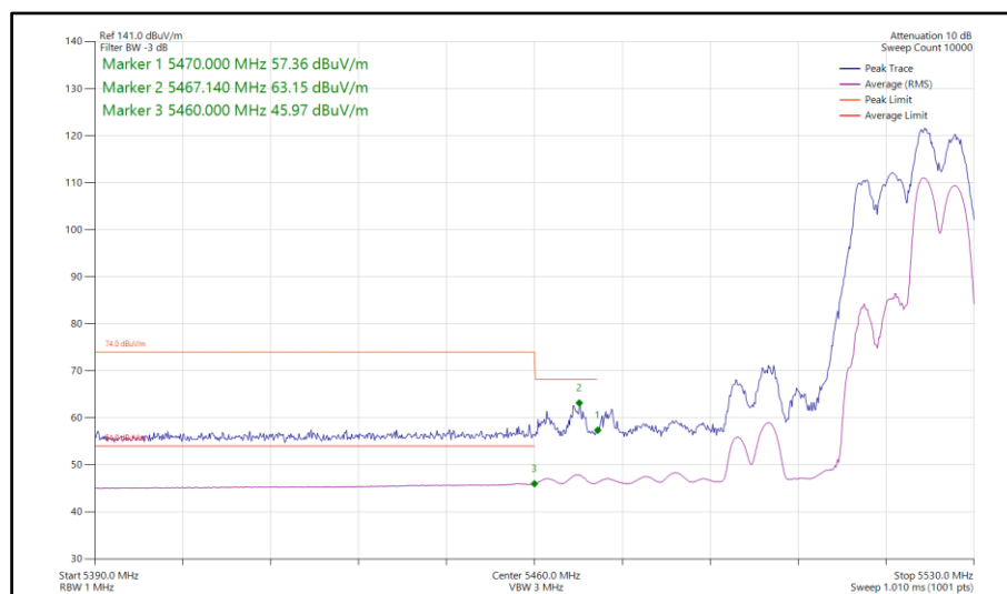
Figure 655 - 802.11ax HE40, RU106-56, SDM, Core 0-1 - 5510 MHz Band Edge Frequency 5470 MHz
