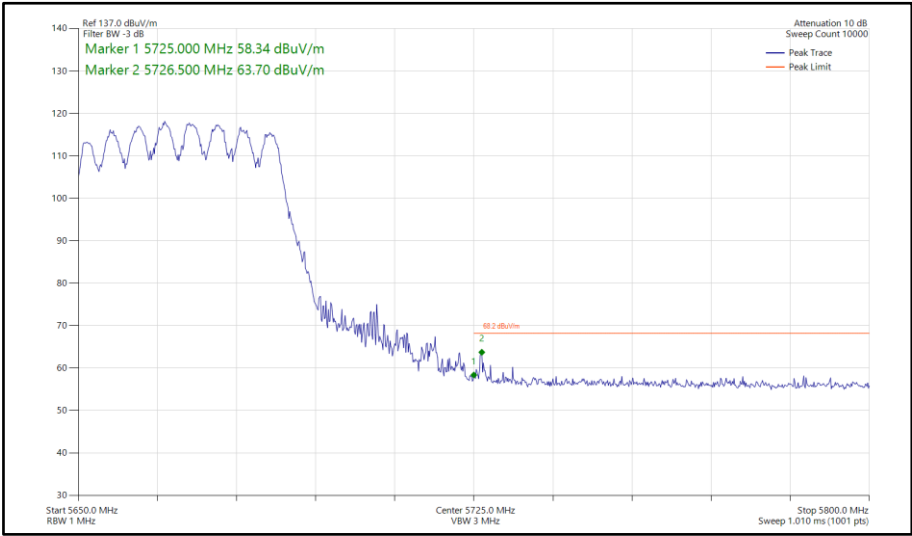
Figure 640 - 802.11ax HE40, SU, CDD, Core 0-1 - 5670 MHz Band Edge Frequency 5725 MHz
