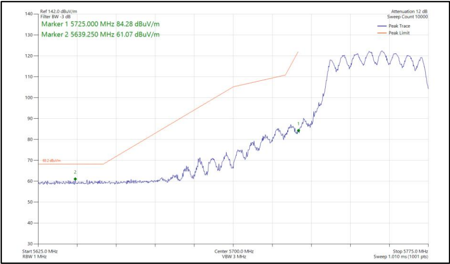
Figure 634 - 802.11n HT40, CDD, Core 0-1 - 5755 MHz Band Edge Frequency 5725 MHz
