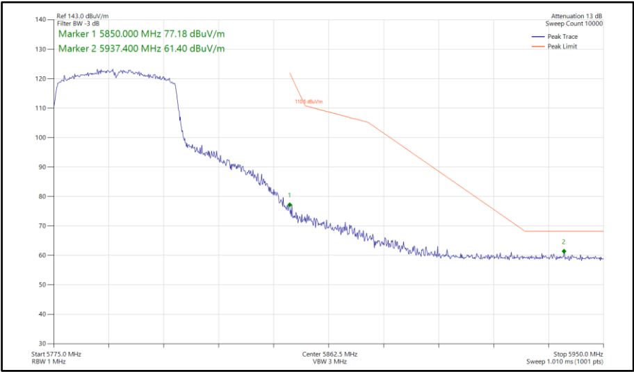
Figure 682 - 802.11ax HE40, SU, TxBF, Core 0-1 - 5795 MHz Band Edge Frequency 5850 MHz
