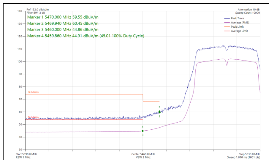
Figure 653 - 802.11n HT40, SDM, Core 0-1 - 5510 MHz Band Edge Frequency 5470 MHz
