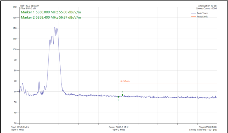
Figure 753 - 802.11ax HE80, RU106-60, CDD, Core 0-1 - 5690 MHz Band Edge Frequency 5850 MHz
