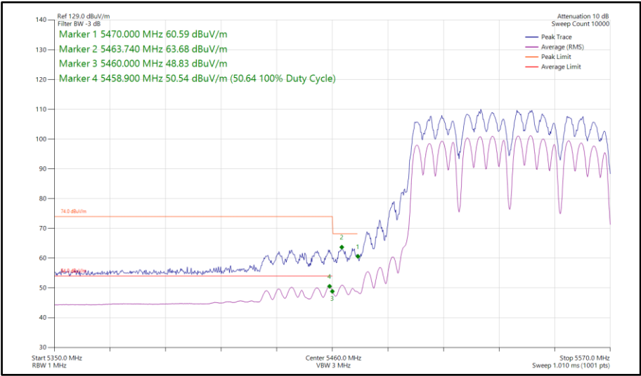
Figure 733 - 802.11a a80, CDD, Core 0-1 - 5530 MHz Band Edge Frequency 5470 MHz
