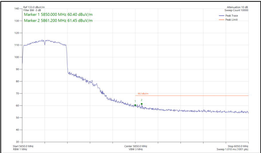
Figure 725 - 802.11ac VHT80, SISO, Core 1 - 5690 MHz Band Edge Frequency 5850 MHz
