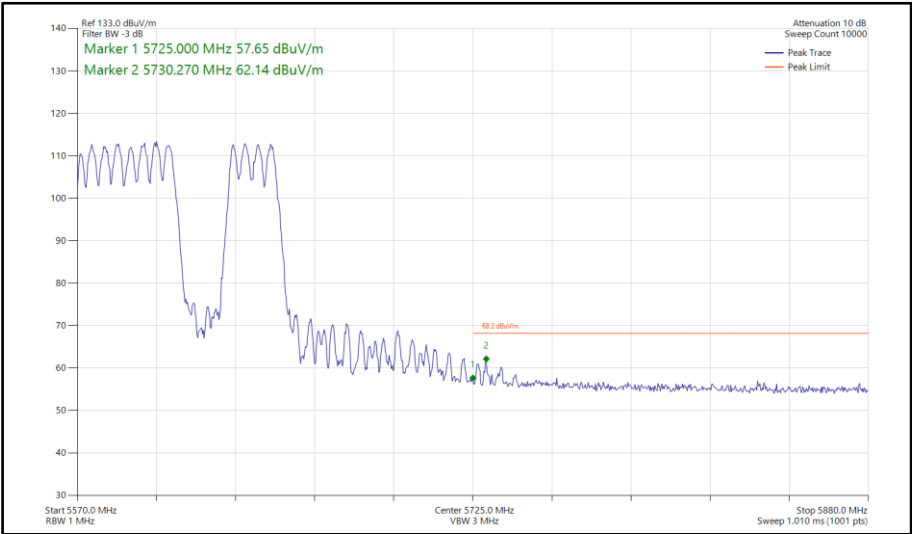
Figure 769 - 802.11be EHT80, RU484+242-92, SDM, Core 0-1 - 5610 MHz Band Edge Frequency 5725 MHz
