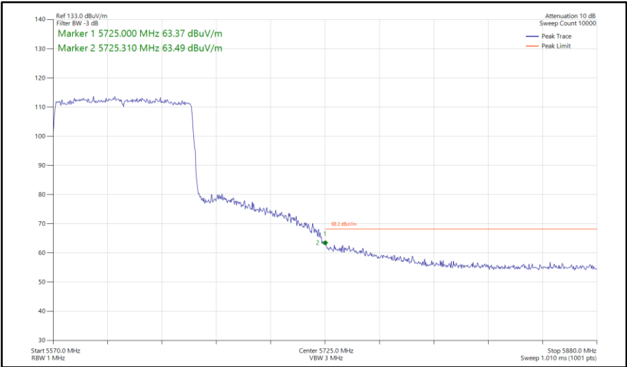
Figure 720 - 802.11ax HE80, SU, SISO, Core 1 - 5610 MHz Band Edge Frequency 5725 MHz
