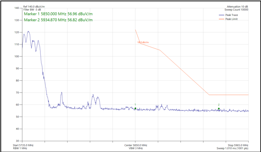
Figure 775 - 802.11ax HE80, RU106-53, SDM, Core 0-1 - 5775 MHz Band Edge Frequency 5850 MHz
