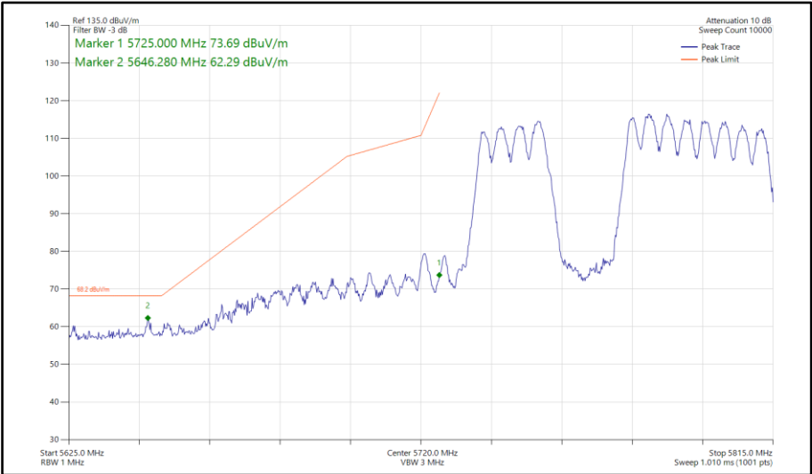
Figure 742 - 802.11be EHT80, RU484+242-91, CDD, Core 0-1 - 5775 MHz Band Edge Frequency 5725 MHz
