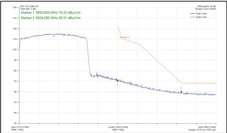
Figure 704 - 802.11ax HE80, SU, SISO, Core 0 - 5775 MHz Band Edge Frequency 5850 MHz
