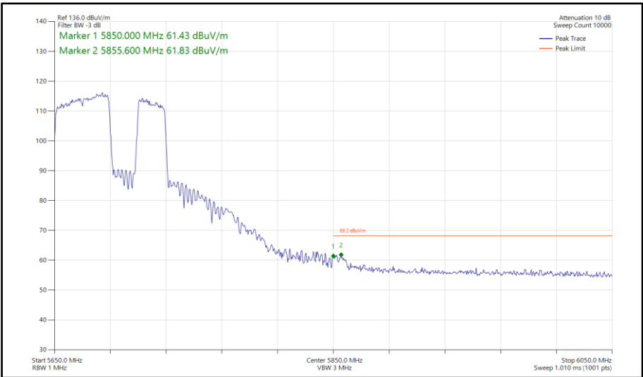
Figure 706 - 802.11be EHT80, RU484+242-92, SISO, Core 0 - 5690 MHz Band Edge Frequency 5850 MHz
