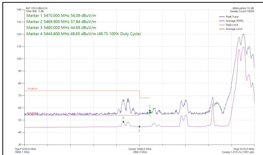
Figure 737 - 802.11be EHT80, RU52+26-80, CDD, Core 0-1 - 5530 MHz Band Edge Frequency 5470 MHz
