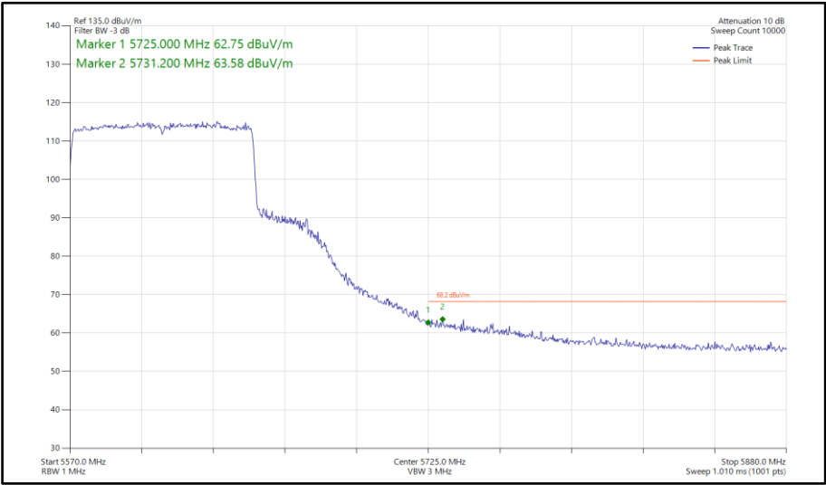
Figure 695 - 802.11ax HE80, SU, SISO, Core 0 - 5610 MHz Band Edge Frequency 5725 MHz
