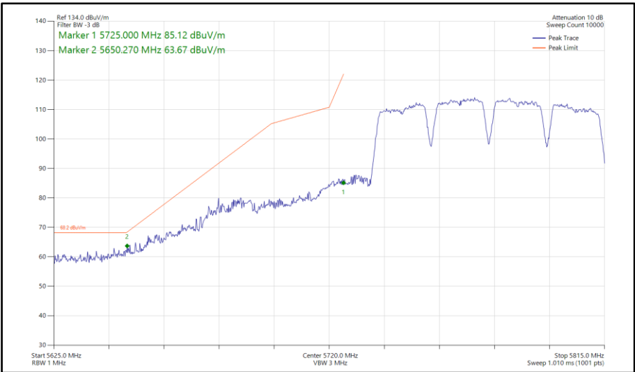
Figure 713 - 802.11a a80, SISO, Core 1 - 5775 MHz Band Edge Frequency 5725 MHz
