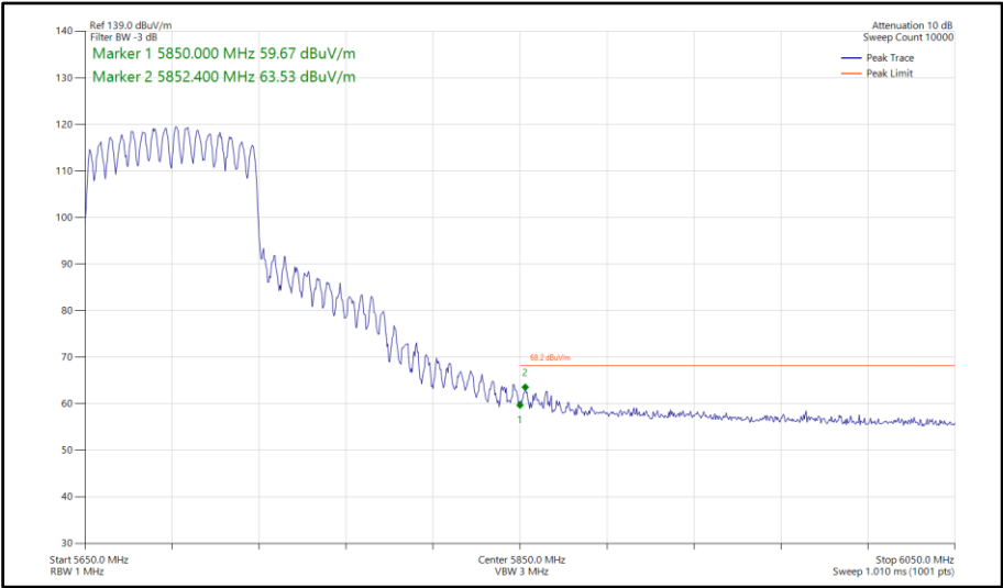
Figure 750 - 802.11ac VHT80, CDD, Core 0-1 - 5690 MHz Band Edge Frequency 5850 MHz
