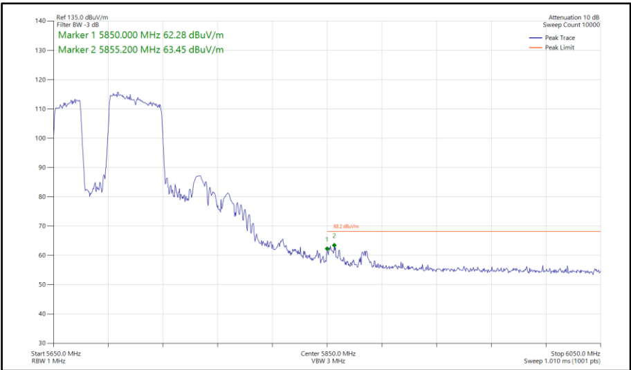
Figure 731 - 802.11be EHT80, RU484+242-91, SISO, Core 1 - 5690 MHz Band Edge Frequency 5850 MHz
