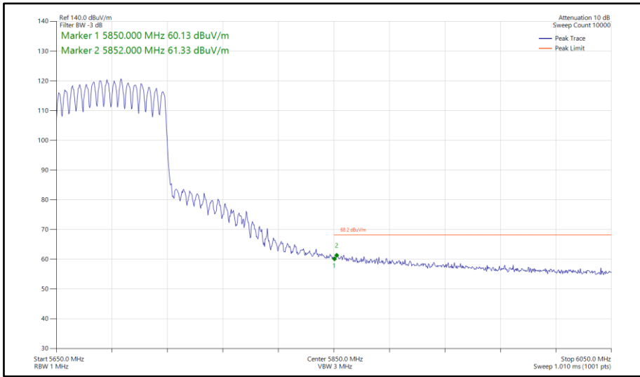
Figure 752 - 802.11ax HE80, SU, CDD, Core 0-1 - 5690 MHz Band Edge Frequency 5850 MHz
