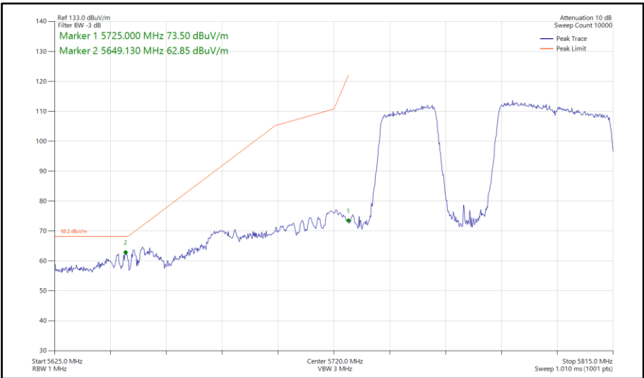
Figure 717 - 802.11be EHT80, RU484+242-91, SISO, Core 1 - 5775 MHz Band Edge Frequency 5725 MHz
