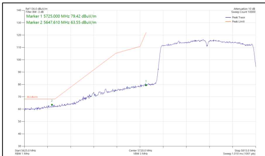
Figure 762 - 802.11ac VHT80, SDM, Core 0-1 - 5775 MHz Band Edge Frequency 5725 MHz
