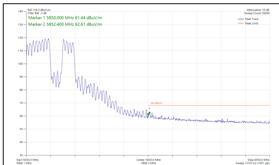
Figure 756 - 802.11be EHT80, RU484+242-92, CDD, Core 0-1 - 5690 MHz Band Edge Frequency 5850 MHz
