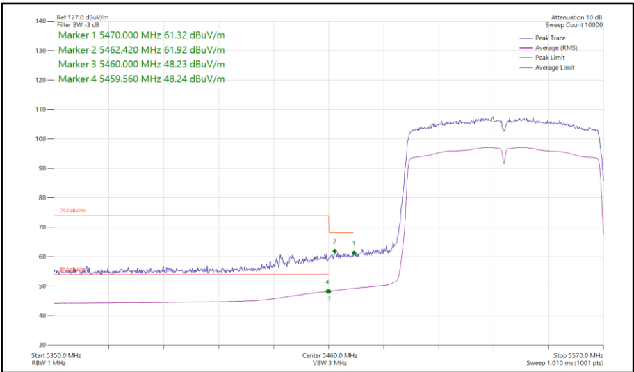
Figure 709 - 802.11ac VHT80, SISO, Core 1 - 5530 MHz Band Edge Frequency 5470 MHz
