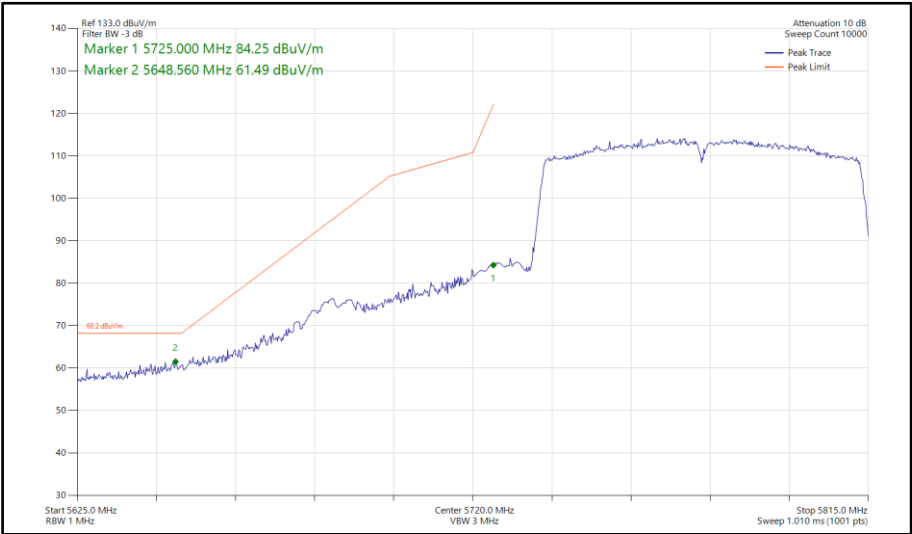
Figure 714 - 802.11ac VHT80, SISO, Core 1 - 5775 MHz Band Edge Frequency 5725 MHz
