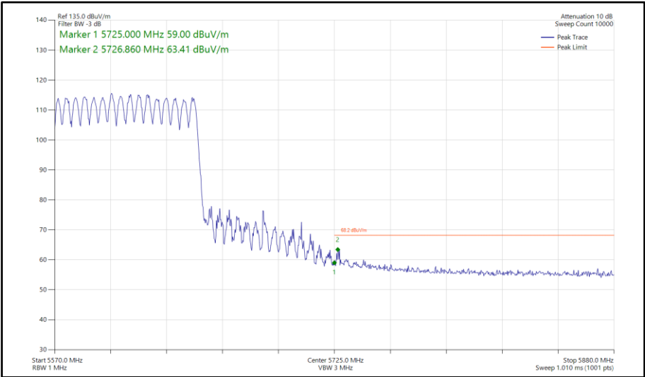
Figure 745 - 802.11ax HE80, SU, CDD, Core 0-1 - 5610 MHz Band Edge Frequency 5725 MHz
