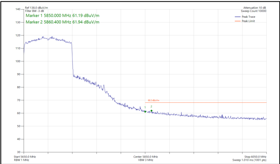
Figure 772 - 802.11ax HE80, SU, SDM, Core 0-1 - 5690 MHz Band Edge Frequency 5850 MHz
