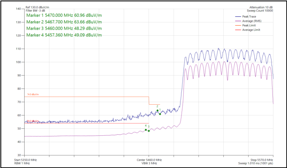
Figure 734 - 802.11ac VHT80, CDD, Core 0-1 - 5530 MHz Band Edge Frequency 5470 MHz
