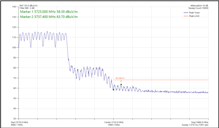
Figure 743 - 802.11a a80, CDD, Core 0-1 - 5610 MHz Band Edge Frequency 5725 MHz
