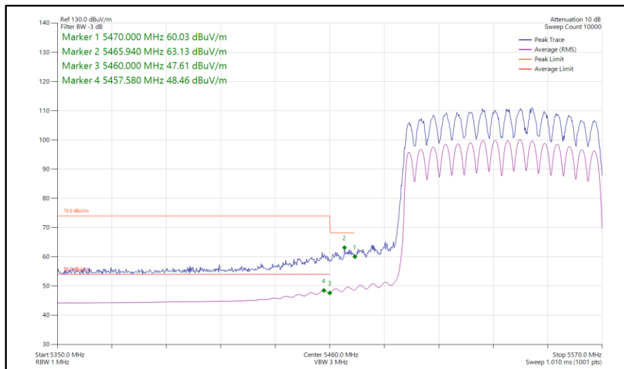
Figure 735 - 802.11ax HE80, SU, CDD, Core 0-1 - 5530 MHz Band Edge Frequency 5470 MHz
