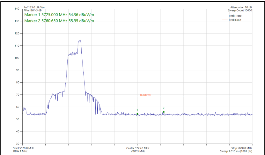
Figure 721 - 802.11ax HE80, RU52-52, SISO, Core 1 - 5610 MHz Band Edge Frequency 5725 MHz
