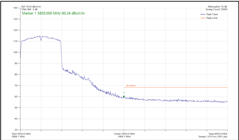
Figure 700 - 802.11ac VHT80, SISO, Core 0 - 5690 MHz Band Edge Frequency 5850 MHz
