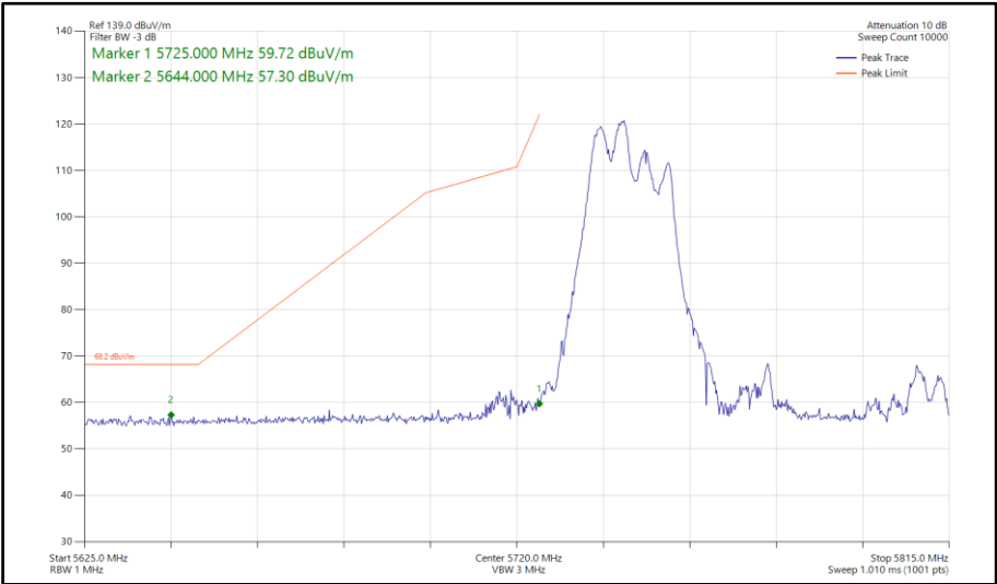
Figure 741 - 802.11ax HE80, RU106-53, CDD, Core 0-1 - 5775 MHz Band Edge Frequency 5725 MHz
