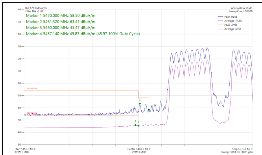
Figure 761 - 802.11be EHT80, RU484+242-92, SDM, Core 0-1 - 5530 MHz Band Edge Frequency 5470 MHz
