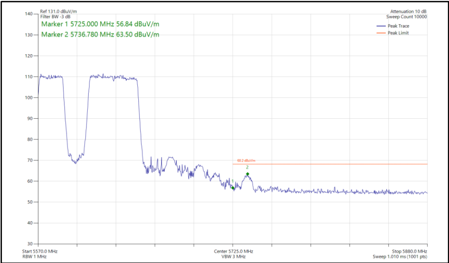
Figure 697 - 802.11be EHT80, RU484+242-91, SISO, Core 0 - 5610 MHz Band Edge Frequency 5725 MHz
