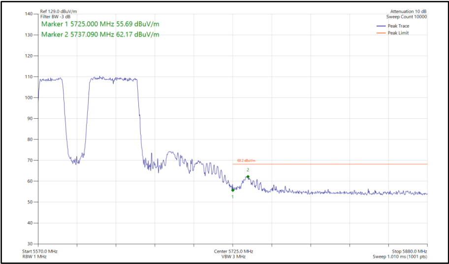
Figure 722 - 802.11be EHT80, RU484+242-91, SISO, Core 1 - 5610 MHz Band Edge Frequency 5725 MHz
