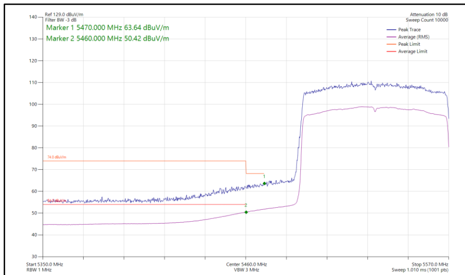
Figure 759 - 802.11ax HE80, SU, SDM, Core 0-1 - 5530 MHz Band Edge Frequency 5470 MHz
