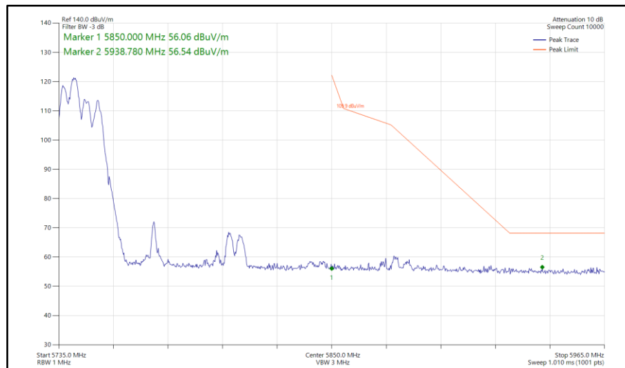
Figure 755 - 802.11ax HE80, RU106-53, CDD, Core 0-1 - 5775 MHz Band Edge Frequency 5850 MHz
