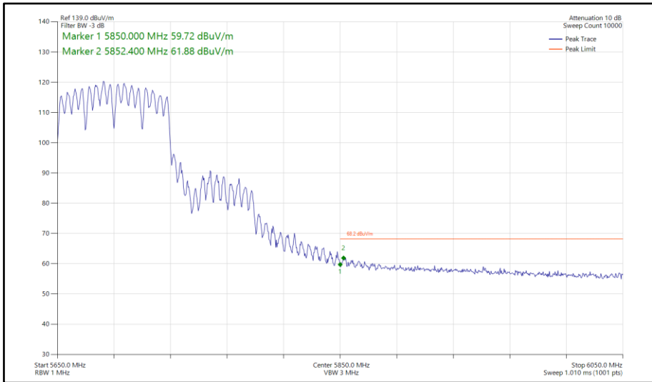
Figure 748 - 802.11a a80, CDD, Core 0-1 - 5690 MHz Band Edge Frequency 5850 MHz
