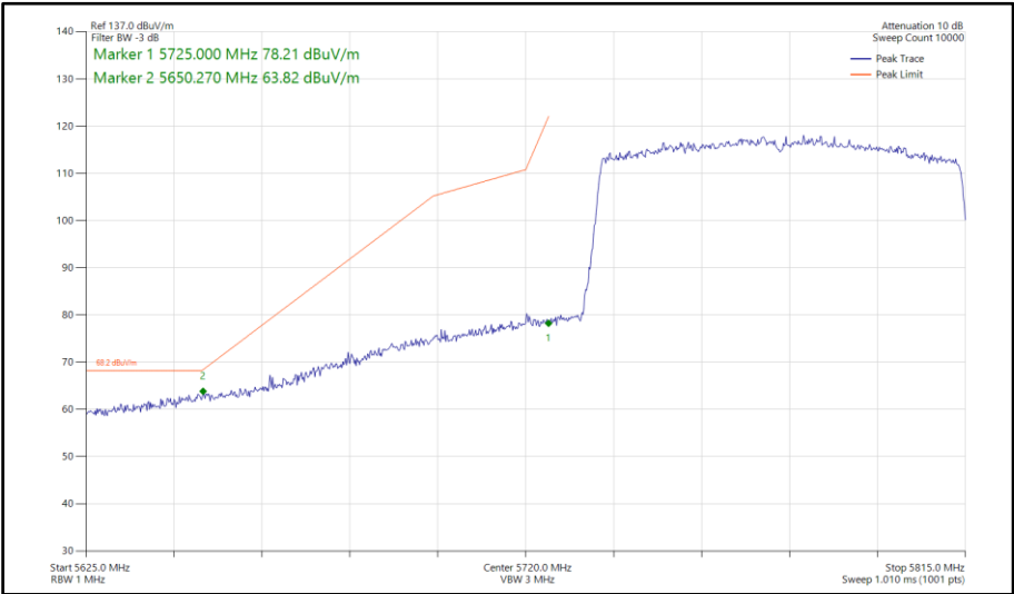
Figure 763 - 802.11ax HE80, SU, SDM, Core 0-1 - 5775 MHz Band Edge Frequency 5725 MHz
