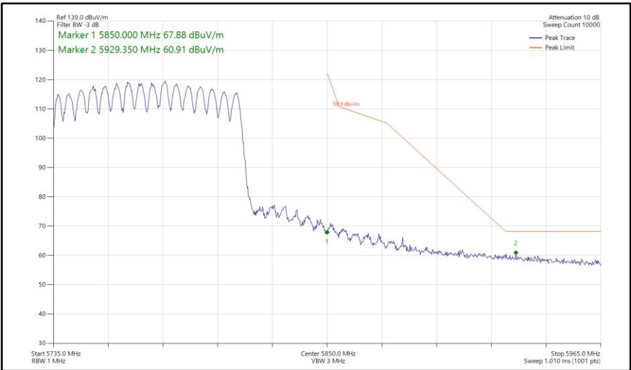
Figure 754 - 802.11ax HE80, SU, CDD, Core 0-1 - 5775 MHz Band Edge Frequency 5850 MHz
