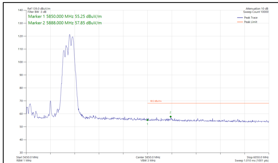
Figure 773 - 802.11ax HE80, RU106-60, SDM, Core 0-1 - 5690 MHz Band Edge Frequency 5850 MHz
