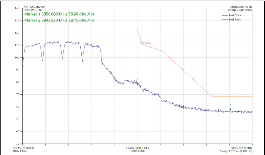
Figure 724 - 802.11a a80, SISO, Core 1 - 5775 MHz Band Edge Frequency 5850 MHz
