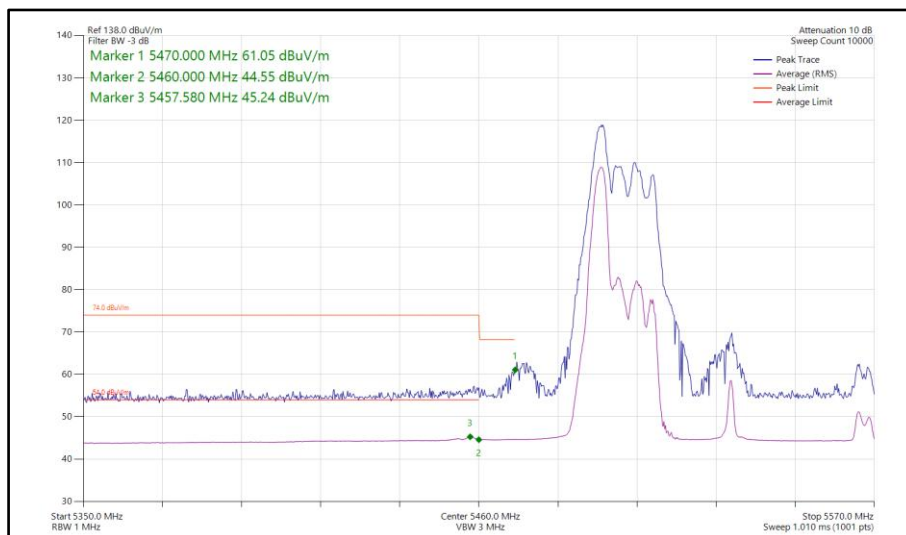
Figure 760 - 802.11ax HE80, RU52-37, SDM, Core 0-1 - 5530 MHz Band Edge Frequency 5470 MHz
