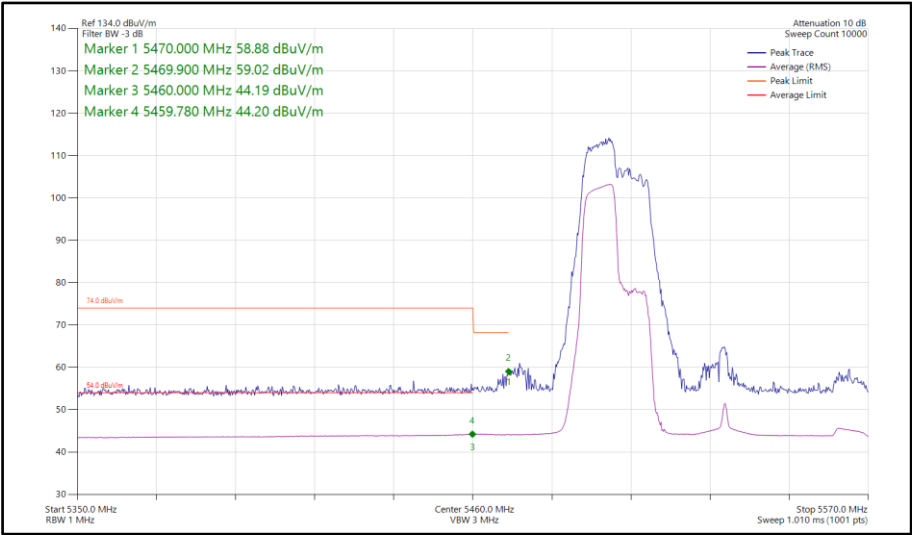
Figure 711 - 802.11ax HE80, RU106-53, SISO, Core 1 - 5530 MHz Band Edge Frequency 5470 MHz
