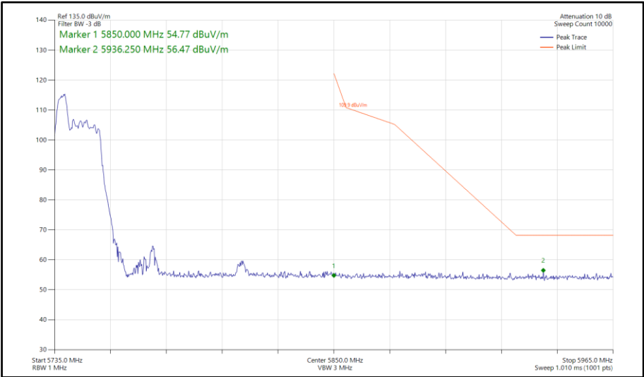
Figure 730 - 802.11ax HE80, RU52-37, SISO, Core 1 - 5775 MHz Band Edge Frequency 5850 MHz
