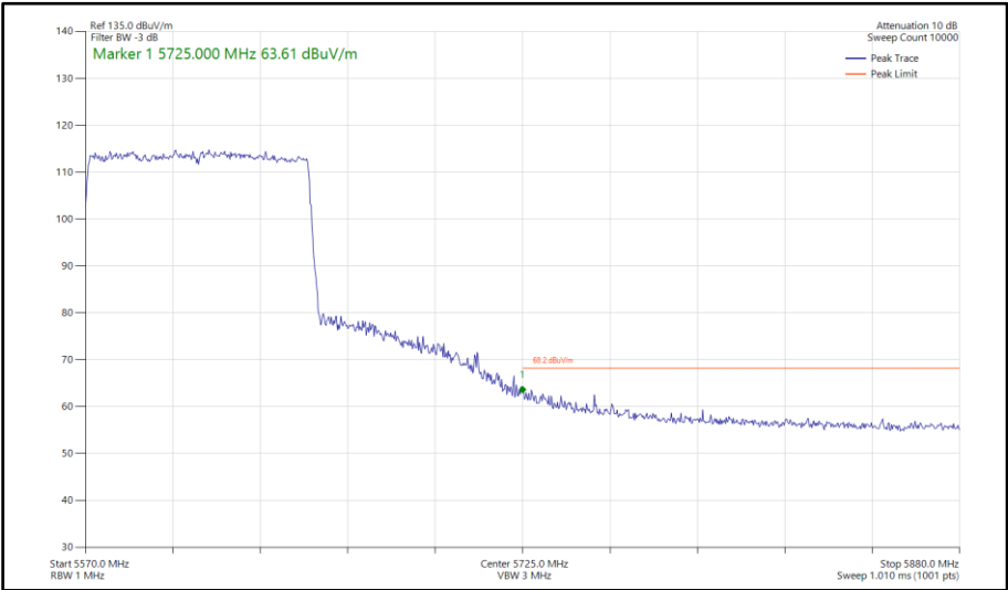
Figure 767 - 802.11ax HE80, SU, SDM, Core 0-1 - 5610 MHz Band Edge Frequency 5725 MHz
