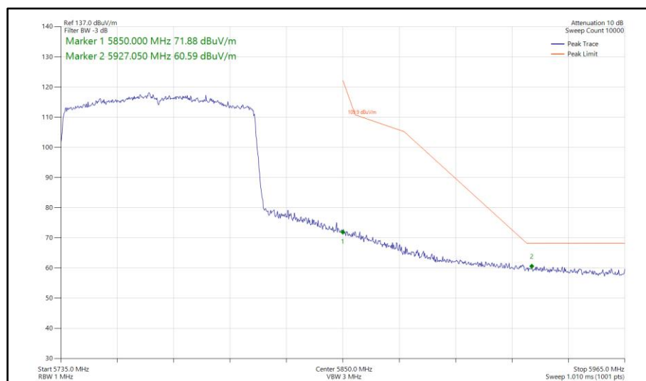
Figure 774 - 802.11ax HE80, SU, SDM, Core 0-1 - 5775 MHz Band Edge Frequency 5850 MHz
