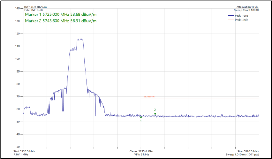
Figure 696 - 802.11ax HE80, RU106-60, SISO, Core 0 - 5610 MHz Band Edge Frequency 5725 MHz
