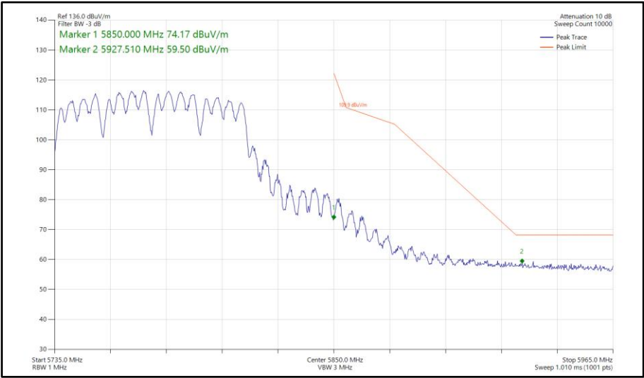
Figure 749 - 802.11a a80, CDD, Core 0-1 - 5775 MHz Band Edge Frequency 5850 MHz
