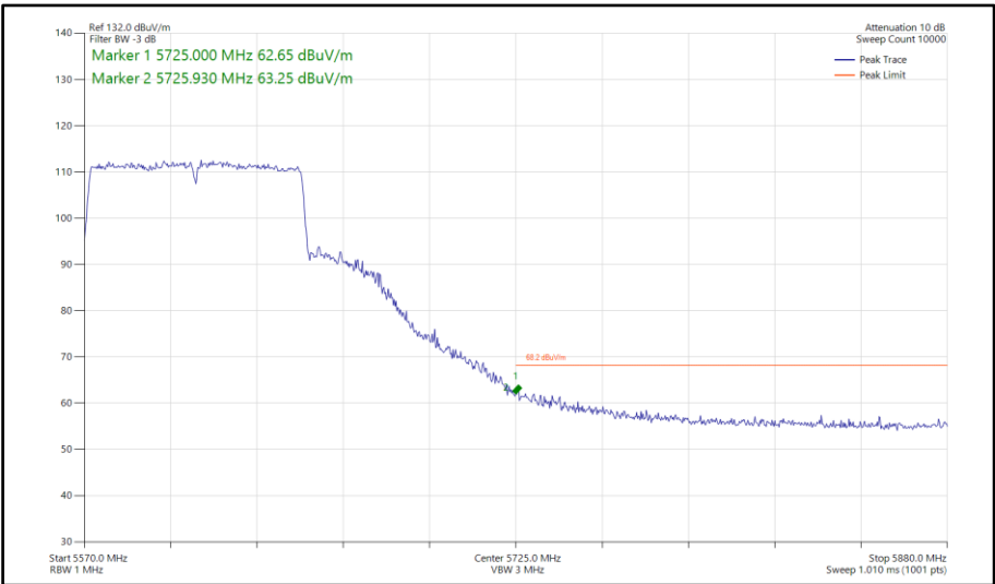
Figure 719 - 802.11ac VHT80, SISO, Core 1 - 5610 MHz Band Edge Frequency 5725 MHz
