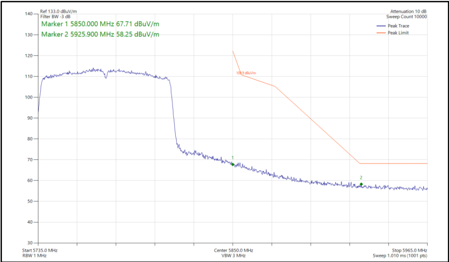
Figure 726 - 802.11ac VHT80, SISO, Core 1 - 5775 MHz Band Edge Frequency 5850 MHz
