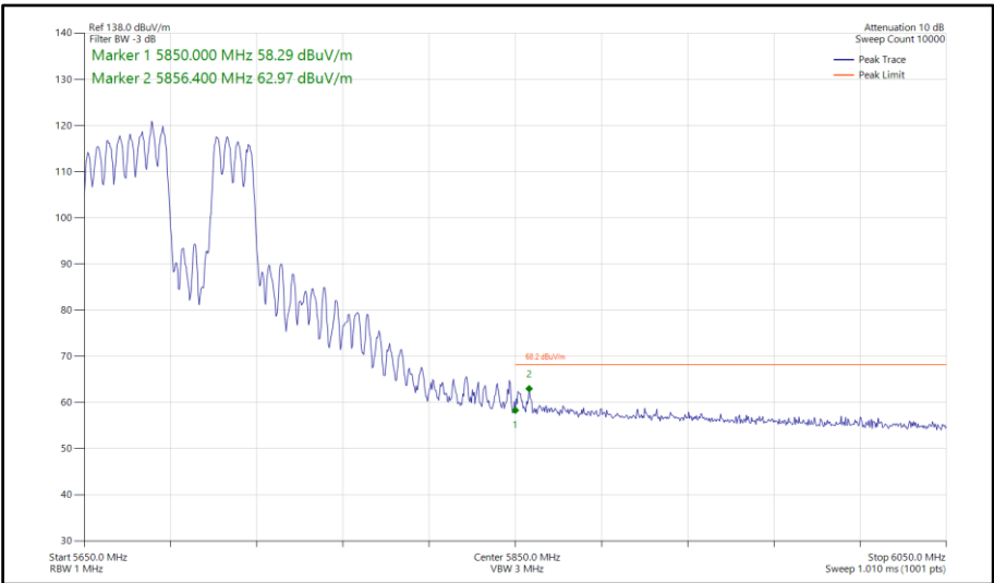
Figure 776 - 802.11be EHT80, RU484+242-92, SDM, Core 0-1 - 5690 MHz Band Edge Frequency 5850 MHz
