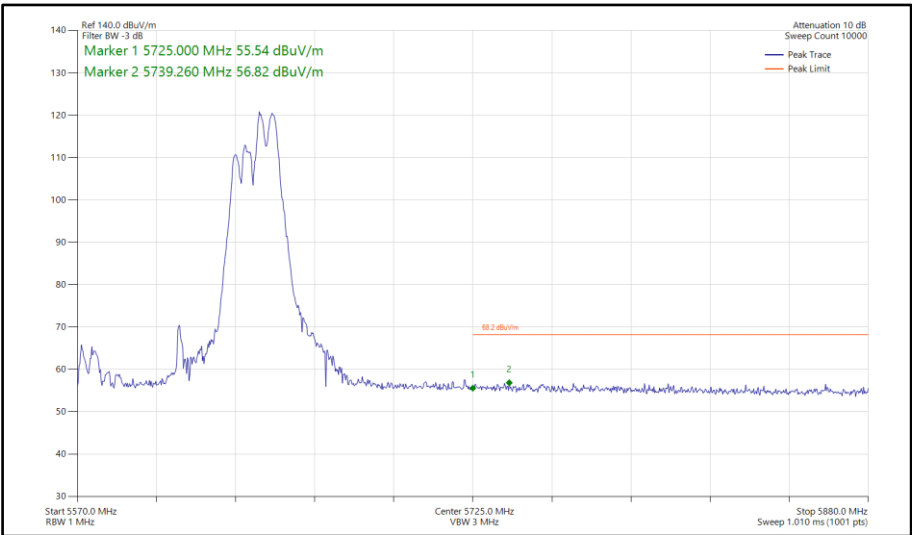
Figure 768 - 802.11ax HE80, RU106-60, SDM, Core 0-1 - 5610 MHz Band Edge Frequency 5725 MHz
