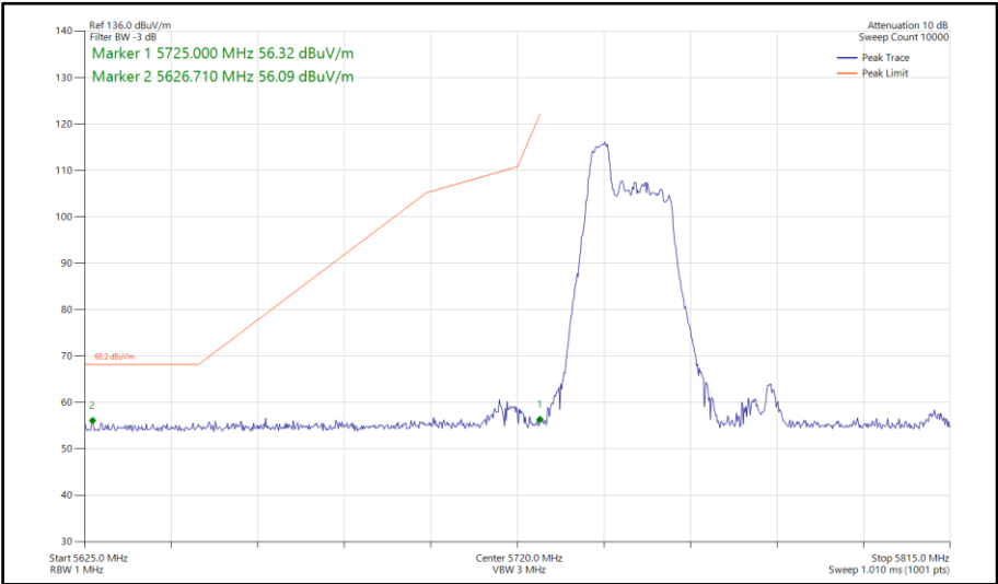
Figure 716 - 802.11ax HE80, RU52-37, SISO, Core 1 - 5775 MHz Band Edge Frequency 5725 MHz
