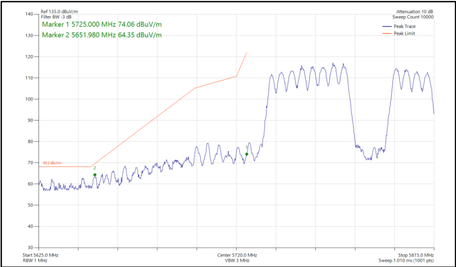
Figure 765 - 802.11be EHT80, RU484+242-92, SDM, Core 0-1 - 5775 MHz Band Edge Frequency 5725 MHz
