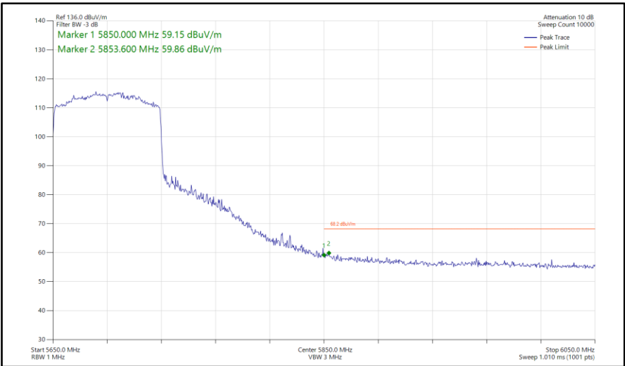
Figure 702 - 802.11ax HE80, SU, SISO, Core 0 - 5690 MHz Band Edge Frequency 5850 MHz
