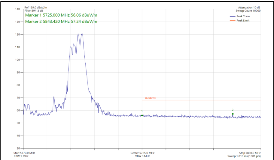
Figure 746 - 802.11ax HE80, RU106-60, CDD, Core 0-1 - 5610 MHz Band Edge Frequency 5725 MHz
