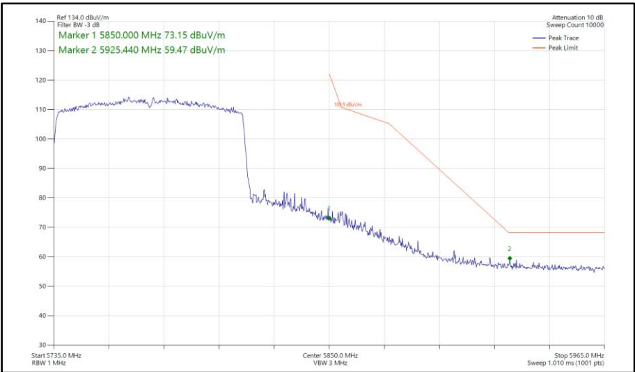
Figure 729 - 802.11ax HE80, SU, SISO, Core 1 - 5775 MHz Band Edge Frequency 5850 MHz
