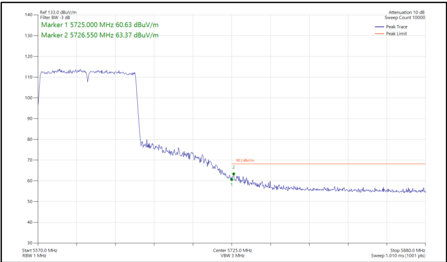
Figure 766 - 802.11ac VHT80, SDM, Core 0-1 - 5610 MHz Band Edge Frequency 5725 MHz
