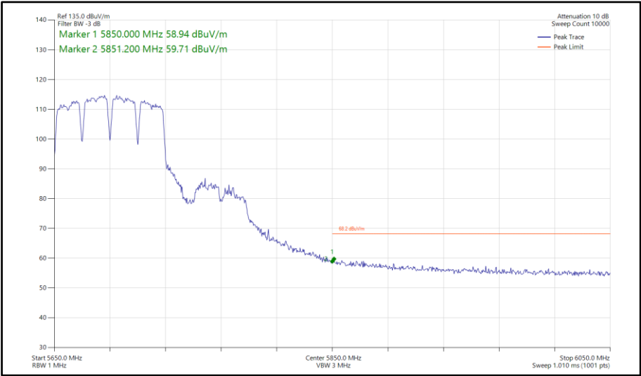
Figure 723 - 802.11a a80, SISO, Core 1 - 5690 MHz Band Edge Frequency 5850 MHz
