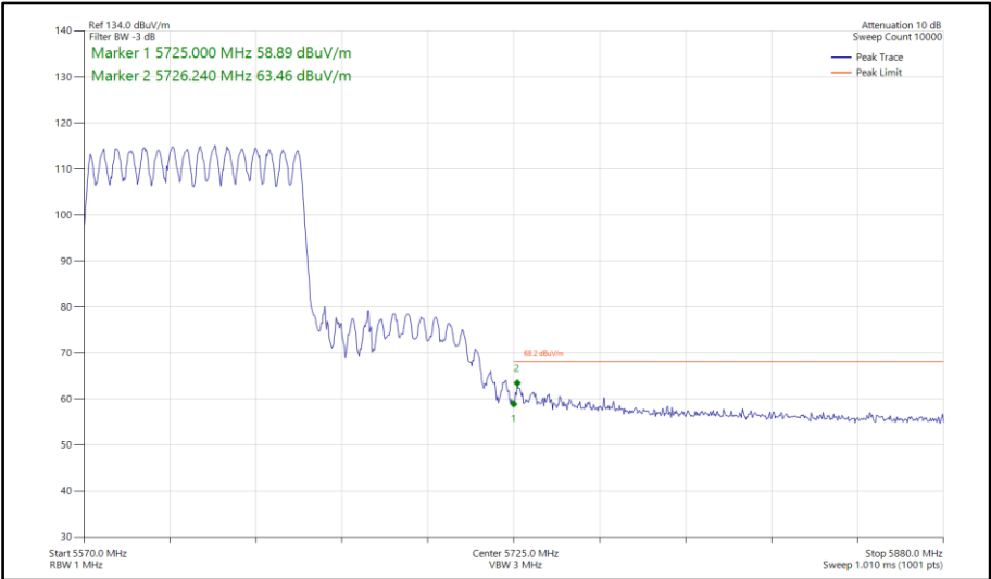
Figure 744 - 802.11ac VHT80, CDD, Core 0-1 - 5610 MHz Band Edge Frequency 5725 MHz
