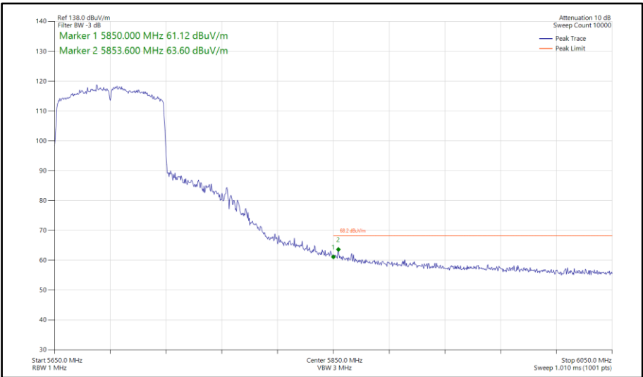
Figure 770 - 802.11ac VHT80, SDM, Core 0-1 - 5690 MHz Band Edge Frequency 5850 MHz
