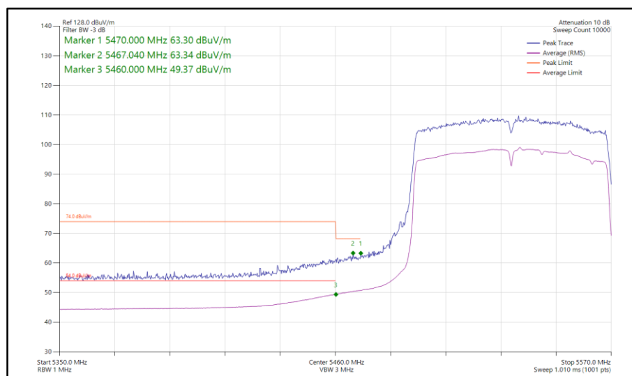
Figure 758 - 802.11ac VHT80, SDM, Core 0-1 - 5530 MHz Band Edge Frequency 5470 MHz
