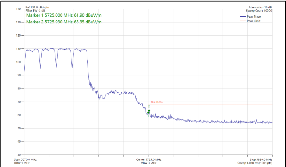
Figure 718 - 802.11a a80, SISO, Core 1 - 5610 MHz Band Edge Frequency 5725 MHz
