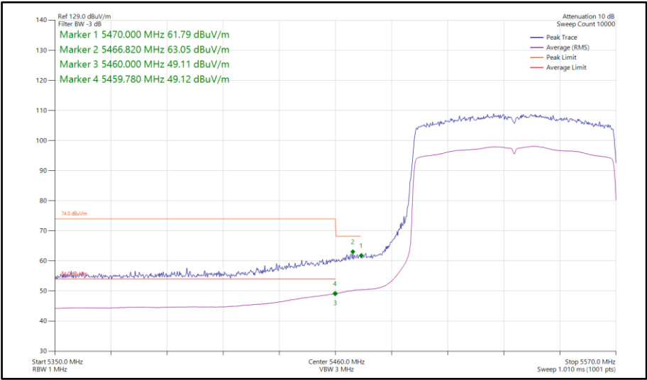
Figure 710 - 802.11ax HE80, SU, SISO, Core 1 - 5530 MHz Band Edge Frequency 5470 MHz
