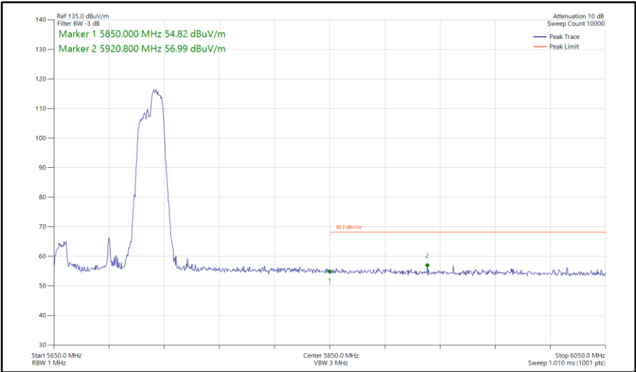
Figure 703 - 802.11ax HE80, RU106-60, SISO, Core 0 - 5690 MHz Band Edge Frequency 5850 MHz
