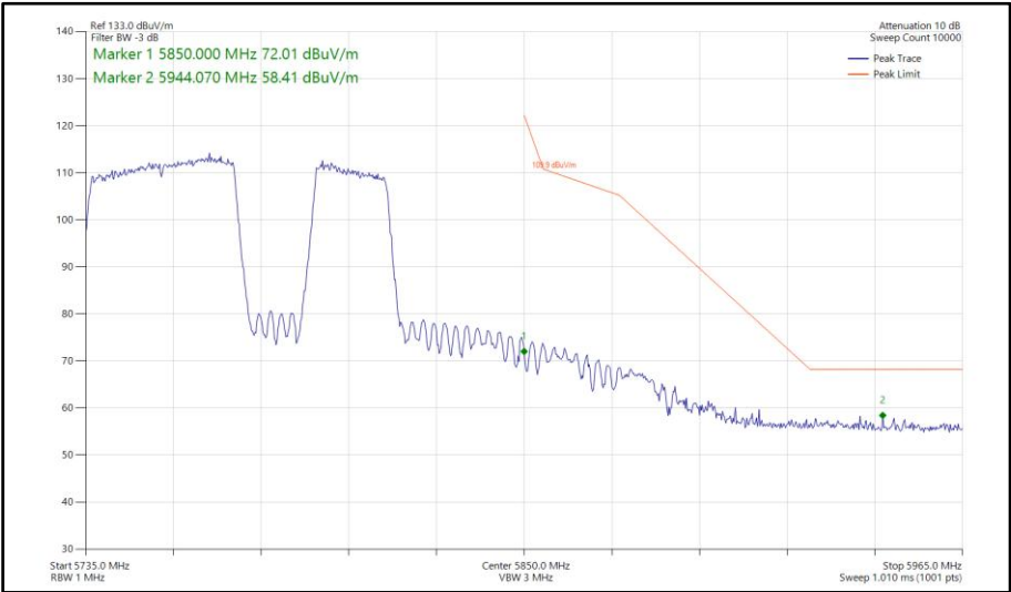
Figure 707 - 802.11be EHT80, RU484+242-92, SISO, Core 0 - 5775 MHz Band Edge Frequency 5850 MHz
