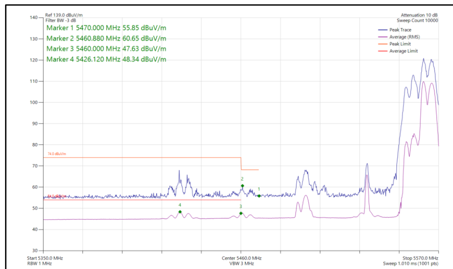
Figure 736 - 802.11ax HE80, RU106-60, CDD, Core 0-1 - 5530 MHz Band Edge Frequency 5470 MHz
