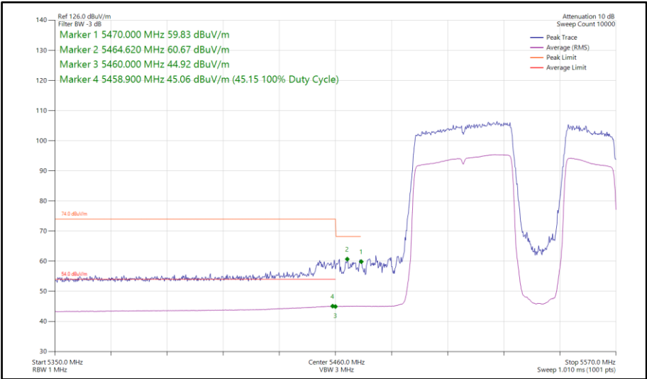
Figure 712 - 802.11be EHT80, RU484+242-92, SISO, Core 1 - 5530 MHz Band Edge Frequency 5470 MHz
