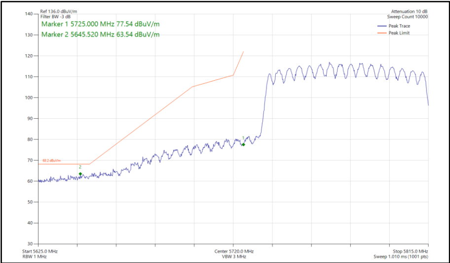
Figure 739 - 802.11ac VHT80, CDD, Core 0-1 - 5775 MHz Band Edge Frequency 5725 MHz
