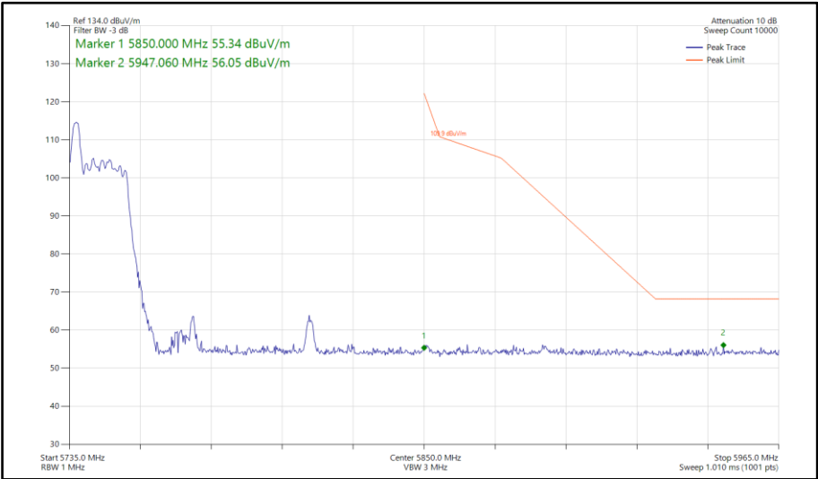
Figure 705 - 802.11ax HE80, RU26-0, SISO, Core 0 - 5775 MHz Band Edge Frequency 5850 MHz
