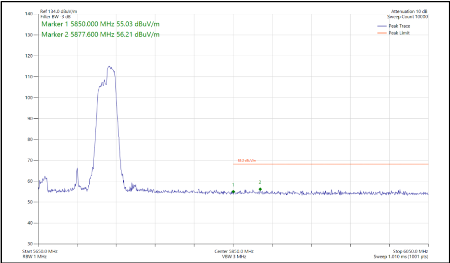
Figure 728 - 802.11ax HE80, RU106-60, SISO, Core 1 - 5690 MHz Band Edge Frequency 5850 MHz
