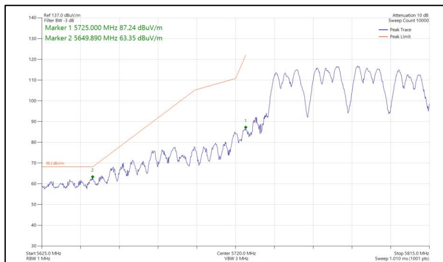
Figure 738 - 802.11a a80, CDD, Core 0-1 - 5775 MHz Band Edge Frequency 5725 MHz
