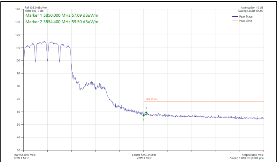
Figure 698 - 802.11a a80, SISO, Core 0 - 5690 MHz Band Edge Frequency 5850 MHz
