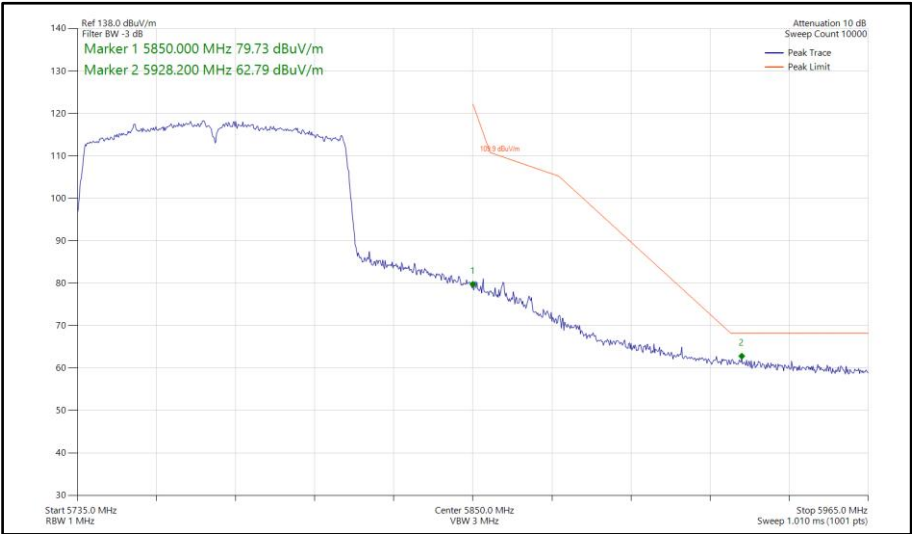
Figure 771 - 802.11ac VHT80, SDM, Core 0-1 - 5775 MHz Band Edge Frequency 5850 MHz
