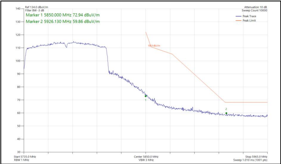
Figure 701 - 802.11ac VHT80, SISO, Core 0 - 5775 MHz Band Edge Frequency 5850 MHz
