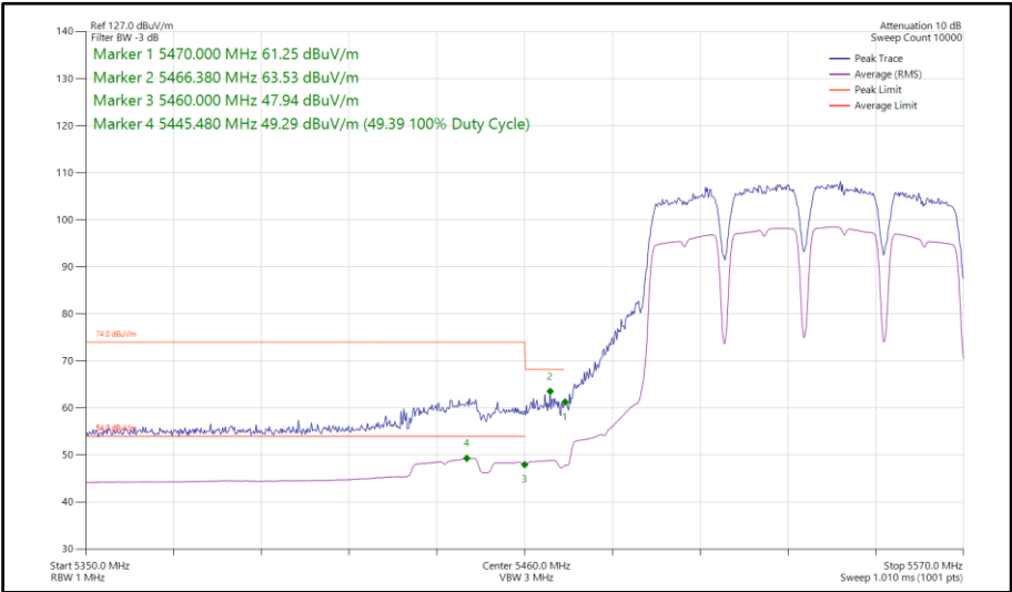
Figure 708 - 802.11a a80, SISO, Core 1 - 5530 MHz Band Edge Frequency 5470 MHz
