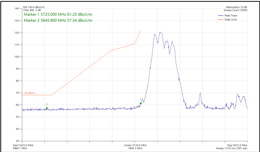
Figure 764 - 802.11ax HE80, RU106-53, SDM, Core 0-1 - 5775 MHz Band Edge Frequency 5725 MHz
