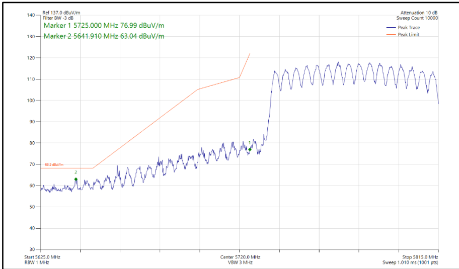
Figure 740 - 802.11ax HE80, SU, CDD, Core 0-1 - 5775 MHz Band Edge Frequency 5725 MHz
