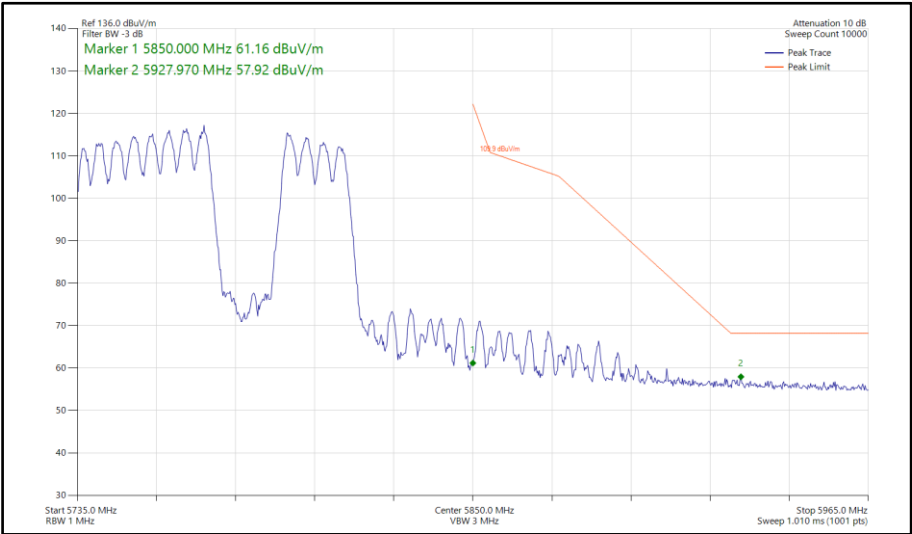
Figure 757 - 802.11be EHT80, RU484+242-92, CDD, Core 0-1 - 5775 MHz Band Edge Frequency 5850 MHz
