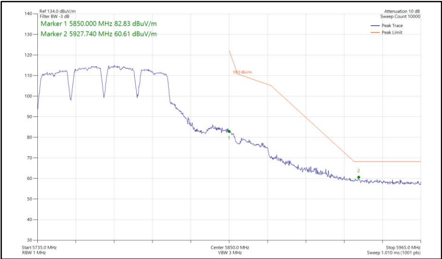
Figure 699 - 802.11a a80, SISO, Core 0 - 5775 MHz Band Edge Frequency 5850 MHz
