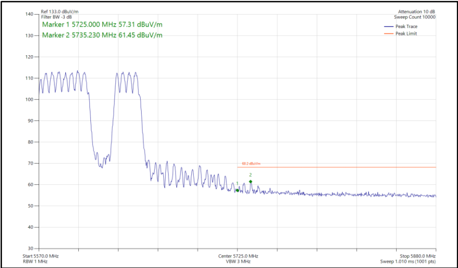
Figure 747 - 802.11be EHT80, RU484+242-92, CDD, Core 0-1 - 5610 MHz Band Edge Frequency 5725 MHz
