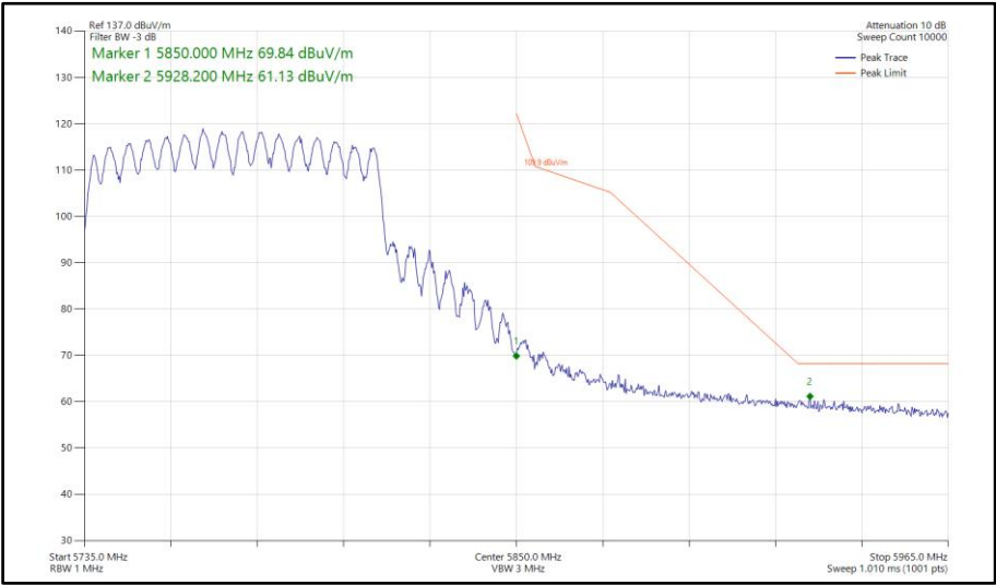
Figure 751 - 802.11ac VHT80, CDD, Core 0-1 - 5775 MHz Band Edge Frequency 5850 MHz
