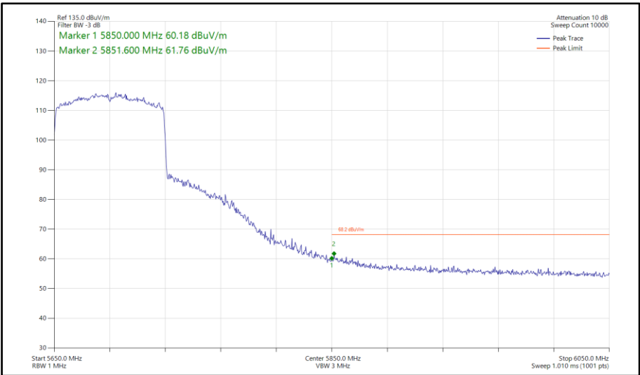
Figure 727 - 802.11ax HE80, SU, SISO, Core 1 - 5690 MHz Band Edge Frequency 5850 MHz
