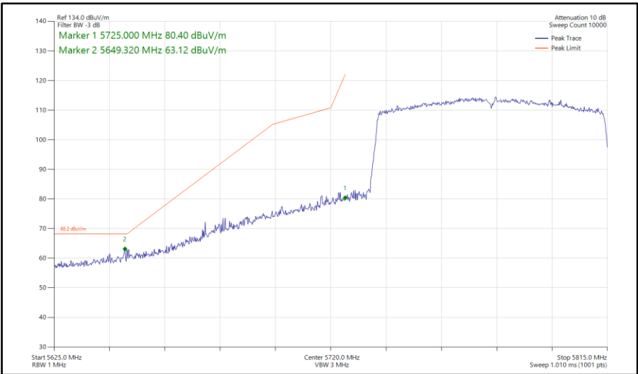
Figure 715 - 802.11ax HE80, SU, SISO, Core 1 - 5775 MHz Band Edge Frequency 5725 MHz
