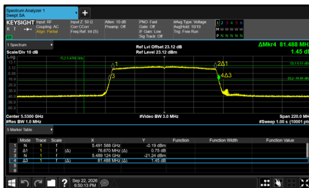
Figure 289 - 802.11ax HE80 SU Minimum 26 dB EBW
