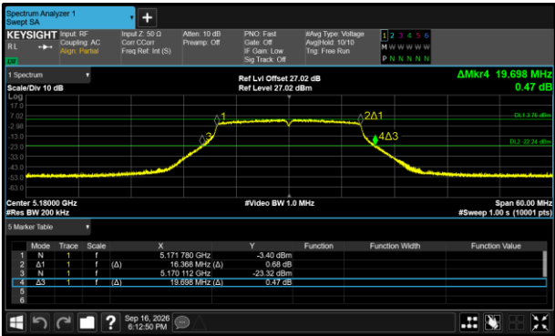
Figure 309 - 802.11a20 Minimum 26 dB EBW
