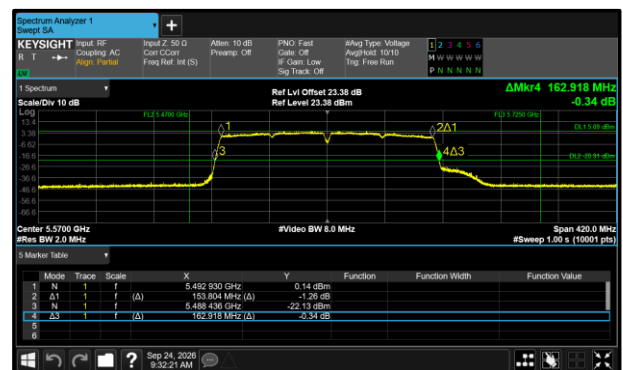
Figure 324 - 802.11ac VHT160 Maximum 26 dB EBW
