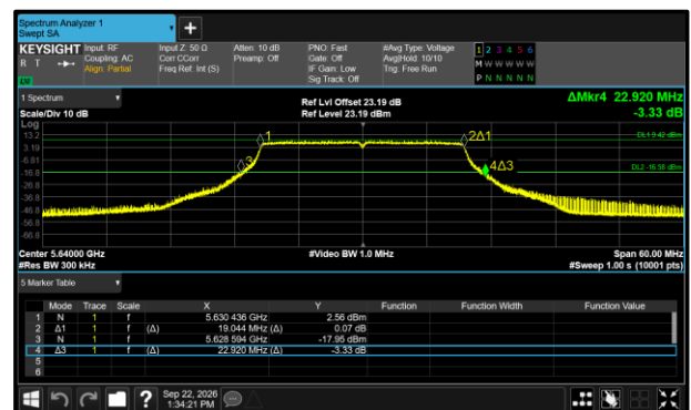
Figure 286 - 802.11ax HE20 SU Maximum 26 dB EBW
