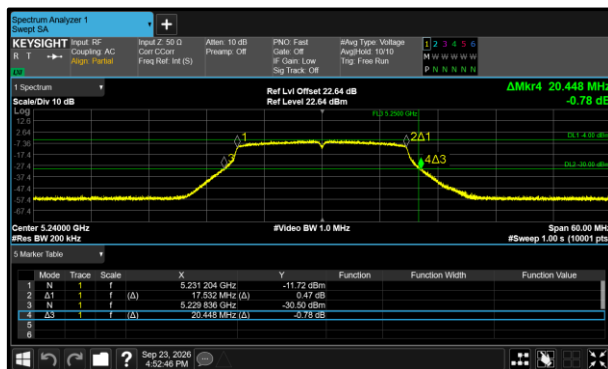
Figure 333 - 802.11ac VHT20 Minimum 99% OBW
