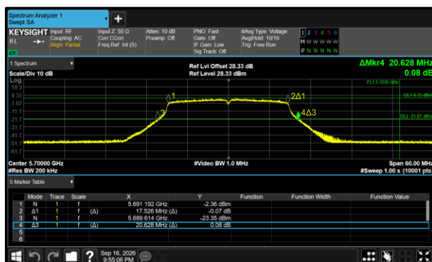
Figure 293 - 802.11n HT20 Minimum 26 dB EBW
