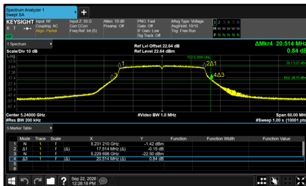
Figure 277 - 802.11n HT20 Minimum 26 dB EBW
