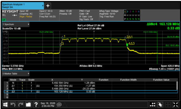
Figure 275 - 802.11a160 Minimum 26 dB EBW
