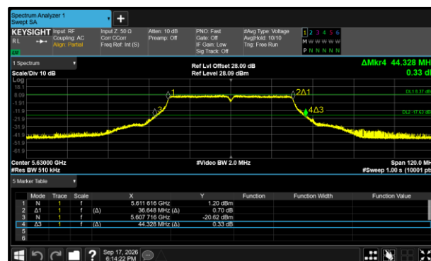
Figure 296 - 802.11n HT40 Maximum 26 dB EBW
