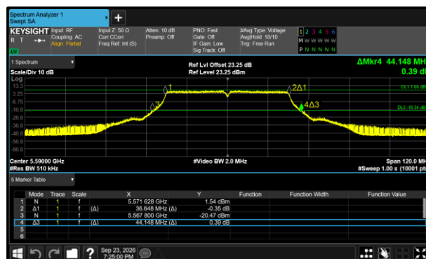
Figure 336 - 802.11ac VHT40 Maximum 99% OBW
