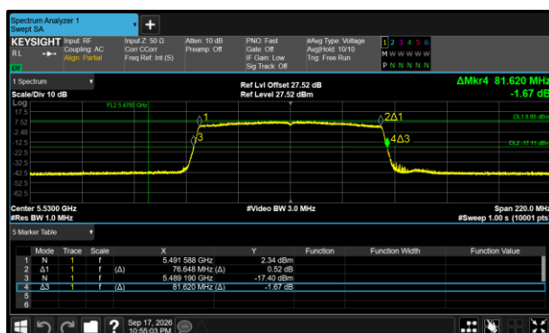
Figure 265 - 802.11ax HE80 SU Minimum 26 dB EBW
