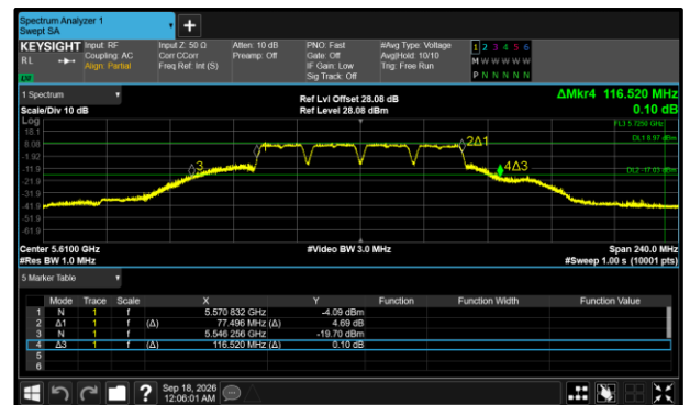
Figure 314 - 802.11a80 Maximum 26 dB EBW
