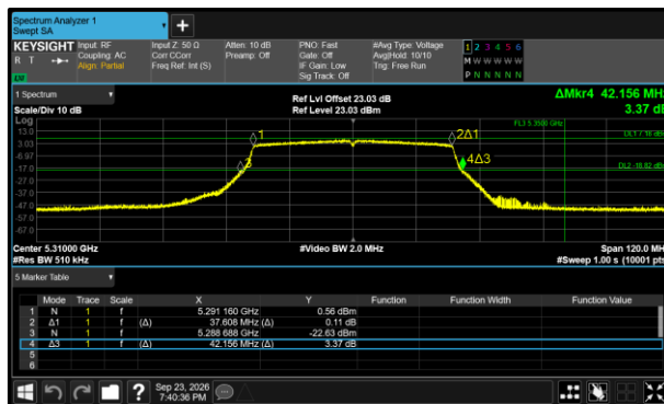
Figure 327 - 802.11ax HE40 SU Minimum 26 dB EBW
