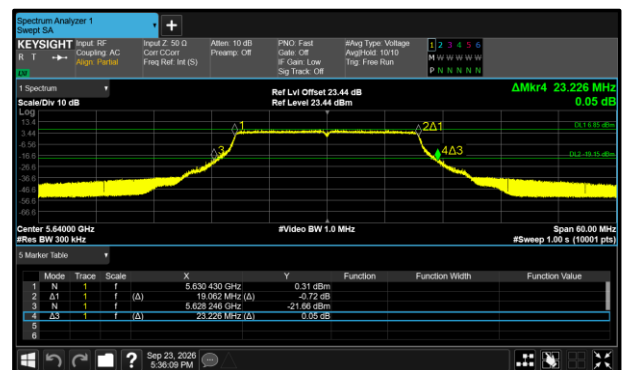
Figure 326 - 802.11ax HE20 SU Maximum 26 dB EBW
