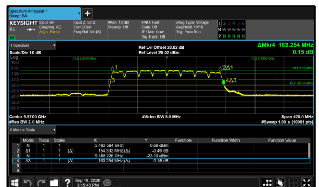
Figure 316 - 802.11a160 Maximum 26 dB EBW
