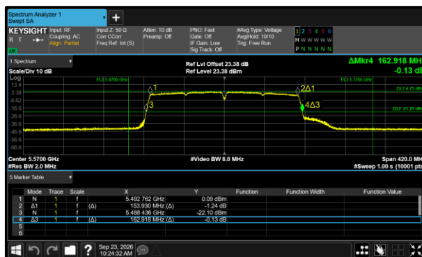
Figure 283 - 802.11ac VHT160 Minimum 26 dB EBW
