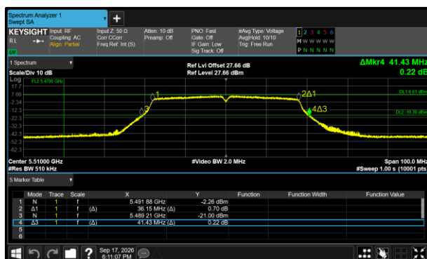
Figure 295 - 802.11n HT40 Minimum 26 dB EBW
