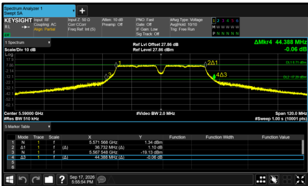
Figure 312 - 802.11a40 Maximum 26 dB EBW
