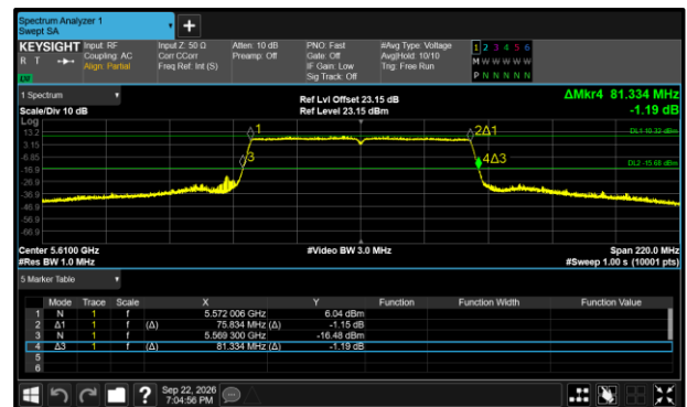
Figure 282 - 802.11ac VHT80 Maximum 26 dB EBW
