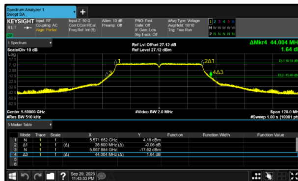
Figure 280 - 802.11n HT40 Maximum 26 dB EBW
