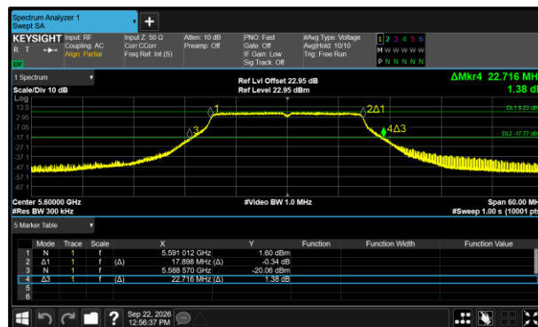
Figure 278 - 802.11n HT20 Maximum 26 dB EBW
