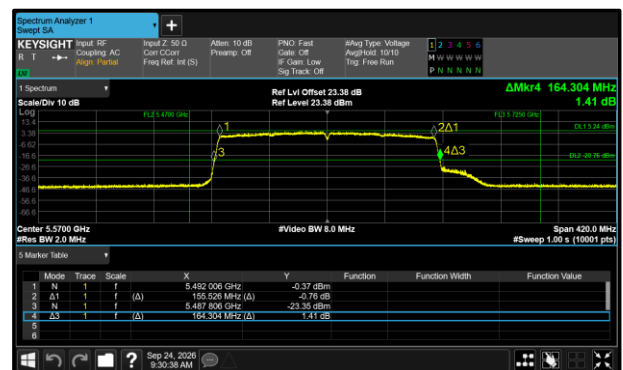
Figure 332 - 802.11ax HE160 SU Maximum 26 dB EBW
