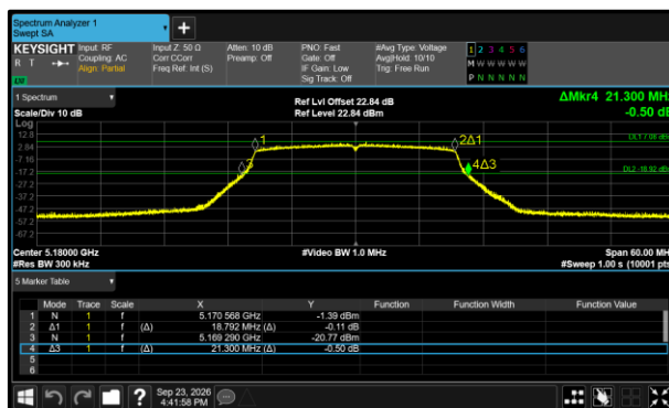
Figure 325 - 802.11ax HE20 SU Minimum 26 dB EBW
