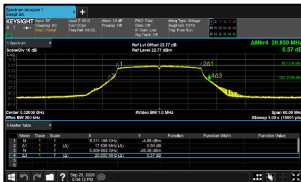
Figure 317 - 802.11ac VHT20 Minimum 26 dB EBW
