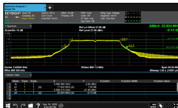
Figure 294 - 802.11n HT20 Maximum 26 dB EBW
