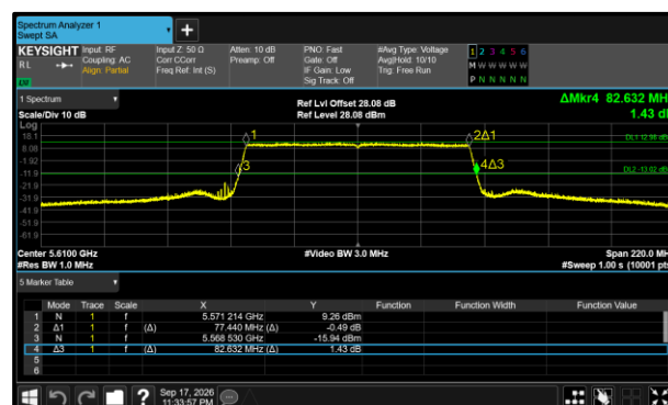
Figure 266 - 802.11ax HE80 SU Maximum 26 dB EBW
