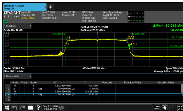
Figure 281 - 802.11ac VHT80 Minimum 26 dB EBW
