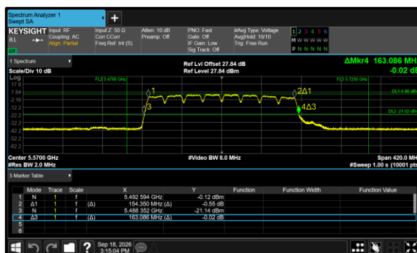
Figure 315 - 802.11a160 Minimum 26 dB EBW
