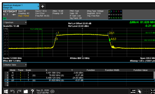
Figure 329 - 802.11ax HE80 SU Minimum 26 dB EBW
