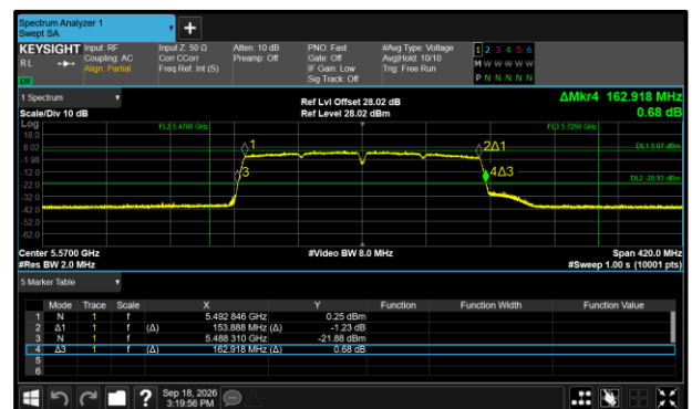
Figure 300 - 802.11ac VHT160 Maximum 26 dB EBW
