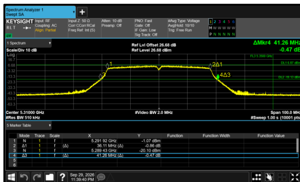
Figure 279 - 802.11n HT40 Minimum 26 dB EBW
