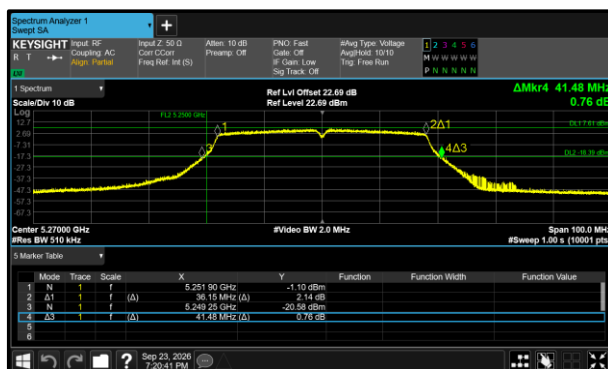
Figure 319 - 802.11ac VHT40 Minimum 26 dB EBW
