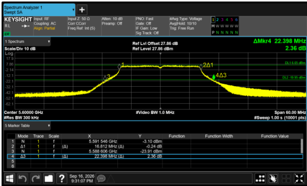
Figure 310 - 802.11a20 Maximum 26 dB EBW
