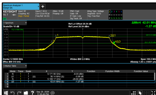
Figure 335 - 802.11ac VHT40 Minimum 99% OBW
