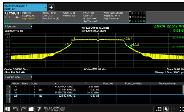
Figure 334 - 802.11ac VHT20 Maximum 99% OBW
