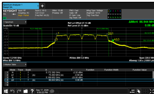
Figure 313 - 802.11a80 Minimum 26 dB EBW
