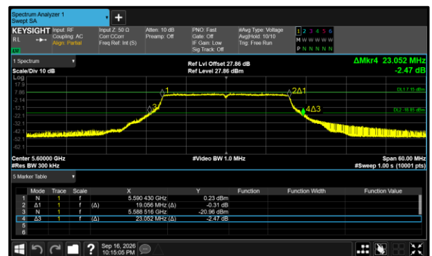
Figure 302 - 802.11ax HE20 SU Maximum 26 dB EBW
