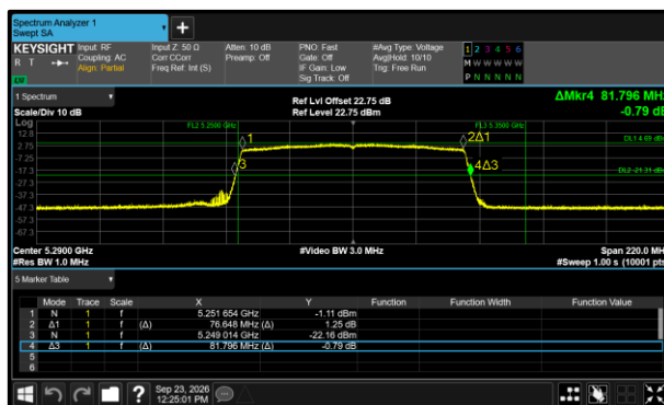
Figure 345 - 802.11ax HE80 SU Minimum 99% OBW
