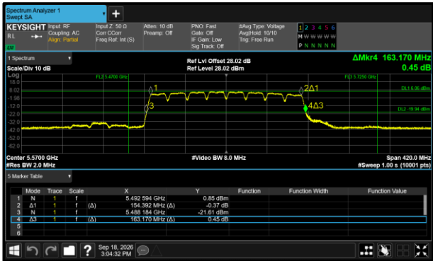
Figure 276 - 802.11a160 Maximum 26 dB EBW
