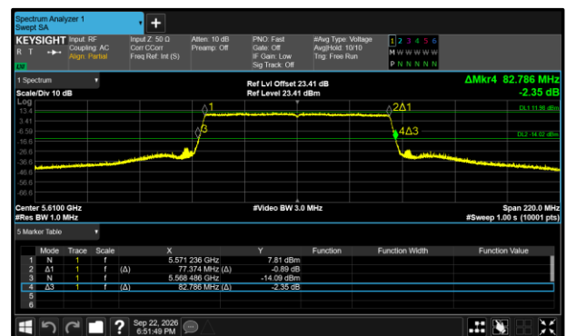
Figure 290 - 802.11ax HE80 SU Maximum 26 dB EBW
