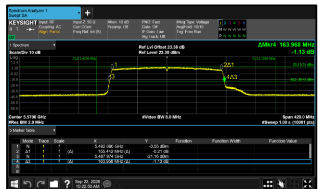
Figure 292 - 802.11ax HE160 SU Maximum 26 dB EBW
