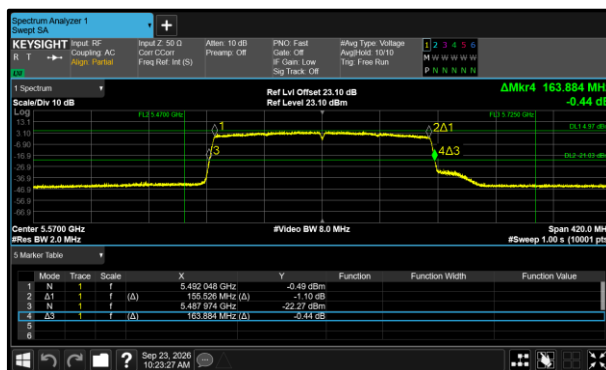
Figure 291 - 802.11ax HE160 SU Minimum 26 dB EBW
