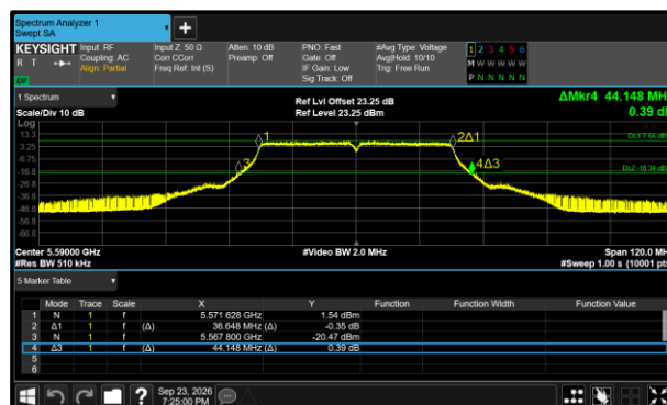
Figure 320 - 802.11ac VHT40 Maximum 26 dB EBW
