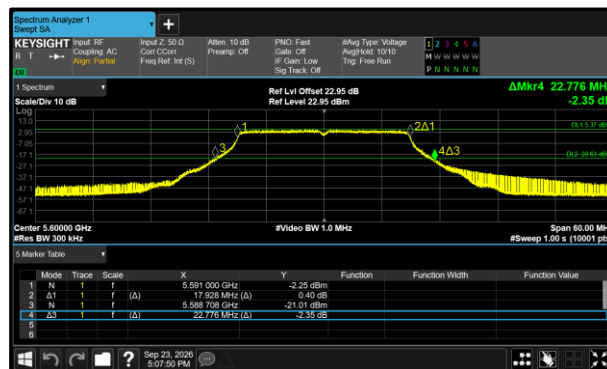
Figure 318 - 802.11ac VHT20 Maximum 26 dB EBW
