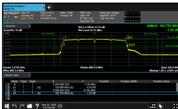
Figure 323 - 802.11ac VHT160 Minimum 26 dB EBW
