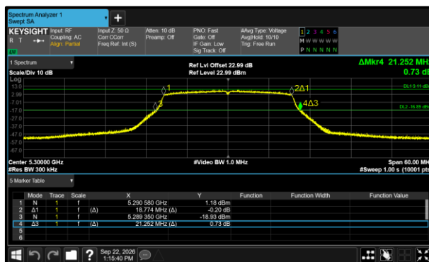
Figure 285 - 802.11ax HE20 SU Minimum 26 dB EBW
