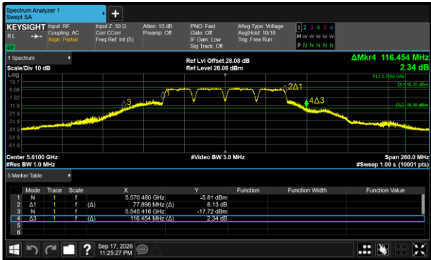
Figure 274 - 802.11a80 Maximum 26 dB EBW
