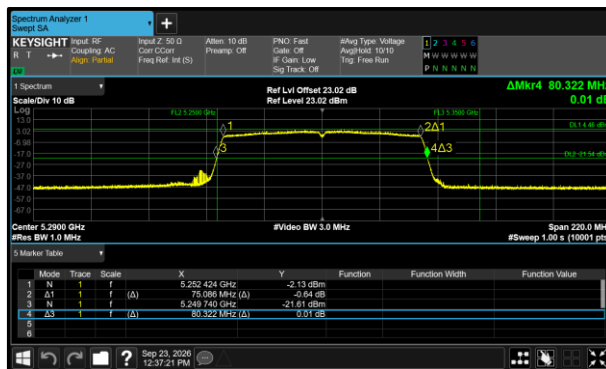
Figure 321 - 802.11ac VHT80 Minimum 26 dB EBW
