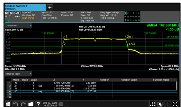
Figure 284 - 802.11ac VHT160 Maximum 26 dB EBW
