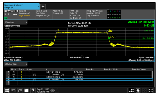
Figure 330 - 802.11ax HE80 SU Maximum 26 dB EBW
