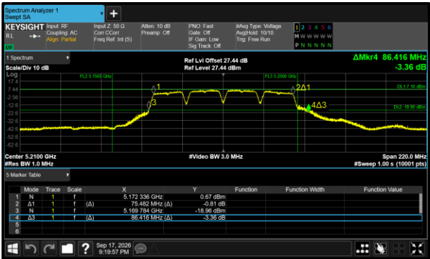
Figure 273 - 802.11a80 Minimum 26 dB EBW
