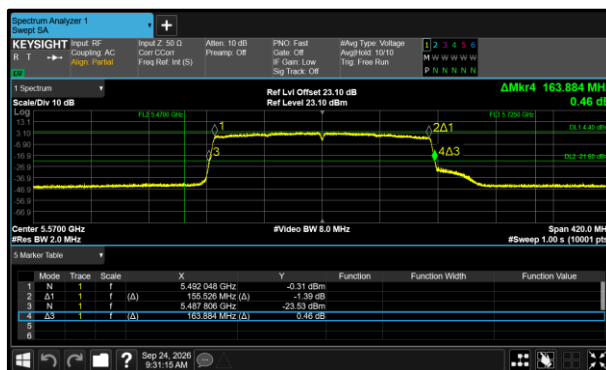
Figure 331 - 802.11ax HE160 SU Minimum 26 dB EBW
