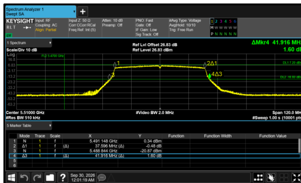
Figure 287 - 802.11ax HE40 SU Minimum 26 dB EBW
