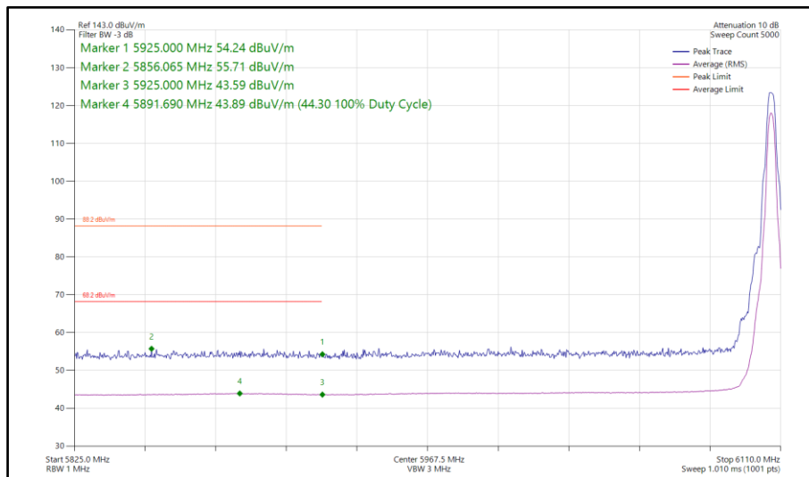
Figure 312 - Narrowband HDT6, MIMO, Core 0-1 - 6106 MHz Band Edge Frequency 5925 MHz
