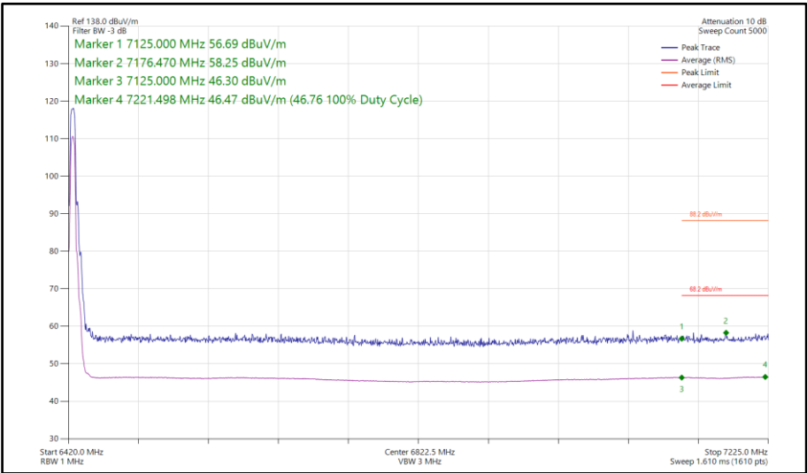
Figure 266 - Narrowband HDRPM12, SISO, Core 0 - 6425 MHz Band Edge Frequency 7125 MHz
