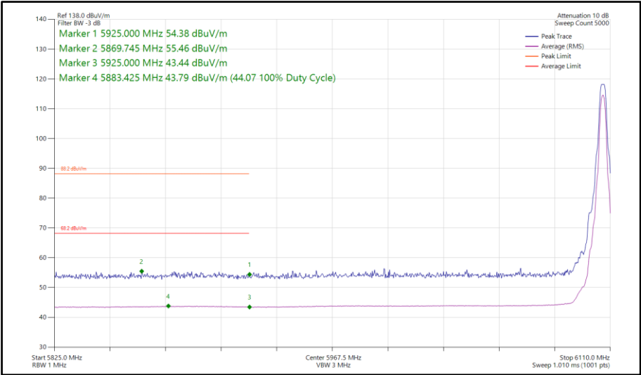
Figure 279 - Narrowband HDT4, SISO, Core 1 - 6106 MHz Band Edge Frequency 5925 MHz
