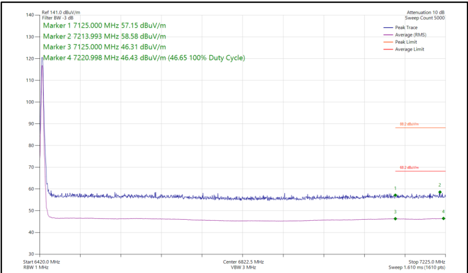
Figure 294 - Narrowband HDT3, SISO, Core 1 - 6425 MHz Band Edge Frequency 7125 MHz
