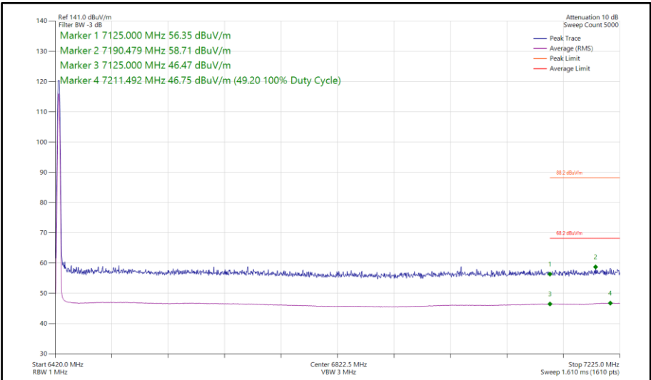
Figure 304 - Narrowband CS1LE2M, SISO, Core 1 - 6425 MHz Band Edge Frequency 7125 MHz
