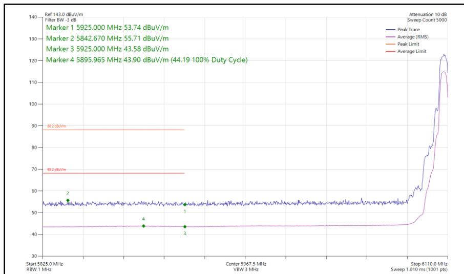
Figure 314 - Narrowband HDRPM12, MIMO, Core 0-1 - 6107 MHz Band Edge Frequency 5925 MHz
