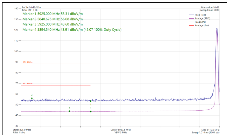
Figure 305 - Narrowband DH5, MIMO, Core 0-1 - 6106 MHz Band Edge Frequency 5925 MHz
