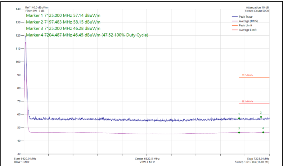
Figure 258 - Narrowband HDR4, SISO, Core 0 - 6425 MHz Band Edge Frequency 7125 MHz
