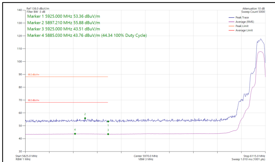
Figure 284 - Narrowband HDRPL24, SISO, Core 1 - 6109 MHz Band Edge Frequency 5925 MHz
