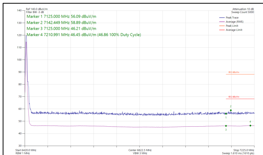
Figure 264 - Narrowband HDT6, SISO, Core 0 - 6425 MHz Band Edge Frequency 7125 MHz
