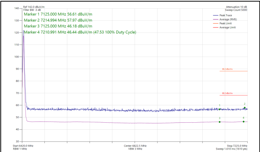
Figure 322 - Narrowband HDR4, MIMO, Core 0-1 - 6425 MHz Band Edge Frequency 7125 MHz
