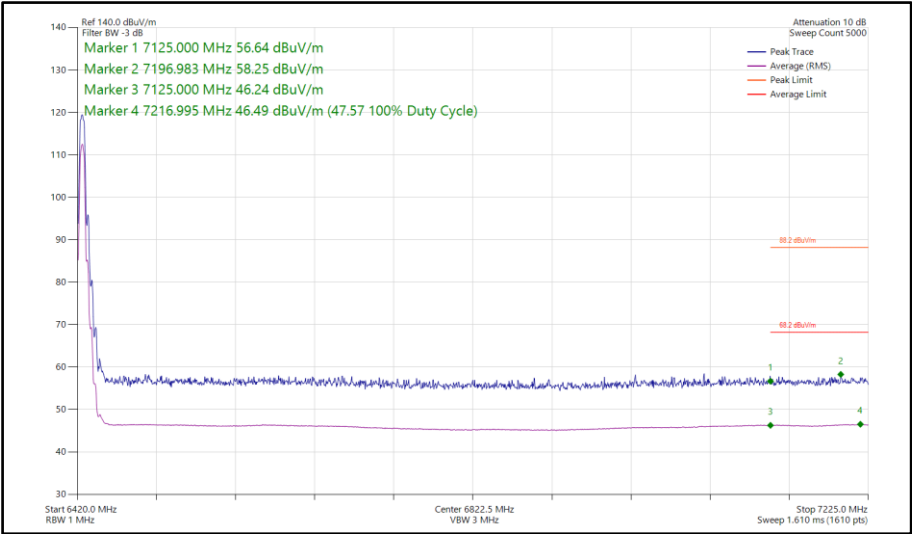
Figure 259 - Narrowband HDR8, SISO, Core 0 - 6425 MHz Band Edge Frequency 7125 MHz
