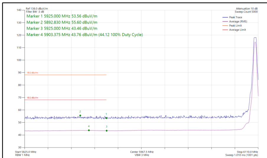
Figure 281 - Narrowband HDRPS2, SISO, Core 1 - 6106 MHz Band Edge Frequency 5925 MHz
