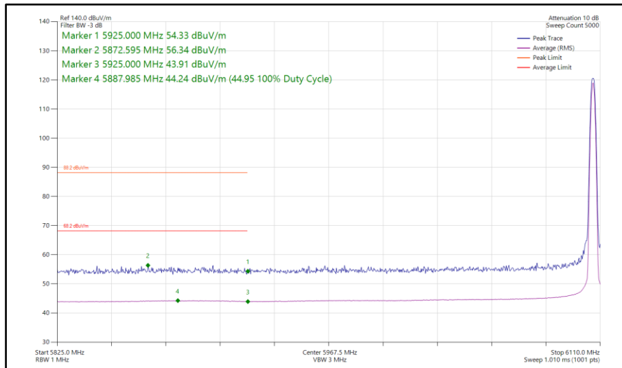
Figure 255 - Narrowband CS1LE1M, SISO, Core 0 - 6106 MHz Band Edge Frequency 5925 MHz
