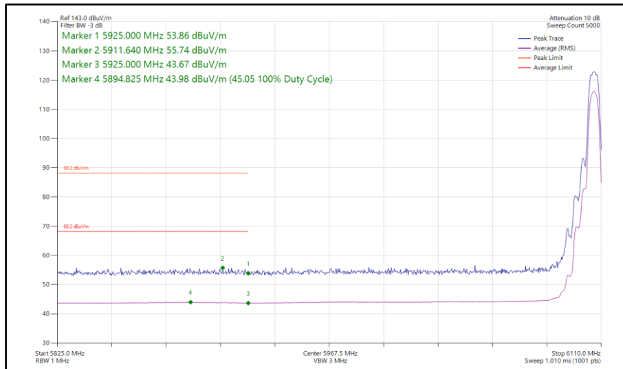
Figure 307 - Narrowband HDR8, MIMO, Core 0-1 - 6106 MHz Band Edge Frequency 5925 MHz
