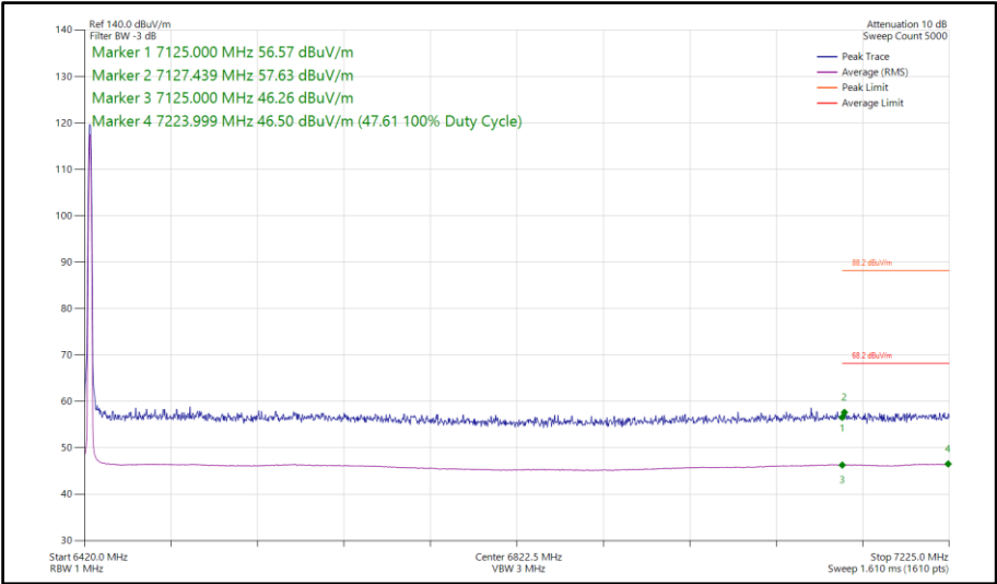
Figure 257 - Narrowband DH5, SISO, Core 0 - 6425 MHz Band Edge Frequency 7125 MHz
