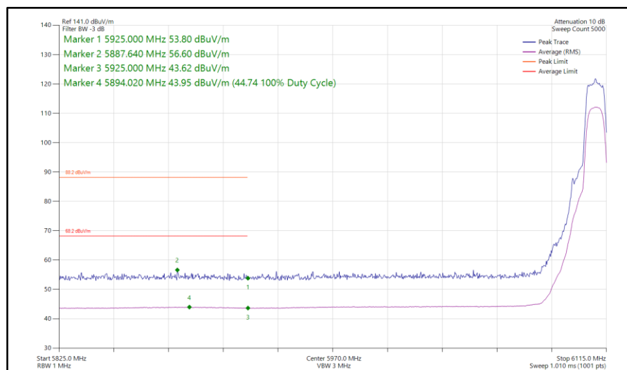
Figure 318 - Narrowband XHDRPL24, MIMO, Core 0-1 - 6109 MHz Band Edge Frequency 5925 MHz
