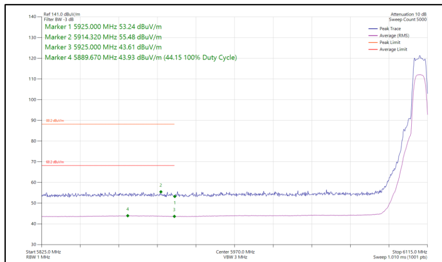
Figure 315 - Narrowband HDRPL8, MIMO, Core 0-1 - 6109 MHz Band Edge Frequency 5925 MHz
