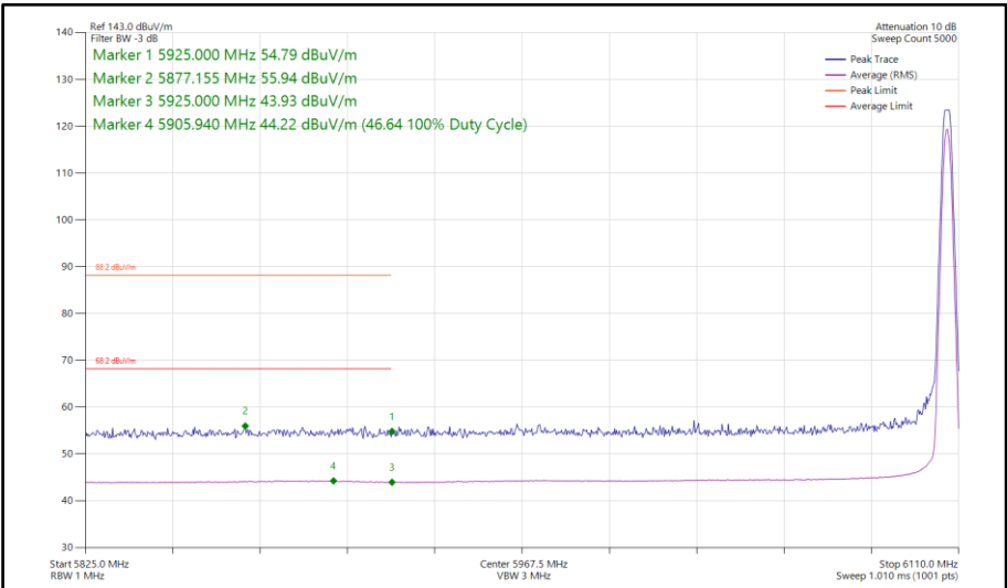
Figure 320 - Narrowband CS1LE2M, MIMO, Core 0-1 - 6106 MHz Band Edge Frequency 5925 MHz
