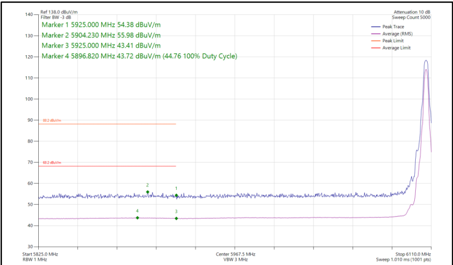
Figure 274 - Narrowband HDR4, SISO, Core 1 - 6106 MHz Band Edge Frequency 5925 MHz
