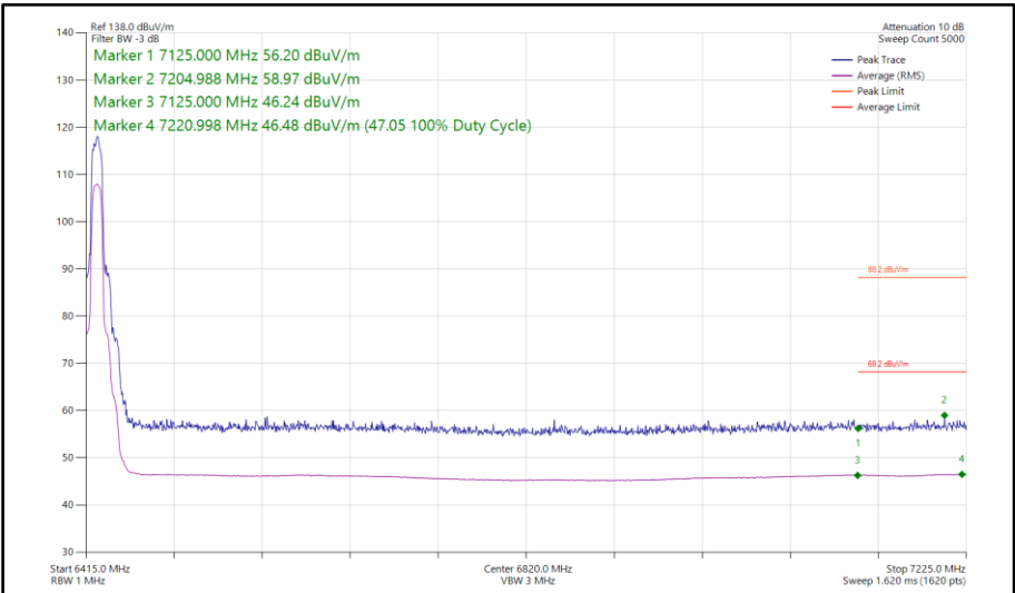
Figure 268 - Narrowband HDRPL24, SISO, Core 0 - 6425 MHz Band Edge Frequency 7125 MHz
