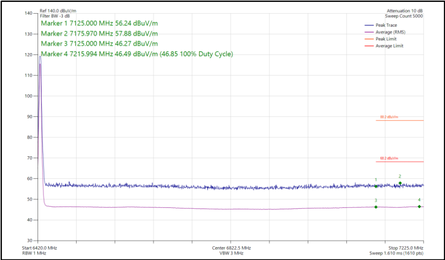
Figure 265 - Narrowband HDRPS2, SISO, Core 0 - 6425 MHz Band Edge Frequency 7125 MHz
