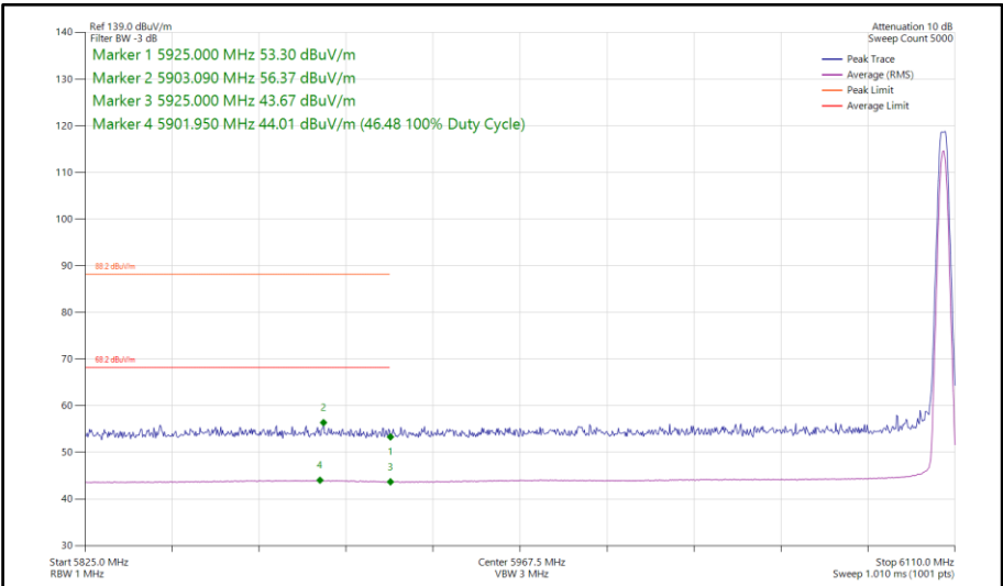
Figure 288 - Narrowband CS1LE2M, SISO, Core 1 - 6106 MHz Band Edge Frequency 5925 MHz
