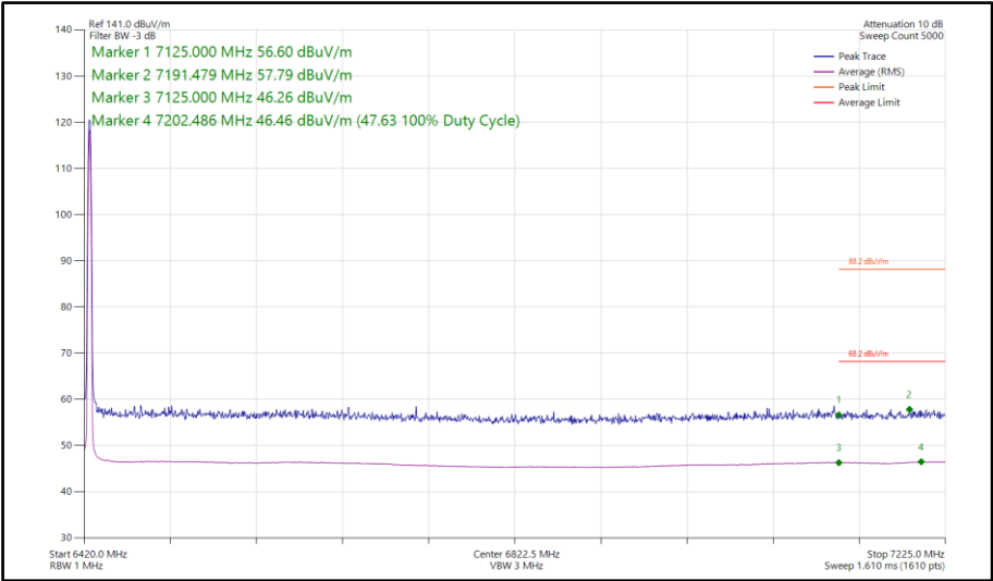
Figure 289 - Narrowband DH5, SISO, Core 1 - 6425 MHz Band Edge Frequency 7125 MHz
