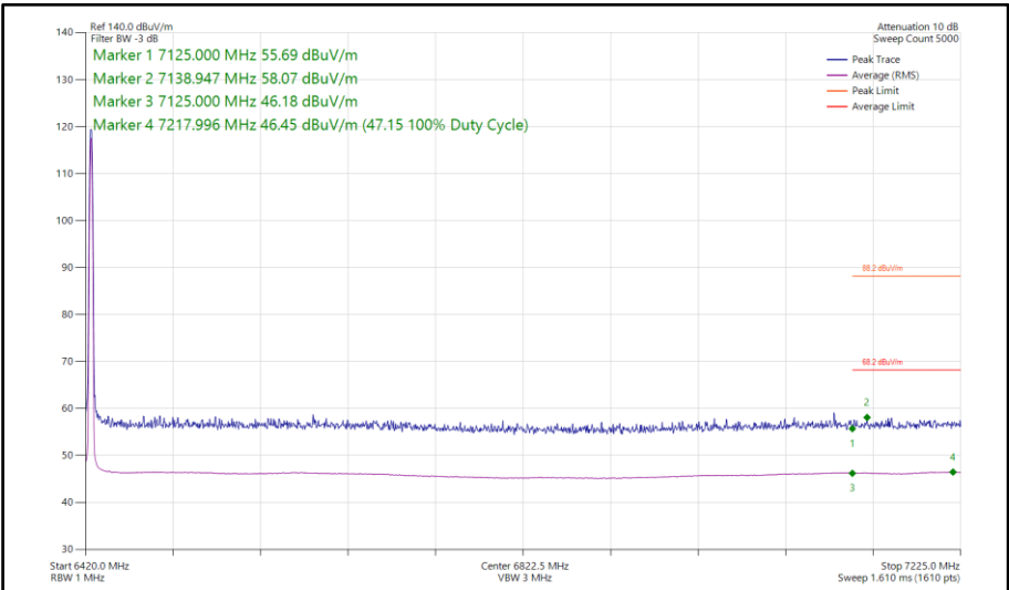
Figure 260 - Narrowband LE1M, SISO, Core 0 - 6425 MHz Band Edge Frequency 7125 MHz
