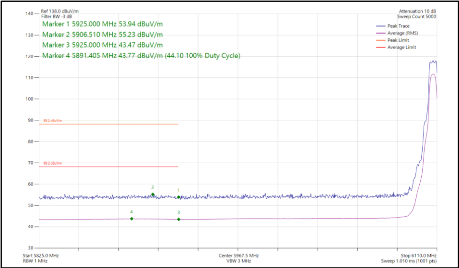
Figure 285 - Narrowband XHDRPM8, SISO, Core 1 - 6107 MHz Band Edge Frequency 5925 MHz
