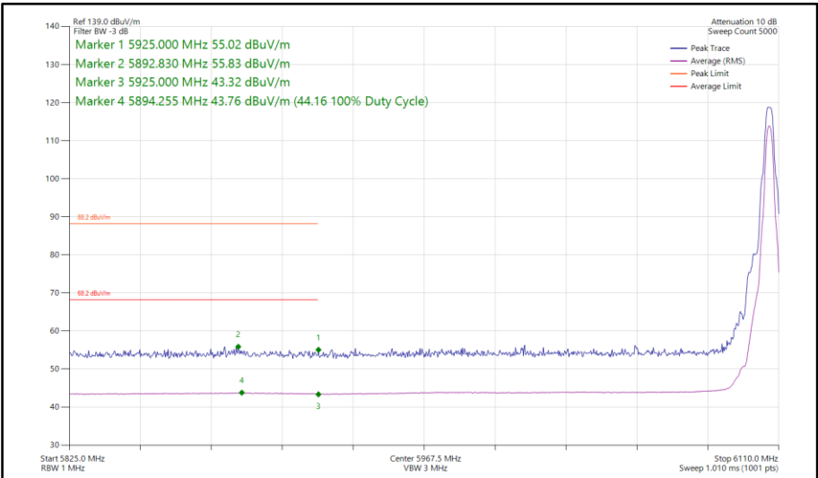
Figure 280 - Narrowband HDT6, SISO, Core 1 - 6106 MHz Band Edge Frequency 5925 MHz
