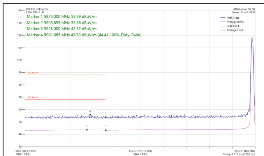
Figure 276 - Narrowband LE1M, SISO, Core 1 - 6106 MHz Band Edge Frequency 5925 MHz
