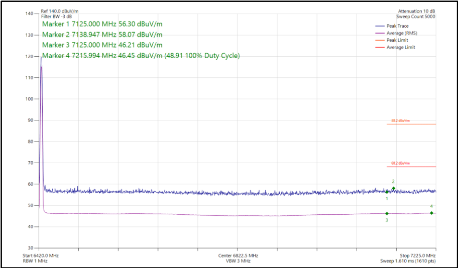
Figure 261 - Narrowband LE2M, SISO, Core 0 - 6425 MHz Band Edge Frequency 7125 MHz
