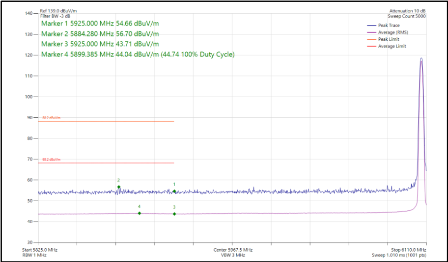
Figure 287 - Narrowband CS1LE1M, SISO, Core 1 - 6106 MHz Band Edge Frequency 5925 MHz
