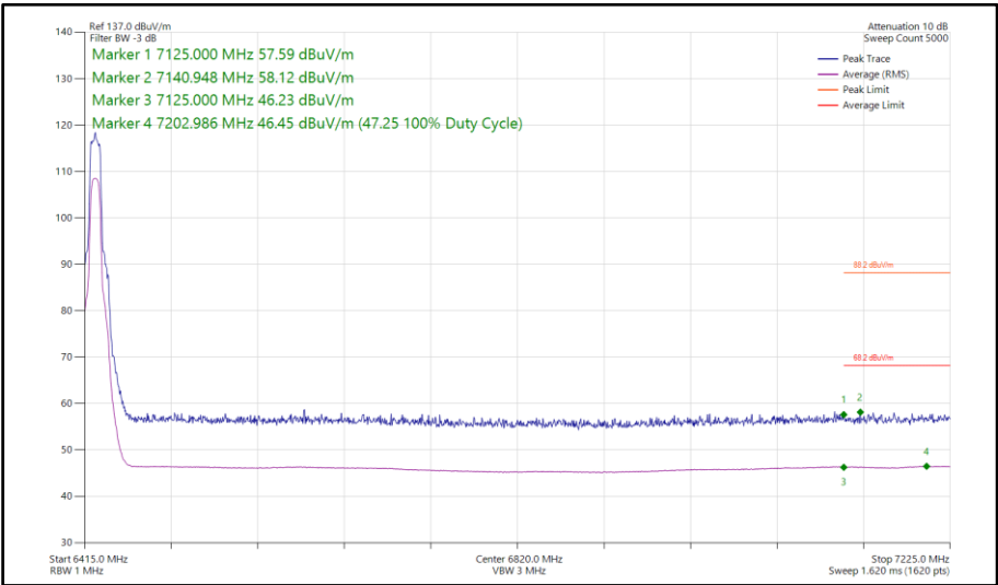
Figure 270 - Narrowband XHDRPL24, SISO, Core 0 - 6425 MHz Band Edge Frequency 7125 MHz
