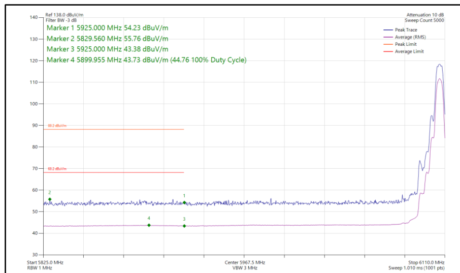
Figure 275 - Narrowband HDR8, SISO, Core 1 - 6106 MHz Band Edge Frequency 5925 MHz
