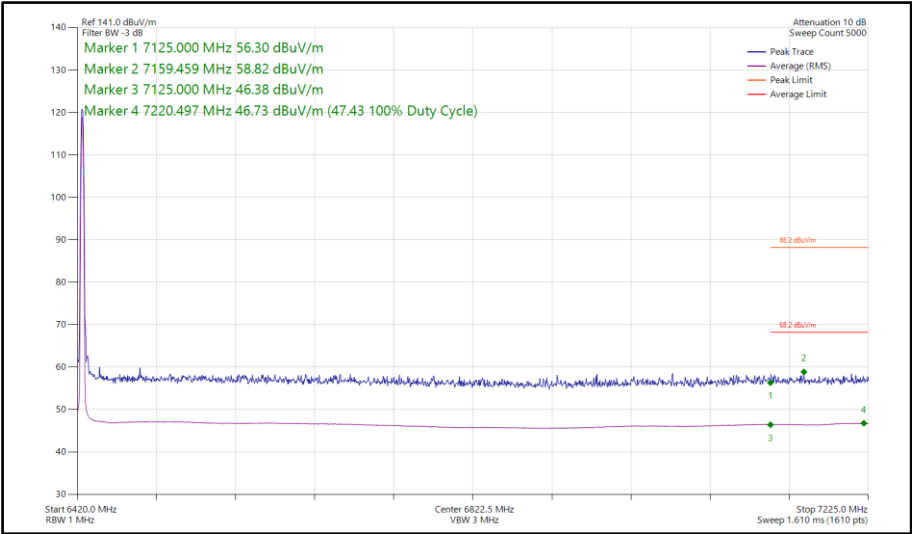
Figure 303 - Narrowband CS1LE1M, SISO, Core 1 - 6425 MHz Band Edge Frequency 7125 MHz
