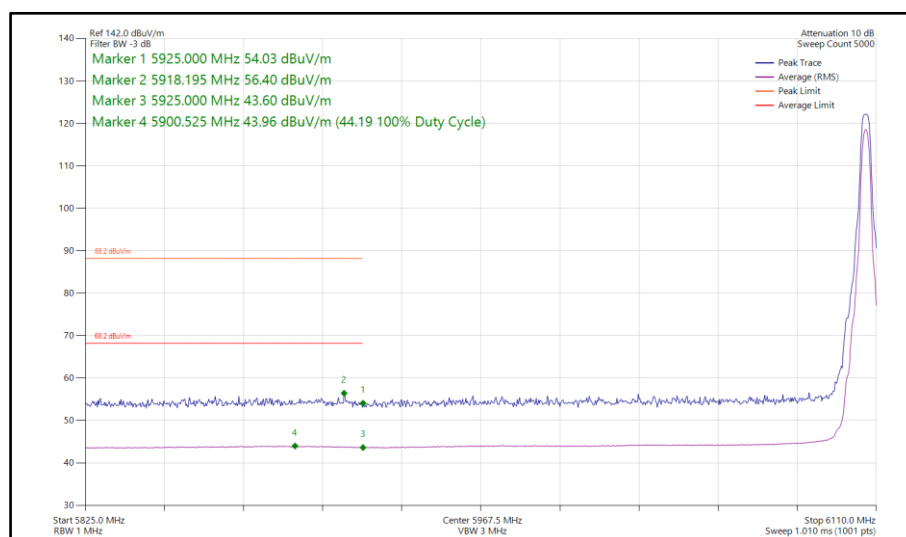
Figure 310 - Narrowband HDT3, MIMO, Core 0-1 - 6106 MHz Band Edge Frequency 5925 MHz
