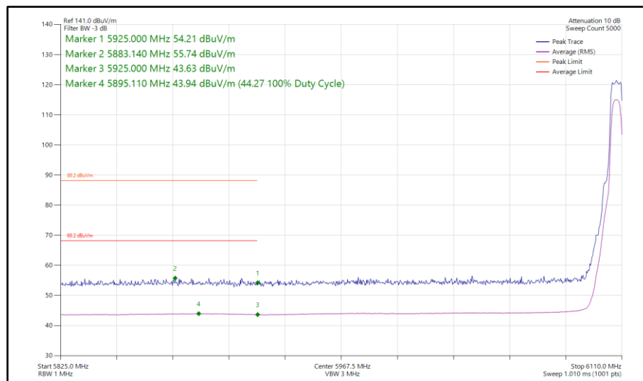
Figure 317 - Narrowband XHDRPM8, MIMO, Core 0-1 - 6107 MHz Band Edge Frequency 5925 MHz
