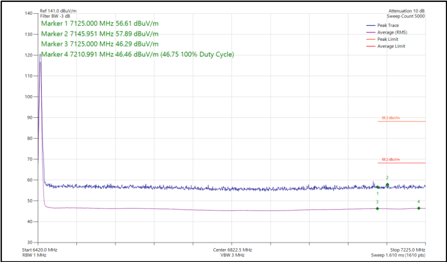
Figure 297 - Narrowband HDRPS2, SISO, Core 1 - 6425 MHz Band Edge Frequency 7125 MHz
