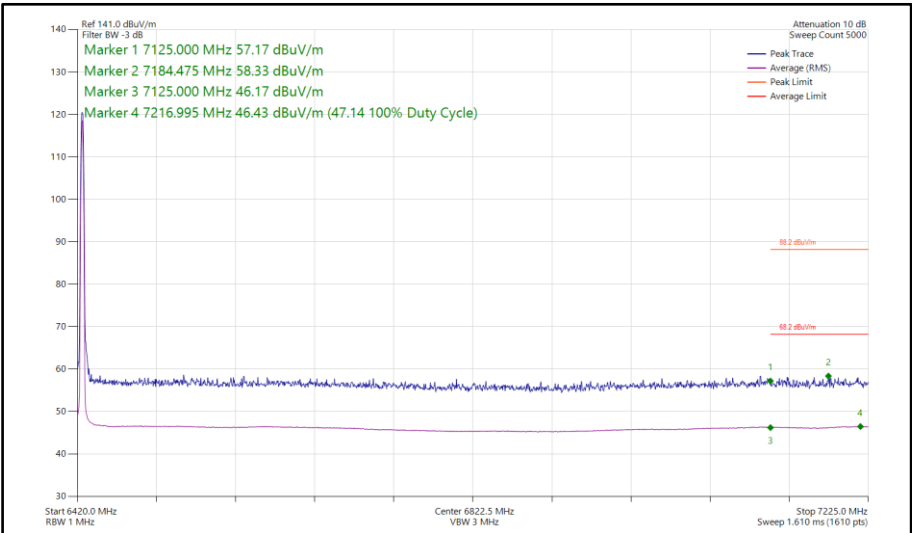
Figure 292 - Narrowband LE1M, SISO, Core 1 - 6425 MHz Band Edge Frequency 7125 MHz
