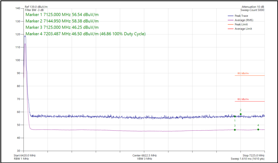
Figure 269 - Narrowband XHDRPM8, SISO, Core 0 - 6425 MHz Band Edge Frequency 7125 MHz
