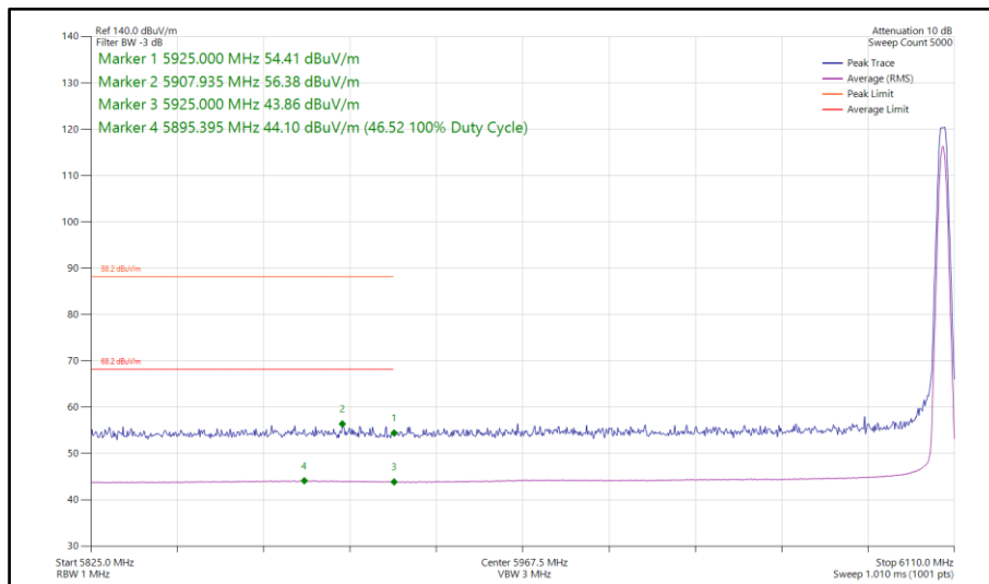
Figure 256 - Narrowband CS1LE2M, SISO, Core 0 - 6106 MHz Band Edge Frequency 5925 MHz
