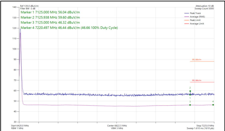
Figure 262 - Narrowband HDT3, SISO, Core 0 - 6425 MHz Band Edge Frequency 7125 MHz
