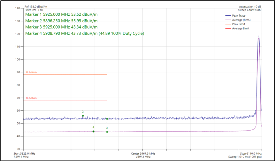
Figure 273 - Narrowband DH5, SISO, Core 1 - 6106 MHz Band Edge Frequency 5925 MHz
