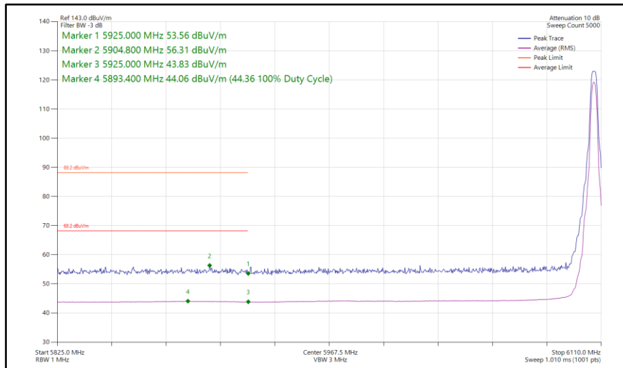
Figure 311 - Narrowband HDT4, MIMO, Core 0-1 - 6106 MHz Band Edge Frequency 5925 MHz
