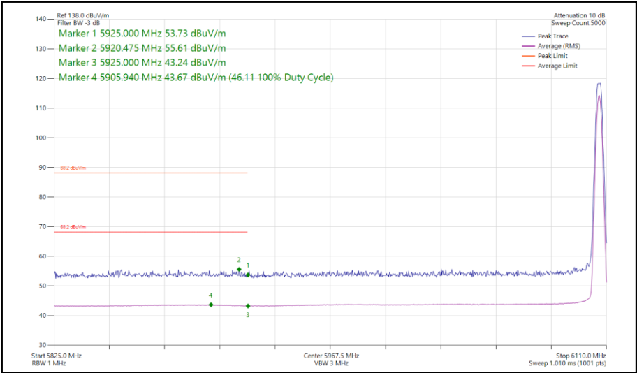
Figure 277 - Narrowband LE2M, SISO, Core 1 - 6106 MHz Band Edge Frequency 5925 MHz
