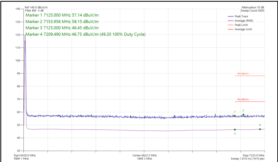
Figure 272 - Narrowband CS1LE2M, SISO, Core 0 - 6425 MHz Band Edge Frequency 7125 MHz
