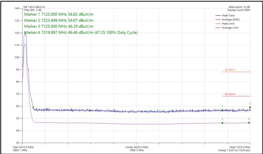
Figure 302 - Narrowband XHDRPL24, SISO, Core 1 - 6425 MHz Band Edge Frequency 7125 MHz
