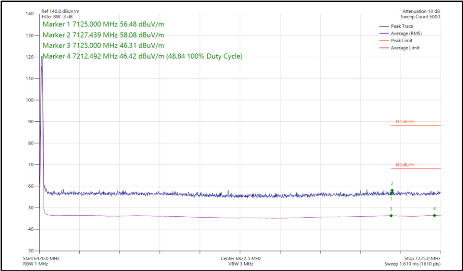
Figure 293 - Narrowband LE2M, SISO, Core 1 - 6425 MHz Band Edge Frequency 7125 MHz
