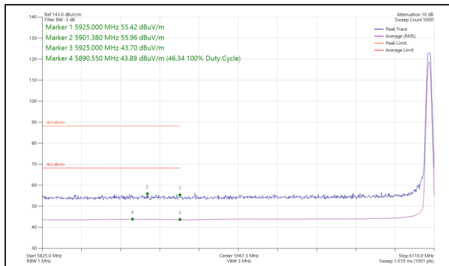
Figure 309 - Narrowband LE2M, MIMO, Core 0-1 - 6106 MHz Band Edge Frequency 5925 MHz
