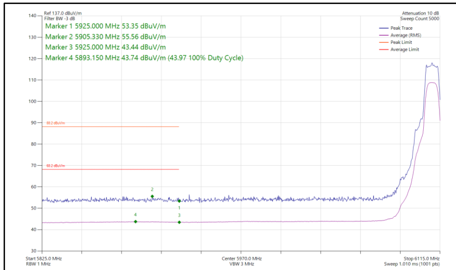
Figure 283 - Narrowband HDRPL8, SISO, Core 1 - 6109 MHz Band Edge Frequency 5925 MHz
