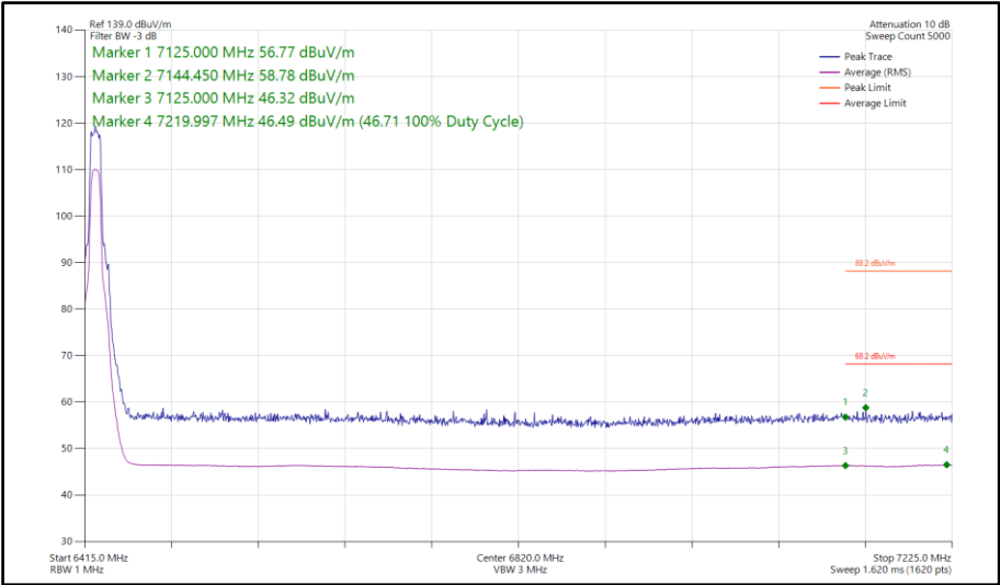
Figure 267 - Narrowband HDRPL8, SISO, Core 0 - 6425 MHz Band Edge Frequency 7125 MHz
