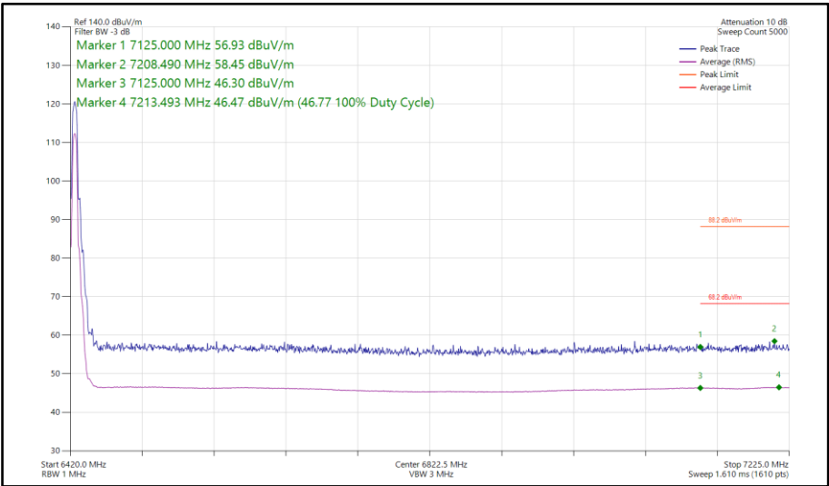
Figure 298 - Narrowband HDRPM12, SISO, Core 1 - 6425 MHz Band Edge Frequency 7125 MHz
