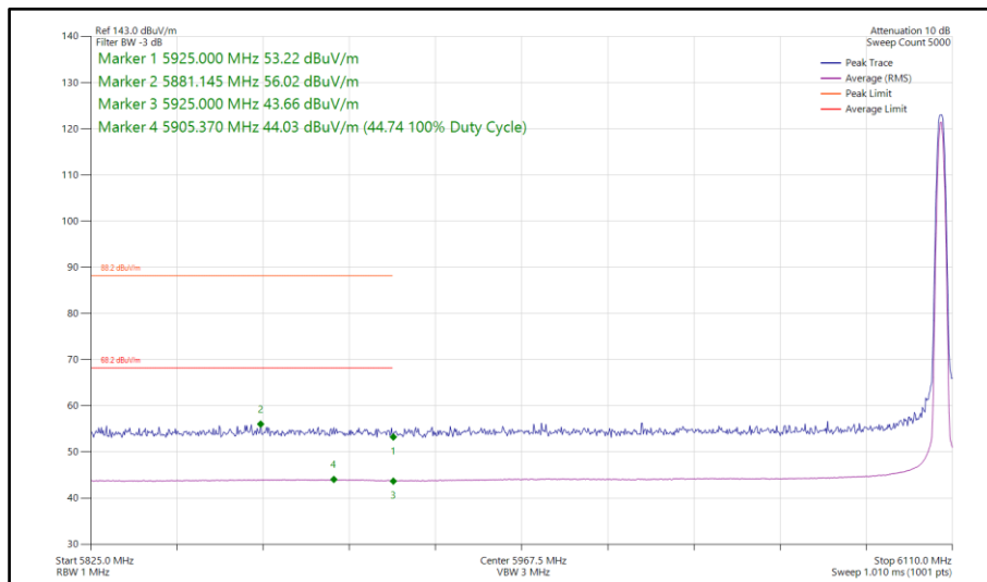
Figure 308 - Narrowband LE1M, MIMO, Core 0-1 - 6106 MHz Band Edge Frequency 5925 MHz
