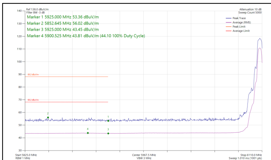
Figure 282 - Narrowband HDRPM12, SISO, Core 1 - 6107 MHz Band Edge Frequency 5925 MHz
