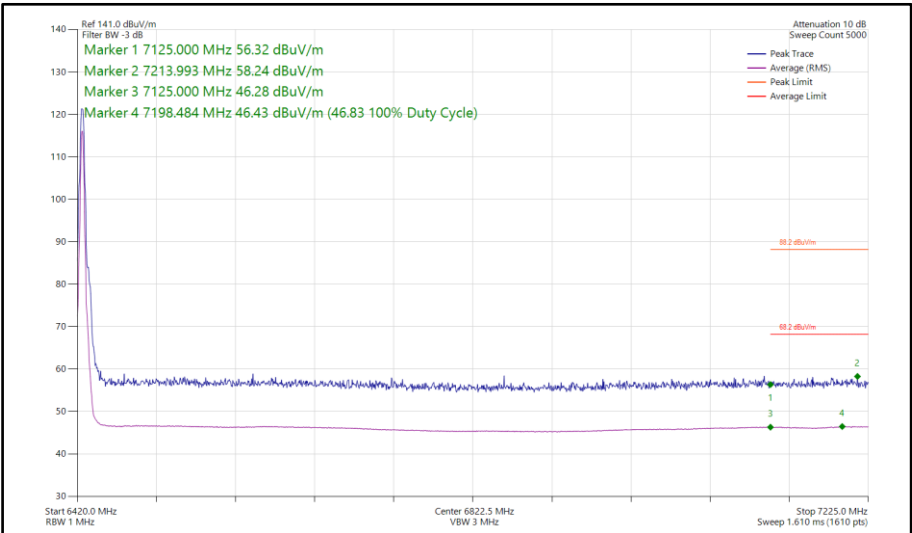
Figure 296 - Narrowband HDT6, SISO, Core 1 - 6425 MHz Band Edge Frequency 7125 MHz
