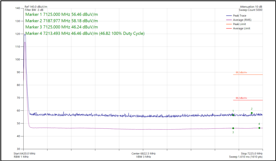
Figure 301 - Narrowband XHDRPM8, SISO, Core 1 - 6425 MHz Band Edge Frequency 7125 MHz
