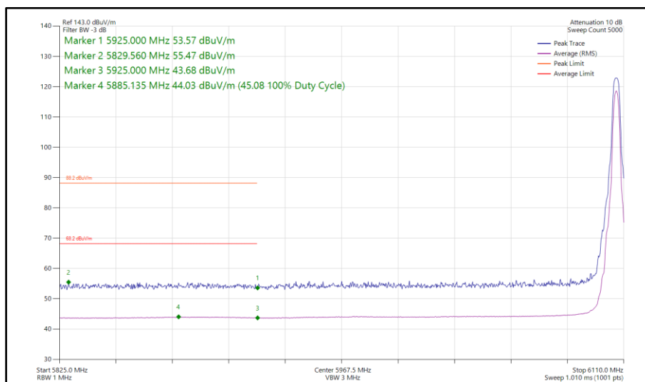
Figure 306 - Narrowband HDR4, MIMO, Core 0-1 - 6106 MHz Band Edge Frequency 5925 MHz
