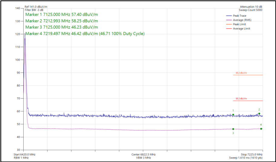
Figure 295 - Narrowband HDT4, SISO, Core 1 - 6425 MHz Band Edge Frequency 7125 MHz
