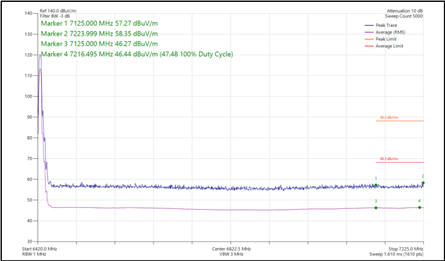
Figure 291 - Narrowband HDR8, SISO, Core 1 - 6425 MHz Band Edge Frequency 7125 MHz
