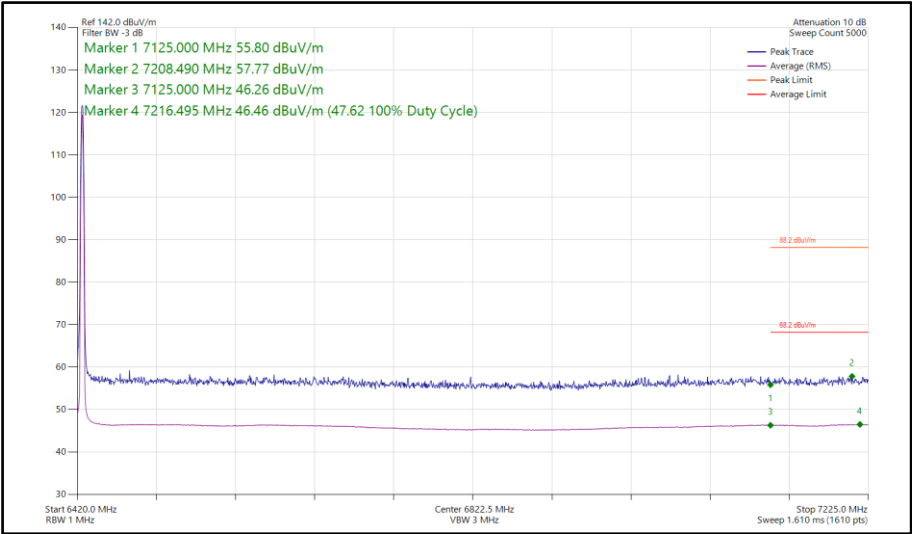
Figure 321 - Narrowband DH5, MIMO, Core 0-1 - 6425 MHz Band Edge Frequency 7125 MHz
