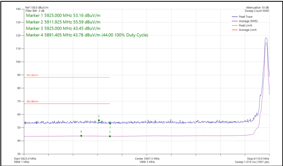
Figure 278 - Narrowband HDT3, SISO, Core 1 - 6106 MHz Band Edge Frequency 5925 MHz
