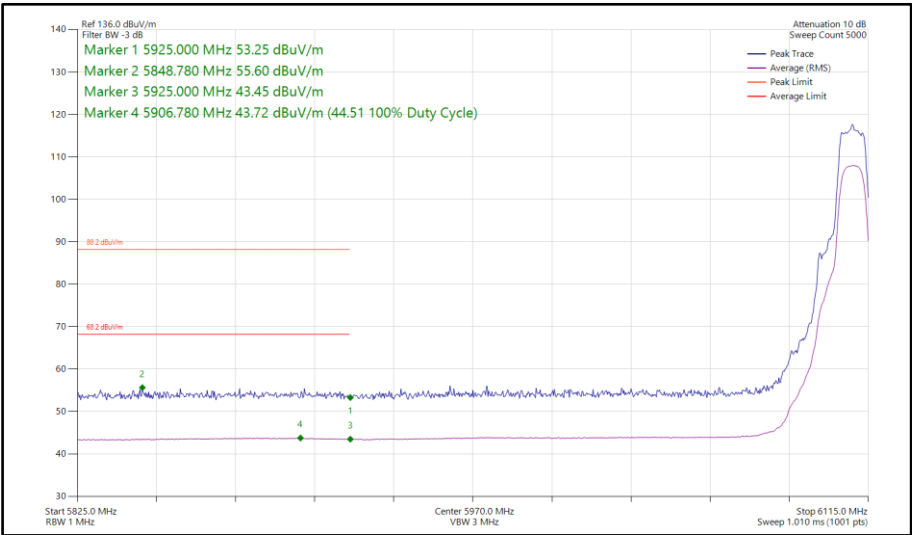
Figure 286 - Narrowband XHDRPL24, SISO, Core 1 - 6109 MHz Band Edge Frequency 5925 MHz
