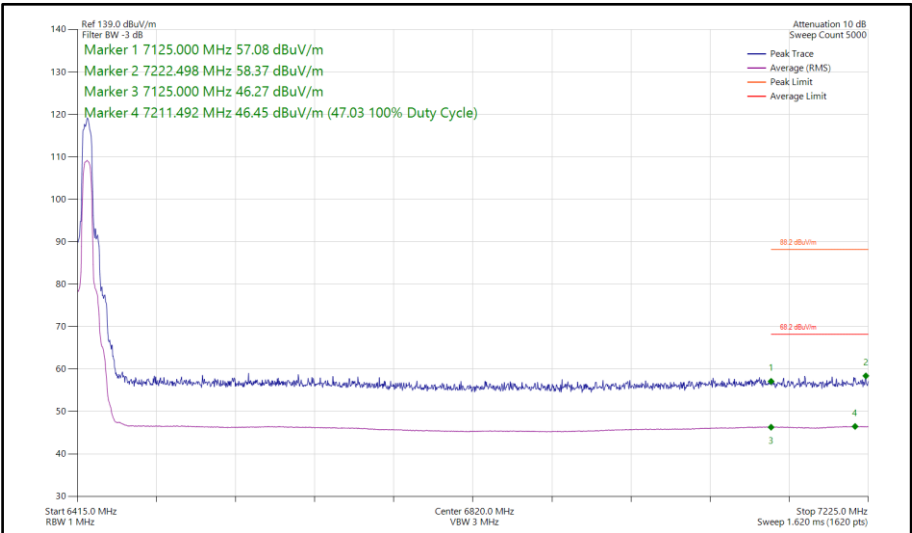
Figure 300 - Narrowband HDRPL24, SISO, Core 1 - 6425 MHz Band Edge Frequency 7125 MHz
