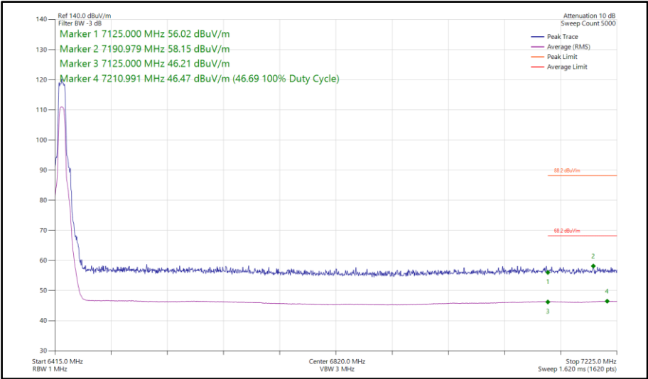
Figure 299 - Narrowband HDRPL8, SISO, Core 1 - 6425 MHz Band Edge Frequency 7125 MHz
