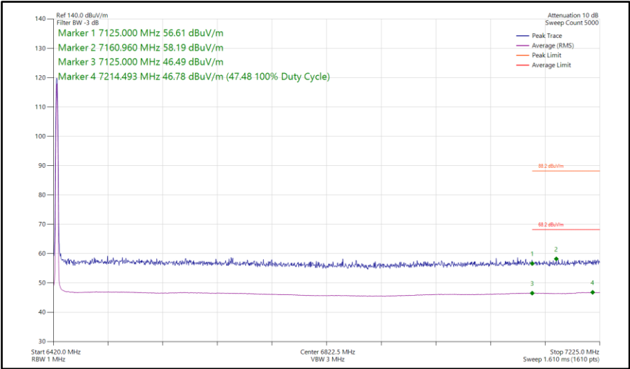
Figure 271 - Narrowband CS1LE1M, SISO, Core 0 - 6425 MHz Band Edge Frequency 7125 MHz
