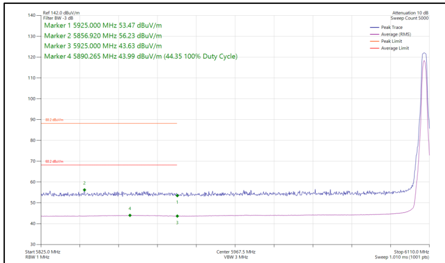
Figure 313 - Narrowband HDRPS2, MIMO, Core 0-1 - 6106 MHz Band Edge Frequency 5925 MHz
