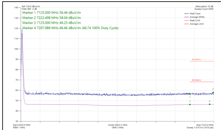
Figure 263 - Narrowband HDT4, SISO, Core 0 - 6425 MHz Band Edge Frequency 7125 MHz
