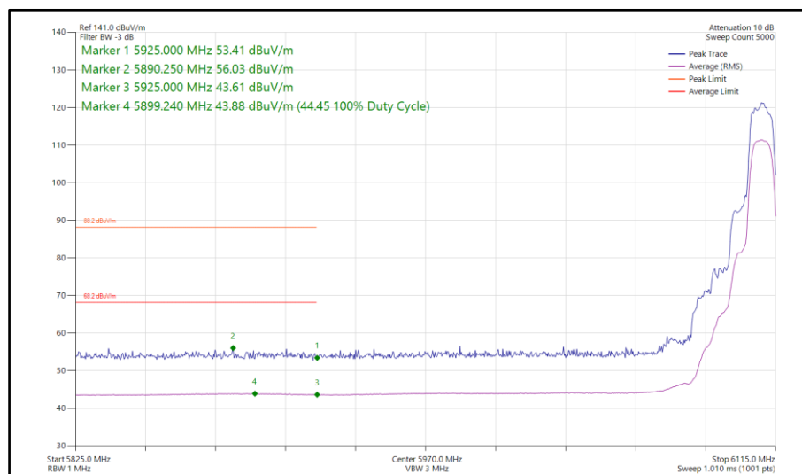
Figure 316 - Narrowband HDRPL24, MIMO, Core 0-1 - 6109 MHz Band Edge Frequency 5925 MHz
