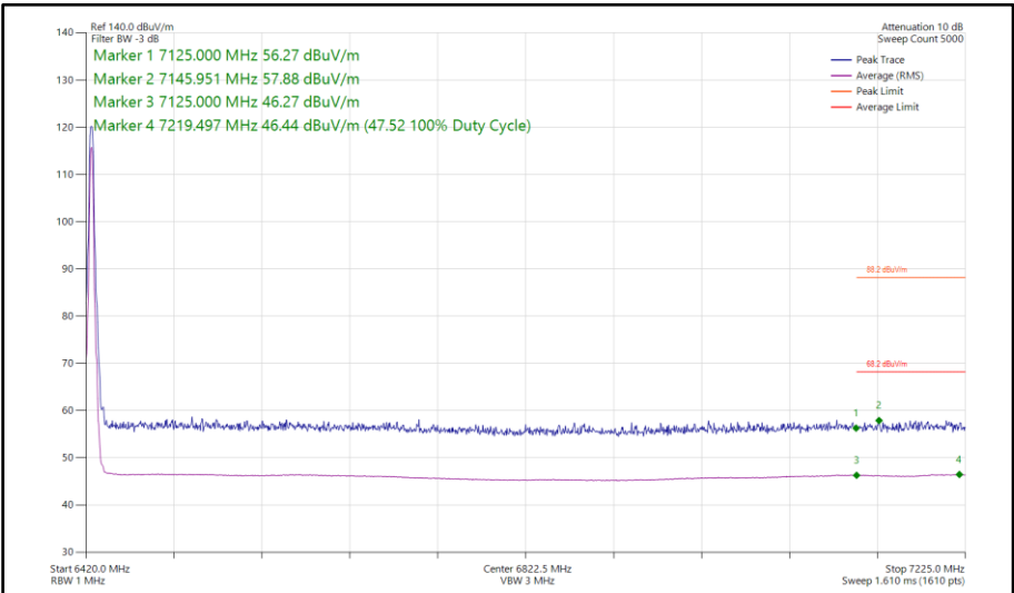
Figure 290 - Narrowband HDR4, SISO, Core 1 - 6425 MHz Band Edge Frequency 7125 MHz
