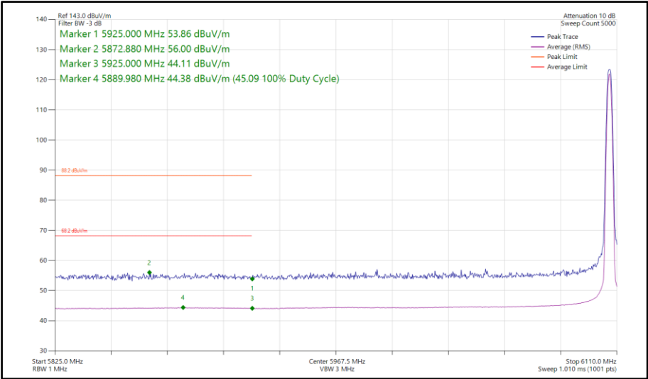
Figure 319 - Narrowband CS1LE1M, MIMO, Core 0-1 - 6106 MHz Band Edge Frequency 5925 MHz
