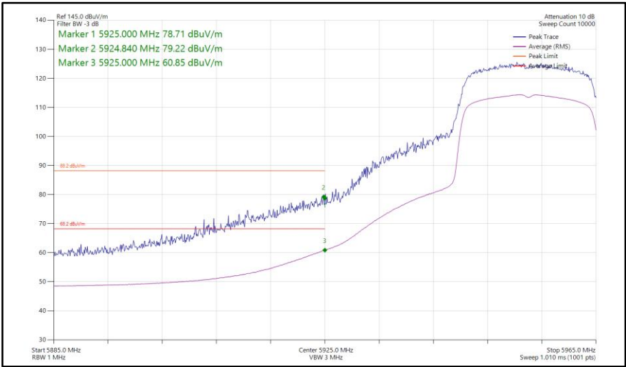
Figure 331 - 802.11ax HE20, SU, TxBF, Core 0-1 - 5955 MHz Band Edge Frequency 5925 MHz
