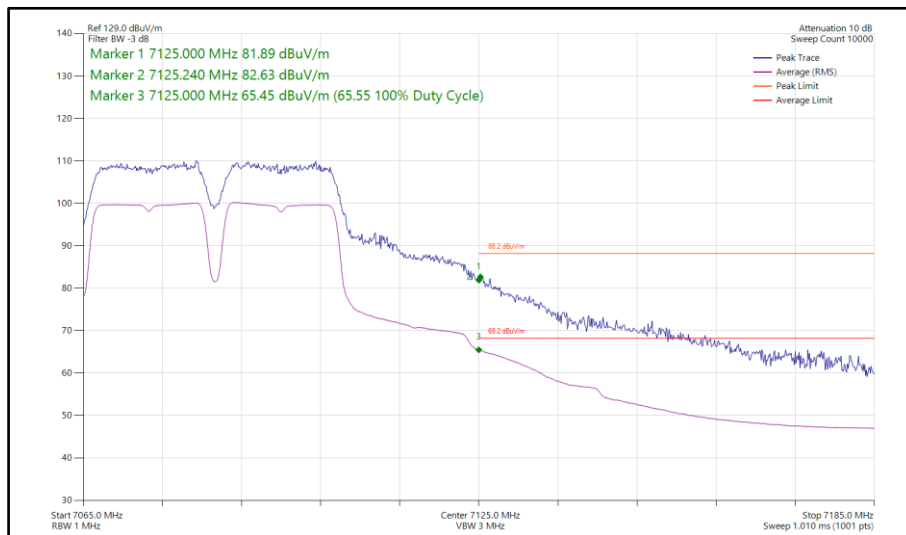
Figure 338 - 802.11a a40, SISO, Core 0 - 7085 MHz Band Edge Frequency 7125 MHz
