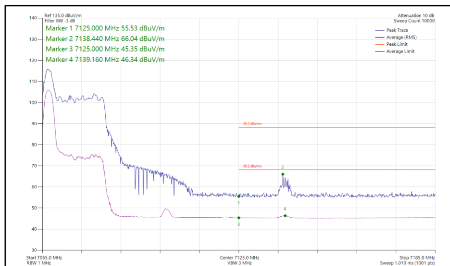
Figure 340 - 802.11ax HE40, RU26-0, SISO, Core 0 - 7085 MHz Band Edge Frequency 7125 MHz
