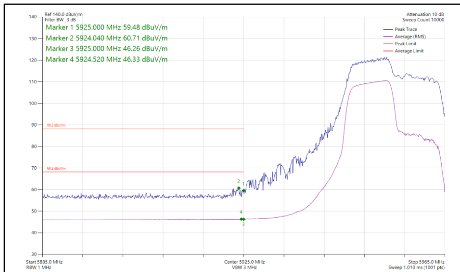
Figure 307 - 802.11ax HE20, RU106-53, SISO, Core 1 - 5955 MHz Band Edge Frequency 5925 MHz
