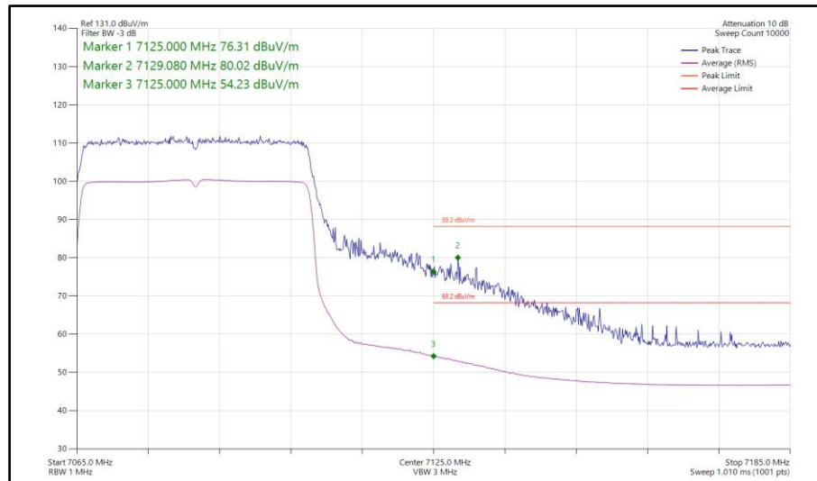
Figure 339 - 802.11ax HE40, SU, SISO, Core 0 - 7085 MHz Band Edge Frequency 7125 MHz
