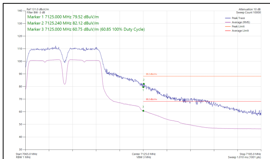
Figure 346 - 802.11a a40, SISO, Core 1 - 7085 MHz Band Edge Frequency 7125 MHz
