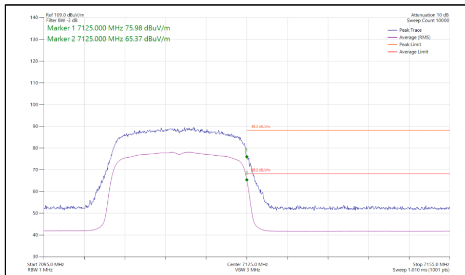
Figure 329 - 802.11ax HE20, SU, SDM, Core 0-1 - 7115 MHz Band Edge Frequency 7125 MHz
