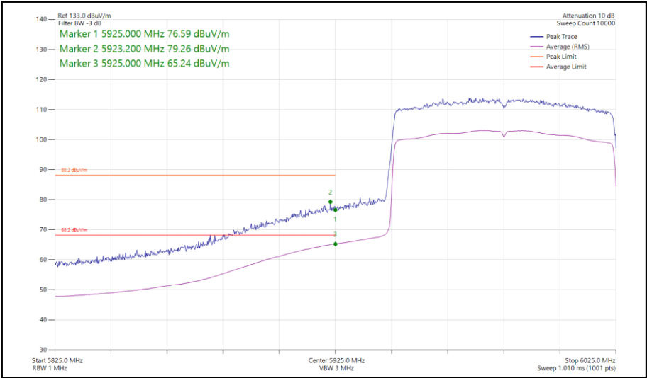
Figure 375 - 802.11ax HE80, SU, SISO, Core 1 - 5985 MHz Band Edge Frequency 5925 MHz
