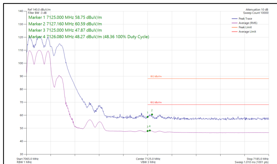
Figure 363 - 802.11be EHT40, RU106+26-82, SDM, Core 0-1 - 7085 MHz Band Edge Frequency 7125 MHz
