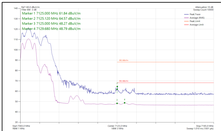
Figure 362 - 802.11ax HE40, RU106-53, SDM, Core 0-1 - 7085 MHz Band Edge Frequency 7125 MHz
