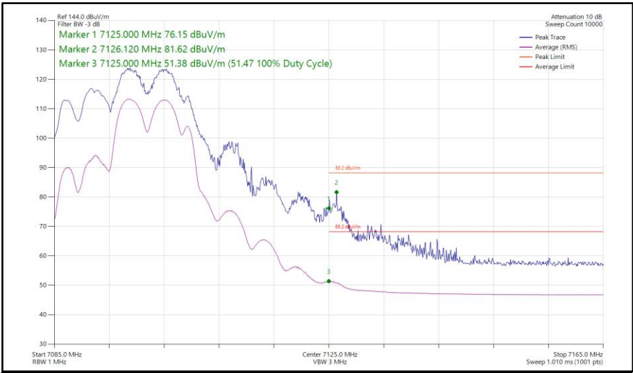
Figure 322 - 802.11be EHT20, RU106+26-83, CDD, Core 0-1 - 7095 MHz Band Edge Frequency 7125 MHz
