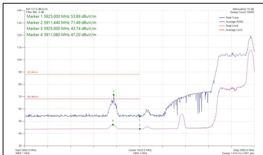
Figure 336 - 802.11ax HE40, RU26-17, SISO, Core 0 - 5965 MHz Band Edge Frequency 5925 MHz
