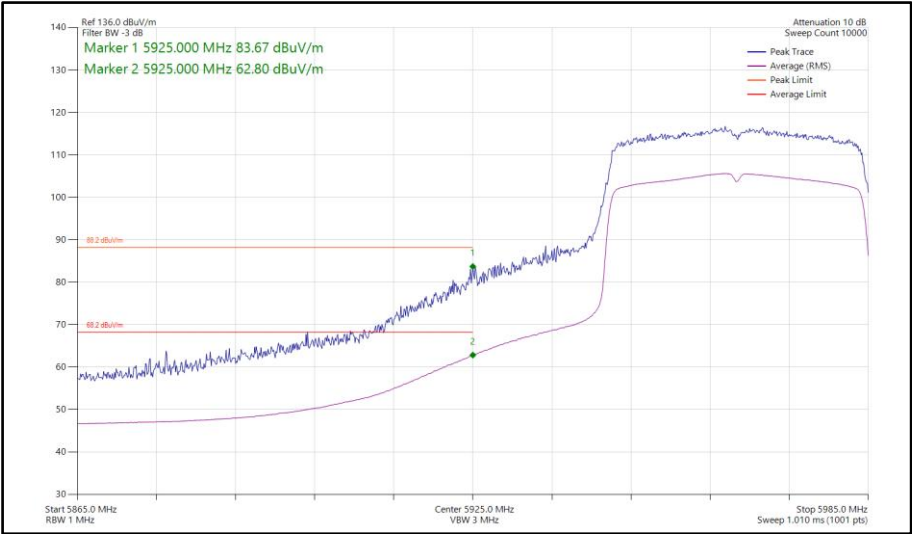
Figure 343 - 802.11ax HE40, SU, SISO, Core 1 - 5965 MHz Band Edge Frequency 5925 MHz
