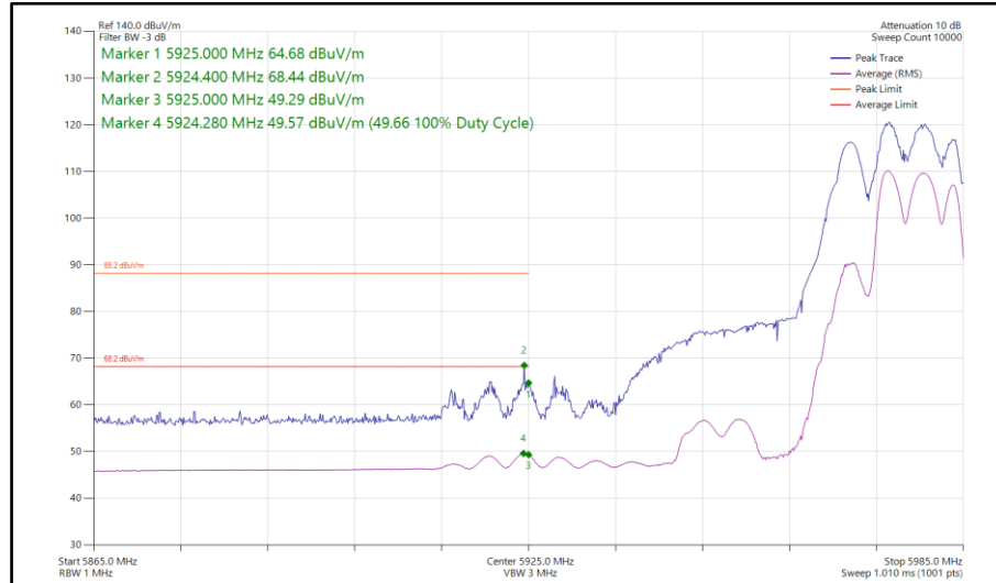
Figure 360 - 802.11be EHT40, RU106+26-85, SDM, Core 0-1 - 5965 MHz Band Edge Frequency 5925 MHz
