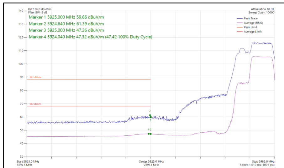
Figure 345 - 802.11be EHT40, RU106+26-85, SISO, Core 1 - 5965 MHz Band Edge Frequency 5925 MHz
