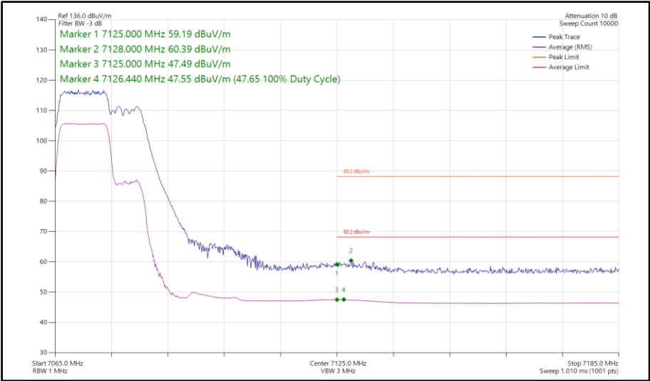
Figure 349 - 802.11be EHT40, RU106+26-82, SISO, Core 1 - 7085 MHz Band Edge Frequency 7125 MHz
