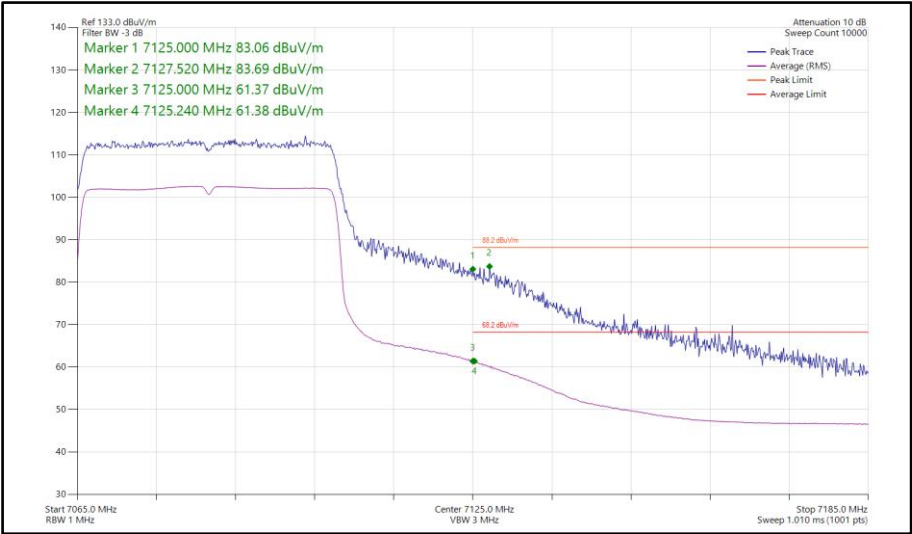
Figure 347 - 802.11ax HE40, SU, SISO, Core 1 - 7085 MHz Band Edge Frequency 7125 MHz
