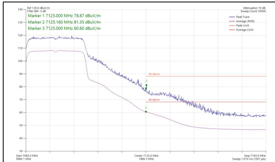
Figure 310 - 802.11ax HE20, SU, SISO, Core 1 - 7095 MHz Band Edge Frequency 7125 MHz
