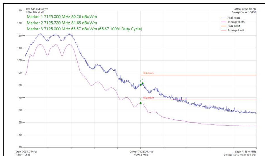
Figure 317 - 802.11a, CDD, Core 0-1 - 7095 MHz Band Edge Frequency 7125 MHz
