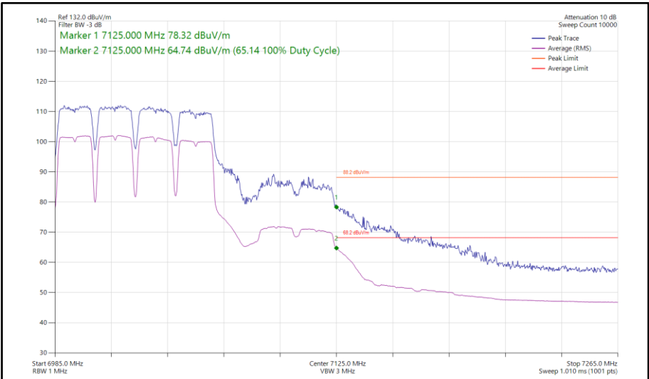
Figure 370 - 802.11a a80, SISO, Core 0 - 7025 MHz Band Edge Frequency 7125 MHz
