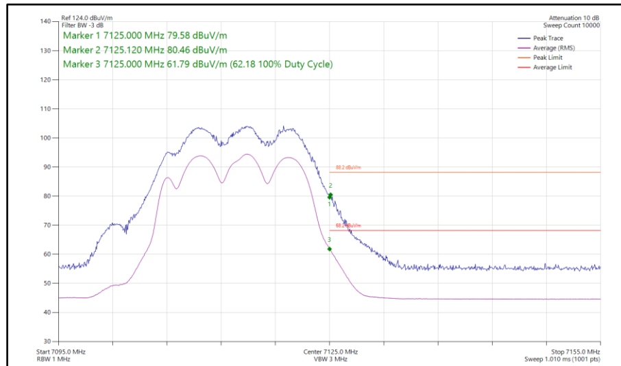
Figure 318 - 802.11a, CDD, Core 0-1 - 7115 MHz Band Edge Frequency 7125 MHz
