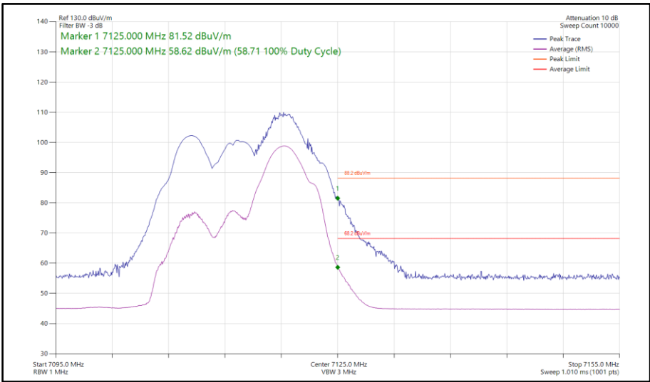
Figure 323 - 802.11be EHT20, RU52+26-72, CDD, Core 0-1 - 7115 MHz Band Edge Frequency 7125 MHz
