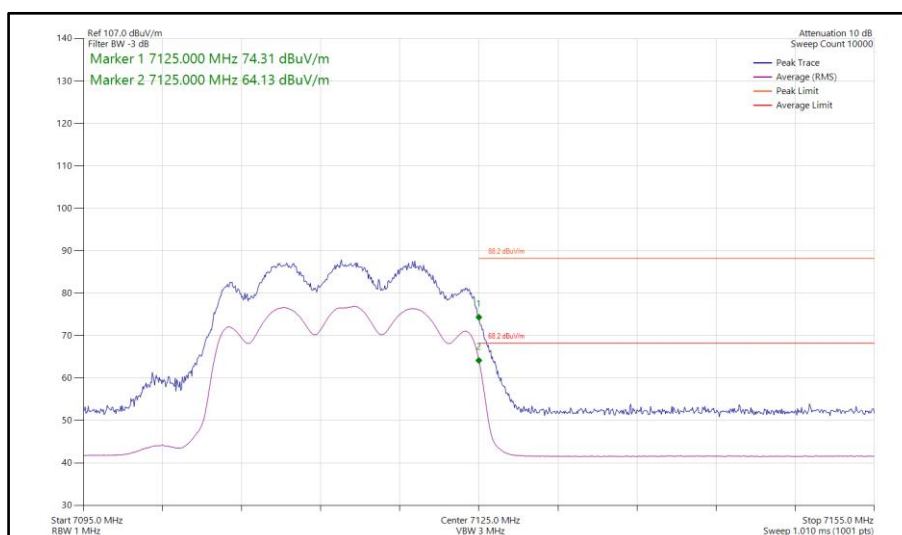
Figure 321 - 802.11ax HE20, SU, CDD, Core 0-1 - 7115 MHz Band Edge Frequency 7125 MHz
