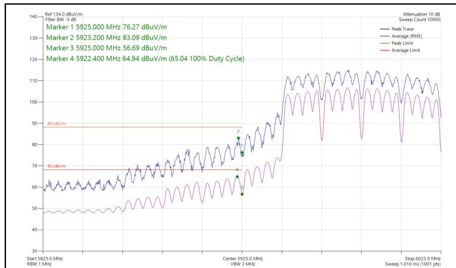
Figure 382 - 802.11a a80, CDD, Core 0-1 - 5985 MHz Band Edge Frequency 5925 MHz
