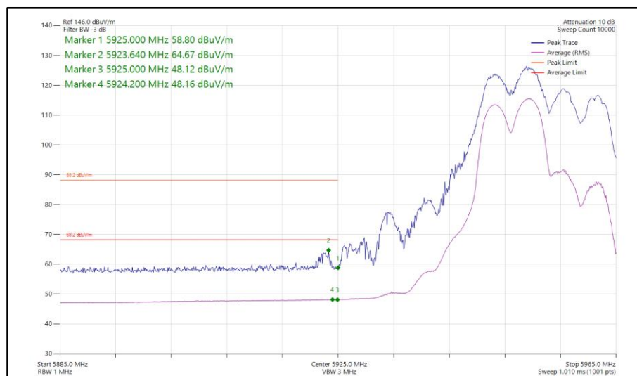
Figure 315 - 802.11ax HE20, RU106-53, CDD, Core 0-1 - 5955 MHz Band Edge Frequency 5925 MHz
