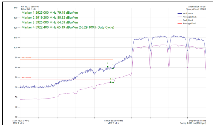
Figure 374 - 802.11a a80, SISO, Core 1 - 5985 MHz Band Edge Frequency 5925 MHz
