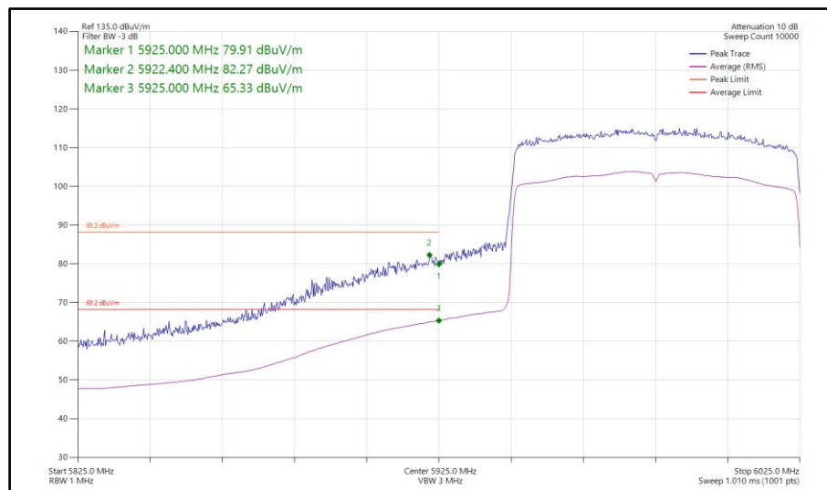
Figure 367 - 802.11ax HE80, SU, SISO, Core 0 - 5985 MHz Band Edge Frequency 5925 MHz
