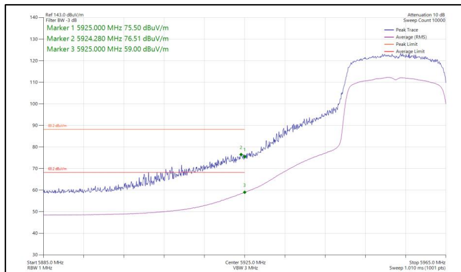
Figure 324 - 802.11ax HE20, SU, SDM, Core 0-1 - 5955 MHz Band Edge Frequency 5925 MHz
