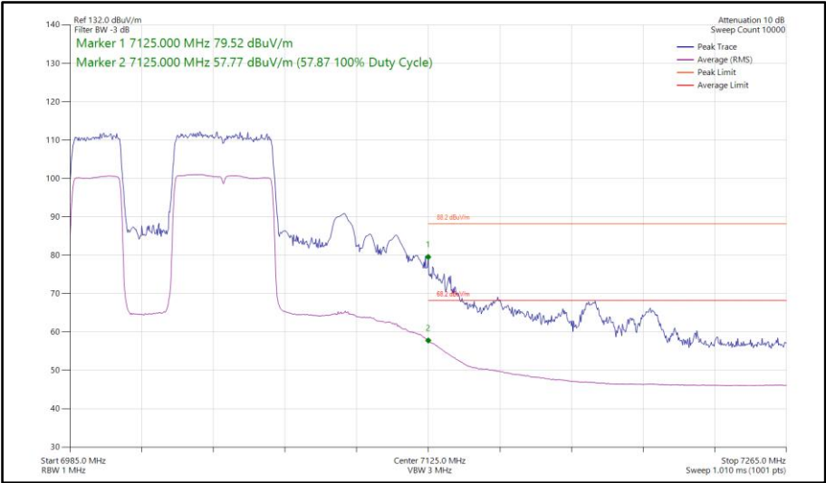
Figure 381 - 802.11be EHT80, RU484+242-91, SISO, Core 1 - 7025 MHz Band Edge Frequency 7125 MHz
