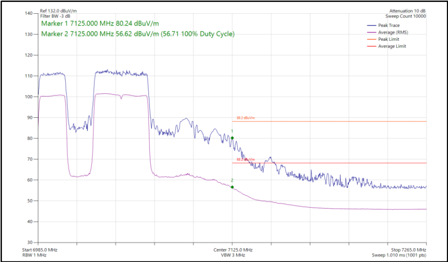
Figure 373 - 802.11be EHT80, RU484+242-91, SISO, Core 0 - 7025 MHz Band Edge Frequency 7125 MHz
