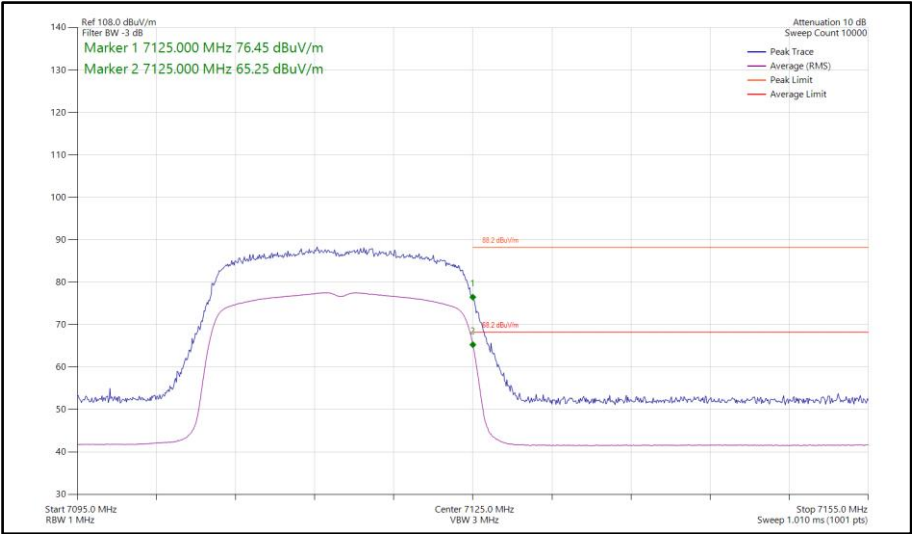
Figure 333 - 802.11ax HE20, SU, TxBF, Core 0-1 - 7115 MHz Band Edge Frequency 7125 MHz
