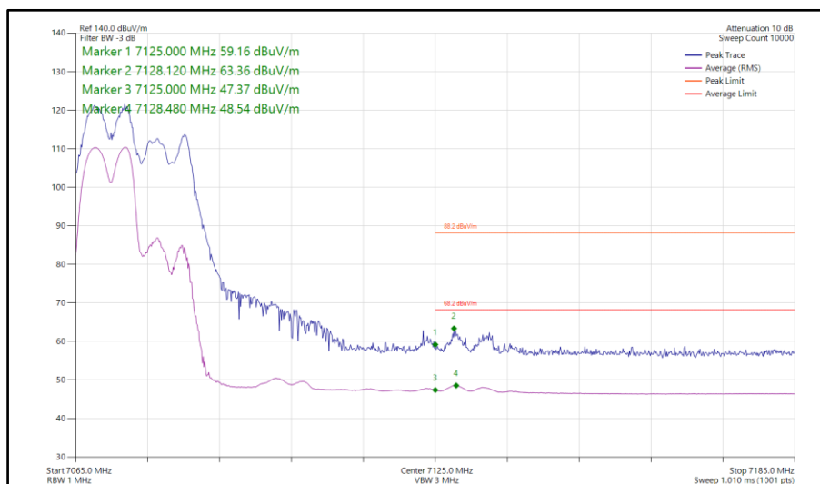
Figure 356 - 802.11ax HE40, RU106-53, CDD, Core 0-1 - 7085 MHz Band Edge Frequency 7125 MHz
