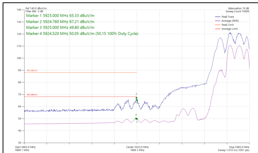
Figure 353 - 802.11be EHT40, RU106+26-85, CDD, Core 0-1 - 5965 MHz Band Edge Frequency 5925 MHz
