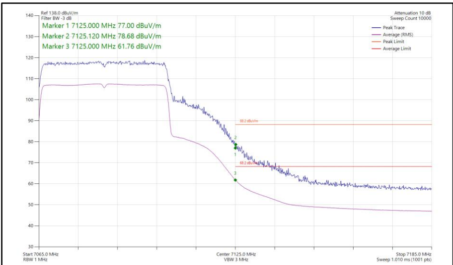
Figure 365 - 802.11ax HE40, SU, TxBF, Core 0-1 - 7085 MHz Band Edge Frequency 7125 MHz
