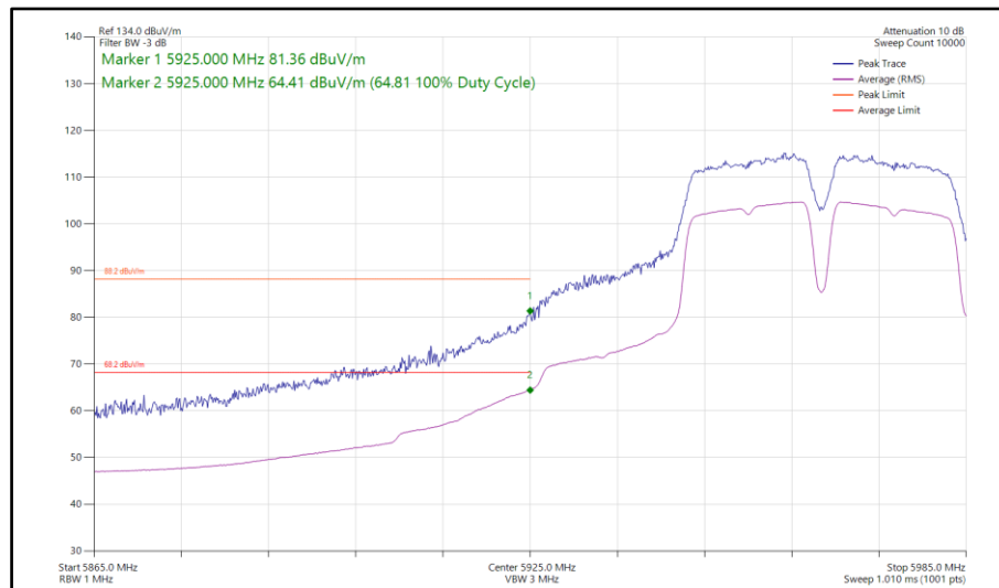
Figure 342 - 802.11a a40, SISO, Core 1 - 5965 MHz Band Edge Frequency 5925 MHz
