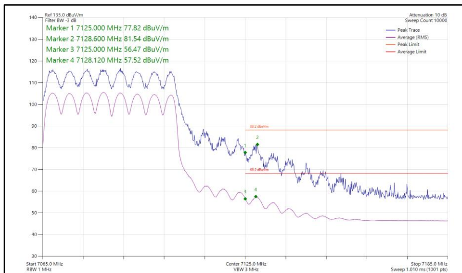
Figure 355 - 802.11ax HE40, SU, CDD, Core 0-1 - 7085 MHz Band Edge Frequency 7125 MHz
