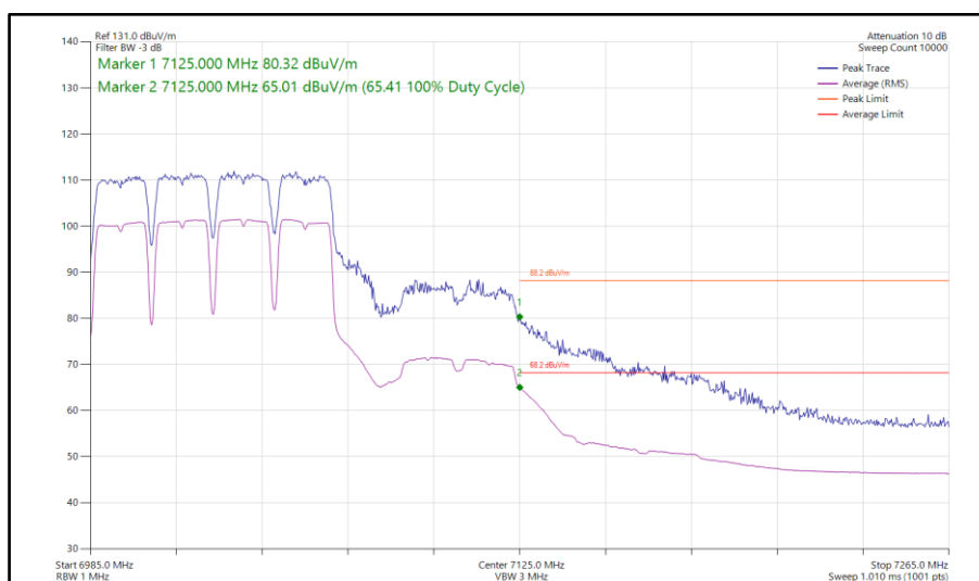
Figure 378 - 802.11a a80, SISO, Core 1 - 7025 MHz Band Edge Frequency 7125 MHz
