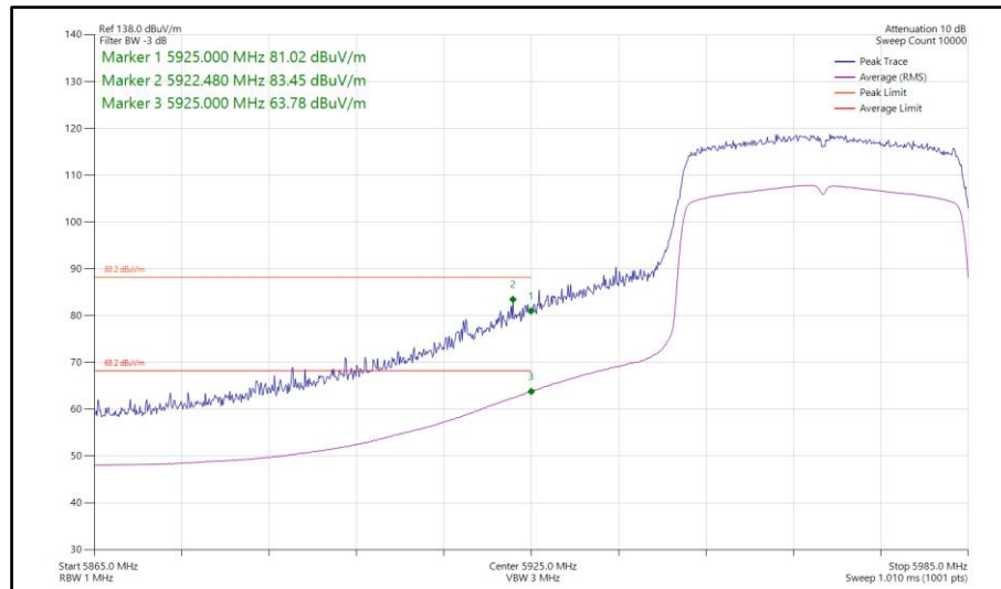
Figure 335 - 802.11ax HE40, SU, SISO, Core 0 - 5965 MHz Band Edge Frequency 5925 MHz
