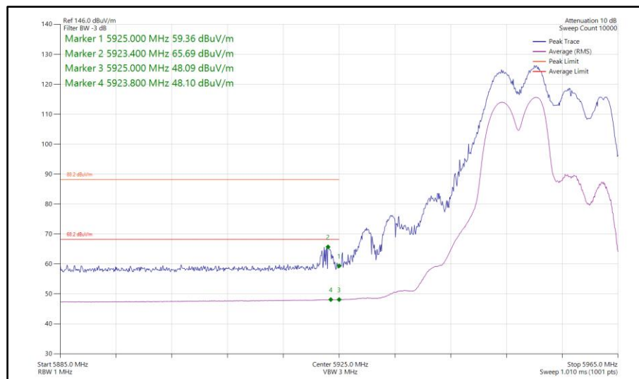
Figure 325 - 802.11ax HE20, RU106-53, SDM, Core 0-1 - 5955 MHz Band Edge Frequency 5925 MHz
