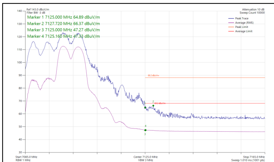
Figure 328 - 802.11ax HE20, RU106-54, SDM, Core 0-1 - 7095 MHz Band Edge Frequency 7125 MHz
