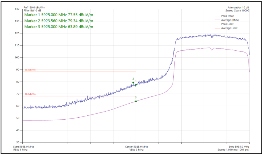
Figure 358 - 802.11ax HE40, SU, SDM, Core 0-1 - 5965 MHz Band Edge Frequency 5925 MHz
