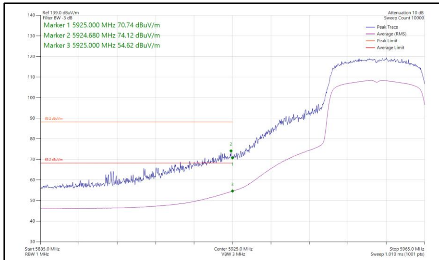
Figure 306 - 802.11ax HE20, SU, SISO, Core 1 - 5955 MHz Band Edge Frequency 5925 MHz
