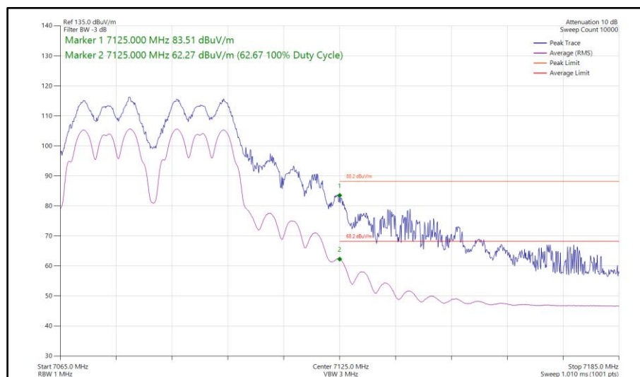
Figure 354 - 802.11a a40, CDD, Core 0-1 - 7085 MHz Band Edge Frequency 7125 MHz
