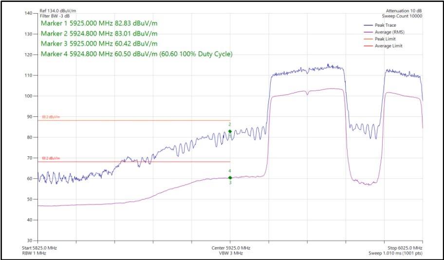
Figure 369 - 802.11be EHT80, RU484+242-92, SISO, Core 0 - 5985 MHz Band Edge Frequency 5925 MHz
