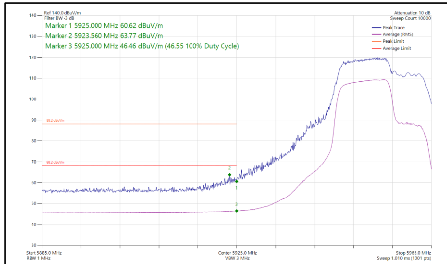
Figure 308 - 802.11be EHT20, RU106+26-82, SISO, Core 1 - 5955 MHz Band Edge Frequency 5925 MHz
