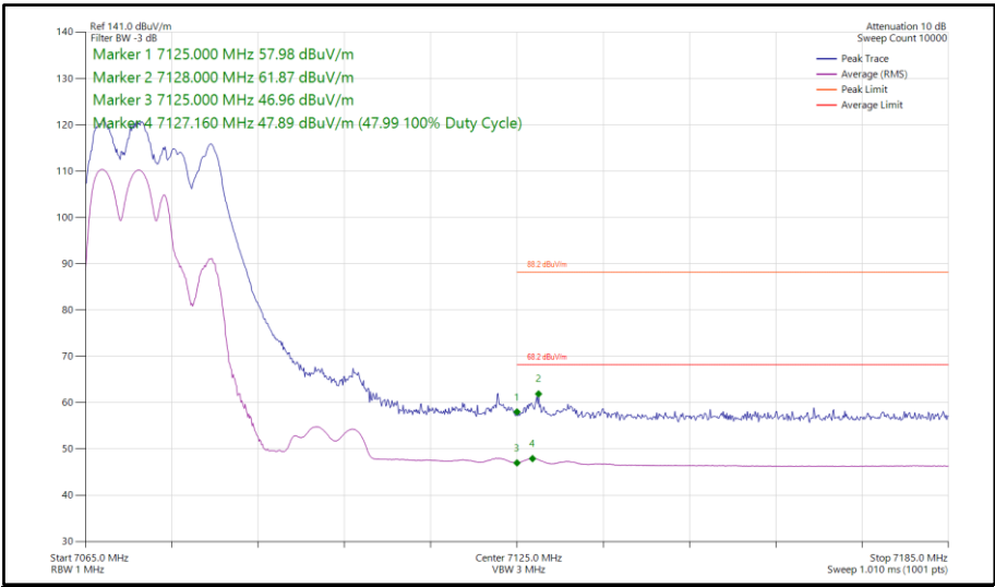
Figure 357 - 802.11be EHT40, RU106+26-82, CDD, Core 0-1 - 7085 MHz Band Edge Frequency 7125 MHz
