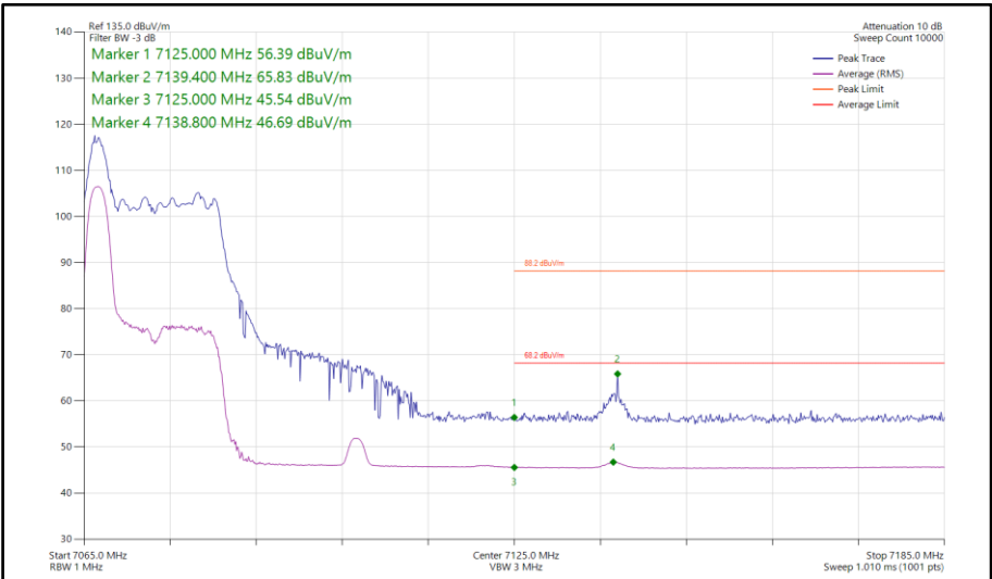
Figure 348 - 802.11ax HE40, RU26-0, SISO, Core 1 - 7085 MHz Band Edge Frequency 7125 MHz
