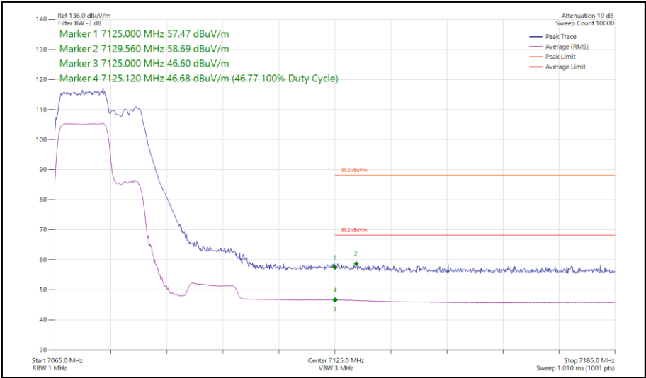
Figure 341 - 802.11be EHT40, RU106+26-82, SISO, Core 0 - 7085 MHz Band Edge Frequency 7125 MHz
