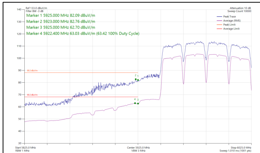
Figure 366 - 802.11a a80, SISO, Core 0 - 5985 MHz Band Edge Frequency 5925 MHz
