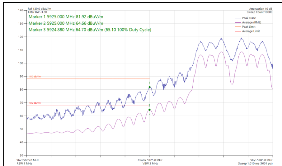
Figure 350 - 802.11a a40, CDD, Core 0-1 - 5965 MHz Band Edge Frequency 5925 MHz
