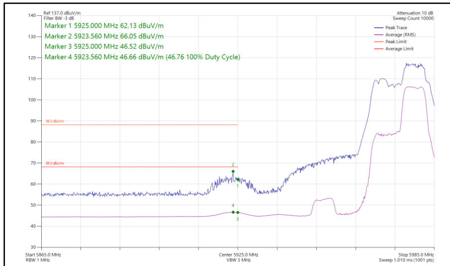
Figure 337 - 802.11be EHT40, RU52+26-75, SISO, Core 0 - 5965 MHz Band Edge Frequency 5925 MHz
