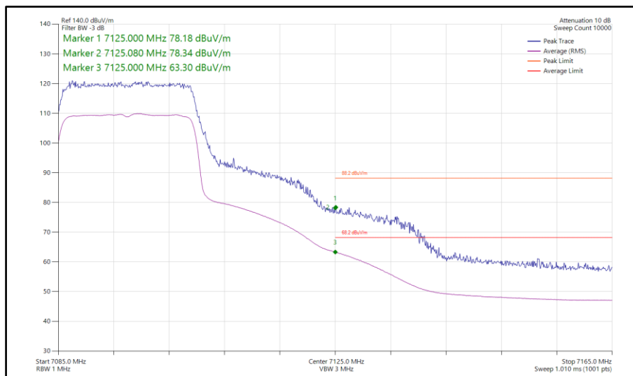
Figure 327 - 802.11ax HE20, SU, SDM, Core 0-1 - 7095 MHz Band Edge Frequency 7125 MHz
