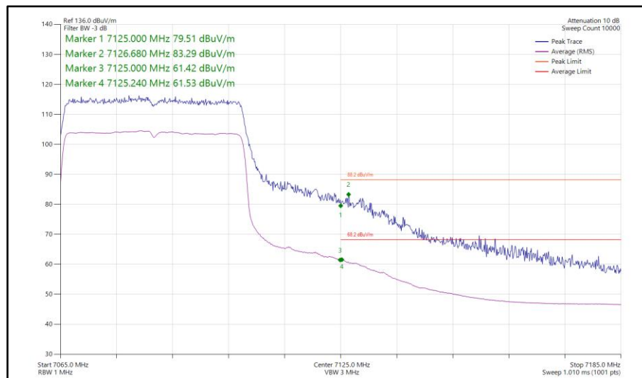
Figure 361 - 802.11ax HE40, SU, SDM, Core 0-1 - 7085 MHz Band Edge Frequency 7125 MHz
