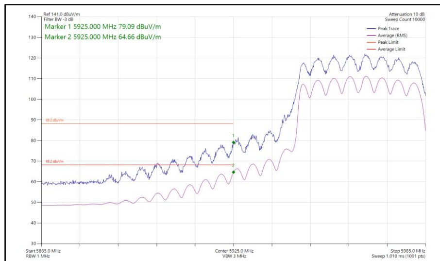
Figure 351 - 802.11ax HE40, SU, CDD, Core 0-1 - 5965 MHz Band Edge Frequency 5925 MHz
