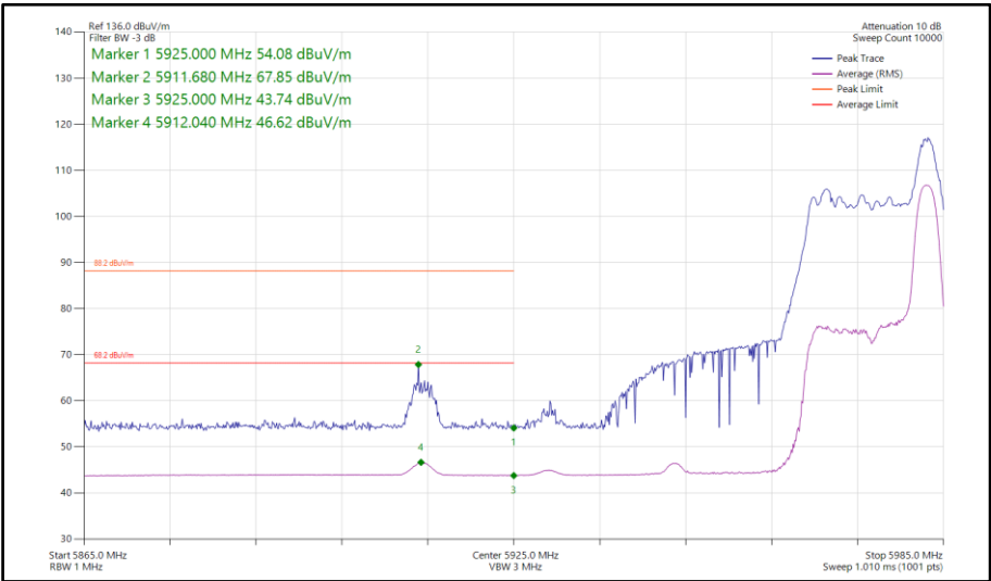
Figure 344 - 802.11ax HE40, RU26-17, SISO, Core 1 - 5965 MHz Band Edge Frequency 5925 MHz
