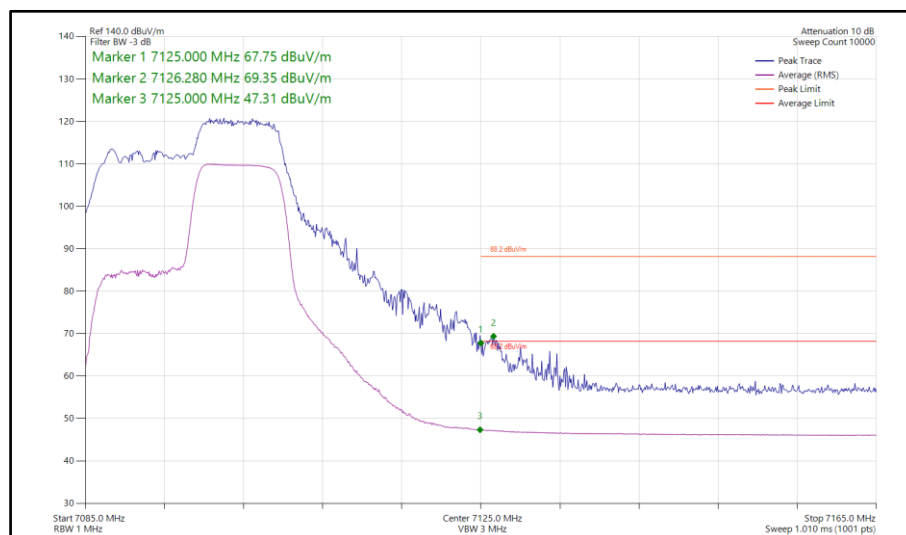
Figure 311 - 802.11ax HE20, RU106-54, SISO, Core 1 - 7095 MHz Band Edge Frequency 7125 MHz
