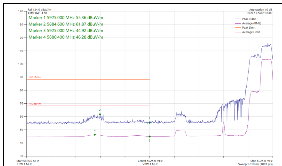
Figure 368 - 802.11ax HE80, RU106-60, SISO, Core 0 - 5985 MHz Band Edge Frequency 5925 MHz
