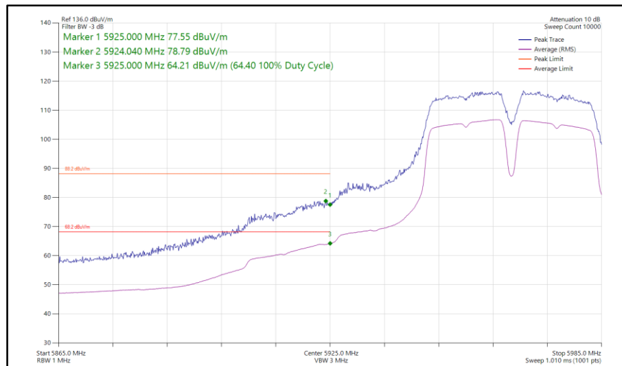
Figure 334 - 802.11a a40, SISO, Core 0 - 5965 MHz Band Edge Frequency 5925 MHz
