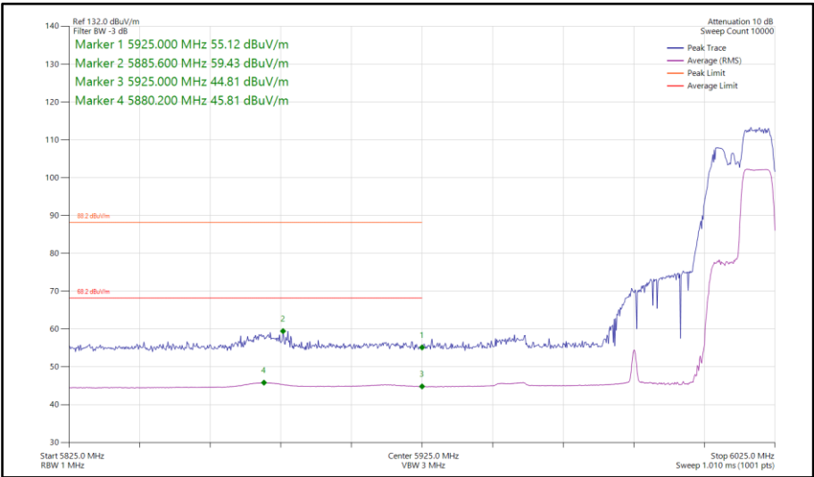
Figure 376 - 802.11ax HE80, RU106-60, SISO, Core 1 - 5985 MHz Band Edge Frequency 5925 MHz
