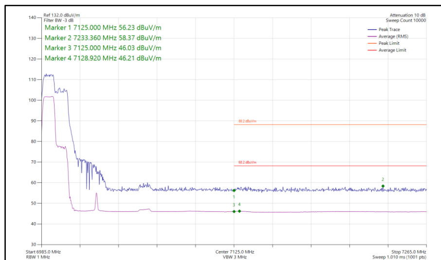
Figure 380 - 802.11ax HE80, RU106-53, SISO, Core 1 - 7025 MHz Band Edge Frequency 7125 MHz
