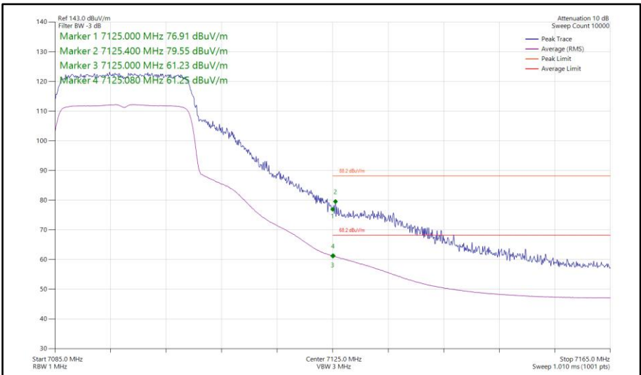
Figure 332 - 802.11ax HE20, SU, TxBF, Core 0-1 - 7095 MHz Band Edge Frequency 7125 MHz
