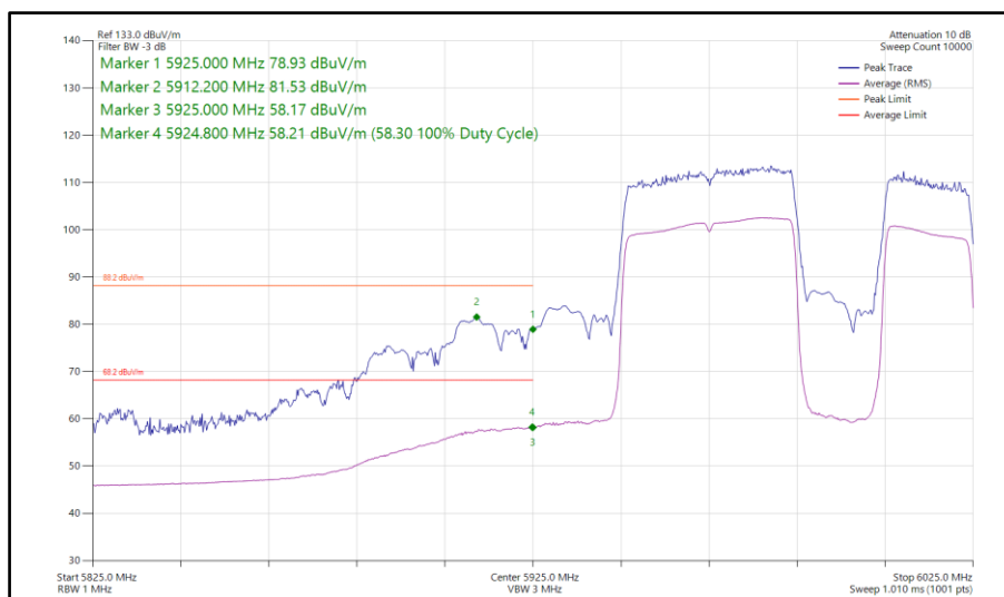
Figure 377 - 802.11be EHT80, RU484+242-92, SISO, Core 1 - 5985 MHz Band Edge Frequency 5925 MHz
