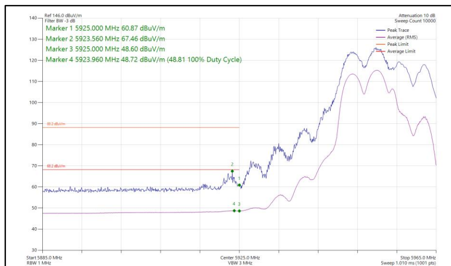
Figure 326 - 802.11be EHT20, RU106+26-82, SDM, Core 0-1 - 5955 MHz Band Edge Frequency 5925 MHz
