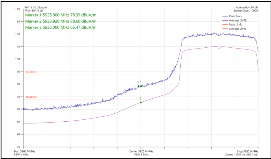
Figure 364 - 802.11ax HE40, SU, TxBF, Core 0-1 - 5965 MHz Band Edge Frequency 5925 MHz
