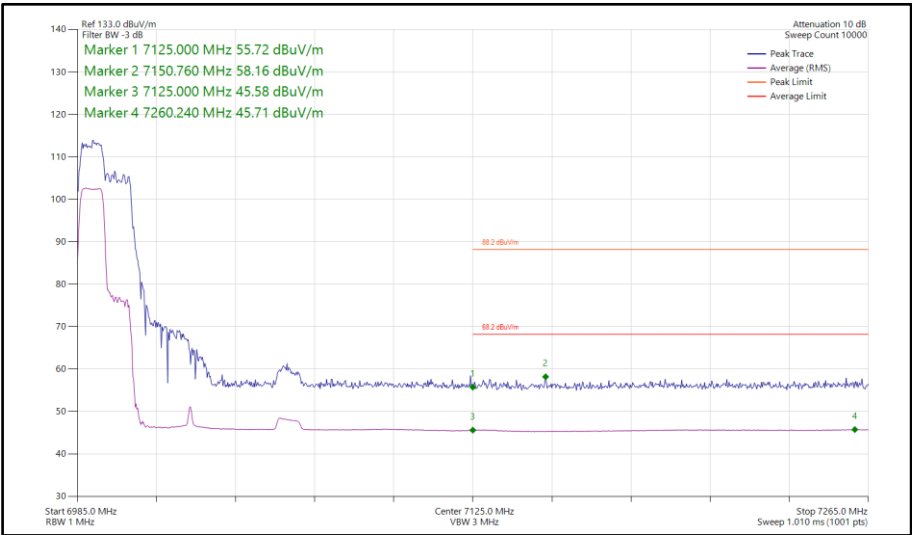
Figure 372 - 802.11ax HE80, RU106-53, SISO, Core 0 - 7025 MHz Band Edge Frequency 7125 MHz
