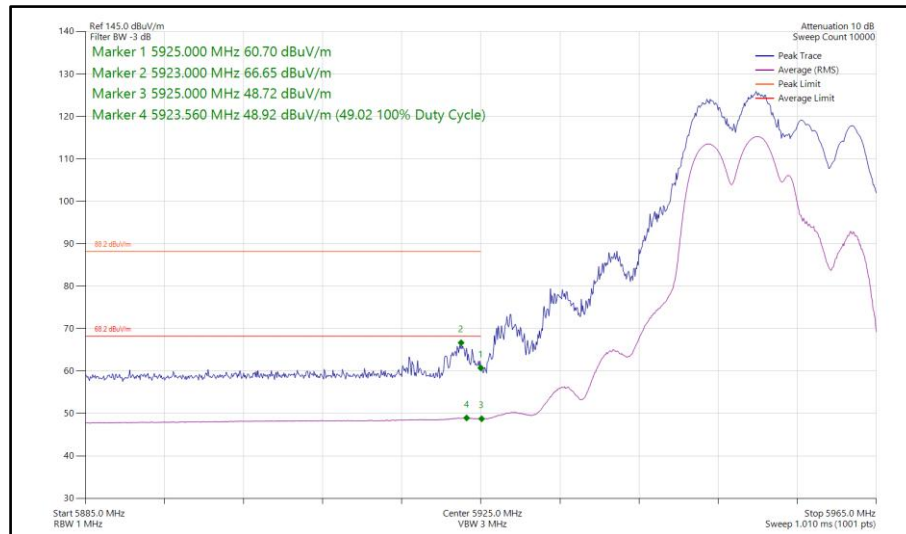
Figure 316 - 802.11be EHT20, RU106+26-82, CDD, Core 0-1 - 5955 MHz Band Edge Frequency 5925 MHz
