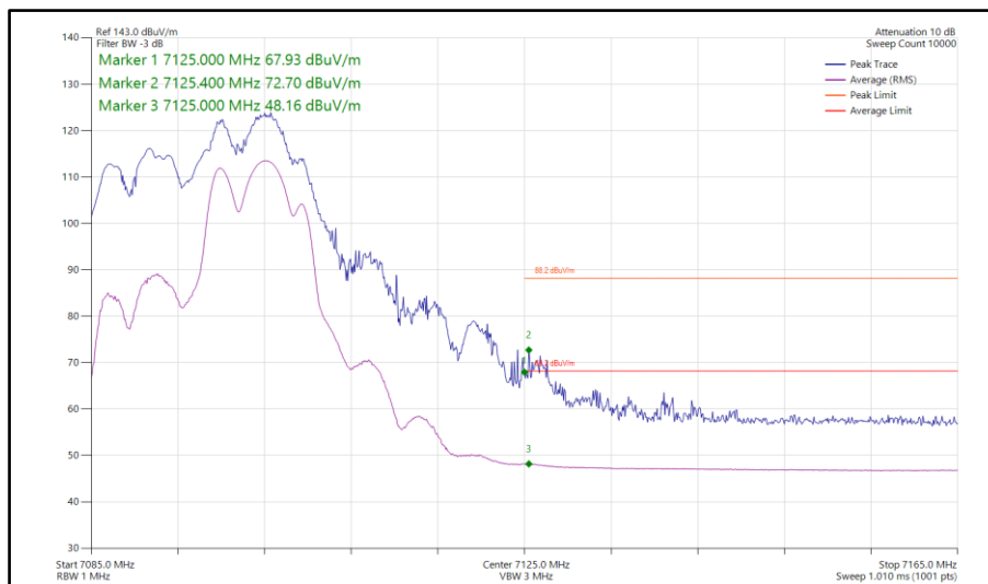
Figure 320 - 802.11ax HE20, RU106-54, CDD, Core 0-1 - 7095 MHz Band Edge Frequency 7125 MHz
