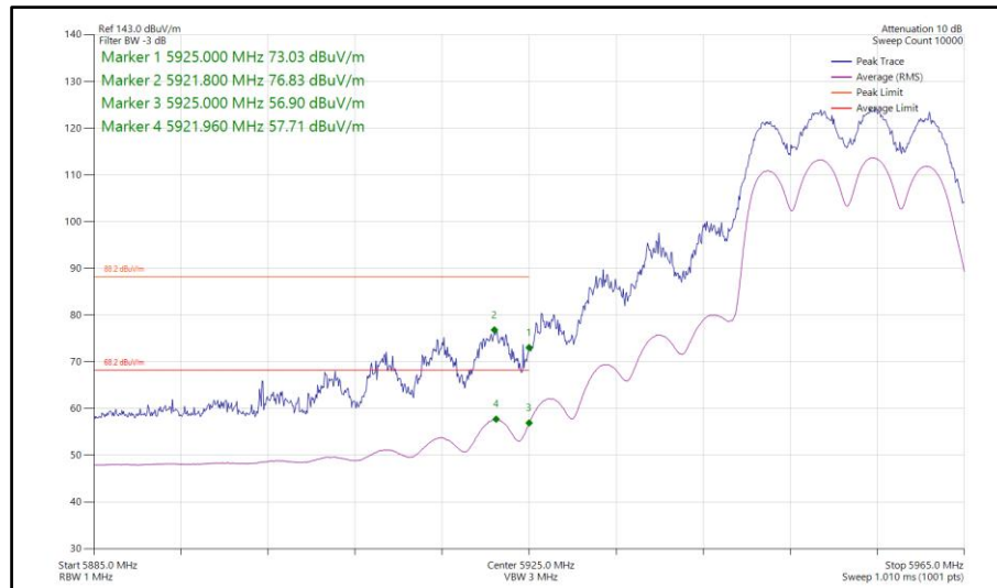
Figure 314 - 802.11ax HE20, SU, CDD, Core 0-1 - 5955 MHz Band Edge Frequency 5925 MHz
