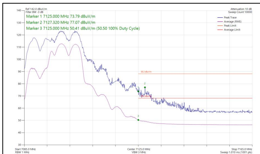
Figure 330 - 802.11be EHT20, RU106+26-83, SDM, Core 0-1 - 7095 MHz Band Edge Frequency 7125 MHz
