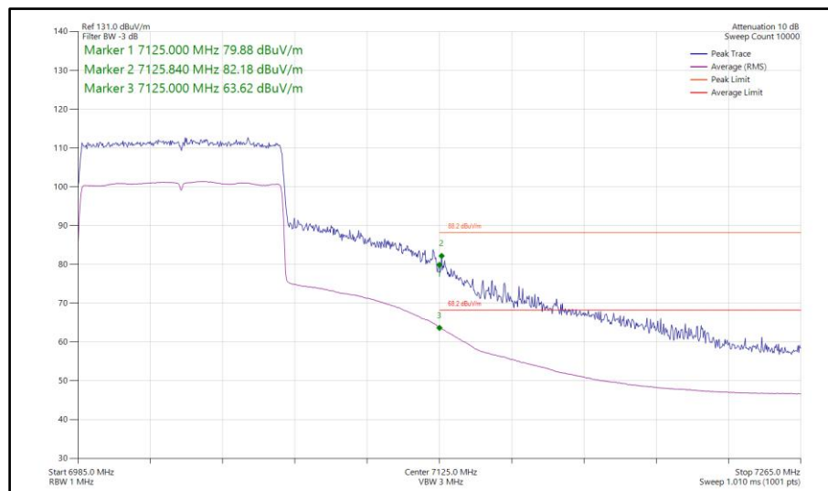
Figure 379 - 802.11ax HE80, SU, SISO, Core 1 - 7025 MHz Band Edge Frequency 7125 MHz
