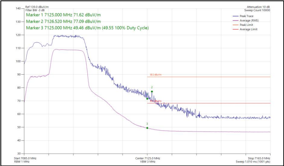
Figure 312 - 802.11be EHT20, RU106+26-83, SISO, Core 1 - 7095 MHz Band Edge Frequency 7125 MHz
