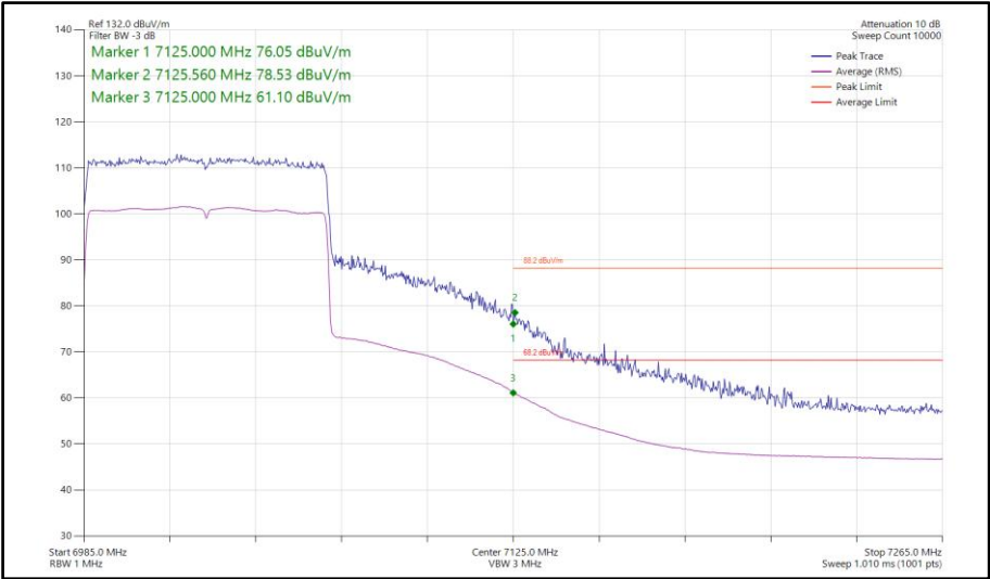
Figure 371 - 802.11ax HE80, SU, SISO, Core 0 - 7025 MHz Band Edge Frequency 7125 MHz
