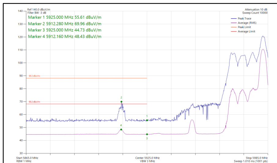
Figure 352 - 802.11ax HE40, RU26-17, CDD, Core 0-1 - 5965 MHz Band Edge Frequency 5925 MHz
