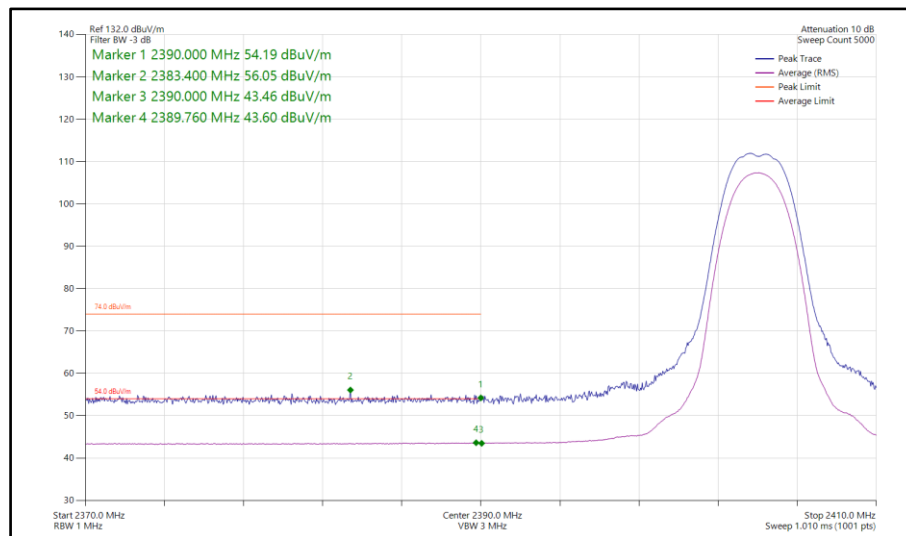
Figure 87 - Bluetooth HDR4, MIMO, Core 0-1 - 2404 MHz Band Edge Frequency 2390 MHz
