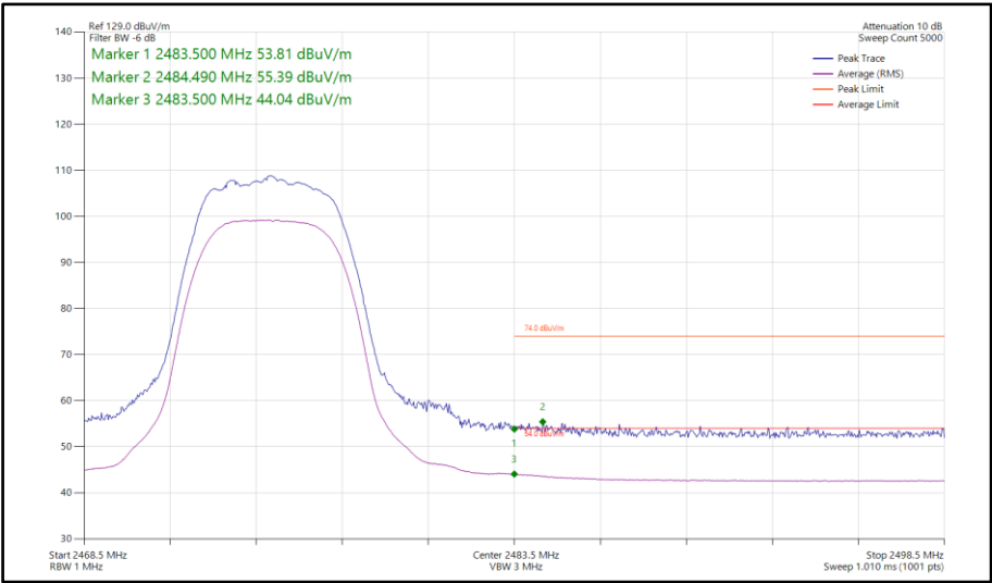
Figure 81 - Bluetooth HDRPM12, SISO, Core 2 - 2475 MHz Band Edge Frequency 2483.5 MHz
