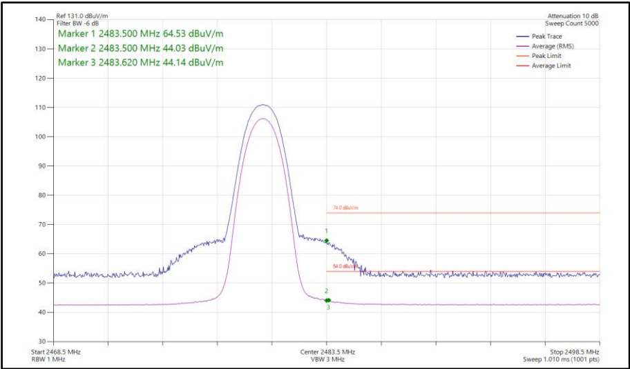
Figure 100 - Bluetooth 3DH5, MIMO, Core 0-1 - 2480 MHz Band Edge Frequency 2483.5 MHz
