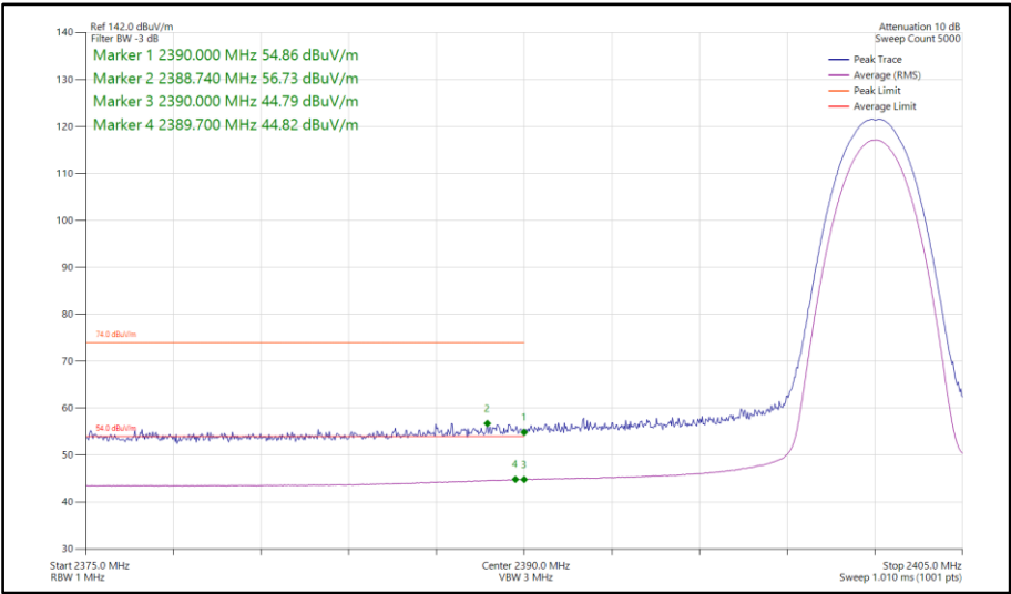
Figure 113 - Bluetooth 2DH5, SISO, Core 0 - 2402 MHz Band Edge Frequency 2390 MHz
