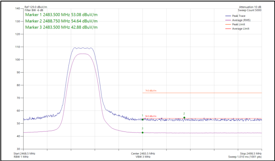
Figure 108 - Bluetooth HDRPS2, MIMO, Core 0-1 - 2476 MHz Band Edge Frequency 2483.5 MHz
