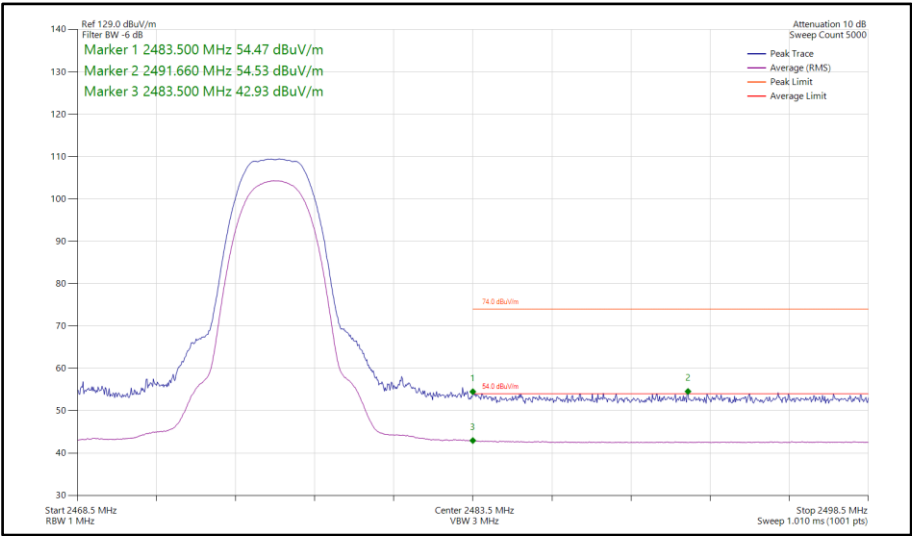
Figure 101 - Bluetooth HDR4, MIMO, Core 0-1 - 2476 MHz Band Edge Frequency 2483.5 MHz
