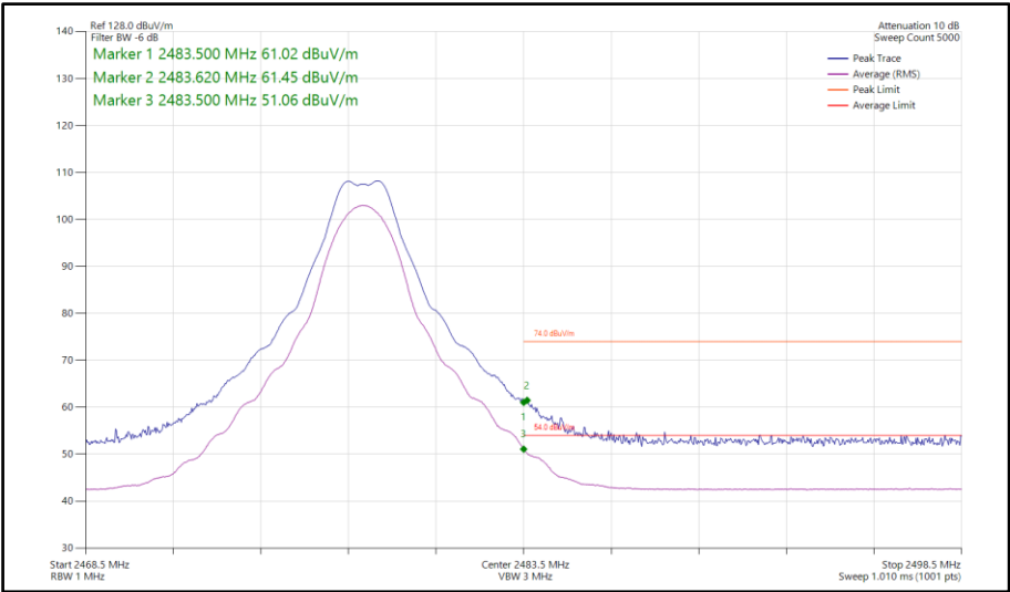
Figure 112 - Bluetooth CS1LE2M, MIMO, Core 0-1 - 2478 MHz Band Edge Frequency 2483.5 MHz
