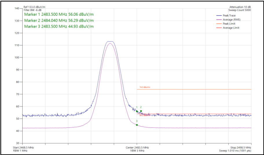
Figure 103 - Bluetooth LE1M, MIMO, Core 0-1 - 2480 MHz Band Edge Frequency 2483.5 MHz
