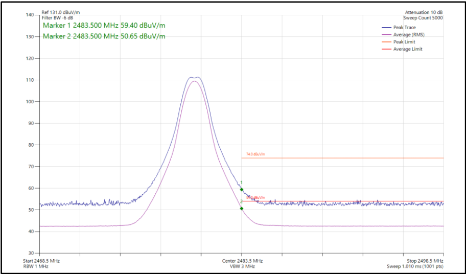
Figure 111 - Bluetooth CS1LE1M, MIMO, Core 0-1 - 2480 MHz Band Edge Frequency 2483.5 MHz
