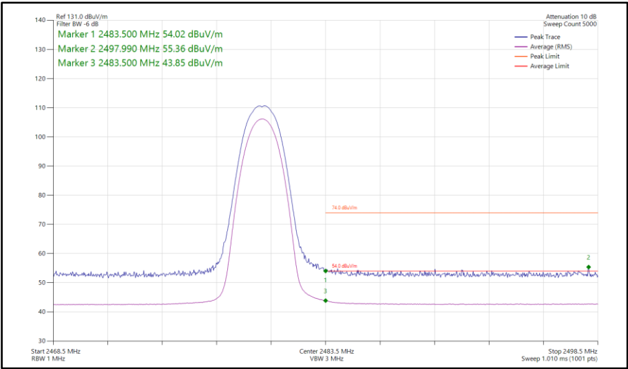
Figure 99 - Bluetooth 2DH5, MIMO, Core 0-1 - 2480 MHz Band Edge Frequency 2483.5 MHz
