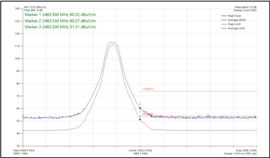
Figure 83 - Bluetooth CS1LE1M, SISO, Core 2 - 2480 MHz Band Edge Frequency 2483.5 MHz
