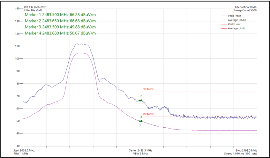
Figure 107 - Bluetooth HDT6, MIMO, Core 0-1 - 2476 MHz Band Edge Frequency 2483.5 MHz
