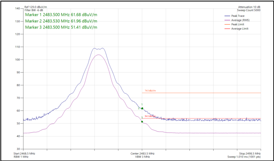
Figure 84 - Bluetooth CS1LE2M, SISO, Core 2 - 2478 MHz Band Edge Frequency 2483.5 MHz
