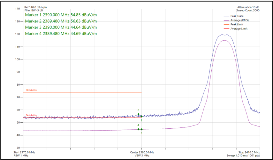
Figure 115 - Bluetooth HDR4, SISO, Core 0 - 2404 MHz Band Edge Frequency 2390 MHz
