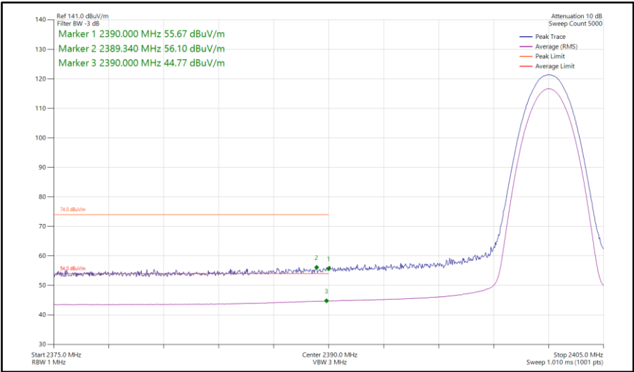
Figure 114 - Bluetooth 3DH5, SISO, Core 0 - 2402 MHz Band Edge Frequency 2390 MHz
