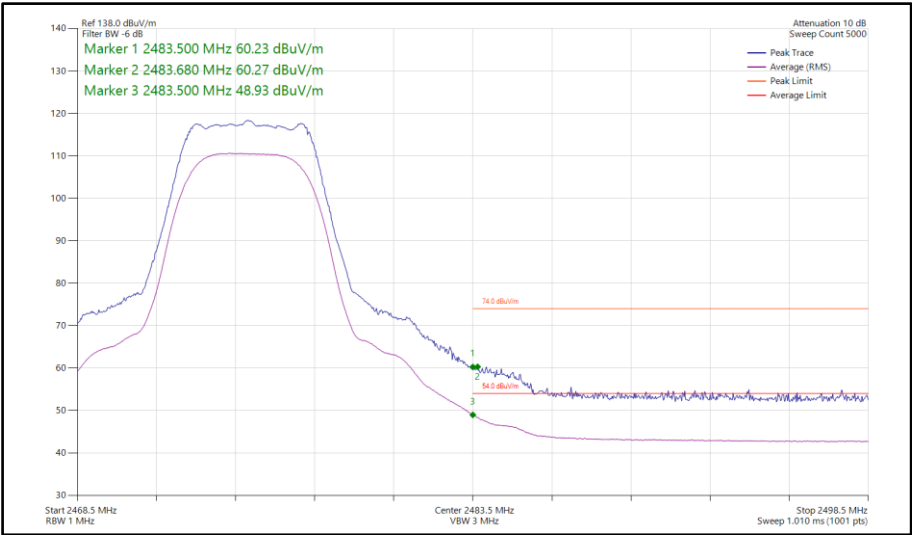
Figure 138 - Bluetooth XHDRPM8, SISO, Core 0 - 2475 MHz Band Edge Frequency 2483.5 MHz
