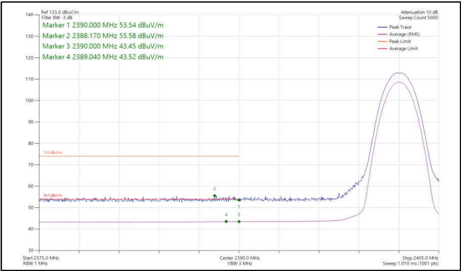
Figure 85 - Bluetooth 2DH5, MIMO, Core 0-1 - 2402 MHz Band Edge Frequency 2390 MHz
