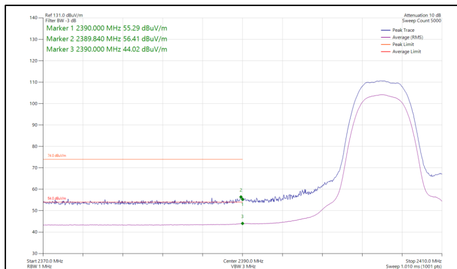
Figure 88 - Bluetooth HDR8, MIMO, Core 0-1 - 2404 MHz Band Edge Frequency 2390 MHz
