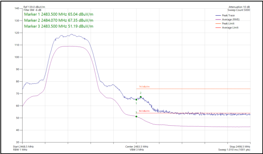
Figure 137 - Bluetooth HDRPM12, SISO, Core 0 - 2475 MHz Band Edge Frequency 2483.5 MHz
