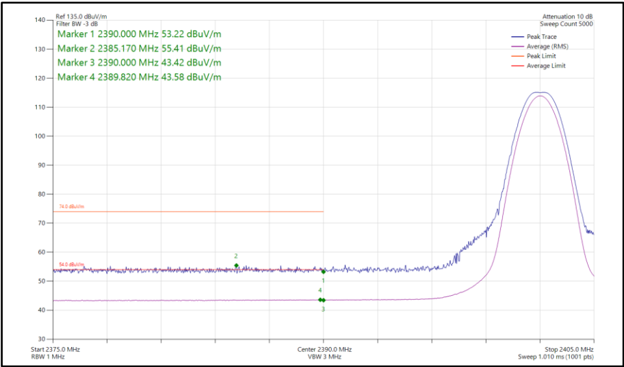
Figure 89 - Bluetooth LE1M, MIMO, Core 0-1 - 2402 MHz Band Edge Frequency 2390 MHz
