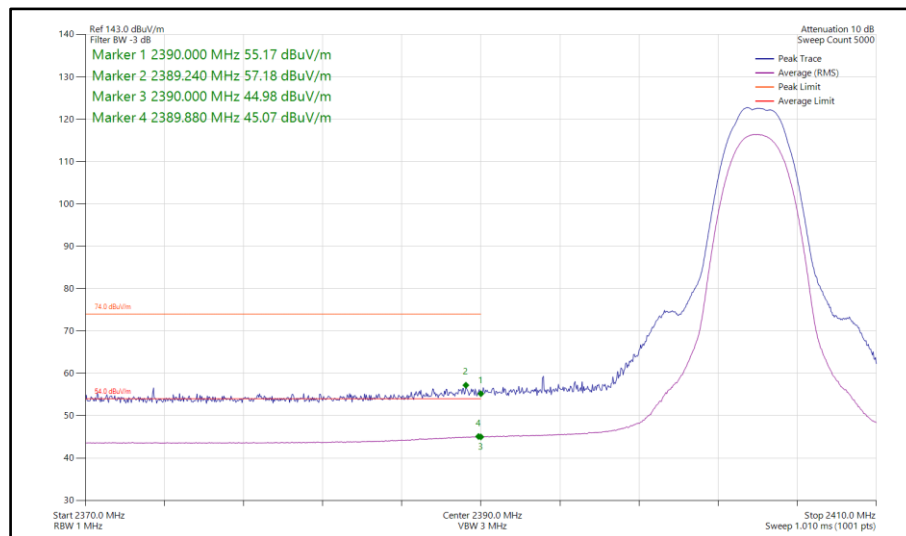
Figure 121 - Bluetooth HDT6, SISO, Core 0 - 2404 MHz Band Edge Frequency 2390 MHz
