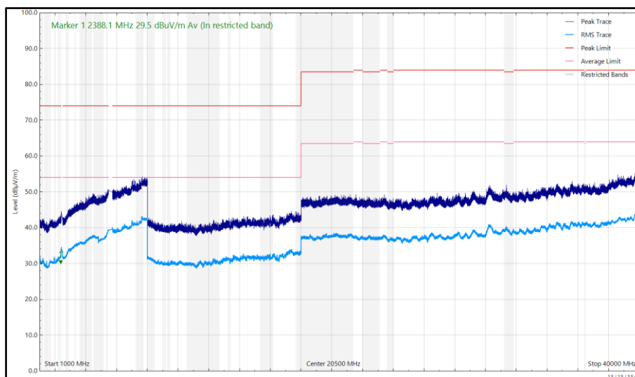
Figure 3 - U-NII-2C - 5640 MHz (CH128), HT20, CDD, Core 0 + Core 1 and 2441 MHz, DH5, ePA, Core 0 + Core 1, 1 GHz to 40 GHz, Horizontal
