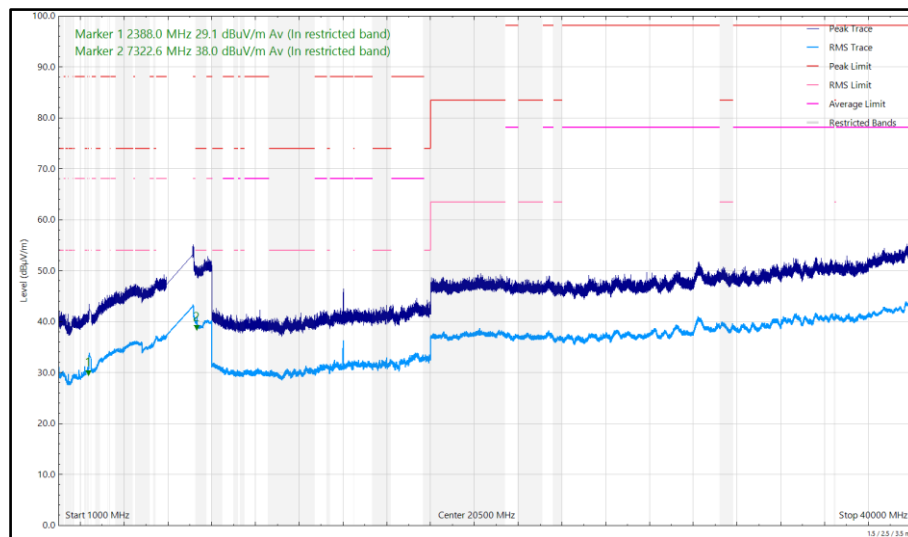
Figure 7 - U-NII-8 - 6995 MHz (CH209), HE20, SU, CDD, Core 0 + Core 1 and 2441 MHz, DH5, ePA, Core 0 + Core 1, 1 GHz to 40 GHz, Horizontal
