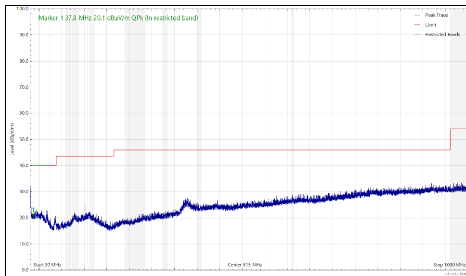
Figure 30 - 2437 MHz (CH6), HT20, CDD, Core 0 + Core 1 and 2450 MHz (CH20), Thread, iPA, Core 2 and 5788 MHz, DH5, ePA, Core 0 + Core 1, 30 MHz to 1 GHz, Horizontal (Peak)
