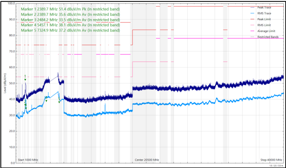
Figure 9 - U-NII-8 - 6995 MHz (CH209), HE20, SU, CDD, Core 0 + Core 1 and 2441 MHz, DH5, ePA, Core 0 + Core 1, 1 GHz to 40 GHz, Vertical
