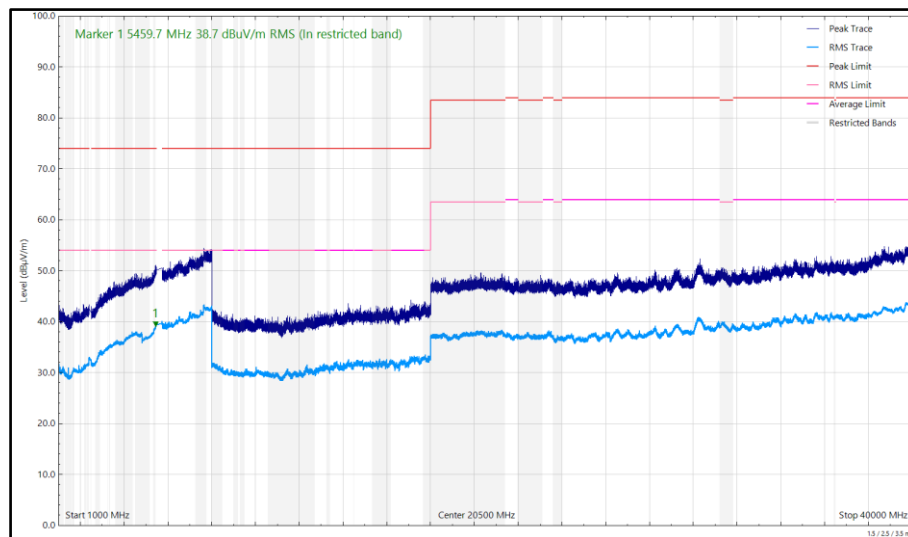
Figure 15 - U-NII-2C - 5640 MHz (CH128), HT20, CDD, Core 0 + Core 1 and 2440 MHz (CH18), Thread, ePA, Core 1, 1 GHz to 40 GHz, Horizontal
