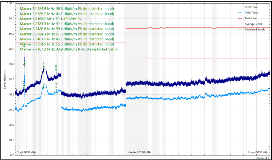
Figure 37 - 2437 MHz (CH6), HT20, Core 0 + Core 1 and U-NII-2C - 5640 MHz (CH128), HT20, CDD, Core 0 + Core 1 and 2450 MHz, DH5, iPA, Core 2, 1 GHz to 40 GHz, Vertical
