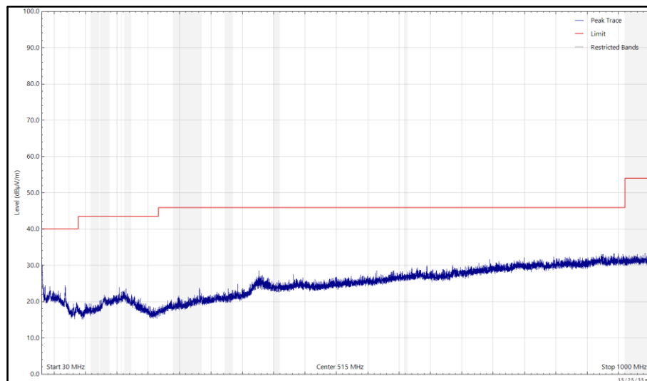
Figure 34 - 2437 MHz (CH6), HT20, Core 0 + Core 1 and 5640 MHz (CH128), HT20, CDD, Core 0 + Core 1 and 2450 MHz, DH5, iPA, Core 2, 30 MHz to 1 GHz, Horizontal (Peak)
