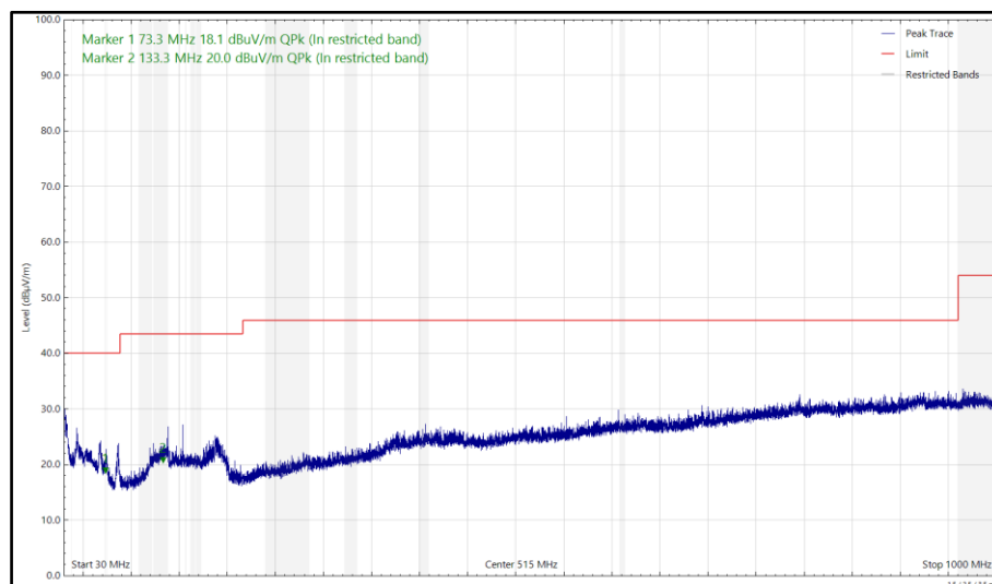
Figure 8 - U-NII-8 - 6995 MHz (CH209), HE20, SU, CDD, Core 0 + Core 1 and 2441 MHz, DH5, ePA, Core 0 + Core 1, 30 MHz to 1 GHz, Vertical (Peak)
