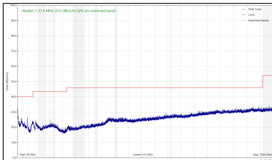
Figure 52 - 2441 MHz, DH5, ePA, Core 0 + Core 1 and 5788 MHz, DH5, ePA, Core 0 + Core 1, 30 MHz to 1 GHz, Vertical (Peak)
