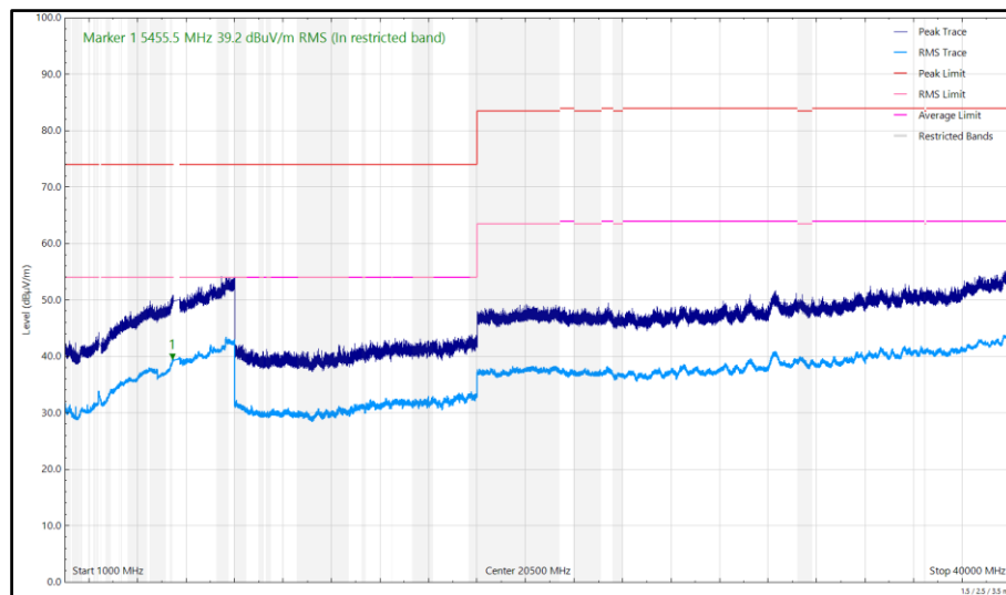
Figure 11 - U-NII-2C - 5640 MHz (CH128), HT20, CDD, Core 0 + Core 1 and 2440 MHz (CH18), Thread, ePA, Core 0, 1 GHz to 40 GHz, Horizontal
