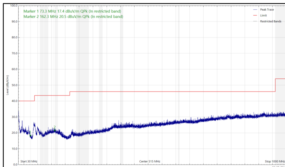
Figure 12 - U-NII-2C - 5640 MHz (CH128), HT20, CDD, Core 0 + Core 1 and 2440 MHz (CH18), Thread, ePA, Core 0, 30 MHz to 1 GHz, Vertical (Peak)
