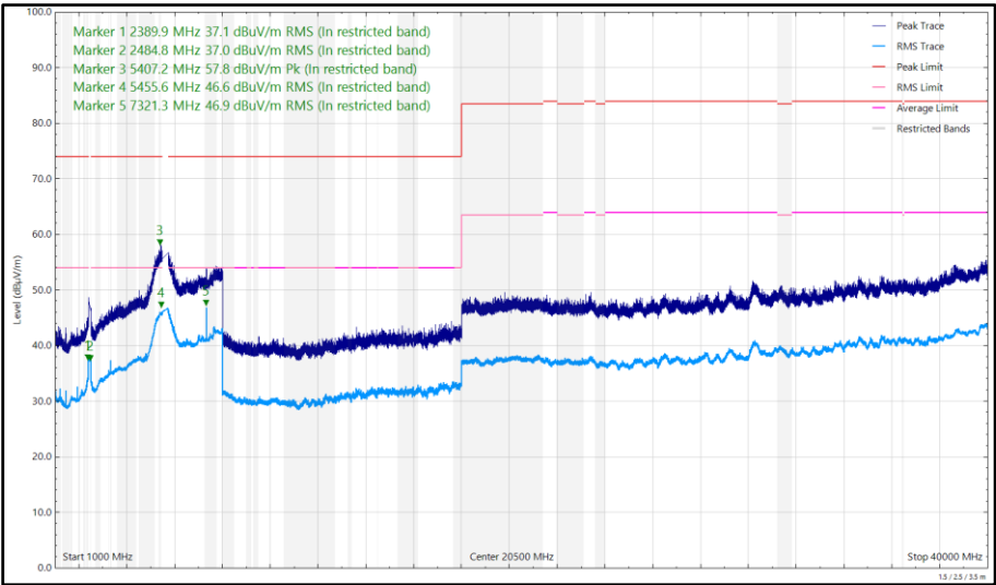
Figure 17 - U-NII-2C - 5640 MHz (CH128), HT20, CDD, Core 0 + Core 1 and 2440 MHz (CH18), Thread, ePA, Core 1, 1 GHz to 40 GHz, Vertical
