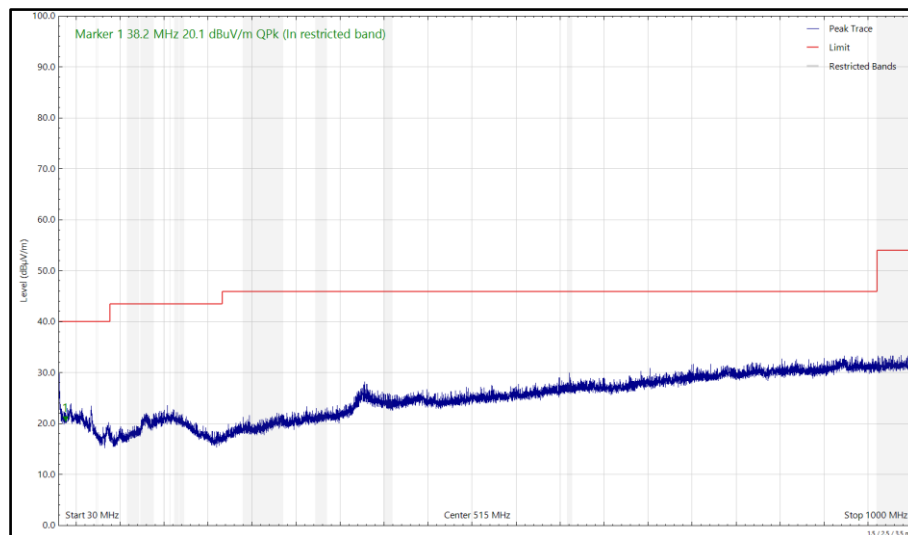
Figure 22 - U-NII-8 - 6995 MHz (CH209), HE20, SU, CDD, Core 0 + Core 1 and 2440 MHz (CH18), Thread, ePA, Core 1, 30 MHz to 1 GHz, Horizontal (Peak)
