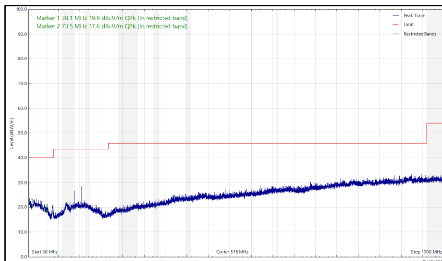
Figure 6 - U-NII-8 - 6995 MHz (CH209), HE20, SU, CDD, Core 0 + Core 1 and 2441 MHz, DH5, ePA, Core 0 + Core 1, 30 MHz to 1 GHz, Horizontal (Peak)
