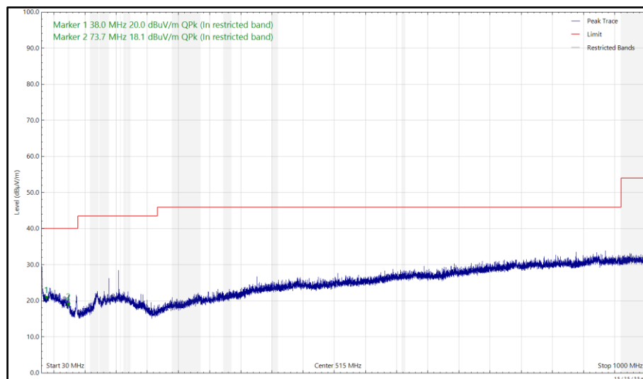
Figure 2 - U-NII-2C - 5640 MHz (CH128), HT20, CDD, Core 0 + Core 1 and 2441 MHz, DH5, ePA, Core 0 + Core 1, 30 MHz to 1 GHz, Horizontal (Peak)
