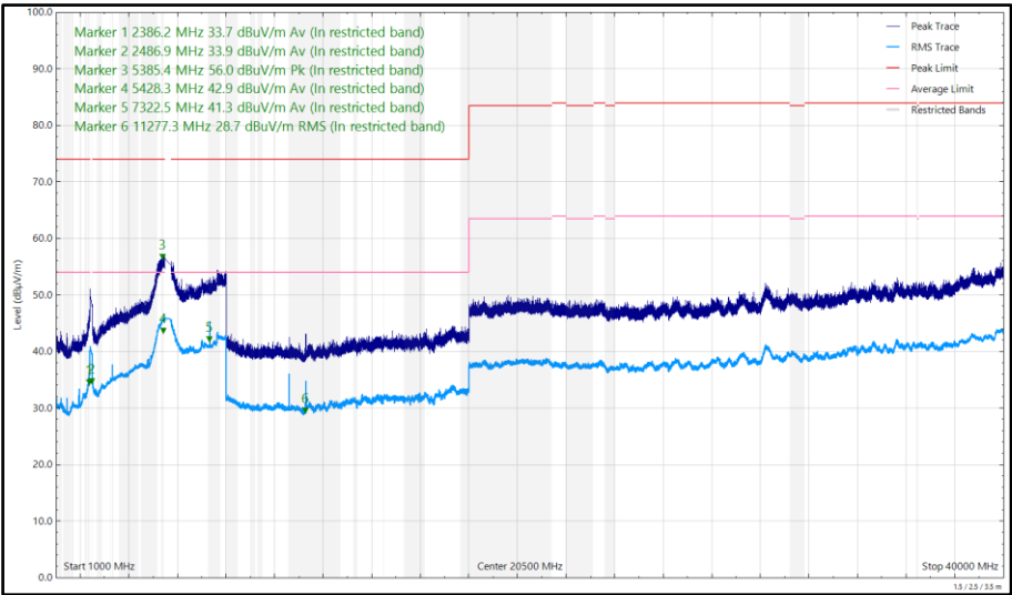
Figure 5 - U-NII-2C - 5640 MHz (CH128), HT20, CDD, Core 0 + Core 1 and 2441 MHz, DH5, ePA, Core 0 + Core 1, 1 GHz to 40 GHz, Vertical
