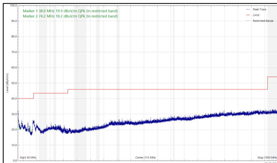
Figure 16 - U-NII-2C - 5640 MHz (CH128), HT20, CDD, Core 0 + Core 1 and 2440 MHz (CH18), Thread, ePA, Core 1, 30 MHz to 1 GHz, Vertical (Peak)
