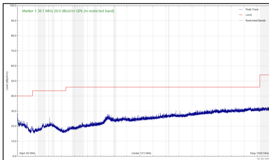
Figure 10 - U-NII-2C - 5640 MHz (CH128), HT20, CDD, Core 0 + Core 1 and 2440 MHz (CH18), Thread, ePA, Core 0, 30 MHz to 1 GHz, Horizontal (Peak)
