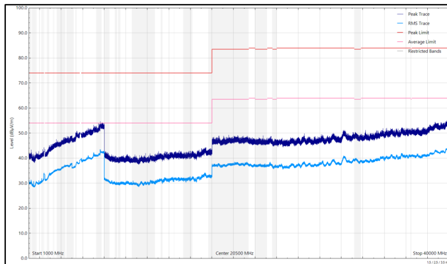
Figure 51 - 2441 MHz, DH5, ePA, Core 0 + Core 1 and 5788 MHz, DH5, ePA, Core 0 + Core 1, 1 GHz to 40 GHz, Horizontal
