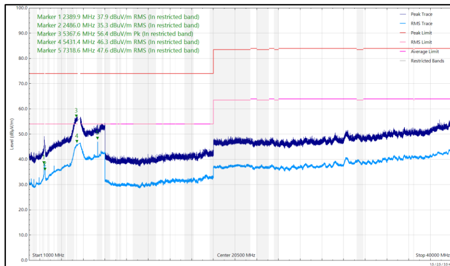
Figure 13 - U-NII-2C - 5640 MHz (CH128), HT20, CDD, Core 0 + Core 1 and 2440 MHz (CH18), Thread, ePA, Core 0, 1 GHz to 40 GHz, Vertical
