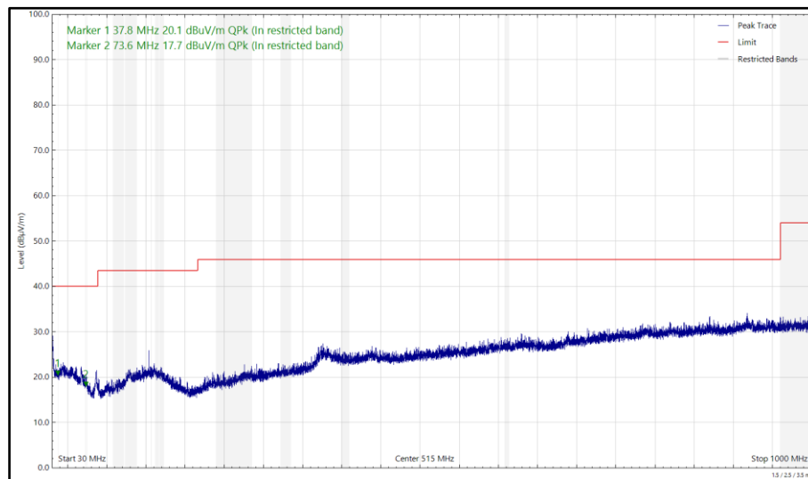
Figure 14 - U-NII-2C - 5640 MHz (CH128), HT20, CDD, Core 0 + Core 1 and 2440 MHz (CH18), Thread, ePA, Core 1, 30 MHz to 1 GHz, Horizontal (Peak)
