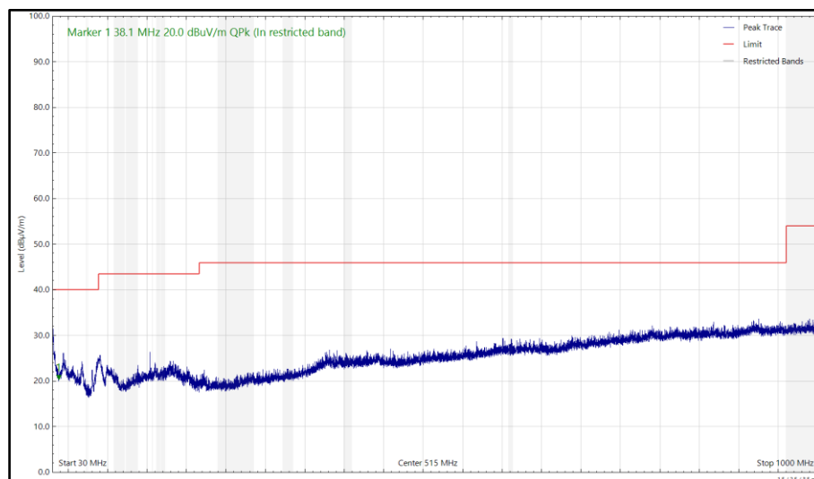
Figure 24 - U-NII-8 - 6995 MHz (CH209), HE20, SU, CDD, Core 0 + Core 1 and 2440 MHz (CH18), Thread, ePA, Core 1, 30 MHz to 1 GHz, Vertical (Peak)
