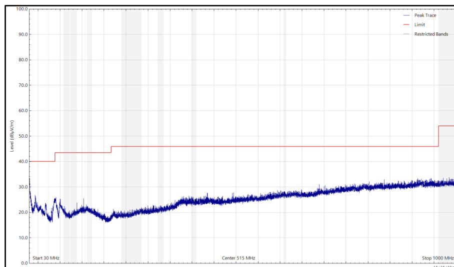
Figure 36 - 2437 MHz (CH6), HT20, Core 0 + Core 1 and 5640 MHz (CH128), HT20, CDD, Core 0 + Core 1 and 2450 MHz, DH5, iPA, Core 2, 30 MHz to 1 GHz, Vertical (Peak)
