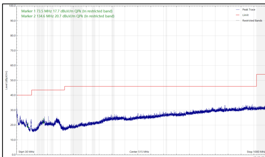
Figure 4 - U-NII-2C - 5640 MHz (CH128), HT20, CDD, Core 0 + Core 1 and 2441 MHz, DH5, ePA, Core 0 + Core 1, 30 MHz to 1 GHz, Vertical (Peak)
