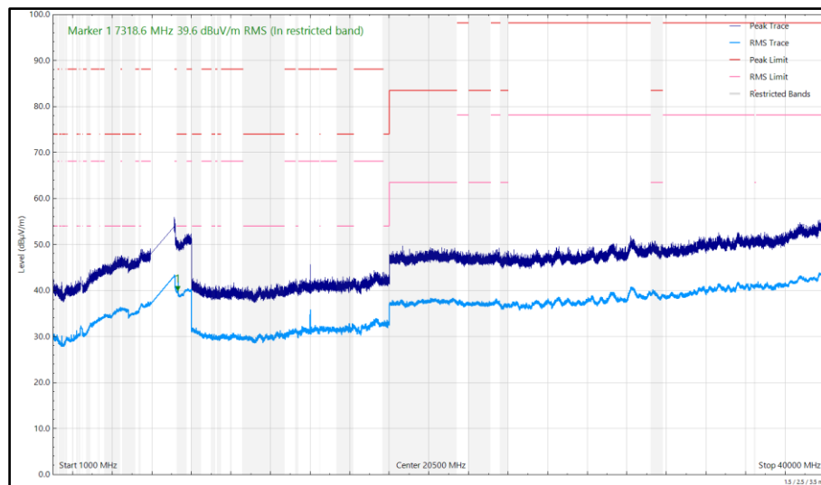
Figure 23 - U-NII-8 - 6995 MHz (CH209), HE20, SU, CDD, Core 0 + Core 1 and 2440 MHz (CH18), Thread, ePA, Core 1, 1 GHz to 40 GHz, Horizontal
