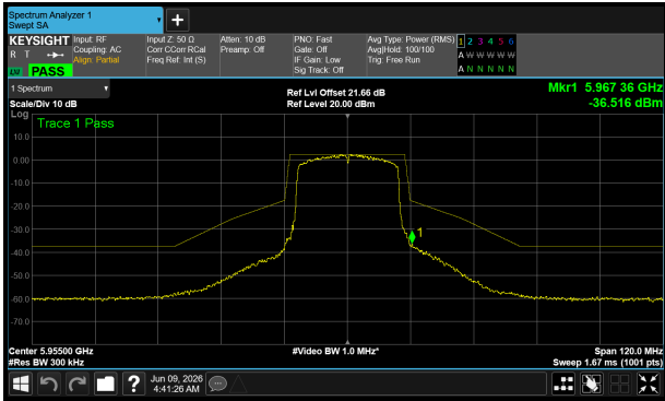
5955 MHz – Core 1
