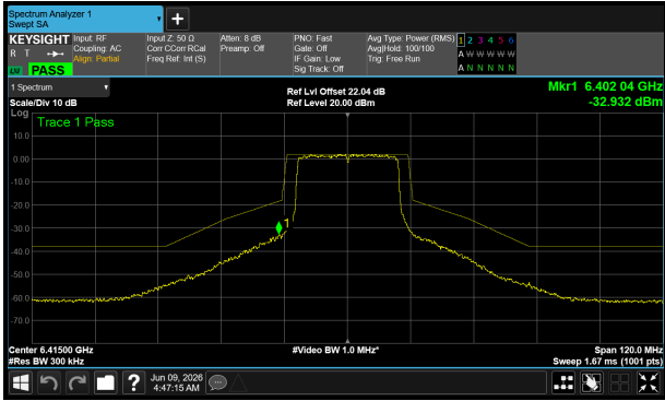
6415 MHz – Core 1
