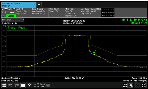
6175 MHz – Core 0
