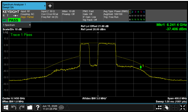
6145 MHz – Core 1
