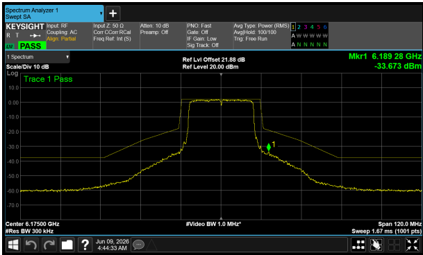
6175 MHz – Core 1
