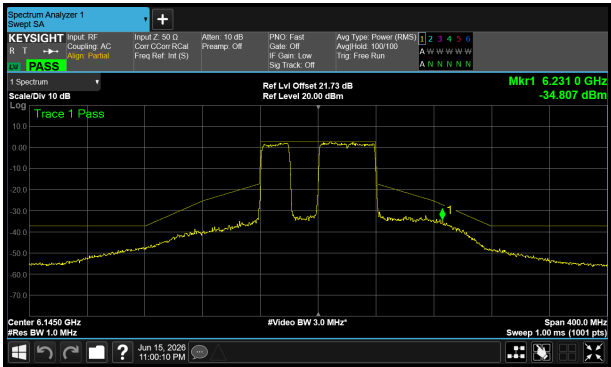
6145 MHz – Core 0
