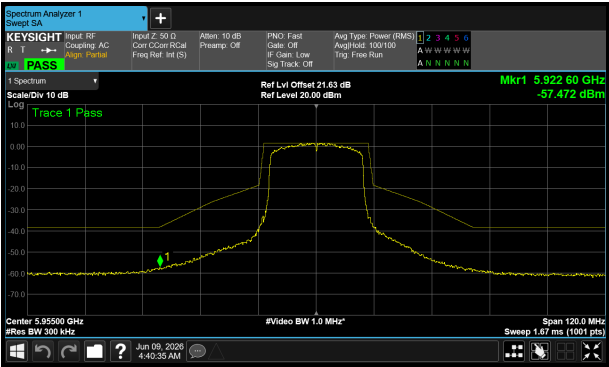
5955 MHz – Core 0
