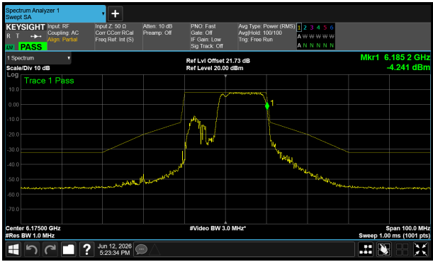
6175 MHz – Core 0
