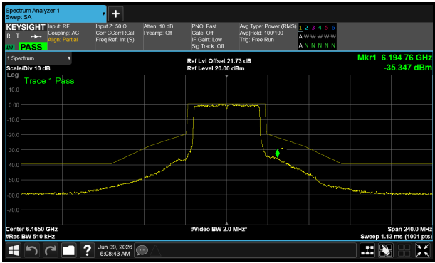
6165 MHz – Core 0
