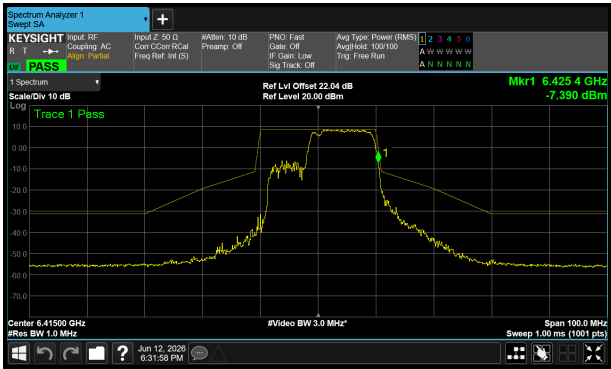
6415 MHz – Core 1
