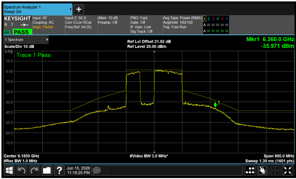
6185 MHz – Core 1
