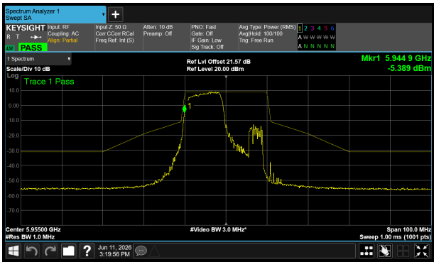
5955 MHz – Core 1
