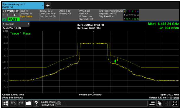
6405 MHz – Core 0
