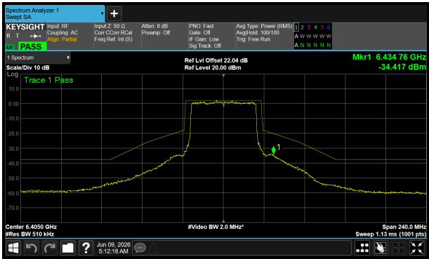
6405 MHz – Core 1
