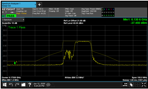
6175 MHz – Core 1
