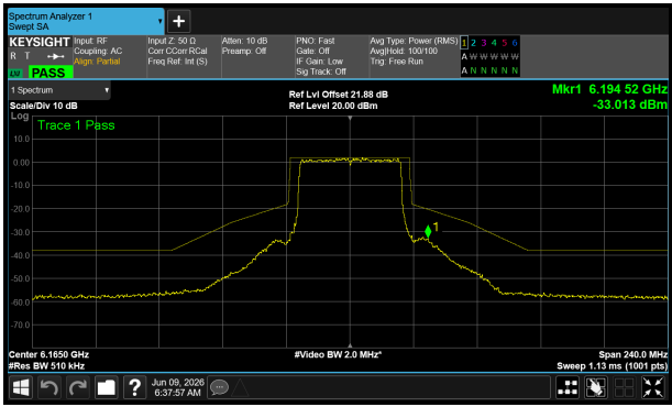
6165 MHz – Core 1
