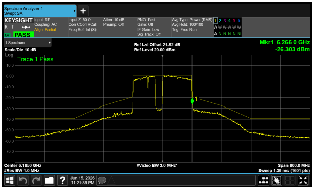
6185 MHz – Core 1
