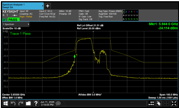
5955 MHz – Core 0
