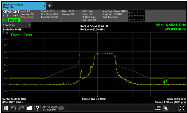
6415 MHz – Core 0
