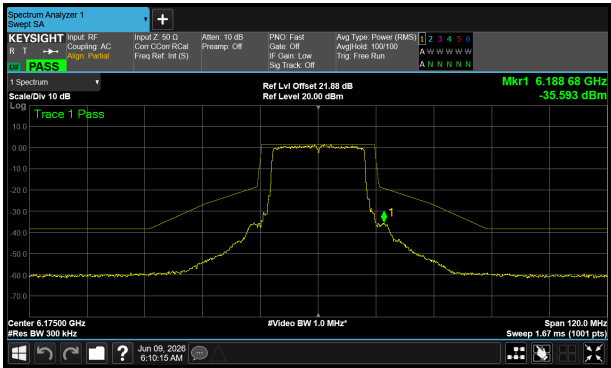
6175 MHz – Core 1
