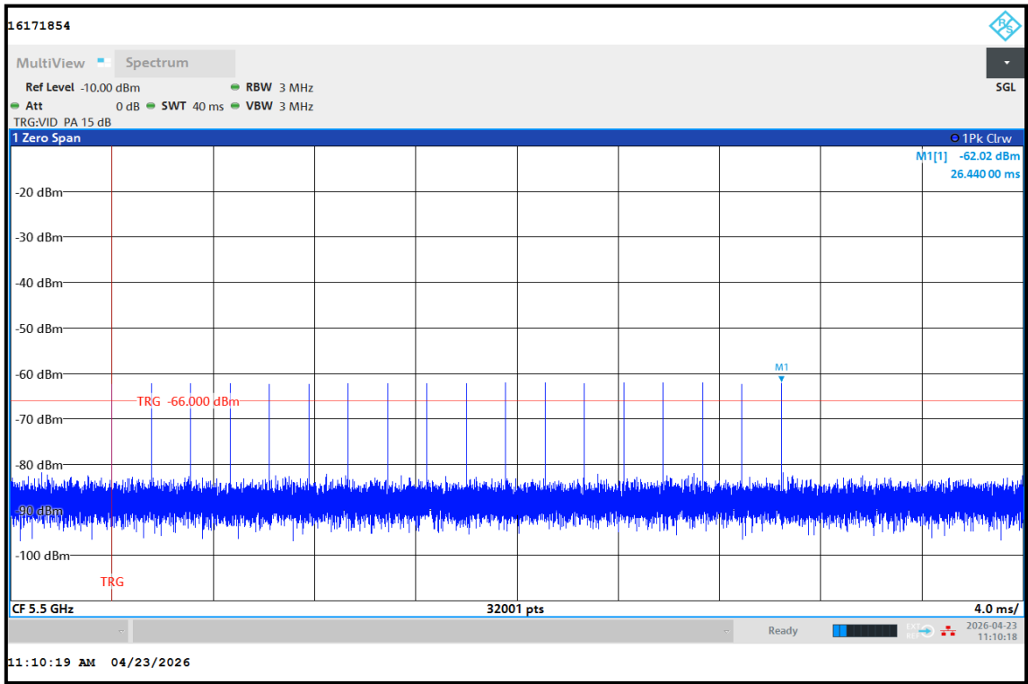
Radar Type 0 – full 18 pulse waveform - Setup 1
