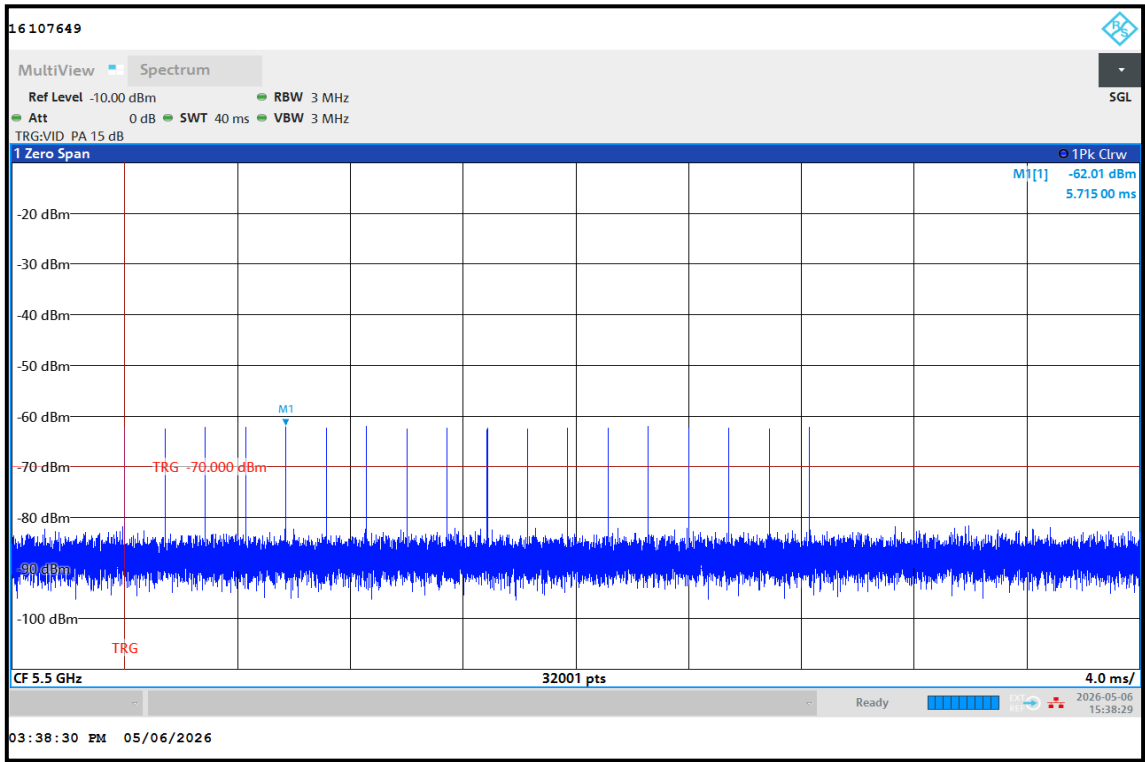
Radar Type 0 – full 18 pulse waveform - Setup 2
