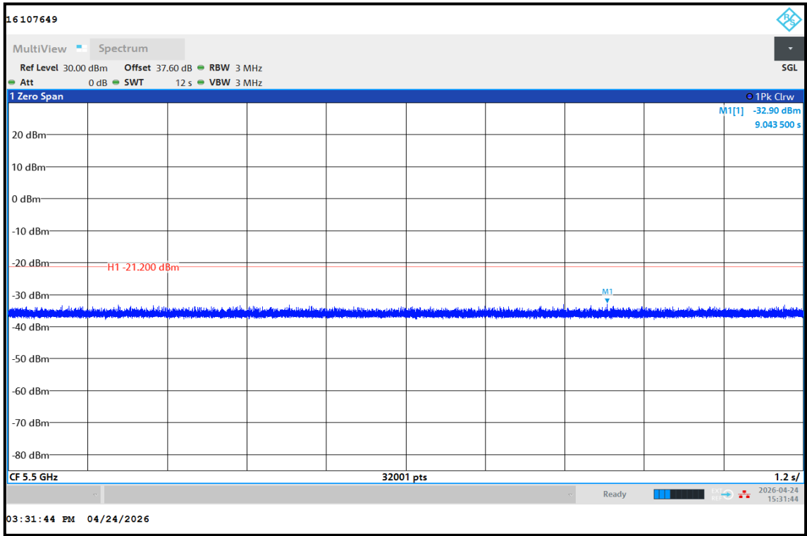
Test System Noise Floor – Setup 1
