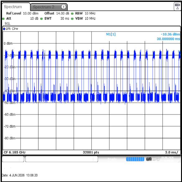
Duty Cycle (31%)
