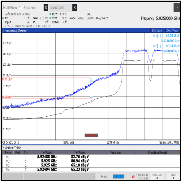
Lower Band Edge / Channel 3
