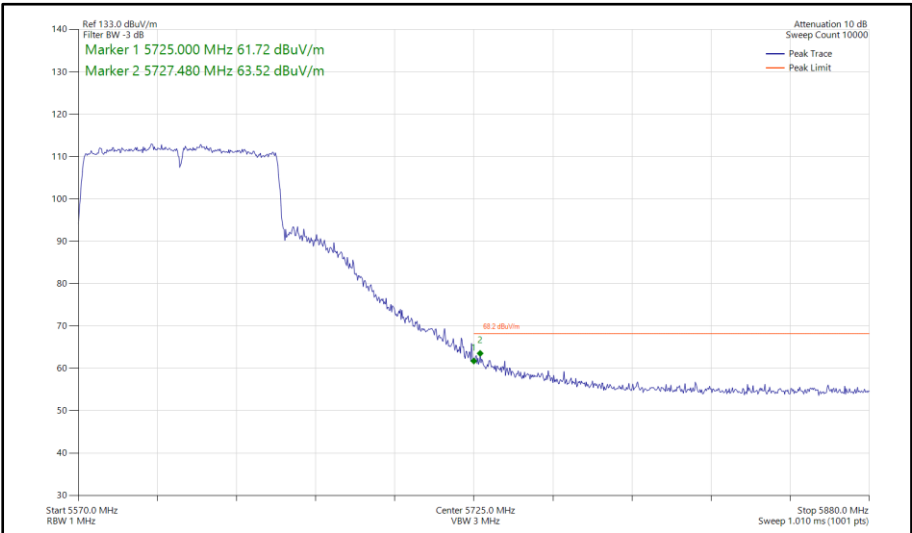
Figure 1066 - 802.11ac VHT80, SISO, Core 1 - 5610 MHz Band Edge Frequency 5725 MHz
