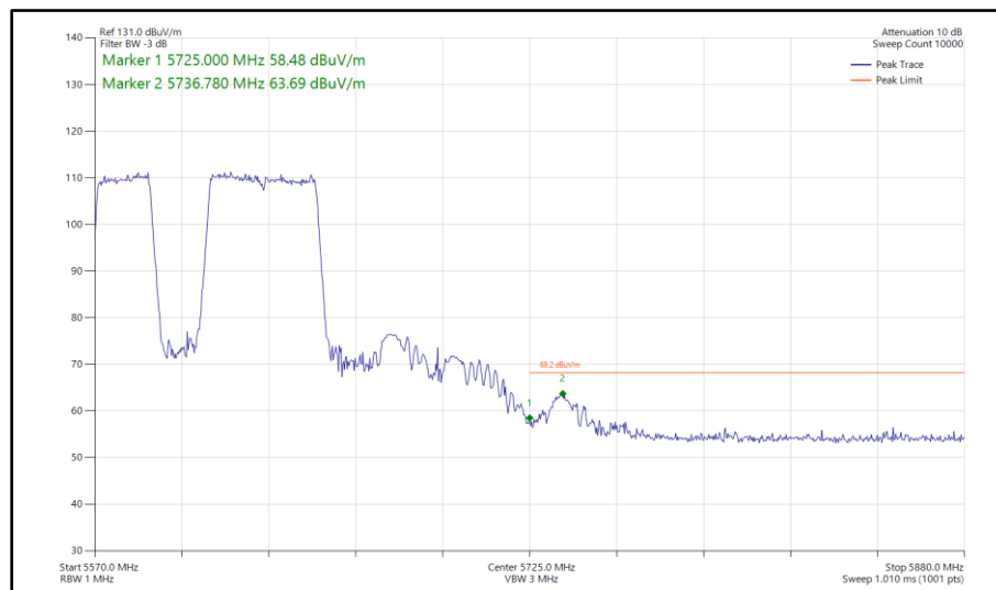
Figure 1069 - 802.11be EHT80, 484+242-91, SISO, Core 1 - 5610 MHz Band Edge Frequency 5725 MHz
