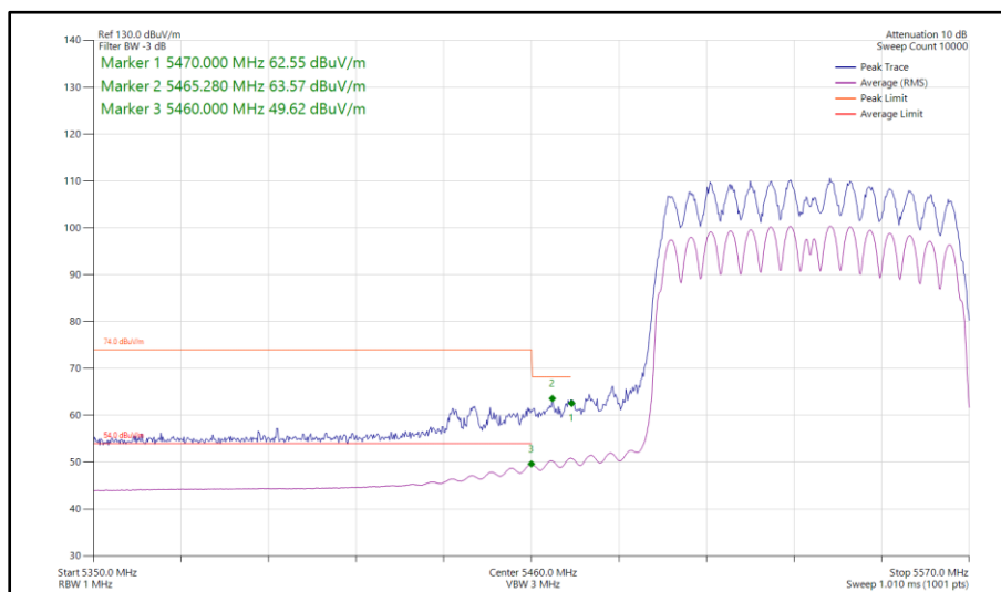
Figure 1081 - 802.11ac VHT80, CDD, Core 0-1 - 5530 MHz Band Edge Frequency 5470 MHz
