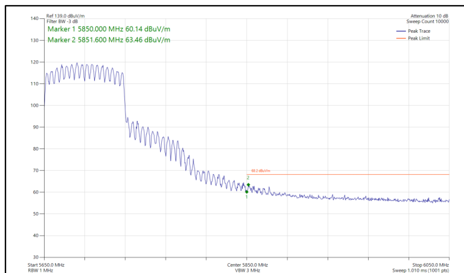
Figure 1097 - 802.11ac VHT80, CDD, Core 0-1 - 5690 MHz Band Edge Frequency 5850 MHz
