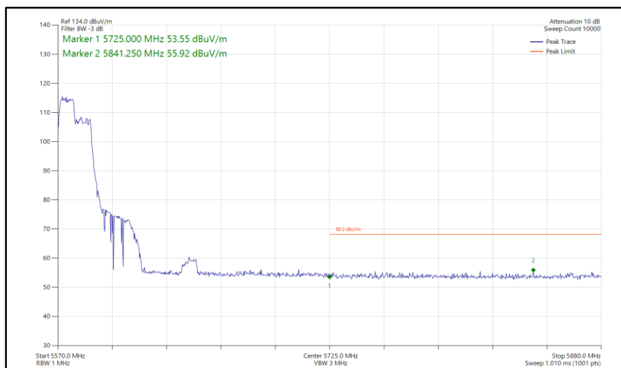
Figure 1068 - 802.11ax HE80, RU 106-53, SISO, Core 1 - 5610 MHz Band Edge Frequency 5725 MHz
