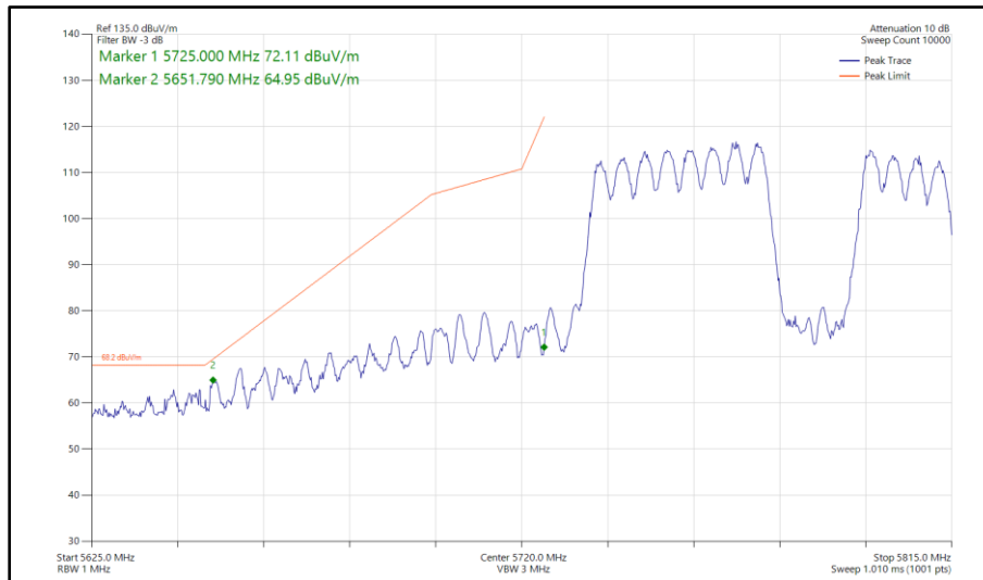
Figure 1112 - 802.11be EHT80, 484+242-92, SDM, Core 0-1 - 5775 MHz Band Edge Frequency 5725 MHz
