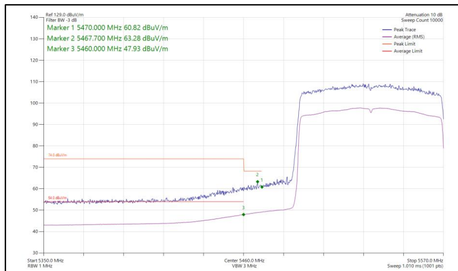
Figure 1126 - 802.11ax HE80, SU, TxBF, Core 0-1 - 5530 MHz Band Edge Frequency 5470 MHz
