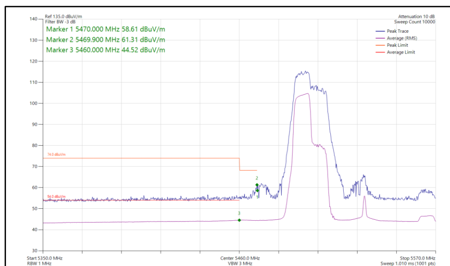
Figure 1058 - 802.11ax HE80, RU 106-53, SISO, Core 1 - 5530 MHz Band Edge Frequency 5470 MHz
