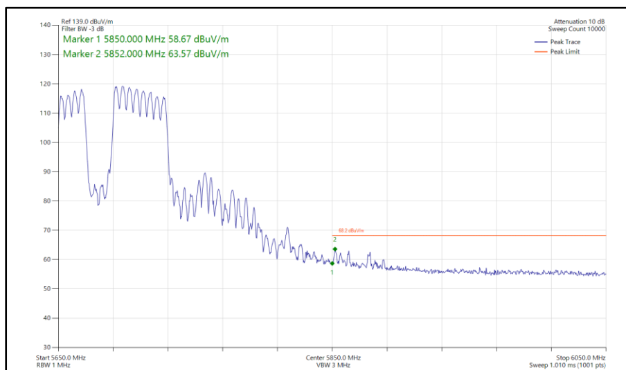
Figure 1103 - 802.11be EHT80, RU 484+242-91, CDD, Core 0-1 - 5690 MHz Band Edge Frequency 5850 MHz
