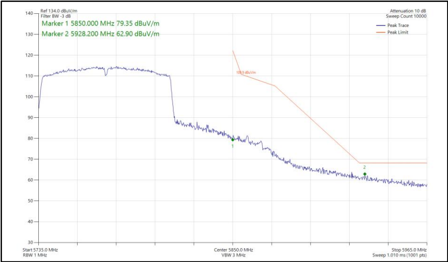
Figure 1073 - 802.11ac VHT80, SISO, Core 1 - 5775 MHz Band Edge Frequency 5850 MHz
