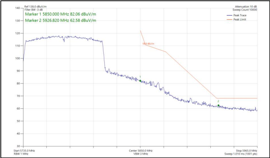
Figure 1118 - 802.11ac VHT80, SDM, Core 0-1 - 5775 MHz Band Edge Frequency 5850 MHz
