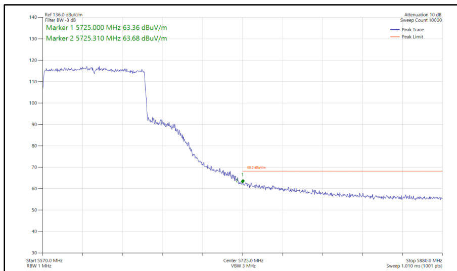
Figure 1130 - 802.11ax HE80, SU, TxBF, Core 0-1 - 5610 MHz Band Edge Frequency 5725 MHz
