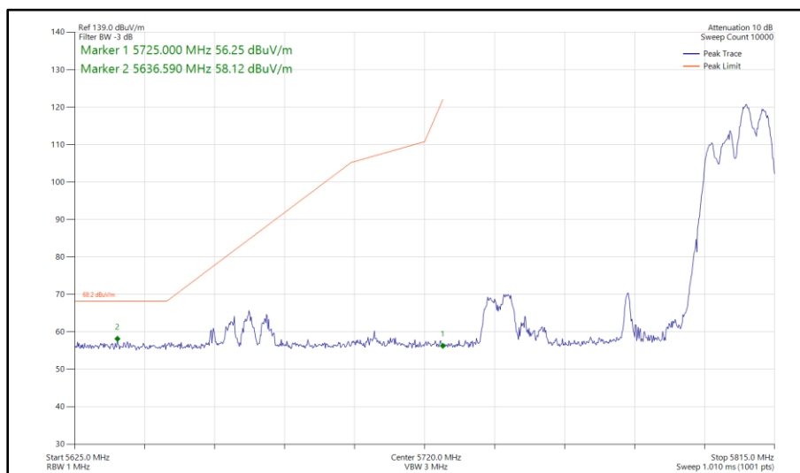
Figure 1111 - 802.11ax HE80, RU 106-60, SDM, Core 0-1 - 5775 MHz Band Edge Frequency 5725 MHz
