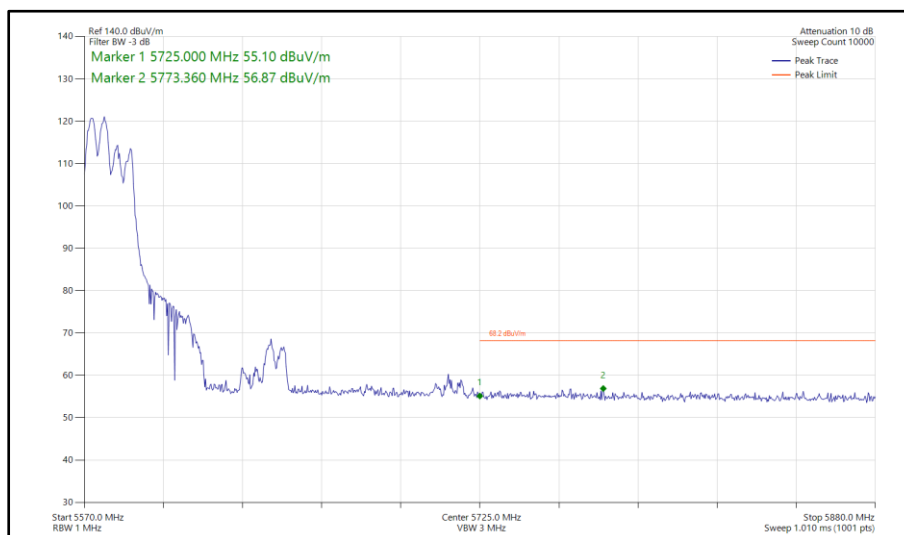
Figure 1093 - 802.11ax HE80, RU 106-53, CDD, Core 0-1 - 5610 MHz Band Edge Frequency 5725 MHz
