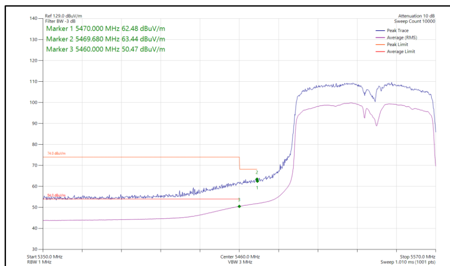
Figure 1125 - 802.11ac VHT80, TxBF, Core 0-1 - 5530 MHz Band Edge Frequency 5470 MHz
