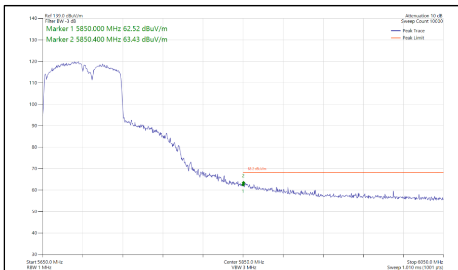
Figure 1131 - 802.11ac VHT80, TxBF, Core 0-1 - 5690 MHz Band Edge Frequency 5850 MHz
