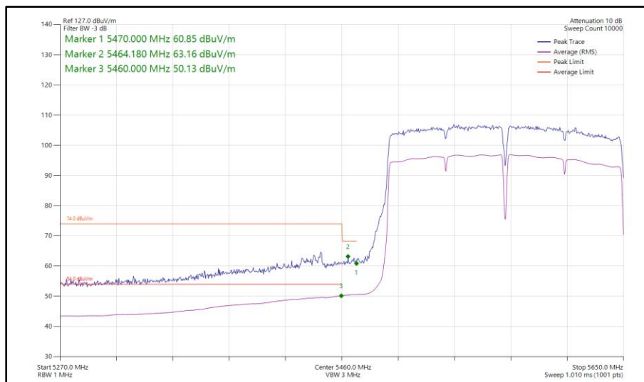
Figure 1136 - 802.11ac VHT160, SISO, Core 0 - 5570 MHz Band Edge Frequency 5470 MHz
