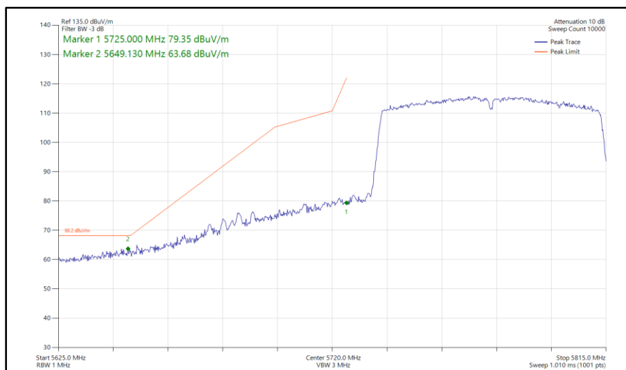
Figure 1109 - 802.11ac VHT80, SDM, Core 0-1 - 5775 MHz Band Edge Frequency 5725 MHz
