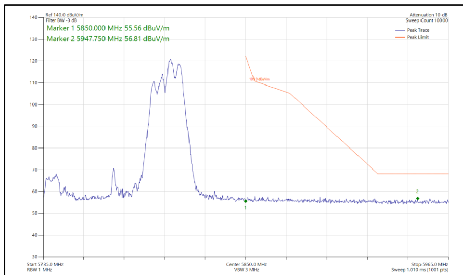
Figure 1122 - 802.11ax HE80, RU 106-60, SDM, Core 0-1 - 5775 MHz Band Edge Frequency 5850 MHz
