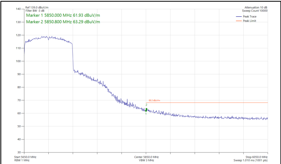
Figure 1133 - 802.11ax HE80, SU, TxBF, Core 0-1 - 5690 MHz Band Edge Frequency 5850 MHz
