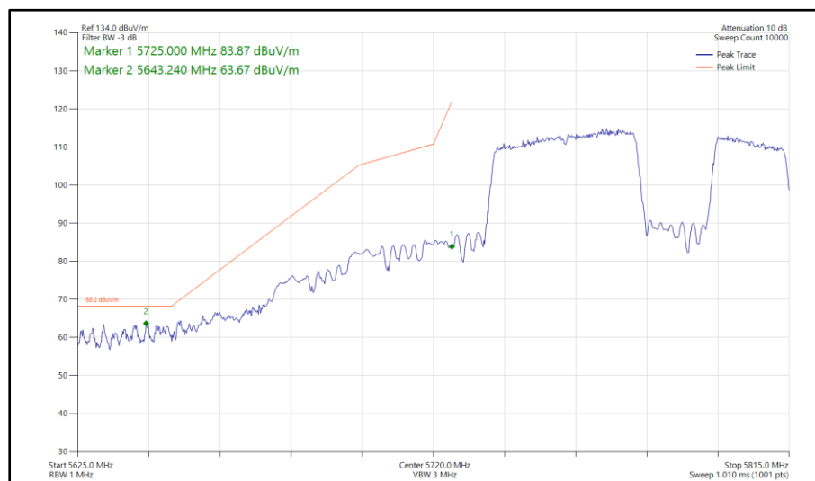
Figure 1064 - 802.11be EHT80, RU 484+242-92, SISO, Core 1 - 5775 MHz Band Edge Frequency 5725 MHz
