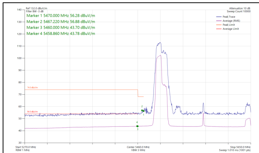
Figure 1138 - 802.11ax HE160, RU 106-53P, SISO, Core 0 - 5570 MHz Band Edge Frequency 5470 MHz
