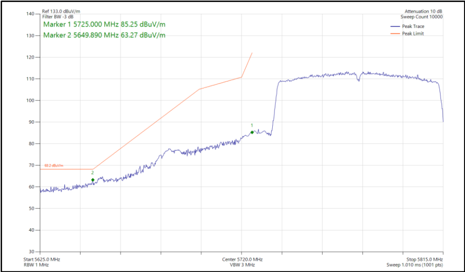
Figure 1061 - 802.11ac VHT80, SISO, Core 1 - 5775 MHz Band Edge Frequency 5725 MHz
