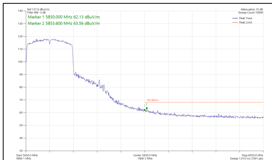
Figure 1117 - 802.11ac VHT80, SDM, Core 0-1 - 5690 MHz Band Edge Frequency 5850 MHz
