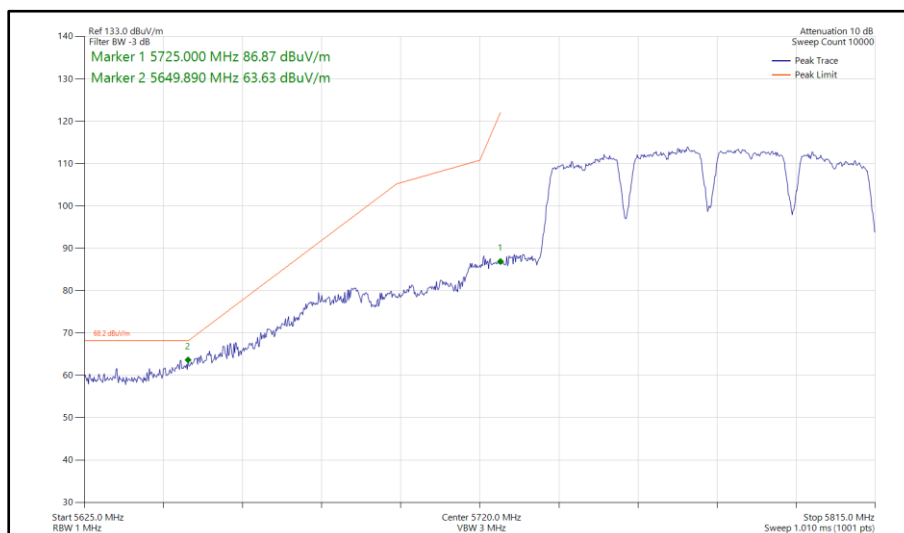
Figure 1060 - 802.11a a80, SISO, Core 1 - 5775 MHz Band Edge Frequency 5725 MHz
