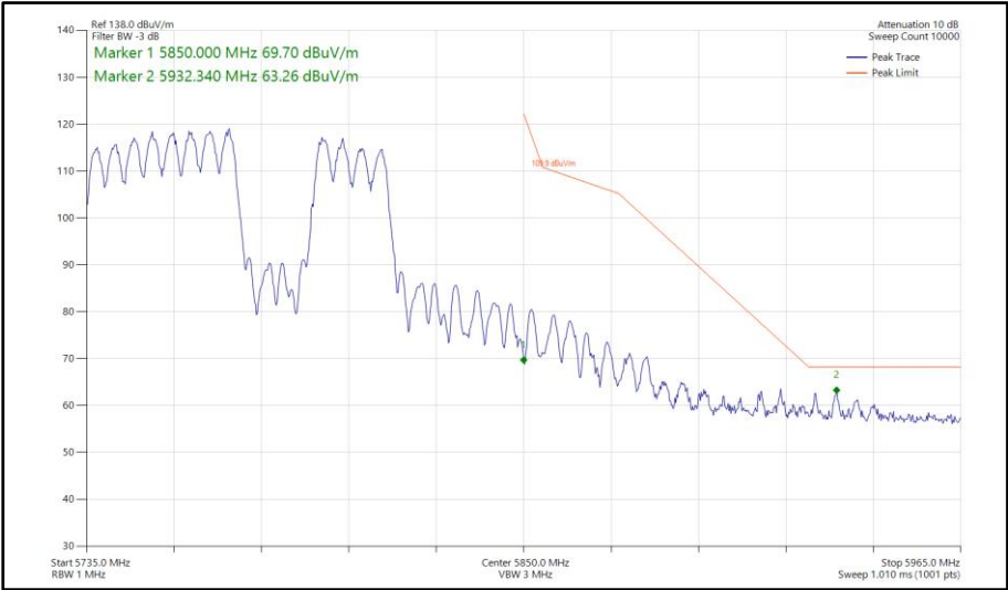
Figure 1104 - 802.11be EHT80, RU 484+242-92, CDD, Core 0-1 - 5775 MHz Band Edge Frequency 5850 MHz
