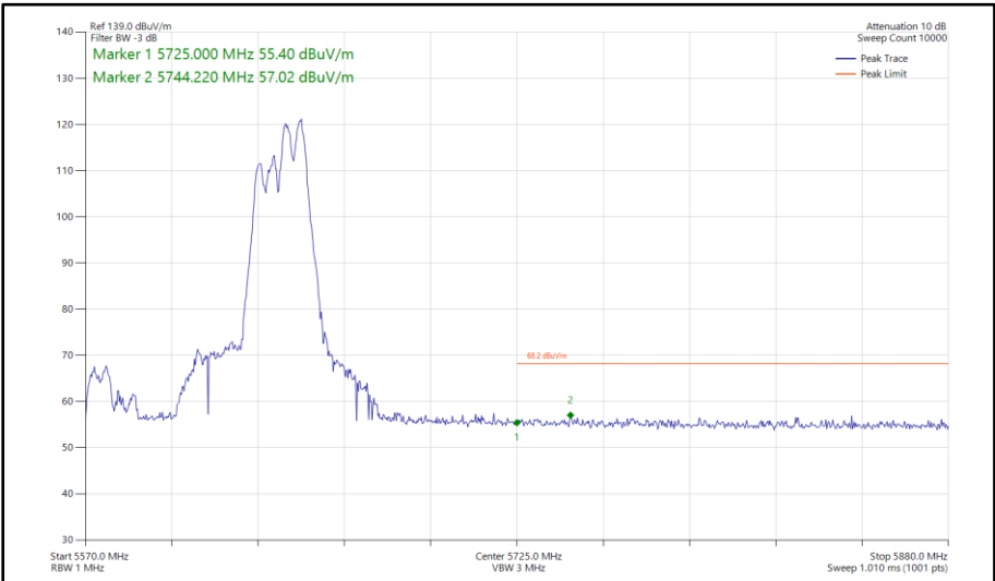
Figure 1115 - 802.11ax HE80, RU 106-60, SDM, Core 0-1 - 5610 MHz Band Edge Frequency 5725 MHz
