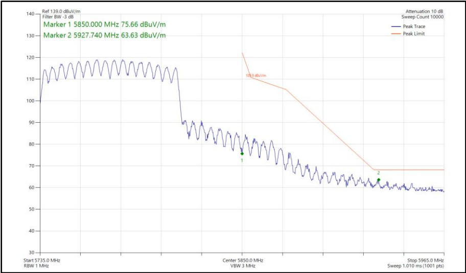
Figure 1098 - 802.11ac VHT80, CDD, Core 0-1 - 5775 MHz Band Edge Frequency 5850 MHz
