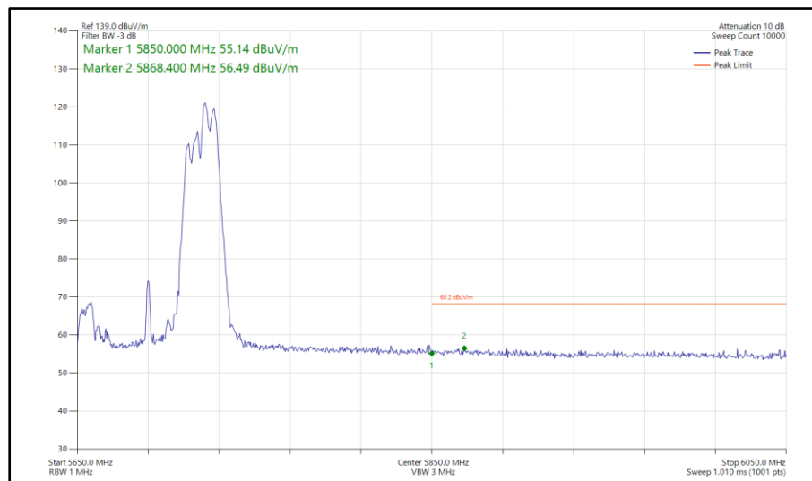
Figure 1100 - 802.11ax HE80, RU 106-60, CDD, Core 0-1 - 5690 MHz Band Edge Frequency 5850 MHz
