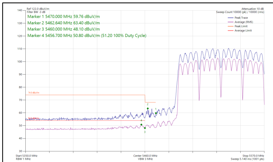
Figure 1080 - 802.11a a80, CDD, Core 0-1 - 5530 MHz Band Edge Frequency 5470 MHz
