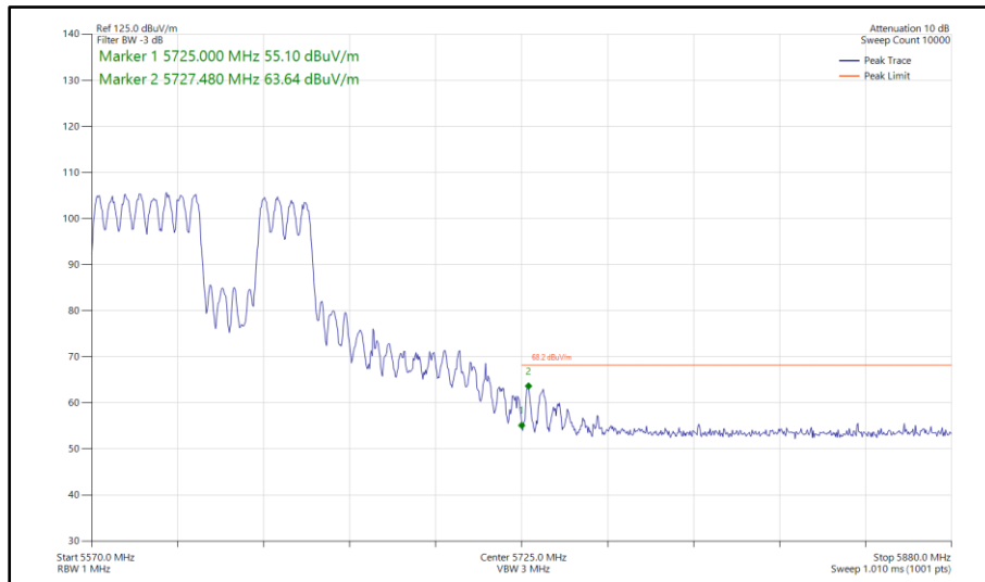
Figure 1094 - 802.11be EHT80, RU 484+242-92, CDD, Core 0-1 - 5610 MHz Band Edge Frequency 5725 MHz
