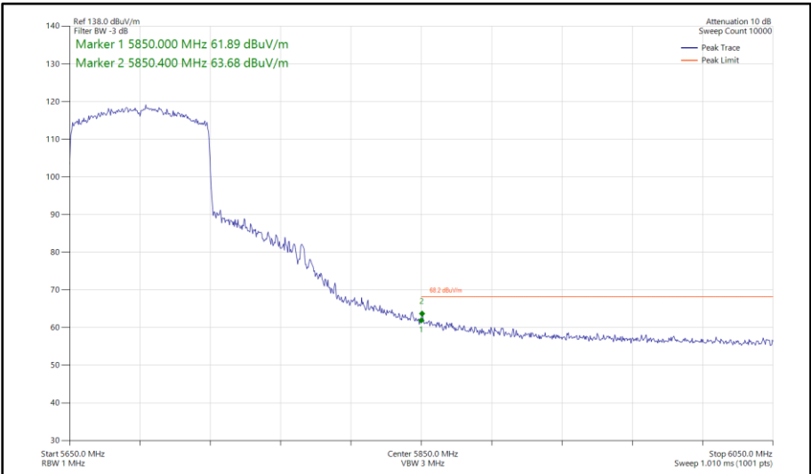
Figure 1119 - 802.11ax HE80, SU, SDM, Core 0-1 - 5690 MHz Band Edge Frequency 5850 MHz
