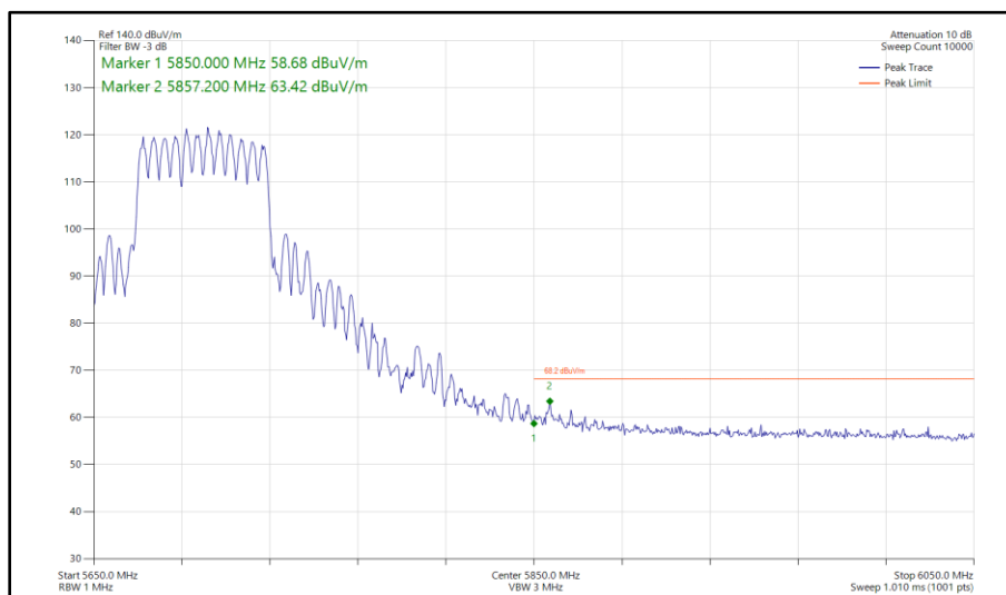
Figure 1123 - 802.11be EHT80, RU 484+242-90, SDM, Core 0-1 - 5690 MHz Band Edge Frequency 5850 MHz
