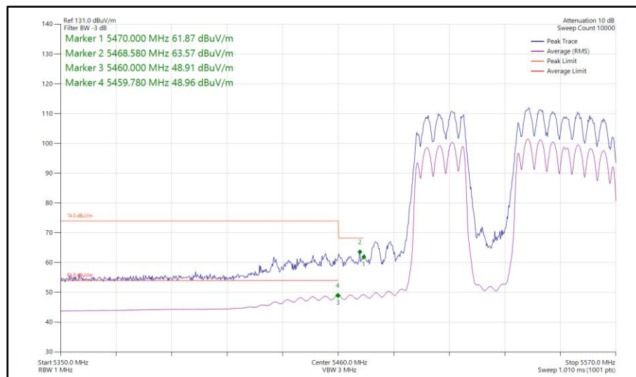
Figure 1084 - 802.11be EHT80, 484+242-91, CDD, Core 0-1 - 5530 MHz Band Edge Frequency 5470 MHz
