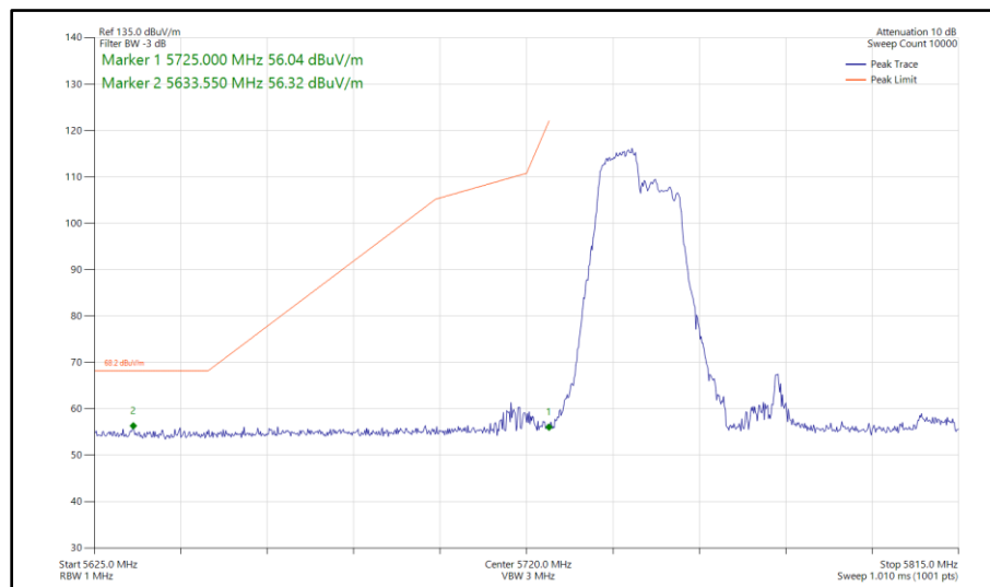
Figure 1063 - 802.11ax HE80, RU 106-53, SISO, Core 1 - 5775 MHz Band Edge Frequency 5725 MHz
