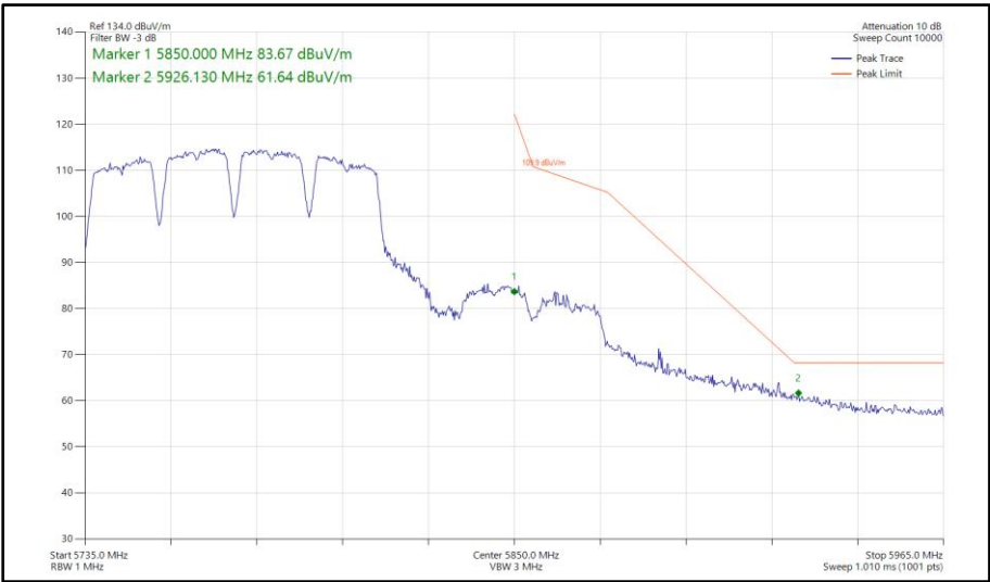
Figure 1071 - 802.11a a80, SISO, Core 1 - 5775 MHz Band Edge Frequency 5850 MHz
