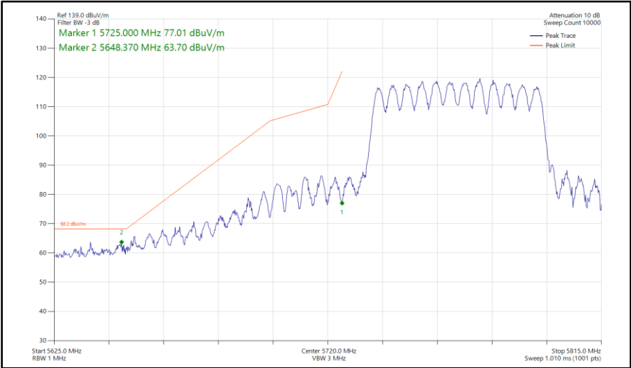
Figure 1089 - 802.11be EHT80, RU 484+242-93, CDD, Core 0-1 - 5775 MHz Band Edge Frequency 5725 MHz
