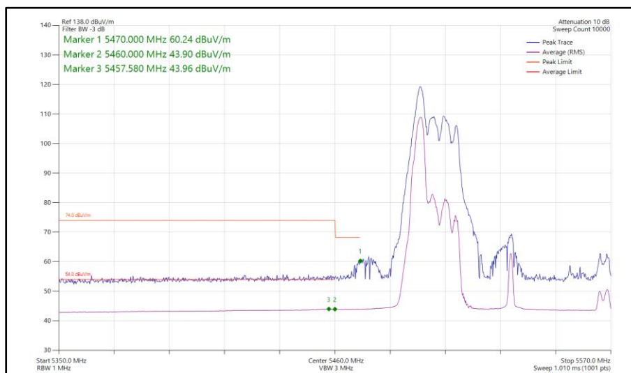
Figure 1107 - 802.11ax HE80, RU 52-37, SDM, Core 0-1 - 5530 MHz Band Edge Frequency 5470 MHz
