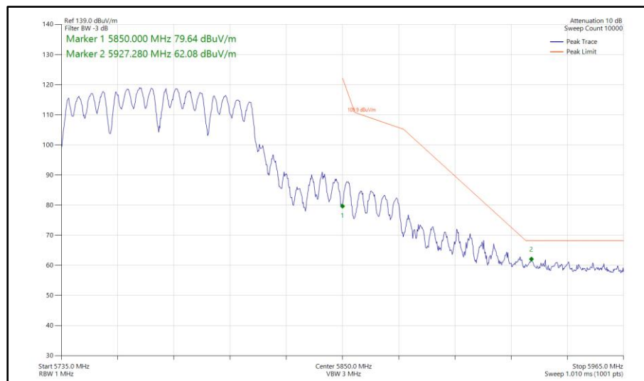
Figure 1096 - 802.11a a80, CDD, Core 0-1 - 5775 MHz Band Edge Frequency 5850 MHz
