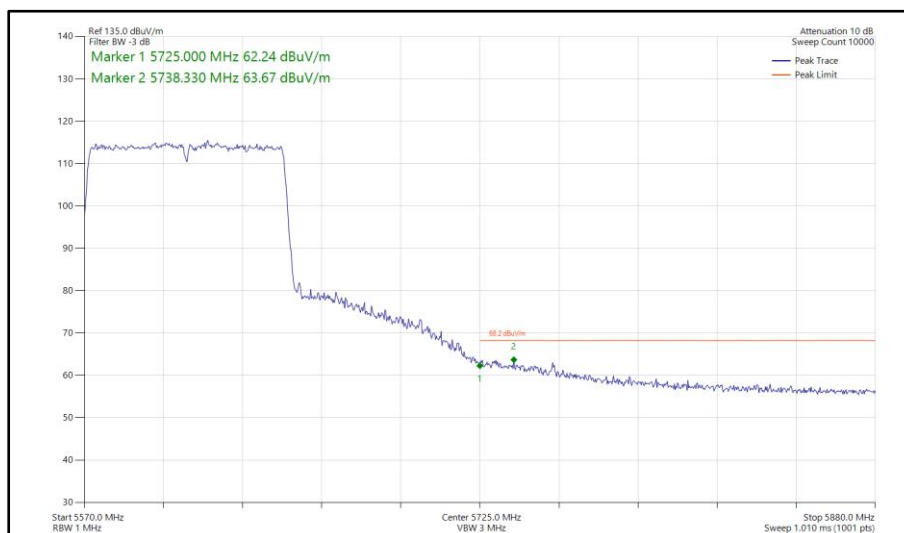
Figure 1113 - 802.11ac VHT80, SDM, Core 0-1 - 5610 MHz Band Edge Frequency 5725 MHz
