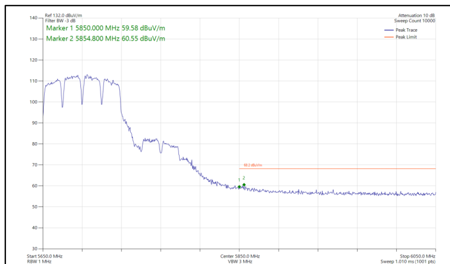
Figure 1070 - 802.11a a80, SISO, Core 1 - 5690 MHz Band Edge Frequency 5850 MHz
