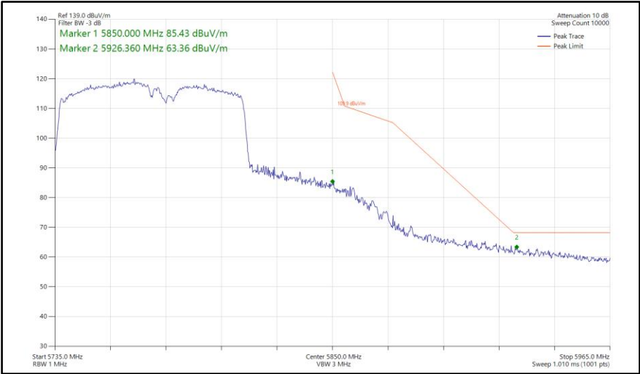
Figure 1132 - 802.11ac VHT80, TxBF, Core 0-1 - 5775 MHz Band Edge Frequency 5850 MHz
