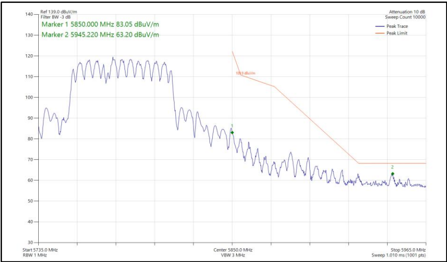
Figure 1124 - 802.11be EHT80, RU 484+242-90, SDM, Core 0-1 - 5775 MHz Band Edge Frequency 5850 MHz
