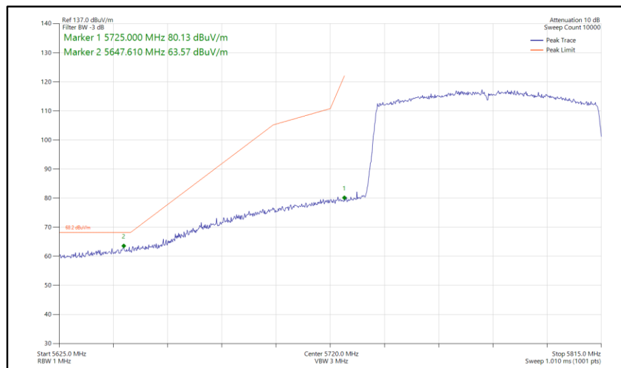
Figure 1128 - 802.11ax HE80, SU, TxBF, Core 0-1 - 5775 MHz Band Edge Frequency 5725 MHz
