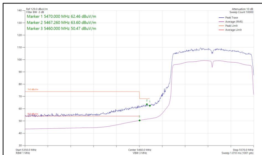
Figure 1056 - 802.11ac VHT80, SISO, Core 1 - 5530 MHz Band Edge Frequency 5470 MHz
