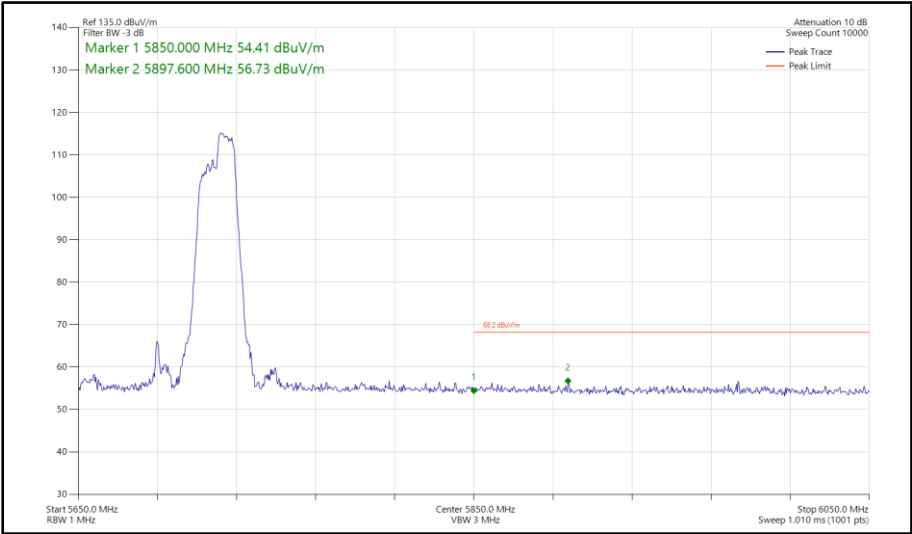
Figure 1075 - 802.11ax HE80, RU 106-60, SISO, Core 1 - 5690 MHz Band Edge Frequency 5850 MHz
