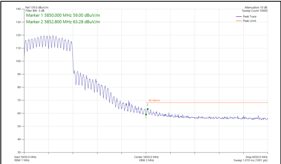
Figure 1099 - 802.11ax HE80, SU, CDD, Core 0-1 - 5690 MHz Band Edge Frequency 5850 MHz
