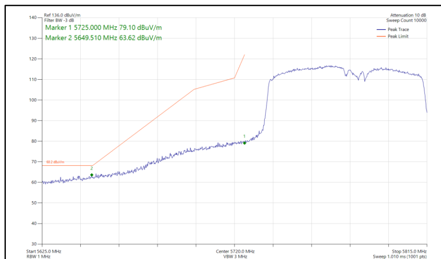
Figure 1127 - 802.11ac VHT80, TxBF, Core 0-1 - 5775 MHz Band Edge Frequency 5725 MHz
