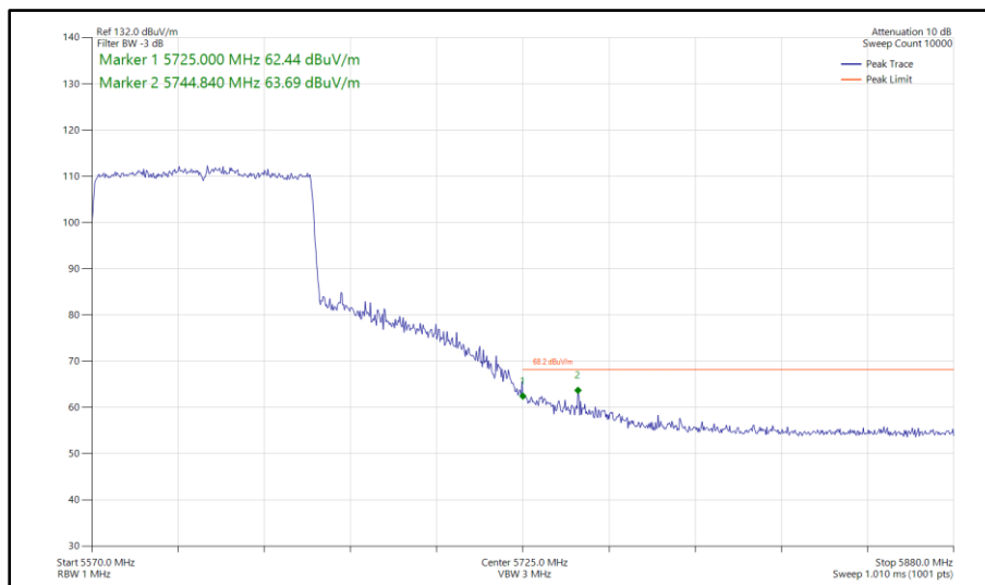
Figure 1067 - 802.11ax HE80, SU, SISO, Core 1 - 5610 MHz Band Edge Frequency 5725 MHz
