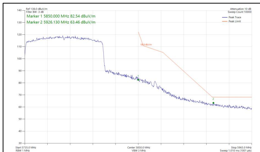
Figure 1121 - 802.11ax HE80, SU, SDM, Core 0-1 - 5775 MHz Band Edge Frequency 5850 MHz
