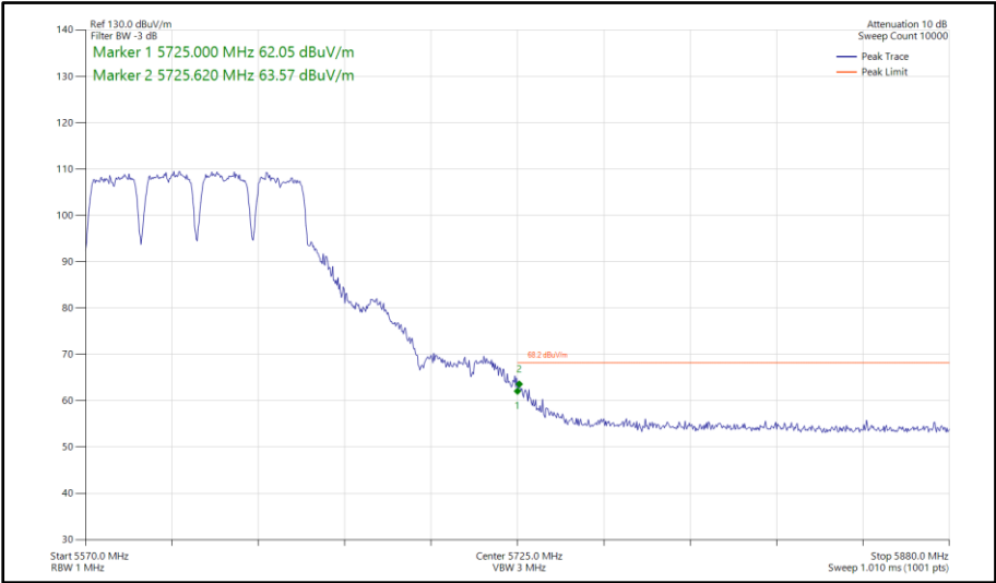
Figure 1065 - 802.11a a80, SISO, Core 1 - 5610 MHz Band Edge Frequency 5725 MHz
