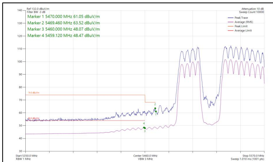
Figure 1108 - 802.11be EHT80, RU 484+242-91, SDM, Core 0-1 - 5530 MHz Band Edge Frequency 5470 MHz
