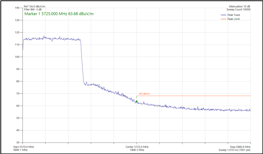
Figure 1114 - 802.11ax HE80, SU, SDM, Core 0-1 - 5610 MHz Band Edge Frequency 5725 MHz
