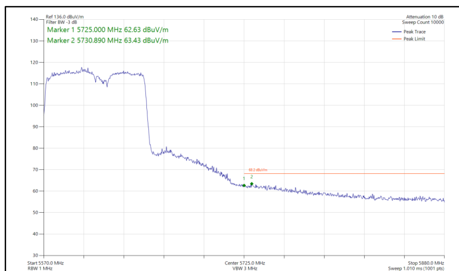
Figure 1129 - 802.11ac VHT80, TxBF, Core 0-1 - 5610 MHz Band Edge Frequency 5725 MHz
