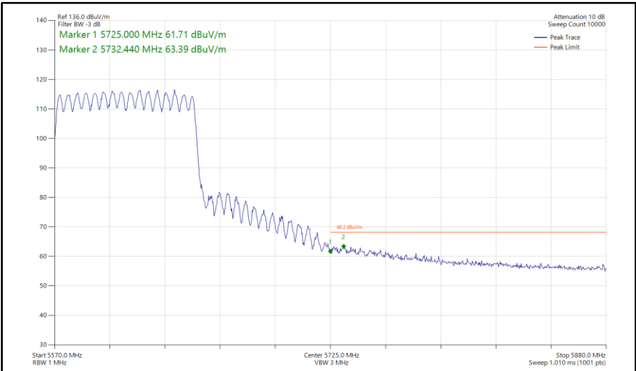
Figure 1091 - 802.11ac VHT80, CDD, Core 0-1 - 5610 MHz Band Edge Frequency 5725 MHz
