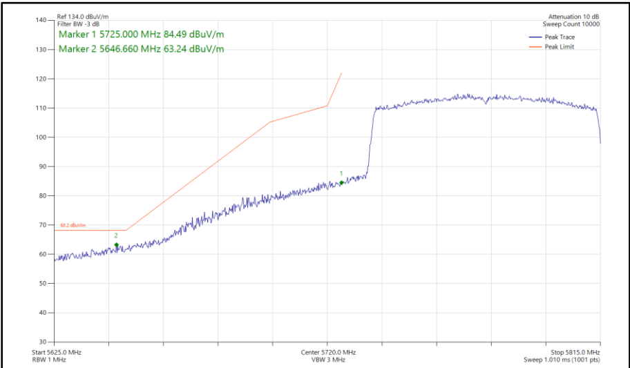
Figure 1062 - 802.11ax HE80, SU, SISO, Core 1 - 5775 MHz Band Edge Frequency 5725 MHz
