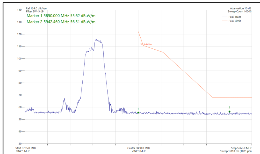
Figure 1077 - 802.11ax HE80, RU 106-60, SISO, Core 1 - 5775 MHz Band Edge Frequency 5850 MHz
