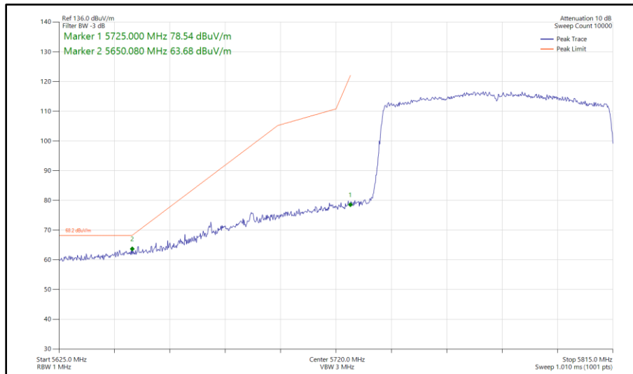
Figure 1110 - 802.11ax HE80, SU, SDM, Core 0-1 - 5775 MHz Band Edge Frequency 5725 MHz
