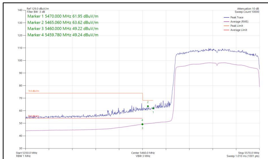
Figure 1057 - 802.11ax HE80, SU, SISO, Core 1 - 5530 MHz Band Edge Frequency 5470 MHz
