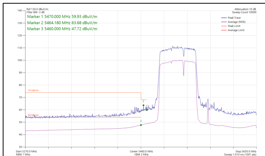
Figure 1139 - 802.11be EHT160, RU 484+242-93, SISO, Core 0 - 5570 MHz Band Edge Frequency 5470 MHz
