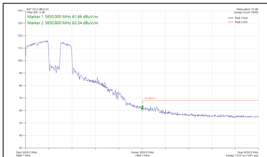
Figure 1078 - 802.11be EHT80, RU 484+242-92, SISO, Core 1 - 5690 MHz Band Edge Frequency 5850 MHz
