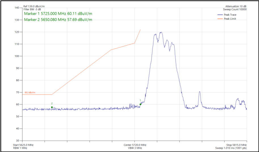
Figure 1088 - 802.11ax HE80, RU 106-53, CDD, Core 0-1 - 5775 MHz Band Edge Frequency 5725 MHz
