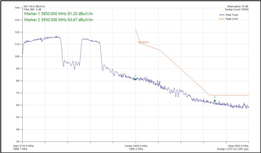
Figure 1079 - 802.11be EHT80, RU 484+242-92, SISO, Core 1 - 5775 MHz Band Edge Frequency 5850 MHz
