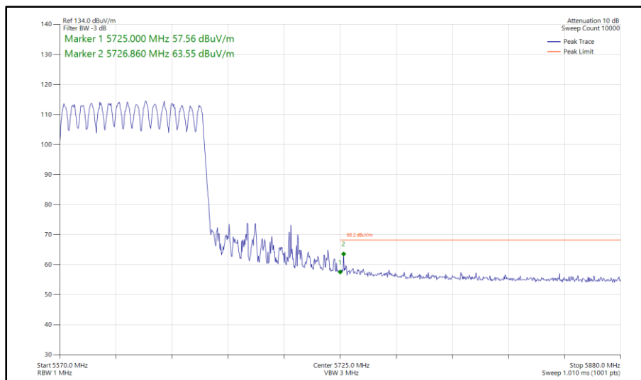
Figure 1092 - 802.11ax HE80, SU, CDD, Core 0-1 - 5610 MHz Band Edge Frequency 5725 MHz
