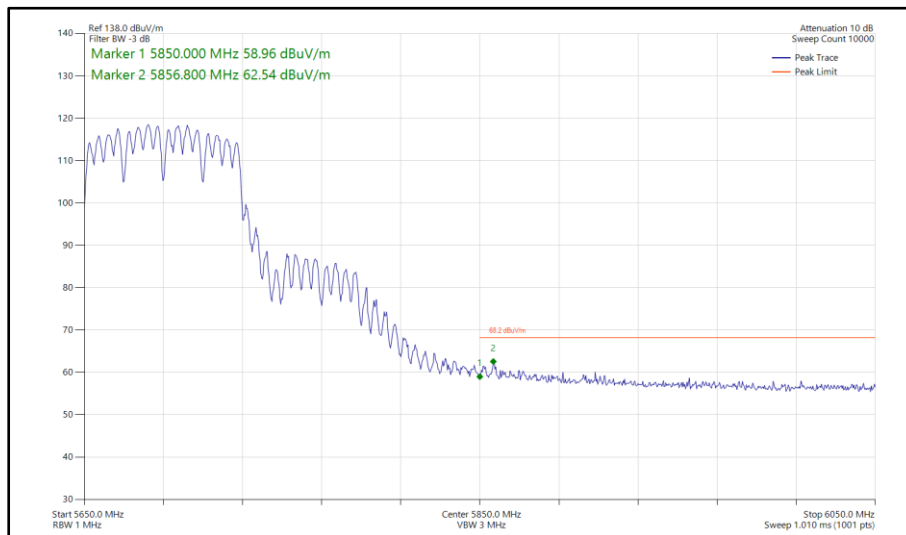
Figure 1095 - 802.11a a80, CDD, Core 0-1 - 5690 MHz Band Edge Frequency 5850 MHz
