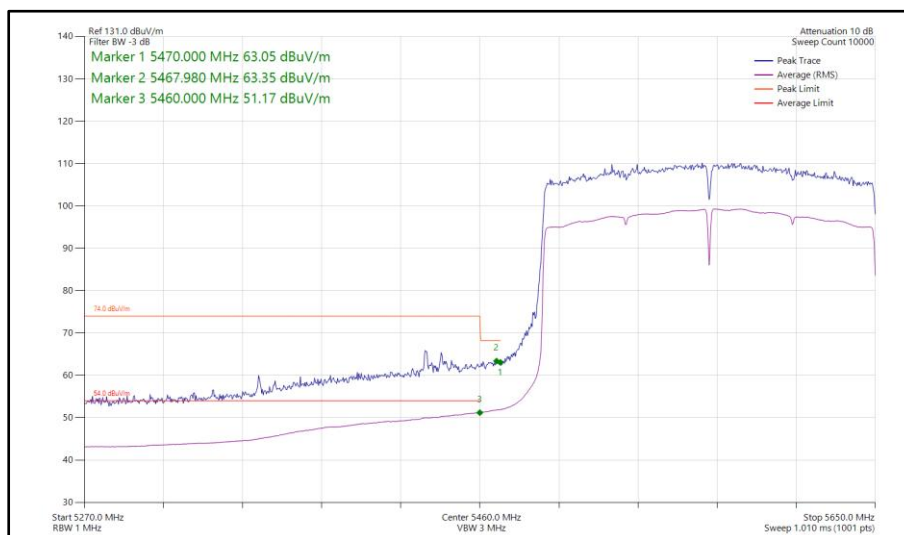
Figure 1137 - 802.11ax HE160, SU, SISO, Core 0 - 5570 MHz Band Edge Frequency 5470 MHz
