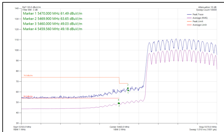
Figure 1082 - 802.11ax HE80, SU, CDD, Core 0-1 - 5530 MHz Band Edge Frequency 5470 MHz
