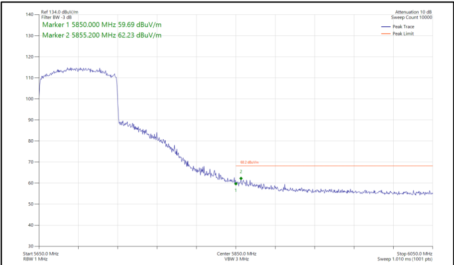
Figure 1074 - 802.11ax HE80, SU, SISO, Core 1 - 5690 MHz Band Edge Frequency 5850 MHz
