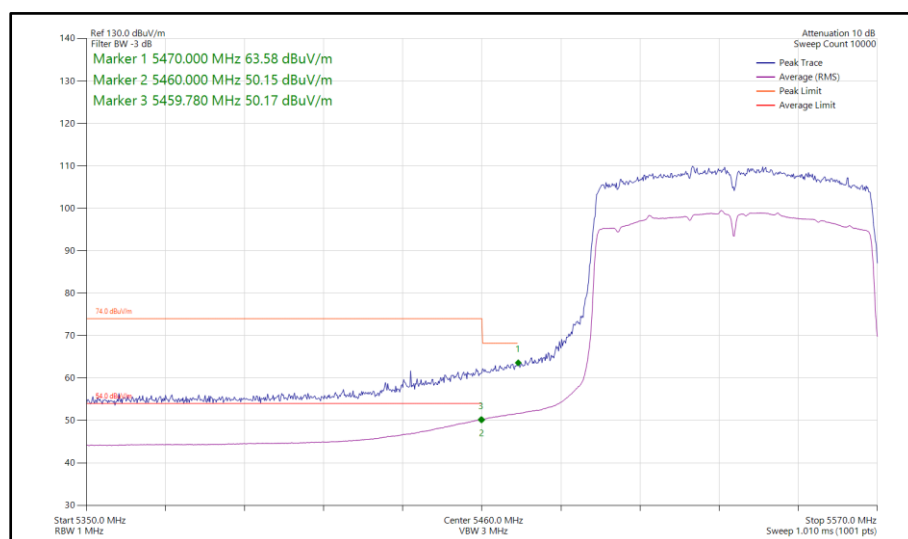
Figure 1105 - 802.11ac VHT80, SDM, Core 0-1 - 5530 MHz Band Edge Frequency 5470 MHz
