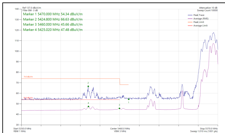
Figure 1083 - 802.11ax HE80, RU 106-60, CDD, Core 0-1 - 5530 MHz Band Edge Frequency 5470 MHz
