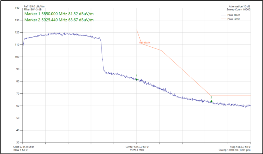
Figure 1134 - 802.11ax HE80, SU, TxBF, Core 0-1 - 5775 MHz Band Edge Frequency 5850 MHz
