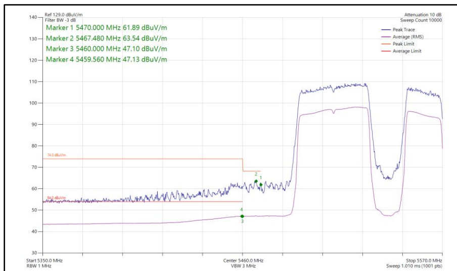
Figure 1059 - 802.11be EHT80, RU 484+242-92, SISO, Core 1 - 5530 MHz Band Edge Frequency 5470 MHz
