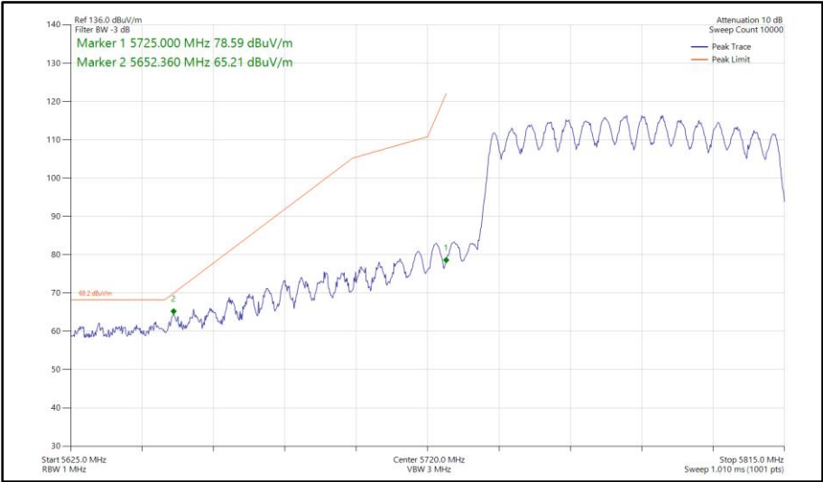
Figure 1086 - 802.11ac VHT80, CDD, Core 0-1 - 5775 MHz Band Edge Frequency 5725 MHz
