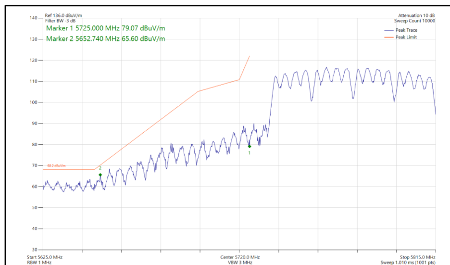
Figure 1085 - 802.11a a80, CDD, Core 0-1 - 5775 MHz Band Edge Frequency 5725 MHz
