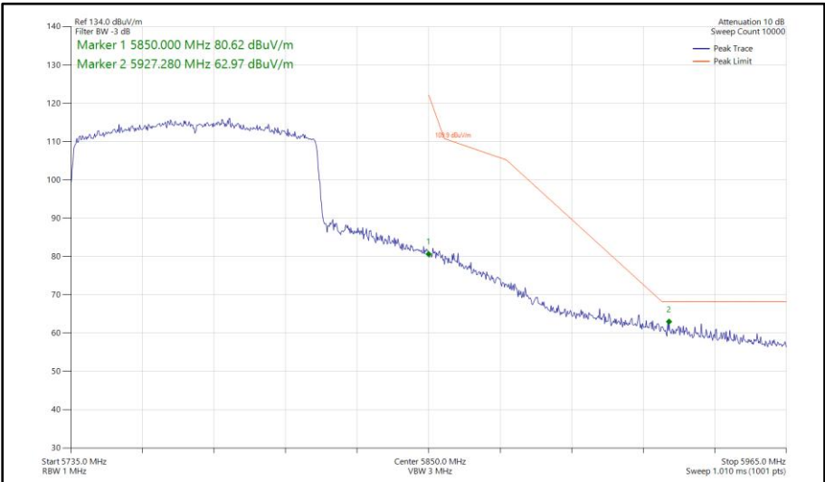
Figure 1076 - 802.11ax HE80, SU, SISO, Core 1 - 5775 MHz Band Edge Frequency 5850 MHz
