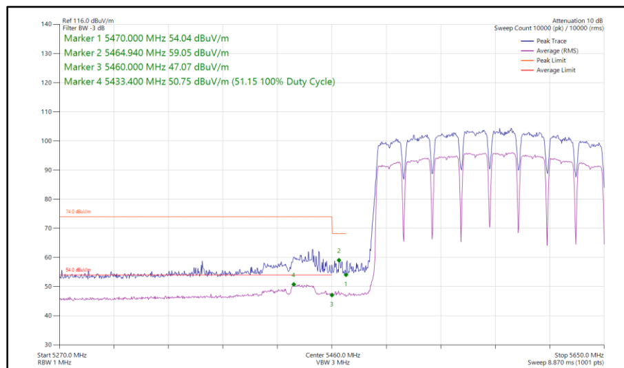
Figure 1135 - 802.11a a160, SISO, Core 0 - 5570 MHz Band Edge Frequency 5470 MHz
