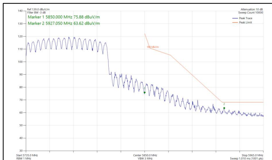
Figure 1101 - 802.11ax HE80, SU, CDD, Core 0-1 - 5775 MHz Band Edge Frequency 5850 MHz
