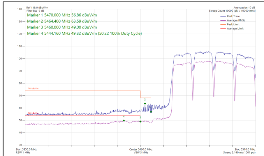
Figure 1055 - 802.11a a80, SISO, Core 1 - 5530 MHz Band Edge Frequency 5470 MHz
