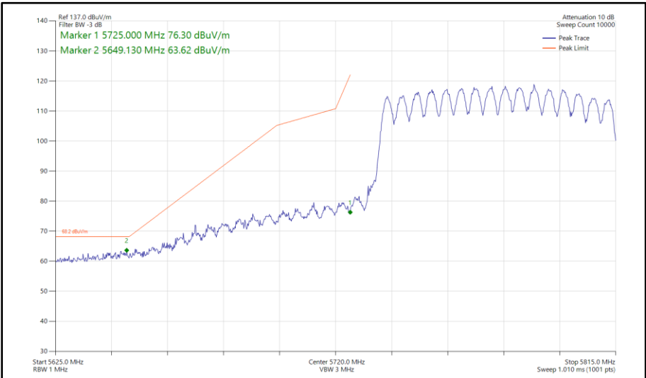
Figure 1087 - 802.11ax HE80, SU, CDD, Core 0-1 - 5775 MHz Band Edge Frequency 5725 MHz
