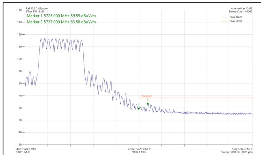
Figure 1116 - 802.11be EHT80, RU 484+242-90, SDM, Core 0-1 - 5610 MHz Band Edge Frequency 5725 MHz
