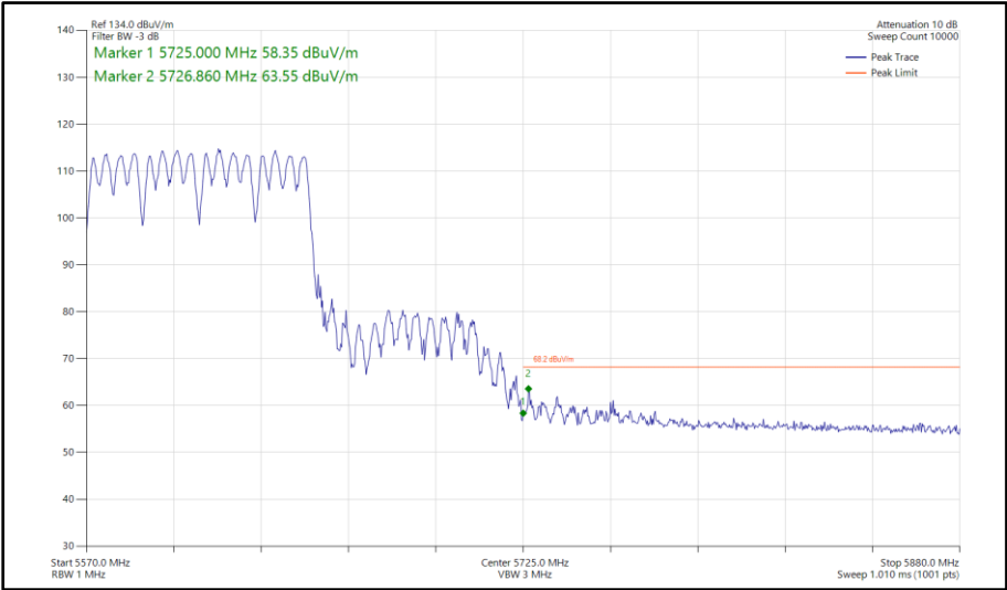
Figure 1090 - 802.11a a80, CDD, Core 0-1 - 5610 MHz Band Edge Frequency 5725 MHz
