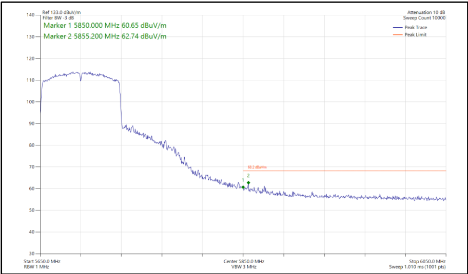
Figure 1072 - 802.11ac VHT80, SISO, Core 1 - 5690 MHz Band Edge Frequency 5850 MHz
