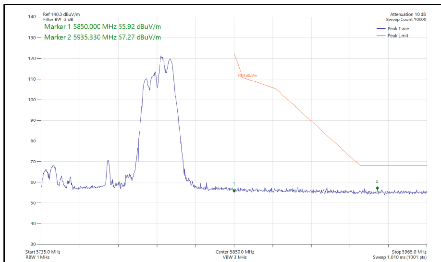
Figure 1102 - 802.11ax HE80, RU 106-60, CDD, Core 0-1 - 5775 MHz Band Edge Frequency 5850 MHz
