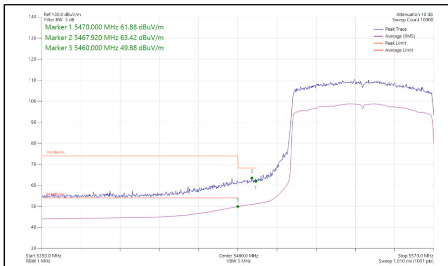
Figure 1106 - 802.11ax HE80, SU, SDM, Core 0-1 - 5530 MHz Band Edge Frequency 5470 MHz
