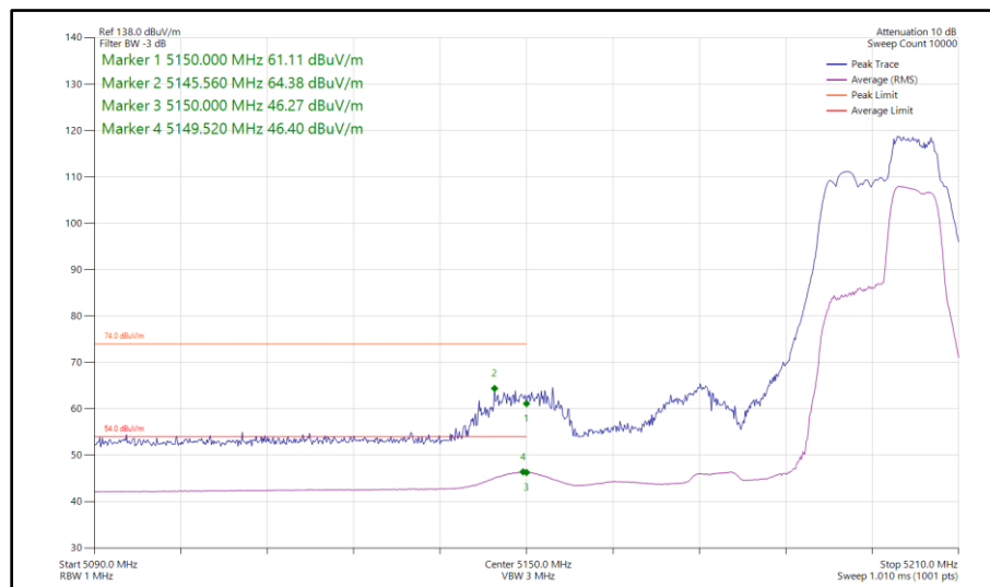
Figure 144 - 802.11be EHT40 RU 52+26-75, SISO, Core 0 - 5190 MHz Band Edge Frequency 5150 MHz
