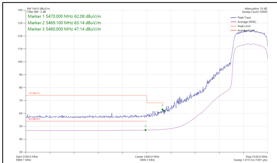
Figure 134 - 802.11ax HE20, SU, TxBF, Core 0-1 - 5520 MHz Band Edge Frequency 5460 MHz
