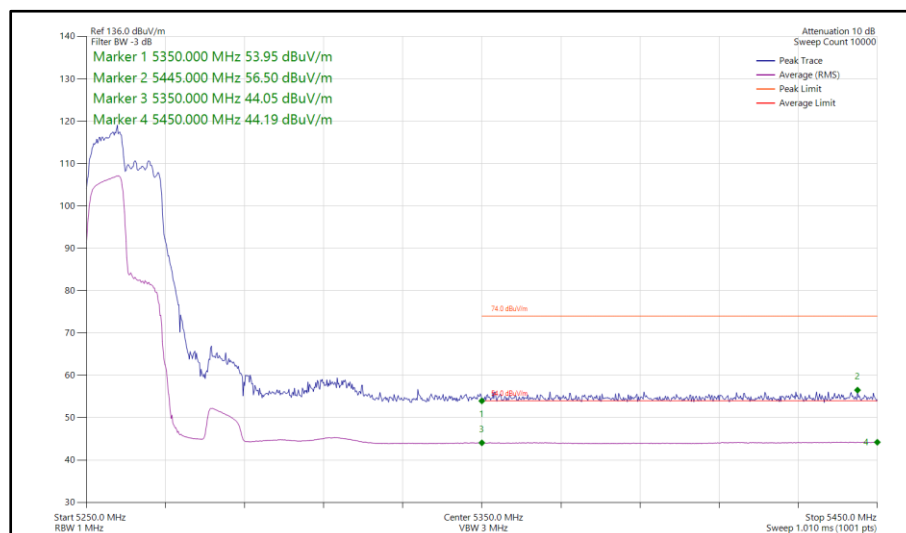
Figure 186 - 802.11ax HE40, RU 106-53, SISO, Core 1 - 5270 MHz Band Edge Frequency 5350 MHz
