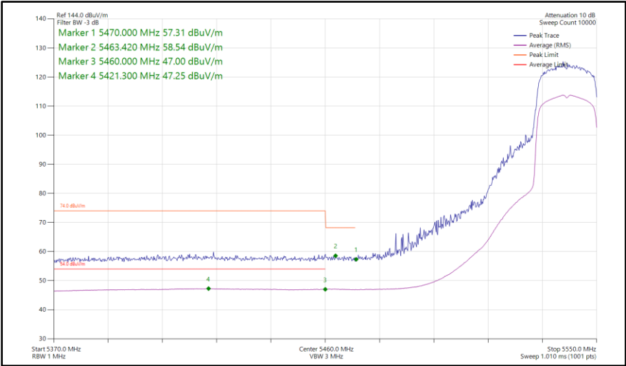
Figure 135 - 802.11ax HE20, SU, TxBF, Core 0-1 - 5540 MHz Band Edge Frequency 5460 MHz
