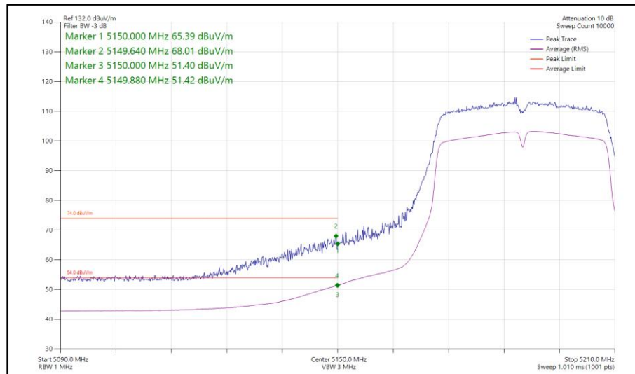
Figure 138 - 802.11n HT40, SISO, Core 0 - 5190 MHz Band Edge Frequency 5150 MHz
