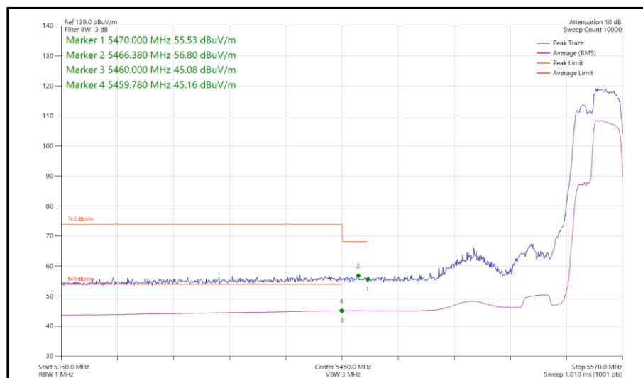
Figure 169 - 802.11be EHT40 RU 106+26-85, SISO, Core 0 - 5550 MHz Band Edge Frequency 5460 MHz
