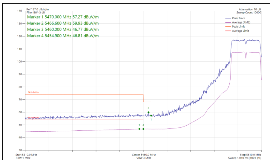
Figure 161 - 802.11n HT40, SISO, Core 0 - 5590 MHz Band Edge Frequency 5460 MHz
