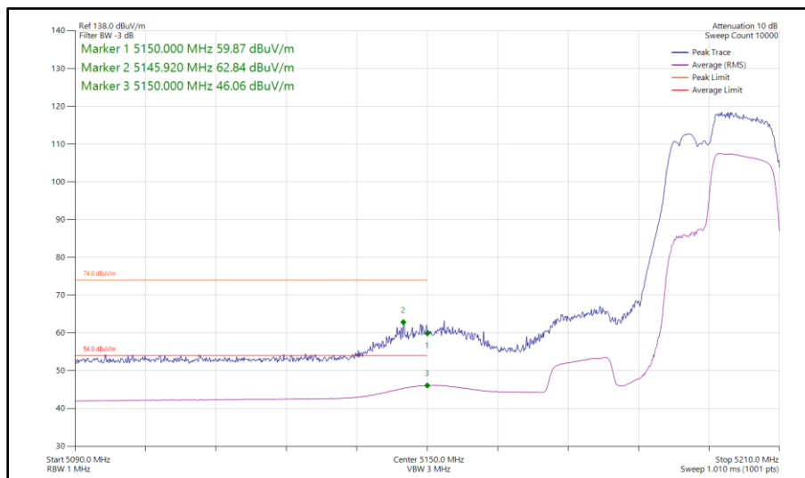
Figure 179 - 802.11be EHT40 RU 106+26-85, SISO, Core 1 - 5190 MHz Band Edge Frequency 5150 MHz
