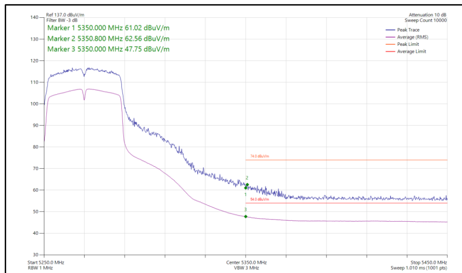
Figure 183 - 802.11n HT40, SISO, Core 1 - 5270 MHz Band Edge Frequency 5350 MHz
