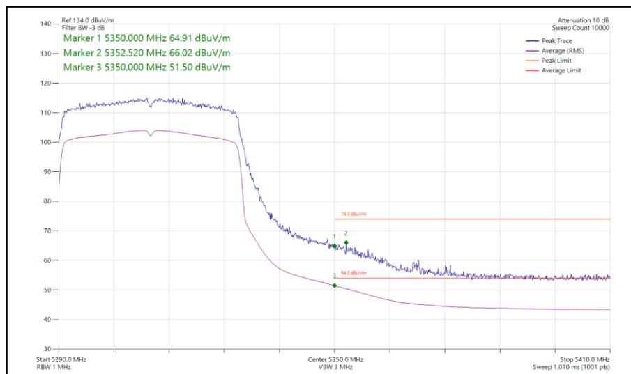
Figure 187 - 802.11ax HE40, SU, SISO, Core 1 - 5310 MHz Band Edge Frequency 5350 MHz
