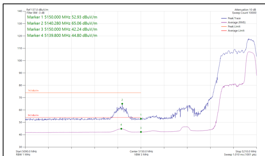
Figure 141 - 802.11ax HE40, RU 52-44, SISO, Core 0 - 5190 MHz Band Edge Frequency 5150 MHz
