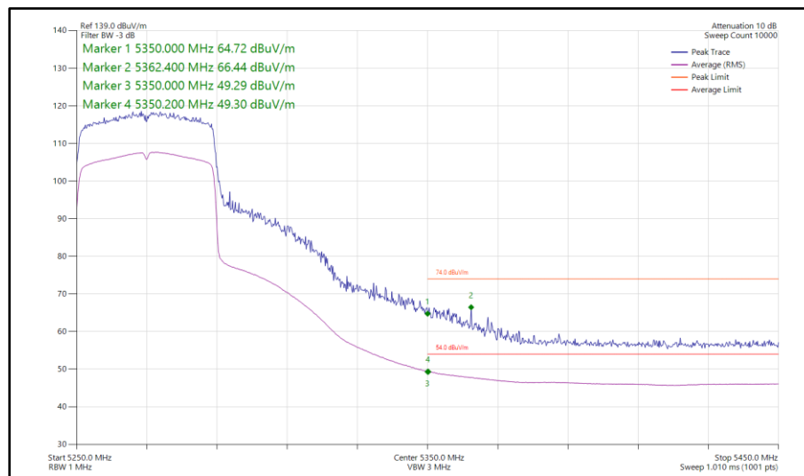
Figure 150 - 802.11ax HE40, SU, SISO, Core 0 - 5270 MHz Band Edge Frequency 5350 MHz
