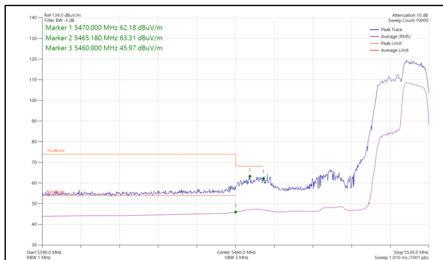
Figure 163 - 802.11ax HE40, RU 106-56, SISO, Core 0 - 5510 MHz Band Edge Frequency 5460 MHz
