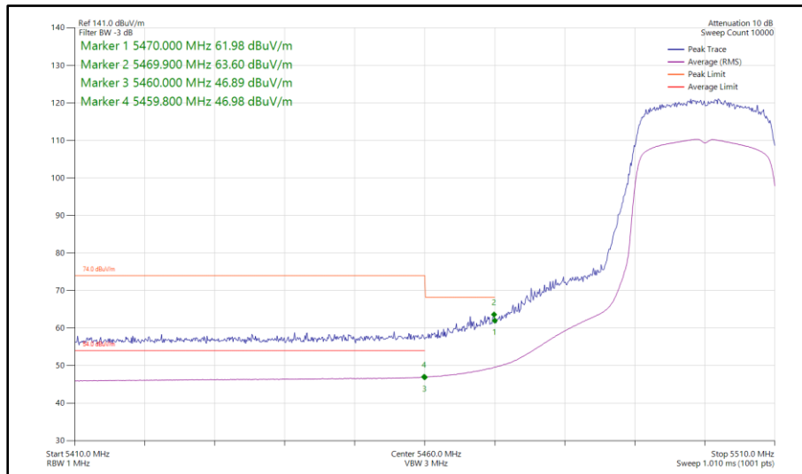
Figure 133 - 802.11ax HE20, SU, TxBF, Core 0-1 - 5500 MHz Band Edge Frequency 5460 MHz
