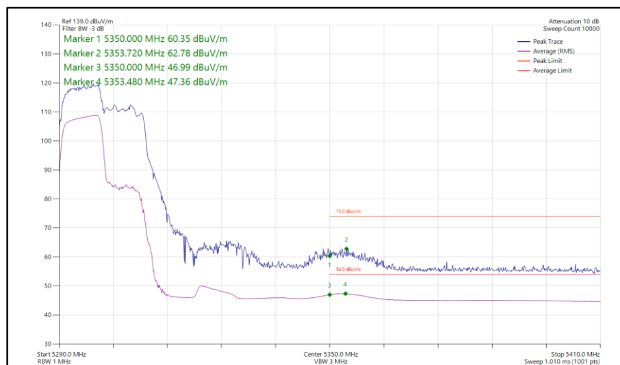
Figure 153 - 802.11ax HE40, RU 106-53, SISO, Core 0 - 5310 MHz Band Edge Frequency 5350 MHz
