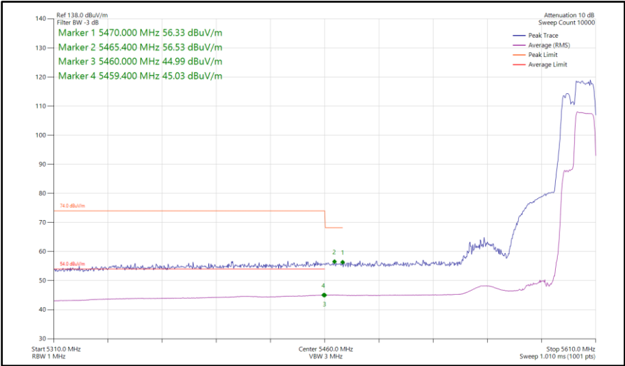
Figure 170 - 802.11be EHT40 RU 106+26-85, SISO, Core 0 - 5590 MHz Band Edge Frequency 5460 MHz
