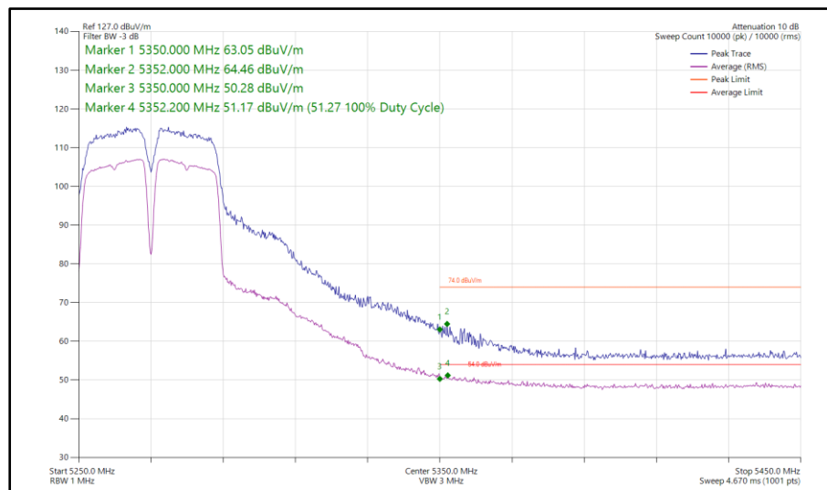
Figure 146 - 802.11a a40, SISO, Core 0 - 5270 MHz Band Edge Frequency 5350 MHz
