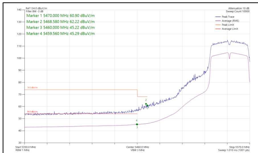
Figure 195 - 802.11n HT40, SISO, Core 1 - 5550 MHz Band Edge Frequency 5460 MHz
