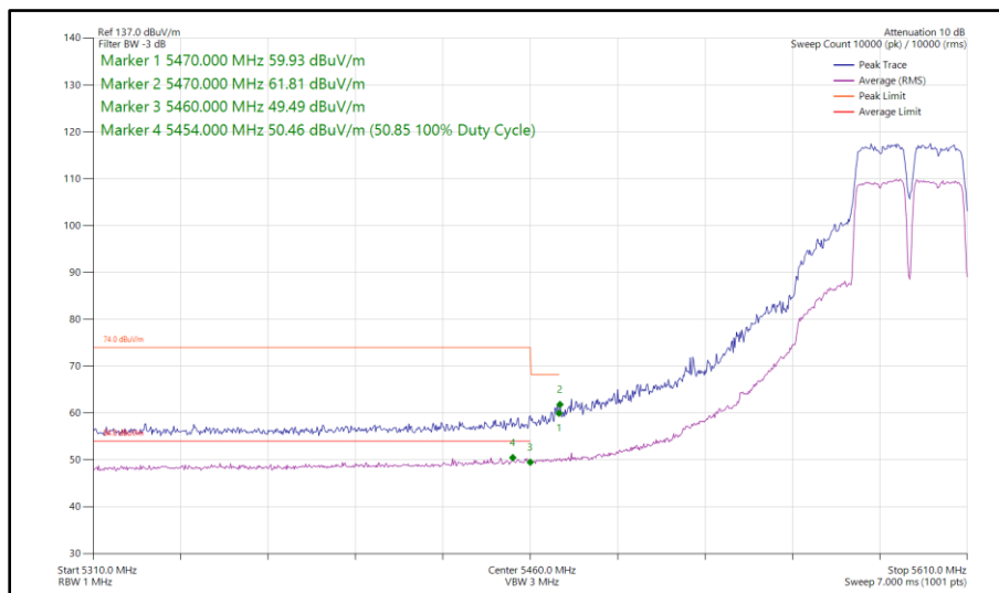
Figure 158 - 802.11a a40, SISO, Core 0 - 5590 MHz Band Edge Frequency 5460 MHz
