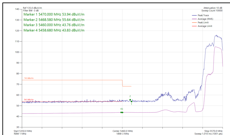
Figure 200 - 802.11ax HE40, RU 106-56, SISO, Core 1 - 5550 MHz Band Edge Frequency 5460 MHz
