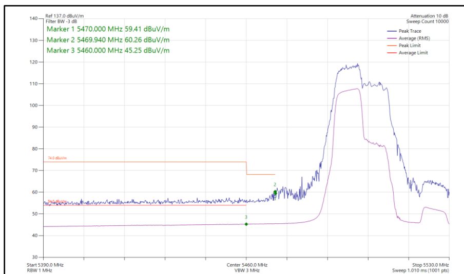
Figure 198 - 802.11ax HE40, RU 106-53, SISO, Core 1 - 5510 MHz Band Edge Frequency 5460 MHz
