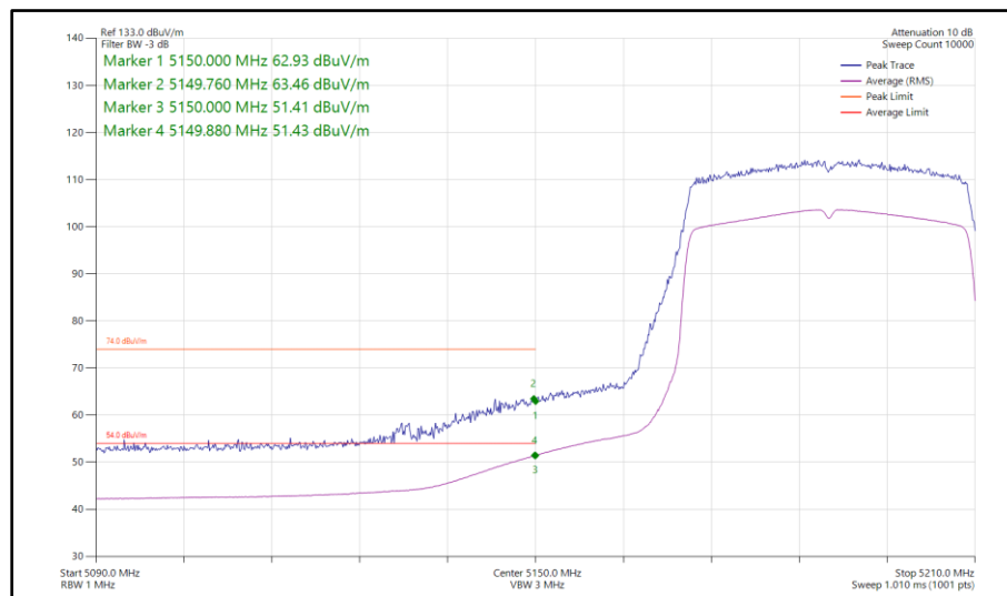
Figure 175 - 802.11ax HE40, SU, SISO, Core 1 - 5190 MHz Band Edge Frequency 5150 MHz
