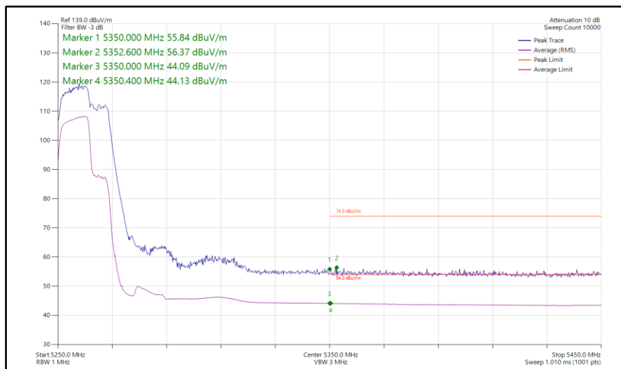
Figure 189 - 802.11be EHT40 RU 106+26-82, SISO, Core 1 - 5270 MHz Band Edge Frequency 5350 MHz
