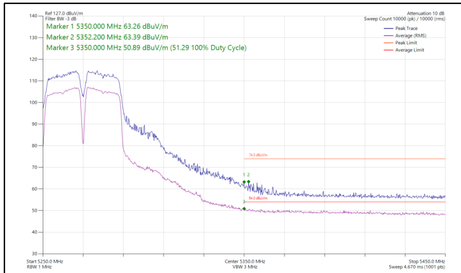
Figure 181 - 802.11a a40, SISO, Core 1 - 5270 MHz Band Edge Frequency 5350 MHz
