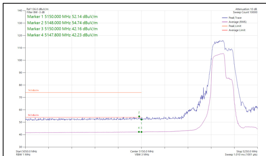
Figure 145 - 802.11be EHT40 RU 106+26-82, SISO, Core 0 - 5230 MHz Band Edge Frequency 5150 MHz
