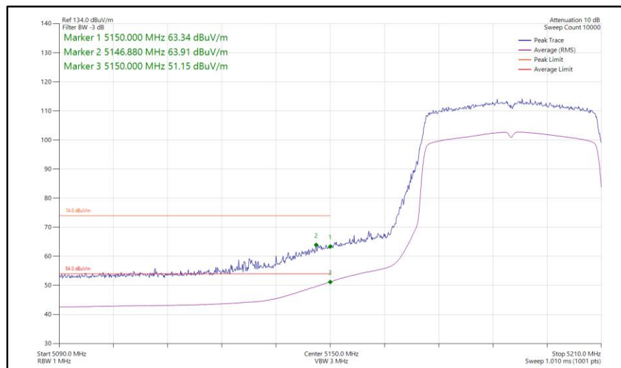
Figure 140 - 802.11ax HE40, SU, SISO, Core 0 - 5190 MHz Band Edge Frequency 5150 MHz
