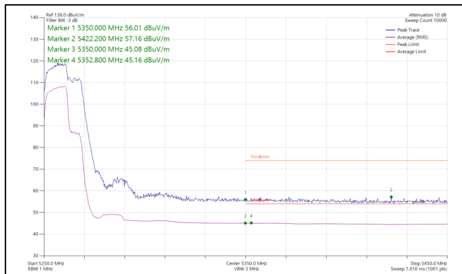
Figure 154 - 802.11be EHT40 RU 106+26-82, SISO, Core 0 - 5270 MHz Band Edge Frequency 5350 MHz
