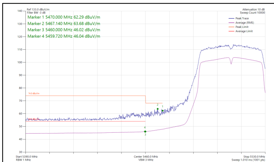
Figure 159 - 802.11n HT40, SISO, Core 0 - 5510 MHz Band Edge Frequency 5460 MHz
