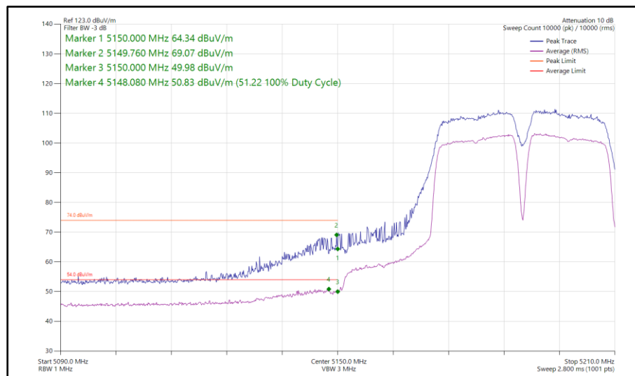
Figure 171 - 802.11a a40, SISO, Core 1 - 5190 MHz Band Edge Frequency 5150 MHz
