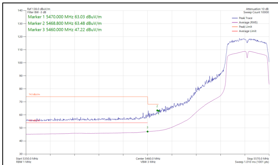
Figure 160 - 802.11n HT40, SISO, Core 0 - 5550 MHz Band Edge Frequency 5460 MHz
