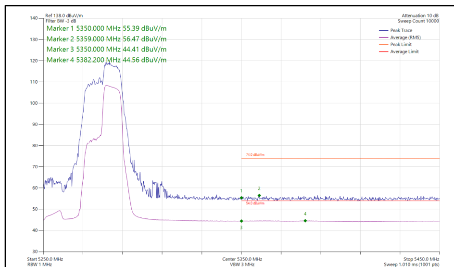
Figure 151 - 802.11ax HE40, RU 106-56, SISO, Core 0 - 5270 MHz Band Edge Frequency 5350 MHz
