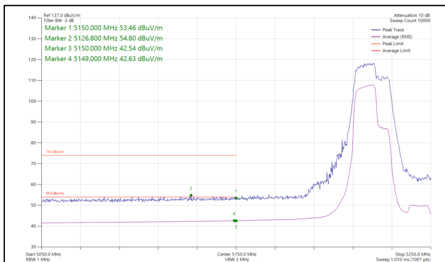
Figure 180 - 802.11be EHT40 RU 106+26-82, SISO, Core 1 - 5230 MHz Band Edge Frequency 5150 MHz
