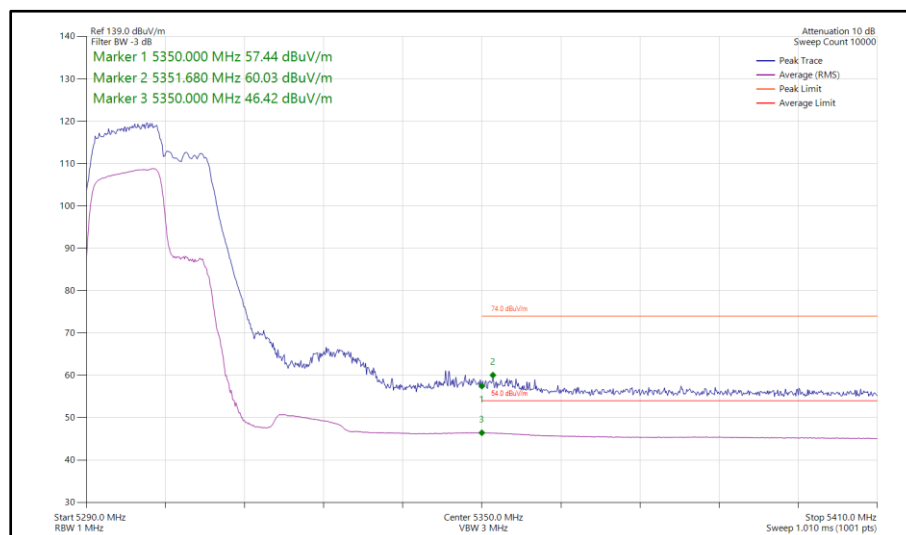
Figure 155 - 802.11be EHT40 RU 106+26-82, SISO, Core 0 - 5310 MHz Band Edge Frequency 5350 MHz
