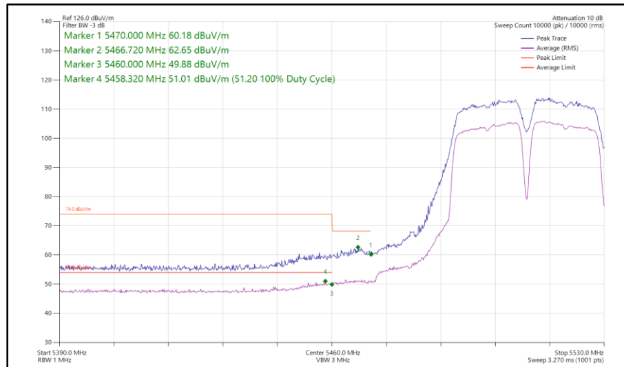
Figure 156 - 802.11a a40, SISO, Core 0 - 5510 MHz Band Edge Frequency 5460 MHz
