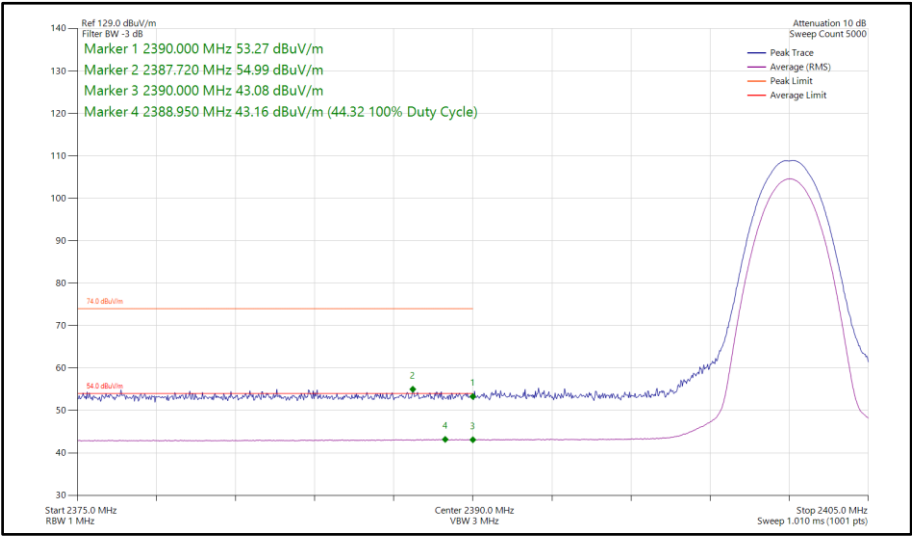
Figure 73 - Bluetooth 2DH5, MIMO, Core 0-1 - 2402 MHz Band Edge Frequency 2390 MHz
