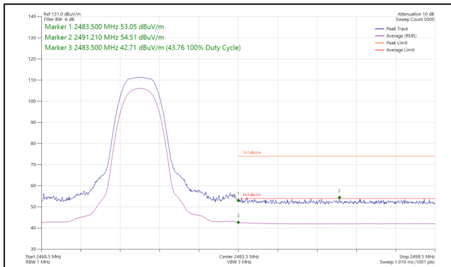
Figure 87 - Bluetooth HDR4, MIMO, Core 0-1 - 2476 MHz Band Edge Frequency 2483.5 MHz
