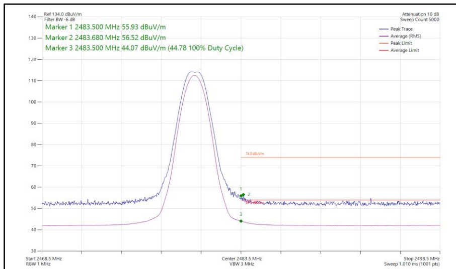
Figure 89 - Bluetooth LE1M, MIMO, Core 0-1 - 2480 MHz Band Edge Frequency 2483.5 MHz
