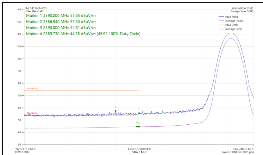
Figure 97 - Bluetooth 2DH5, SISO, Core 0 - 2402 MHz Band Edge Frequency 2390 MHz
