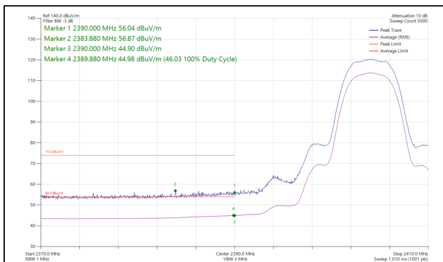
Figure 124 - Bluetooth HDR8, SISO, Core 1 - 2404 MHz Band Edge Frequency 2390 MHz
