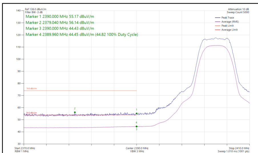
Figure 108 - Bluetooth XHDRPM8, SISO, Core 0 - 2404 MHz Band Edge Frequency 2390 MHz
