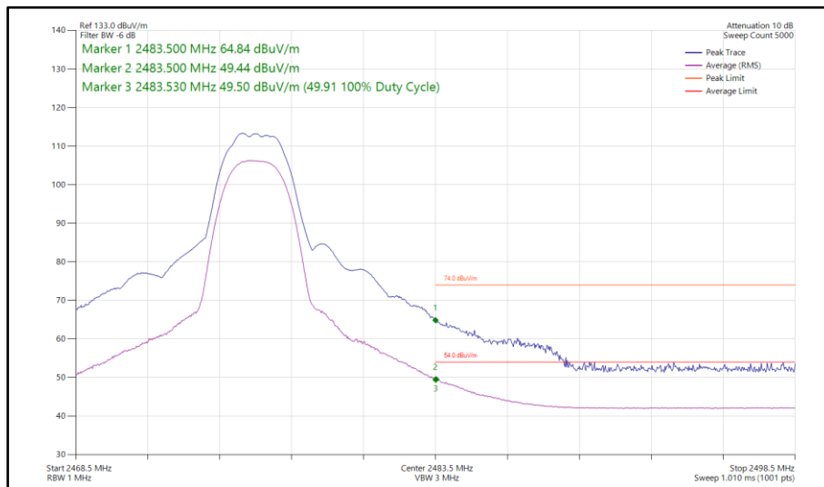
Figure 69 - Bluetooth HDT6, SISO, Core 2 - 2476 MHz Band Edge Frequency 2483.5 MHz
