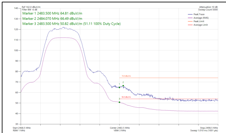
Figure 119 - Bluetooth HDRPM12, SISO, Core 0 - 2475 MHz Band Edge Frequency 2483.5 MHz
