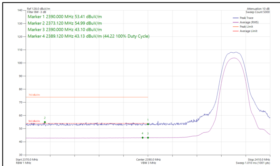
Figure 75 - Bluetooth HDR4, MIMO, Core 0-1 - 2404 MHz Band Edge Frequency 2390 MHz
