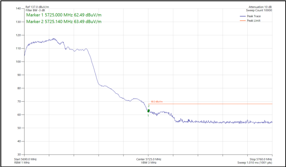
Figure 807 - 802.11be EHT20, RU 106+26-82, CDD, Core 0-1 - 5700 MHz Band Edge Frequency 5725 MHz
