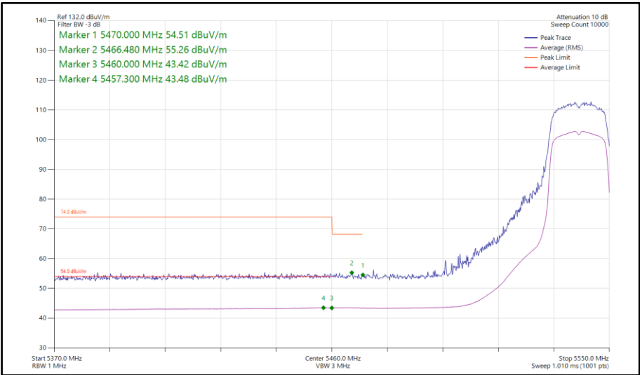
Figure 852 - 802.11ac VHT20, TxBF, Core 0-1 - 5540 MHz Band Edge Frequency 5470 MHz
