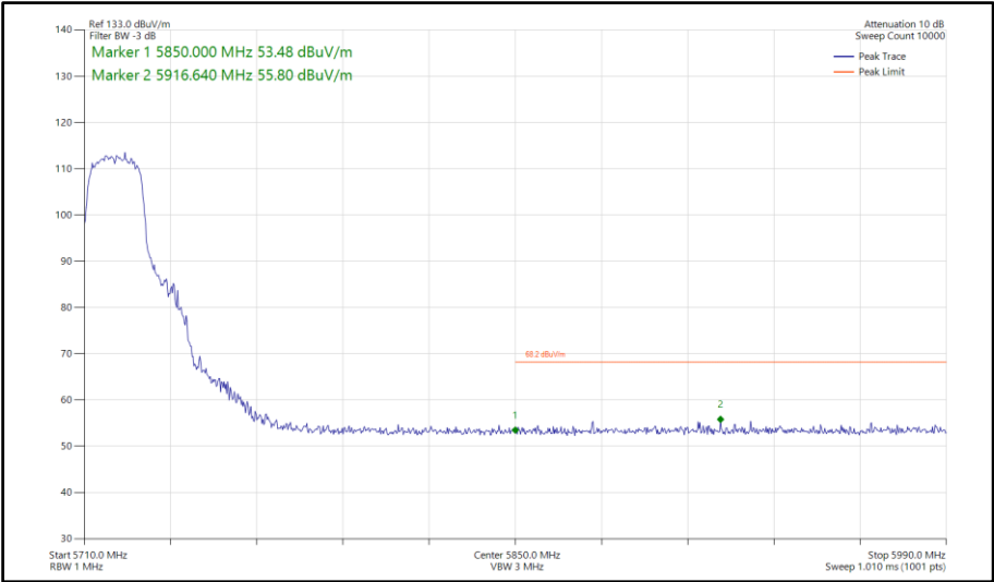
Figure 842 - 802.11n HT20, SDM, Core 0-1 - 5720 MHz Band Edge Frequency 5850 MHz
