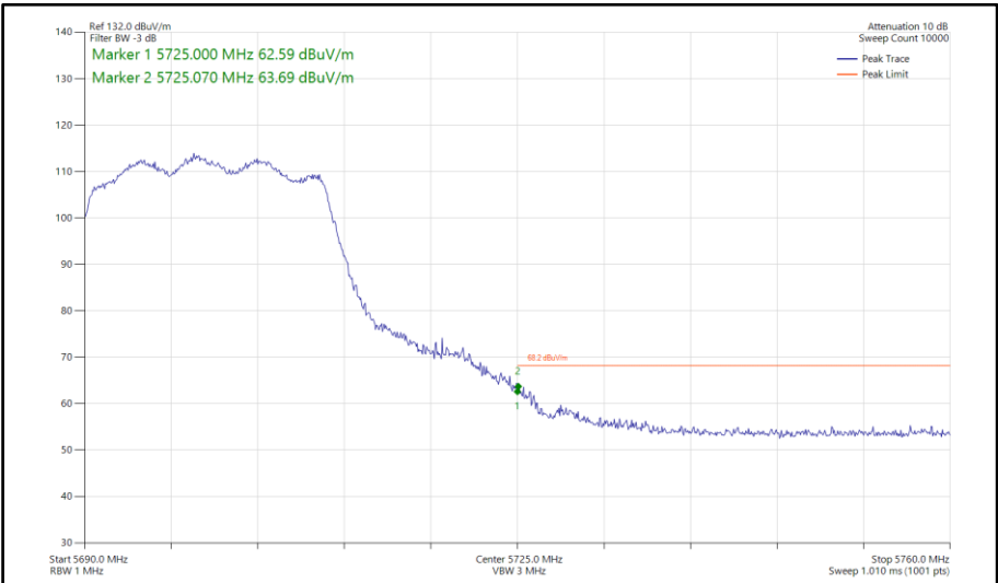
Figure 804 - 802.11ax HE20, SU, CDD, Core 0-1 - 5700 MHz Band Edge Frequency 5725 MHz
