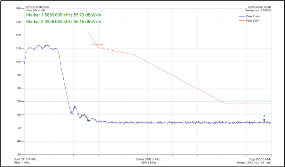
Figure 811 - 802.11n HT20, CDD, Core 0-1 - 5825 MHz Band Edge Frequency 5850 MHz
