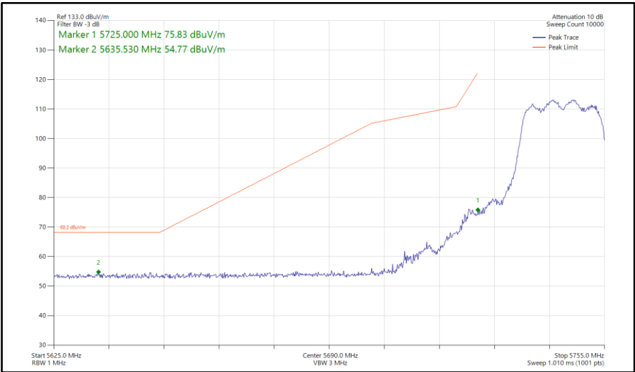
Figure 792 - 802.11ax HE20, SU, CDD, Core 0-1 - 5745 MHz Band Edge Frequency 5725 MHz
