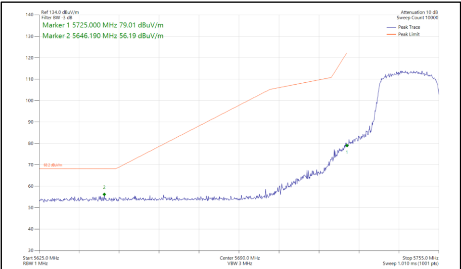
Figure 829 - 802.11ax HE20, SU, SDM, Core 0-1 - 5745 MHz Band Edge Frequency 5725 MHz
