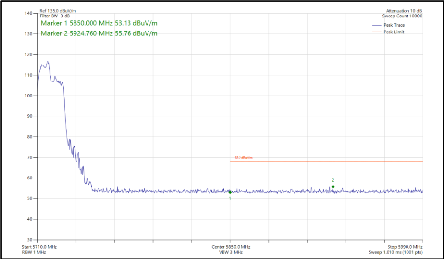
Figure 813 - 802.11ax HE20, RU 106-53, CDD, Core 0-1 - 5720 MHz Band Edge Frequency 5850 MHz
