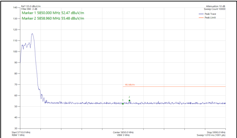
Figure 845 - 802.11ax HE20, RU 52-40, SDM, Core 0-1 - 5720 MHz Band Edge Frequency 5850 MHz
