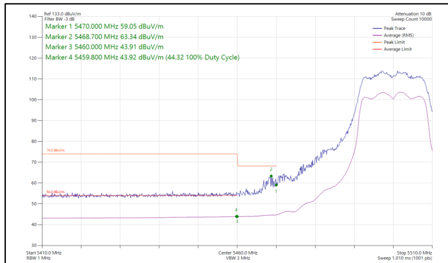
Figure 777 - 802.11a, CDD, Core 0-1 - 5500 MHz Band Edge Frequency 5470 MHz
