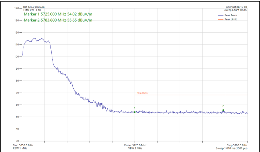
Figure 798 - 802.11n HT20, CDD, Core 0-1 - 5660 MHz Band Edge Frequency 5725 MHz
