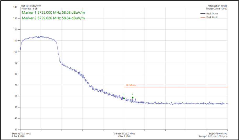
Figure 836 - 802.11ax HE20, SU, SDM, Core 0-1 - 5680 MHz Band Edge Frequency 5725 MHz
