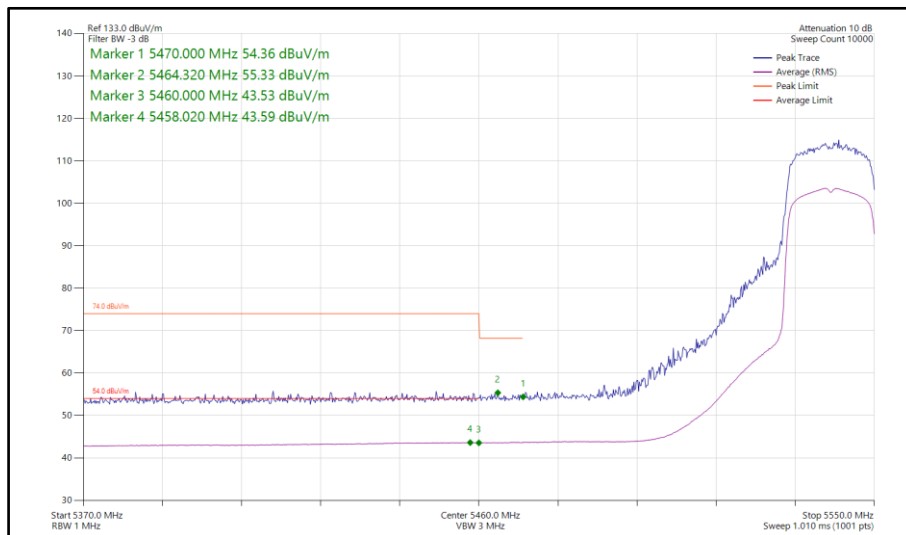
Figure 825 - 802.11ax HE20, SU, SDM, Core 0-1 - 5540 MHz Band Edge Frequency 5470 MHz
