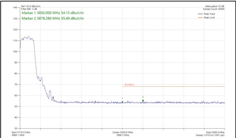
Figure 812 - 802.11ax HE20, SU, CDD, Core 0-1 - 5720 MHz Band Edge Frequency 5850 MHz
