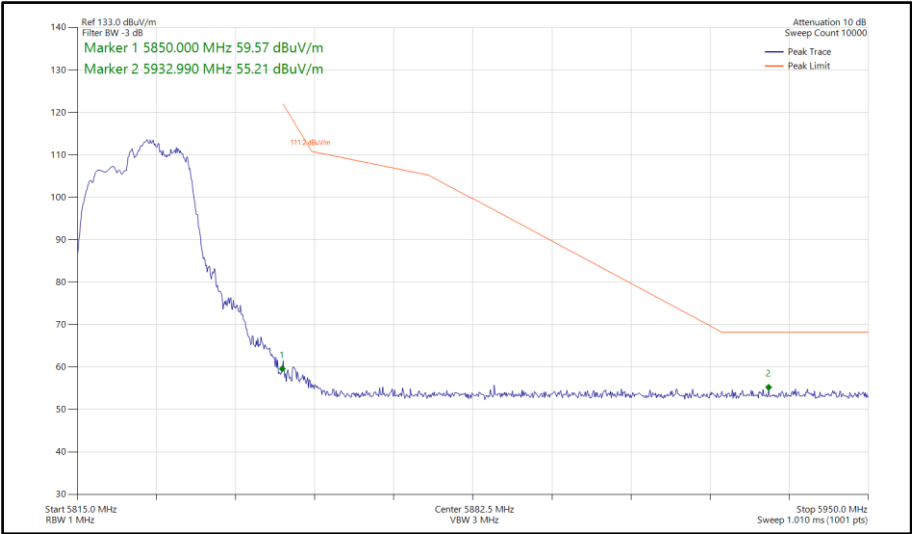
Figure 817 - 802.11be EHT20, RU 106+26-83, CDD, Core 0-1 - 5825 MHz Band Edge Frequency 5850 MHz
