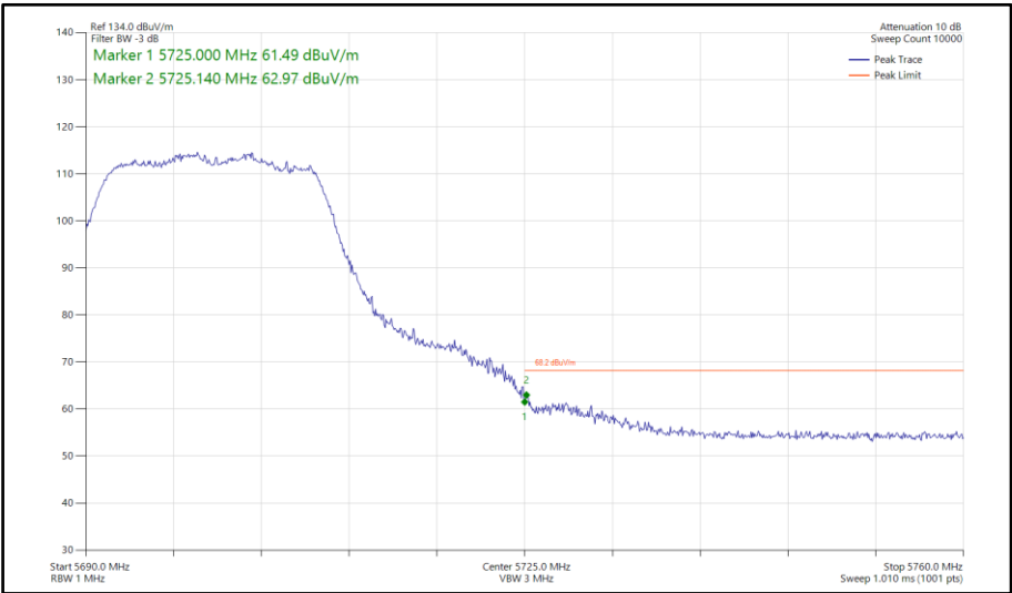
Figure 800 - 802.11n HT20, CDD, Core 0-1 - 5700 MHz Band Edge Frequency 5725 MHz
