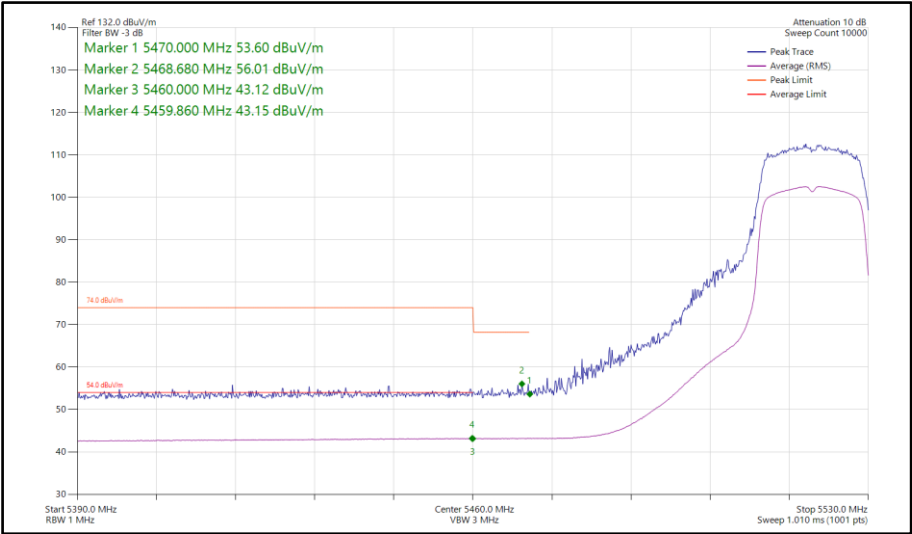
Figure 851 - 802.11ac VHT20, TxBF, Core 0-1 - 5520 MHz Band Edge Frequency 5470 MHz
