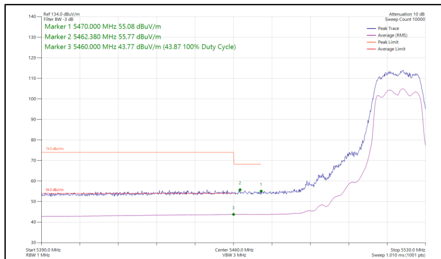
Figure 778 - 802.11a, CDD, Core 0-1 - 5520 MHz Band Edge Frequency 5470 MHz
