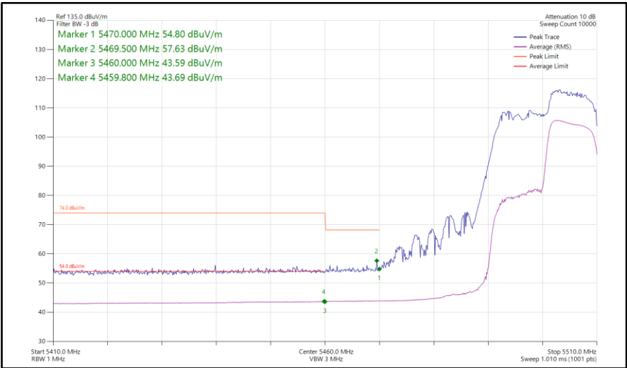
Figure 784 - 802.11ax HE20, RU 106-54, CDD, Core 0-1 - 5500 MHz Band Edge Frequency 5470 MHz
