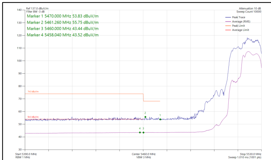
Figure 827 - 802.11be EHT20, RU 106+26-83, SDM, Core 0-1 - 5520 MHz Band Edge Frequency 5470 MHz
