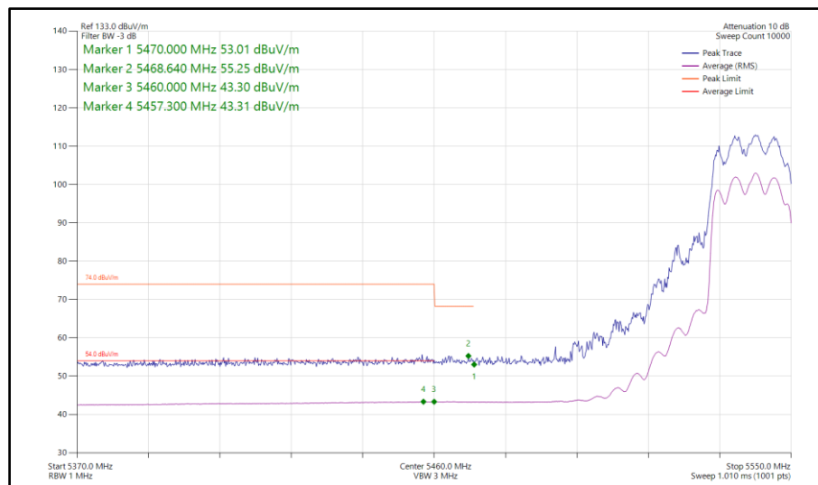
Figure 787 - 802.11ax HE20, SU, CDD, Core 0-1 - 5540 MHz Band Edge Frequency 5470 MHz
