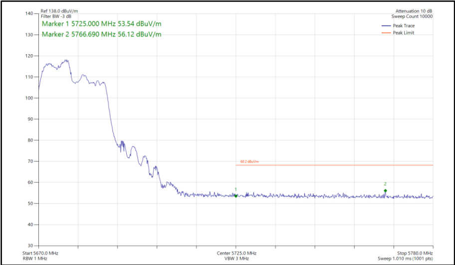
Figure 837 - 802.11ax HE20, RU 106-53, SDM, Core 0-1 - 5680 MHz Band Edge Frequency 5725 MHz
