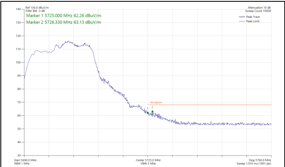
Figure 841 - 802.11be EHT20, RU 106+26-83, SDM, Core 0-1 - 5700 MHz Band Edge Frequency 5725 MHz
