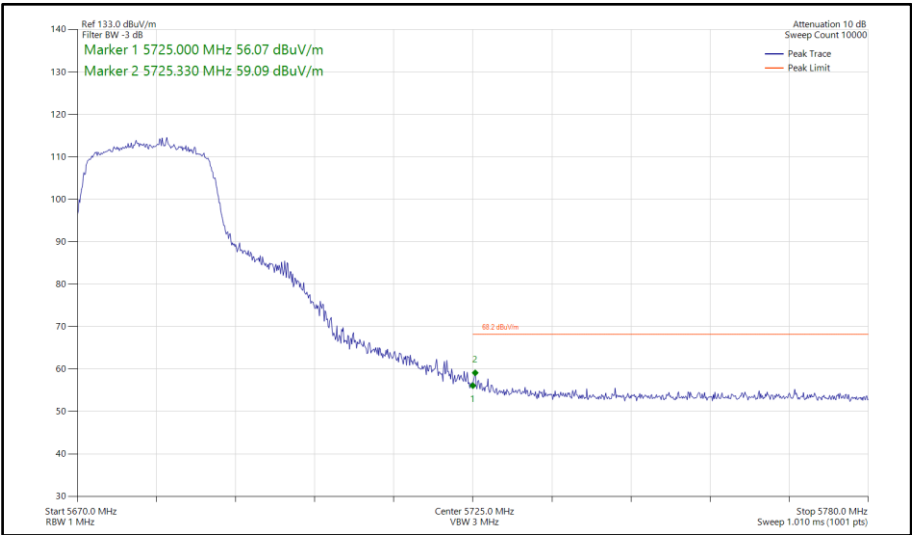
Figure 833 - 802.11n HT20, SDM, Core 0-1 - 5680 MHz Band Edge Frequency 5725 MHz
