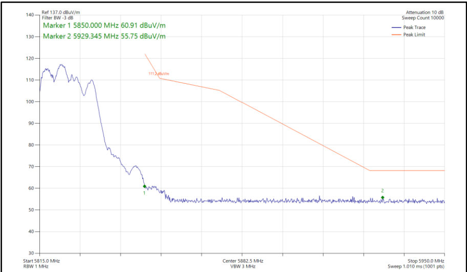
Figure 849 - 802.11be EHT20, RU 106+26-82, SDM, Core 0-1 - 5825 MHz Band Edge Frequency 5850 MHz
