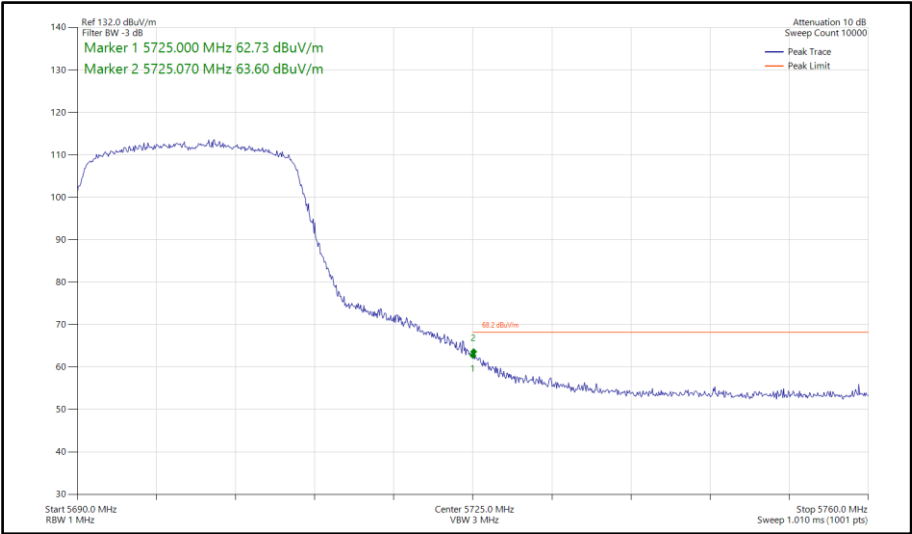
Figure 838 - 802.11ax HE20, SU, SDM, Core 0-1 - 5700 MHz Band Edge Frequency 5725 MHz
