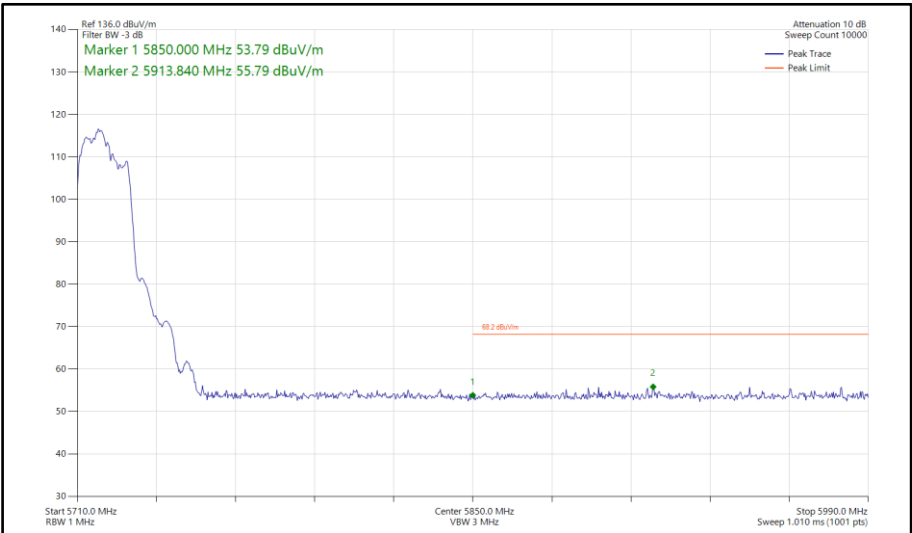
Figure 816 - 802.11be EHT20, RU 106+26-82, CDD, Core 0-1 - 5720 MHz Band Edge Frequency 5850 MHz
