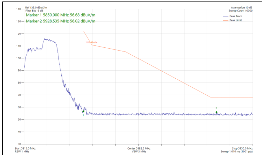
Figure 774 - 802.11ax HE20, RU 106-54, SISO, Core 1 - 5825 MHz Band Edge Frequency 5850 MHz
