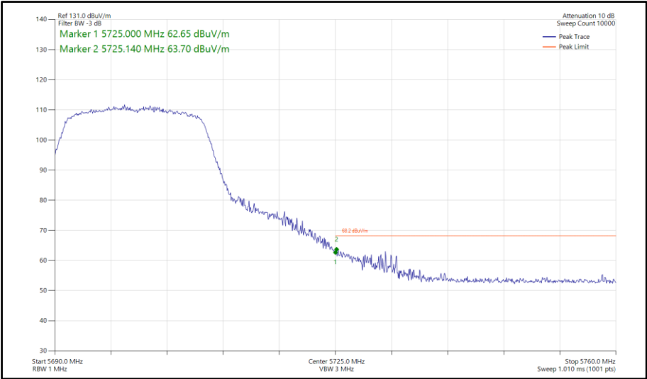
Figure 834 - 802.11n HT20, SDM, Core 0-1 - 5700 MHz Band Edge Frequency 5725 MHz
