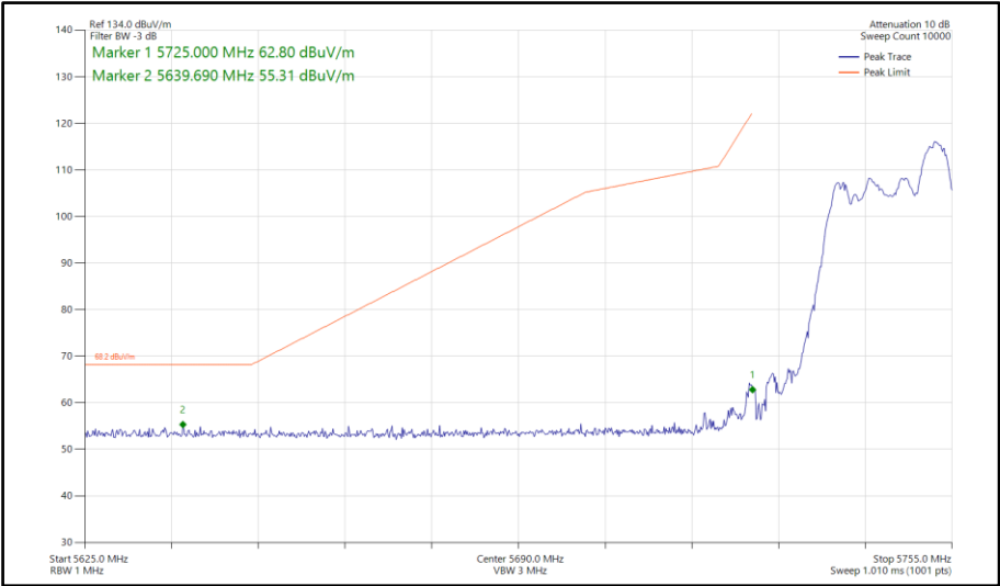
Figure 793 - 802.11ax HE20, RU 52-40, CDD, Core 0-1 - 5745 MHz Band Edge Frequency 5725 MHz
