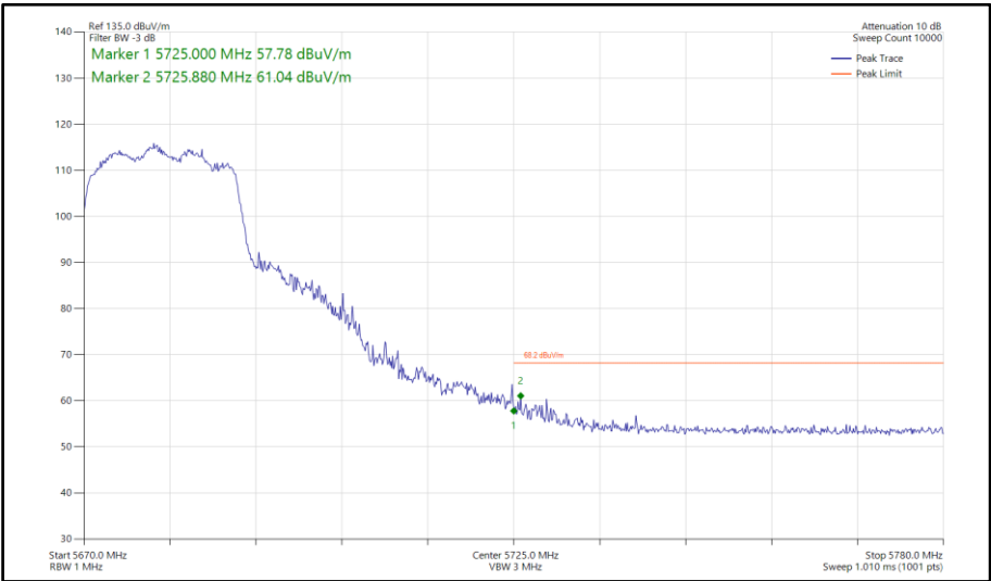
Figure 802 - 802.11ax HE20, SU, CDD, Core 0-1 - 5680 MHz Band Edge Frequency 5725 MHz
