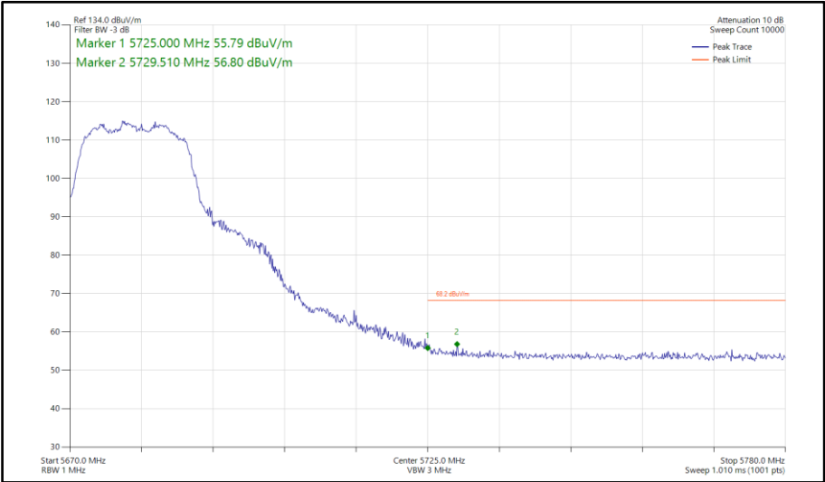
Figure 796 - 802.11a, CDD, Core 0-1 - 5680 MHz Band Edge Frequency 5725 MHz
