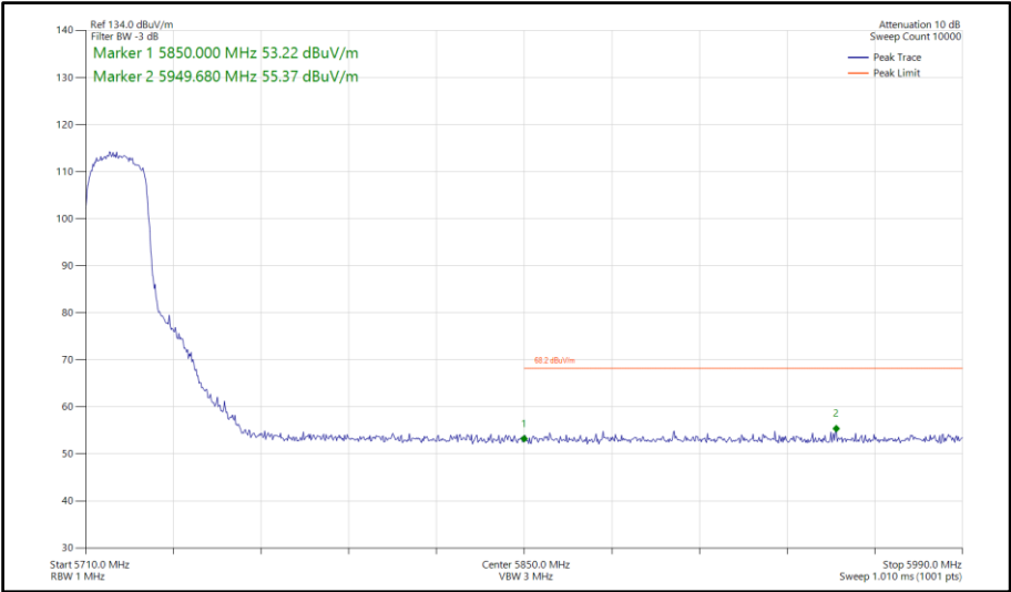
Figure 844 - 802.11ax HE20, SU, SDM, Core 0-1 - 5720 MHz Band Edge Frequency 5850 MHz
