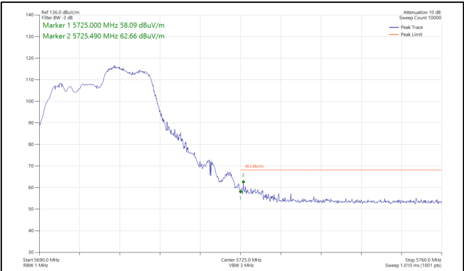
Figure 839 - 802.11ax HE20, RU 106-54, SDM, Core 0-1 - 5700 MHz Band Edge Frequency 5725 MHz
