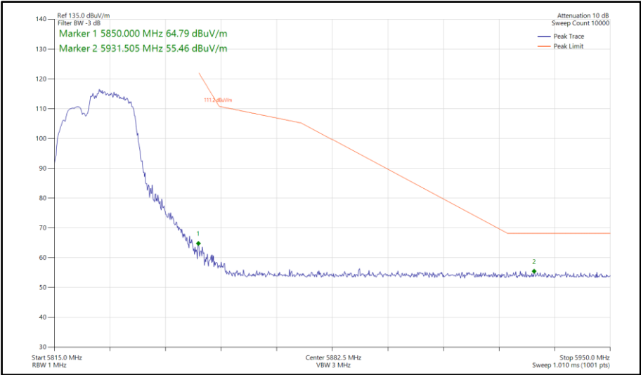
Figure 776 - 802.11be EHT20, RU 106+26-83, SISO, Core 1 - 5825 MHz Band Edge Frequency 5850 MHz
