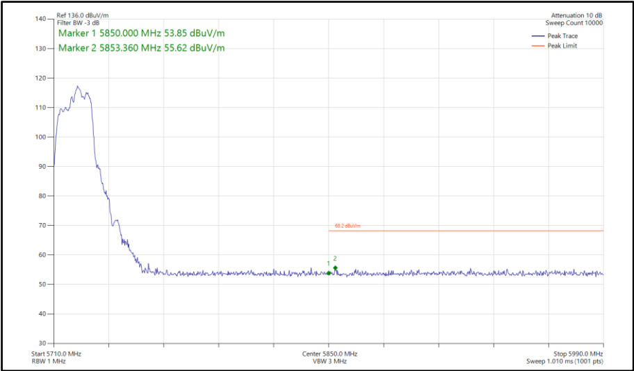
Figure 848 - 802.11be EHT20, RU 106+26-83, SDM, Core 0-1 - 5720 MHz Band Edge Frequency 5850 MHz
