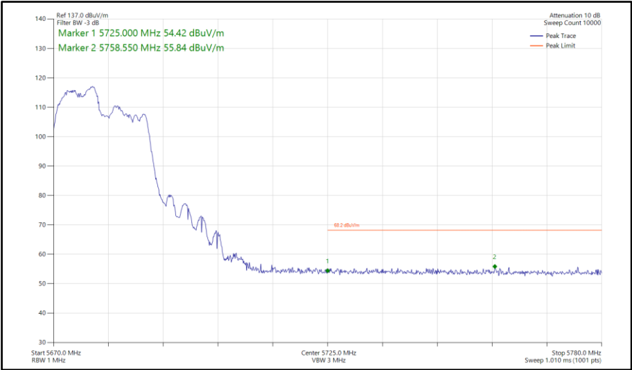
Figure 803 - 802.11ax HE20, RU 106-53, CDD, Core 0-1 - 5680 MHz Band Edge Frequency 5725 MHz
