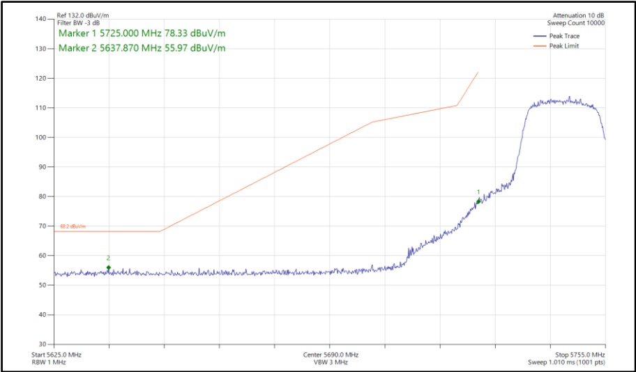
Figure 828 - 802.11n HT20, SDM, Core 0-1 - 5745 MHz Band Edge Frequency 5725 MHz
