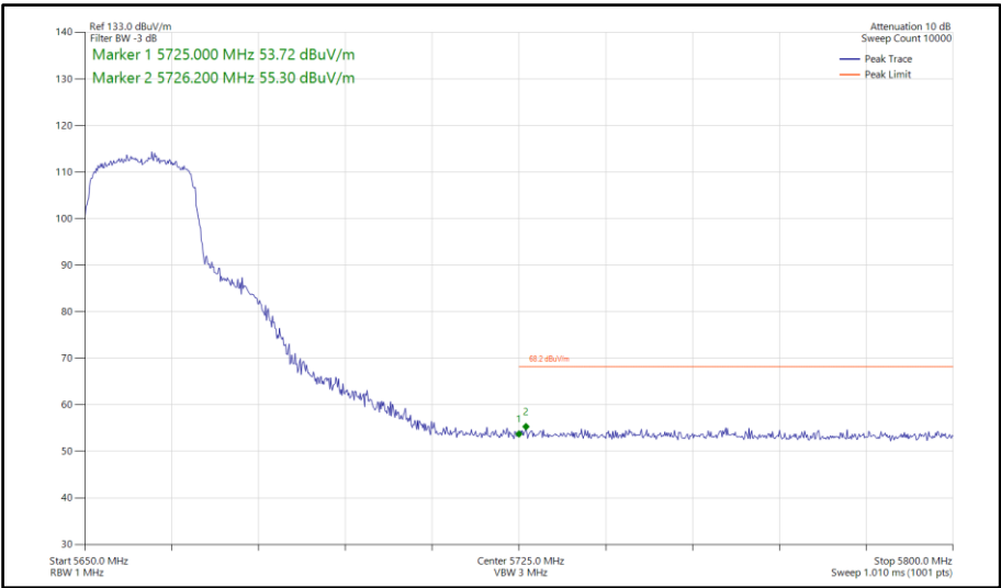
Figure 832 - 802.11n HT20, SDM, Core 0-1 - 5660 MHz Band Edge Frequency 5725 MHz
