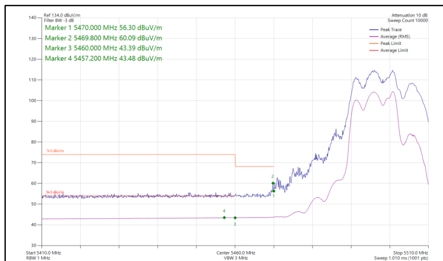
Figure 788 - 802.11be EHT20, RU 106+26-82, CDD, Core 0-1 - 5500 MHz Band Edge Frequency 5470 MHz
