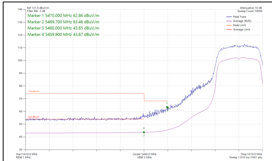
Figure 818 - 802.11n HT20, SDM, Core 0-1 - 5500 MHz Band Edge Frequency 5470 MHz
