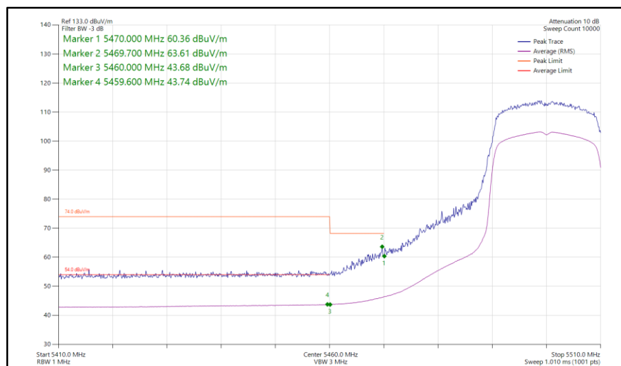
Figure 821 - 802.11ax HE20, SU, SDM, Core 0-1 - 5500 MHz Band Edge Frequency 5470 MHz
