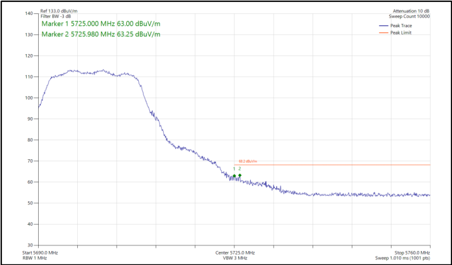
Figure 797 - 802.11a, CDD, Core 0-1 - 5700 MHz Band Edge Frequency 5725 MHz
