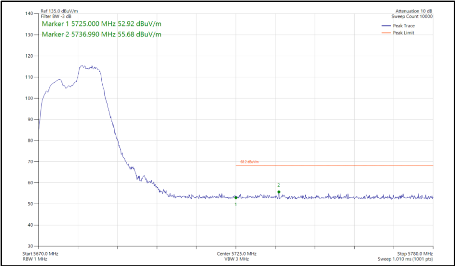
Figure 840 - 802.11be EHT20, RU 52+26-72, SDM, Core 0-1 - 5680 MHz Band Edge Frequency 5725 MHz
