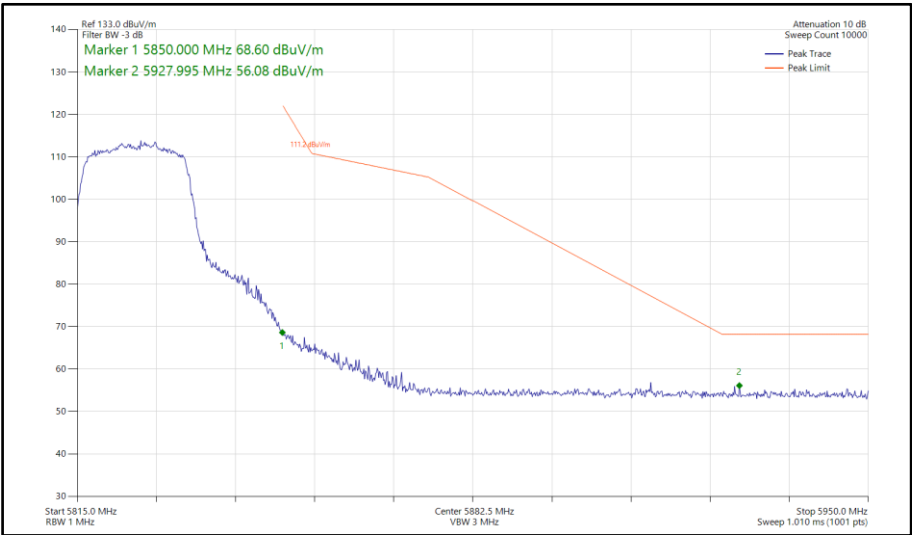
Figure 843 - 802.11n HT20, SDM, Core 0-1 - 5825 MHz Band Edge Frequency 5850 MHz
