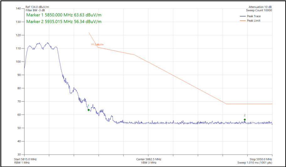
Figure 809 - 802.11a, CDD, Core 0-1 - 5825 MHz Band Edge Frequency 5850 MHz
