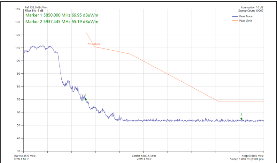
Figure 814 - 802.11ax HE20, SU, CDD, Core 0-1 - 5825 MHz Band Edge Frequency 5850 MHz
